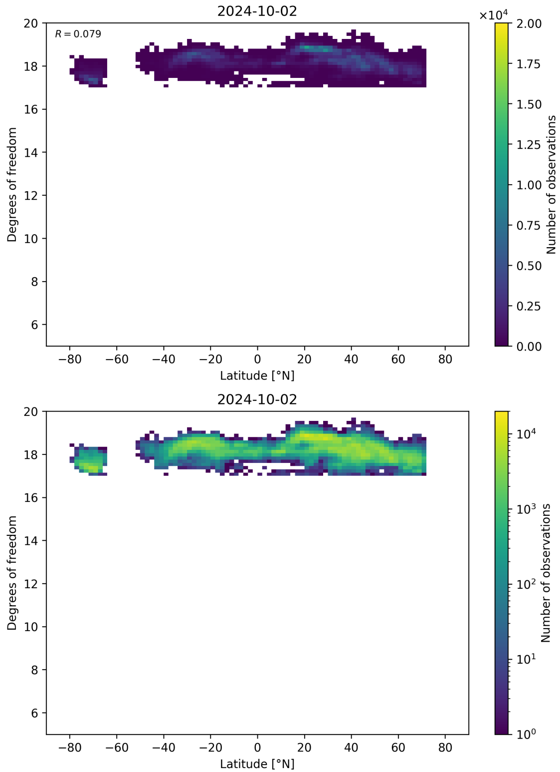
Figure 55: Scatter density plot of “Latitude” against “Degrees of freedom” for 2024-10-01 to 2024-10-03.
