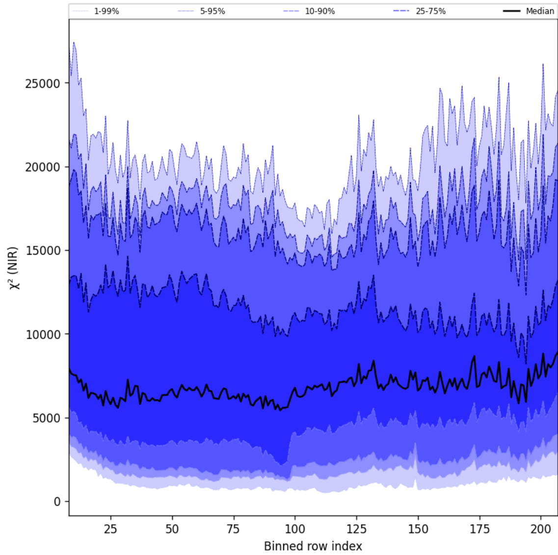
Figure 40: Along track statistics of “ \chi^2 (NIR)” for 2024-10-01 to 2024-10-03
