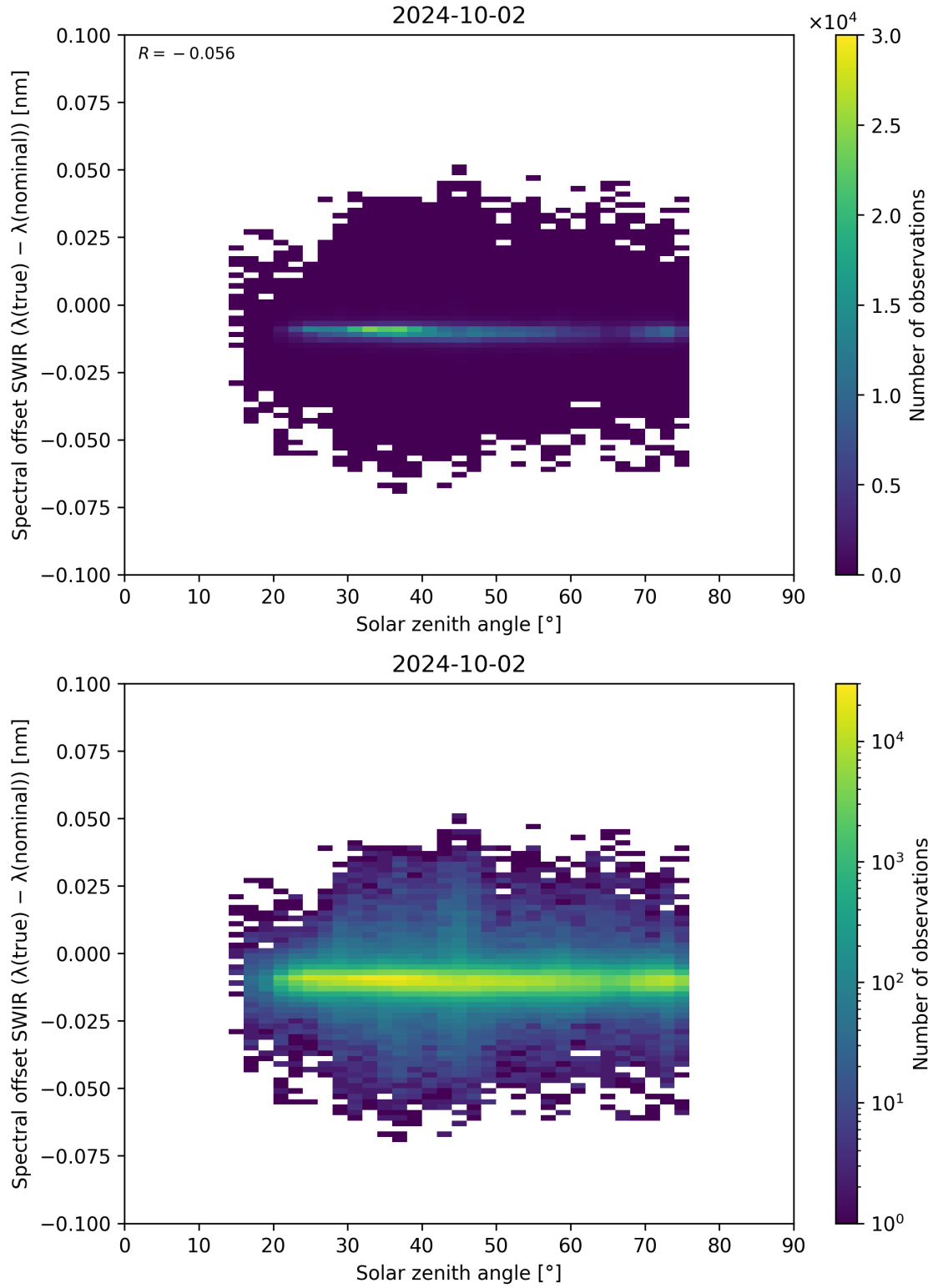
Figure 104: Scatter density plot of “Solar zenith angle” against “Spectral offset SWIR ( \lambda_{\text{true}} - \lambda_{\text{nominal}} )” for 2024-10-01 to 2024-10-03.
