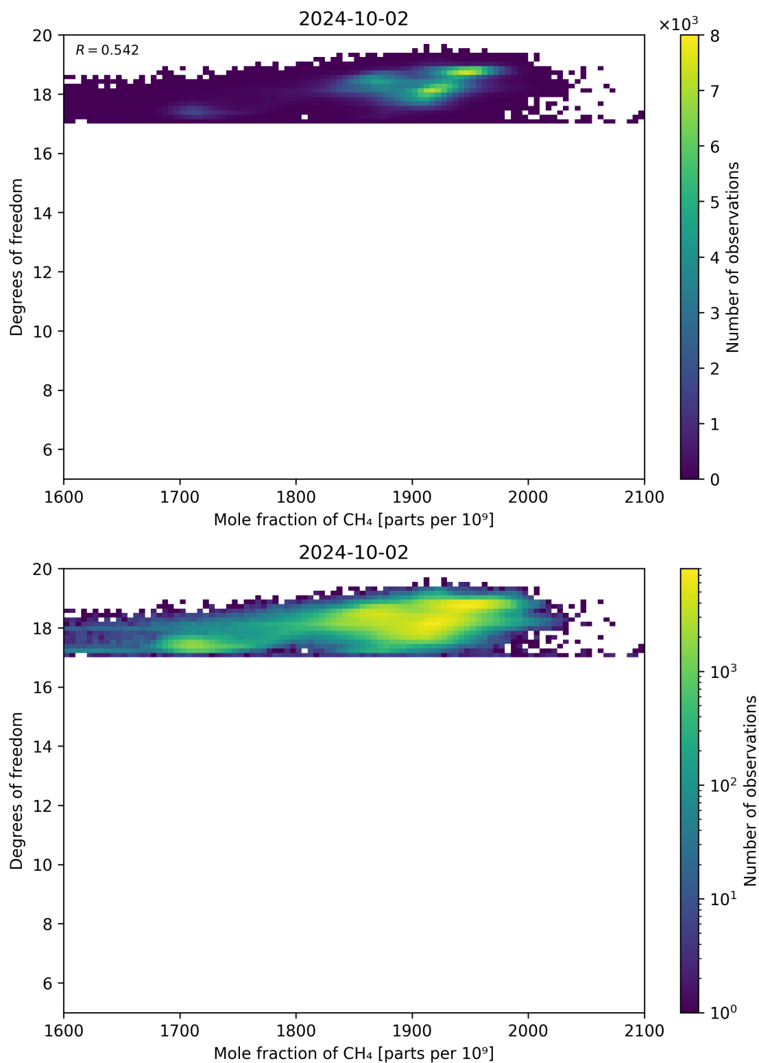
Figure 72: Scatter density plot of “Mole fraction of CH 4 ” against “Degrees of freedom” for 2024-10-01 to 2024-10-03.
