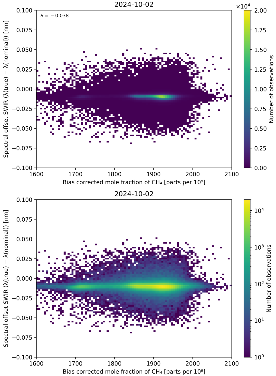
Figure 69: Scatter density plot of “Bias corrected mole fraction of \text{CH}_4 ” against “Spectral offset SWIR ( \lambda_{\text{true}} - \lambda_{\text{nominal}} )” for 2024-10-01 to 2024-10-03.
