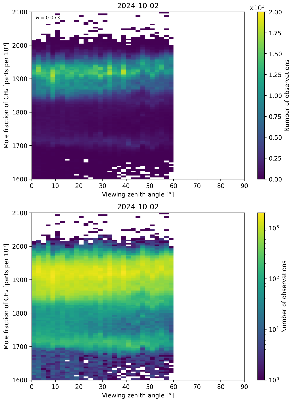
Figure 110: Scatter density plot of “Viewing zenith angle” against “Mole fraction of CH 4 ” for 2024-10-01 to 2024-10-03.
