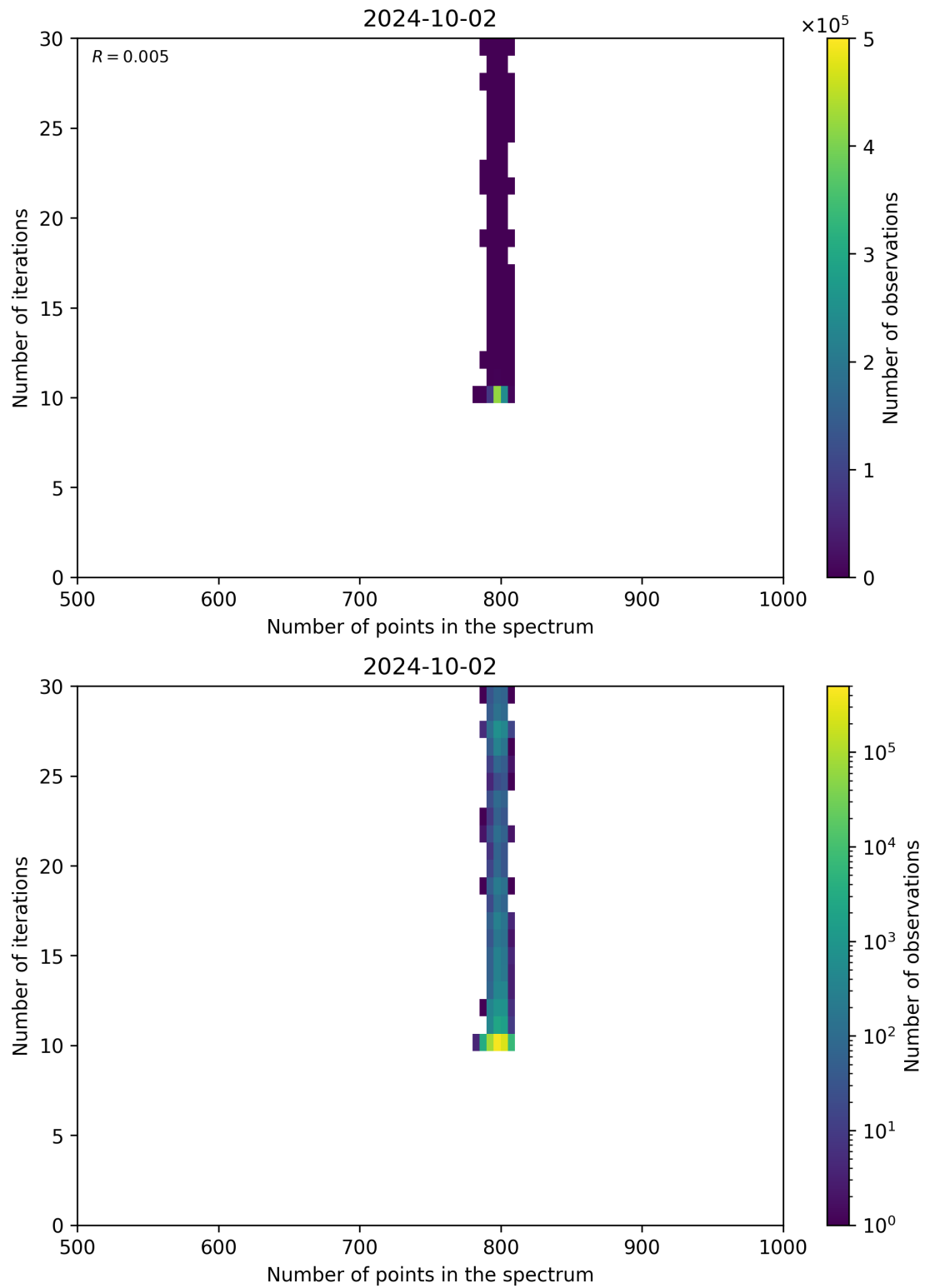
Figure 92: Scatter density plot of “Number of points in the spectrum” against “Number of iterations” for 2024-10-01 to 2024-10-03.
