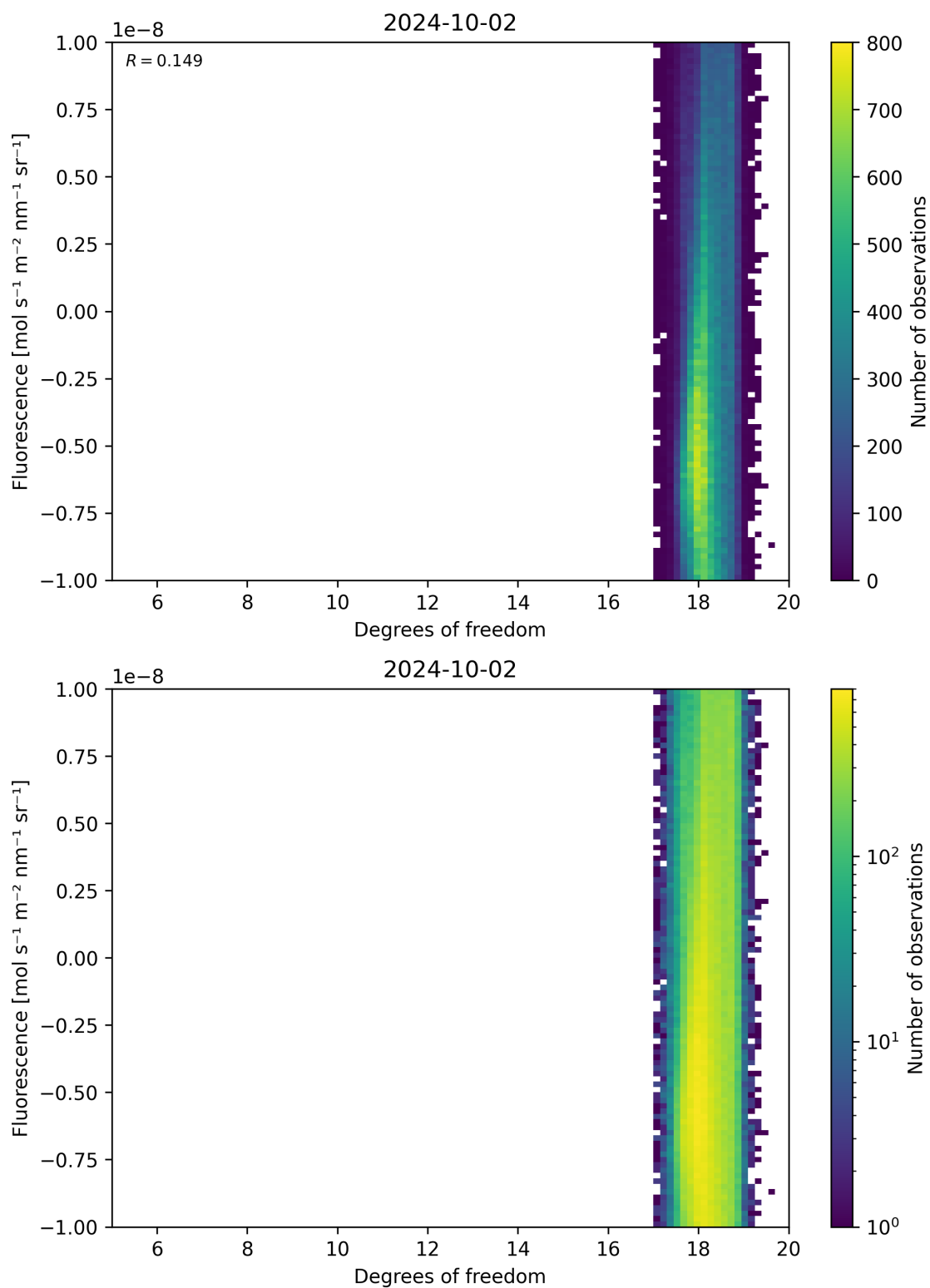
Figure 51: Scatter density plot of “Degrees of freedom” against “Fluorescence” for 2024-10-01 to 2024-10-03.
