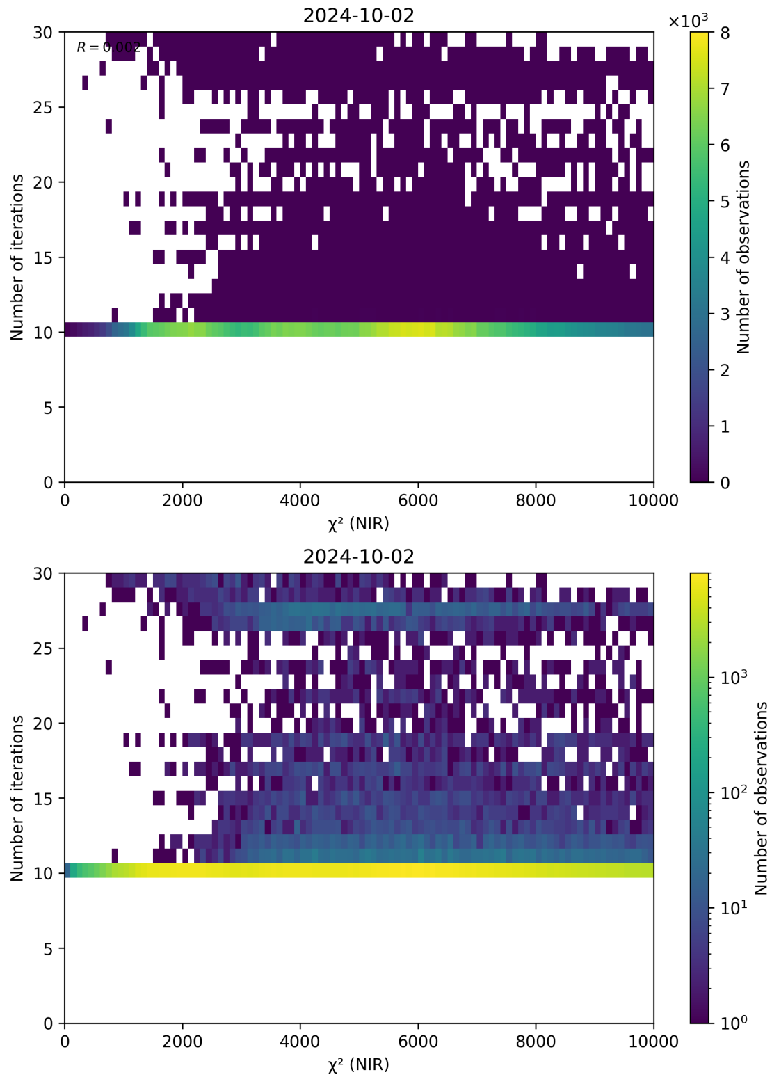
Figure 46: Scatter density plot of “ \chi^2 (NIR)” against “Number of iterations” for 2024-10-01 to 2024-10-03.
