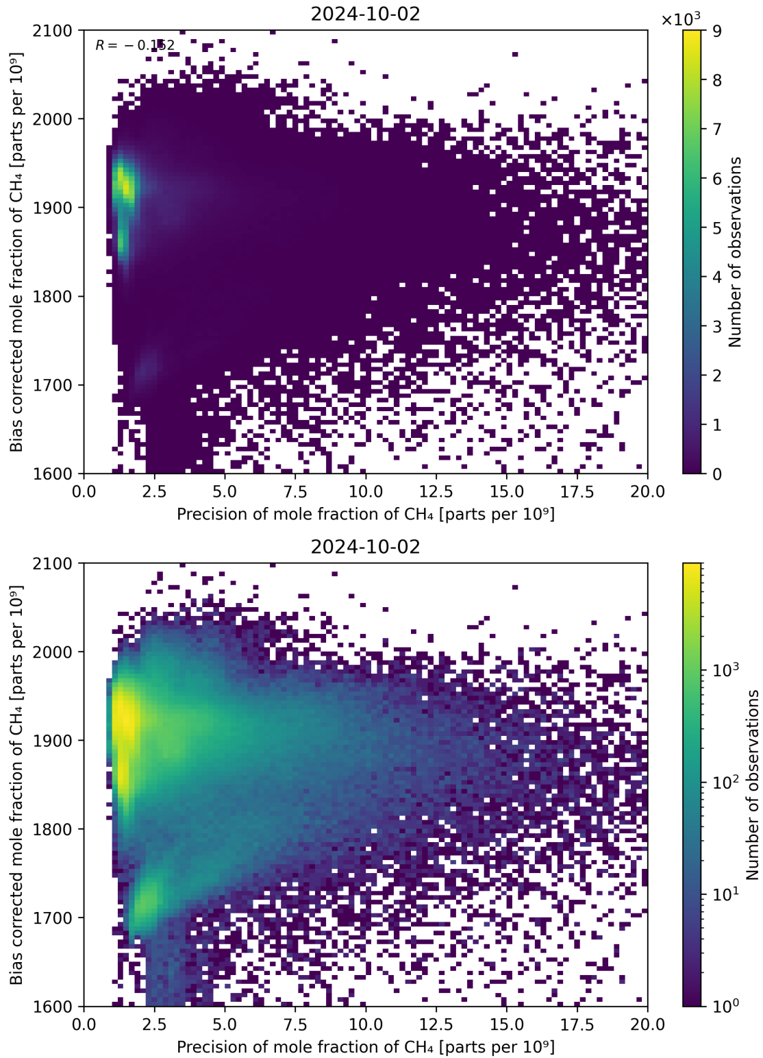
Figure 82: Scatter density plot of “Precision of mole fraction of CH 4 ” against “Bias corrected mole fraction of CH 4 ” for 2024-10-01 to 2024-10-03.
