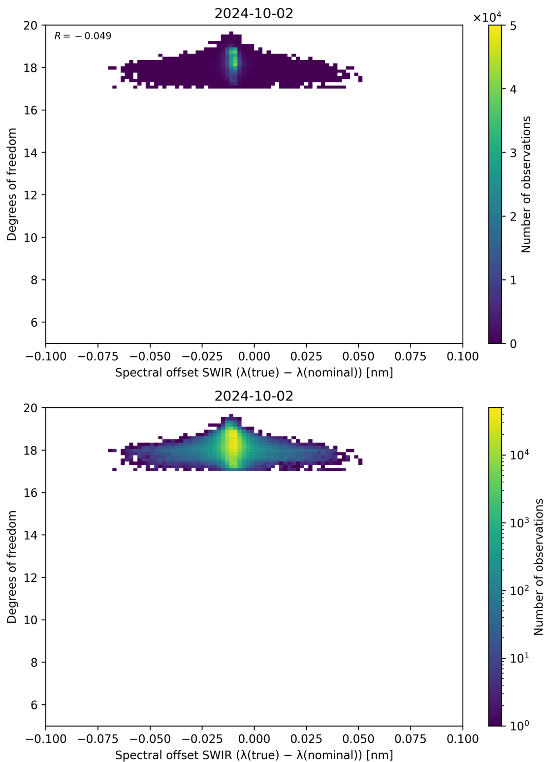
Figure 119: Scatter density plot of “Spectral offset SWIR ( \lambda_{\text{true}} - \lambda_{\text{nominal}} )” against “Degrees of freedom” for 2024-10-01 to 2024-10-03.
