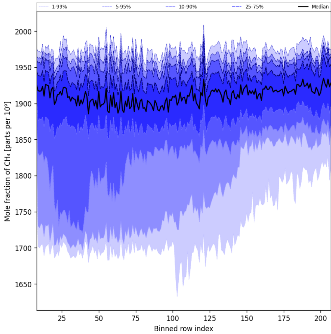
Figure 34: Along track statistics of “Mole fraction of CH 4 ” for 2024-10-01 to 2024-10-03
