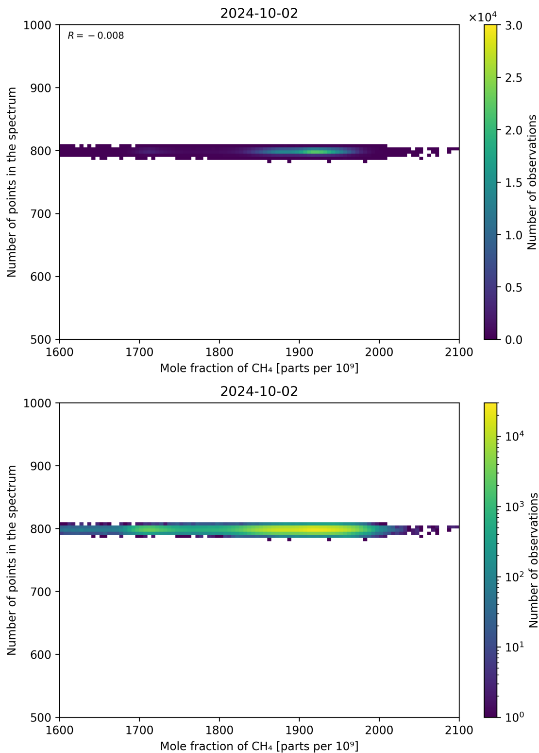
Figure 77: Scatter density plot of “Mole fraction of CH 4 ” against “Number of points in the spectrum” for 2024-10-01 to 2024-10-03.
