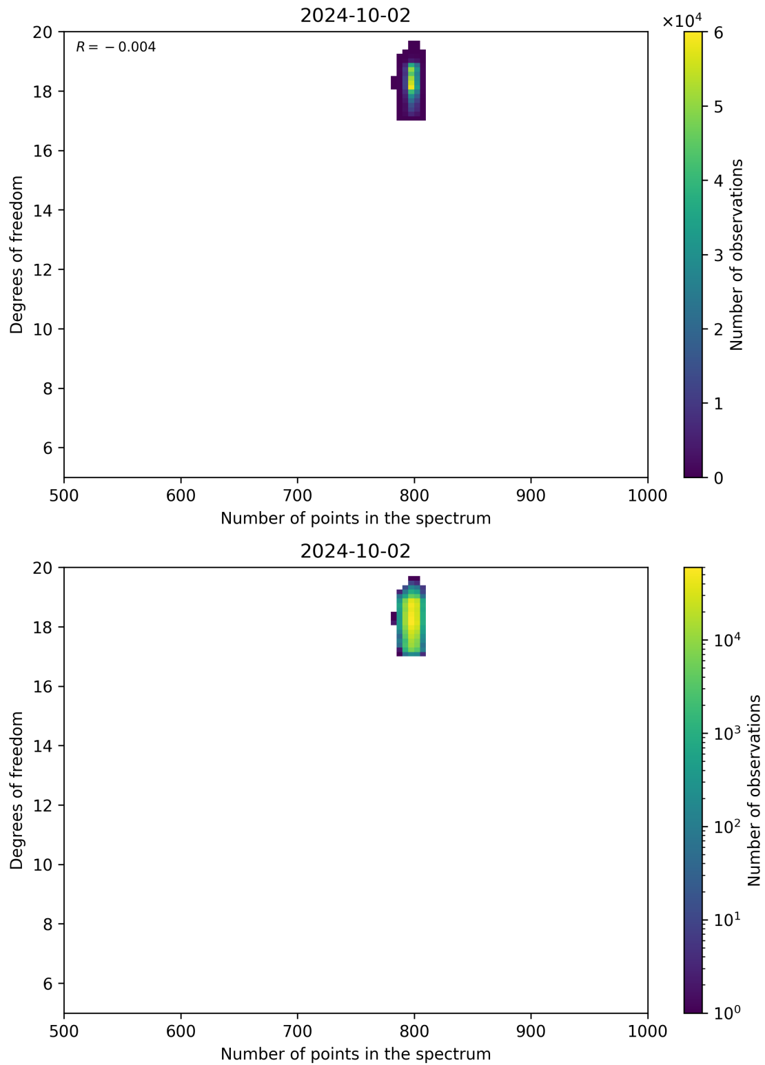
Figure 90: Scatter density plot of “Number of points in the spectrum” against “Degrees of freedom” for 2024-10-01 to 2024-10-03.
