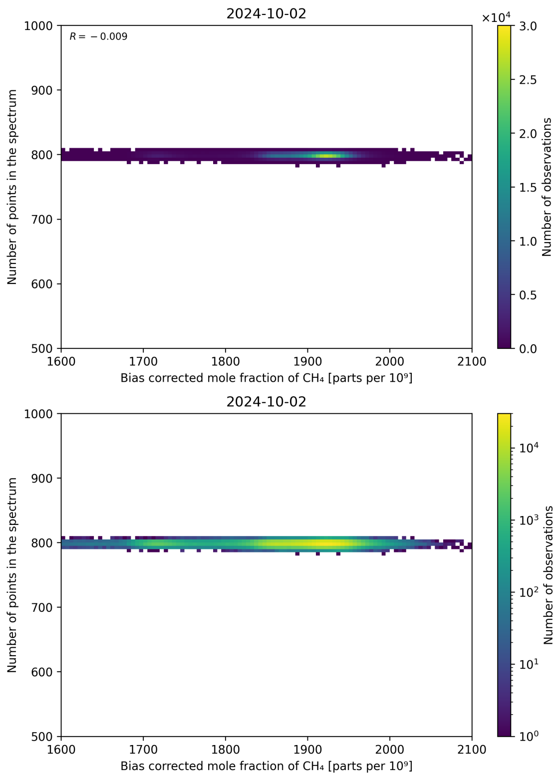
Figure 68: Scatter density plot of “Bias corrected mole fraction of CH 4 ” against “Number of points in the spectrum” for 2024-10-01 to 2024-10-03.
