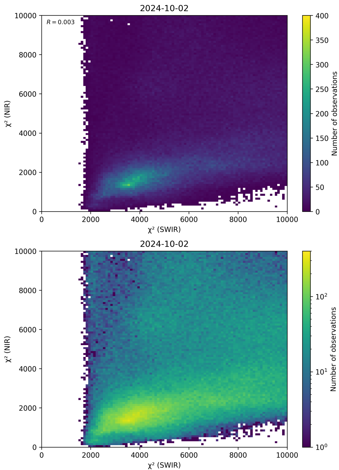
Figure 47: Scatter density plot of “ \chi^2 (SWIR)” against “ \chi^2 (NIR)” for 2024-10-01 to 2024-10-03.
