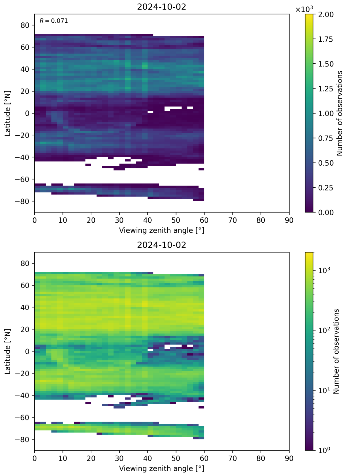
Figure 109: Scatter density plot of “Viewing zenith angle” against “Latitude” for 2024-10-01 to 2024-10-03.
