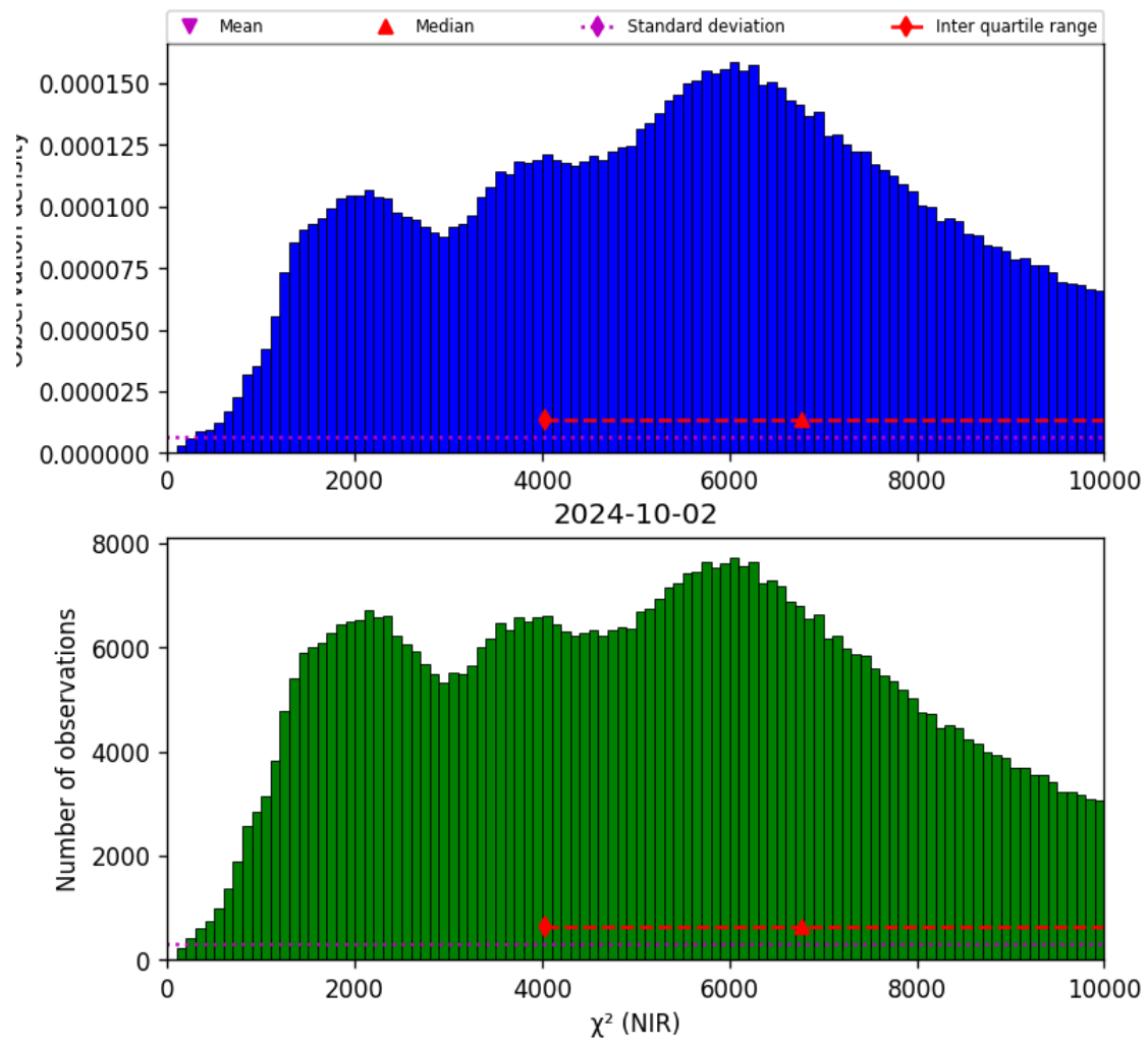
Figure 29: Histogram of “ \chi^2 (NIR)” for 2024-10-01 to 2024-10-03
