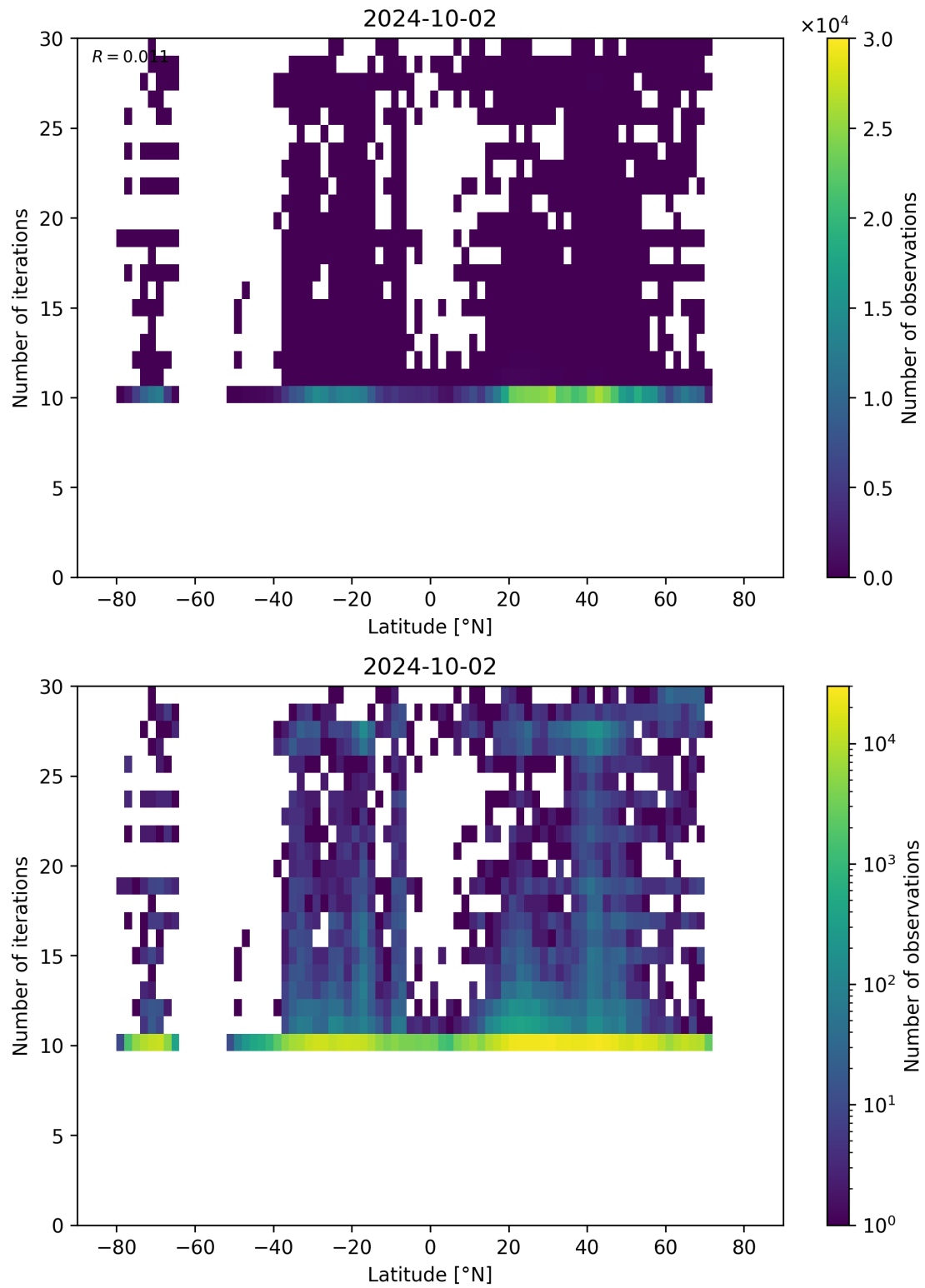
Figure 60: Scatter density plot of “Latitude” against “Number of iterations” for 2024-10-01 to 2024-10-03.
