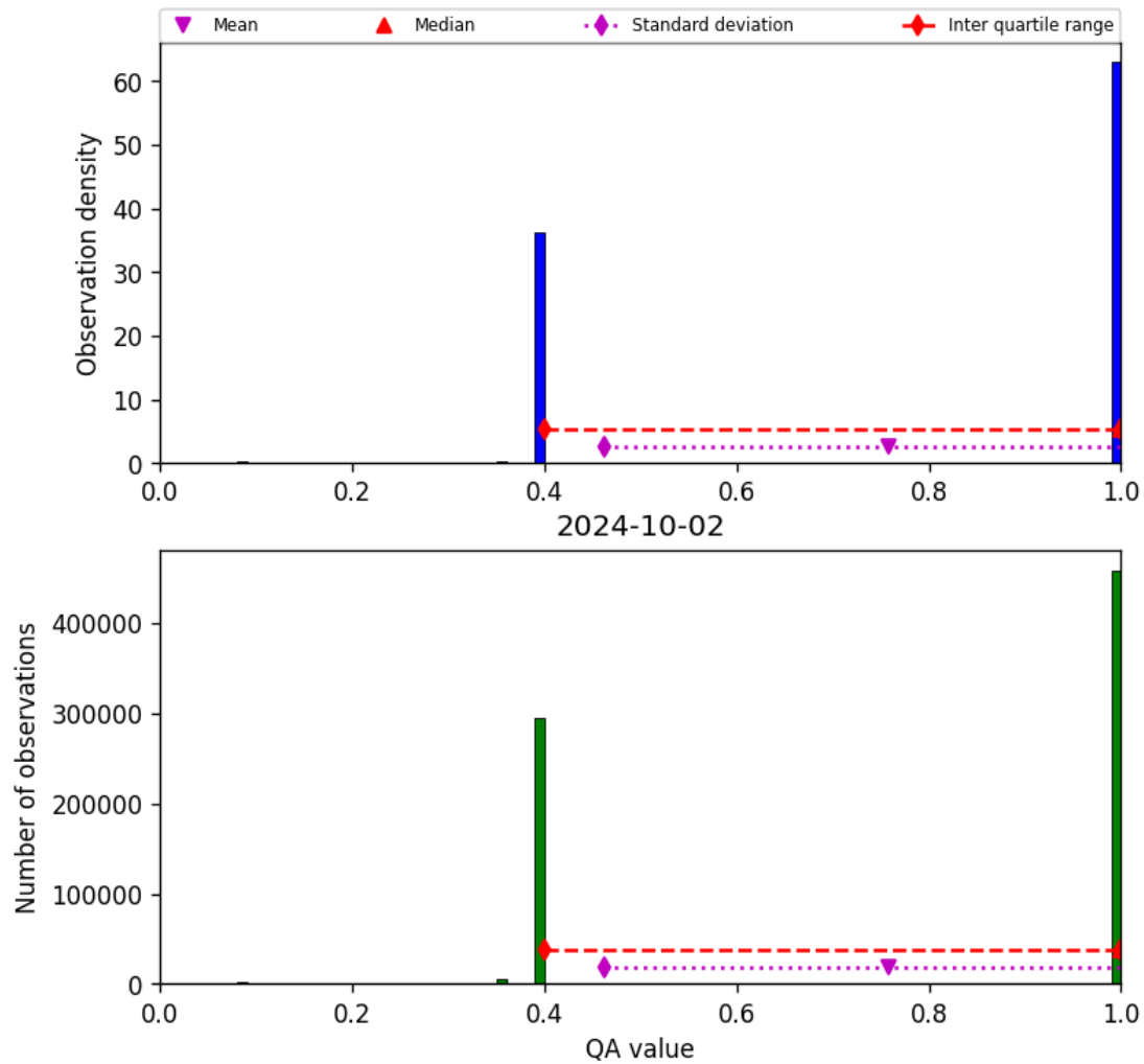
Figure 22: Histogram of “QA value” for 2024-10-01 to 2024-10-03
