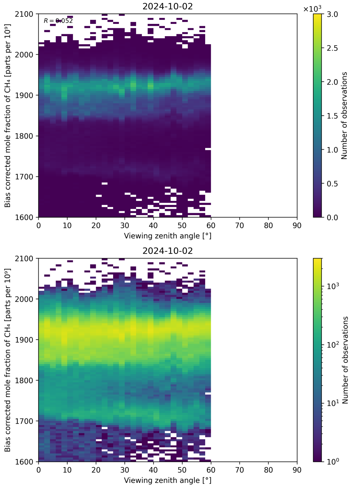
Figure 111: Scatter density plot of “Viewing zenith angle” against “Bias corrected mole fraction of CH 4 ” for 2024-10-01 to 2024-10-03.
