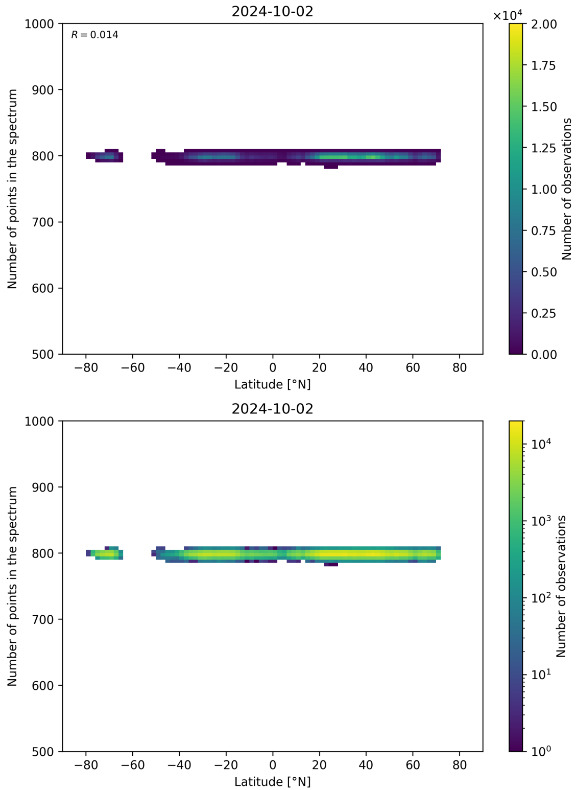
Figure 61: Scatter density plot of “Latitude” against “Number of points in the spectrum” for 2024-10-01 to 2024-10-03.
