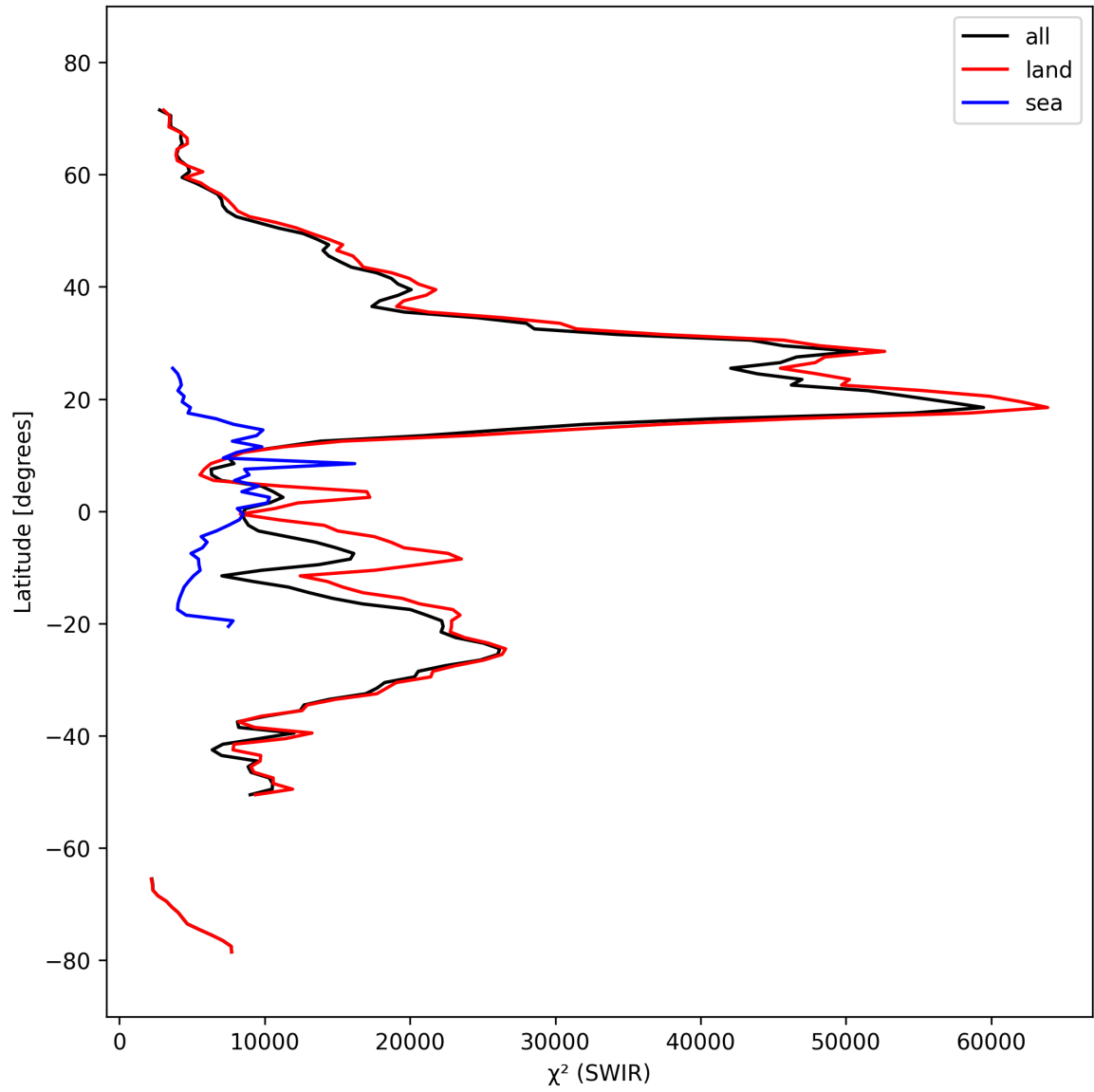
Figure 17: Zonal average of “ \chi^2 (SWIR)” for 2024-10-01 to 2024-10-03.
