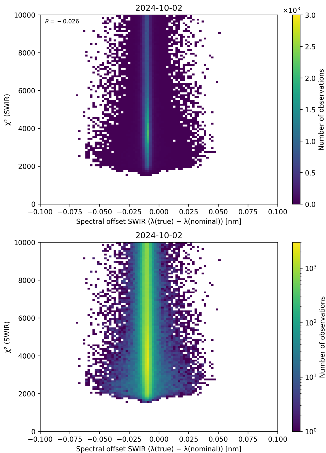
Figure 118: Scatter density plot of “Spectral offset SWIR ( \lambda_{\text{true}} - \lambda_{\text{nominal}} )” against “ \chi^2 (SWIR)” for 2024-10-01 to 2024-10-03.
