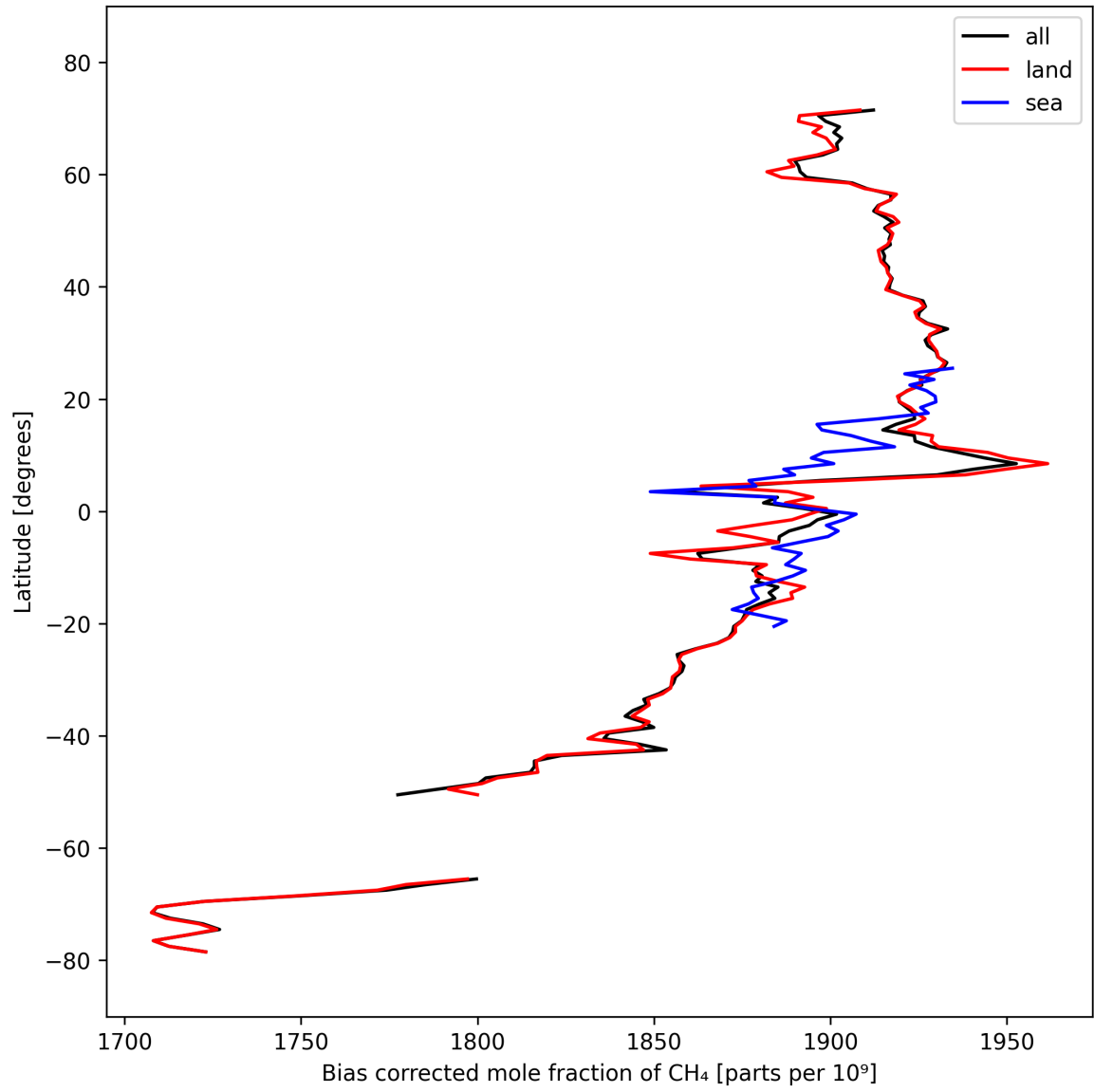
Figure 14: Zonal average of “Bias corrected mole fraction of CH 4 ” for 2024-10-01 to 2024-10-03.
