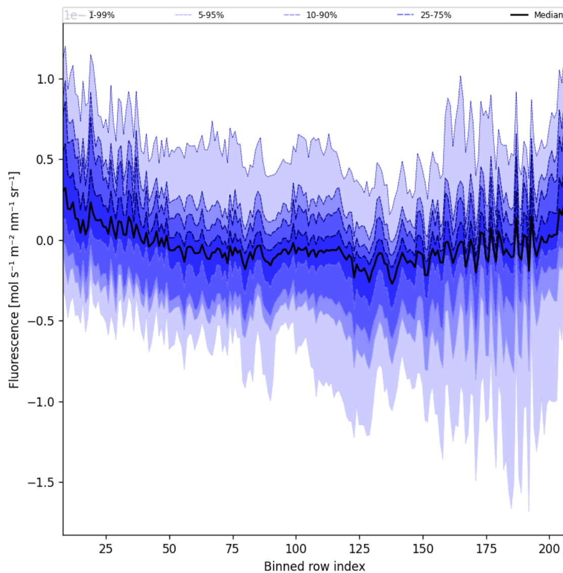
Figure 43: Along track statistics of “Fluorescence” for 2024-10-01 to 2024-10-03
