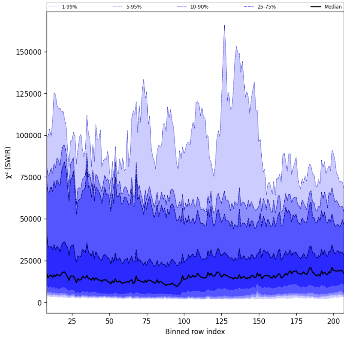
Figure 39: Along track statistics of “ \chi^2 (SWIR)” for 2024-10-01 to 2024-10-03
