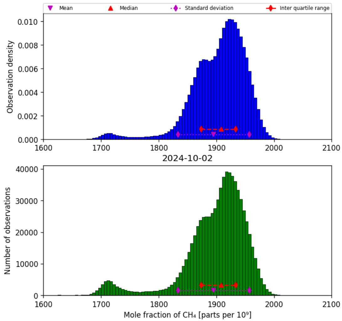
Figure 23: Histogram of “Mole fraction of CH 4 ” for 2024-10-01 to 2024-10-03
