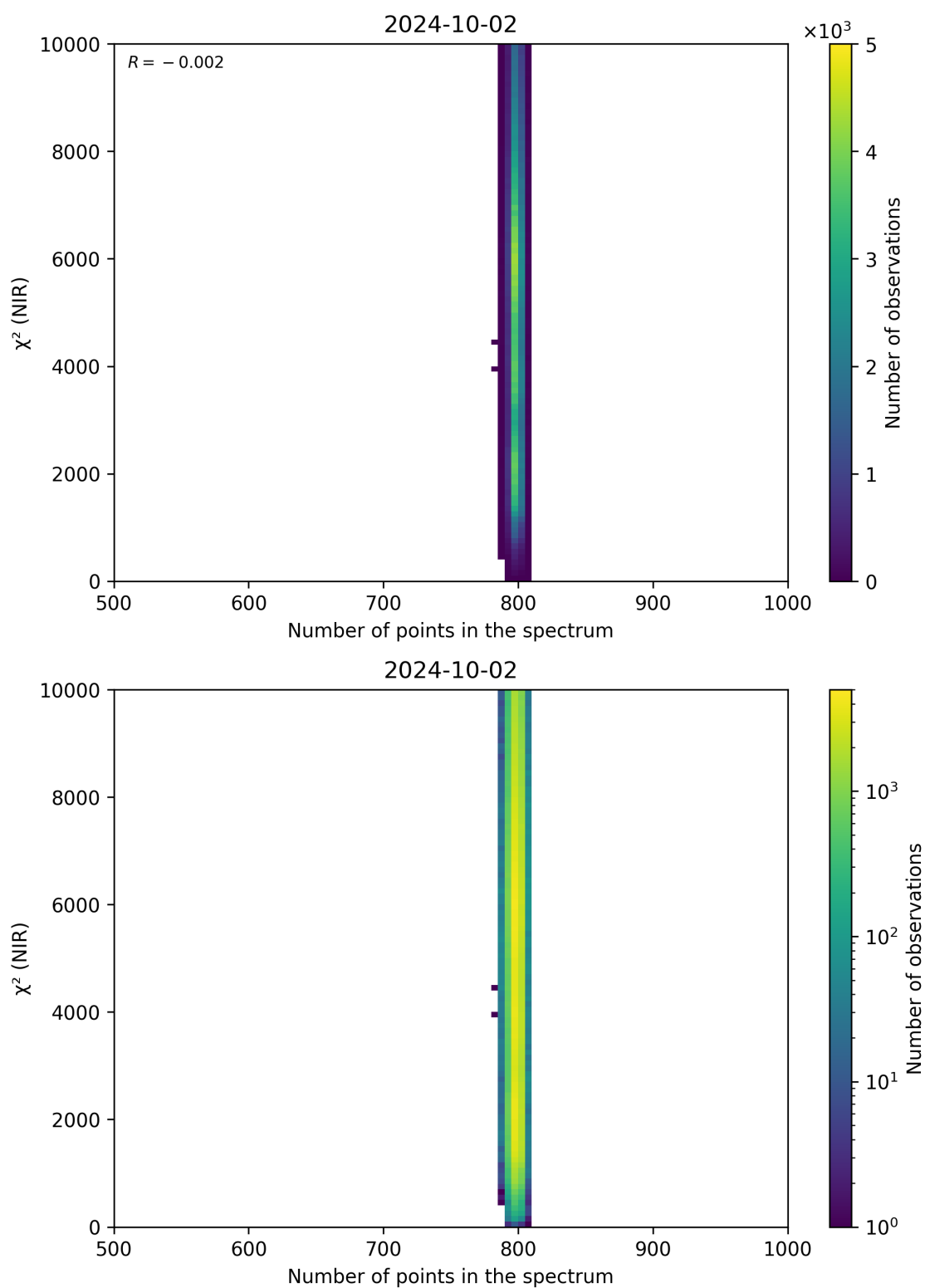
Figure 88: Scatter density plot of “Number of points in the spectrum” against “ \chi^2 (NIR)” for 2024-10-01 to 2024-10-03.
