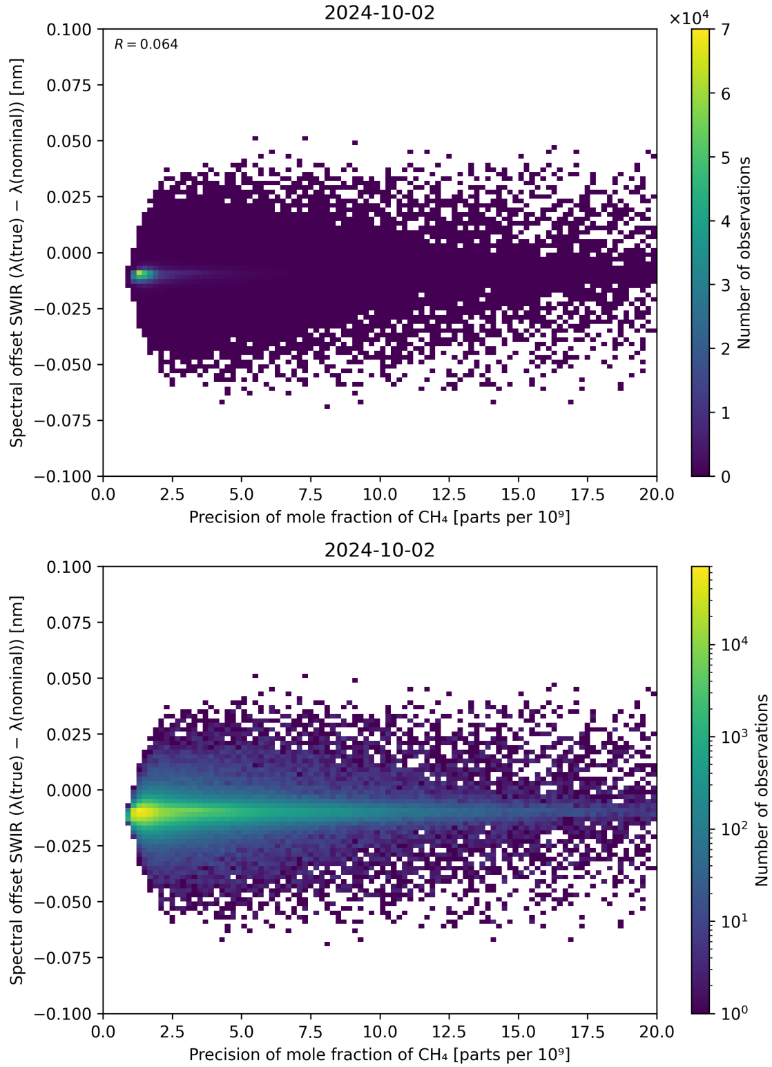
Figure 85: Scatter density plot of “Precision of mole fraction of CH 4 ” against “Spectral offset SWIR ( \lambda_{\text{true}} - \lambda_{\text{nominal}} )” for 2024-10-01 to 2024-10-03.
