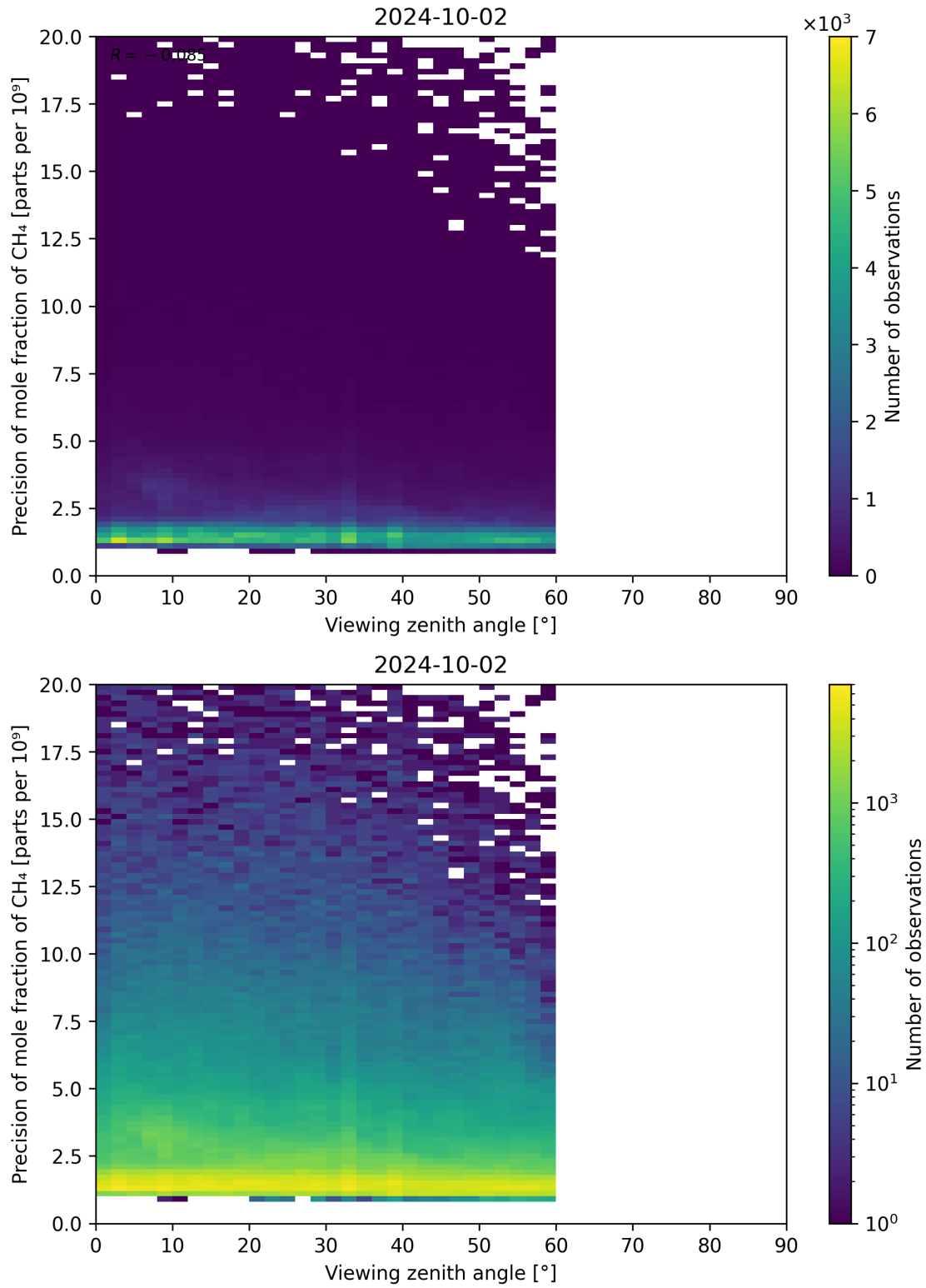
Figure 112: Scatter density plot of “Viewing zenith angle” against “Precision of mole fraction of CH 4 ” for 2024-10-01 to 2024-10-03.
