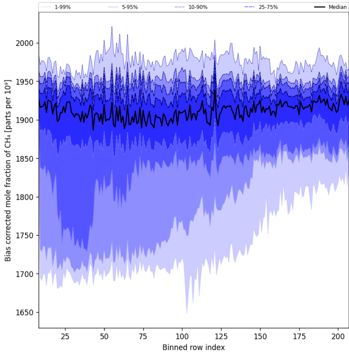
Figure 36: Along track statistics of “Bias corrected mole fraction of CH 4 ” for 2024-10-01 to 2024-10-03
