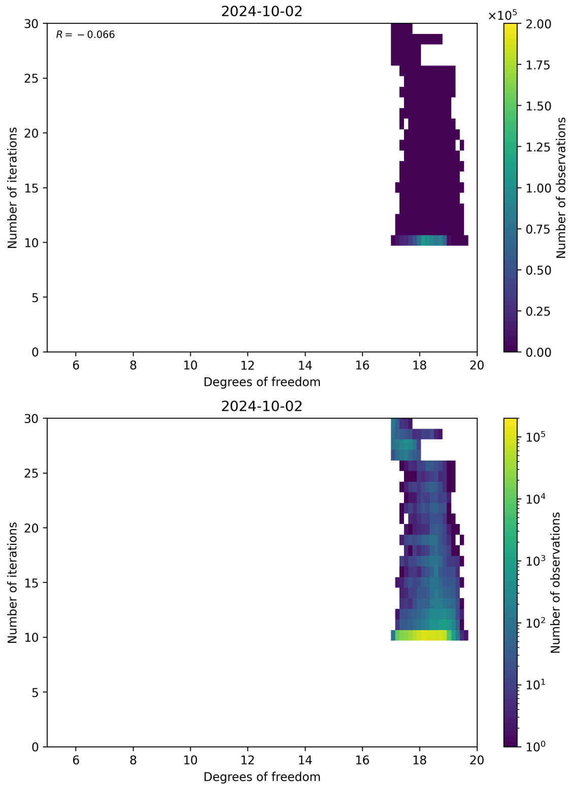
Figure 52: Scatter density plot of “Degrees of freedom” against “Number of iterations” for 2024-10-01 to 2024-10-03.
