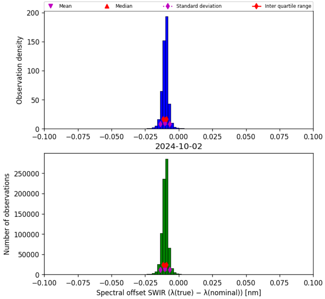
Figure 27: Histogram of “Spectral offset SWIR ( \lambda_{\text{true}} - \lambda_{\text{nominal}} )” for 2024-10-01 to 2024-10-03
