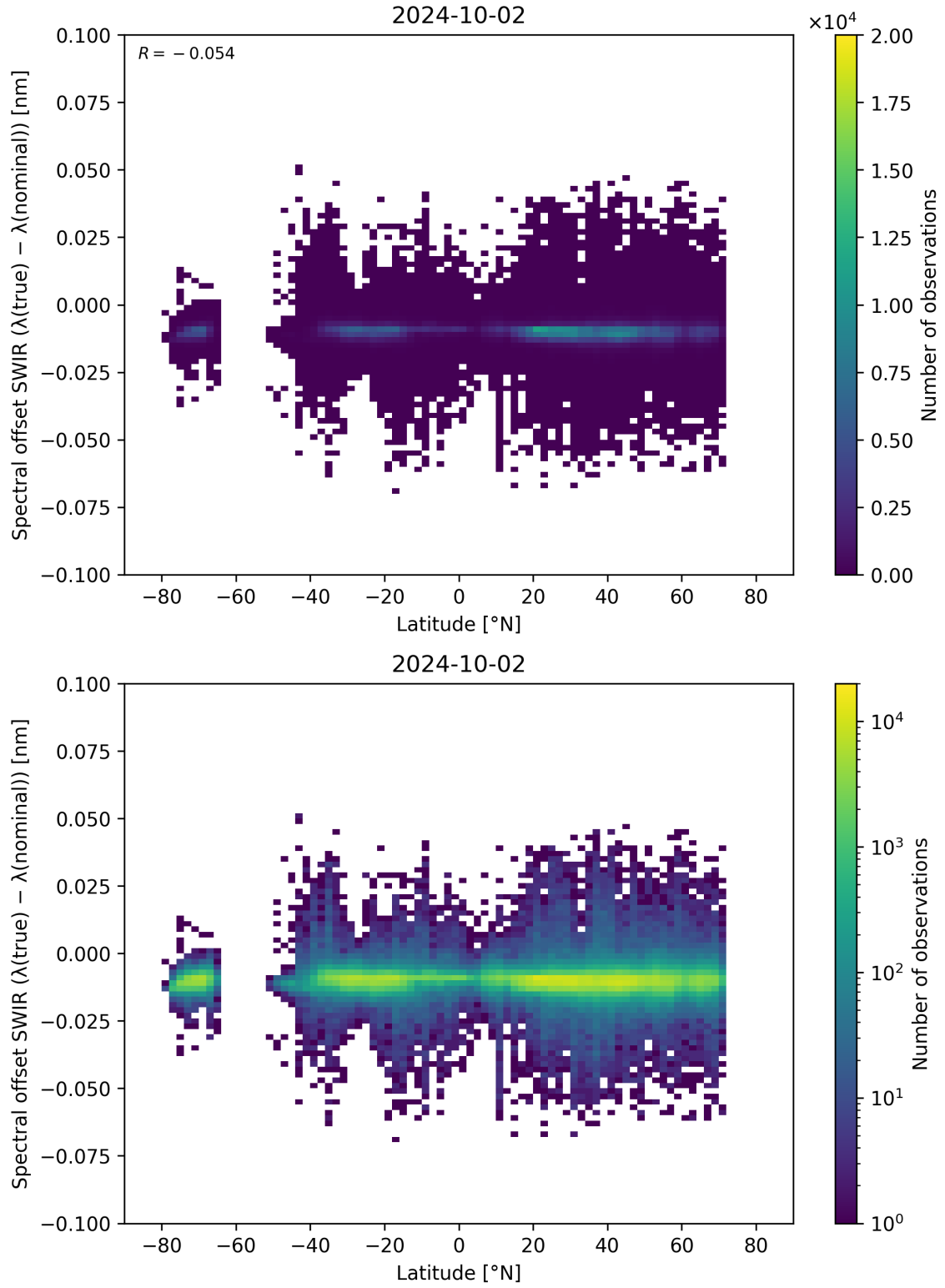
Figure 62: Scatter density plot of “Latitude” against “Spectral offset SWIR ( \lambda_{\text{true}} - \lambda_{\text{nominal}} )” for 2024-10-01 to 2024-10-03.
