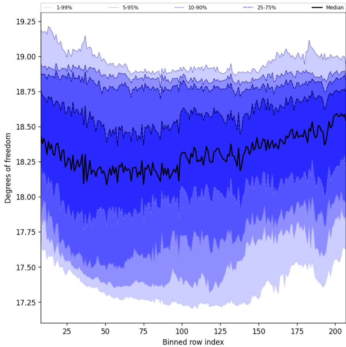
Figure 41: Along track statistics of “Degrees of freedom” for 2024-10-01 to 2024-10-03
