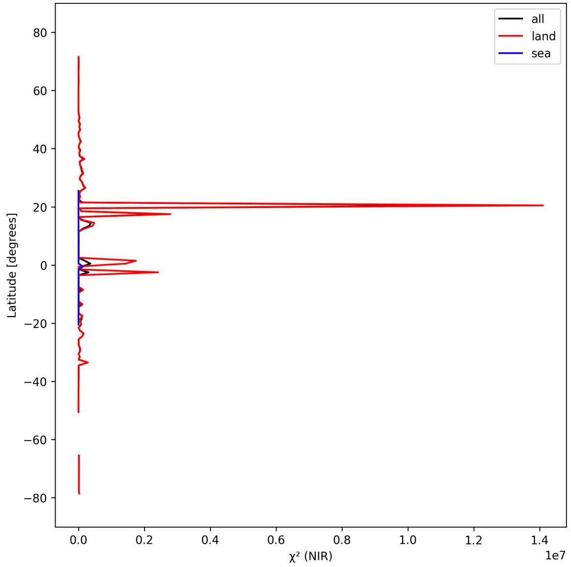
Figure 18: Zonal average of “ \chi^2 (NIR)” for 2024-10-01 to 2024-10-03.
