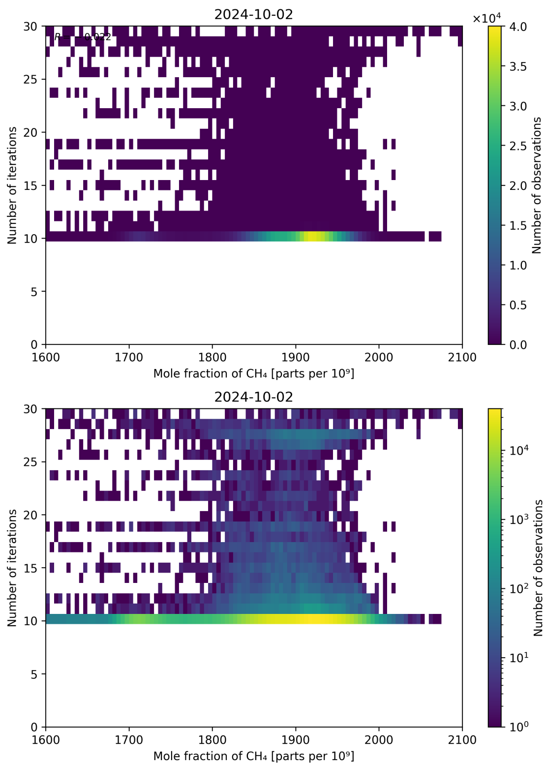
Figure 76: Scatter density plot of “Mole fraction of CH 4 ” against “Number of iterations” for 2024-10-01 to 2024-10-03.
