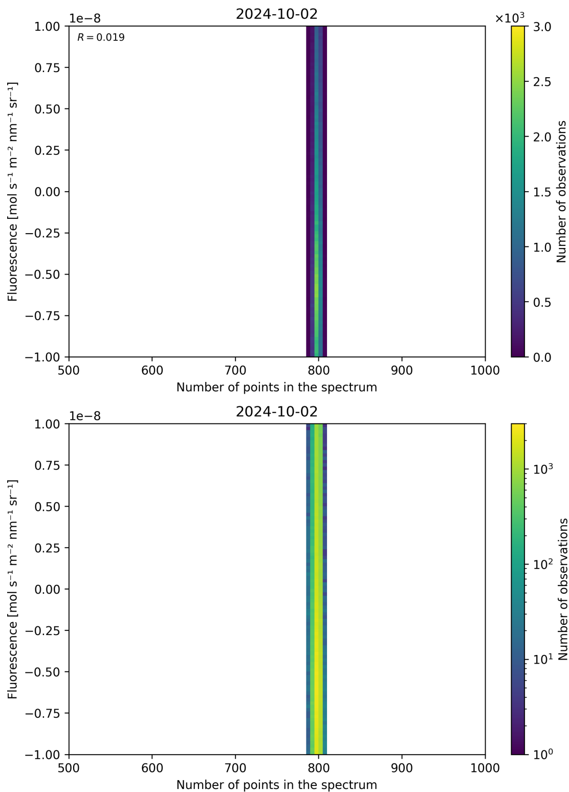
Figure 91: Scatter density plot of “Number of points in the spectrum” against “Fluorescence” for 2024-10-01 to 2024-10-03.
