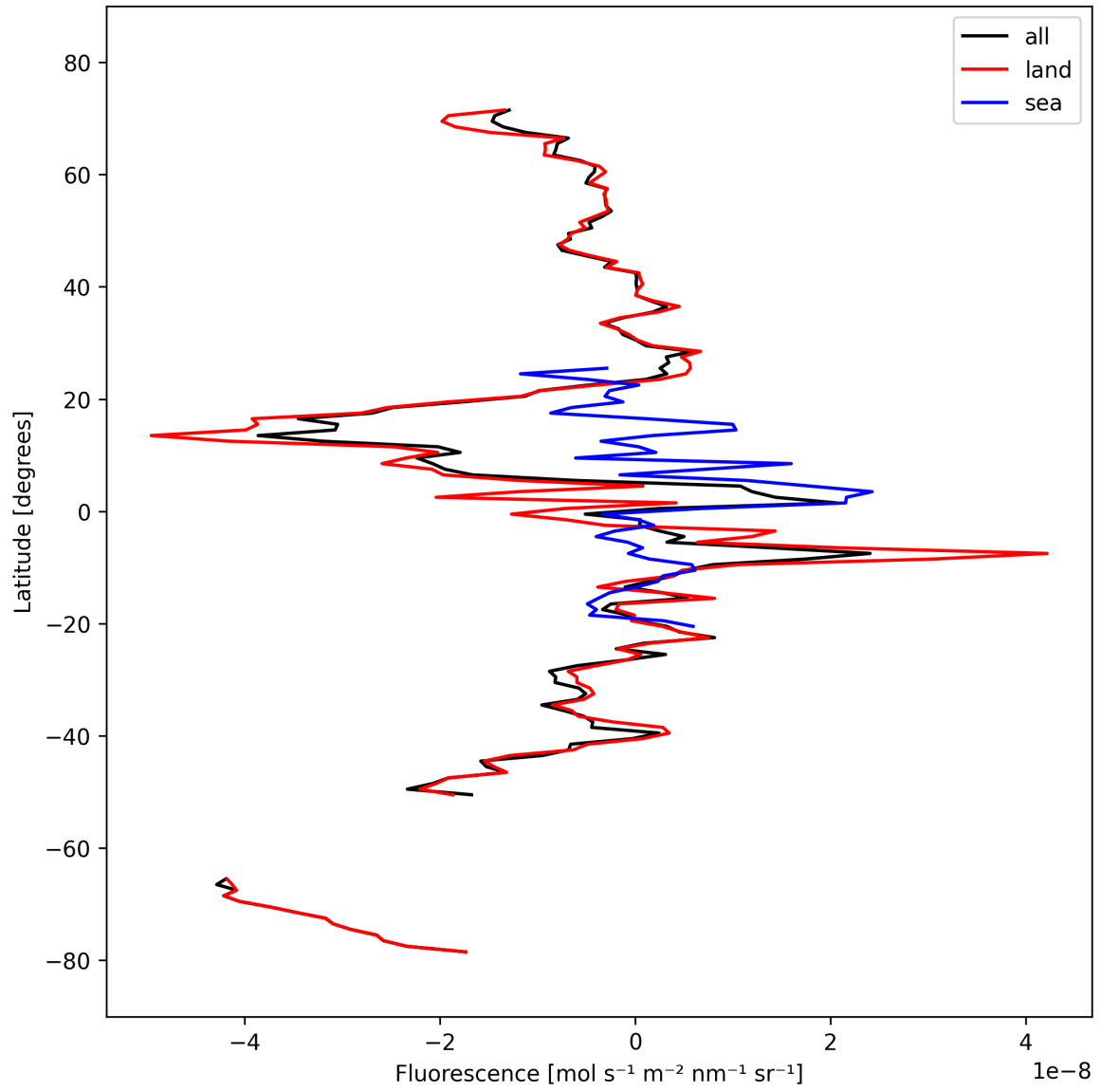
Figure 21: Zonal average of “Fluorescence” for 2024-10-01 to 2024-10-03.
