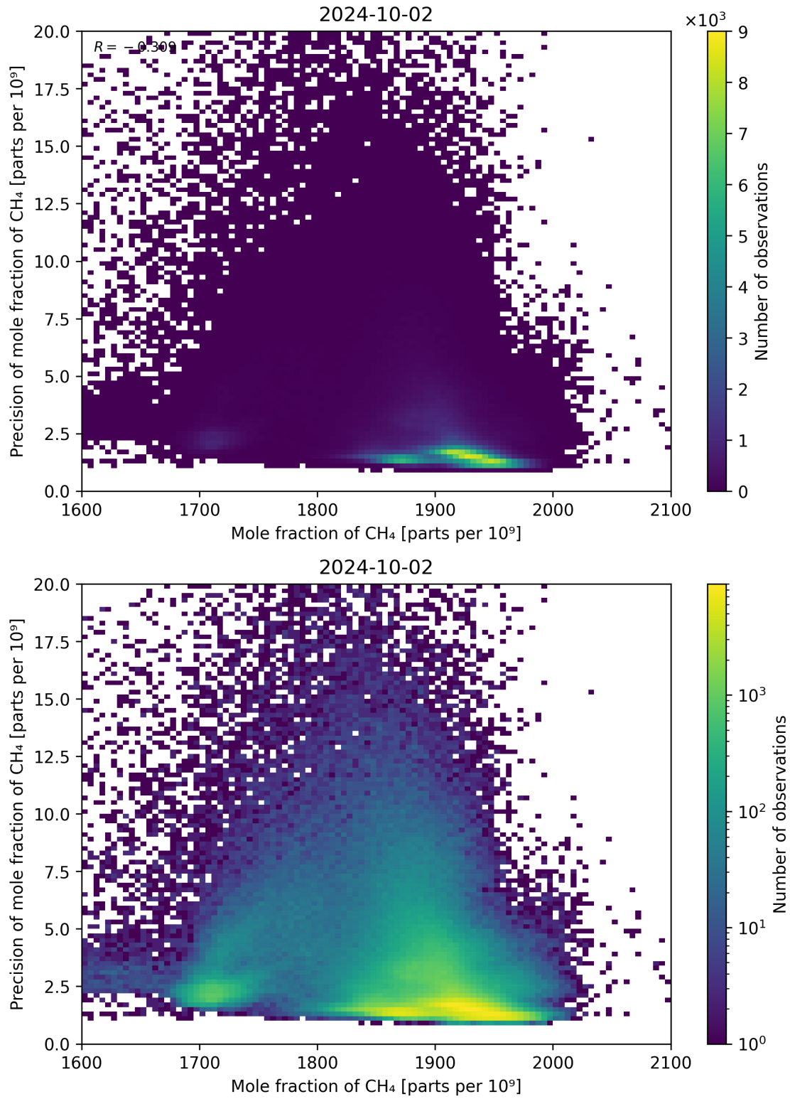
Figure 75: Scatter density plot of “Mole fraction of CH 4 ” against “Precision of mole fraction of CH 4 ” for 2024-10-01 to 2024-10-03.
