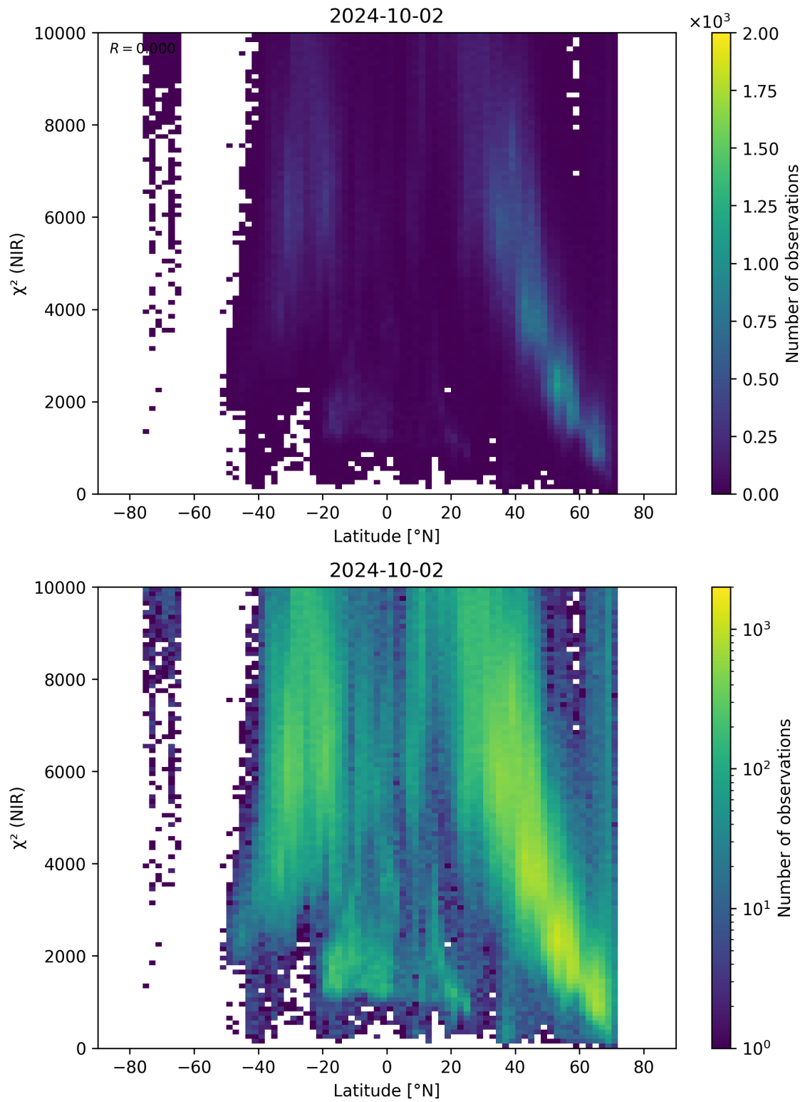
Figure 53: Scatter density plot of “Latitude” against “ \chi^2 (NIR)” for 2024-10-01 to 2024-10-03.
