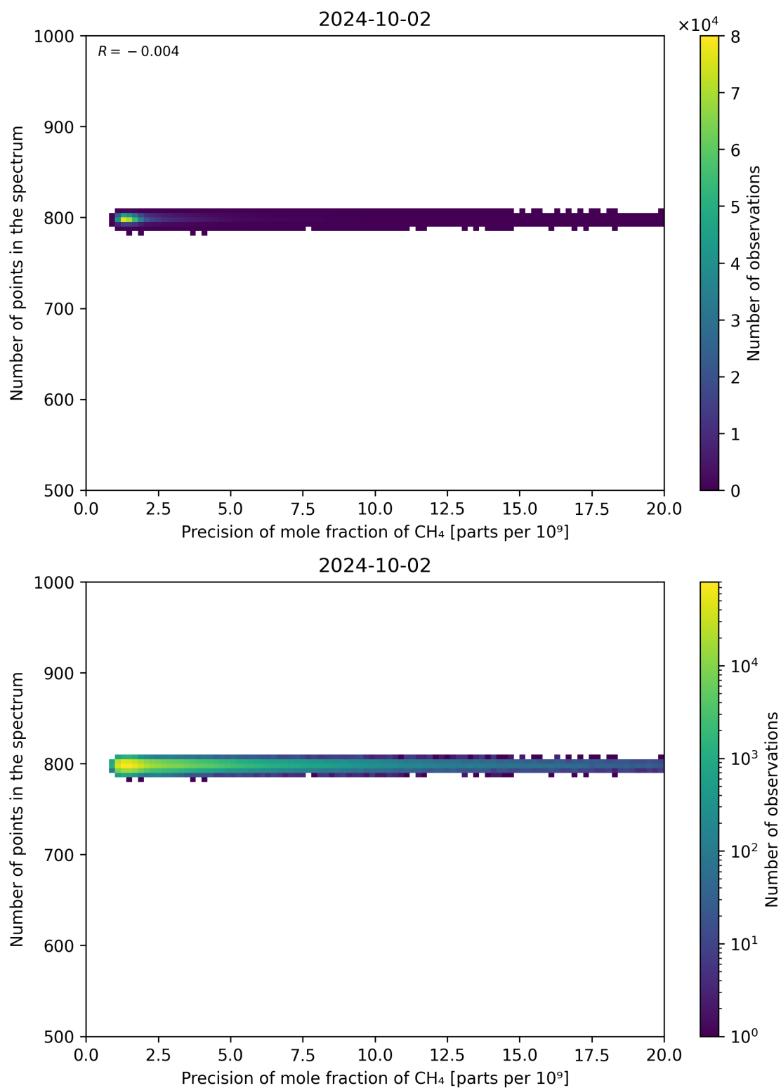
Figure 84: Scatter density plot of “Precision of mole fraction of CH 4 ” against “Number of points in the spectrum” for 2024-10-01 to 2024-10-03.
