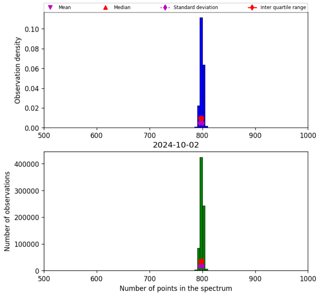
Figure 26: Histogram of “Number of points in the spectrum” for 2024-10-01 to 2024-10-03
