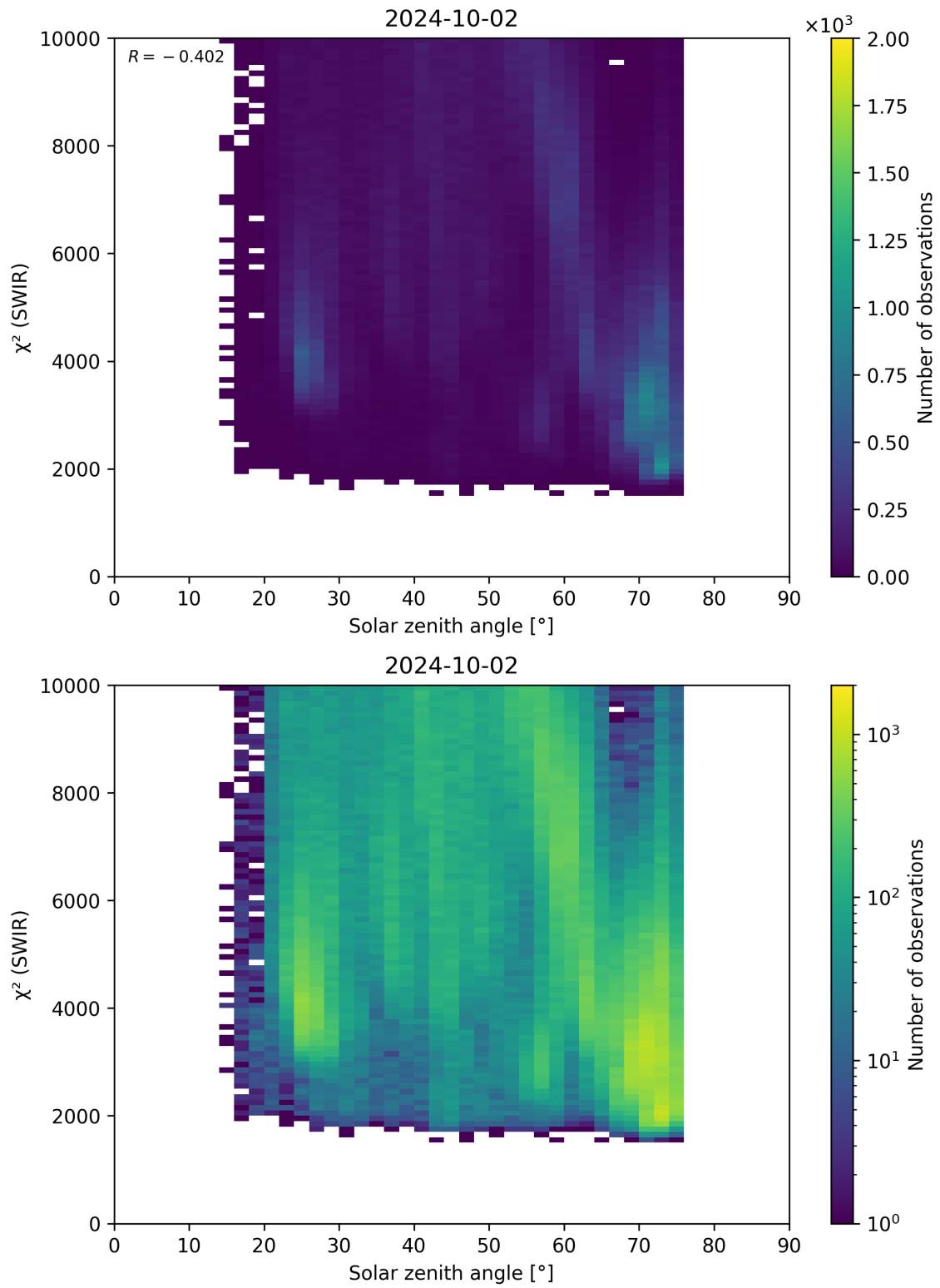
Figure 95: Scatter density plot of “Solar zenith angle” against “ \chi^2 (SWIR)” for 2024-10-01 to 2024-10-03.
