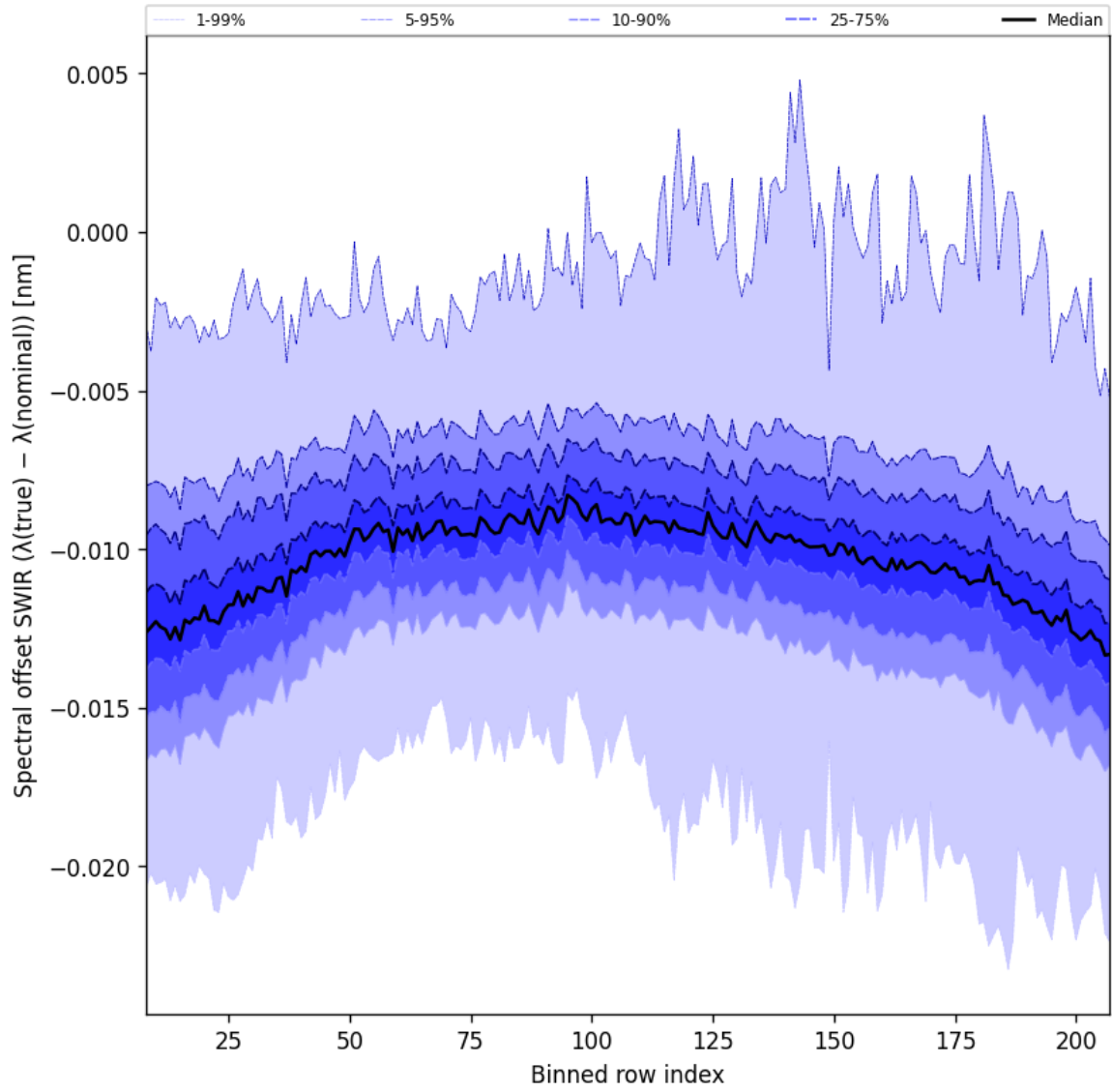
Figure 38: Along track statistics of “Spectral offset SWIR ( \lambda_{\text{true}} - \lambda_{\text{nominal}} )” for 2024-10-01 to 2024-10-03
