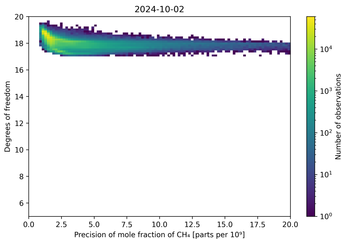
Figure 80: Scatter density plot of “Precision of mole fraction of CH 4 ” against “Degrees of freedom” for 2024-10-01 to 2024-10-03.
