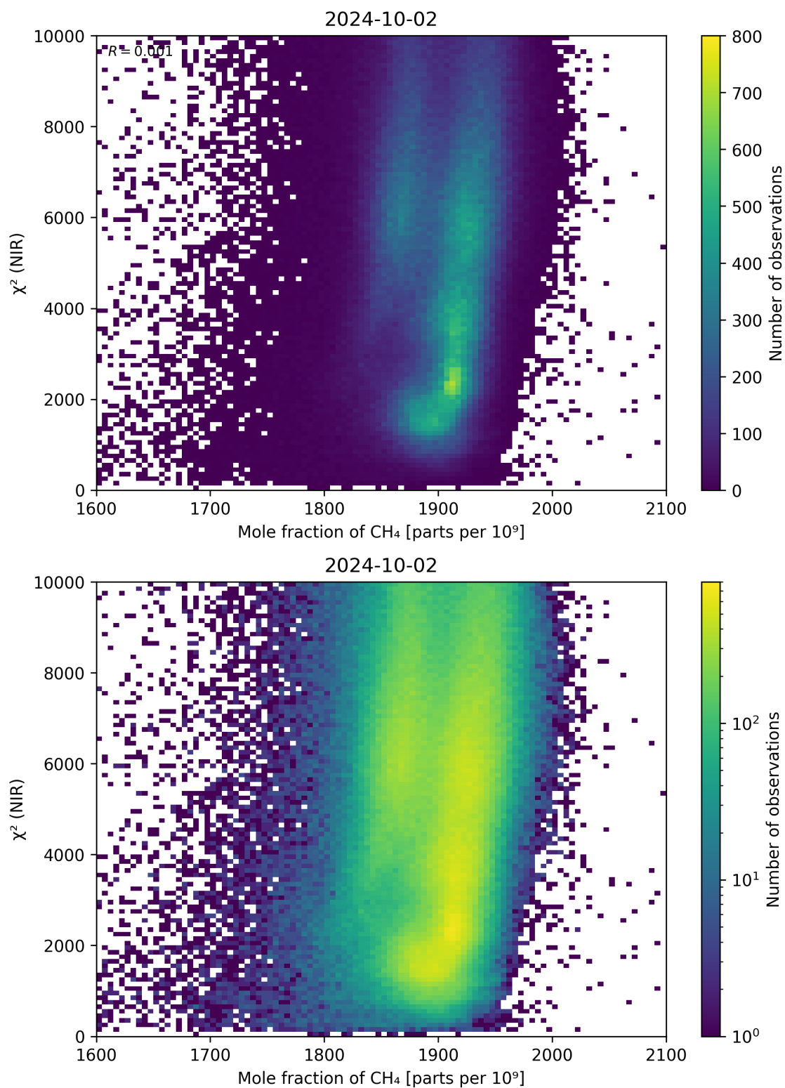
Figure 70: Scatter density plot of “Mole fraction of CH 4 ” against “ \chi^2 (NIR)” for 2024-10-01 to 2024-10-03.
