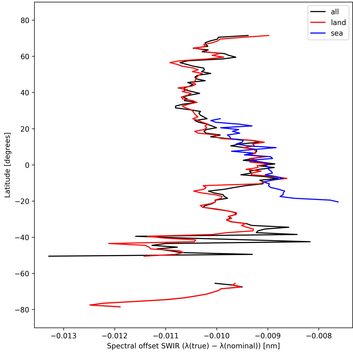
Figure 16: Zonal average of “Spectral offset SWIR ( \lambda_{\text{true}} - \lambda_{\text{nominal}} )” for 2024-10-01 to 2024-10-03.
