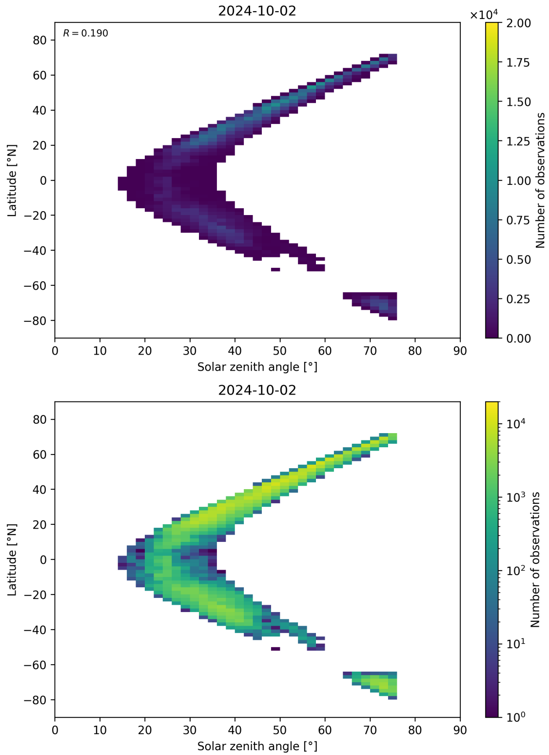
Figure 98: Scatter density plot of “Solar zenith angle” against “Latitude” for 2024-10-01 to 2024-10-03.
