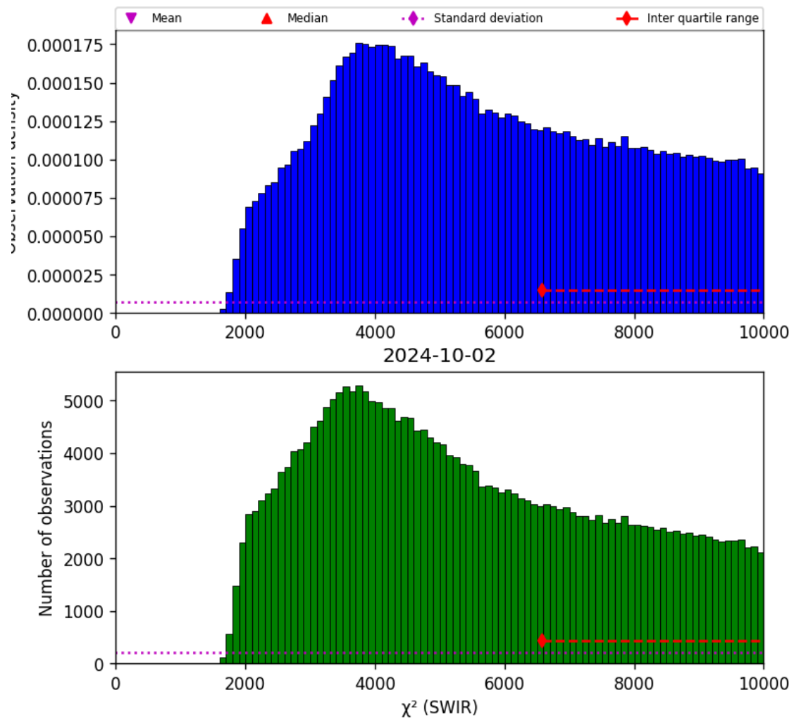
Figure 28: Histogram of “ \chi^2 (SWIR)” for 2024-10-01 to 2024-10-03
