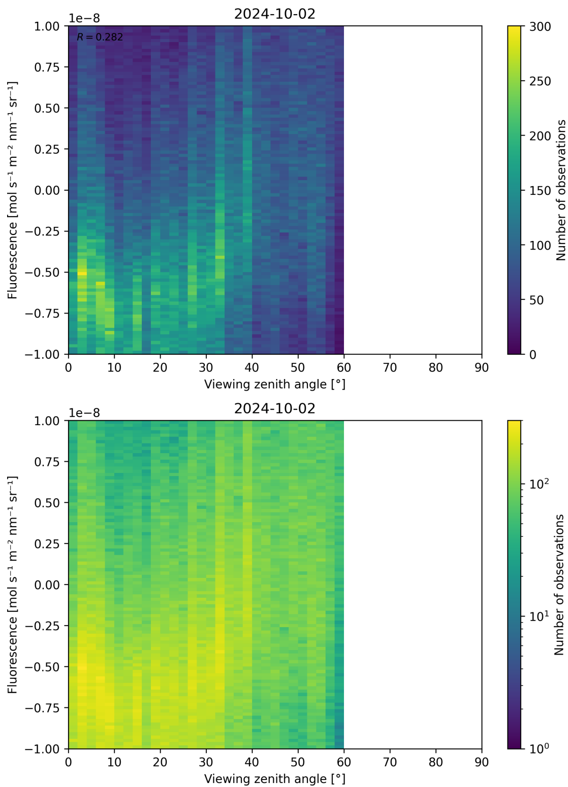
Figure 108: Scatter density plot of “Viewing zenith angle” against “Fluorescence” for 2024-10-01 to 2024-10-03.
