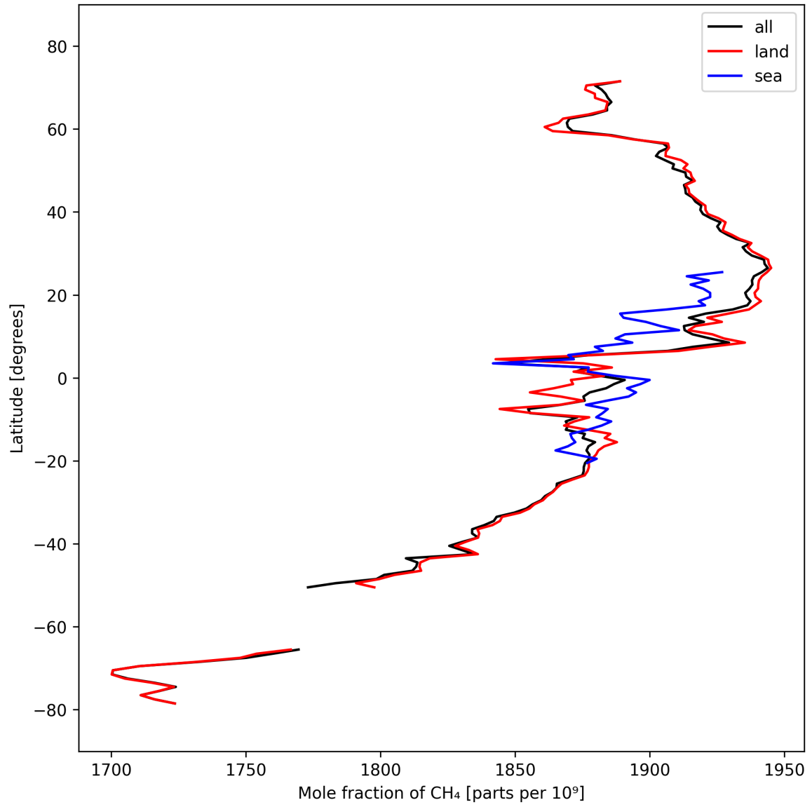
Figure 12: Zonal average of “Mole fraction of CH 4 ” for 2024-10-01 to 2024-10-03.
