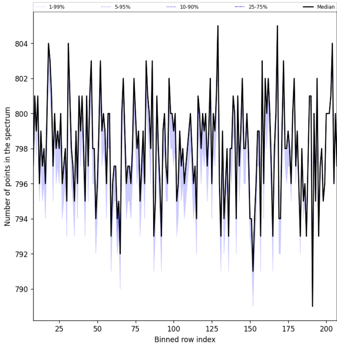
Figure 37: Along track statistics of “Number of points in the spectrum” for 2024-10-01 to 2024-10-03
