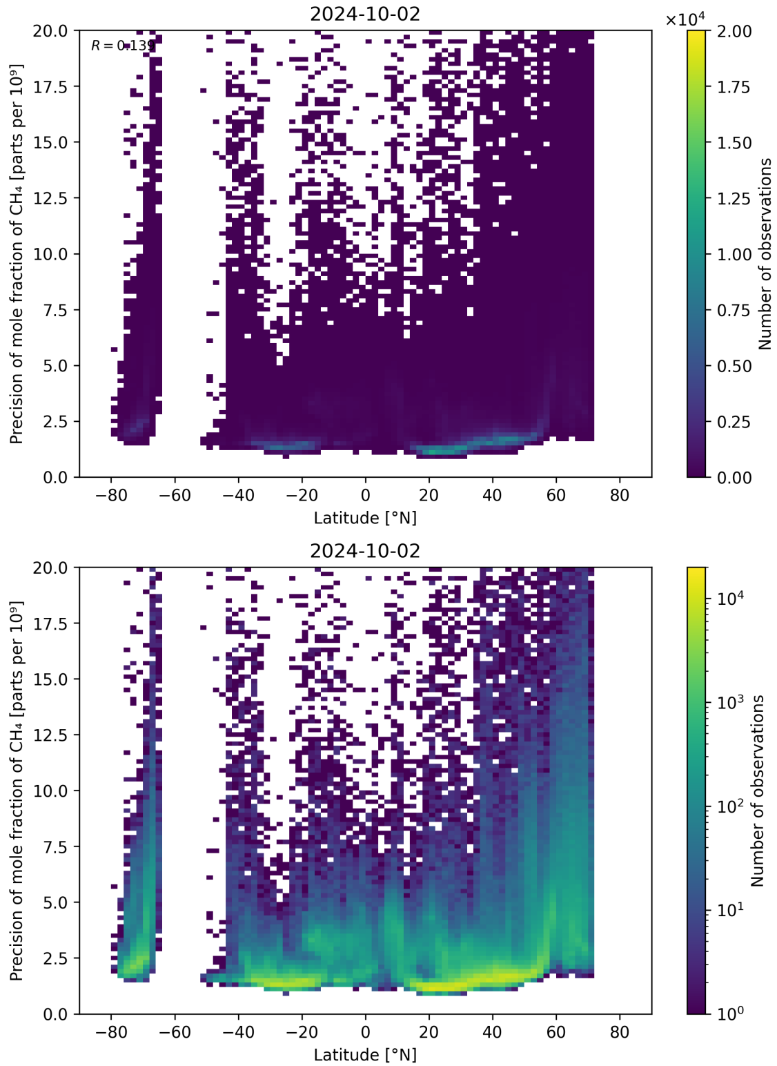
Figure 59: Scatter density plot of “Latitude” against “Precision of mole fraction of CH 4 ” for 2024-10-01 to 2024-10-03.
