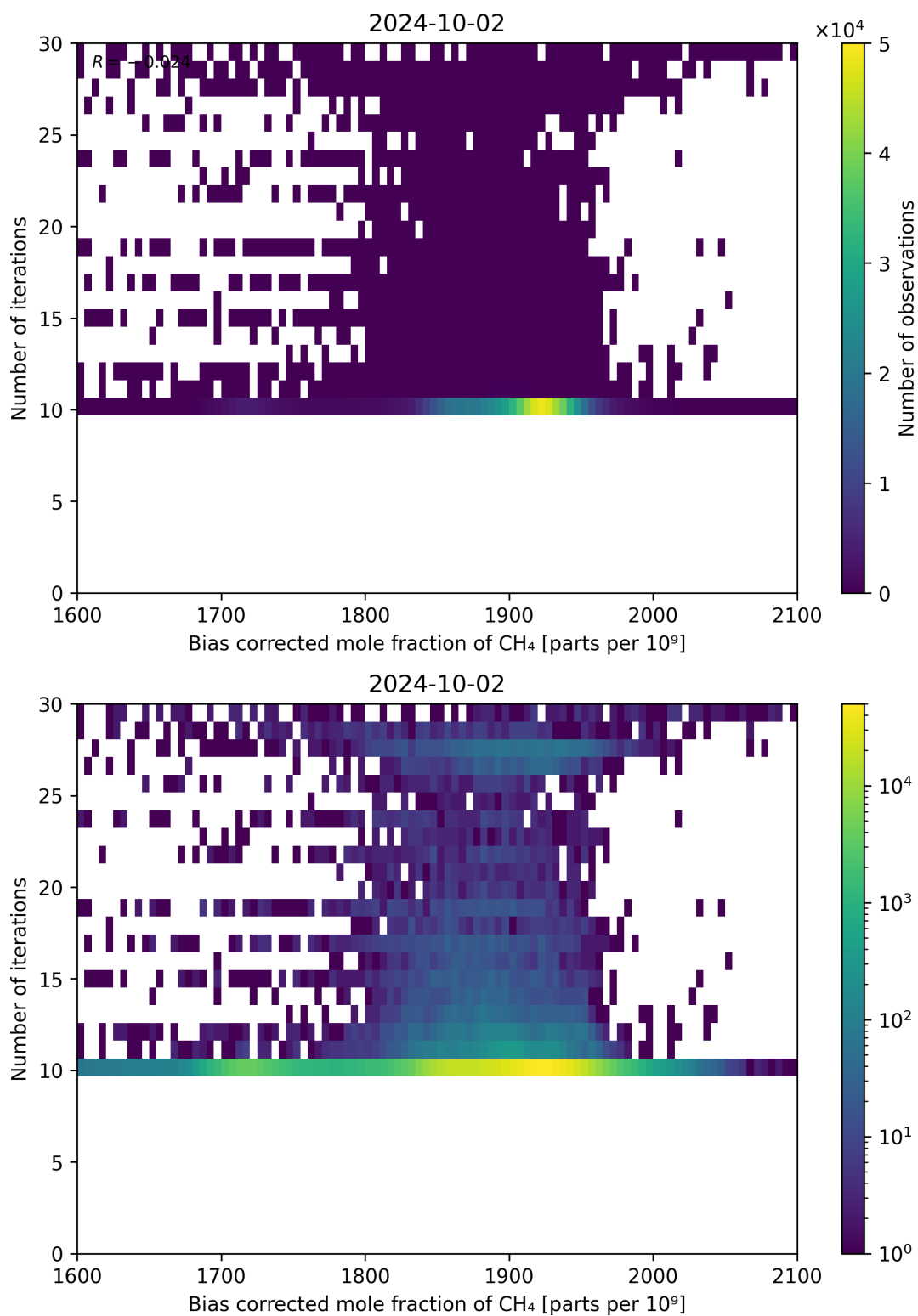
Figure 67: Scatter density plot of “Bias corrected mole fraction of \text{CH}_4 ” against “Number of iterations” for 2024-10-01 to 2024-10-03.
