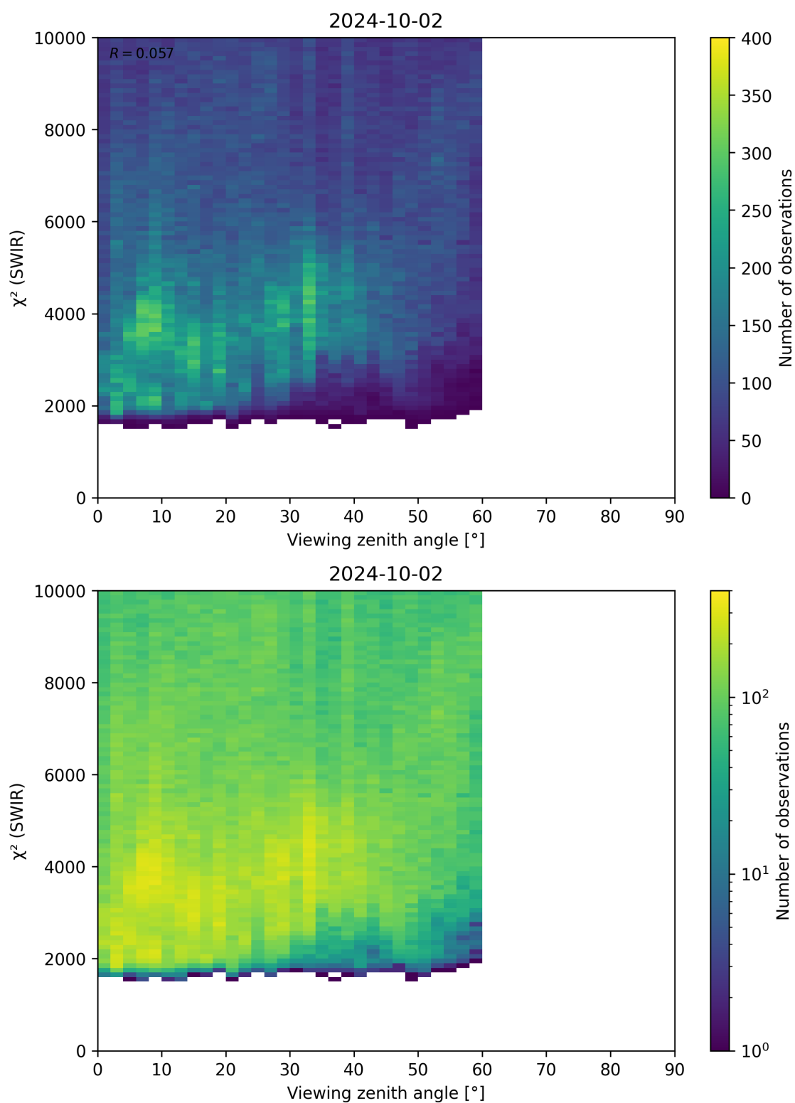
Figure 106: Scatter density plot of “Viewing zenith angle” against “ \chi^2 (SWIR)” for 2024-10-01 to 2024-10-03.
