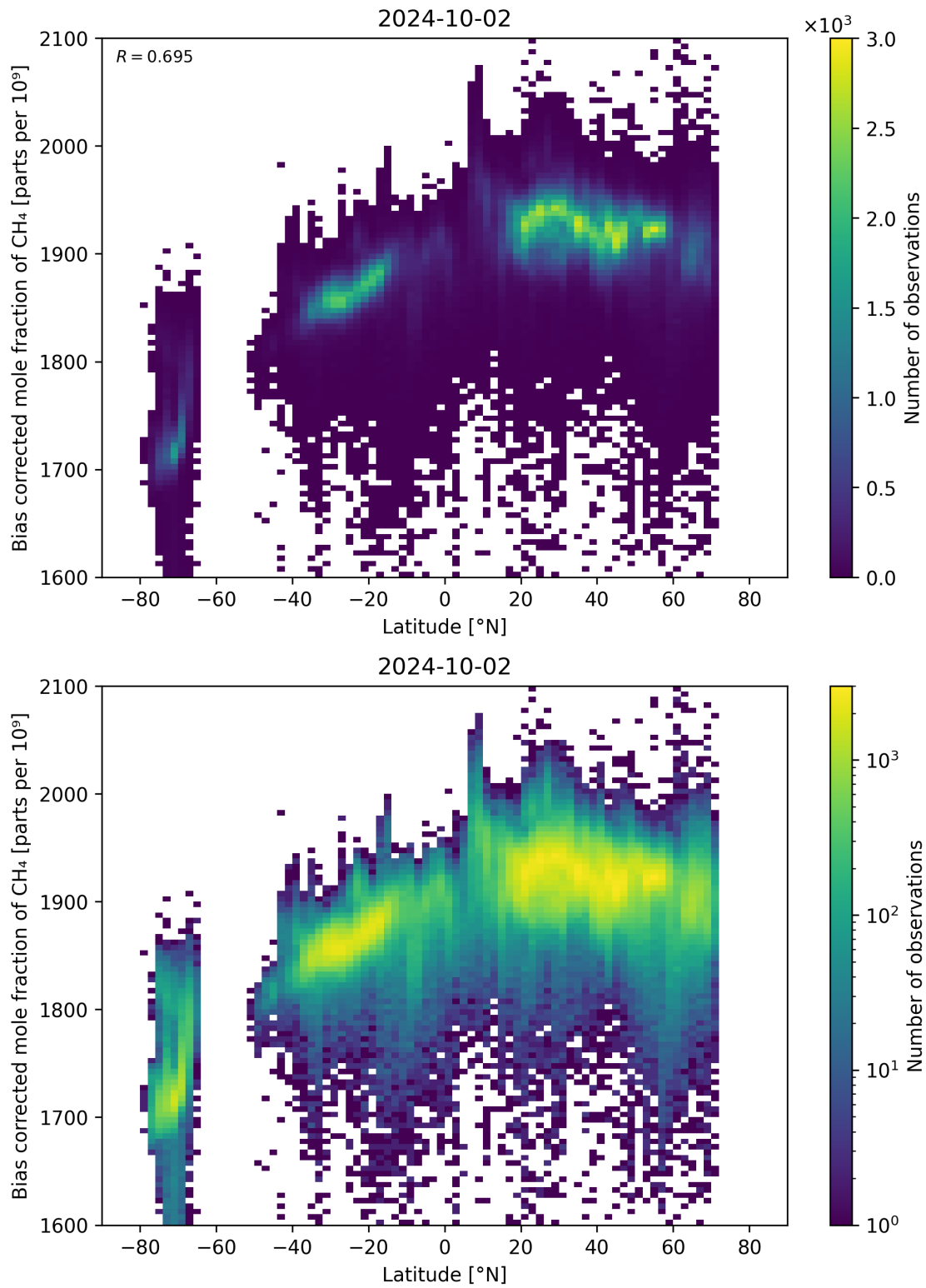
Figure 58: Scatter density plot of “Latitude” against “Bias corrected mole fraction of \text{CH}_4 ” for 2024-10-01 to 2024-10-03.
