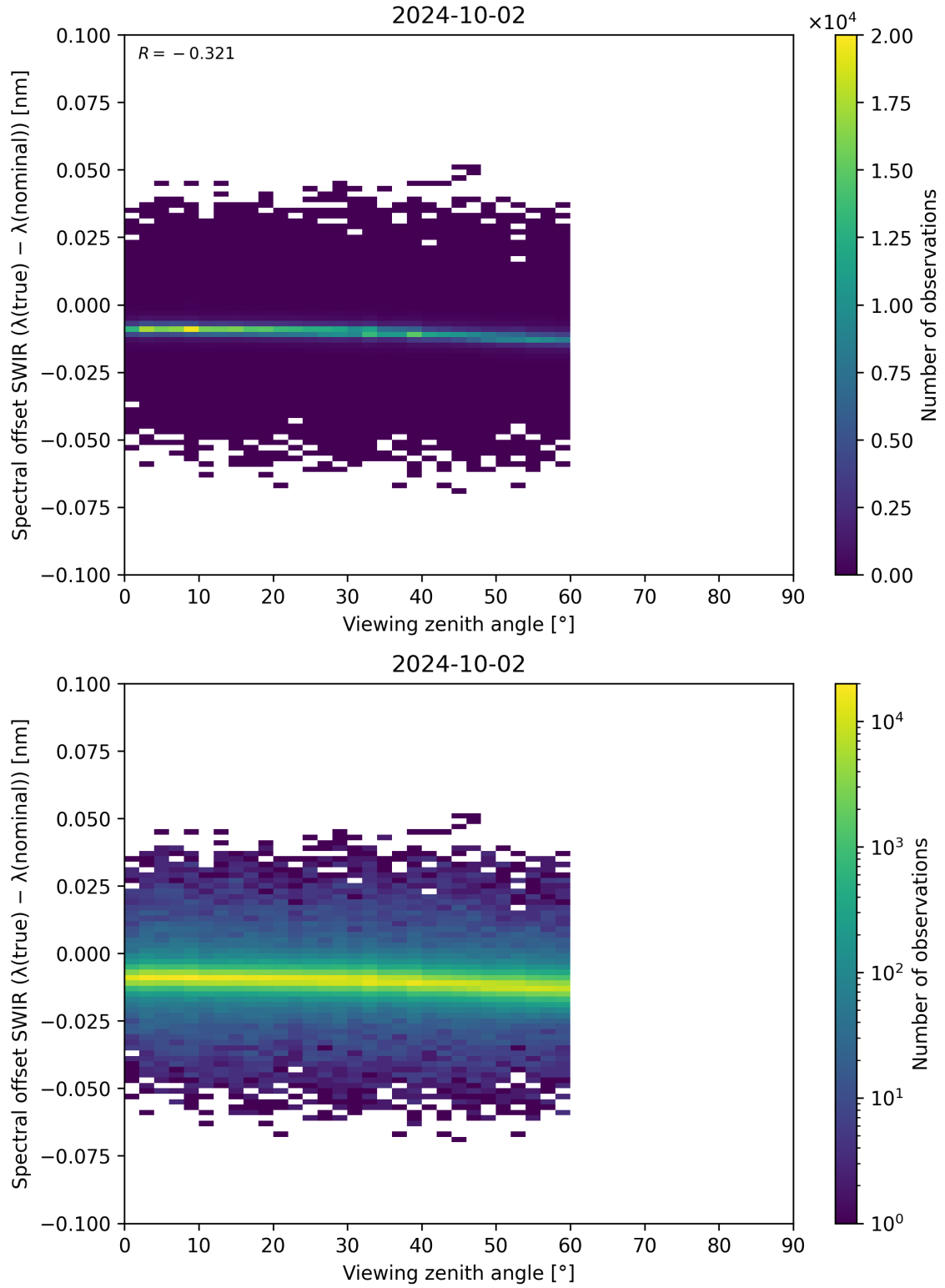
Figure 116: Scatter density plot of “Viewing zenith angle” against “Spectral offset SWIR ( \lambda_{\text{true}} - \lambda_{\text{nominal}} )” for 2024-10-01 to 2024-10-03.
