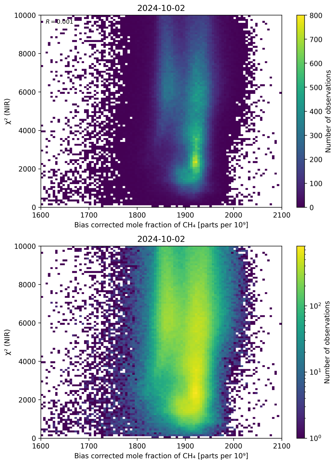
Figure 63: Scatter density plot of “Bias corrected mole fraction of \text{CH}_4 ” against “ \chi^2 (NIR)” for 2024-10-01 to 2024-10-03.
