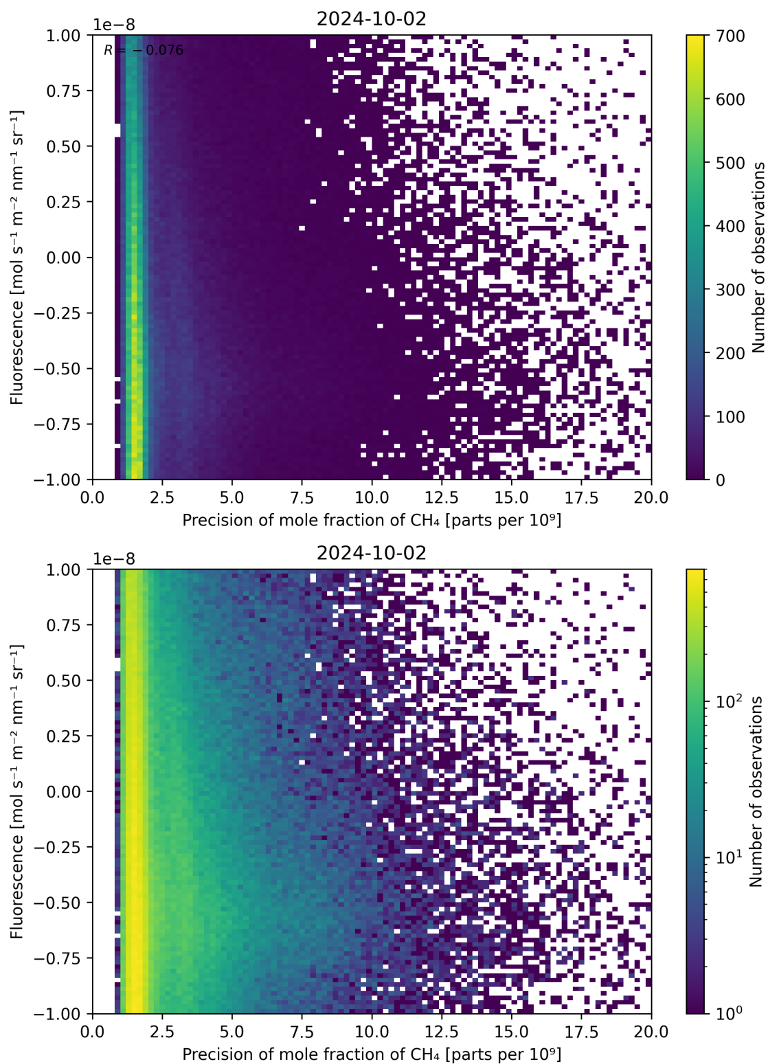
Figure 81: Scatter density plot of “Precision of mole fraction of \text{CH}_4 ” against “Fluorescence” for 2024-10-01 to 2024-10-03.
