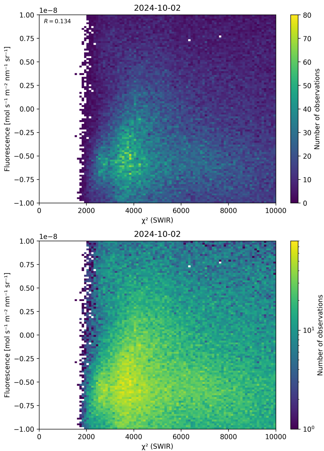
Figure 49: Scatter density plot of “ \chi^2 (SWIR)” against “Fluorescence” for 2024-10-01 to 2024-10-03.
