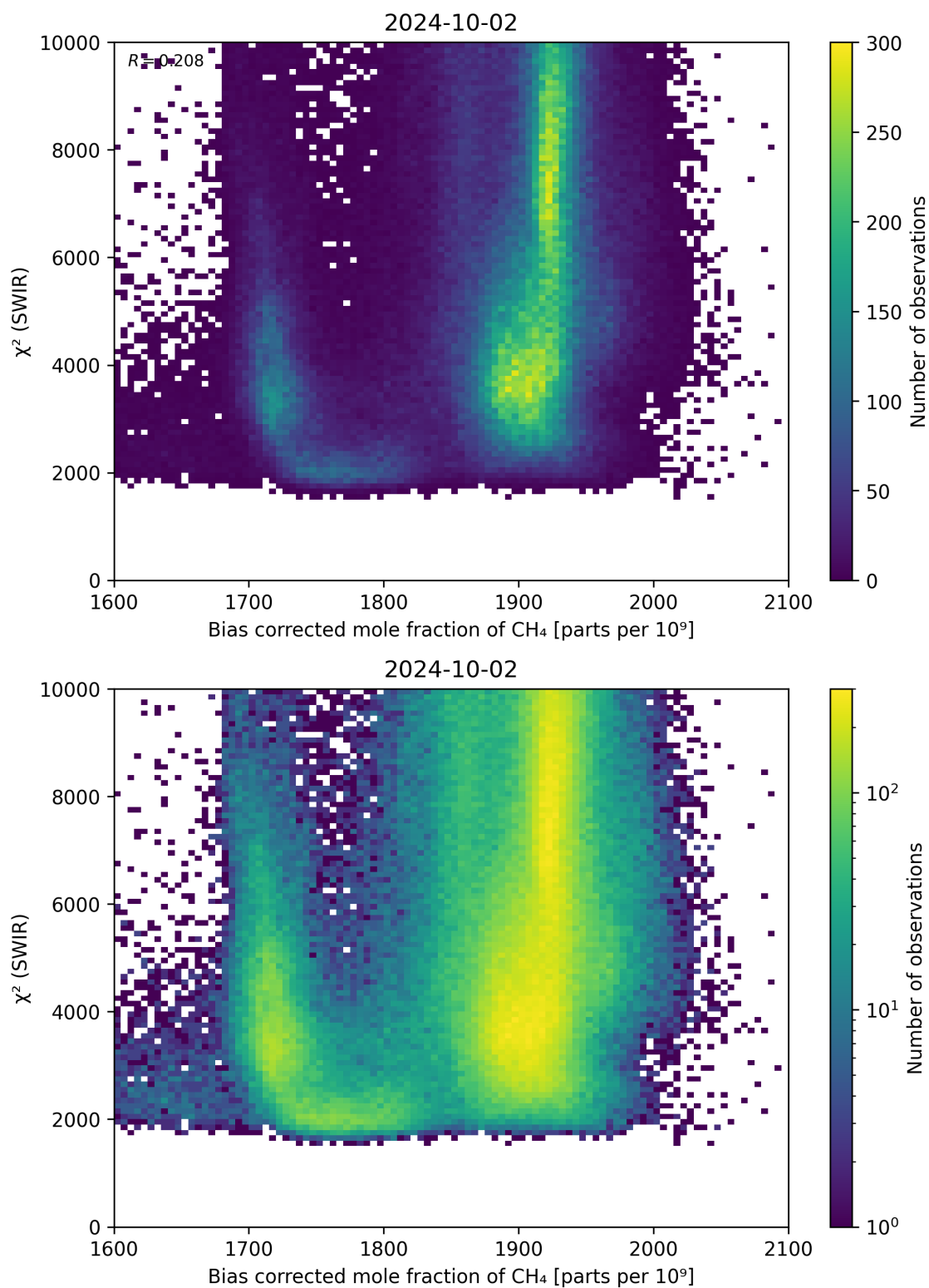
Figure 64: Scatter density plot of “Bias corrected mole fraction of \text{CH}_4 ” against “ \chi^2 (SWIR)” for 2024-10-01 to 2024-10-03.
