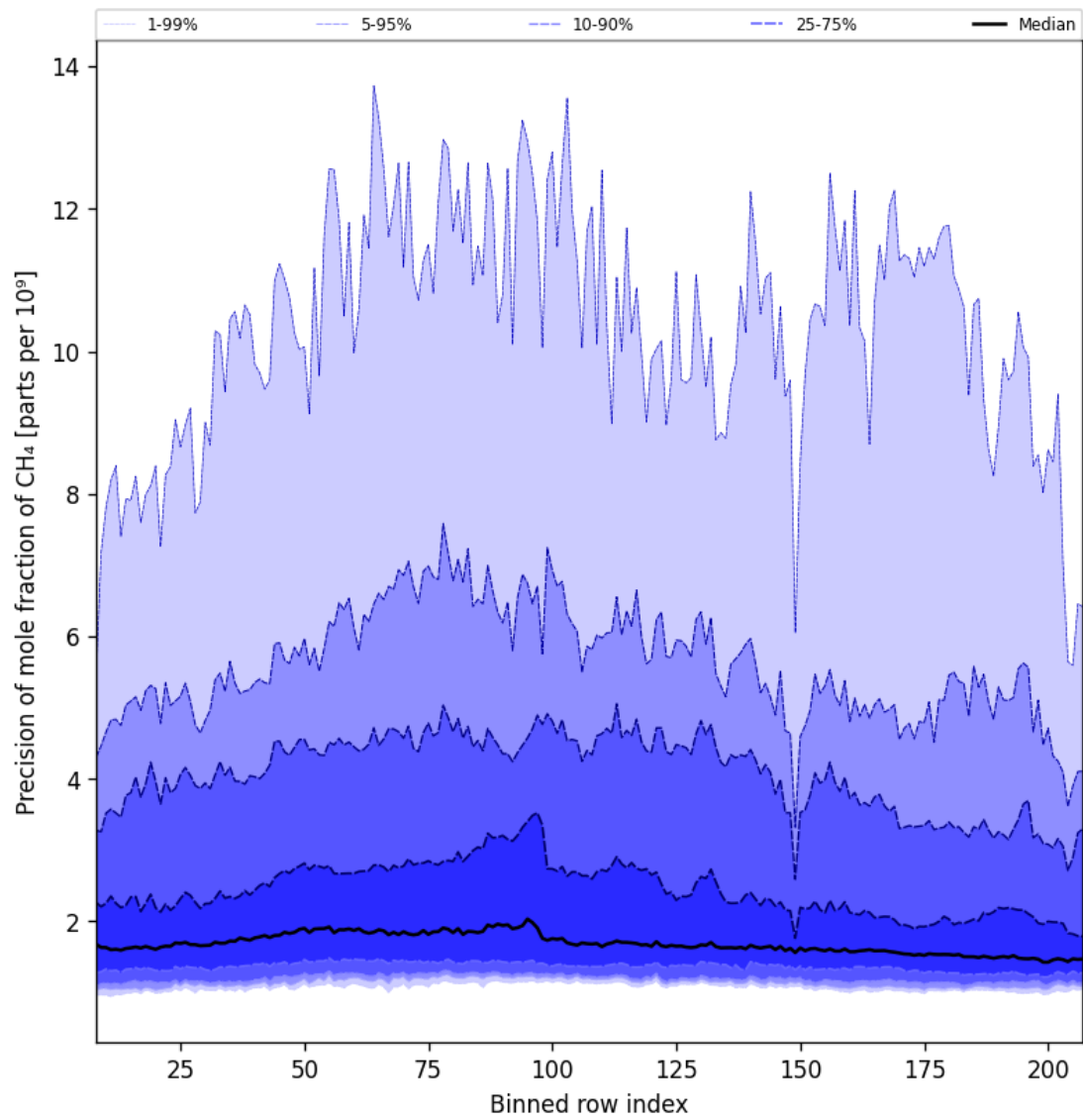
Figure 35: Along track statistics of “Precision of mole fraction of CH 4 ” for 2024-10-01 to 2024-10-03
