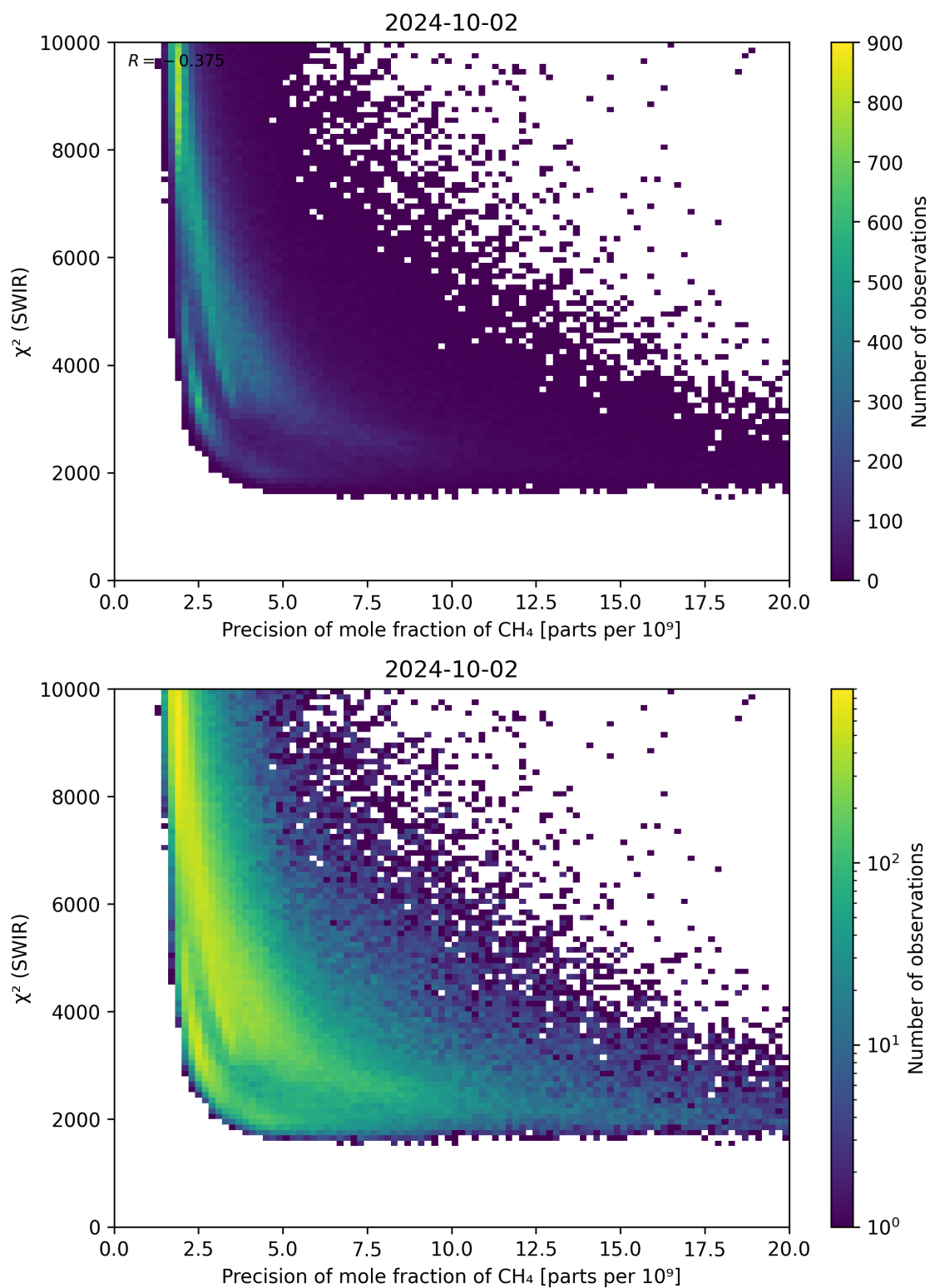
Figure 79: Scatter density plot of “Precision of mole fraction of \text{CH}_4 ” against “ \chi^2 (SWIR)” for 2024-10-01 to 2024-10-03.
