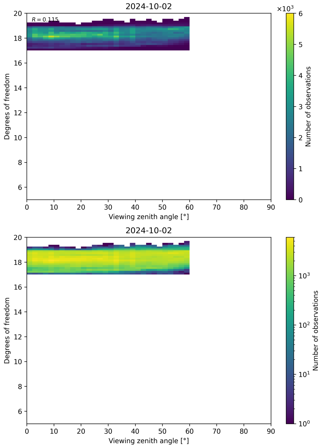
Figure 107: Scatter density plot of “Viewing zenith angle” against “Degrees of freedom” for 2024-10-01 to 2024-10-03.
