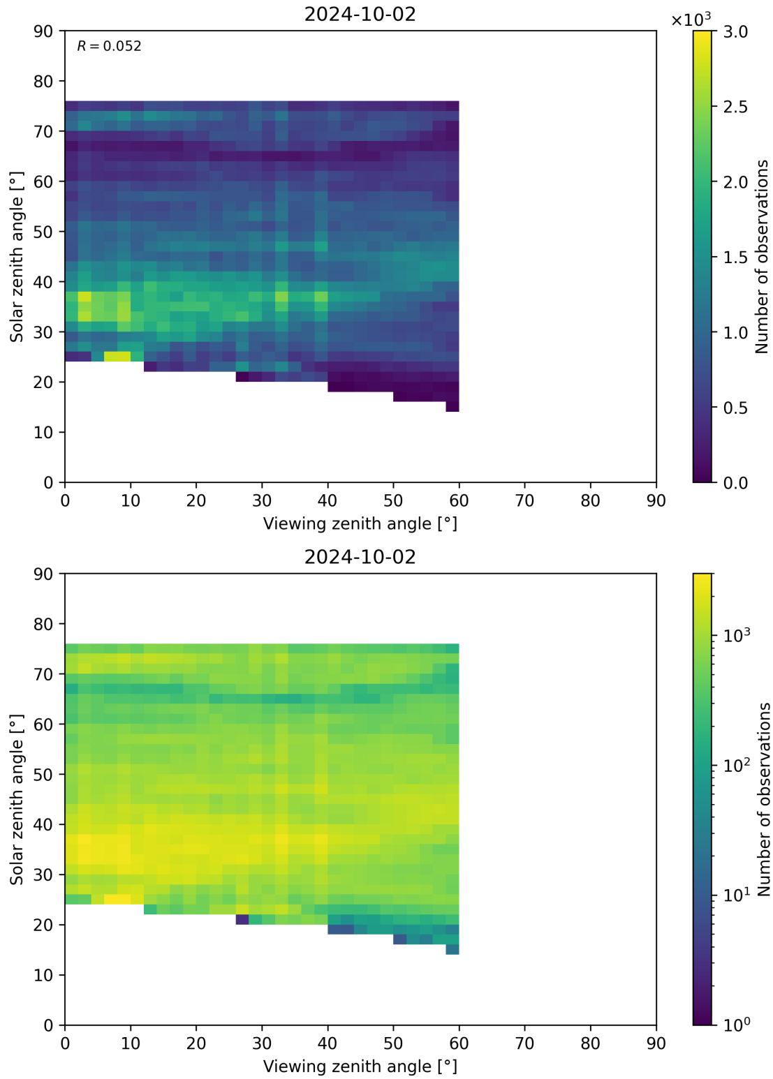
Figure 115: Scatter density plot of “Viewing zenith angle” against “Solar zenith angle” for 2024-10-01 to 2024-10-03.
