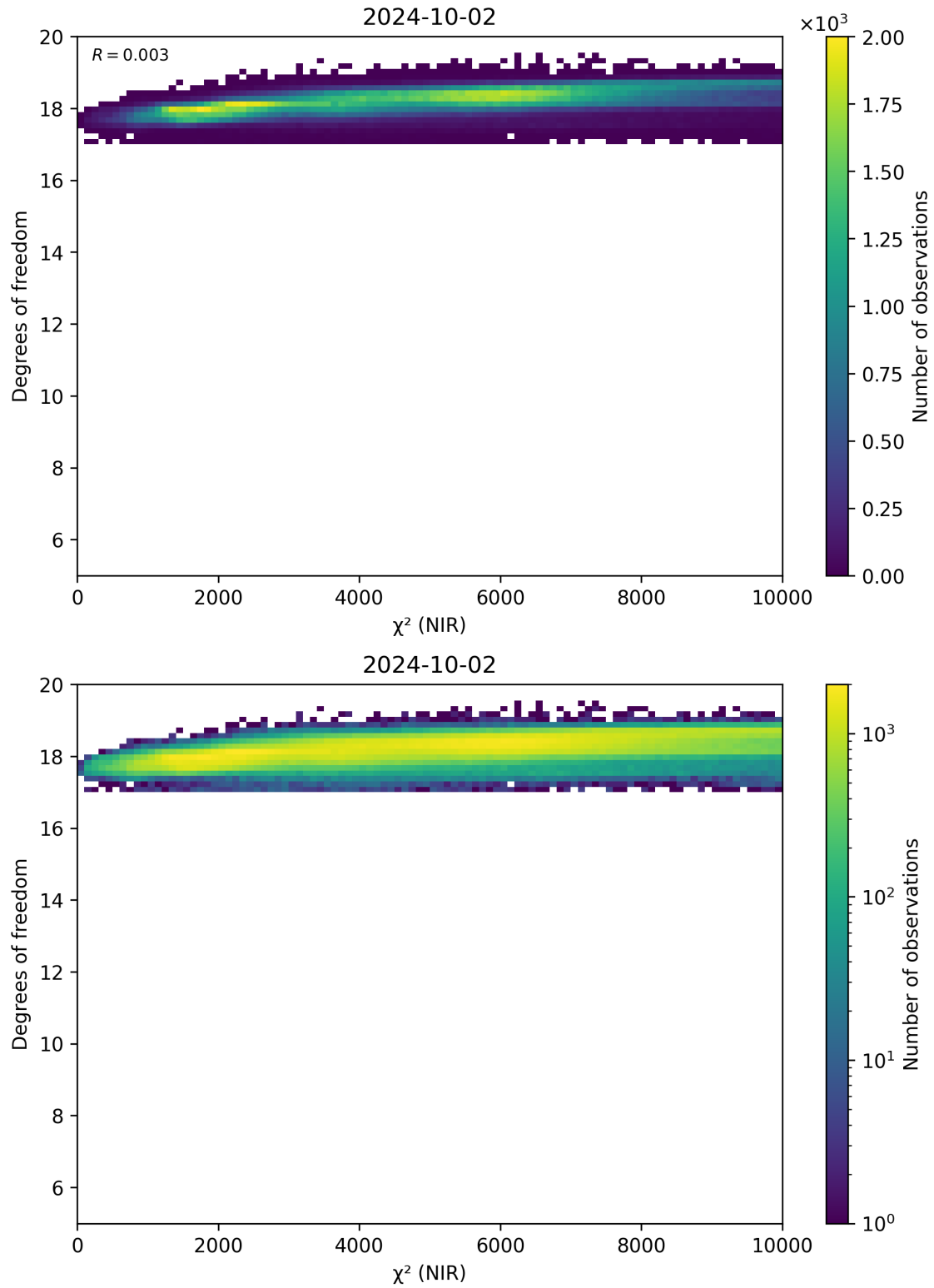
Figure 44: Scatter density plot of “ \chi^2 (NIR)” against “Degrees of freedom” for 2024-10-01 to 2024-10-03.
