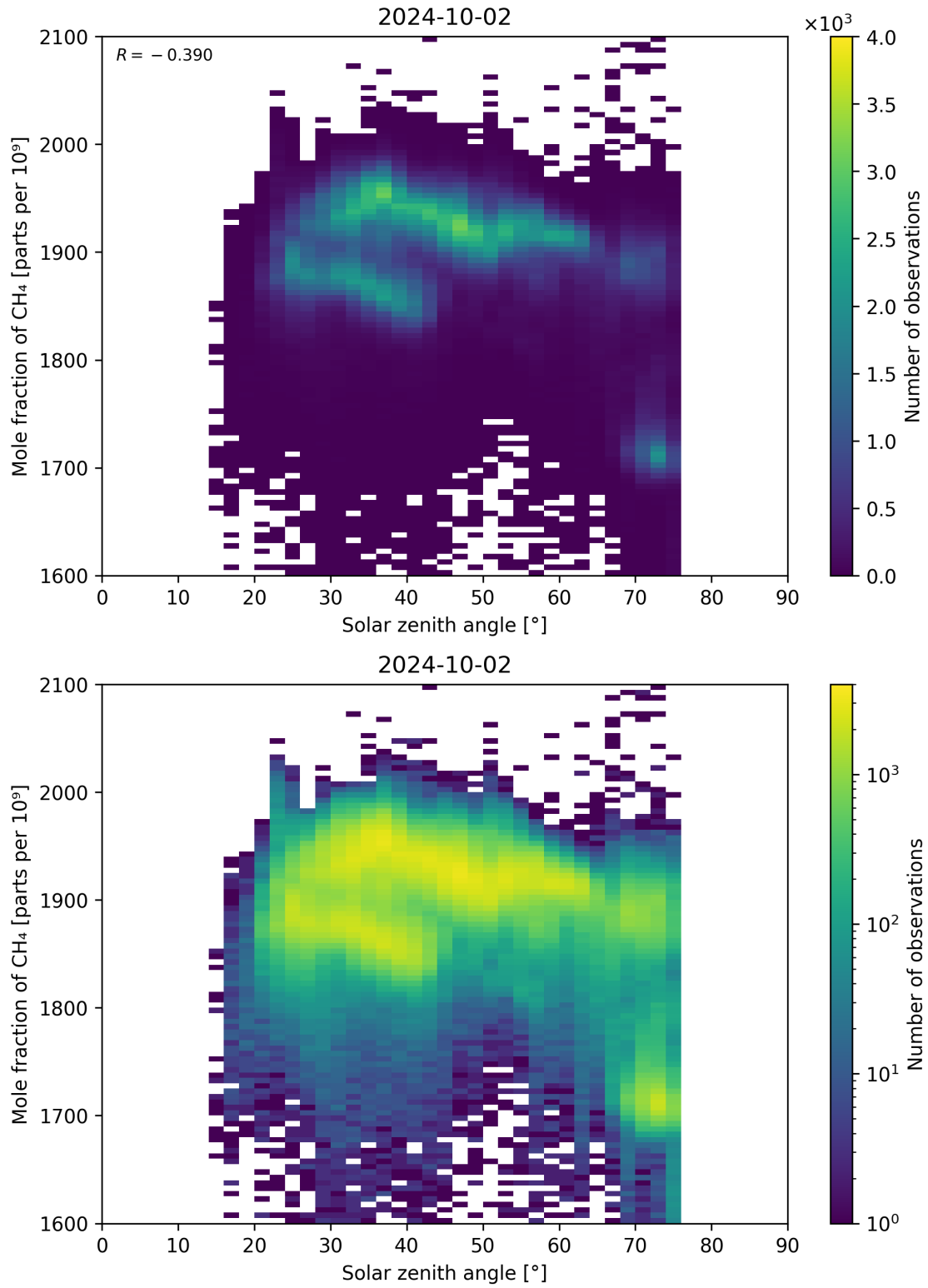
Figure 99: Scatter density plot of “Solar zenith angle” against “Mole fraction of CH 4 ” for 2024-10-01 to 2024-10-03.
