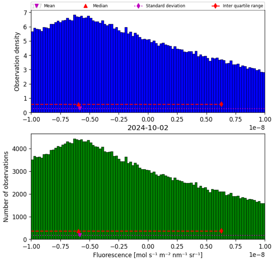
Figure 32: Histogram of “Fluorescence” for 2024-10-01 to 2024-10-03
