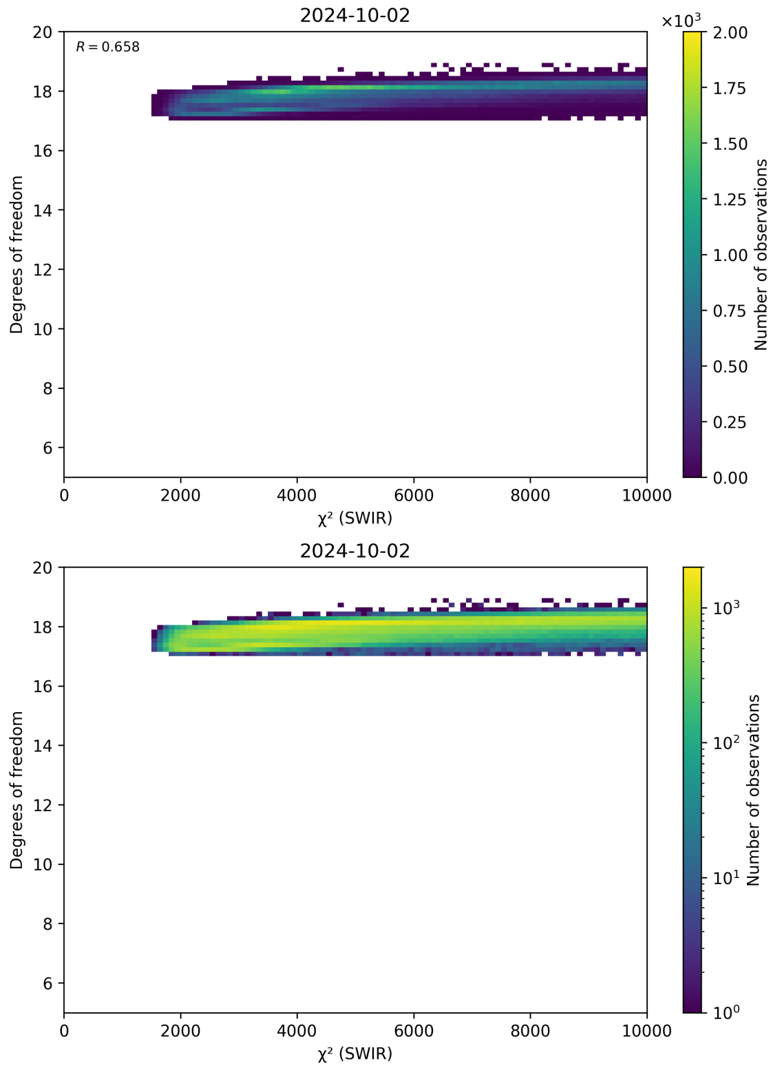
Figure 48: Scatter density plot of “ \chi^2 (SWIR)” against “Degrees of freedom” for 2024-10-01 to 2024-10-03.
