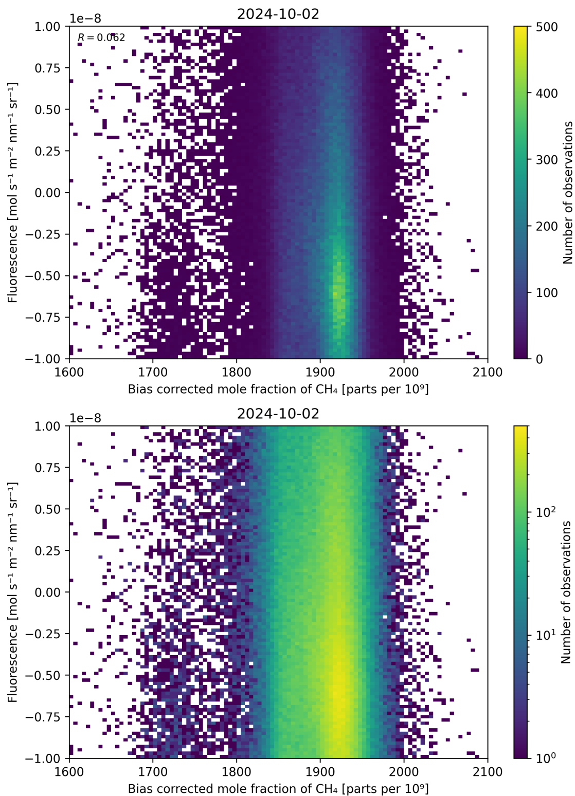
Figure 66: Scatter density plot of “Bias corrected mole fraction of CH 4 ” against “Fluorescence” for 2024-10-01 to 2024-10-03.
