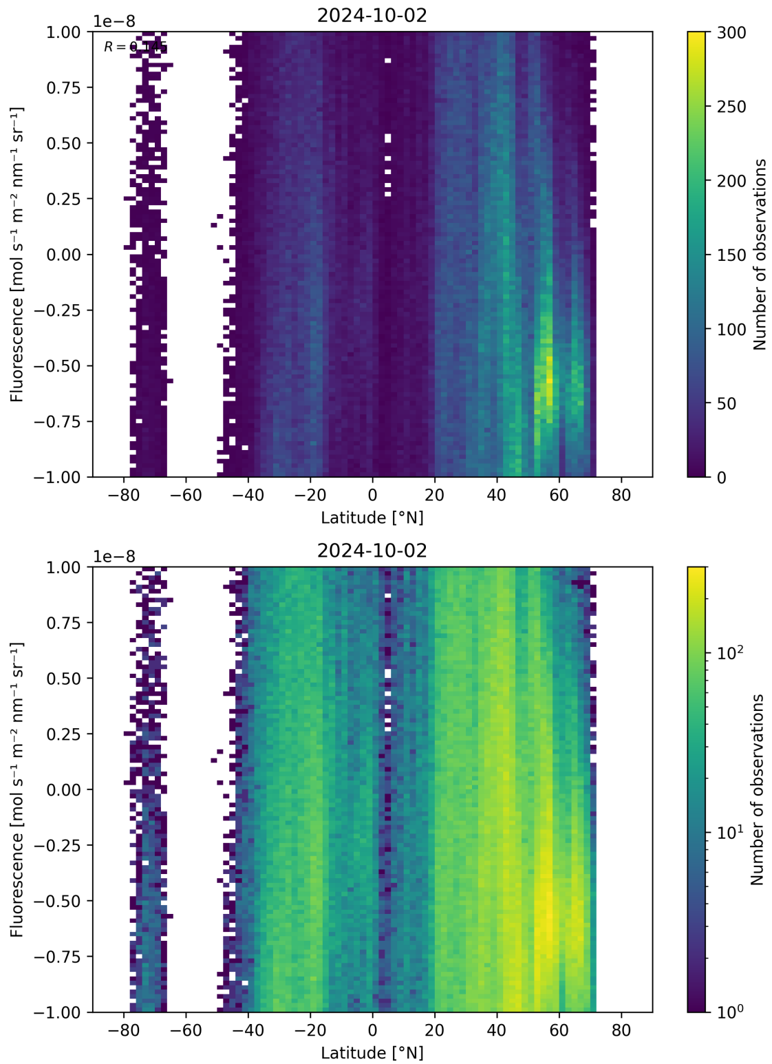
Figure 56: Scatter density plot of “Latitude” against “Fluorescence” for 2024-10-01 to 2024-10-03.
