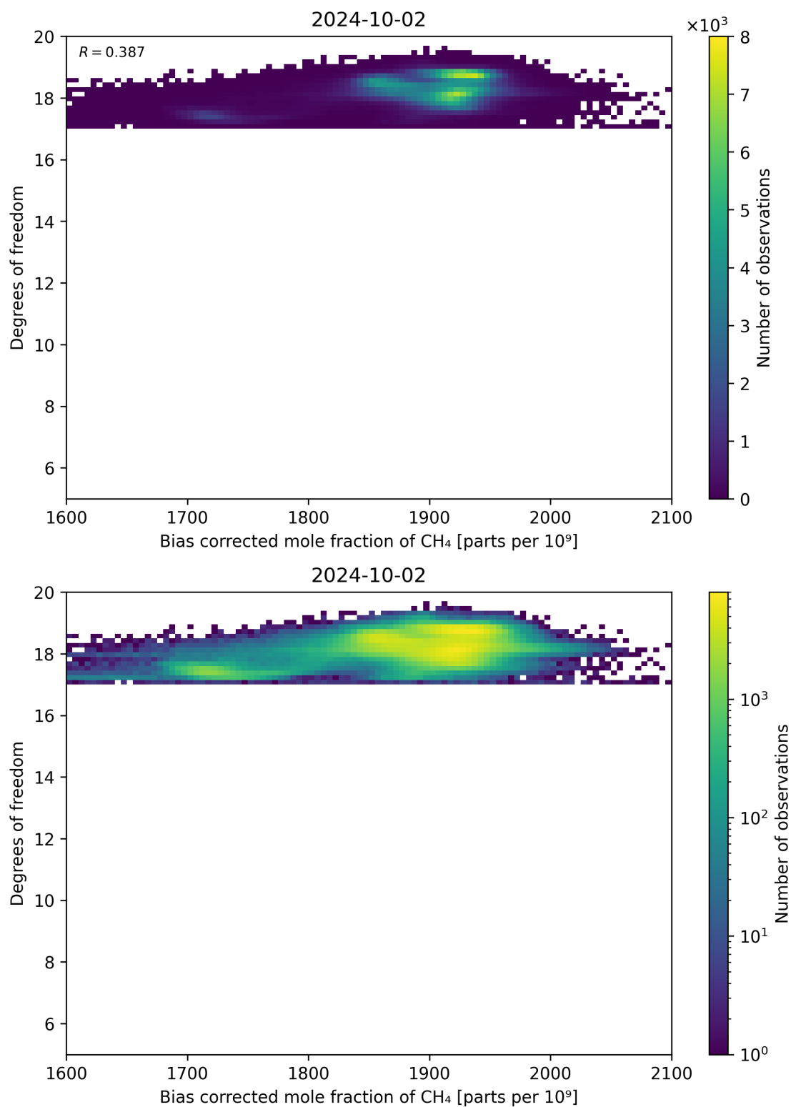
Figure 65: Scatter density plot of “Bias corrected mole fraction of CH 4 ” against “Degrees of freedom” for 2024-10-01 to 2024-10-03.
