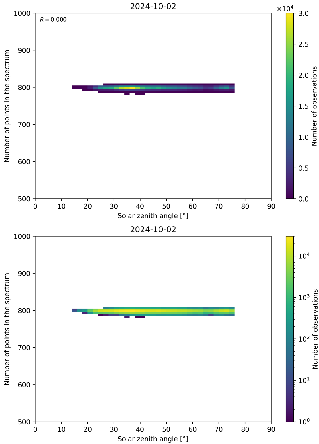
Figure 103: Scatter density plot of “Solar zenith angle” against “Number of points in the spectrum” for 2024-10-01 to 2024-10-03.
