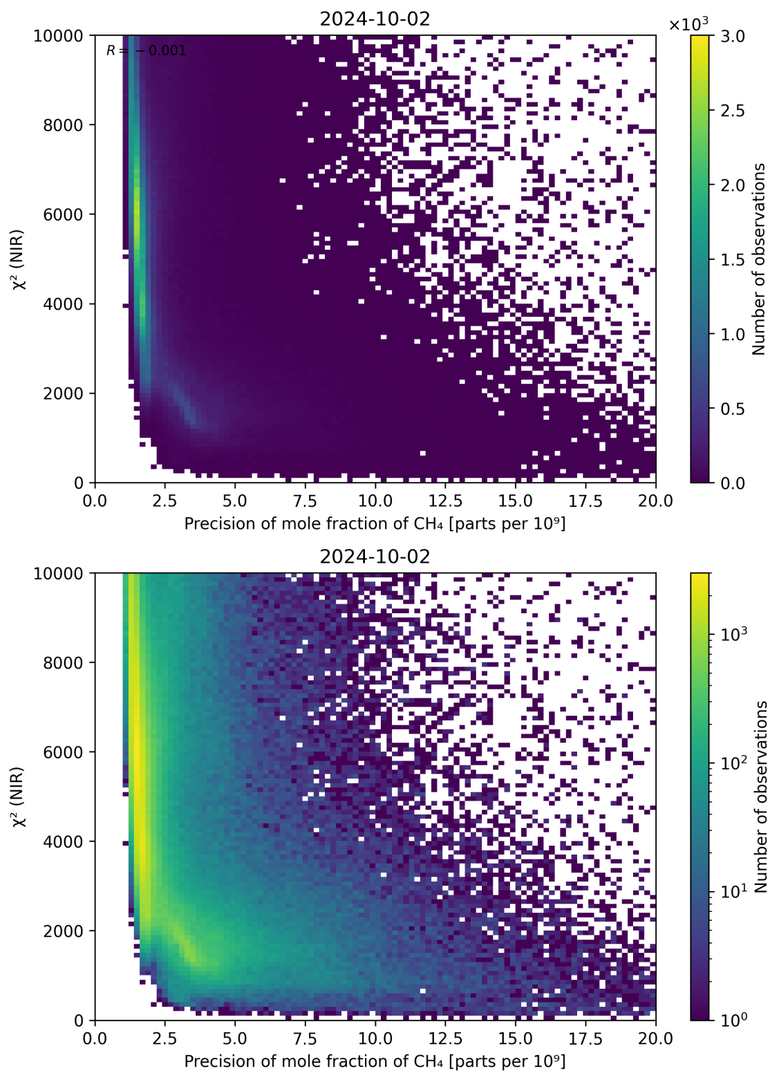
Figure 78: Scatter density plot of “Precision of mole fraction of \text{CH}_4 ” against “ \chi^2 (NIR)” for 2024-10-01 to 2024-10-03.
