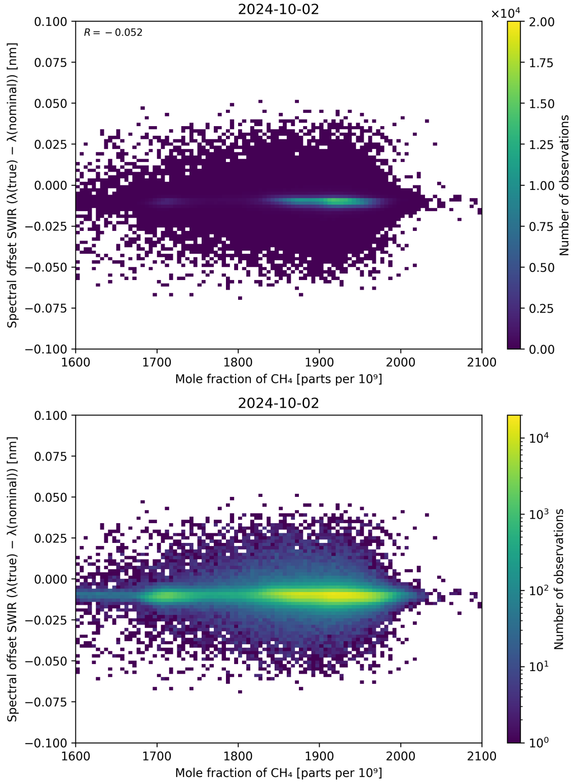
Figure 86: Scatter density plot of “Mole fraction of CH 4 ” against “Spectral offset SWIR ( \lambda_{\text{true}} - \lambda_{\text{nominal}} )” for 2024-10-01 to 2024-10-03.
