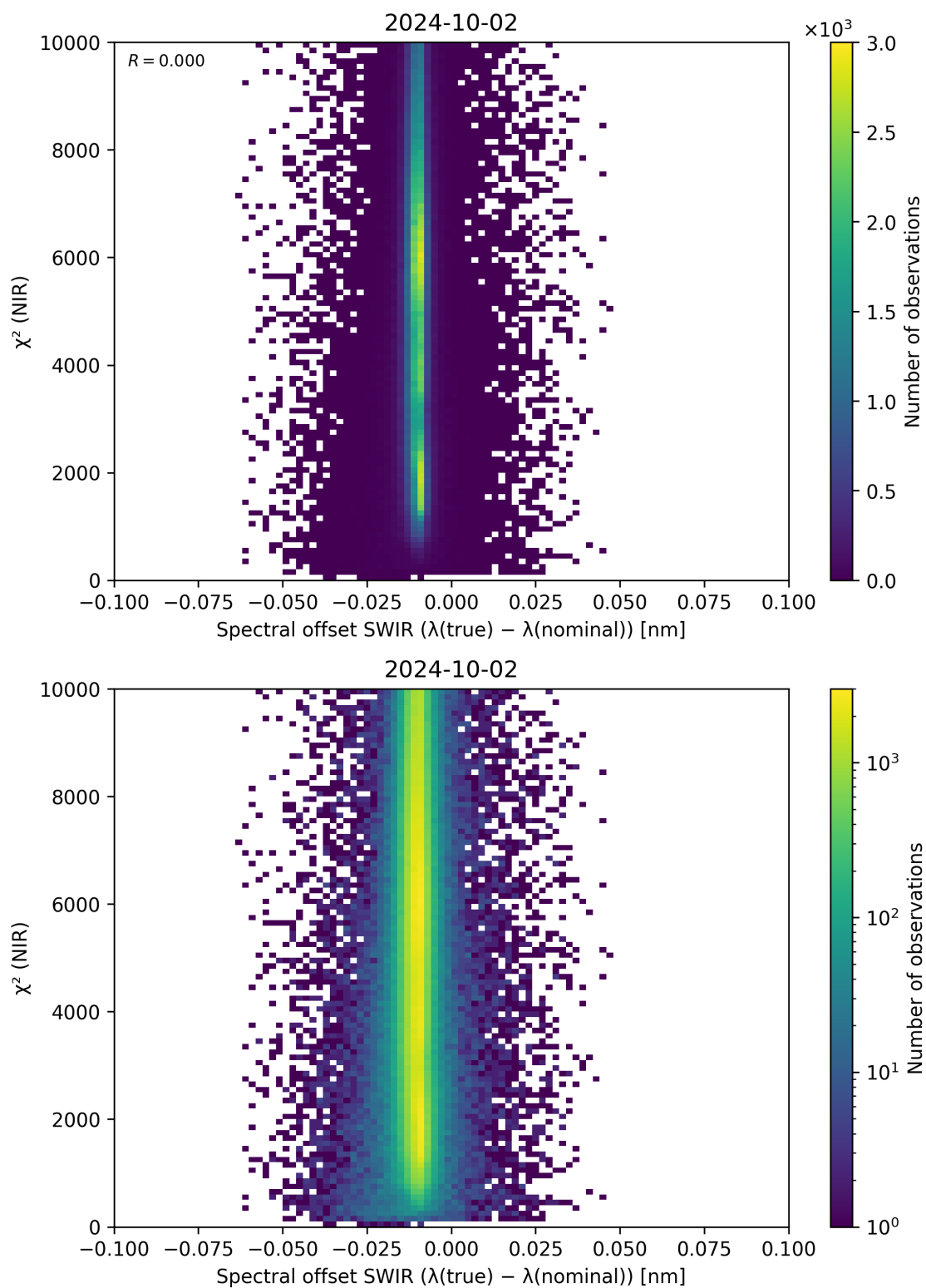
Figure 117: Scatter density plot of “Spectral offset SWIR ( \lambda_{\text{true}} - \lambda_{\text{nominal}} )” against “ \chi^2 (NIR)” for 2024-10-01 to 2024-10-03.
