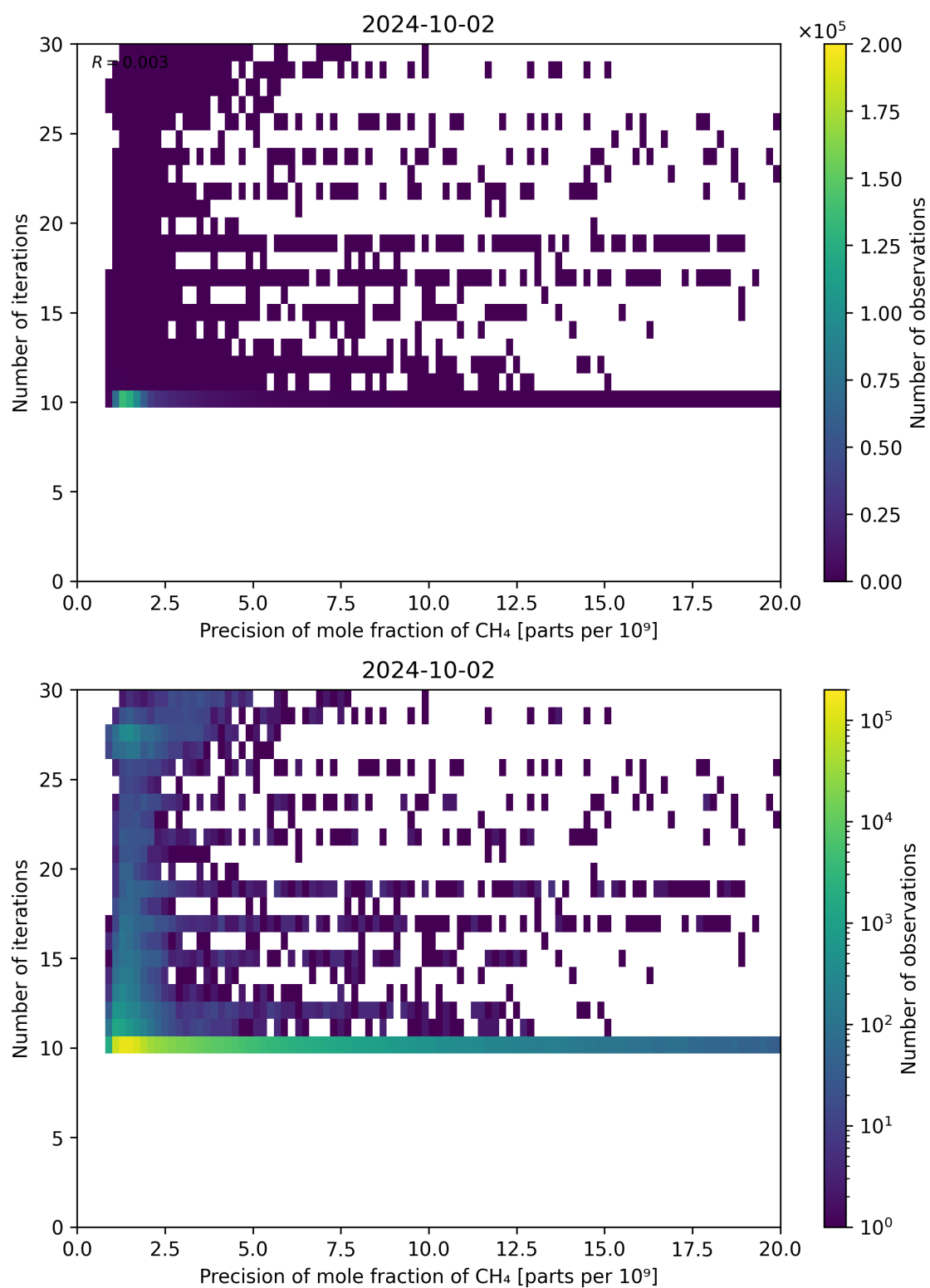
Figure 83: Scatter density plot of “Precision of mole fraction of CH 4 ” against “Number of iterations” for 2024-10-01 to 2024-10-03.
