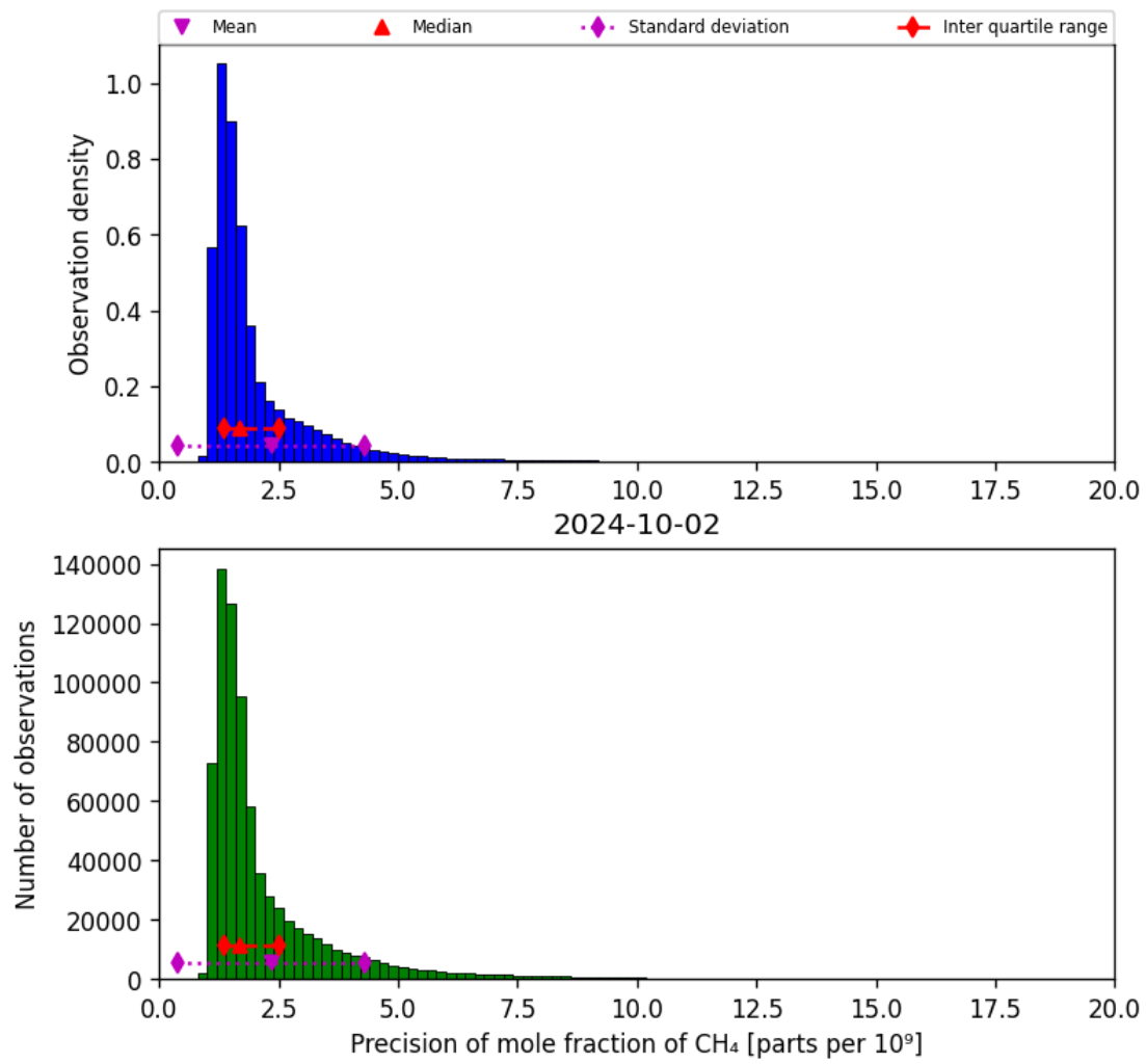
Figure 24: Histogram of “Precision of mole fraction of CH 4 ” for 2024-10-01 to 2024-10-03
