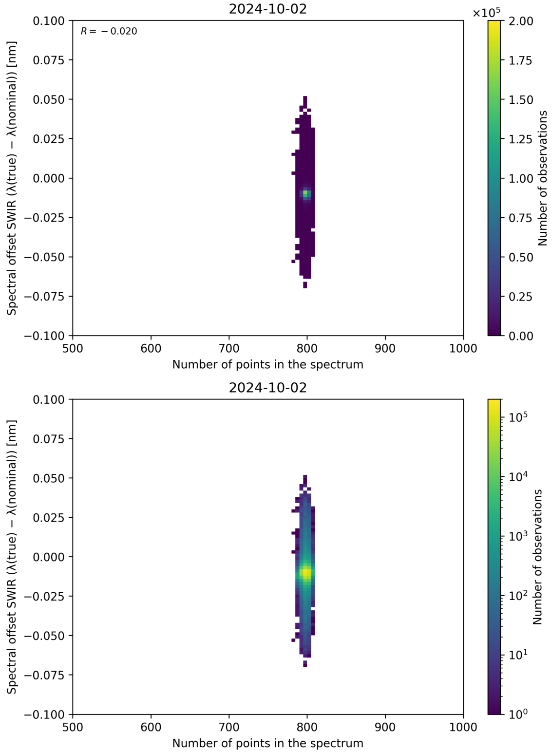
Figure 93: Scatter density plot of “Number of points in the spectrum” against “Spectral offset SWIR ( \lambda_{\text{true}} - \lambda_{\text{nominal}} )” for 2024-10-01 to 2024-10-03.
