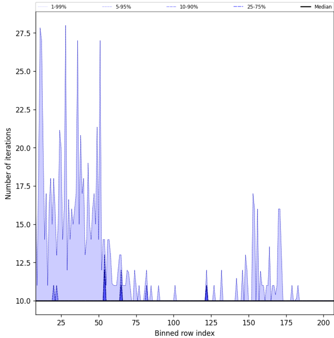
Figure 42: Along track statistics of “Number of iterations” for 2024-10-01 to 2024-10-03
