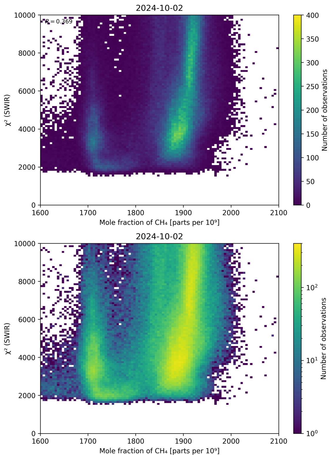
Figure 71: Scatter density plot of “Mole fraction of \text{CH}_4 ” against “ \chi^2 (SWIR)” for 2024-10-01 to 2024-10-03.
