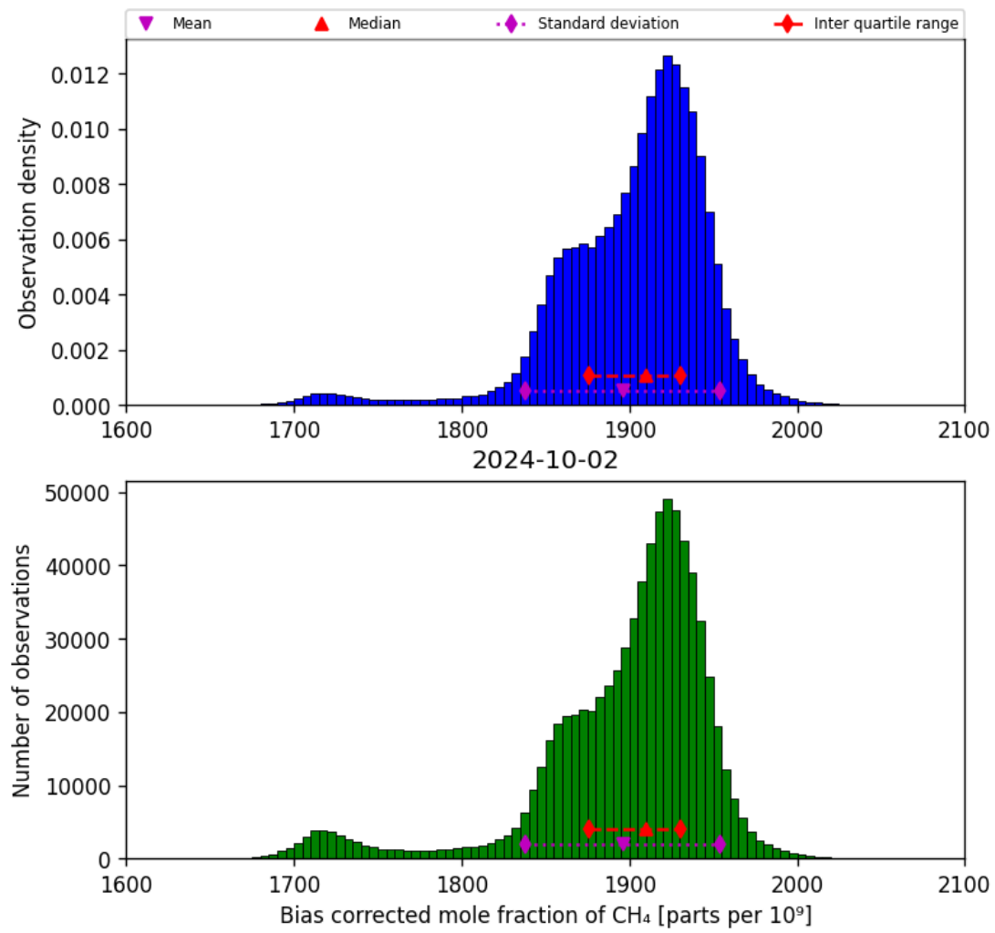
Figure 25: Histogram of “Bias corrected mole fraction of CH 4 ” for 2024-10-01 to 2024-10-03
