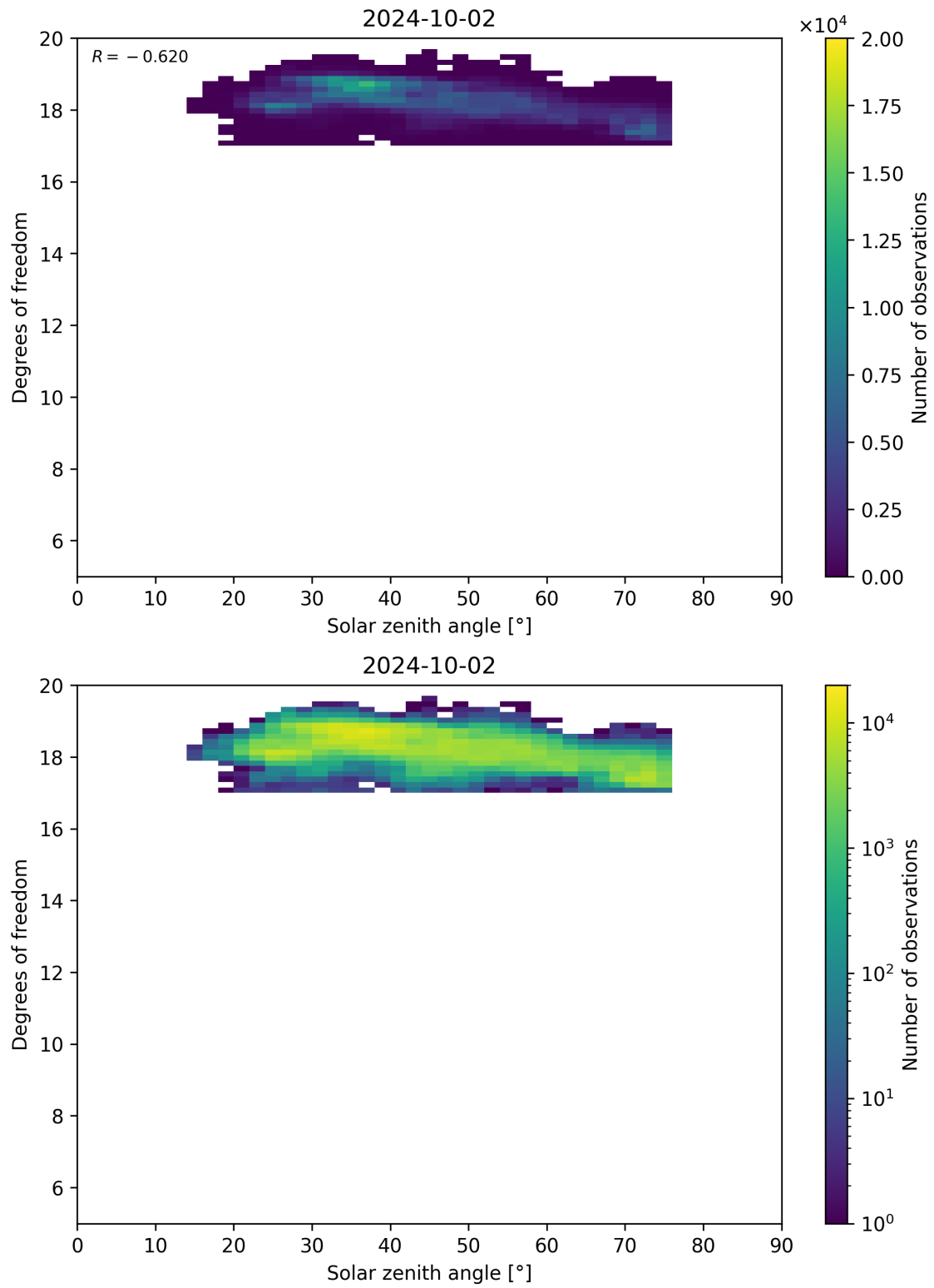
Figure 96: Scatter density plot of “Solar zenith angle” against “Degrees of freedom” for 2024-10-01 to 2024-10-03.
