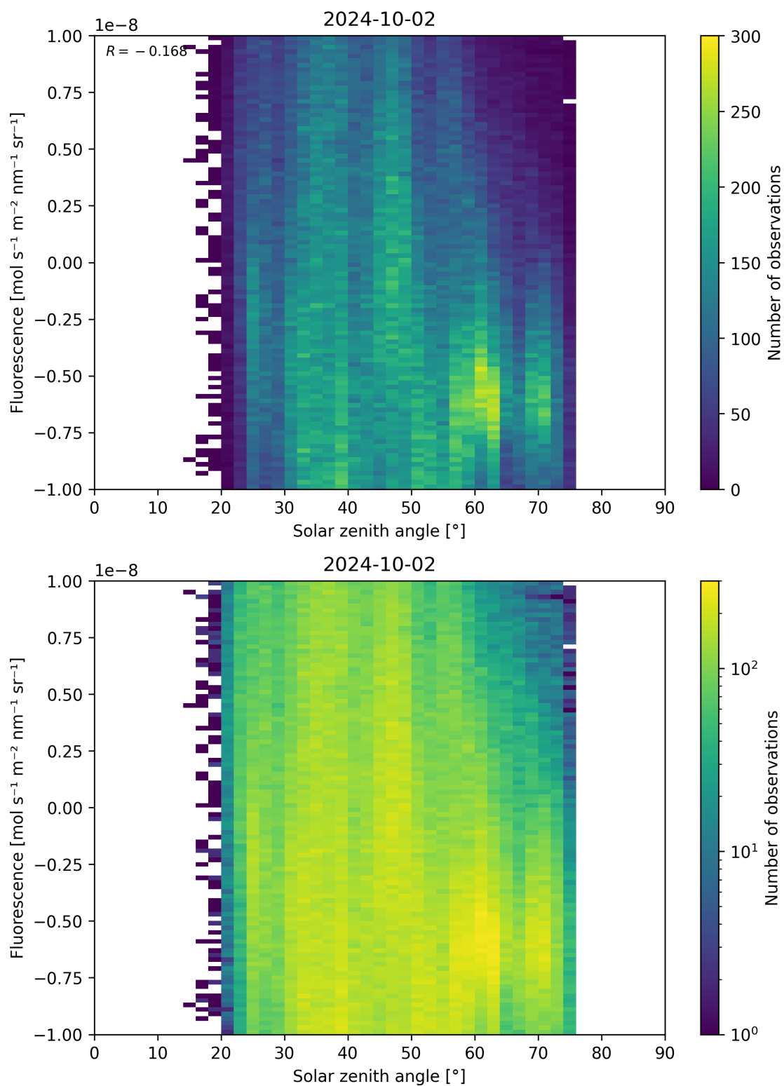
Figure 97: Scatter density plot of “Solar zenith angle” against “Fluorescence” for 2024-10-01 to 2024-10-03.
