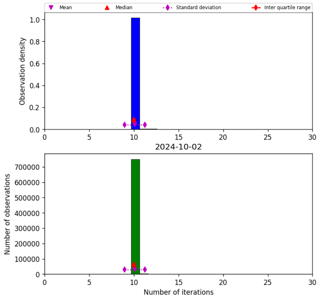
Figure 31: Histogram of “Number of iterations” for 2024-10-01 to 2024-10-03
