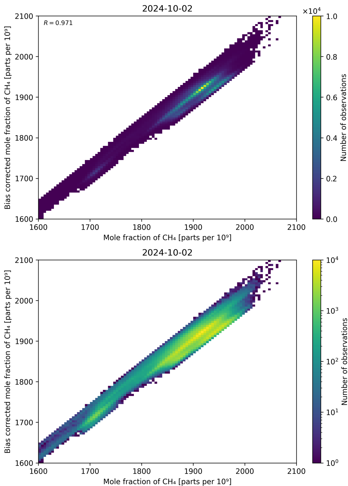
Figure 74: Scatter density plot of “Mole fraction of CH 4 ” against “Bias corrected mole fraction of CH 4 ” for 2024-10-01 to 2024-10-03.
