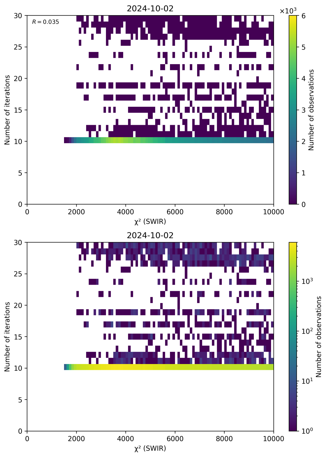
Figure 50: Scatter density plot of “ \chi^2 (SWIR)” against “Number of iterations” for 2024-10-01 to 2024-10-03.
