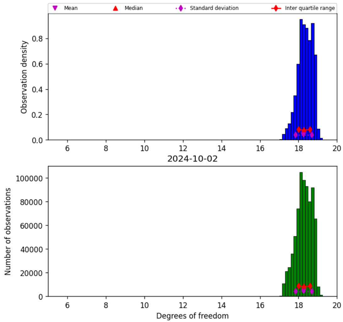
Figure 30: Histogram of “Degrees of freedom” for 2024-10-01 to 2024-10-03
