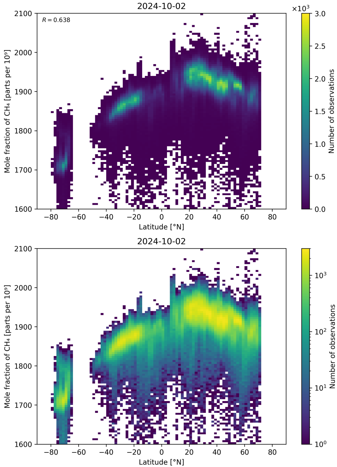
Figure 57: Scatter density plot of “Latitude” against “Mole fraction of \text{CH}_4 ” for 2024-10-01 to 2024-10-03.
