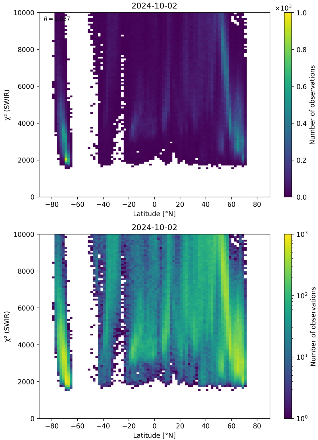
Figure 54: Scatter density plot of “Latitude” against “ \chi^2 (SWIR)” for 2024-10-01 to 2024-10-03.
