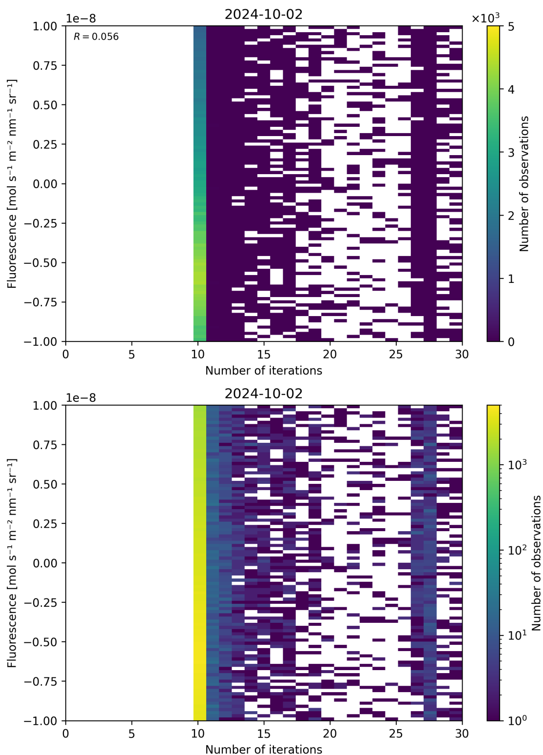
Figure 87: Scatter density plot of “Number of iterations” against “Fluorescence” for 2024-10-01 to 2024-10-03.
