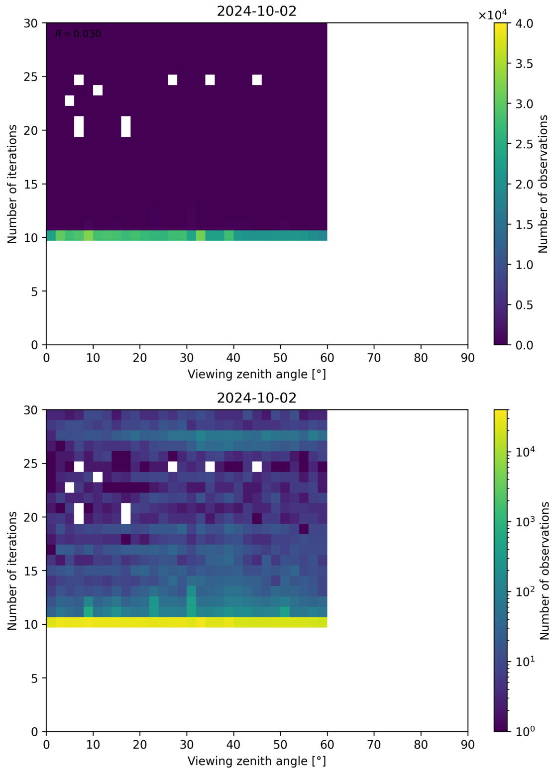
Figure 113: Scatter density plot of “Viewing zenith angle” against “Number of iterations” for 2024-10-01 to 2024-10-03.
