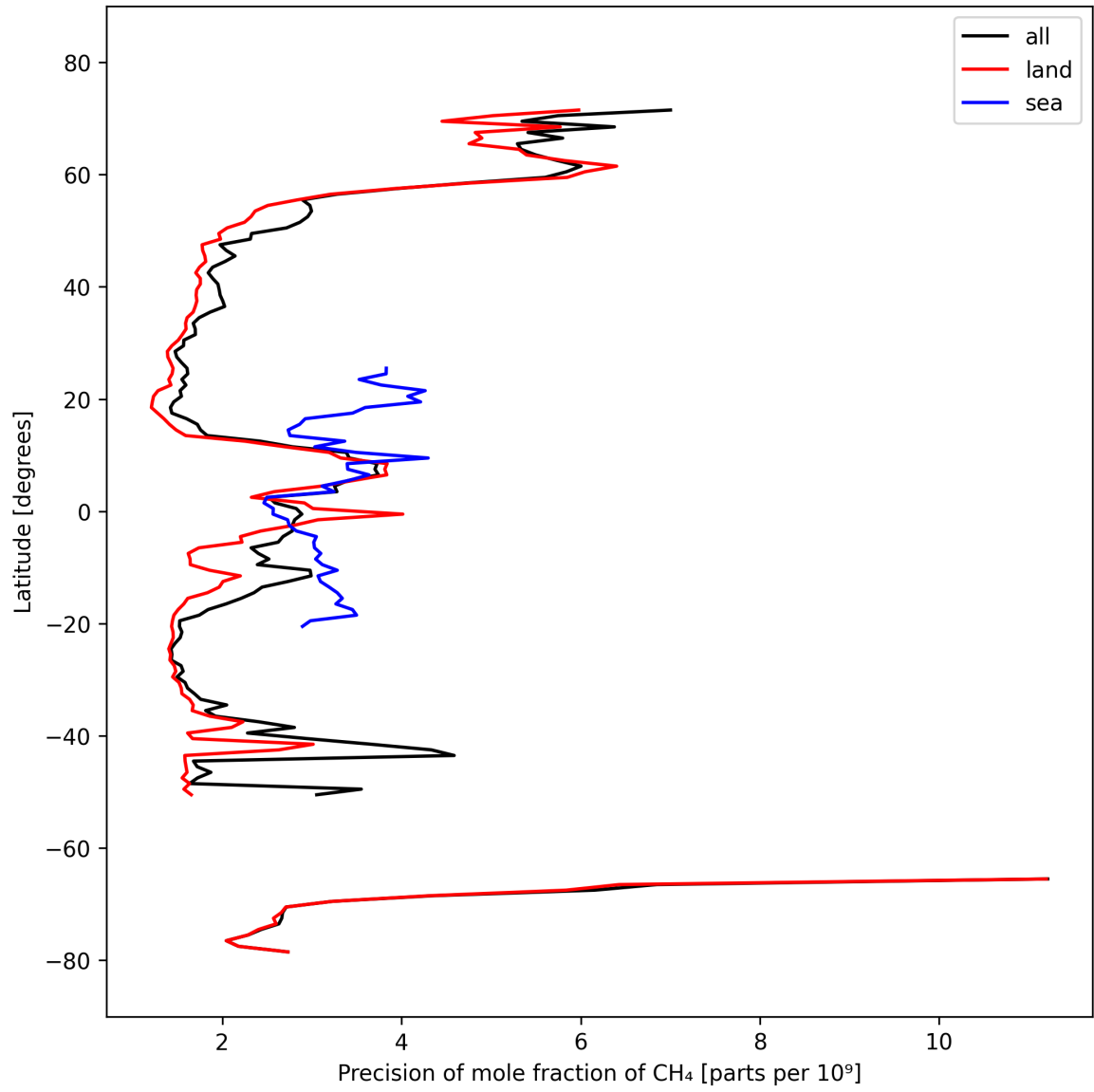
Figure 13: Zonal average of “Precision of mole fraction of CH 4 ” for 2024-10-01 to 2024-10-03.
