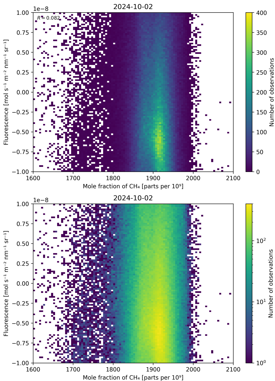
Figure 73: Scatter density plot of “Mole fraction of \text{CH}_4 ” against “Fluorescence” for 2024-10-01 to 2024-10-03.
