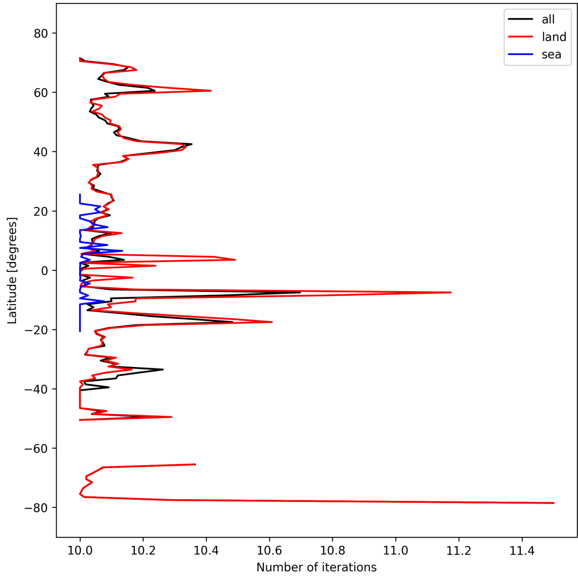
Figure 20: Zonal average of “Number of iterations” for 2024-10-01 to 2024-10-03.
