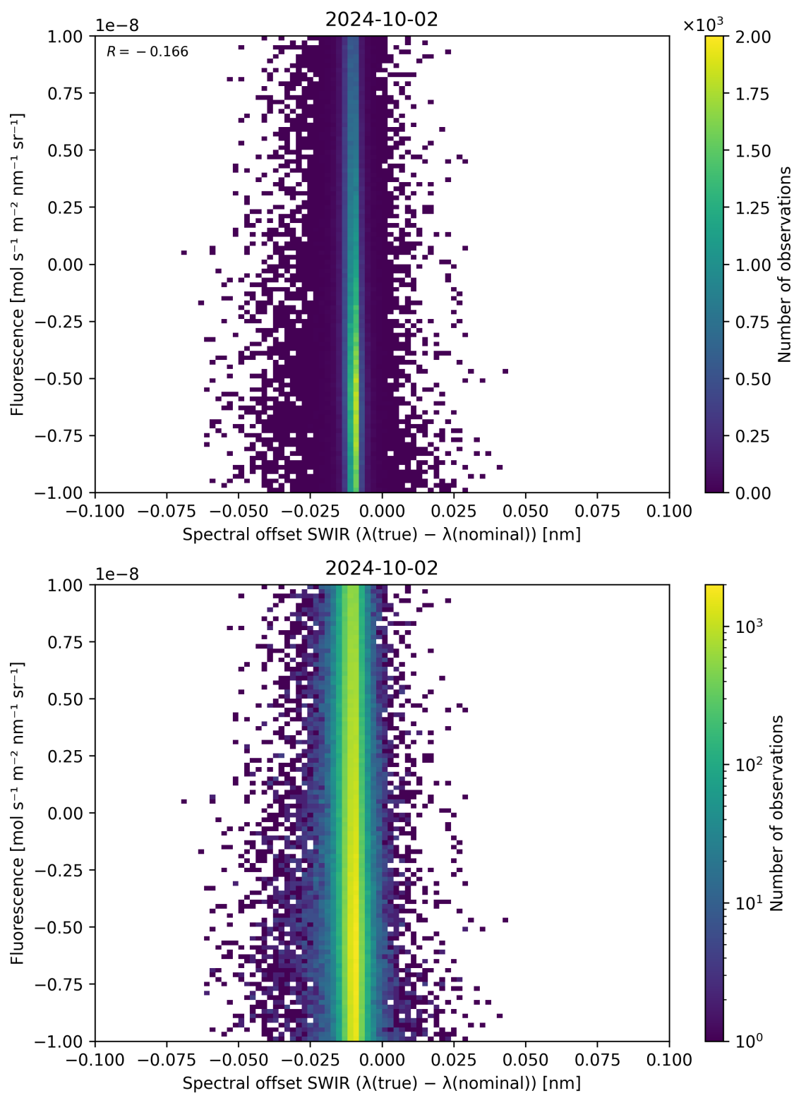
Figure 120: Scatter density plot of “Spectral offset SWIR ( \lambda_{\text{true}} - \lambda_{\text{nominal}} )” against “Fluorescence” for 2024-10-01 to 2024-10-03.
