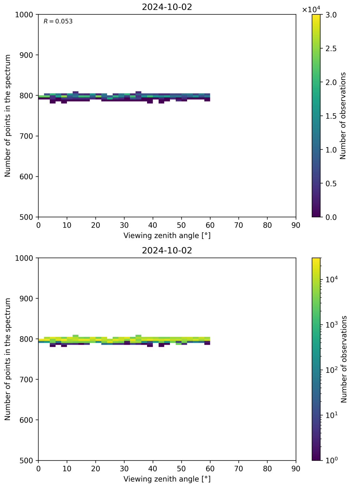
Figure 114: Scatter density plot of “Viewing zenith angle” against “Number of points in the spectrum” for 2024-10-01 to 2024-10-03.
