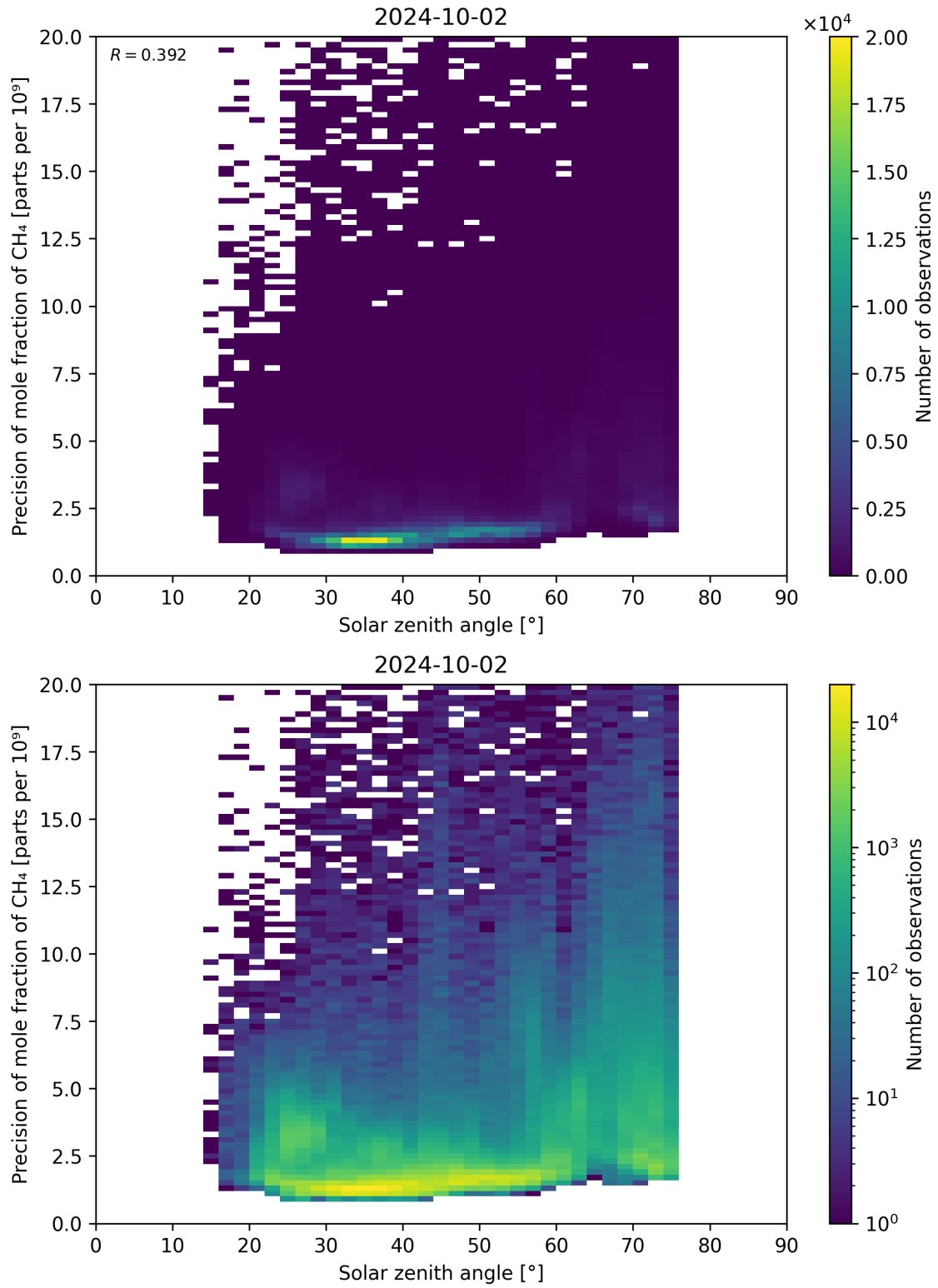
Figure 101: Scatter density plot of “Solar zenith angle” against “Precision of mole fraction of CH 4 ” for 2024-10-01 to 2024-10-03.
