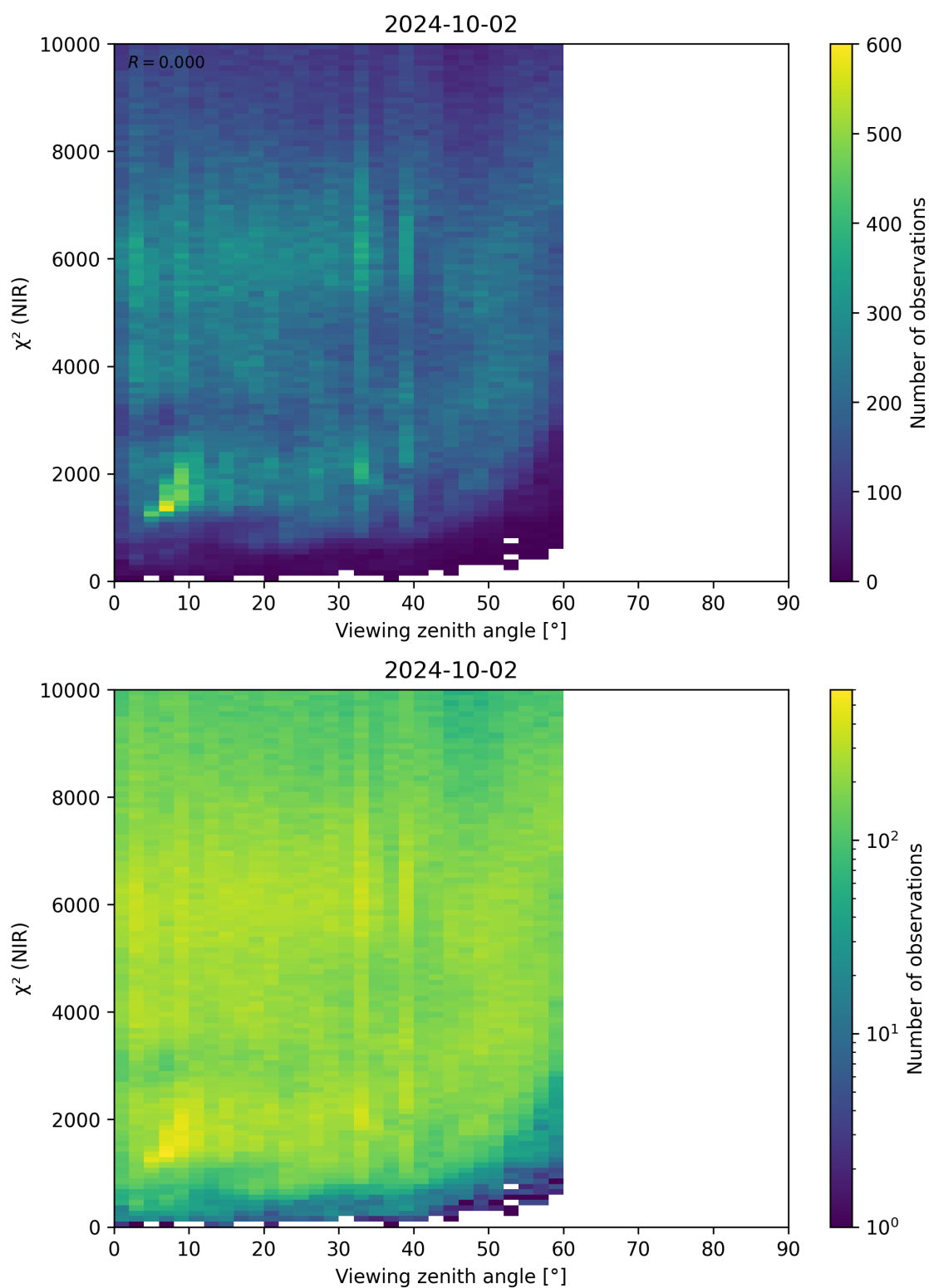
Figure 105: Scatter density plot of “Viewing zenith angle” against “ \chi^2 (NIR)” for 2024-10-01 to 2024-10-03.
