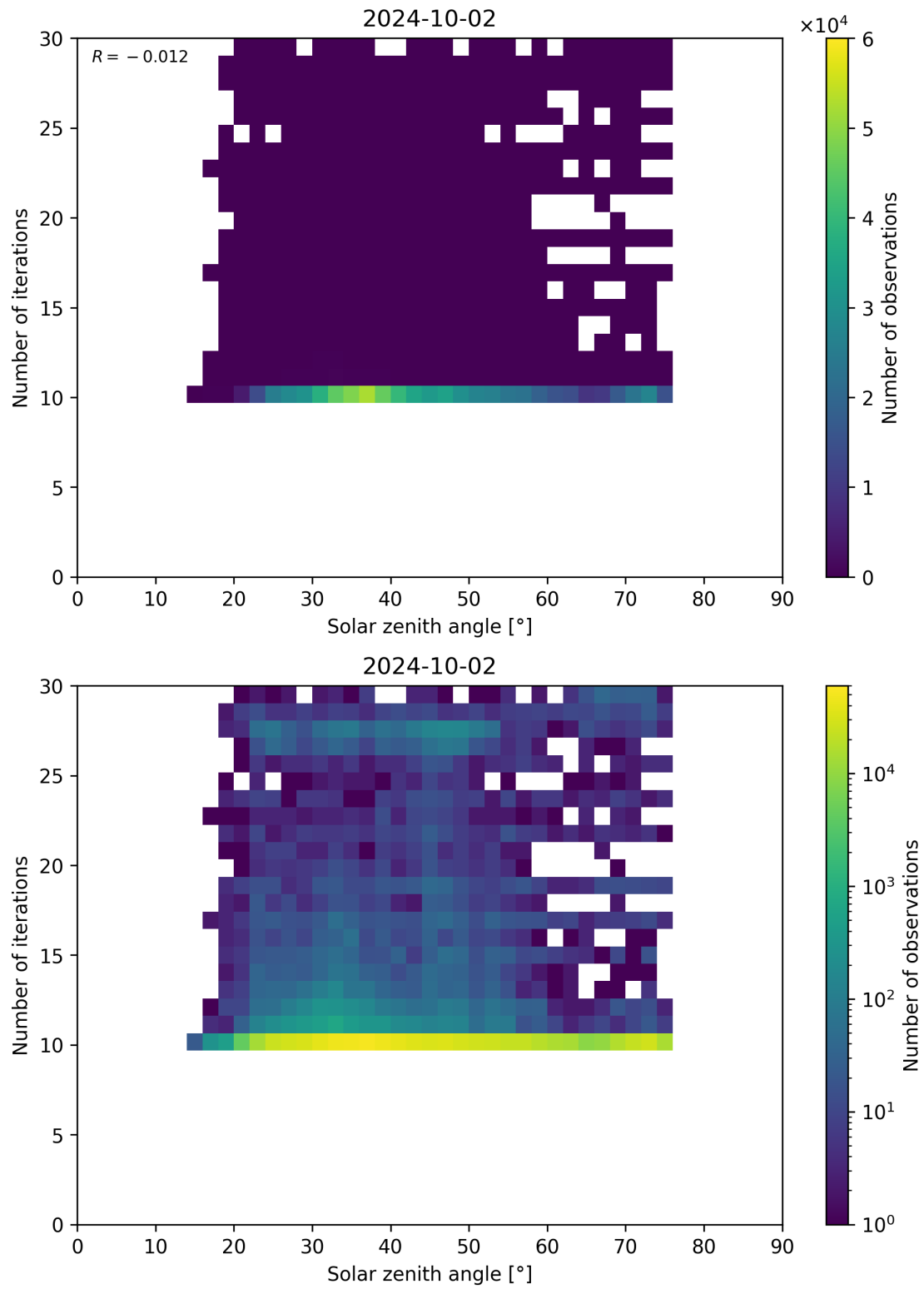
Figure 102: Scatter density plot of “Solar zenith angle” against “Number of iterations” for 2024-10-01 to 2024-10-03.
