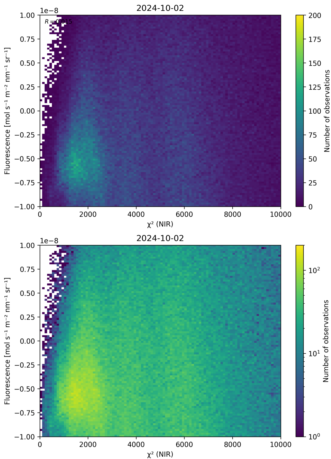
Figure 45: Scatter density plot of “ \chi^2 (NIR)” against “Fluorescence” for 2024-10-01 to 2024-10-03.
