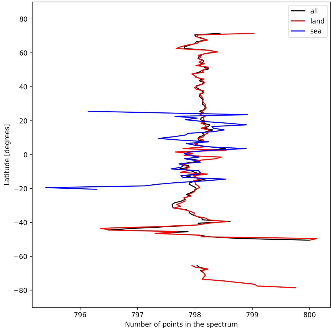
Figure 15: Zonal average of “Number of points in the spectrum” for 2024-10-01 to 2024-10-03.
