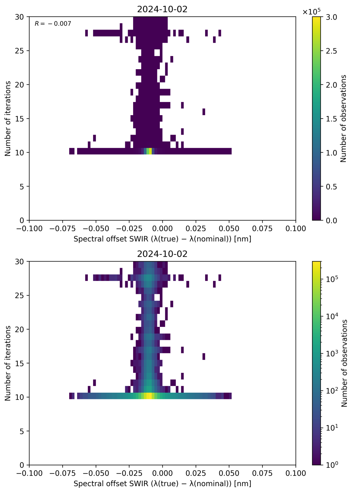
Figure 121: Scatter density plot of “Spectral offset SWIR ( \lambda_{\text{true}} - \lambda_{\text{nominal}} )” against “Number of iterations” for 2024-10-01 to 2024-10-03.
