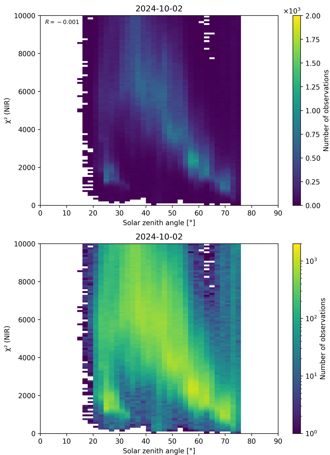
Figure 94: Scatter density plot of “Solar zenith angle” against “ \chi^2 (NIR)” for 2024-10-01 to 2024-10-03.
