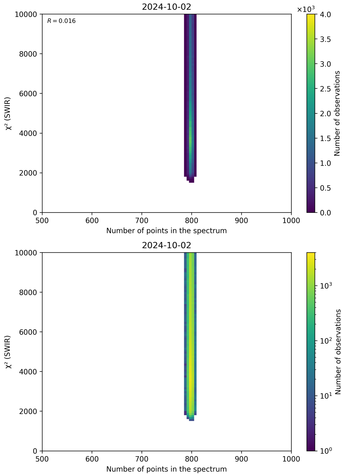
Figure 89: Scatter density plot of “Number of points in the spectrum” against “ \chi^2 (SWIR)” for 2024-10-01 to 2024-10-03.
