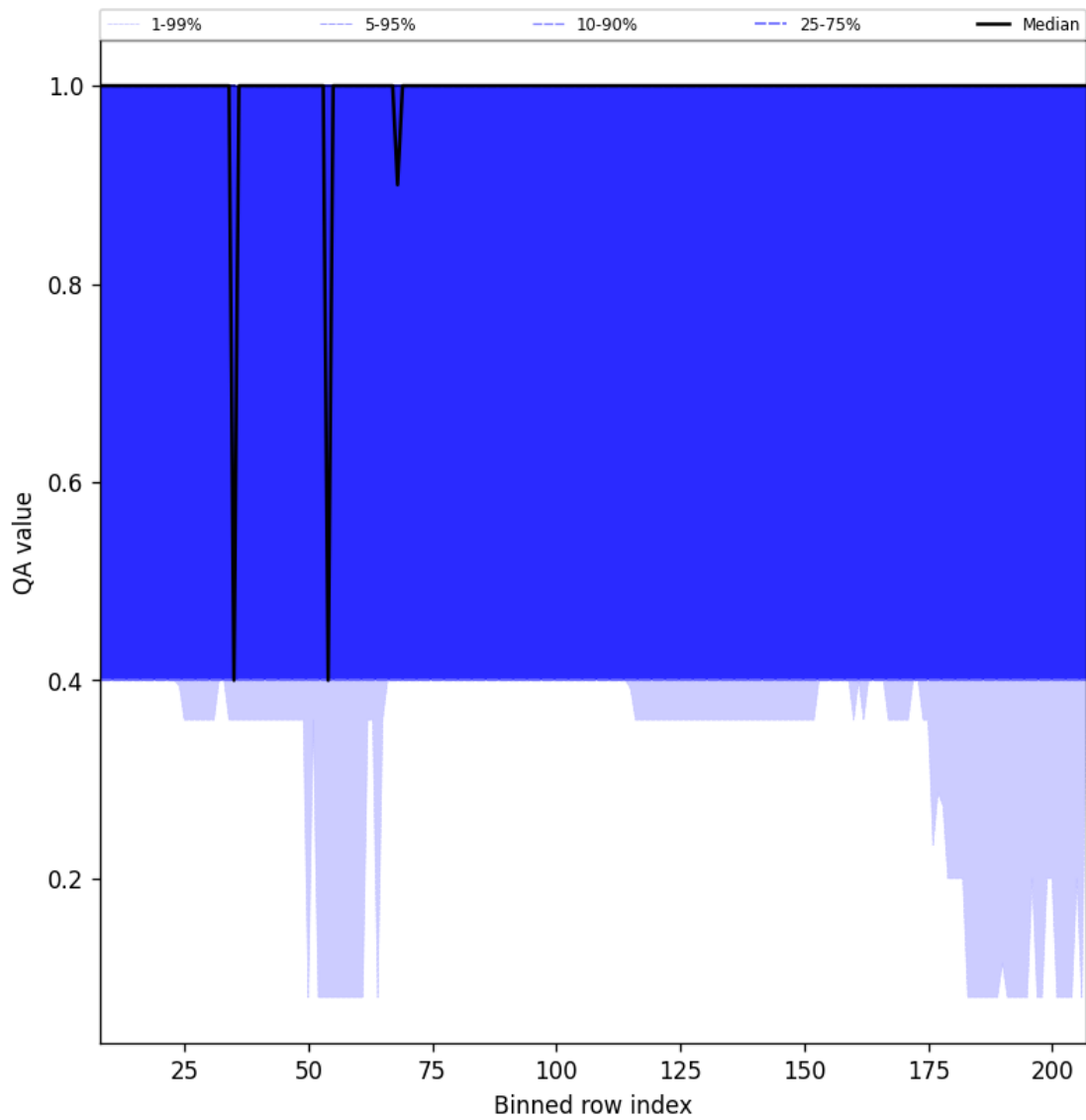
Figure 33: Along track statistics of “QA value” for 2024-10-01 to 2024-10-03
