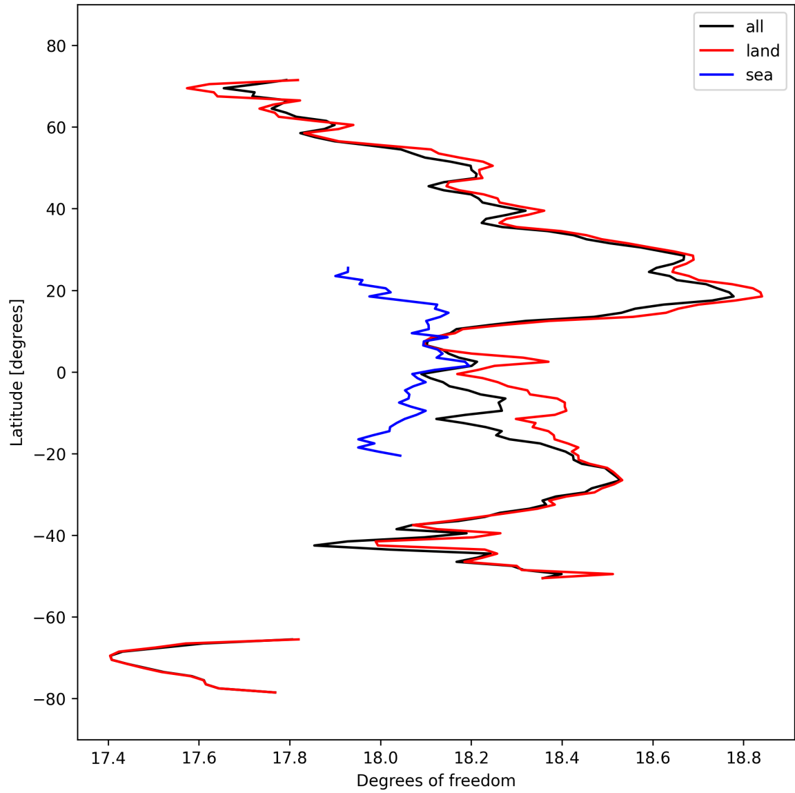
Figure 19: Zonal average of “Degrees of freedom” for 2024-10-01 to 2024-10-03.
