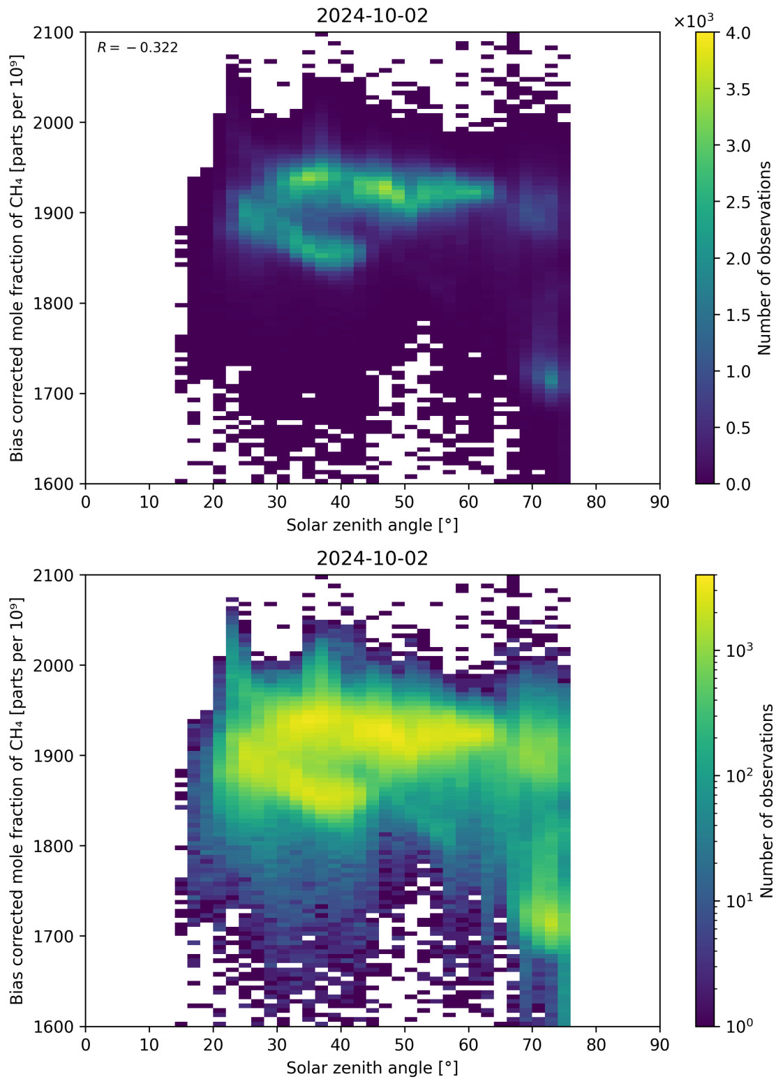
Figure 100: Scatter density plot of “Solar zenith angle” against “Bias corrected mole fraction of CH 4 ” for 2024-10-01 to 2024-10-03.
