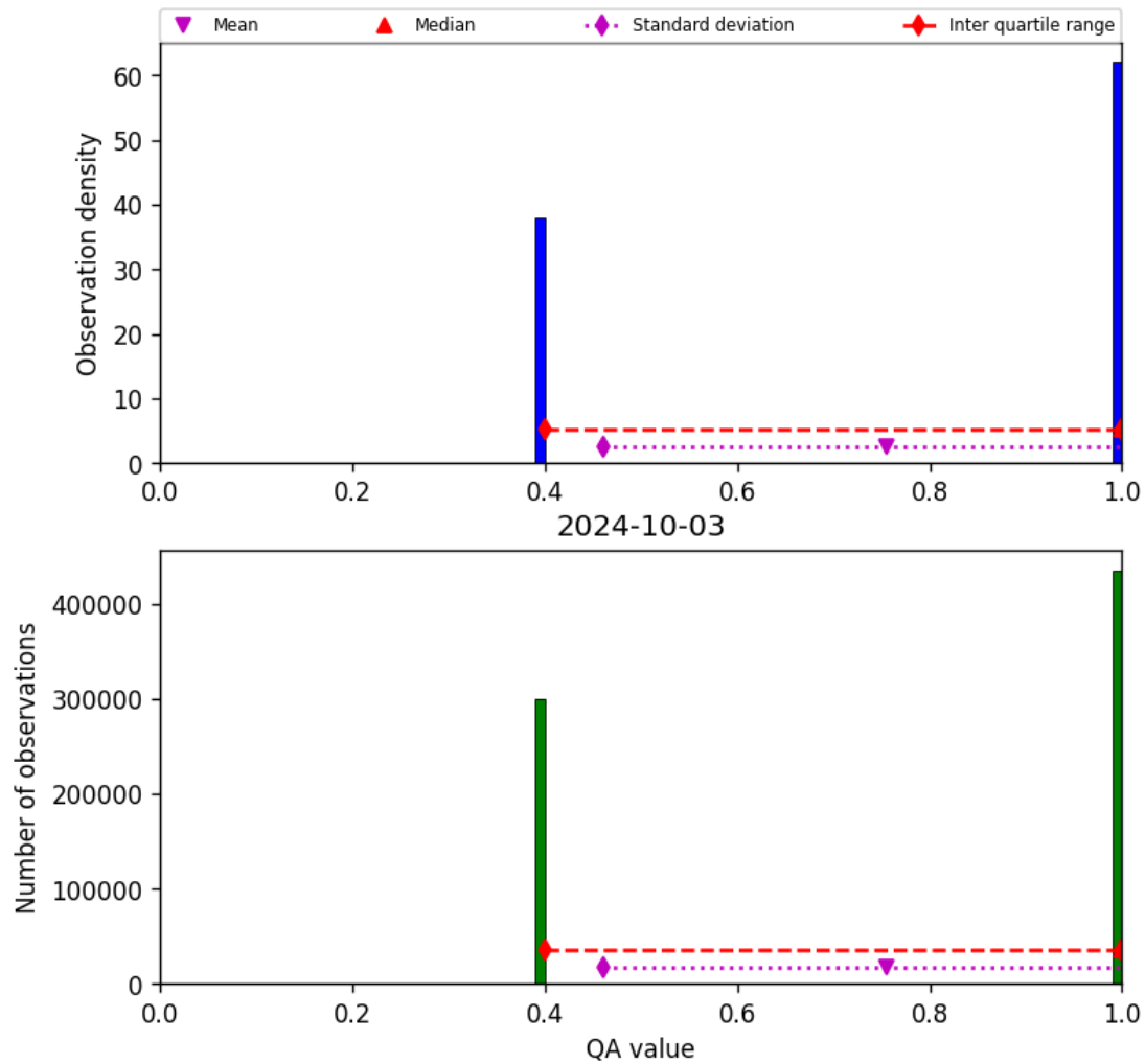
Figure 22: Histogram of “QA value” for 2024-10-03 to 2024-10-04
