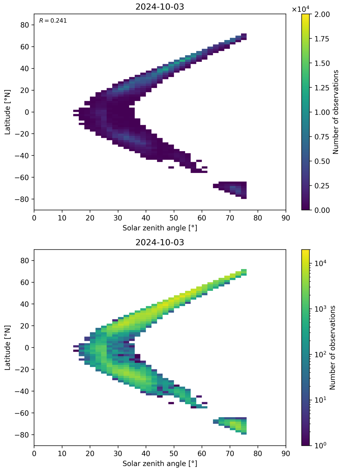
Figure 98: Scatter density plot of “Solar zenith angle” against “Latitude” for 2024-10-03 to 2024-10-04.
