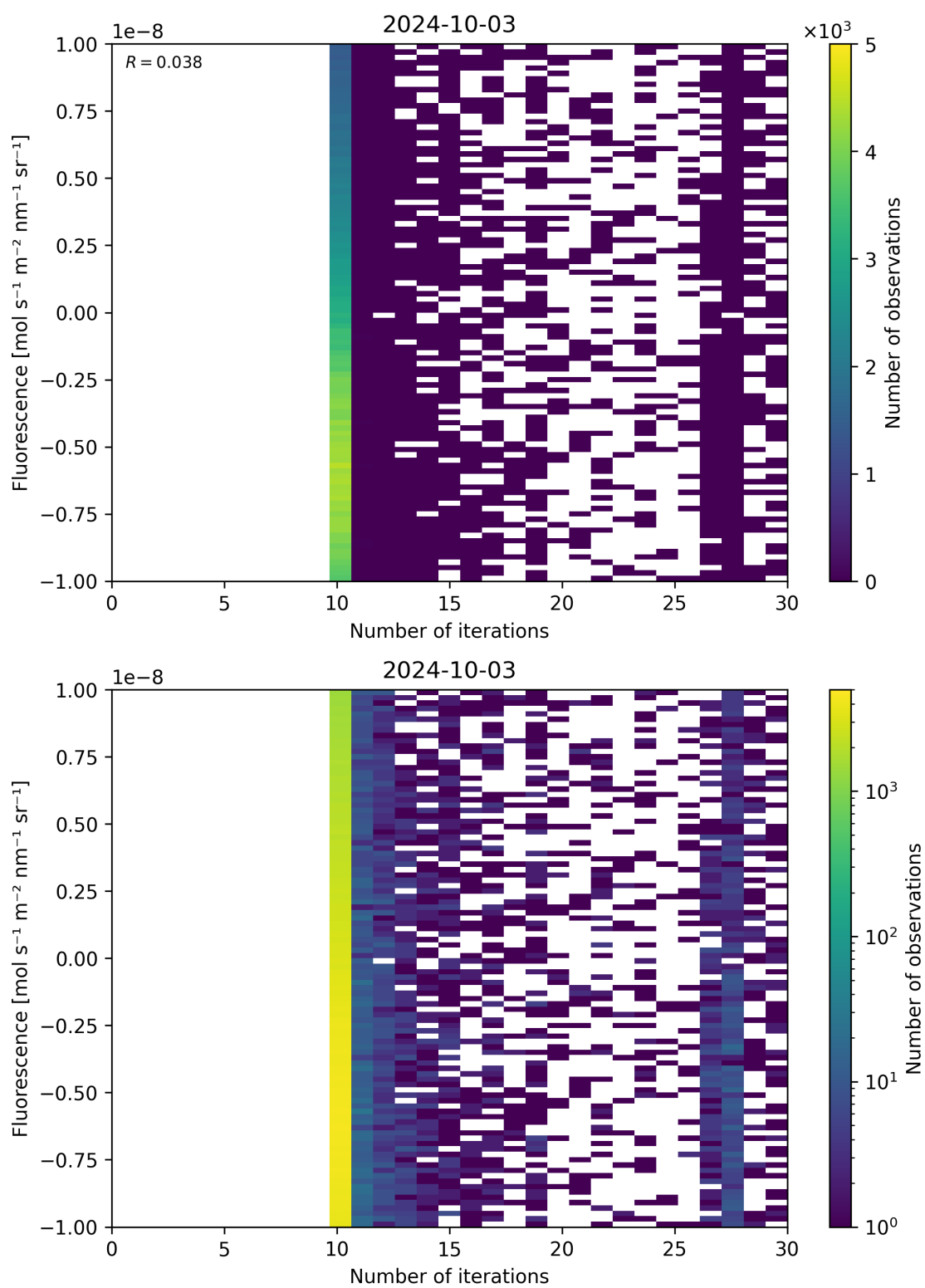
Figure 87: Scatter density plot of "Number of iterations" against "Fluorescence" for 2024-10-03 to 2024-10-04.
