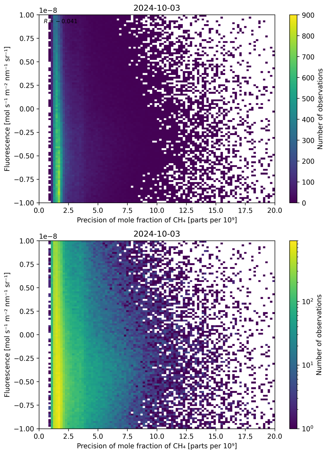
Figure 81: Scatter density plot of “Precision of mole fraction of \text{CH}_4 ” against “Fluorescence” for 2024-10-03 to 2024-10-04.
