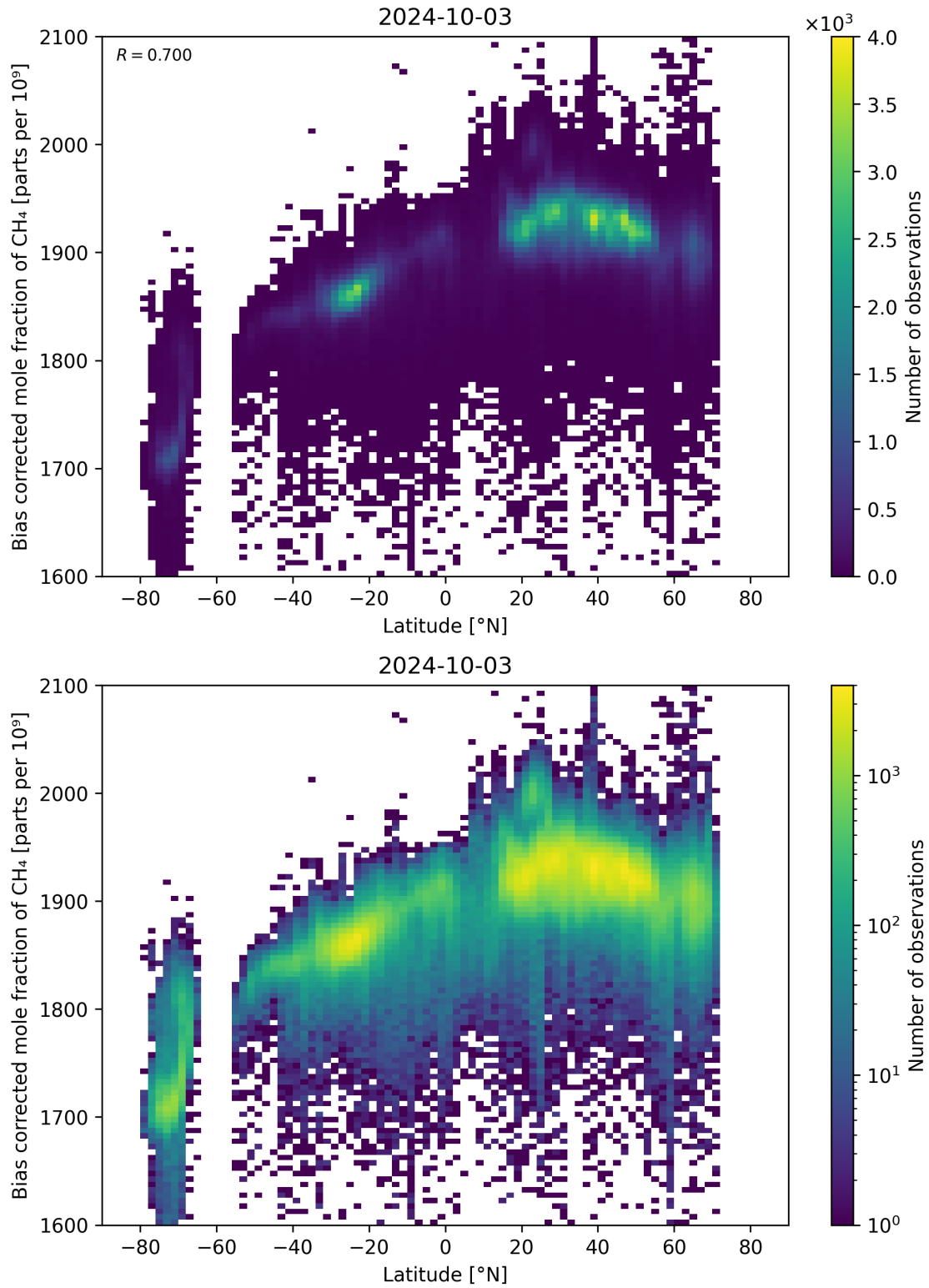
Figure 58: Scatter density plot of “Latitude” against “Bias corrected mole fraction of CH 4 ” for 2024-10-03 to 2024-10-04.
