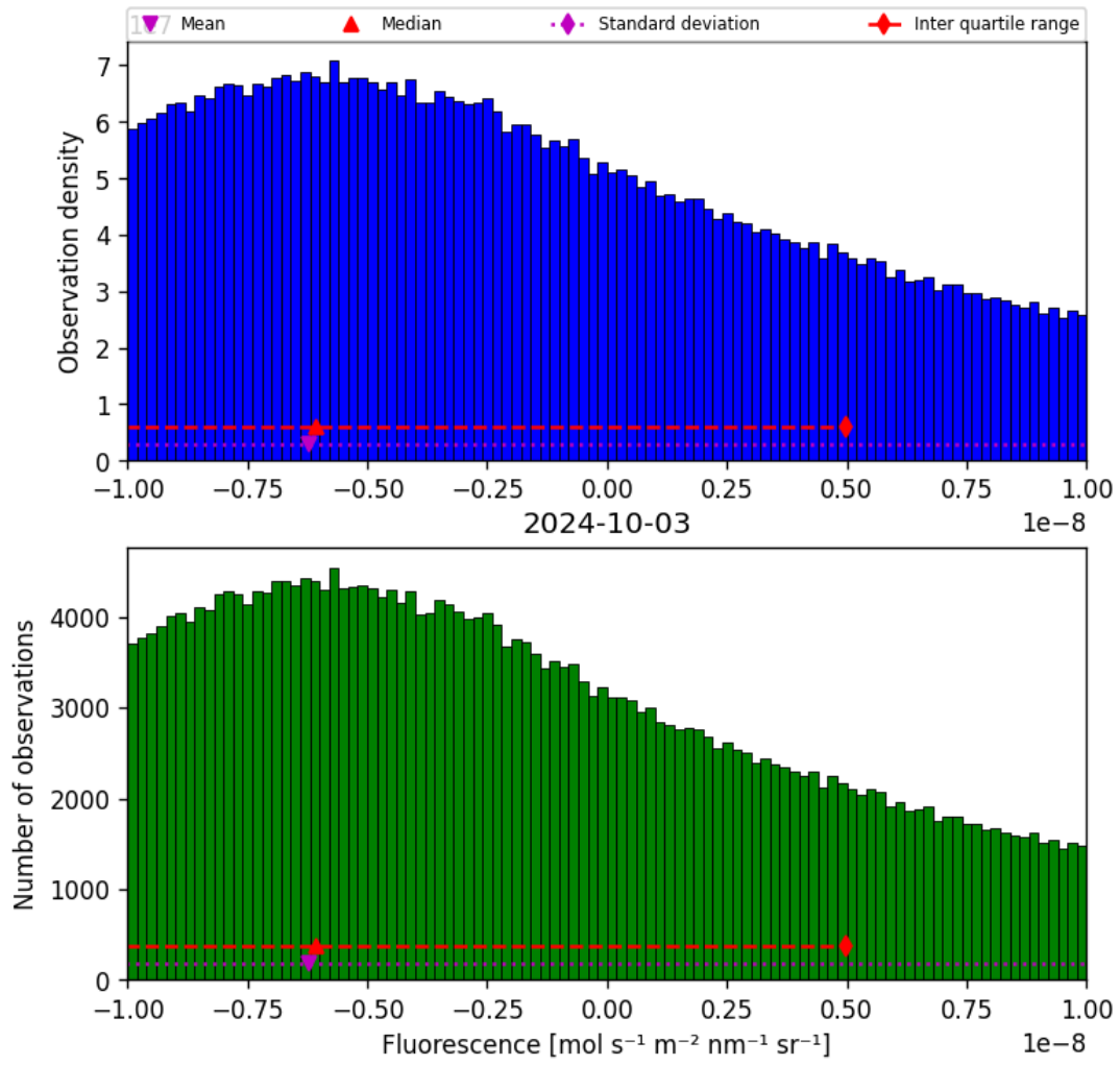
Figure 32: Histogram of “Fluorescence” for 2024-10-03 to 2024-10-04
