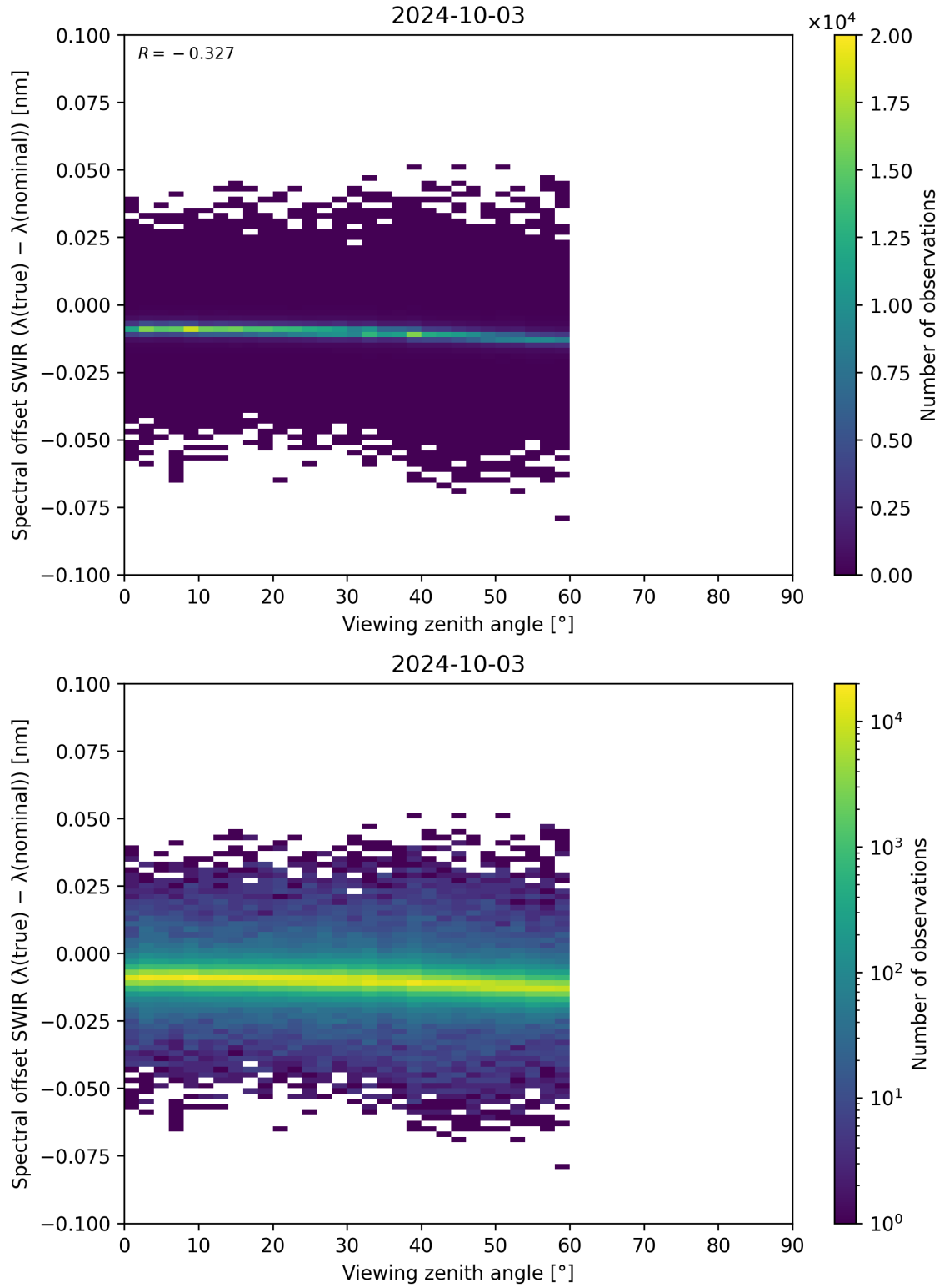
Figure 116: Scatter density plot of “Viewing zenith angle” against “Spectral offset SWIR ( \lambda_{\text{true}} - \lambda_{\text{nominal}} )” for 2024-10-03 to 2024-10-04.
