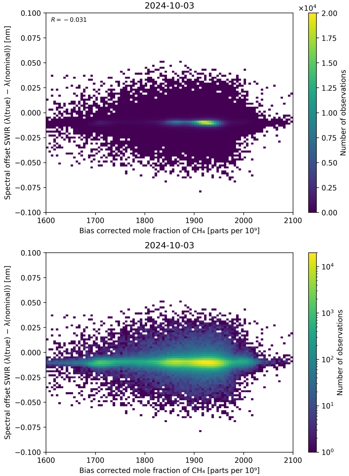
Figure 69: Scatter density plot of “Bias corrected mole fraction of \text{CH}_4 ” against “Spectral offset SWIR ( \lambda_{\text{true}} - \lambda_{\text{nominal}} )” for 2024-10-03 to 2024-10-04.
