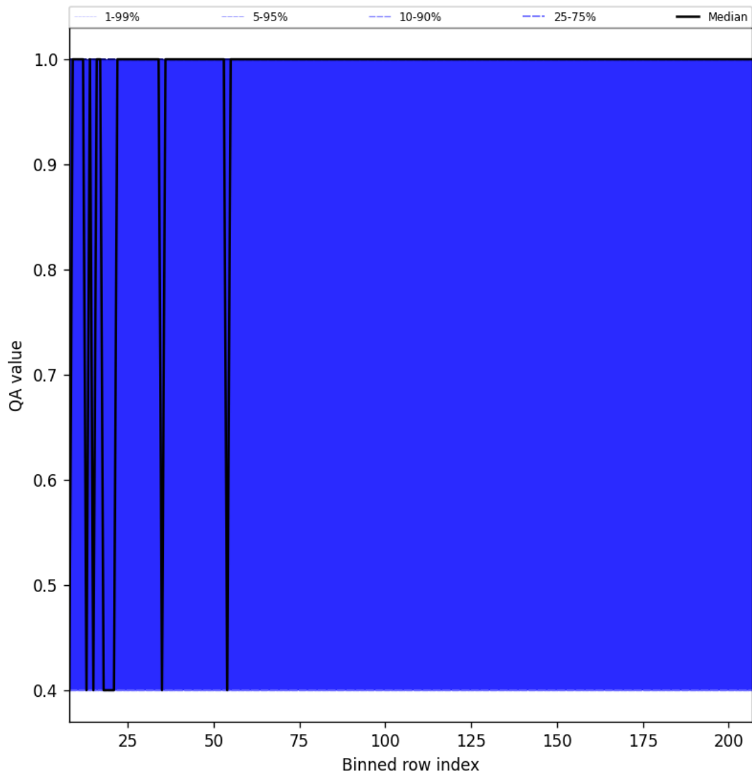
Figure 33: Along track statistics of “QA value” for 2024-10-03 to 2024-10-04
