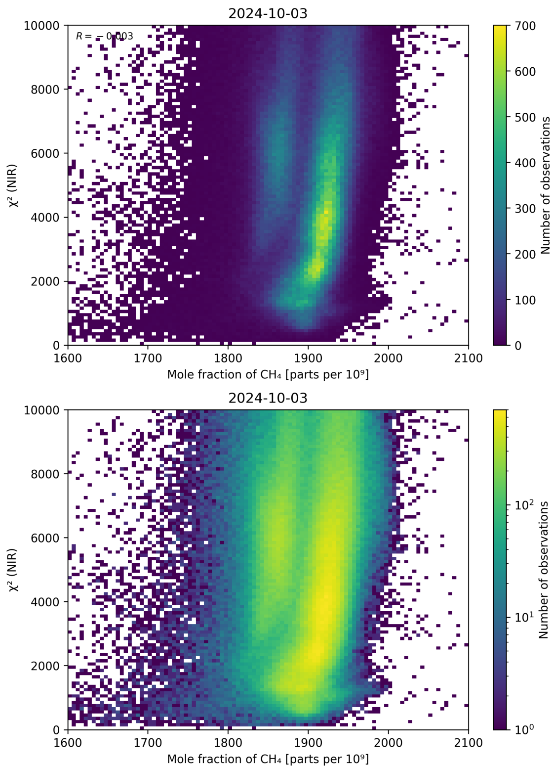
Figure 70: Scatter density plot of “Mole fraction of CH 4 ” against “ \chi^2 (NIR)” for 2024-10-03 to 2024-10-04.
