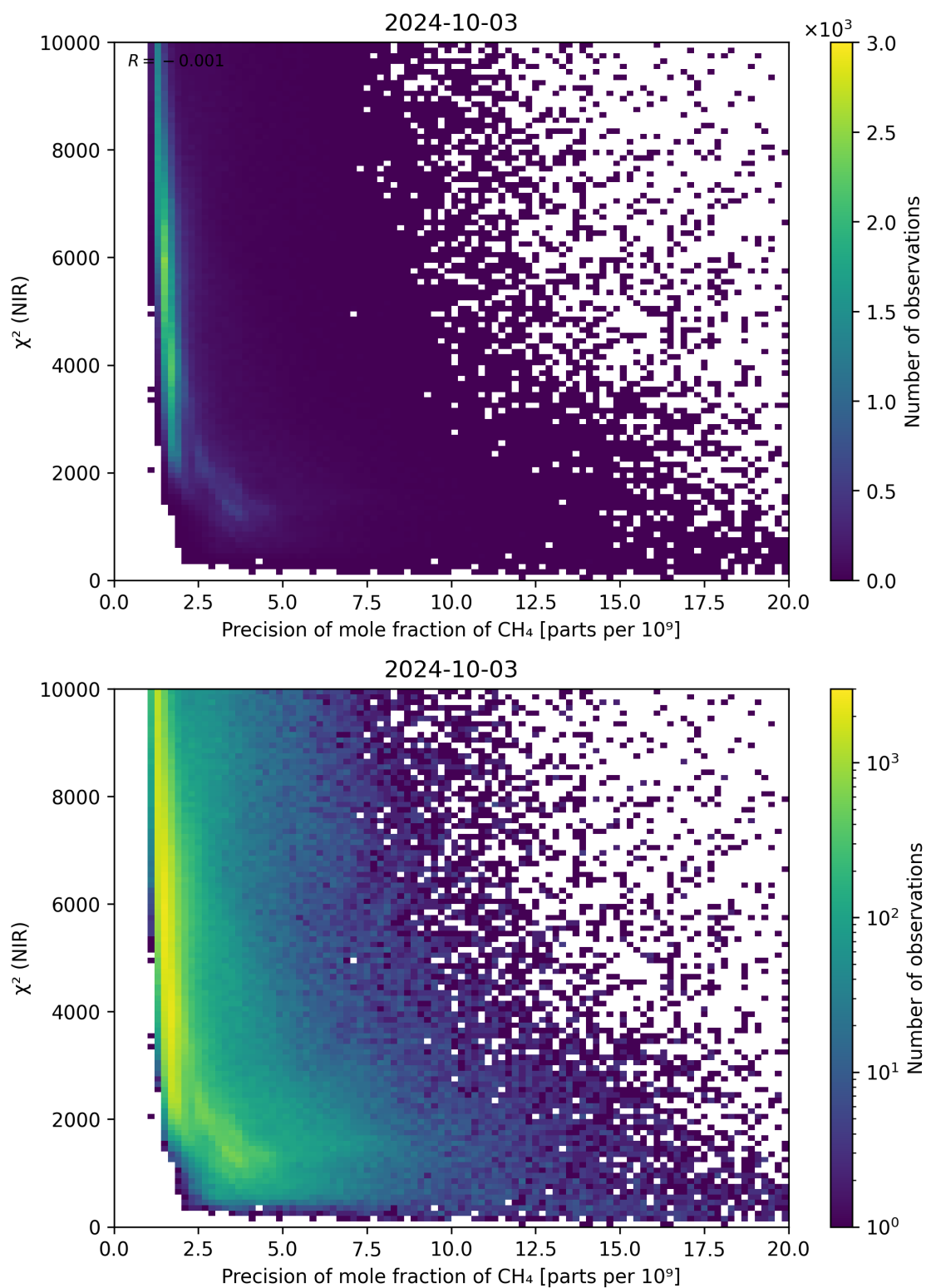
Figure 78: Scatter density plot of “Precision of mole fraction of CH 4 ” against “ \chi^2 (NIR)” for 2024-10-03 to 2024-10-04.
