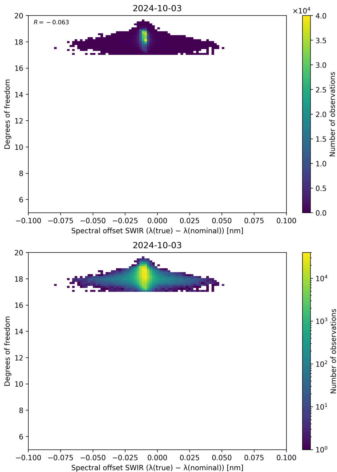
Figure 119: Scatter density plot of “Spectral offset SWIR ( \lambda_{\text{true}} - \lambda_{\text{nominal}} )” against “Degrees of freedom” for 2024-10-03 to 2024-10-04.
