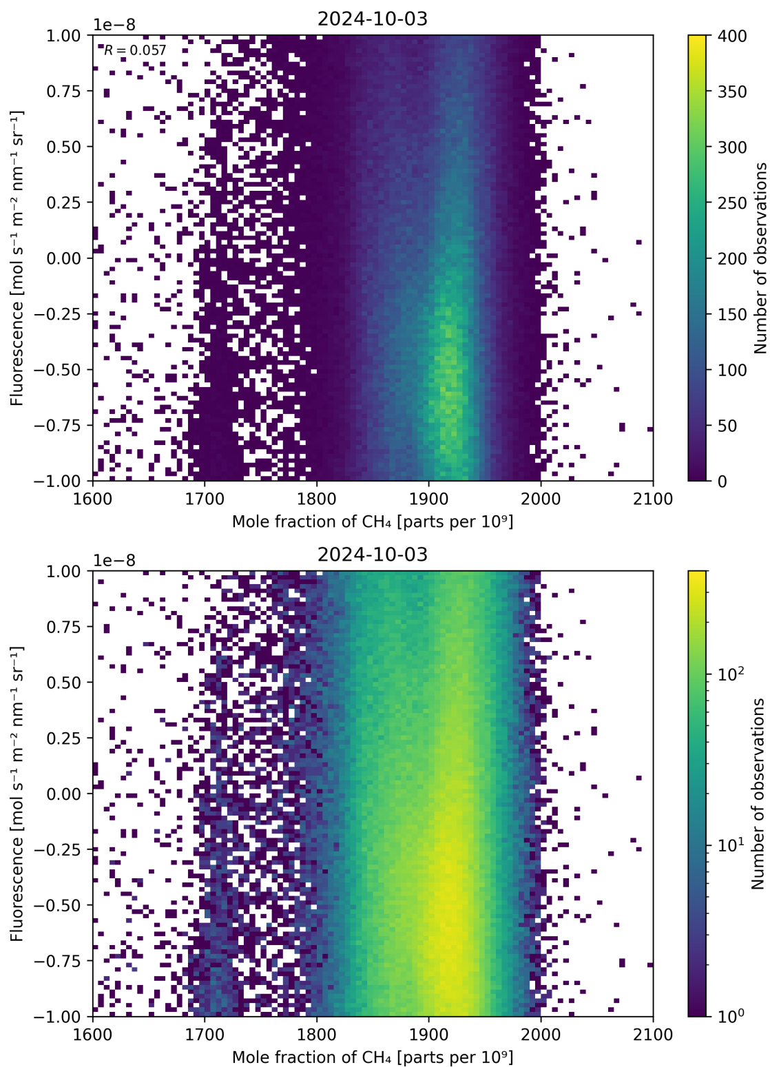
Figure 73: Scatter density plot of “Mole fraction of \text{CH}_4 ” against “Fluorescence” for 2024-10-03 to 2024-10-04.
