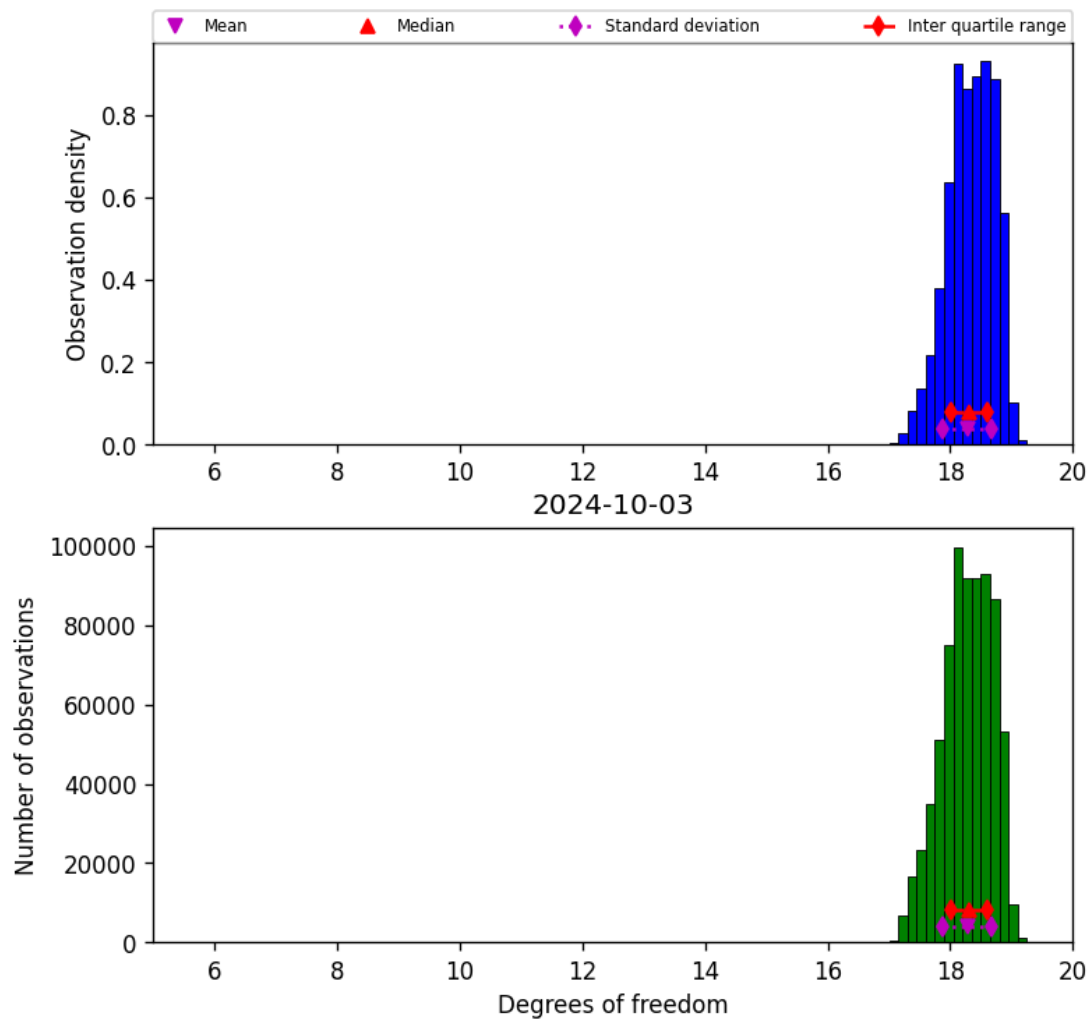
Figure 30: Histogram of “Degrees of freedom” for 2024-10-03 to 2024-10-04
