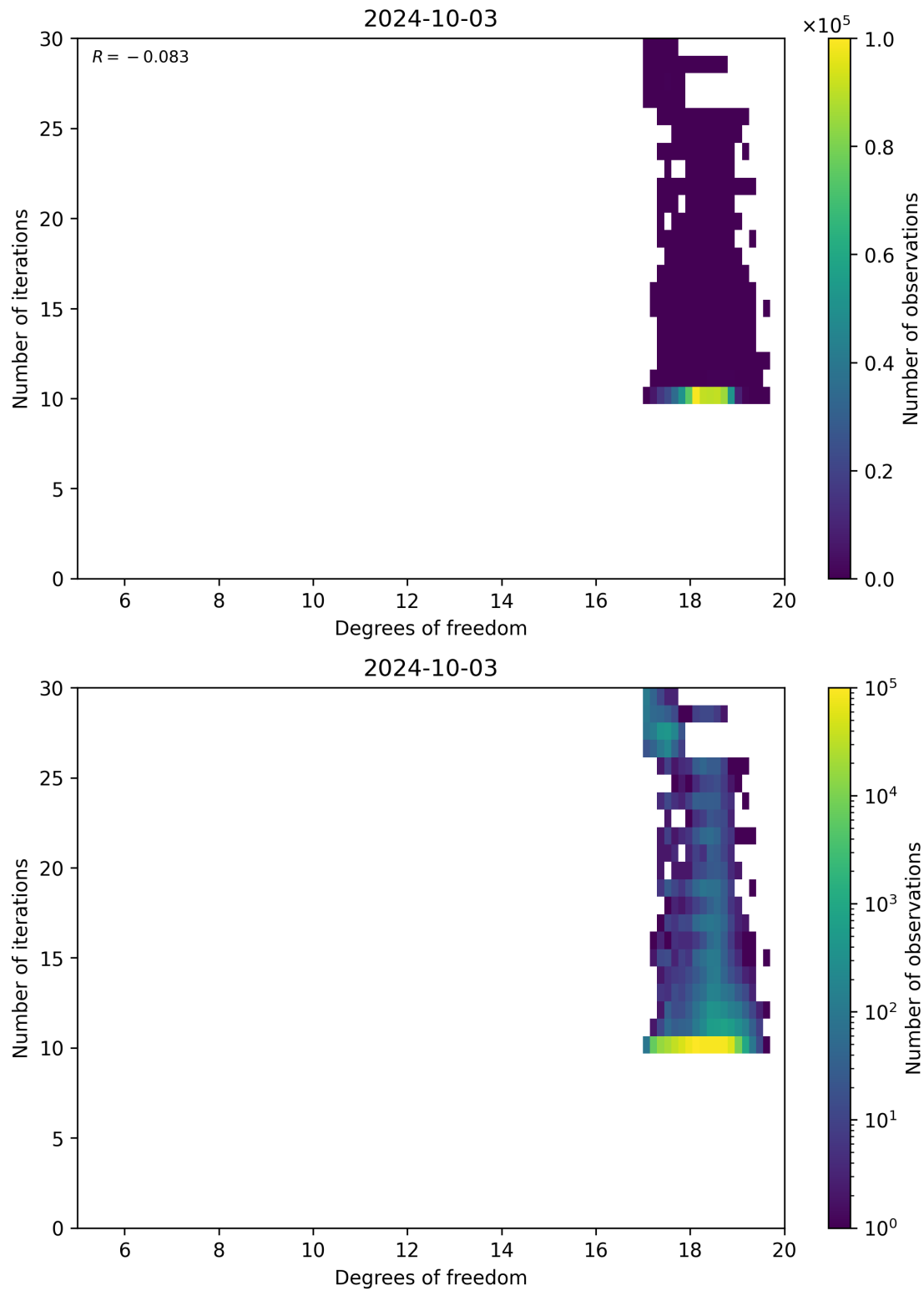
Figure 52: Scatter density plot of “Degrees of freedom” against “Number of iterations” for 2024-10-03 to 2024-10-04.
