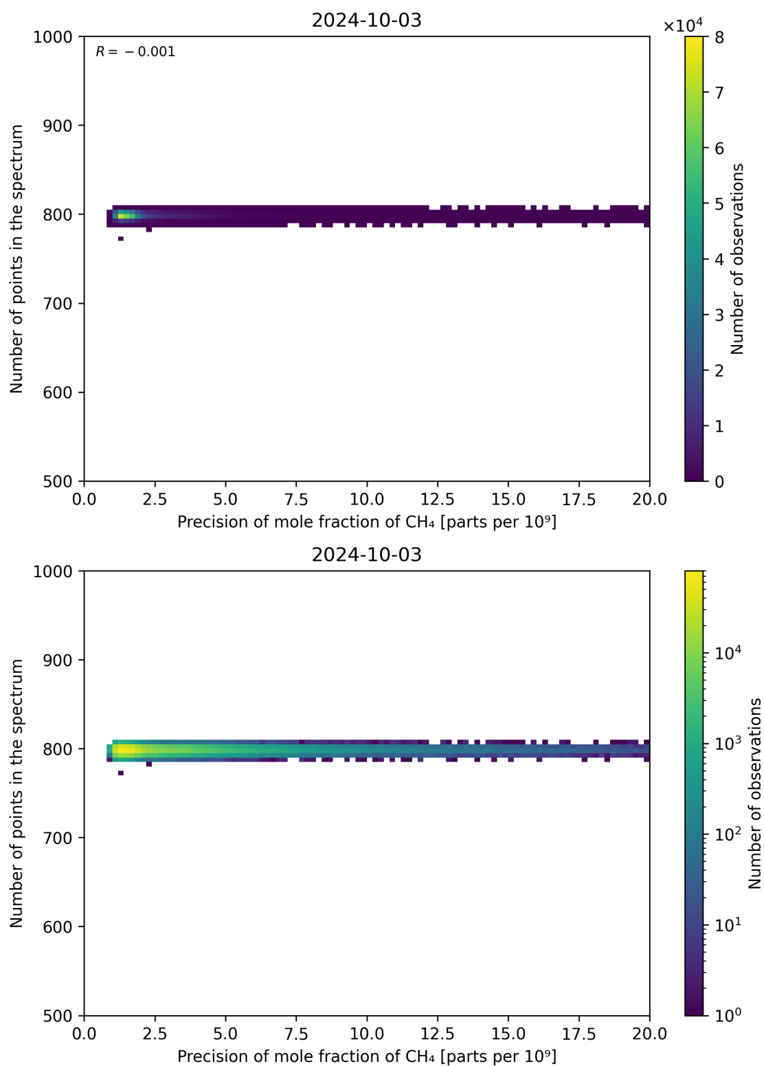
Figure 84: Scatter density plot of “Precision of mole fraction of CH 4 ” against “Number of points in the spectrum” for 2024-10-03 to 2024-10-04.
