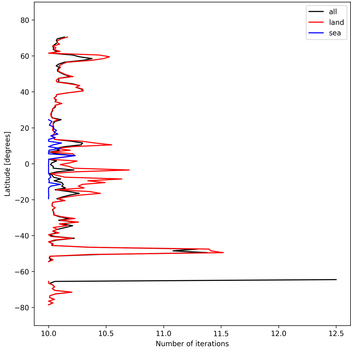
Figure 20: Zonal average of “Number of iterations” for 2024-10-03 to 2024-10-04.
