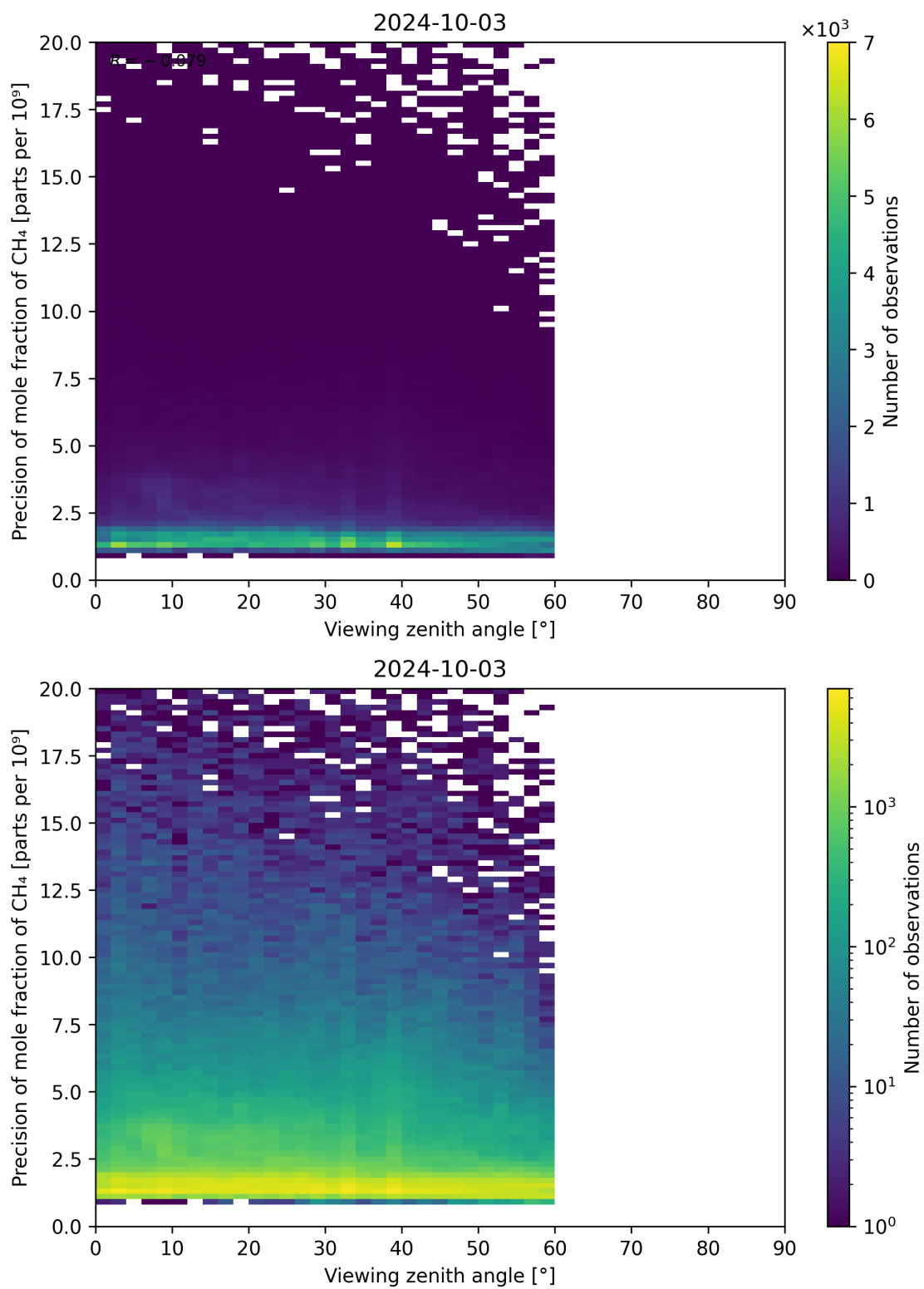
Figure 112: Scatter density plot of “Viewing zenith angle” against “Precision of mole fraction of CH 4 ” for 2024-10-03 to 2024-10-04.
