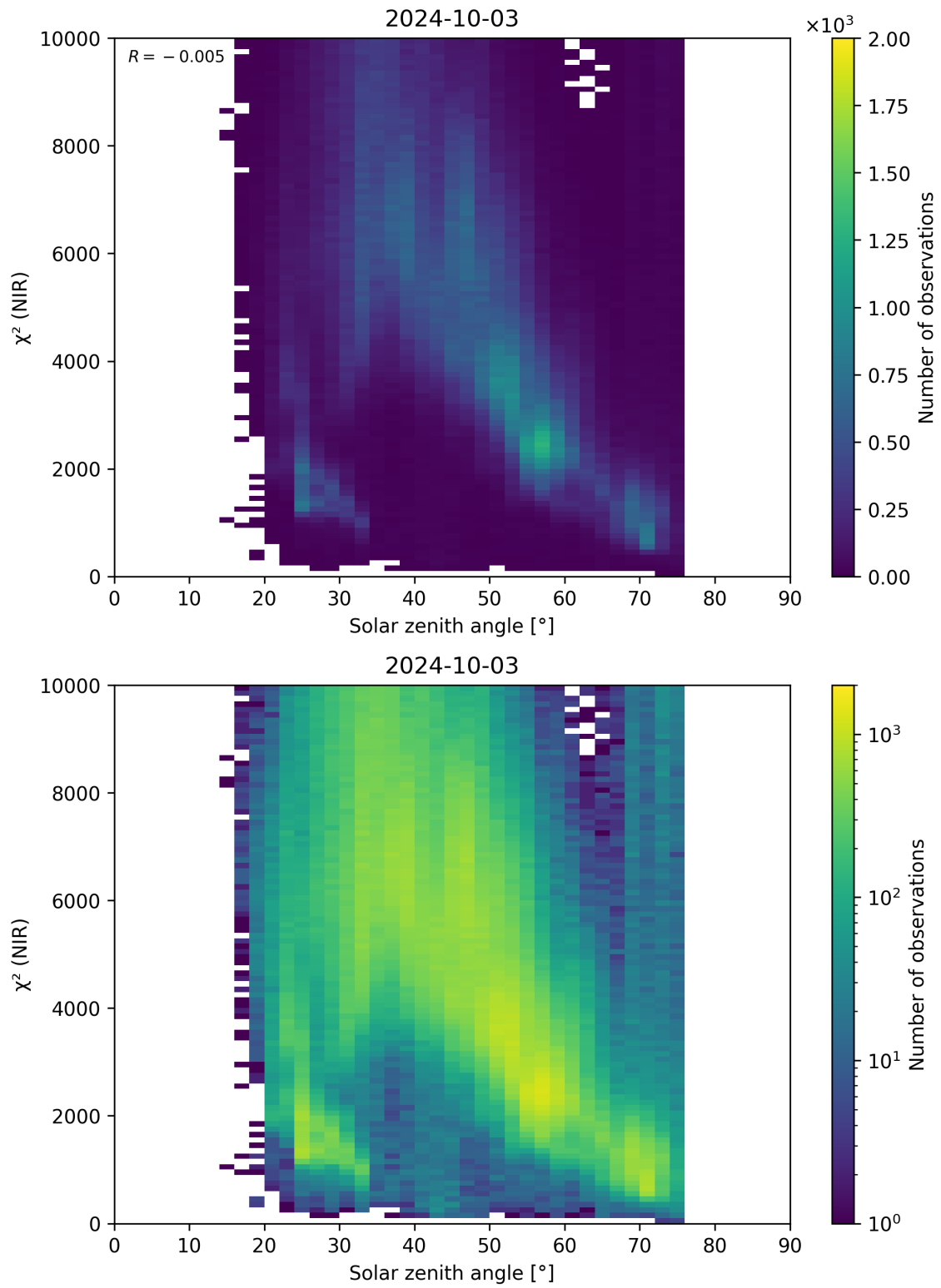
Figure 94: Scatter density plot of “Solar zenith angle” against “ \chi^2 (NIR)” for 2024-10-03 to 2024-10-04.
