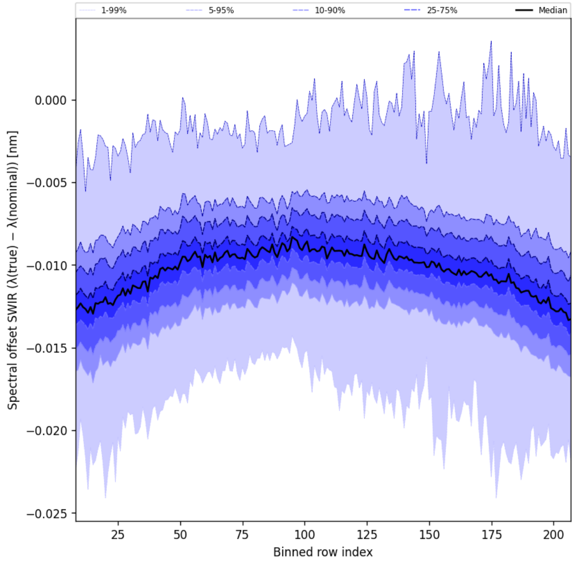
Figure 38: Along track statistics of “Spectral offset SWIR ( \lambda_{\text{true}} - \lambda_{\text{nominal}} )” for 2024-10-03 to 2024-10-04
