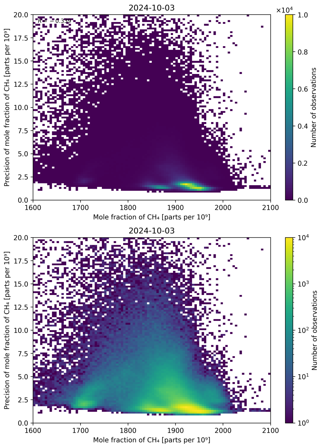
Figure 75: Scatter density plot of “Mole fraction of CH 4 ” against “Precision of mole fraction of CH 4 ” for 2024-10-03 to 2024-10-04.
