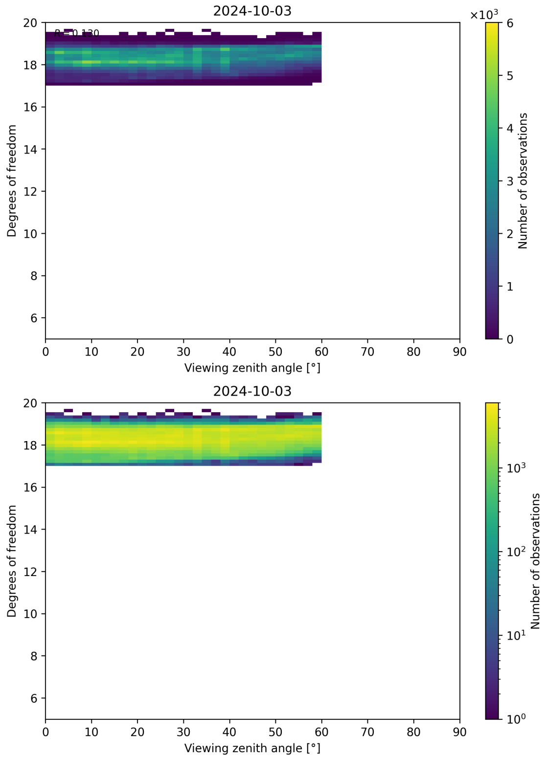
Figure 107: Scatter density plot of “Viewing zenith angle” against “Degrees of freedom” for 2024-10-03 to 2024-10-04.
