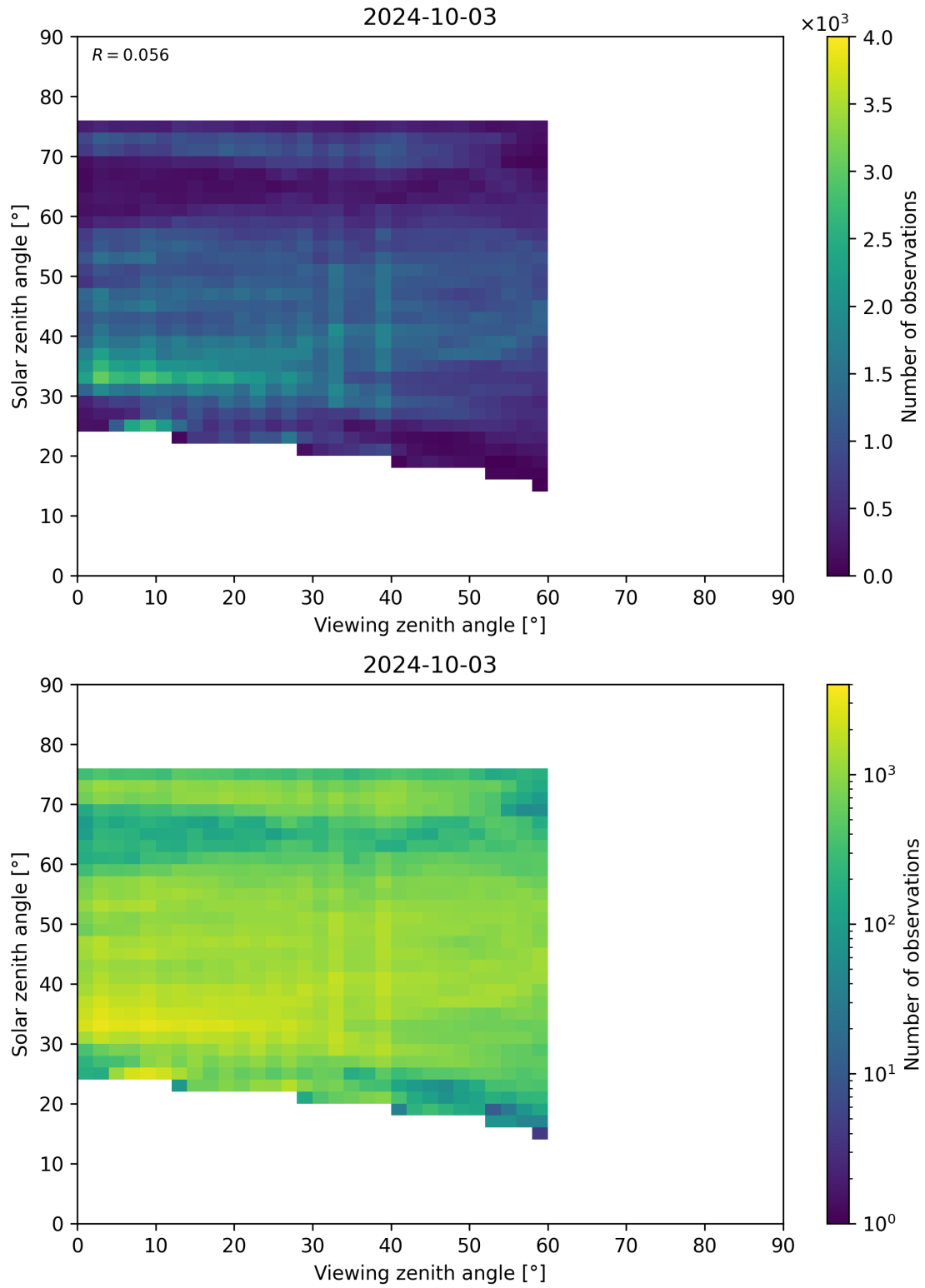
Figure 115: Scatter density plot of “Viewing zenith angle” against “Solar zenith angle” for 2024-10-03 to 2024-10-04.
