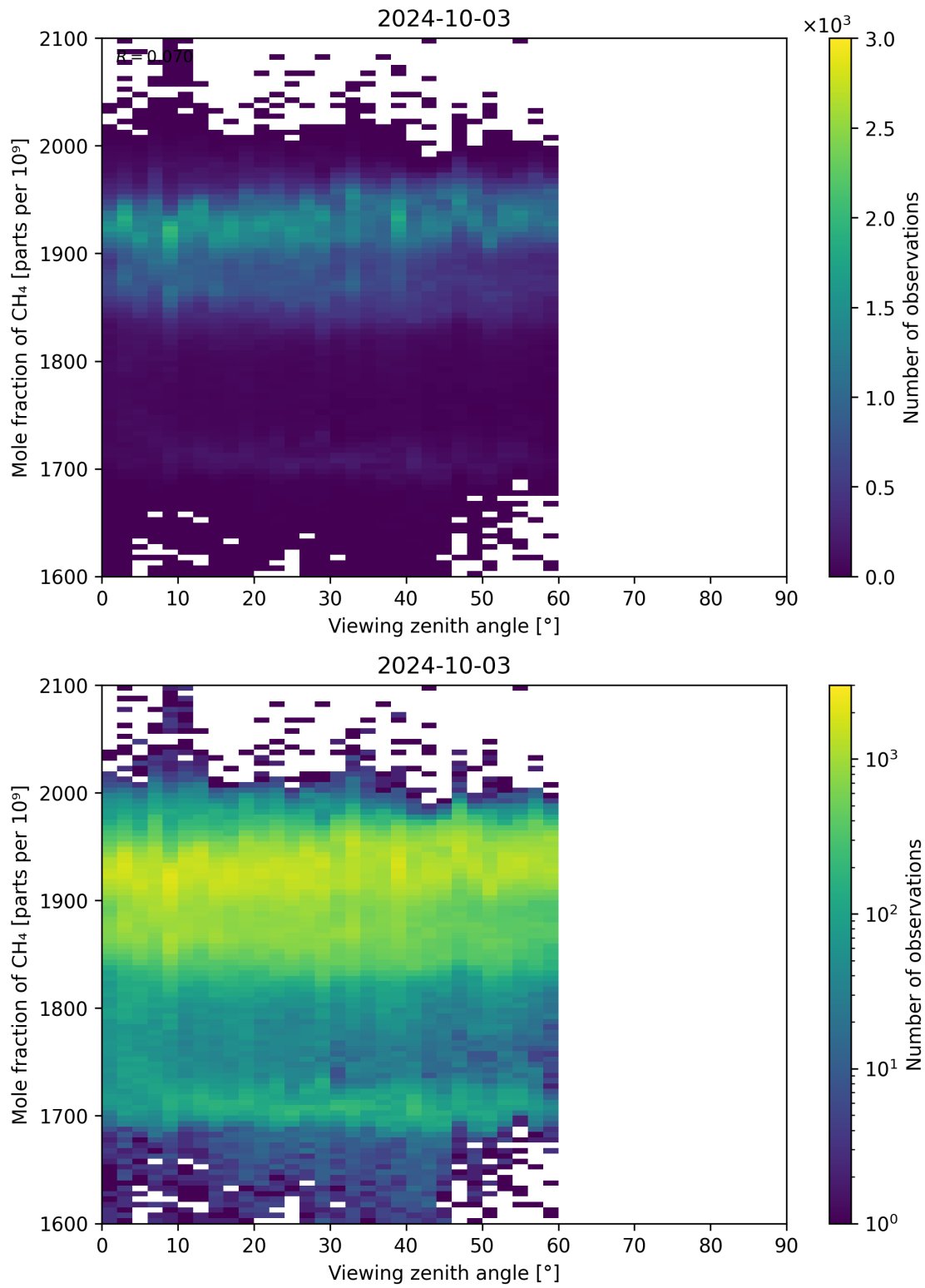
Figure 110: Scatter density plot of “Viewing zenith angle” against “Mole fraction of CH 4 ” for 2024-10-03 to 2024-10-04.
