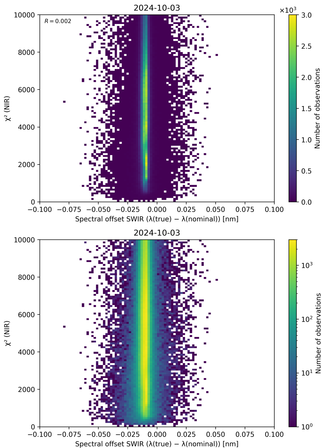
Figure 117: Scatter density plot of “Spectral offset SWIR ( \lambda_{\text{true}} - \lambda_{\text{nominal}} )” against “ \chi^2 (NIR)” for 2024-10-03 to 2024-10-04.
