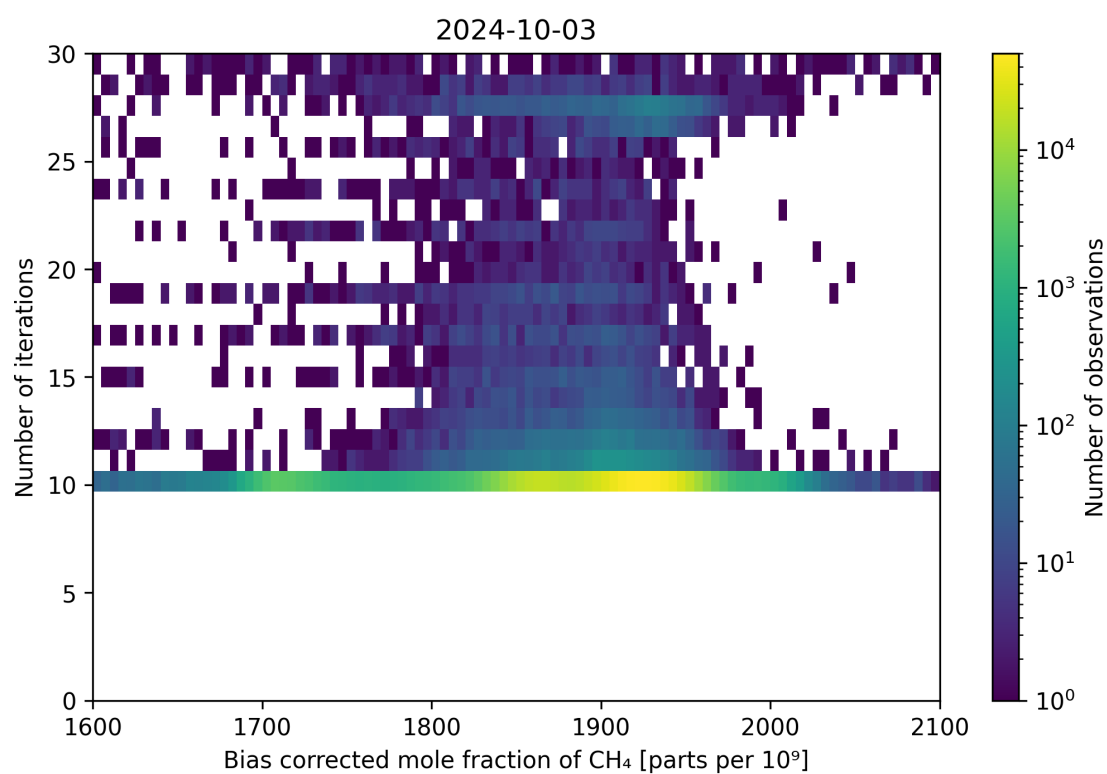
Figure 67: Scatter density plot of “Bias corrected mole fraction of \text{CH}_4 ” against “Number of iterations” for 2024-10-03 to 2024-10-04.
