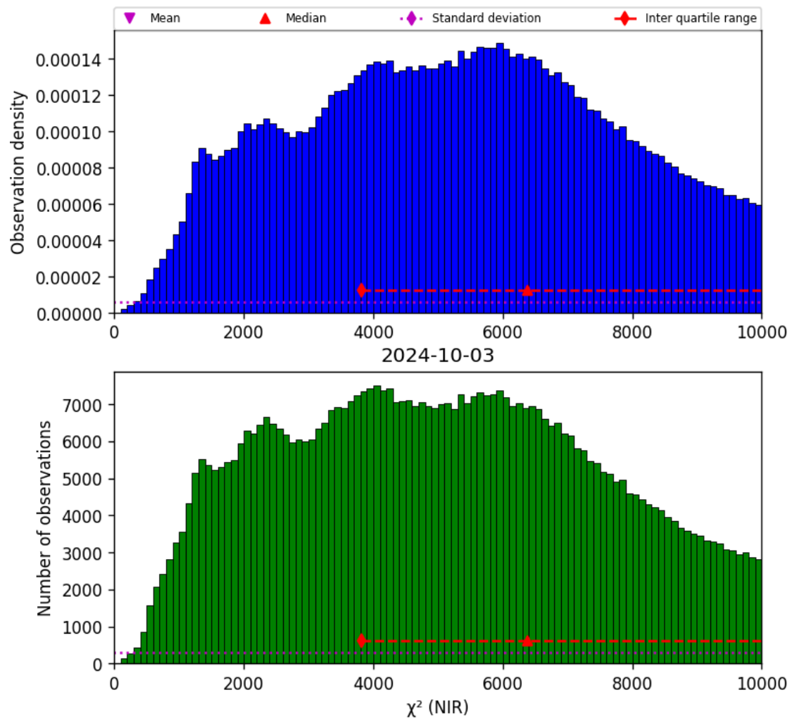
Figure 29: Histogram of “ \chi^2 (NIR)” for 2024-10-03 to 2024-10-04
