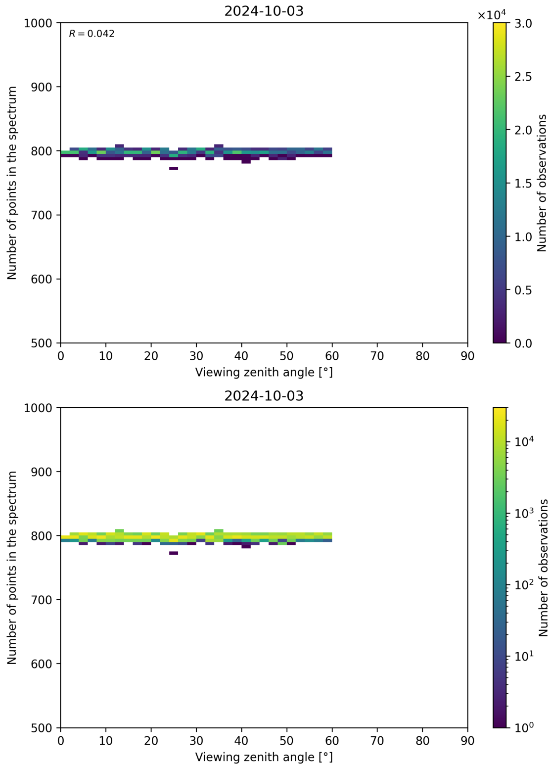
Figure 114: Scatter density plot of “Viewing zenith angle” against “Number of points in the spectrum” for 2024-10-03 to 2024-10-04.
