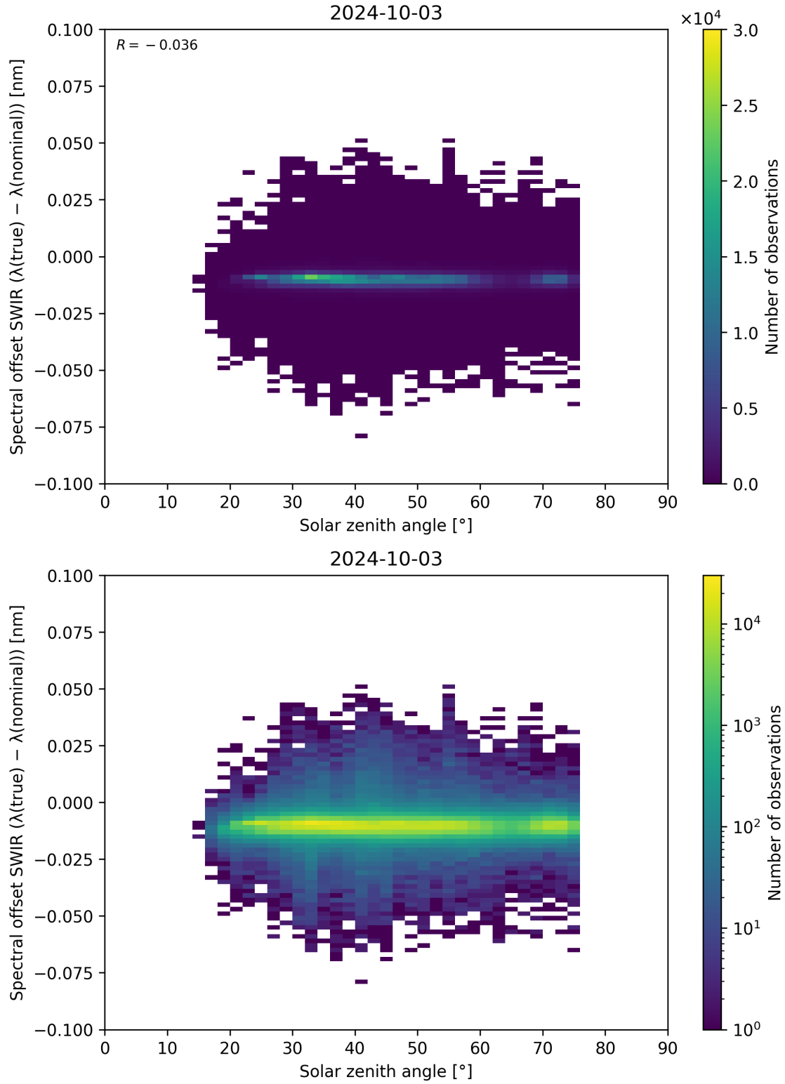
Figure 104: Scatter density plot of “Solar zenith angle” against “Spectral offset SWIR ( \lambda_{\text{true}} - \lambda_{\text{nominal}} )” for 2024-10-03 to 2024-10-04.
