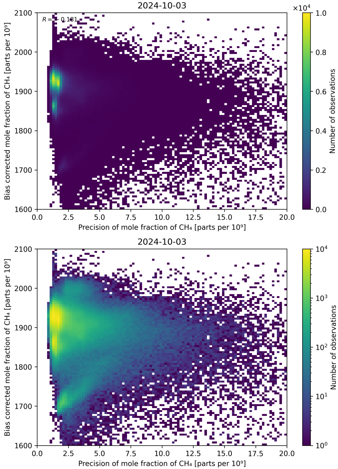
Figure 82: Scatter density plot of “Precision of mole fraction of CH 4 ” against “Bias corrected mole fraction of CH 4 ” for 2024-10-03 to 2024-10-04.
