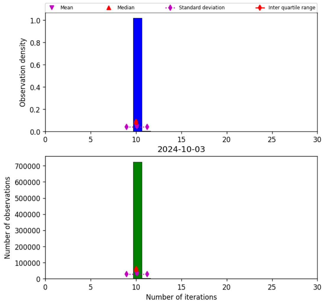
Figure 31: Histogram of “Number of iterations” for 2024-10-03 to 2024-10-04
