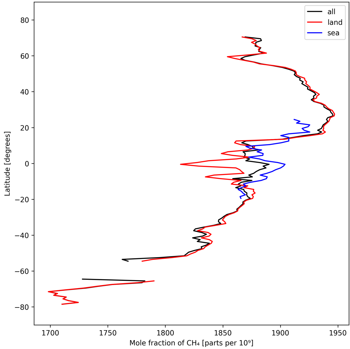
Figure 12: Zonal average of “Mole fraction of CH 4 ” for 2024-10-03 to 2024-10-04.
