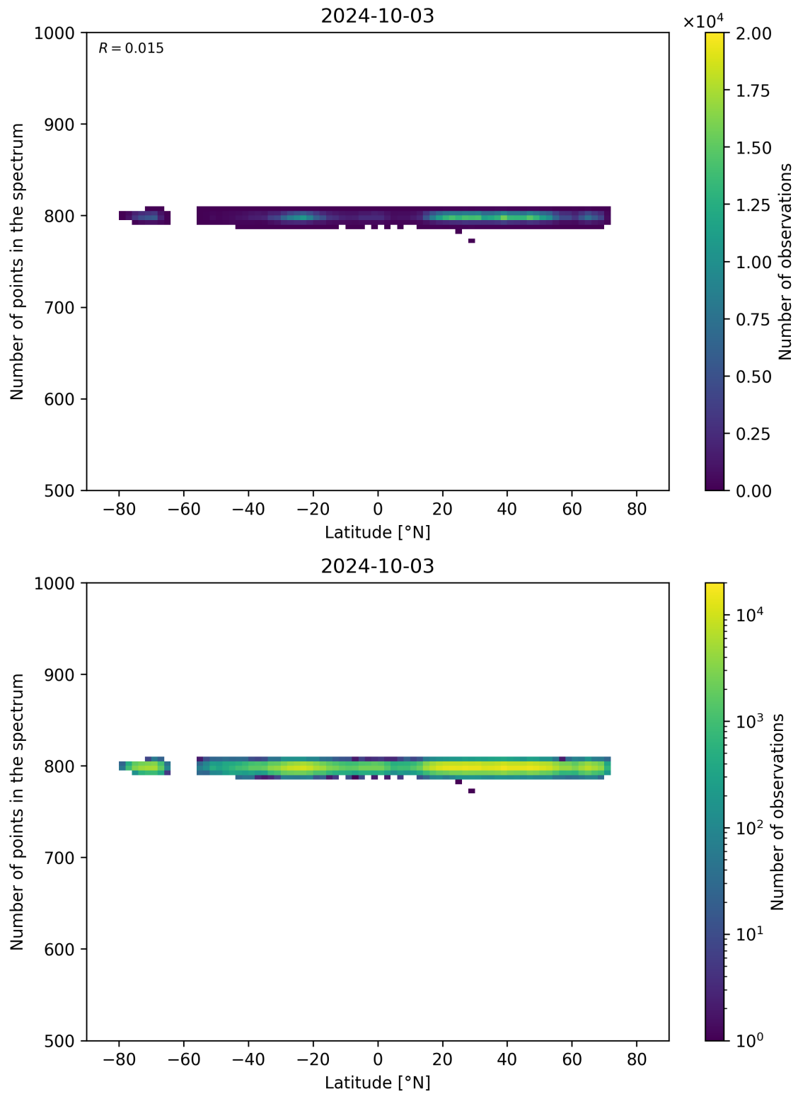
Figure 61: Scatter density plot of “Latitude” against “Number of points in the spectrum” for 2024-10-03 to 2024-10-04.
