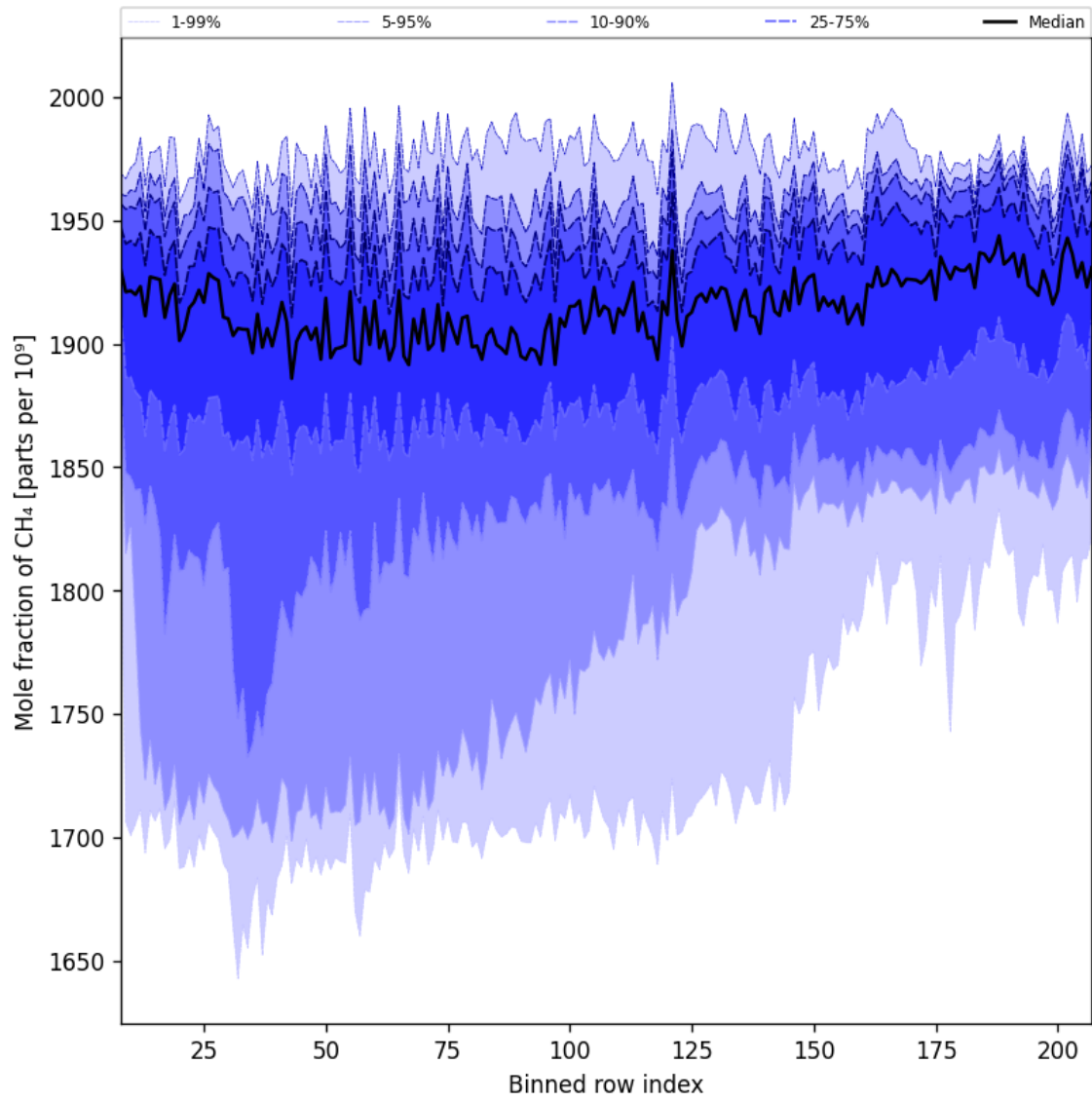
Figure 34: Along track statistics of “Mole fraction of CH 4 ” for 2024-10-03 to 2024-10-04
