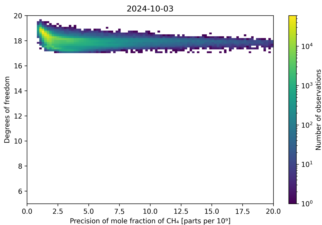
Figure 80: Scatter density plot of “Precision of mole fraction of CH 4 ” against “Degrees of freedom” for 2024-10-03 to 2024-10-04.
