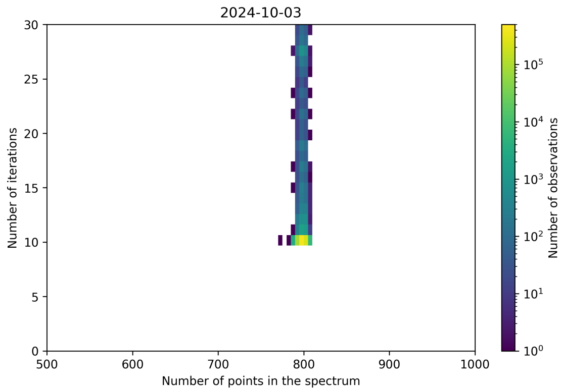
Figure 92: Scatter density plot of “Number of points in the spectrum” against “Number of iterations” for 2024-10-03 to 2024-10-04.
