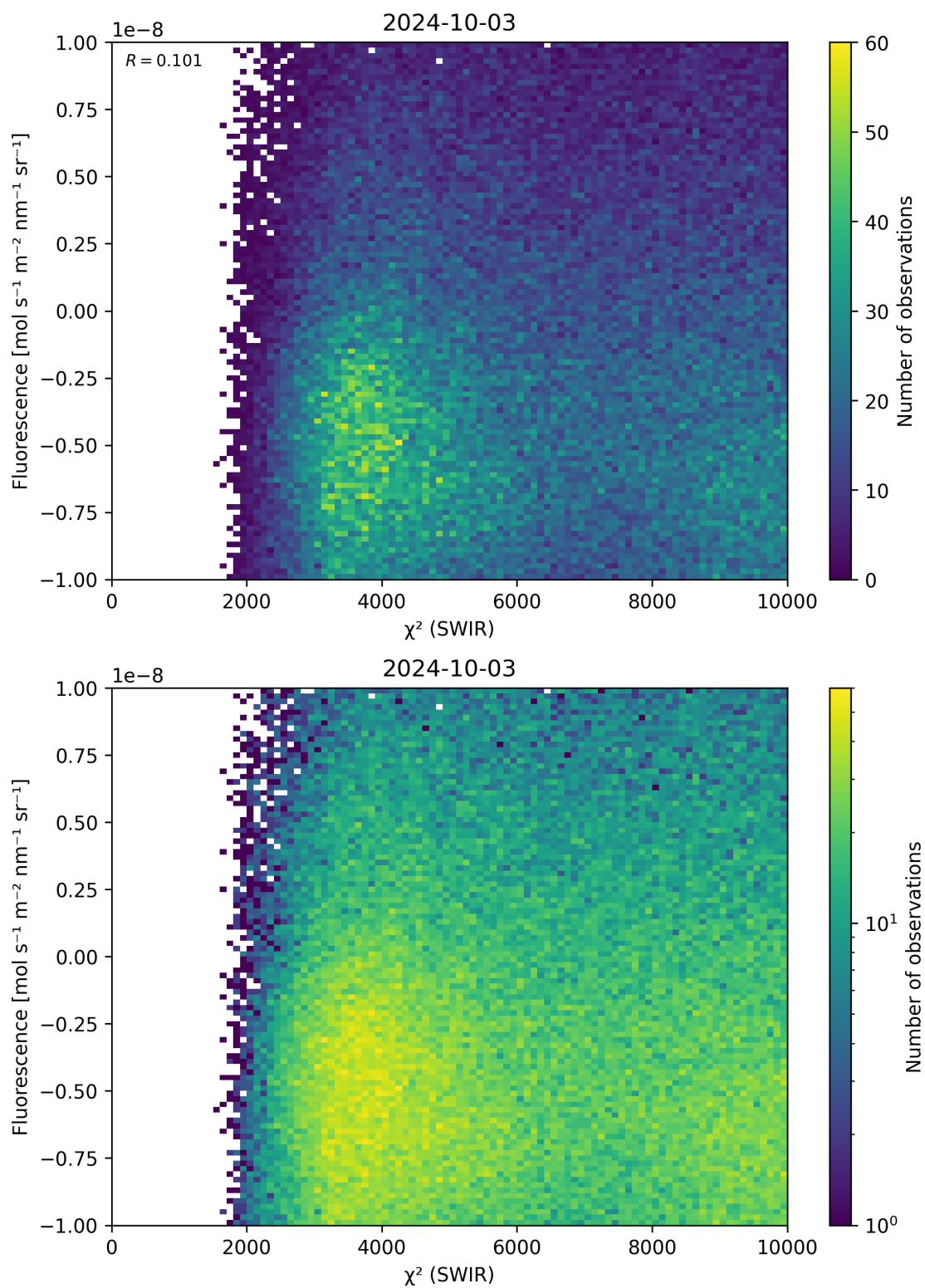
Figure 49: Scatter density plot of “ \chi^2 (SWIR)” against “Fluorescence” for 2024-10-03 to 2024-10-04.
