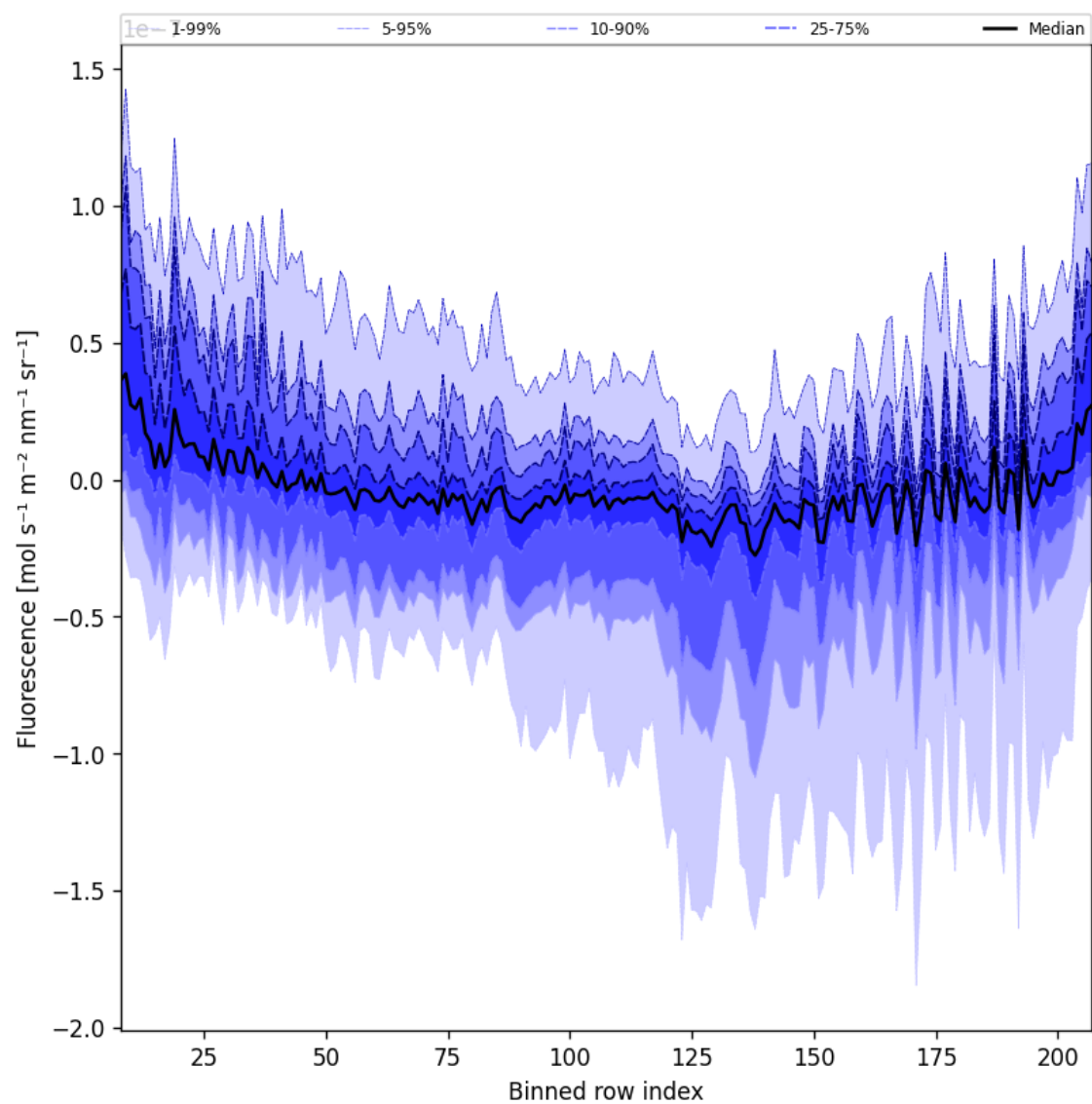
Figure 43: Along track statistics of "Fluorescence" for 2024-10-03 to 2024-10-04
