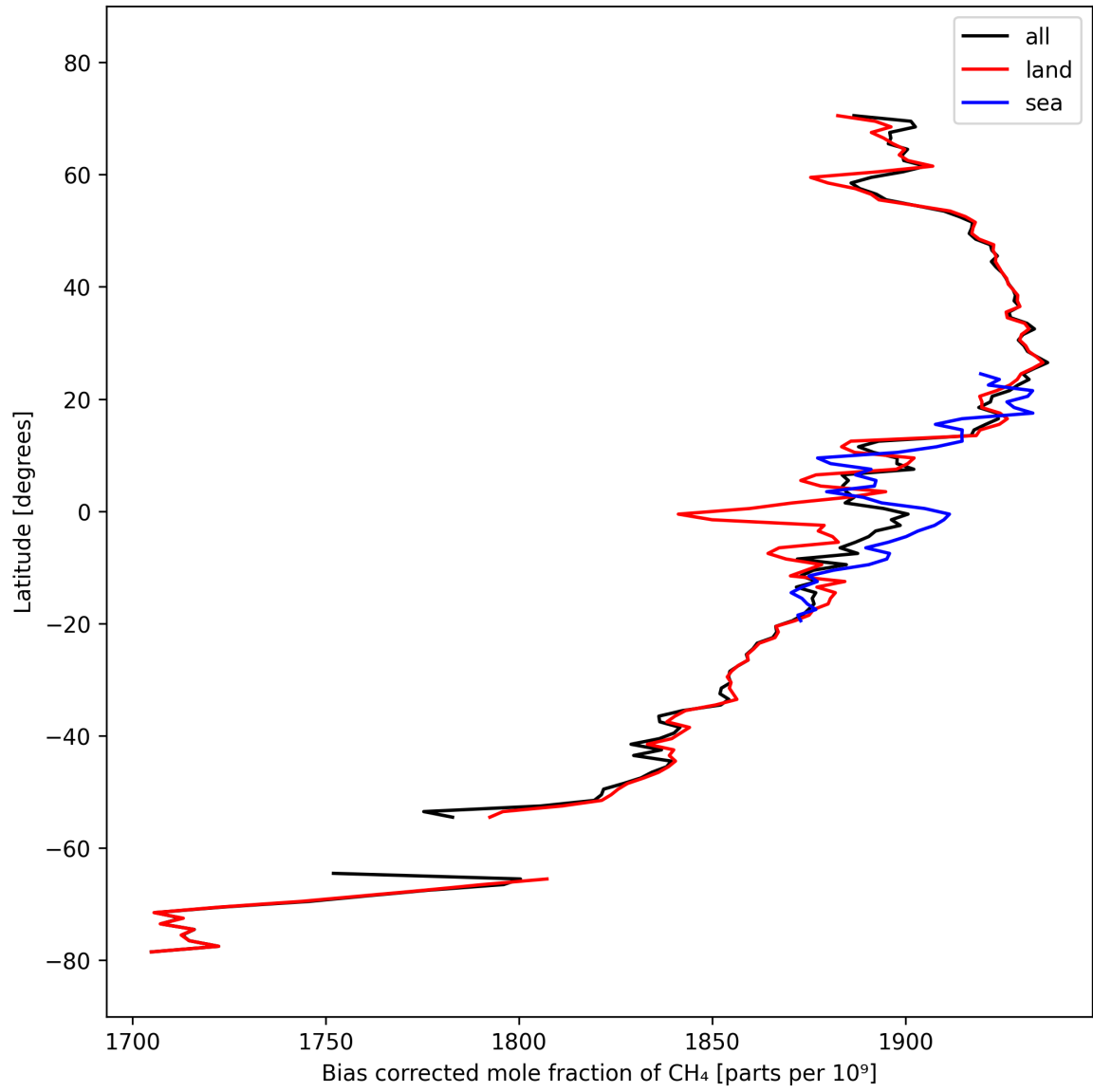
Figure 14: Zonal average of “Bias corrected mole fraction of CH 4 ” for 2024-10-03 to 2024-10-04.
