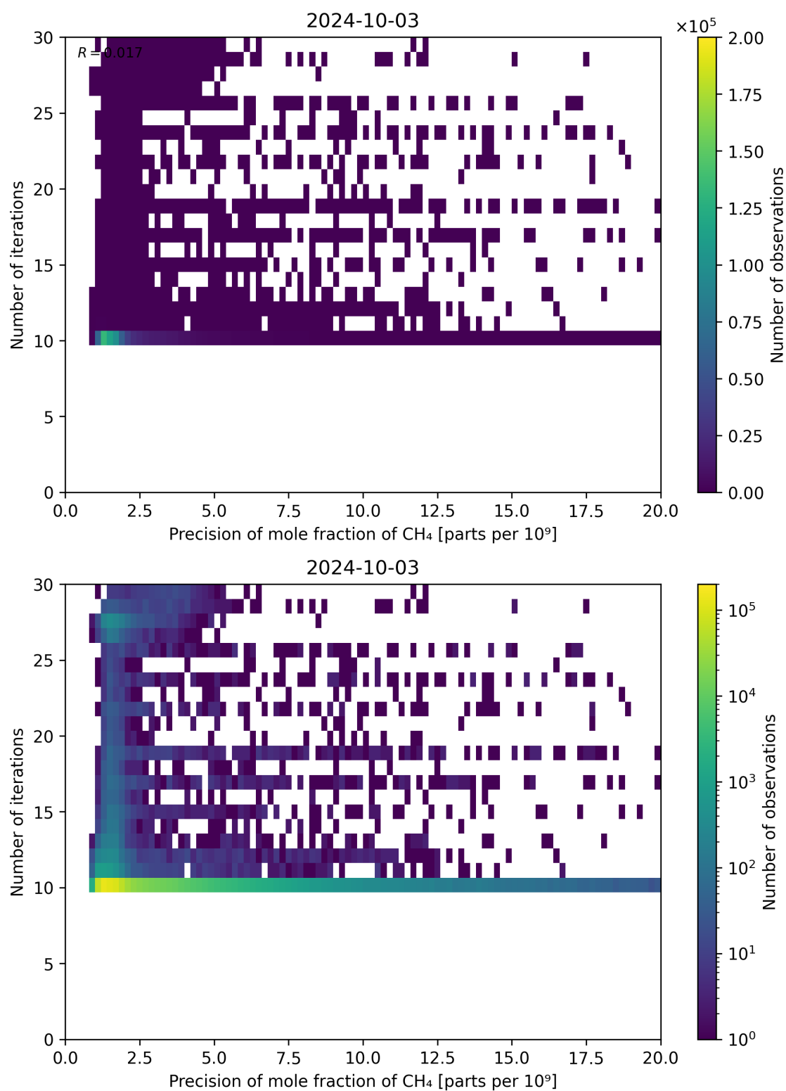
Figure 83: Scatter density plot of “Precision of mole fraction of CH 4 ” against “Number of iterations” for 2024-10-03 to 2024-10-04.
