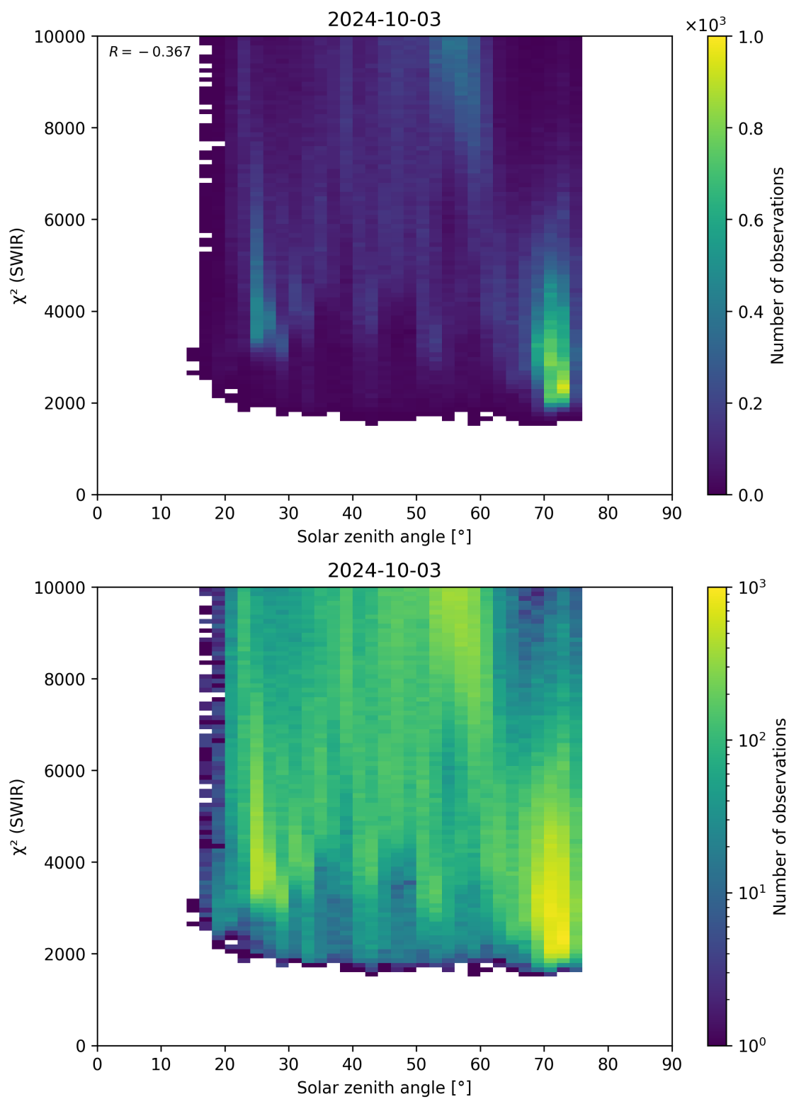
Figure 95: Scatter density plot of “Solar zenith angle” against “ \chi^2 (SWIR)” for 2024-10-03 to 2024-10-04.
