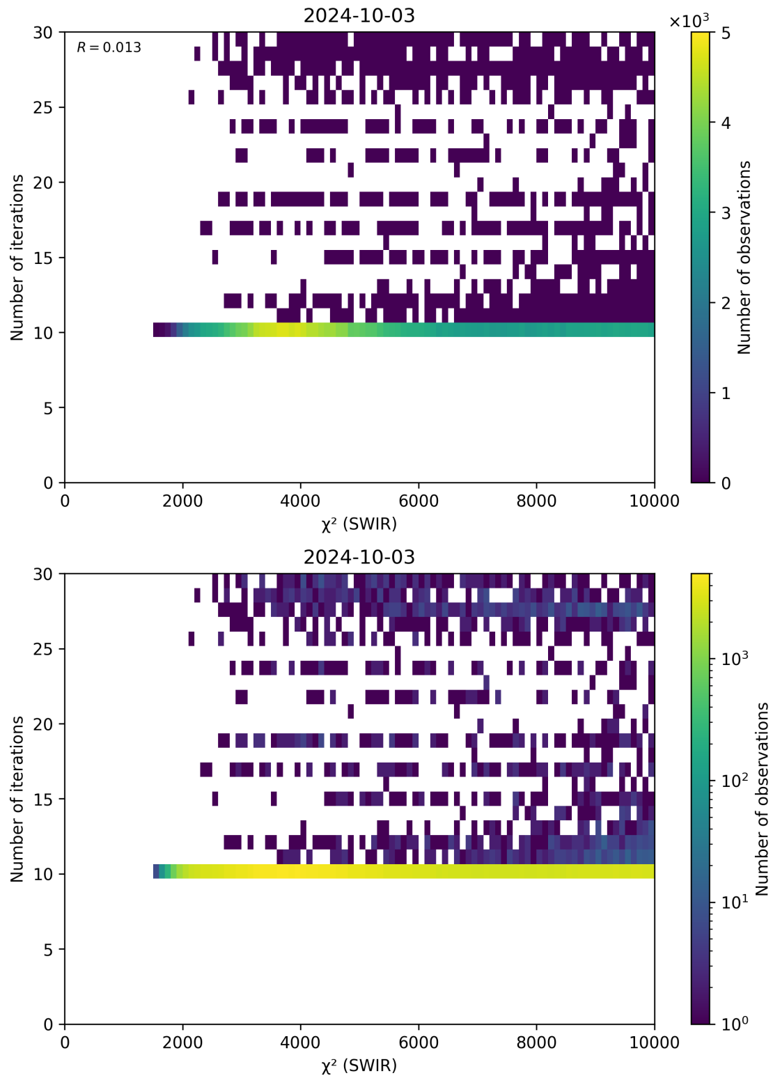
Figure 50: Scatter density plot of “ \chi^2 (SWIR)” against “Number of iterations” for 2024-10-03 to 2024-10-04.
