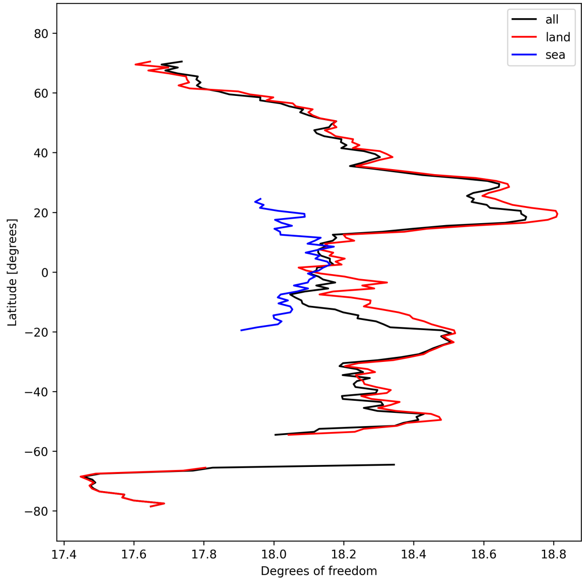
Figure 19: Zonal average of “Degrees of freedom” for 2024-10-03 to 2024-10-04.
