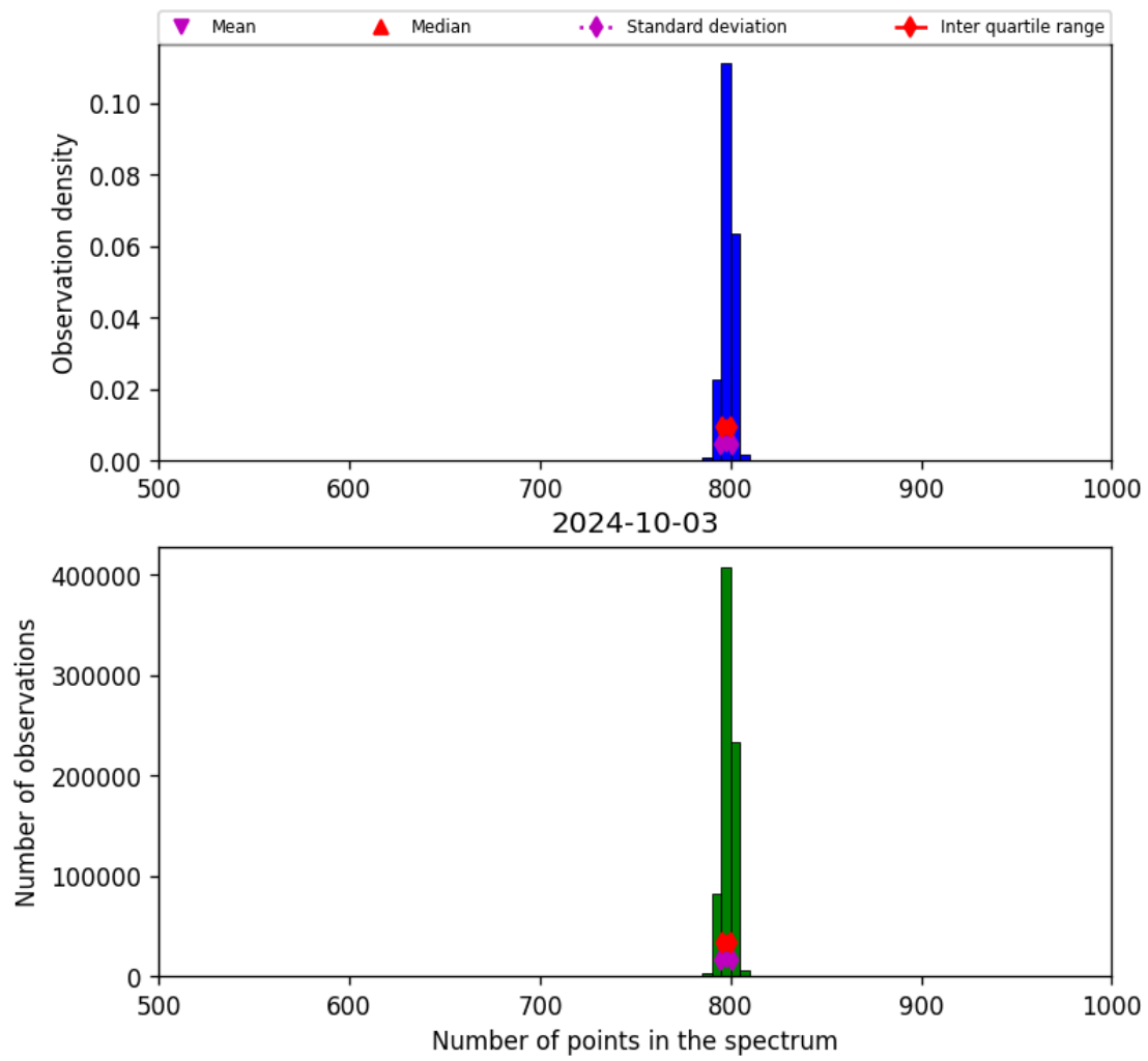
Figure 26: Histogram of “Number of points in the spectrum” for 2024-10-03 to 2024-10-04
