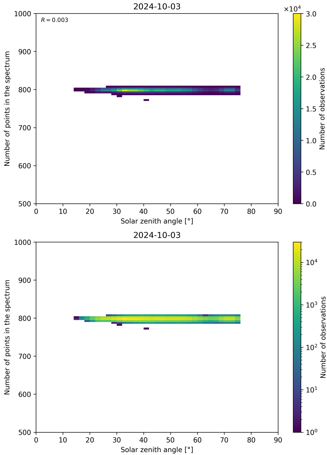
Figure 103: Scatter density plot of “Solar zenith angle” against “Number of points in the spectrum” for 2024-10-03 to 2024-10-04.
