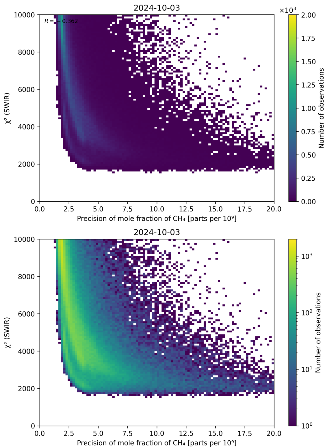
Figure 79: Scatter density plot of “Precision of mole fraction of \text{CH}_4 ” against “ \chi^2 (SWIR)” for 2024-10-03 to 2024-10-04.
