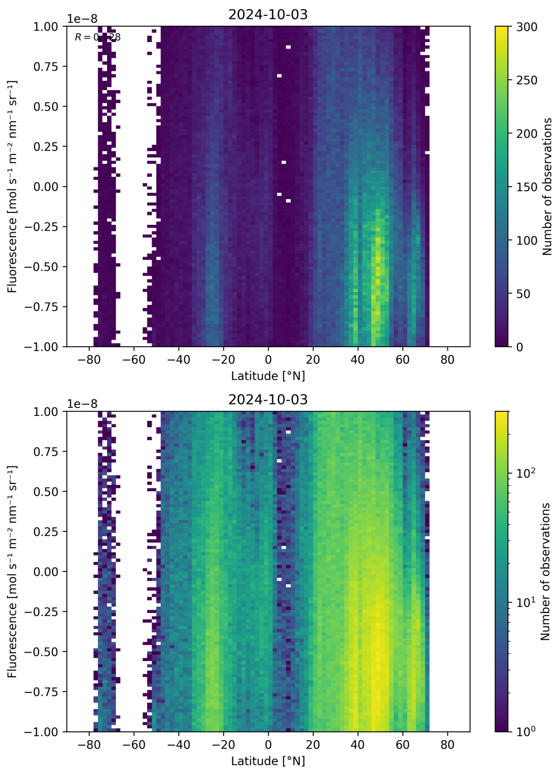
Figure 56: Scatter density plot of “Latitude” against “Fluorescence” for 2024-10-03 to 2024-10-04.
