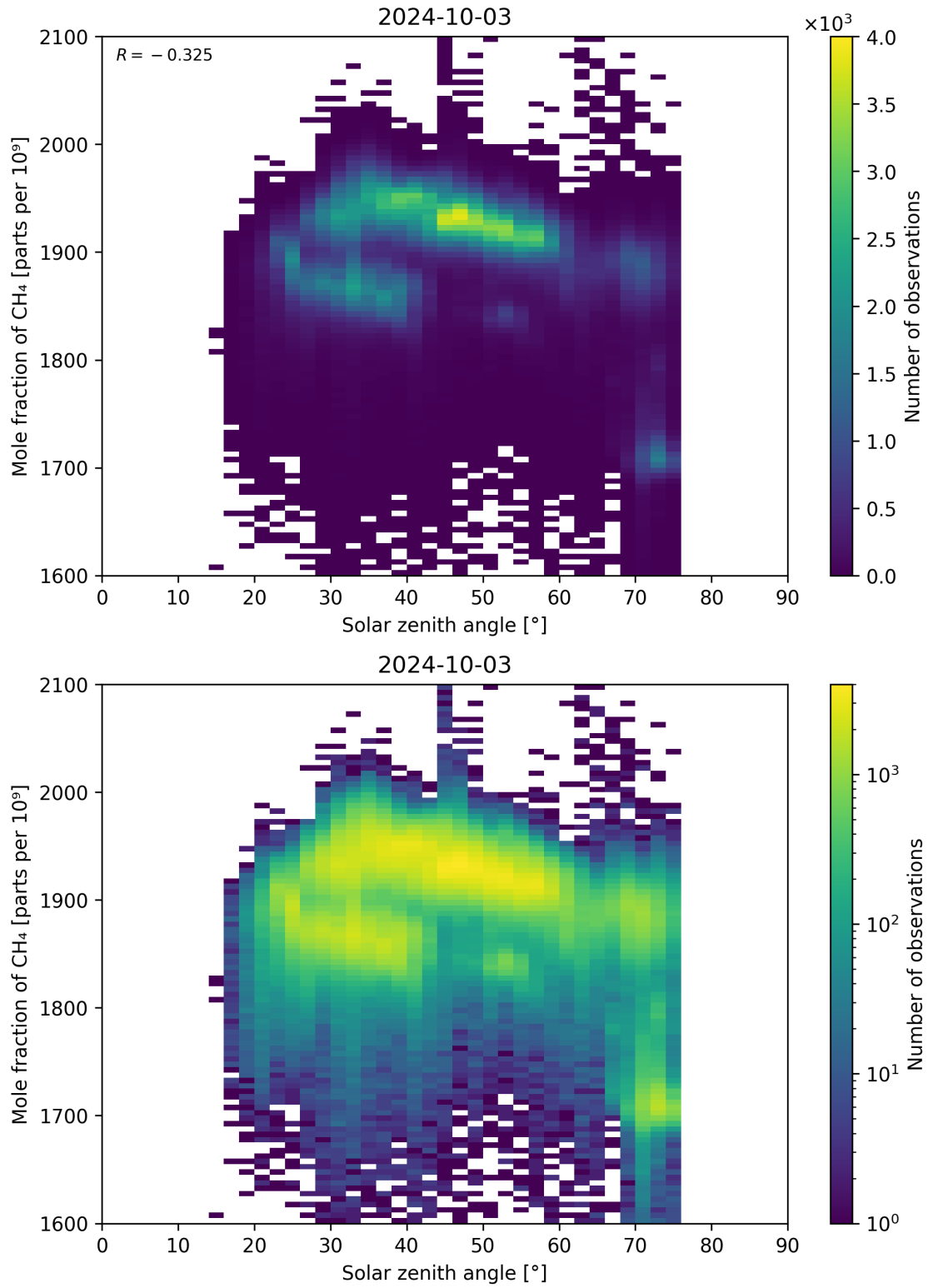
Figure 99: Scatter density plot of “Solar zenith angle” against “Mole fraction of CH 4 ” for 2024-10-03 to 2024-10-04.
