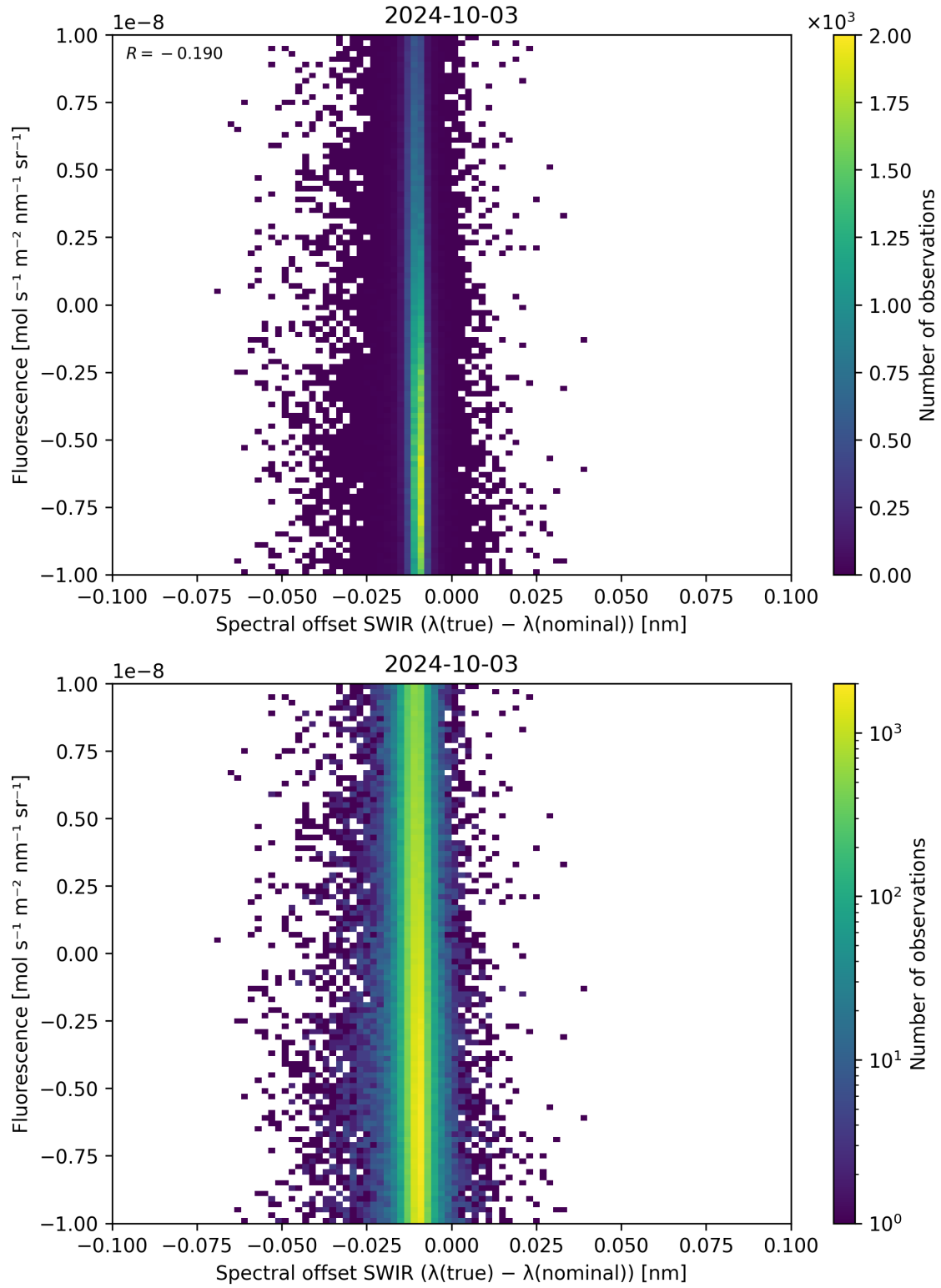
Figure 120: Scatter density plot of “Spectral offset SWIR ( \lambda_{\text{true}} - \lambda_{\text{nominal}} )” against “Fluorescence” for 2024-10-03 to 2024-10-04.
