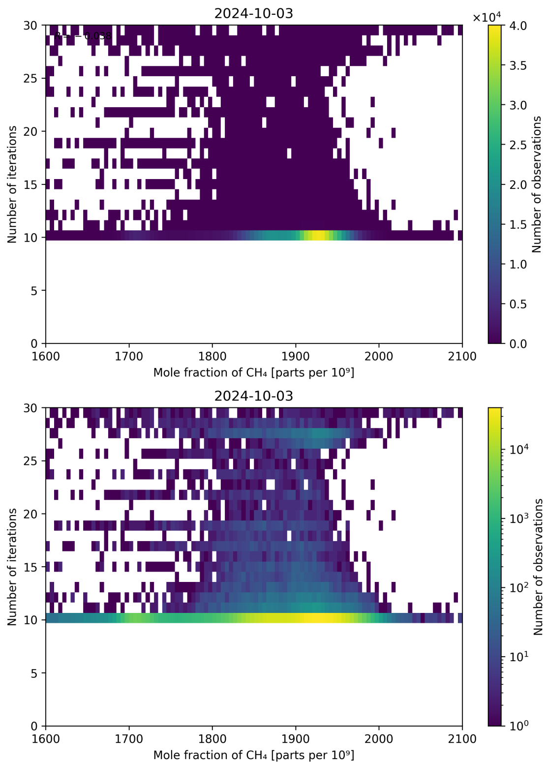
Figure 76: Scatter density plot of “Mole fraction of CH 4 ” against “Number of iterations” for 2024-10-03 to 2024-10-04.
