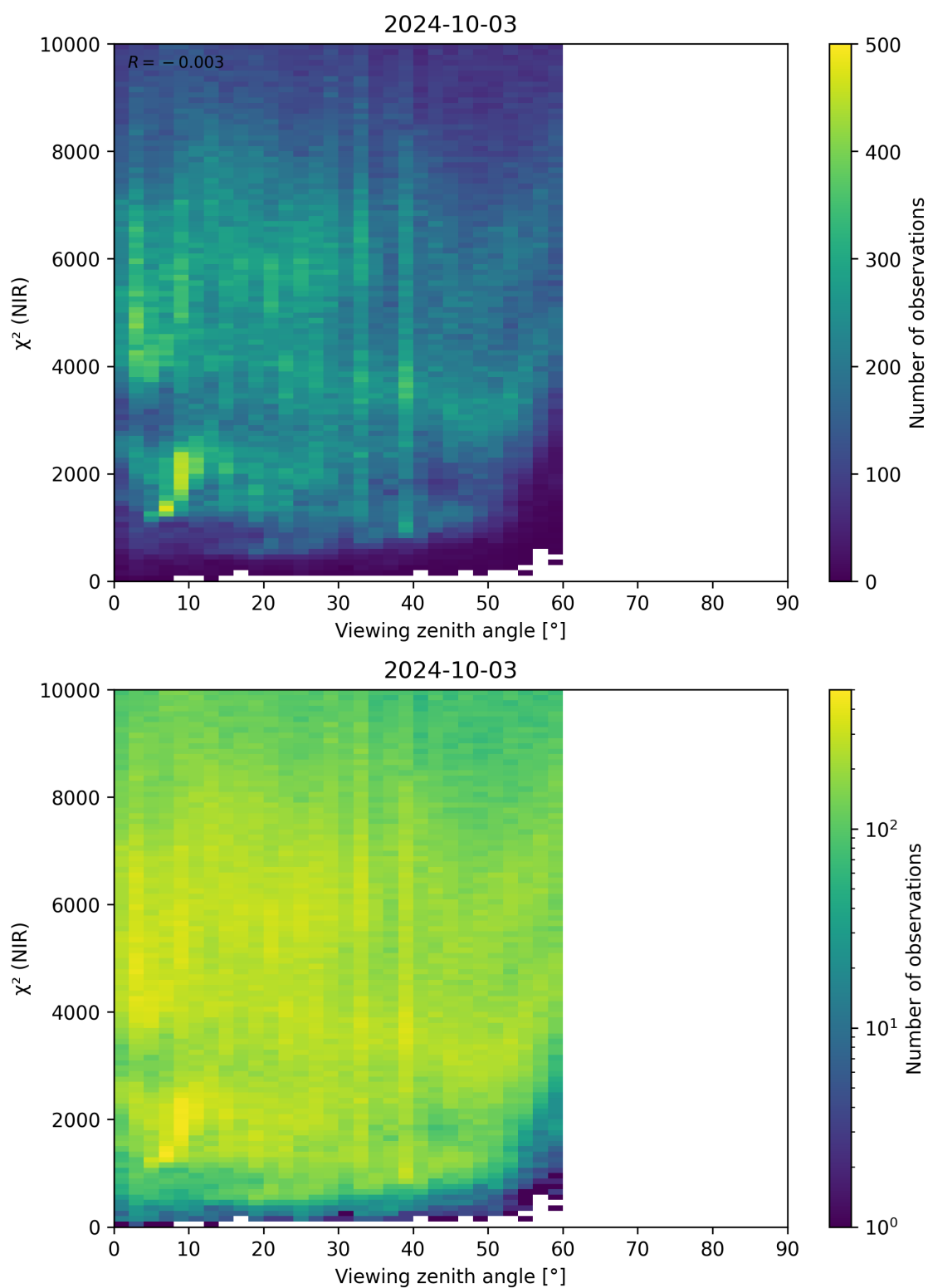
Figure 105: Scatter density plot of “Viewing zenith angle” against “ \chi^2 (NIR)” for 2024-10-03 to 2024-10-04.
