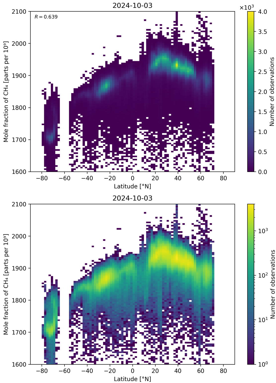
Figure 57: Scatter density plot of “Latitude” against “Mole fraction of CH 4 ” for 2024-10-03 to 2024-10-04.
