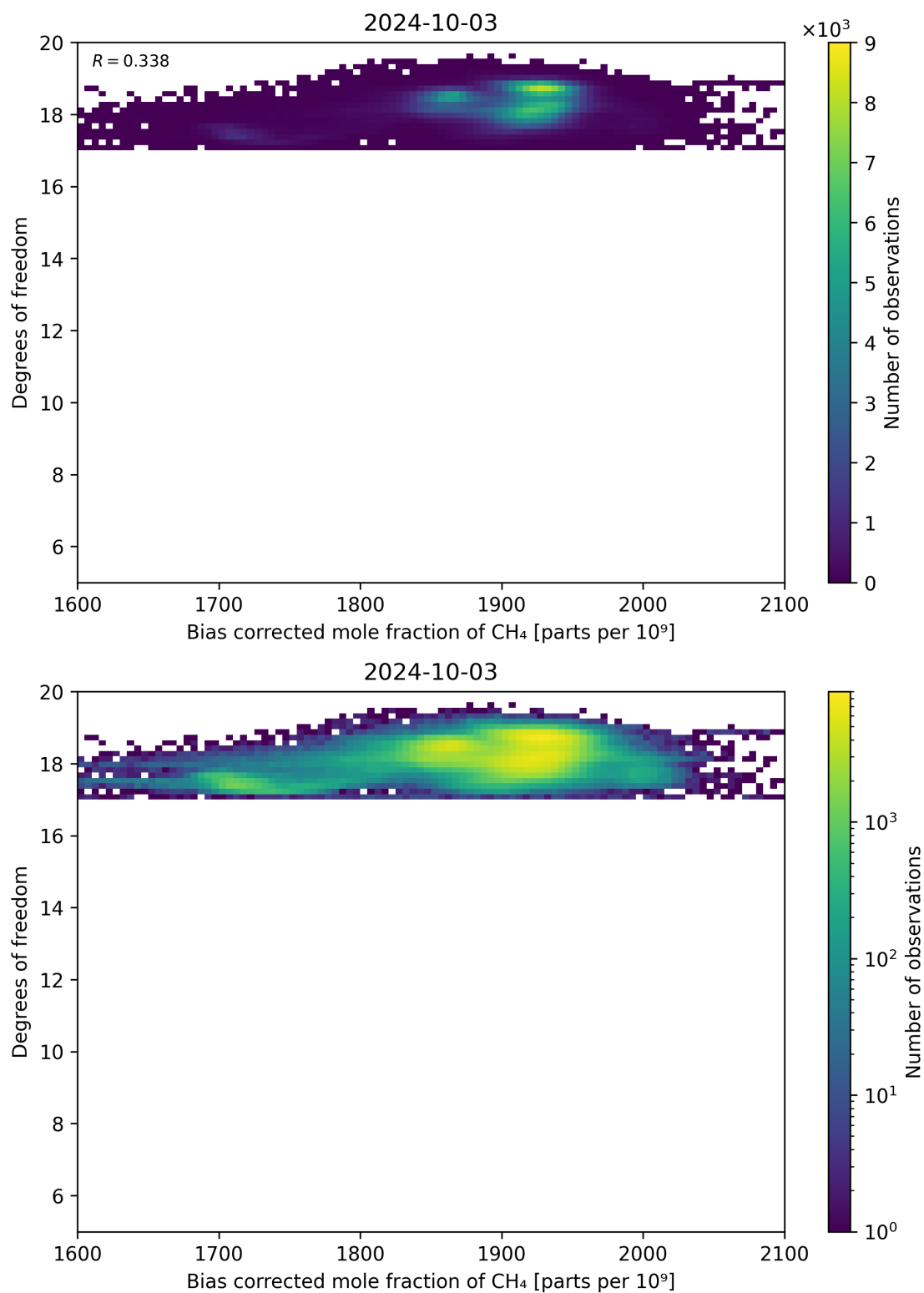
Figure 65: Scatter density plot of “Bias corrected mole fraction of CH 4 ” against “Degrees of freedom” for 2024-10-03 to 2024-10-04.
