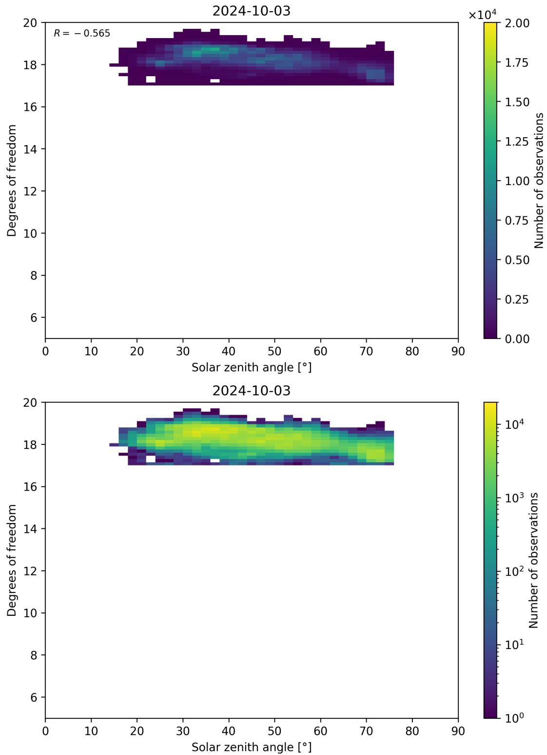
Figure 96: Scatter density plot of “Solar zenith angle” against “Degrees of freedom” for 2024-10-03 to 2024-10-04.
