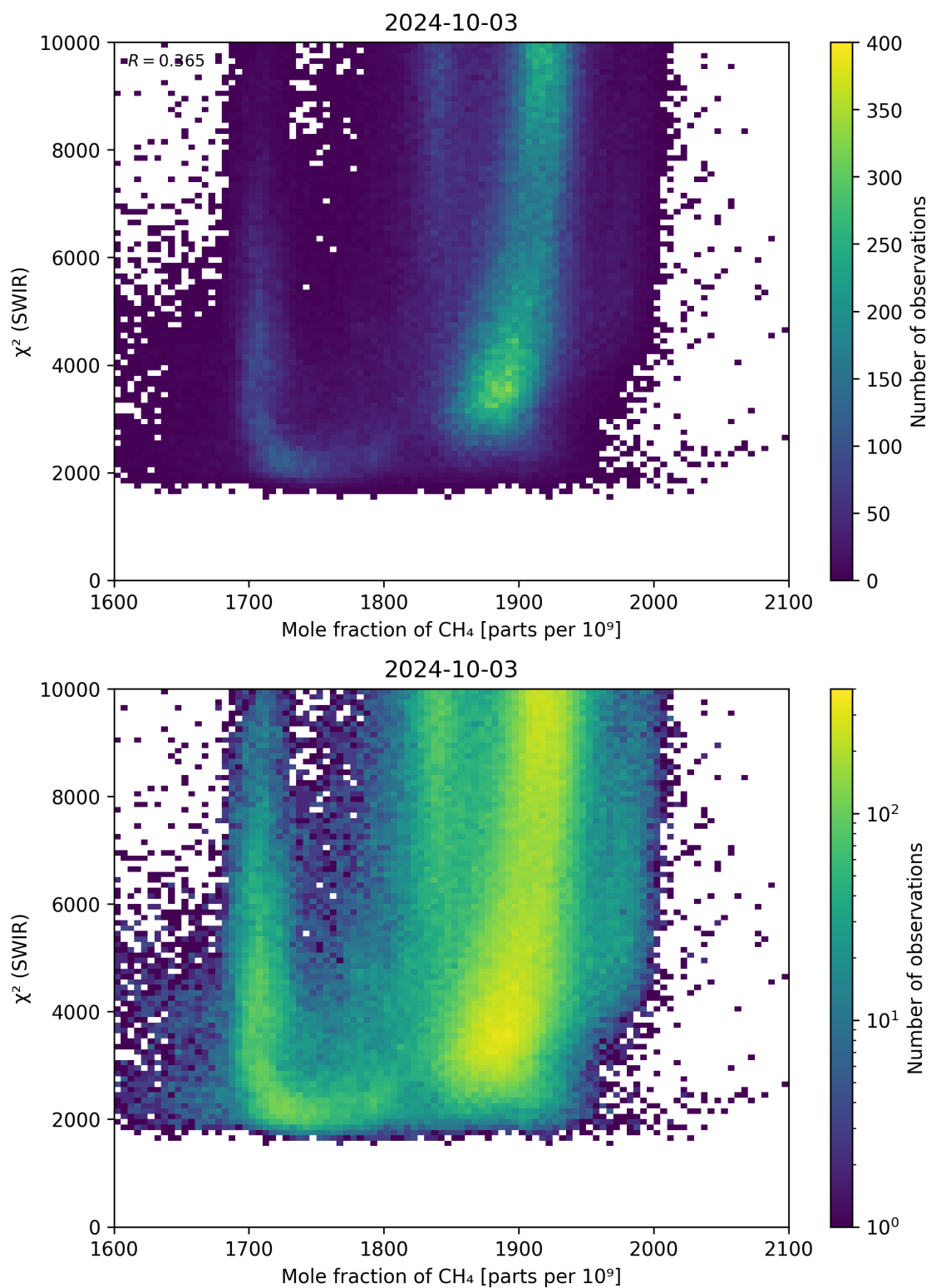
Figure 71: Scatter density plot of “Mole fraction of \text{CH}_4 ” against “ \chi^2 (SWIR)” for 2024-10-03 to 2024-10-04.
