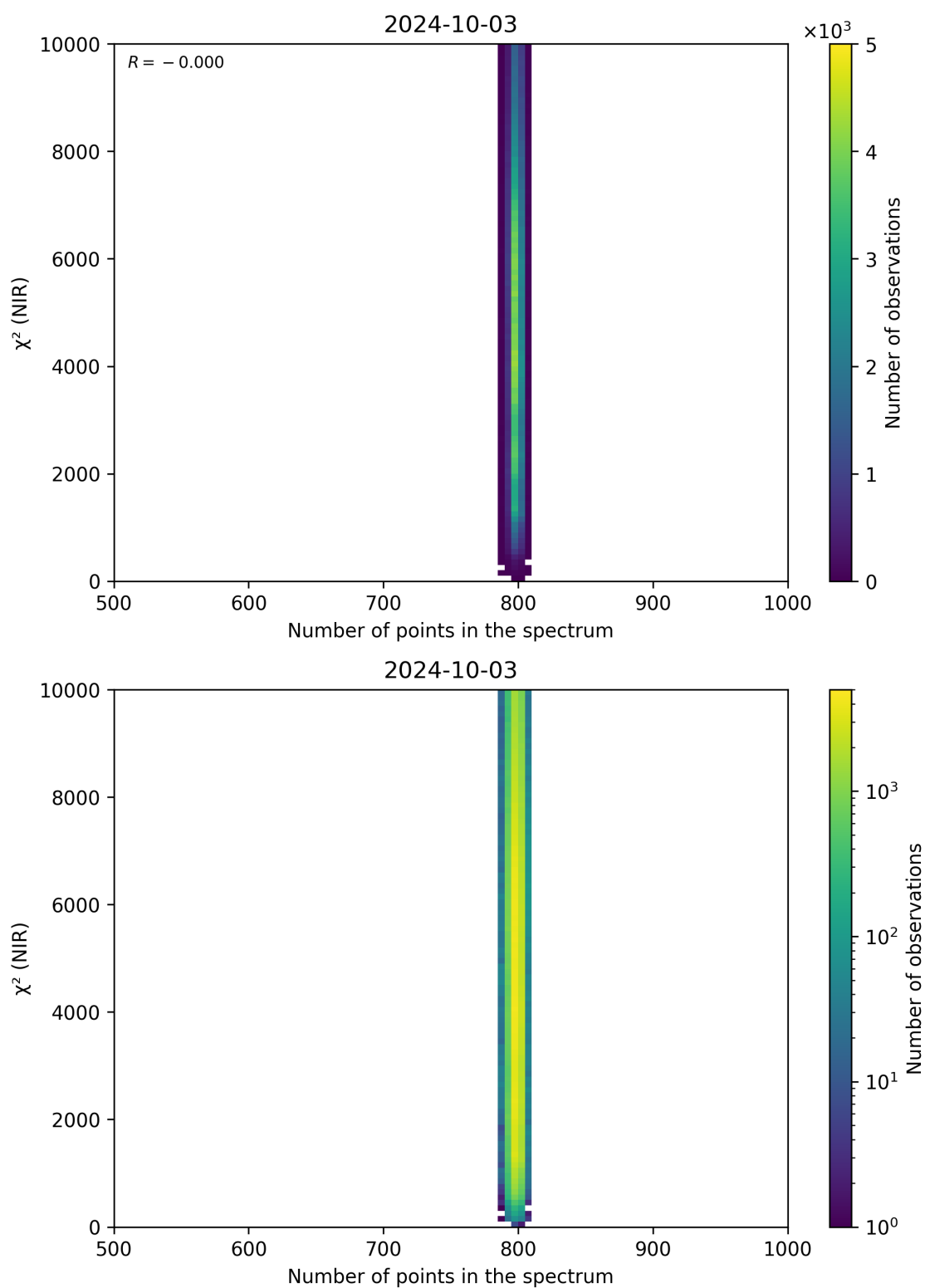
Figure 88: Scatter density plot of “Number of points in the spectrum” against “ \chi^2 (NIR)” for 2024-10-03 to 2024-10-04.
