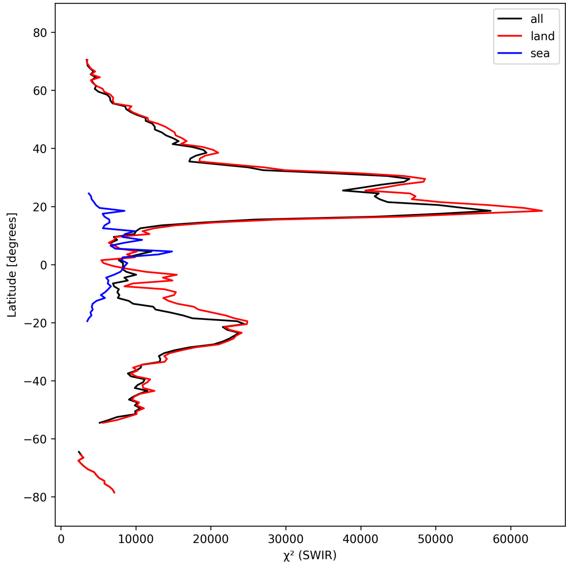
Figure 17: Zonal average of “ \chi^2 (SWIR)” for 2024-10-03 to 2024-10-04.
