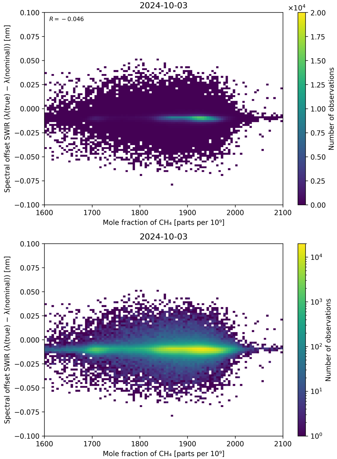
Figure 86: Scatter density plot of “Mole fraction of CH 4 ” against “Spectral offset SWIR ( \lambda_{\text{true}} - \lambda_{\text{nominal}} )” for 2024-10-03 to 2024-10-04.
