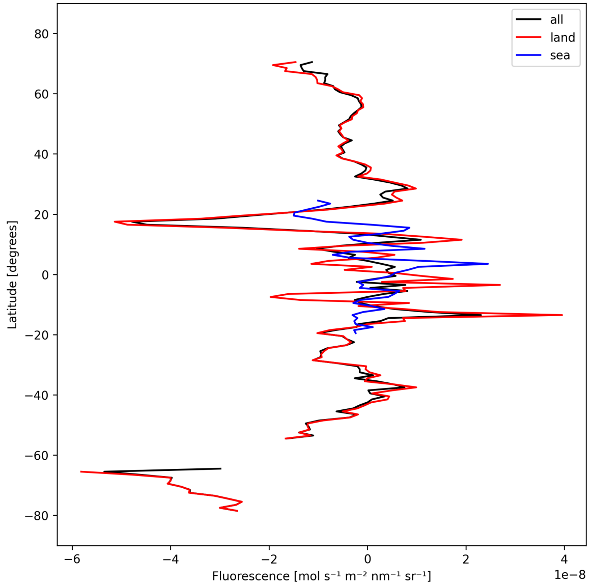
Figure 21: Zonal average of “Fluorescence” for 2024-10-03 to 2024-10-04.
