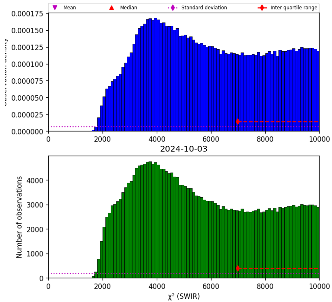
Figure 28: Histogram of “ \chi^2 (SWIR)” for 2024-10-03 to 2024-10-04
