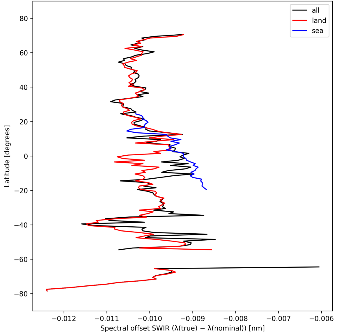
Figure 16: Zonal average of “Spectral offset SWIR ( \lambda_{\text{true}} - \lambda_{\text{nominal}} )” for 2024-10-03 to 2024-10-04.
