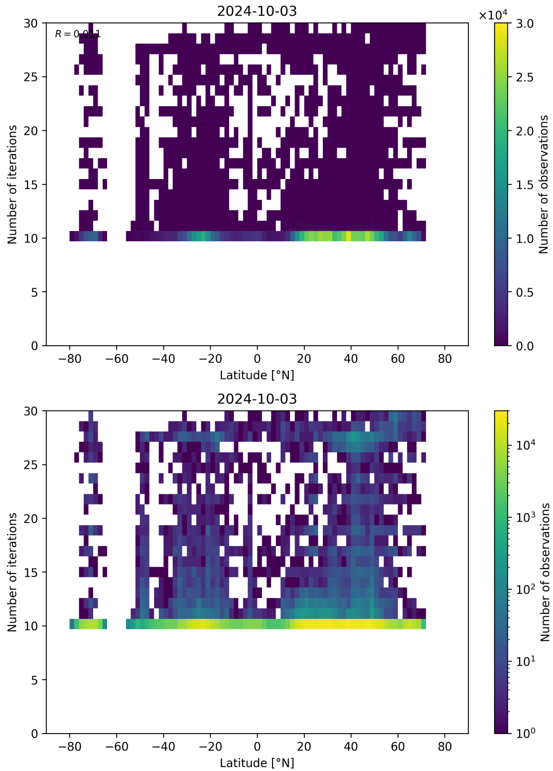
Figure 60: Scatter density plot of “Latitude” against “Number of iterations” for 2024-10-03 to 2024-10-04.
