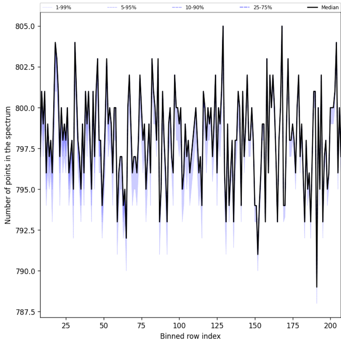
Figure 37: Along track statistics of “Number of points in the spectrum” for 2024-10-03 to 2024-10-04
