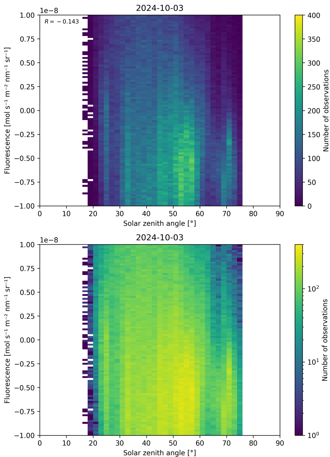
Figure 97: Scatter density plot of “Solar zenith angle” against “Fluorescence” for 2024-10-03 to 2024-10-04.
