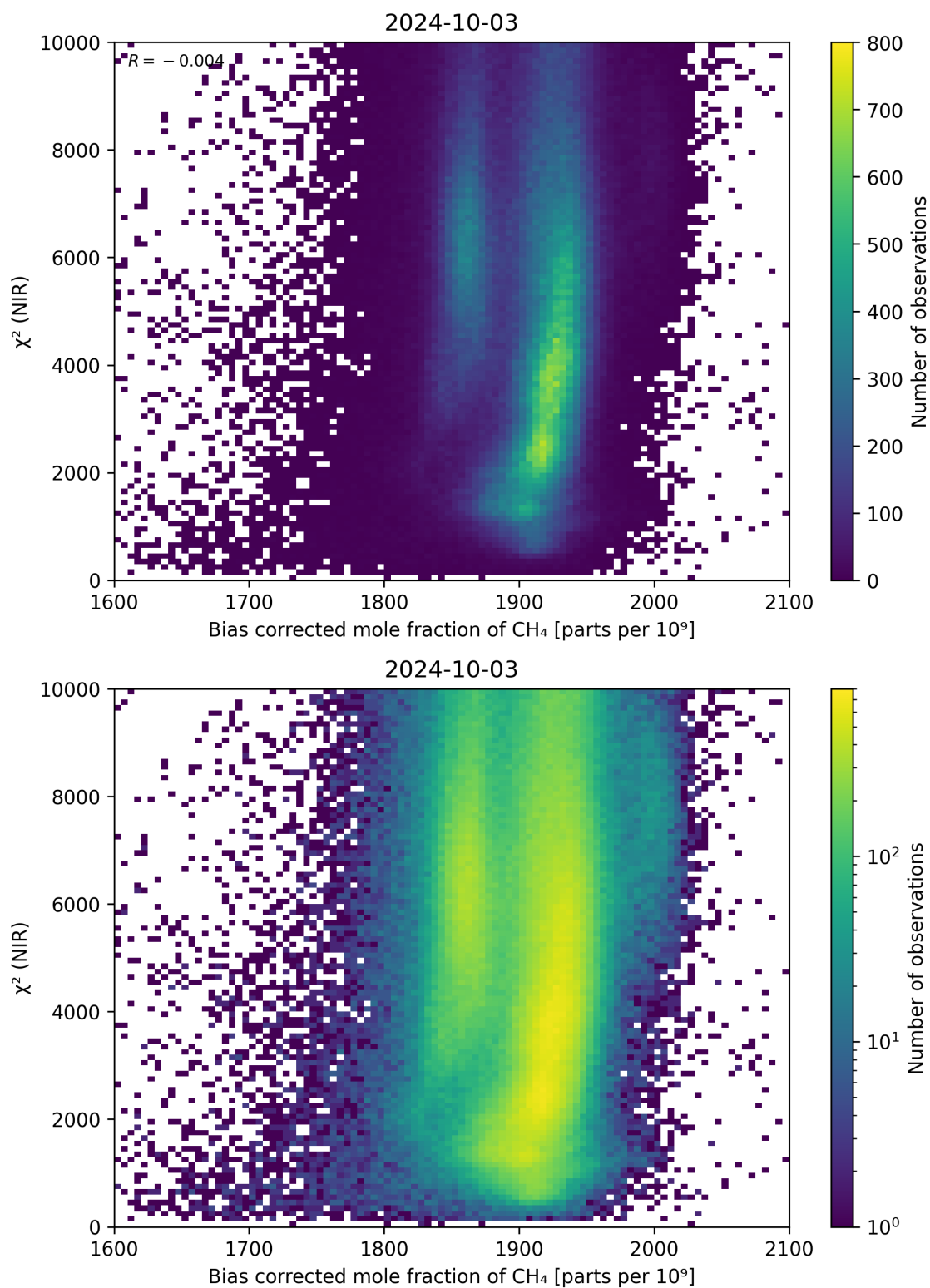
Figure 63: Scatter density plot of “Bias corrected mole fraction of CH 4 ” against “ \chi^2 (NIR)” for 2024-10-03 to 2024-10-04.
