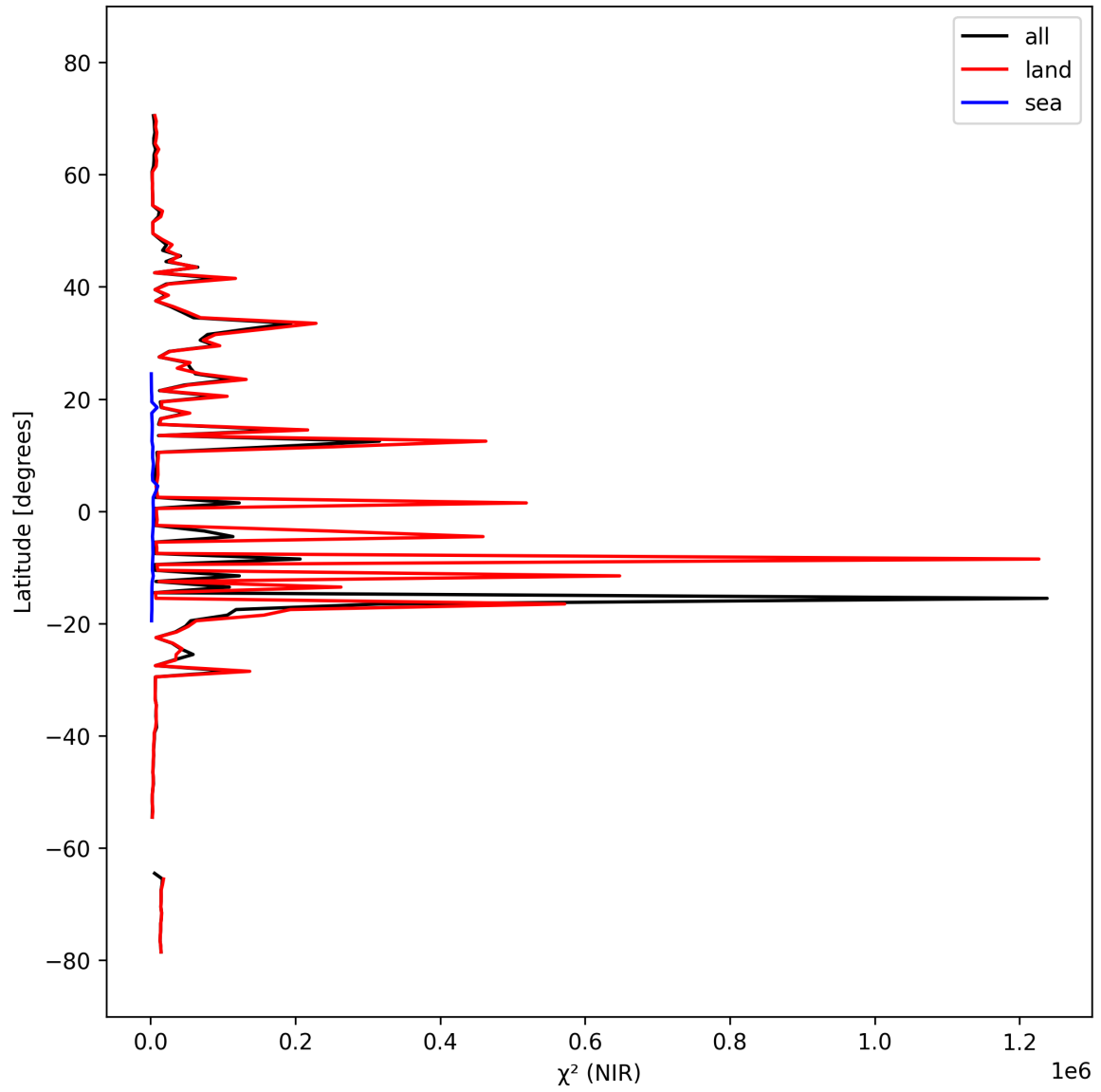
Figure 18: Zonal average of “ \chi^2 (NIR)” for 2024-10-03 to 2024-10-04.
