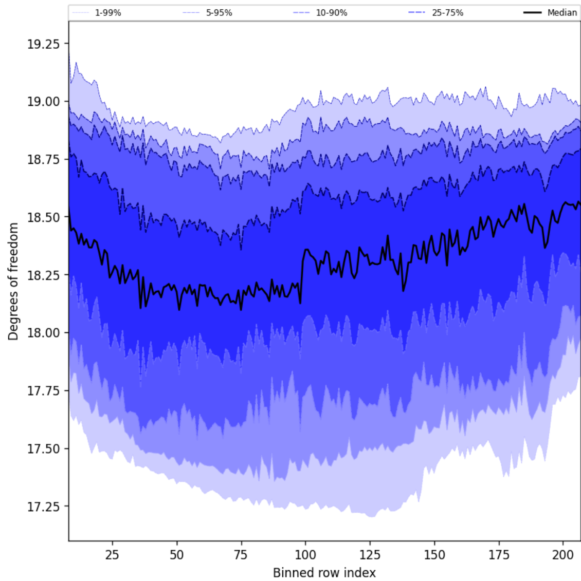
Figure 41: Along track statistics of “Degrees of freedom” for 2024-10-03 to 2024-10-04
