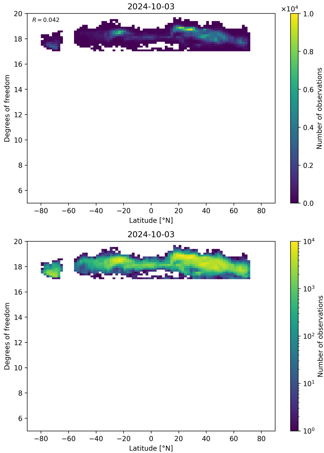
Figure 55: Scatter density plot of “Latitude” against “Degrees of freedom” for 2024-10-03 to 2024-10-04.
