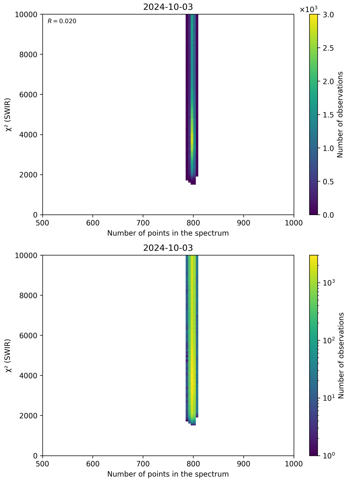
Figure 89: Scatter density plot of “Number of points in the spectrum” against “ \chi^2 (SWIR)” for 2024-10-03 to 2024-10-04.
