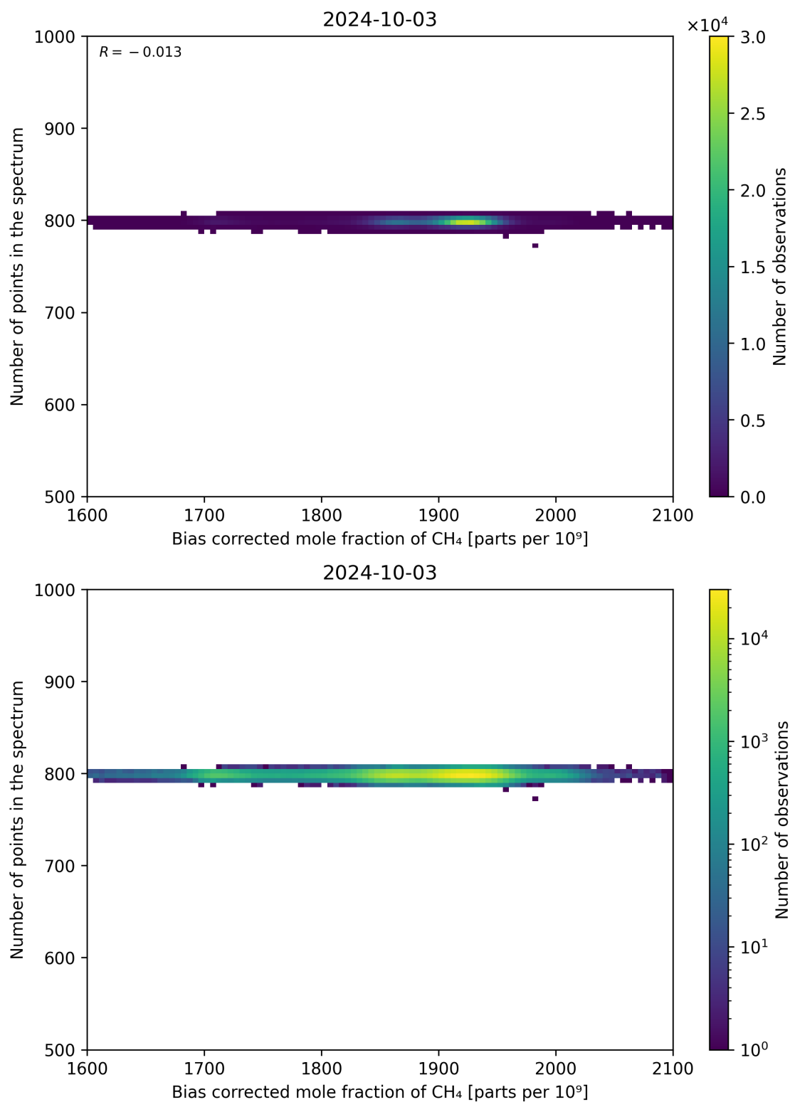
Figure 68: Scatter density plot of “Bias corrected mole fraction of CH 4 ” against “Number of points in the spectrum” for 2024-10-03 to 2024-10-04.
