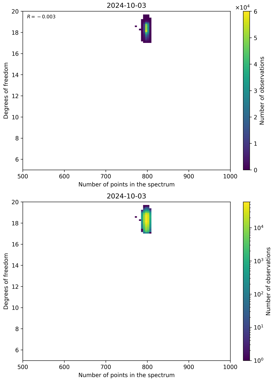
Figure 90: Scatter density plot of “Number of points in the spectrum” against “Degrees of freedom” for 2024-10-03 to 2024-10-04.
