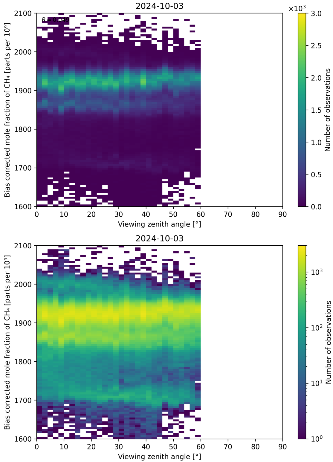
Figure 111: Scatter density plot of “Viewing zenith angle” against “Bias corrected mole fraction of CH 4 ” for 2024-10-03 to 2024-10-04.
