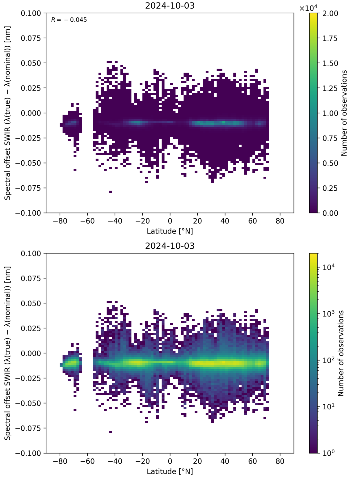
Figure 62: Scatter density plot of “Latitude” against “Spectral offset SWIR ( \lambda_{\text{true}} - \lambda_{\text{nominal}} )” for 2024-10-03 to 2024-10-04.
