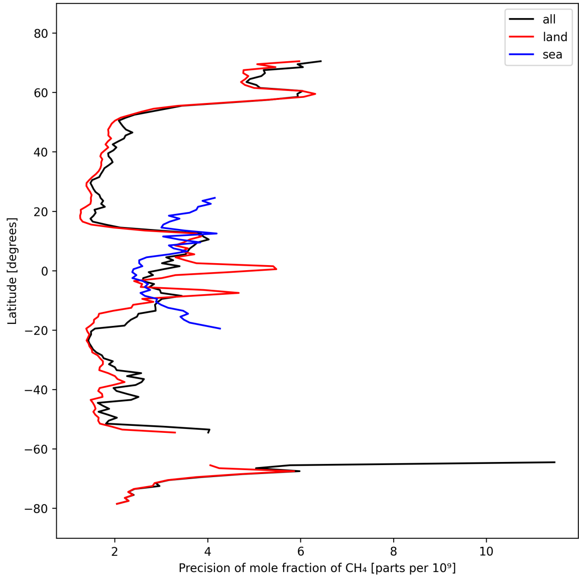
Figure 13: Zonal average of “Precision of mole fraction of CH 4 ” for 2024-10-03 to 2024-10-04.
