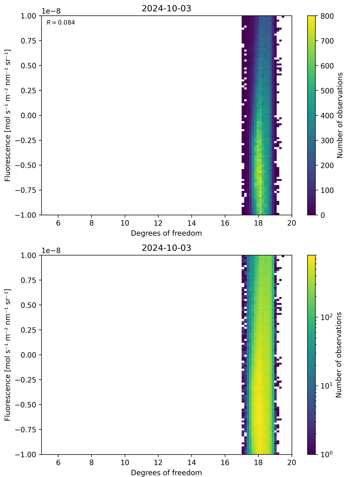
Figure 51: Scatter density plot of “Degrees of freedom” against “Fluorescence” for 2024-10-03 to 2024-10-04.
