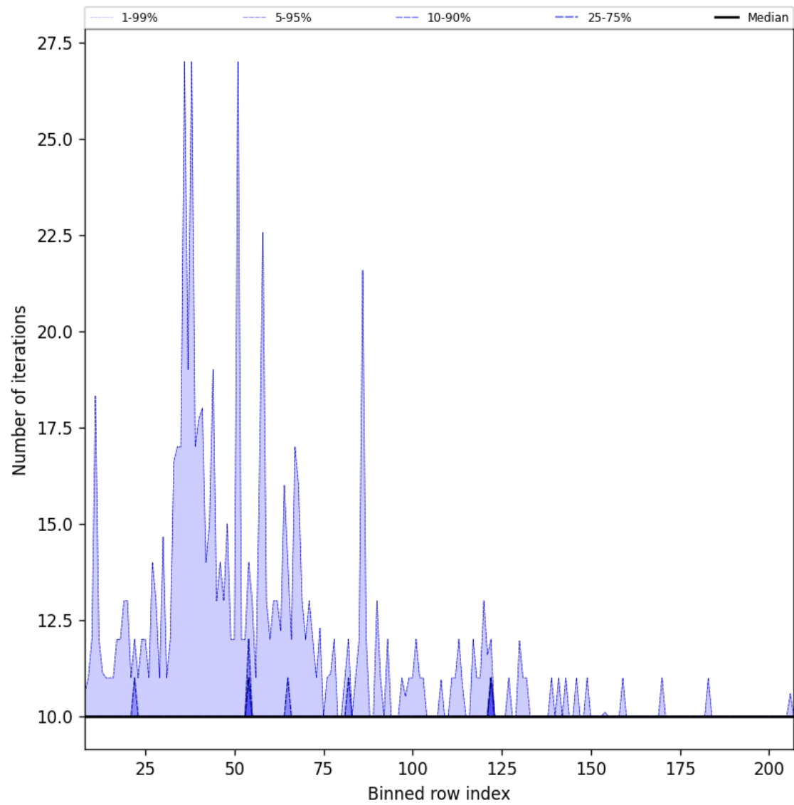
Figure 42: Along track statistics of “Number of iterations” for 2024-10-03 to 2024-10-04
