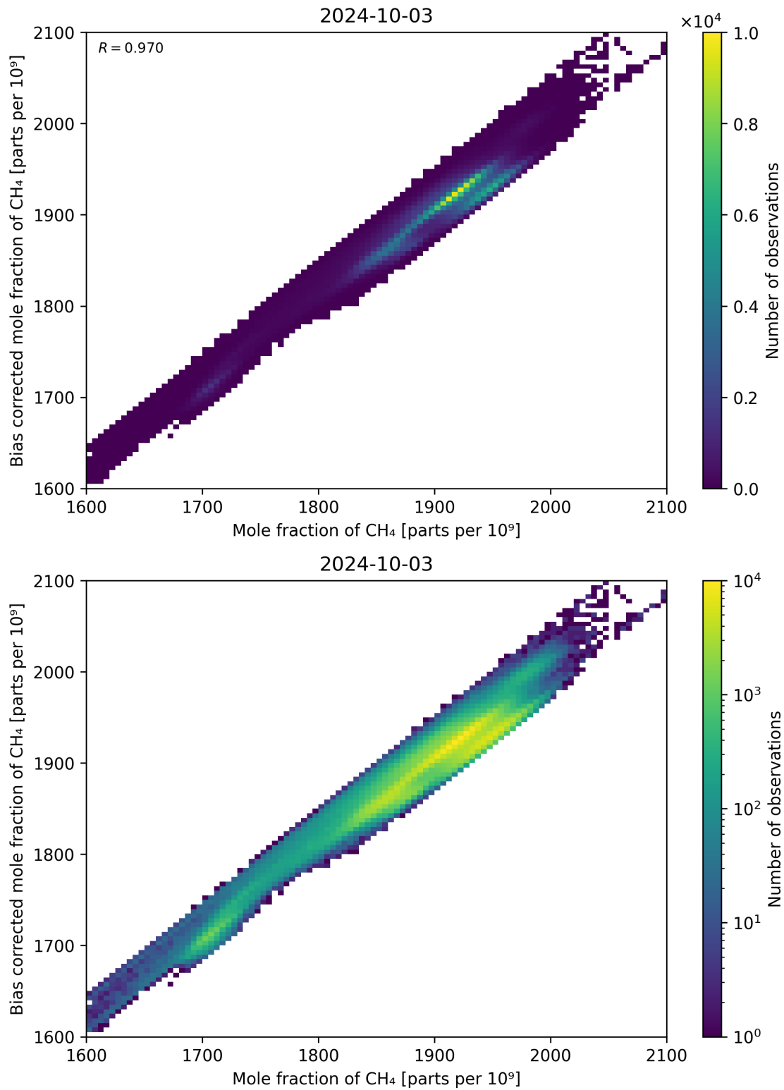
Figure 74: Scatter density plot of “Mole fraction of CH 4 ” against “Bias corrected mole fraction of CH 4 ” for 2024-10-03 to 2024-10-04.
