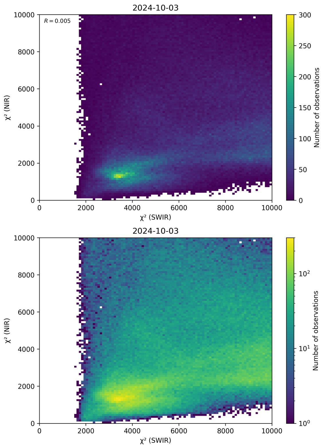
Figure 47: Scatter density plot of “ \chi^2 (SWIR)” against “ \chi^2 (NIR)” for 2024-10-03 to 2024-10-04.
