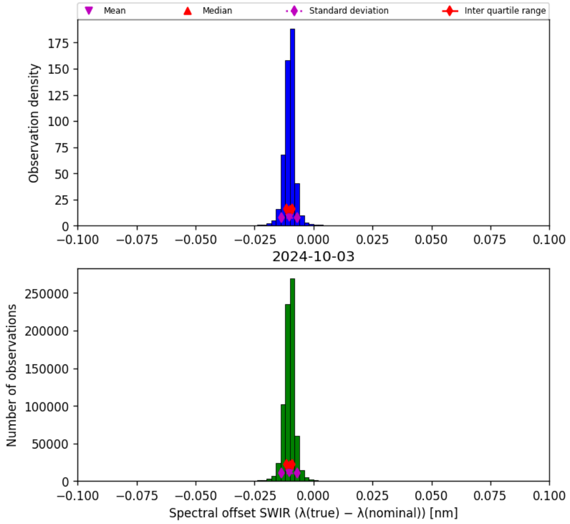
Figure 27: Histogram of “Spectral offset SWIR ( \lambda_{\text{true}} - \lambda_{\text{nominal}} )” for 2024-10-03 to 2024-10-04
