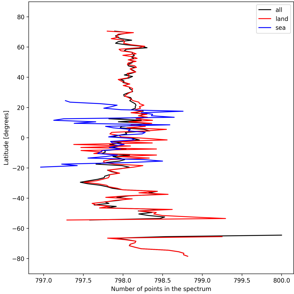
Figure 15: Zonal average of “Number of points in the spectrum” for 2024-10-03 to 2024-10-04.
