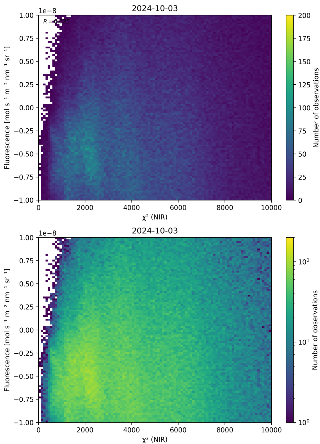
Figure 45: Scatter density plot of “ \chi^2 (NIR)” against “Fluorescence” for 2024-10-03 to 2024-10-04.
