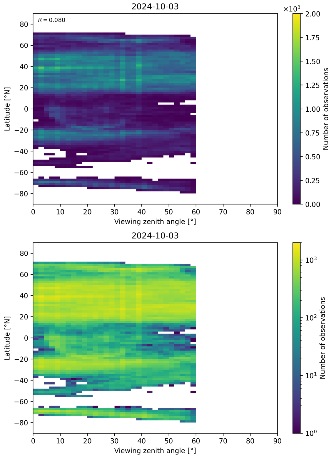
Figure 109: Scatter density plot of “Viewing zenith angle” against “Latitude” for 2024-10-03 to 2024-10-04.
