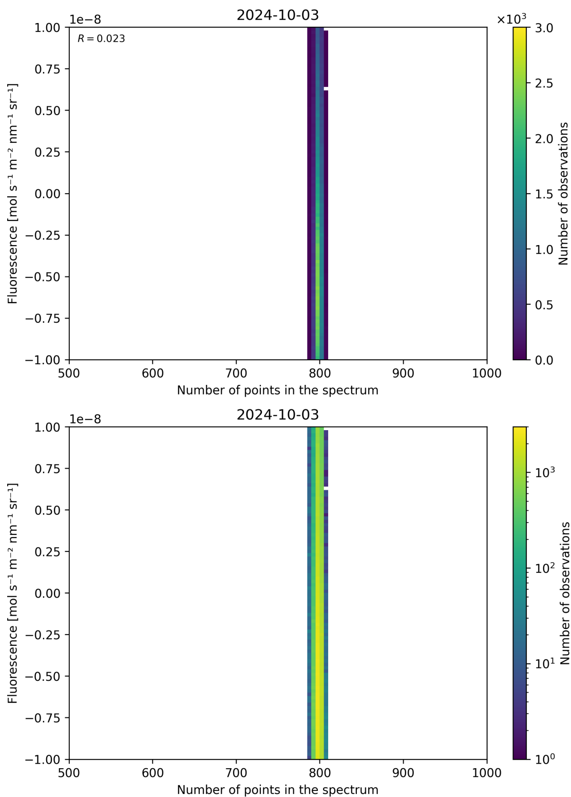
Figure 91: Scatter density plot of “Number of points in the spectrum” against “Fluorescence” for 2024-10-03 to 2024-10-04.
