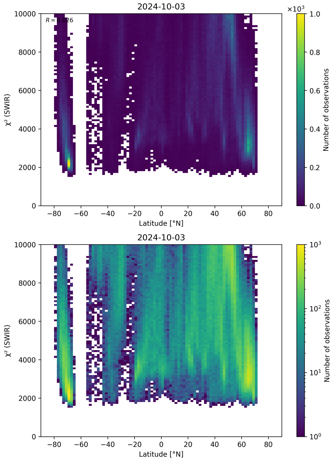
Figure 54: Scatter density plot of “Latitude” against “ \chi^2 (SWIR)” for 2024-10-03 to 2024-10-04.
