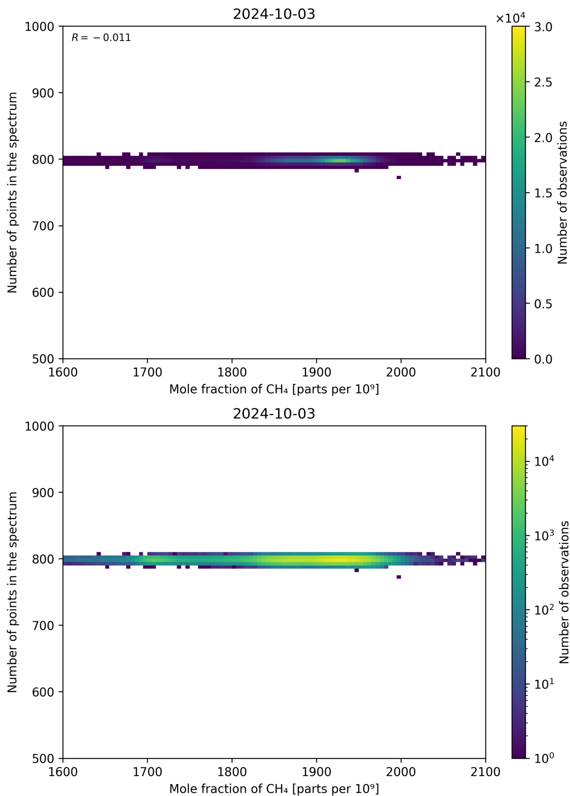
Figure 77: Scatter density plot of “Mole fraction of CH 4 ” against “Number of points in the spectrum” for 2024-10-03 to 2024-10-04.
