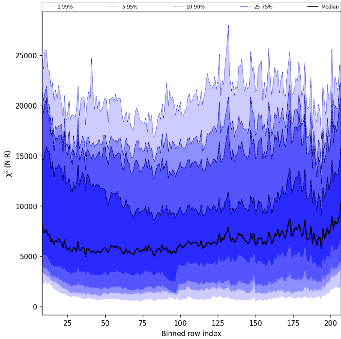
Figure 40: Along track statistics of " \chi^2 (NIR)" for 2024-10-03 to 2024-10-04
