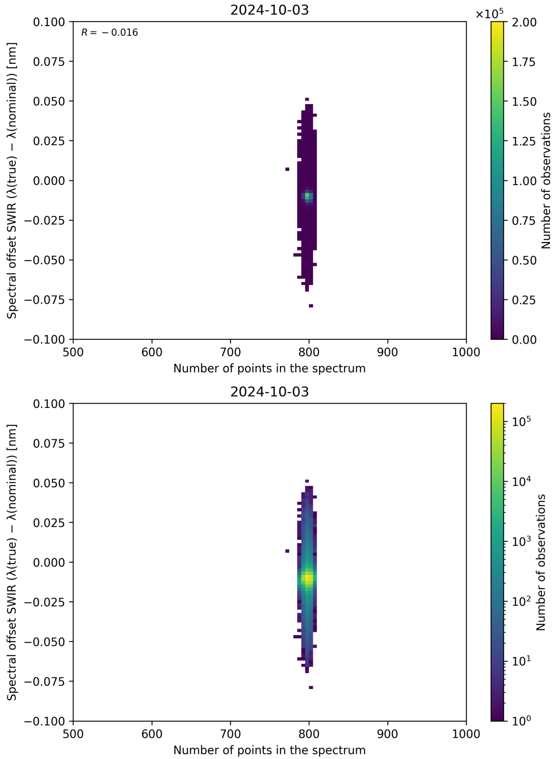
Figure 93: Scatter density plot of “Number of points in the spectrum” against “Spectral offset SWIR ( \lambda_{\text{true}} - \lambda_{\text{nominal}} )” for 2024-10-03 to 2024-10-04.
