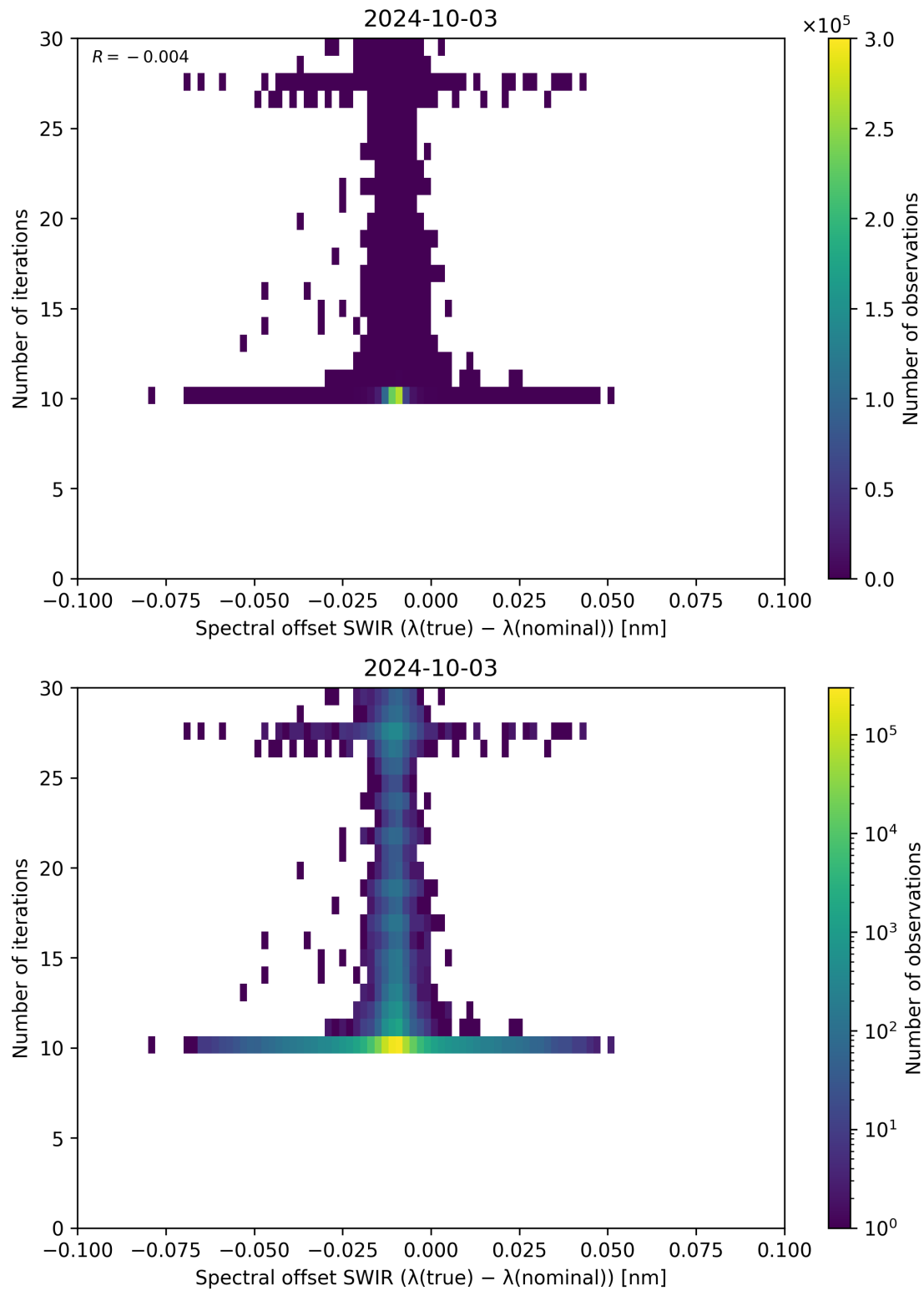
Figure 121: Scatter density plot of “Spectral offset SWIR ( \lambda_{\text{true}} - \lambda_{\text{nominal}} )” against “Number of iterations” for 2024-10-03 to 2024-10-04.
