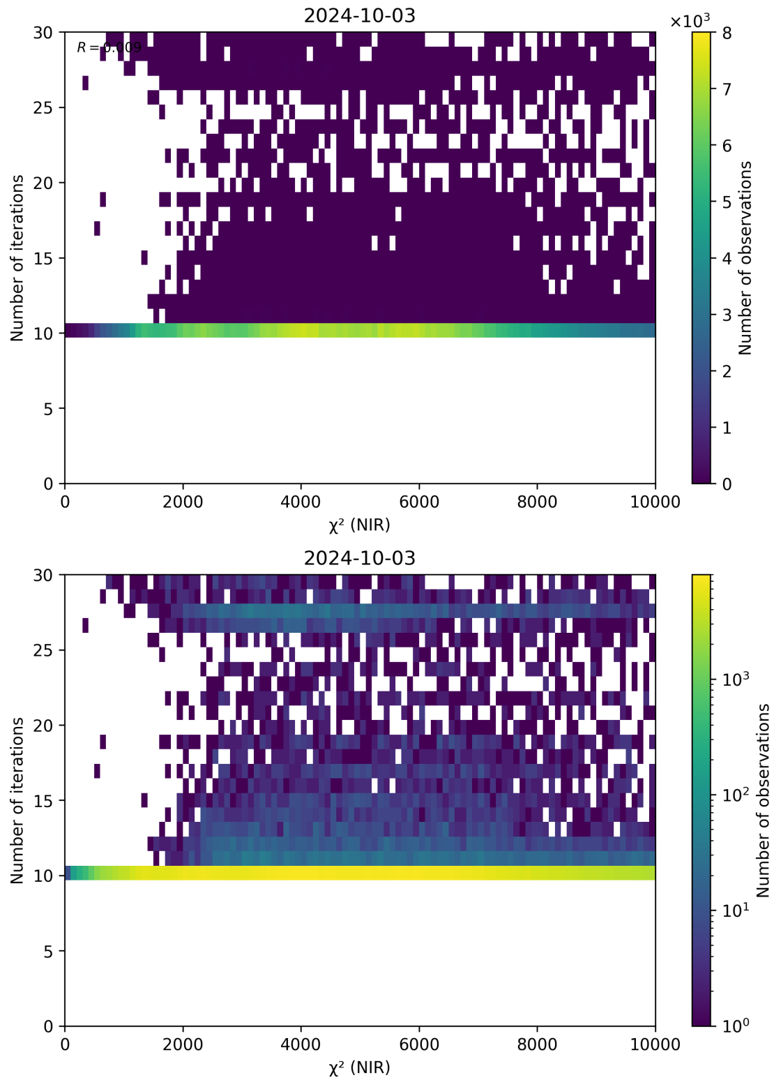
Figure 46: Scatter density plot of “ \chi^2 (NIR)” against “Number of iterations” for 2024-10-03 to 2024-10-04.
