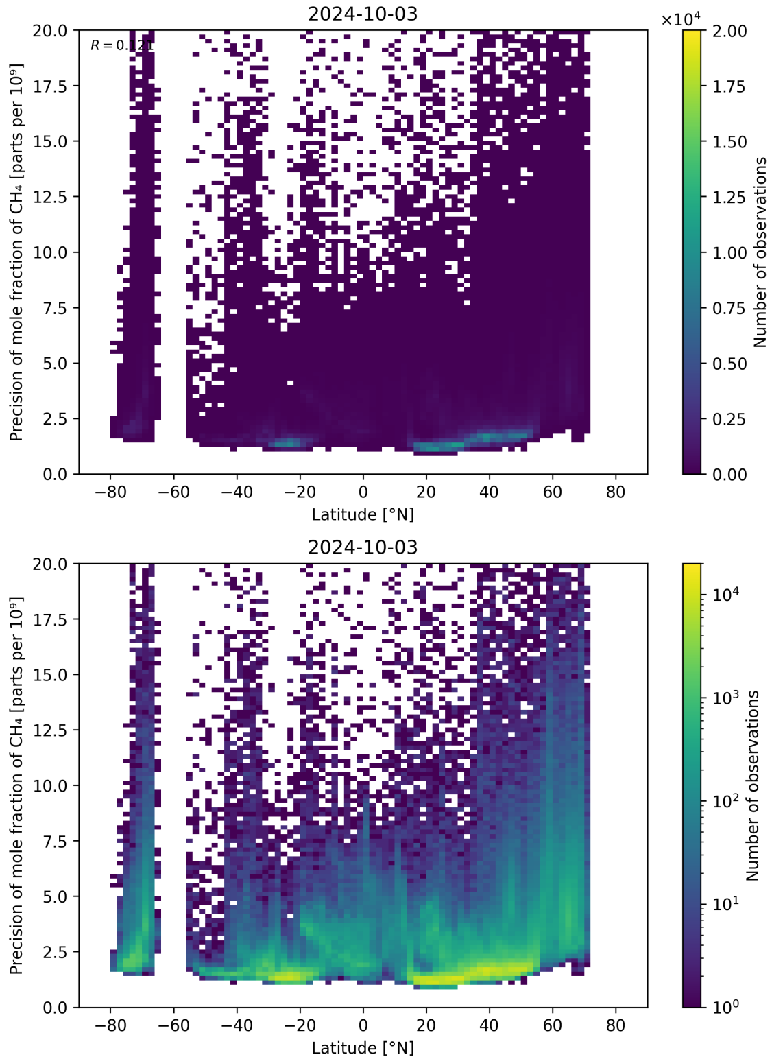
Figure 59: Scatter density plot of “Latitude” against “Precision of mole fraction of CH 4 ” for 2024-10-03 to 2024-10-04.
