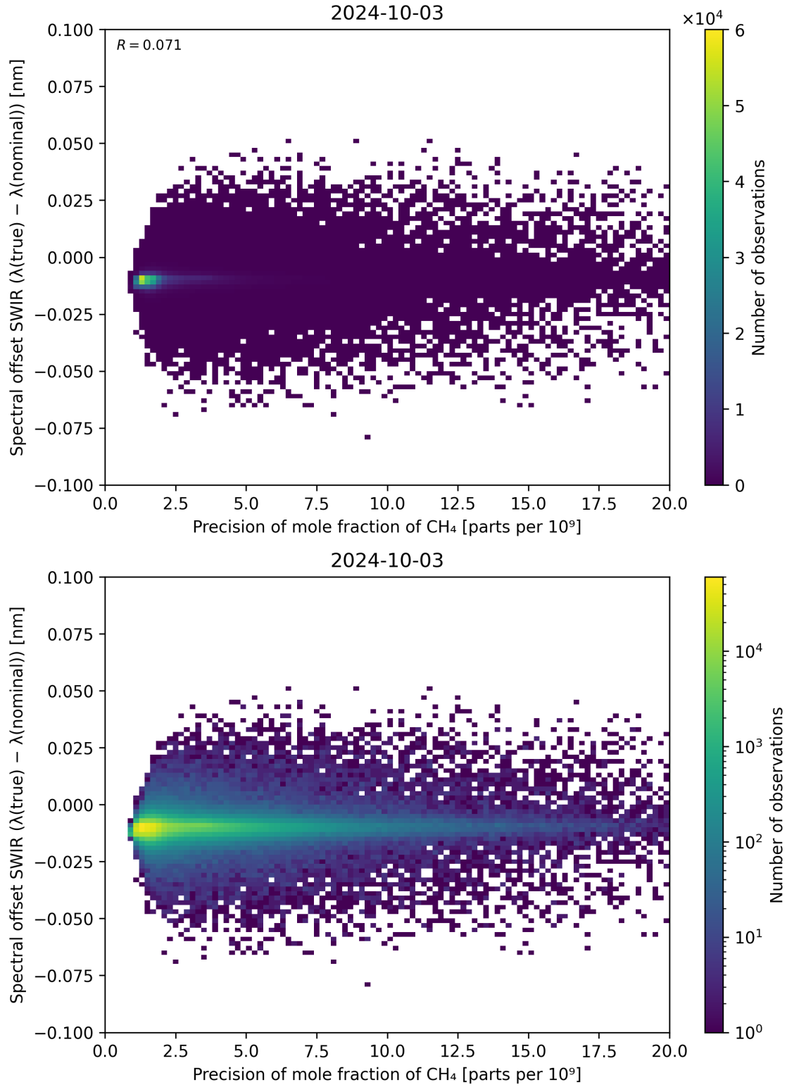
Figure 85: Scatter density plot of “Precision of mole fraction of CH 4 ” against “Spectral offset SWIR ( \lambda_{\text{true}} - \lambda_{\text{nominal}} )” for 2024-10-03 to 2024-10-04.
