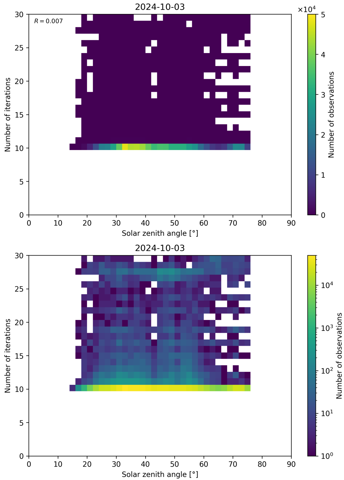
Figure 102: Scatter density plot of “Solar zenith angle” against “Number of iterations” for 2024-10-03 to 2024-10-04.
