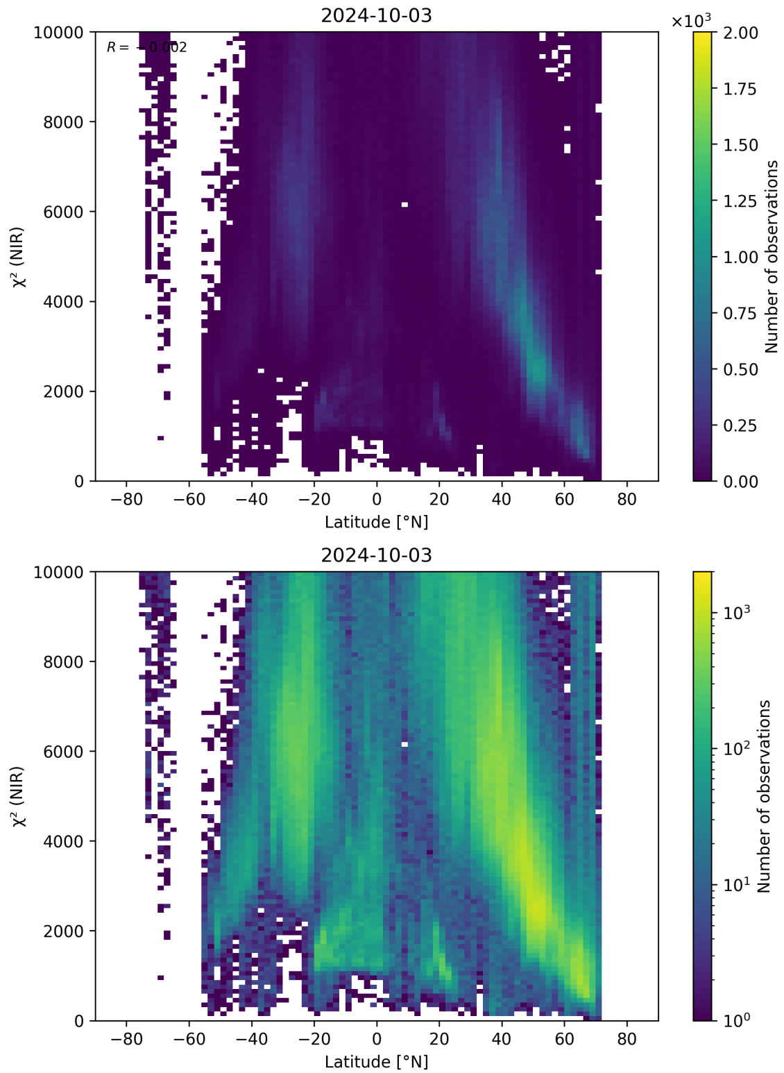
Figure 53: Scatter density plot of “Latitude” against “ \chi^2 (NIR)” for 2024-10-03 to 2024-10-04.
