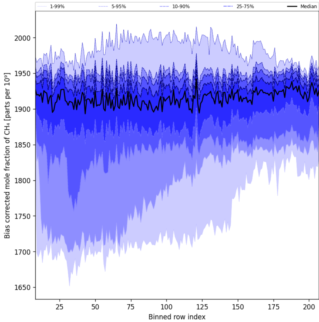
Figure 36: Along track statistics of “Bias corrected mole fraction of CH 4 ” for 2024-10-03 to 2024-10-04
