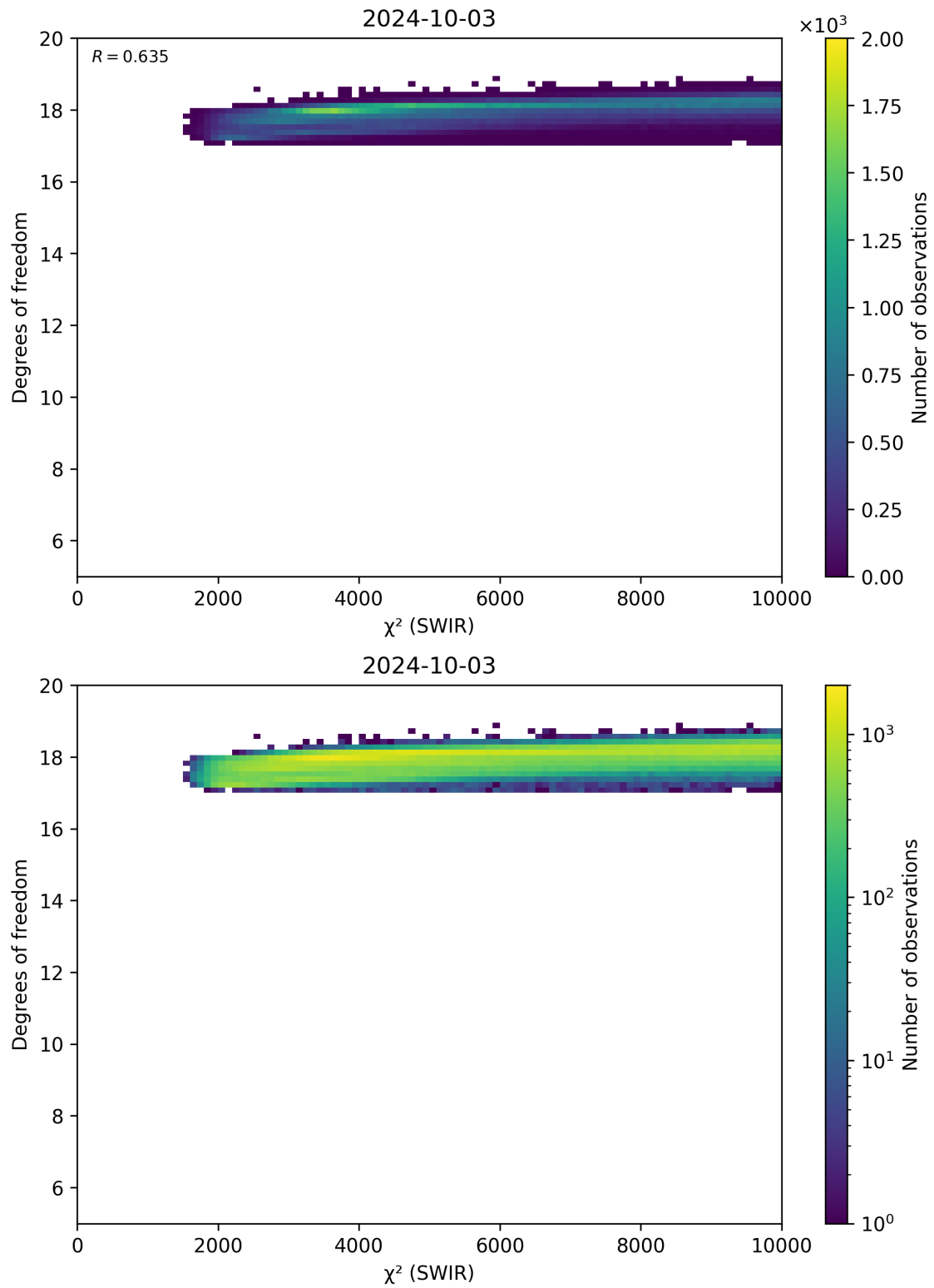
Figure 48: Scatter density plot of “ \chi^2 (SWIR)” against “Degrees of freedom” for 2024-10-03 to 2024-10-04.
