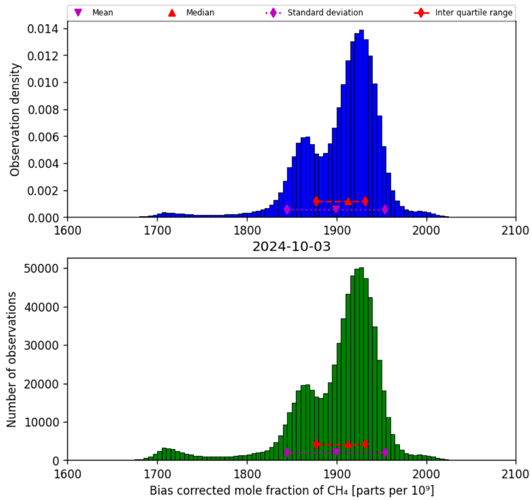
Figure 25: Histogram of “Bias corrected mole fraction of CH 4 ” for 2024-10-03 to 2024-10-04
