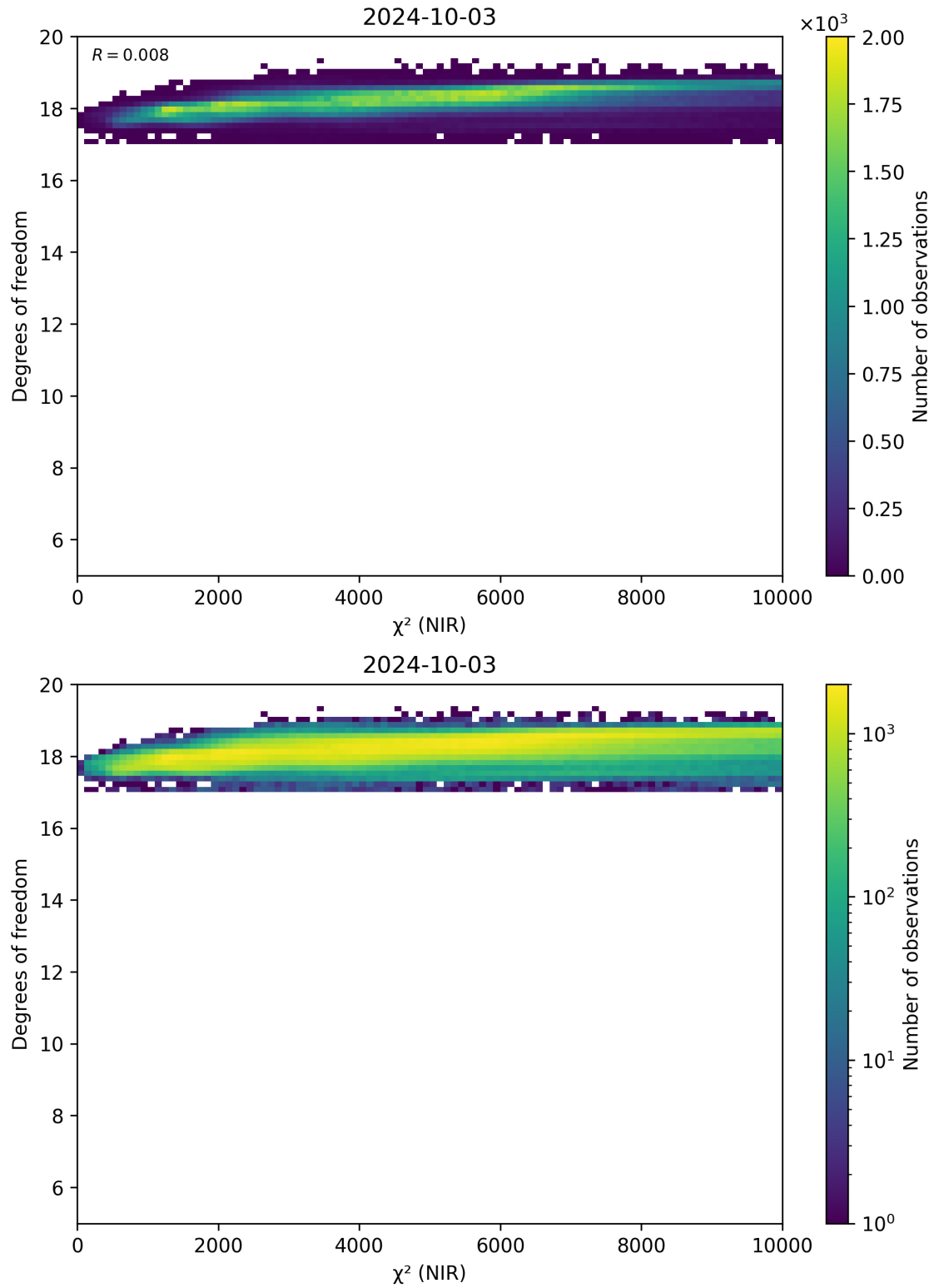
Figure 44: Scatter density plot of “ \chi^2 (NIR)” against “Degrees of freedom” for 2024-10-03 to 2024-10-04.
