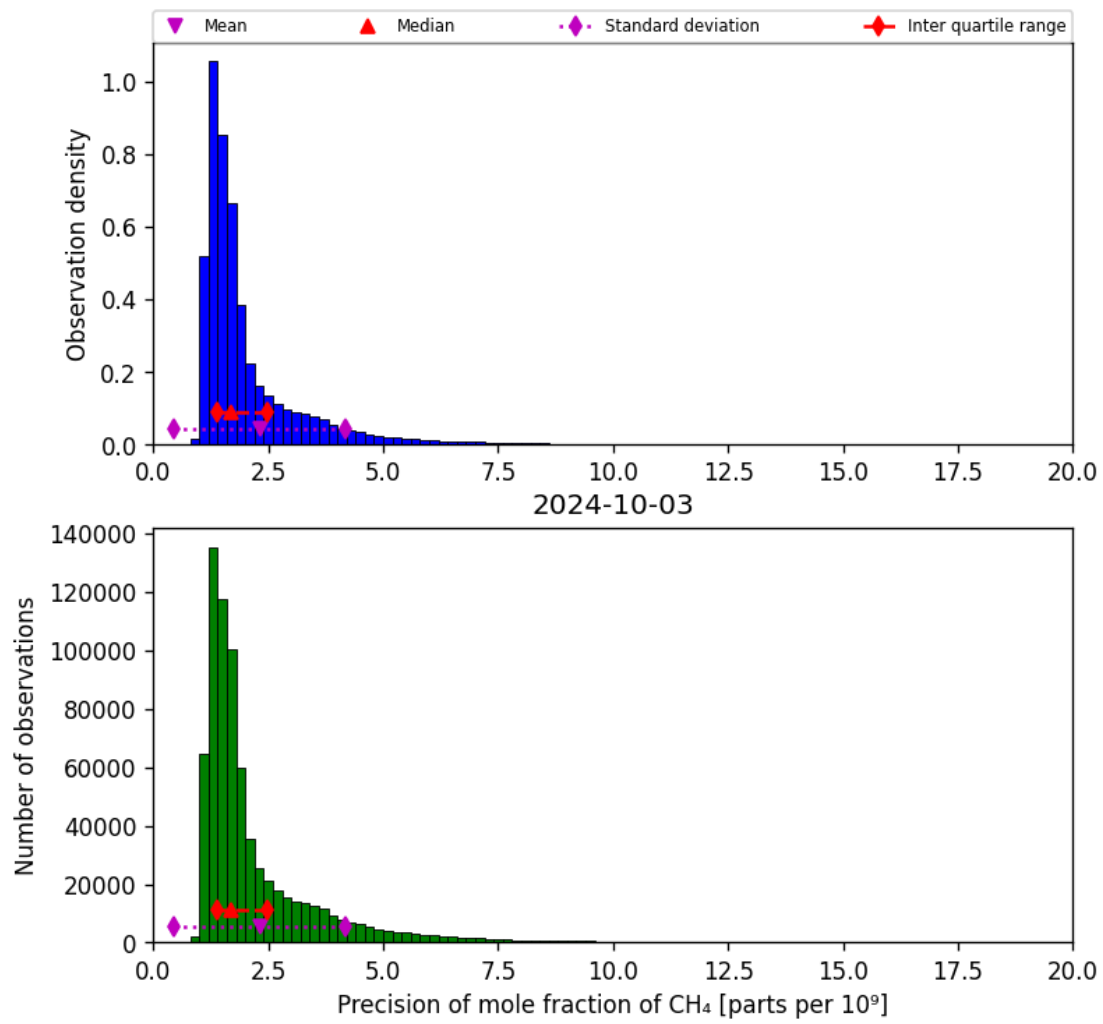
Figure 24: Histogram of “Precision of mole fraction of CH 4 ” for 2024-10-03 to 2024-10-04
