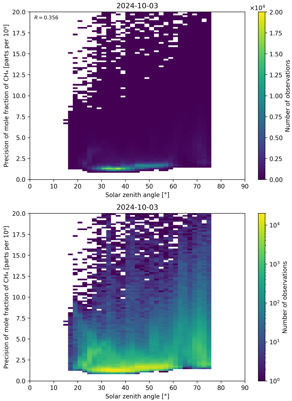
Figure 101: Scatter density plot of “Solar zenith angle” against “Precision of mole fraction of CH 4 ” for 2024-10-03 to 2024-10-04.
