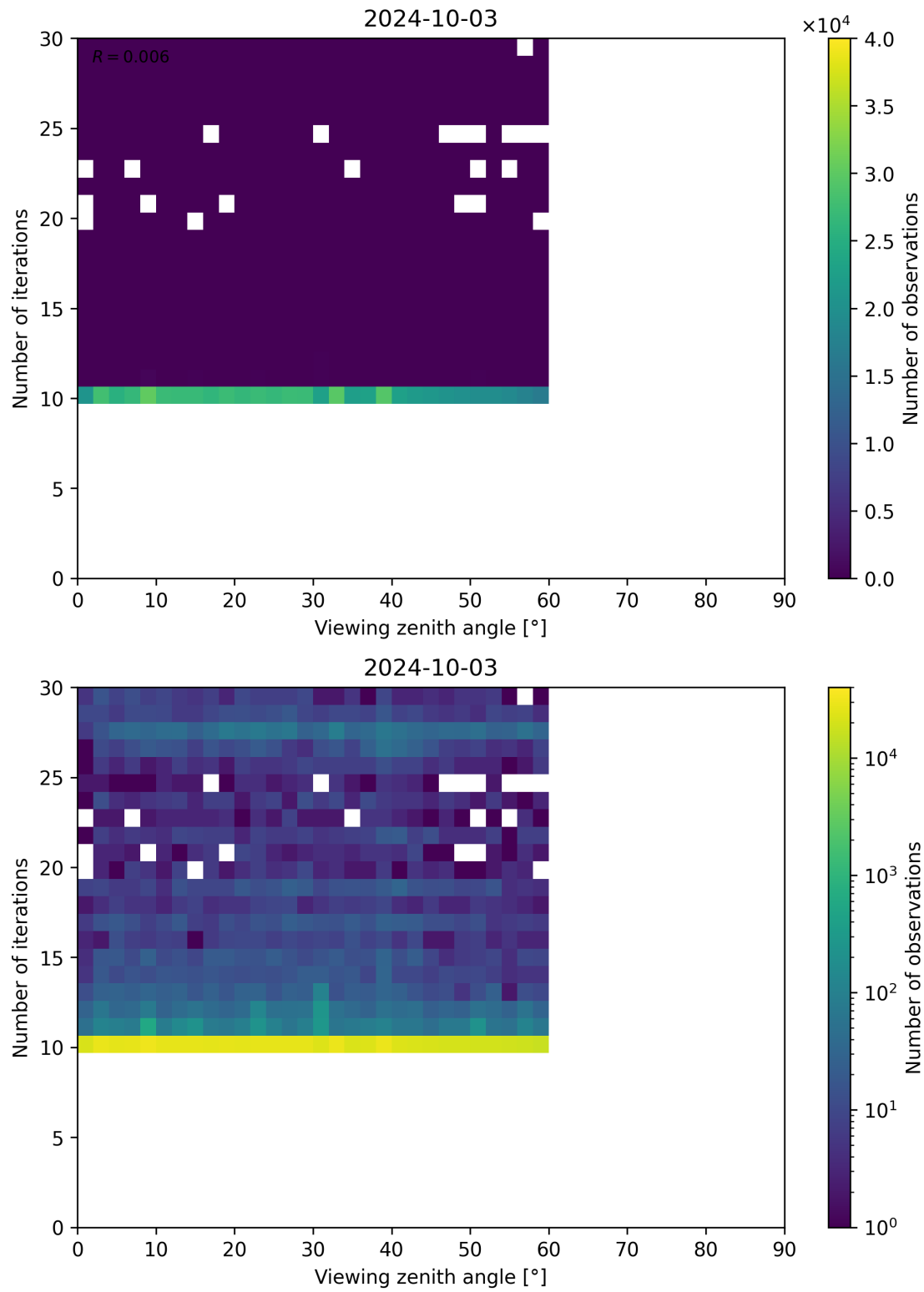
Figure 113: Scatter density plot of “Viewing zenith angle” against “Number of iterations” for 2024-10-03 to 2024-10-04.
