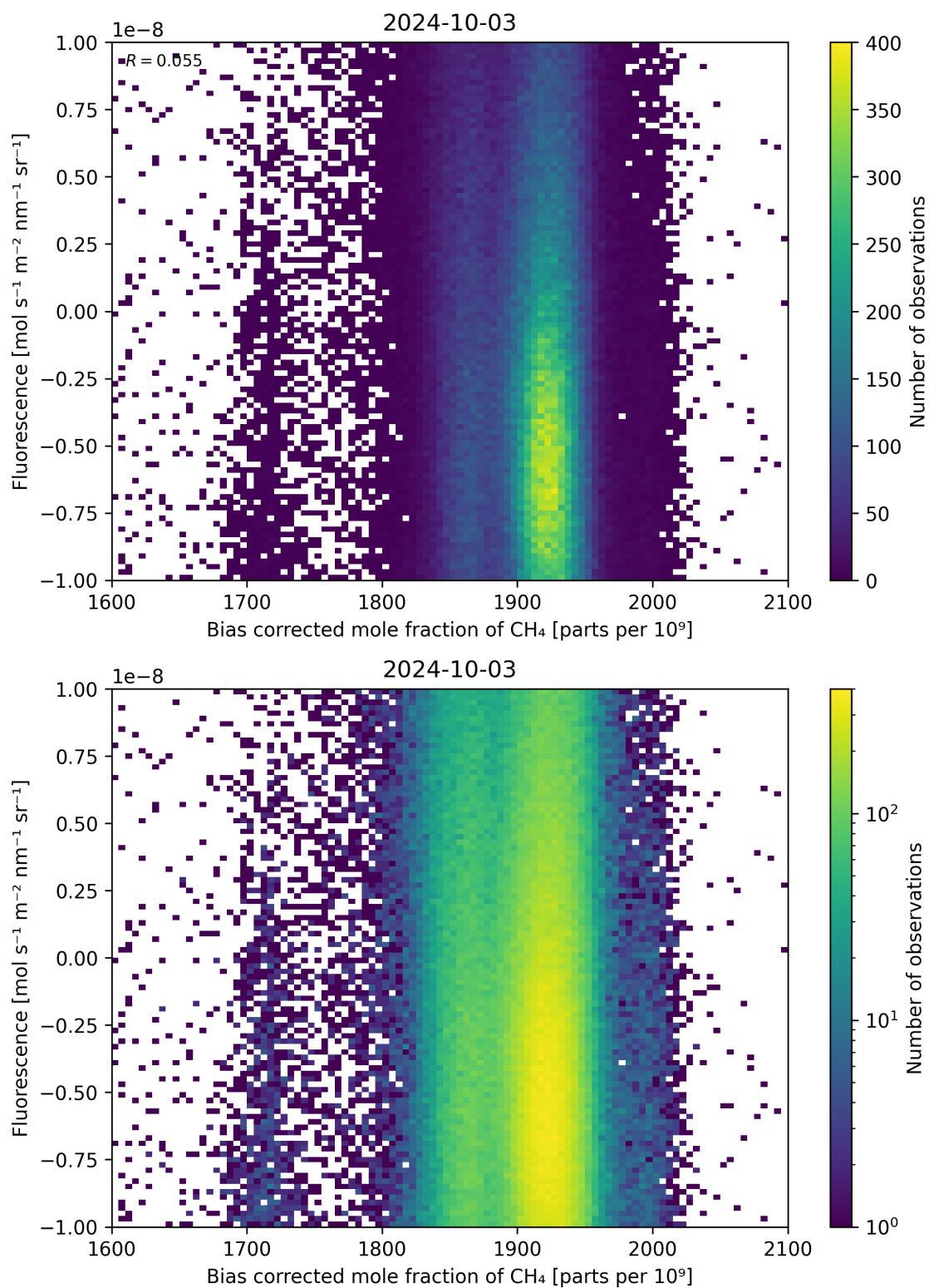
Figure 66: Scatter density plot of “Bias corrected mole fraction of \text{CH}_4 ” against “Fluorescence” for 2024-10-03 to 2024-10-04.
