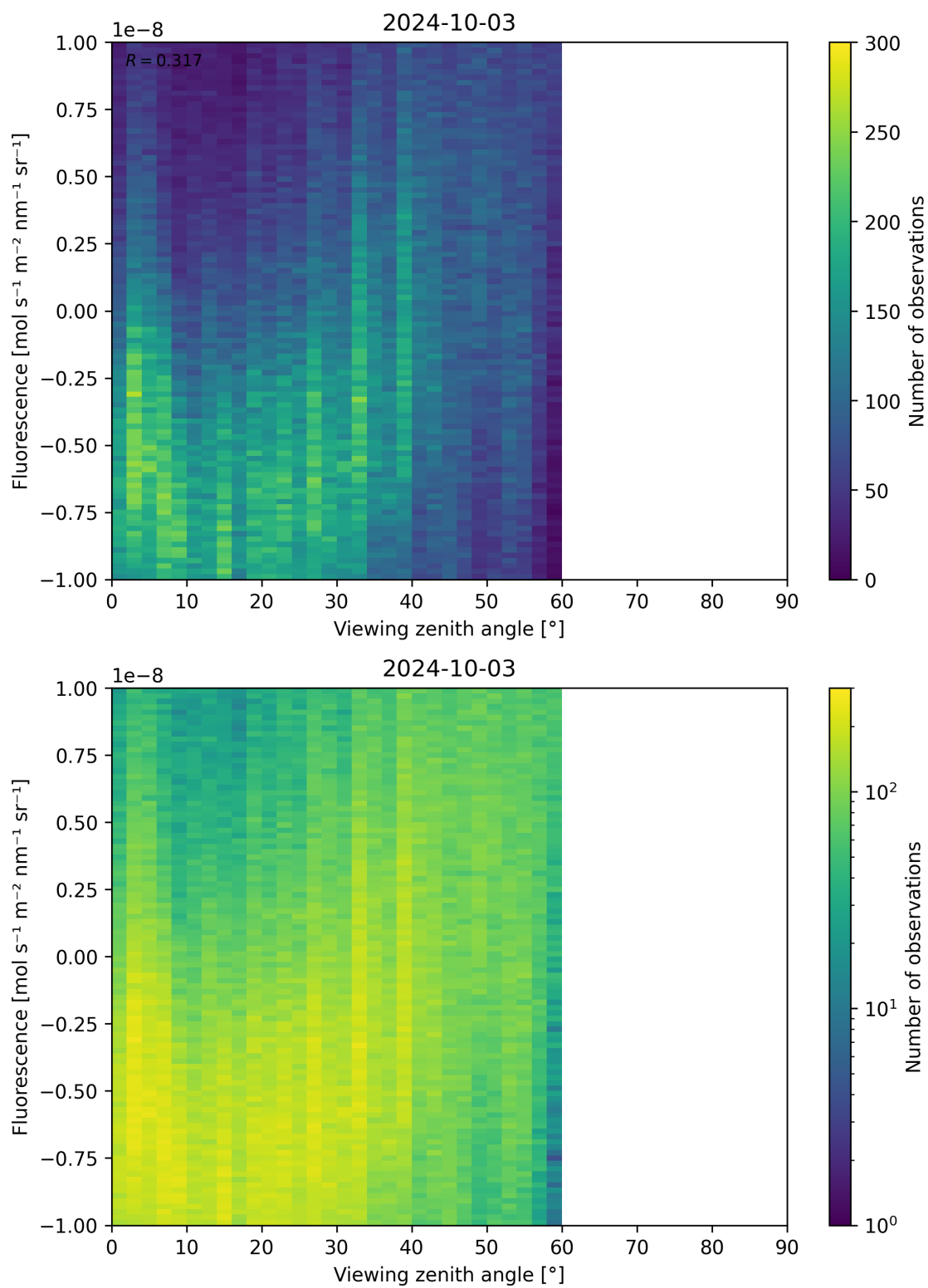
Figure 108: Scatter density plot of “Viewing zenith angle” against “Fluorescence” for 2024-10-03 to 2024-10-04.
