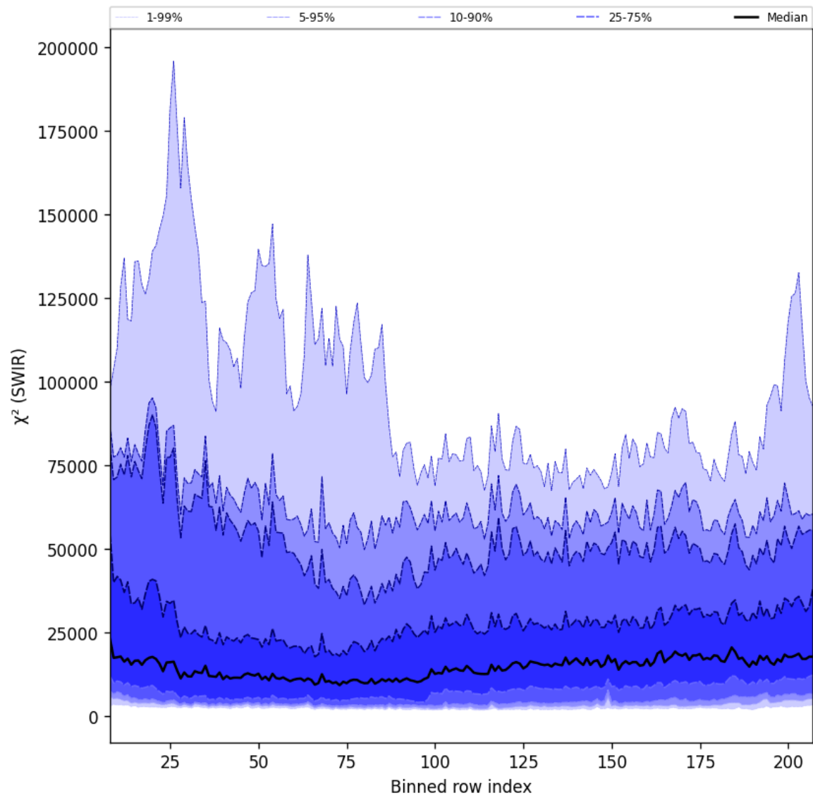
Figure 39: Along track statistics of “ \chi^2 (SWIR)” for 2024-10-03 to 2024-10-04
