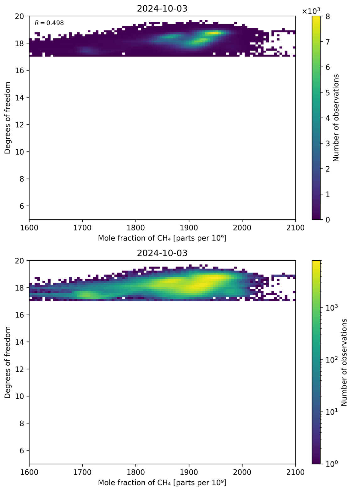
Figure 72: Scatter density plot of “Mole fraction of CH 4 ” against “Degrees of freedom” for 2024-10-03 to 2024-10-04.
