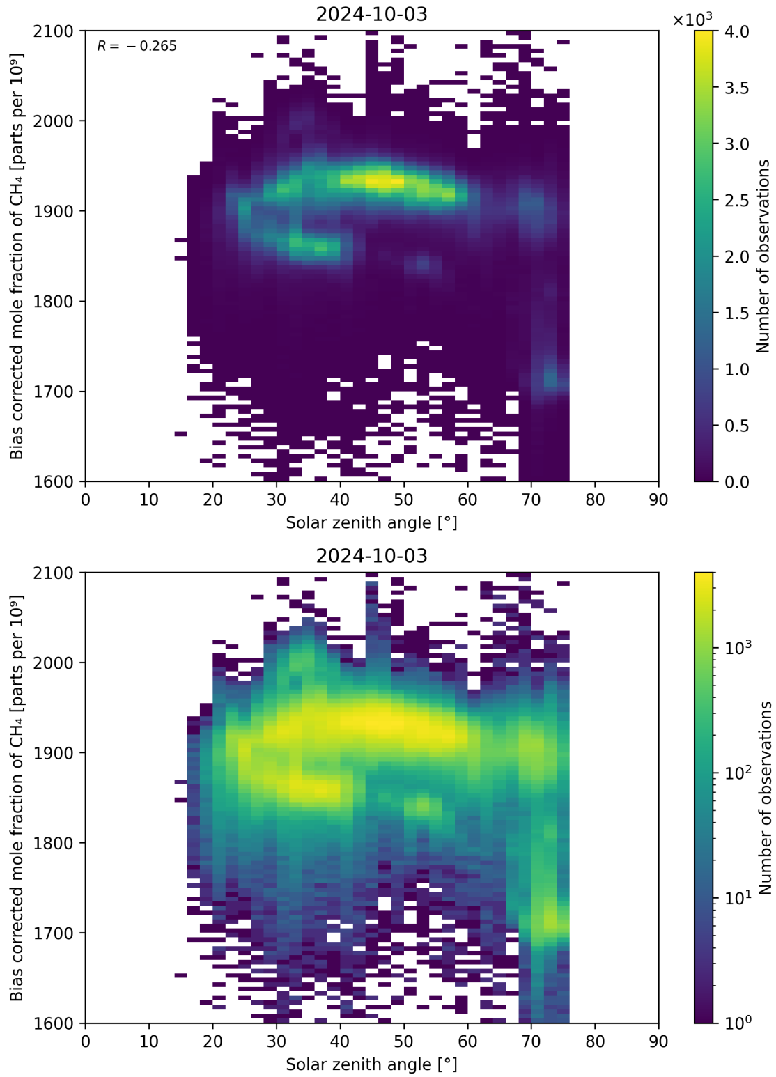
Figure 100: Scatter density plot of “Solar zenith angle” against “Bias corrected mole fraction of \text{CH}_4 ” for 2024-10-03 to 2024-10-04.
