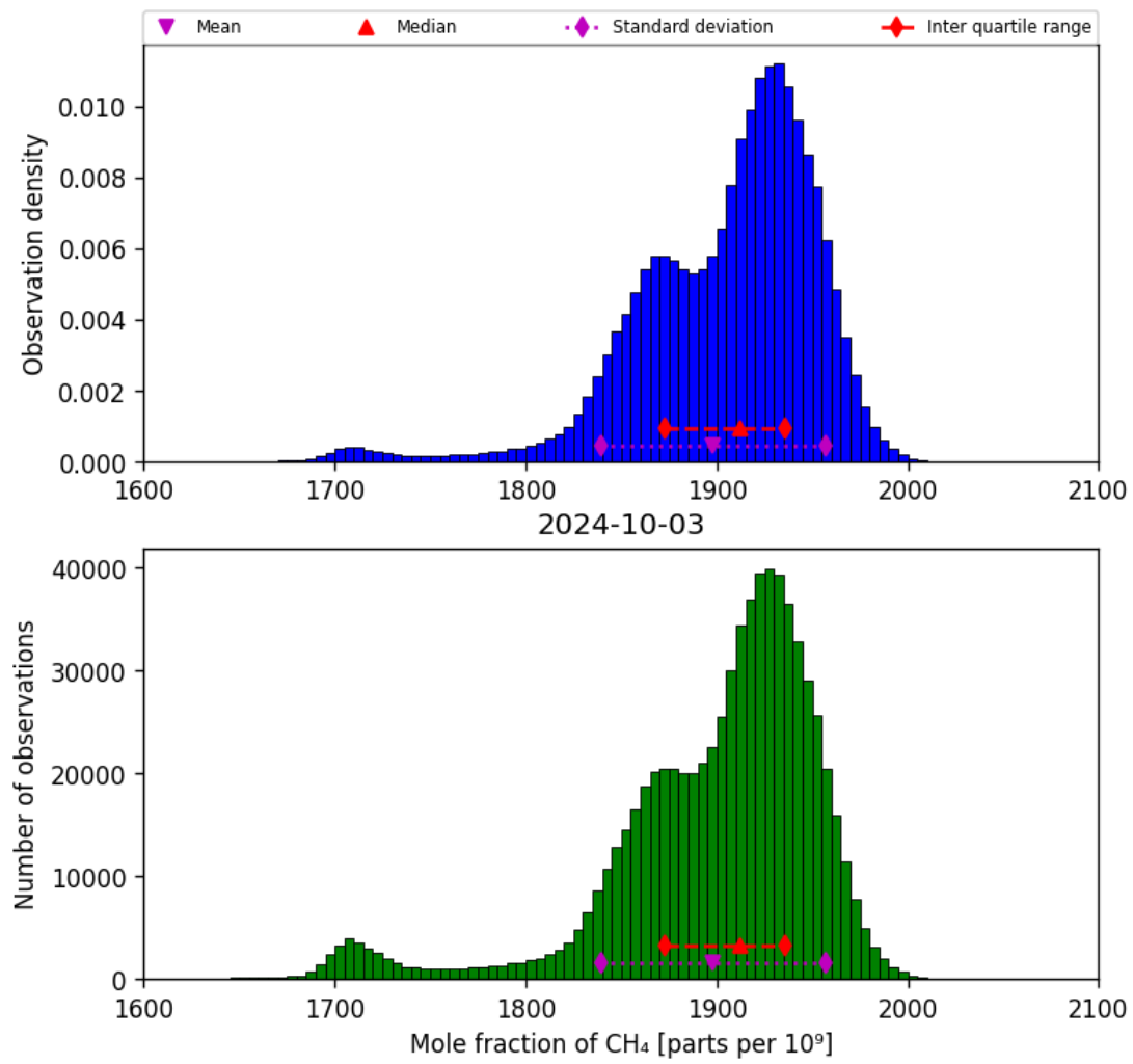
Figure 23: Histogram of “Mole fraction of CH 4 ” for 2024-10-03 to 2024-10-04
