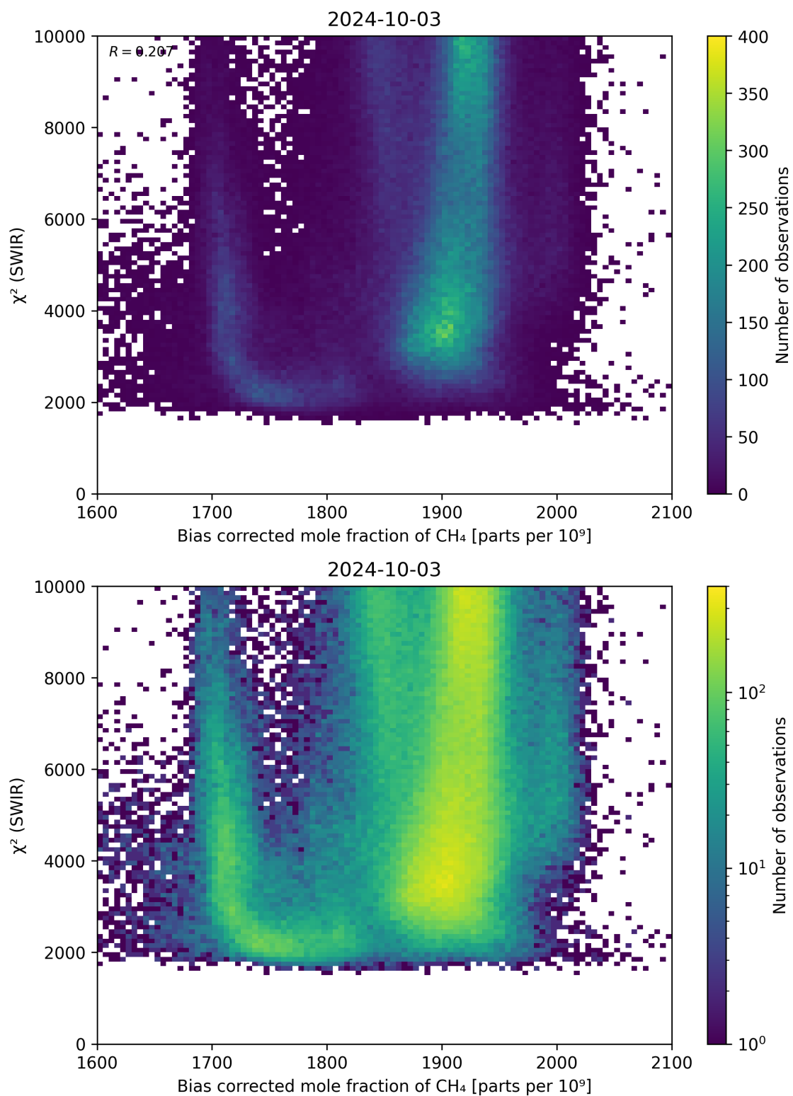
Figure 64: Scatter density plot of “Bias corrected mole fraction of \text{CH}_4 ” against “ \chi^2 (SWIR)” for 2024-10-03 to 2024-10-04.
