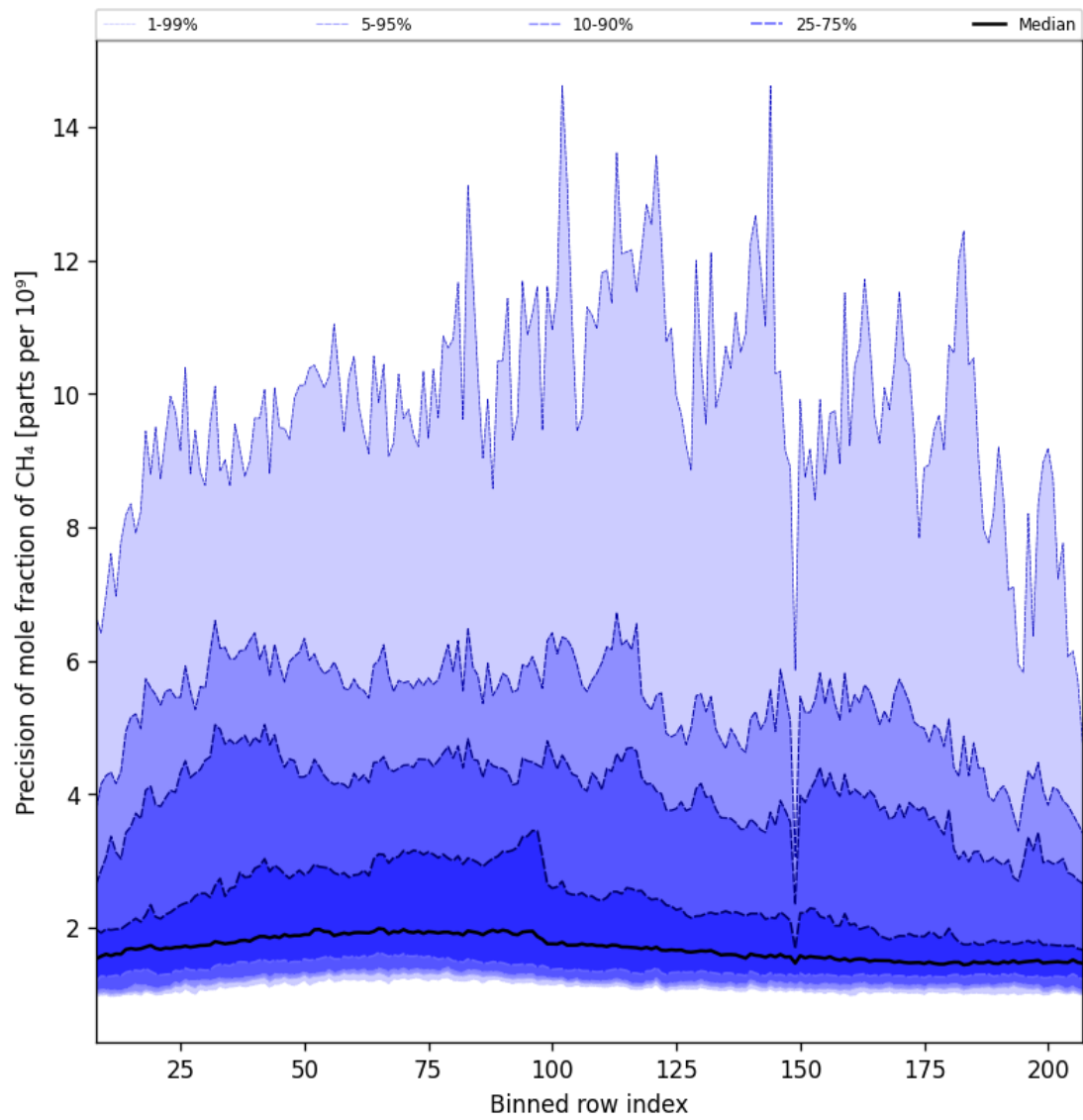
Figure 35: Along track statistics of “Precision of mole fraction of CH 4 ” for 2024-10-03 to 2024-10-04
