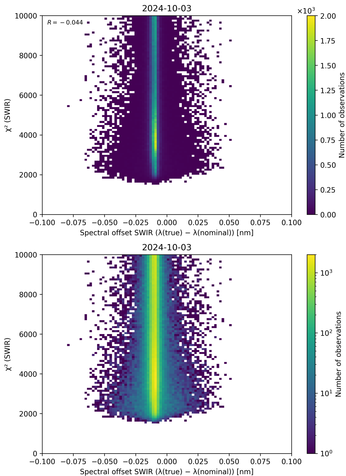
Figure 118: Scatter density plot of “Spectral offset SWIR ( \lambda_{\text{true}} - \lambda_{\text{nominal}} )” against “ \chi^2 (SWIR)” for 2024-10-03 to 2024-10-04.
