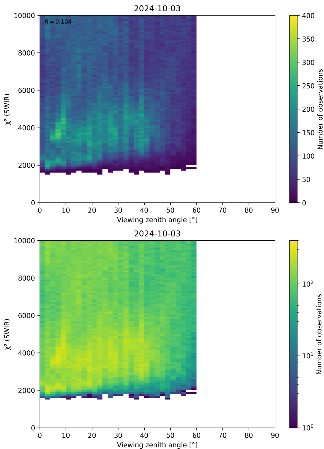
Figure 106: Scatter density plot of “Viewing zenith angle” against “ \chi^2 (SWIR)” for 2024-10-03 to 2024-10-04.
