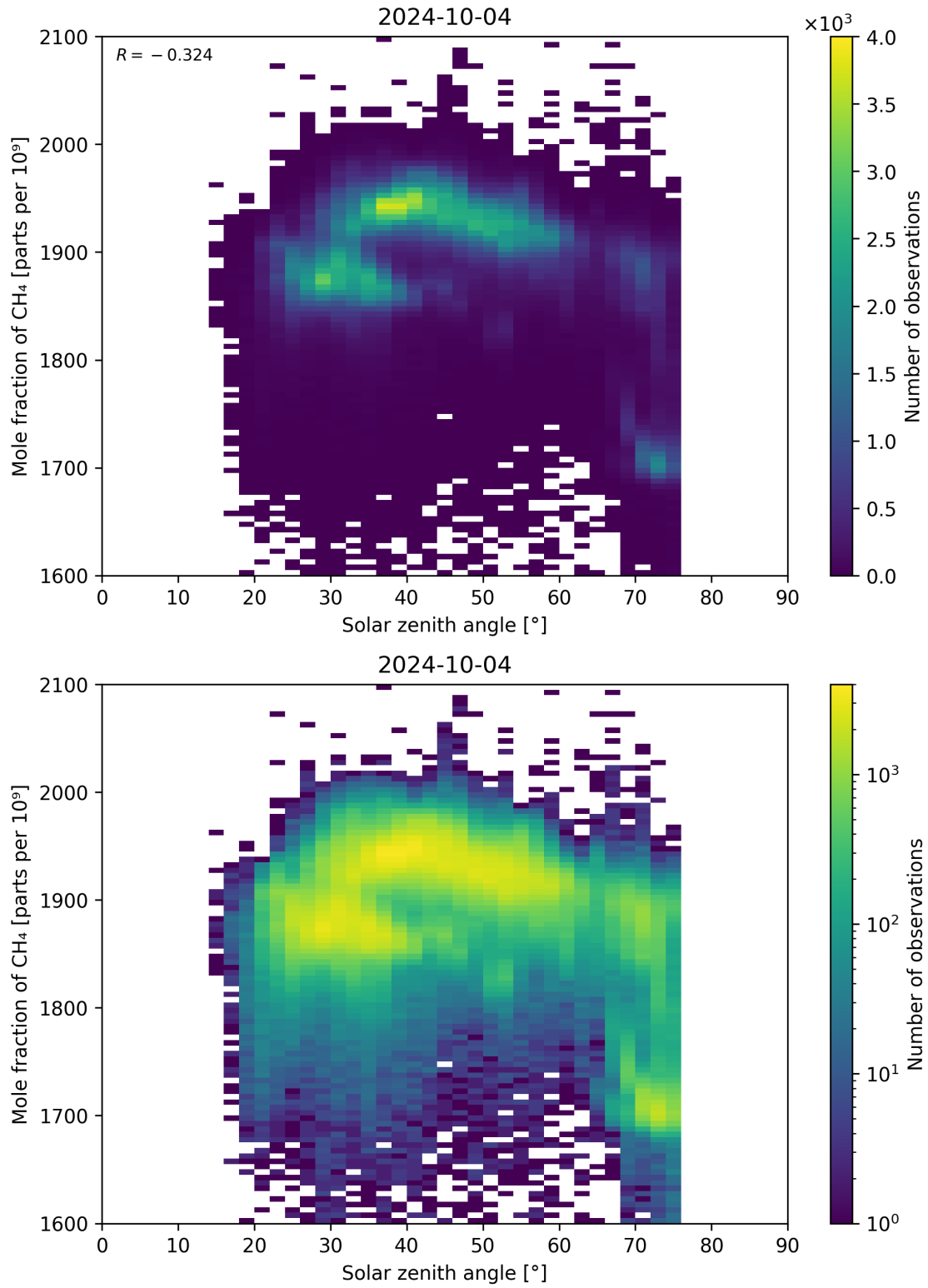
Figure 99: Scatter density plot of “Solar zenith angle” against “Mole fraction of \text{CH}_4 ” for 2024-10-03 to 2024-10-05.
