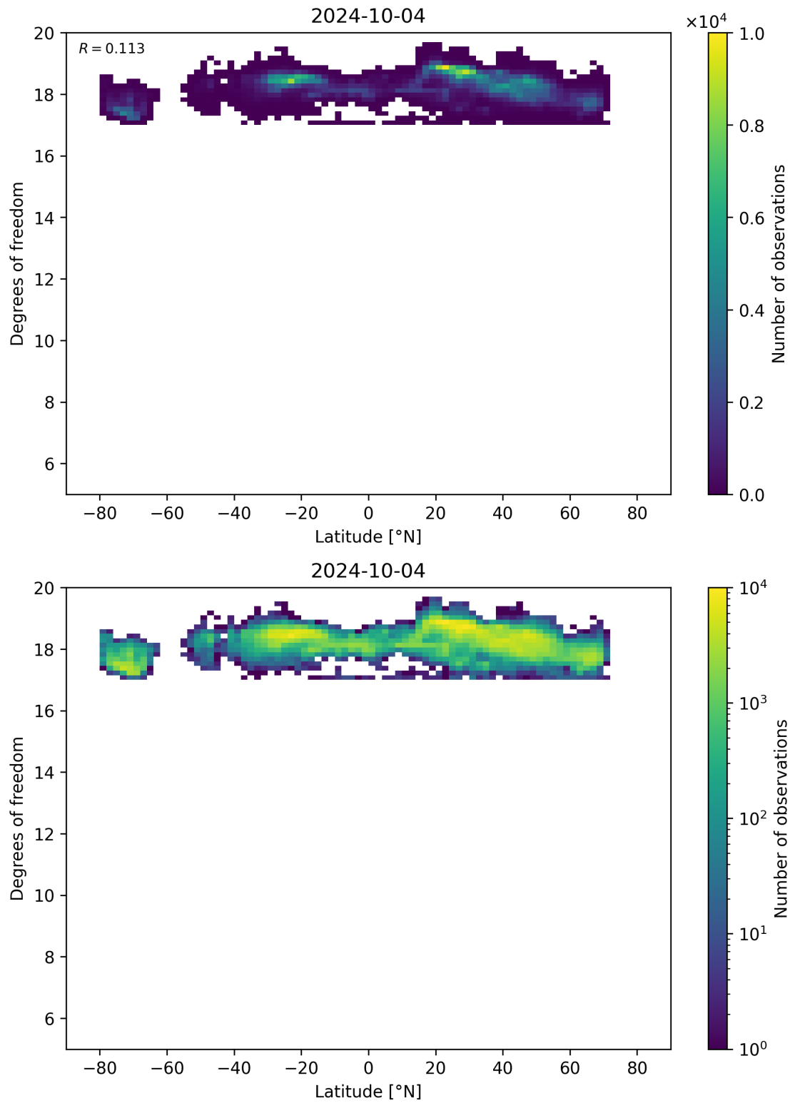
Figure 55: Scatter density plot of “Latitude” against “Degrees of freedom” for 2024-10-03 to 2024-10-05.
