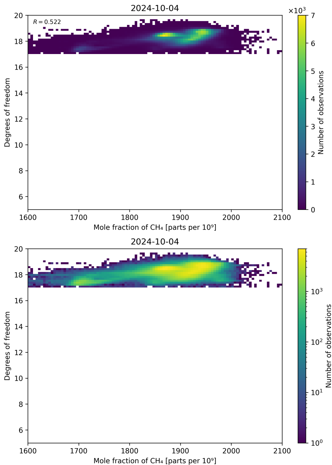
Figure 72: Scatter density plot of “Mole fraction of CH 4 ” against “Degrees of freedom” for 2024-10-03 to 2024-10-05.
