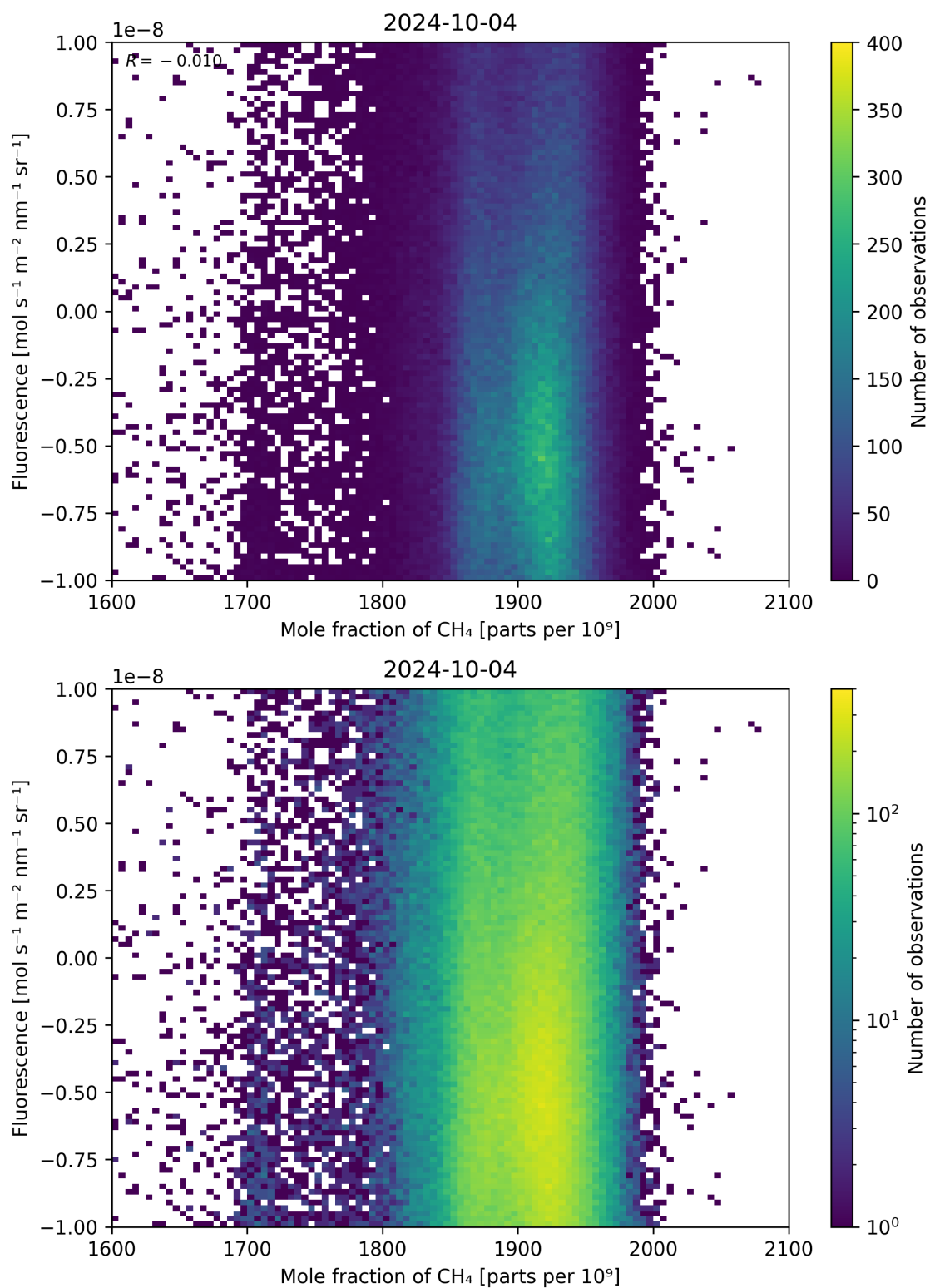
Figure 73: Scatter density plot of “Mole fraction of \text{CH}_4 ” against “Fluorescence” for 2024-10-03 to 2024-10-05.
