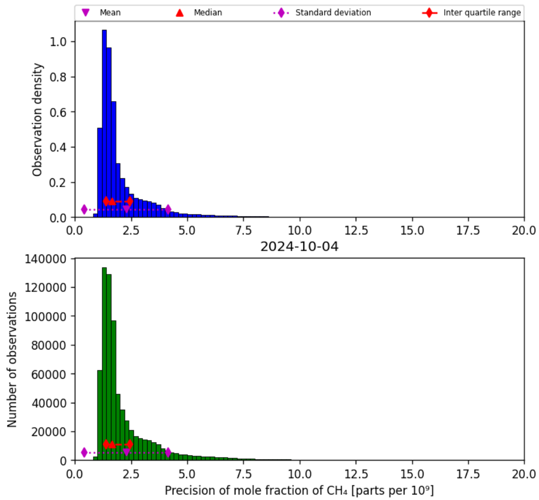
Figure 24: Histogram of “Precision of mole fraction of CH 4 ” for 2024-10-03 to 2024-10-05
