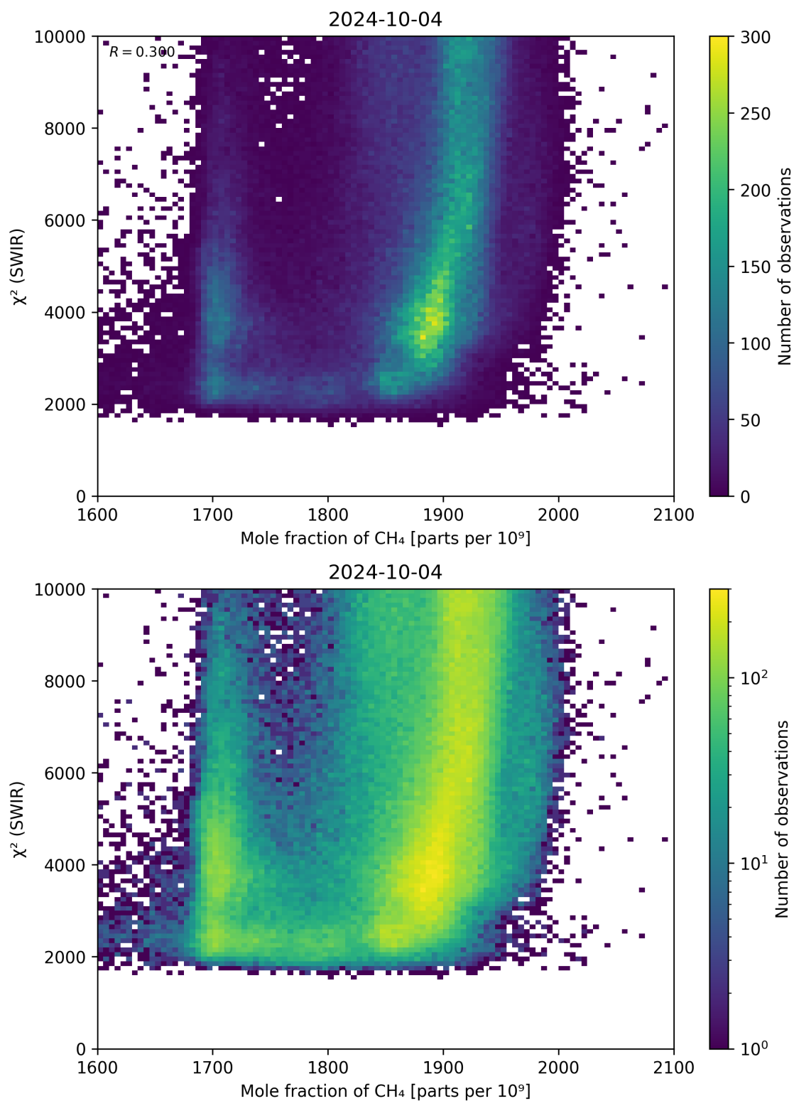
Figure 71: Scatter density plot of “Mole fraction of \text{CH}_4 ” against “ \chi^2 (SWIR)” for 2024-10-03 to 2024-10-05.
