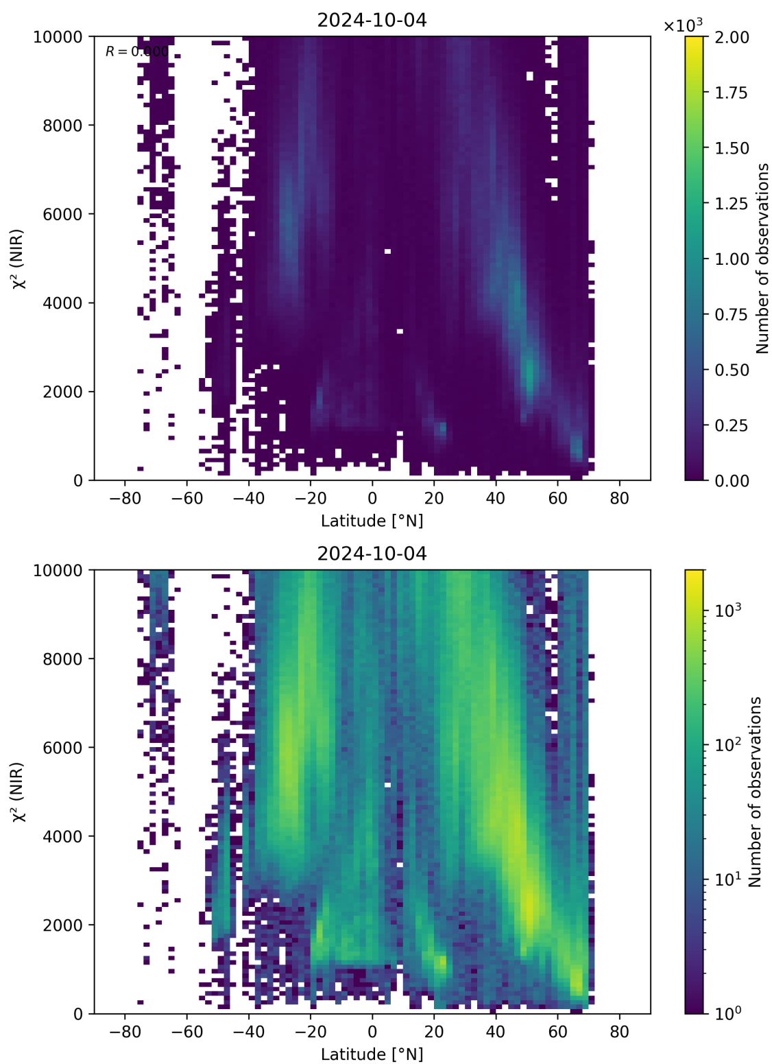
Figure 53: Scatter density plot of “Latitude” against “ \chi^2 (NIR)” for 2024-10-03 to 2024-10-05.
