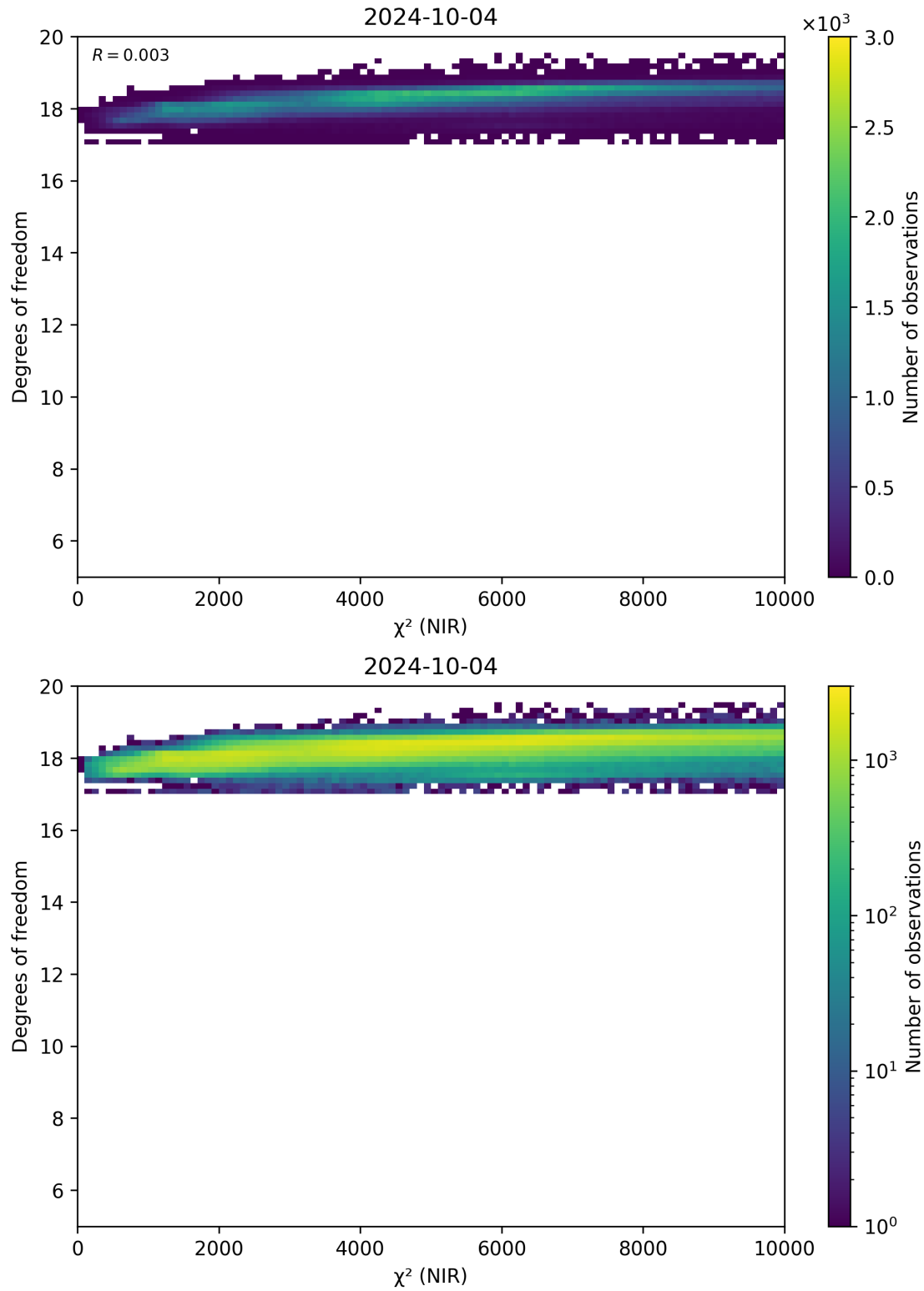
Figure 44: Scatter density plot of “ \chi^2 (NIR)” against “Degrees of freedom” for 2024-10-03 to 2024-10-05.
