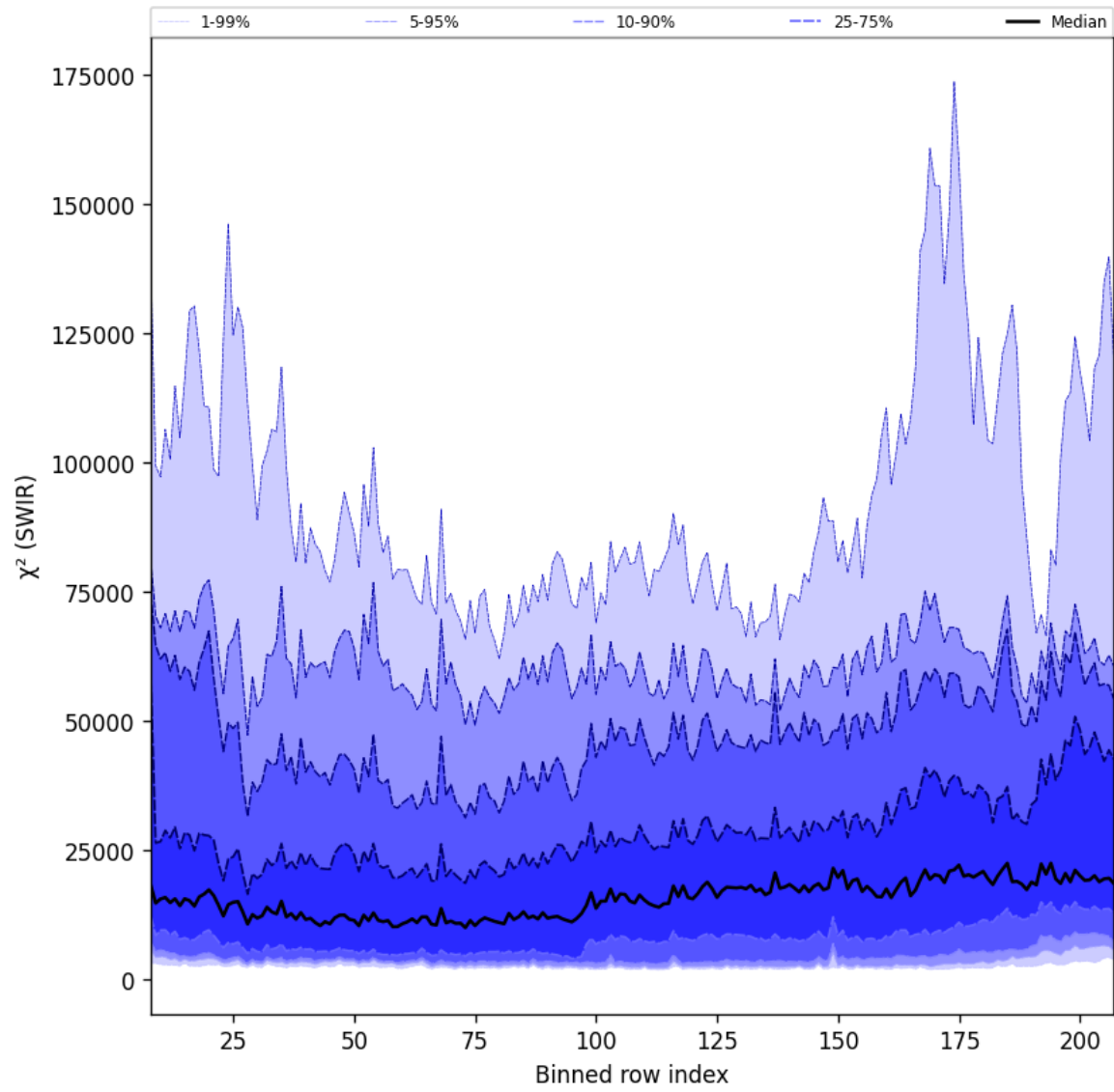
Figure 39: Along track statistics of “ \chi^2 (SWIR)” for 2024-10-03 to 2024-10-05
