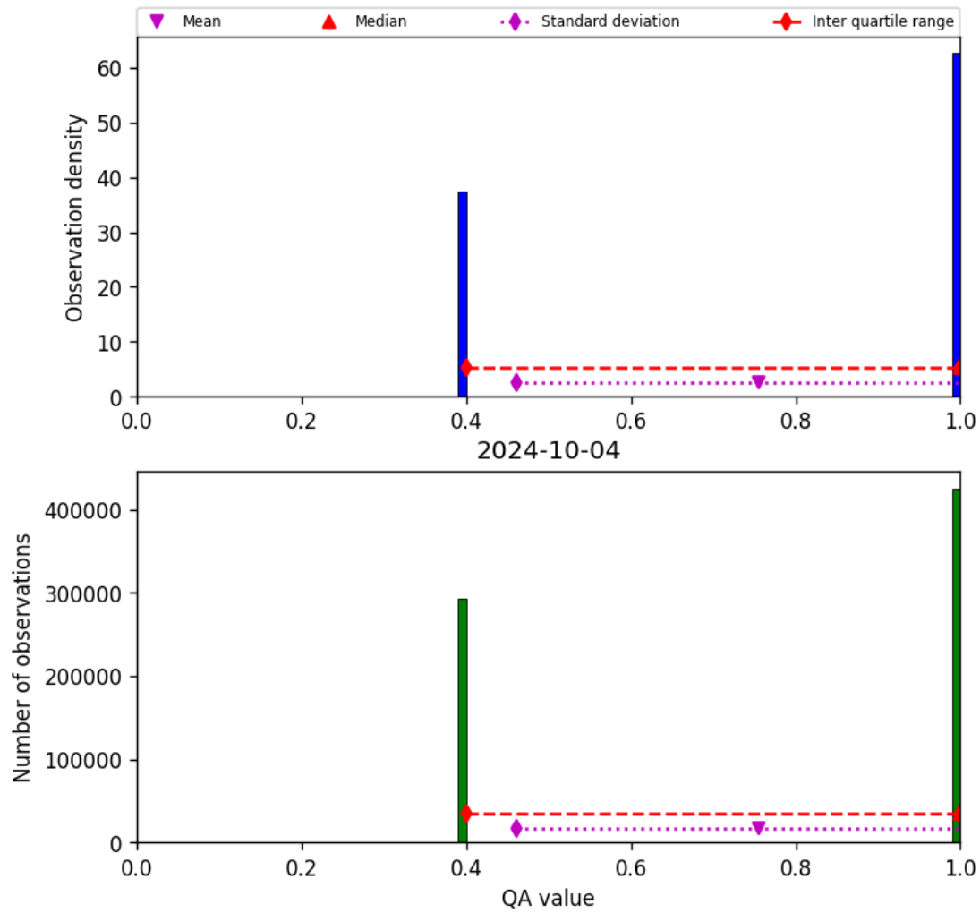
Figure 22: Histogram of “QA value” for 2024-10-03 to 2024-10-05
