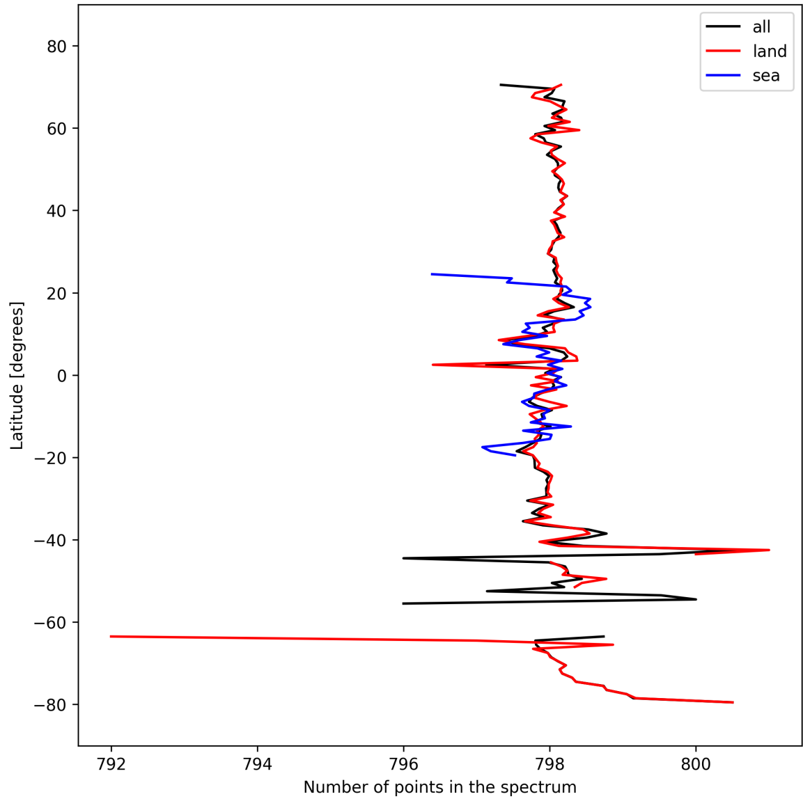
Figure 15: Zonal average of “Number of points in the spectrum” for 2024-10-03 to 2024-10-05.
