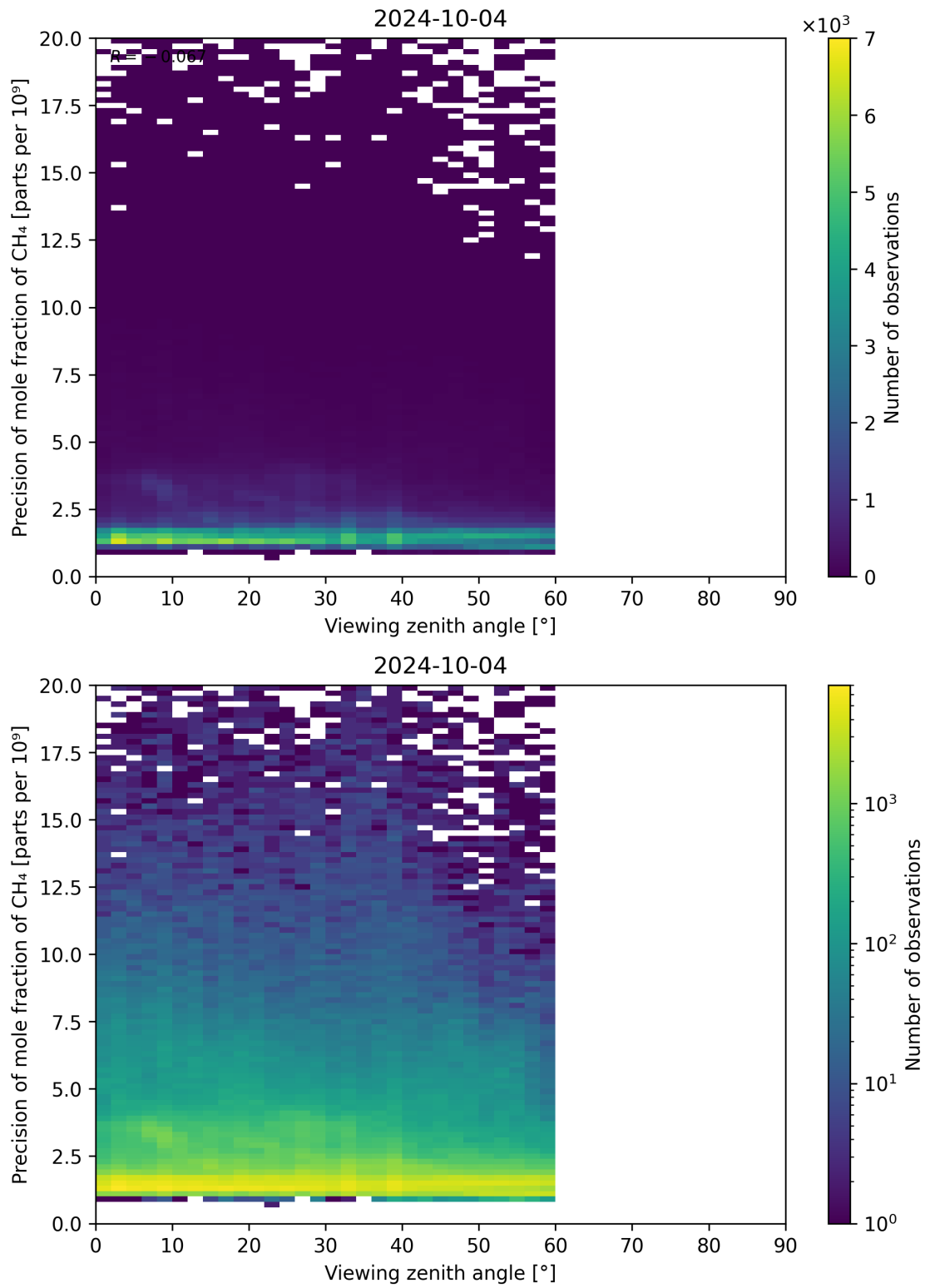
Figure 112: Scatter density plot of “Viewing zenith angle” against “Precision of mole fraction of CH 4 ” for 2024-10-03 to 2024-10-05.
