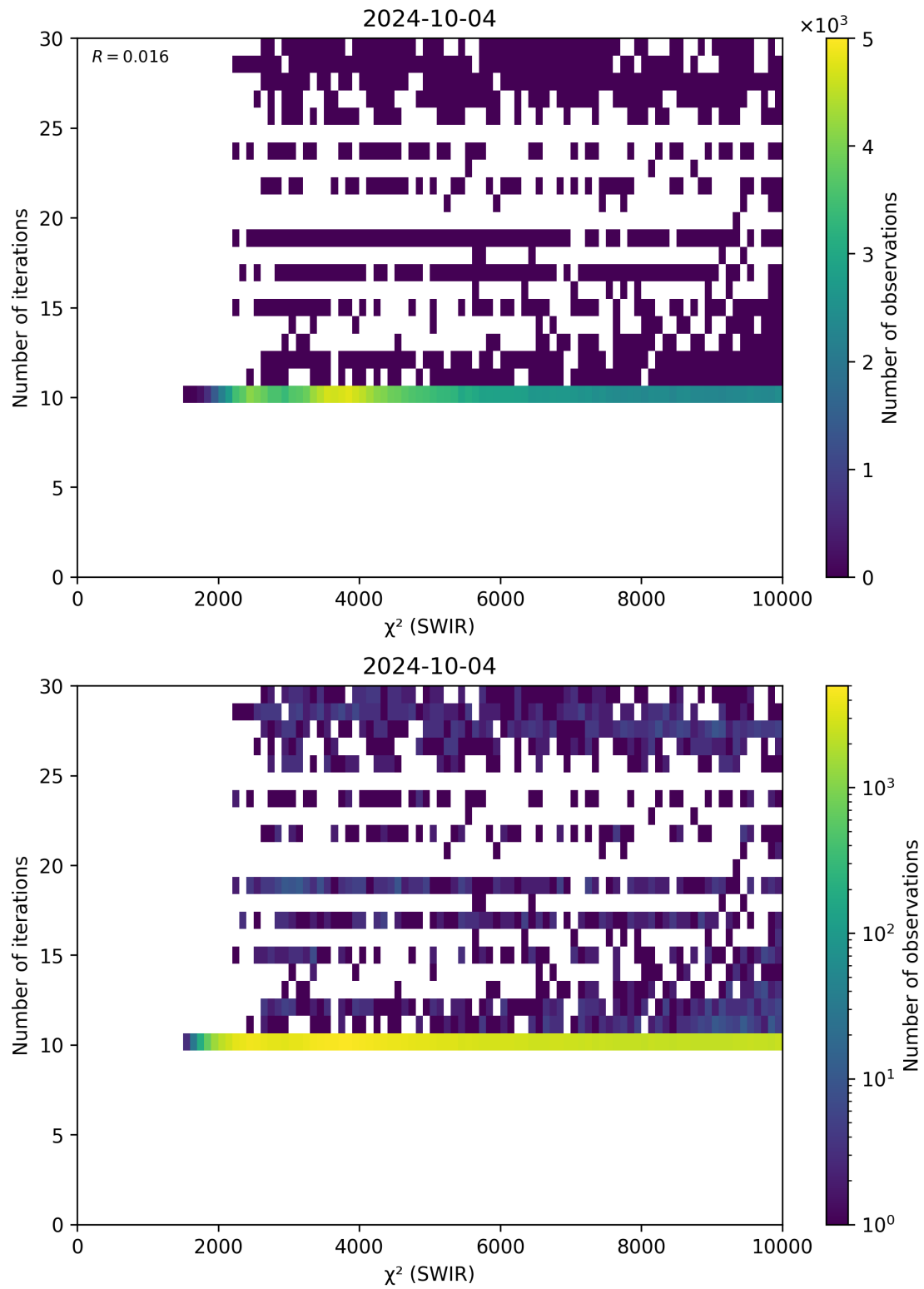
Figure 50: Scatter density plot of “ \chi^2 (SWIR)” against “Number of iterations” for 2024-10-03 to 2024-10-05.
