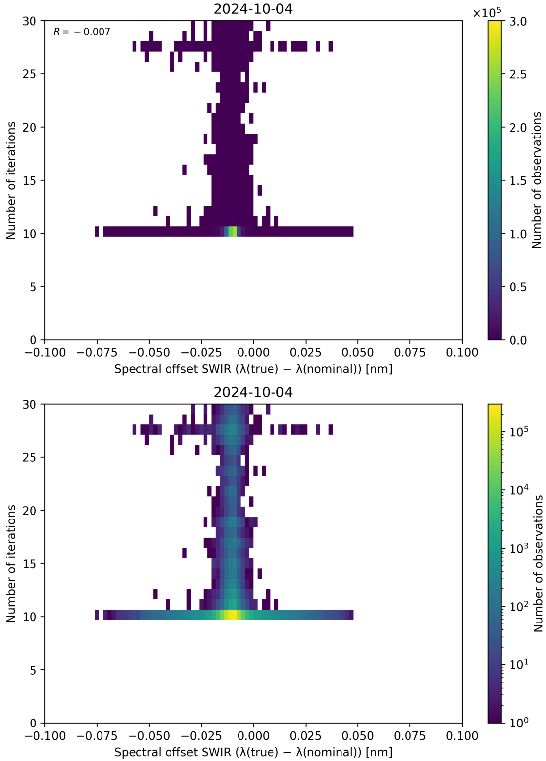
Figure 121: Scatter density plot of “Spectral offset SWIR ( \lambda_{\text{true}} - \lambda_{\text{nominal}} )” against “Number of iterations” for 2024-10-03 to 2024-10-05.
