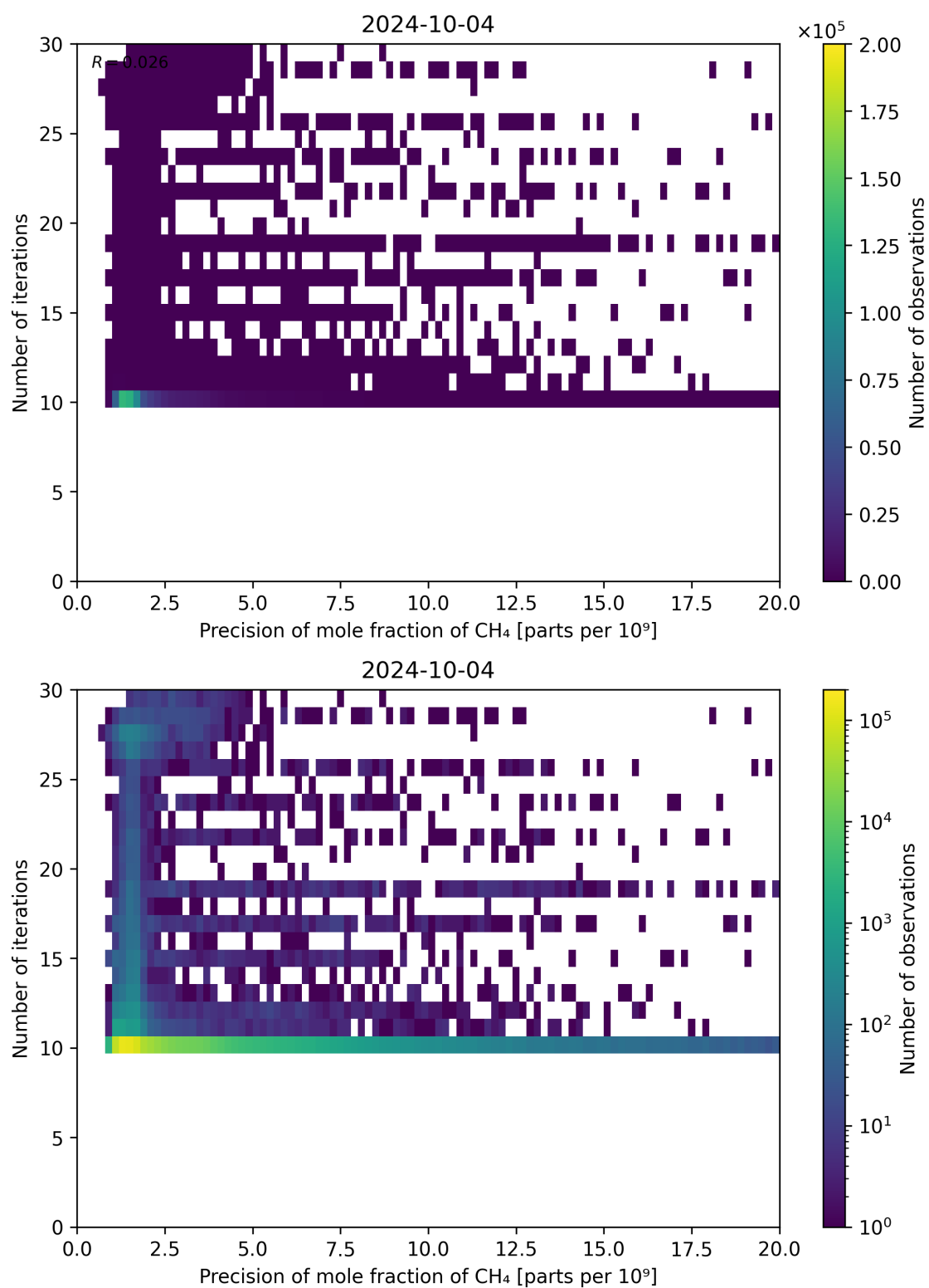
Figure 83: Scatter density plot of “Precision of mole fraction of CH 4 ” against “Number of iterations” for 2024-10-03 to 2024-10-05.
