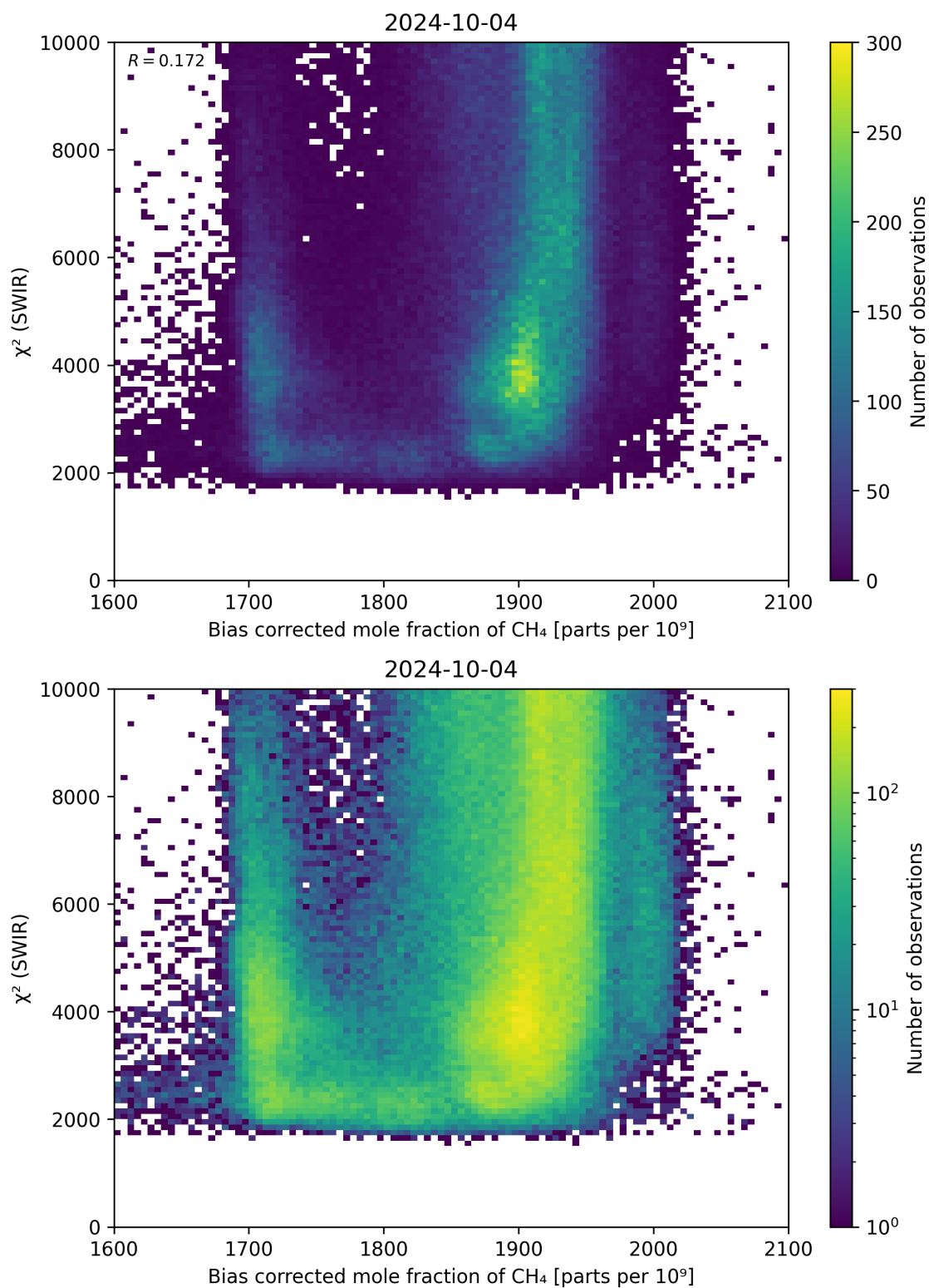
Figure 64: Scatter density plot of “Bias corrected mole fraction of \text{CH}_4 ” against “ \chi^2 (SWIR)” for 2024-10-03 to 2024-10-05.
