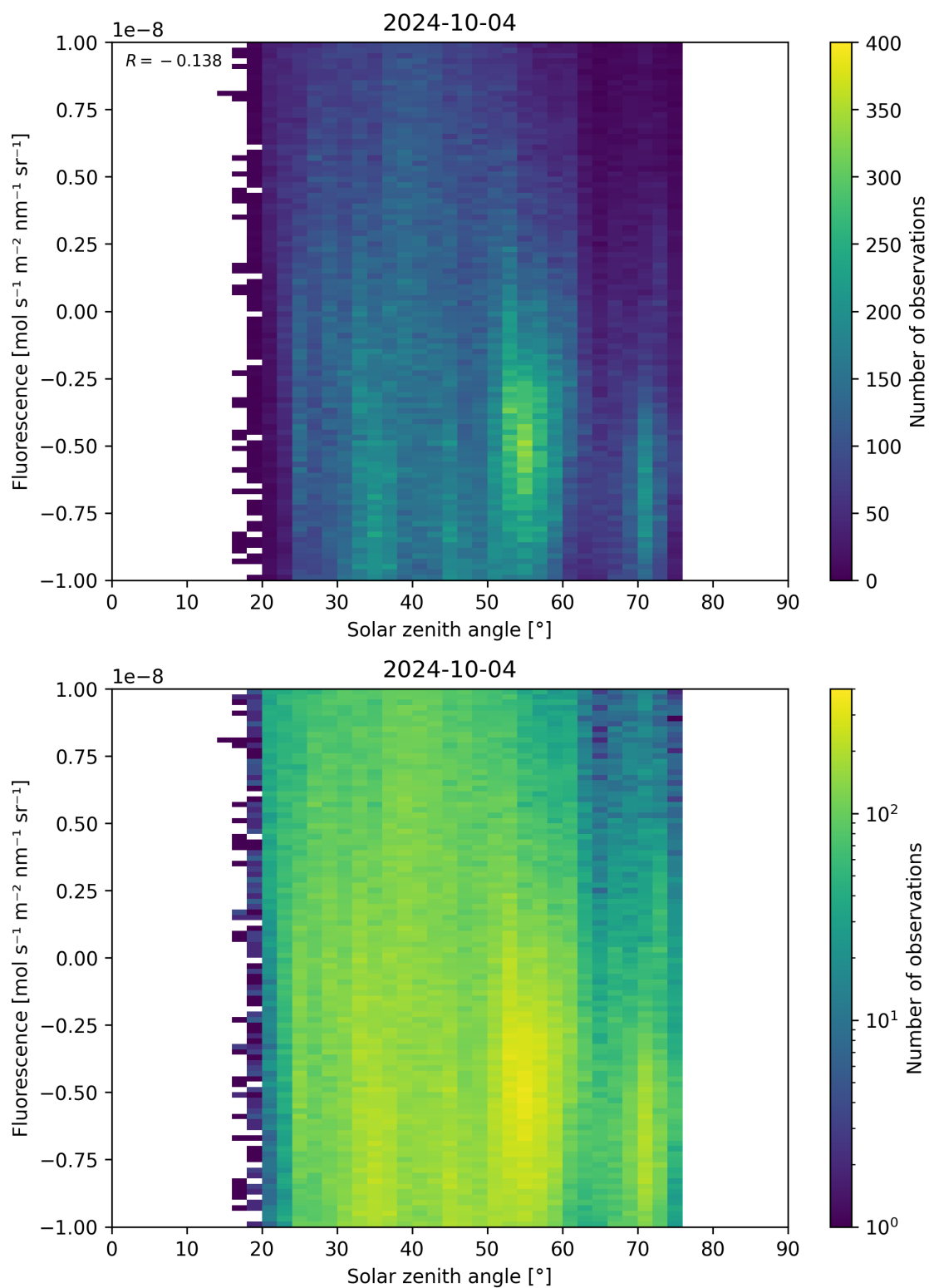
Figure 97: Scatter density plot of “Solar zenith angle” against “Fluorescence” for 2024-10-03 to 2024-10-05.
