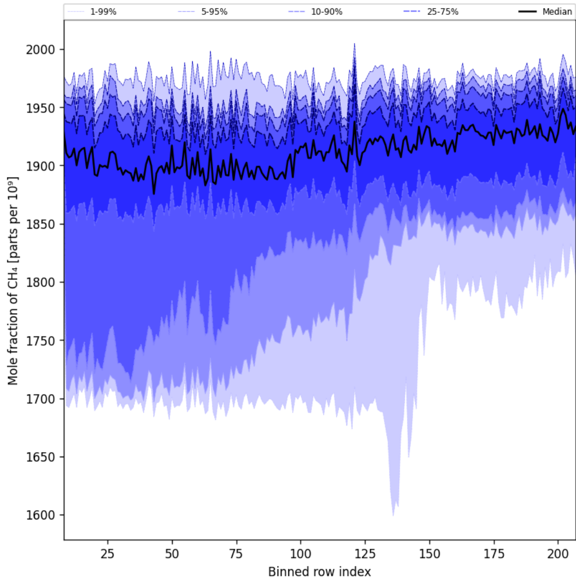
Figure 34: Along track statistics of “Mole fraction of CH 4 ” for 2024-10-03 to 2024-10-05
