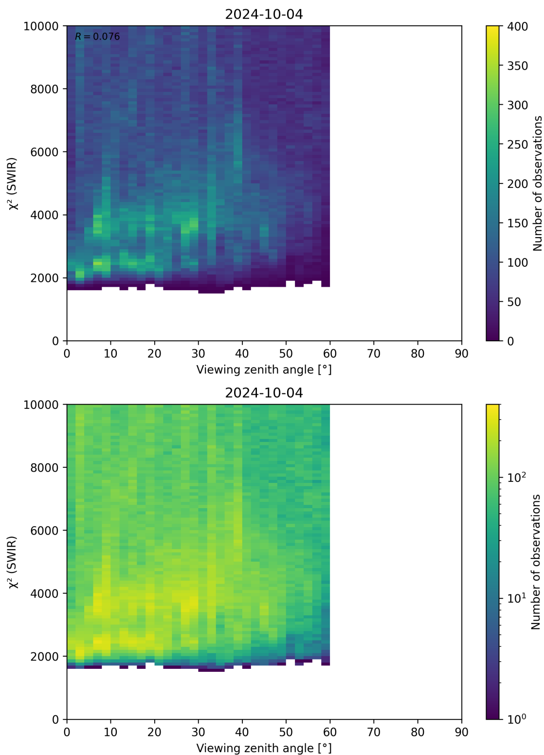
Figure 106: Scatter density plot of “Viewing zenith angle” against “ \chi^2 (SWIR)” for 2024-10-03 to 2024-10-05.
