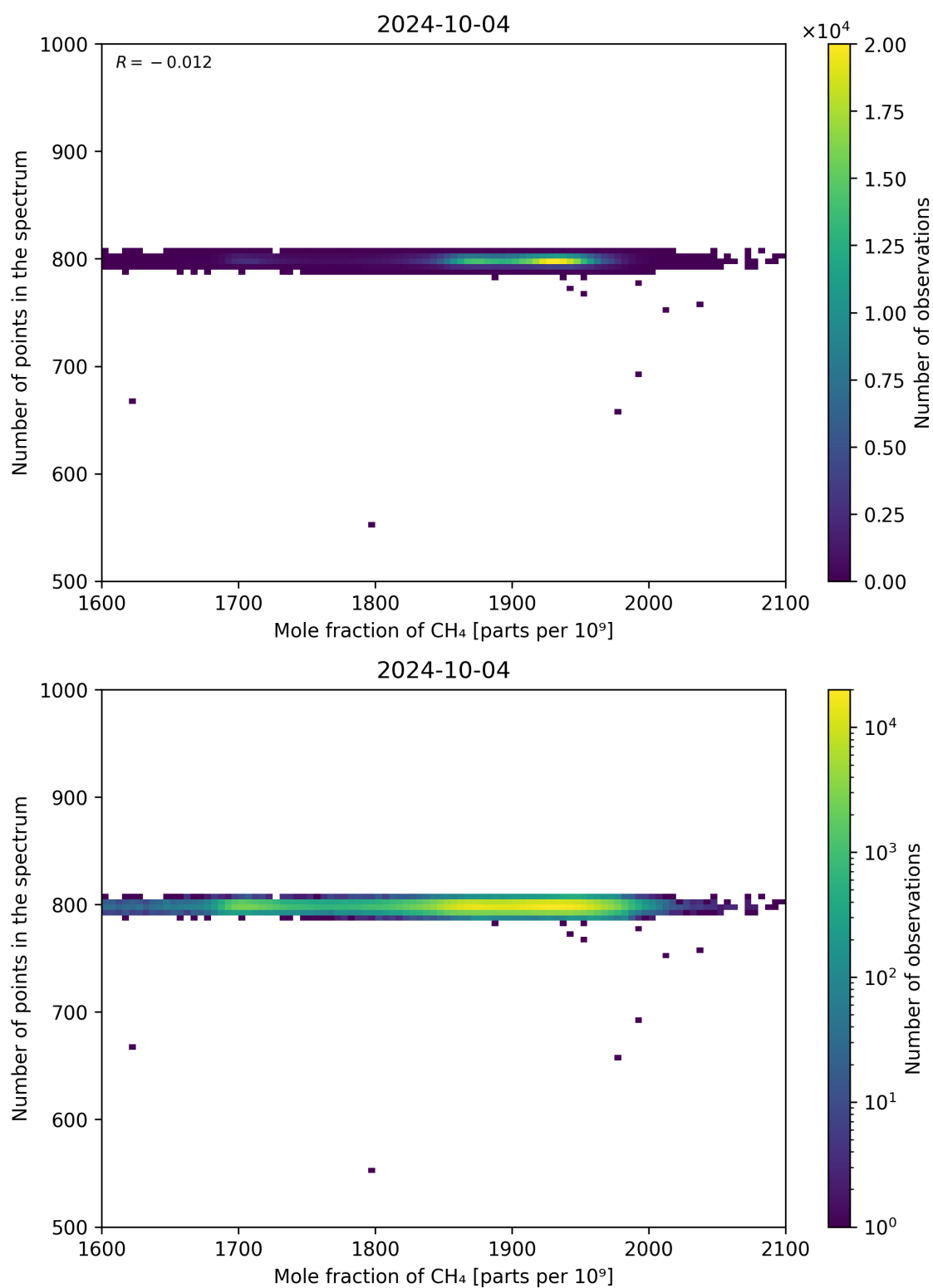
Figure 77: Scatter density plot of “Mole fraction of CH 4 ” against “Number of points in the spectrum” for 2024-10-03 to 2024-10-05.
