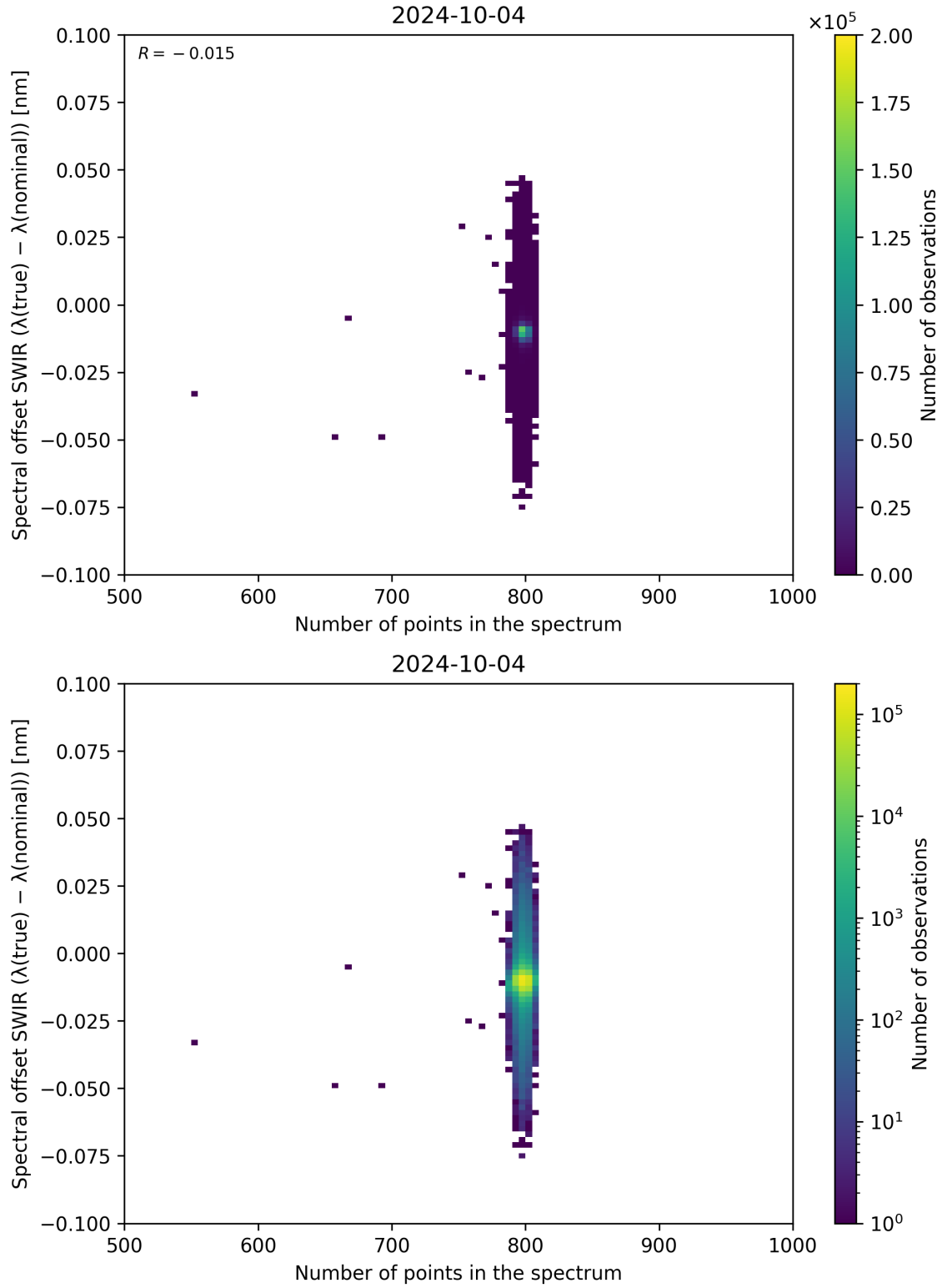
Figure 93: Scatter density plot of “Number of points in the spectrum” against “Spectral offset SWIR ( \lambda_{\text{true}} - \lambda_{\text{nominal}} )” for 2024-10-03 to 2024-10-05.
