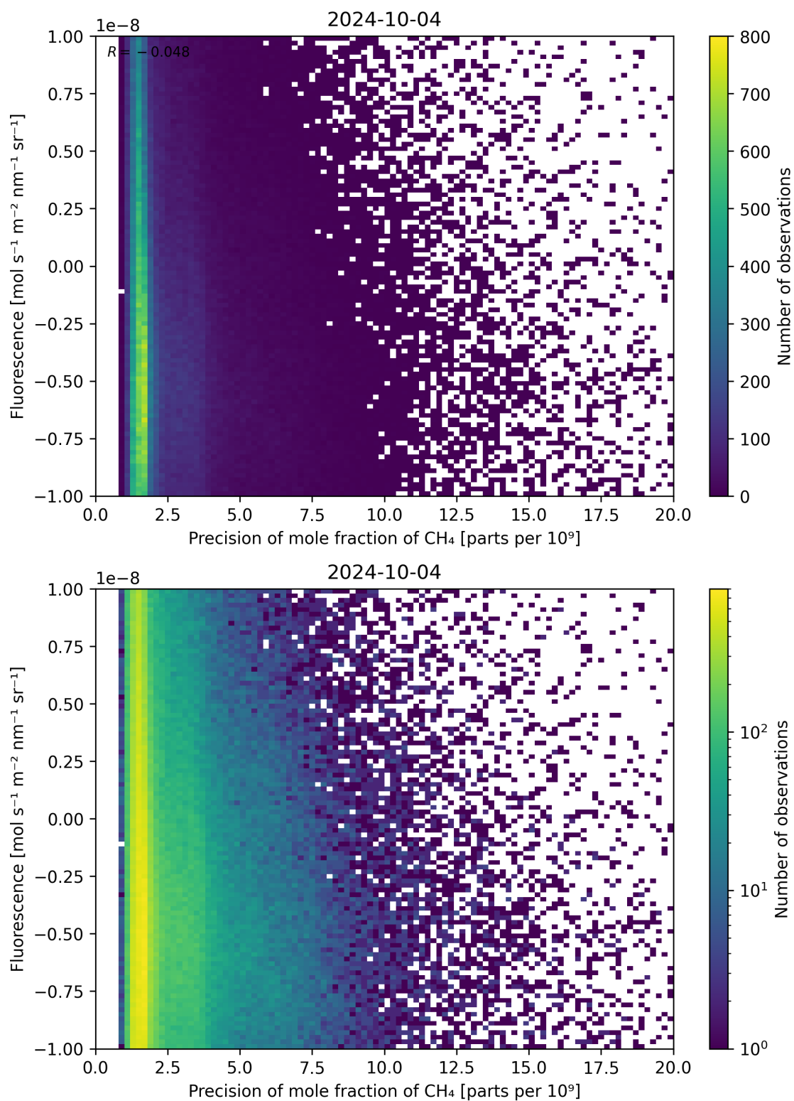
Figure 81: Scatter density plot of “Precision of mole fraction of \text{CH}_4 ” against “Fluorescence” for 2024-10-03 to 2024-10-05.
