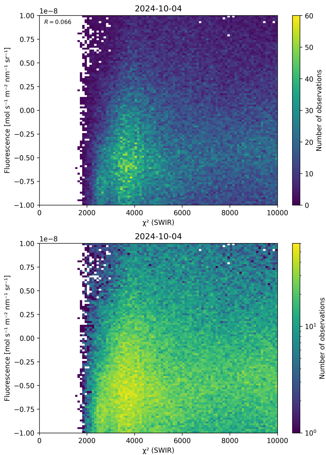
Figure 49: Scatter density plot of “ \chi^2 (SWIR)” against “Fluorescence” for 2024-10-03 to 2024-10-05.
