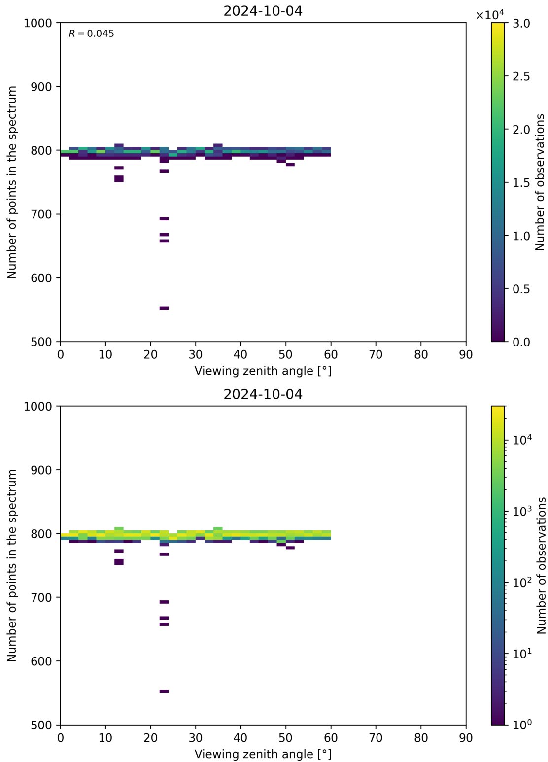
Figure 114: Scatter density plot of “Viewing zenith angle” against “Number of points in the spectrum” for 2024-10-03 to 2024-10-05.
