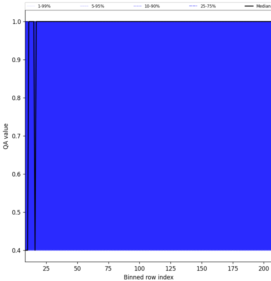
Figure 33: Along track statistics of “QA value” for 2024-10-03 to 2024-10-05
