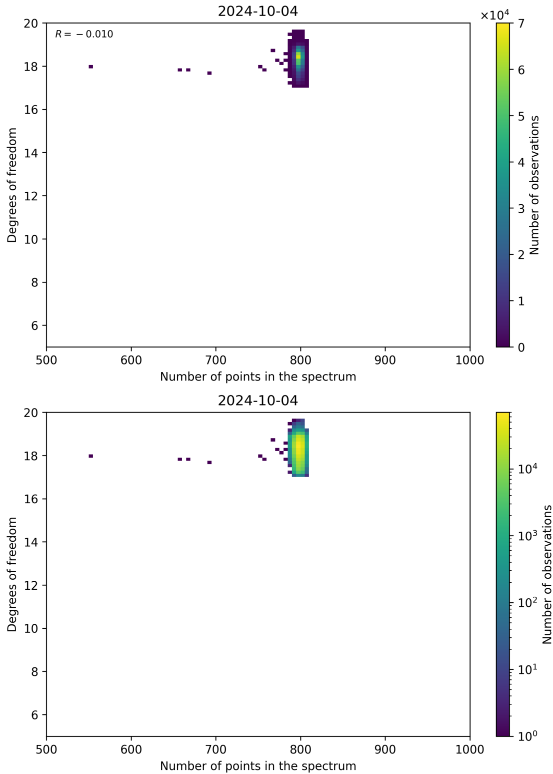
Figure 90: Scatter density plot of “Number of points in the spectrum” against “Degrees of freedom” for 2024-10-03 to 2024-10-05.
