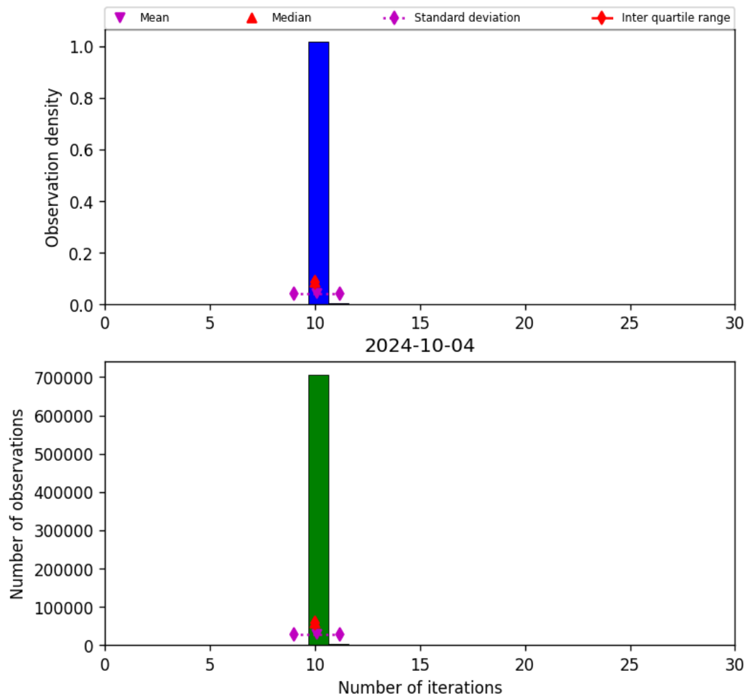
Figure 31: Histogram of “Number of iterations” for 2024-10-03 to 2024-10-05
