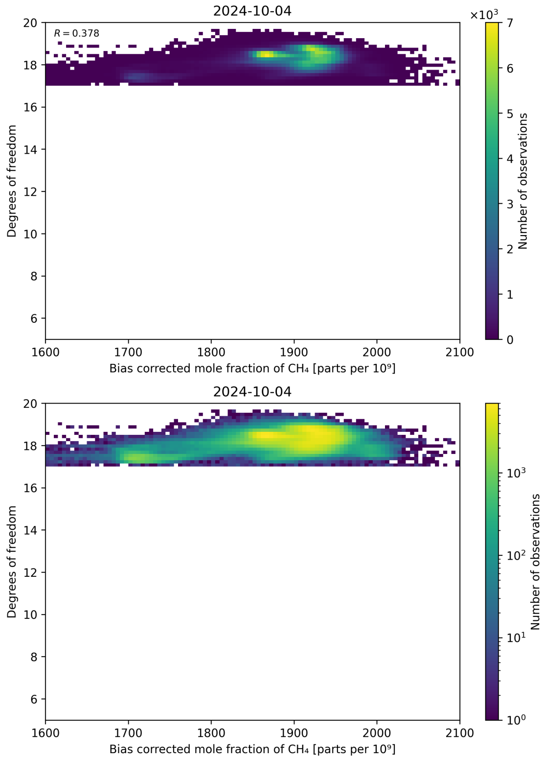
Figure 65: Scatter density plot of “Bias corrected mole fraction of CH 4 ” against “Degrees of freedom” for 2024-10-03 to 2024-10-05.
