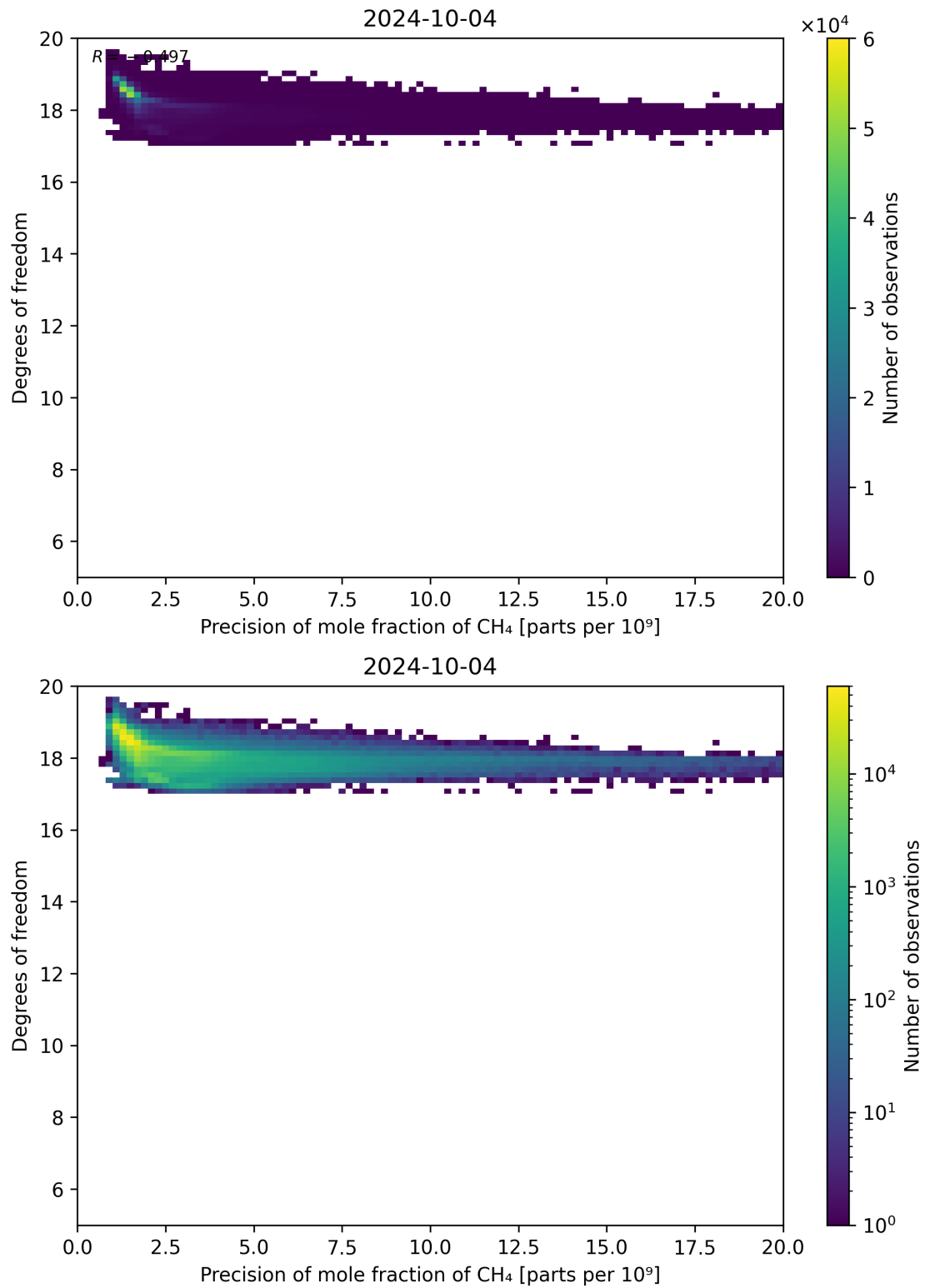
Figure 80: Scatter density plot of “Precision of mole fraction of CH 4 ” against “Degrees of freedom” for 2024-10-03 to 2024-10-05.
