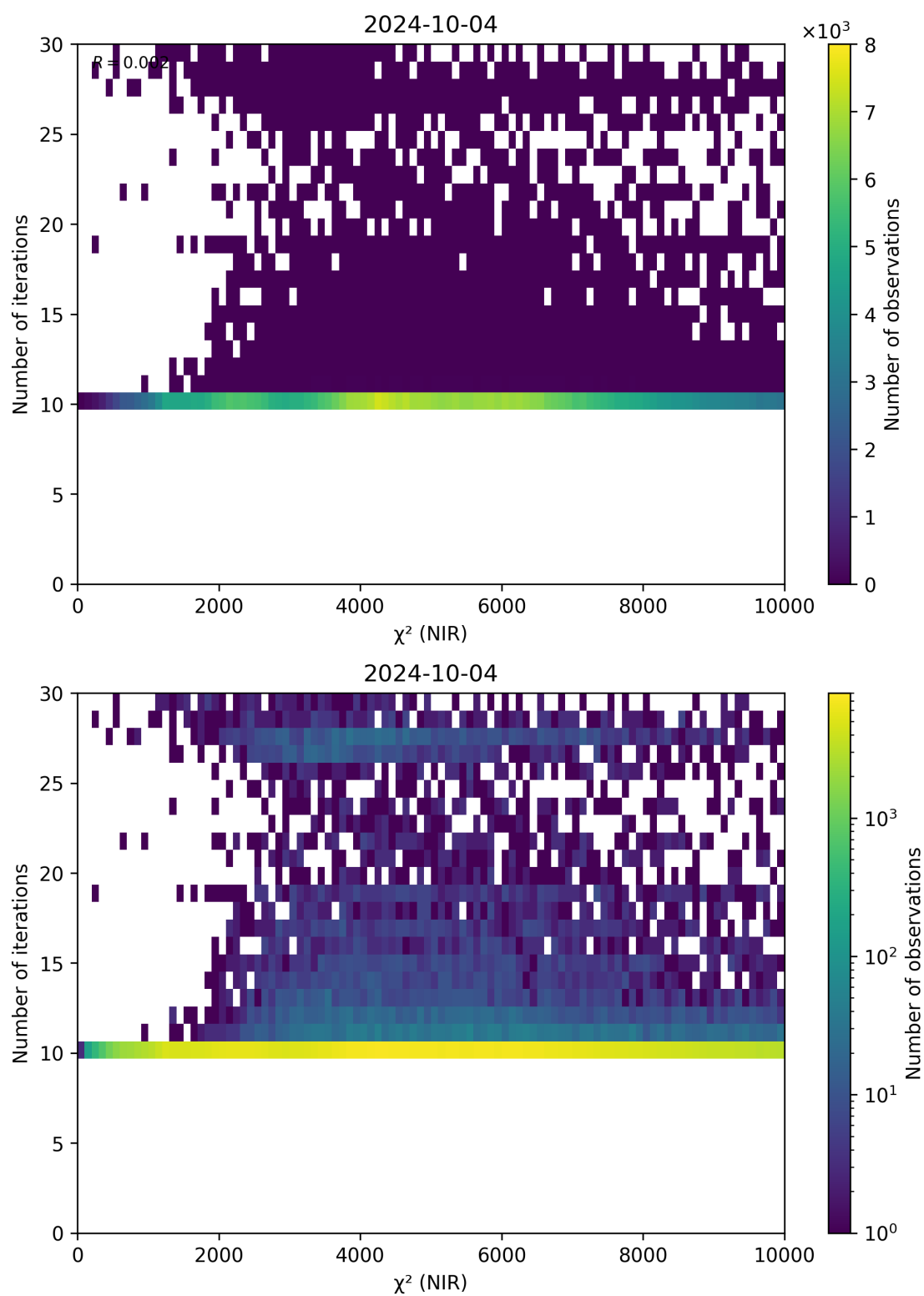
Figure 46: Scatter density plot of “ \chi^2 (NIR)” against “Number of iterations” for 2024-10-03 to 2024-10-05.
