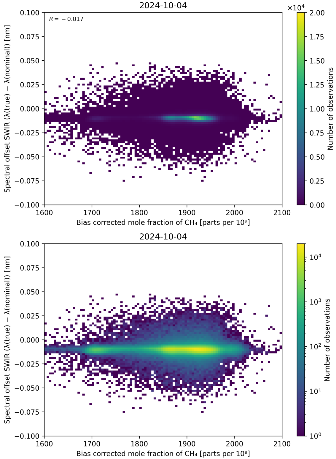
Figure 69: Scatter density plot of “Bias corrected mole fraction of \text{CH}_4 ” against “Spectral offset SWIR ( \lambda_{\text{true}} - \lambda_{\text{nominal}} )” for 2024-10-03 to 2024-10-05.
