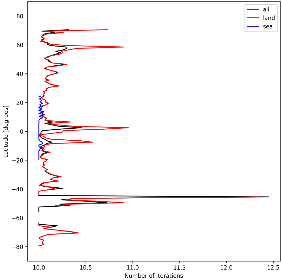
Figure 20: Zonal average of “Number of iterations” for 2024-10-03 to 2024-10-05.
