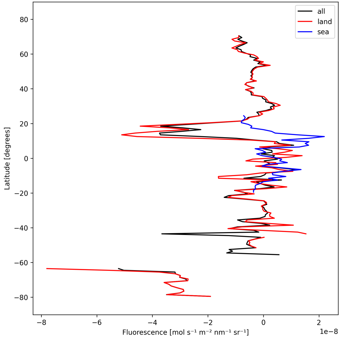
Figure 21: Zonal average of “Fluorescence” for 2024-10-03 to 2024-10-05.
