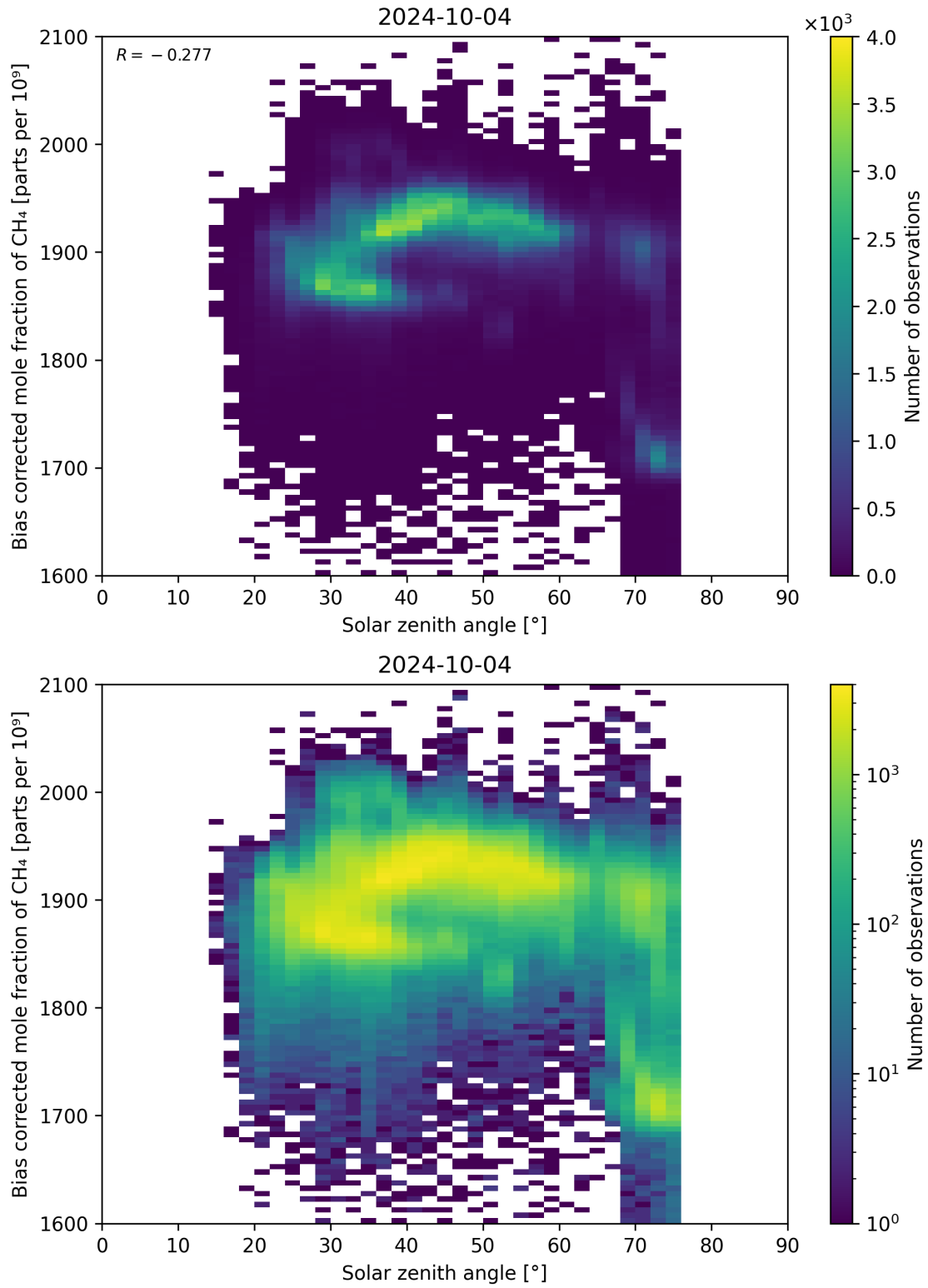
Figure 100: Scatter density plot of “Solar zenith angle” against “Bias corrected mole fraction of \text{CH}_4 ” for 2024-10-03 to 2024-10-05.
