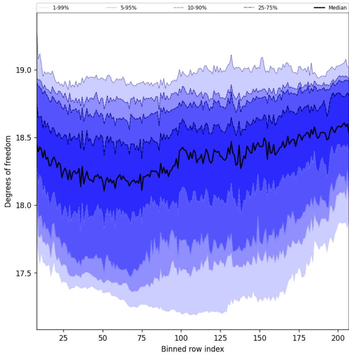
Figure 41: Along track statistics of “Degrees of freedom” for 2024-10-03 to 2024-10-05
