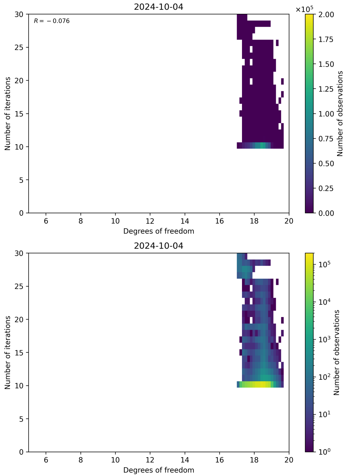
Figure 52: Scatter density plot of “Degrees of freedom” against “Number of iterations” for 2024-10-03 to 2024-10-05.
