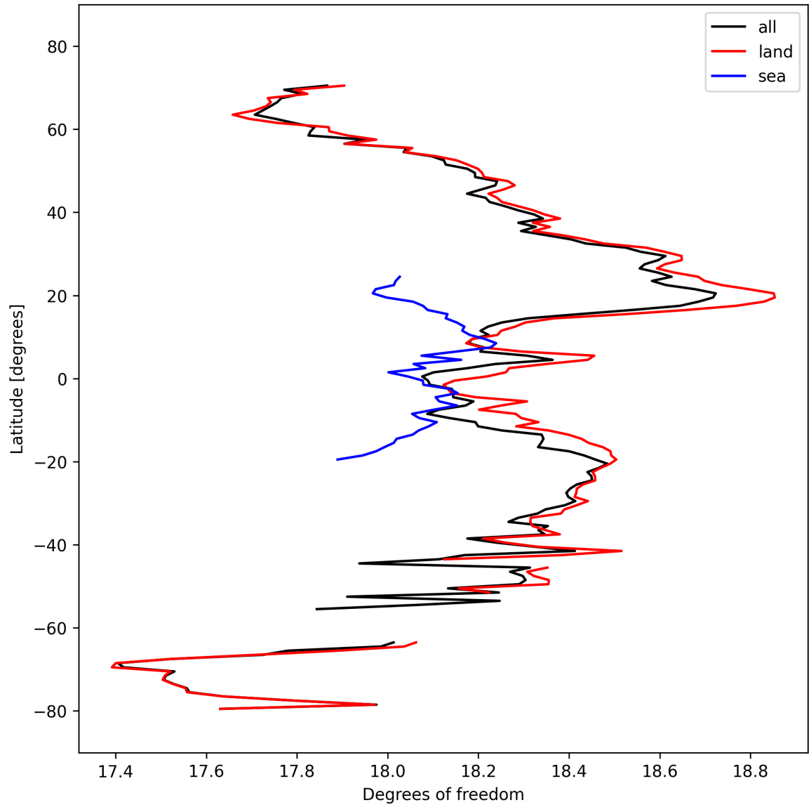
Figure 19: Zonal average of “Degrees of freedom” for 2024-10-03 to 2024-10-05.
