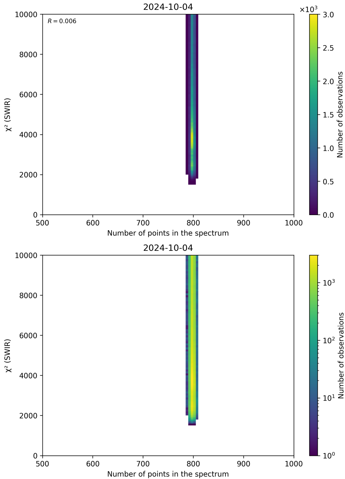
Figure 89: Scatter density plot of “Number of points in the spectrum” against “ \chi^2 (SWIR)” for 2024-10-03 to 2024-10-05.
