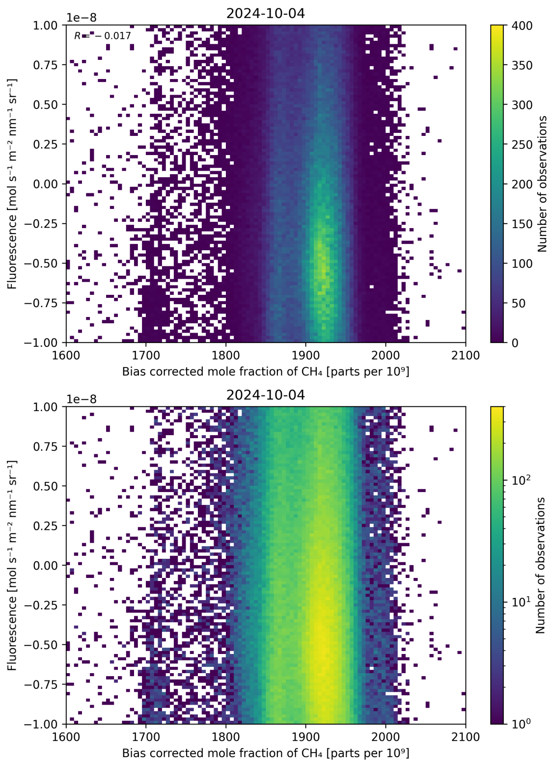
Figure 66: Scatter density plot of “Bias corrected mole fraction of \text{CH}_4 ” against “Fluorescence” for 2024-10-03 to 2024-10-05.
