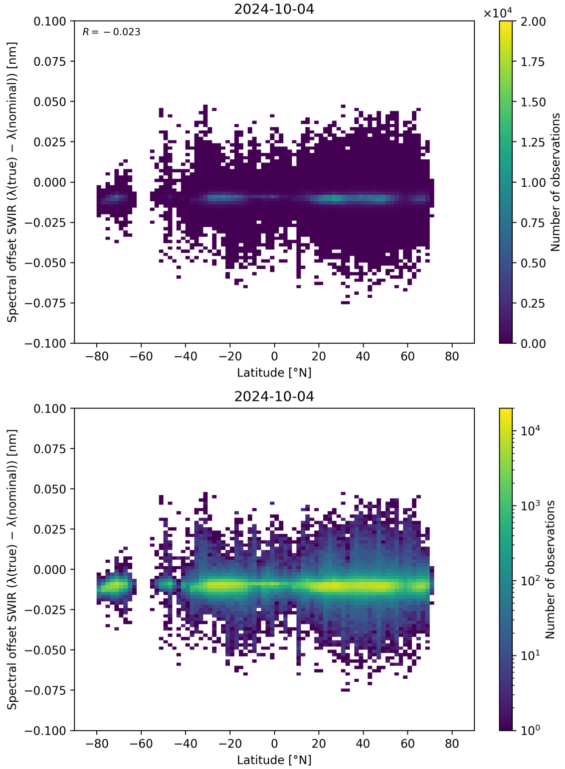
Figure 62: Scatter density plot of “Latitude” against “Spectral offset SWIR ( \lambda_{\text{true}} - \lambda_{\text{nominal}} )” for 2024-10-03 to 2024-10-05.
