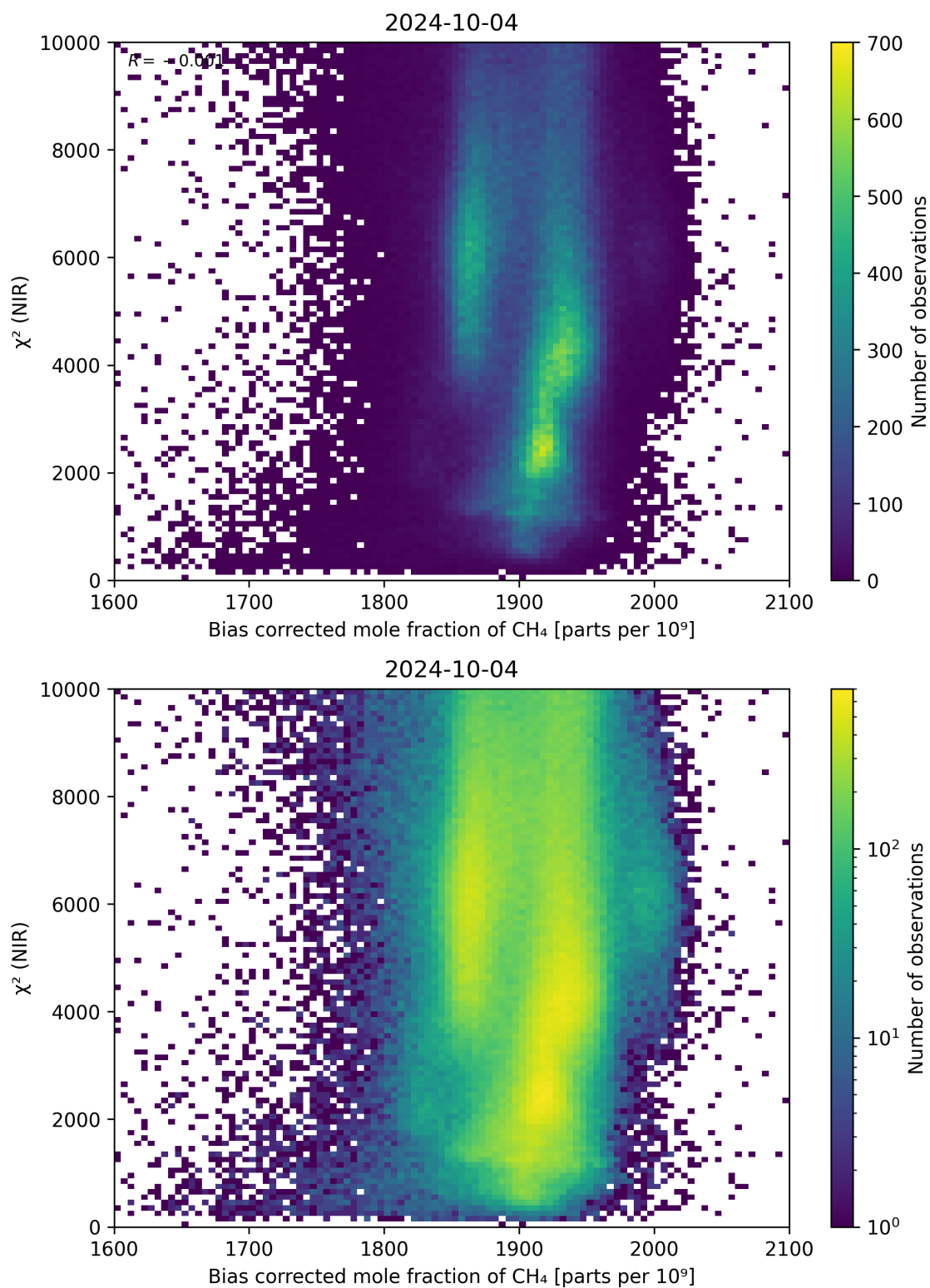
Figure 63: Scatter density plot of “Bias corrected mole fraction of CH 4 ” against “ \chi^2 (NIR)” for 2024-10-03 to 2024-10-05.
