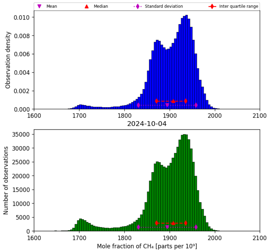
Figure 23: Histogram of “Mole fraction of CH 4 ” for 2024-10-03 to 2024-10-05
