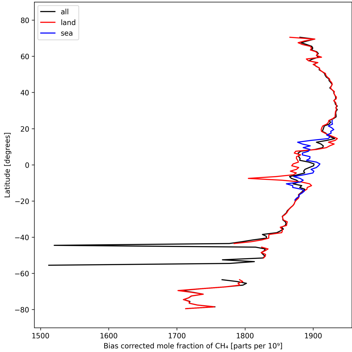
Figure 14: Zonal average of “Bias corrected mole fraction of CH 4 ” for 2024-10-03 to 2024-10-05.
