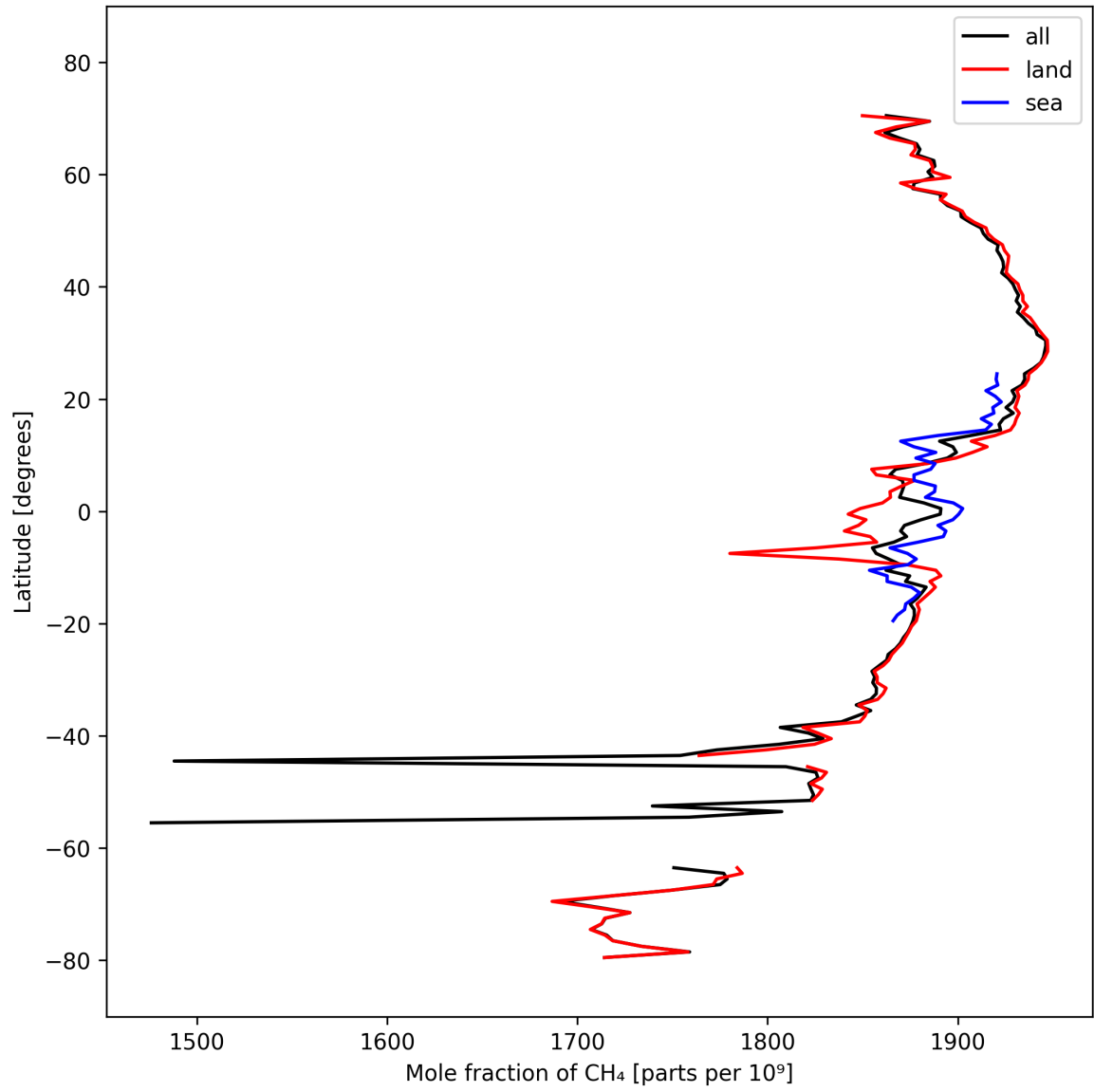
Figure 12: Zonal average of “Mole fraction of \text{CH}_4 ” for 2024-10-03 to 2024-10-05.
