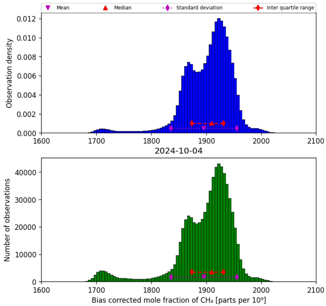
Figure 25: Histogram of “Bias corrected mole fraction of CH 4 ” for 2024-10-03 to 2024-10-05
