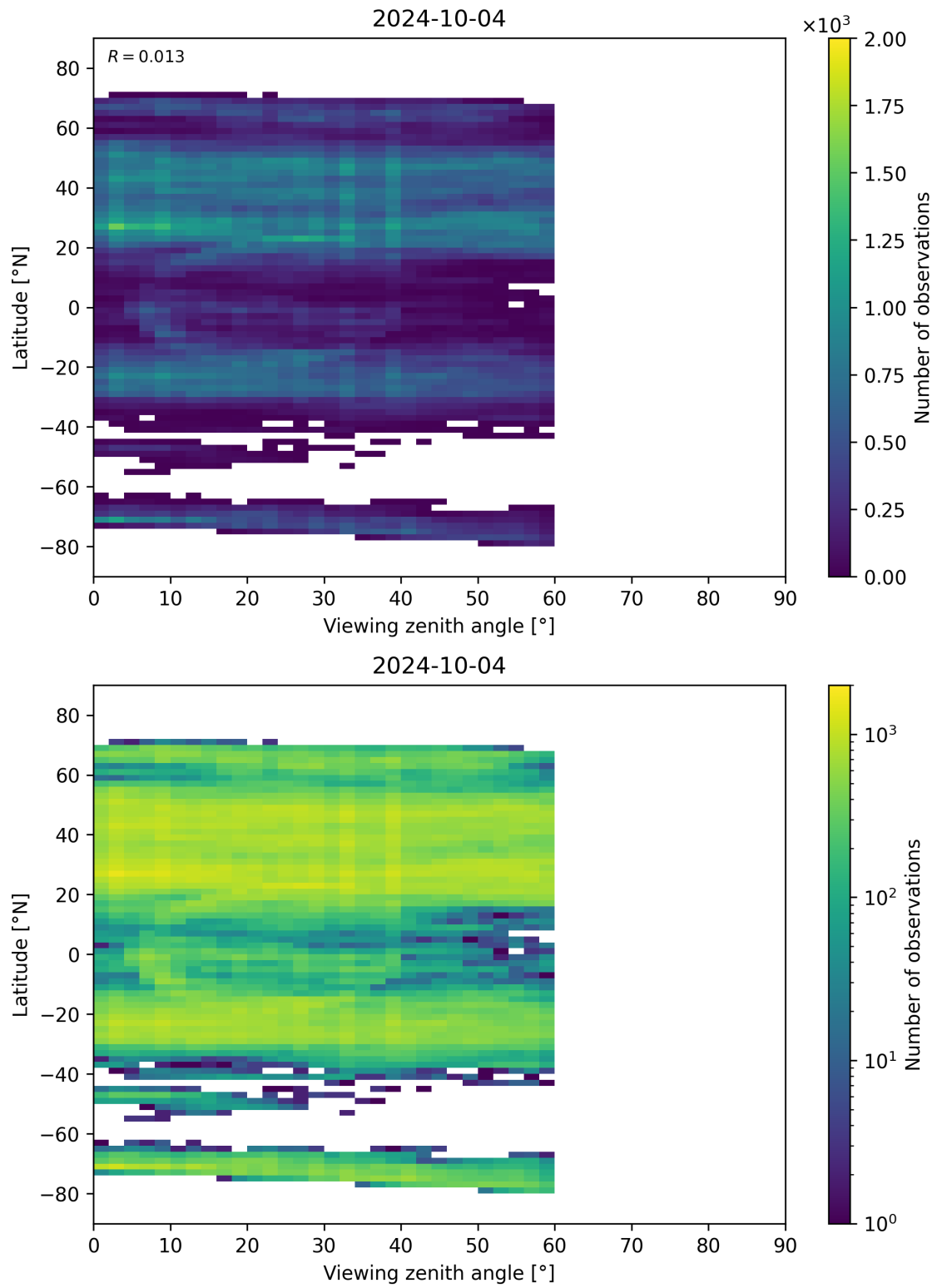
Figure 109: Scatter density plot of “Viewing zenith angle” against “Latitude” for 2024-10-03 to 2024-10-05.
