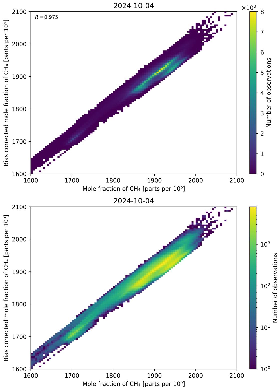
Figure 74: Scatter density plot of “Mole fraction of CH 4 ” against “Bias corrected mole fraction of CH 4 ” for 2024-10-03 to 2024-10-05.
