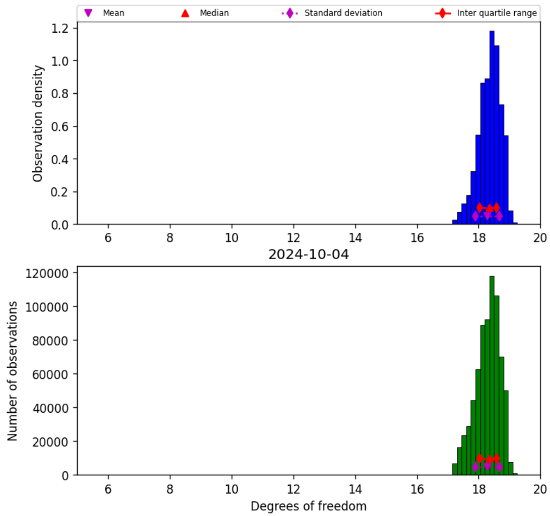
Figure 30: Histogram of “Degrees of freedom” for 2024-10-03 to 2024-10-05
