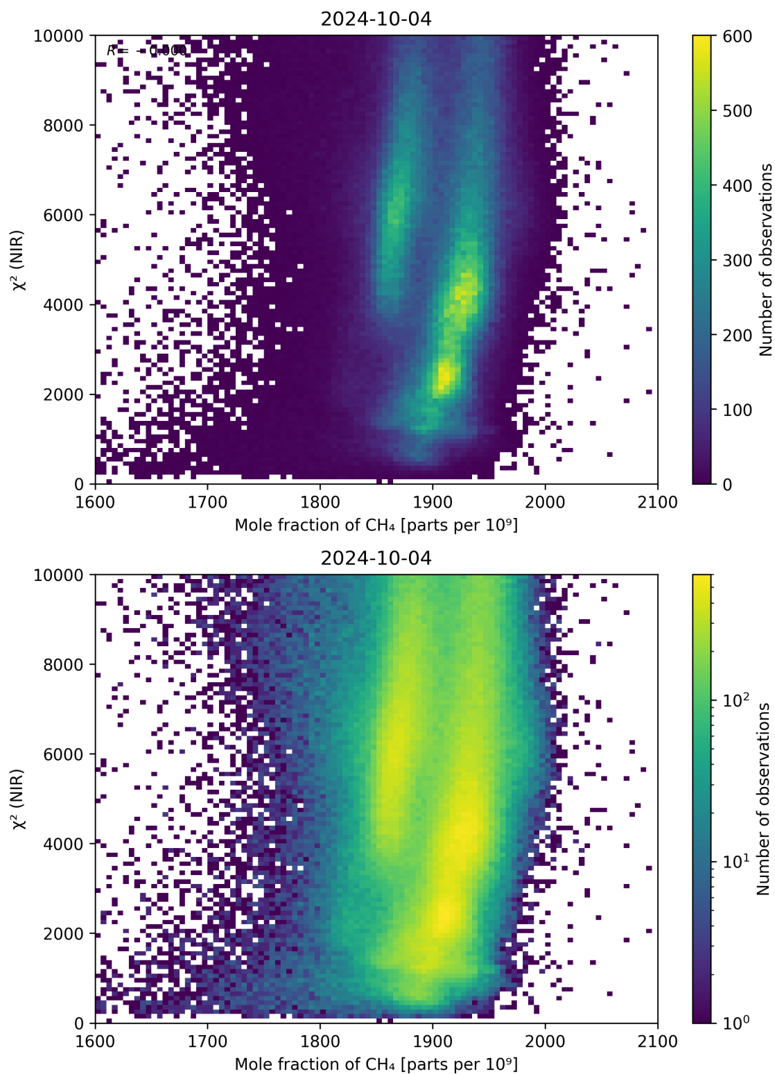
Figure 70: Scatter density plot of “Mole fraction of \text{CH}_4 ” against “ \chi^2 (NIR)” for 2024-10-03 to 2024-10-05.
