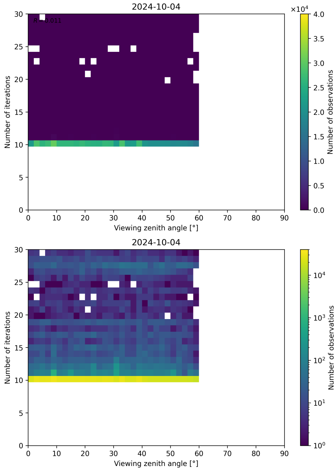
Figure 113: Scatter density plot of “Viewing zenith angle” against “Number of iterations” for 2024-10-03 to 2024-10-05.
