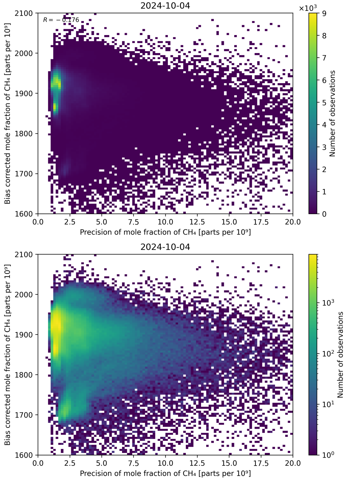
Figure 82: Scatter density plot of “Precision of mole fraction of CH 4 ” against “Bias corrected mole fraction of CH 4 ” for 2024-10-03 to 2024-10-05.
