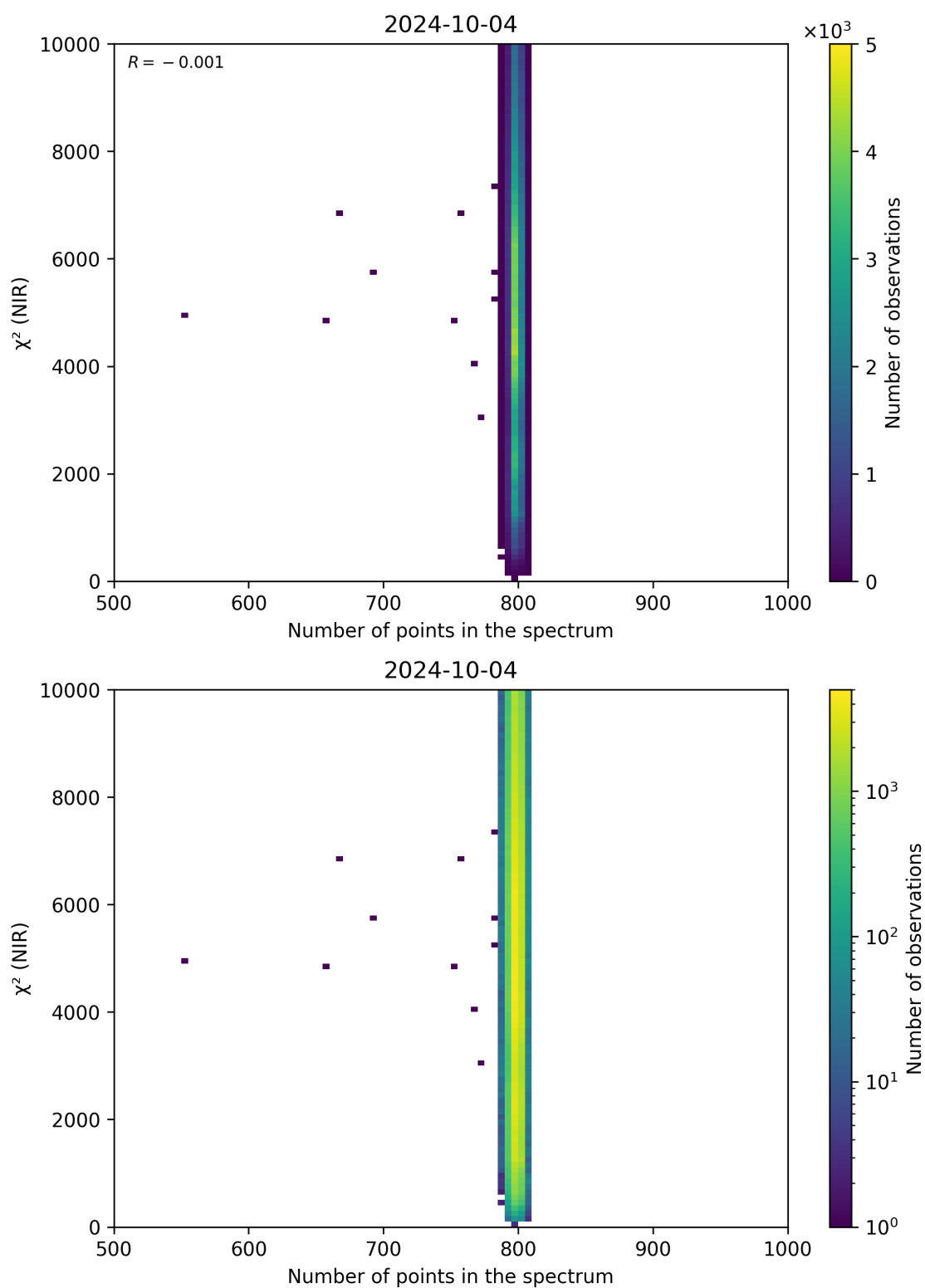
Figure 88: Scatter density plot of “Number of points in the spectrum” against “ \chi^2 (NIR)” for 2024-10-03 to 2024-10-05.
