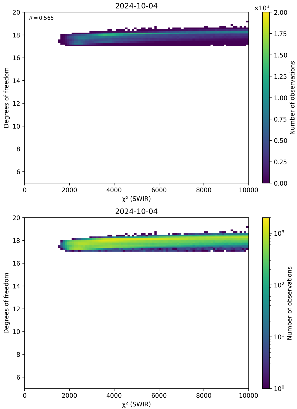
Figure 48: Scatter density plot of “ \chi^2 (SWIR)” against “Degrees of freedom” for 2024-10-03 to 2024-10-05.
