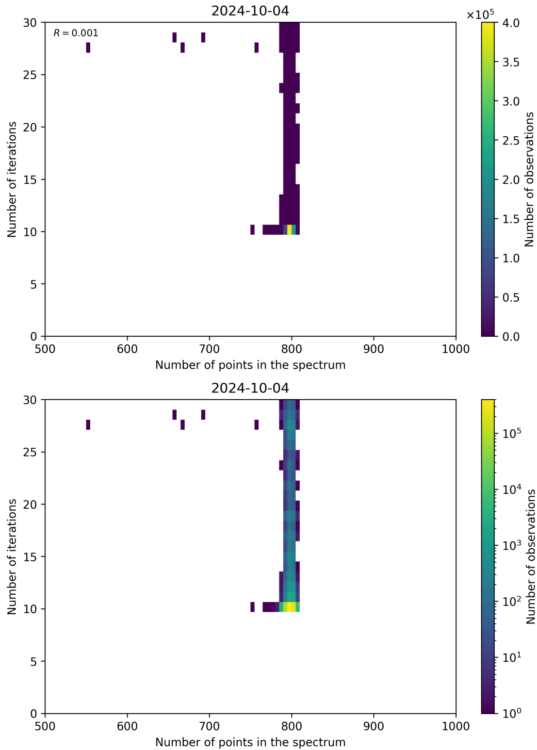
Figure 92: Scatter density plot of “Number of points in the spectrum” against “Number of iterations” for 2024-10-03 to 2024-10-05.
