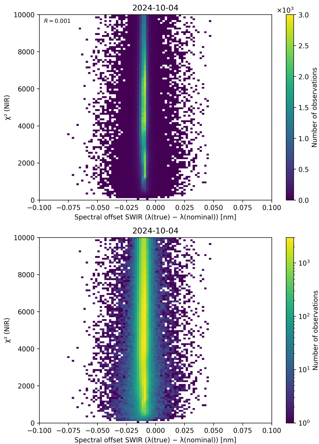
Figure 117: Scatter density plot of “Spectral offset SWIR ( \lambda_{\text{true}} - \lambda_{\text{nominal}} )” against “ \chi^2 (NIR)” for 2024-10-03 to 2024-10-05.
