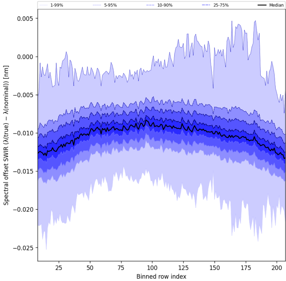
Figure 38: Along track statistics of “Spectral offset SWIR ( \lambda_{\text{true}} - \lambda_{\text{nominal}} )” for 2024-10-03 to 2024-10-05
