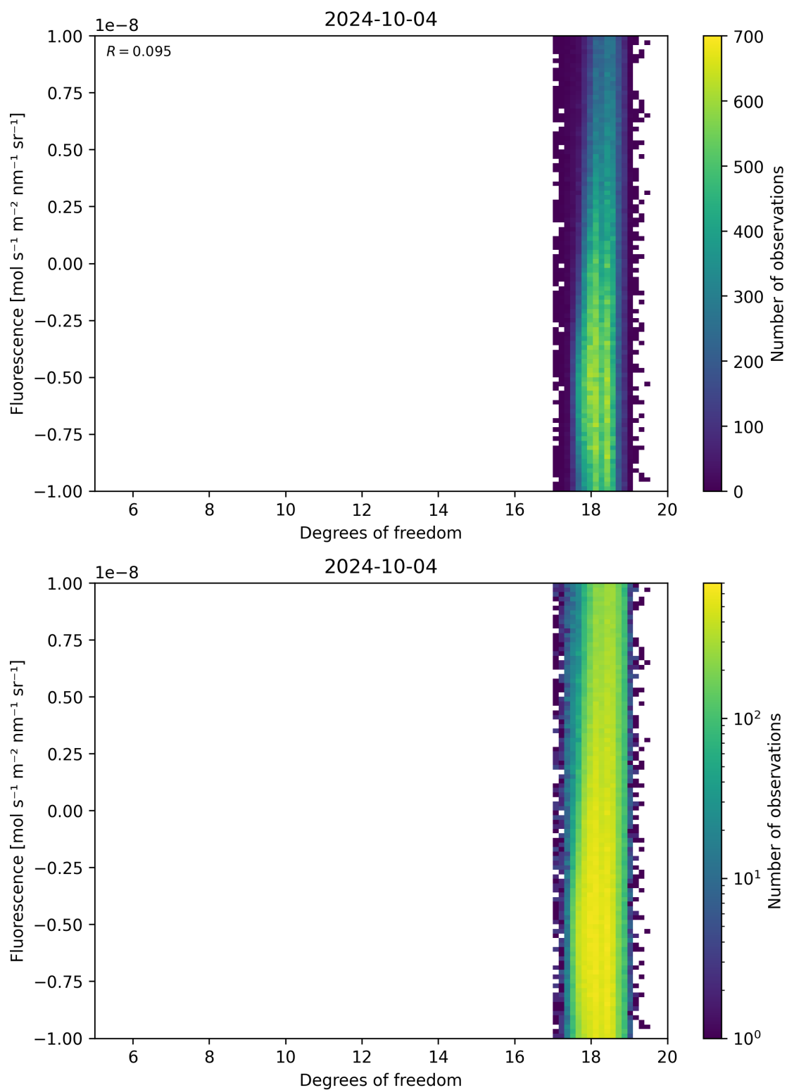
Figure 51: Scatter density plot of “Degrees of freedom” against “Fluorescence” for 2024-10-03 to 2024-10-05.
