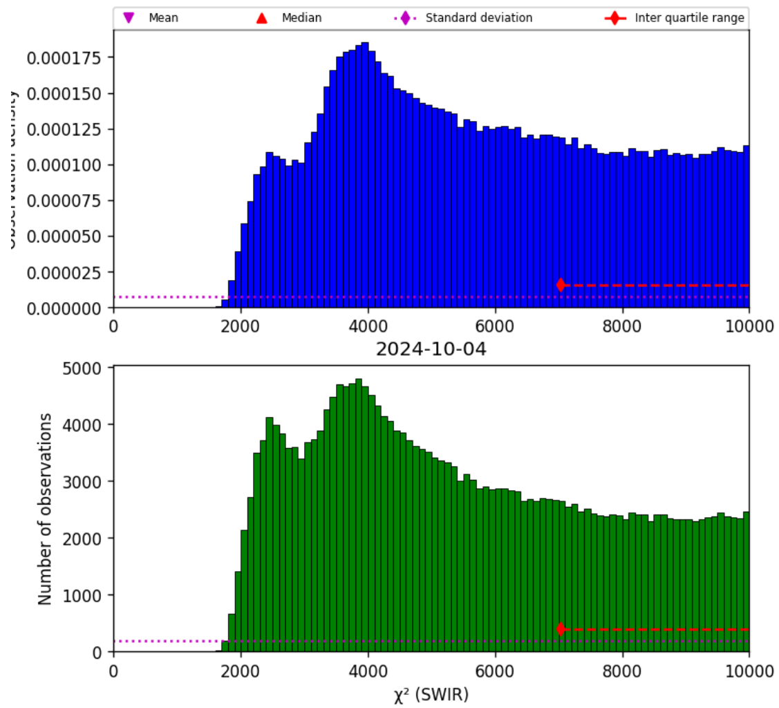
Figure 28: Histogram of “ \chi^2 (SWIR)” for 2024-10-03 to 2024-10-05
