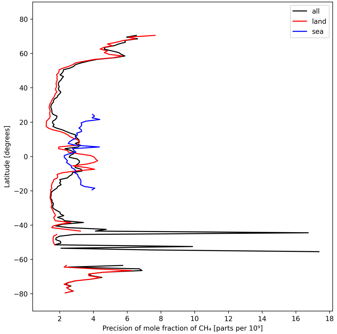
Figure 13: Zonal average of “Precision of mole fraction of CH 4 ” for 2024-10-03 to 2024-10-05.
