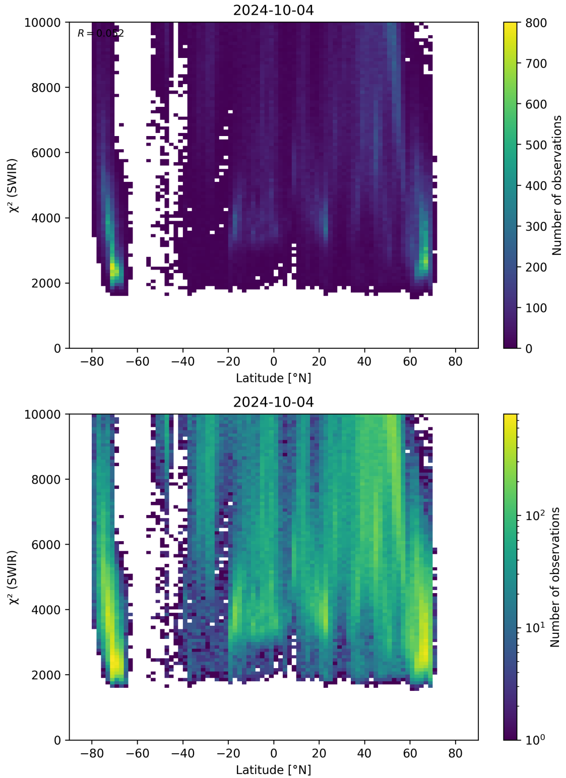
Figure 54: Scatter density plot of “Latitude” against “ \chi^2 (SWIR)” for 2024-10-03 to 2024-10-05.
