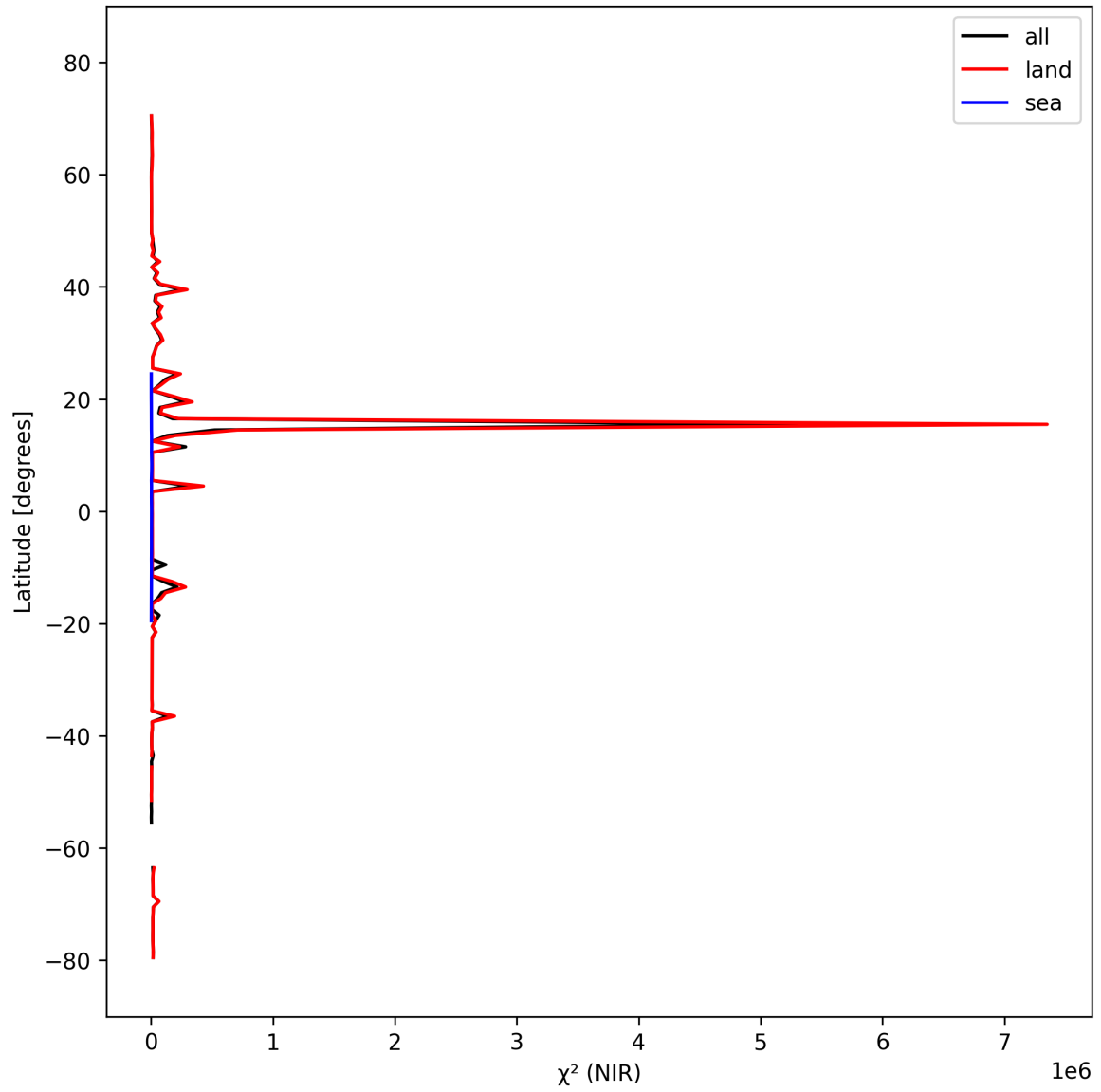
Figure 18: Zonal average of “ \chi^2 (NIR)” for 2024-10-03 to 2024-10-05.
