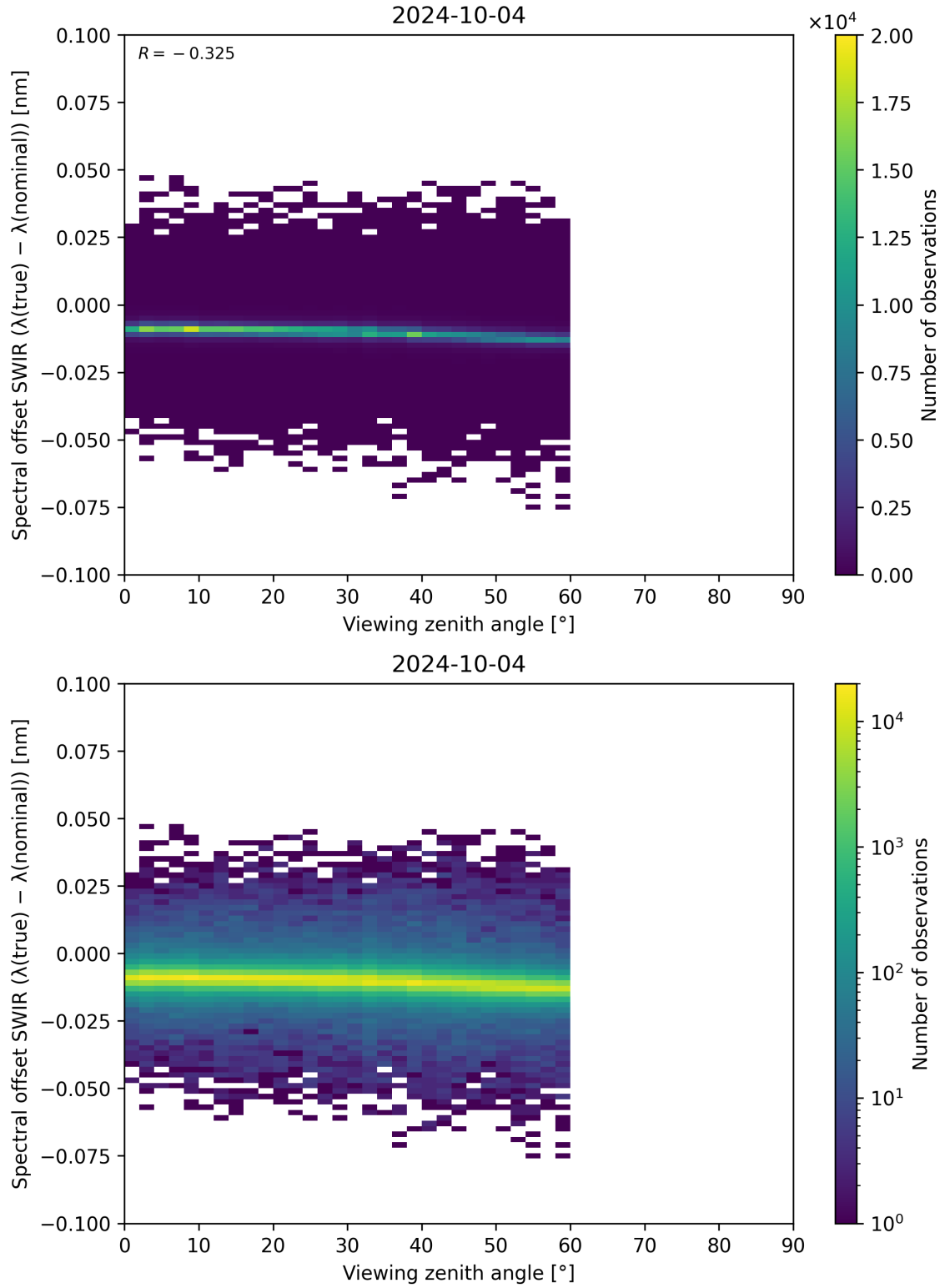
Figure 116: Scatter density plot of “Viewing zenith angle” against “Spectral offset SWIR ( \lambda_{\text{true}} - \lambda_{\text{nominal}} )” for 2024-10-03 to 2024-10-05.
