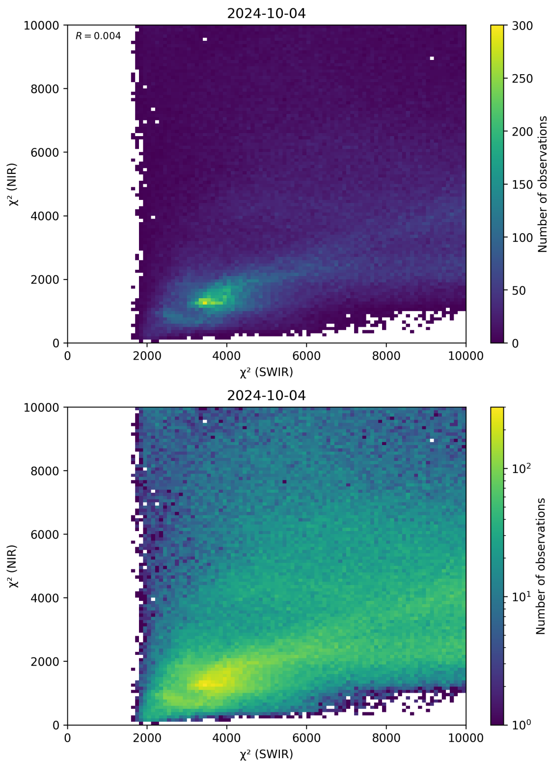
Figure 47: Scatter density plot of “ \chi^2 (SWIR)” against “ \chi^2 (NIR)” for 2024-10-03 to 2024-10-05.
