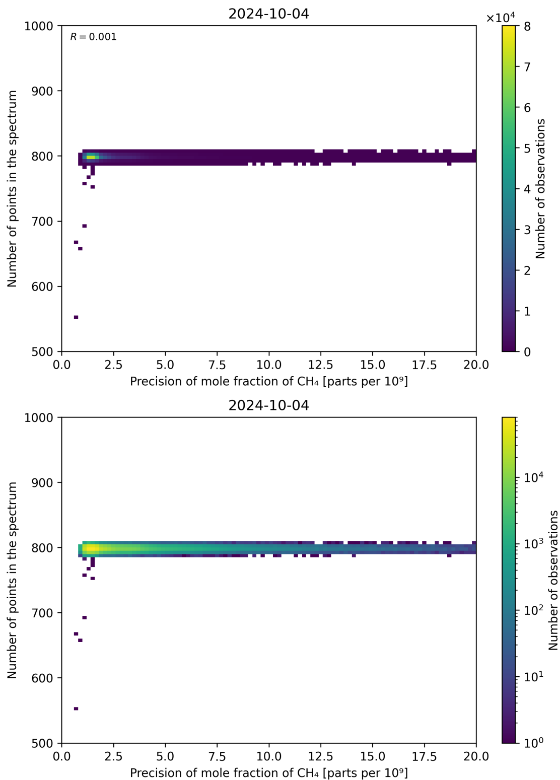
Figure 84: Scatter density plot of “Precision of mole fraction of CH 4 ” against “Number of points in the spectrum” for 2024-10-03 to 2024-10-05.
