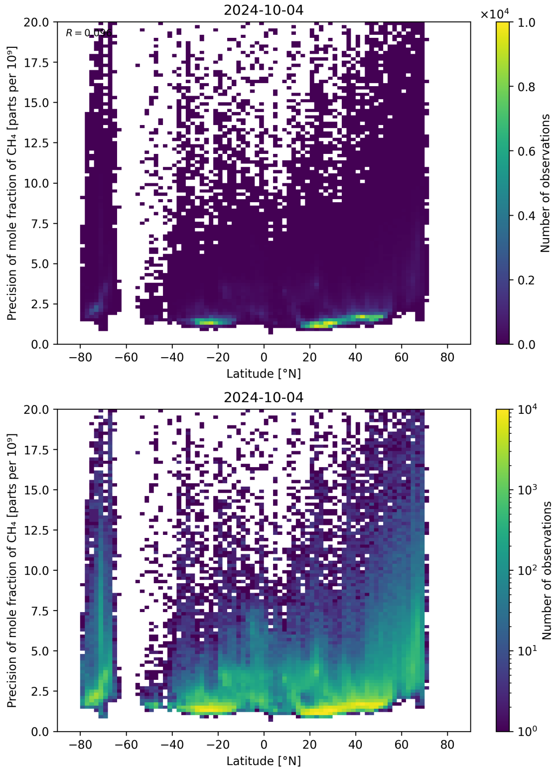
Figure 59: Scatter density plot of “Latitude” against “Precision of mole fraction of CH 4 ” for 2024-10-03 to 2024-10-05.
