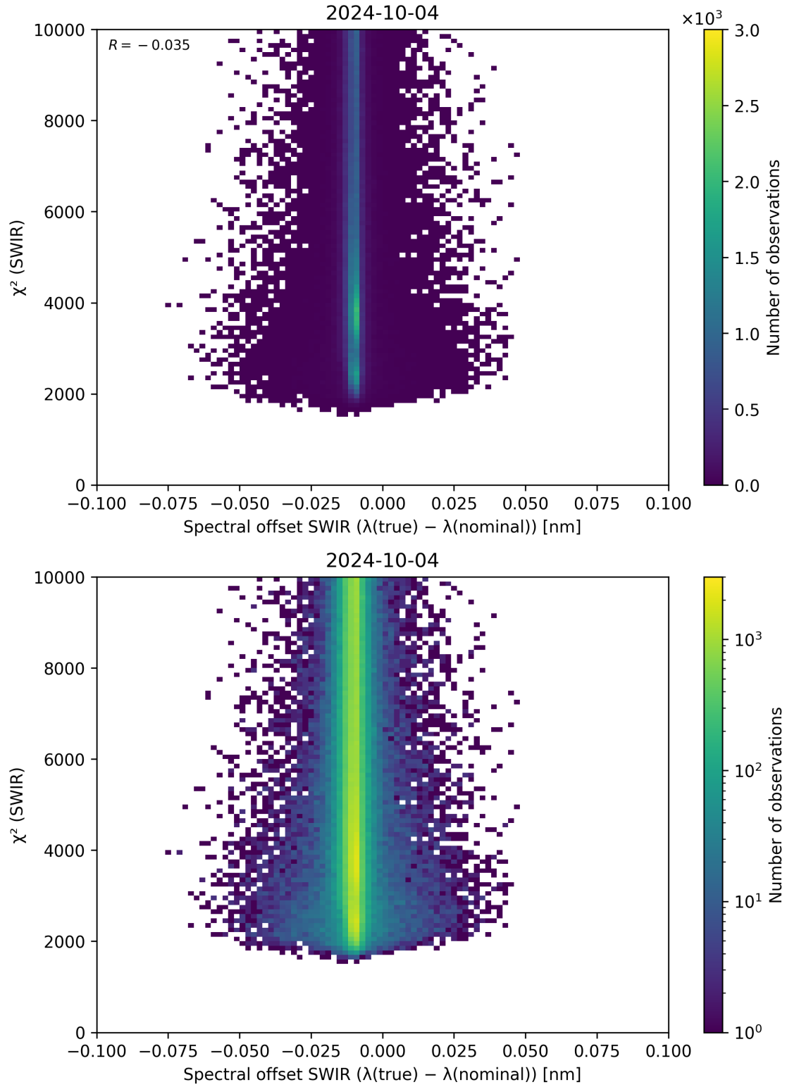
Figure 118: Scatter density plot of “Spectral offset SWIR ( \lambda_{\text{true}} - \lambda_{\text{nominal}} )” against “ \chi^2 (SWIR)” for 2024-10-03 to 2024-10-05.
