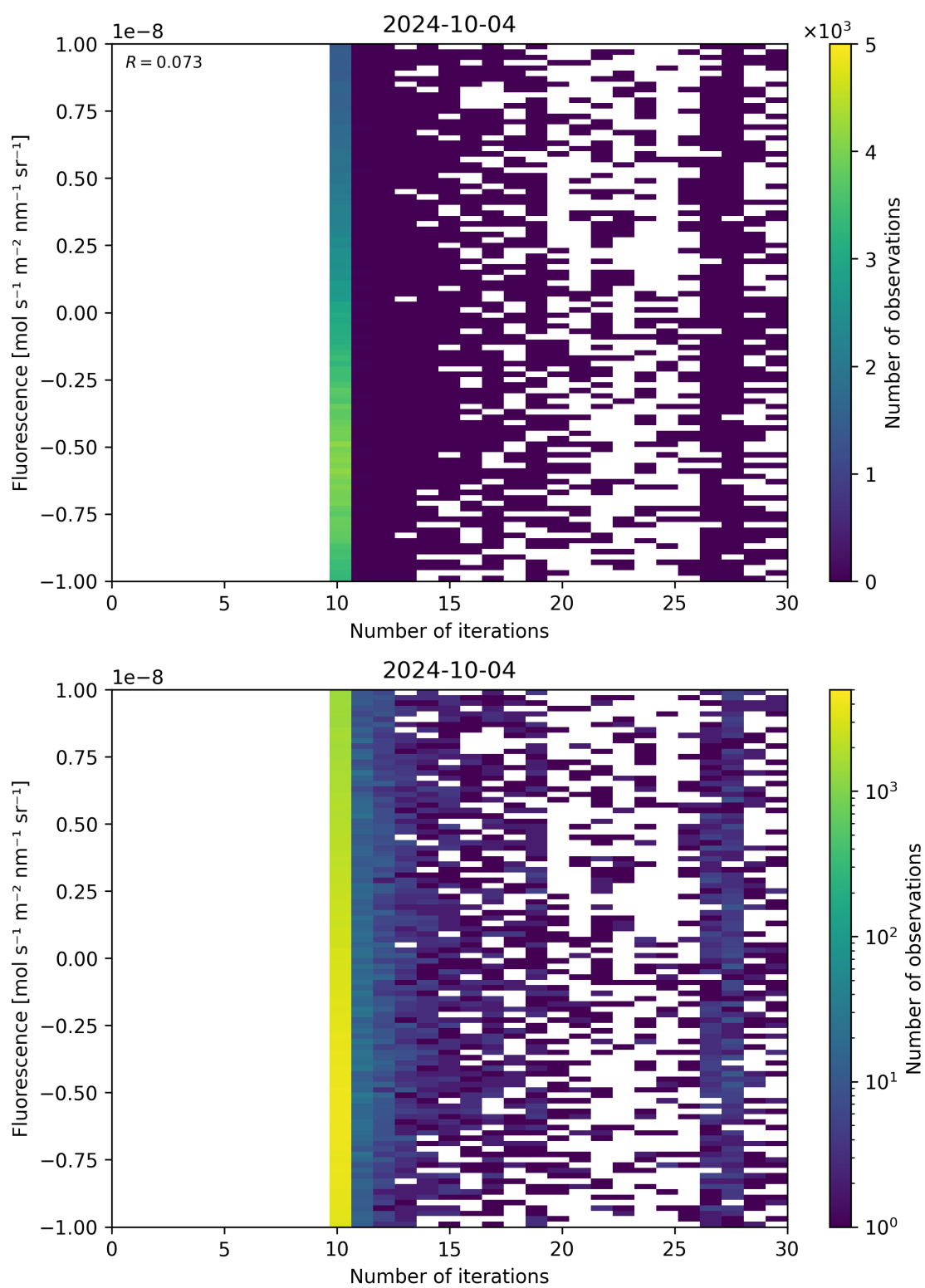
Figure 87: Scatter density plot of “Number of iterations” against “Fluorescence” for 2024-10-03 to 2024-10-05.
