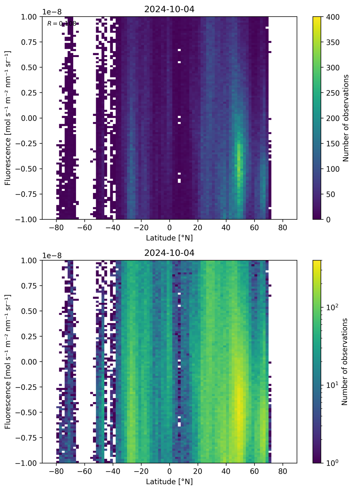
Figure 56: Scatter density plot of “Latitude” against “Fluorescence” for 2024-10-03 to 2024-10-05.
