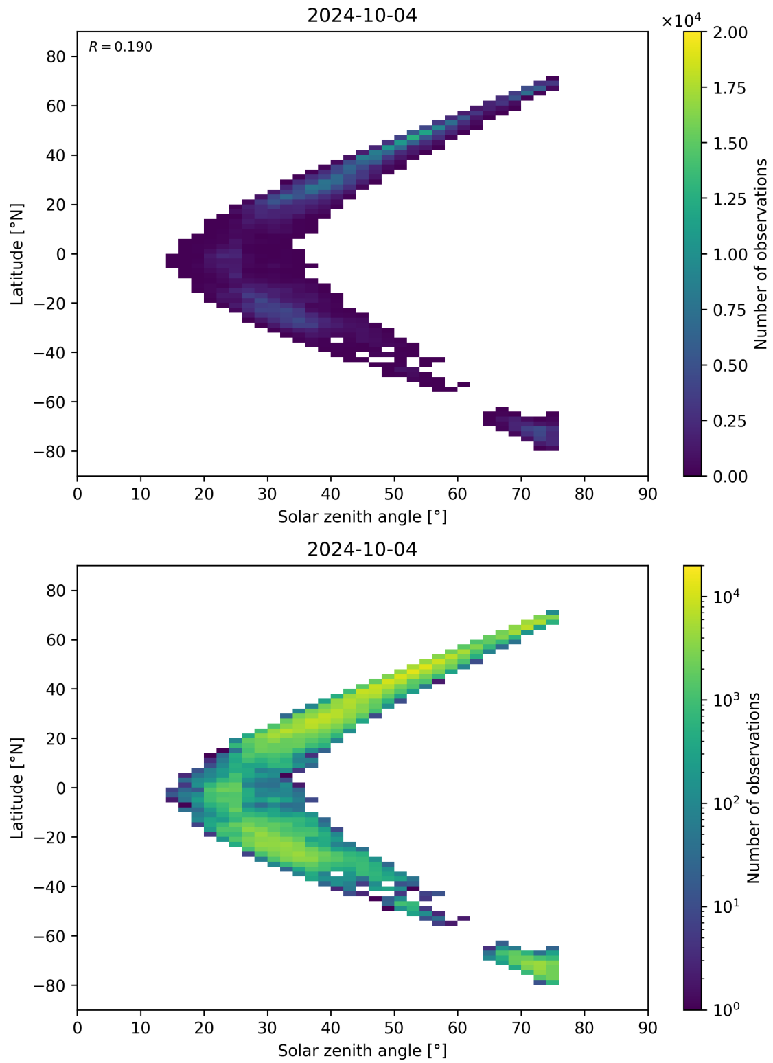
Figure 98: Scatter density plot of “Solar zenith angle” against “Latitude” for 2024-10-03 to 2024-10-05.
