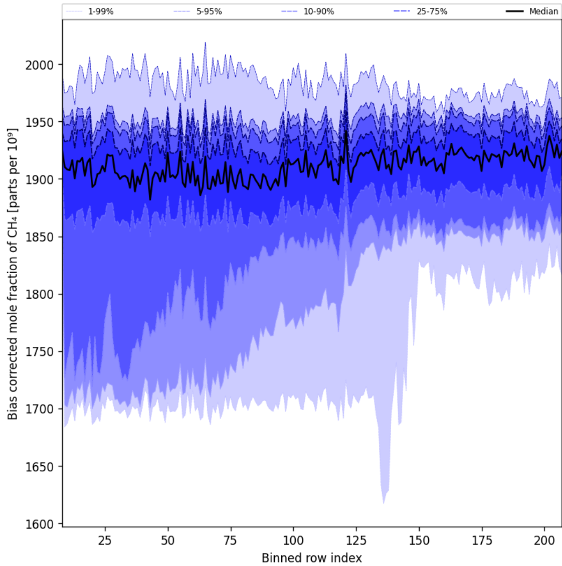
Figure 36: Along track statistics of “Bias corrected mole fraction of CH 4 ” for 2024-10-03 to 2024-10-05
