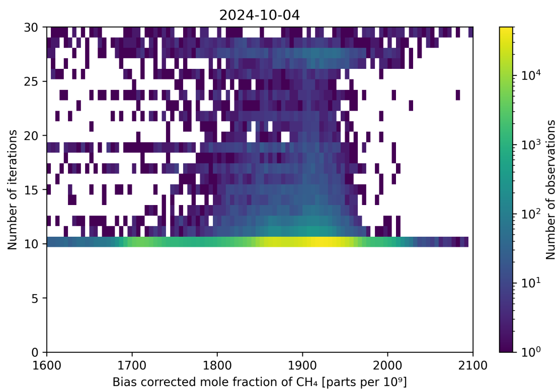
Figure 67: Scatter density plot of “Bias corrected mole fraction of \text{CH}_4 ” against “Number of iterations” for 2024-10-03 to 2024-10-05.
