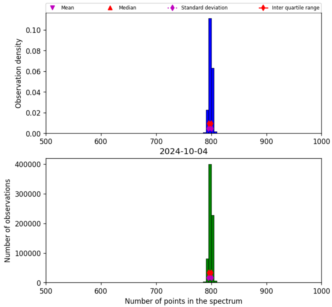
Figure 26: Histogram of “Number of points in the spectrum” for 2024-10-03 to 2024-10-05
