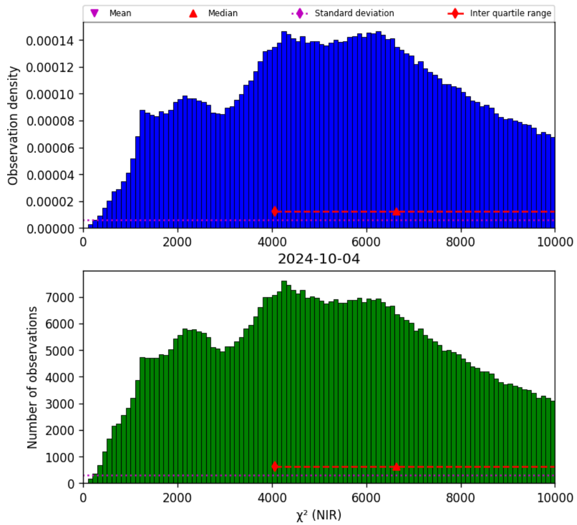
Figure 29: Histogram of " \chi^2 (NIR)" for 2024-10-03 to 2024-10-05
