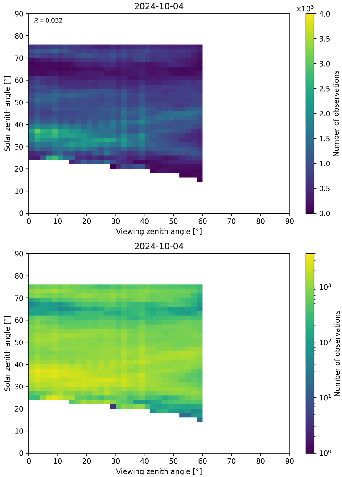
Figure 115: Scatter density plot of “Viewing zenith angle” against “Solar zenith angle” for 2024-10-03 to 2024-10-05.
