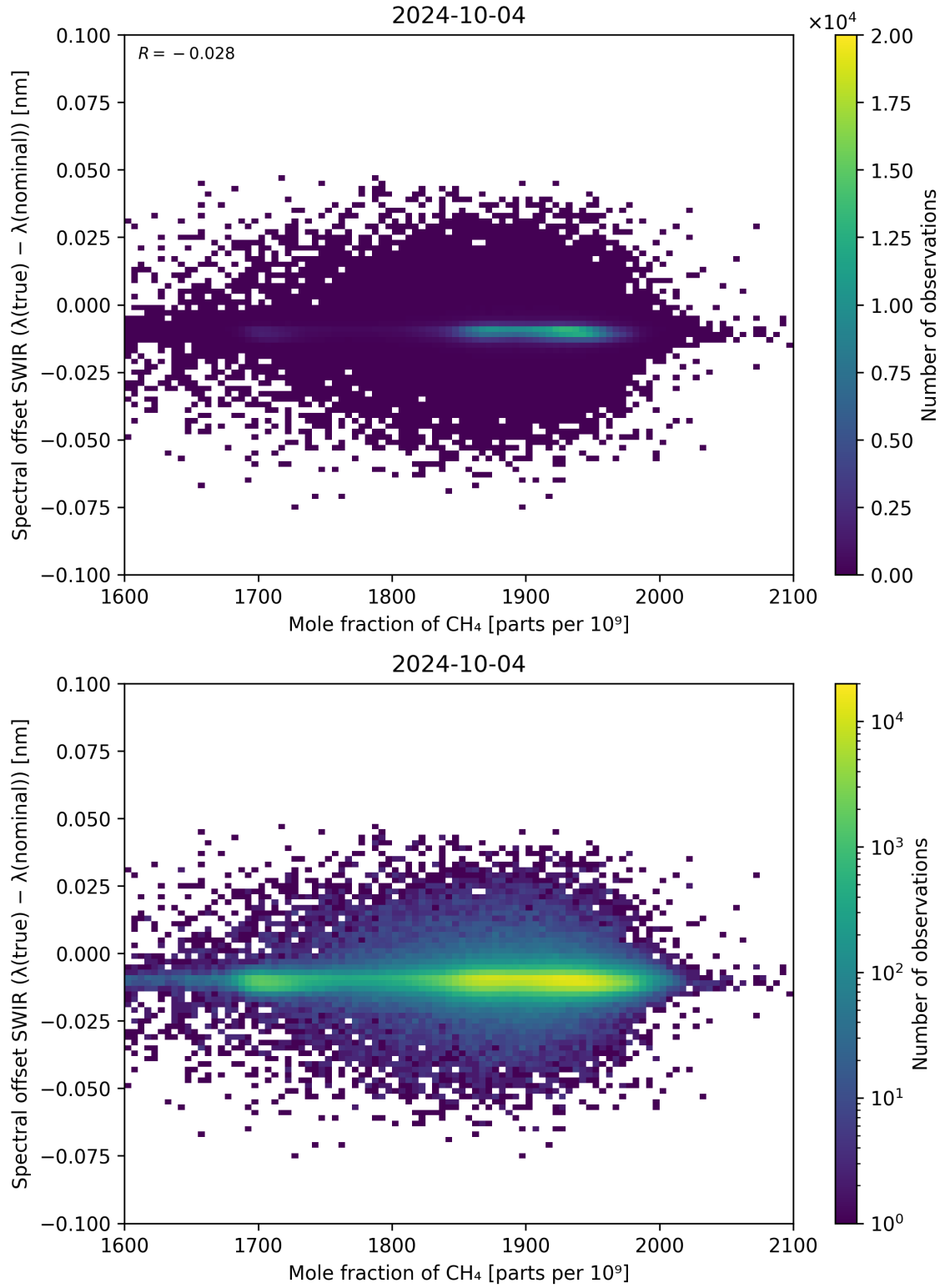
Figure 86: Scatter density plot of “Mole fraction of \text{CH}_4 ” against “Spectral offset SWIR ( \lambda_{\text{true}} - \lambda_{\text{nominal}} )” for 2024-10-03 to 2024-10-05.
