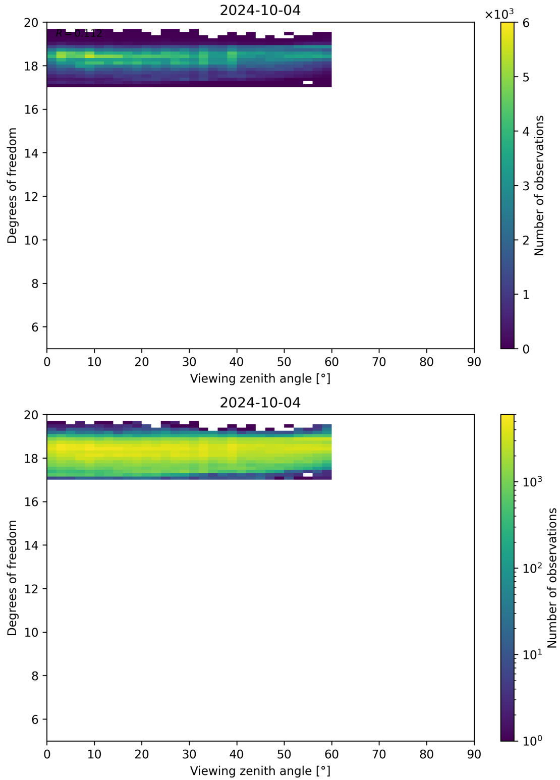
Figure 107: Scatter density plot of “Viewing zenith angle” against “Degrees of freedom” for 2024-10-03 to 2024-10-05.
