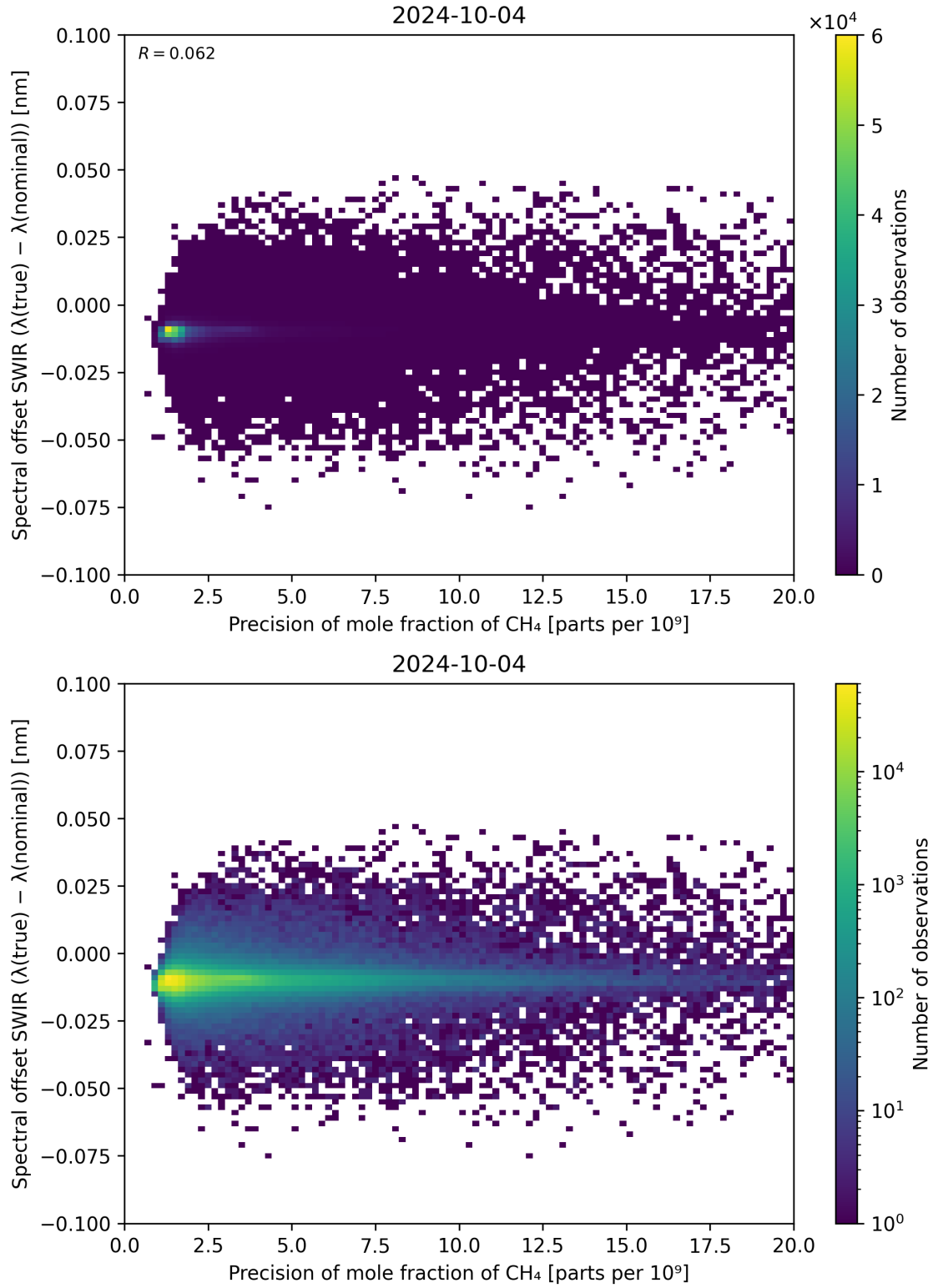
Figure 85: Scatter density plot of “Precision of mole fraction of CH 4 ” against “Spectral offset SWIR ( \lambda_{\text{true}} - \lambda_{\text{nominal}} )” for 2024-10-03 to 2024-10-05.
