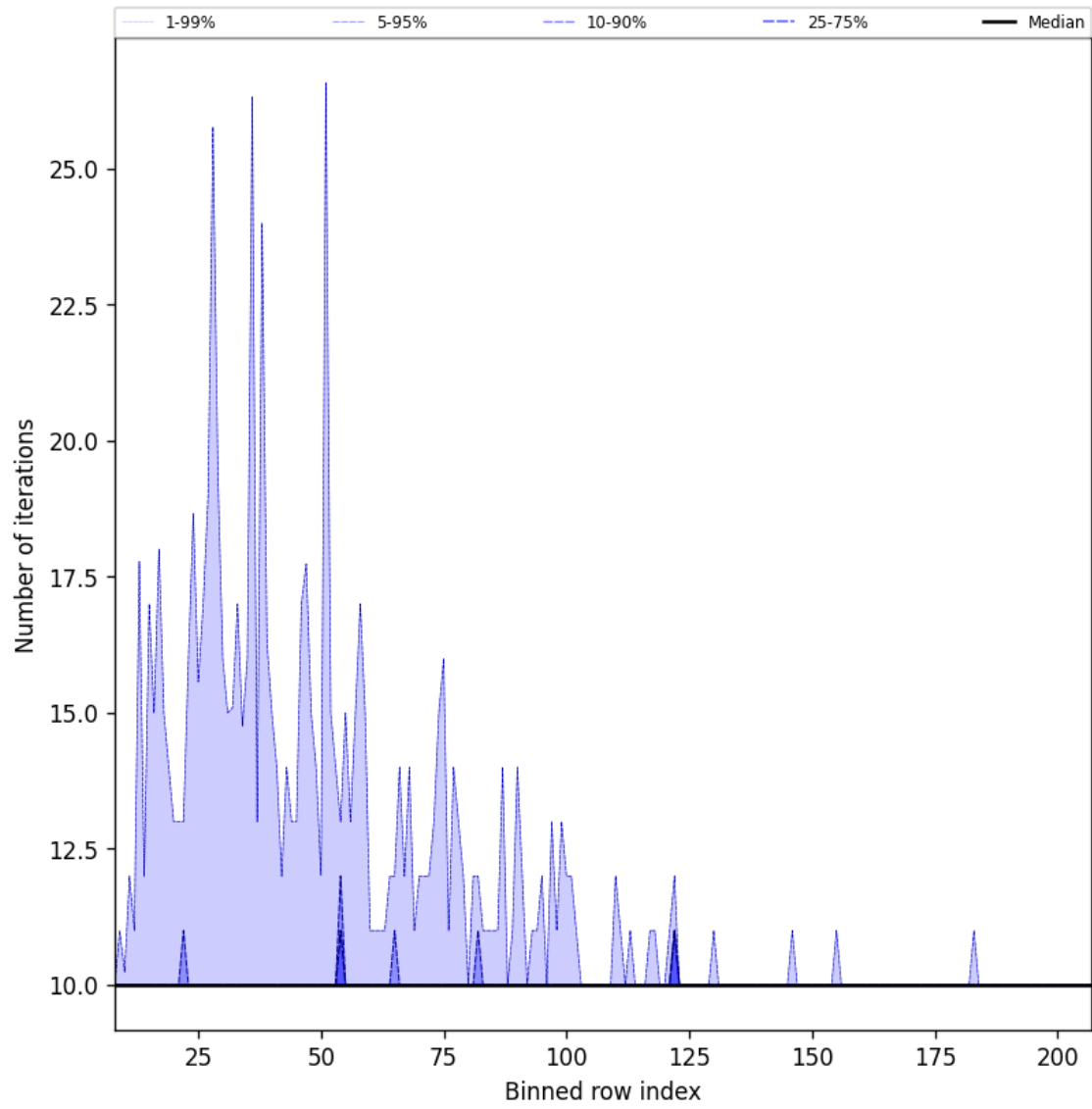
Figure 42: Along track statistics of “Number of iterations” for 2024-10-03 to 2024-10-05
