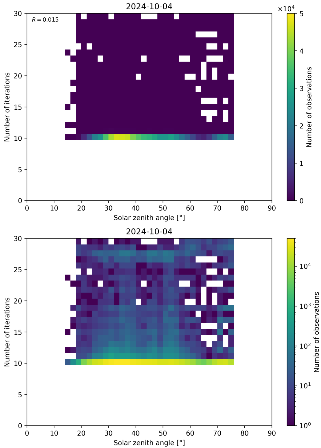
Figure 102: Scatter density plot of “Solar zenith angle” against “Number of iterations” for 2024-10-03 to 2024-10-05.
