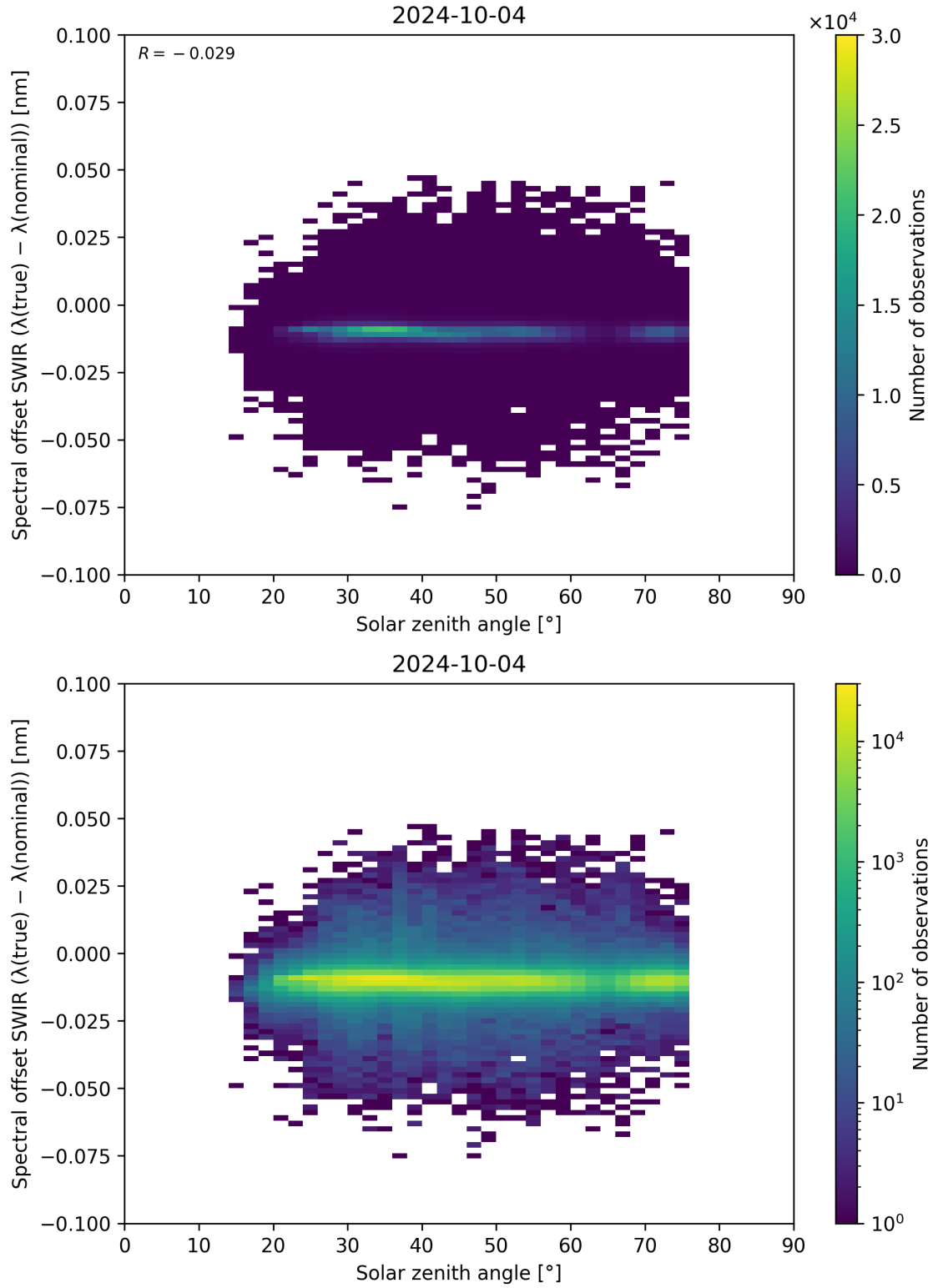
Figure 104: Scatter density plot of “Solar zenith angle” against “Spectral offset SWIR ( \lambda_{\text{true}} - \lambda_{\text{nominal}} )” for 2024-10-03 to 2024-10-05.
