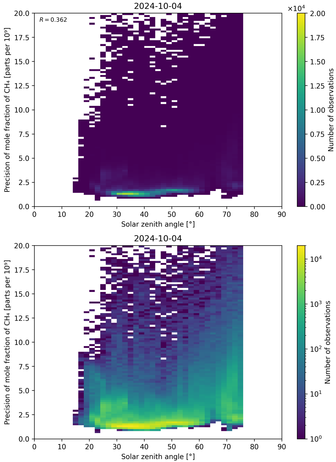
Figure 101: Scatter density plot of “Solar zenith angle” against “Precision of mole fraction of \text{CH}_4 ” for 2024-10-03 to 2024-10-05.
