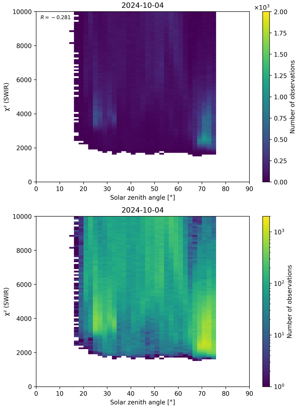
Figure 95: Scatter density plot of “Solar zenith angle” against “ \chi^2 (SWIR)” for 2024-10-03 to 2024-10-05.
