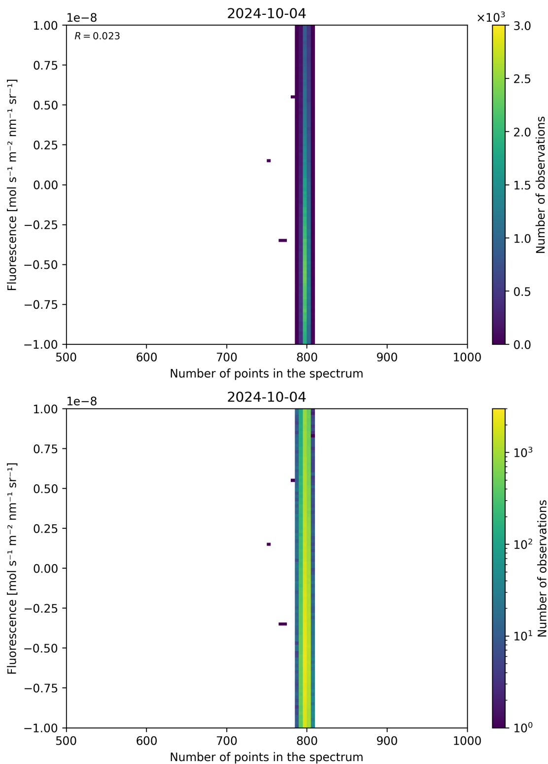
Figure 91: Scatter density plot of “Number of points in the spectrum” against “Fluorescence” for 2024-10-03 to 2024-10-05.
