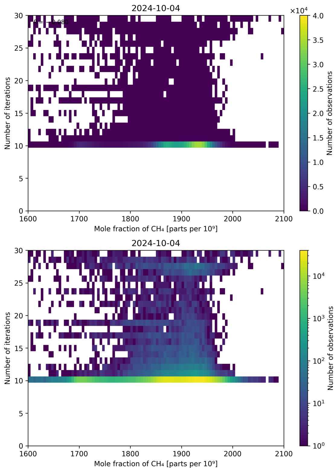
Figure 76: Scatter density plot of “Mole fraction of CH 4 ” against “Number of iterations” for 2024-10-03 to 2024-10-05.
