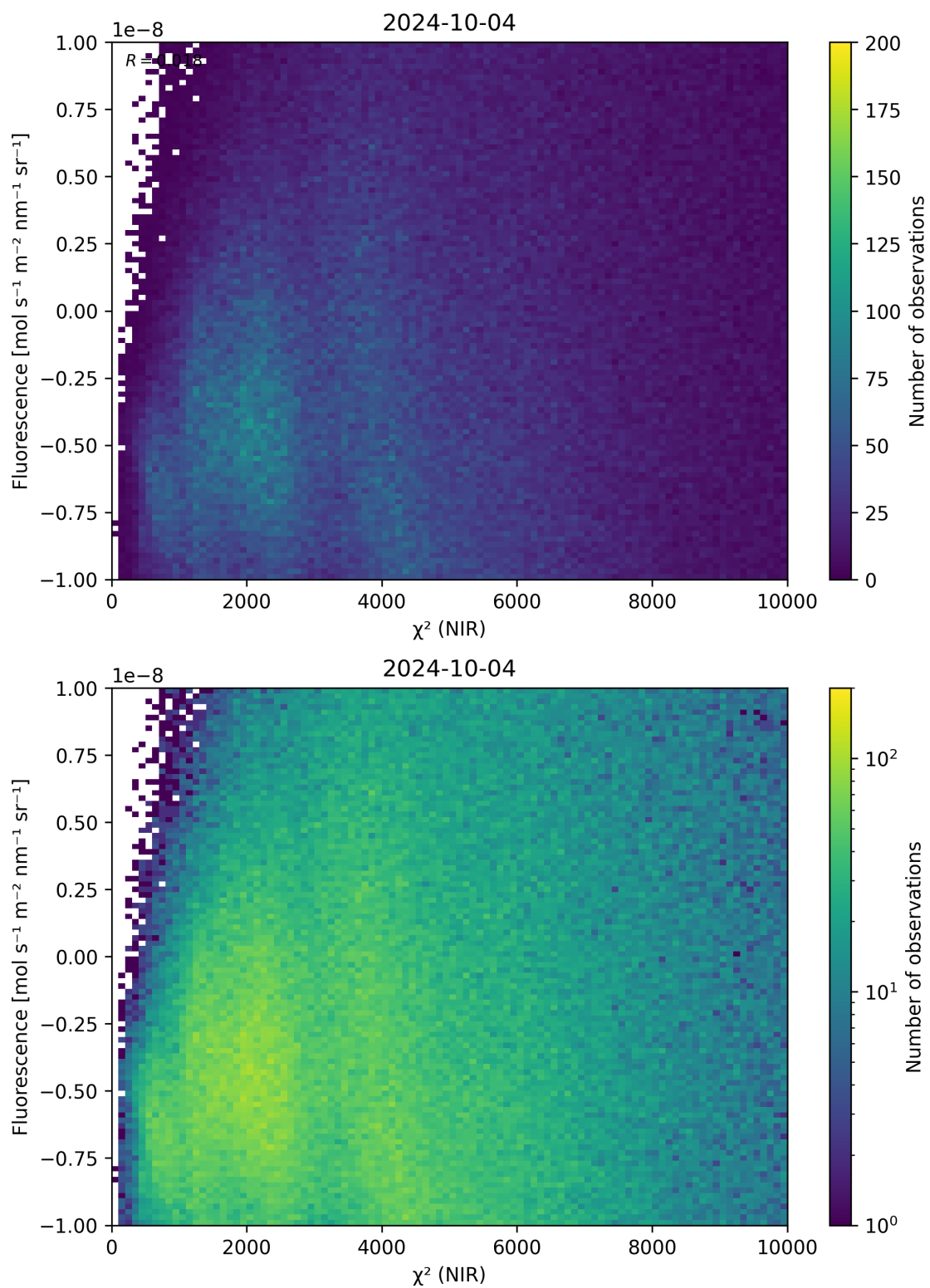
Figure 45: Scatter density plot of “ \chi^2 (NIR)” against “Fluorescence” for 2024-10-03 to 2024-10-05.
