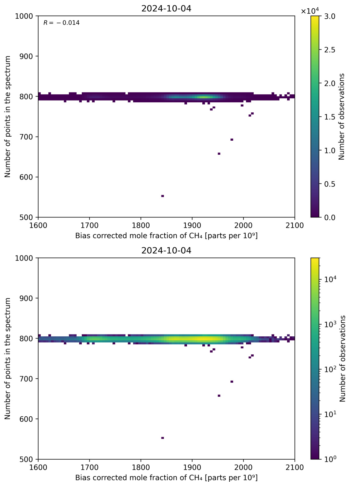
Figure 68: Scatter density plot of “Bias corrected mole fraction of CH 4 ” against “Number of points in the spectrum” for 2024-10-03 to 2024-10-05.
