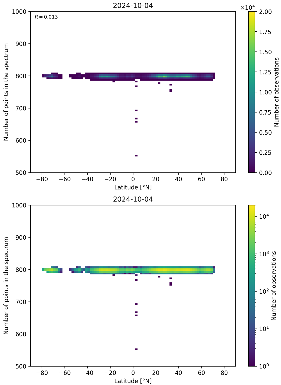
Figure 61: Scatter density plot of “Latitude” against “Number of points in the spectrum” for 2024-10-03 to 2024-10-05.
