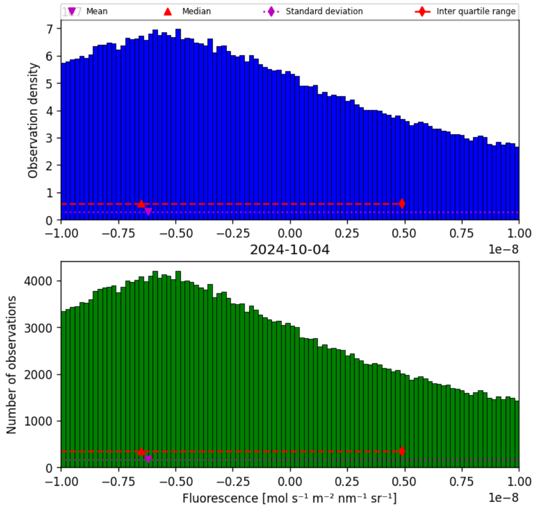
Figure 32: Histogram of “Fluorescence” for 2024-10-03 to 2024-10-05
