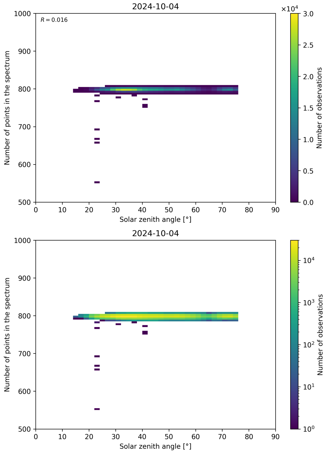
Figure 103: Scatter density plot of “Solar zenith angle” against “Number of points in the spectrum” for 2024-10-03 to 2024-10-05.
