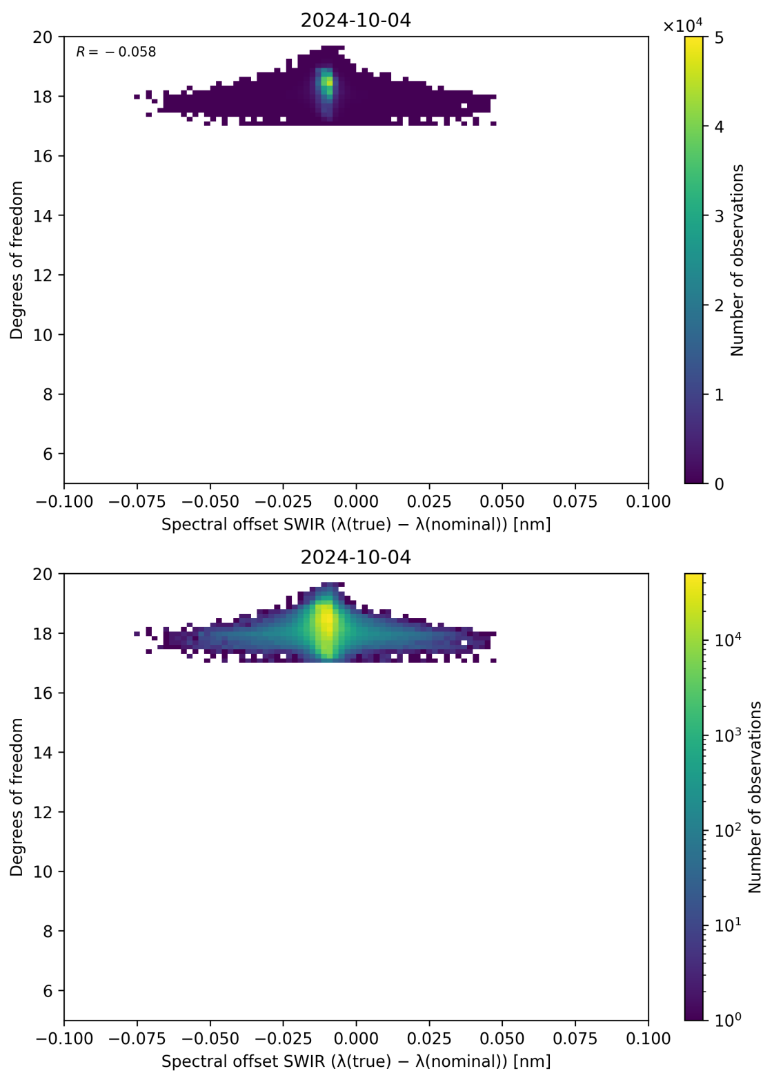
Figure 119: Scatter density plot of “Spectral offset SWIR ( \lambda_{\text{true}} - \lambda_{\text{nominal}} )” against “Degrees of freedom” for 2024-10-03 to 2024-10-05.
