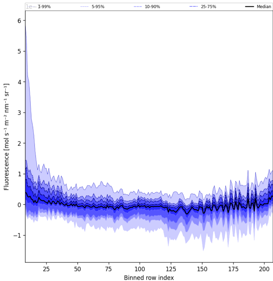
Figure 43: Along track statistics of “Fluorescence” for 2024-10-03 to 2024-10-05
