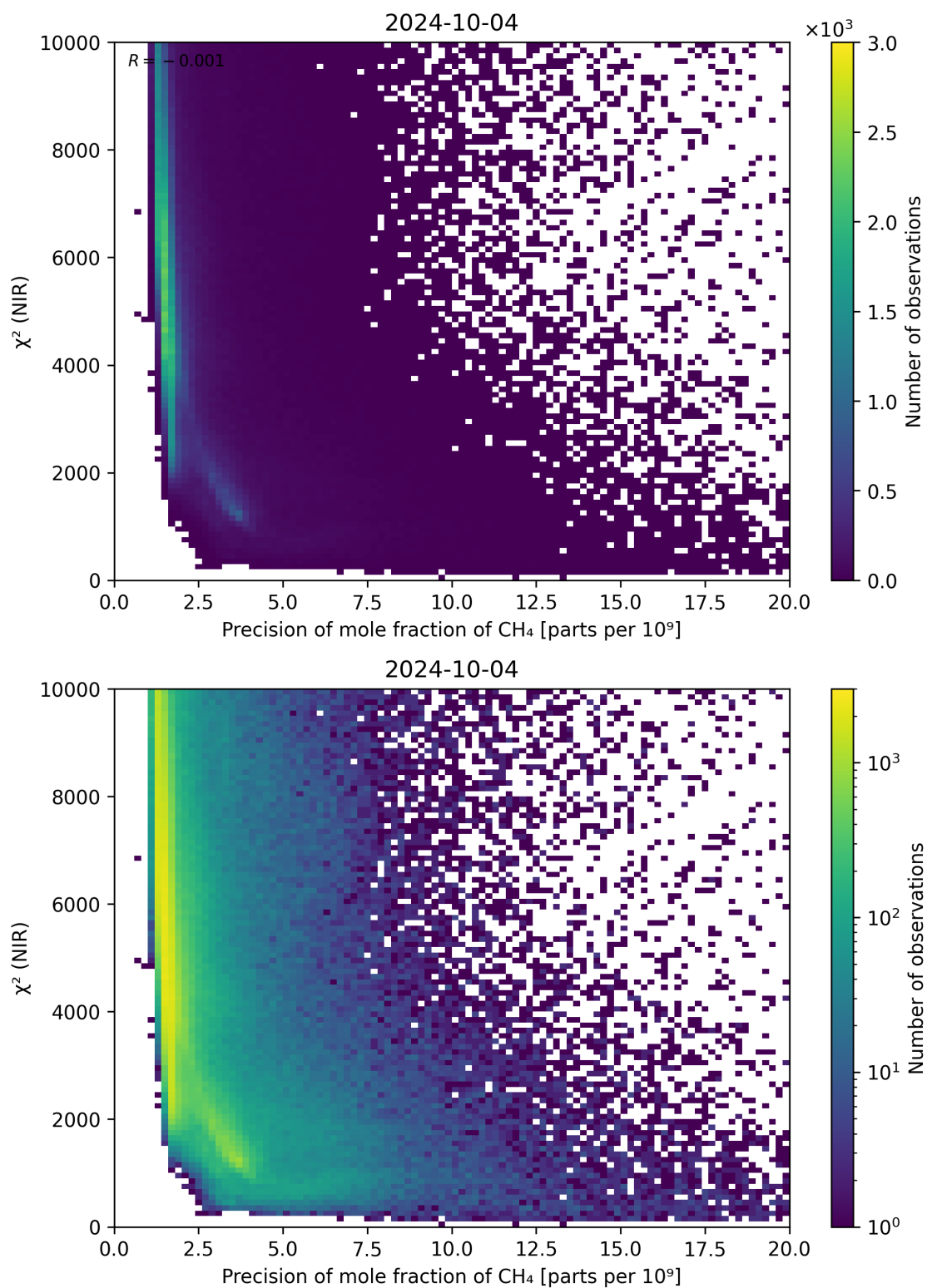
Figure 78: Scatter density plot of “Precision of mole fraction of \text{CH}_4 ” against “ \chi^2 (NIR)” for 2024-10-03 to 2024-10-05.
