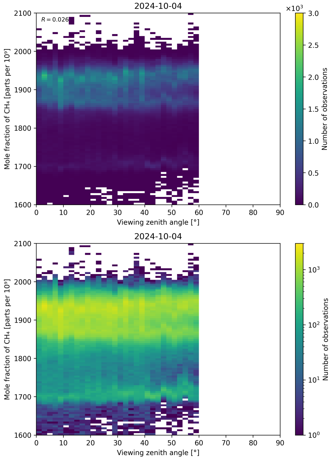
Figure 110: Scatter density plot of “Viewing zenith angle” against “Mole fraction of CH 4 ” for 2024-10-03 to 2024-10-05.
