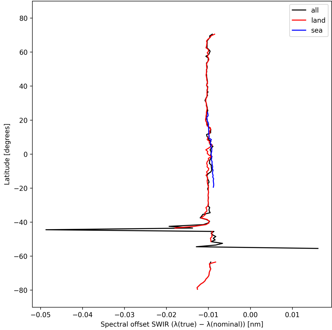
Figure 16: Zonal average of “Spectral offset SWIR ( \lambda_{\text{true}} - \lambda_{\text{nominal}} )” for 2024-10-03 to 2024-10-05.
