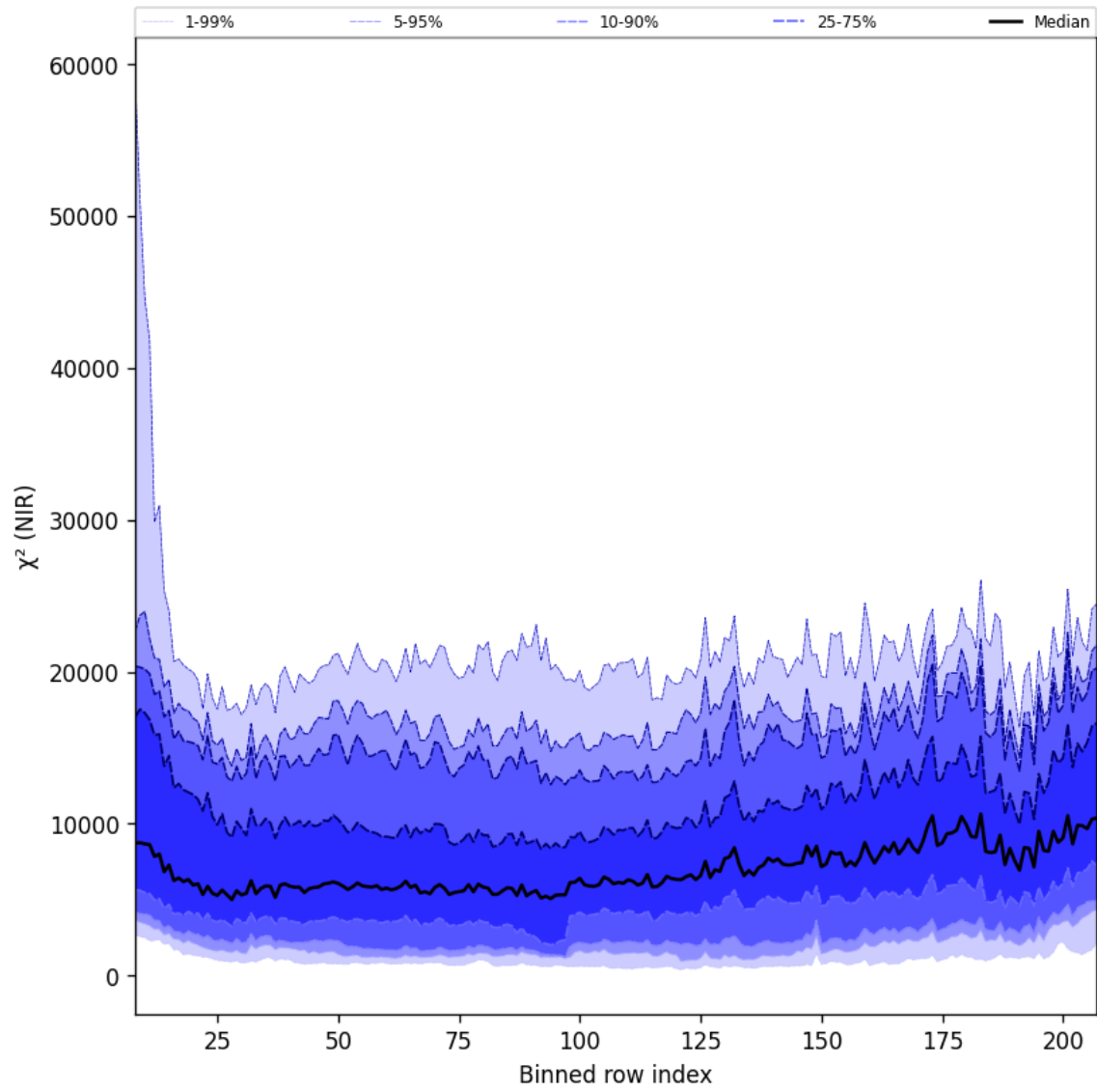
Figure 40: Along track statistics of “ \chi^2 (NIR)” for 2024-10-03 to 2024-10-05
