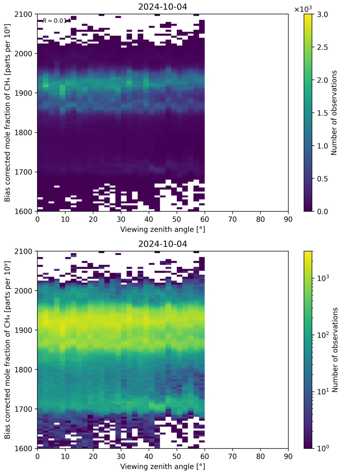
Figure 111: Scatter density plot of “Viewing zenith angle” against “Bias corrected mole fraction of CH 4 ” for 2024-10-03 to 2024-10-05.
