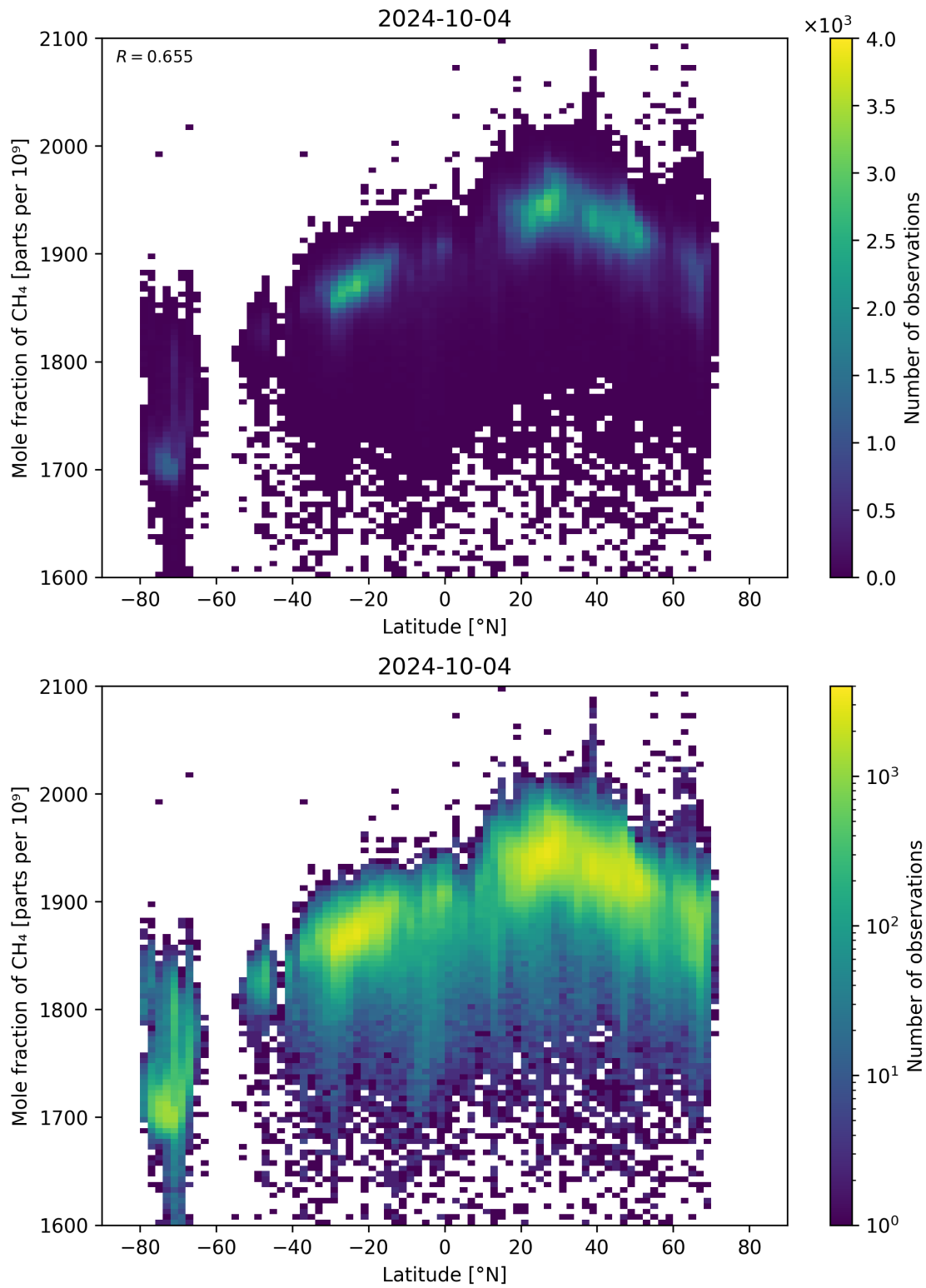
Figure 57: Scatter density plot of “Latitude” against “Mole fraction of CH 4 ” for 2024-10-03 to 2024-10-05.
