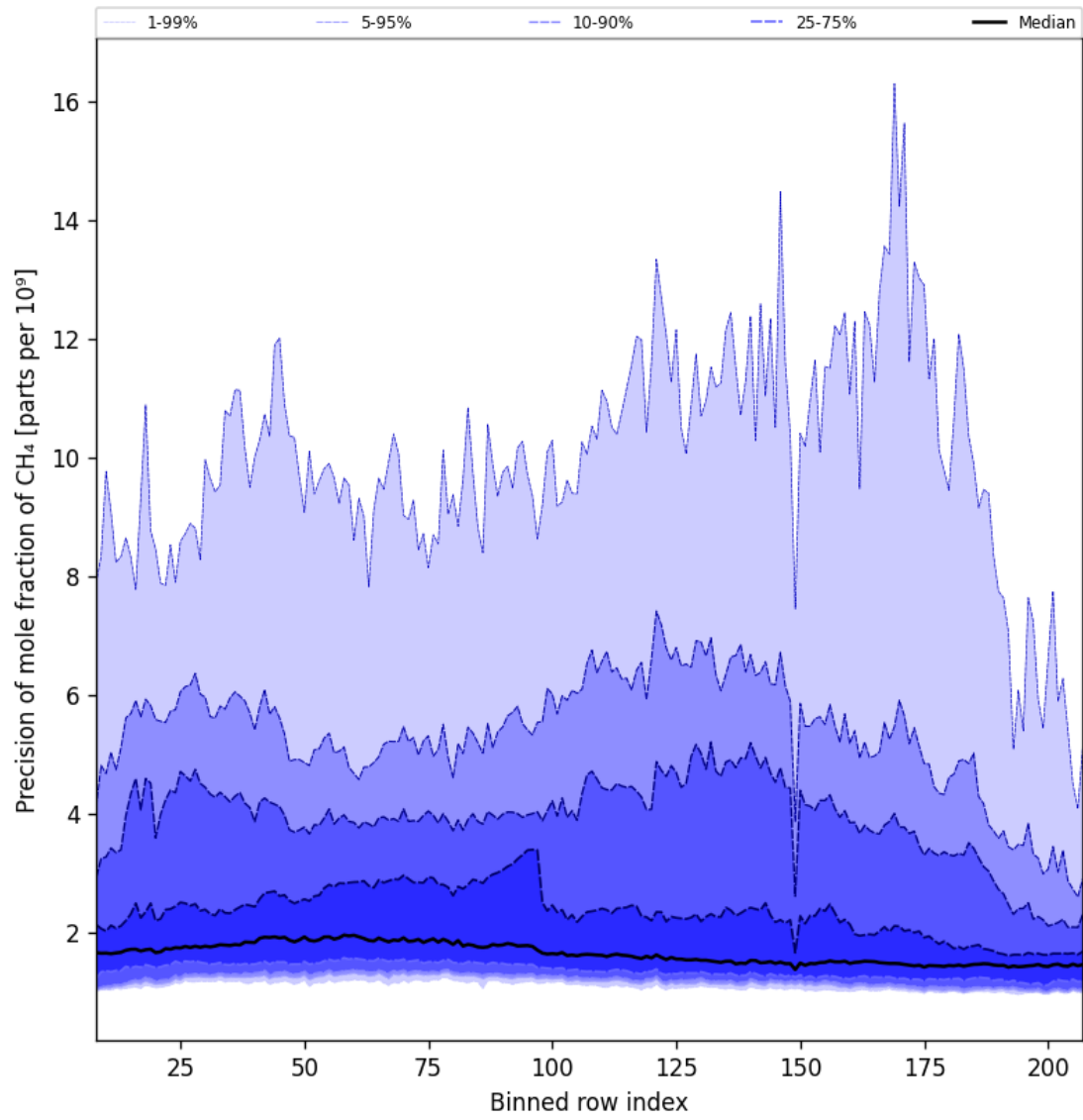
Figure 35: Along track statistics of “Precision of mole fraction of CH 4 ” for 2024-10-03 to 2024-10-05
