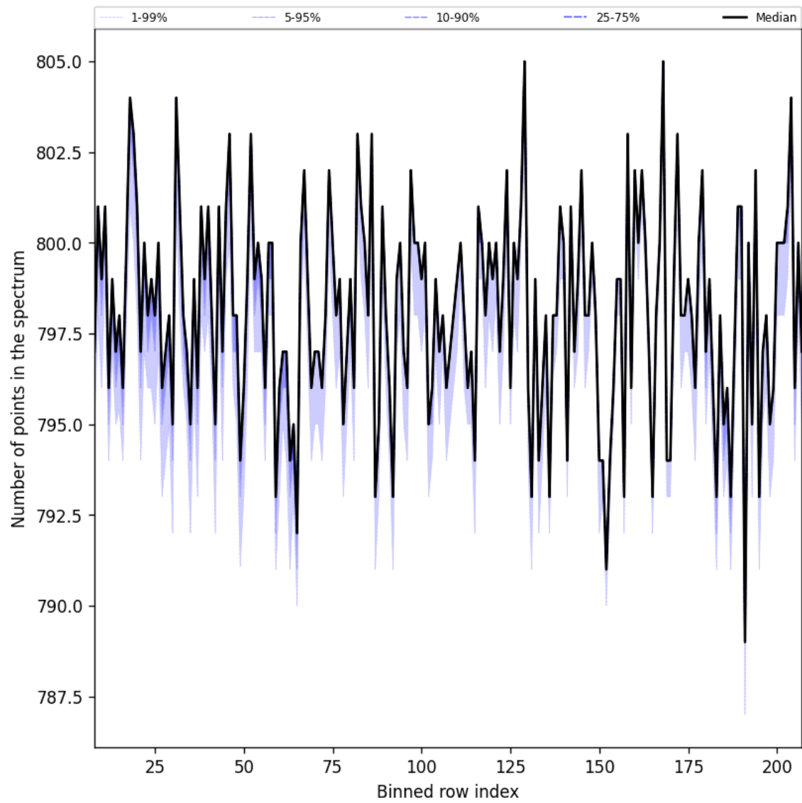
Figure 37: Along track statistics of “Number of points in the spectrum” for 2024-10-03 to 2024-10-05
