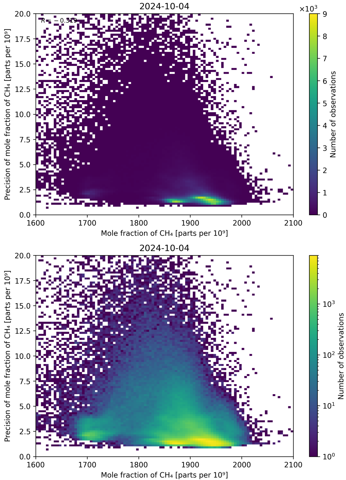
Figure 75: Scatter density plot of “Mole fraction of CH 4 ” against “Precision of mole fraction of CH 4 ” for 2024-10-03 to 2024-10-05.
