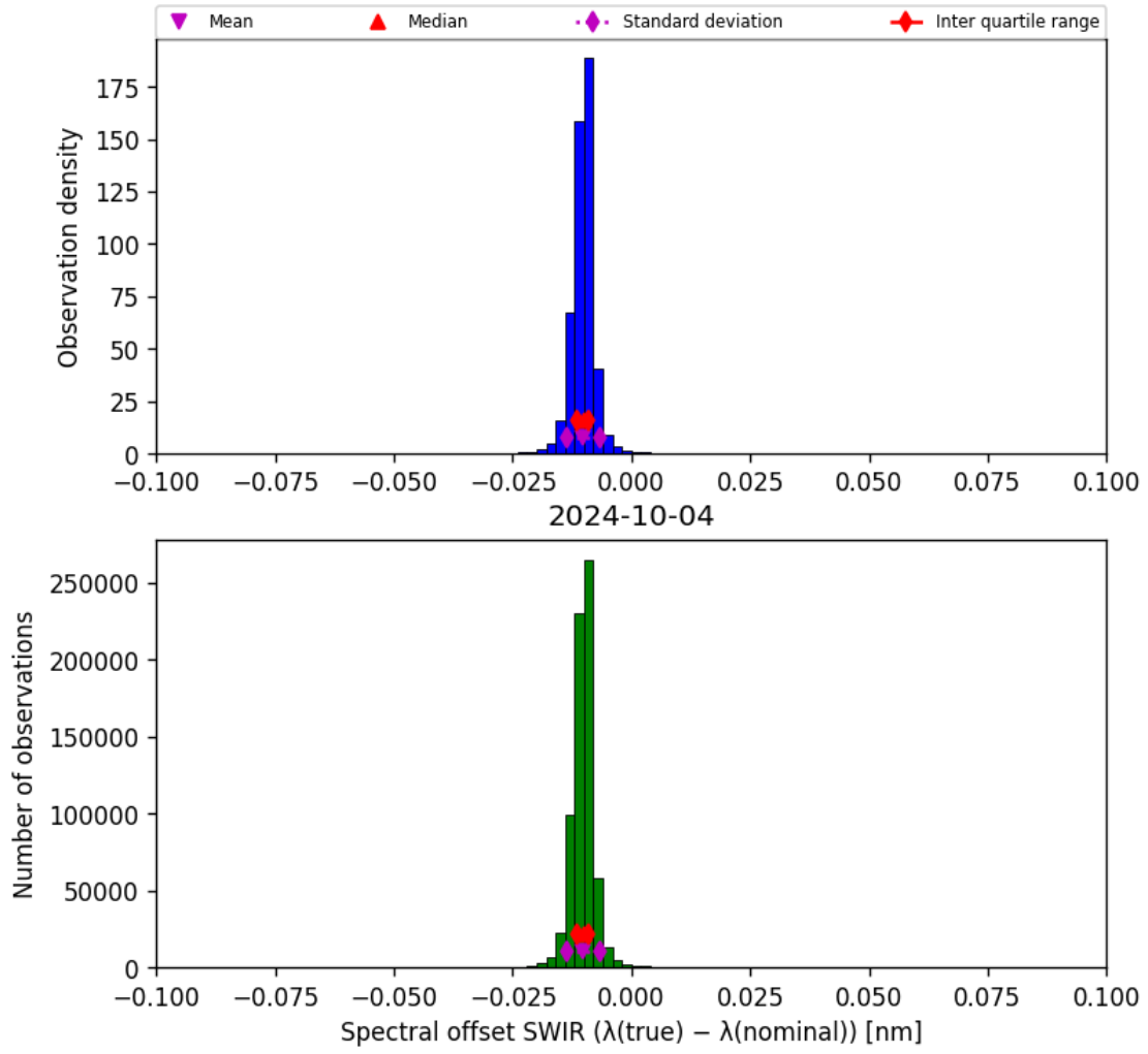
Figure 27: Histogram of “Spectral offset SWIR ( \lambda_{\text{true}} - \lambda_{\text{nominal}} )” for 2024-10-03 to 2024-10-05
