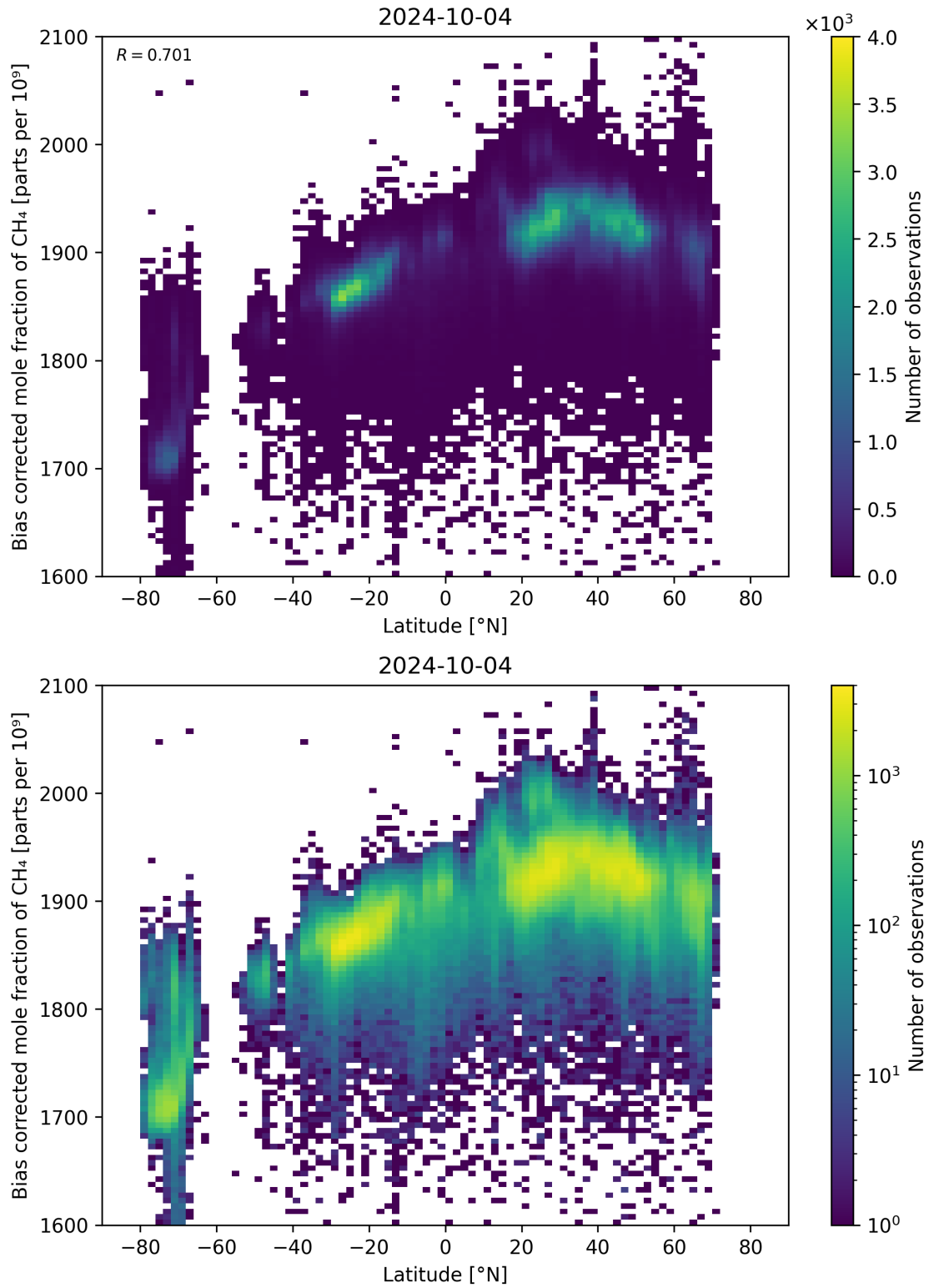
Figure 58: Scatter density plot of “Latitude” against “Bias corrected mole fraction of \text{CH}_4 ” for 2024-10-03 to 2024-10-05.
