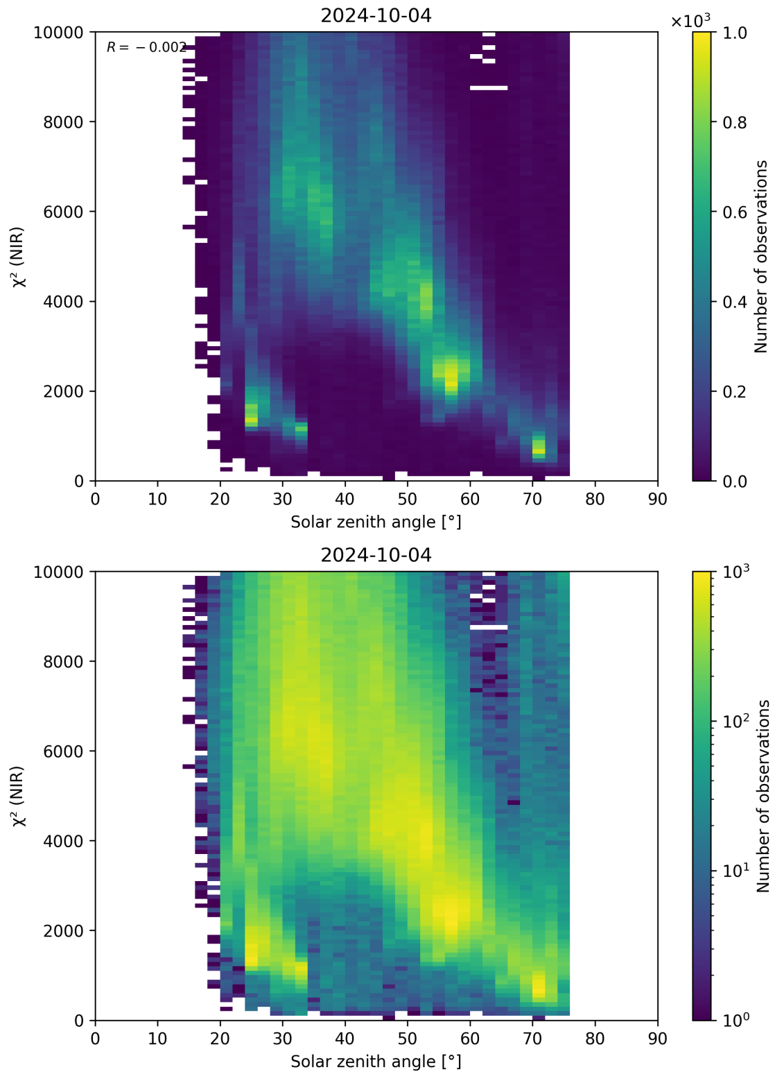
Figure 94: Scatter density plot of “Solar zenith angle” against “ \chi^2 (NIR)” for 2024-10-03 to 2024-10-05.
