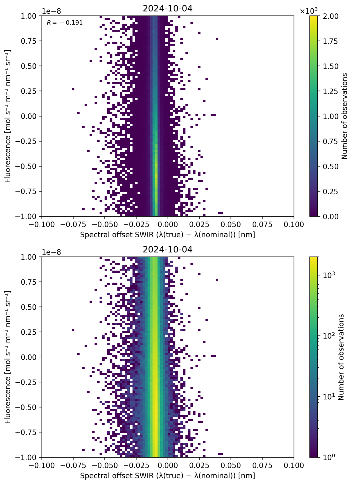
Figure 120: Scatter density plot of “Spectral offset SWIR ( \lambda_{\text{true}} - \lambda_{\text{nominal}} )” against “Fluorescence” for 2024-10-03 to 2024-10-05.
