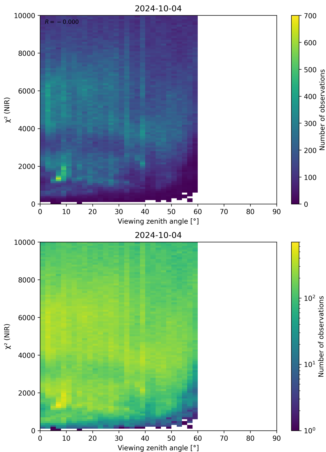
Figure 105: Scatter density plot of “Viewing zenith angle” against “ \chi^2 (NIR)” for 2024-10-03 to 2024-10-05.
