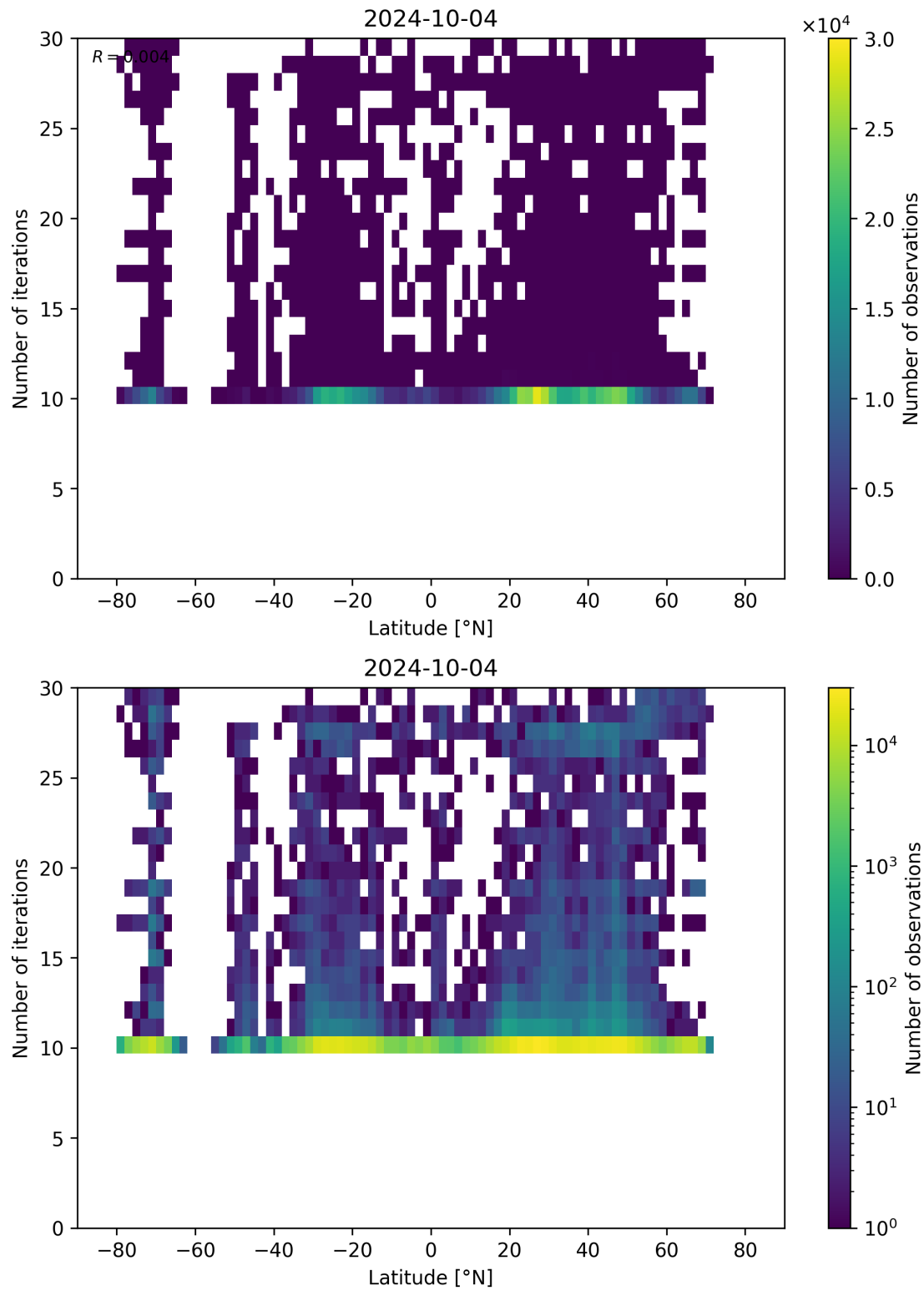
Figure 60: Scatter density plot of “Latitude” against “Number of iterations” for 2024-10-03 to 2024-10-05.
