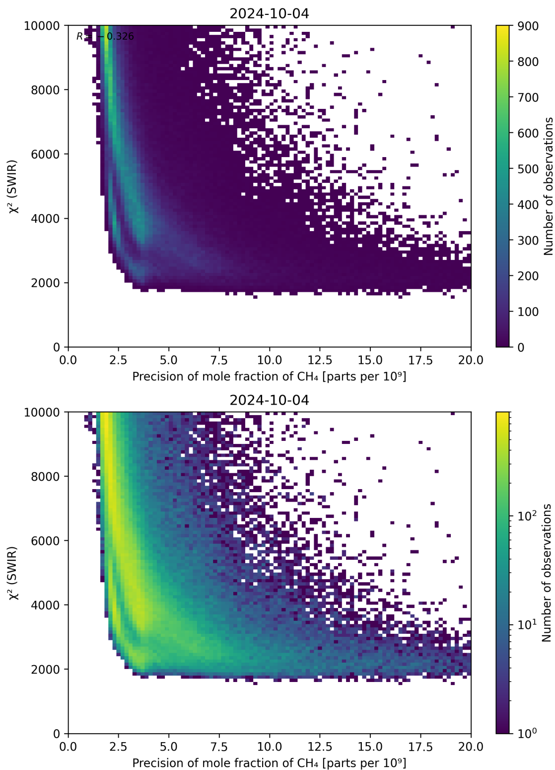
Figure 79: Scatter density plot of “Precision of mole fraction of CH 4 ” against “ \chi^2 (SWIR)” for 2024-10-03 to 2024-10-05.
