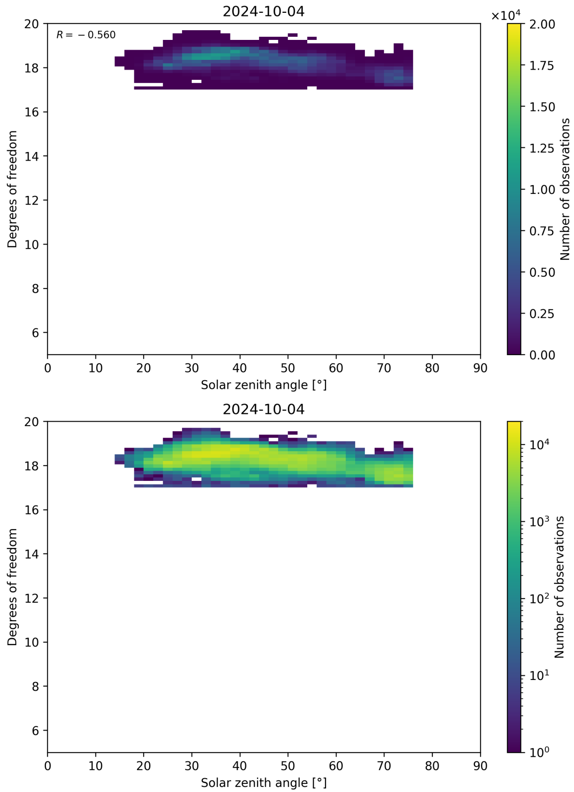
Figure 96: Scatter density plot of “Solar zenith angle” against “Degrees of freedom” for 2024-10-03 to 2024-10-05.
