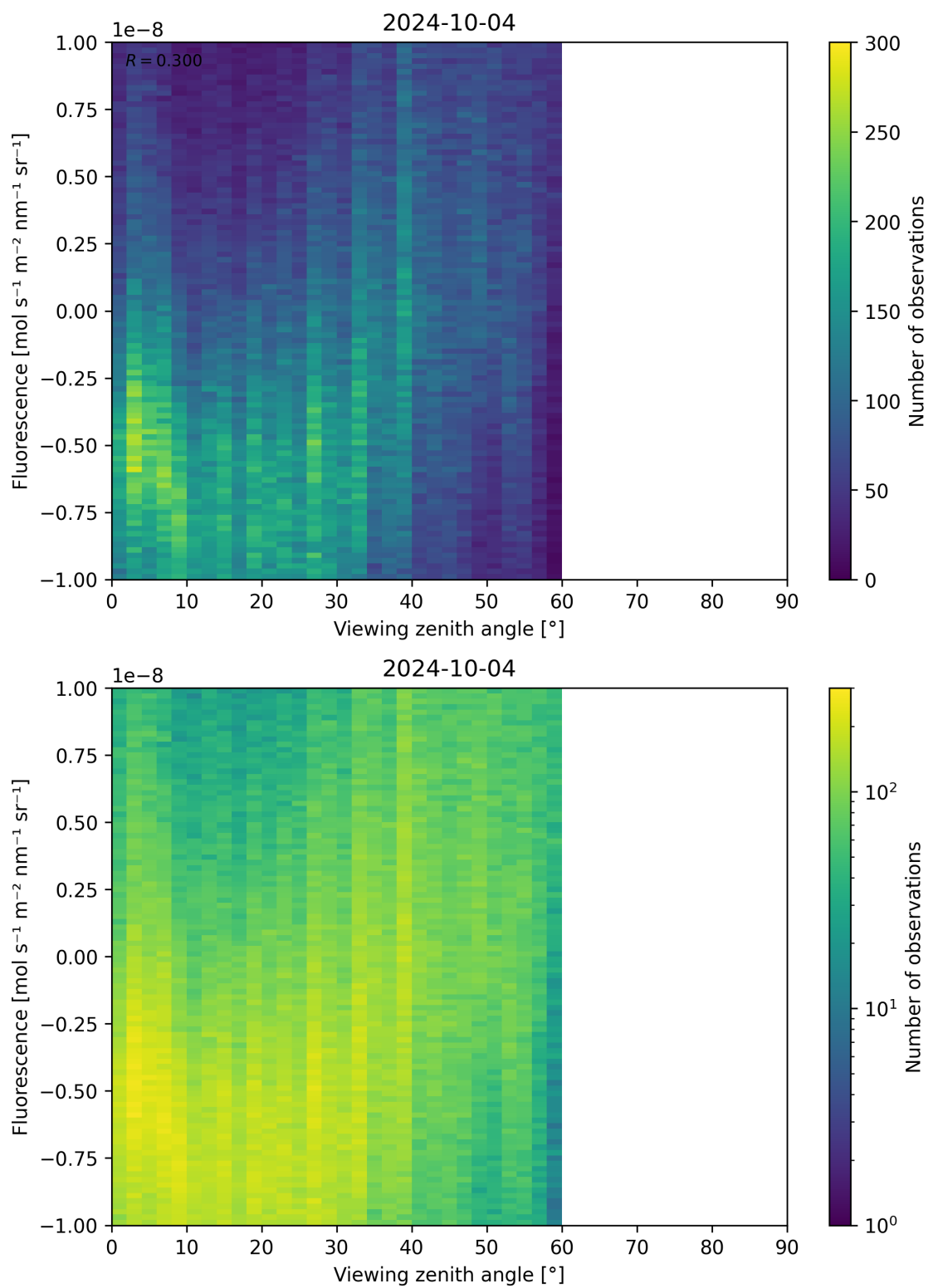
Figure 108: Scatter density plot of “Viewing zenith angle” against “Fluorescence” for 2024-10-03 to 2024-10-05.
