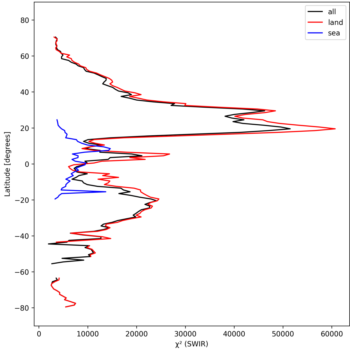
Figure 17: Zonal average of “ \chi^2 (SWIR)” for 2024-10-03 to 2024-10-05.
