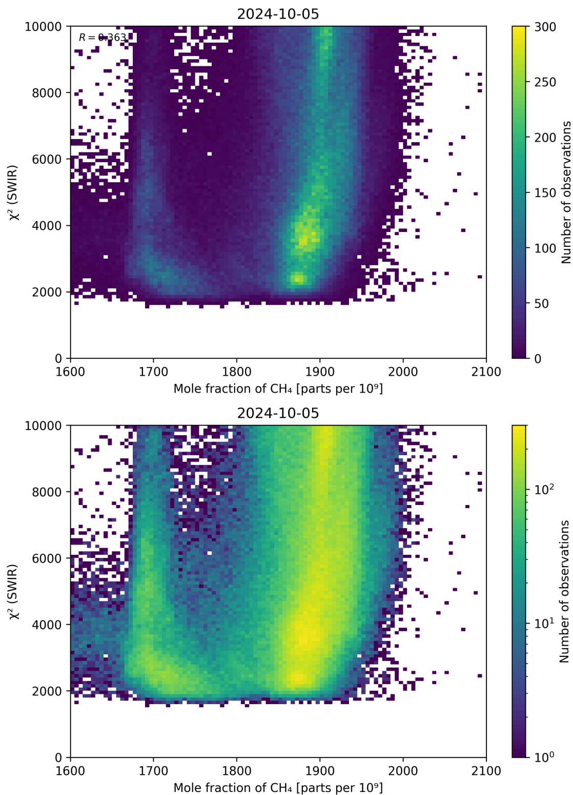
Figure 71: Scatter density plot of “Mole fraction of \text{CH}_4 ” against “ \chi^2 (SWIR)” for 2024-10-04 to 2024-10-06.
