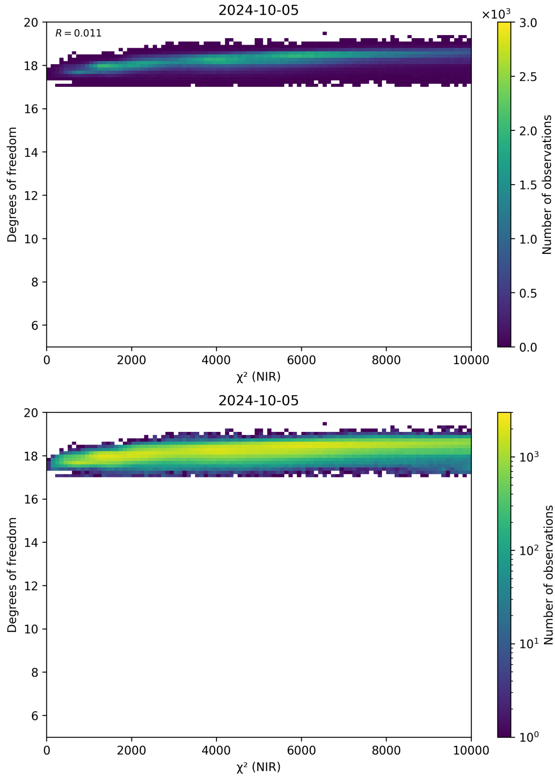
Figure 44: Scatter density plot of “ \chi^2 (NIR)” against “Degrees of freedom” for 2024-10-04 to 2024-10-06.
