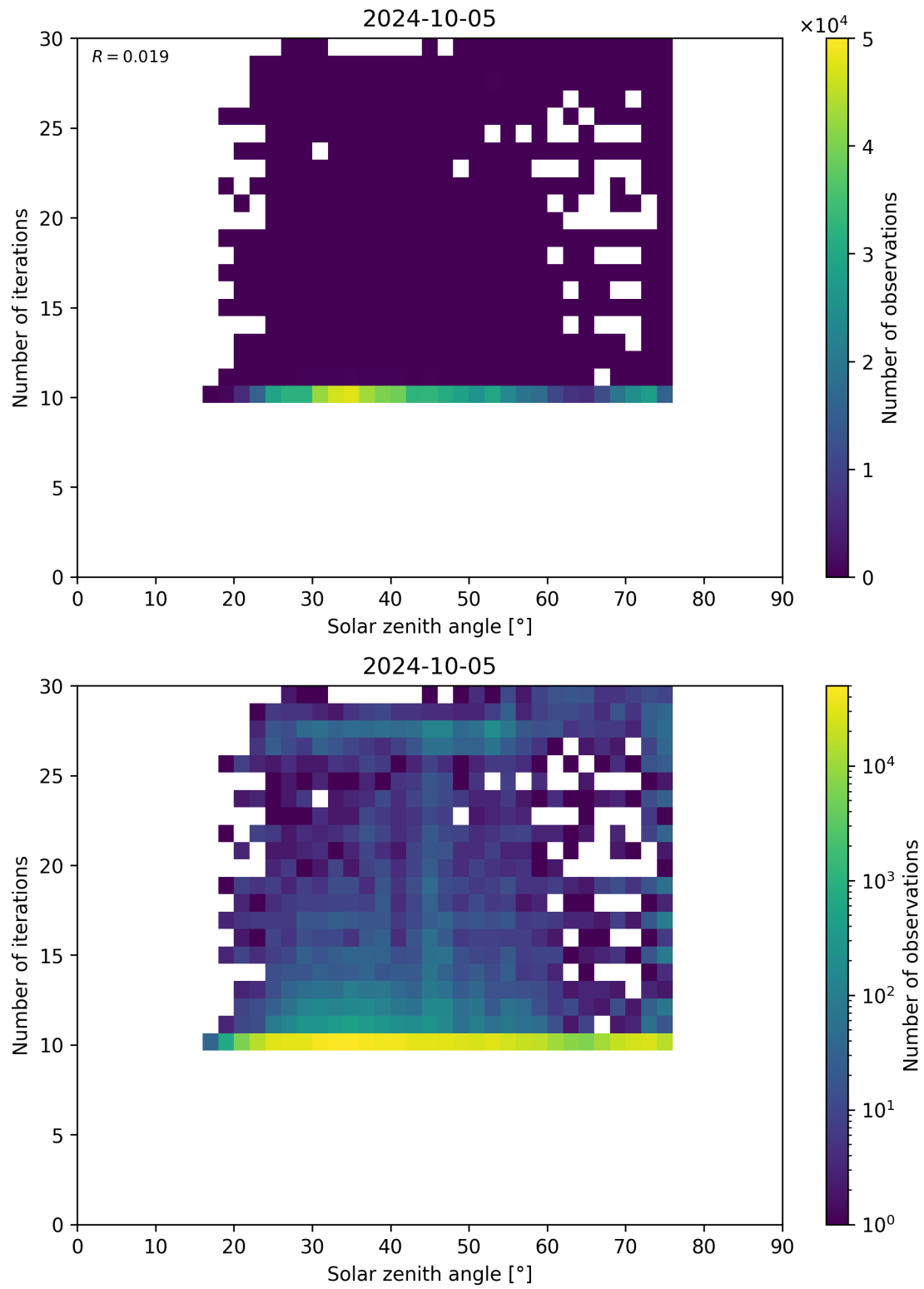
Figure 102: Scatter density plot of “Solar zenith angle” against “Number of iterations” for 2024-10-04 to 2024-10-06.
