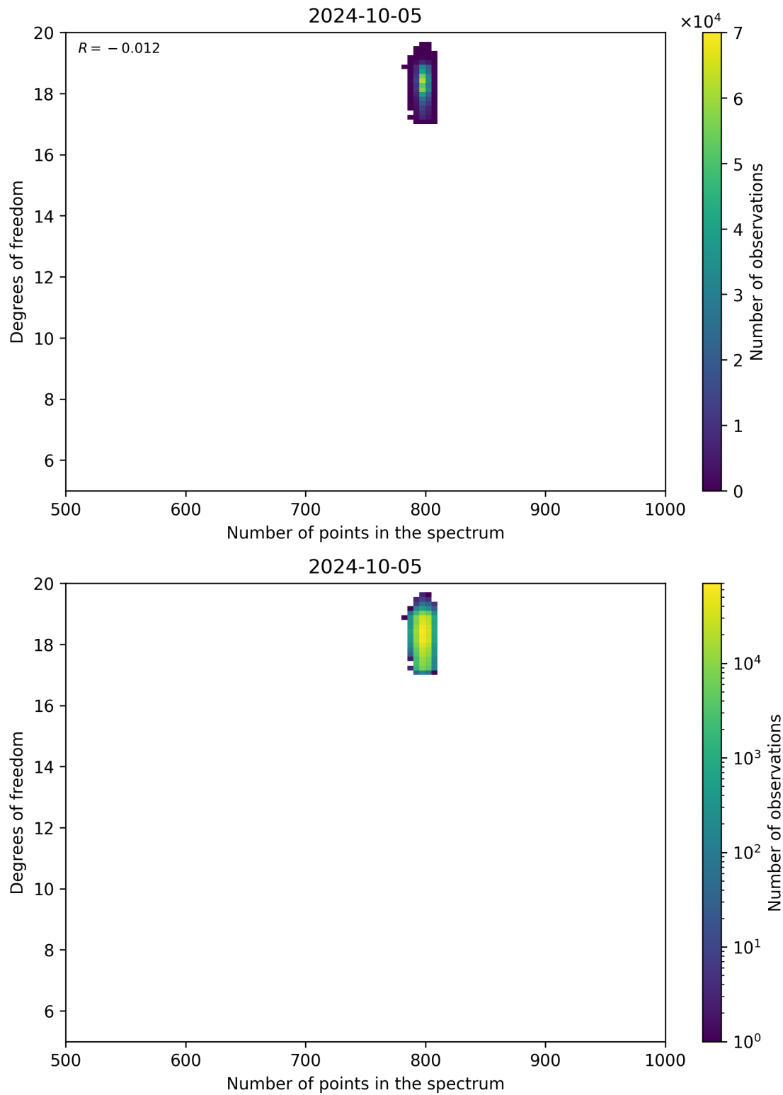
Figure 90: Scatter density plot of “Number of points in the spectrum” against “Degrees of freedom” for 2024-10-04 to 2024-10-06.
