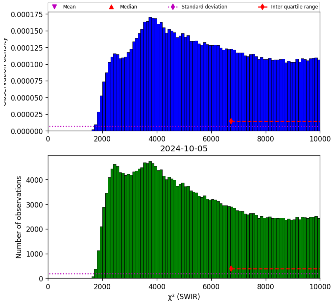
Figure 28: Histogram of “ \chi^2 (SWIR)” for 2024-10-04 to 2024-10-06
