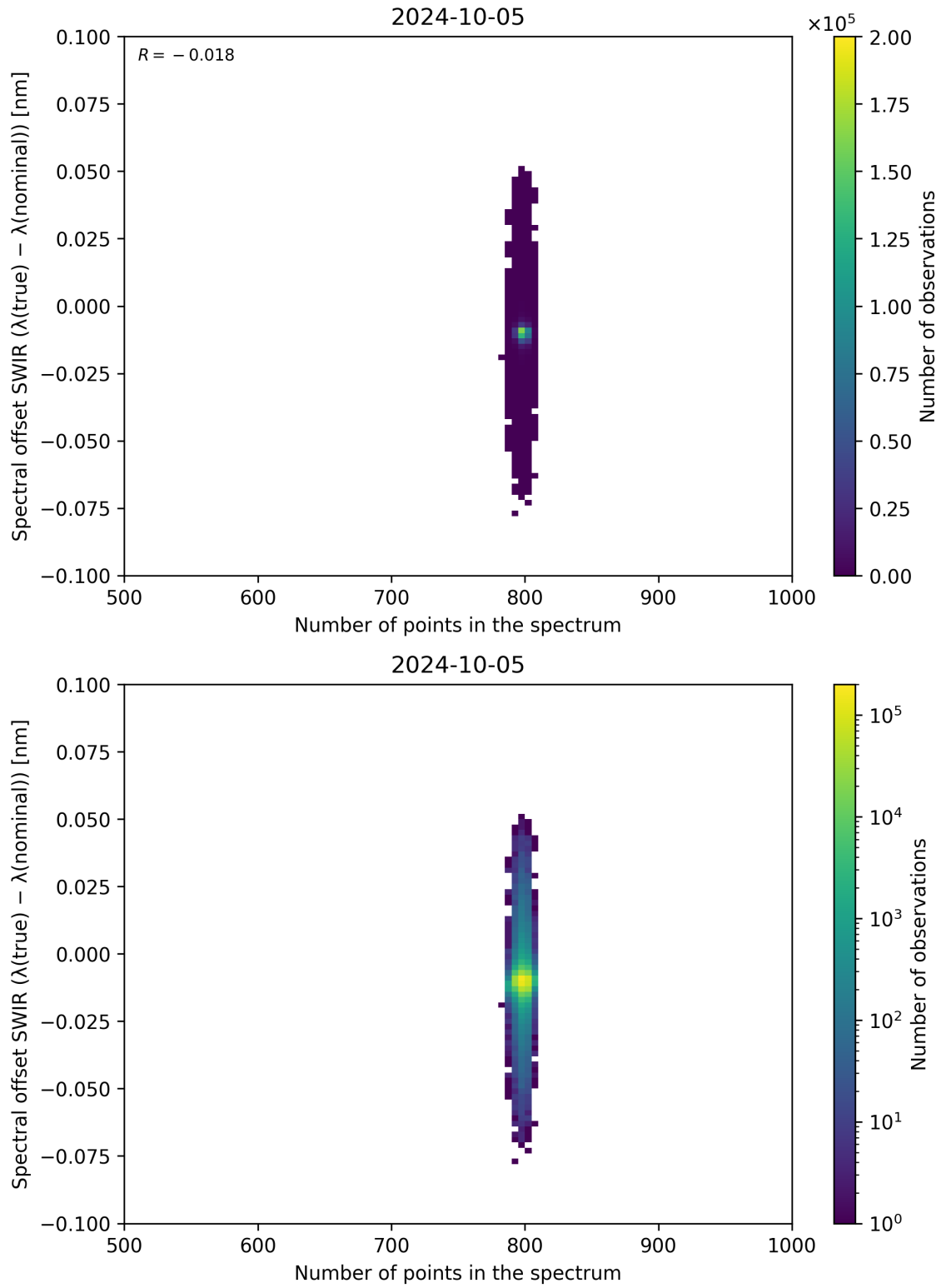
Figure 93: Scatter density plot of “Number of points in the spectrum” against “Spectral offset SWIR ( \lambda_{\text{true}} - \lambda_{\text{nominal}} )” for 2024-10-04 to 2024-10-06.
