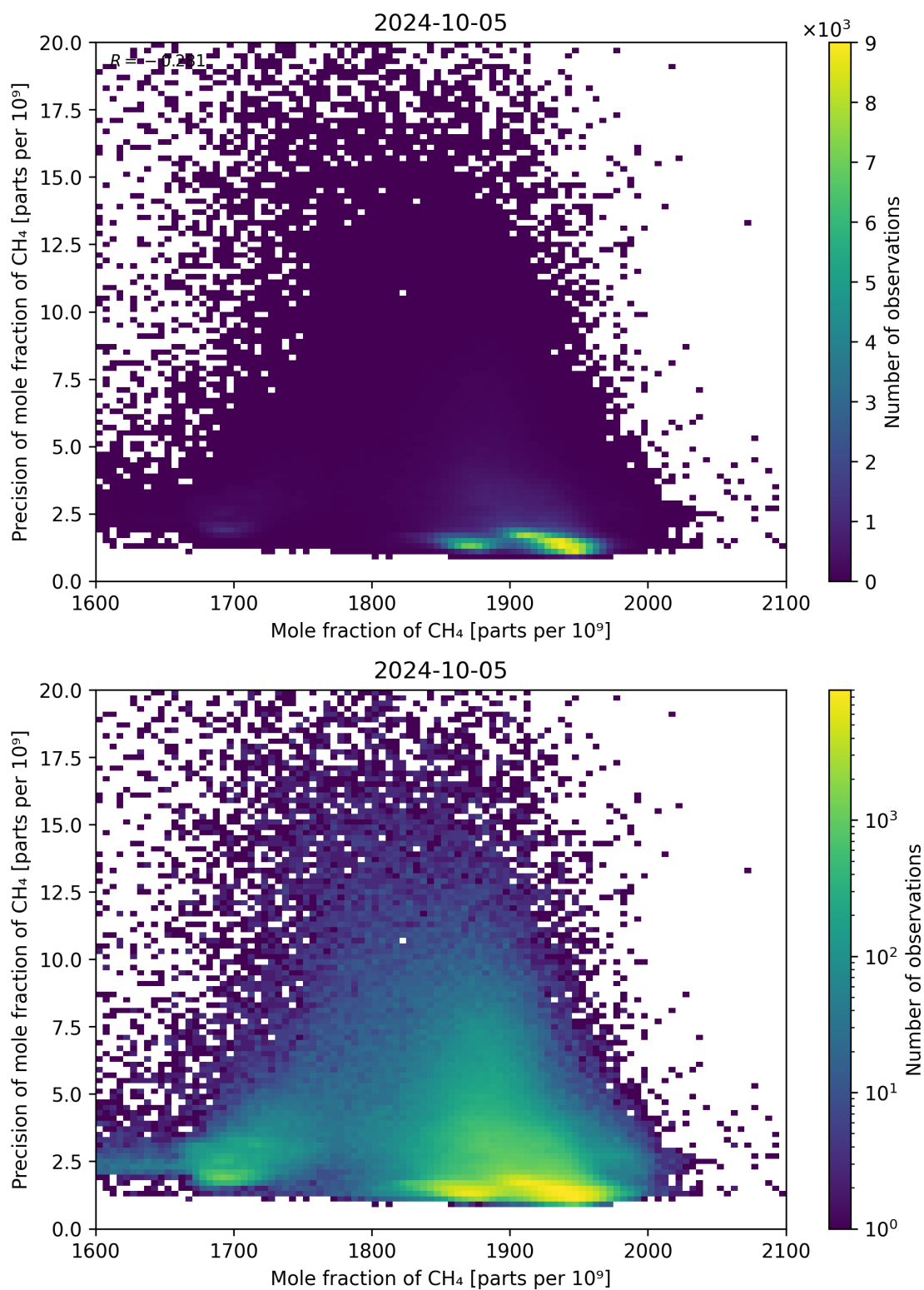
Figure 75: Scatter density plot of “Mole fraction of CH 4 ” against “Precision of mole fraction of CH 4 ” for 2024-10-04 to 2024-10-06.
