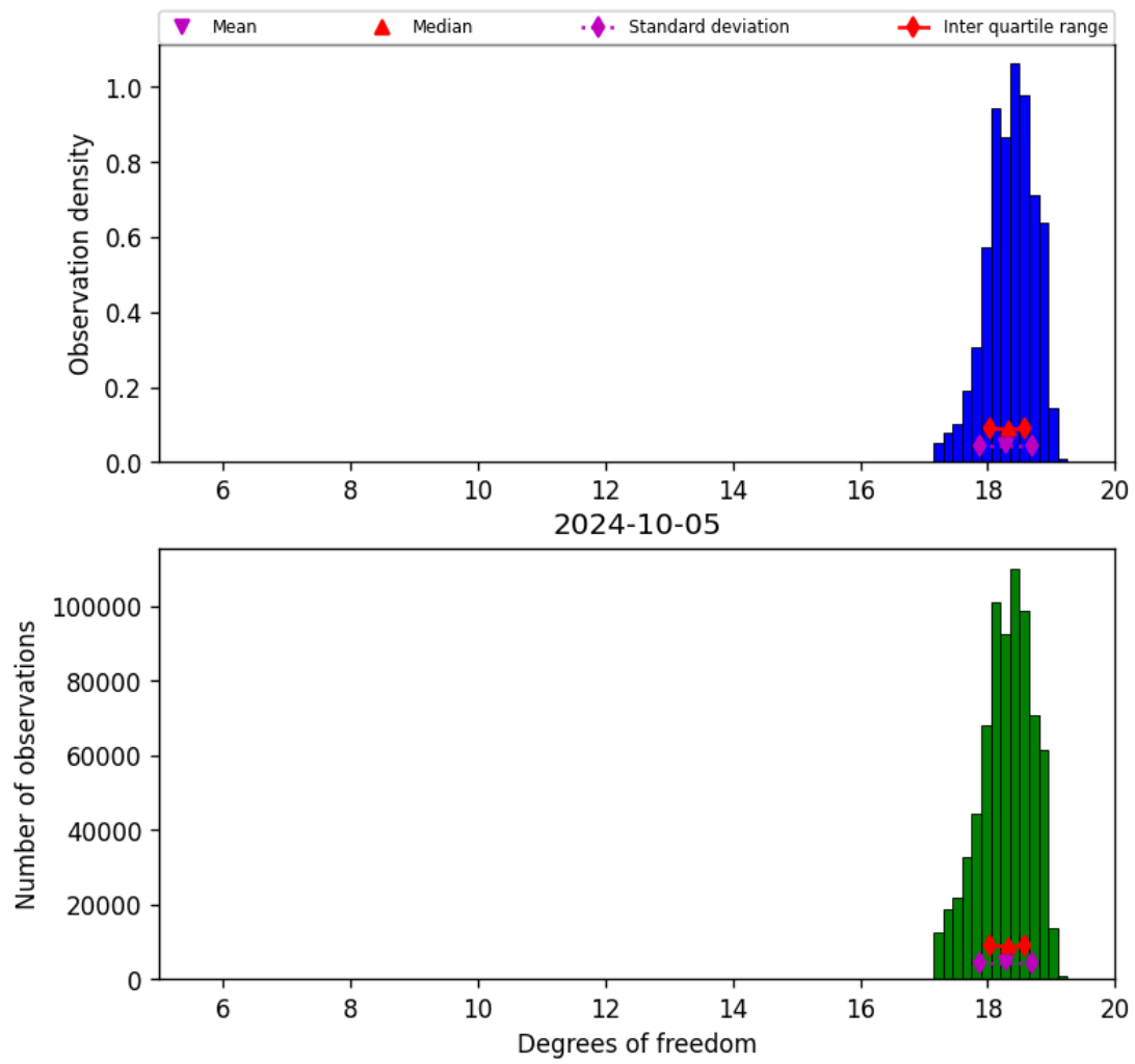
Figure 30: Histogram of “Degrees of freedom” for 2024-10-04 to 2024-10-06
