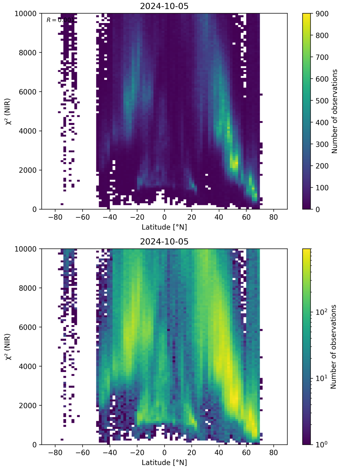
Figure 53: Scatter density plot of “Latitude” against “ \chi^2 (NIR)” for 2024-10-04 to 2024-10-06.
