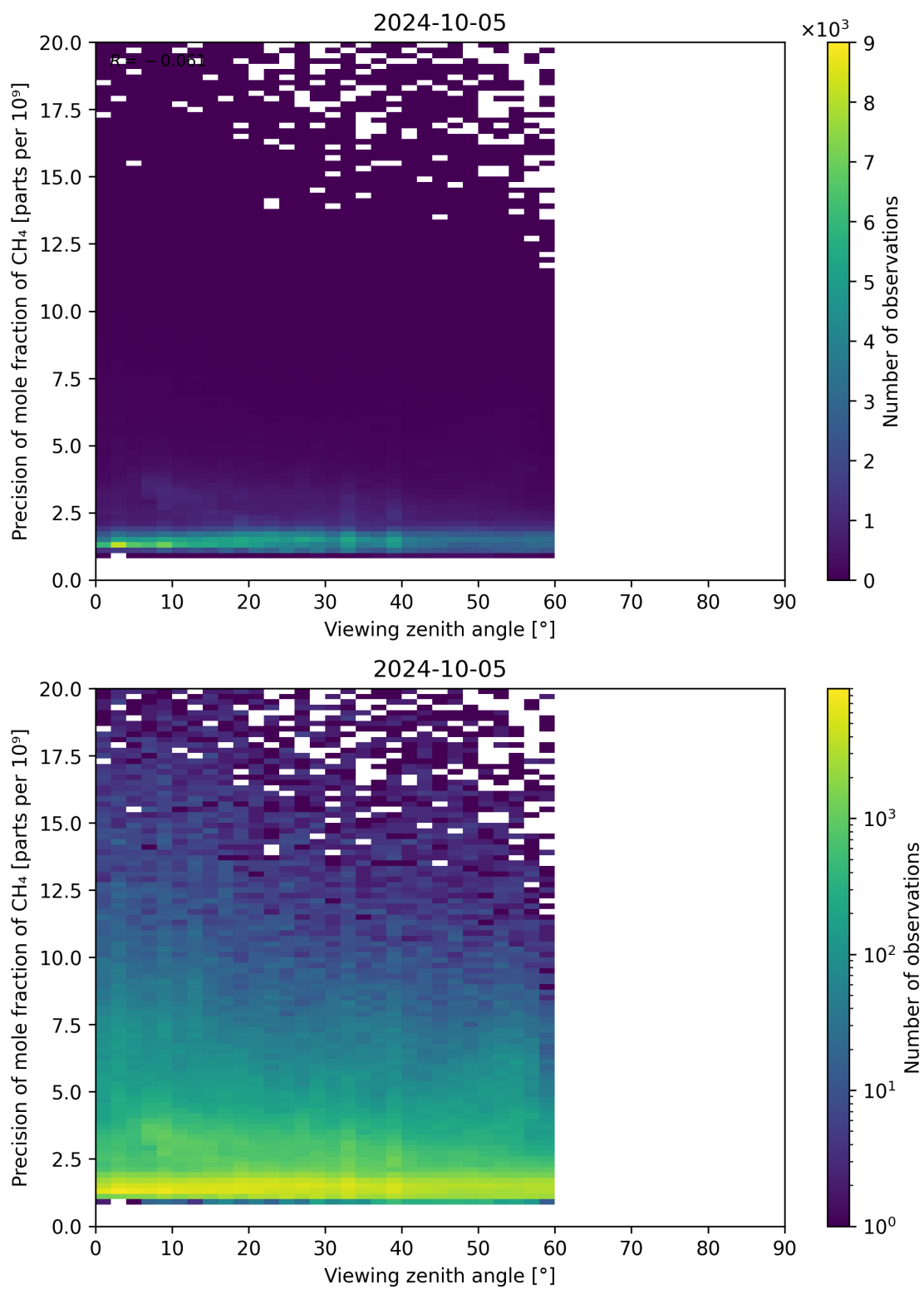
Figure 112: Scatter density plot of “Viewing zenith angle” against “Precision of mole fraction of CH 4 ” for 2024-10-04 to 2024-10-06.
