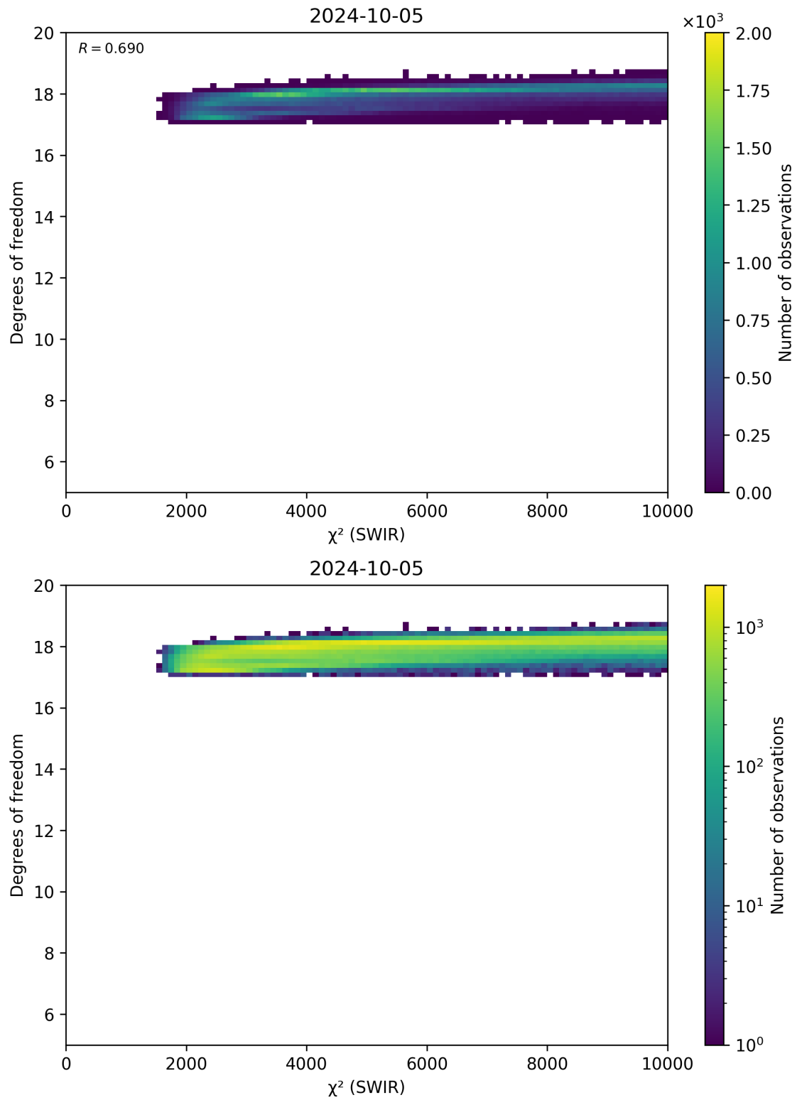
Figure 48: Scatter density plot of " \chi^2 (SWIR)" against "Degrees of freedom" for 2024-10-04 to 2024-10-06.
