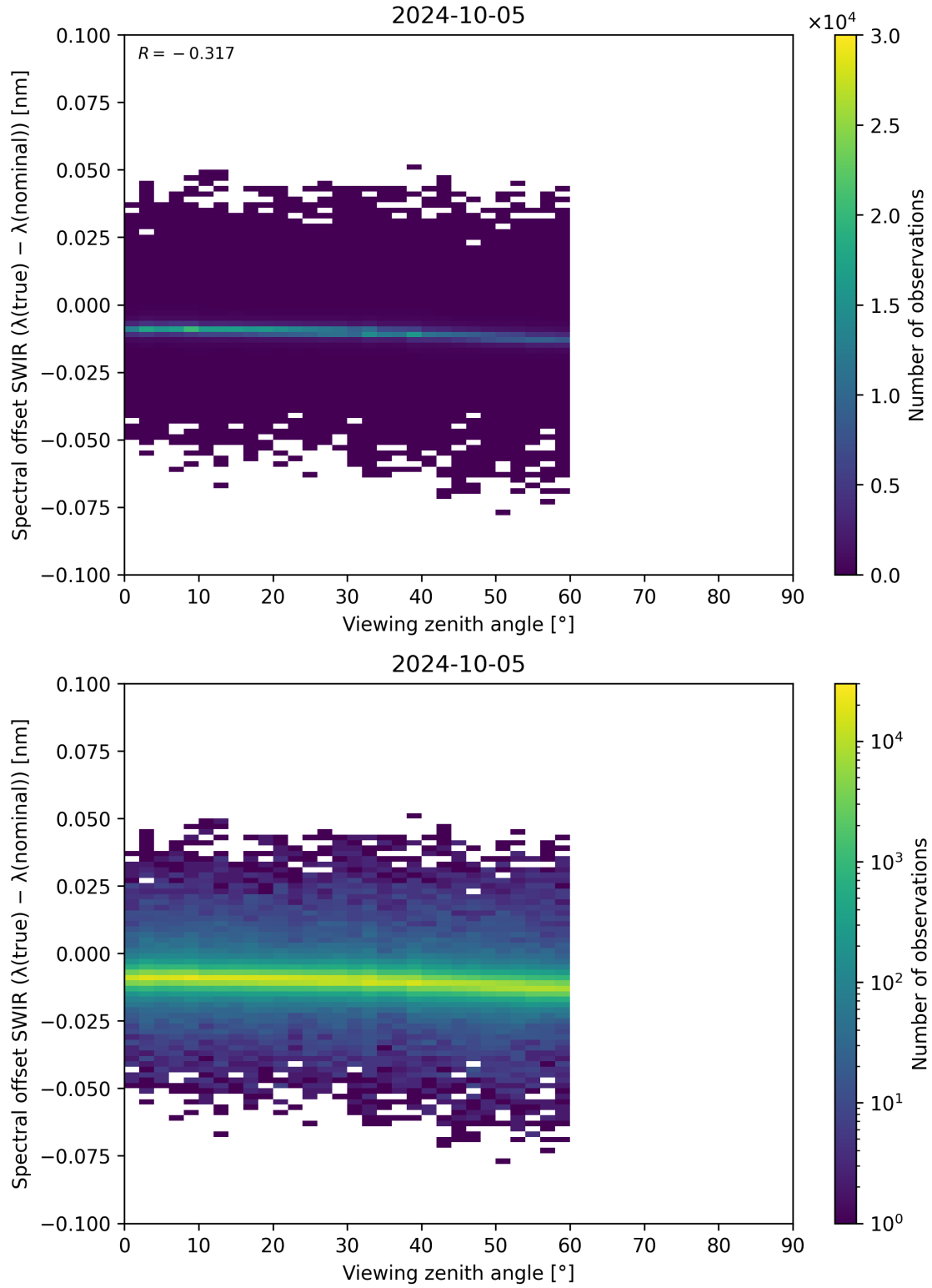
Figure 116: Scatter density plot of “Viewing zenith angle” against “Spectral offset SWIR ( \lambda_{\text{true}} - \lambda_{\text{nominal}} )” for 2024-10-04 to 2024-10-06.
