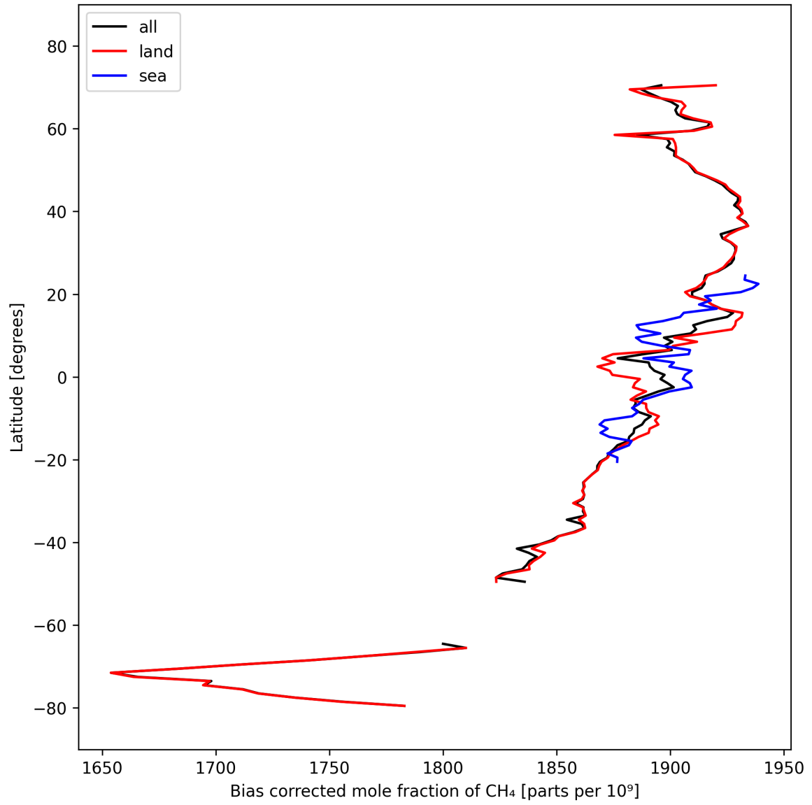
Figure 14: Zonal average of “Bias corrected mole fraction of CH 4 ” for 2024-10-04 to 2024-10-06.
