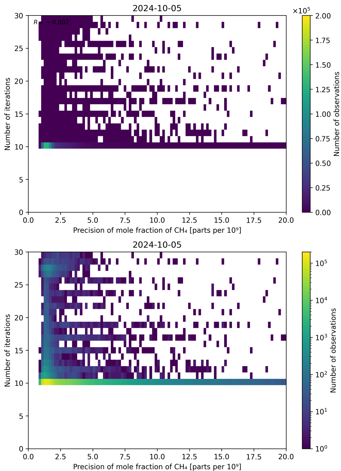
Figure 83: Scatter density plot of “Precision of mole fraction of CH 4 ” against “Number of iterations” for 2024-10-04 to 2024-10-06.
