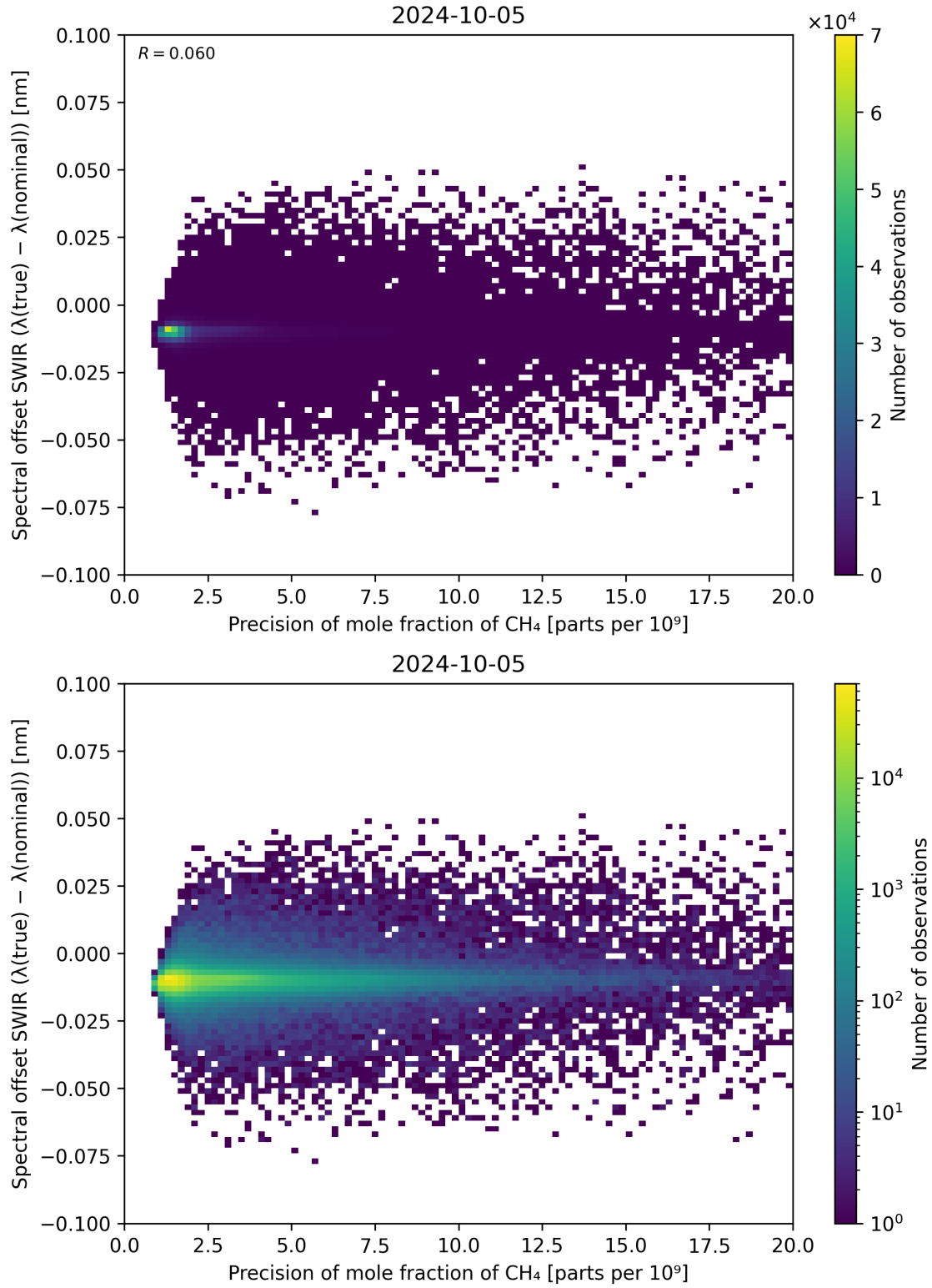
Figure 85: Scatter density plot of “Precision of mole fraction of \text{CH}_4 ” against “Spectral offset SWIR ( \lambda_{\text{true}} - \lambda_{\text{nominal}} )” for 2024-10-04 to 2024-10-06.
