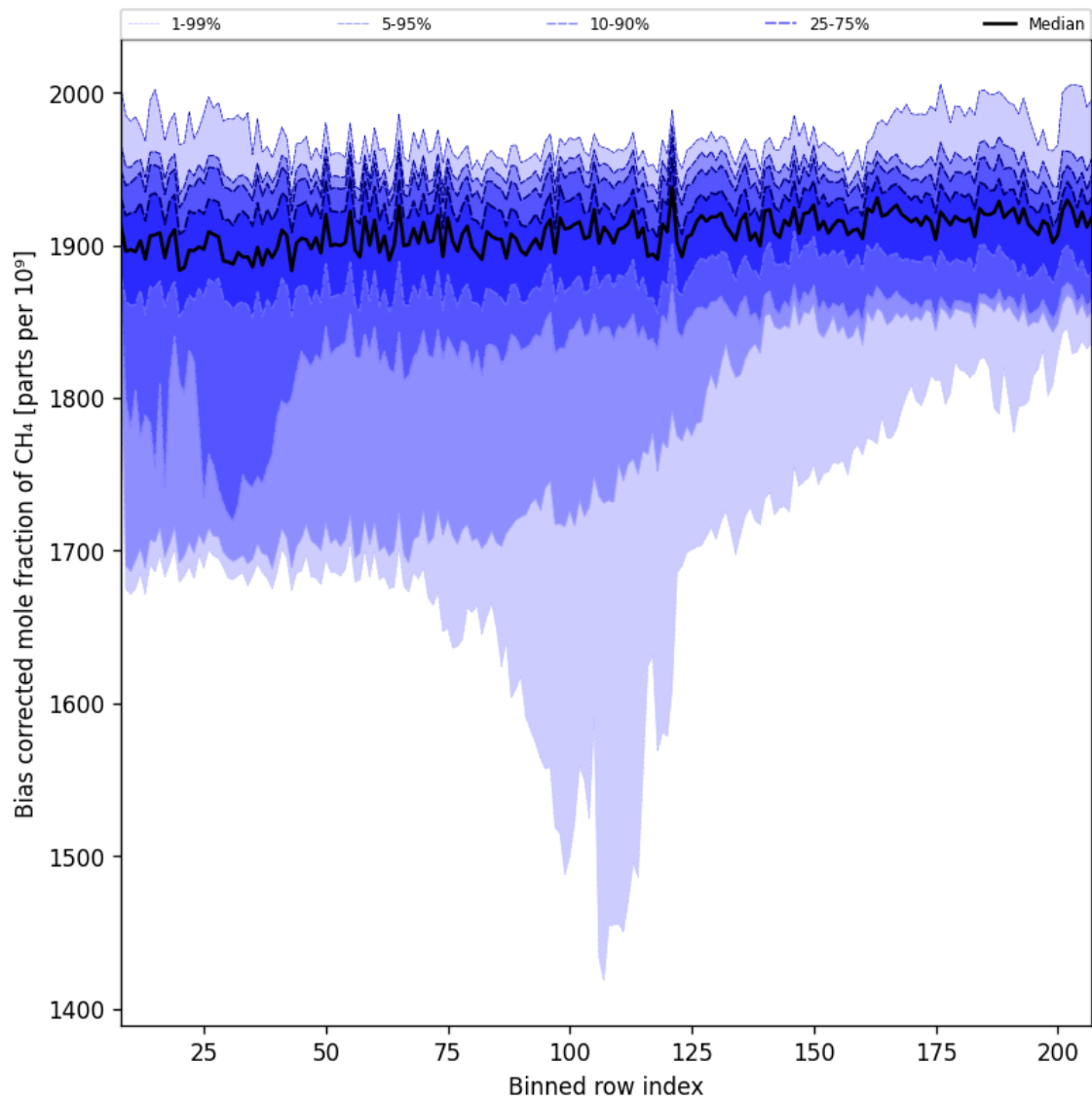
Figure 36: Along track statistics of “Bias corrected mole fraction of CH 4 ” for 2024-10-04 to 2024-10-06
