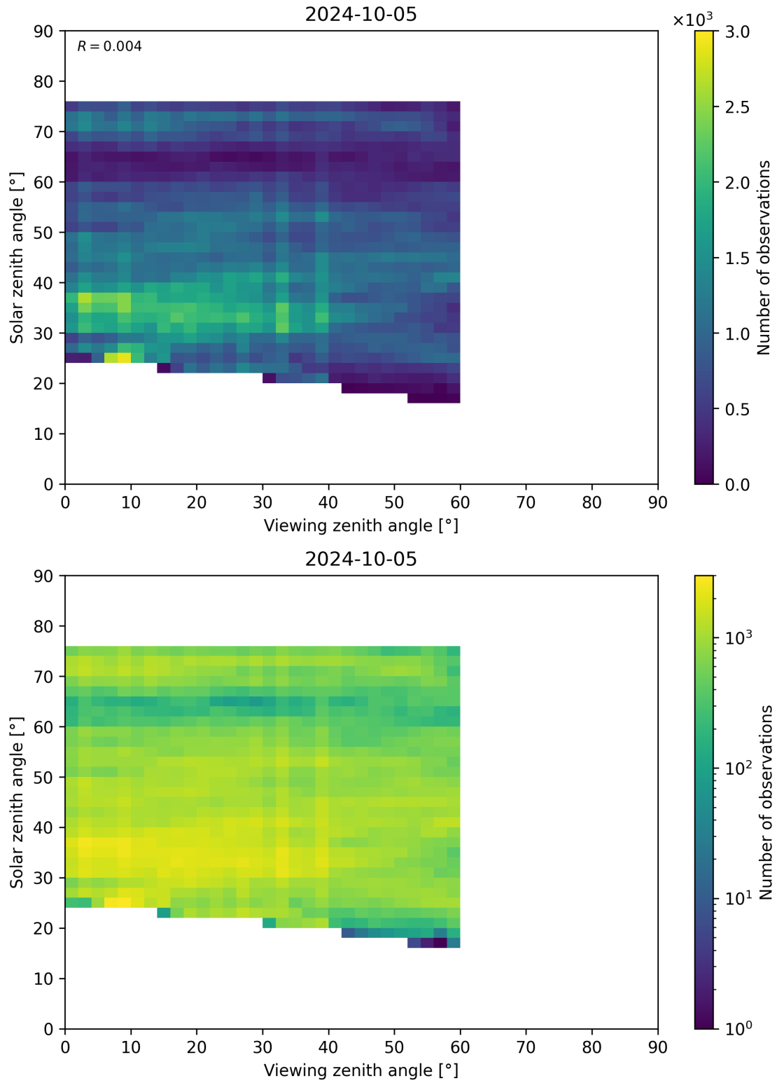
Figure 115: Scatter density plot of “Viewing zenith angle” against “Solar zenith angle” for 2024-10-04 to 2024-10-06.
