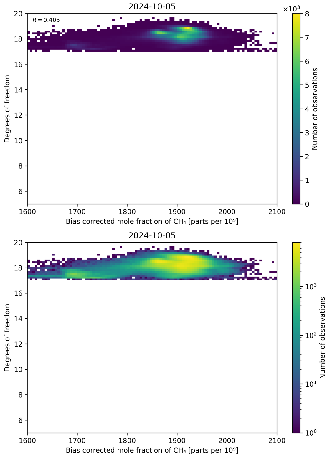
Figure 65: Scatter density plot of “Bias corrected mole fraction of CH 4 ” against “Degrees of freedom” for 2024-10-04 to 2024-10-06.
