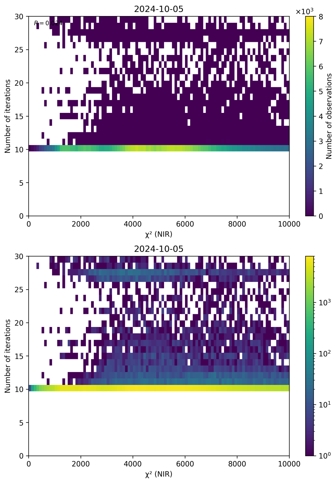
Figure 46: Scatter density plot of “ \chi^2 (NIR)” against “Number of iterations” for 2024-10-04 to 2024-10-06.
