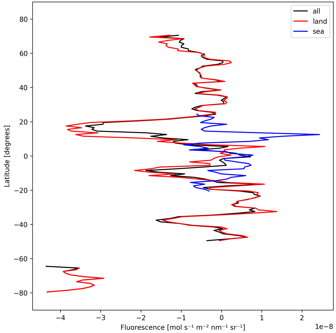
Figure 21: Zonal average of “Fluorescence” for 2024-10-04 to 2024-10-06.
