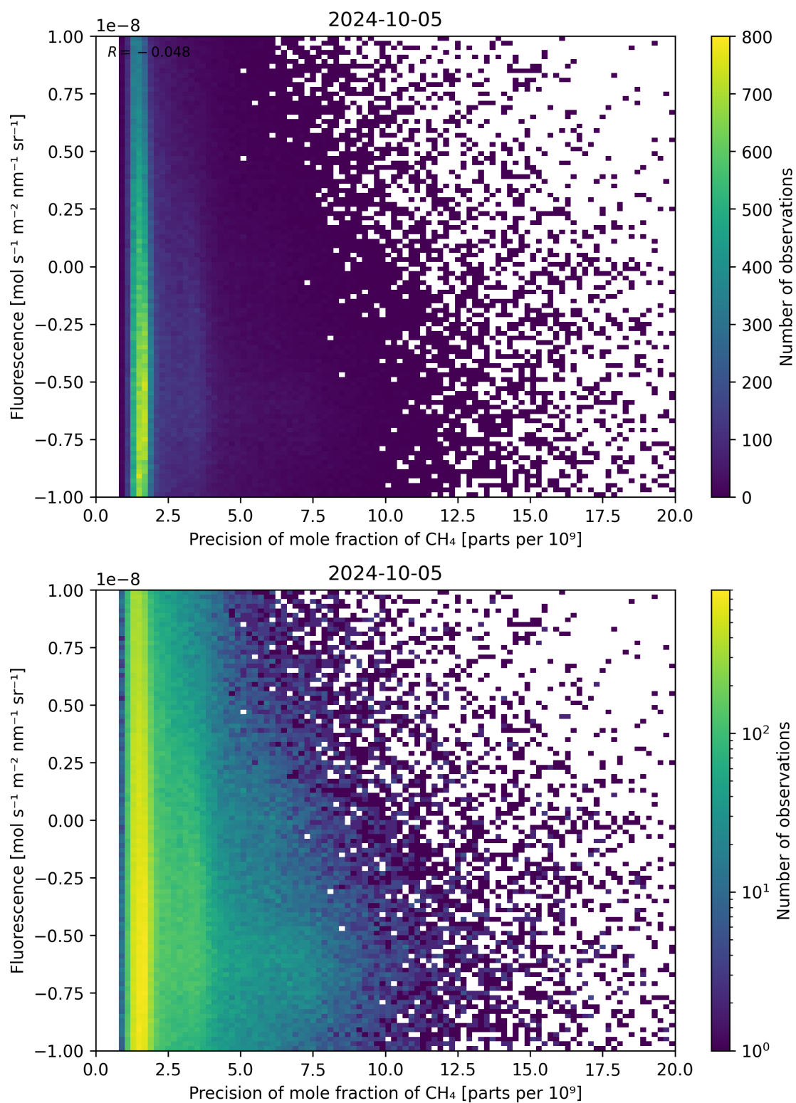
Figure 81: Scatter density plot of “Precision of mole fraction of \text{CH}_4 ” against “Fluorescence” for 2024-10-04 to 2024-10-06.
