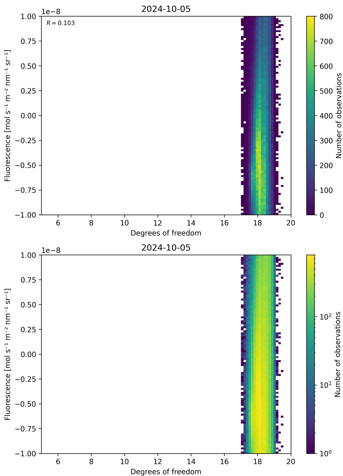
Figure 51: Scatter density plot of “Degrees of freedom” against “Fluorescence” for 2024-10-04 to 2024-10-06.
