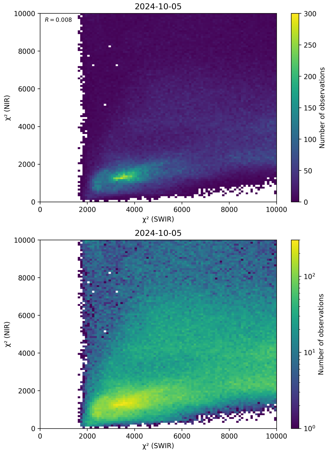
Figure 47: Scatter density plot of “ \chi^2 (SWIR)” against “ \chi^2 (NIR)” for 2024-10-04 to 2024-10-06.
