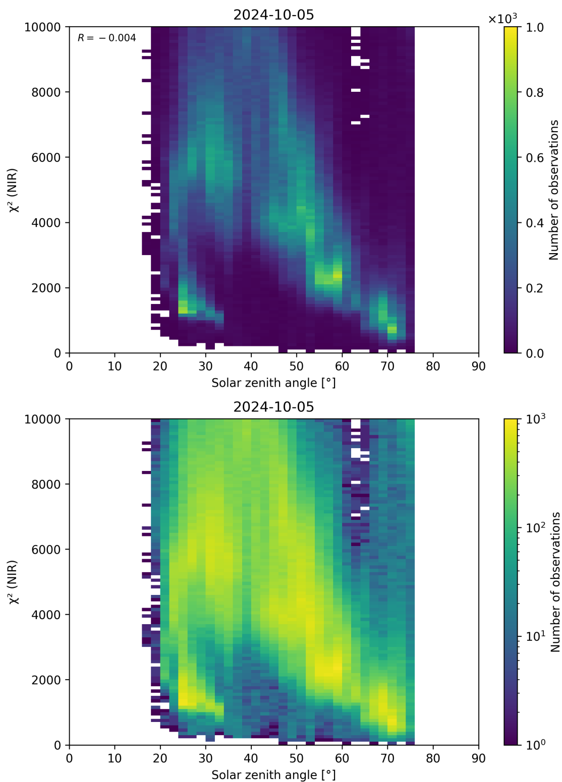
Figure 94: Scatter density plot of “Solar zenith angle” against “ \chi^2 (NIR)” for 2024-10-04 to 2024-10-06.
