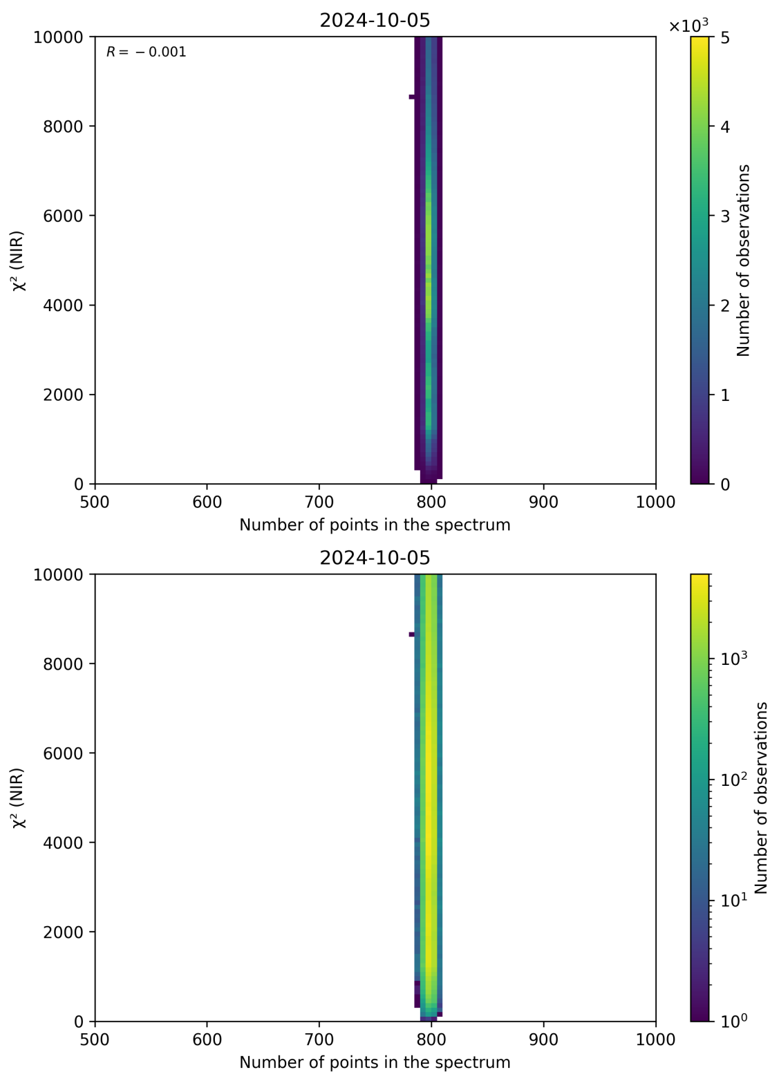
Figure 88: Scatter density plot of “Number of points in the spectrum” against “ \chi^2 (NIR)” for 2024-10-04 to 2024-10-06.
