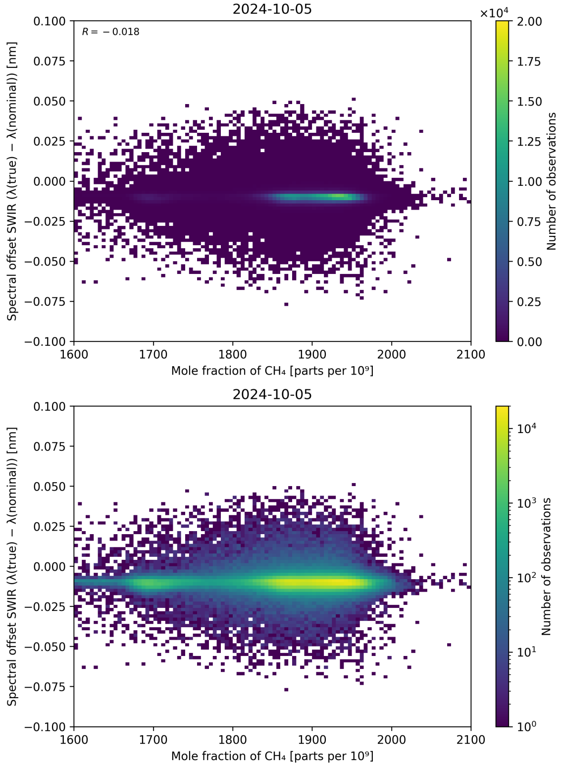
Figure 86: Scatter density plot of “Mole fraction of CH 4 ” against “Spectral offset SWIR ( \lambda_{\text{true}} - \lambda_{\text{nominal}} )” for 2024-10-04 to 2024-10-06.
