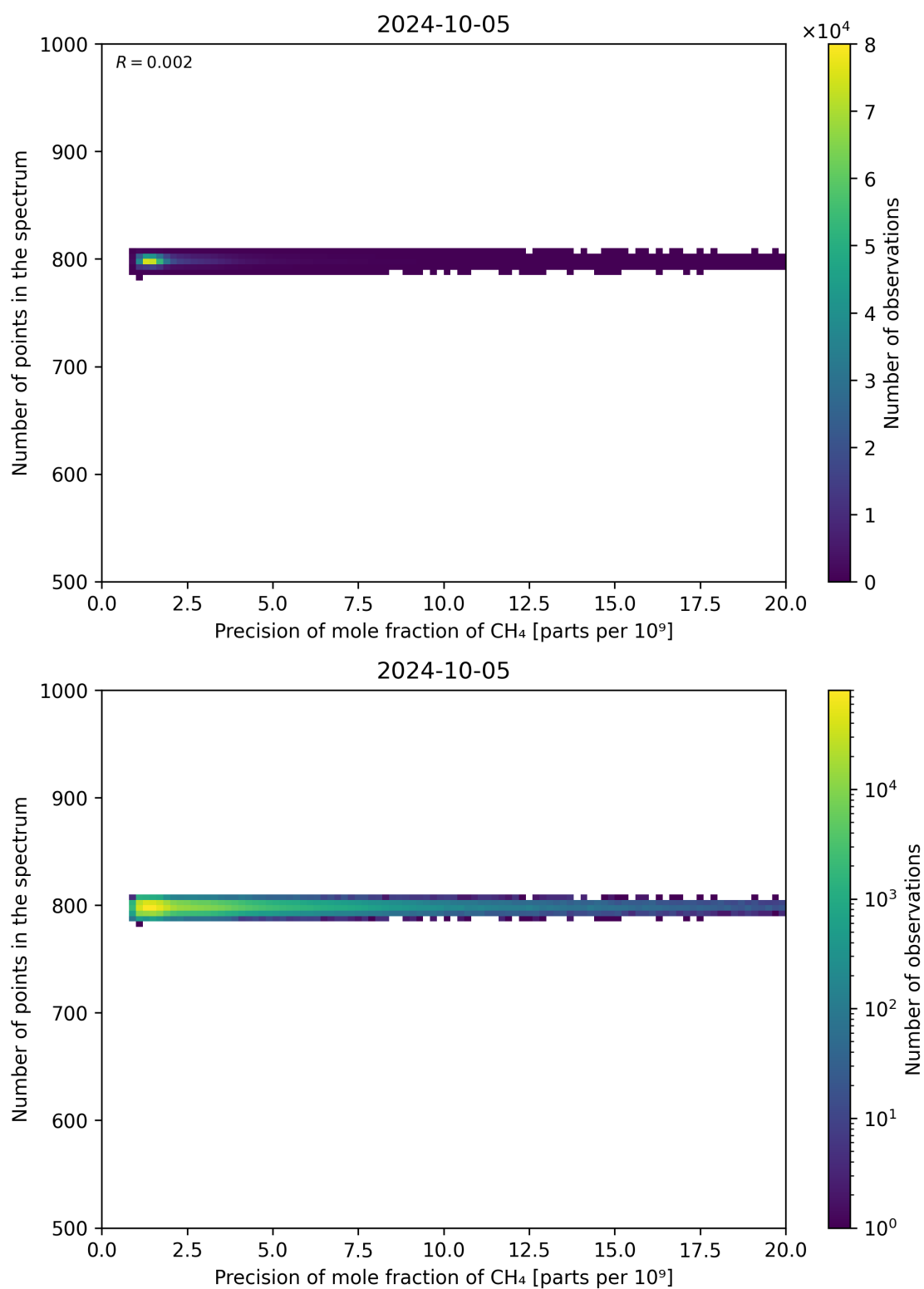
Figure 84: Scatter density plot of “Precision of mole fraction of CH 4 ” against “Number of points in the spectrum” for 2024-10-04 to 2024-10-06.
