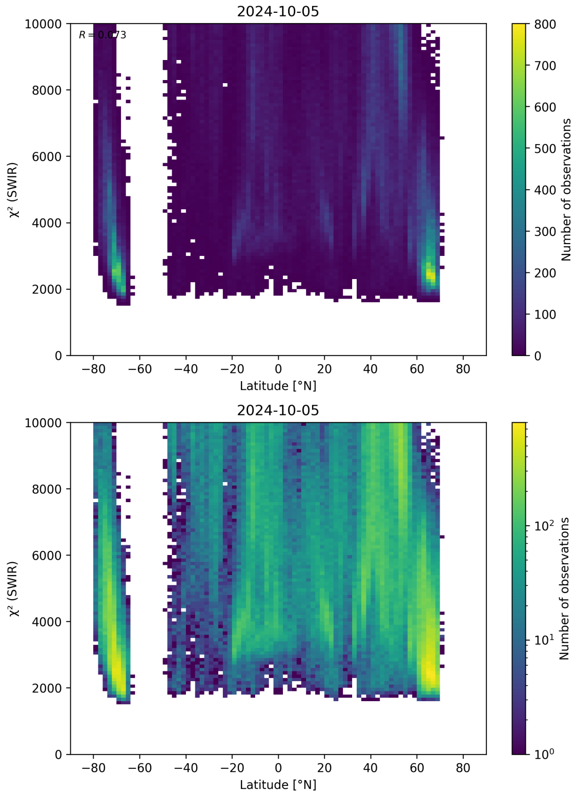
Figure 54: Scatter density plot of “Latitude” against “ \chi^2 (SWIR)” for 2024-10-04 to 2024-10-06.
