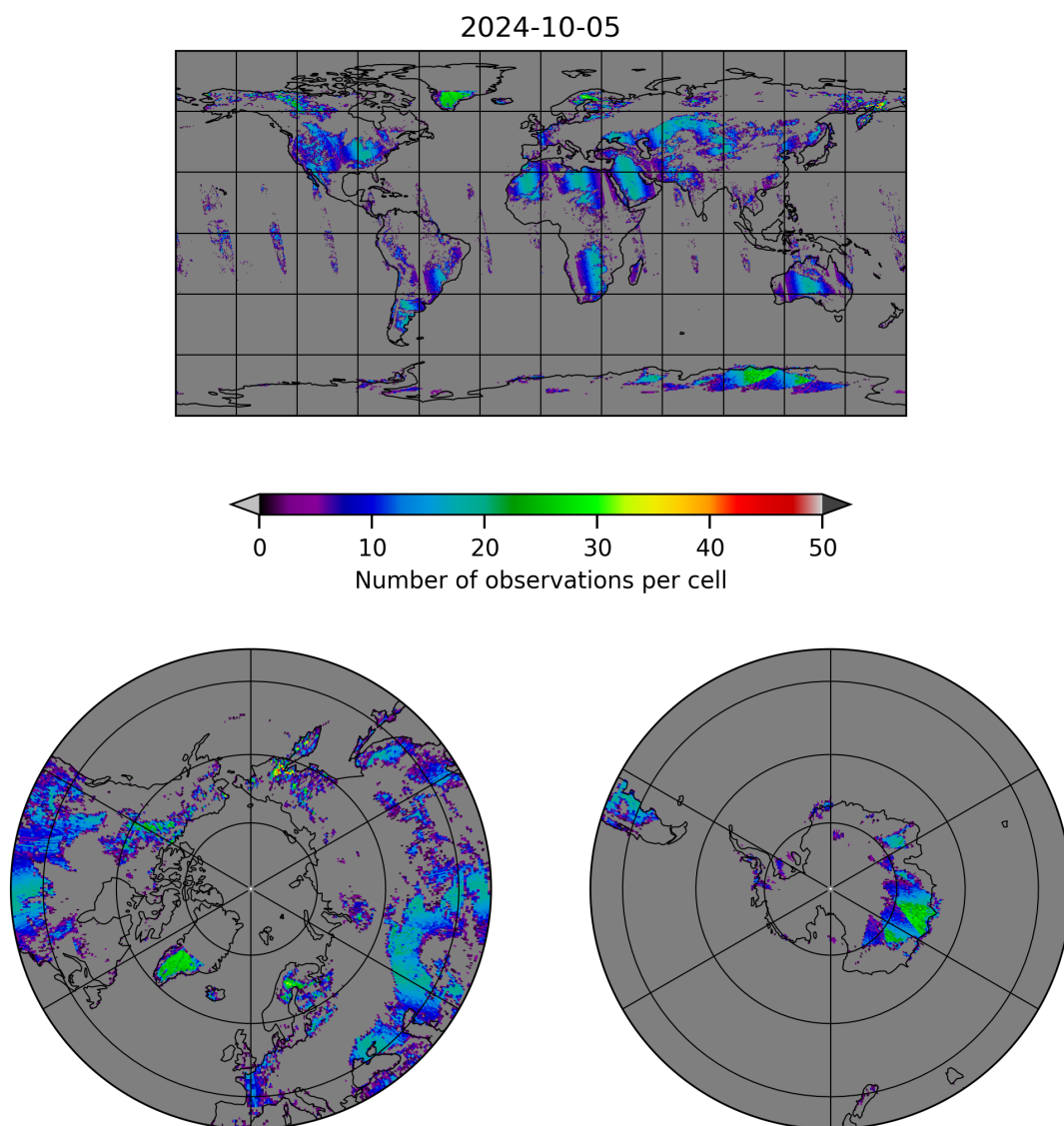
Figure 10: Map of the number of observations for 2024-10-04 to 2024-10-06
