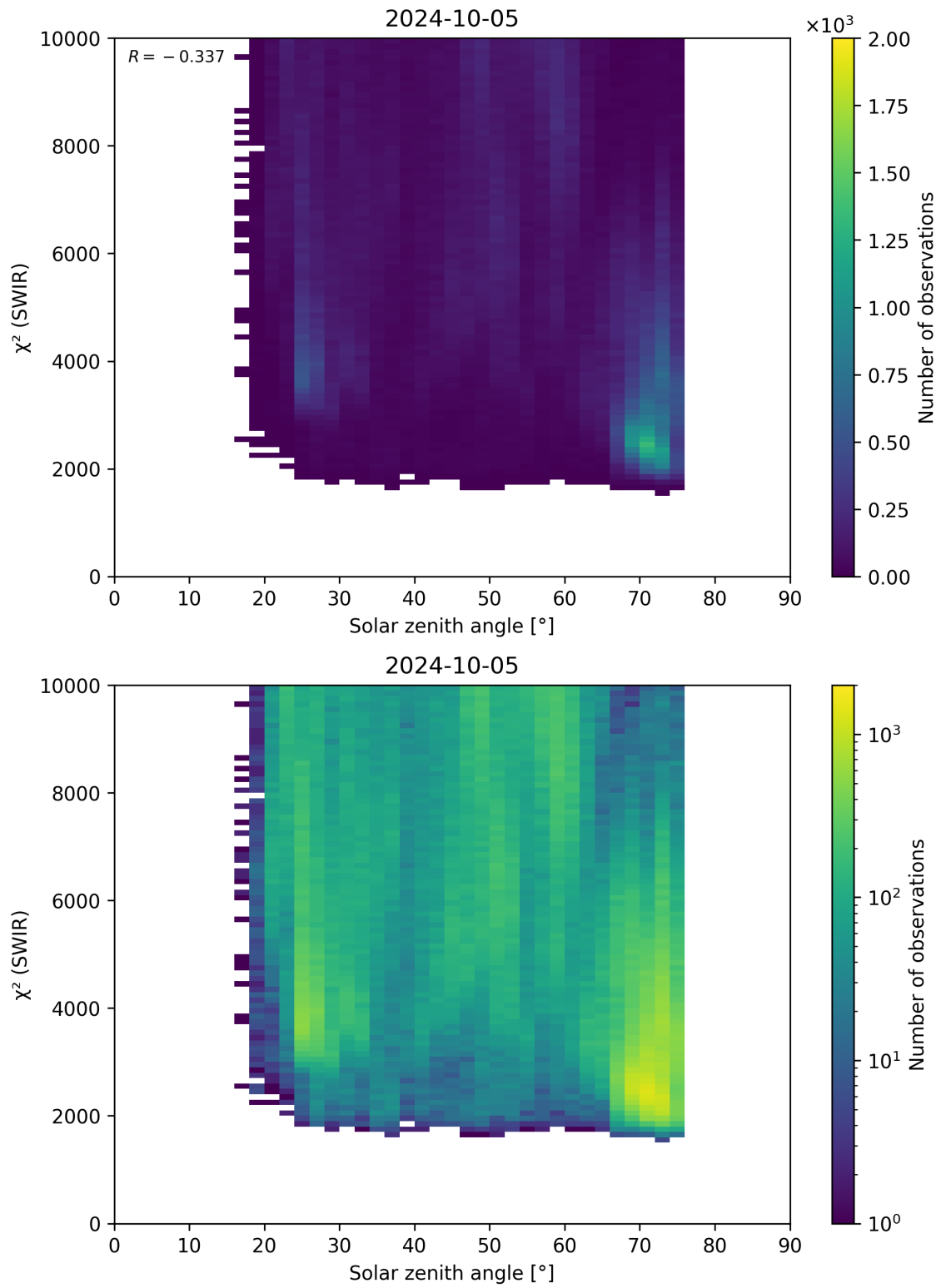
Figure 95: Scatter density plot of “Solar zenith angle” against “ \chi^2 (SWIR)” for 2024-10-04 to 2024-10-06.
