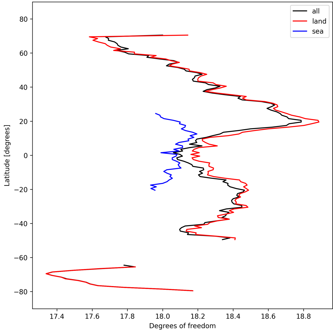
Figure 19: Zonal average of “Degrees of freedom” for 2024-10-04 to 2024-10-06.
