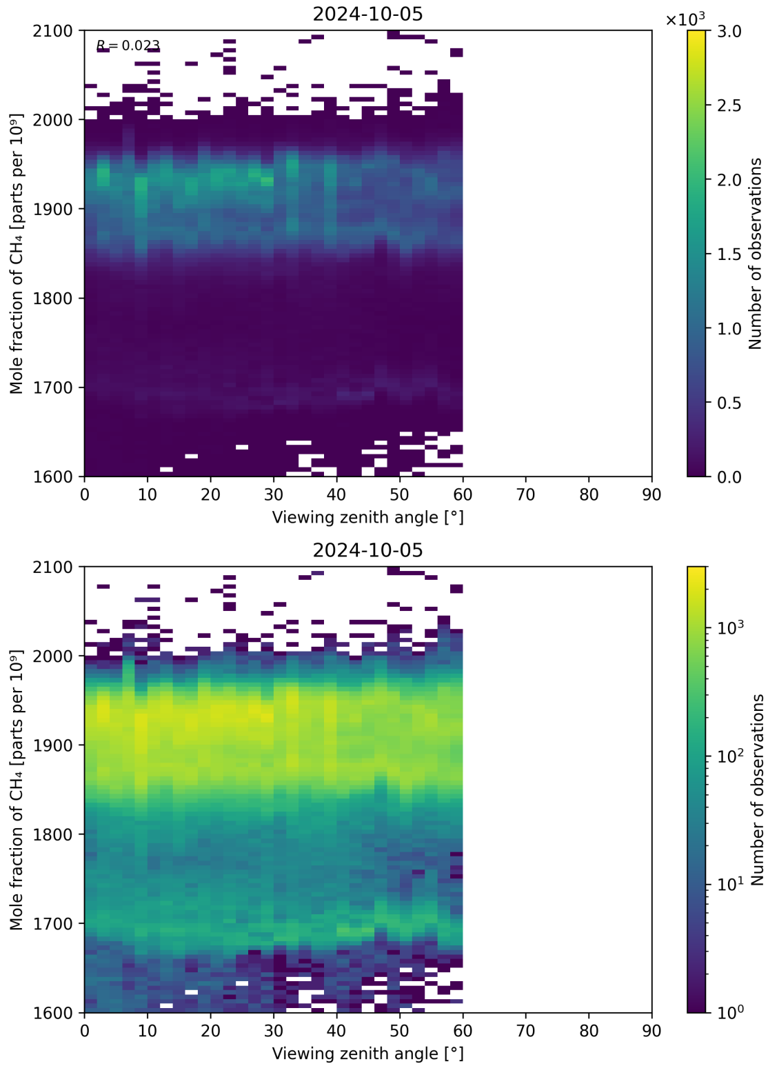
Figure 110: Scatter density plot of “Viewing zenith angle” against “Mole fraction of CH 4 ” for 2024-10-04 to 2024-10-06.
