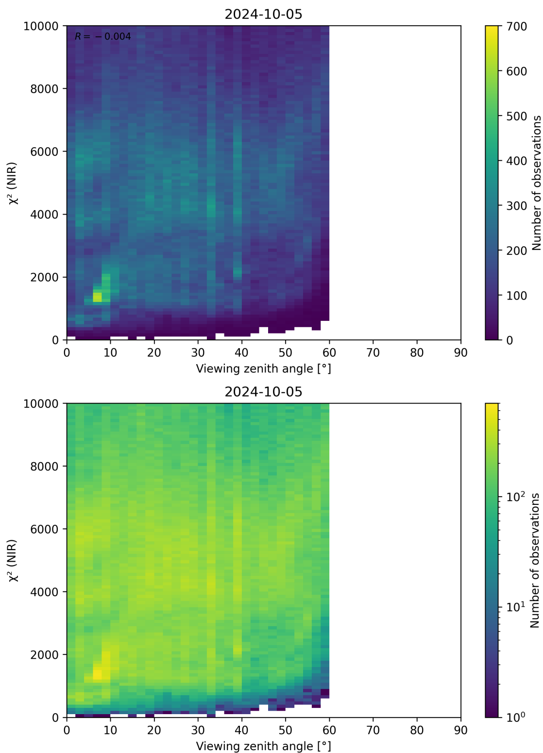
Figure 105: Scatter density plot of “Viewing zenith angle” against “ \chi^2 (NIR)” for 2024-10-04 to 2024-10-06.
