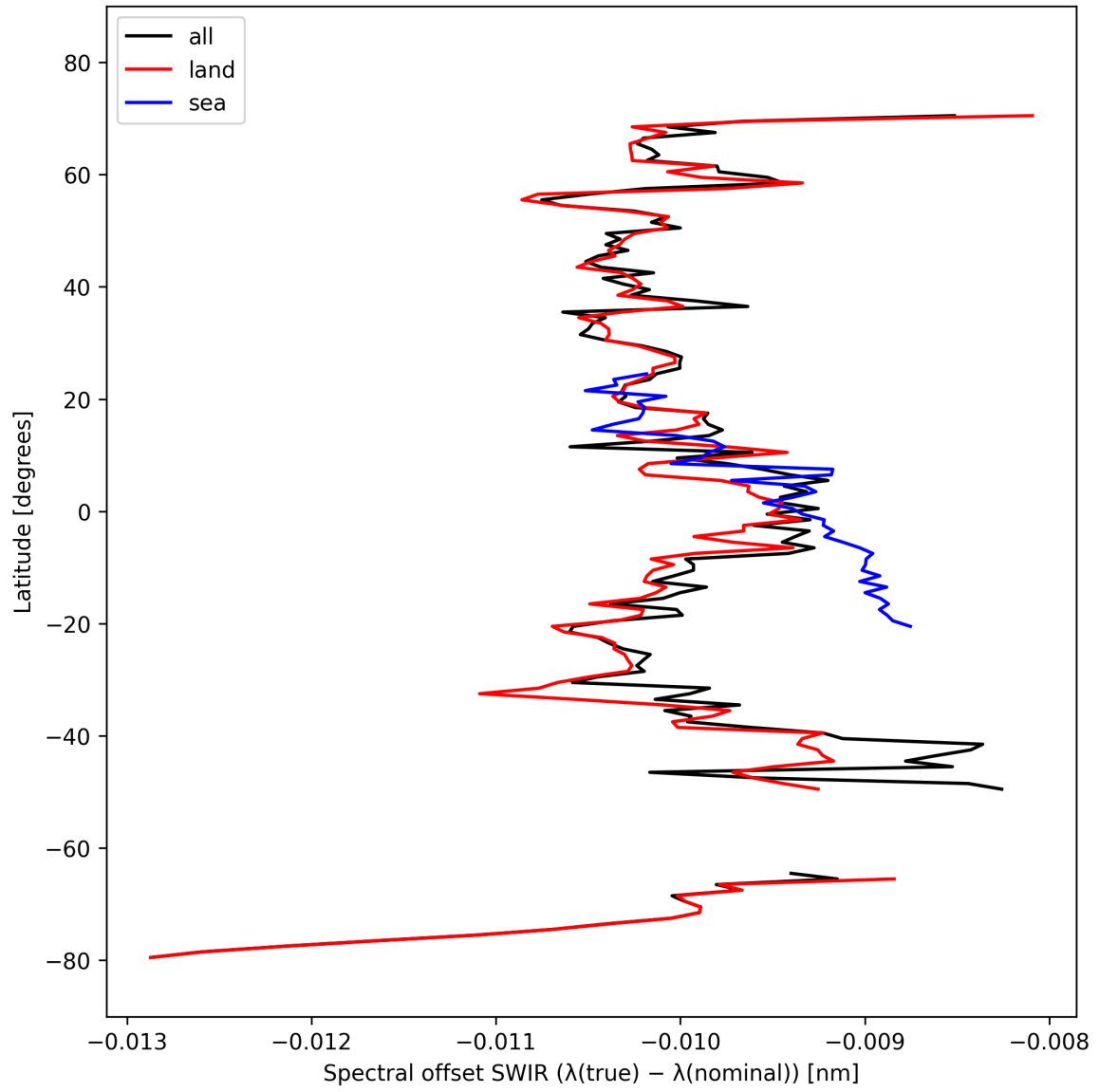
Figure 16: Zonal average of “Spectral offset SWIR ( \lambda_{\text{true}} - \lambda_{\text{nominal}} )” for 2024-10-04 to 2024-10-06.
