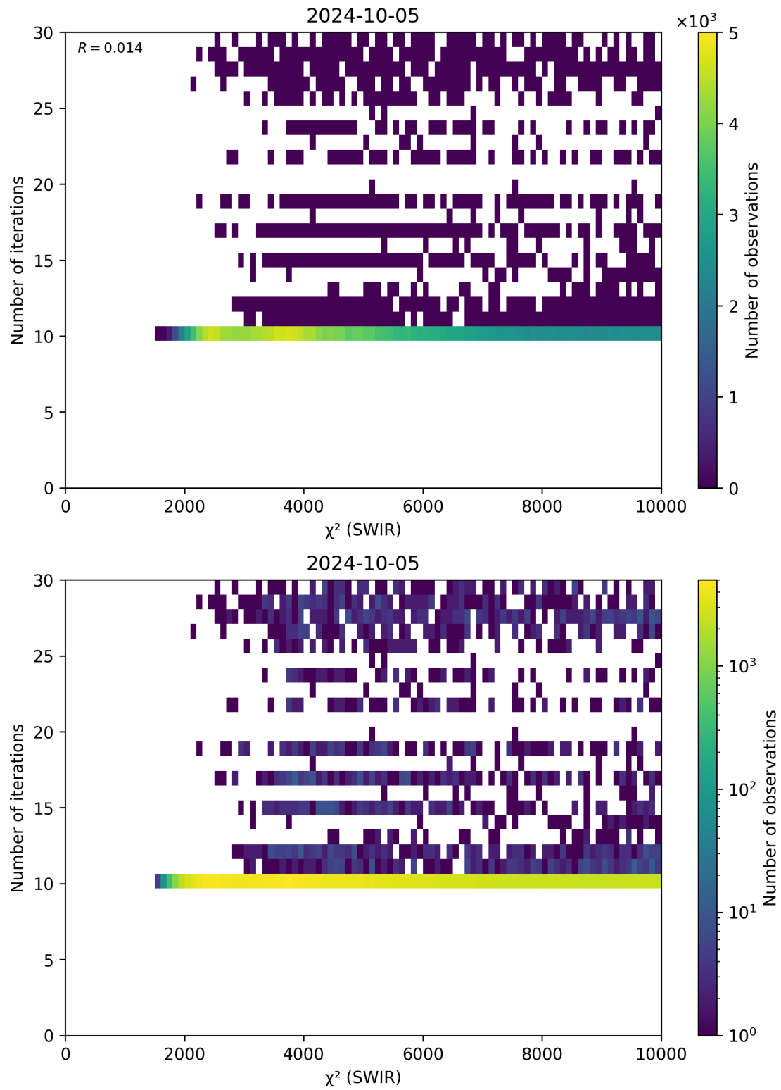
Figure 50: Scatter density plot of “ \chi^2 (SWIR)” against “Number of iterations” for 2024-10-04 to 2024-10-06.
