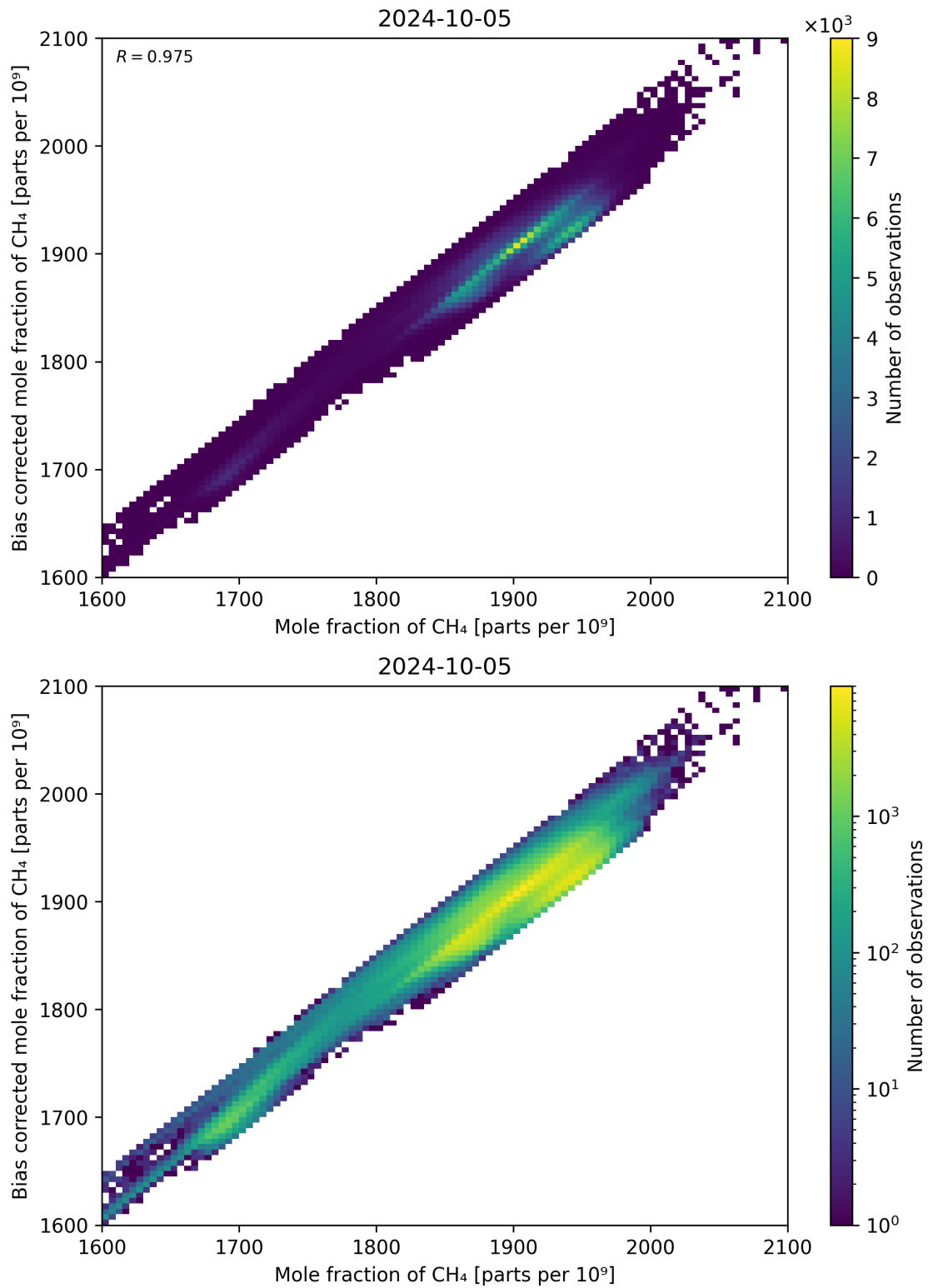
Figure 74: Scatter density plot of “Mole fraction of CH 4 ” against “Bias corrected mole fraction of CH 4 ” for 2024-10-04 to 2024-10-06.
