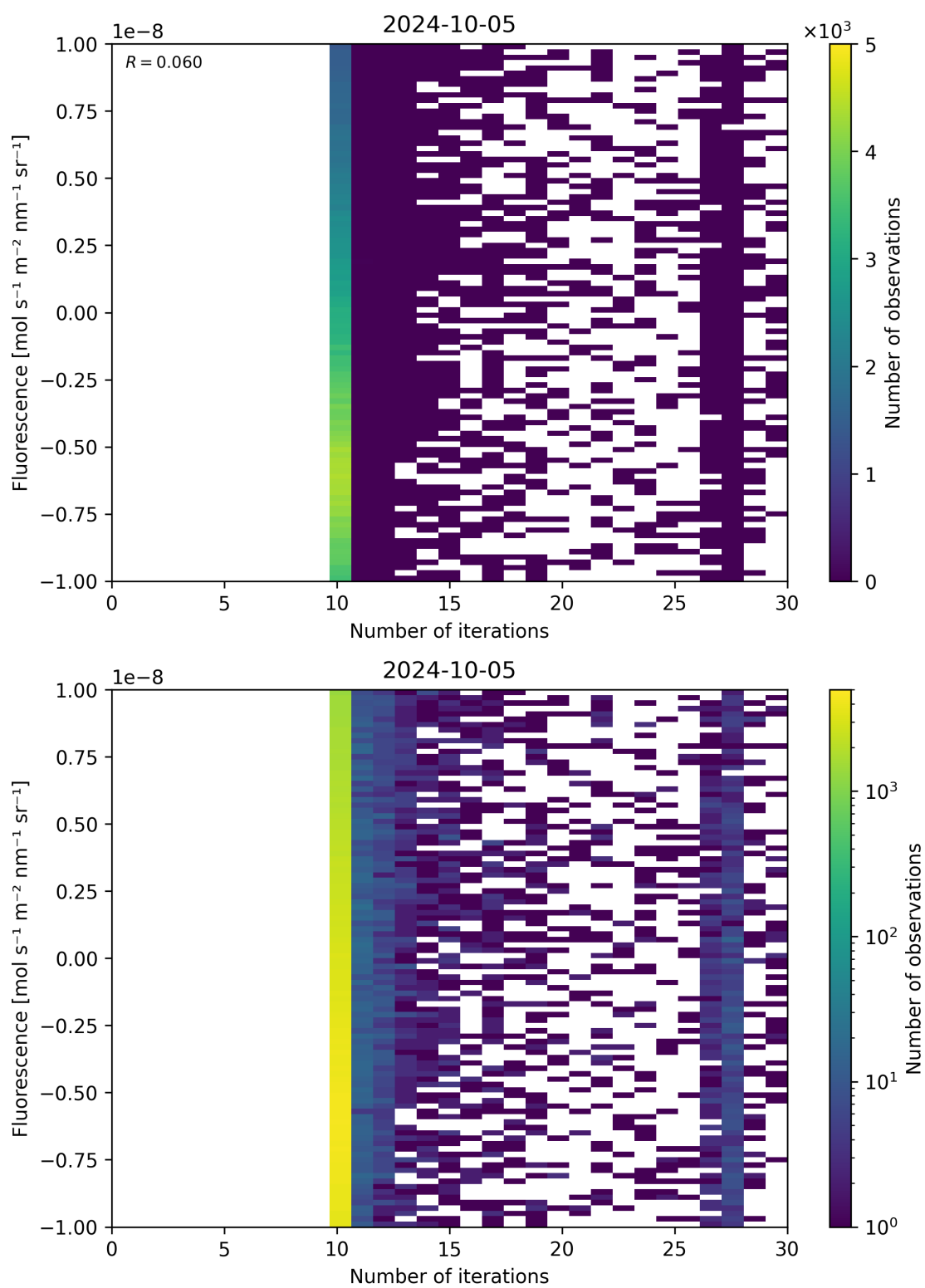
Figure 87: Scatter density plot of “Number of iterations” against “Fluorescence” for 2024-10-04 to 2024-10-06.
