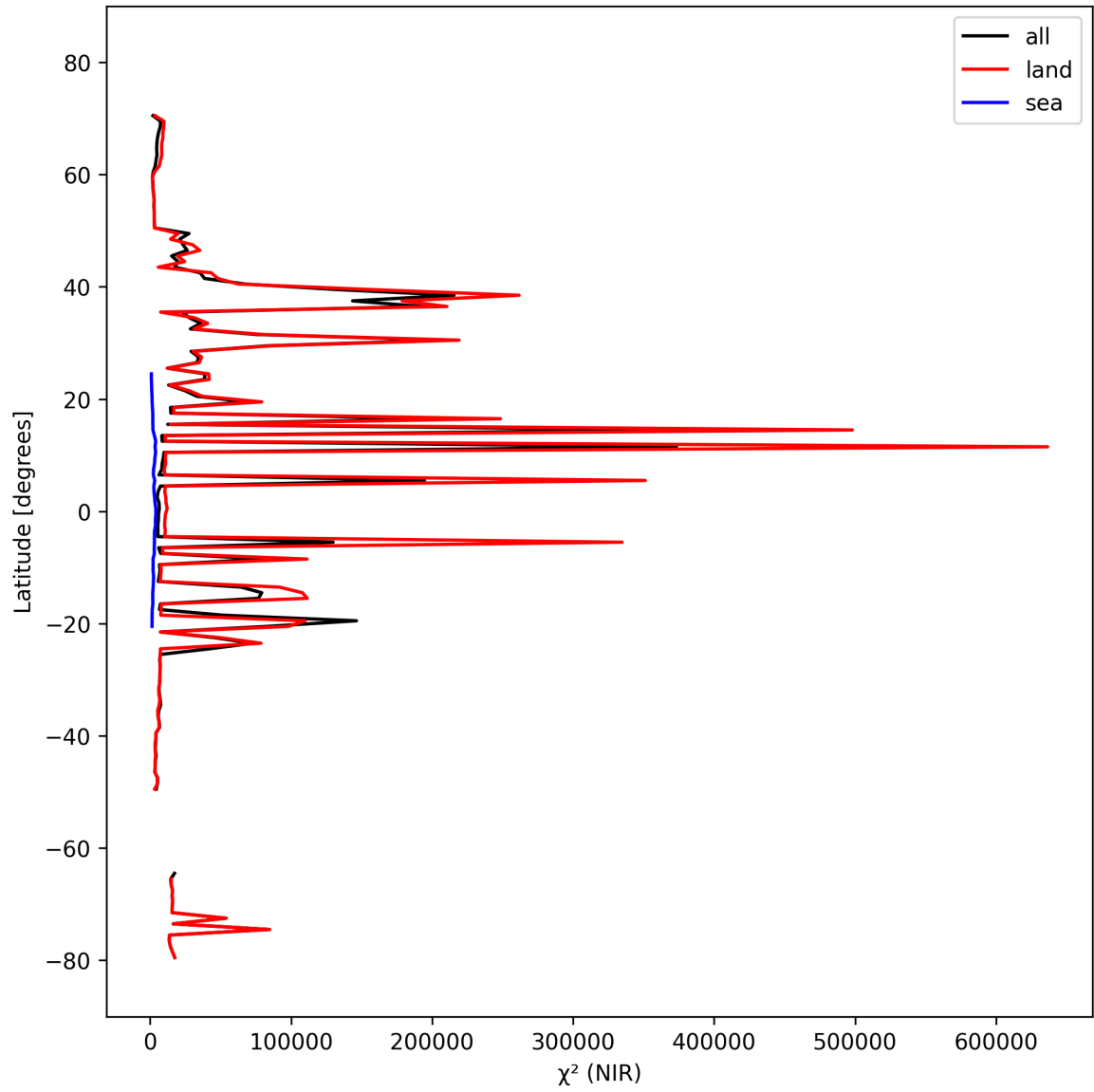
Figure 18: Zonal average of “ \chi^2 (NIR)” for 2024-10-04 to 2024-10-06.
