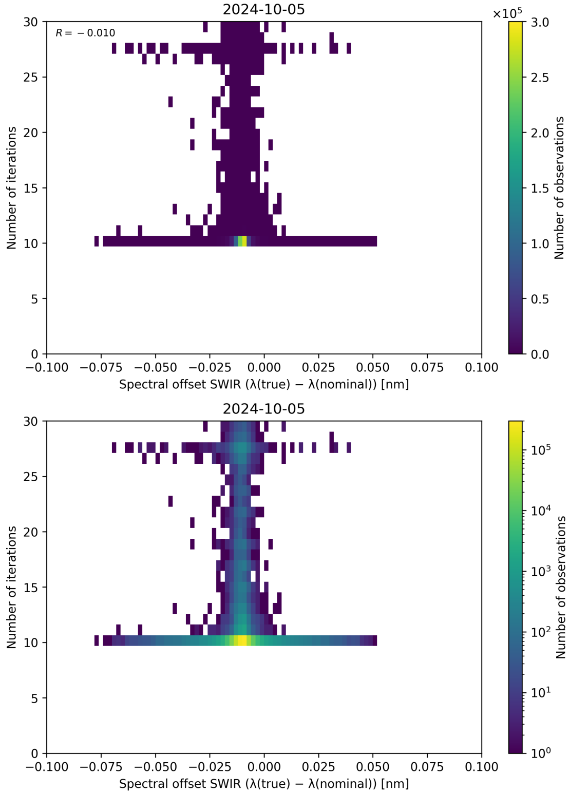
Figure 121: Scatter density plot of “Spectral offset SWIR ( \lambda_{\text{true}} - \lambda_{\text{nominal}} )” against “Number of iterations” for 2024-10-04 to 2024-10-06.
