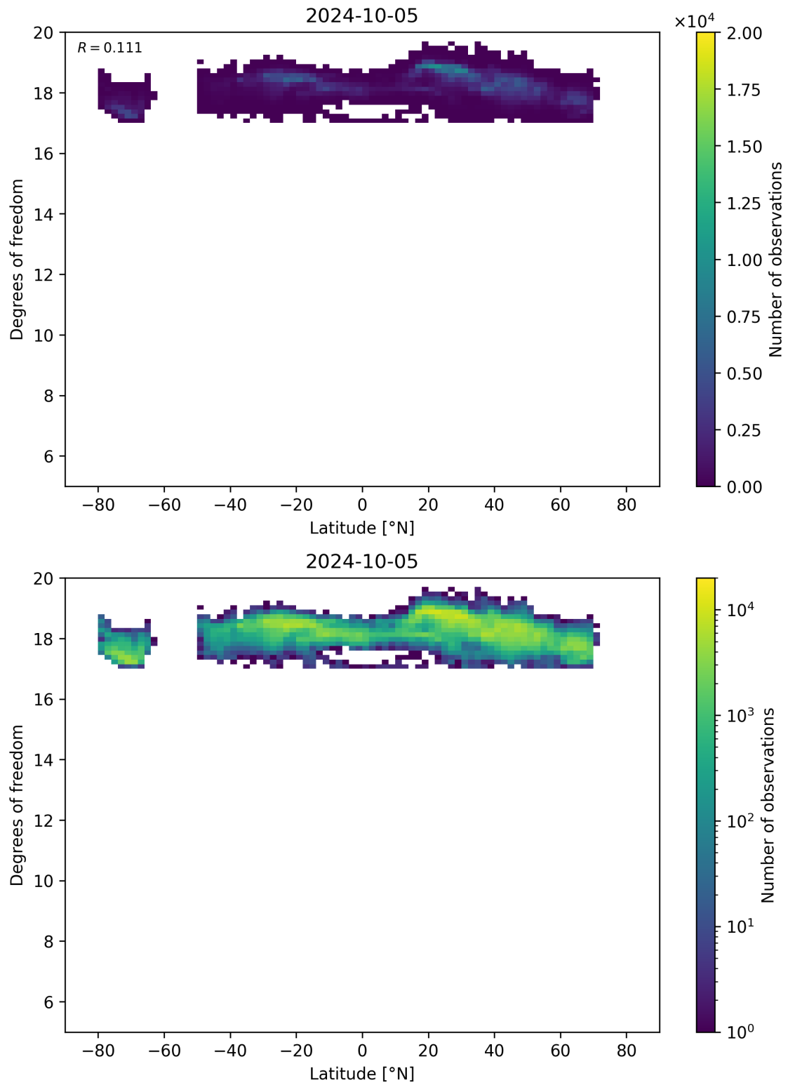
Figure 55: Scatter density plot of “Latitude” against “Degrees of freedom” for 2024-10-04 to 2024-10-06.
