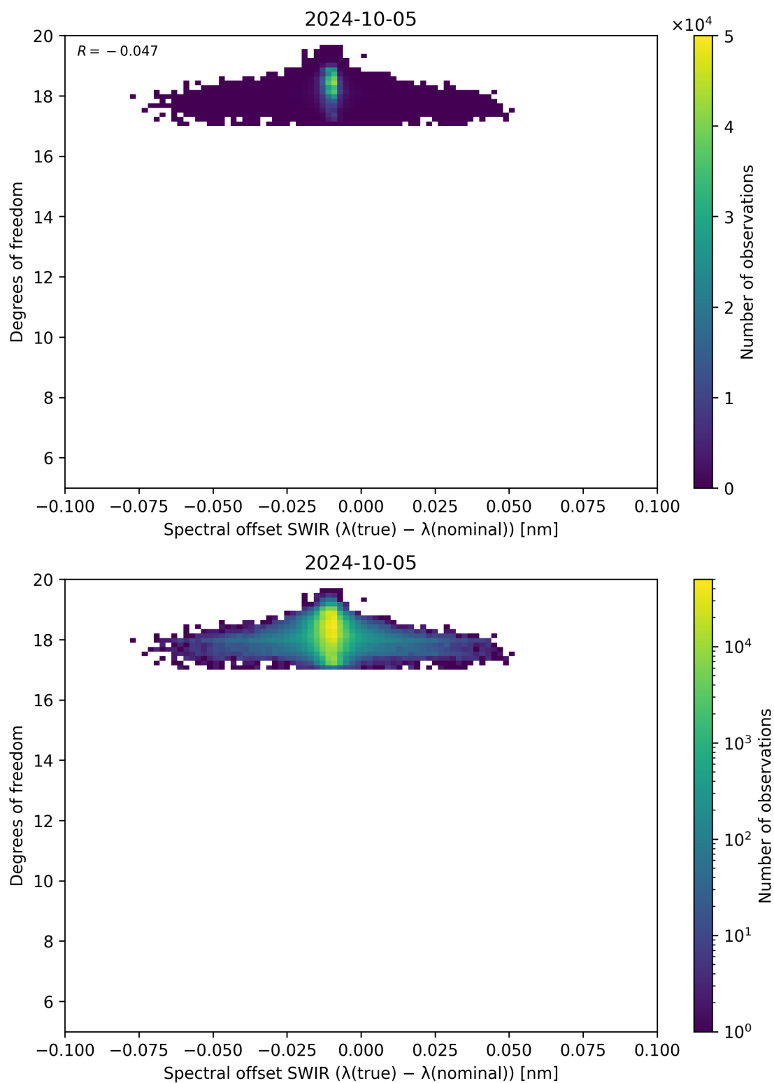
Figure 119: Scatter density plot of “Spectral offset SWIR ( \lambda_{\text{true}} - \lambda_{\text{nominal}} )” against “Degrees of freedom” for 2024-10-04 to 2024-10-06.
