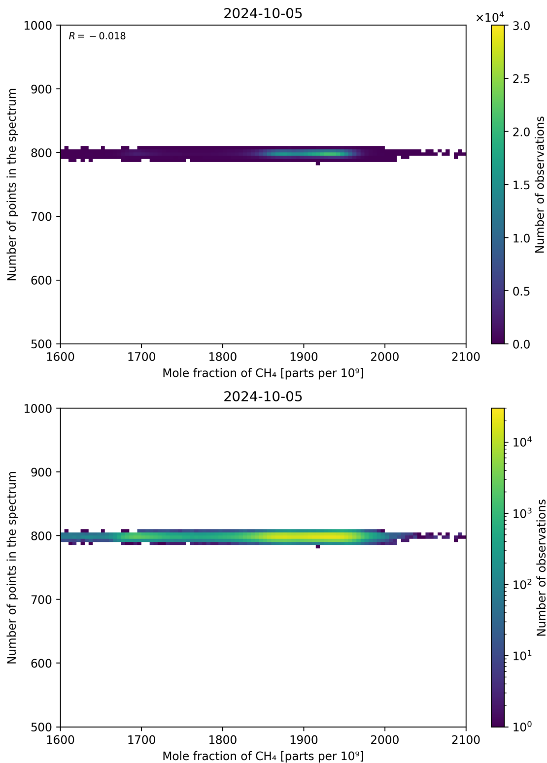
Figure 77: Scatter density plot of “Mole fraction of CH 4 ” against “Number of points in the spectrum” for 2024-10-04 to 2024-10-06.
