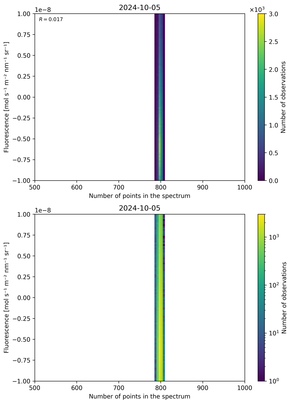
Figure 91: Scatter density plot of “Number of points in the spectrum” against “Fluorescence” for 2024-10-04 to 2024-10-06.
