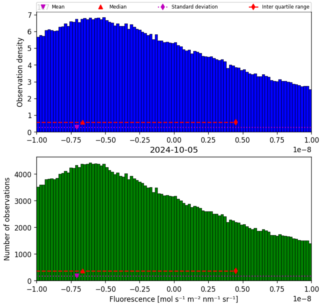
Figure 32: Histogram of “Fluorescence” for 2024-10-04 to 2024-10-06
