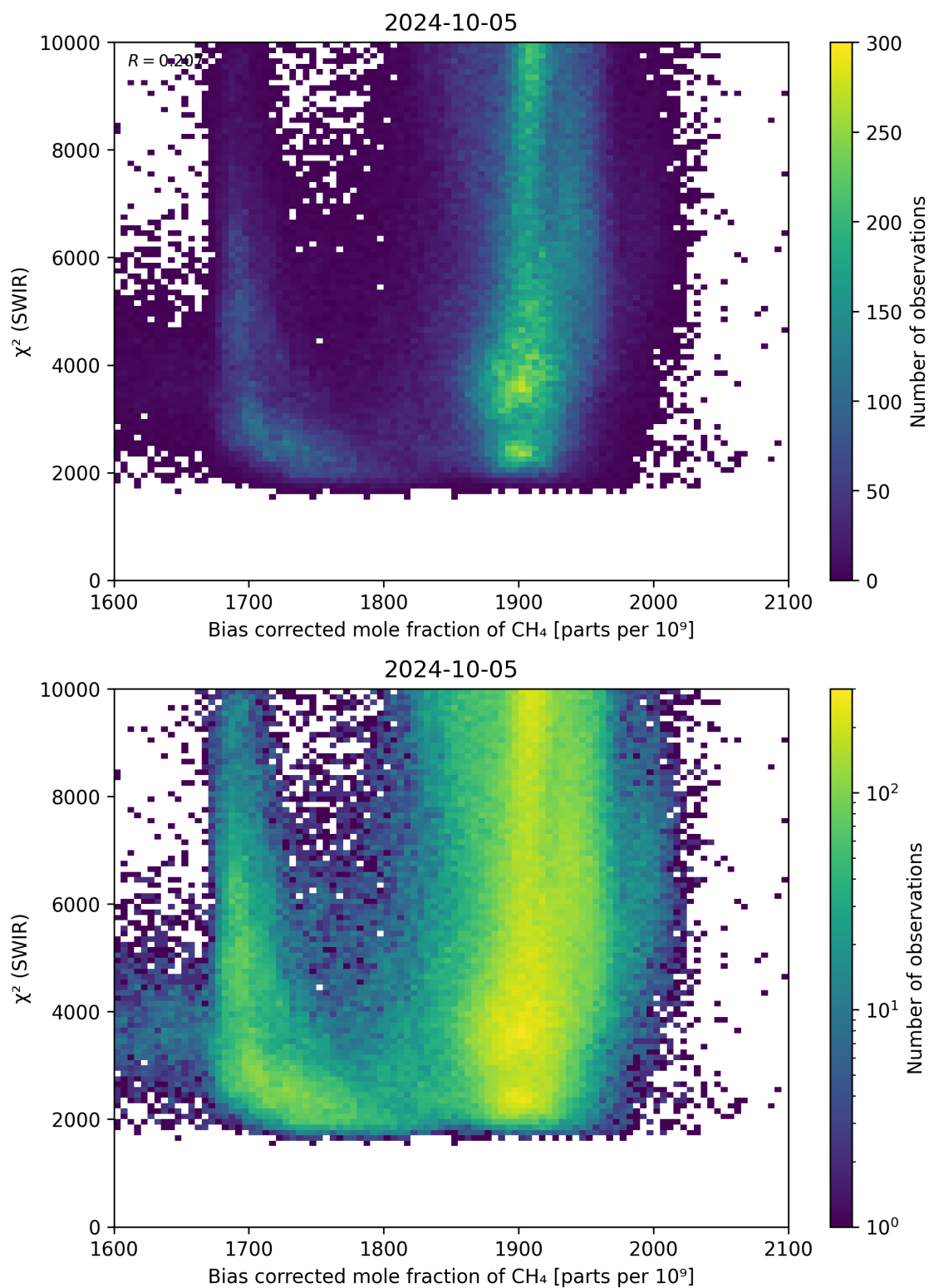
Figure 64: Scatter density plot of “Bias corrected mole fraction of \text{CH}_4 ” against “ \chi^2 (SWIR)” for 2024-10-04 to 2024-10-06.
