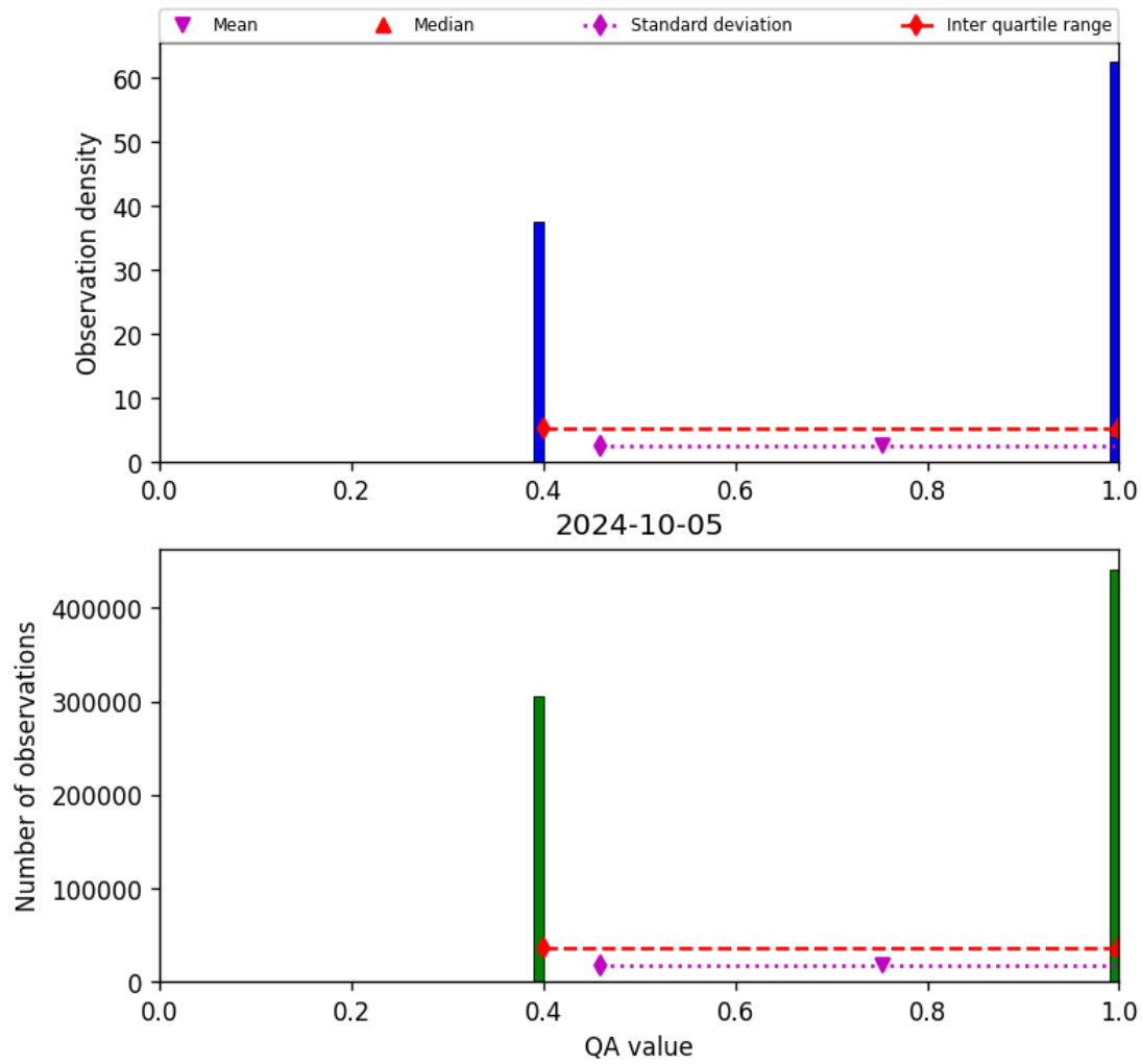
Figure 22: Histogram of “QA value” for 2024-10-04 to 2024-10-06
