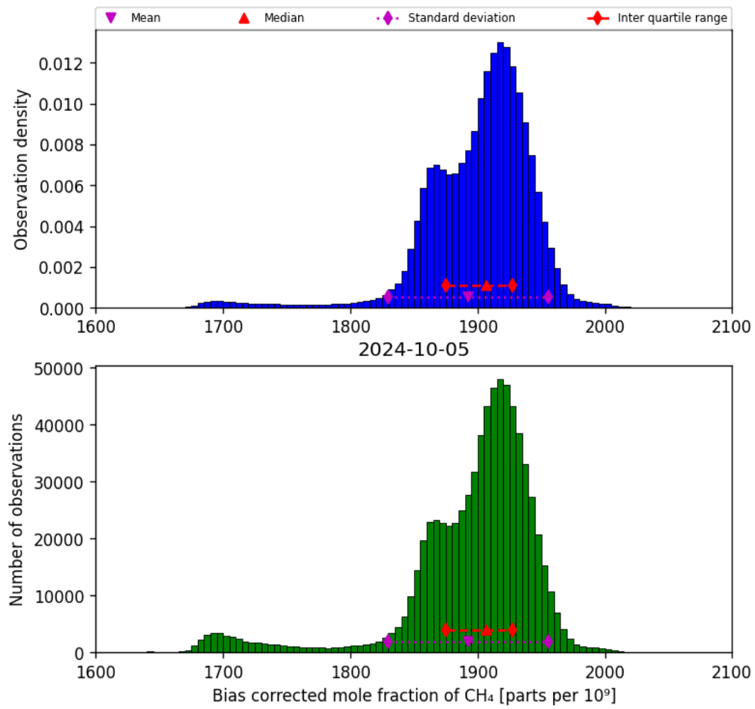
Figure 25: Histogram of “Bias corrected mole fraction of CH 4 ” for 2024-10-04 to 2024-10-06
