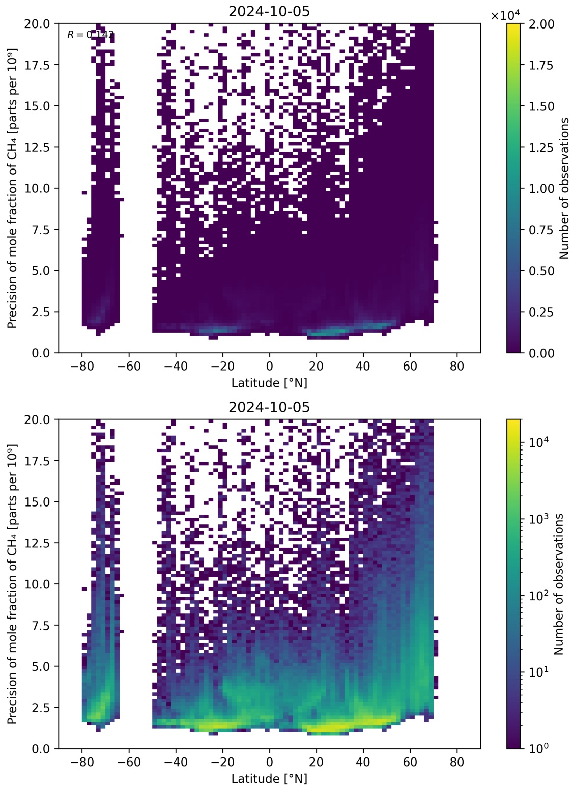
Figure 59: Scatter density plot of “Latitude” against “Precision of mole fraction of \text{CH}_4 ” for 2024-10-04 to 2024-10-06.
