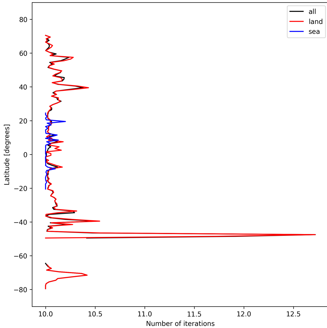
Figure 20: Zonal average of “Number of iterations” for 2024-10-04 to 2024-10-06.
