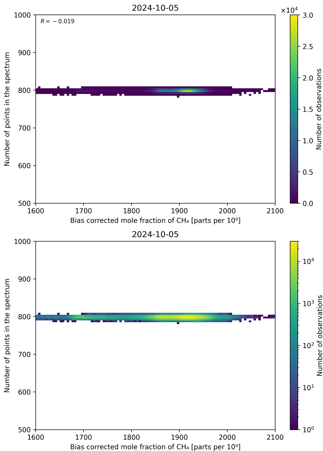
Figure 68: Scatter density plot of “Bias corrected mole fraction of CH 4 ” against “Number of points in the spectrum” for 2024-10-04 to 2024-10-06.
