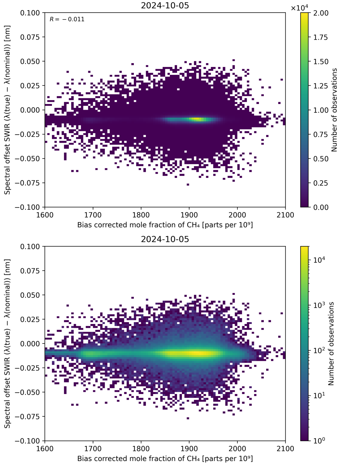
Figure 69: Scatter density plot of “Bias corrected mole fraction of \text{CH}_4 ” against “Spectral offset SWIR ( \lambda_{\text{true}} - \lambda_{\text{nominal}} )” for 2024-10-04 to 2024-10-06.
