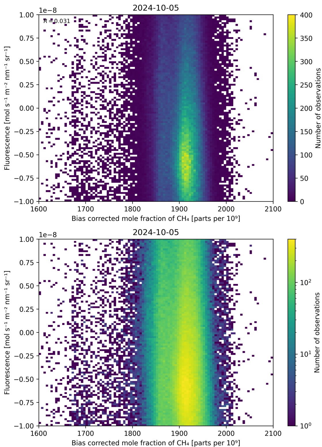
Figure 66: Scatter density plot of “Bias corrected mole fraction of \text{CH}_4 ” against “Fluorescence” for 2024-10-04 to 2024-10-06.
