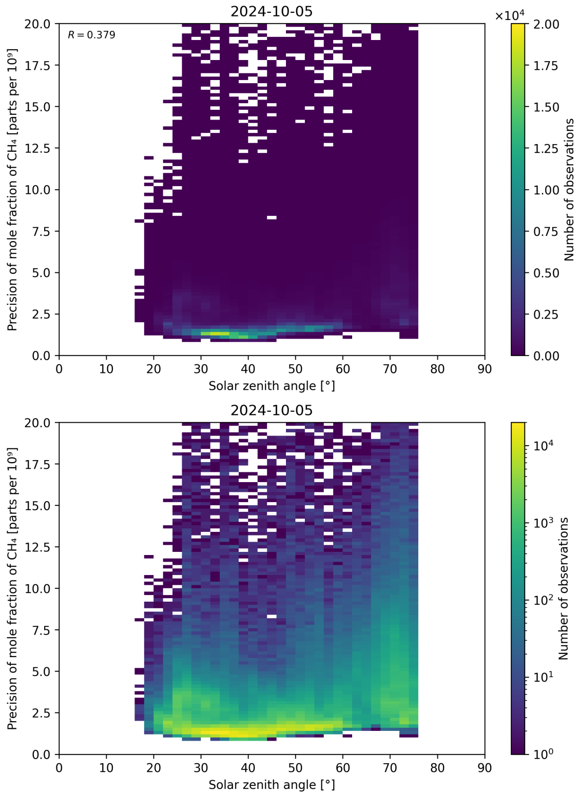
Figure 101: Scatter density plot of “Solar zenith angle” against “Precision of mole fraction of CH 4 ” for 2024-10-04 to 2024-10-06.
