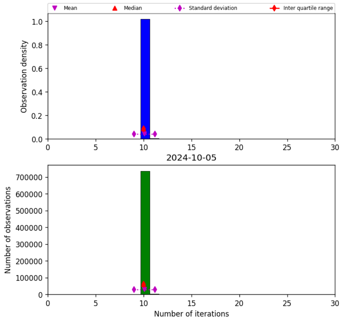
Figure 31: Histogram of “Number of iterations” for 2024-10-04 to 2024-10-06
