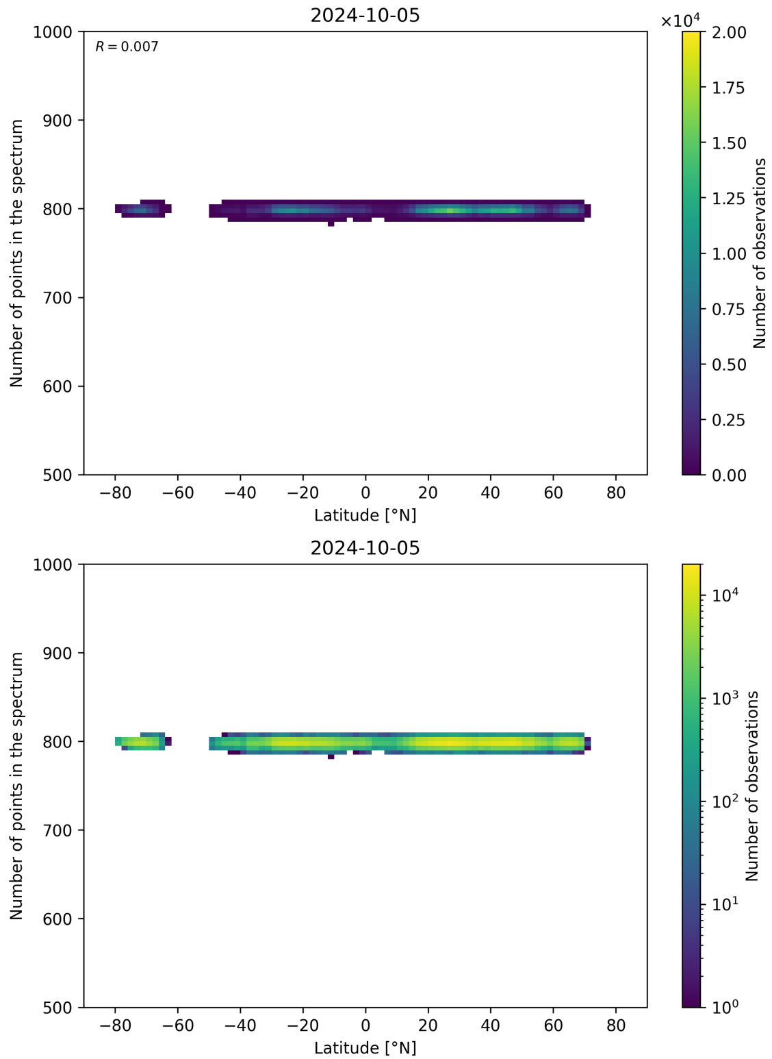
Figure 61: Scatter density plot of “Latitude” against “Number of points in the spectrum” for 2024-10-04 to 2024-10-06.
