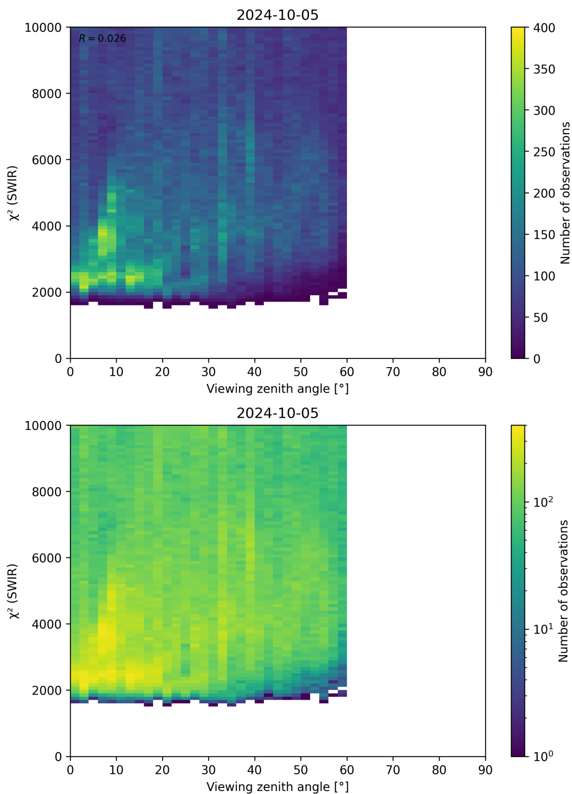
Figure 106: Scatter density plot of “Viewing zenith angle” against “ \chi^2 (SWIR)” for 2024-10-04 to 2024-10-06.
