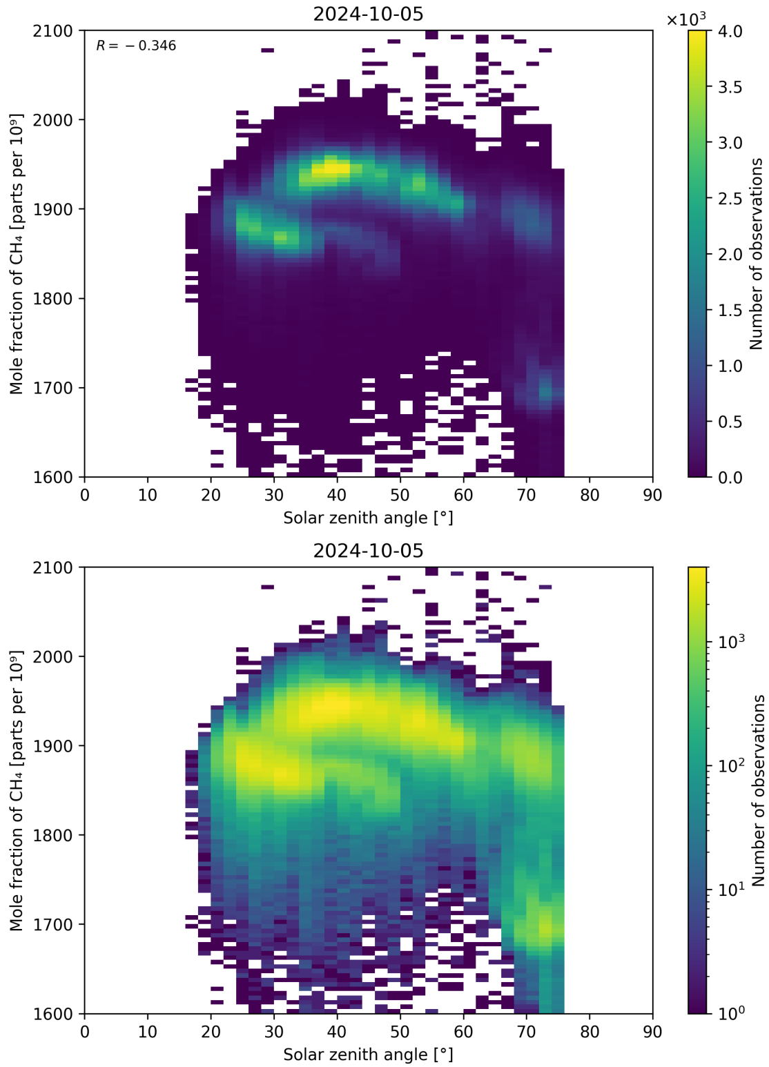
Figure 99: Scatter density plot of “Solar zenith angle” against “Mole fraction of \text{CH}_4 ” for 2024-10-04 to 2024-10-06.
