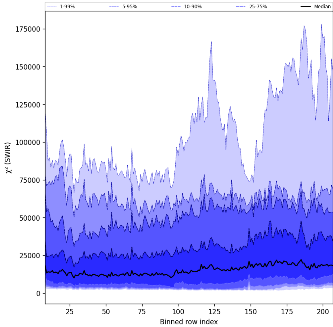
Figure 39: Along track statistics of “ \chi^2 (SWIR)” for 2024-10-04 to 2024-10-06
