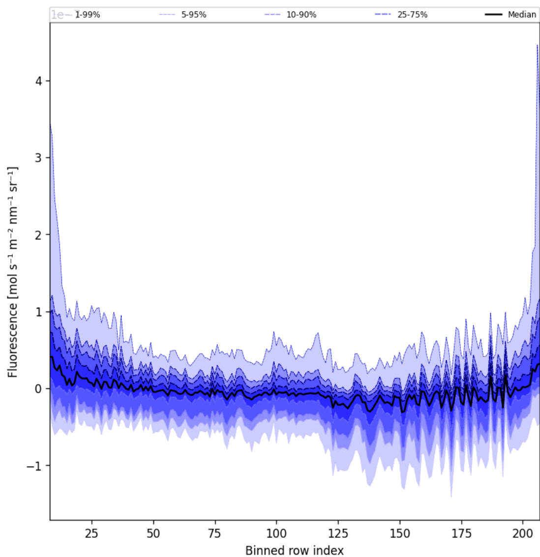
Figure 43: Along track statistics of “Fluorescence” for 2024-10-04 to 2024-10-06
