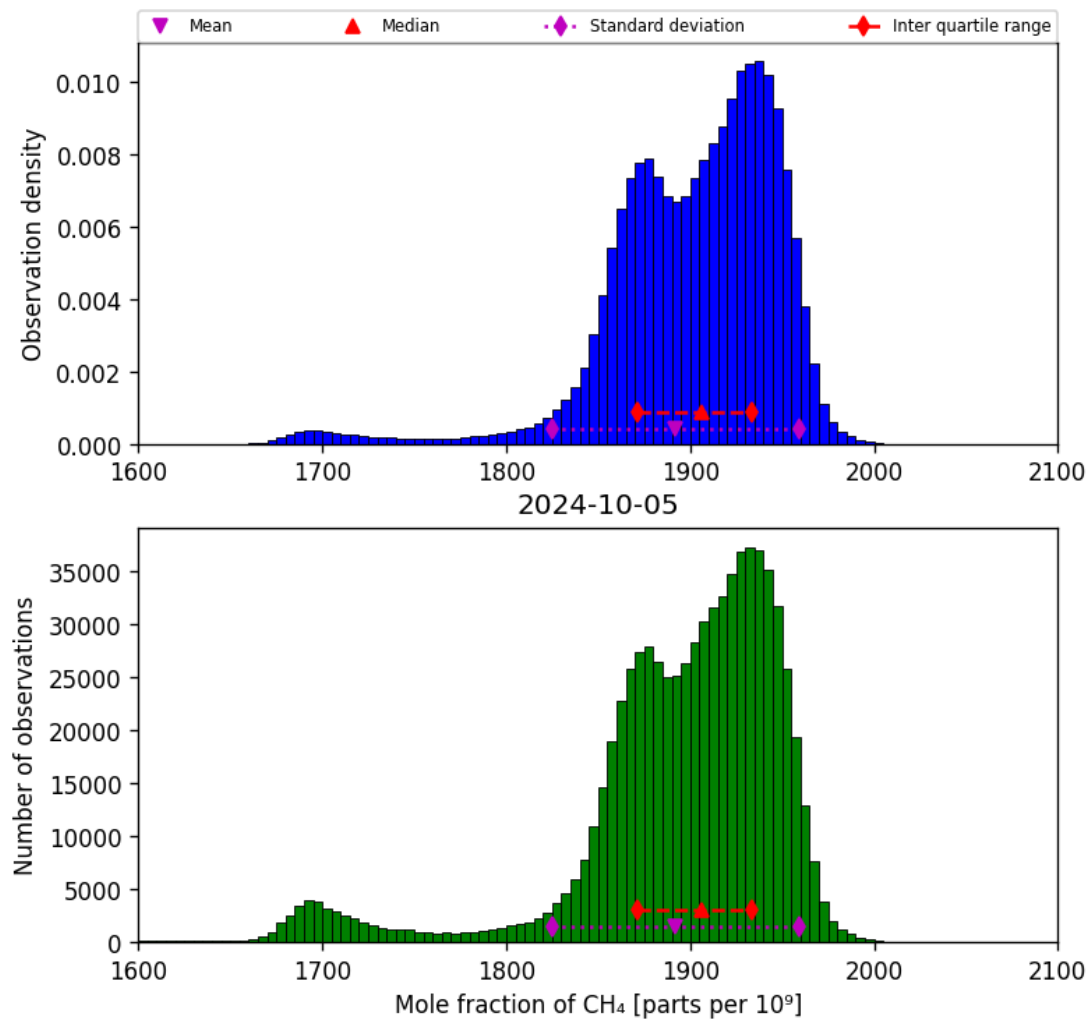
Figure 23: Histogram of “Mole fraction of CH 4 ” for 2024-10-04 to 2024-10-06
