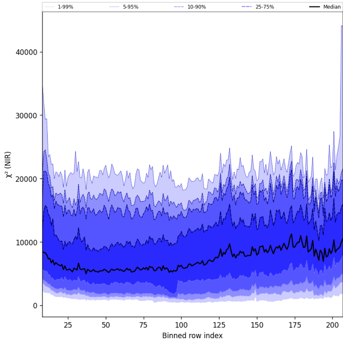
Figure 40: Along track statistics of “ \chi^2 (NIR)” for 2024-10-04 to 2024-10-06
