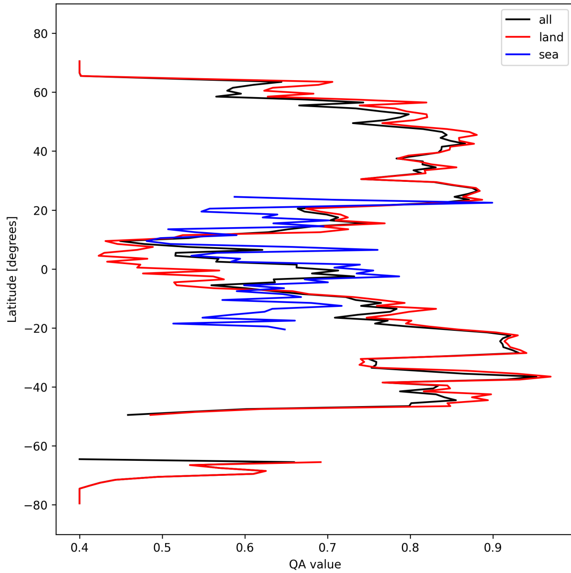
Figure 11: Zonal average of “QA value” for 2024-10-04 to 2024-10-06.
