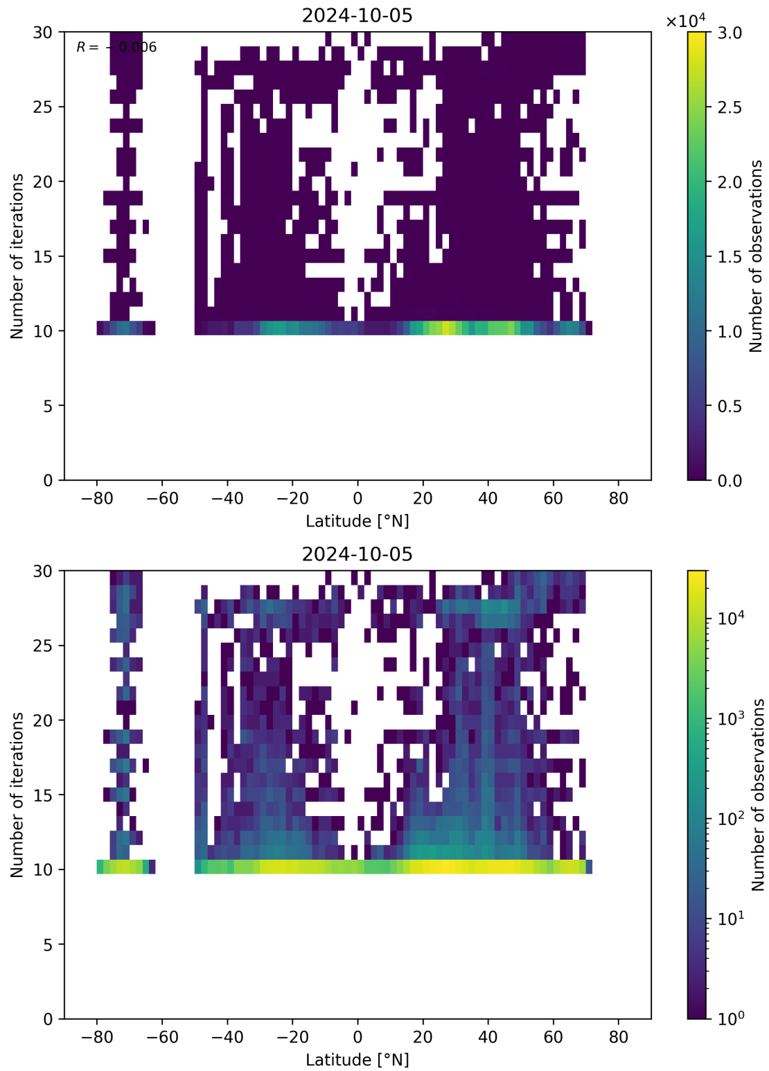
Figure 60: Scatter density plot of “Latitude” against “Number of iterations” for 2024-10-04 to 2024-10-06.
