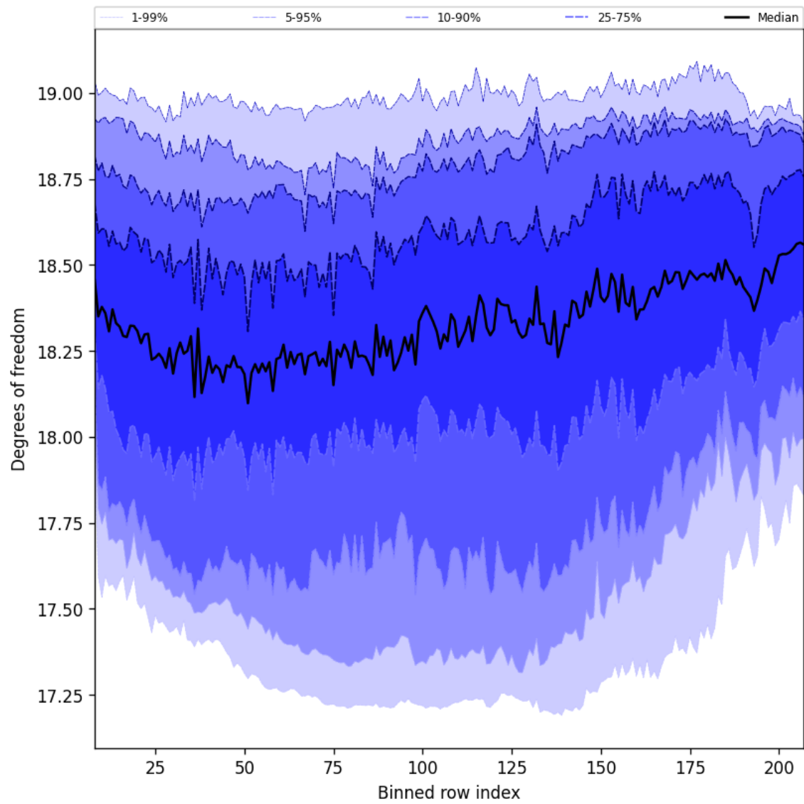
Figure 41: Along track statistics of “Degrees of freedom” for 2024-10-04 to 2024-10-06
