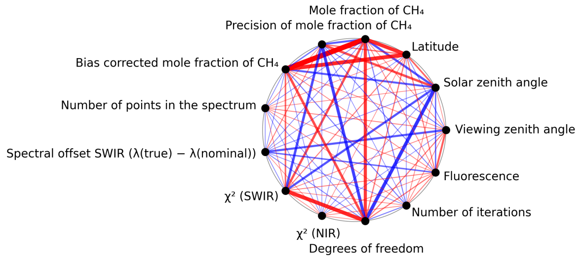
Figure 1: Map of correlation graph for 2024-10-04 to 2024-10-06.
