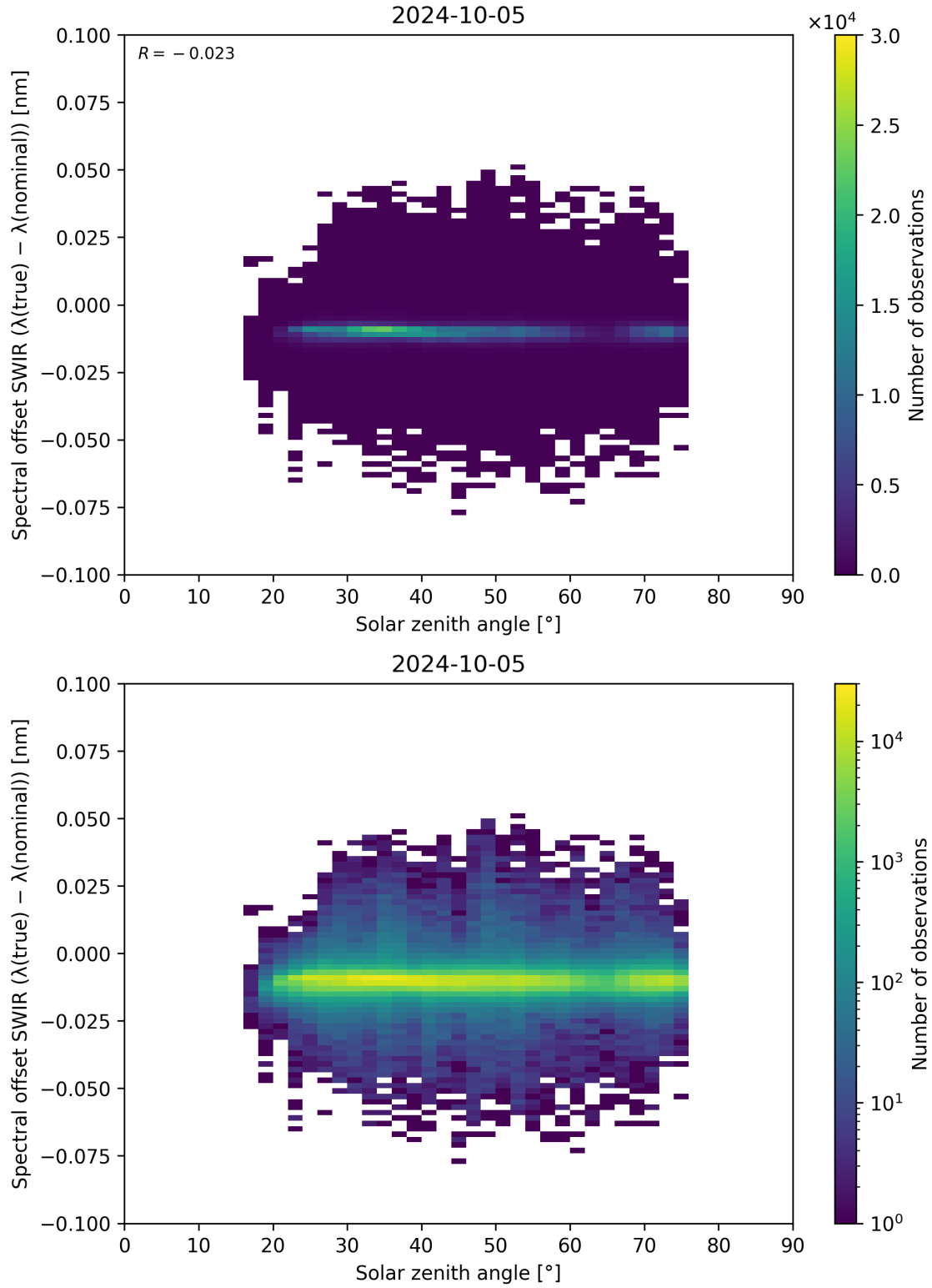
Figure 104: Scatter density plot of “Solar zenith angle” against “Spectral offset SWIR ( \lambda_{\text{true}} - \lambda_{\text{nominal}} )” for 2024-10-04 to 2024-10-06.
