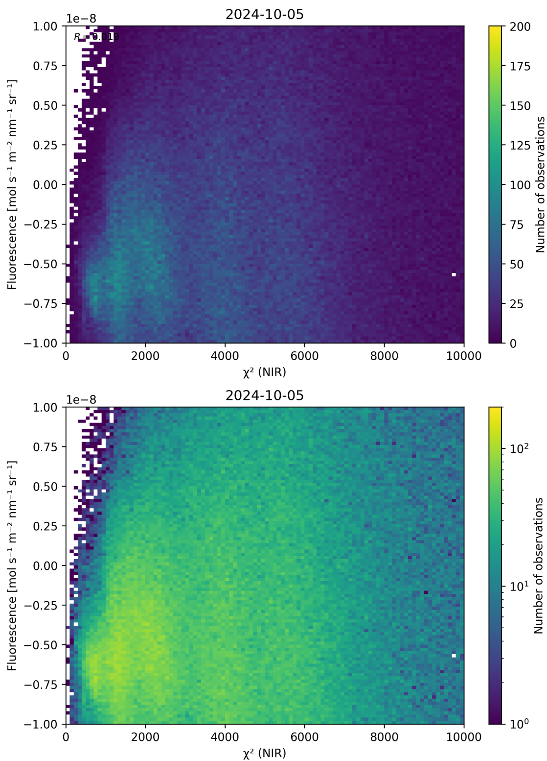
Figure 45: Scatter density plot of “ \chi^2 (NIR)” against “Fluorescence” for 2024-10-04 to 2024-10-06.
