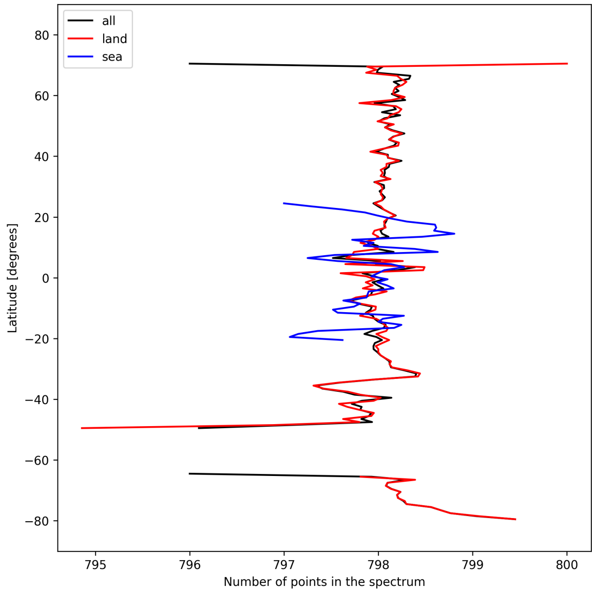
Figure 15: Zonal average of “Number of points in the spectrum” for 2024-10-04 to 2024-10-06.
