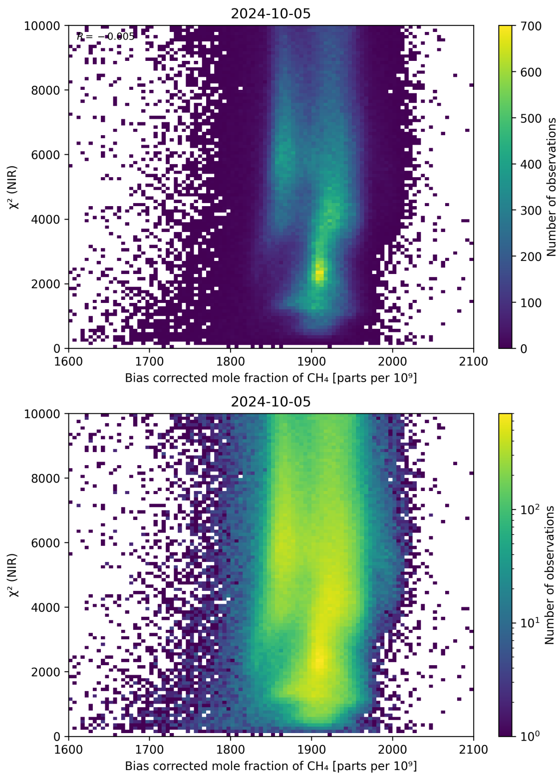
Figure 63: Scatter density plot of “Bias corrected mole fraction of \text{CH}_4 ” against “ \chi^2 (NIR)” for 2024-10-04 to 2024-10-06.
