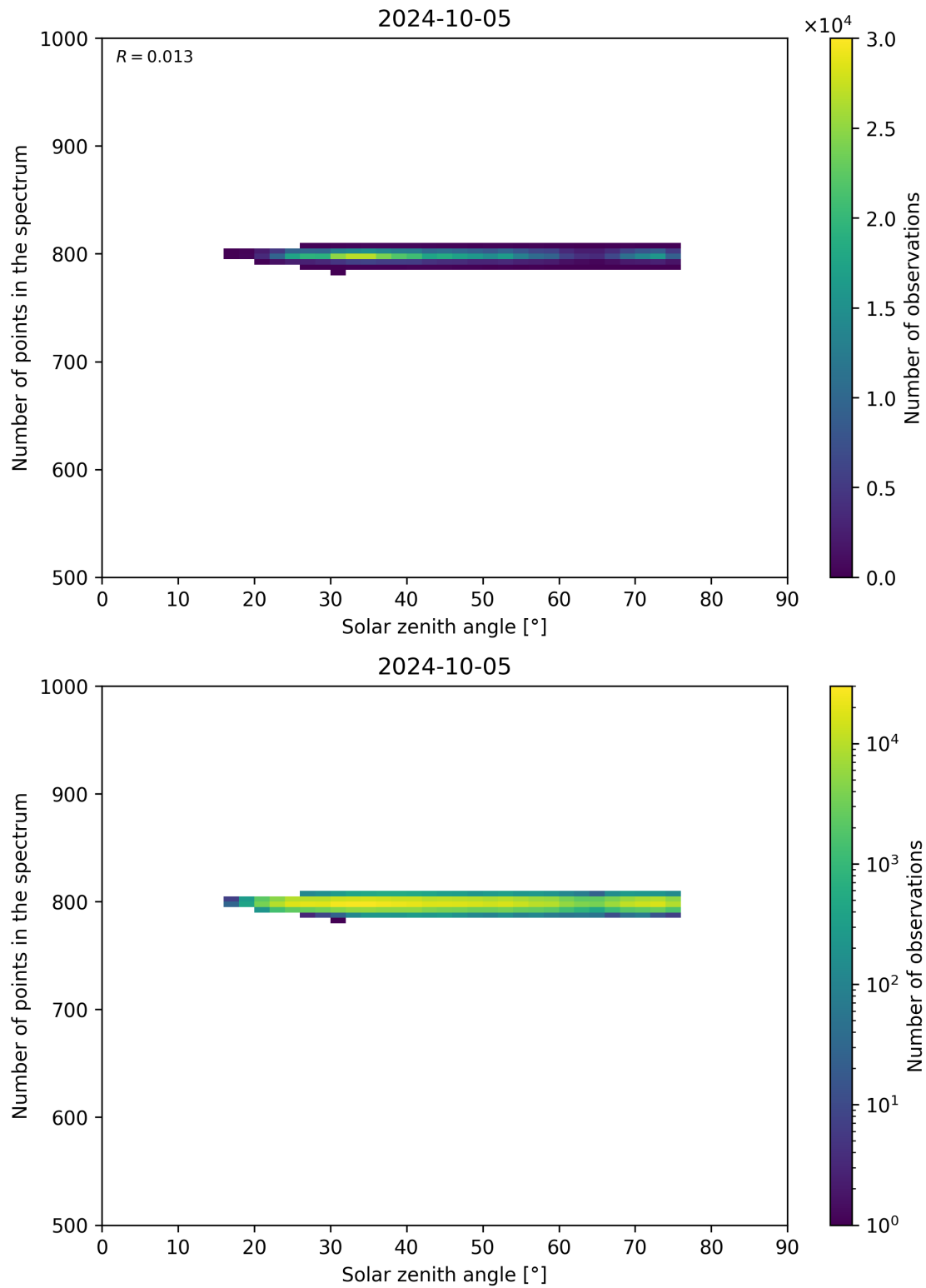
Figure 103: Scatter density plot of “Solar zenith angle” against “Number of points in the spectrum” for 2024-10-04 to 2024-10-06.
