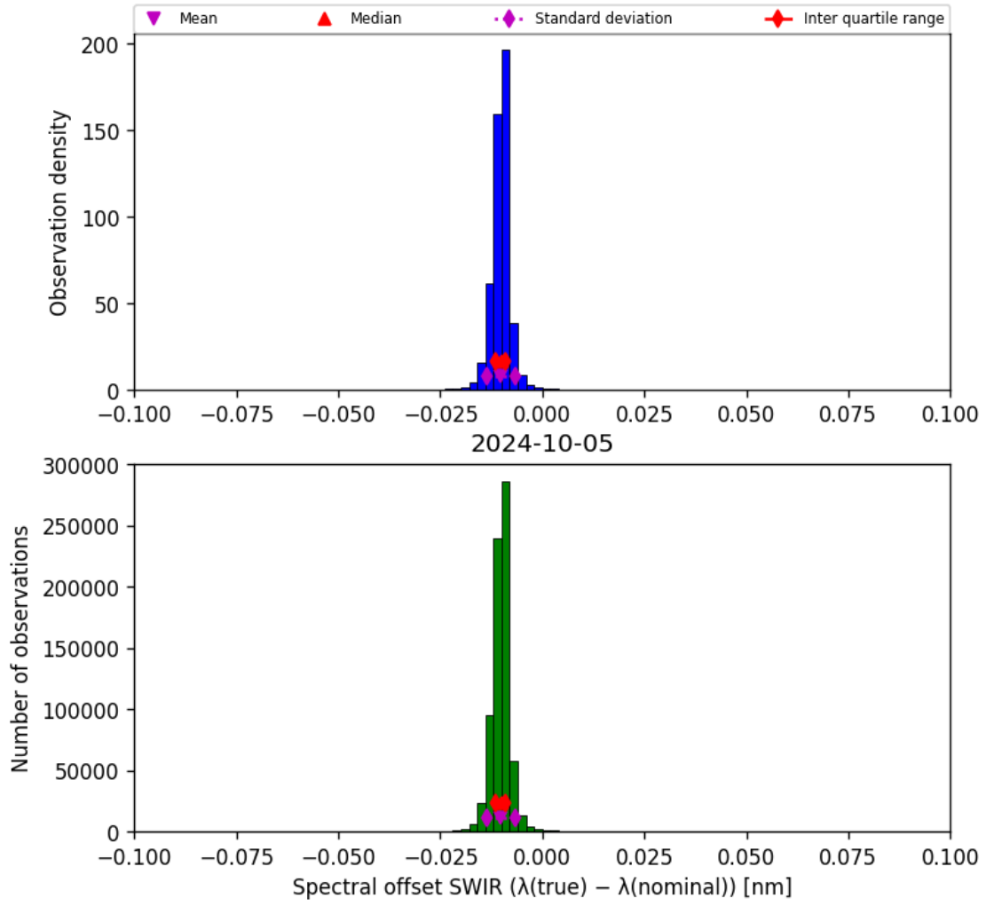
Figure 27: Histogram of “Spectral offset SWIR ( \lambda_{\text{true}} - \lambda_{\text{nominal}} )” for 2024-10-04 to 2024-10-06
