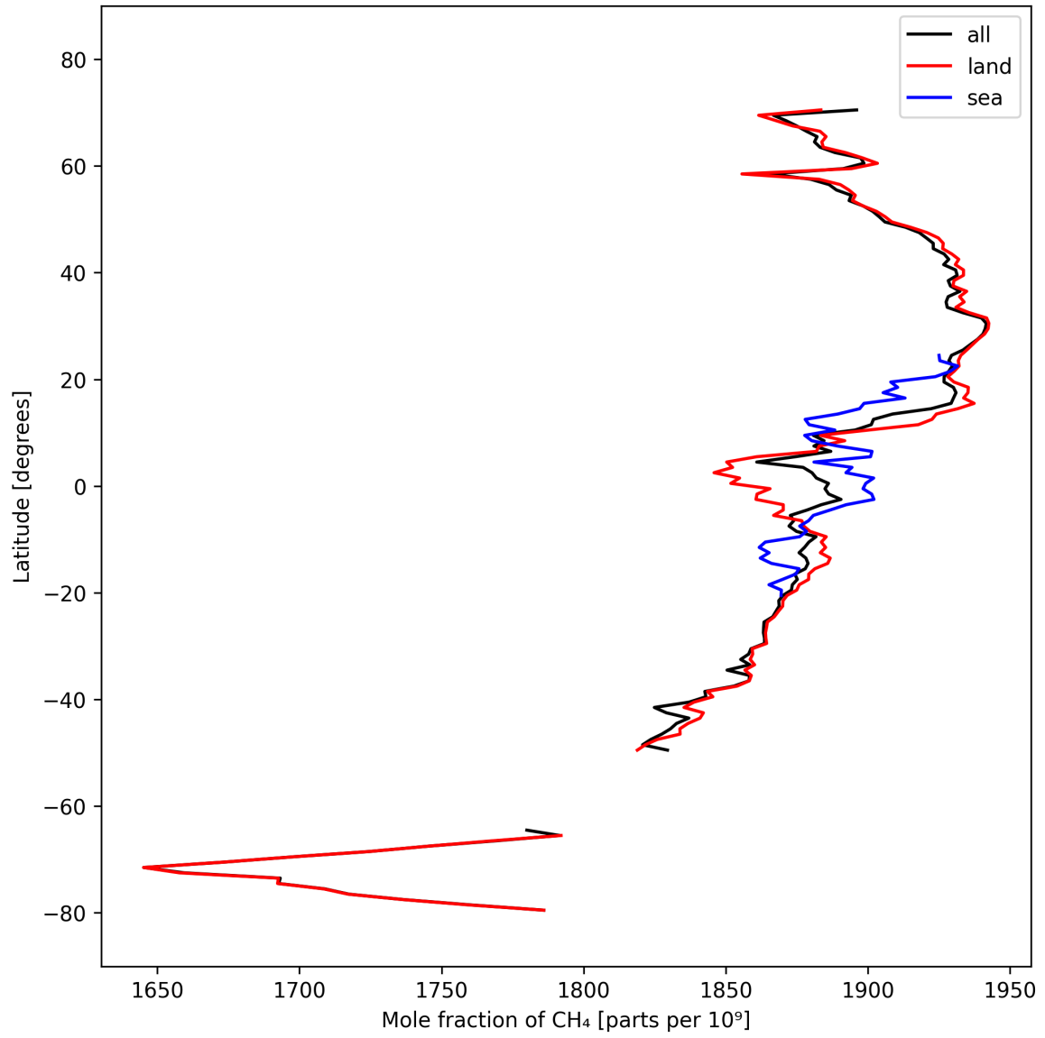
Figure 12: Zonal average of “Mole fraction of CH 4 ” for 2024-10-04 to 2024-10-06.
