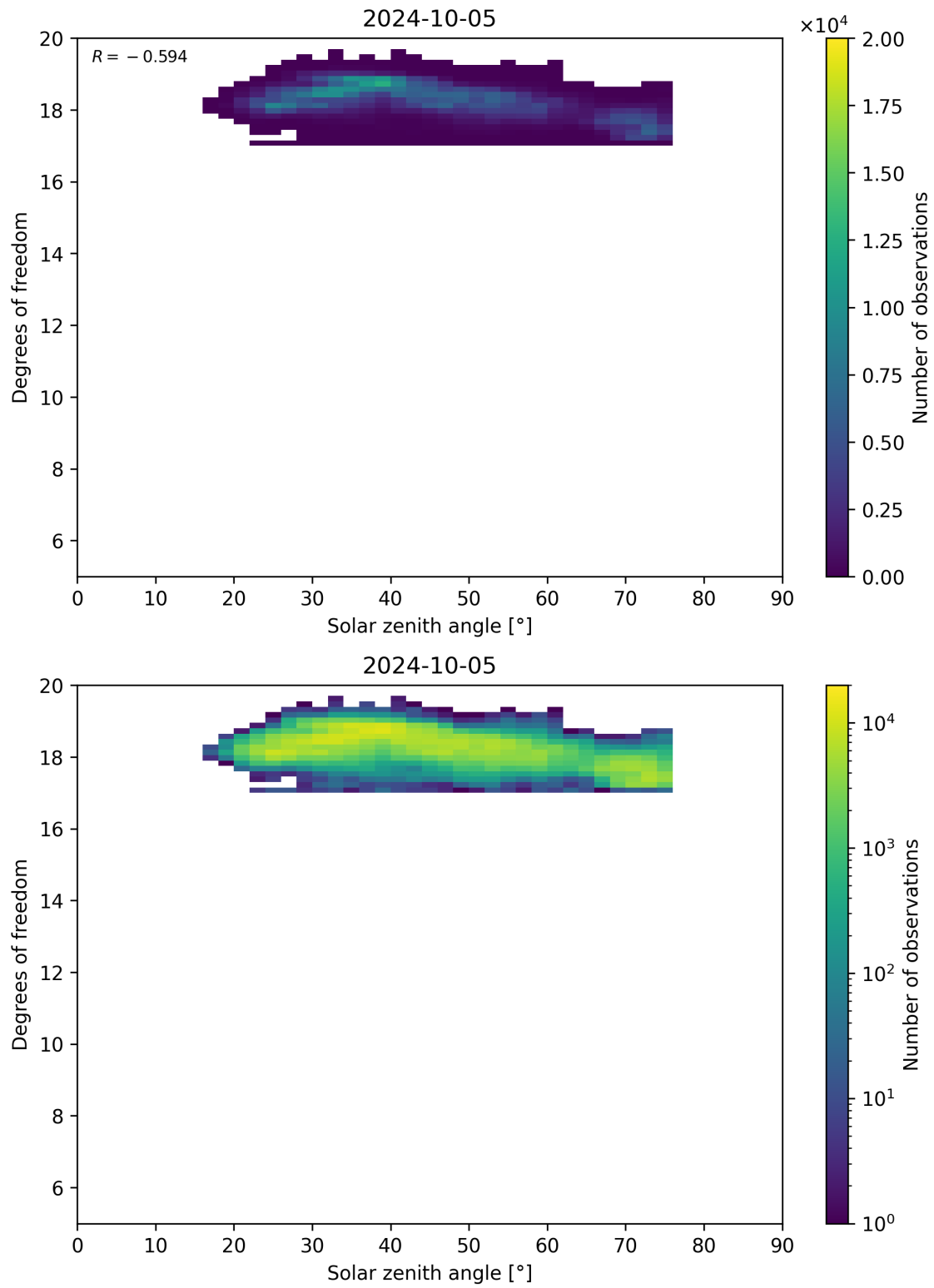
Figure 96: Scatter density plot of “Solar zenith angle” against “Degrees of freedom” for 2024-10-04 to 2024-10-06.
