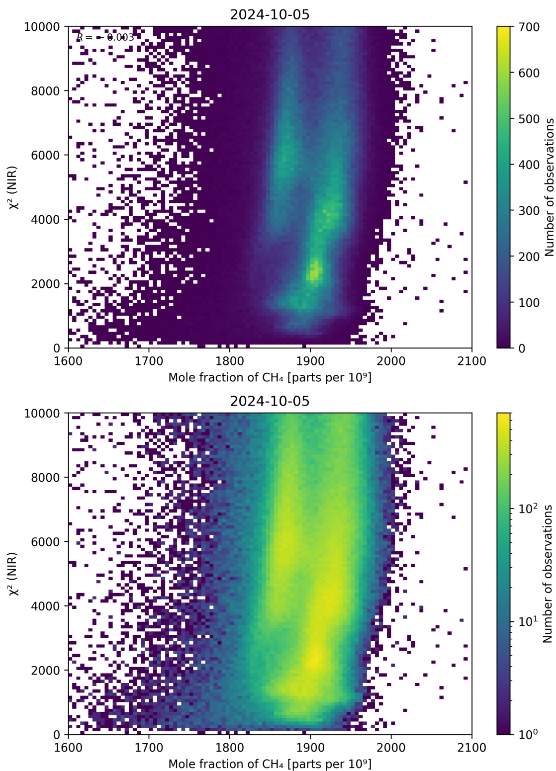
Figure 70: Scatter density plot of “Mole fraction of \text{CH}_4 ” against “ \chi^2 (NIR)” for 2024-10-04 to 2024-10-06.
