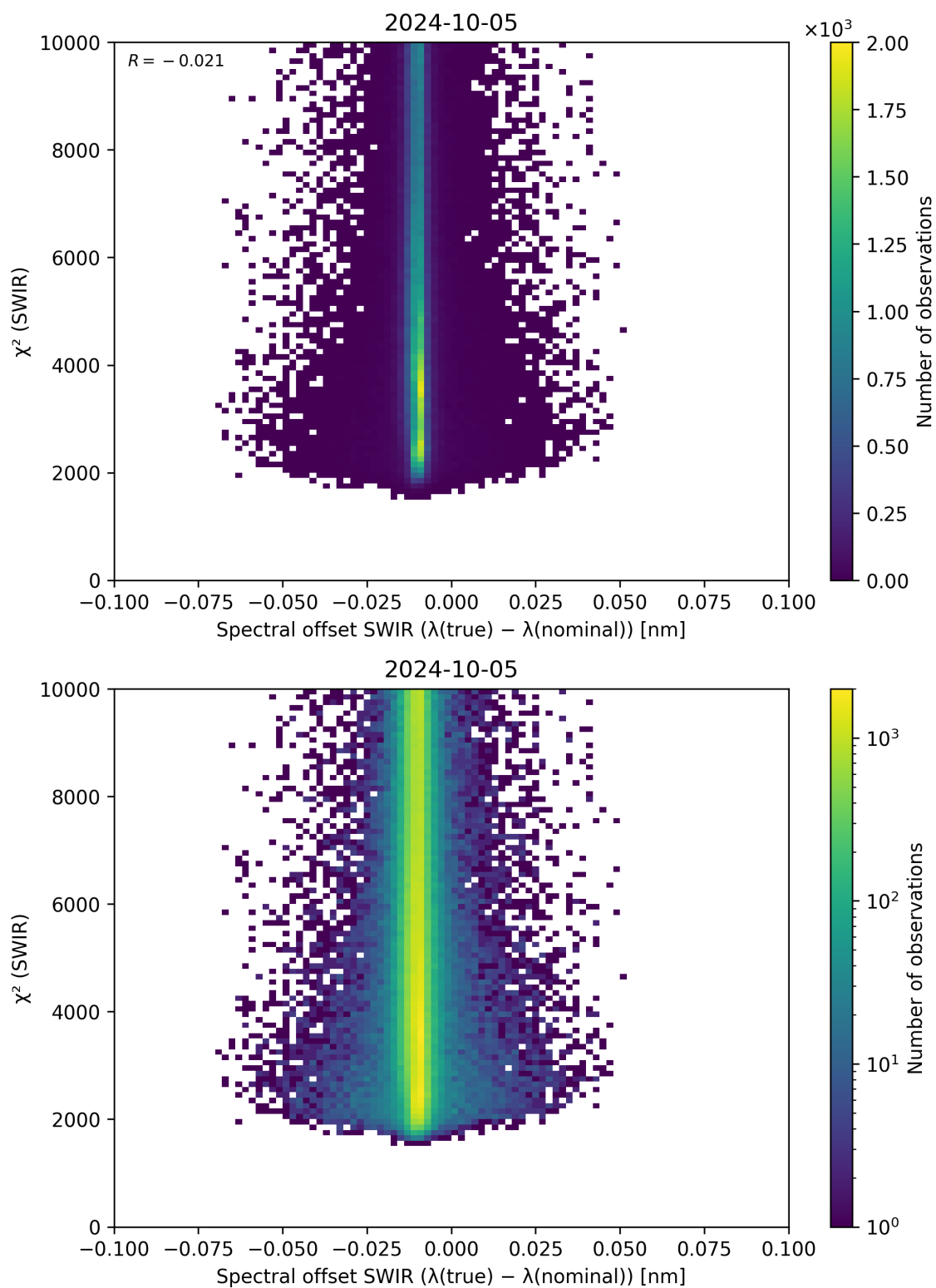
Figure 118: Scatter density plot of “Spectral offset SWIR ( \lambda_{\text{true}} - \lambda_{\text{nominal}} )” against “ \chi^2 (SWIR)” for 2024-10-04 to 2024-10-06.
