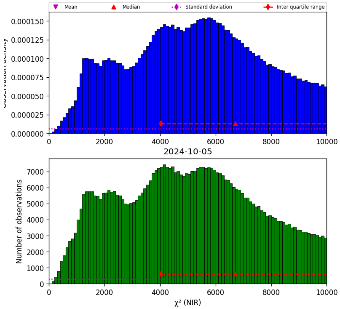
Figure 29: Histogram of “ \chi^2 (NIR)” for 2024-10-04 to 2024-10-06
