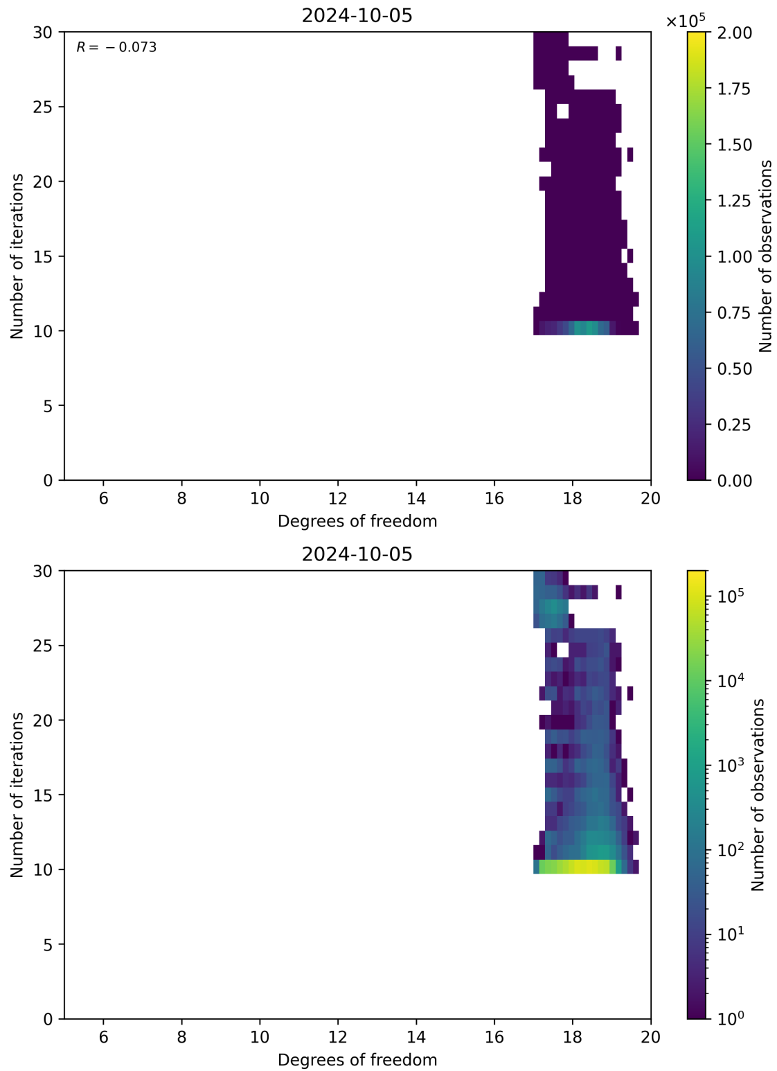
Figure 52: Scatter density plot of “Degrees of freedom” against “Number of iterations” for 2024-10-04 to 2024-10-06.
