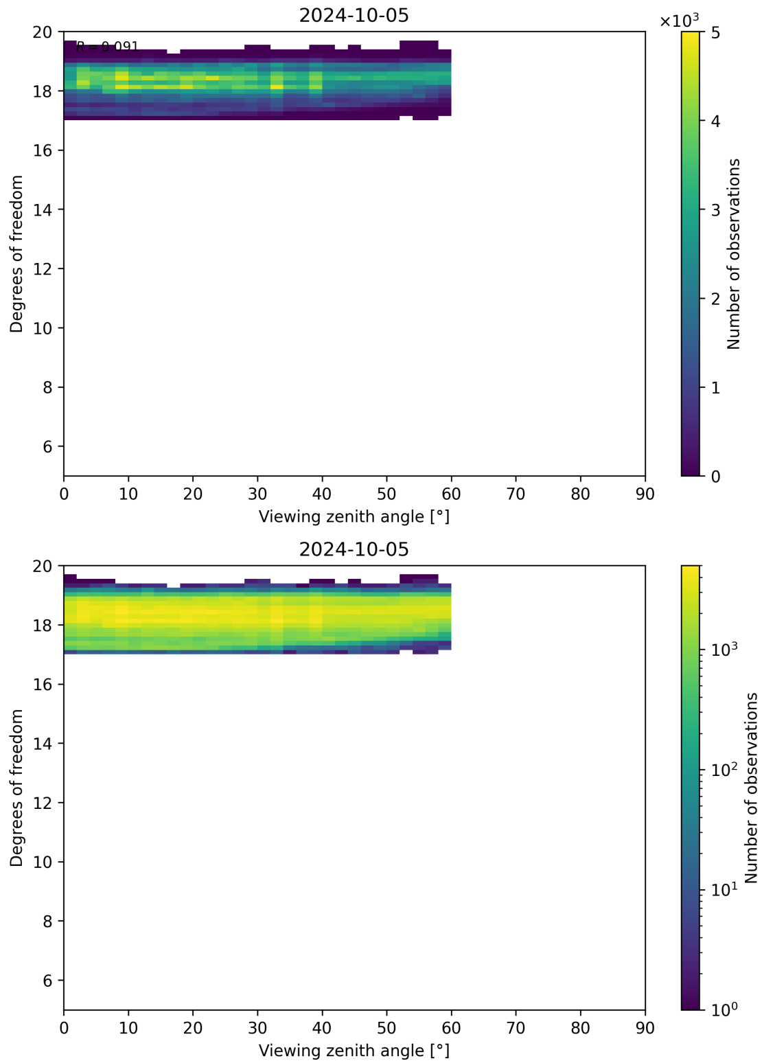
Figure 107: Scatter density plot of “Viewing zenith angle” against “Degrees of freedom” for 2024-10-04 to 2024-10-06.
