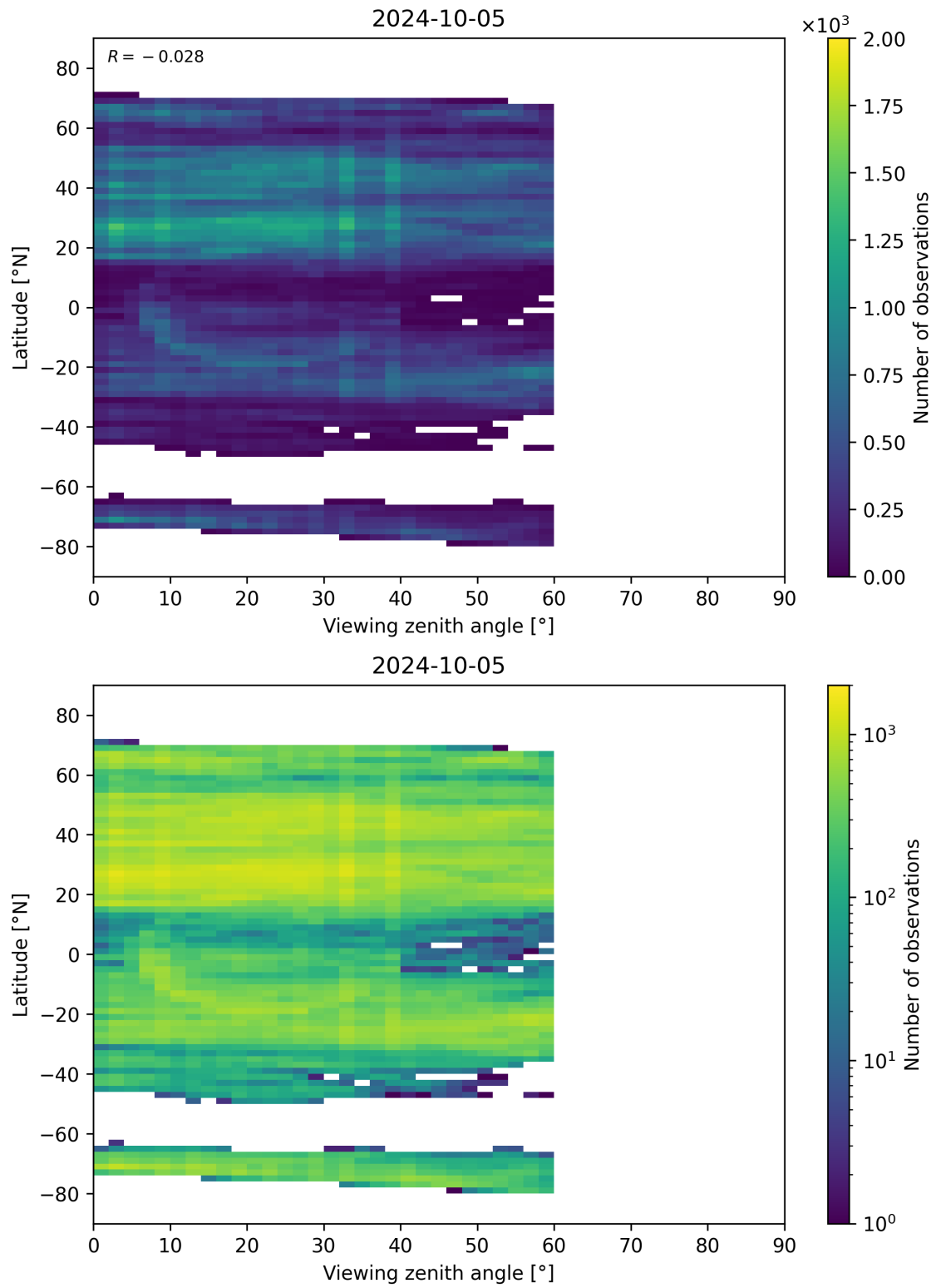
Figure 109: Scatter density plot of “Viewing zenith angle” against “Latitude” for 2024-10-04 to 2024-10-06.
