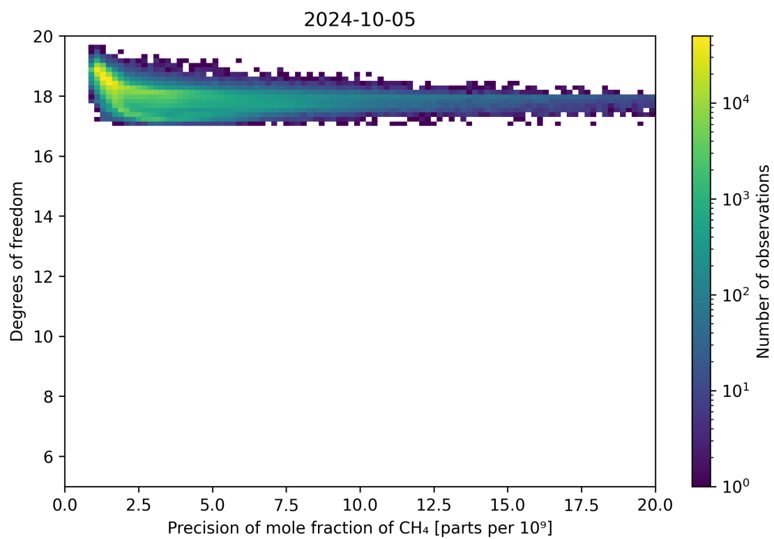
Figure 80: Scatter density plot of “Precision of mole fraction of CH 4 ” against “Degrees of freedom” for 2024-10-04 to 2024-10-06.
