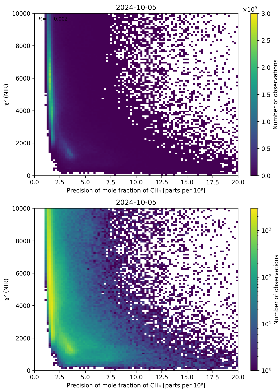
Figure 78: Scatter density plot of “Precision of mole fraction of CH 4 ” against “ \chi^2 (NIR)” for 2024-10-04 to 2024-10-06.
