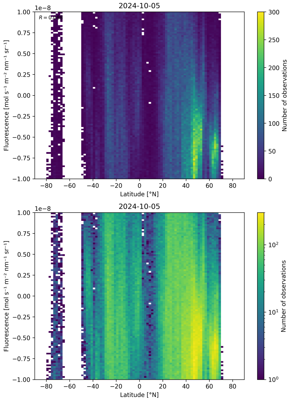
Figure 56: Scatter density plot of “Latitude” against “Fluorescence” for 2024-10-04 to 2024-10-06.
