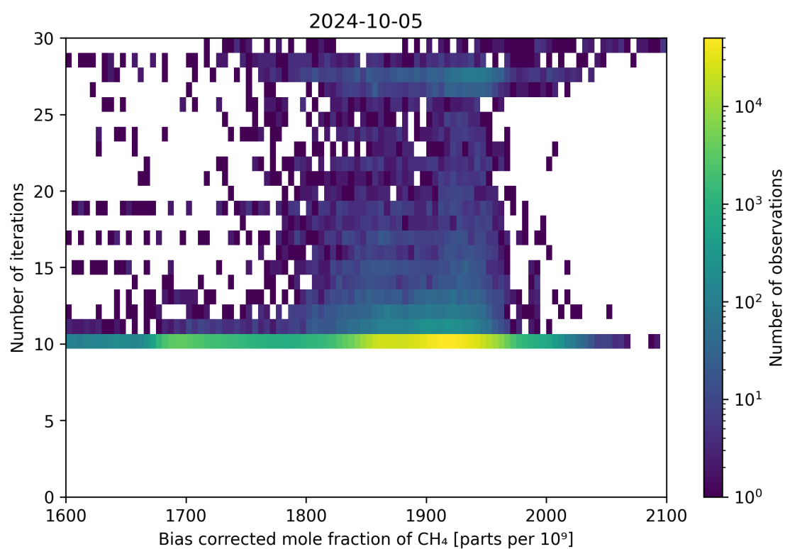
Figure 67: Scatter density plot of “Bias corrected mole fraction of CH 4 ” against “Number of iterations” for 2024-10-04 to 2024-10-06.
