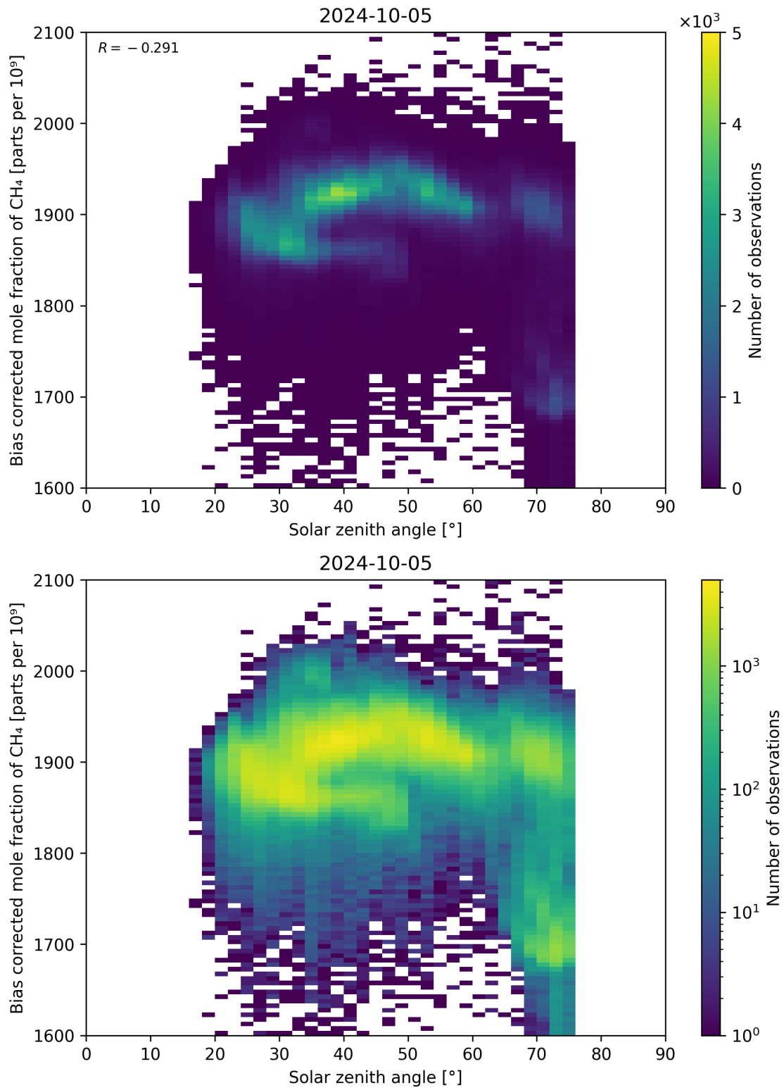
Figure 100: Scatter density plot of “Solar zenith angle” against “Bias corrected mole fraction of \text{CH}_4 ” for 2024-10-04 to 2024-10-06.
