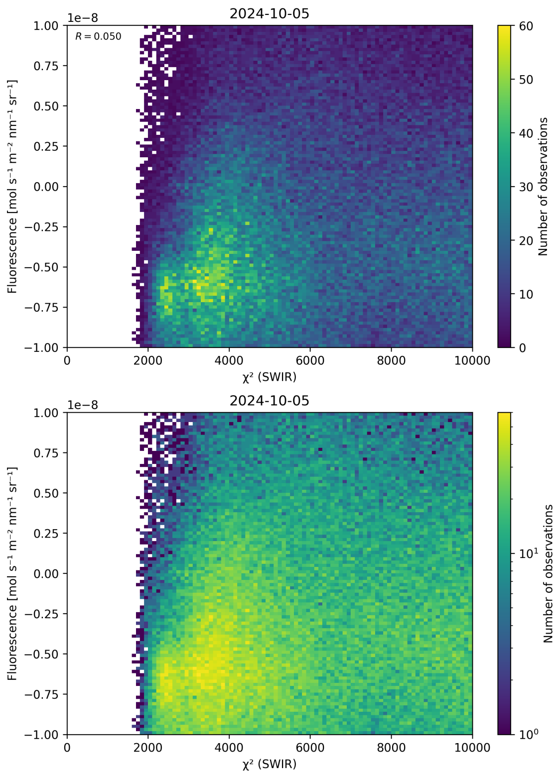
Figure 49: Scatter density plot of “ \chi^2 (SWIR)” against “Fluorescence” for 2024-10-04 to 2024-10-06.
