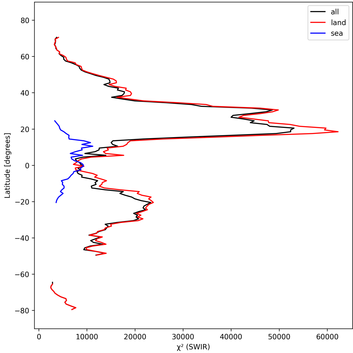
Figure 17: Zonal average of “ \chi^2 (SWIR)” for 2024-10-04 to 2024-10-06.
