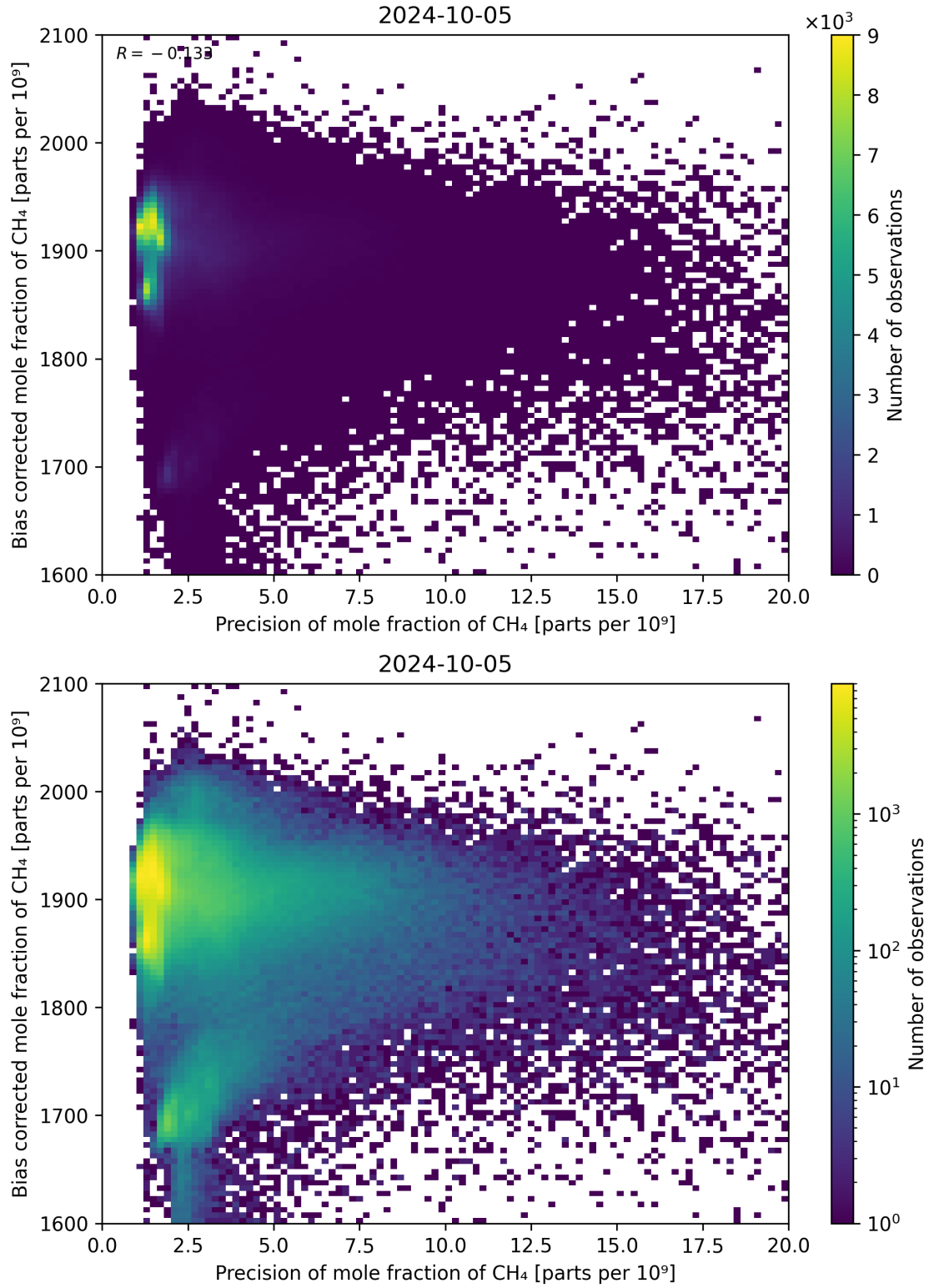
Figure 82: Scatter density plot of “Precision of mole fraction of CH 4 ” against “Bias corrected mole fraction of CH 4 ” for 2024-10-04 to 2024-10-06.
