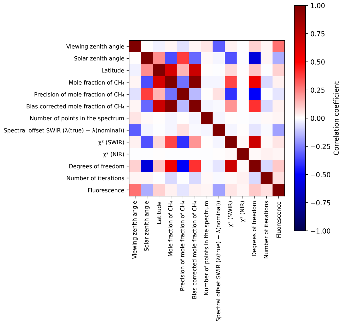
Figure 2: Map of correlation matrix for 2024-10-04 to 2024-10-06.
