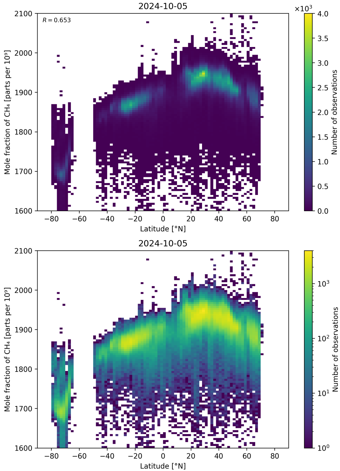
Figure 57: Scatter density plot of “Latitude” against “Mole fraction of \text{CH}_4 ” for 2024-10-04 to 2024-10-06.
