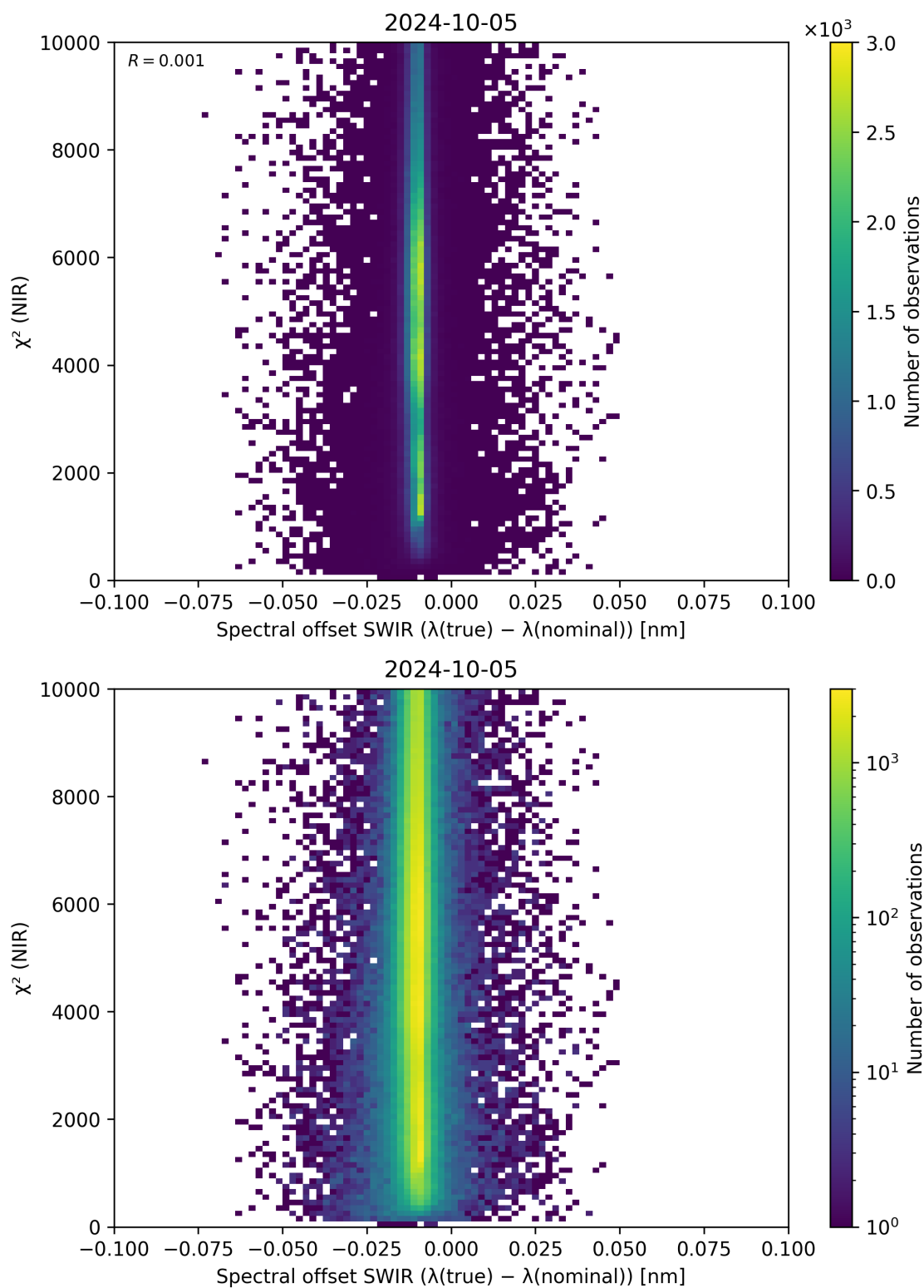
Figure 117: Scatter density plot of “Spectral offset SWIR ( \lambda_{\text{true}} - \lambda_{\text{nominal}} )” against “ \chi^2 (NIR)” for 2024-10-04 to 2024-10-06.
