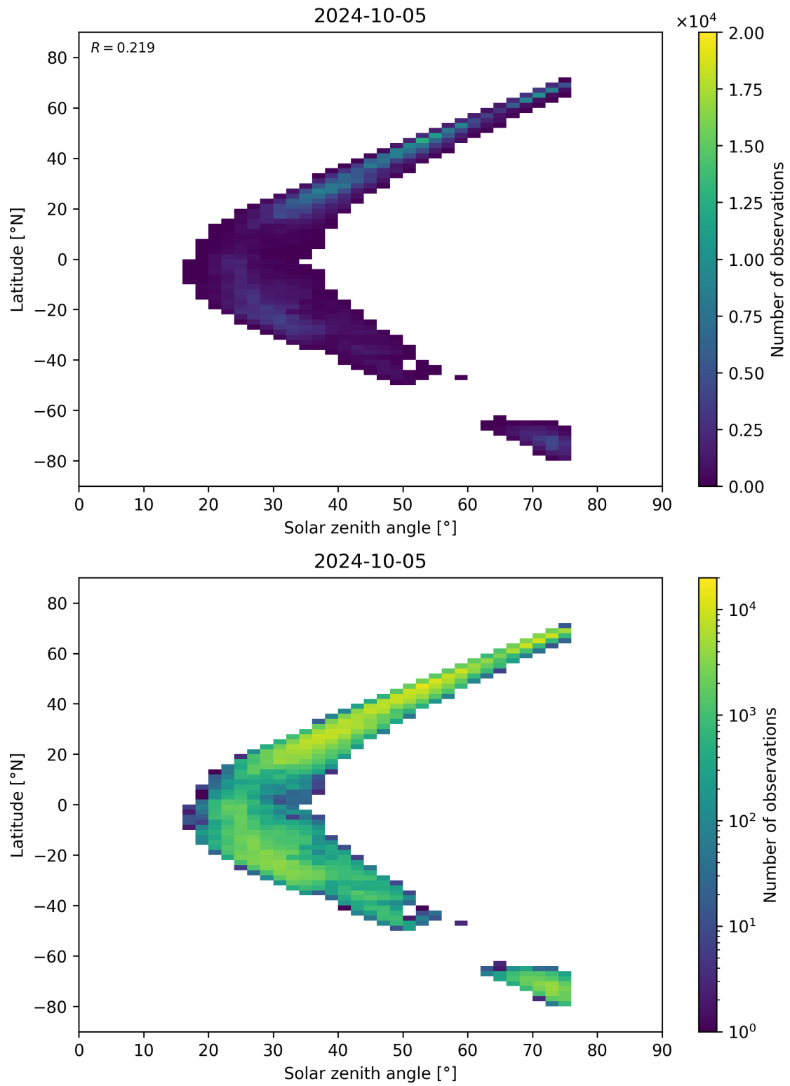
Figure 98: Scatter density plot of “Solar zenith angle” against “Latitude” for 2024-10-04 to 2024-10-06.
