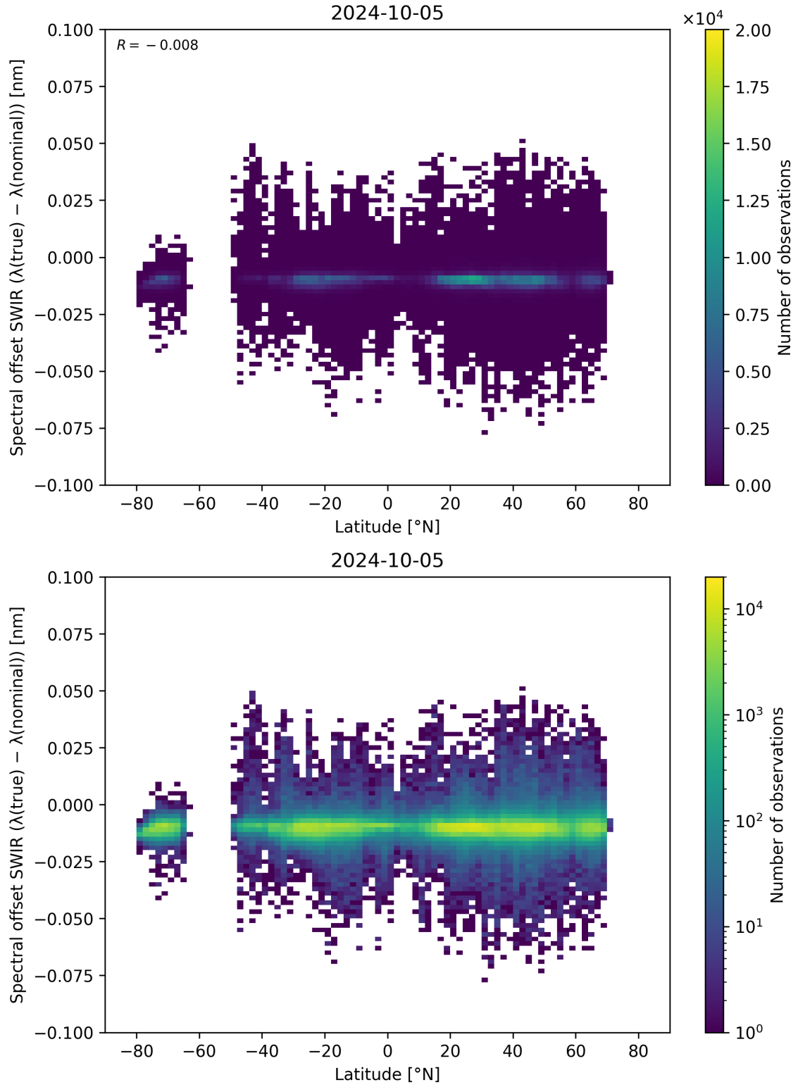
Figure 62: Scatter density plot of “Latitude” against “Spectral offset SWIR ( \lambda_{\text{true}} - \lambda_{\text{nominal}} )” for 2024-10-04 to 2024-10-06.
