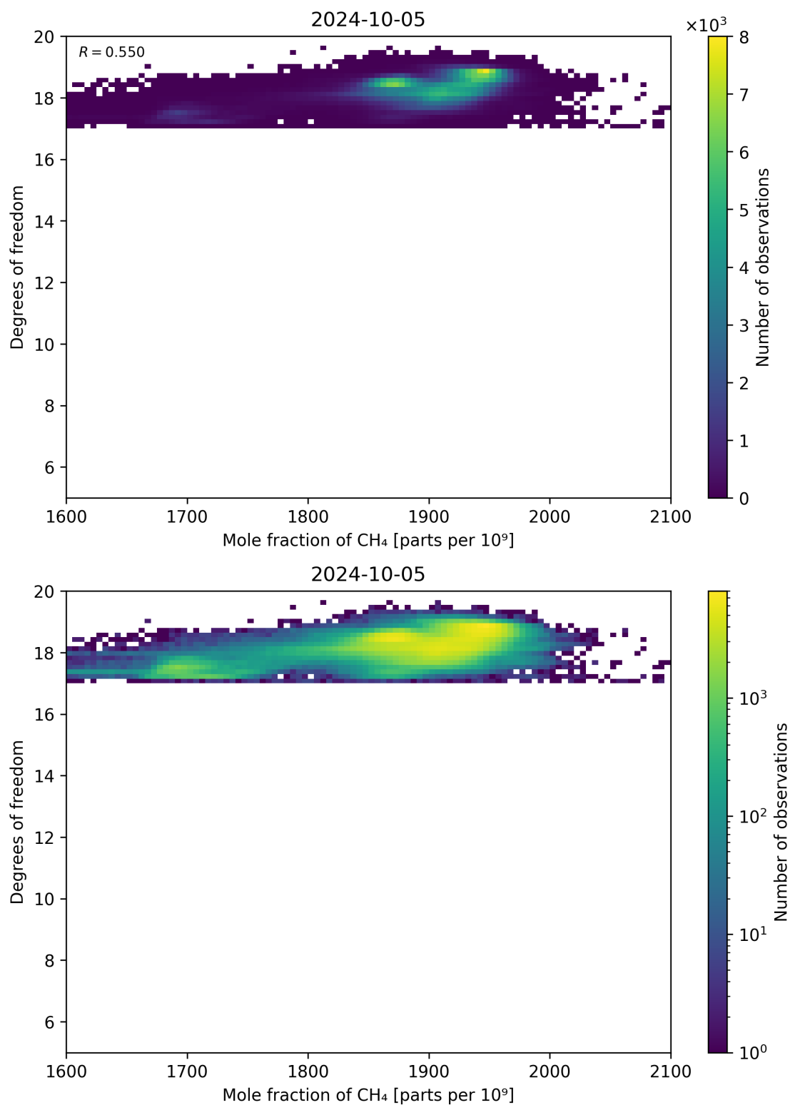
Figure 72: Scatter density plot of “Mole fraction of CH 4 ” against “Degrees of freedom” for 2024-10-04 to 2024-10-06.
