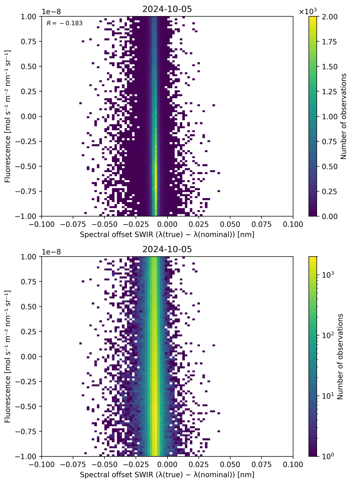
Figure 120: Scatter density plot of “Spectral offset SWIR ( \lambda_{\text{true}} - \lambda_{\text{nominal}} )” against “Fluorescence” for 2024-10-04 to 2024-10-06.
