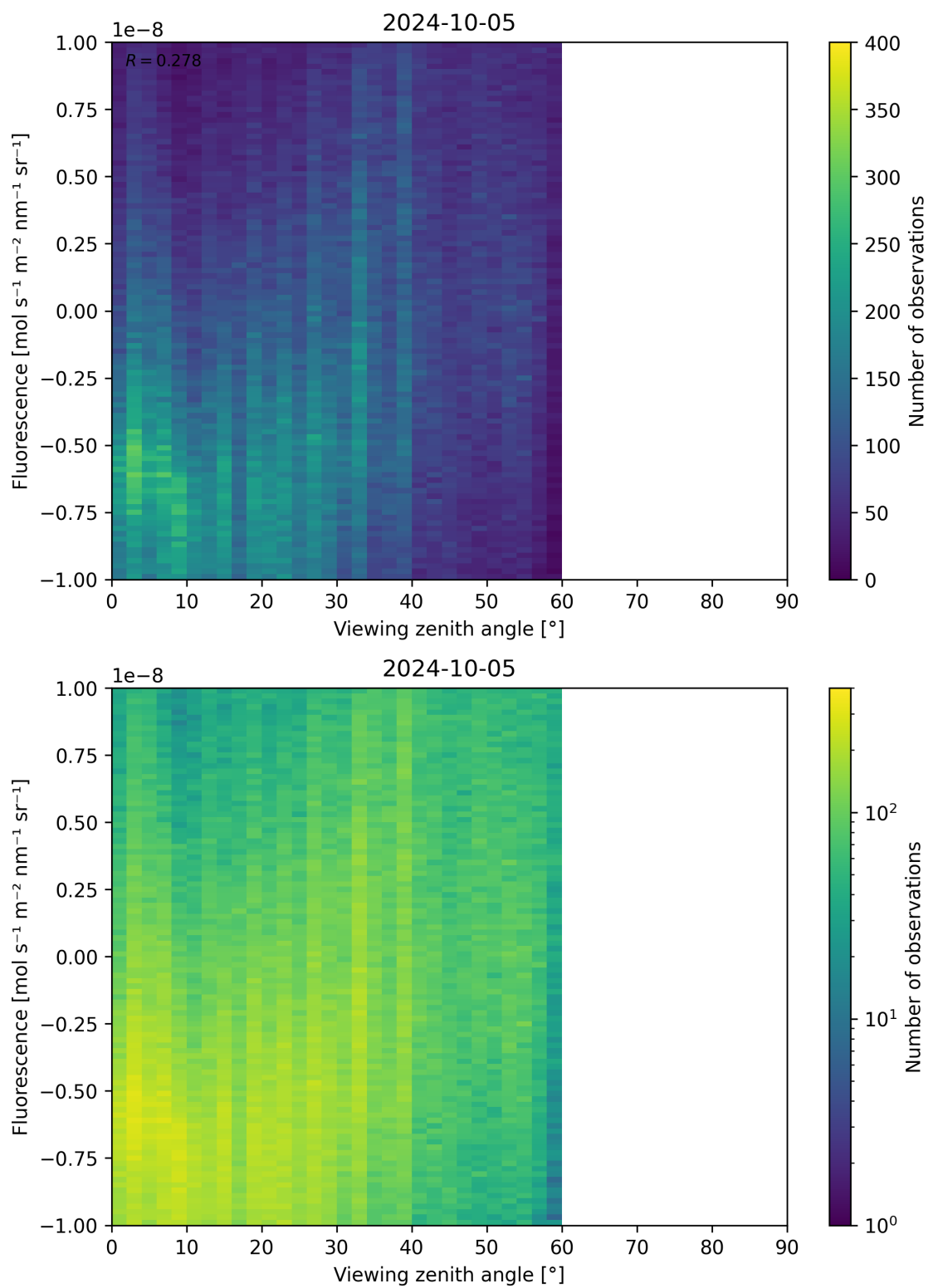
Figure 108: Scatter density plot of “Viewing zenith angle” against “Fluorescence” for 2024-10-04 to 2024-10-06.
