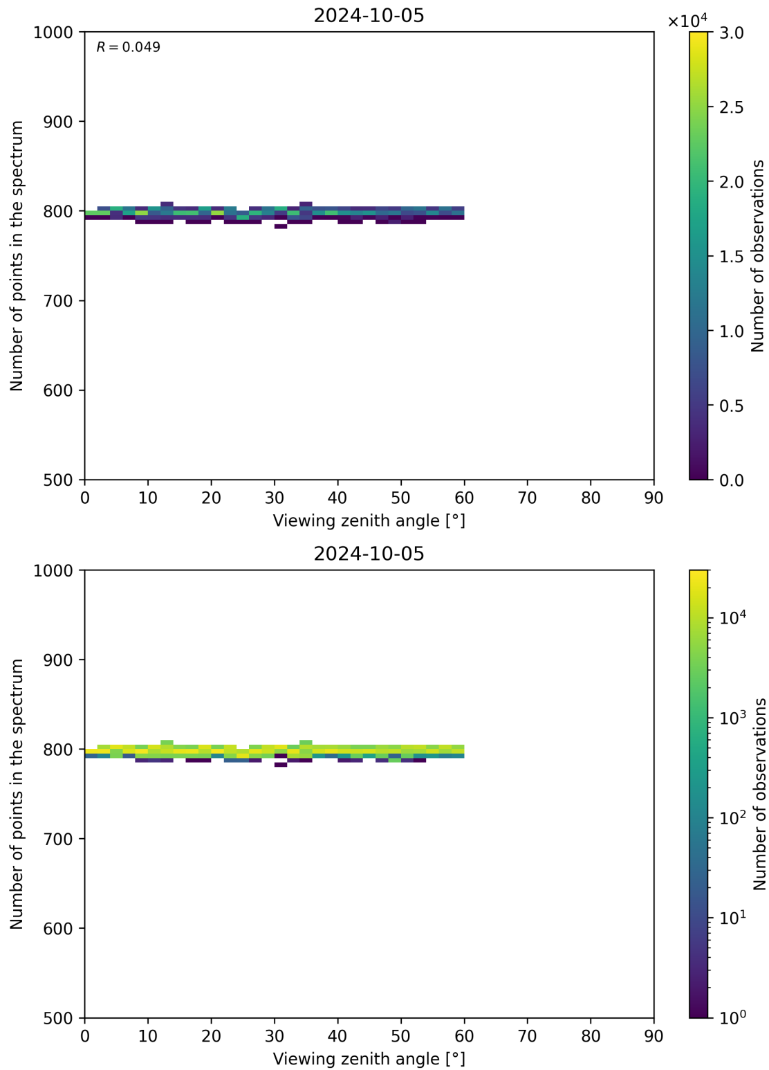
Figure 114: Scatter density plot of “Viewing zenith angle” against “Number of points in the spectrum” for 2024-10-04 to 2024-10-06.
