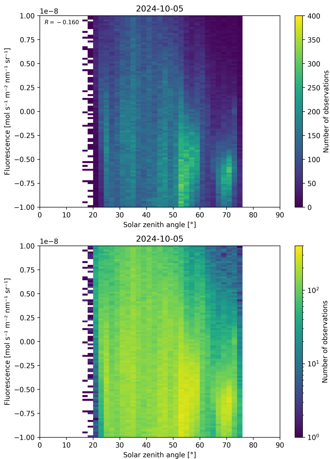
Figure 97: Scatter density plot of “Solar zenith angle” against “Fluorescence” for 2024-10-04 to 2024-10-06.
