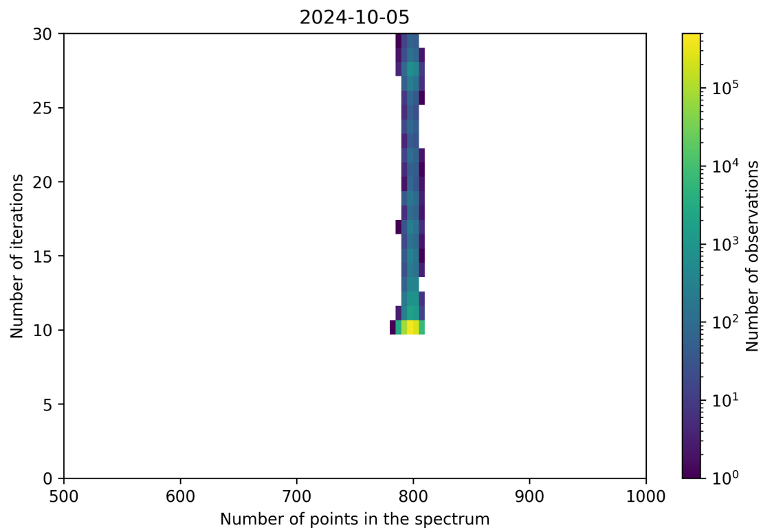
Figure 92: Scatter density plot of “Number of points in the spectrum” against “Number of iterations” for 2024-10-04 to 2024-10-06.
