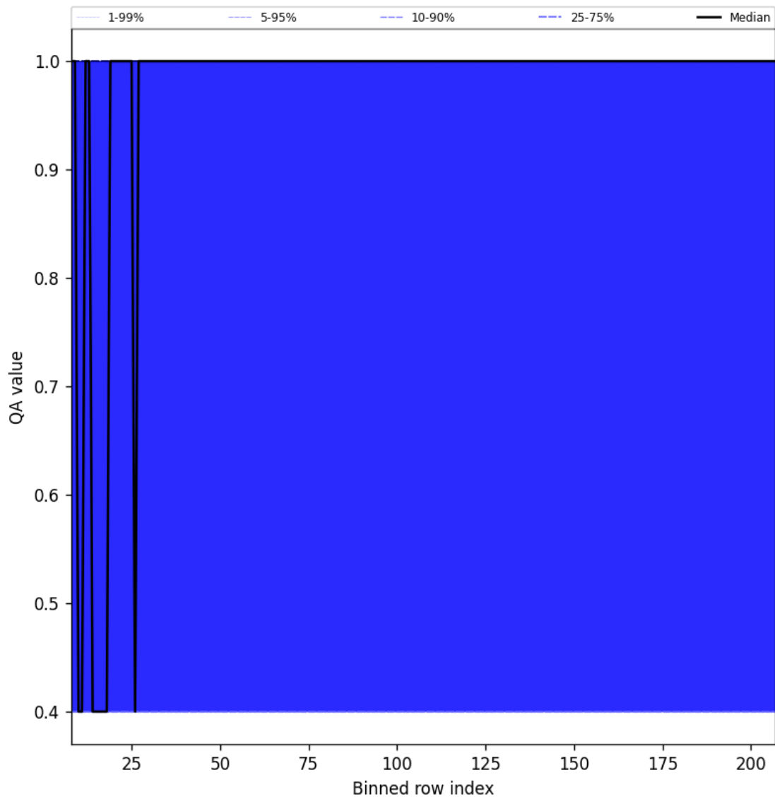
Figure 33: Along track statistics of “QA value” for 2024-10-04 to 2024-10-06
