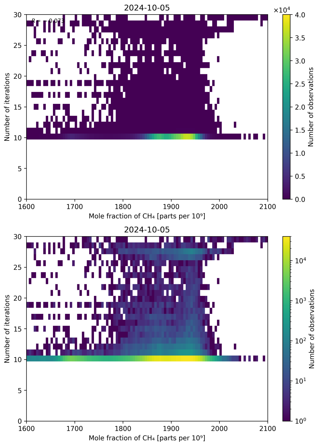
Figure 76: Scatter density plot of “Mole fraction of CH 4 ” against “Number of iterations” for 2024-10-04 to 2024-10-06.
