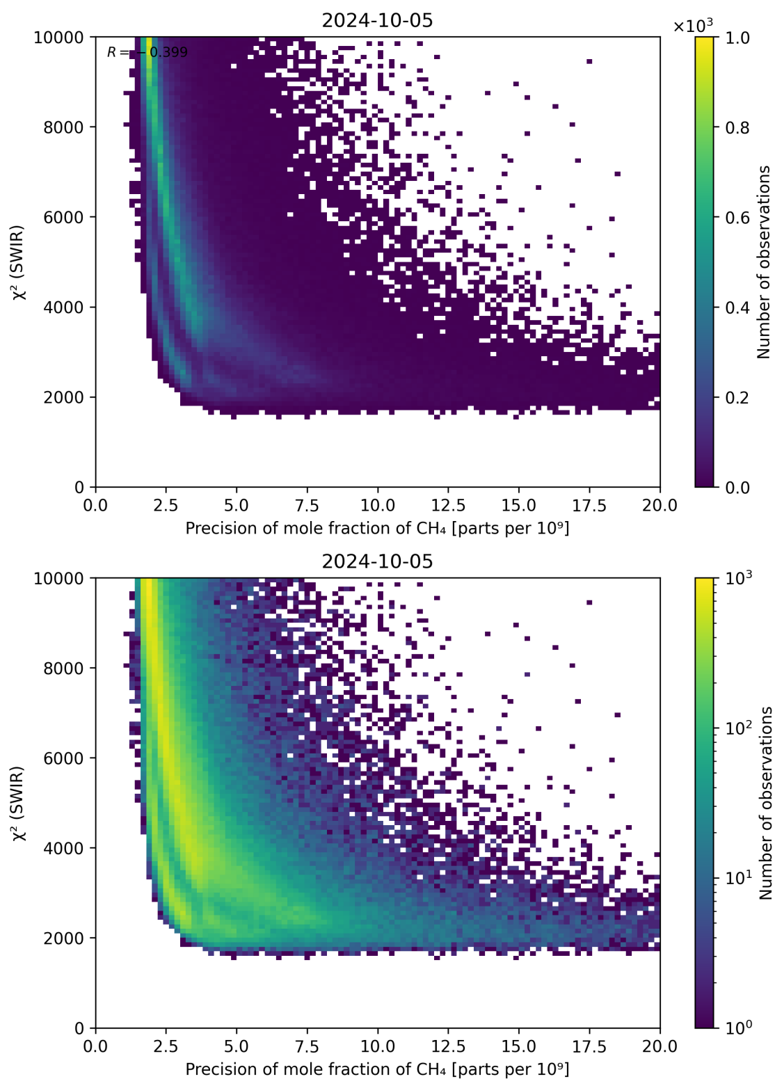
Figure 79: Scatter density plot of “Precision of mole fraction of \text{CH}_4 ” against “ \chi^2 (SWIR)” for 2024-10-04 to 2024-10-06.
