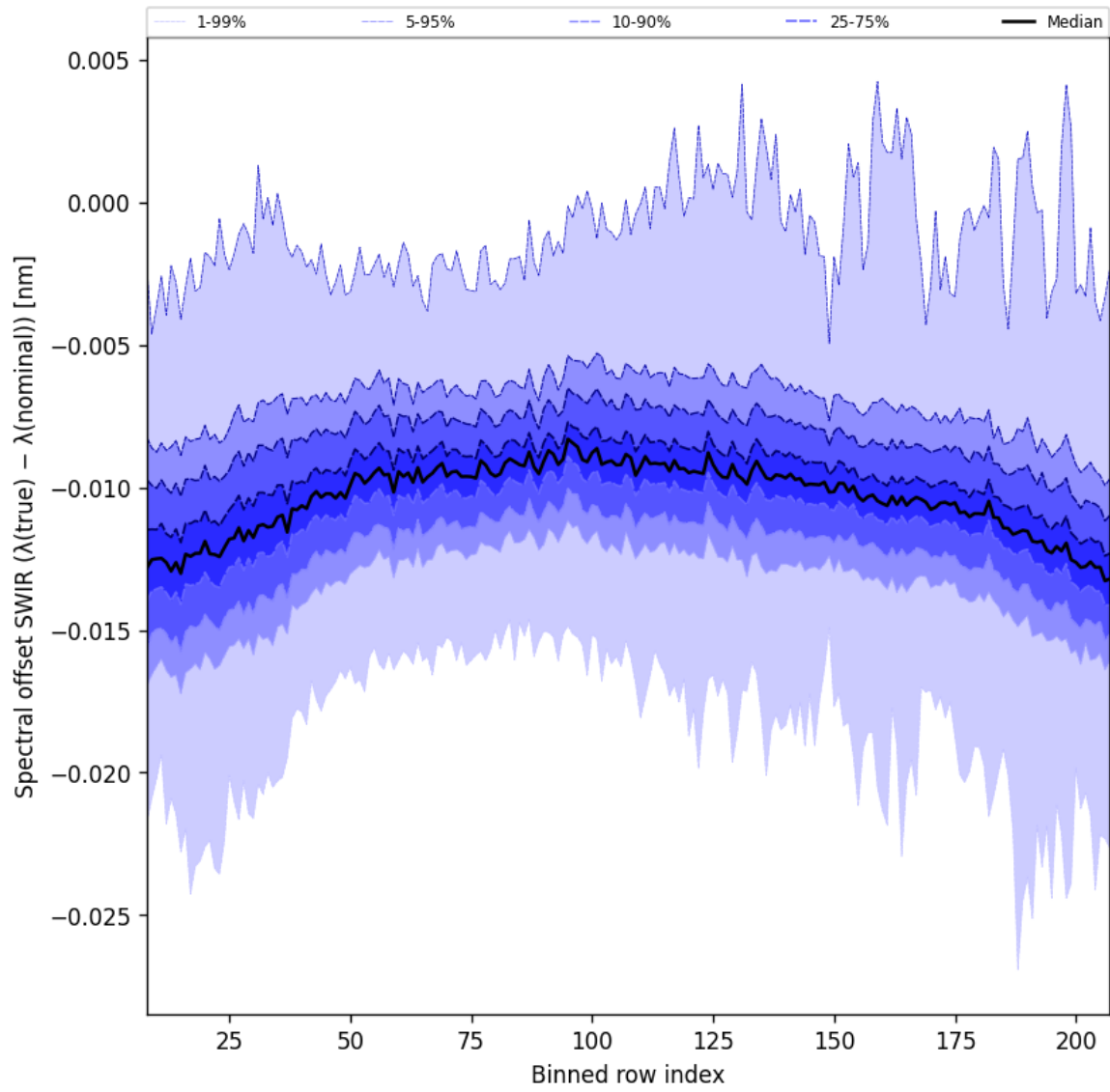
Figure 38: Along track statistics of “Spectral offset SWIR ( \lambda_{\text{true}} - \lambda_{\text{nominal}} )” for 2024-10-04 to 2024-10-06
