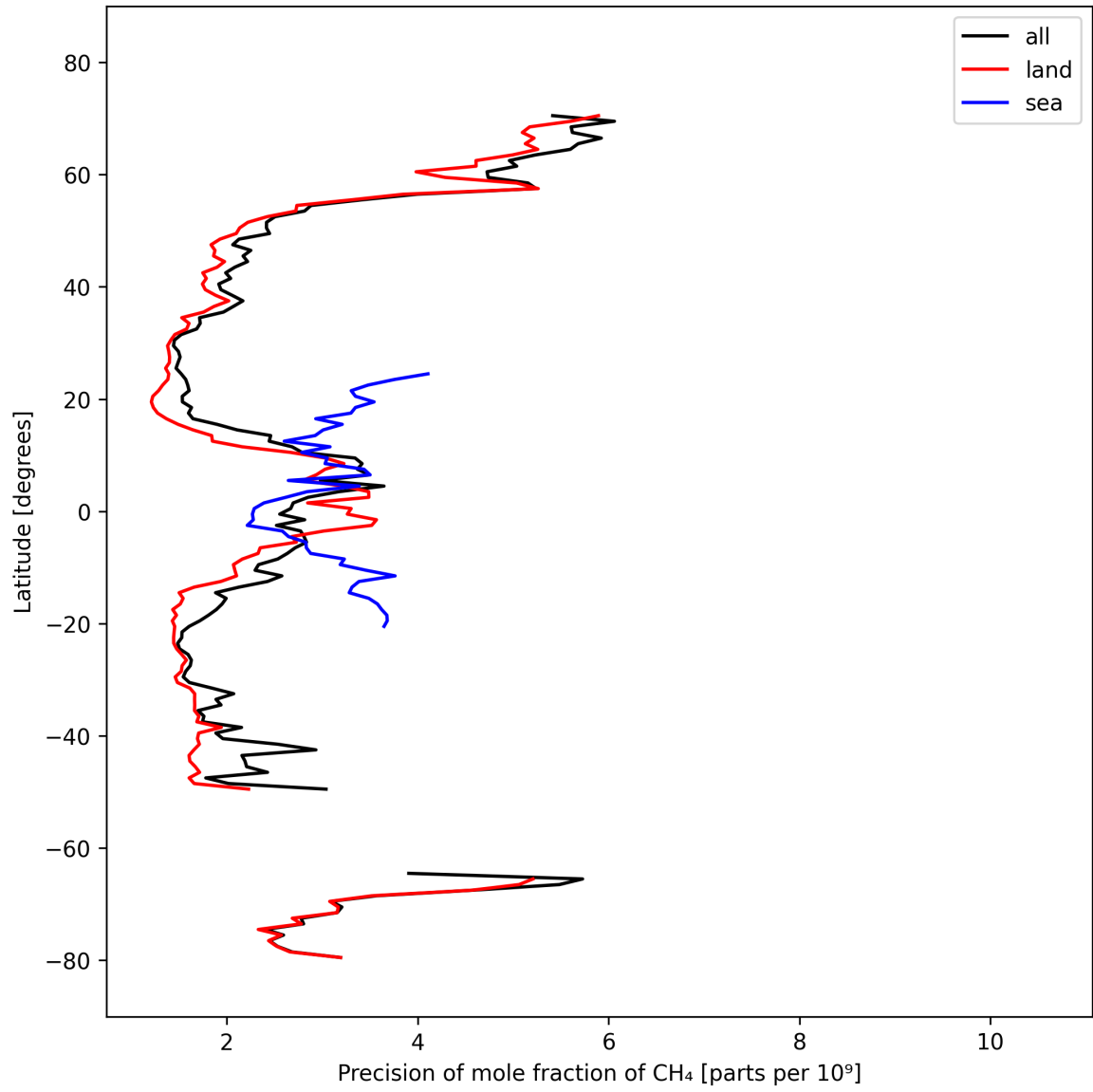
Figure 13: Zonal average of “Precision of mole fraction of CH 4 ” for 2024-10-04 to 2024-10-06.
