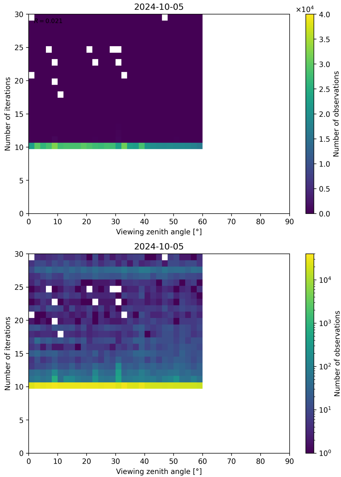
Figure 113: Scatter density plot of “Viewing zenith angle” against “Number of iterations” for 2024-10-04 to 2024-10-06.
