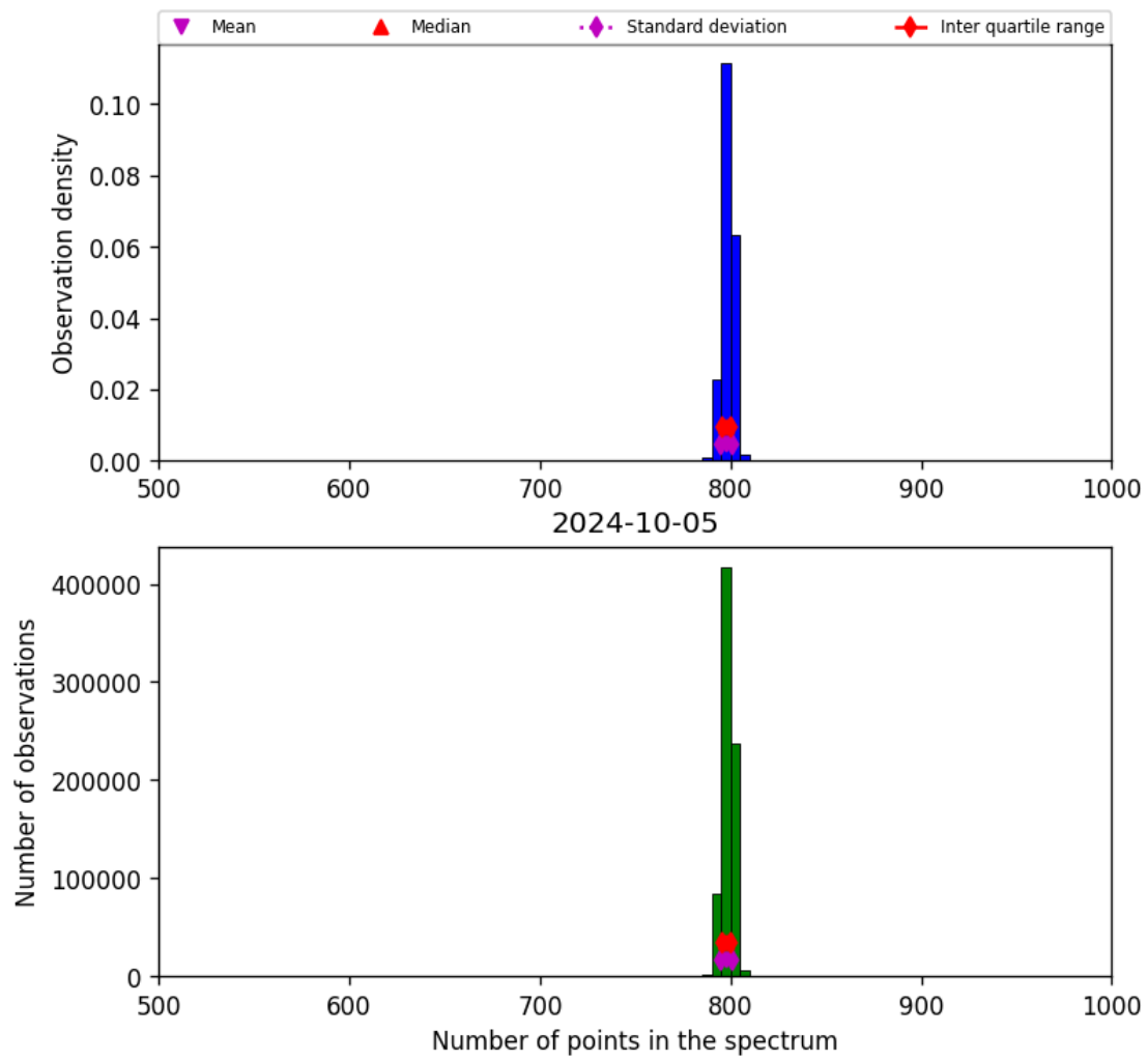
Figure 26: Histogram of “Number of points in the spectrum” for 2024-10-04 to 2024-10-06
