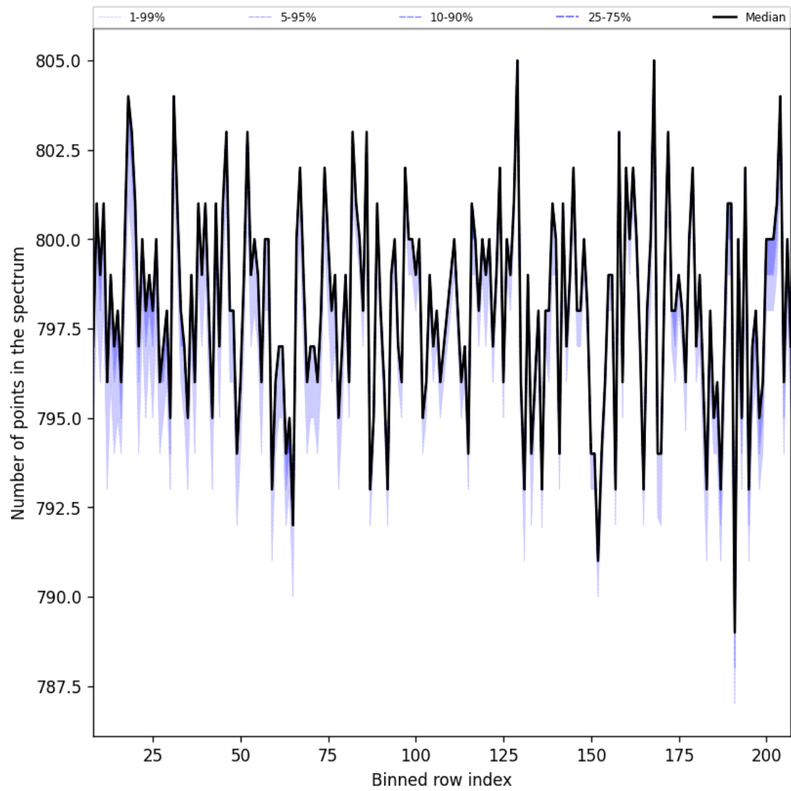
Figure 37: Along track statistics of “Number of points in the spectrum” for 2024-10-04 to 2024-10-06
