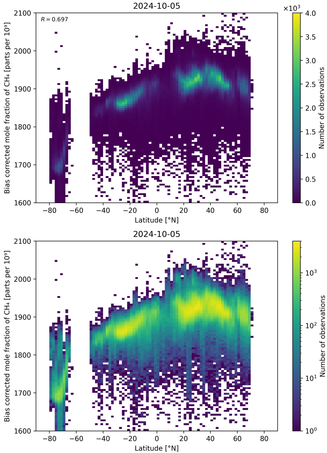
Figure 58: Scatter density plot of “Latitude” against “Bias corrected mole fraction of CH 4 ” for 2024-10-04 to 2024-10-06.
