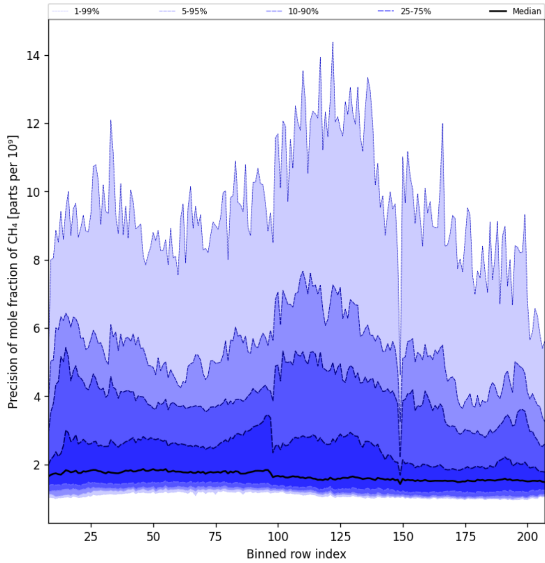
Figure 35: Along track statistics of “Precision of mole fraction of CH 4 ” for 2024-10-04 to 2024-10-06
