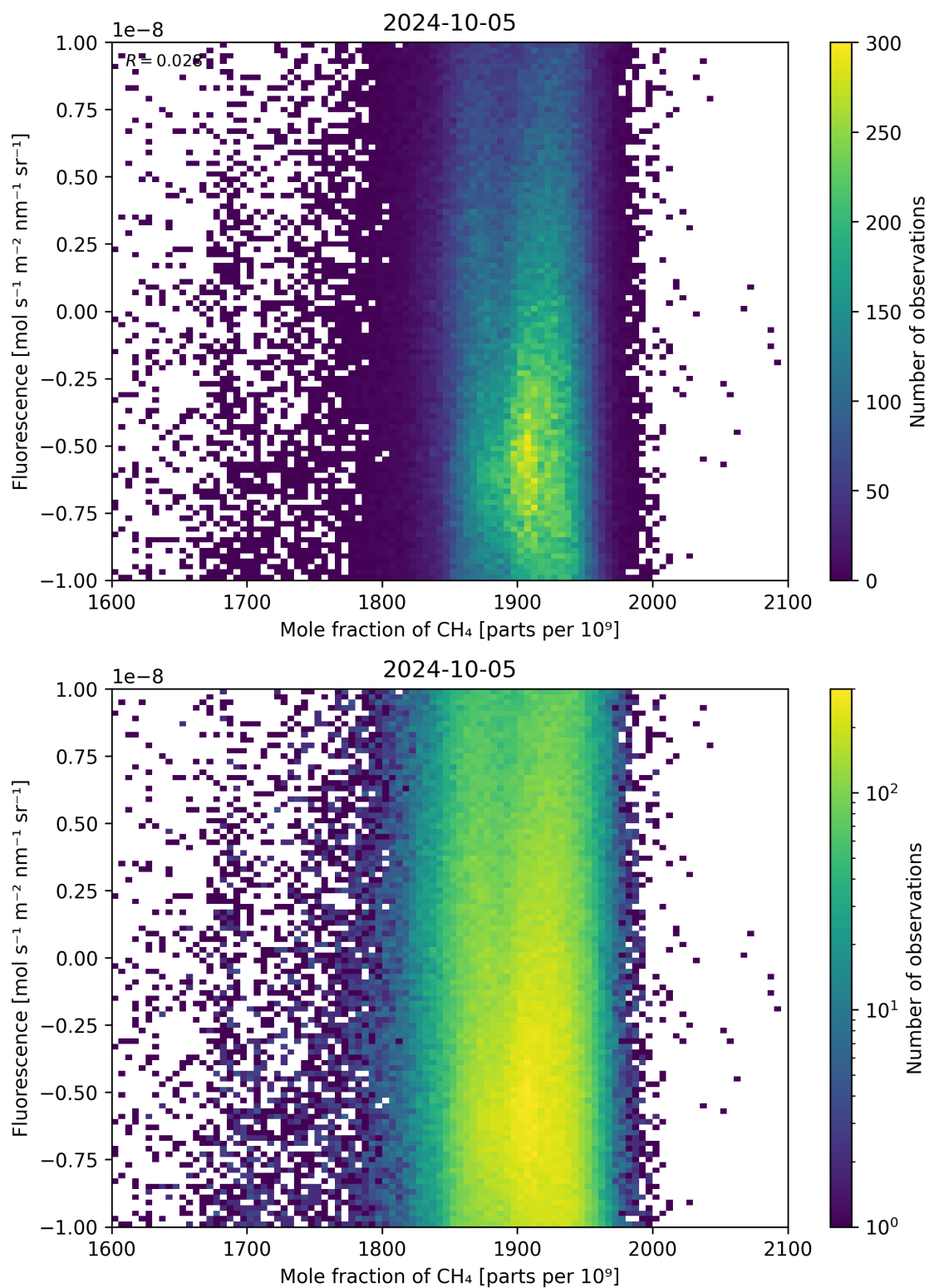
Figure 73: Scatter density plot of “Mole fraction of \text{CH}_4 ” against “Fluorescence” for 2024-10-04 to 2024-10-06.
