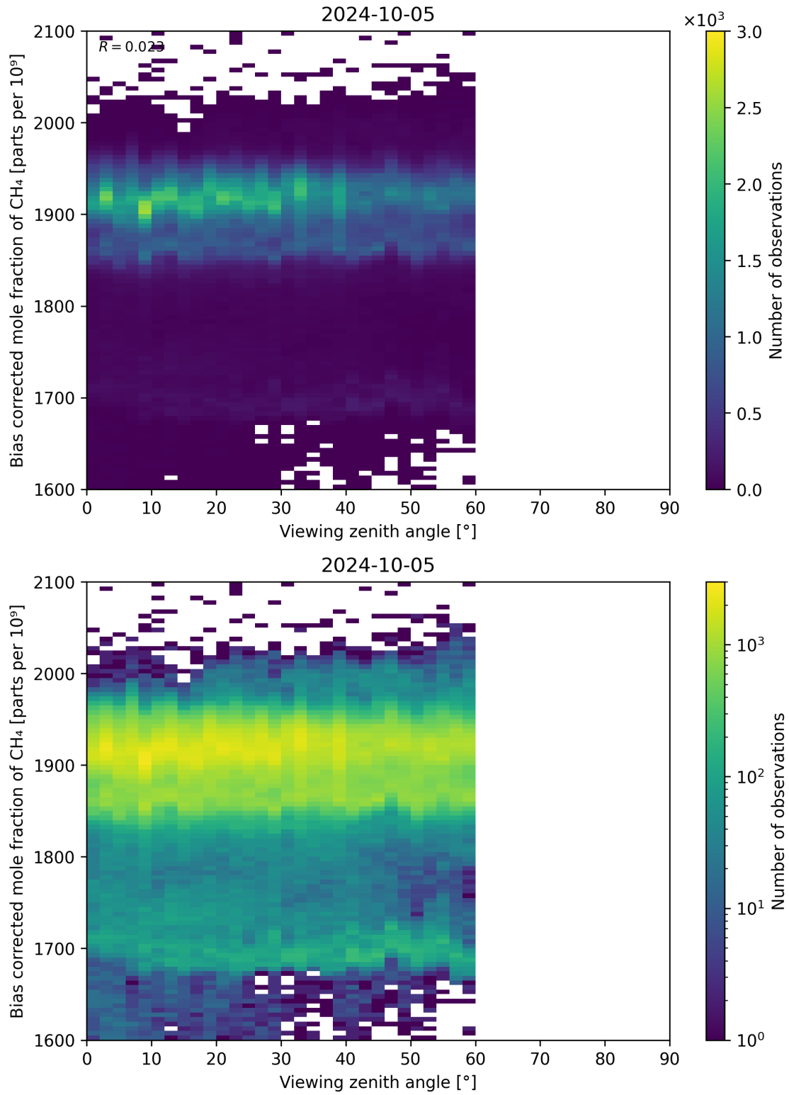
Figure 111: Scatter density plot of “Viewing zenith angle” against “Bias corrected mole fraction of CH 4 ” for 2024-10-04 to 2024-10-06.
