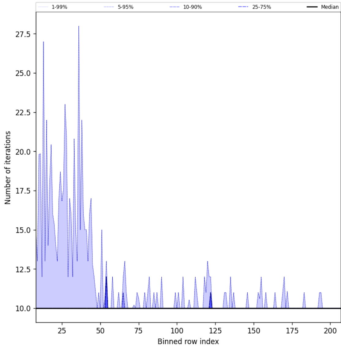
Figure 42: Along track statistics of “Number of iterations” for 2024-10-04 to 2024-10-06
