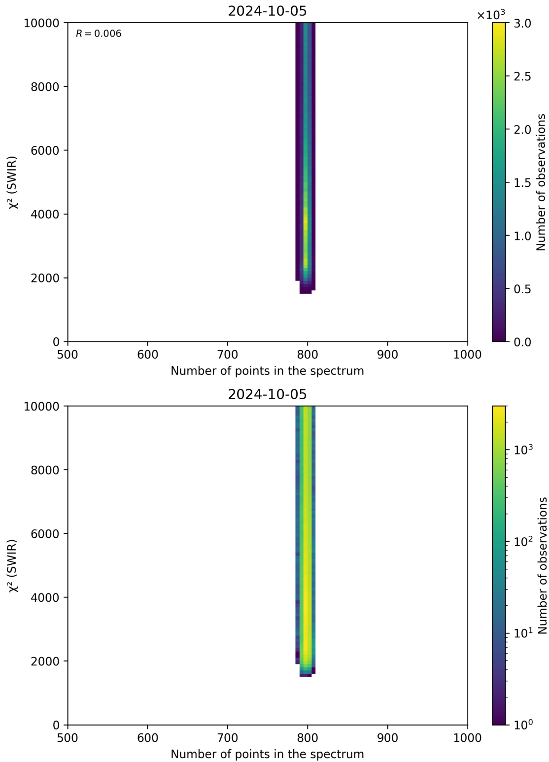
Figure 89: Scatter density plot of “Number of points in the spectrum” against “ \chi^2 (SWIR)” for 2024-10-04 to 2024-10-06.
