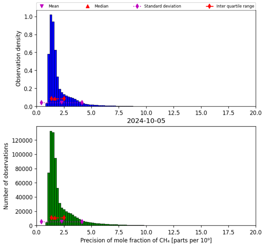
Figure 24: Histogram of “Precision of mole fraction of CH 4 ” for 2024-10-04 to 2024-10-06
