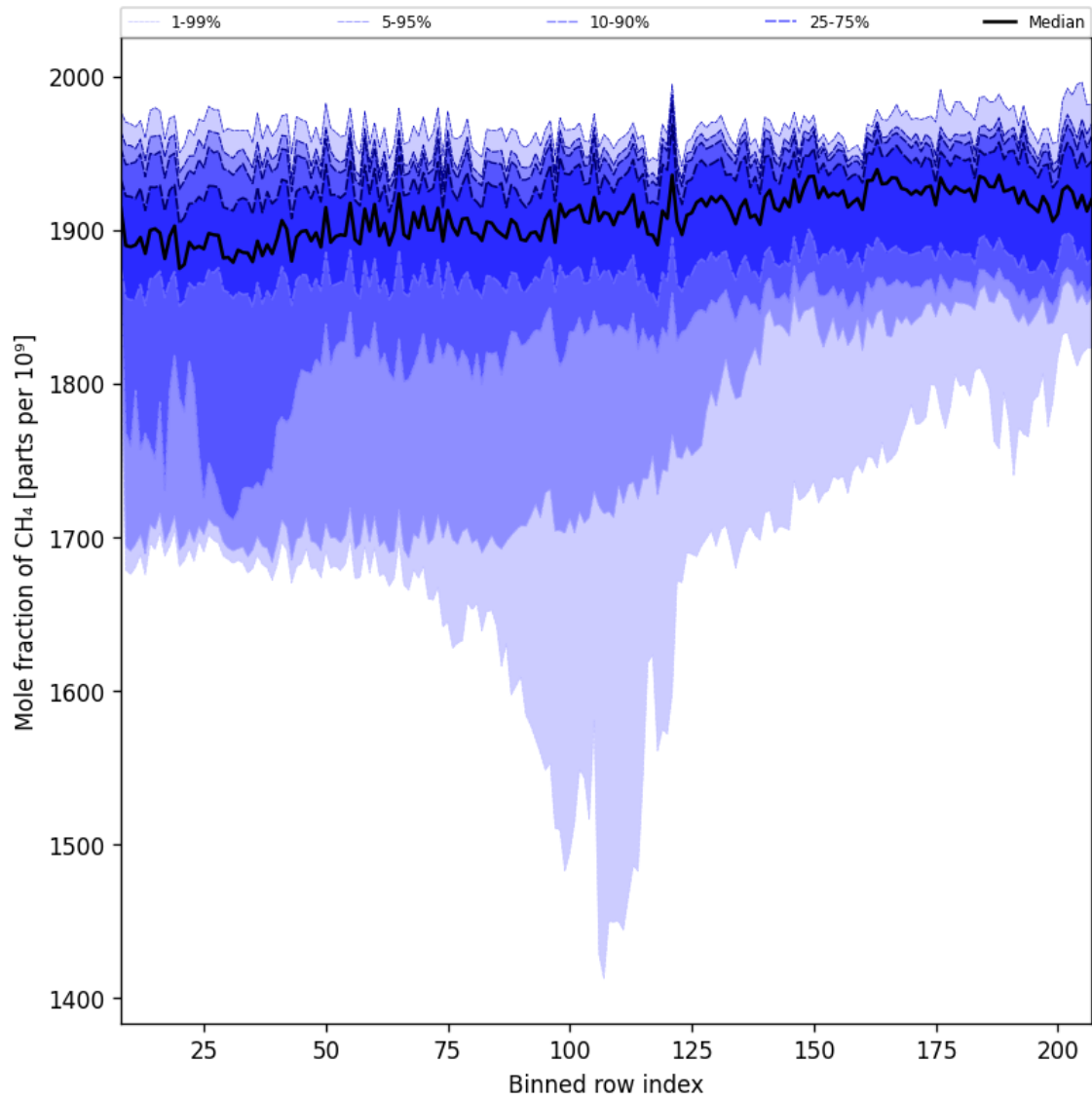
Figure 34: Along track statistics of “Mole fraction of CH 4 ” for 2024-10-04 to 2024-10-06
