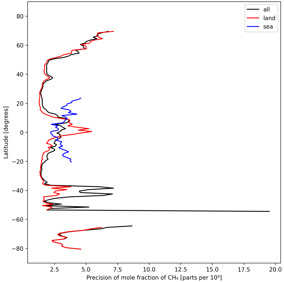
Figure 13: Zonal average of “Precision of mole fraction of CH 4 ” for 2024-10-05 to 2024-10-07.
