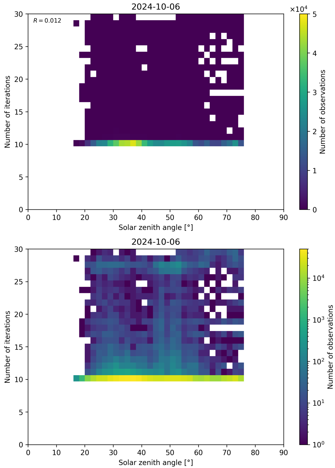
Figure 102: Scatter density plot of “Solar zenith angle” against “Number of iterations” for 2024-10-05 to 2024-10-07.
