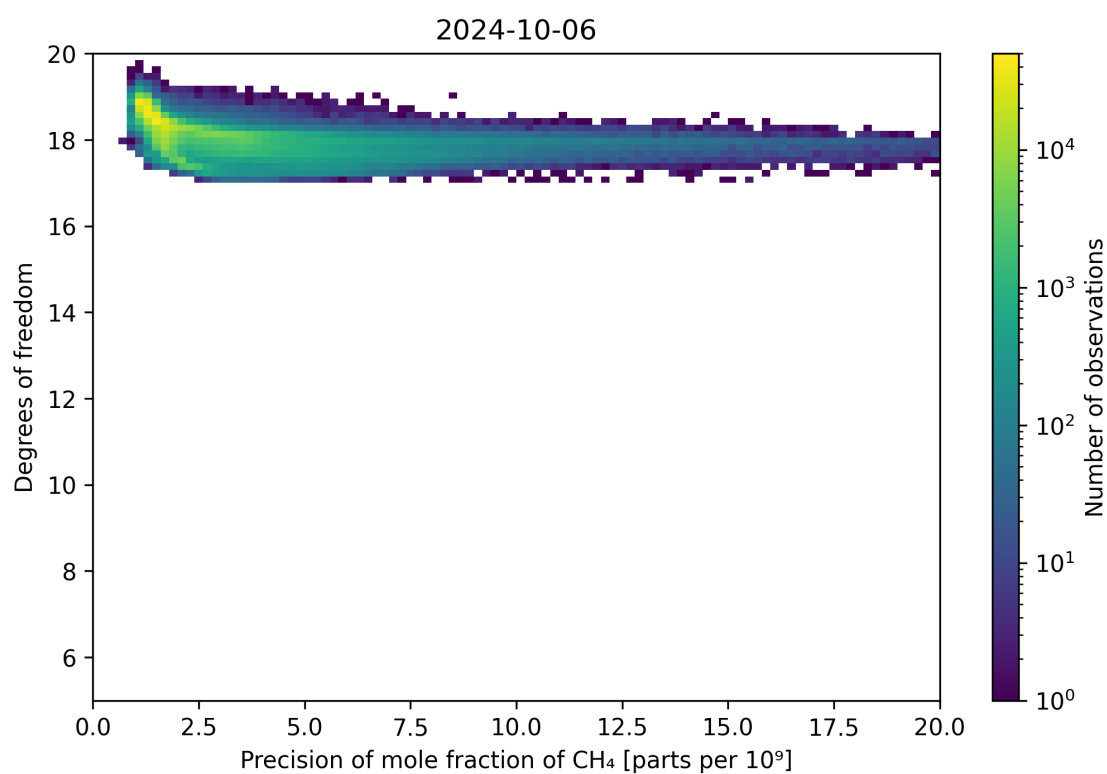
Figure 80: Scatter density plot of “Precision of mole fraction of CH 4 ” against “Degrees of freedom” for 2024-10-05 to 2024-10-07.
