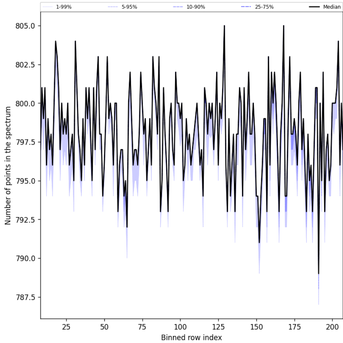
Figure 37: Along track statistics of “Number of points in the spectrum” for 2024-10-05 to 2024-10-07
