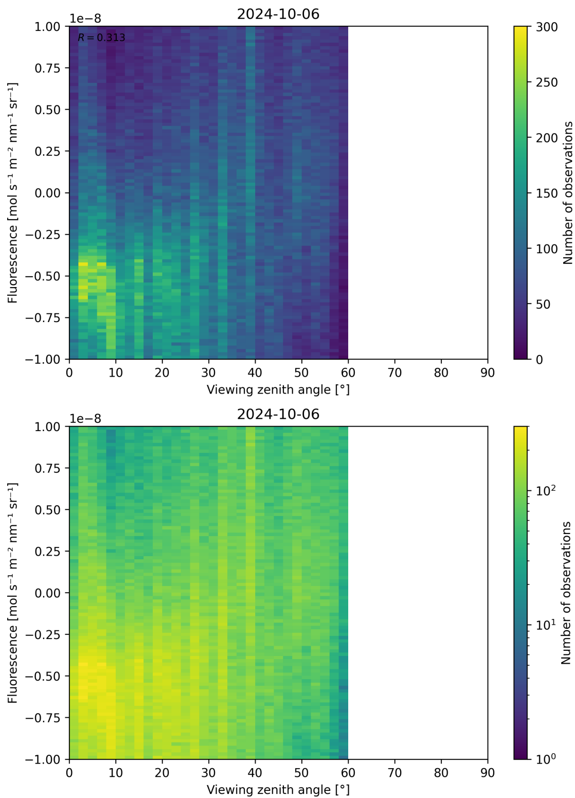
Figure 108: Scatter density plot of “Viewing zenith angle” against “Fluorescence” for 2024-10-05 to 2024-10-07.
