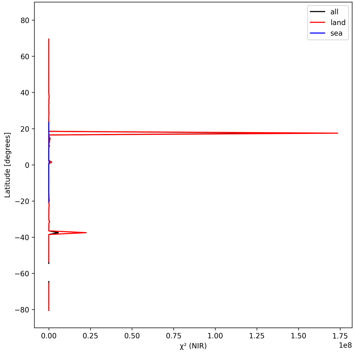
Figure 18: Zonal average of “ \chi^2 (NIR)” for 2024-10-05 to 2024-10-07.
