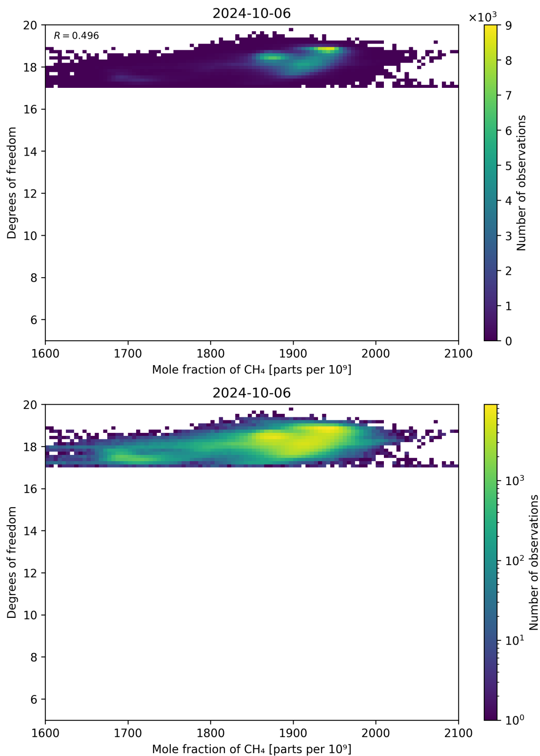
Figure 72: Scatter density plot of “Mole fraction of CH 4 ” against “Degrees of freedom” for 2024-10-05 to 2024-10-07.
