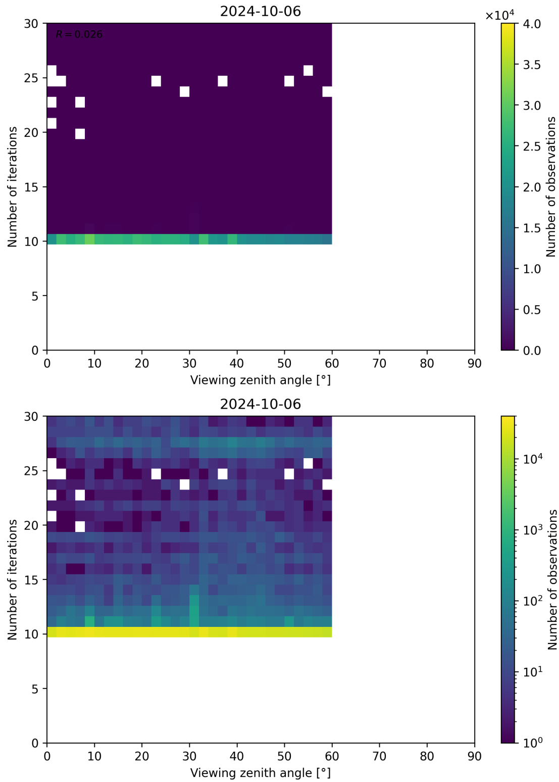
Figure 113: Scatter density plot of “Viewing zenith angle” against “Number of iterations” for 2024-10-05 to 2024-10-07.
