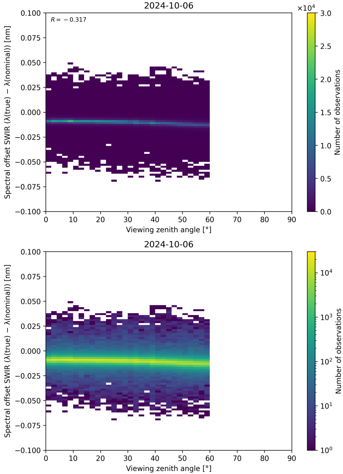
Figure 116: Scatter density plot of “Viewing zenith angle” against “Spectral offset SWIR ( \lambda_{\text{true}} - \lambda_{\text{nominal}} )” for 2024-10-05 to 2024-10-07.
