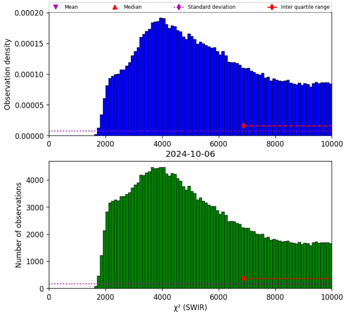
Figure 28: Histogram of " \chi^2 (SWIR)" for 2024-10-05 to 2024-10-07
