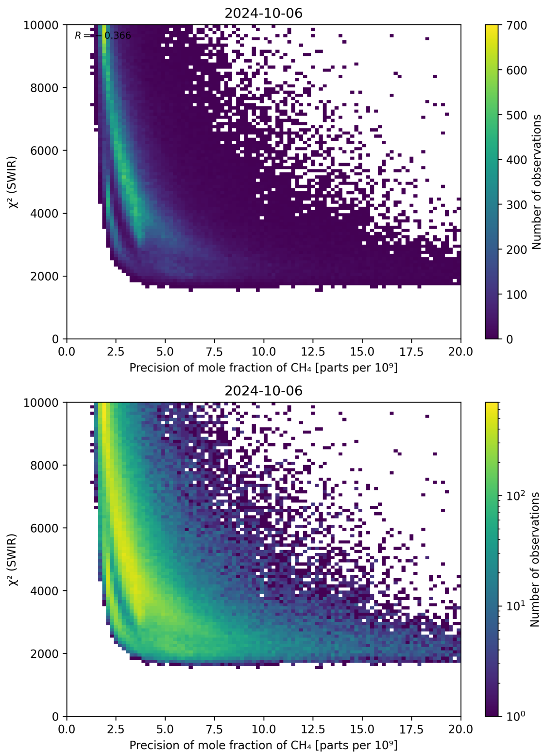
Figure 79: Scatter density plot of “Precision of mole fraction of \text{CH}_4 ” against “ \chi^2 (SWIR)” for 2024-10-05 to 2024-10-07.
