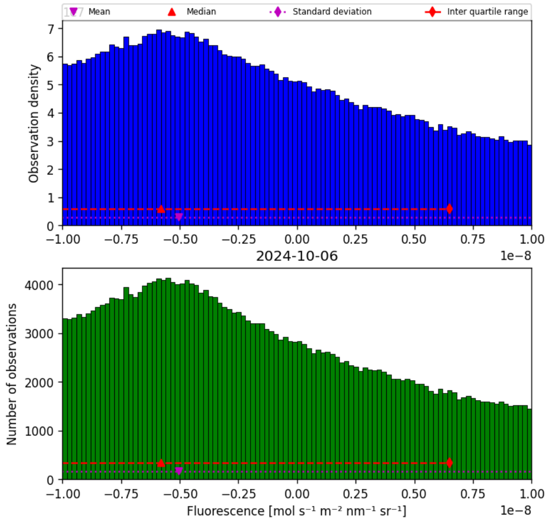
Figure 32: Histogram of “Fluorescence” for 2024-10-05 to 2024-10-07
