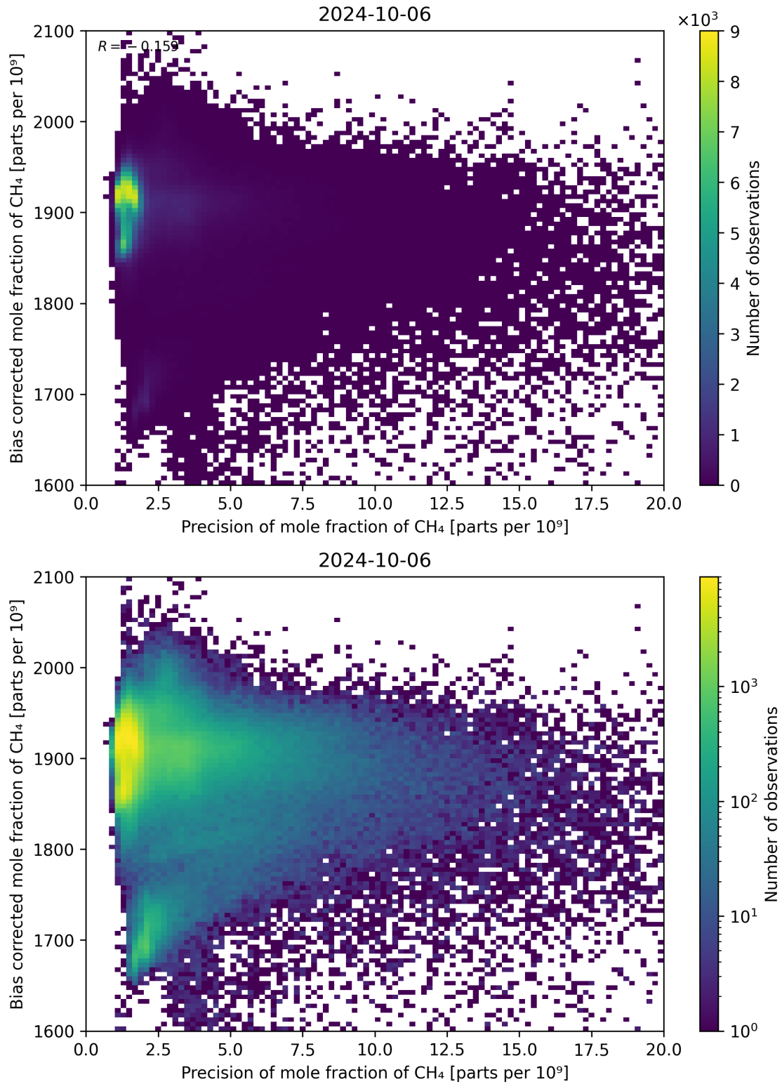
Figure 82: Scatter density plot of “Precision of mole fraction of CH 4 ” against “Bias corrected mole fraction of CH 4 ” for 2024-10-05 to 2024-10-07.
