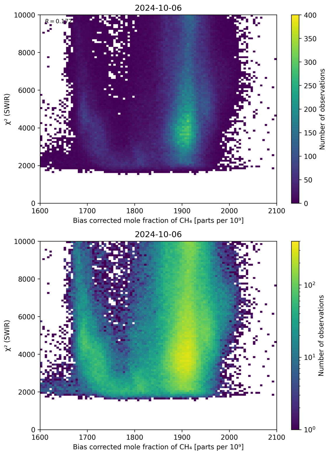
Figure 64: Scatter density plot of “Bias corrected mole fraction of \text{CH}_4 ” against “ \chi^2 (SWIR)” for 2024-10-05 to 2024-10-07.
