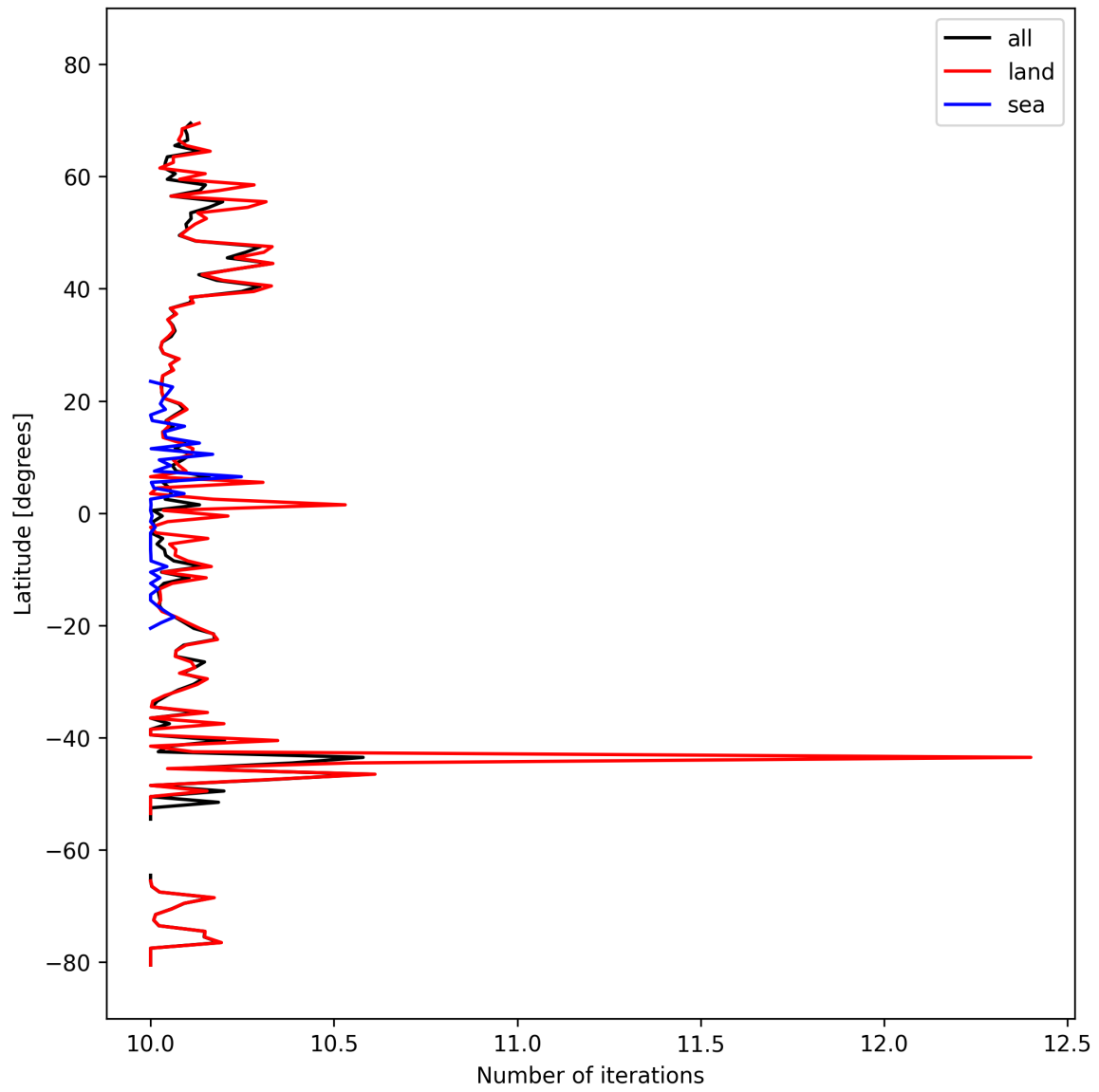
Figure 20: Zonal average of “Number of iterations” for 2024-10-05 to 2024-10-07.
