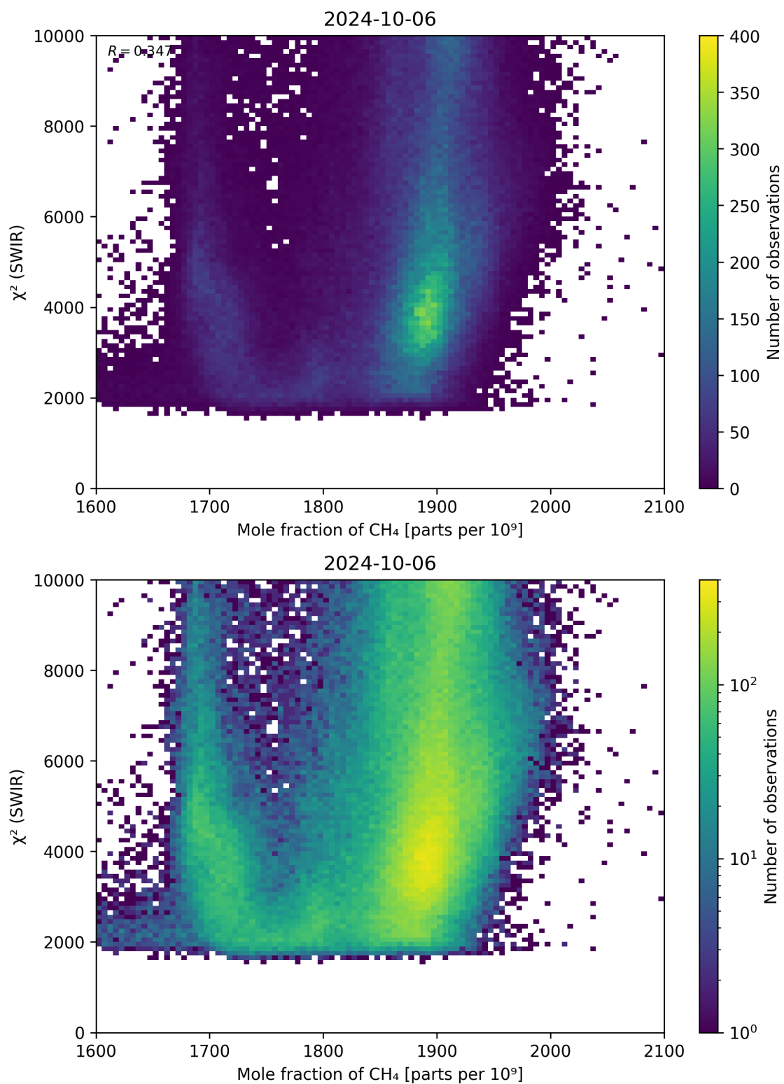
Figure 71: Scatter density plot of “Mole fraction of \text{CH}_4 ” against “ \chi^2 (SWIR)” for 2024-10-05 to 2024-10-07.
