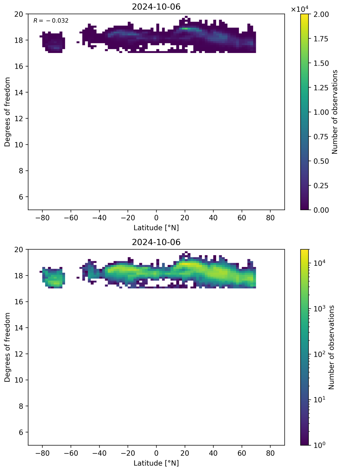
Figure 55: Scatter density plot of “Latitude” against “Degrees of freedom” for 2024-10-05 to 2024-10-07.
