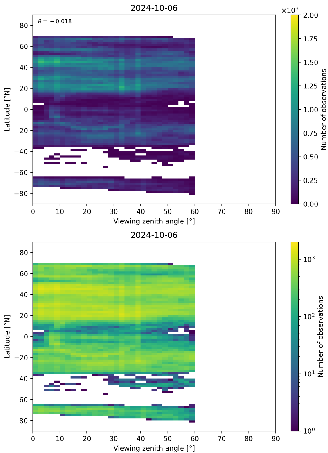
Figure 109: Scatter density plot of “Viewing zenith angle” against “Latitude” for 2024-10-05 to 2024-10-07.
