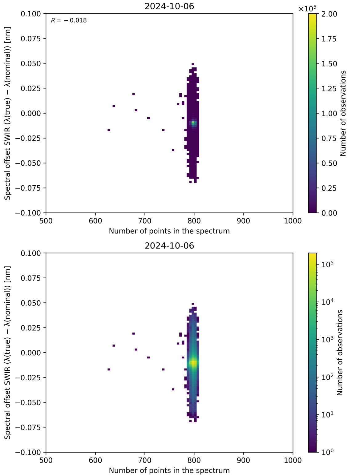
Figure 93: Scatter density plot of “Number of points in the spectrum” against “Spectral offset SWIR ( \lambda_{\text{true}} - \lambda_{\text{nominal}} )” for 2024-10-05 to 2024-10-07.
