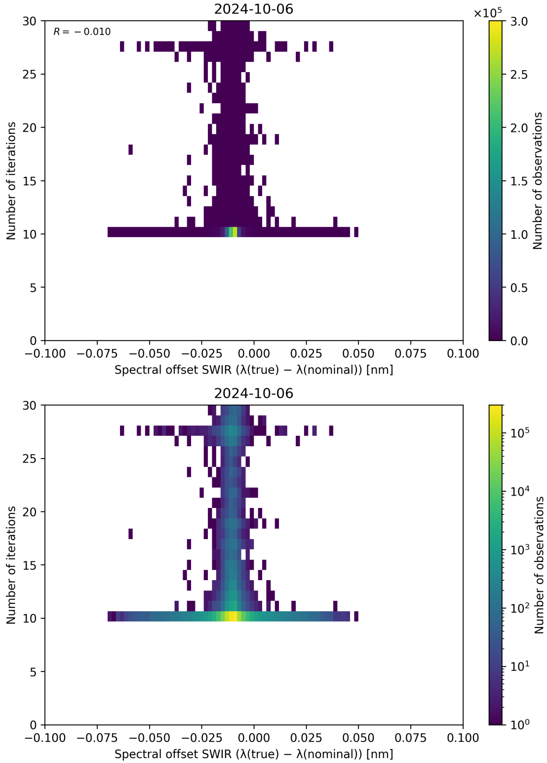
Figure 121: Scatter density plot of “Spectral offset SWIR ( \lambda_{\text{true}} - \lambda_{\text{nominal}} )” against “Number of iterations” for 2024-10-05 to 2024-10-07.
