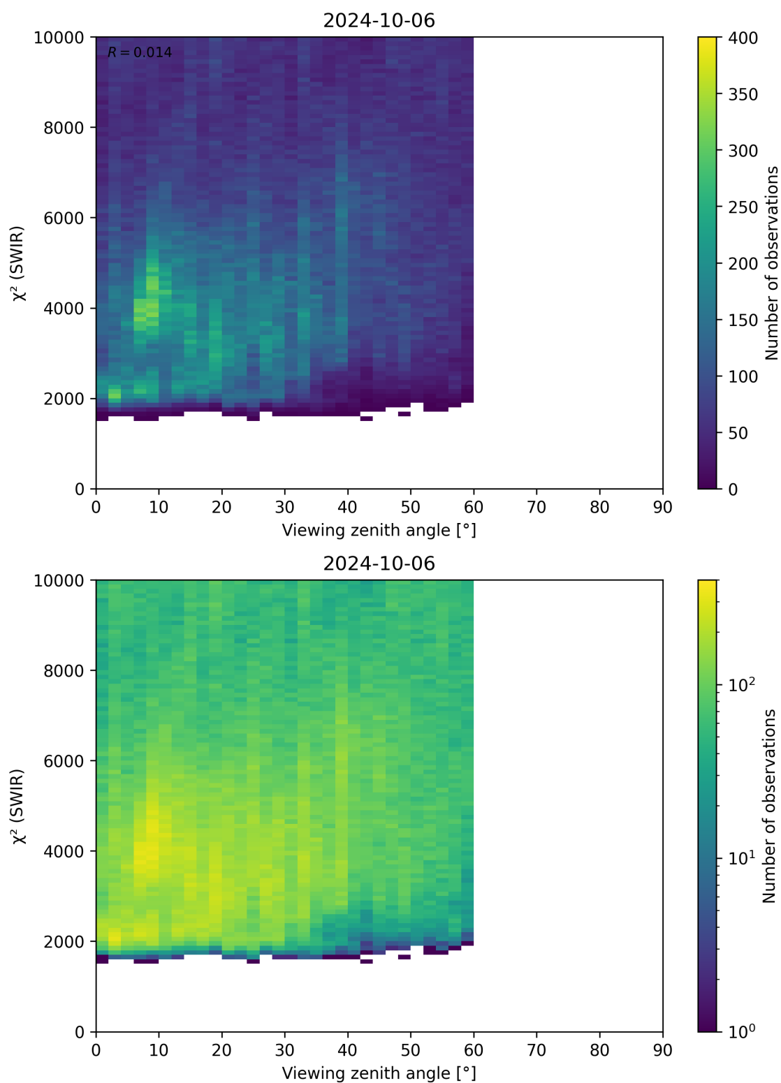
Figure 106: Scatter density plot of “Viewing zenith angle” against “ \chi^2 (SWIR)” for 2024-10-05 to 2024-10-07.
