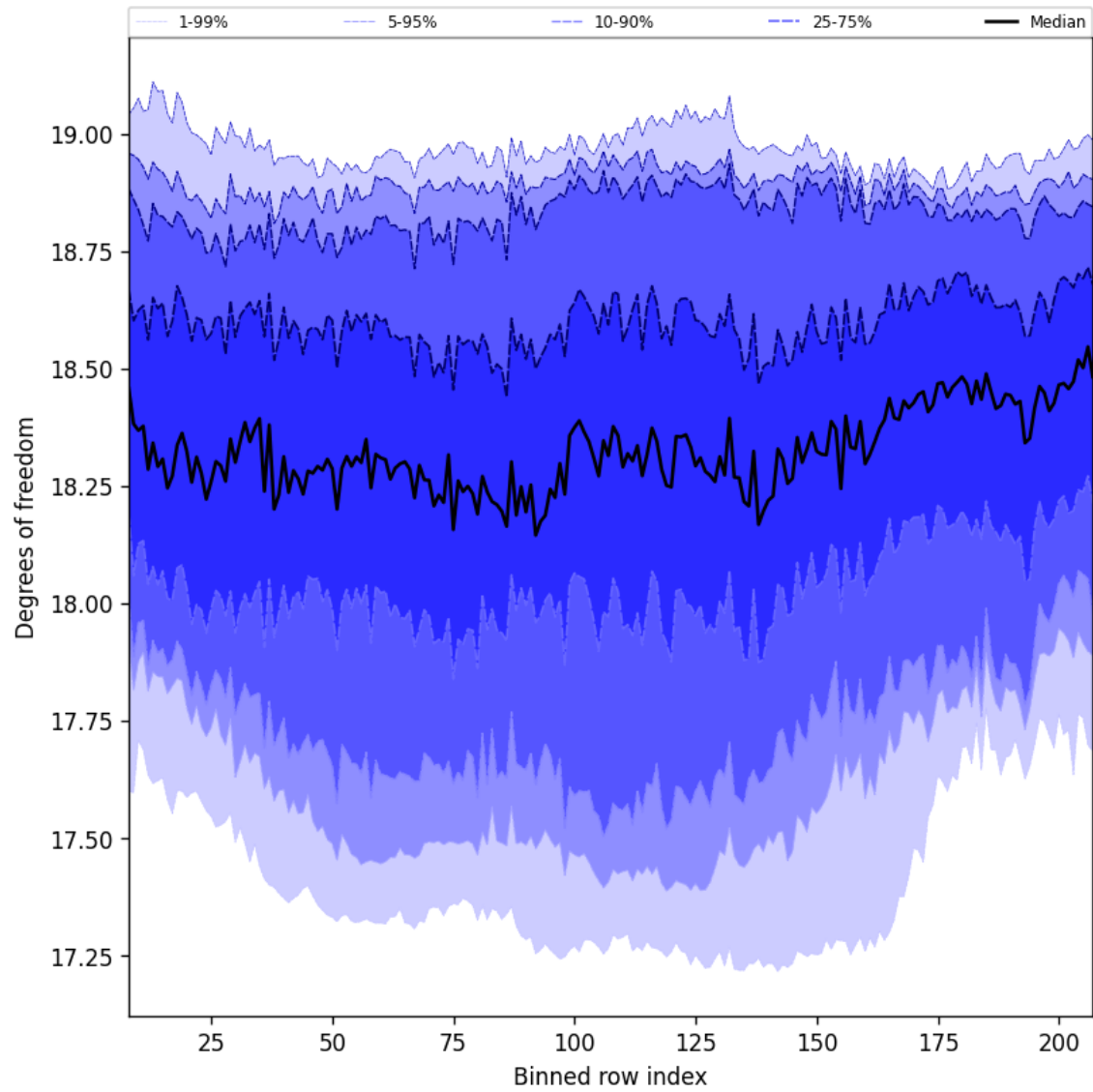
Figure 41: Along track statistics of “Degrees of freedom” for 2024-10-05 to 2024-10-07
