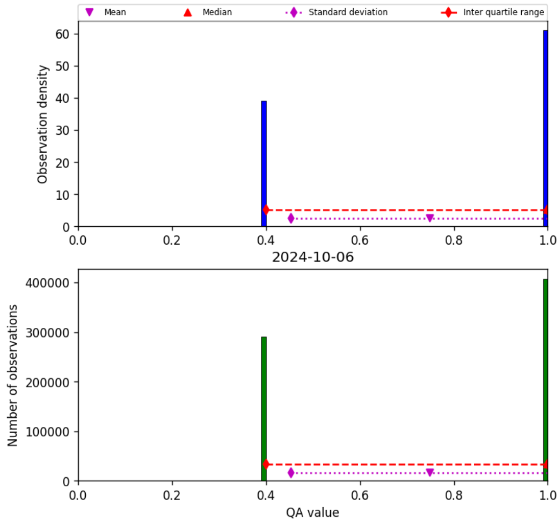
Figure 22: Histogram of “QA value” for 2024-10-05 to 2024-10-07
