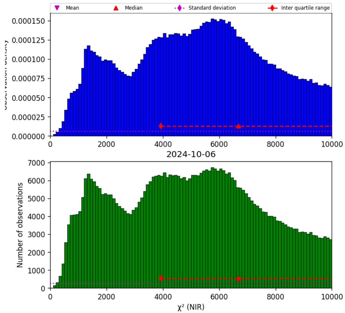
Figure 29: Histogram of “ \chi^2 (NIR)” for 2024-10-05 to 2024-10-07
