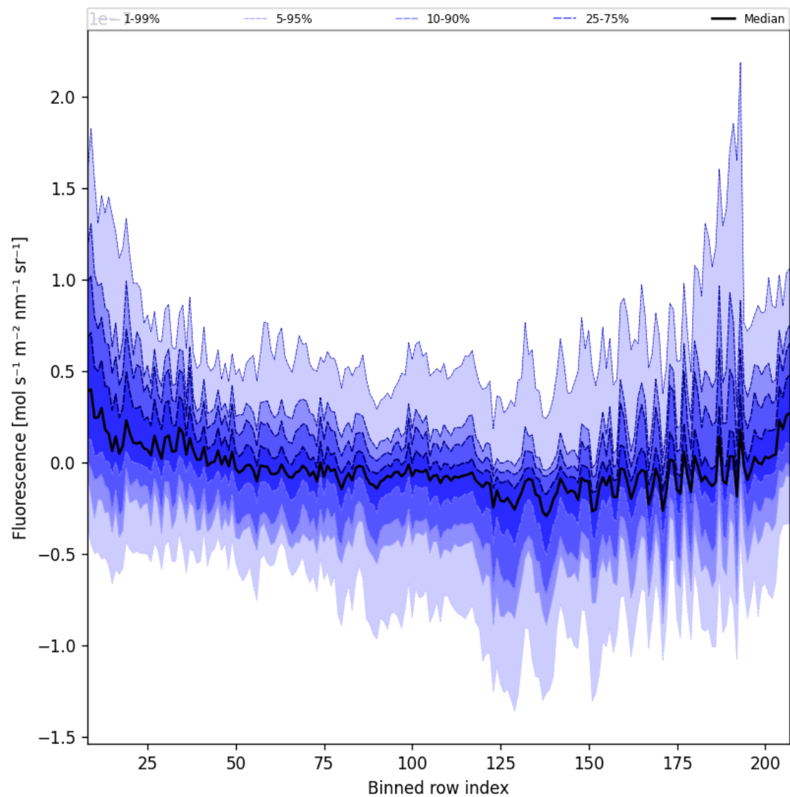
Figure 43: Along track statistics of “Fluorescence” for 2024-10-05 to 2024-10-07
