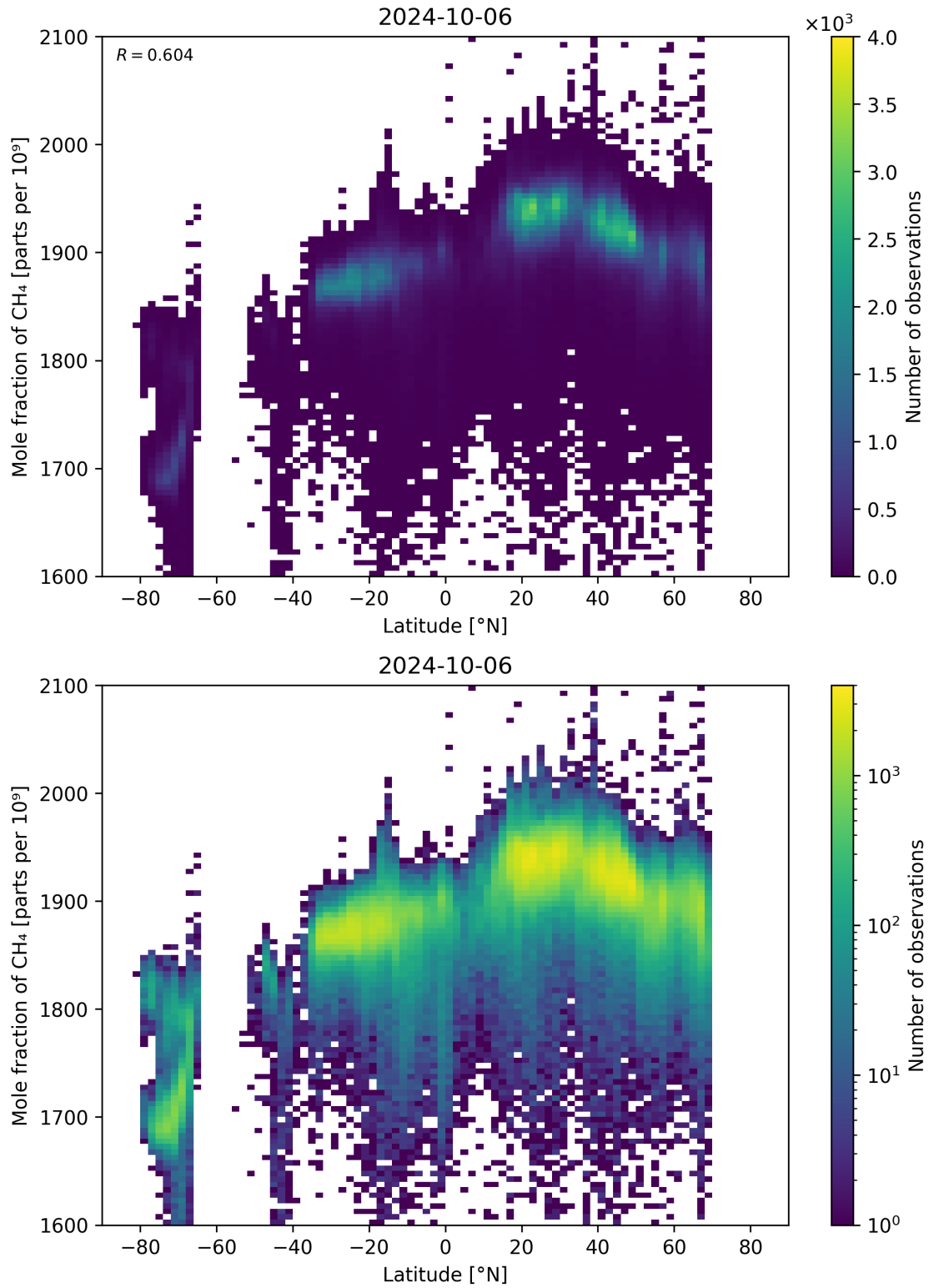
Figure 57: Scatter density plot of “Latitude” against “Mole fraction of CH 4 ” for 2024-10-05 to 2024-10-07.
