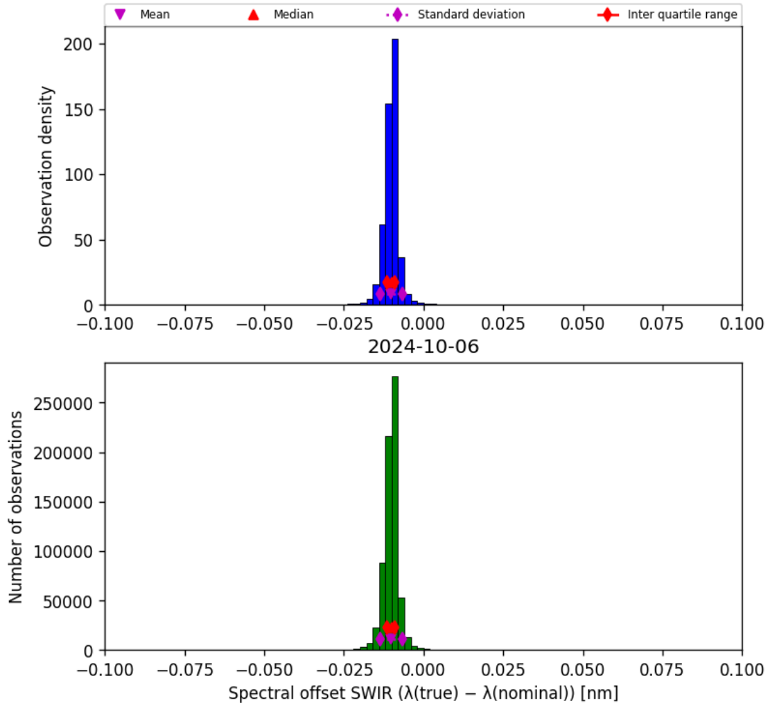
Figure 27: Histogram of “Spectral offset SWIR ( \lambda_{\text{true}} - \lambda_{\text{nominal}} )” for 2024-10-05 to 2024-10-07
