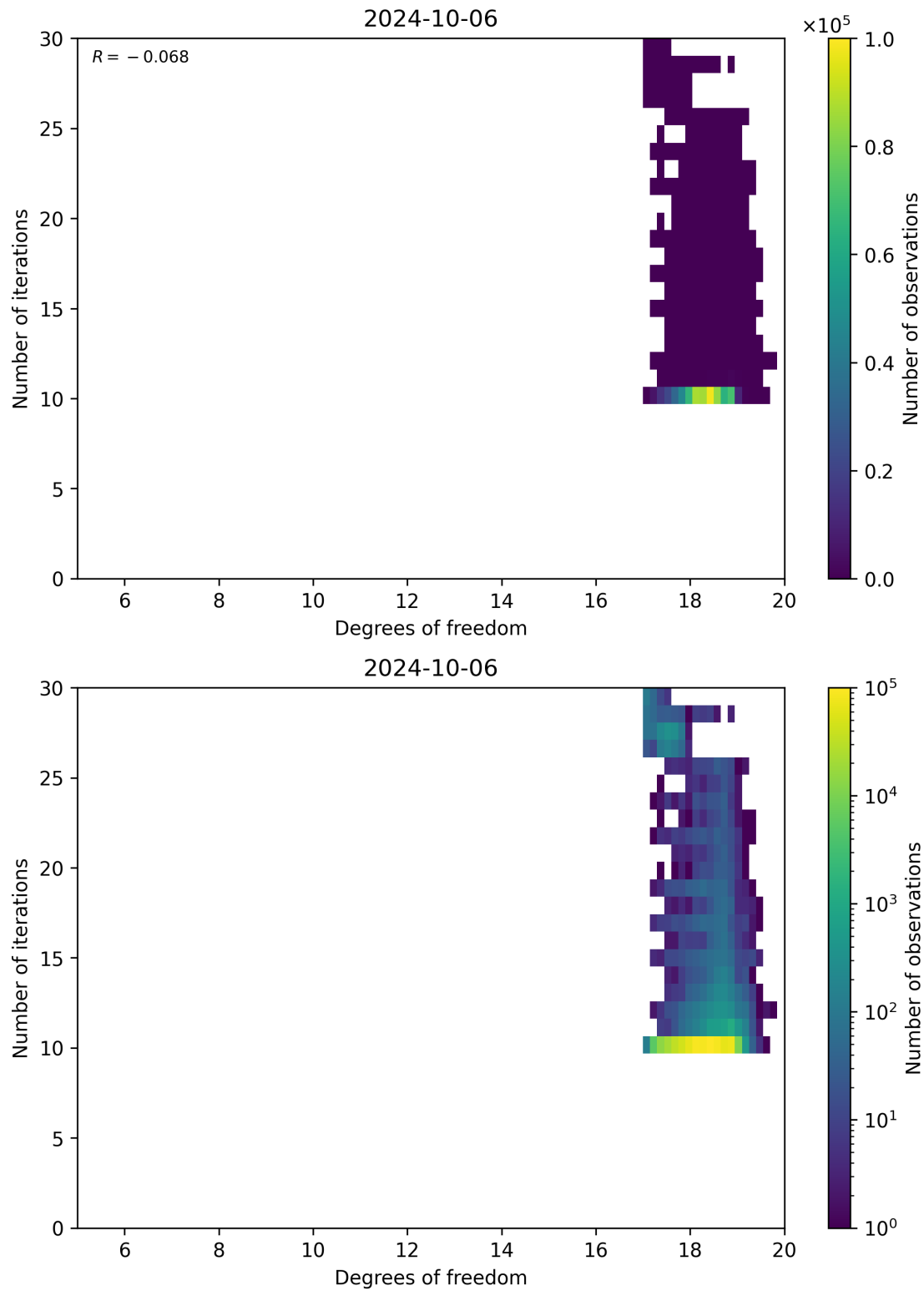
Figure 52: Scatter density plot of “Degrees of freedom” against “Number of iterations” for 2024-10-05 to 2024-10-07.
