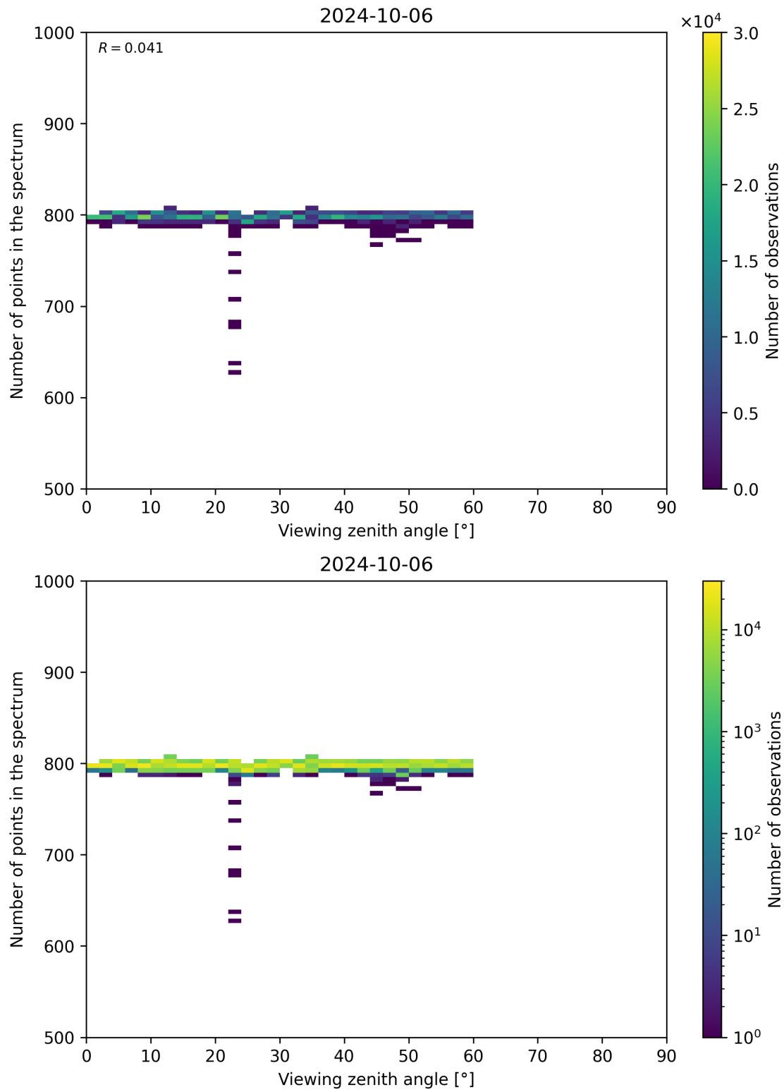
Figure 114: Scatter density plot of “Viewing zenith angle” against “Number of points in the spectrum” for 2024-10-05 to 2024-10-07.
