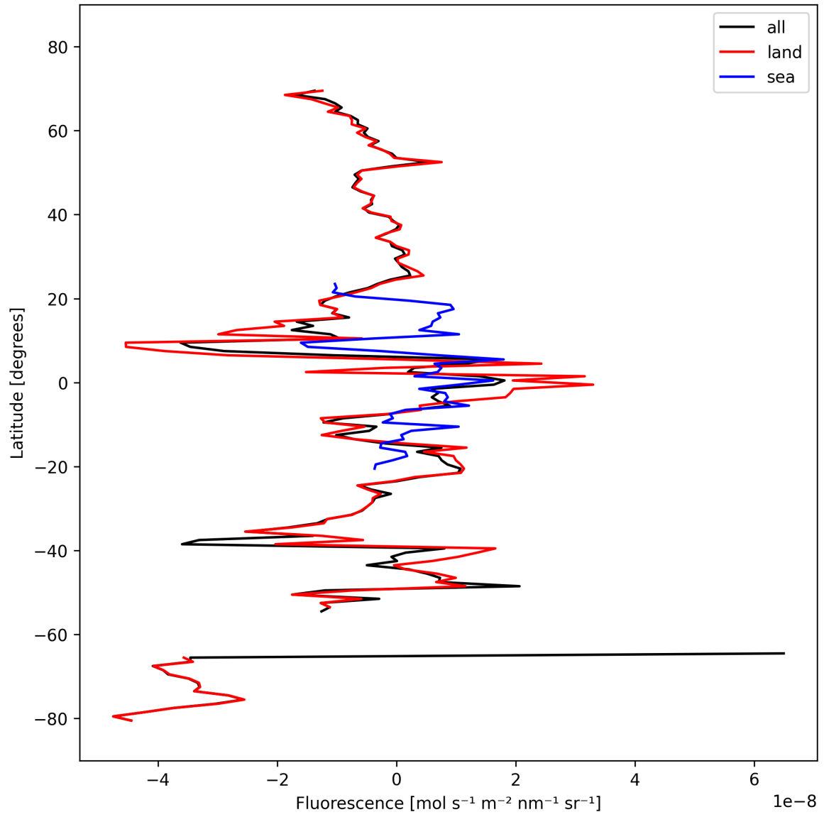
Figure 21: Zonal average of “Fluorescence” for 2024-10-05 to 2024-10-07.
