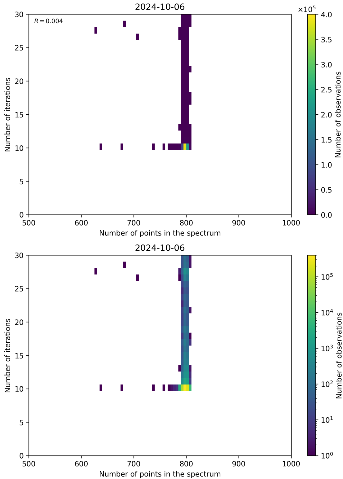
Figure 92: Scatter density plot of “Number of points in the spectrum” against “Number of iterations” for 2024-10-05 to 2024-10-07.
