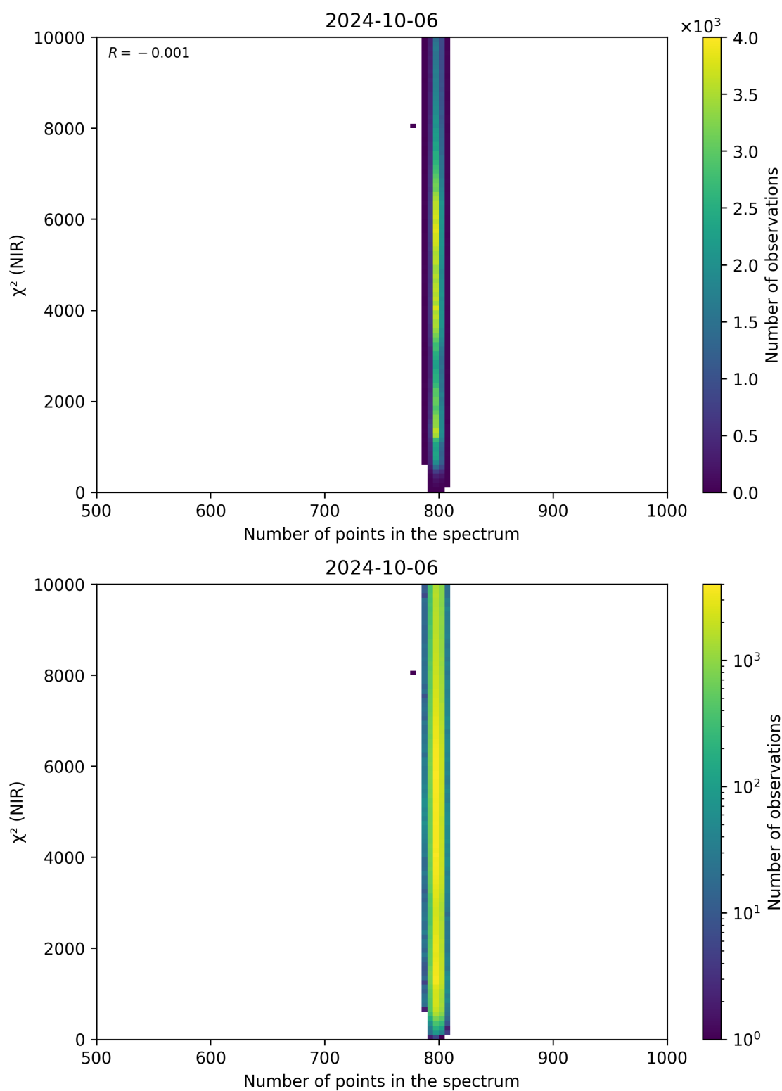
Figure 88: Scatter density plot of “Number of points in the spectrum” against “ \chi^2 (NIR)” for 2024-10-05 to 2024-10-07.
