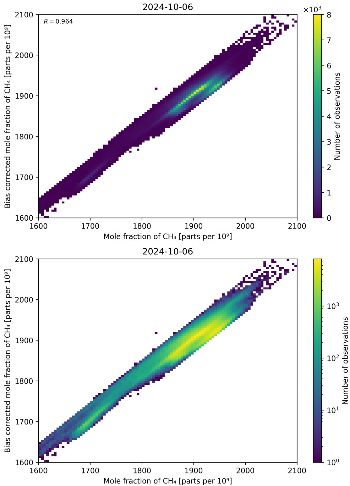
Figure 74: Scatter density plot of “Mole fraction of CH 4 ” against “Bias corrected mole fraction of CH 4 ” for 2024-10-05 to 2024-10-07.
