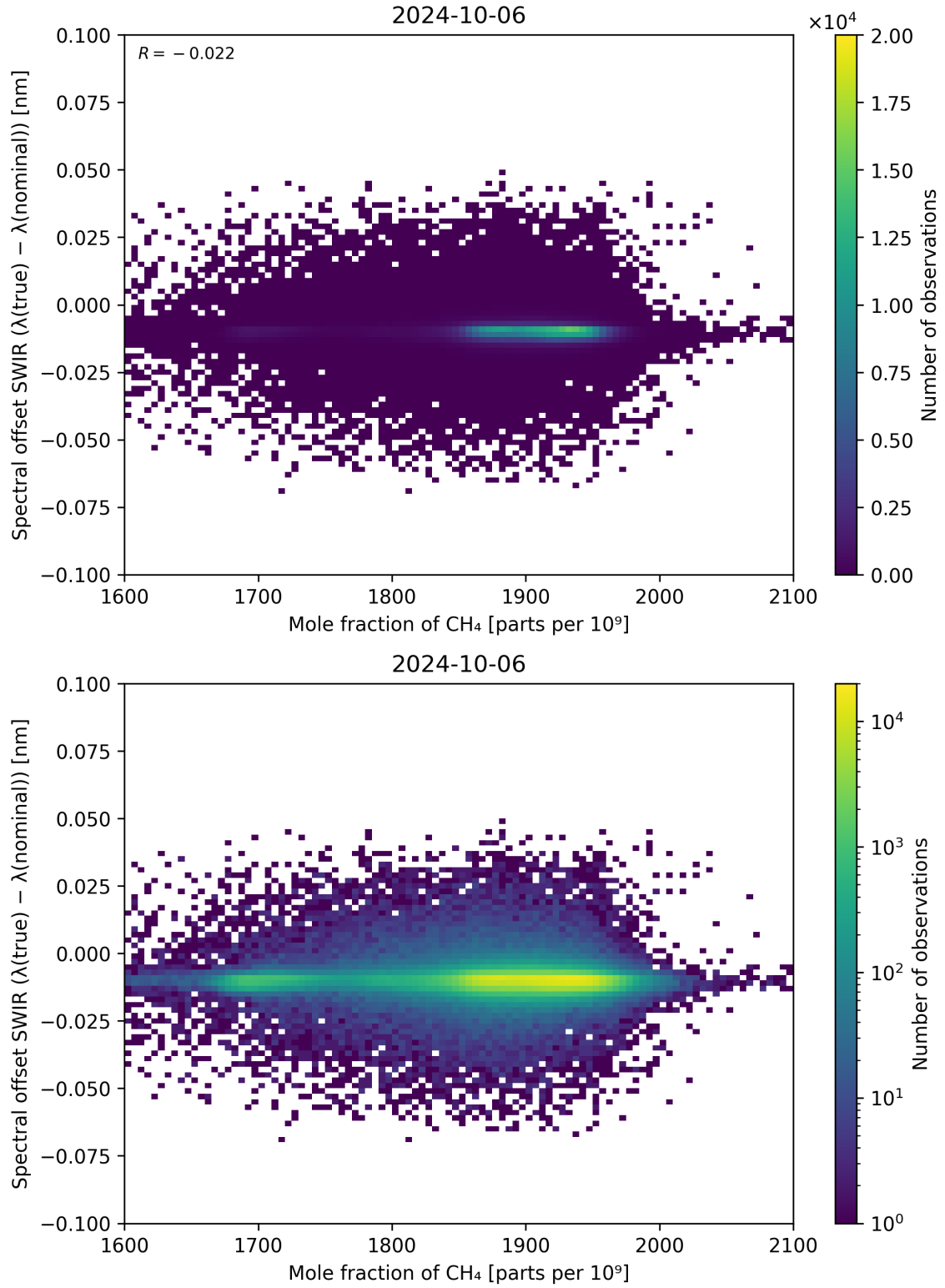
Figure 86: Scatter density plot of “Mole fraction of CH 4 ” against “Spectral offset SWIR ( \lambda_{\text{true}} - \lambda_{\text{nominal}} )” for 2024-10-05 to 2024-10-07.
