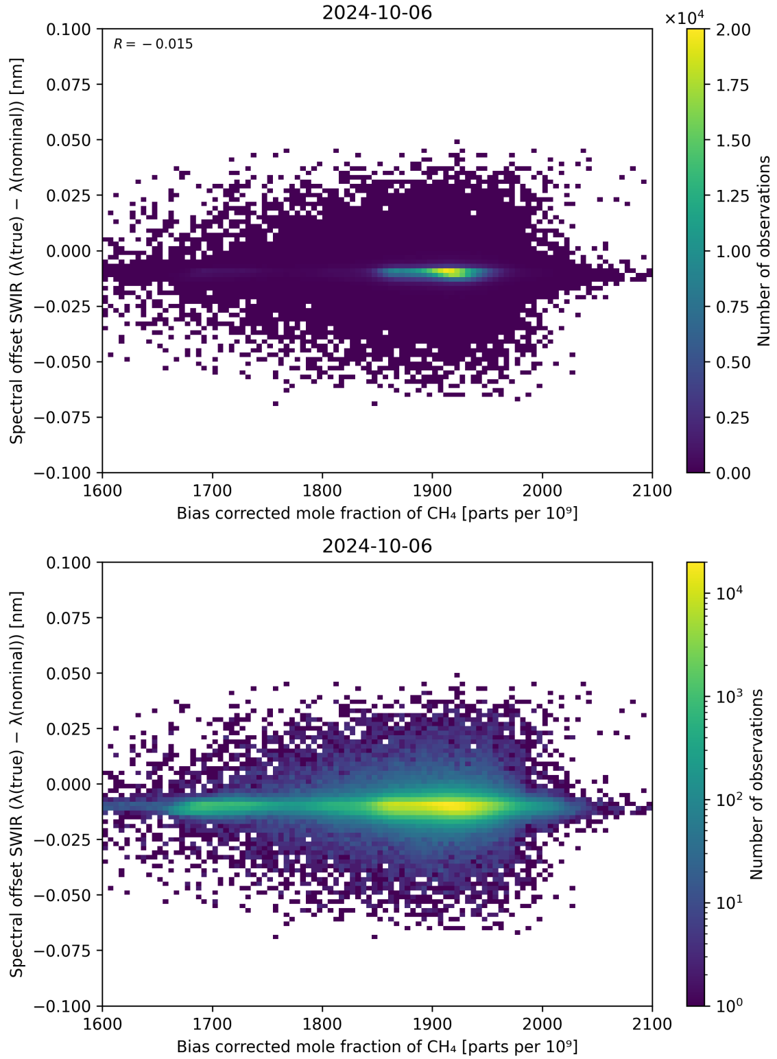
Figure 69: Scatter density plot of “Bias corrected mole fraction of \text{CH}_4 ” against “Spectral offset SWIR ( \lambda_{\text{true}} - \lambda_{\text{nominal}} )” for 2024-10-05 to 2024-10-07.
