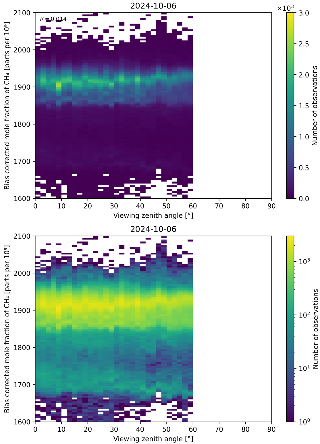
Figure 111: Scatter density plot of “Viewing zenith angle” against “Bias corrected mole fraction of CH 4 ” for 2024-10-05 to 2024-10-07.
