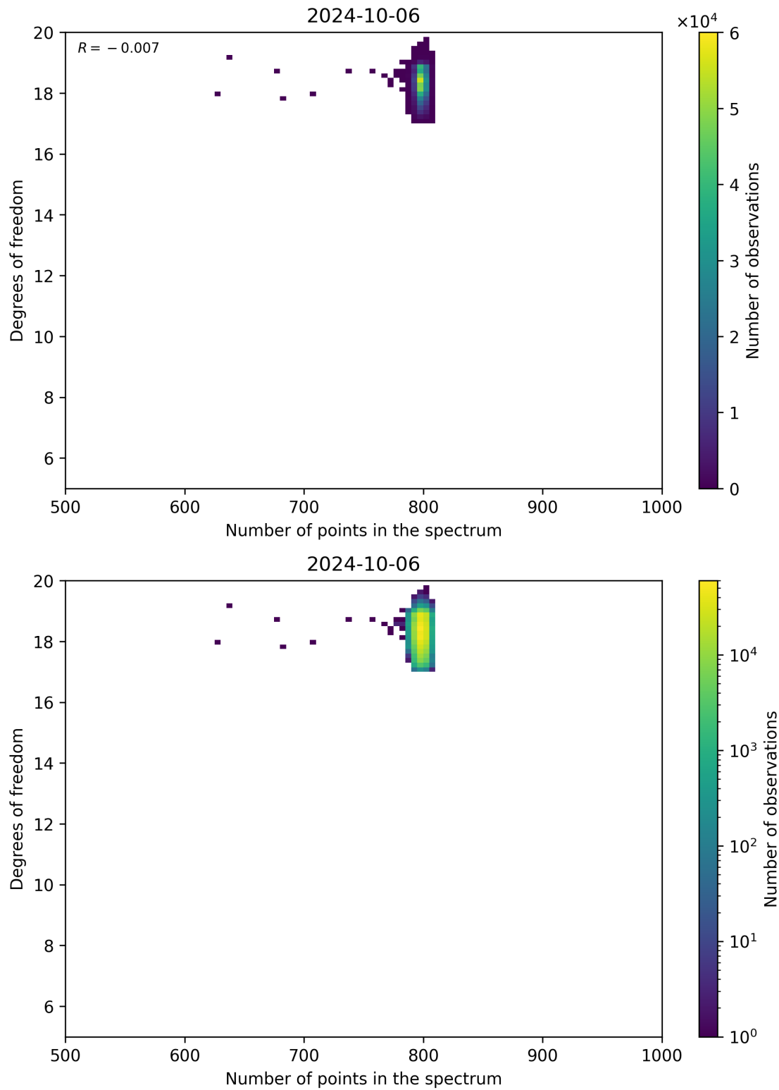
Figure 90: Scatter density plot of “Number of points in the spectrum” against “Degrees of freedom” for 2024-10-05 to 2024-10-07.
