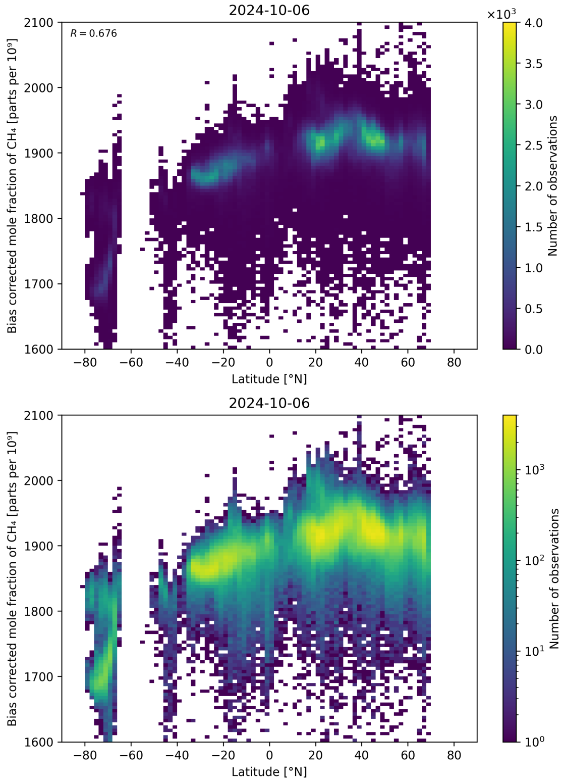
Figure 58: Scatter density plot of “Latitude” against “Bias corrected mole fraction of \text{CH}_4 ” for 2024-10-05 to 2024-10-07.
