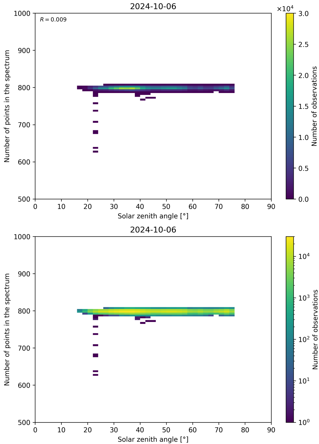
Figure 103: Scatter density plot of “Solar zenith angle” against “Number of points in the spectrum” for 2024-10-05 to 2024-10-07.
