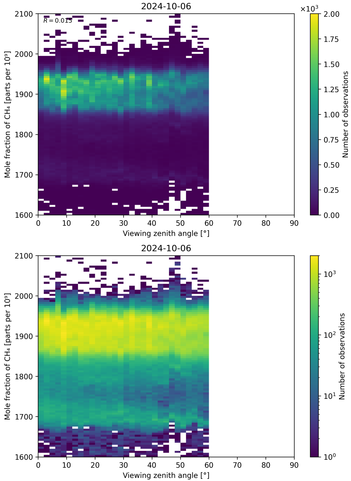
Figure 110: Scatter density plot of “Viewing zenith angle” against “Mole fraction of CH 4 ” for 2024-10-05 to 2024-10-07.
