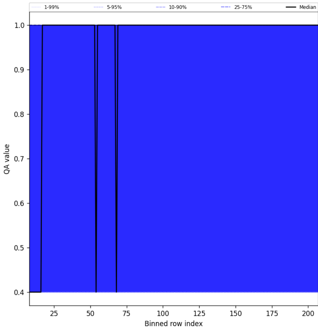
Figure 33: Along track statistics of “QA value” for 2024-10-05 to 2024-10-07
