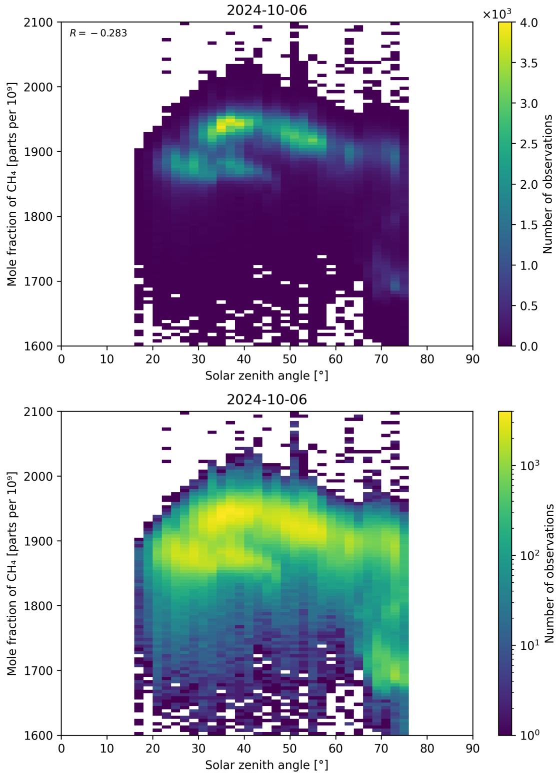
Figure 99: Scatter density plot of “Solar zenith angle” against “Mole fraction of \text{CH}_4 ” for 2024-10-05 to 2024-10-07.
