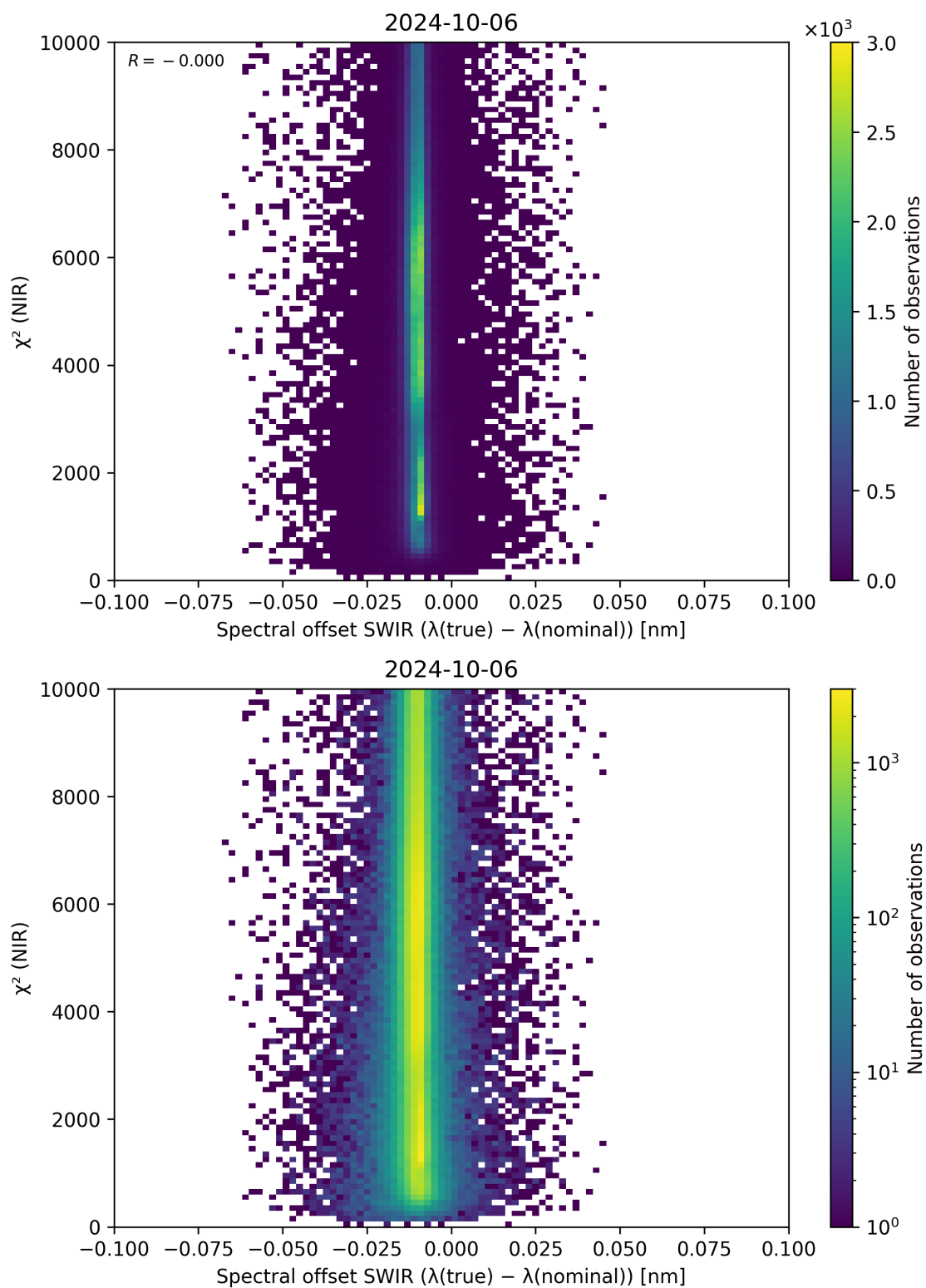
Figure 117: Scatter density plot of “Spectral offset SWIR ( \lambda_{\text{true}} - \lambda_{\text{nominal}} )” against “ \chi^2 (NIR)” for 2024-10-05 to 2024-10-07.
