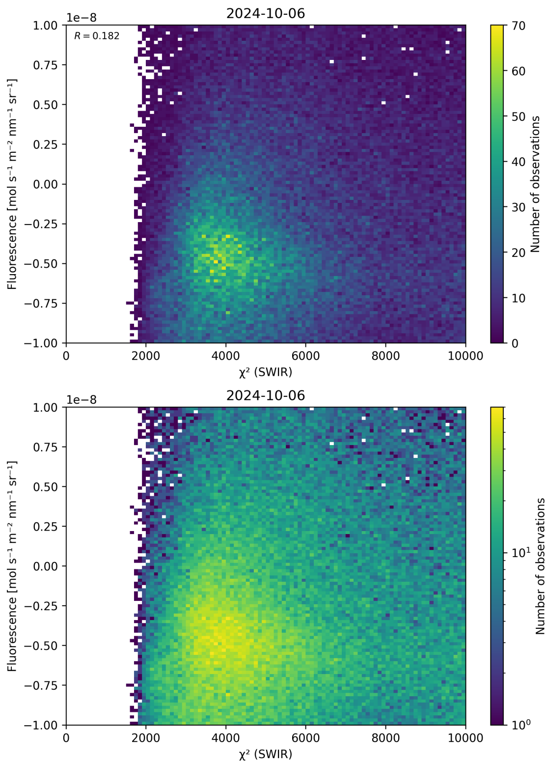
Figure 49: Scatter density plot of “ \chi^2 (SWIR)” against “Fluorescence” for 2024-10-05 to 2024-10-07.
