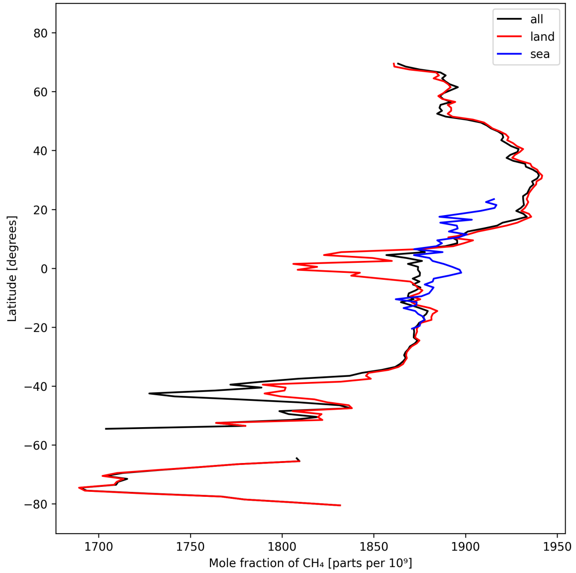
Figure 12: Zonal average of “Mole fraction of CH 4 ” for 2024-10-05 to 2024-10-07.
