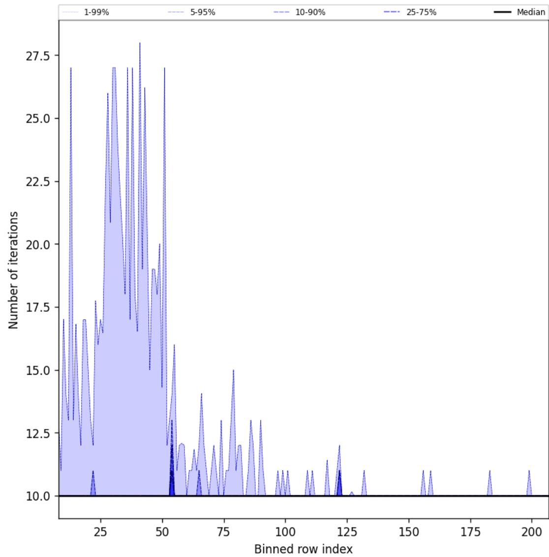
Figure 42: Along track statistics of “Number of iterations” for 2024-10-05 to 2024-10-07
