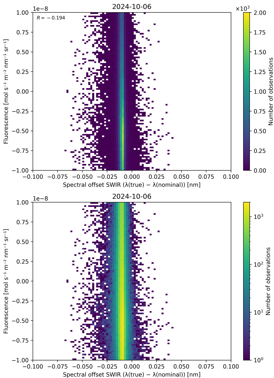
Figure 120: Scatter density plot of “Spectral offset SWIR ( \lambda_{\text{true}} - \lambda_{\text{nominal}} )” against “Fluorescence” for 2024-10-05 to 2024-10-07.
