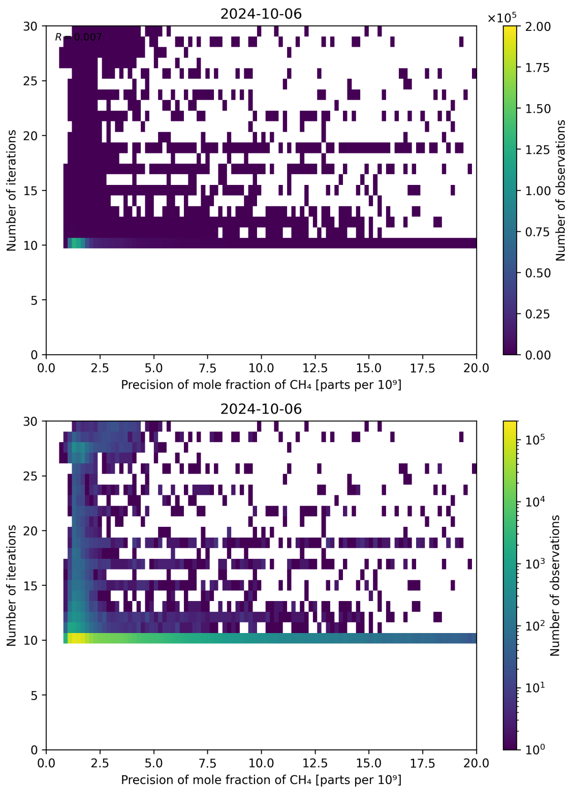
Figure 83: Scatter density plot of “Precision of mole fraction of CH 4 ” against “Number of iterations” for 2024-10-05 to 2024-10-07.
