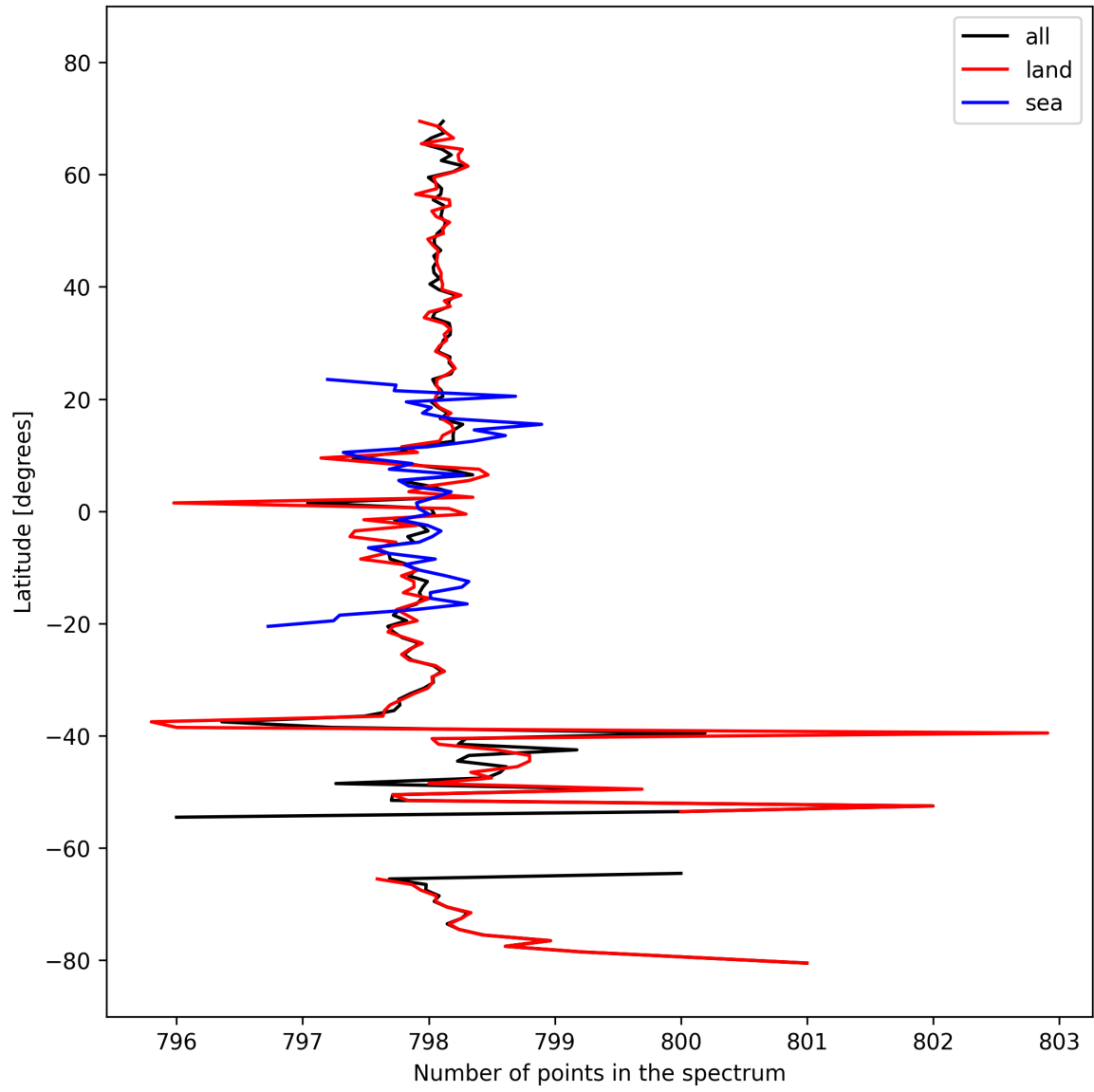
Figure 15: Zonal average of “Number of points in the spectrum” for 2024-10-05 to 2024-10-07.
