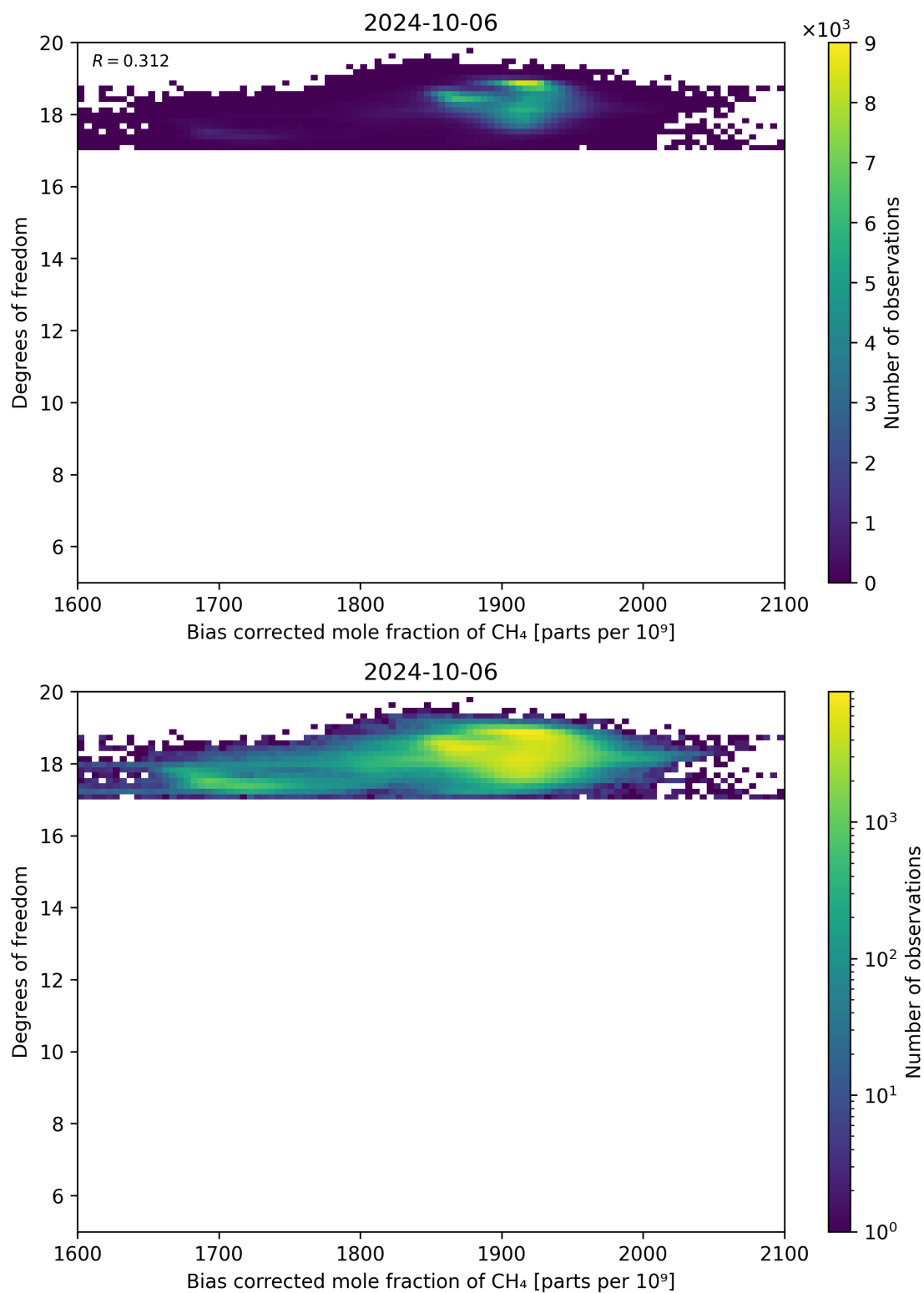
Figure 65: Scatter density plot of “Bias corrected mole fraction of CH 4 ” against “Degrees of freedom” for 2024-10-05 to 2024-10-07.
