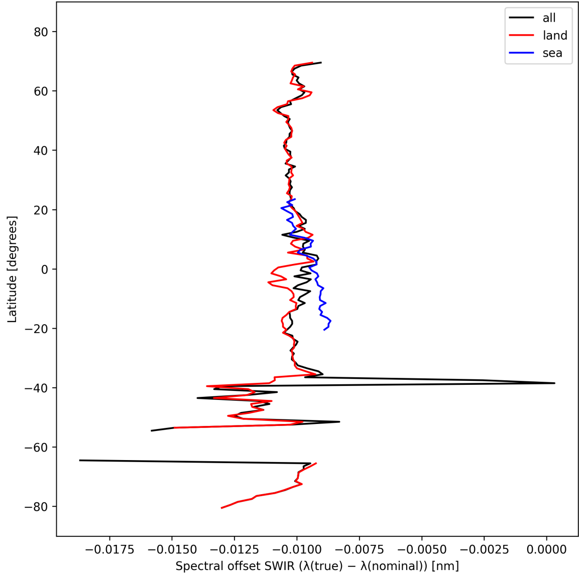
Figure 16: Zonal average of “Spectral offset SWIR ( \lambda_{\text{true}} - \lambda_{\text{nominal}} )” for 2024-10-05 to 2024-10-07.
