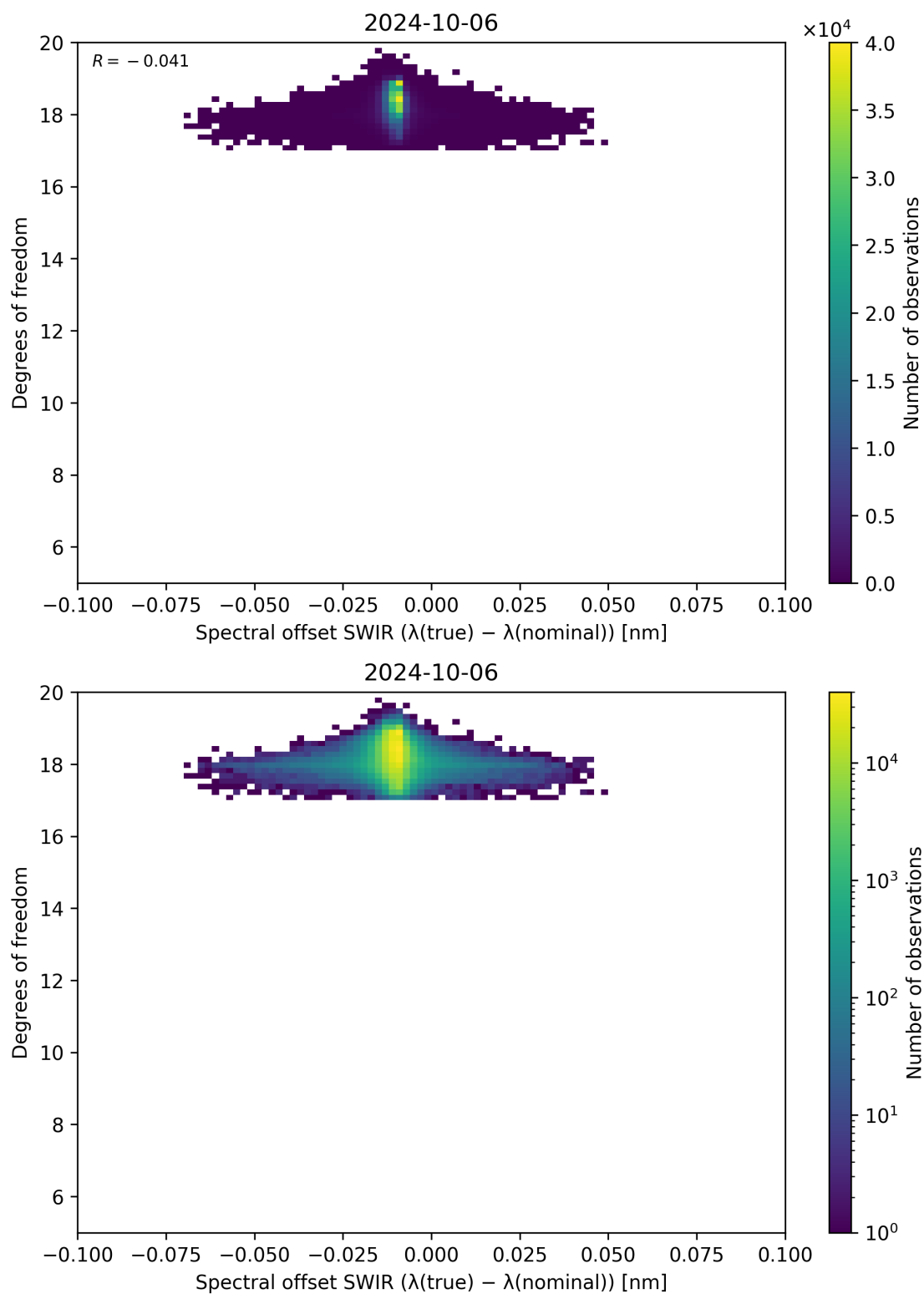
Figure 119: Scatter density plot of “Spectral offset SWIR ( \lambda_{\text{true}} - \lambda_{\text{nominal}} )” against “Degrees of freedom” for 2024-10-05 to 2024-10-07.
