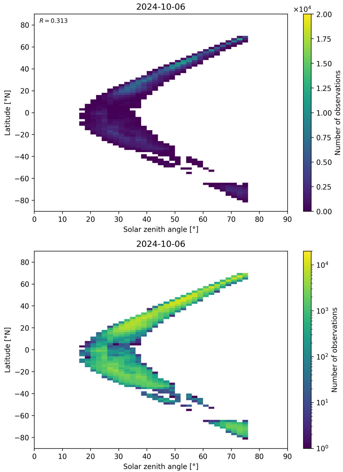
Figure 98: Scatter density plot of “Solar zenith angle” against “Latitude” for 2024-10-05 to 2024-10-07.
