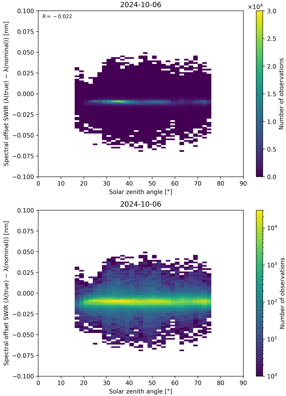
Figure 104: Scatter density plot of “Solar zenith angle” against “Spectral offset SWIR ( \lambda_{\text{true}} - \lambda_{\text{nominal}} )” for 2024-10-05 to 2024-10-07.
