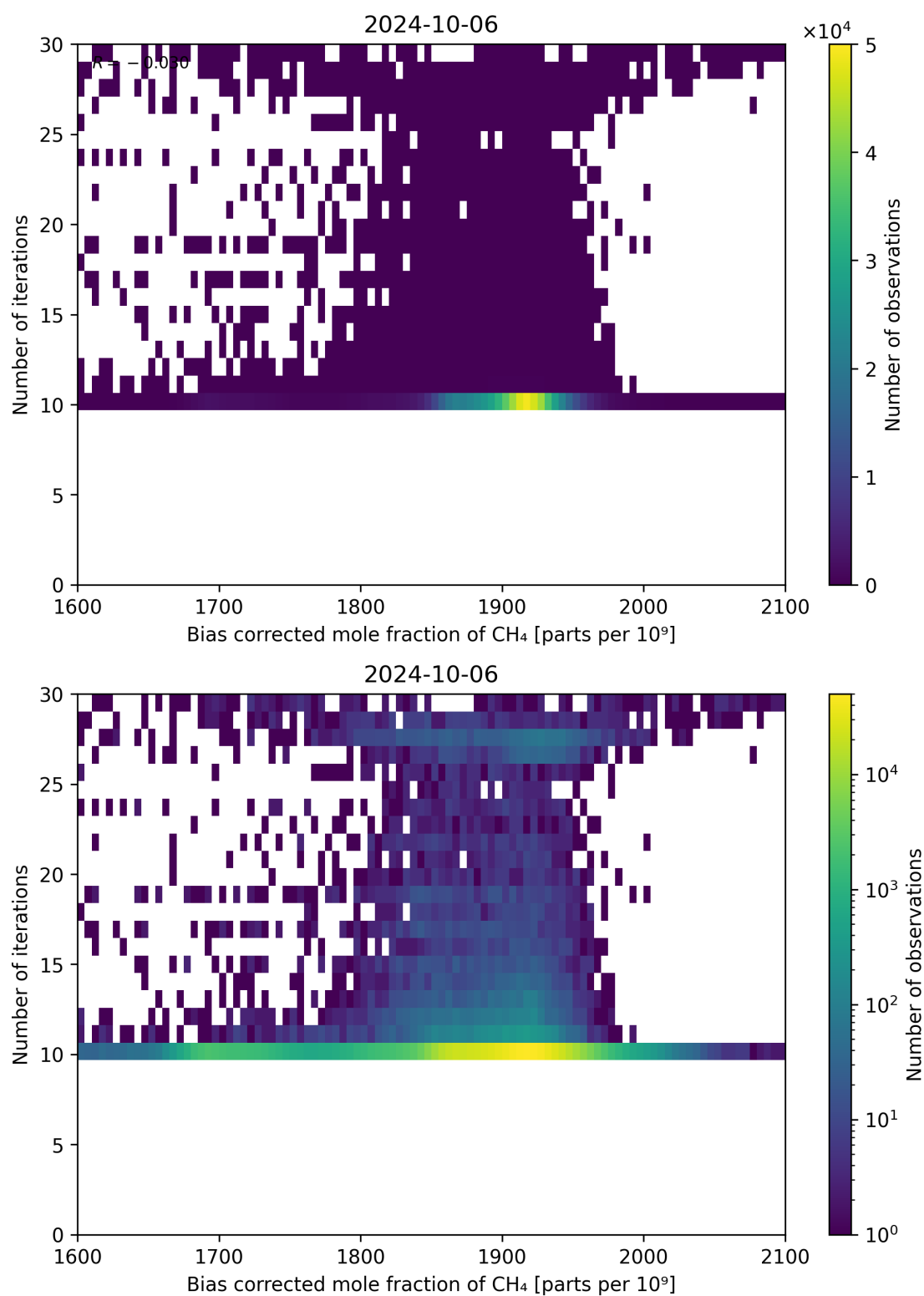
Figure 67: Scatter density plot of “Bias corrected mole fraction of \text{CH}_4 ” against “Number of iterations” for 2024-10-05 to 2024-10-07.
