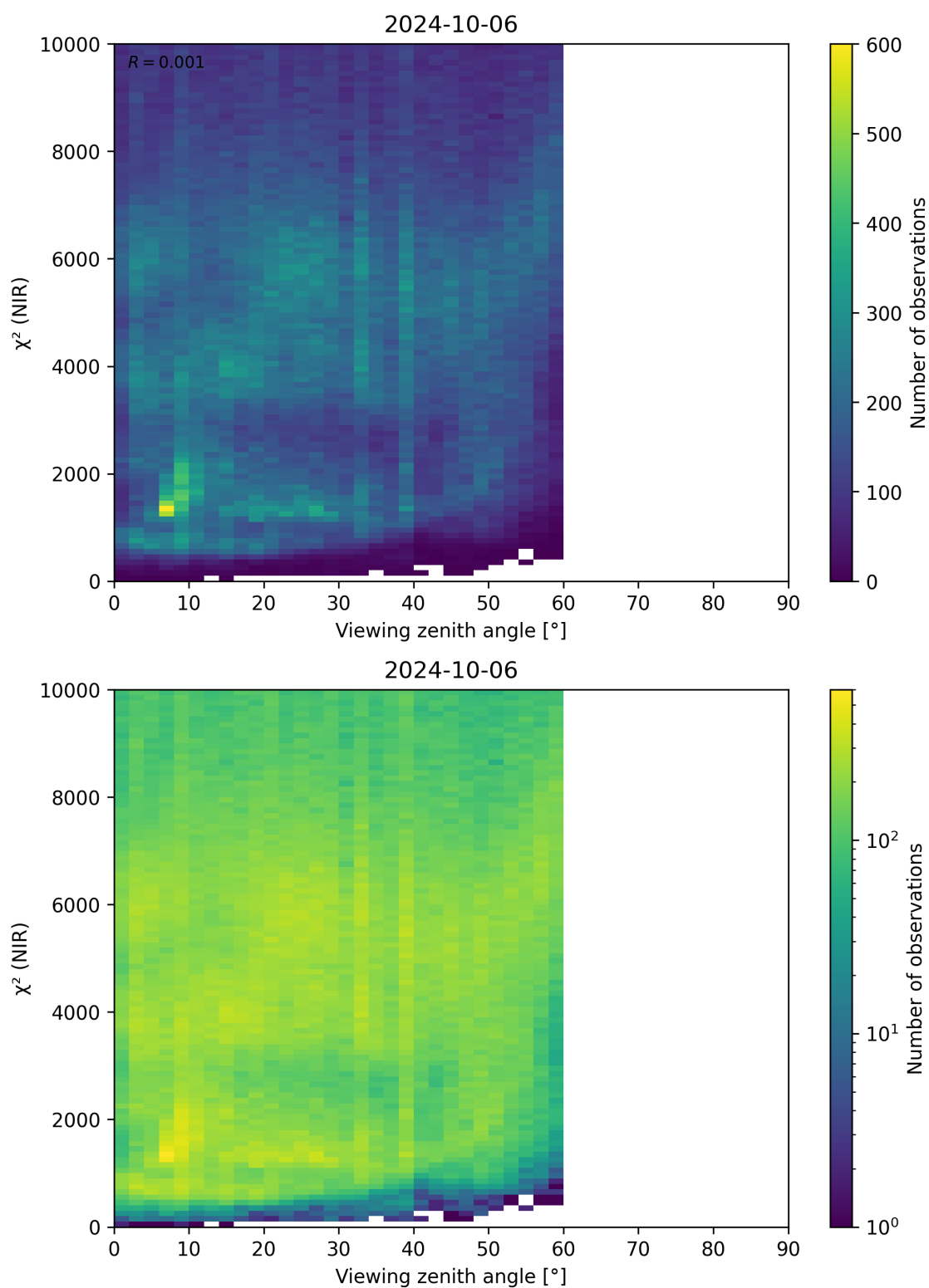
Figure 105: Scatter density plot of “Viewing zenith angle” against “ \chi^2 (NIR)” for 2024-10-05 to 2024-10-07.
