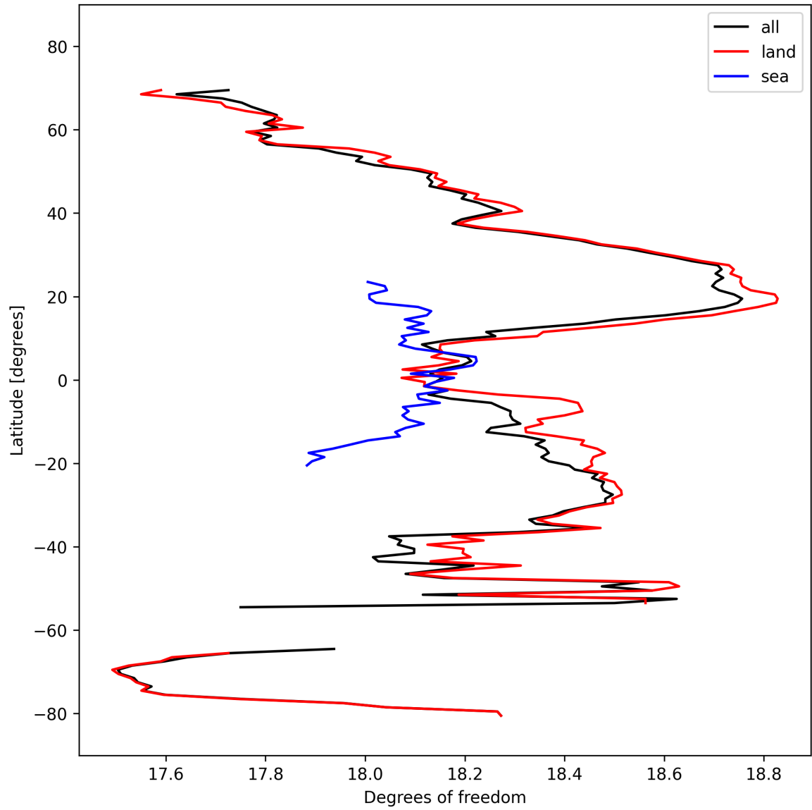
Figure 19: Zonal average of “Degrees of freedom” for 2024-10-05 to 2024-10-07.
