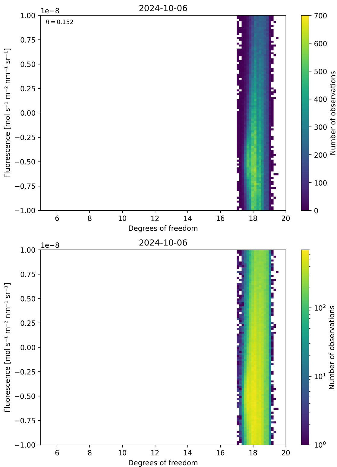
Figure 51: Scatter density plot of “Degrees of freedom” against “Fluorescence” for 2024-10-05 to 2024-10-07.
