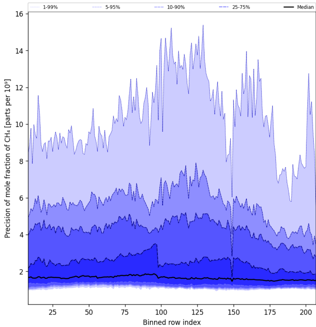
Figure 35: Along track statistics of "Precision of mole fraction of CH 4 " for 2024-10-05 to 2024-10-07
