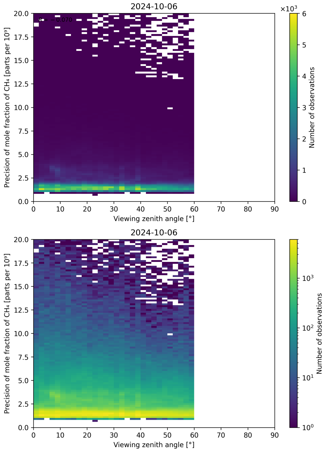
Figure 112: Scatter density plot of “Viewing zenith angle” against “Precision of mole fraction of CH 4 ” for 2024-10-05 to 2024-10-07.
