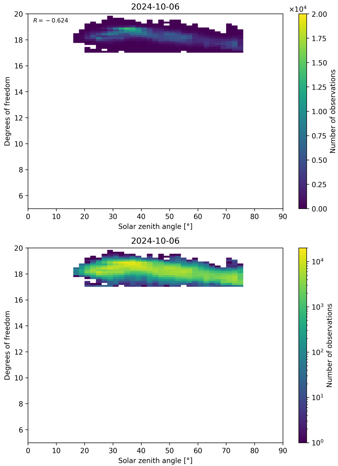
Figure 96: Scatter density plot of “Solar zenith angle” against “Degrees of freedom” for 2024-10-05 to 2024-10-07.
