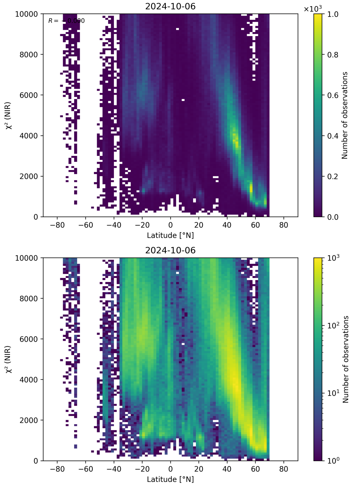
Figure 53: Scatter density plot of “Latitude” against “ \chi^2 (NIR)” for 2024-10-05 to 2024-10-07.
