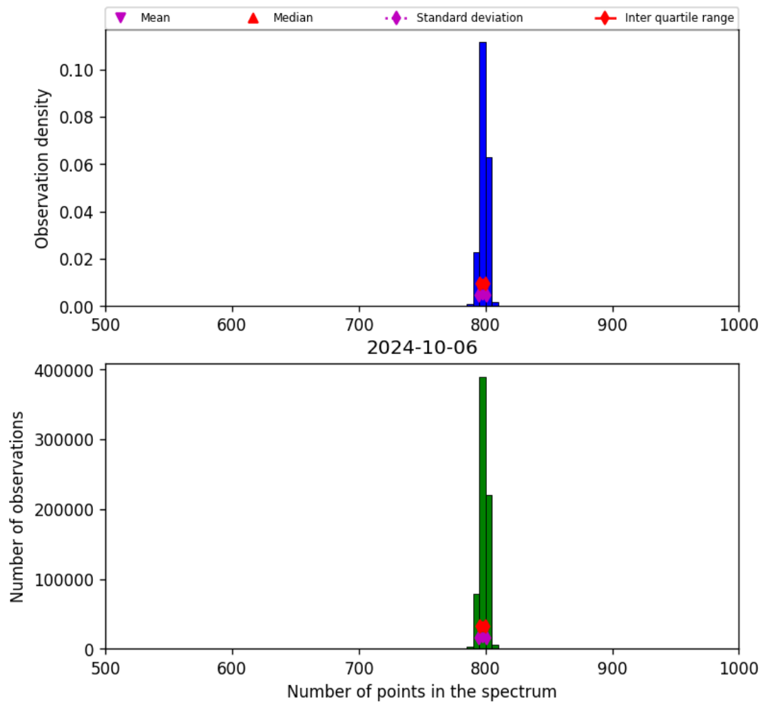
Figure 26: Histogram of “Number of points in the spectrum” for 2024-10-05 to 2024-10-07
