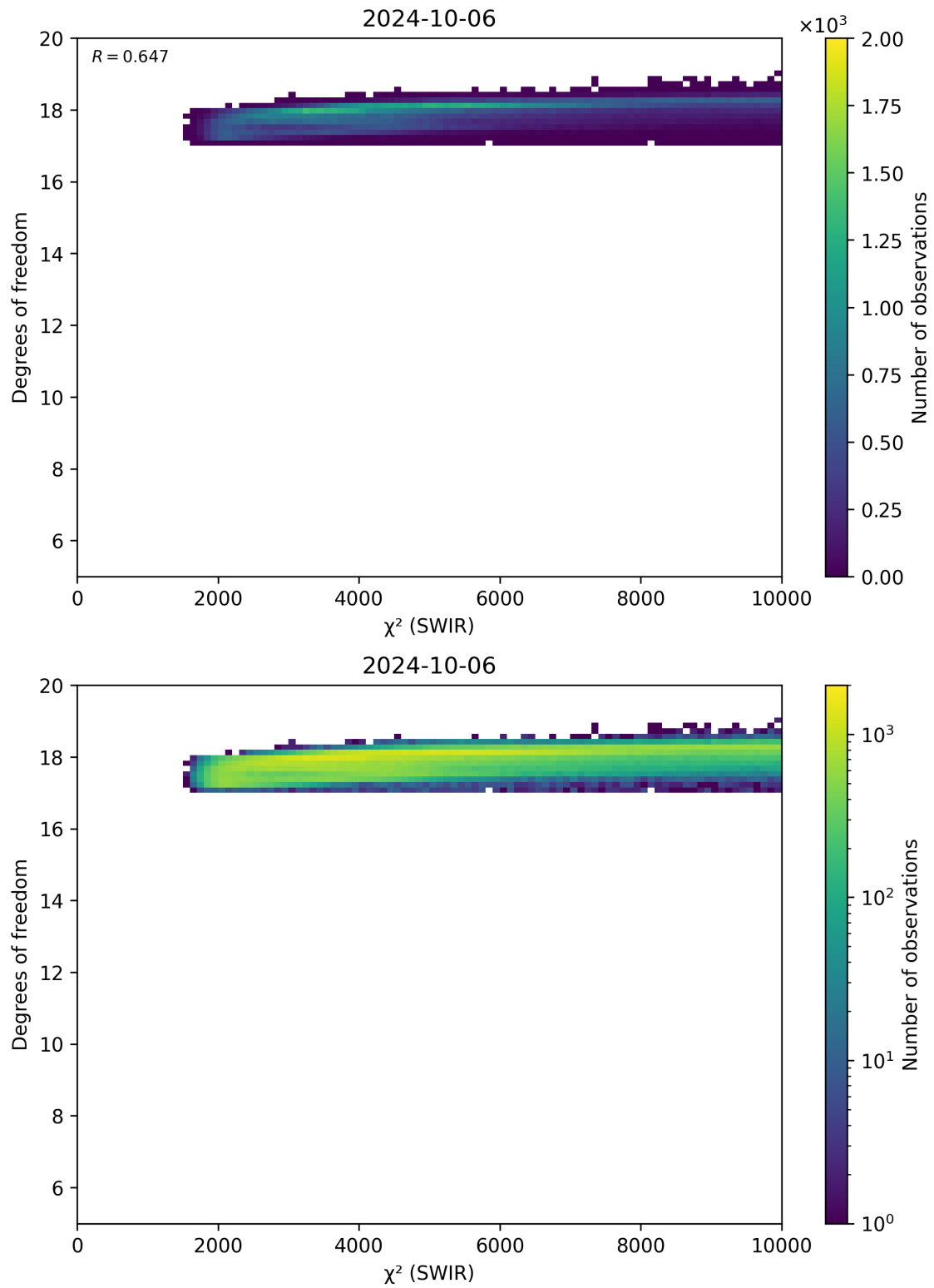
Figure 48: Scatter density plot of " \chi^2 (SWIR)" against "Degrees of freedom" for 2024-10-05 to 2024-10-07.
