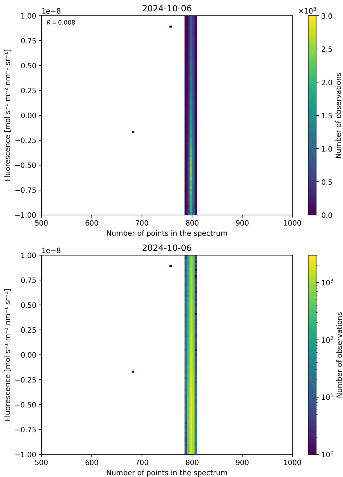
Figure 91: Scatter density plot of “Number of points in the spectrum” against “Fluorescence” for 2024-10-05 to 2024-10-07.
