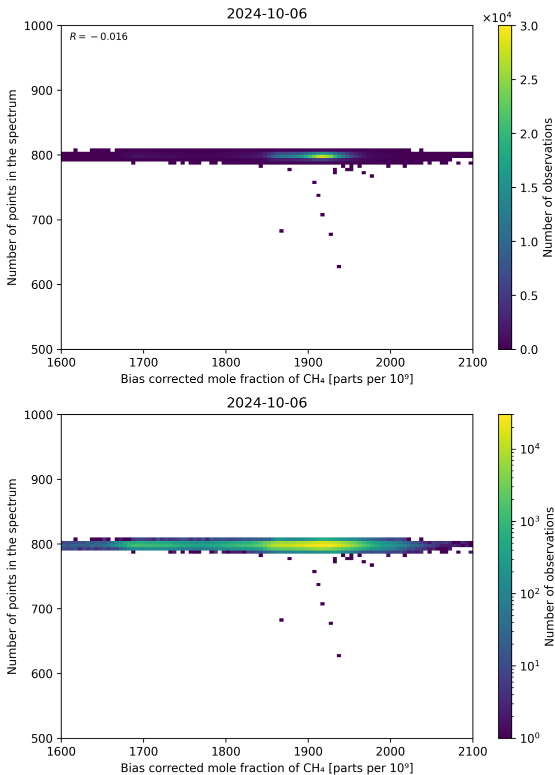
Figure 68: Scatter density plot of “Bias corrected mole fraction of CH 4 ” against “Number of points in the spectrum” for 2024-10-05 to 2024-10-07.
