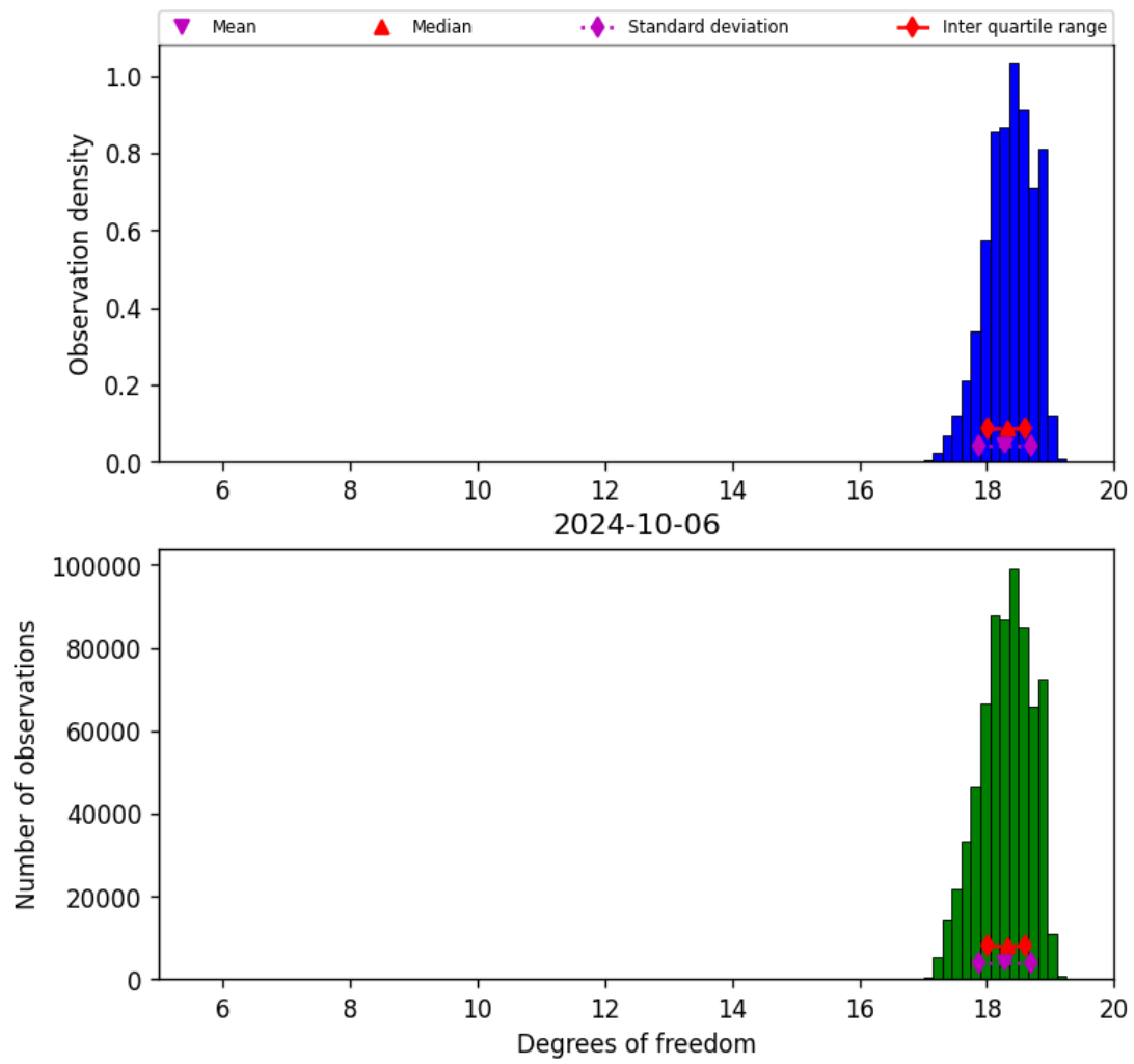
Figure 30: Histogram of “Degrees of freedom” for 2024-10-05 to 2024-10-07
