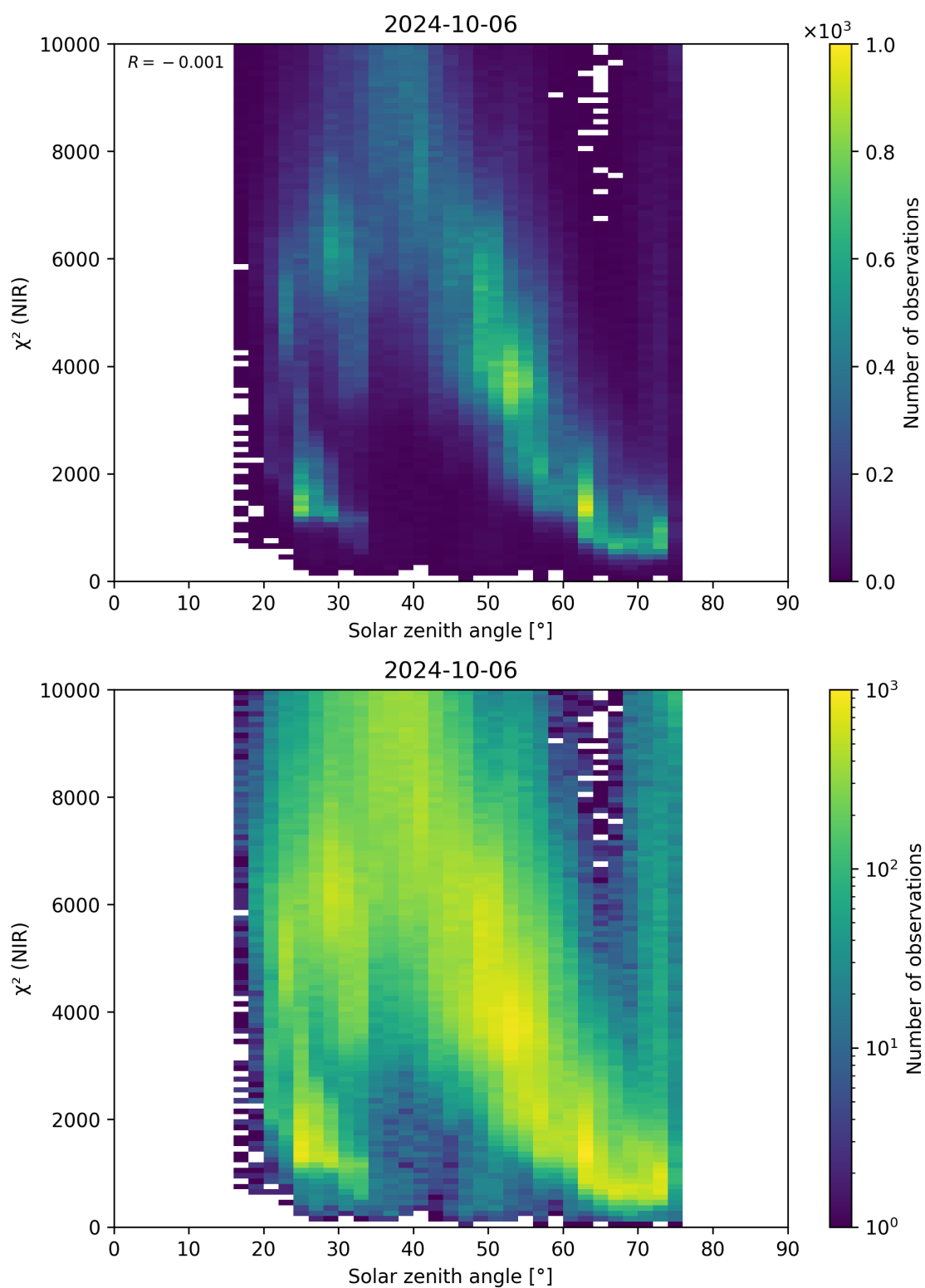
Figure 94: Scatter density plot of “Solar zenith angle” against “ \chi^2 (NIR)” for 2024-10-05 to 2024-10-07.
