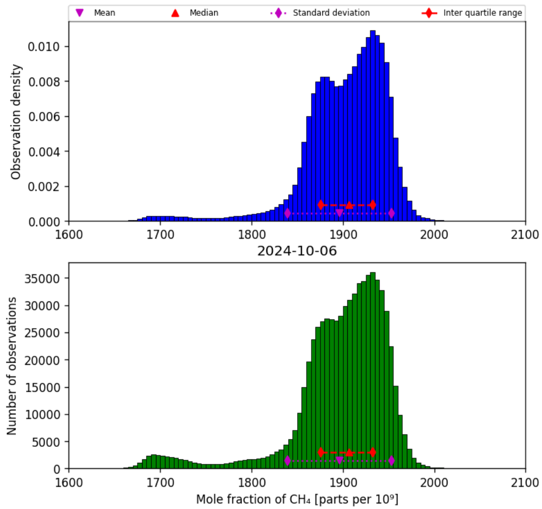
Figure 23: Histogram of “Mole fraction of CH 4 ” for 2024-10-05 to 2024-10-07
