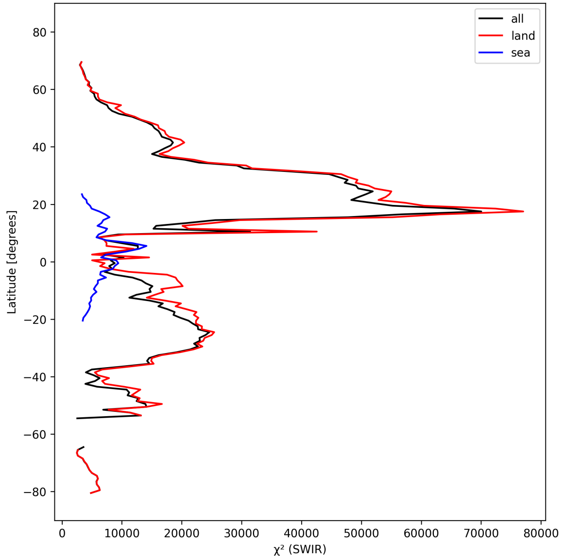
Figure 17: Zonal average of “ \chi^2 (SWIR)” for 2024-10-05 to 2024-10-07.
