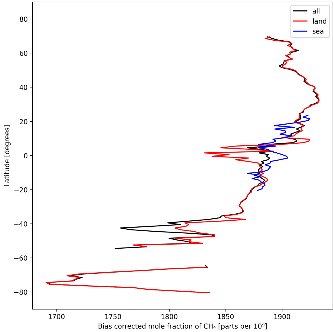
Figure 14: Zonal average of “Bias corrected mole fraction of \text{CH}_4 ” for 2024-10-05 to 2024-10-07.
