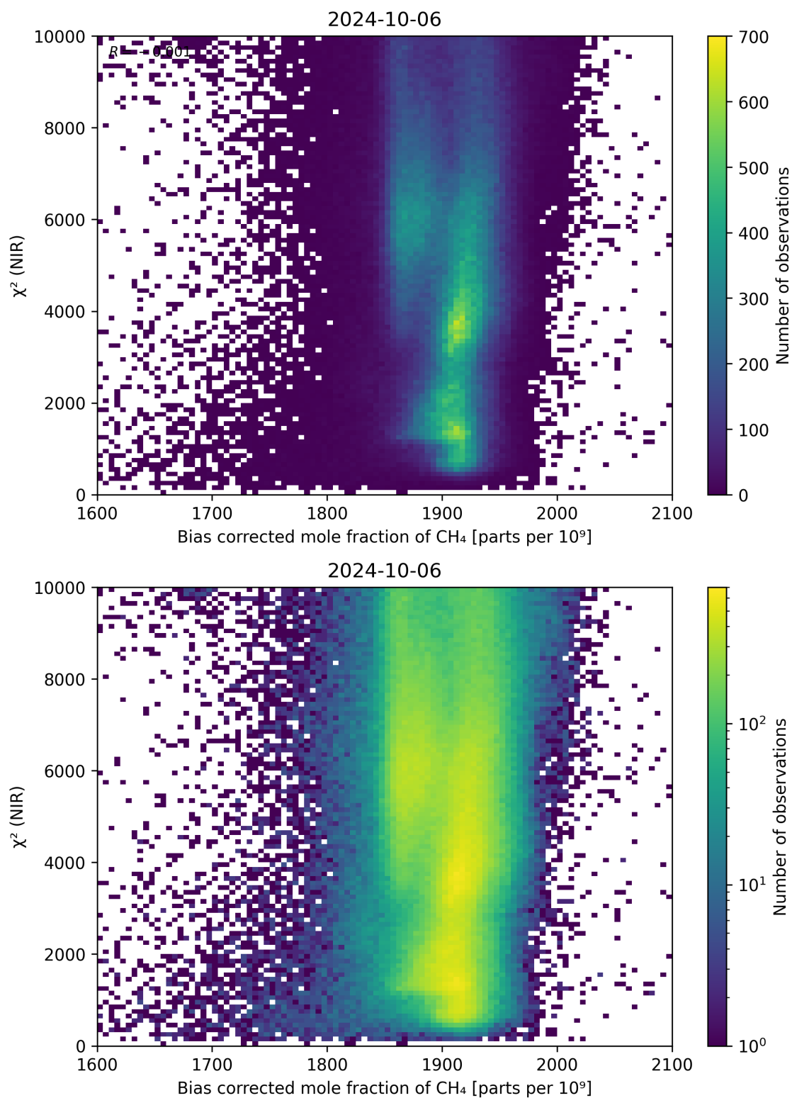
Figure 63: Scatter density plot of “Bias corrected mole fraction of \text{CH}_4 ” against “ \chi^2 (NIR)” for 2024-10-05 to 2024-10-07.
