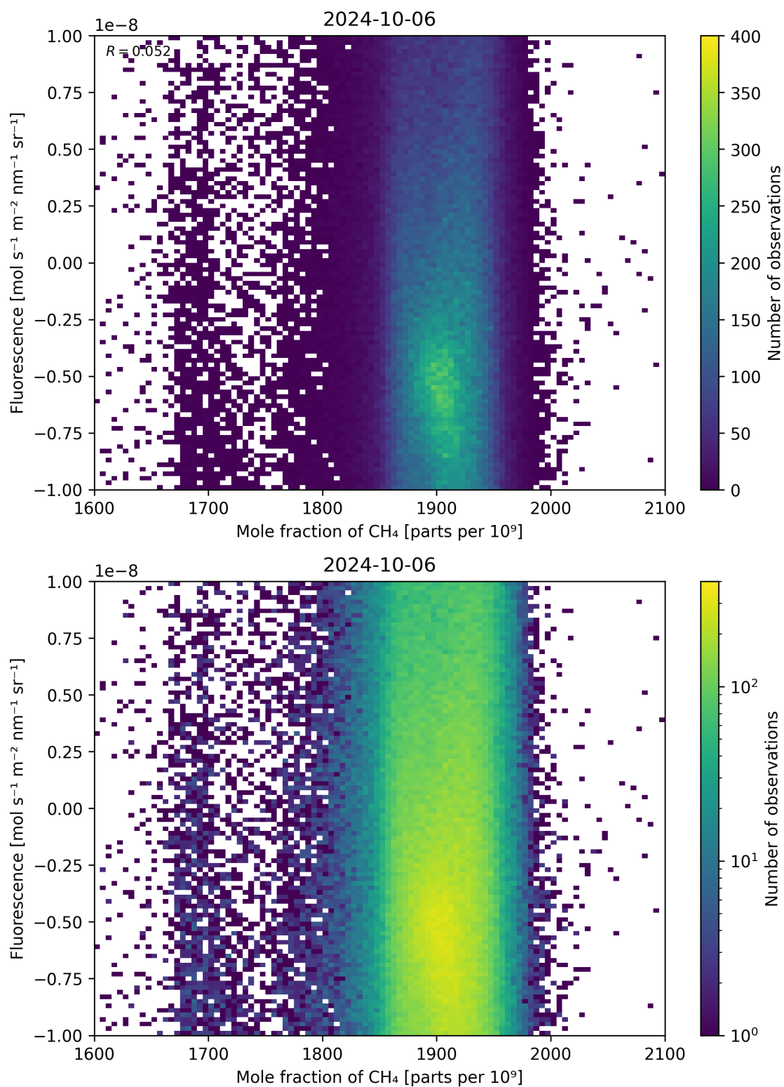
Figure 73: Scatter density plot of “Mole fraction of \text{CH}_4 ” against “Fluorescence” for 2024-10-05 to 2024-10-07.
