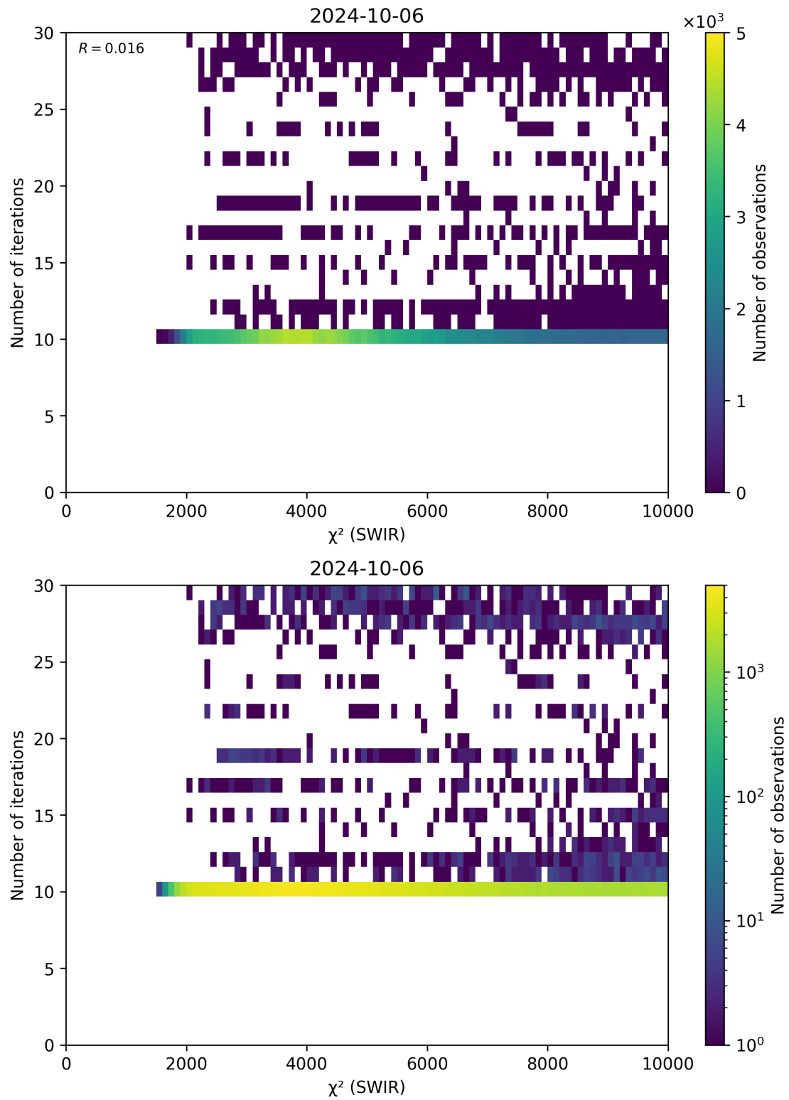
Figure 50: Scatter density plot of “ \chi^2 (SWIR)” against “Number of iterations” for 2024-10-05 to 2024-10-07.
