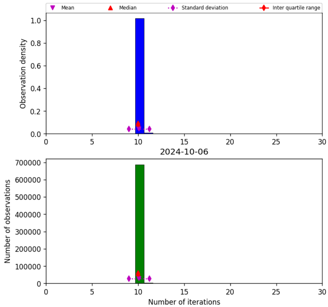
Figure 31: Histogram of “Number of iterations” for 2024-10-05 to 2024-10-07
