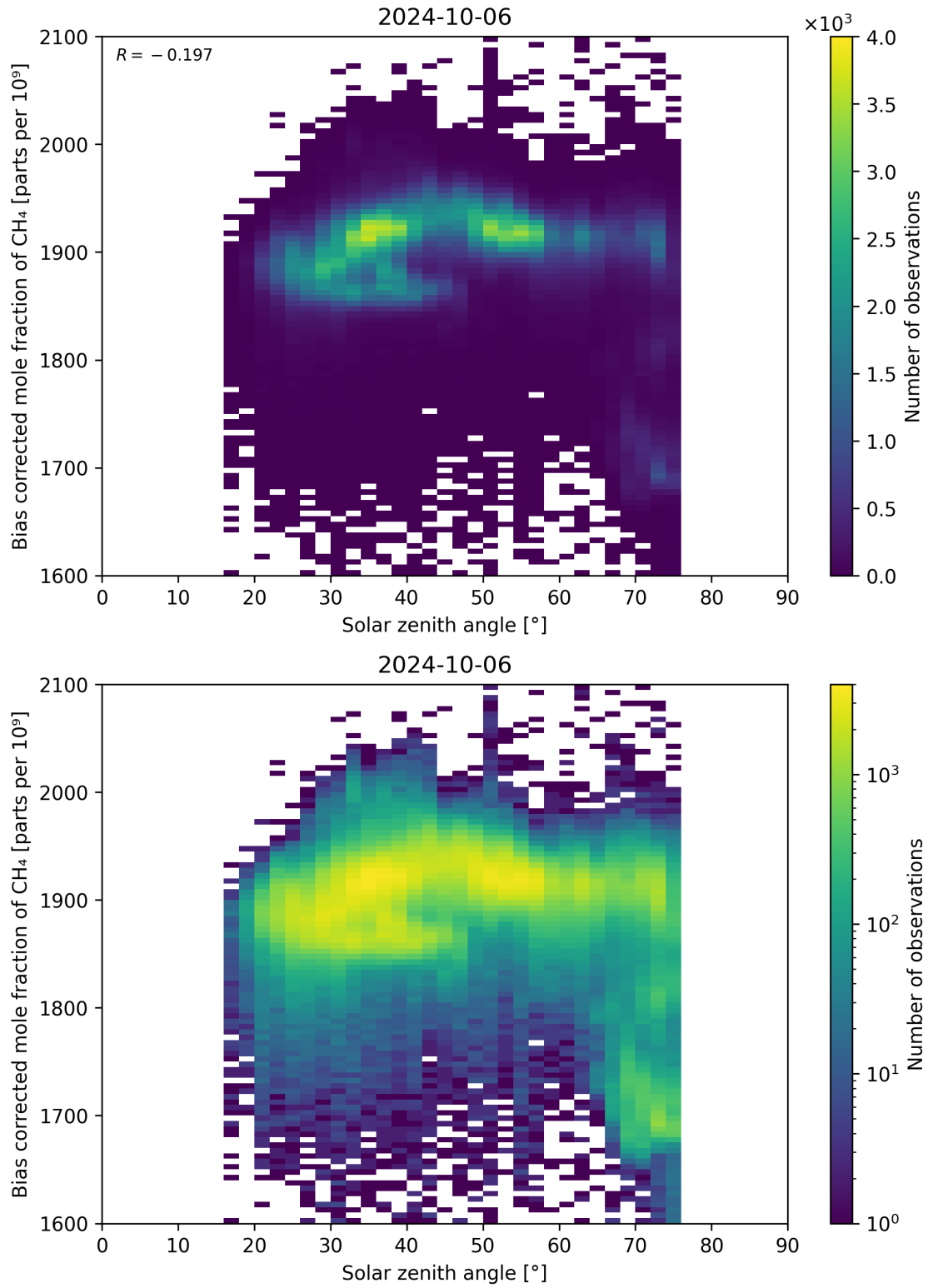
Figure 100: Scatter density plot of “Solar zenith angle” against “Bias corrected mole fraction of \text{CH}_4 ” for 2024-10-05 to 2024-10-07.
