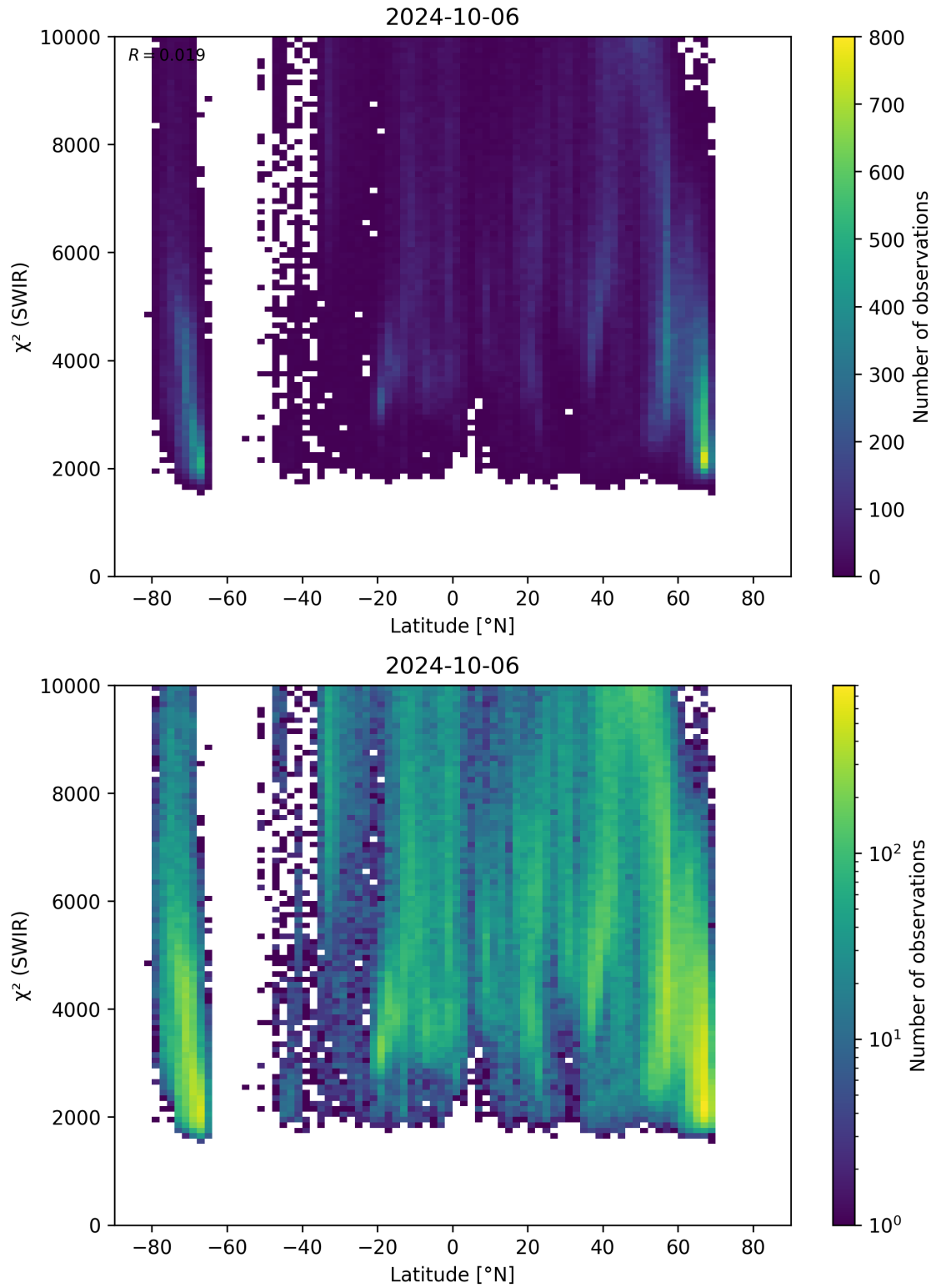
Figure 54: Scatter density plot of “Latitude” against “ \chi^2 (SWIR)” for 2024-10-05 to 2024-10-07.
