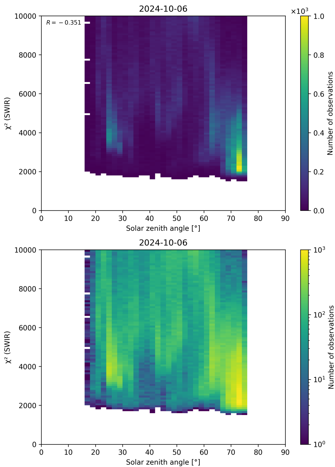
Figure 95: Scatter density plot of “Solar zenith angle” against “ \chi^2 (SWIR)” for 2024-10-05 to 2024-10-07.
