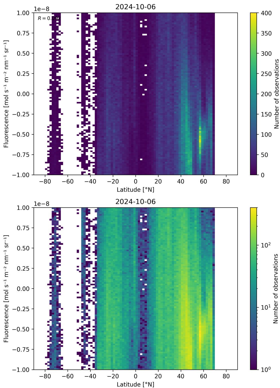
Figure 56: Scatter density plot of “Latitude” against “Fluorescence” for 2024-10-05 to 2024-10-07.
