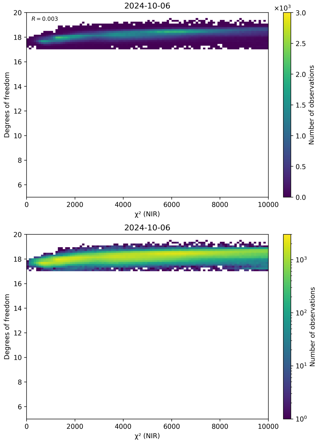
Figure 44: Scatter density plot of “ \chi^2 (NIR)” against “Degrees of freedom” for 2024-10-05 to 2024-10-07.
