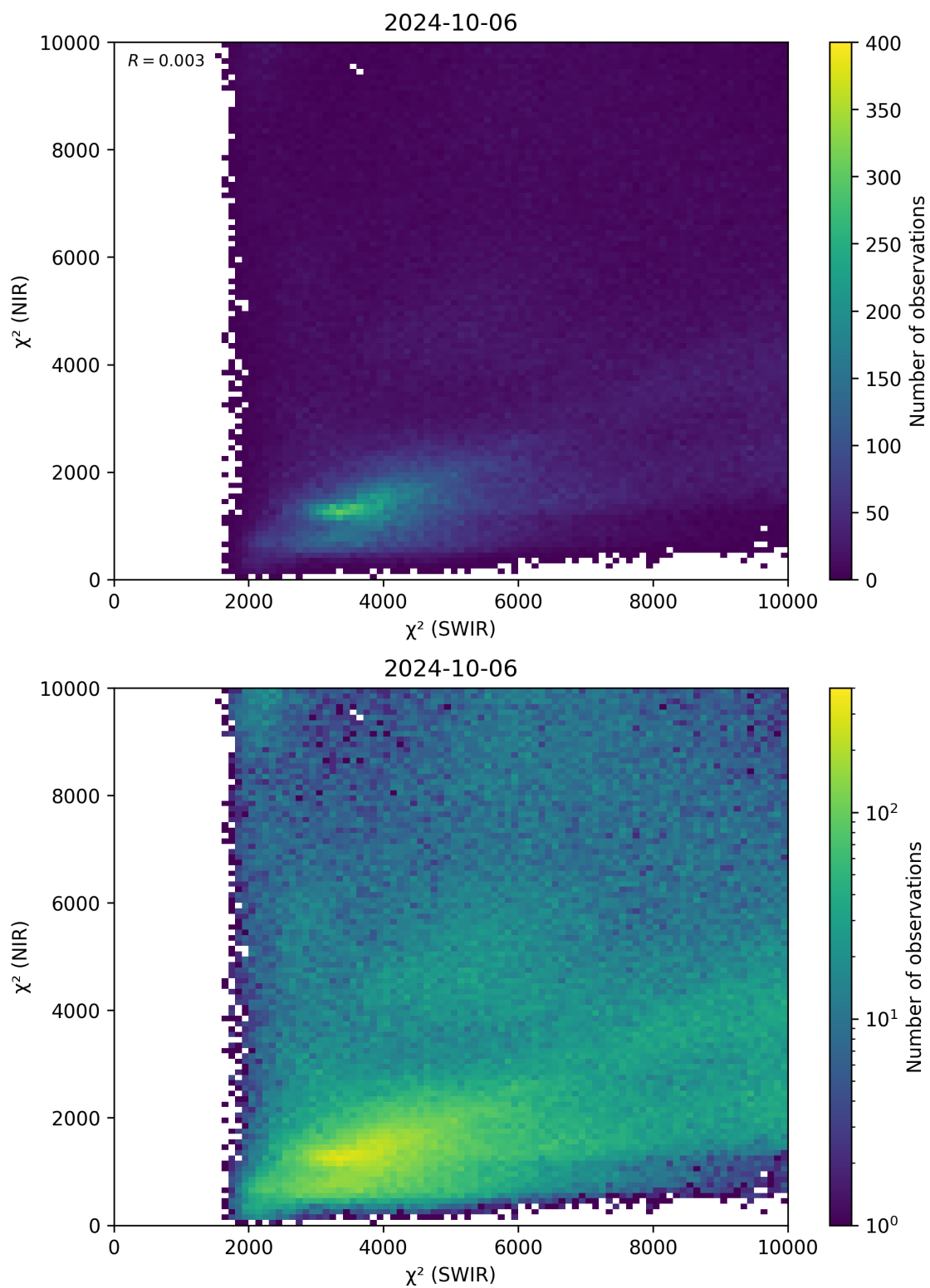
Figure 47: Scatter density plot of “ \chi^2 (SWIR)” against “ \chi^2 (NIR)” for 2024-10-05 to 2024-10-07.
