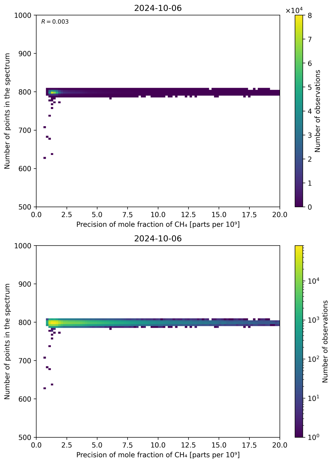
Figure 84: Scatter density plot of “Precision of mole fraction of CH 4 ” against “Number of points in the spectrum” for 2024-10-05 to 2024-10-07.
