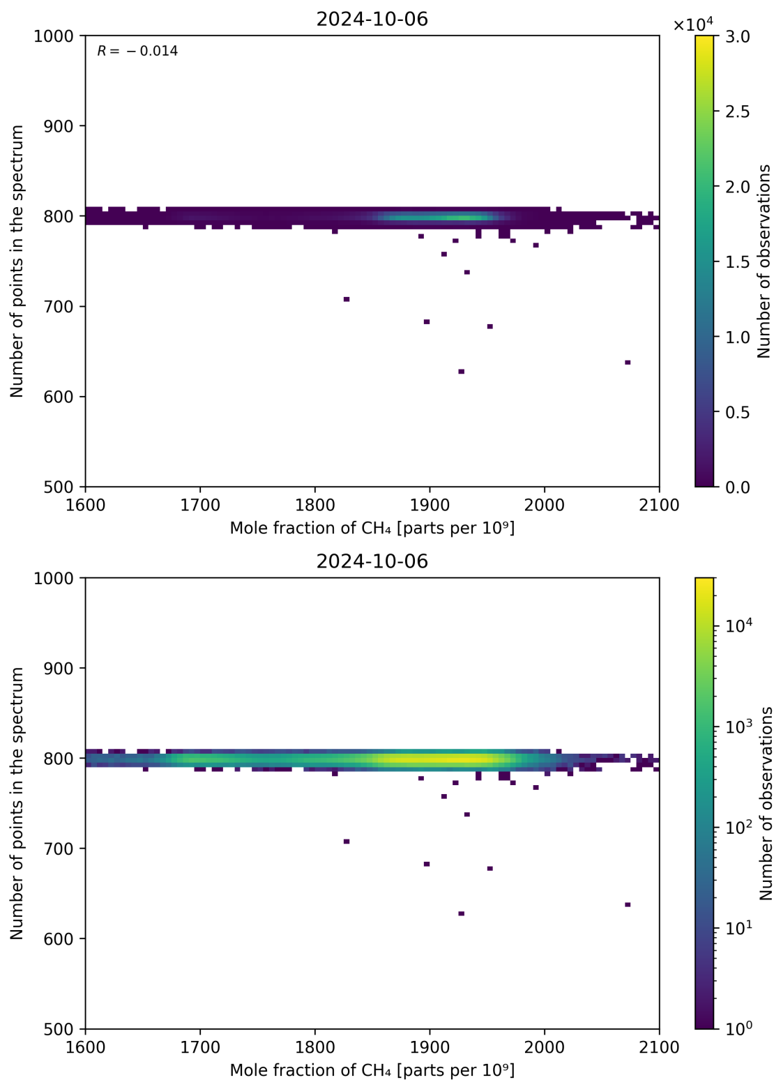
Figure 77: Scatter density plot of “Mole fraction of CH 4 ” against “Number of points in the spectrum” for 2024-10-05 to 2024-10-07.
