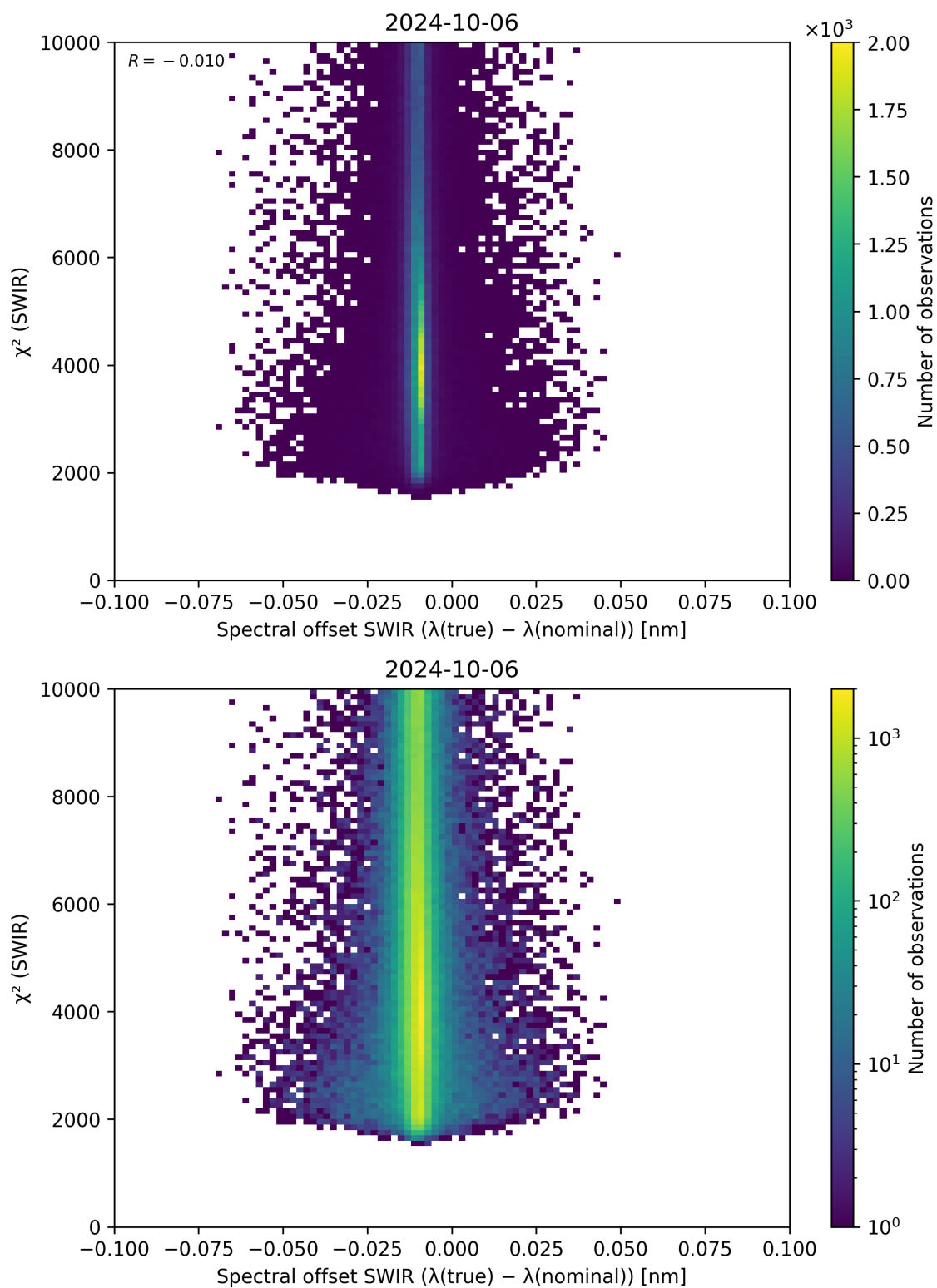
Figure 118: Scatter density plot of “Spectral offset SWIR ( \lambda_{\text{true}} - \lambda_{\text{nominal}} )” against “ \chi^2 (SWIR)” for 2024-10-05 to 2024-10-07.
