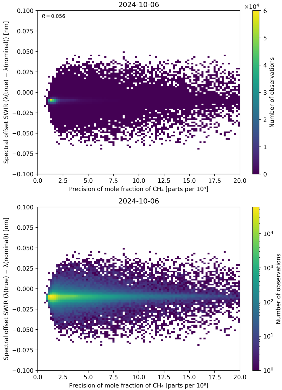
Figure 85: Scatter density plot of “Precision of mole fraction of CH 4 ” against “Spectral offset SWIR ( \lambda_{\text{true}} - \lambda_{\text{nominal}} )” for 2024-10-05 to 2024-10-07.
