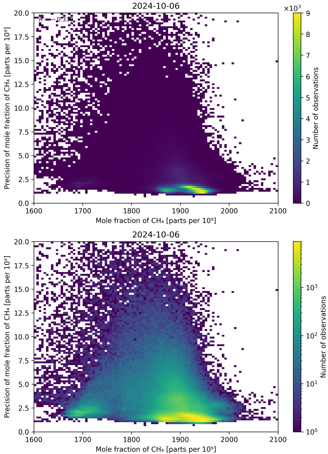
Figure 75: Scatter density plot of “Mole fraction of CH 4 ” against “Precision of mole fraction of CH 4 ” for 2024-10-05 to 2024-10-07.
