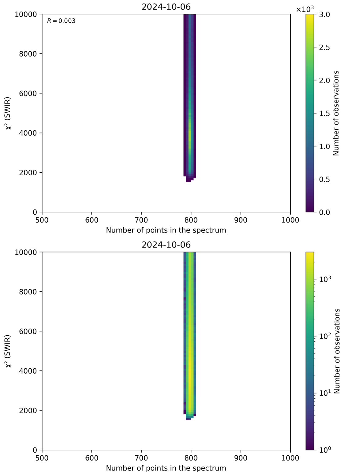
Figure 89: Scatter density plot of “Number of points in the spectrum” against “ \chi^2 (SWIR)” for 2024-10-05 to 2024-10-07.
