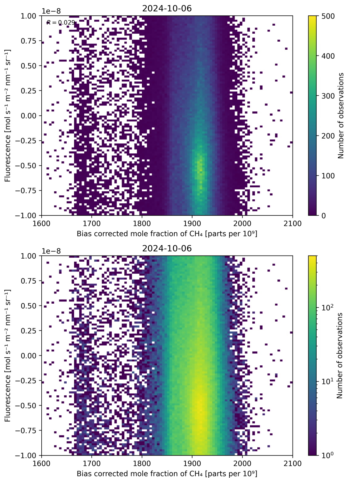
Figure 66: Scatter density plot of “Bias corrected mole fraction of CH 4 ” against “Fluorescence” for 2024-10-05 to 2024-10-07.
