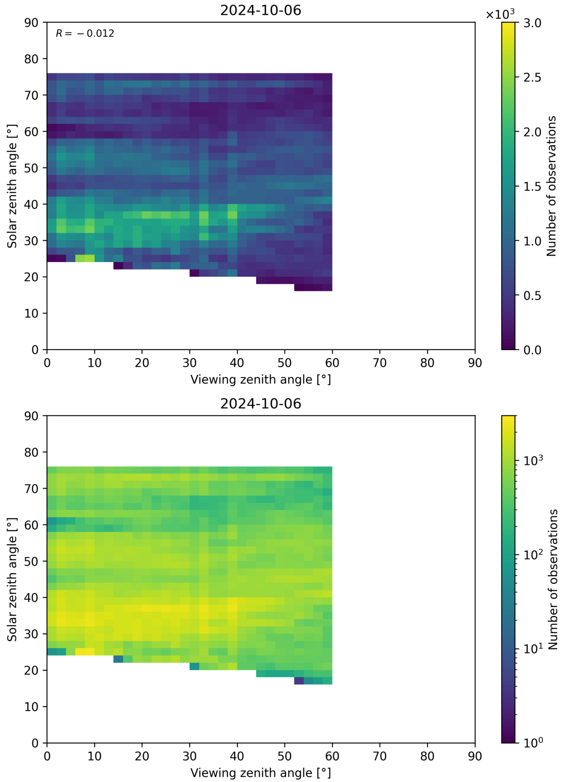
Figure 115: Scatter density plot of “Viewing zenith angle” against “Solar zenith angle” for 2024-10-05 to 2024-10-07.
