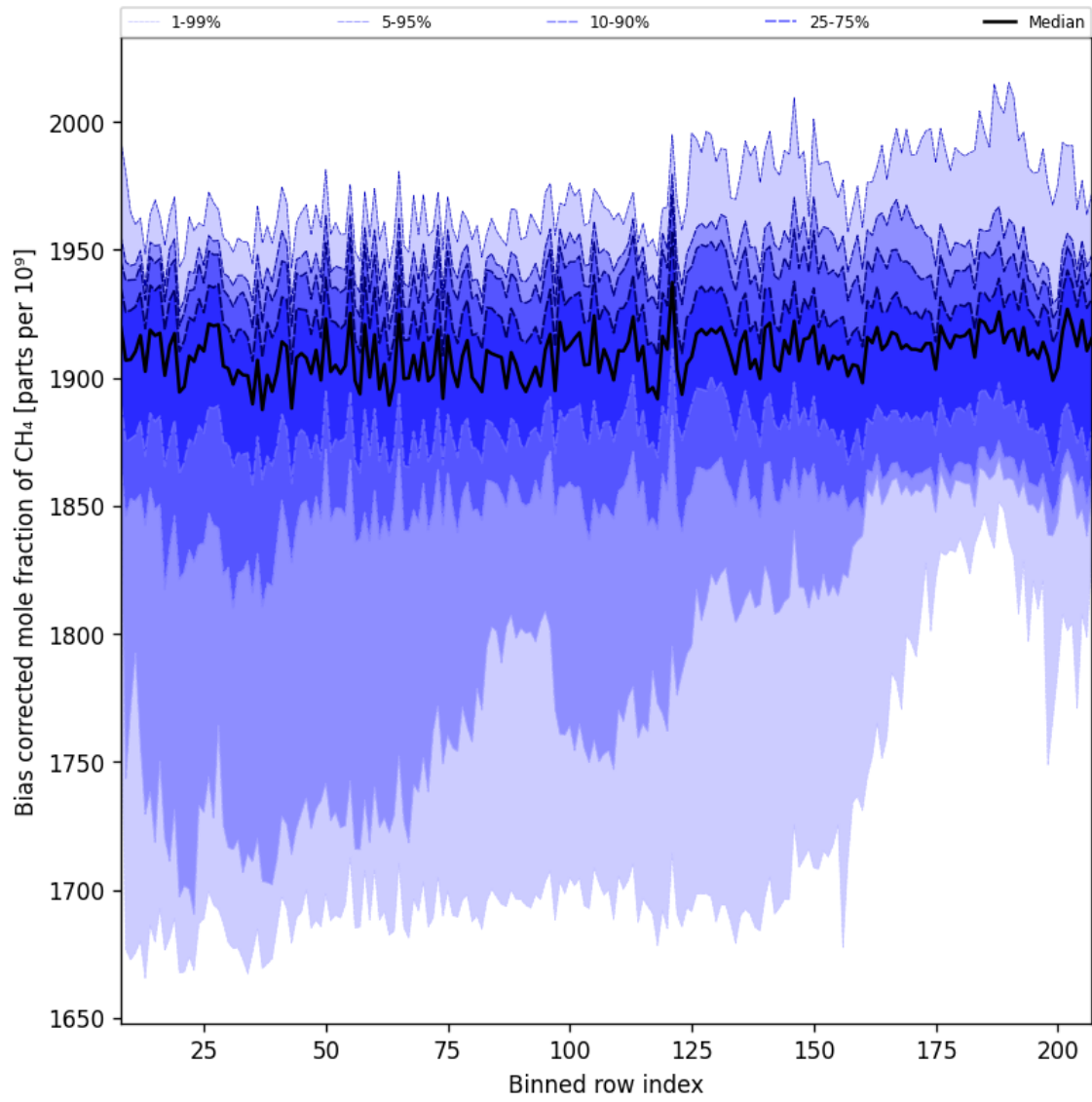
Figure 36: Along track statistics of “Bias corrected mole fraction of CH 4 ” for 2024-10-05 to 2024-10-07
