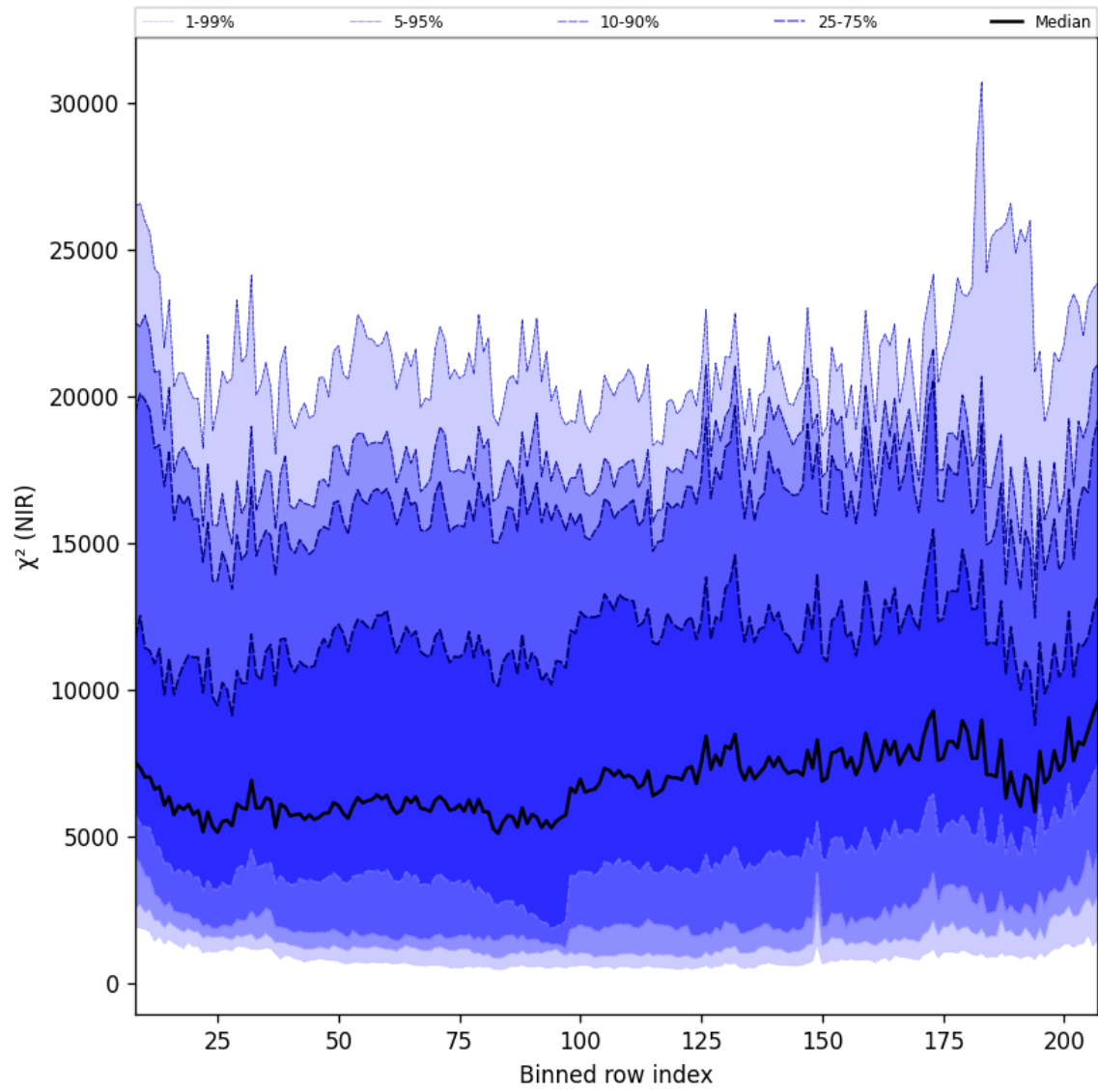
Figure 40: Along track statistics of “ \chi^2 (NIR)” for 2024-10-05 to 2024-10-07
