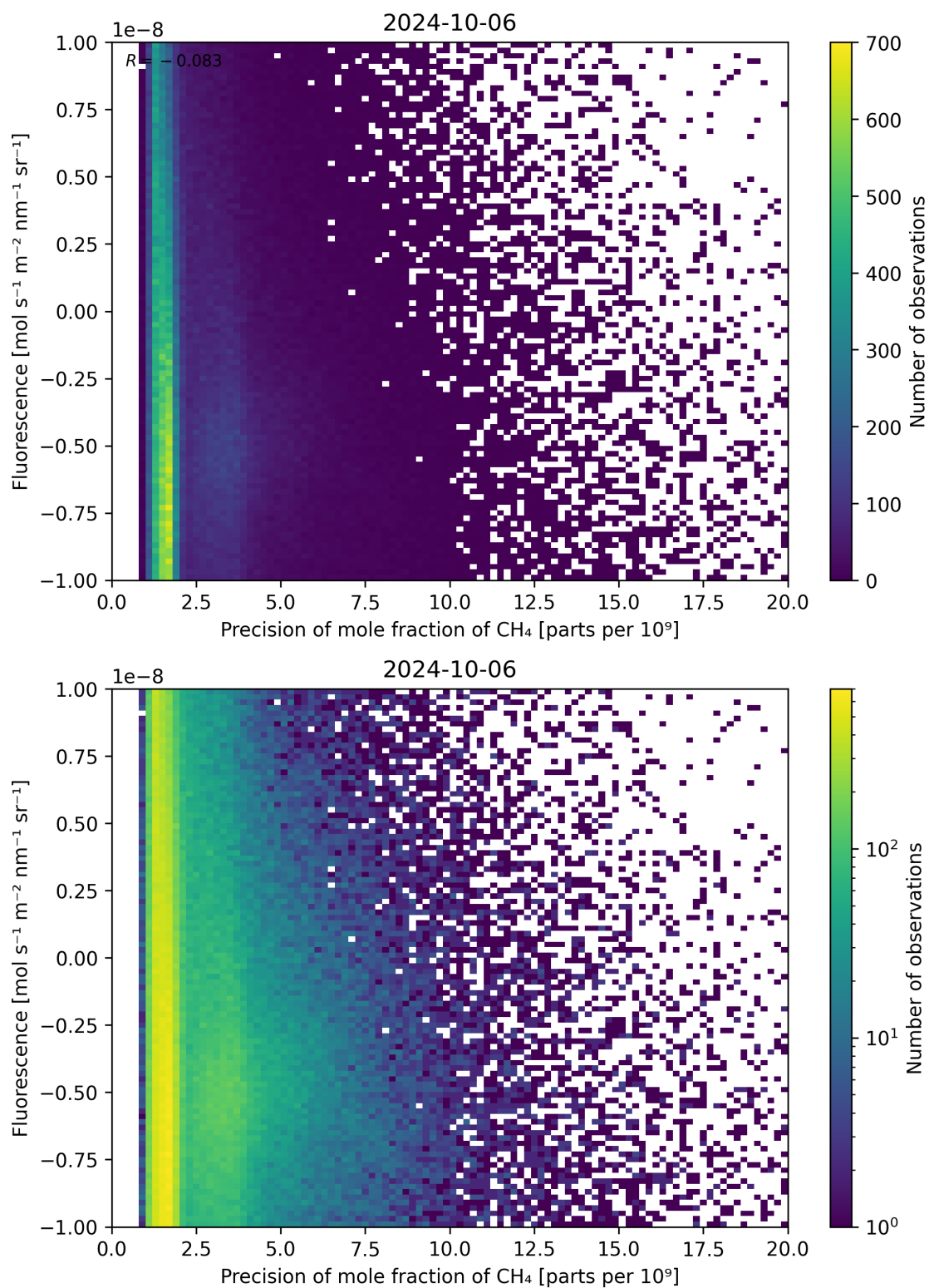
Figure 81: Scatter density plot of “Precision of mole fraction of \text{CH}_4 ” against “Fluorescence” for 2024-10-05 to 2024-10-07.
