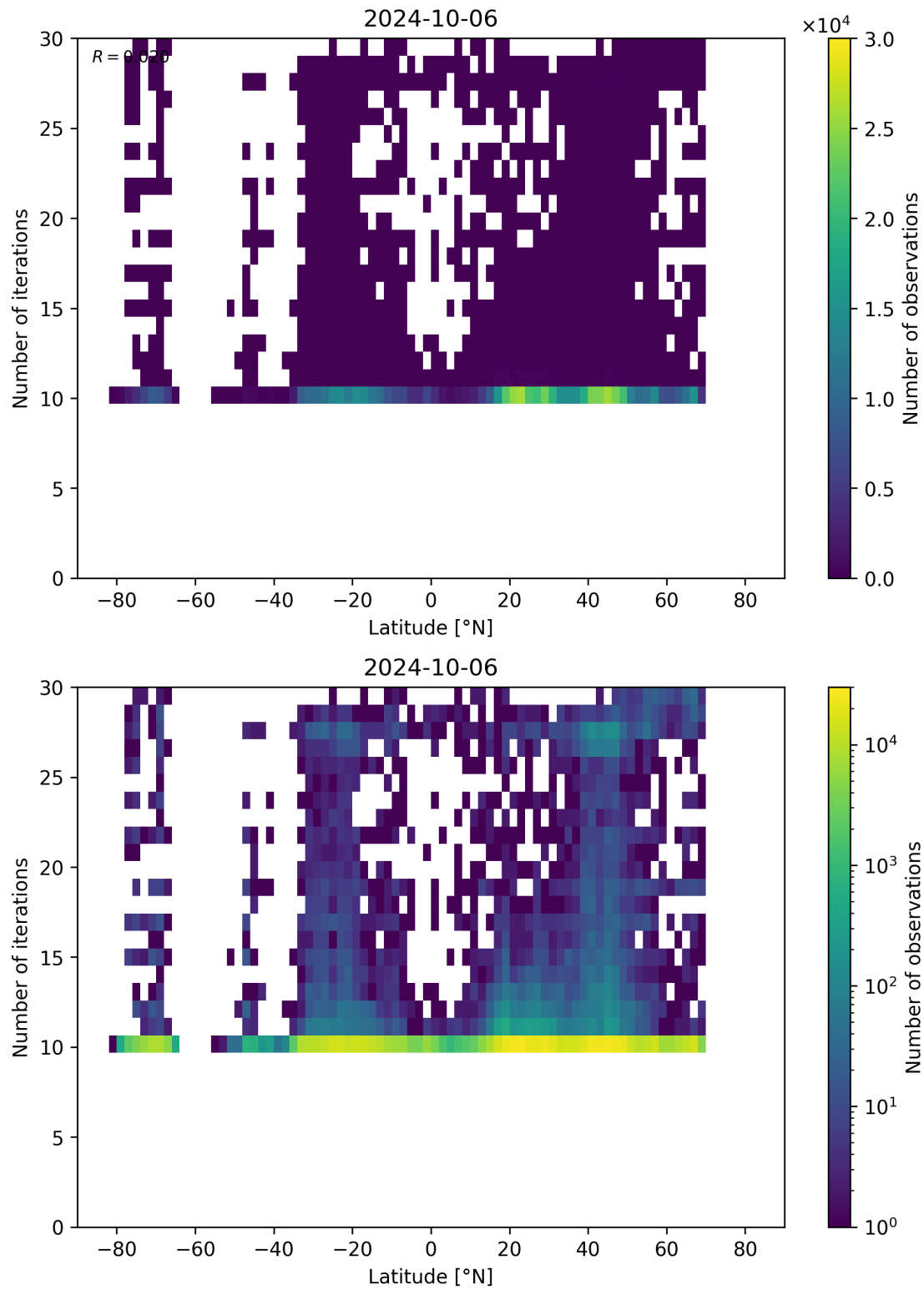
Figure 60: Scatter density plot of “Latitude” against “Number of iterations” for 2024-10-05 to 2024-10-07.
