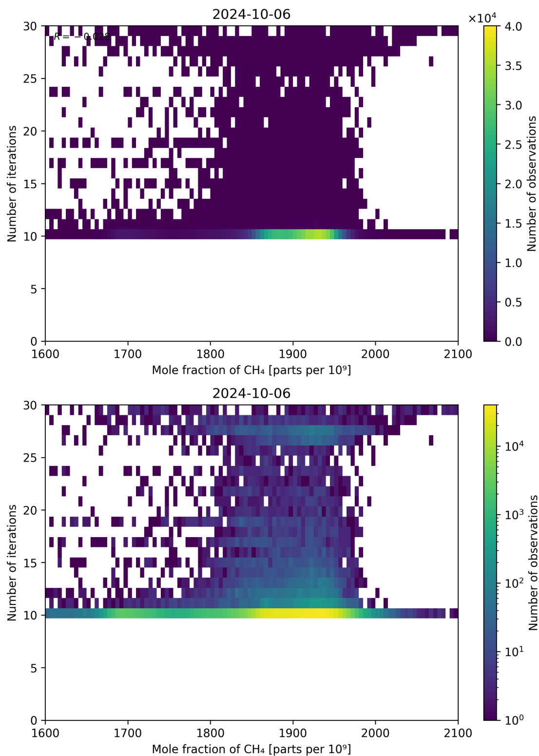
Figure 76: Scatter density plot of “Mole fraction of CH 4 ” against “Number of iterations” for 2024-10-05 to 2024-10-07.
