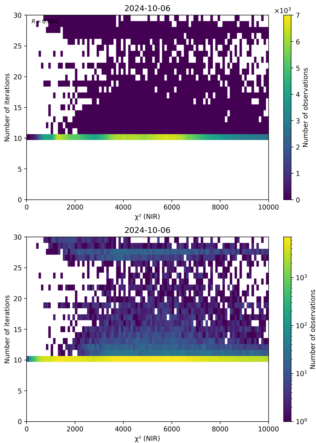
Figure 46: Scatter density plot of “ \chi^2 (NIR)” against “Number of iterations” for 2024-10-05 to 2024-10-07.
