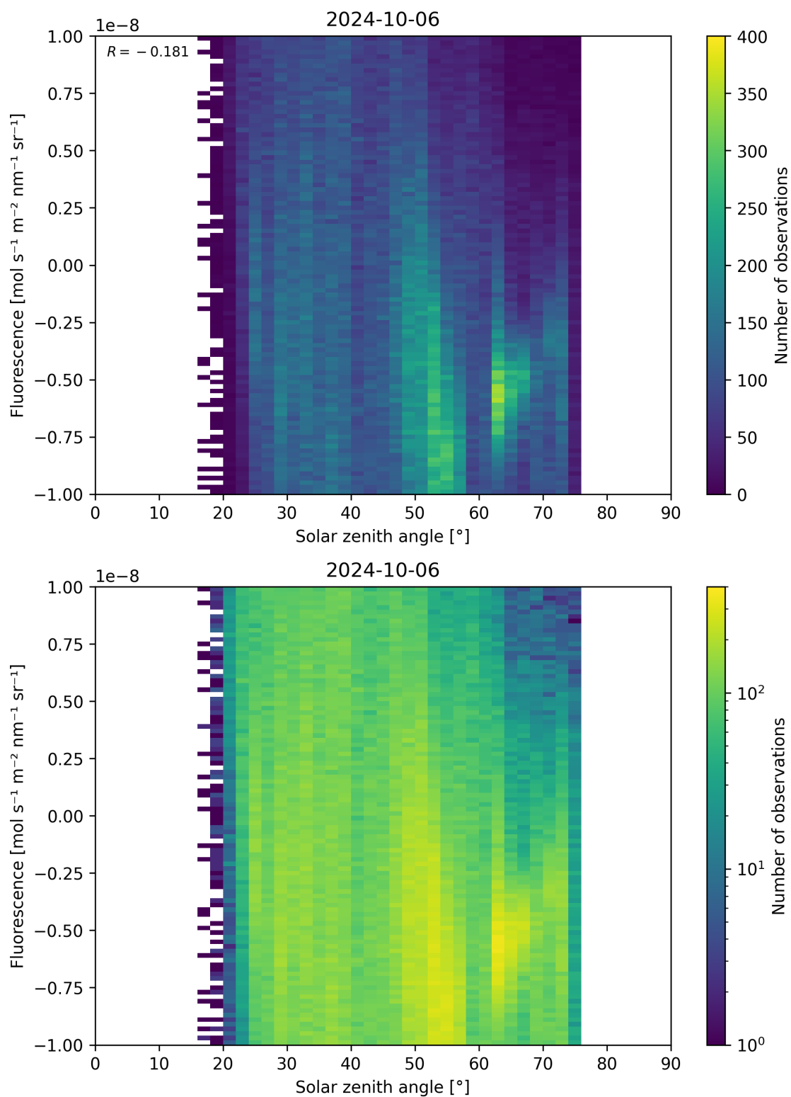
Figure 97: Scatter density plot of “Solar zenith angle” against “Fluorescence” for 2024-10-05 to 2024-10-07.
