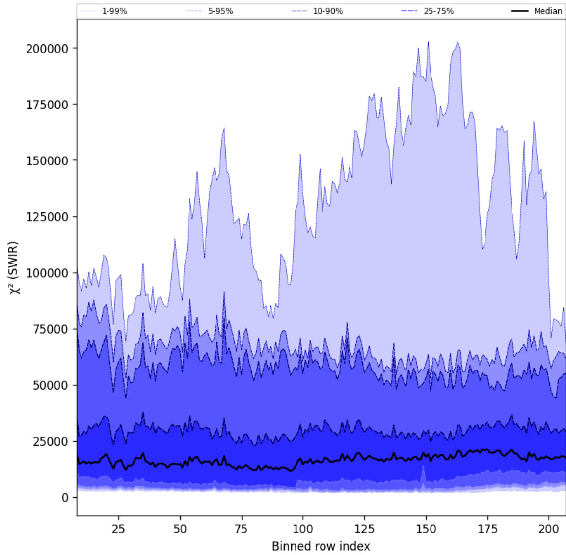
Figure 39: Along track statistics of " \chi^2 (SWIR)" for 2024-10-05 to 2024-10-07
