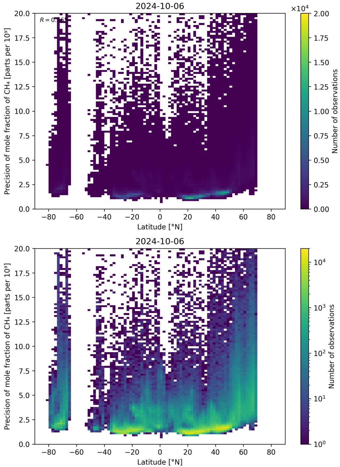
Figure 59: Scatter density plot of “Latitude” against “Precision of mole fraction of \text{CH}_4 ” for 2024-10-05 to 2024-10-07.
