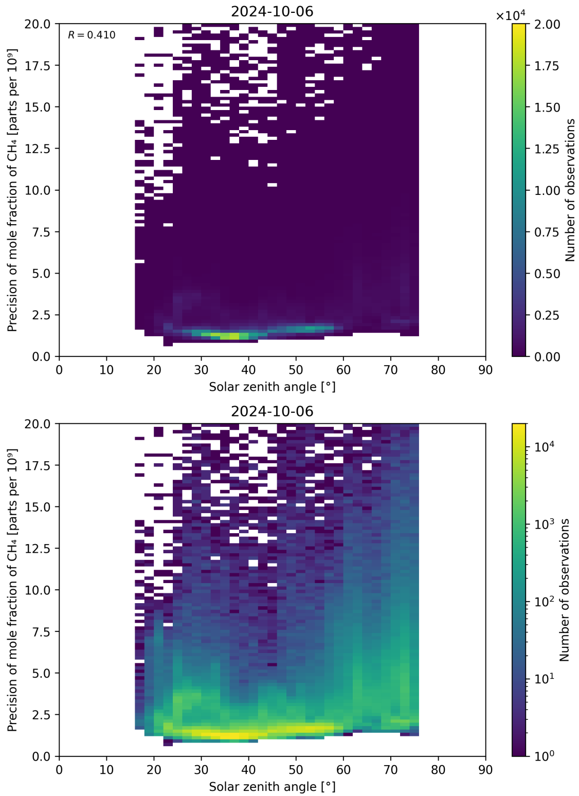
Figure 101: Scatter density plot of “Solar zenith angle” against “Precision of mole fraction of \text{CH}_4 ” for 2024-10-05 to 2024-10-07.
