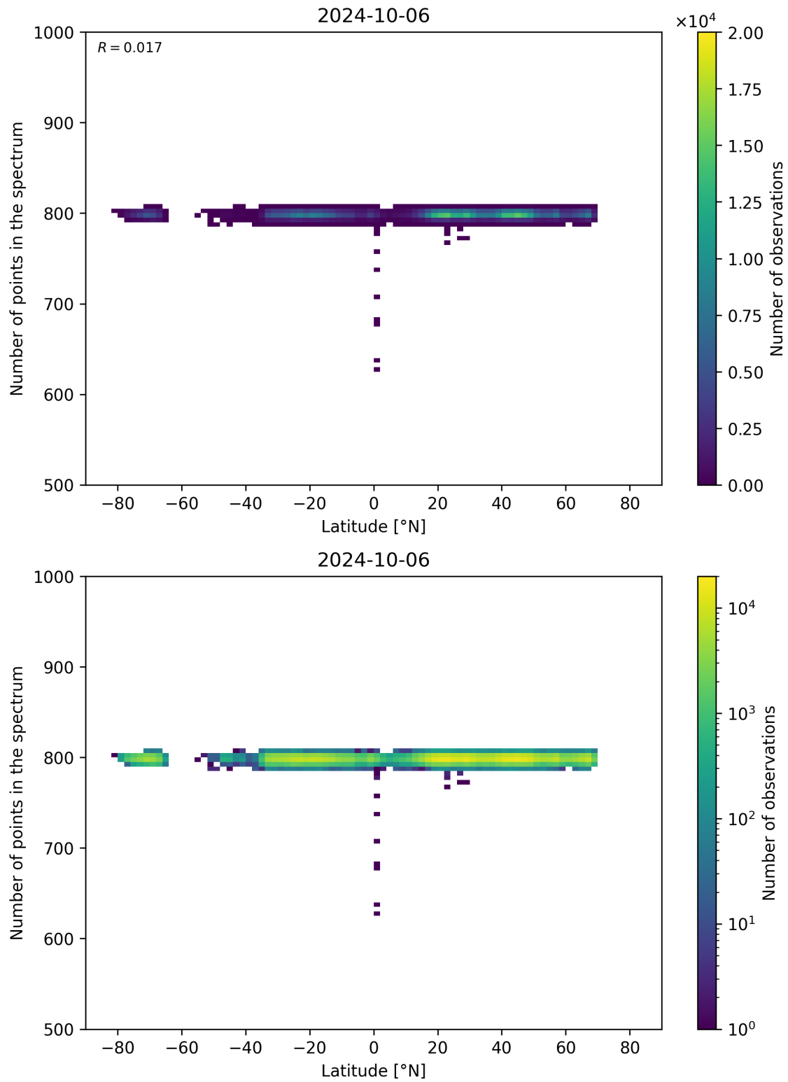
Figure 61: Scatter density plot of “Latitude” against “Number of points in the spectrum” for 2024-10-05 to 2024-10-07.
