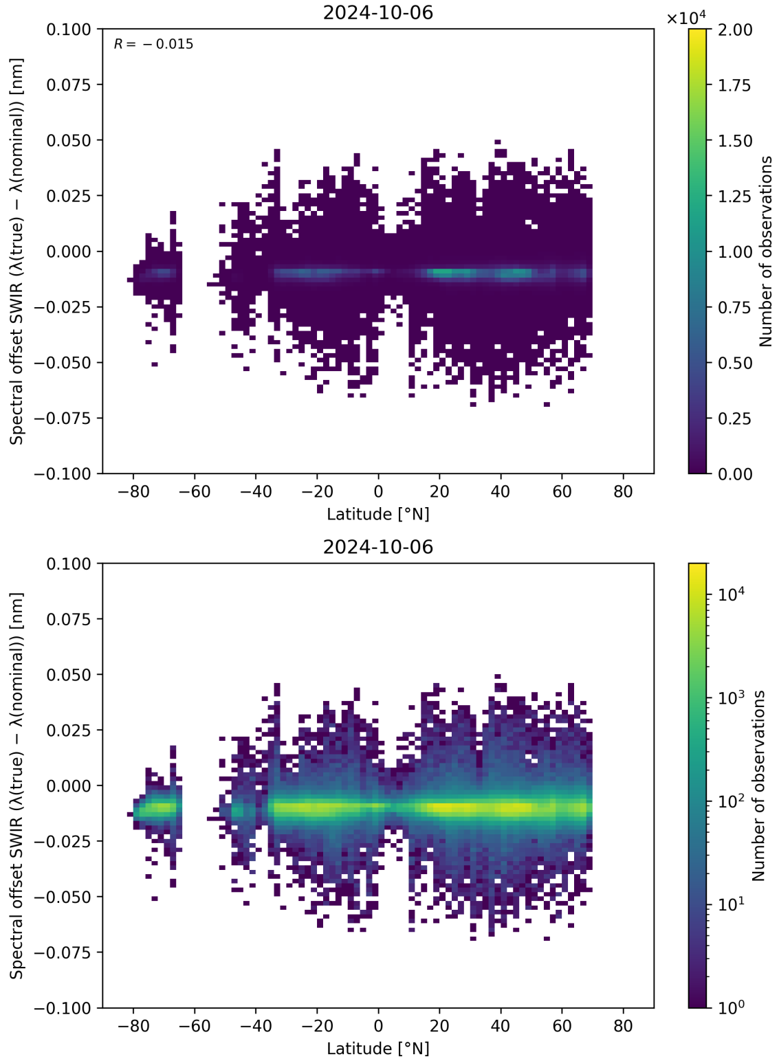
Figure 62: Scatter density plot of “Latitude” against “Spectral offset SWIR ( \lambda_{\text{true}} - \lambda_{\text{nominal}} )” for 2024-10-05 to 2024-10-07.
