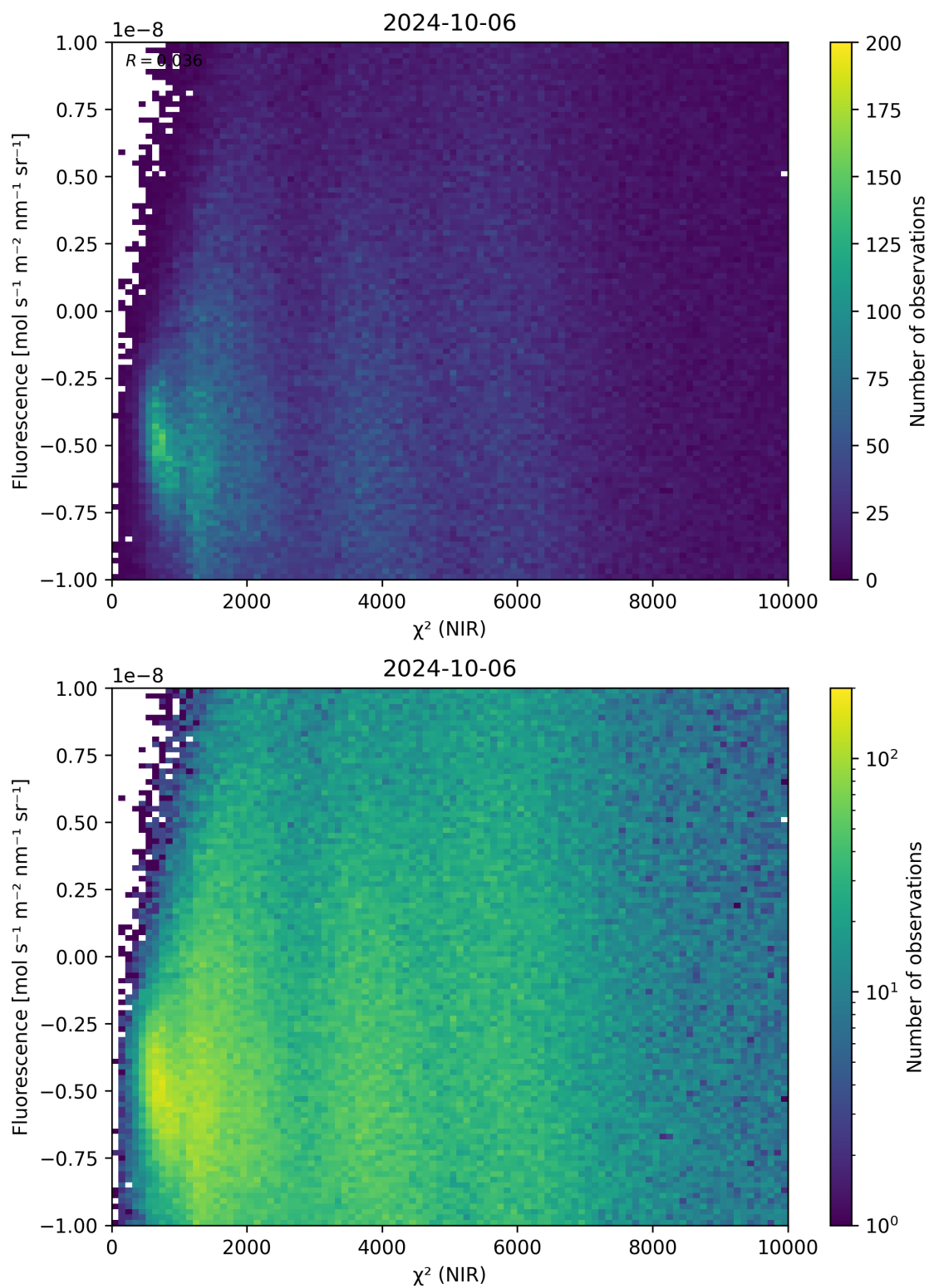
Figure 45: Scatter density plot of “ \chi^2 (NIR)” against “Fluorescence” for 2024-10-05 to 2024-10-07.
