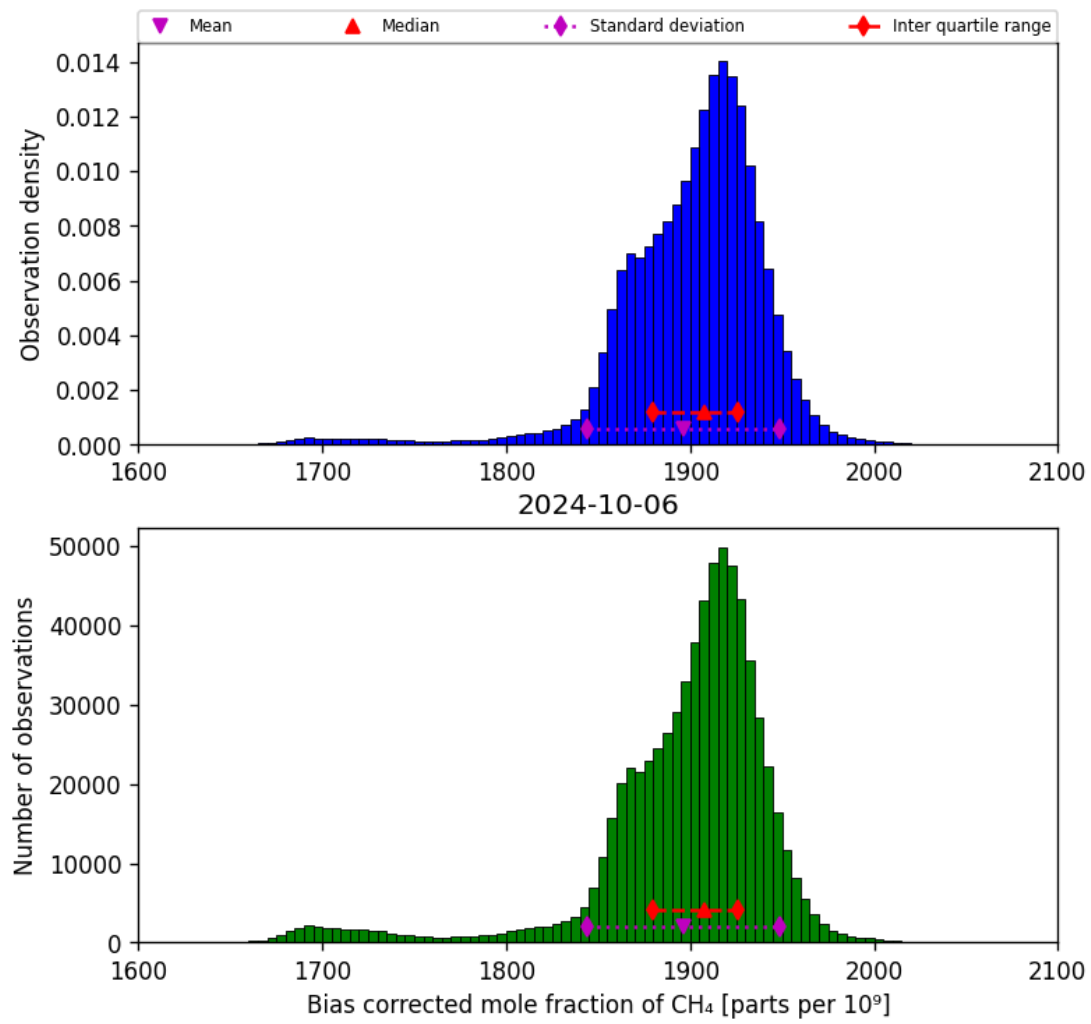
Figure 25: Histogram of “Bias corrected mole fraction of CH 4 ” for 2024-10-05 to 2024-10-07
