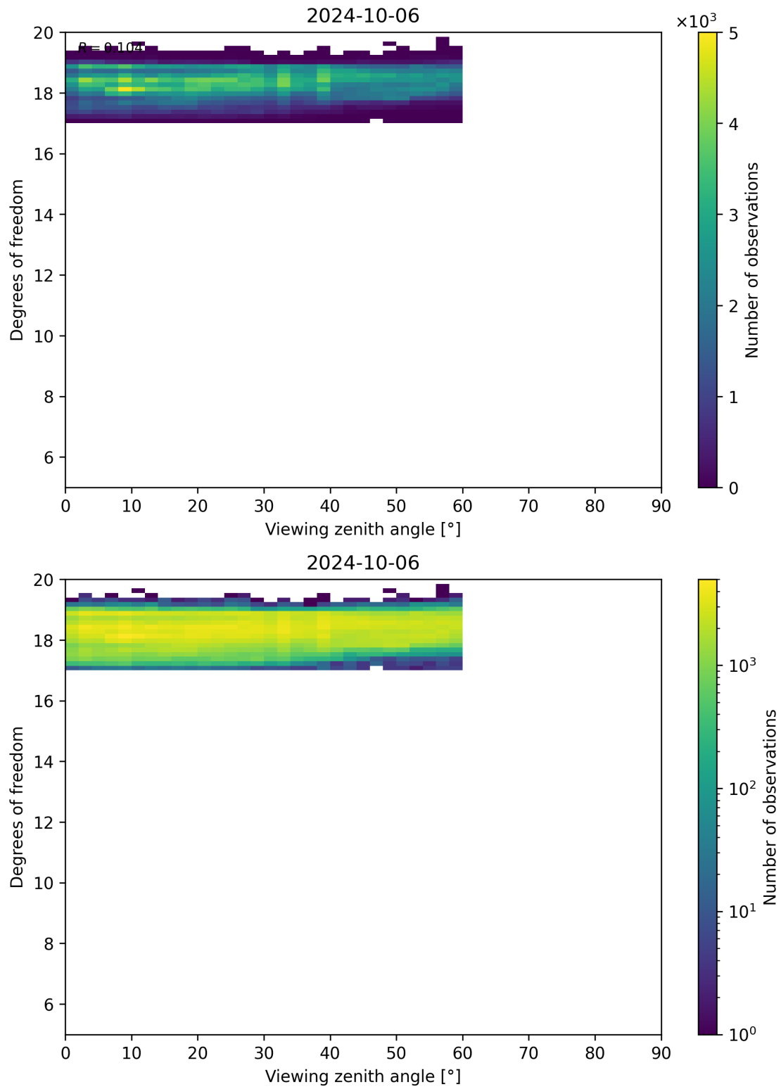
Figure 107: Scatter density plot of “Viewing zenith angle” against “Degrees of freedom” for 2024-10-05 to 2024-10-07.
