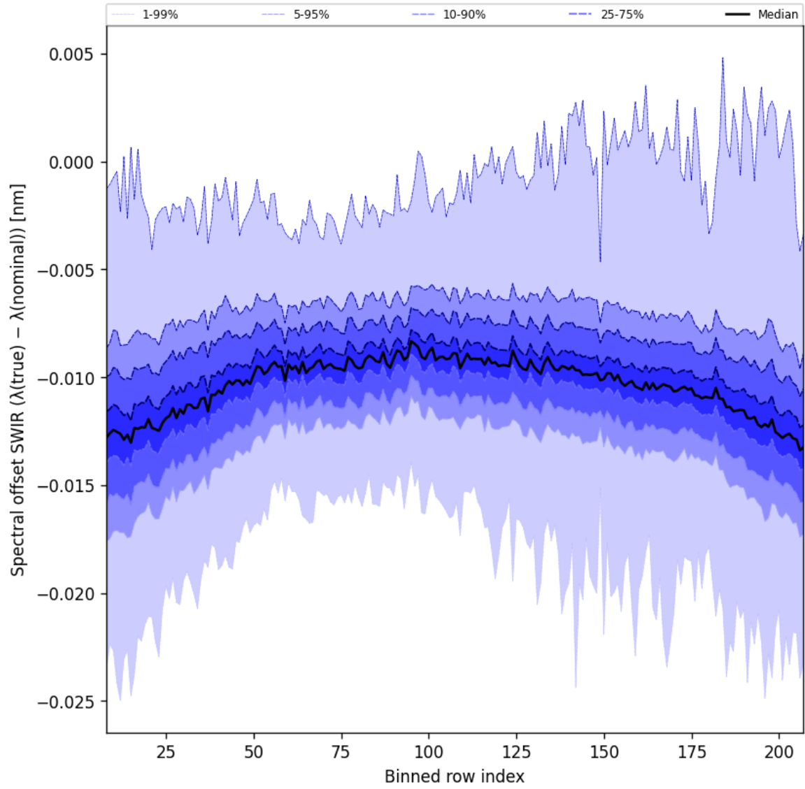
Figure 38: Along track statistics of “Spectral offset SWIR ( \lambda_{\text{true}} - \lambda_{\text{nominal}} )” for 2024-10-05 to 2024-10-07
