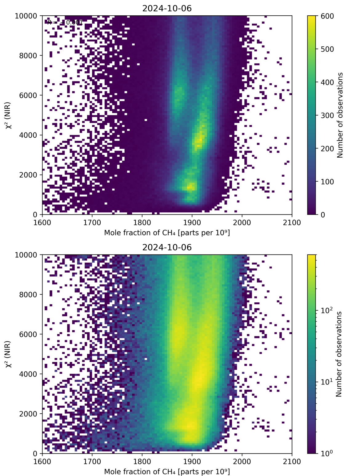
Figure 70: Scatter density plot of “Mole fraction of CH 4 ” against “ \chi^2 (NIR)” for 2024-10-05 to 2024-10-07.
