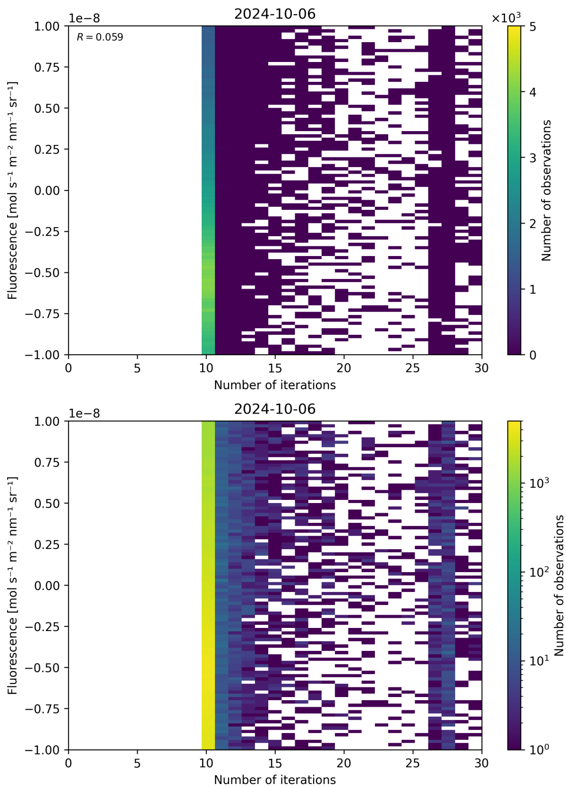
Figure 87: Scatter density plot of “Number of iterations” against “Fluorescence” for 2024-10-05 to 2024-10-07.
