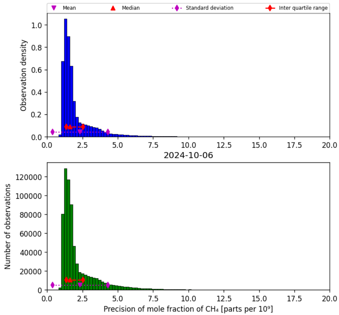
Figure 24: Histogram of “Precision of mole fraction of CH 4 ” for 2024-10-05 to 2024-10-07
