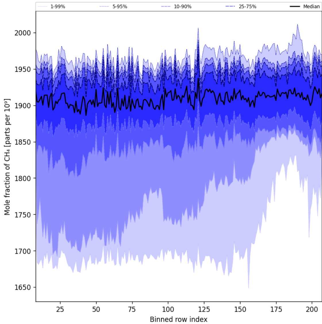
Figure 34: Along track statistics of “Mole fraction of CH 4 ” for 2024-10-05 to 2024-10-07
