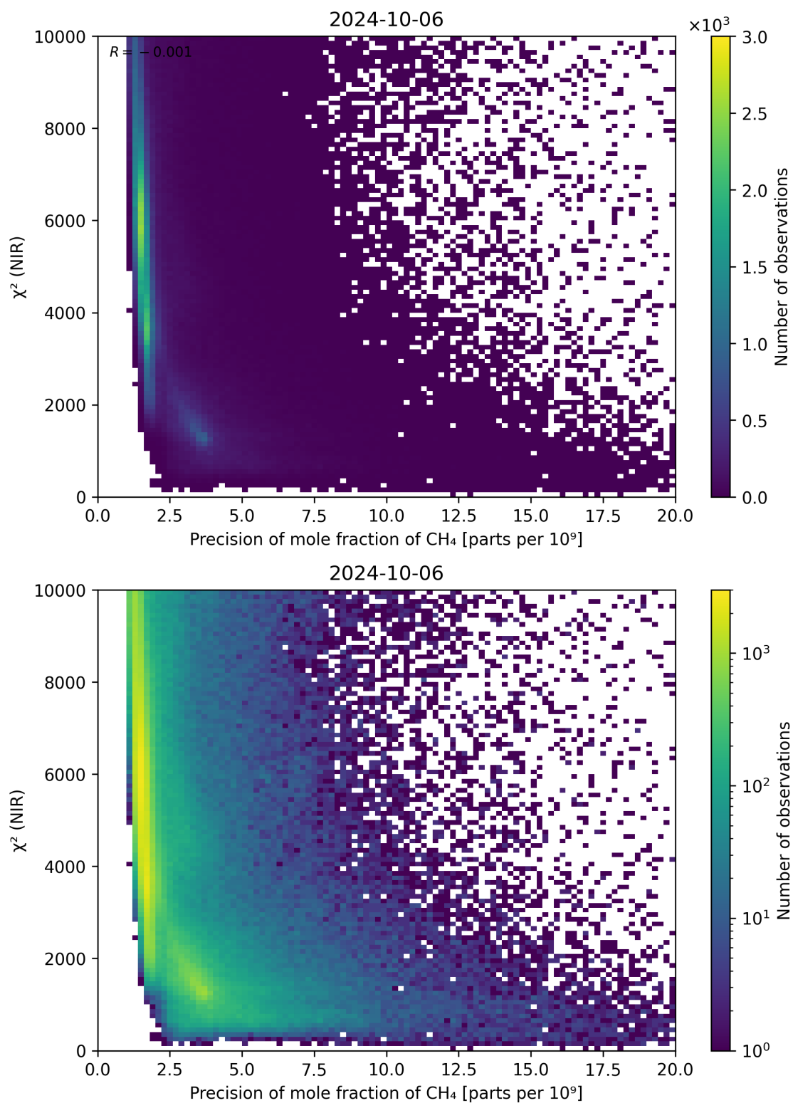
Figure 78: Scatter density plot of “Precision of mole fraction of CH 4 ” against “ \chi^2 (NIR)” for 2024-10-05 to 2024-10-07.
