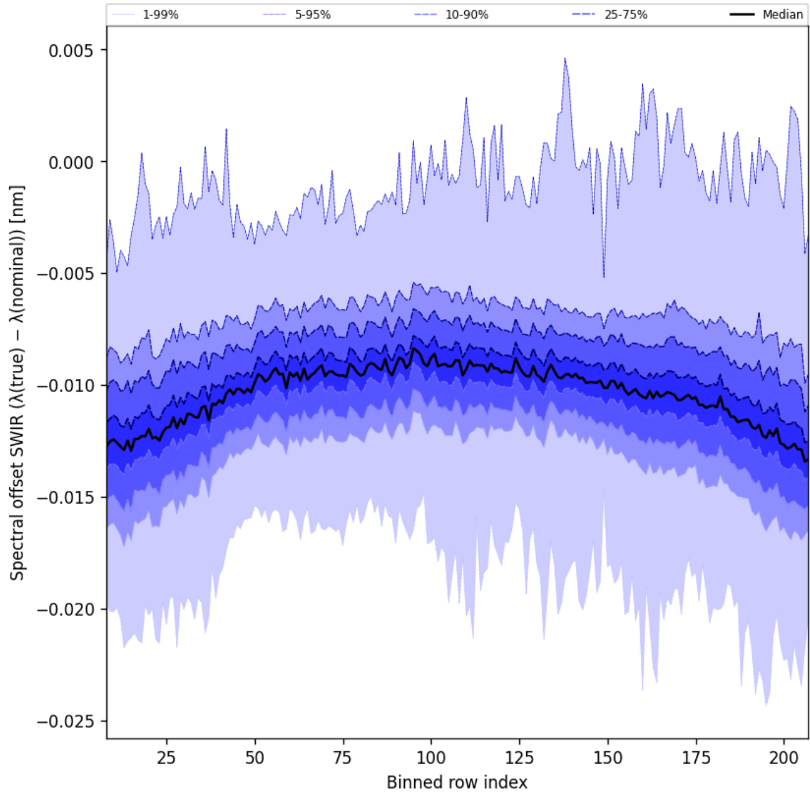
Figure 38: Along track statistics of “Spectral offset SWIR ( \lambda_{\text{true}} - \lambda_{\text{nominal}} )” for 2024-10-06 to 2024-10-08
