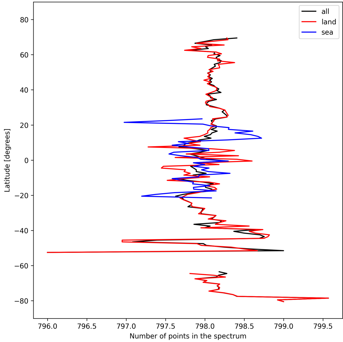
Figure 15: Zonal average of “Number of points in the spectrum” for 2024-10-06 to 2024-10-08.
