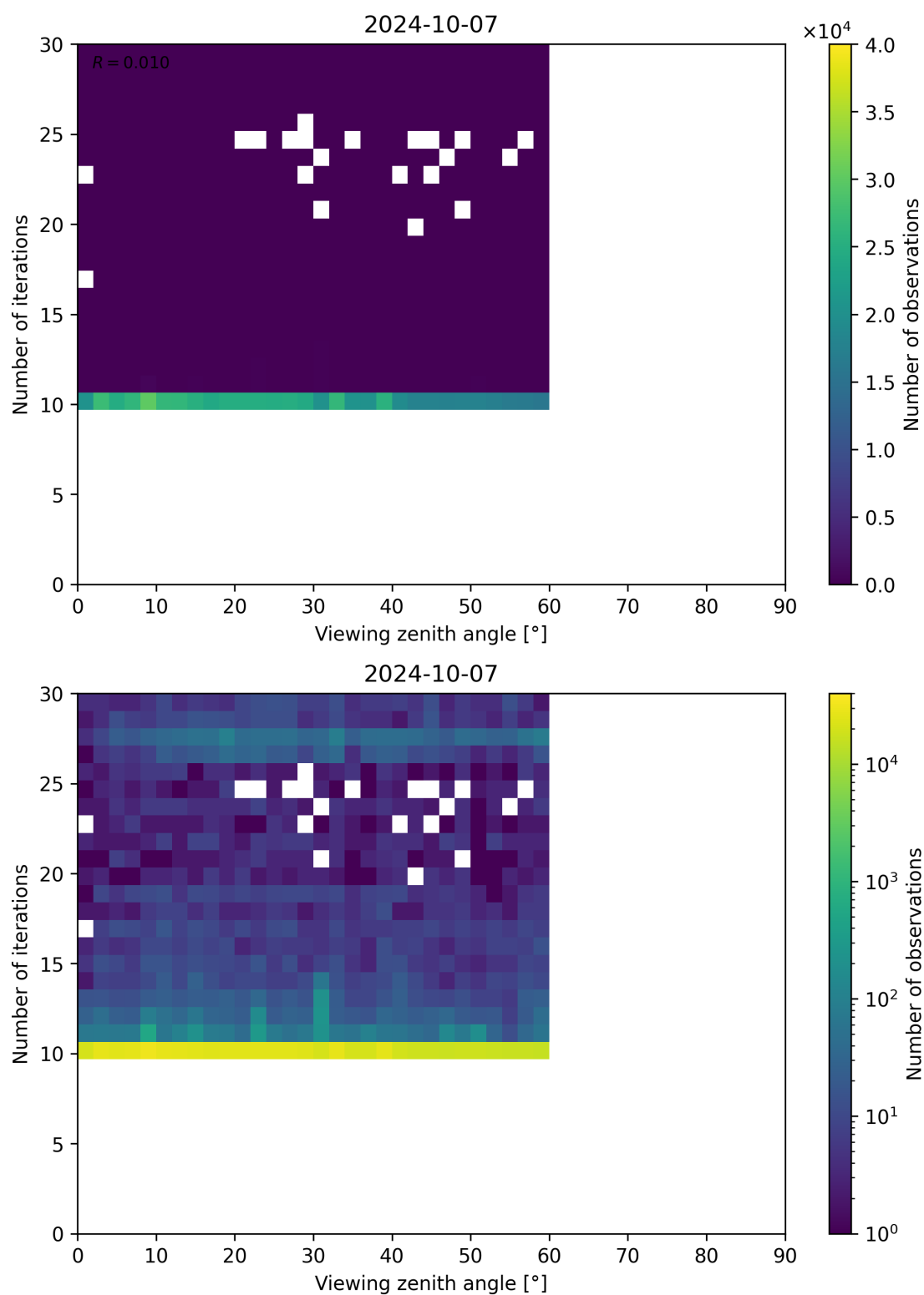
Figure 113: Scatter density plot of “Viewing zenith angle” against “Number of iterations” for 2024-10-06 to 2024-10-08.
