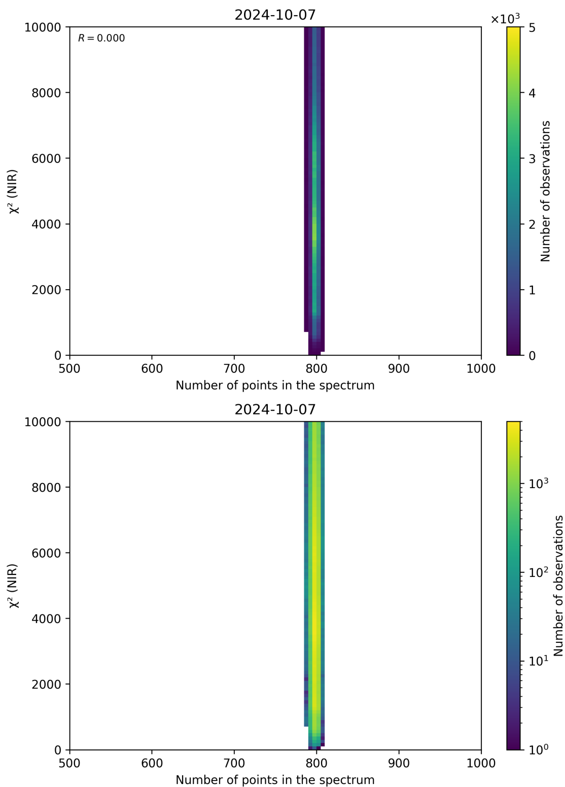
Figure 88: Scatter density plot of “Number of points in the spectrum” against “ \chi^2 (NIR)” for 2024-10-06 to 2024-10-08.
