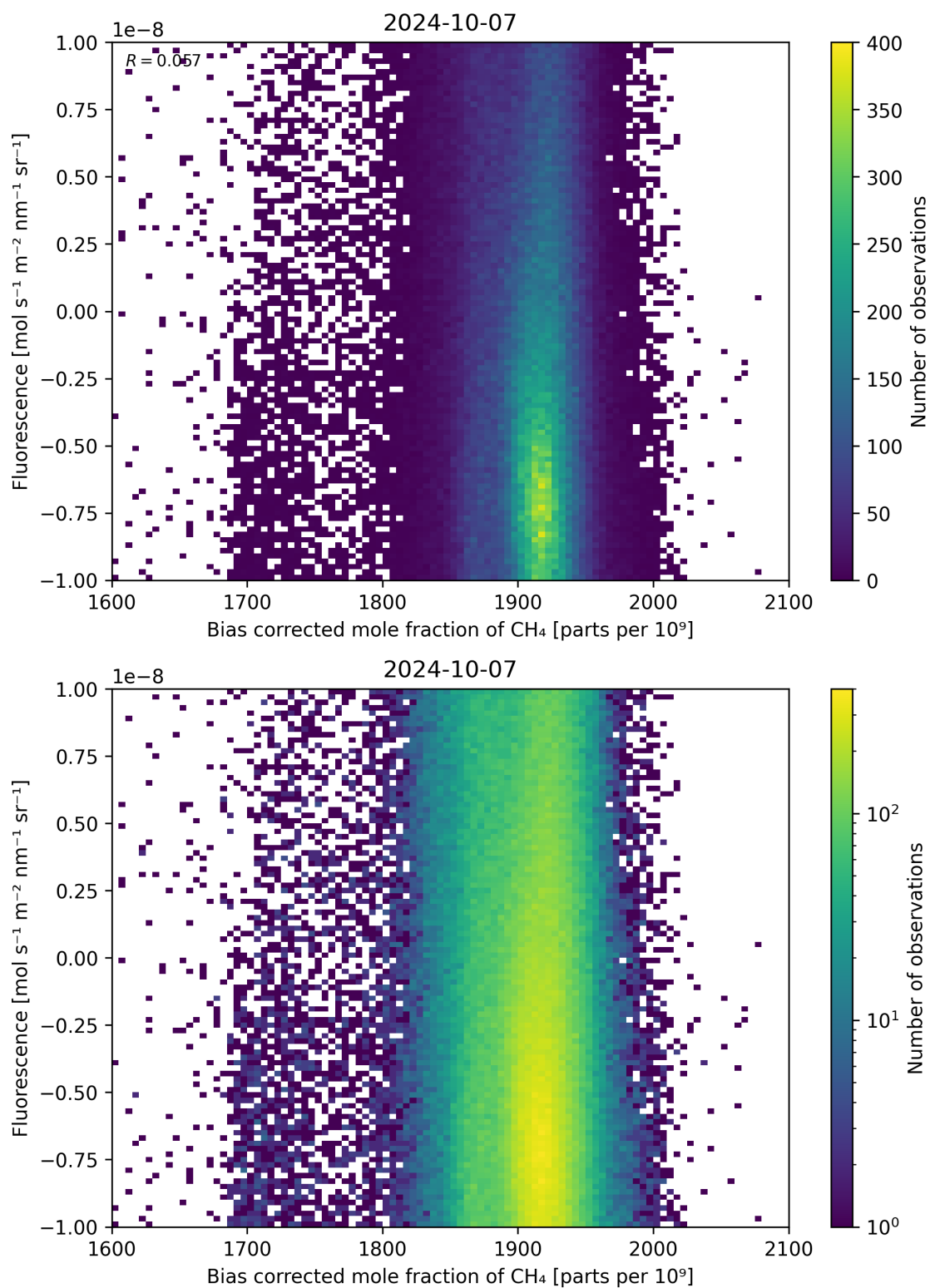
Figure 66: Scatter density plot of “Bias corrected mole fraction of CH 4 ” against “Fluorescence” for 2024-10-06 to 2024-10-08.
