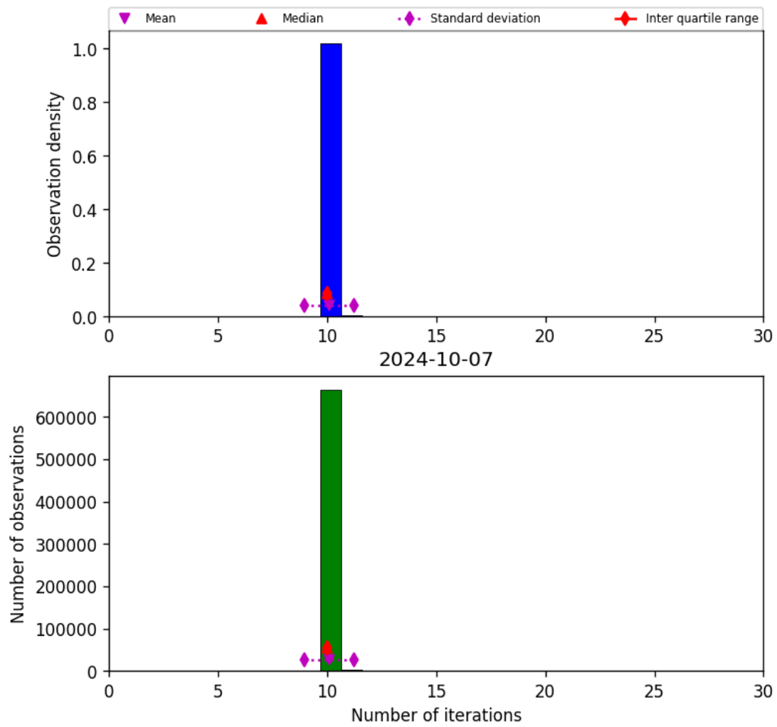
Figure 31: Histogram of “Number of iterations” for 2024-10-06 to 2024-10-08
