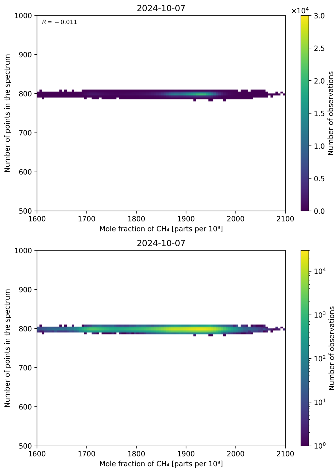
Figure 77: Scatter density plot of “Mole fraction of CH 4 ” against “Number of points in the spectrum” for 2024-10-06 to 2024-10-08.
