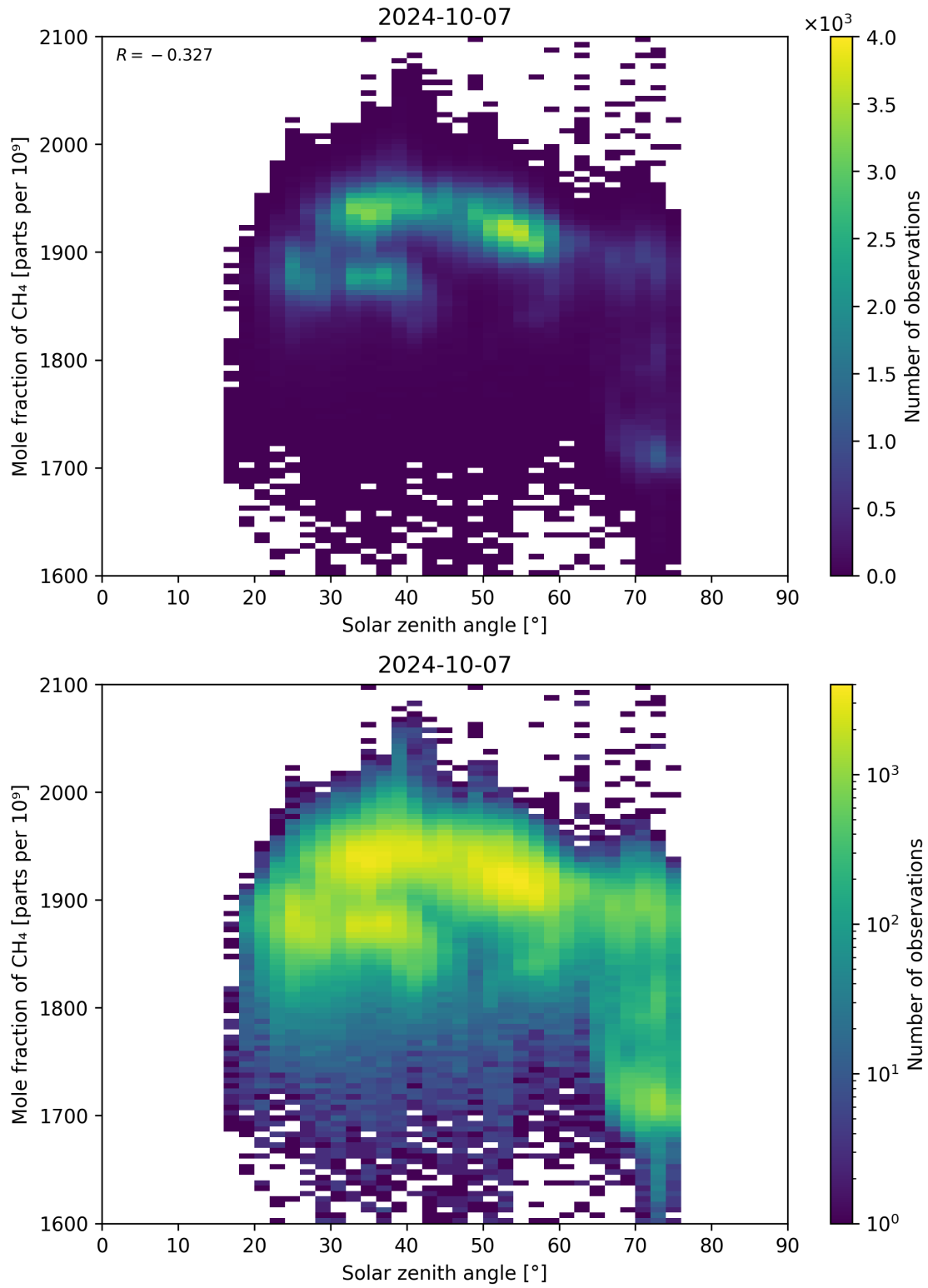
Figure 99: Scatter density plot of “Solar zenith angle” against “Mole fraction of CH 4 ” for 2024-10-06 to 2024-10-08.
