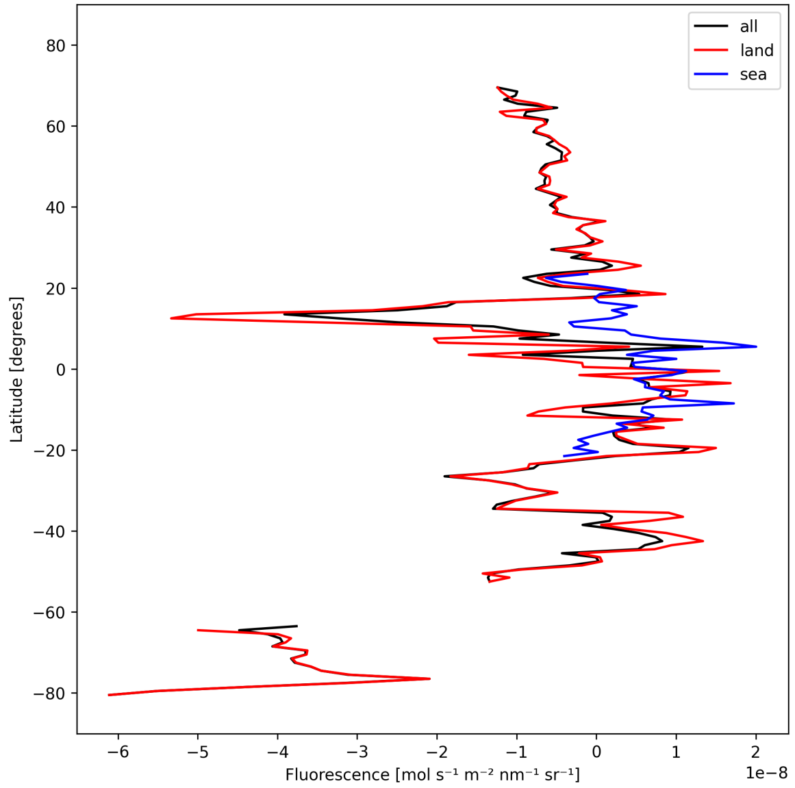
Figure 21: Zonal average of “Fluorescence” for 2024-10-06 to 2024-10-08.
