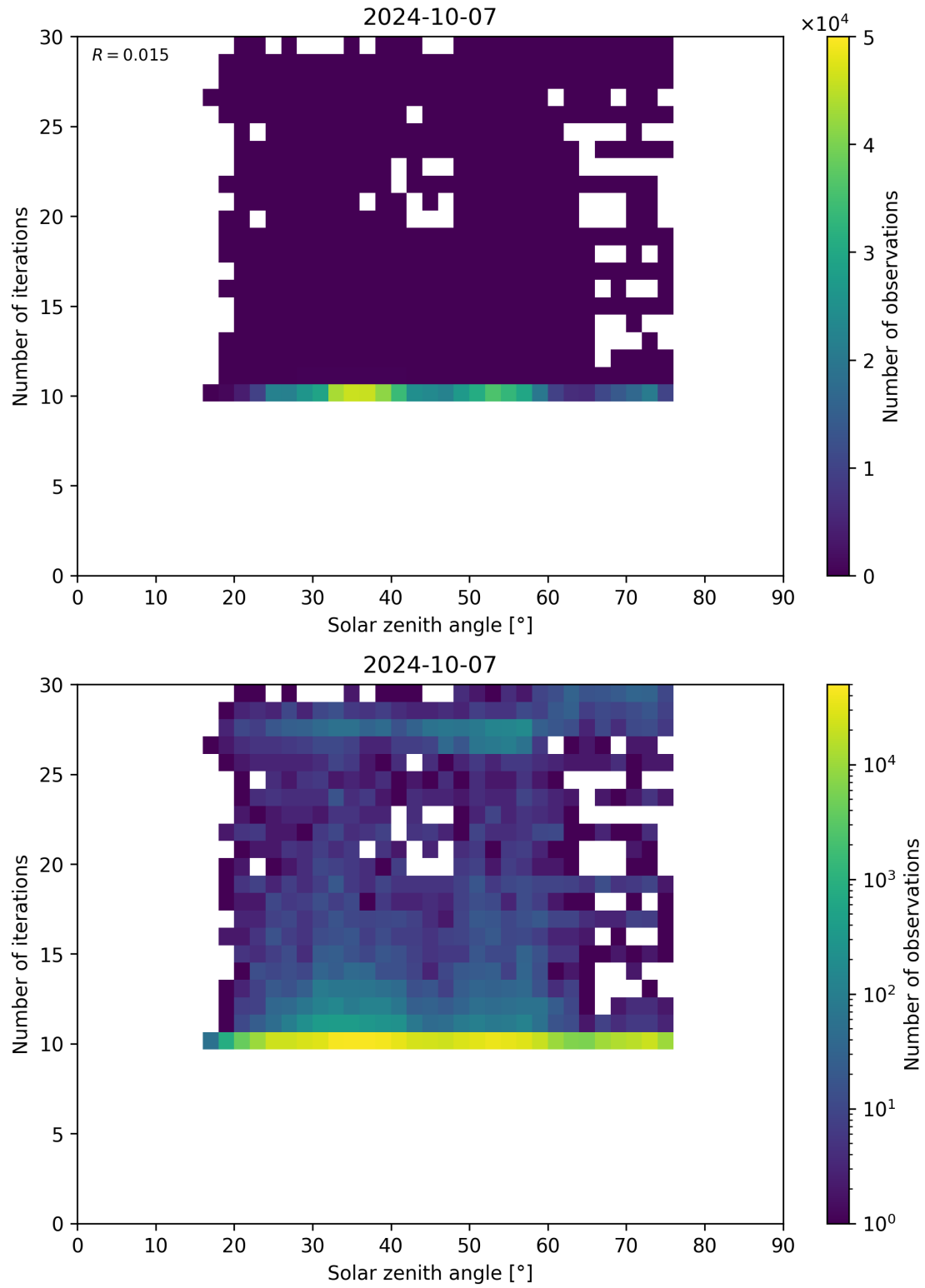
Figure 102: Scatter density plot of “Solar zenith angle” against “Number of iterations” for 2024-10-06 to 2024-10-08.
