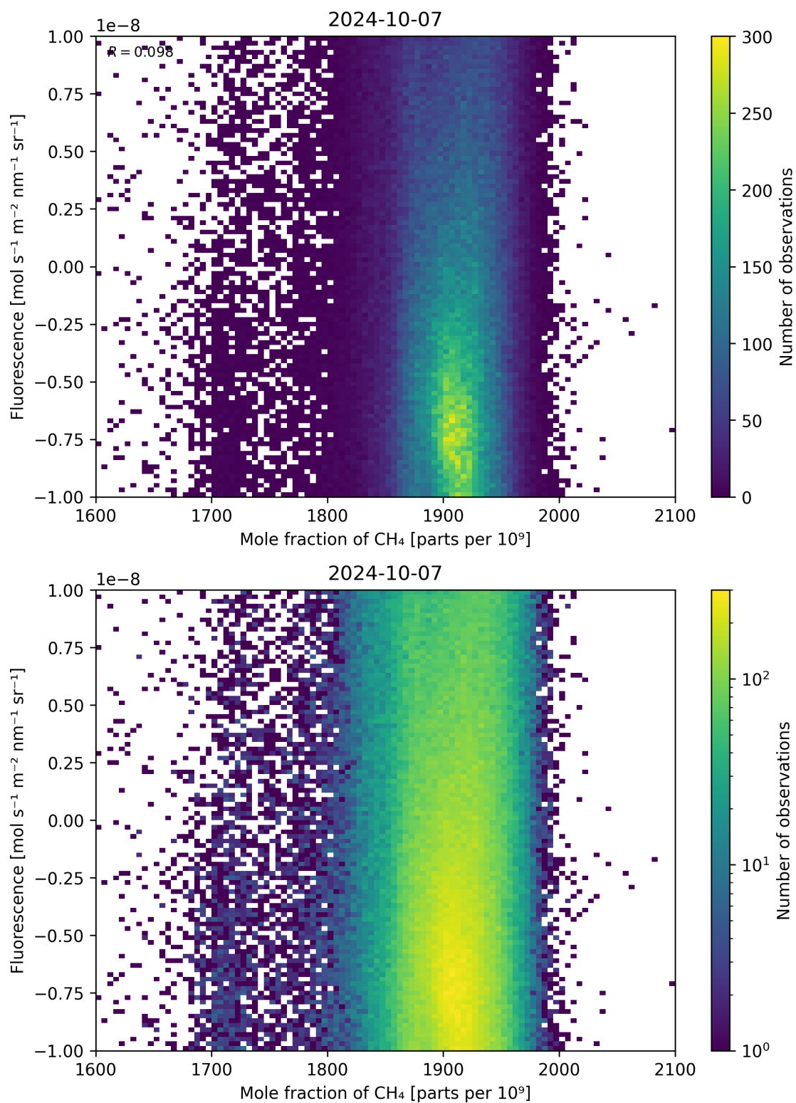
Figure 73: Scatter density plot of “Mole fraction of \text{CH}_4 ” against “Fluorescence” for 2024-10-06 to 2024-10-08.
