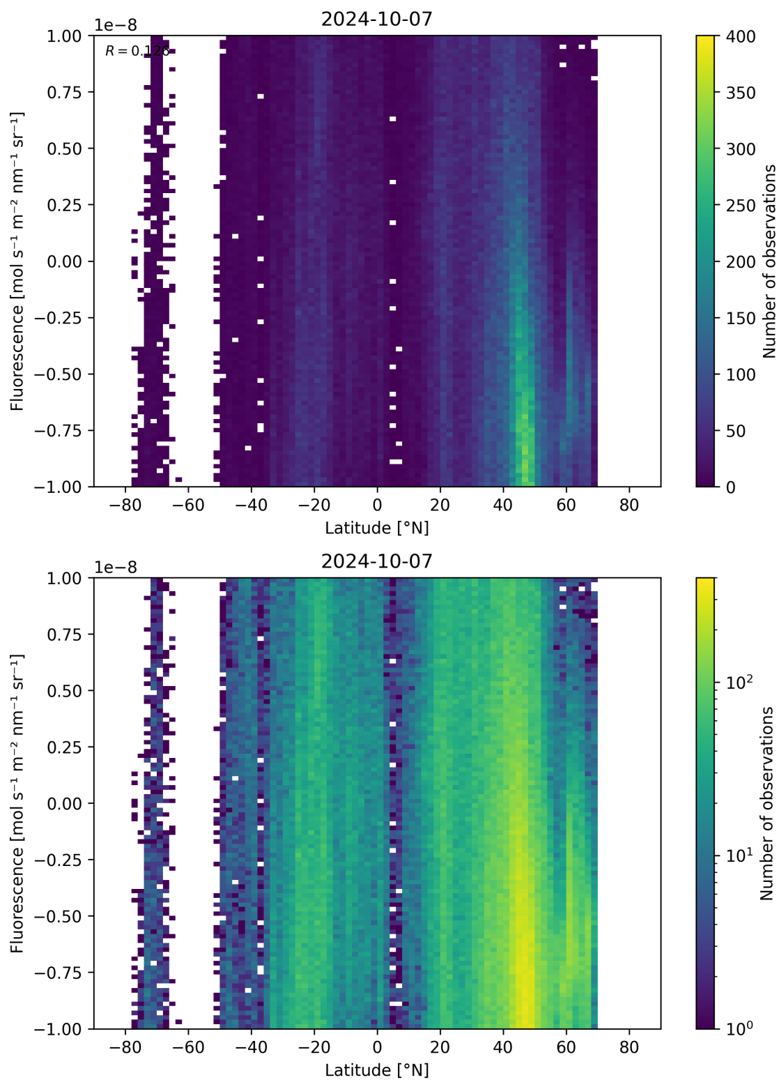
Figure 56: Scatter density plot of “Latitude” against “Fluorescence” for 2024-10-06 to 2024-10-08.
