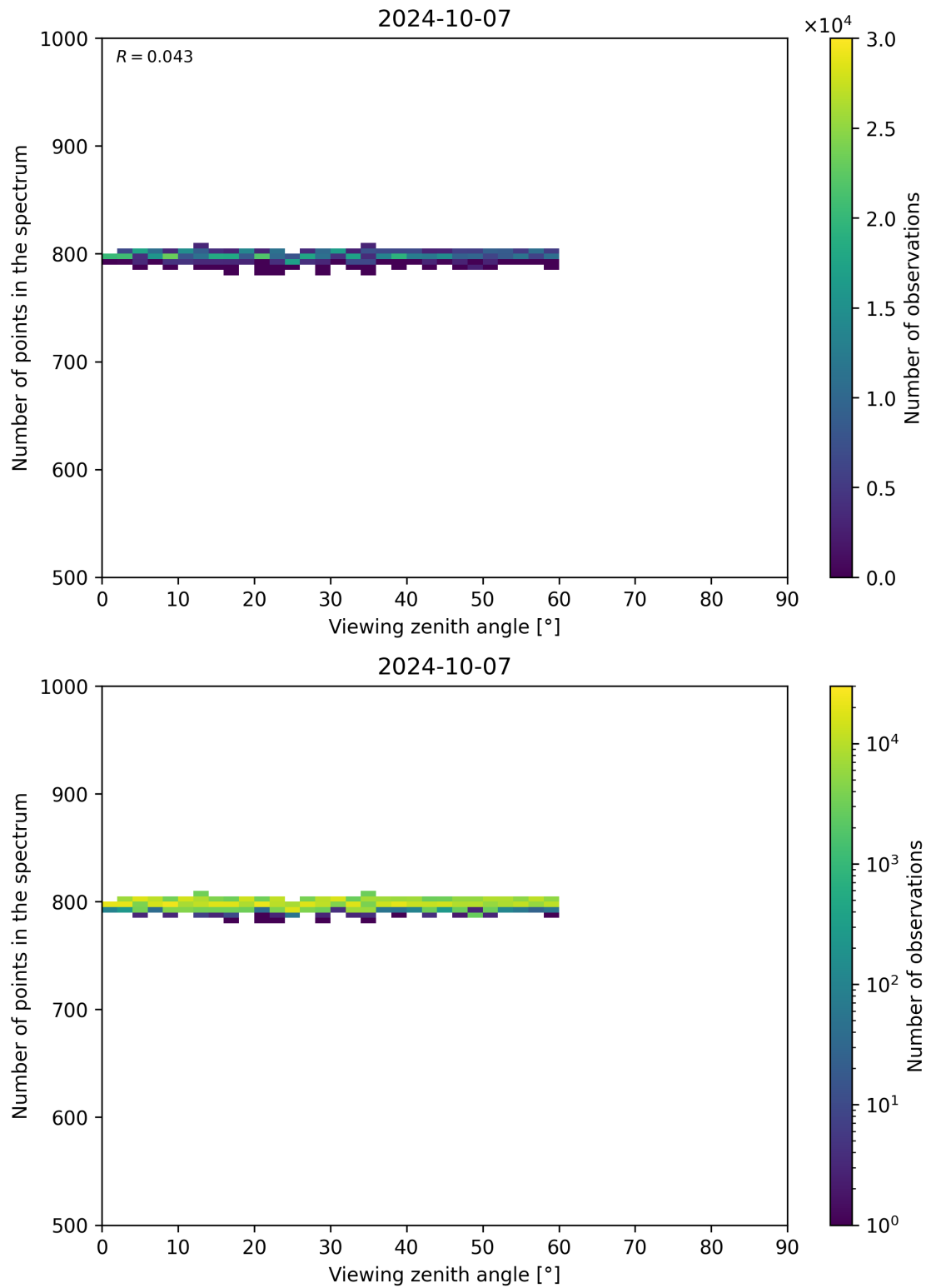
Figure 114: Scatter density plot of “Viewing zenith angle” against “Number of points in the spectrum” for 2024-10-06 to 2024-10-08.
