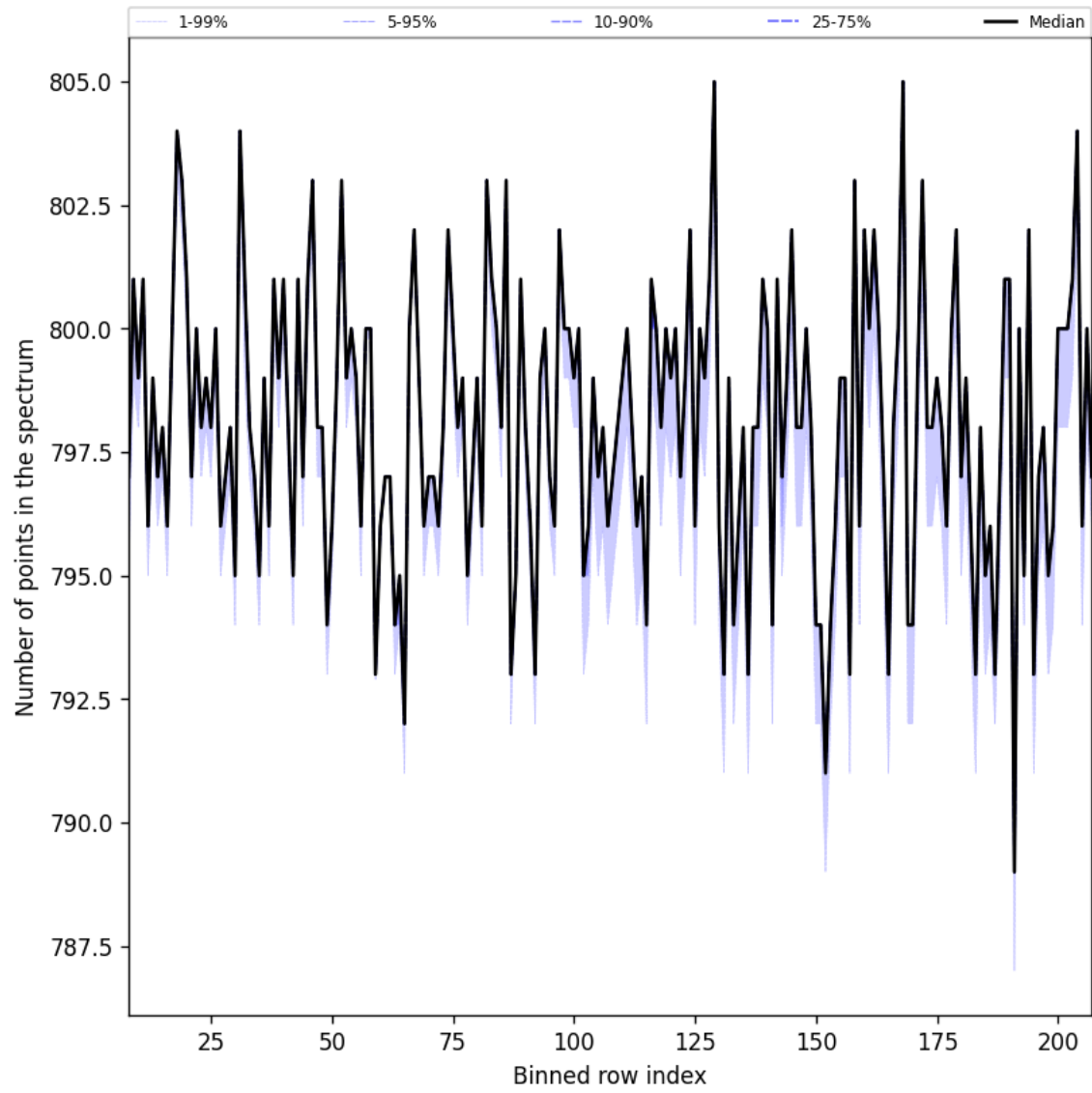
Figure 37: Along track statistics of “Number of points in the spectrum” for 2024-10-06 to 2024-10-08
