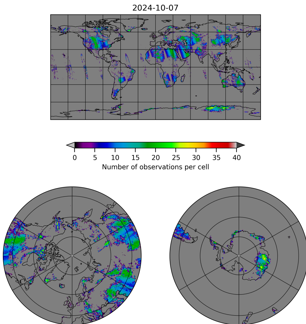
Figure 10: Map of the number of observations for 2024-10-06 to 2024-10-08
