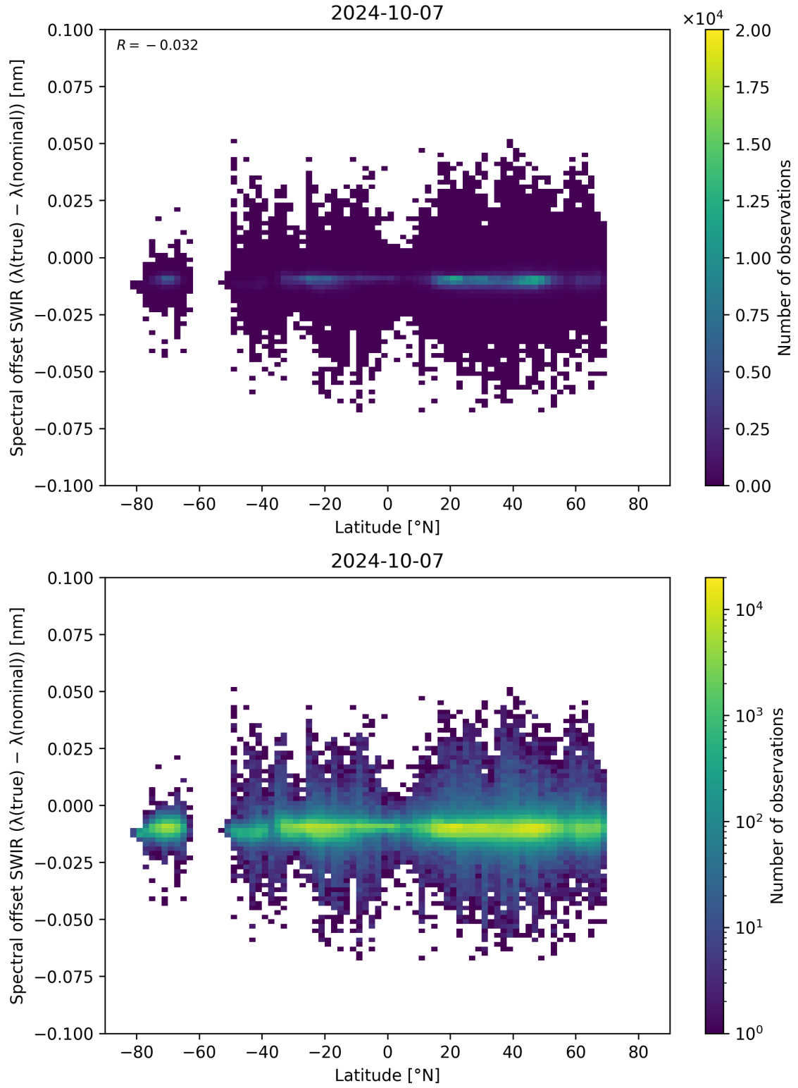
Figure 62: Scatter density plot of “Latitude” against “Spectral offset SWIR ( \lambda_{\text{true}} - \lambda_{\text{nominal}} )” for 2024-10-06 to 2024-10-08.
