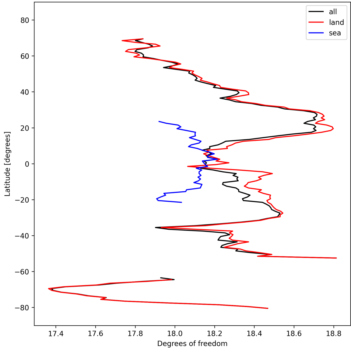
Figure 19: Zonal average of “Degrees of freedom” for 2024-10-06 to 2024-10-08.
