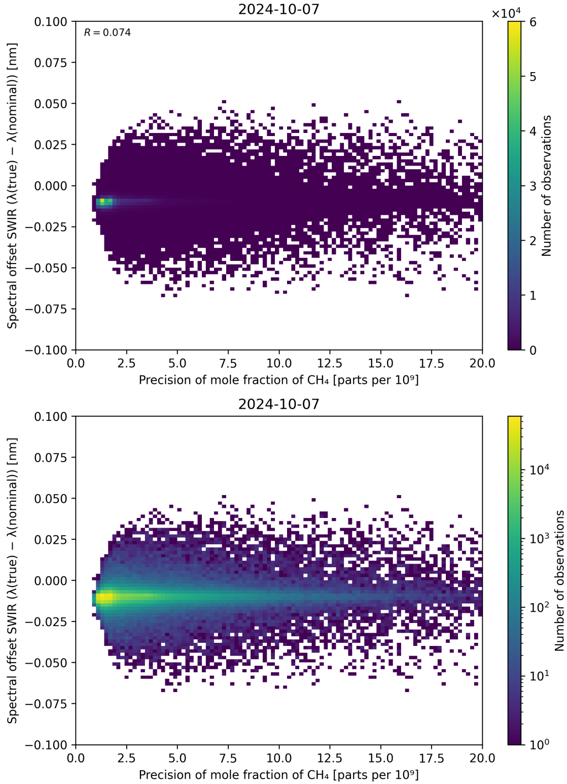
Figure 85: Scatter density plot of “Precision of mole fraction of CH 4 ” against “Spectral offset SWIR ( \lambda_{\text{true}} - \lambda_{\text{nominal}} )” for 2024-10-06 to 2024-10-08.
