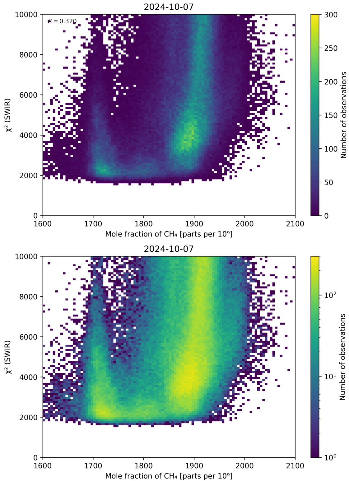
Figure 71: Scatter density plot of “Mole fraction of \text{CH}_4 ” against “ \chi^2 (SWIR)” for 2024-10-06 to 2024-10-08.
