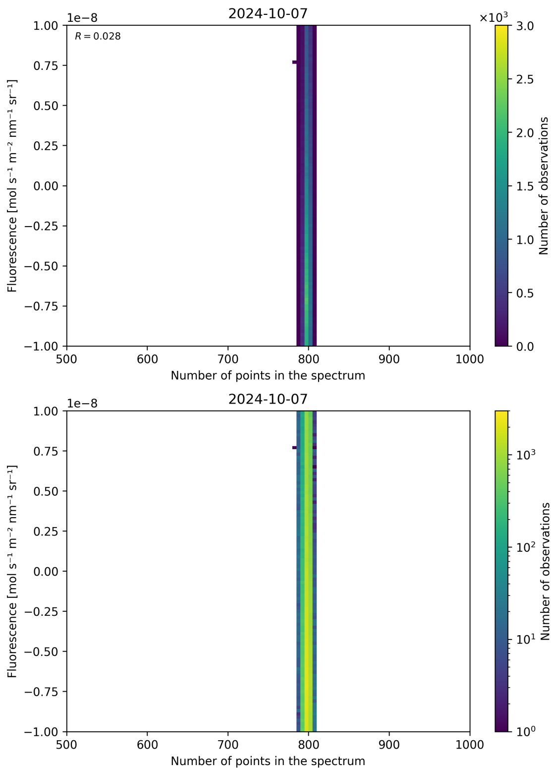
Figure 91: Scatter density plot of “Number of points in the spectrum” against “Fluorescence” for 2024-10-06 to 2024-10-08.
