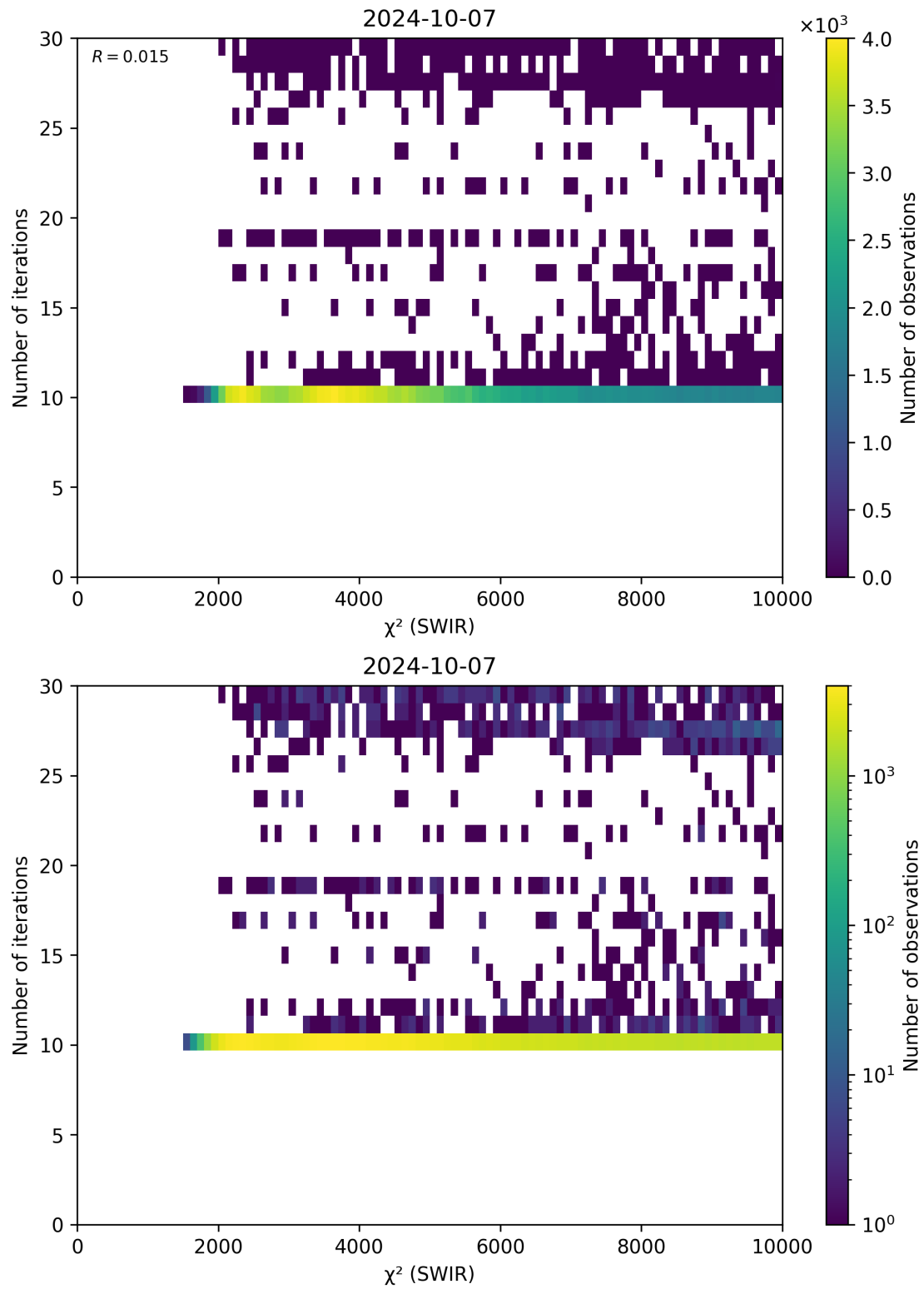
Figure 50: Scatter density plot of “ \chi^2 (SWIR)” against “Number of iterations” for 2024-10-06 to 2024-10-08.
