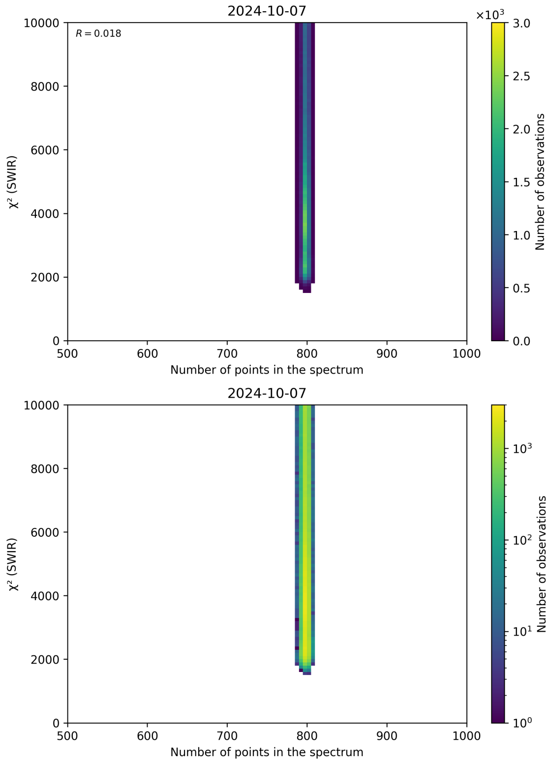
Figure 89: Scatter density plot of “Number of points in the spectrum” against “ \chi^2 (SWIR)” for 2024-10-06 to 2024-10-08.
