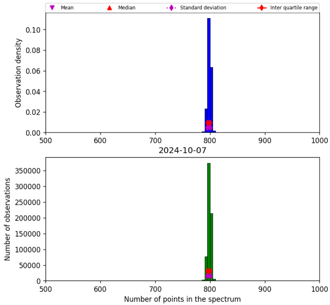
Figure 26: Histogram of “Number of points in the spectrum” for 2024-10-06 to 2024-10-08
