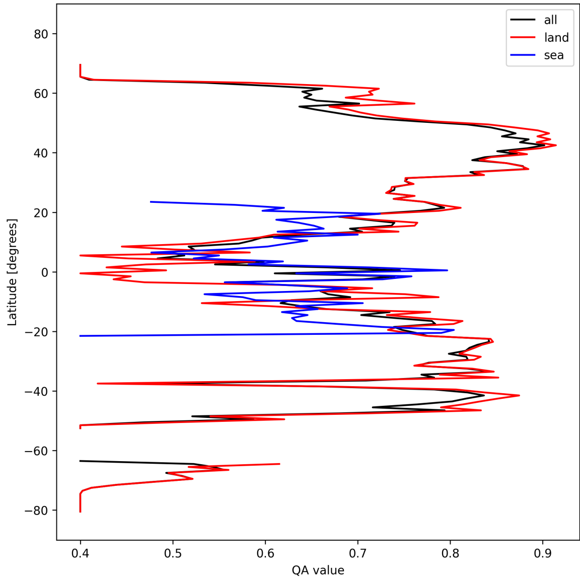
Figure 11: Zonal average of “QA value” for 2024-10-06 to 2024-10-08.
