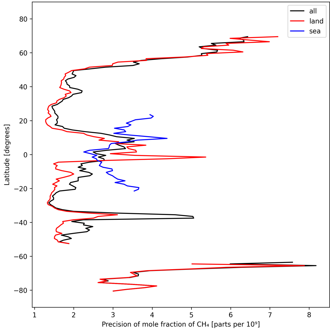
Figure 13: Zonal average of “Precision of mole fraction of CH 4 ” for 2024-10-06 to 2024-10-08.
