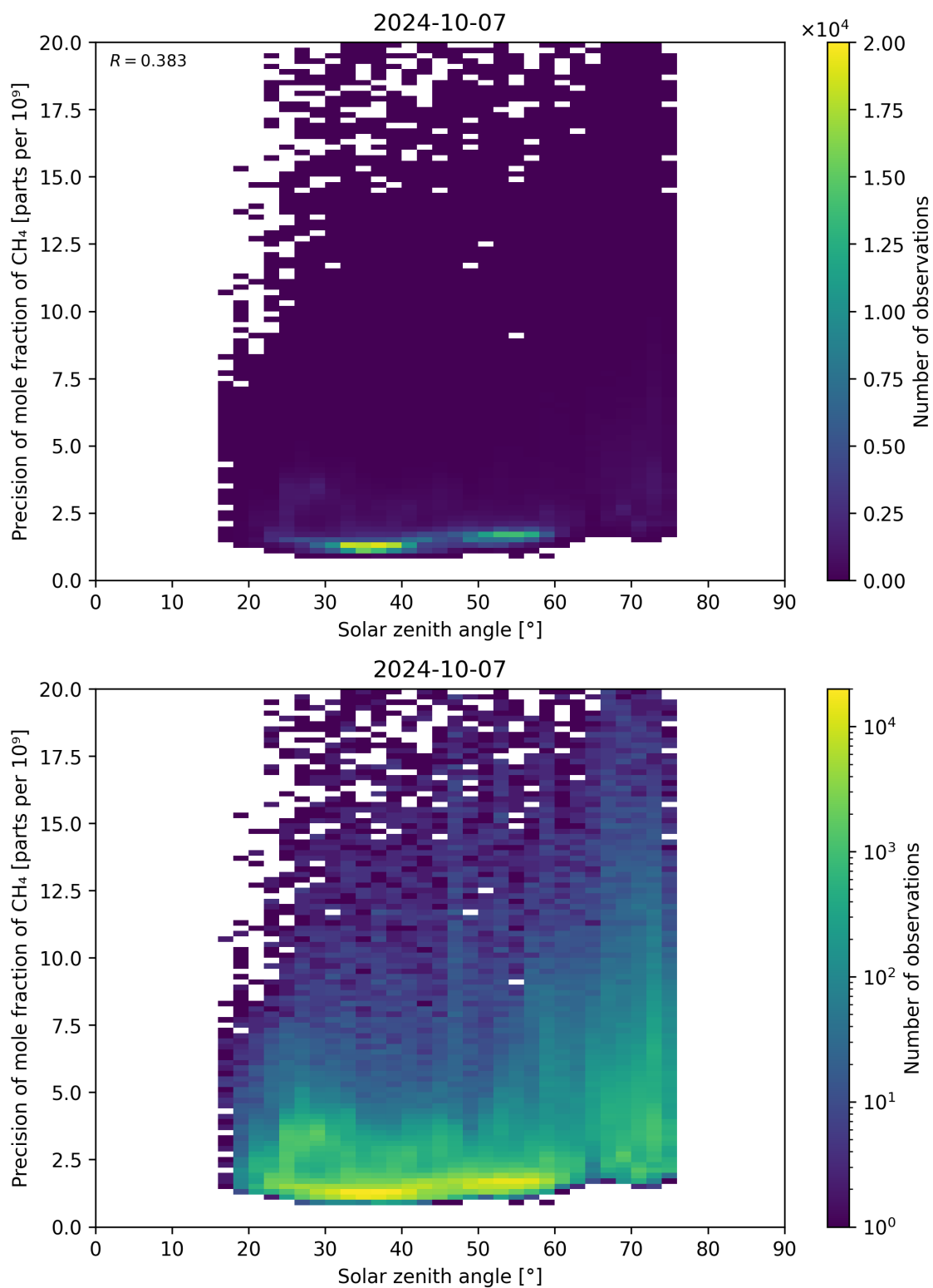
Figure 101: Scatter density plot of “Solar zenith angle” against “Precision of mole fraction of \text{CH}_4 ” for 2024-10-06 to 2024-10-08.
