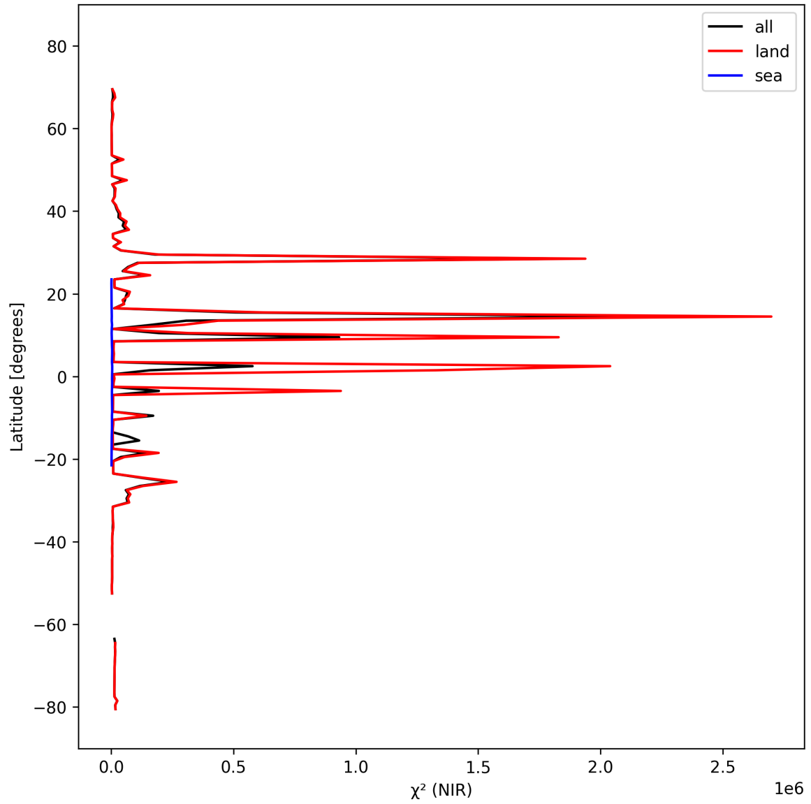
Figure 18: Zonal average of “ \chi^2 (NIR)” for 2024-10-06 to 2024-10-08.
