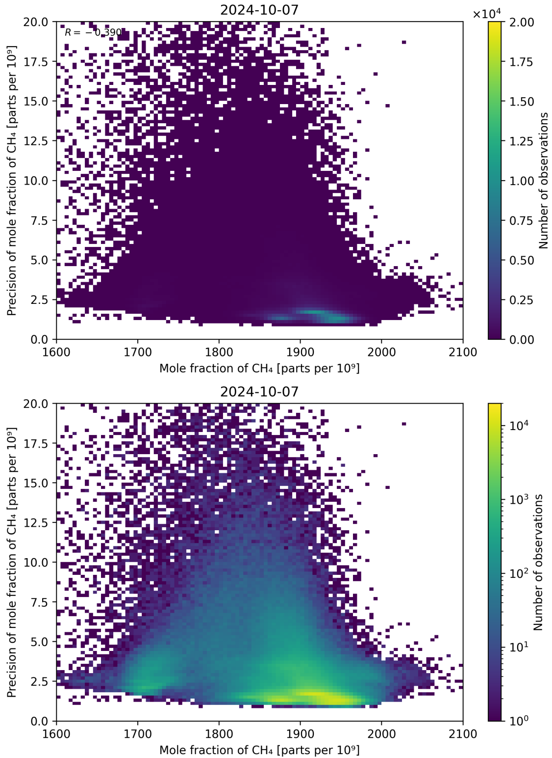
Figure 75: Scatter density plot of “Mole fraction of CH 4 ” against “Precision of mole fraction of CH 4 ” for 2024-10-06 to 2024-10-08.
