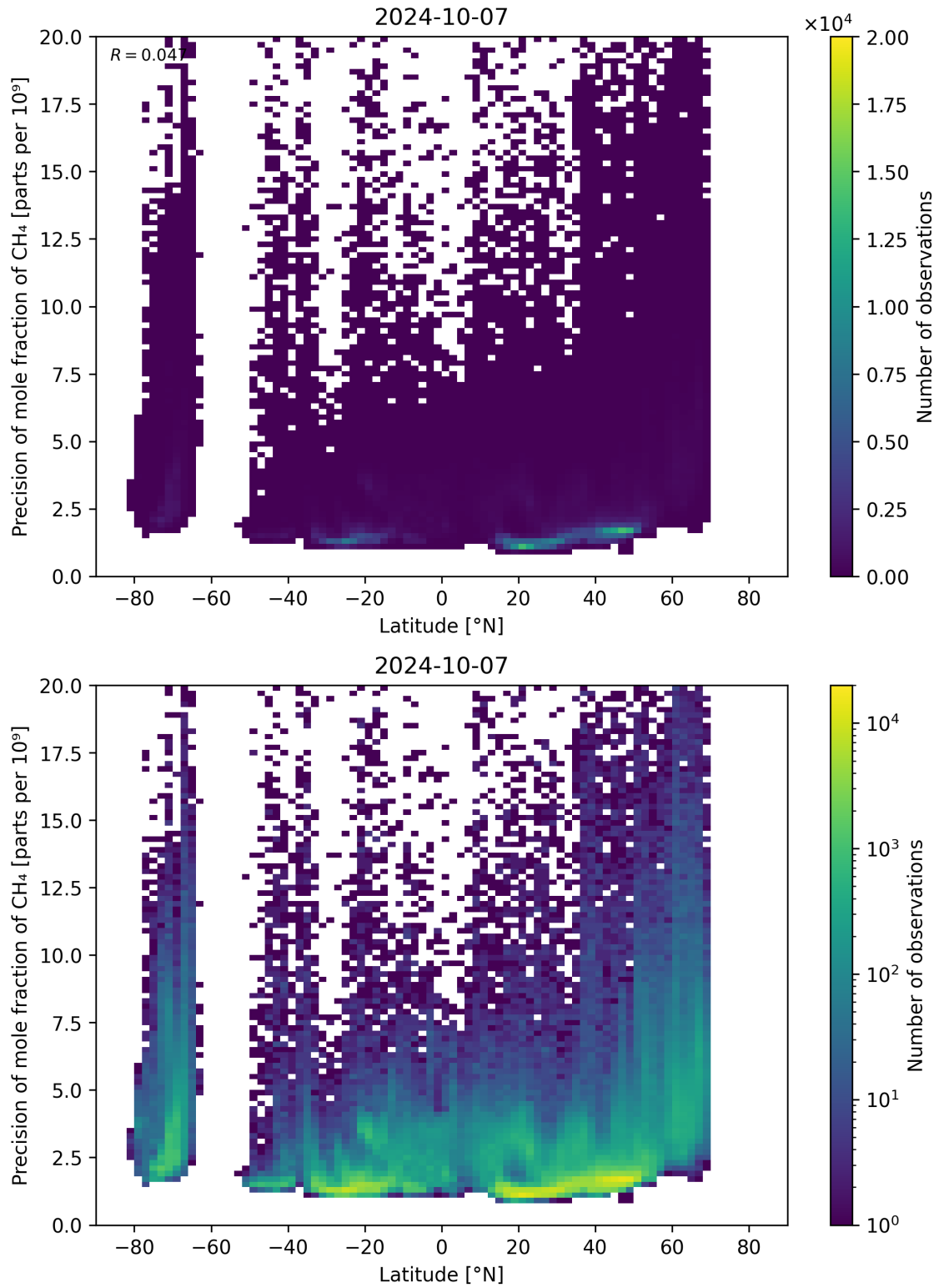
Figure 59: Scatter density plot of “Latitude” against “Precision of mole fraction of \text{CH}_4 ” for 2024-10-06 to 2024-10-08.
