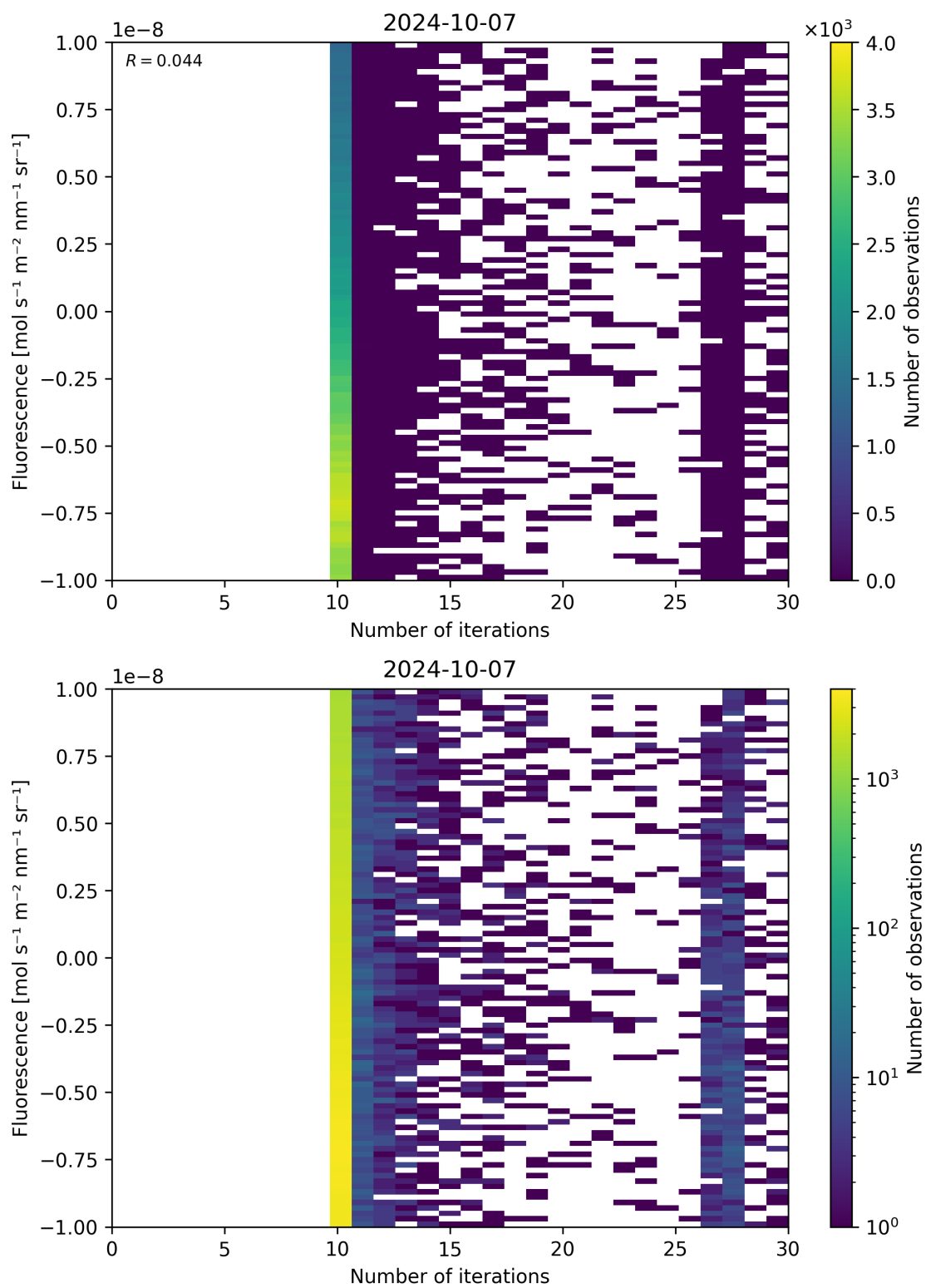
Figure 87: Scatter density plot of “Number of iterations” against “Fluorescence” for 2024-10-06 to 2024-10-08.
