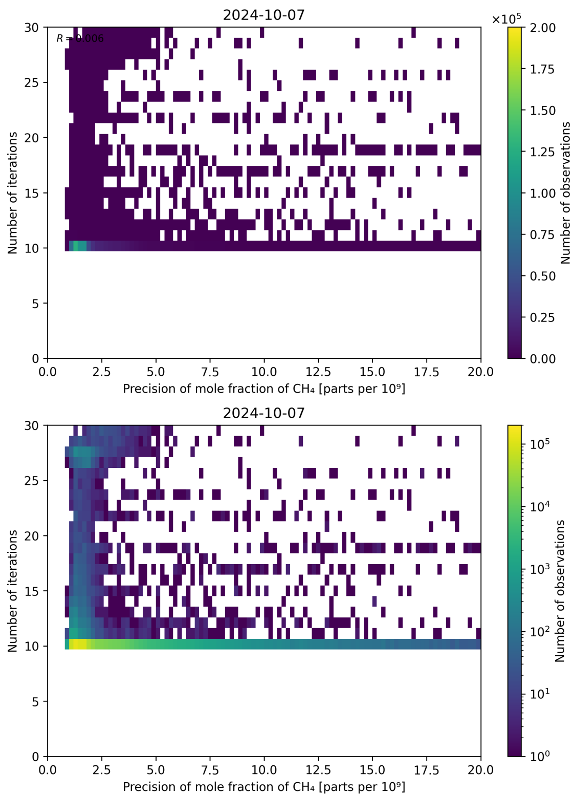
Figure 83: Scatter density plot of “Precision of mole fraction of CH 4 ” against “Number of iterations” for 2024-10-06 to 2024-10-08.
