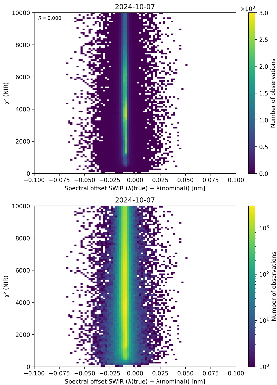
Figure 117: Scatter density plot of “Spectral offset SWIR ( \lambda_{\text{true}} - \lambda_{\text{nominal}} )” against “ \chi^2 (NIR)” for 2024-10-06 to 2024-10-08.
