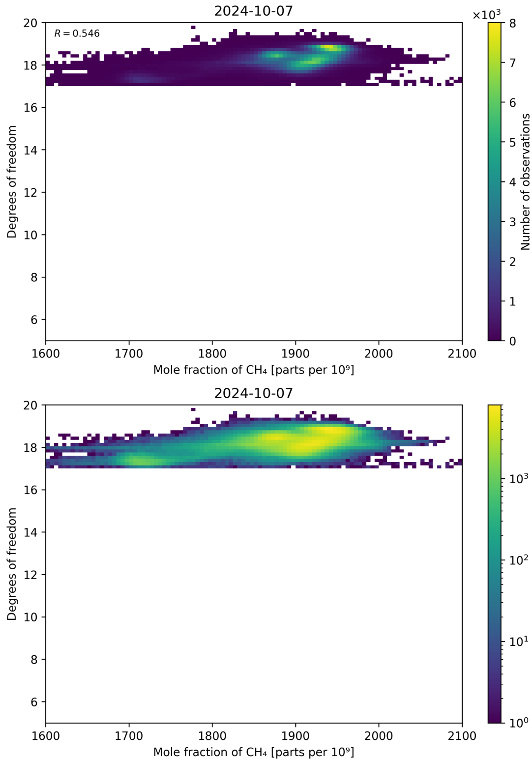
Figure 72: Scatter density plot of “Mole fraction of CH 4 ” against “Degrees of freedom” for 2024-10-06 to 2024-10-08.
