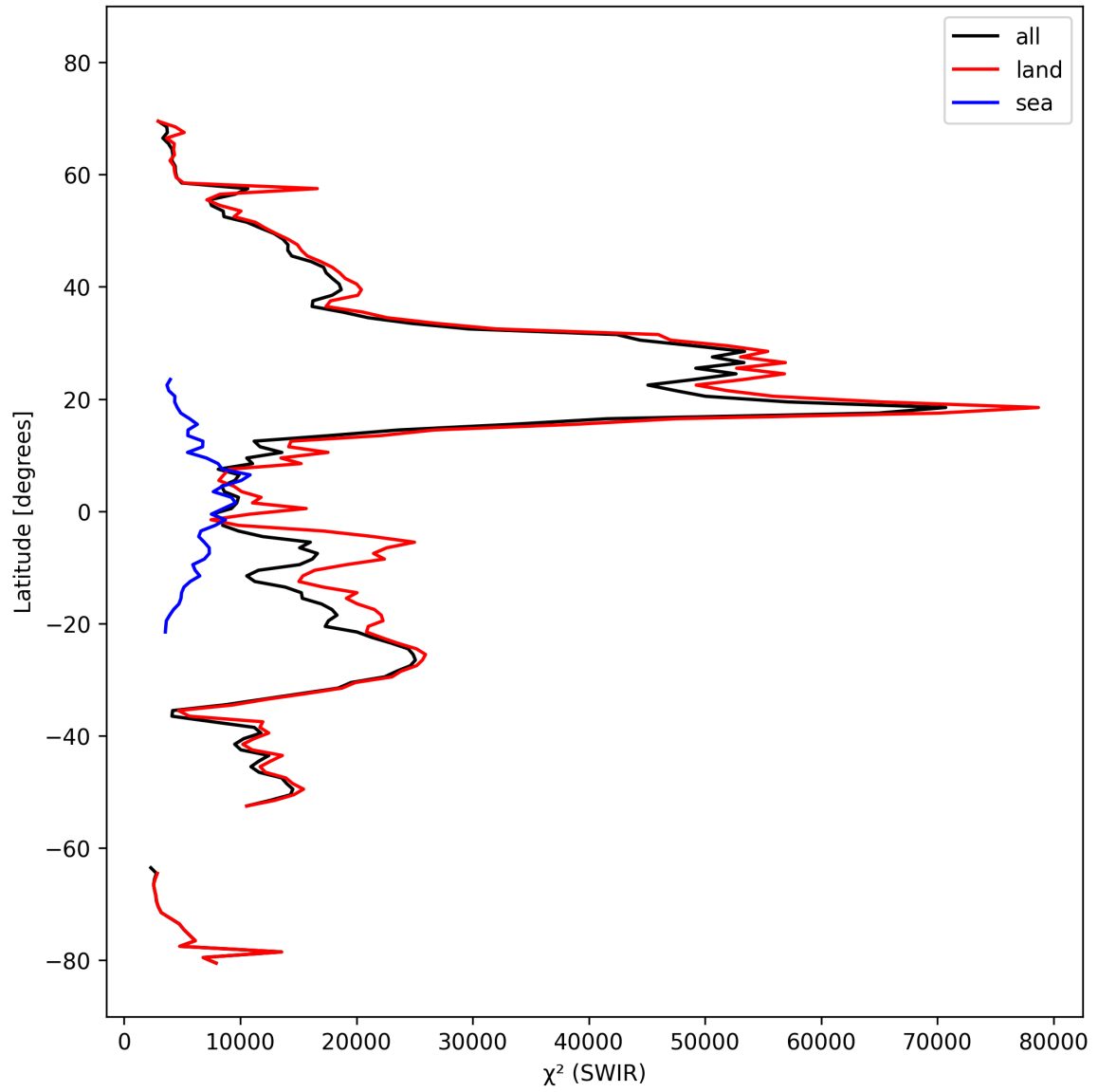
Figure 17: Zonal average of “ \chi^2 (SWIR)” for 2024-10-06 to 2024-10-08.
