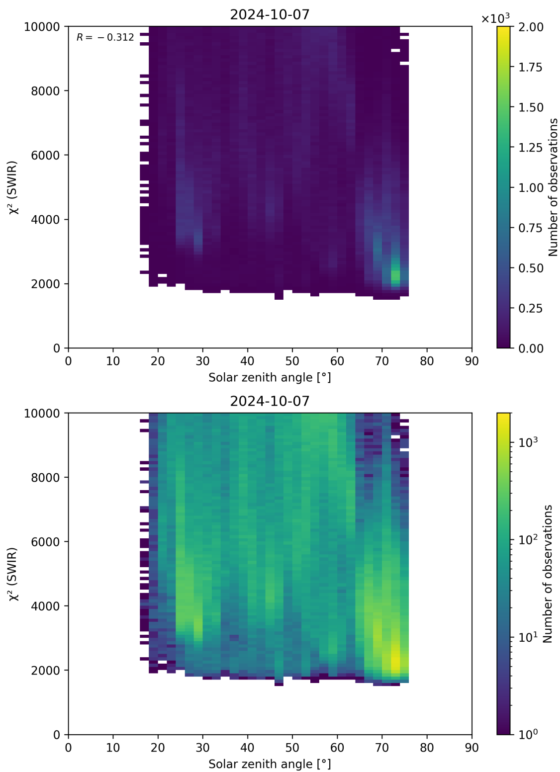
Figure 95: Scatter density plot of “Solar zenith angle” against “ \chi^2 (SWIR)” for 2024-10-06 to 2024-10-08.
