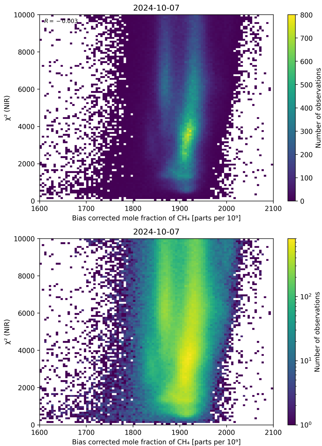
Figure 63: Scatter density plot of “Bias corrected mole fraction of \text{CH}_4 ” against “ \chi^2 (NIR)” for 2024-10-06 to 2024-10-08.
