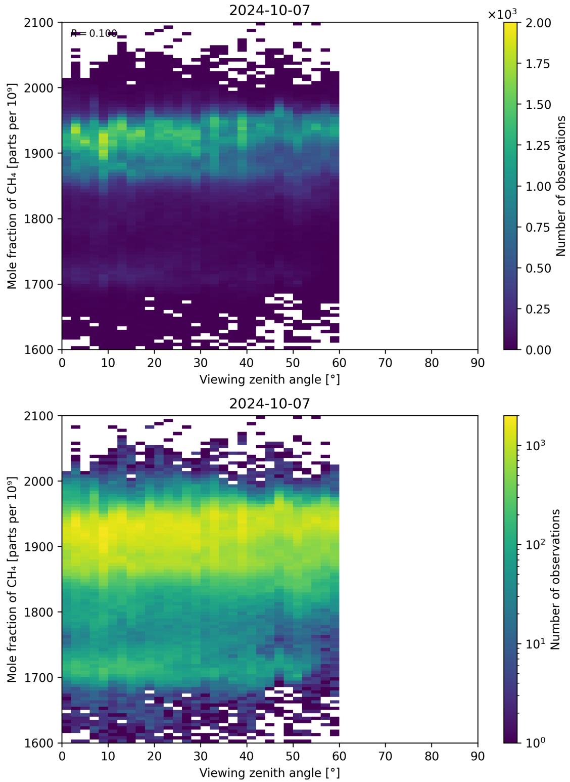
Figure 110: Scatter density plot of “Viewing zenith angle” against “Mole fraction of CH 4 ” for 2024-10-06 to 2024-10-08.
