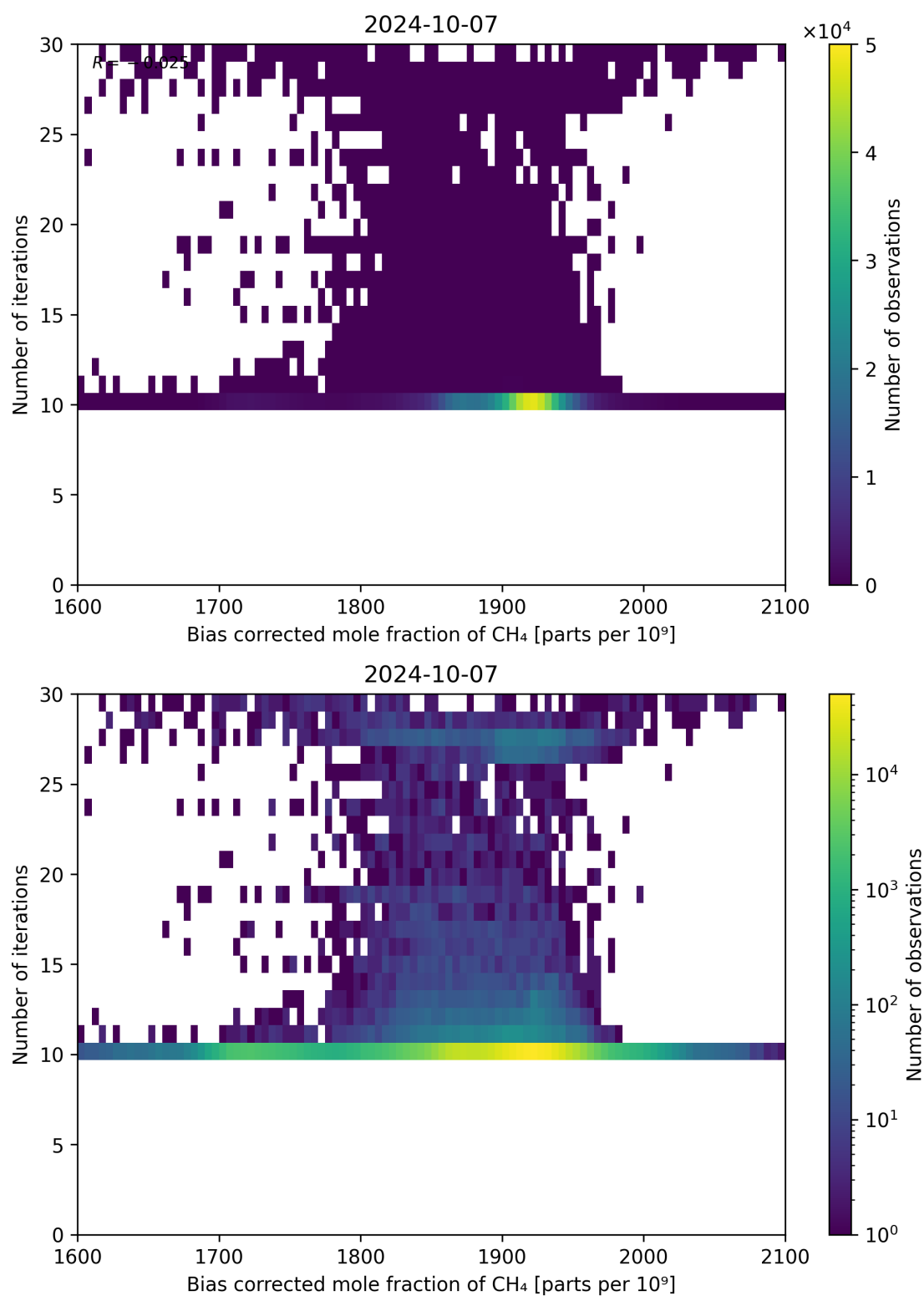
Figure 67: Scatter density plot of “Bias corrected mole fraction of CH 4 ” against “Number of iterations” for 2024-10-06 to 2024-10-08.
