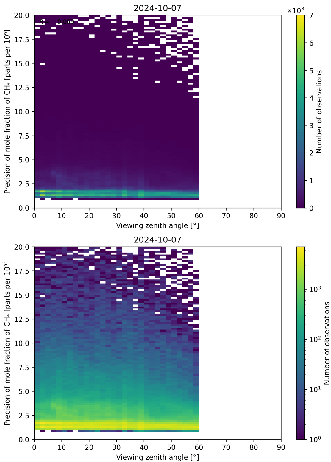
Figure 112: Scatter density plot of “Viewing zenith angle” against “Precision of mole fraction of CH 4 ” for 2024-10-06 to 2024-10-08.
