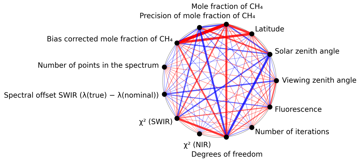
Figure 1: Map of correlation graph for 2024-10-06 to 2024-10-08.
