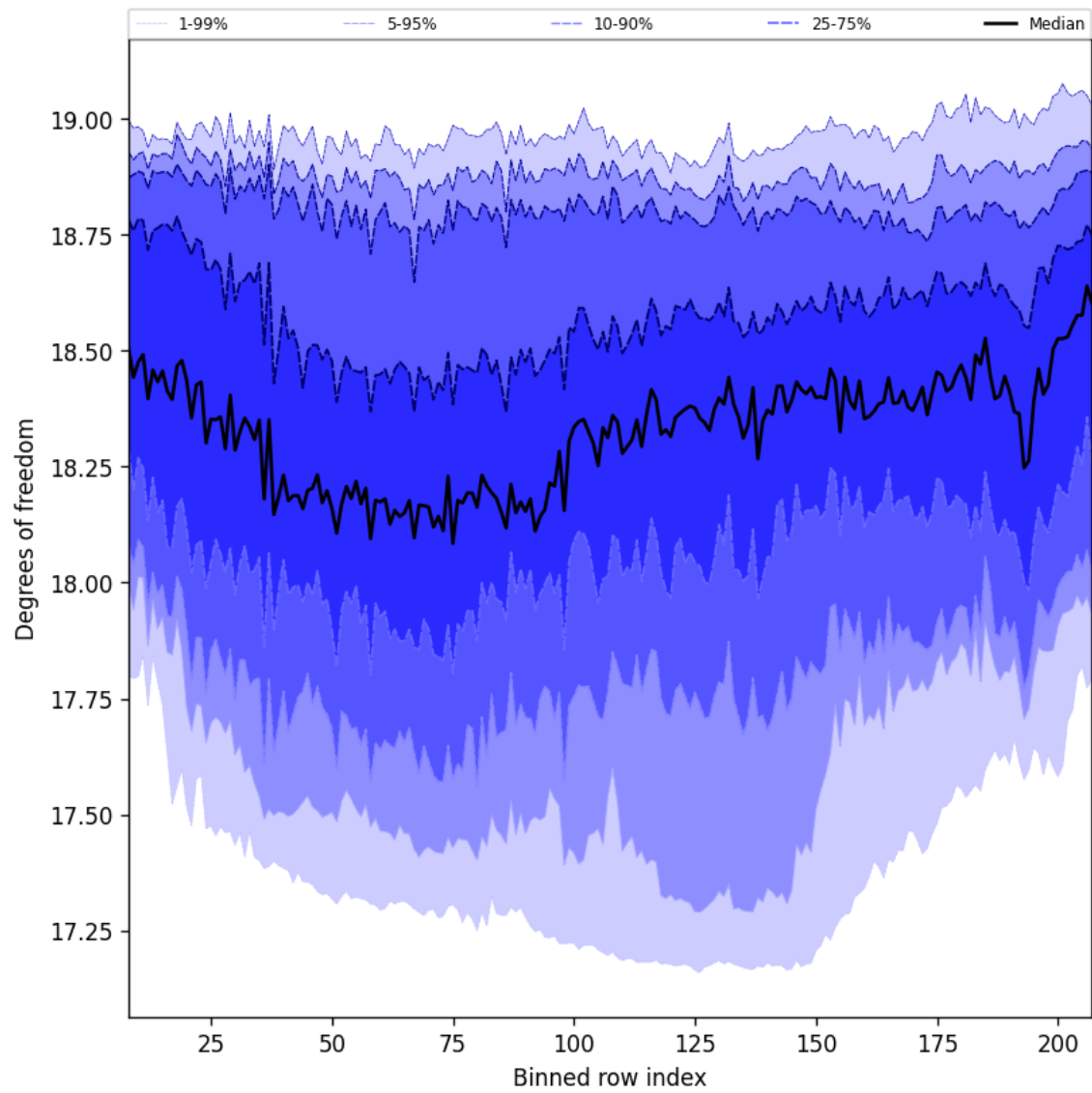
Figure 41: Along track statistics of “Degrees of freedom” for 2024-10-06 to 2024-10-08
