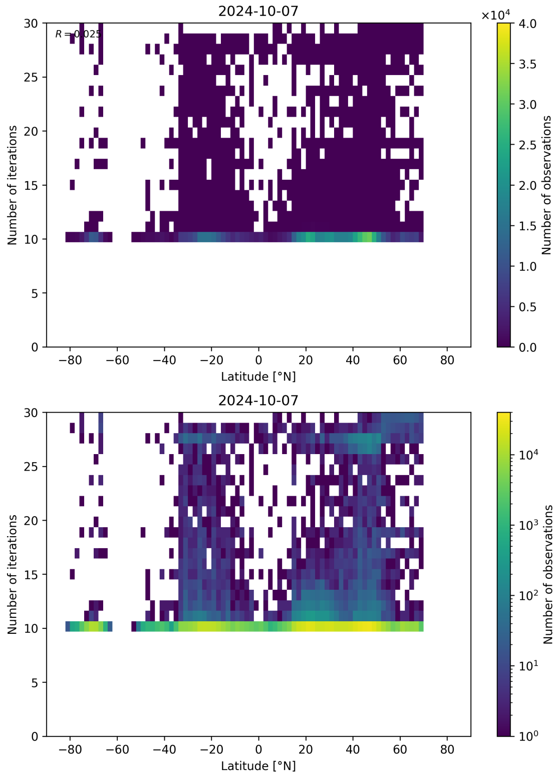
Figure 60: Scatter density plot of “Latitude” against “Number of iterations” for 2024-10-06 to 2024-10-08.
