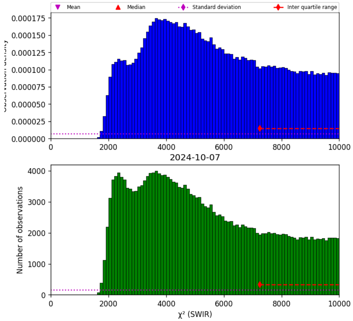
Figure 28: Histogram of “ \chi^2 (SWIR)” for 2024-10-06 to 2024-10-08
