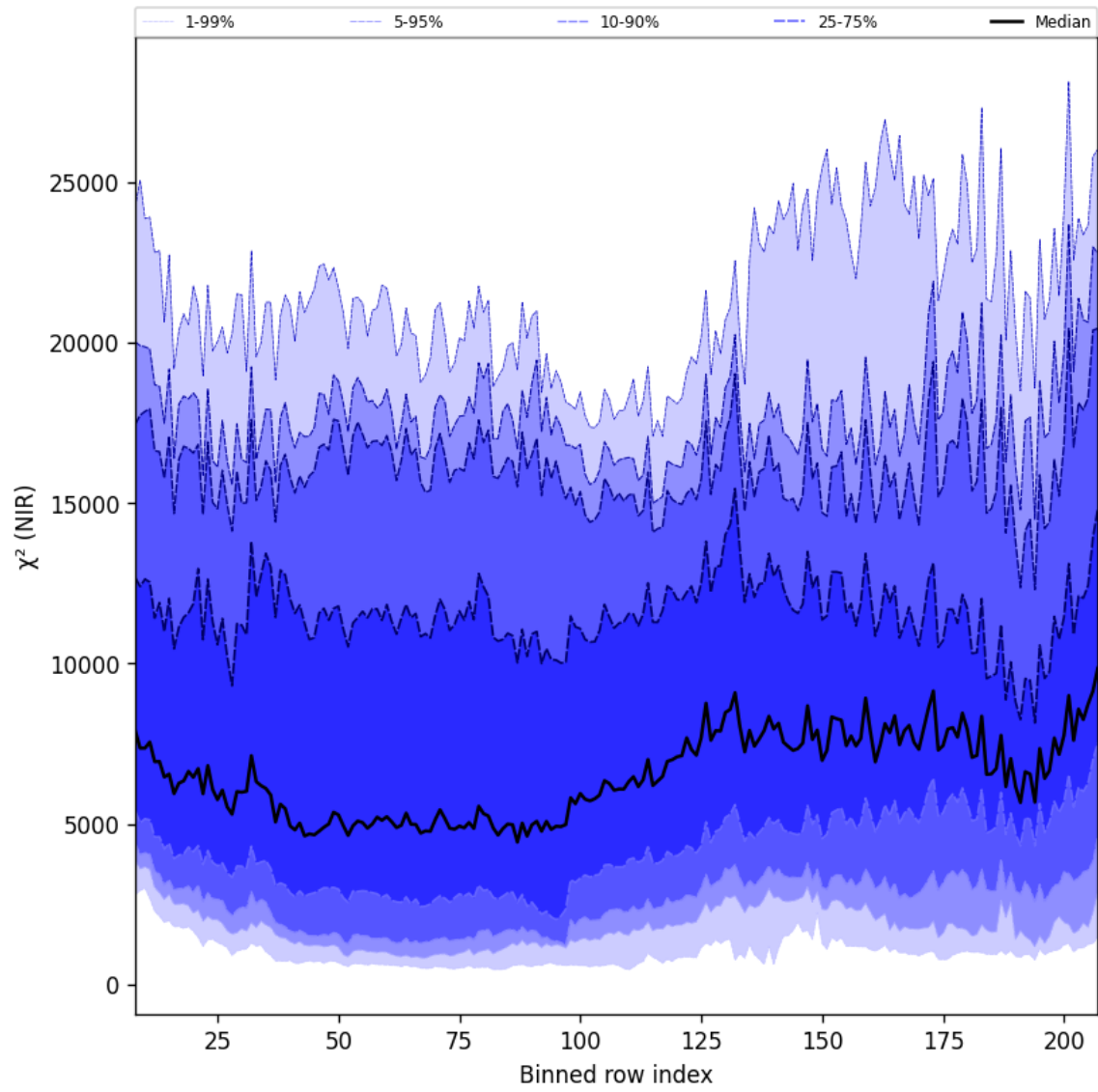
Figure 40: Along track statistics of “ \chi^2 (NIR)” for 2024-10-06 to 2024-10-08
