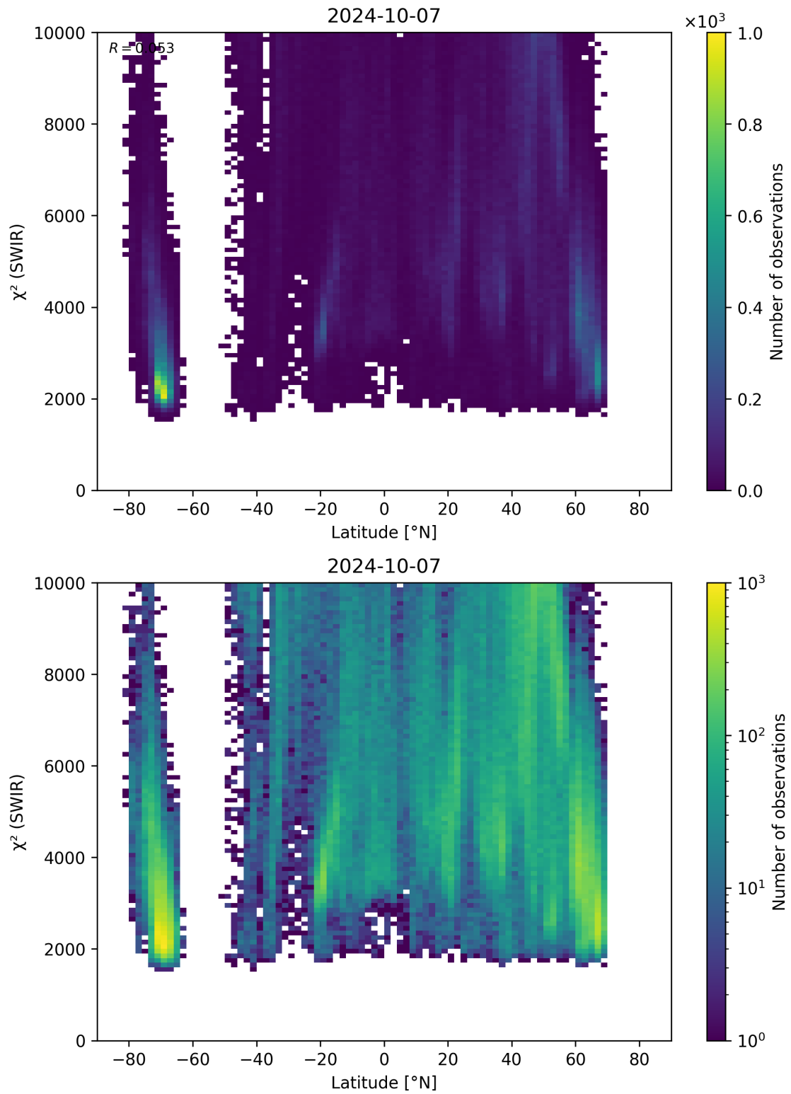
Figure 54: Scatter density plot of “Latitude” against “ \chi^2 (SWIR)” for 2024-10-06 to 2024-10-08.
