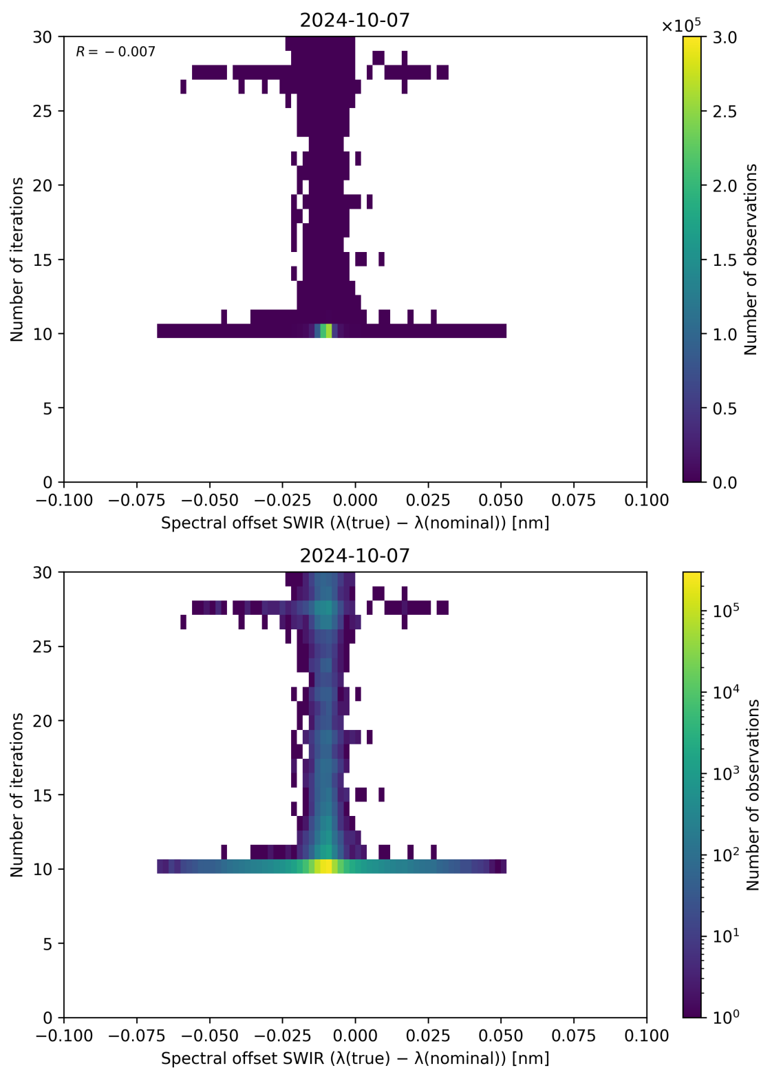
Figure 121: Scatter density plot of “Spectral offset SWIR ( \lambda_{\text{true}} - \lambda_{\text{nominal}} )” against “Number of iterations” for 2024-10-06 to 2024-10-08.
