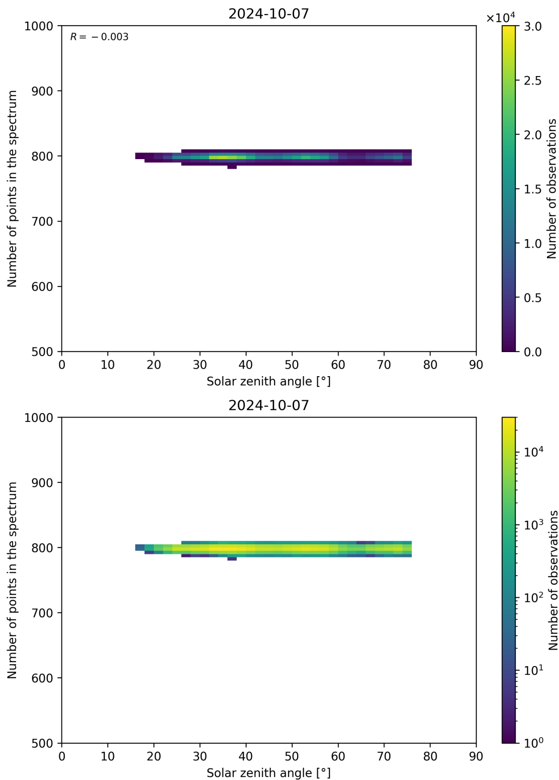
Figure 103: Scatter density plot of “Solar zenith angle” against “Number of points in the spectrum” for 2024-10-06 to 2024-10-08.
