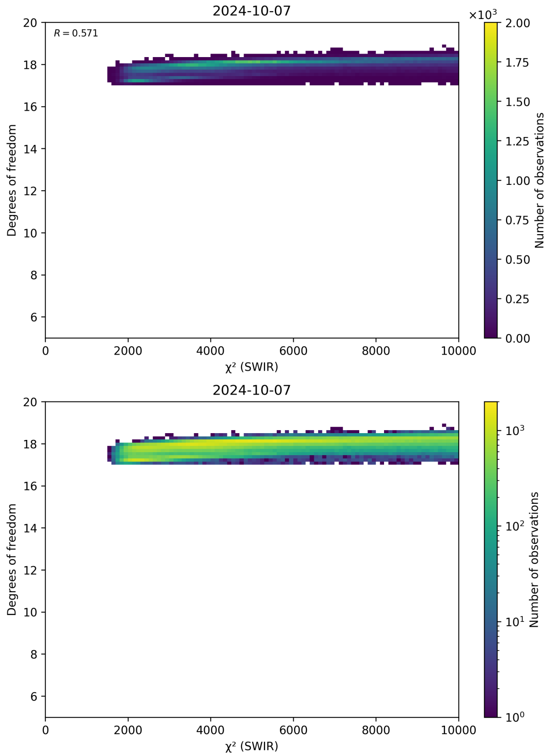
Figure 48: Scatter density plot of “ \chi^2 (SWIR)” against “Degrees of freedom” for 2024-10-06 to 2024-10-08.
