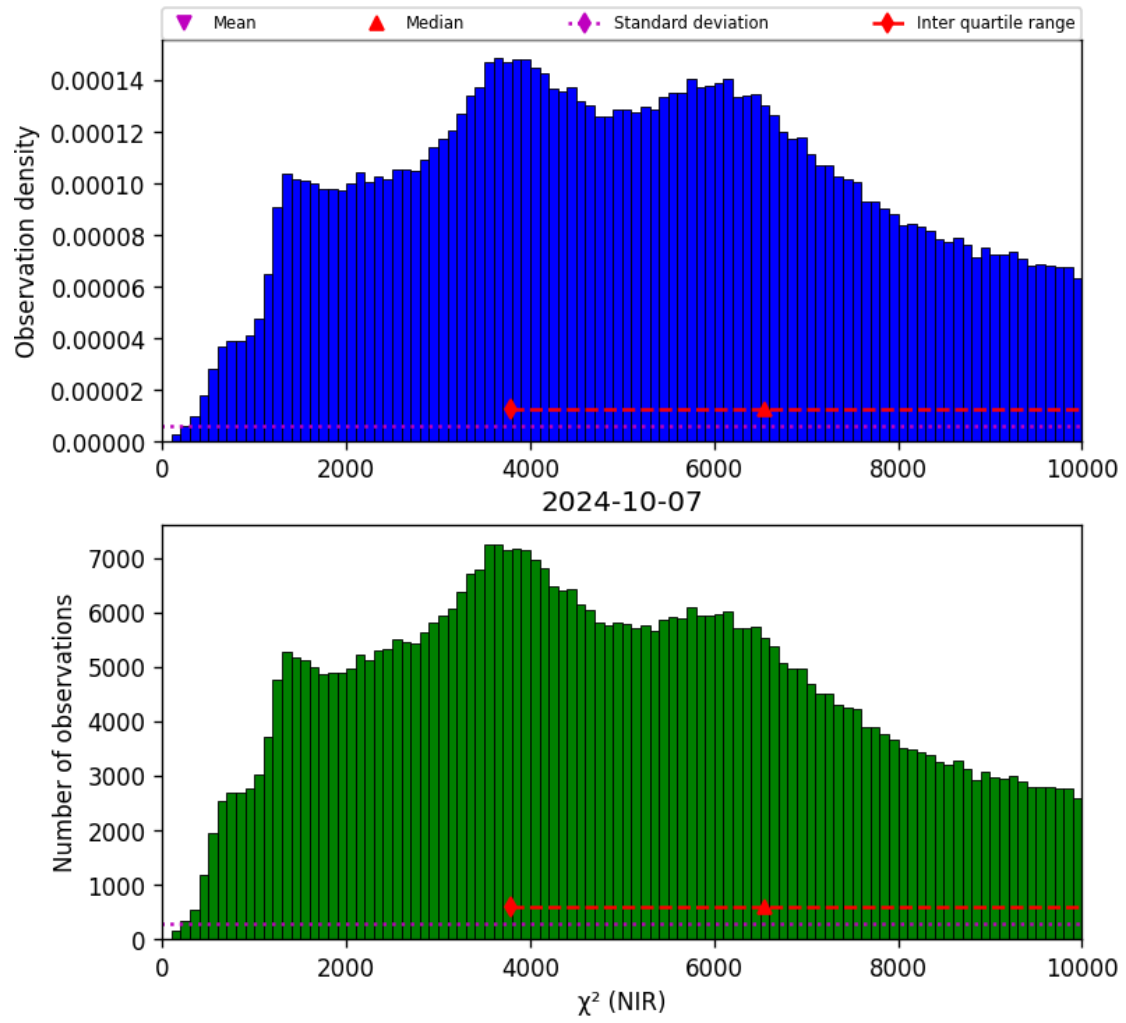
Figure 29: Histogram of " \chi^2 (NIR)" for 2024-10-06 to 2024-10-08
