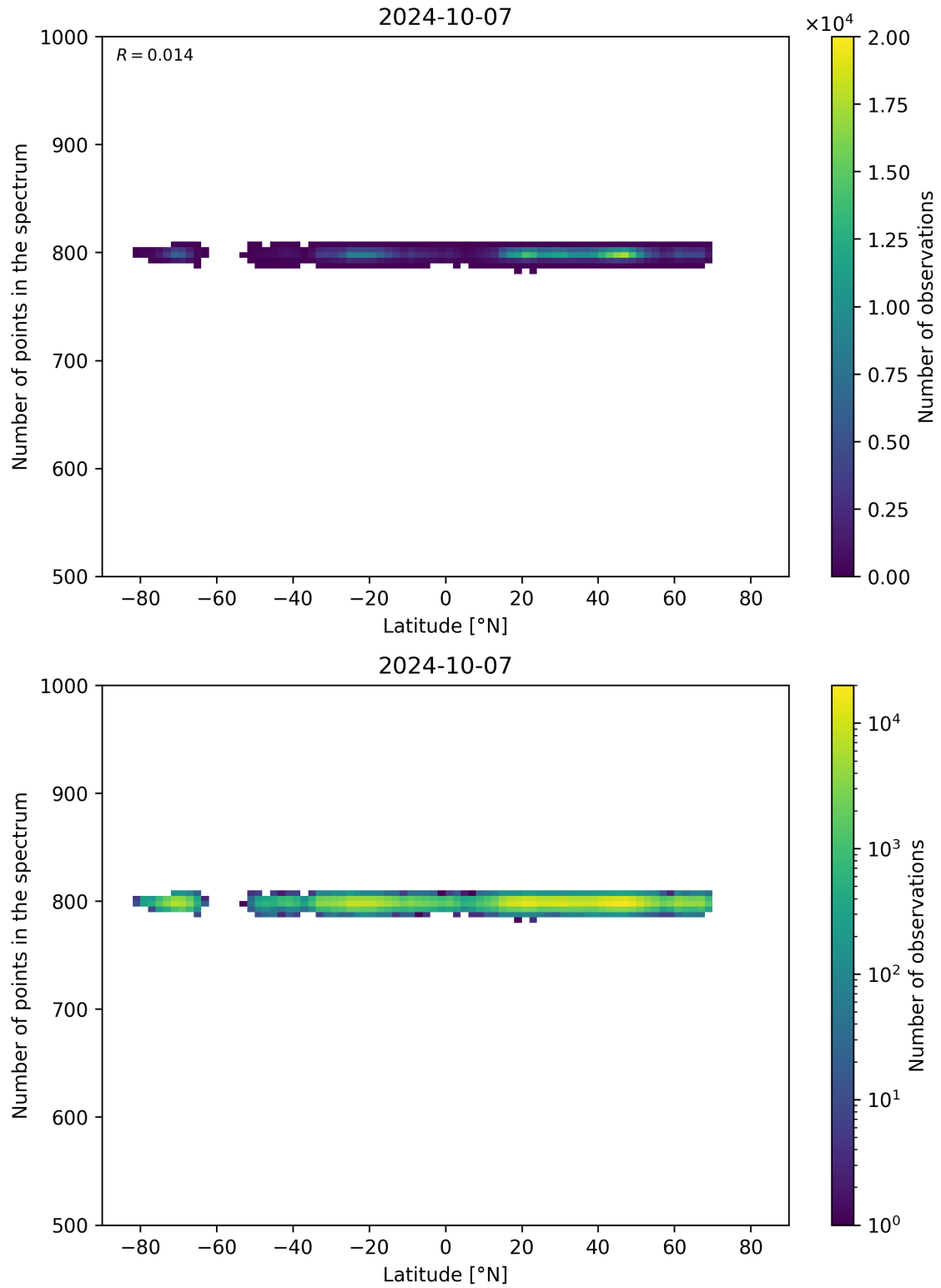
Figure 61: Scatter density plot of “Latitude” against “Number of points in the spectrum” for 2024-10-06 to 2024-10-08.
