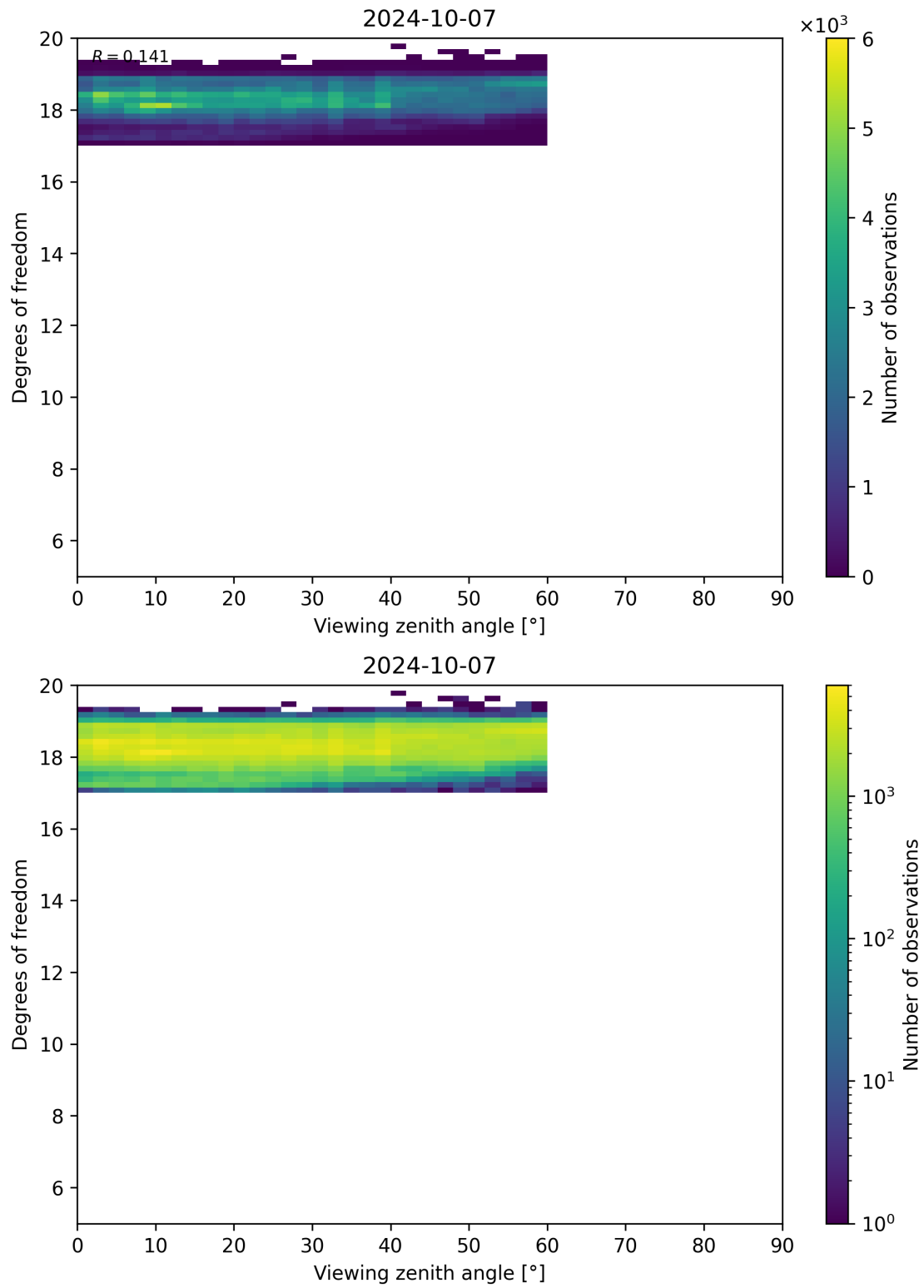
Figure 107: Scatter density plot of “Viewing zenith angle” against “Degrees of freedom” for 2024-10-06 to 2024-10-08.
