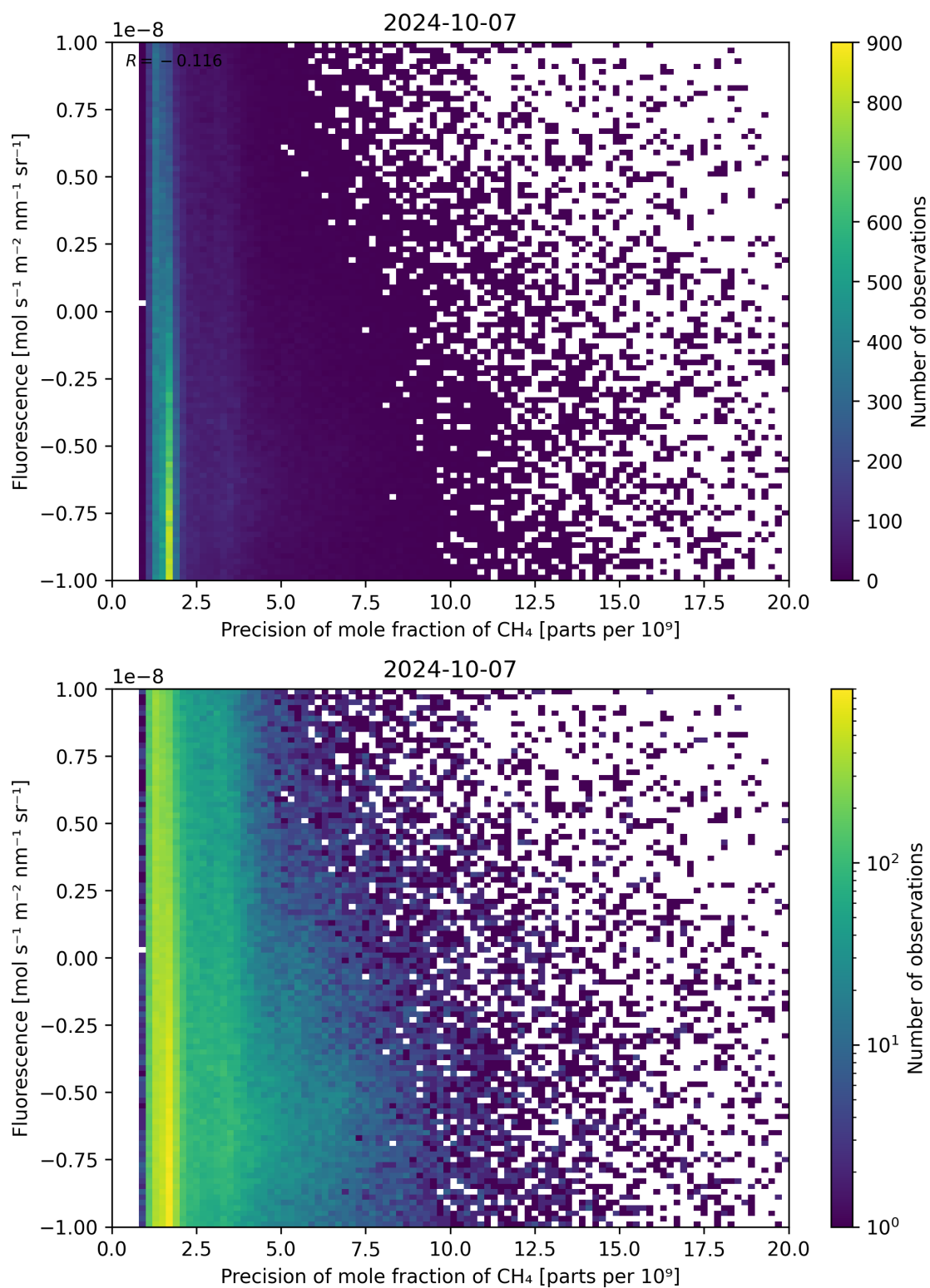
Figure 81: Scatter density plot of “Precision of mole fraction of \text{CH}_4 ” against “Fluorescence” for 2024-10-06 to 2024-10-08.
