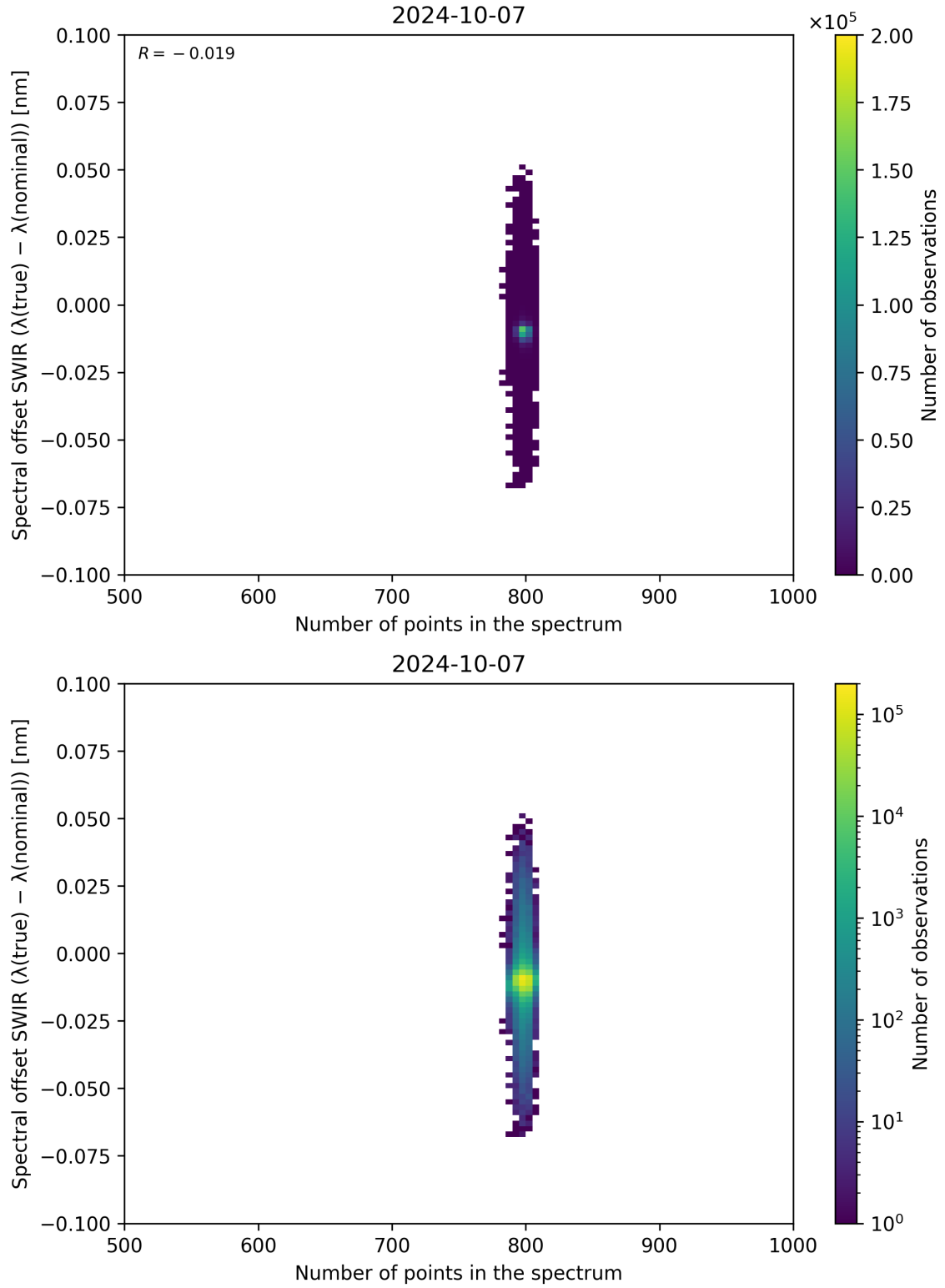
Figure 93: Scatter density plot of “Number of points in the spectrum” against “Spectral offset SWIR ( \lambda_{\text{true}} - \lambda_{\text{nominal}} )” for 2024-10-06 to 2024-10-08.
