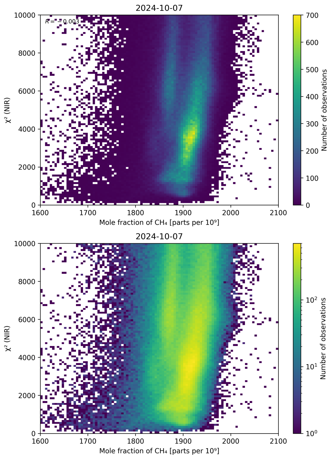
Figure 70: Scatter density plot of “Mole fraction of CH 4 ” against “ \chi^2 (NIR)” for 2024-10-06 to 2024-10-08.
