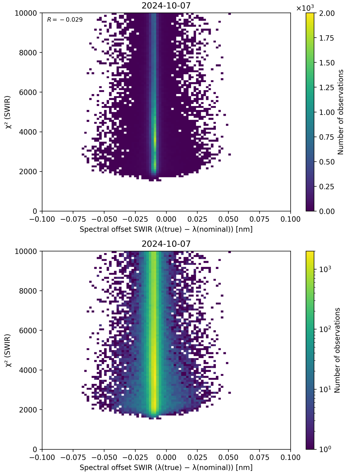
Figure 118: Scatter density plot of “Spectral offset SWIR ( \lambda_{\text{true}} - \lambda_{\text{nominal}} )” against “ \chi^2 (SWIR)” for 2024-10-06 to 2024-10-08.
