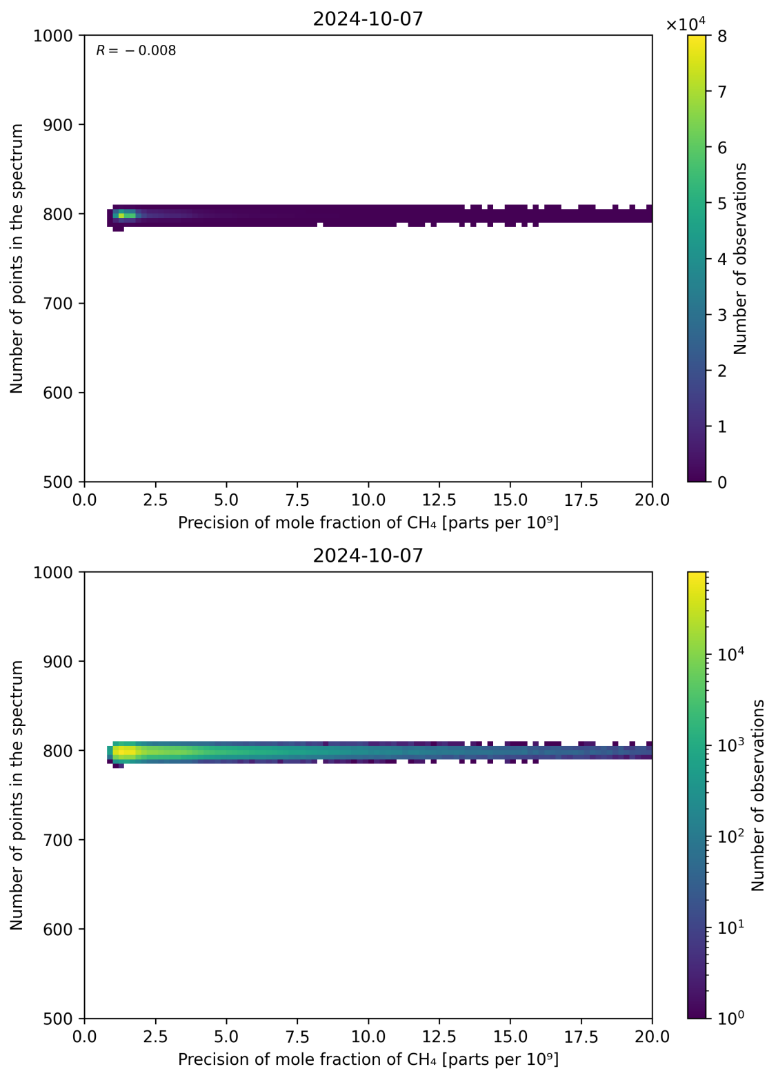
Figure 84: Scatter density plot of “Precision of mole fraction of CH 4 ” against “Number of points in the spectrum” for 2024-10-06 to 2024-10-08.
