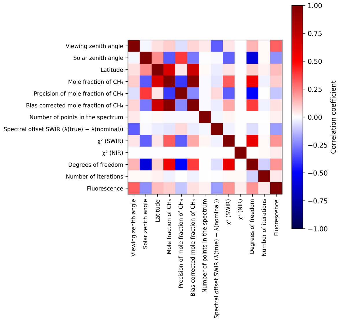
Figure 2: Map of correlation matrix for 2024-10-06 to 2024-10-08.
