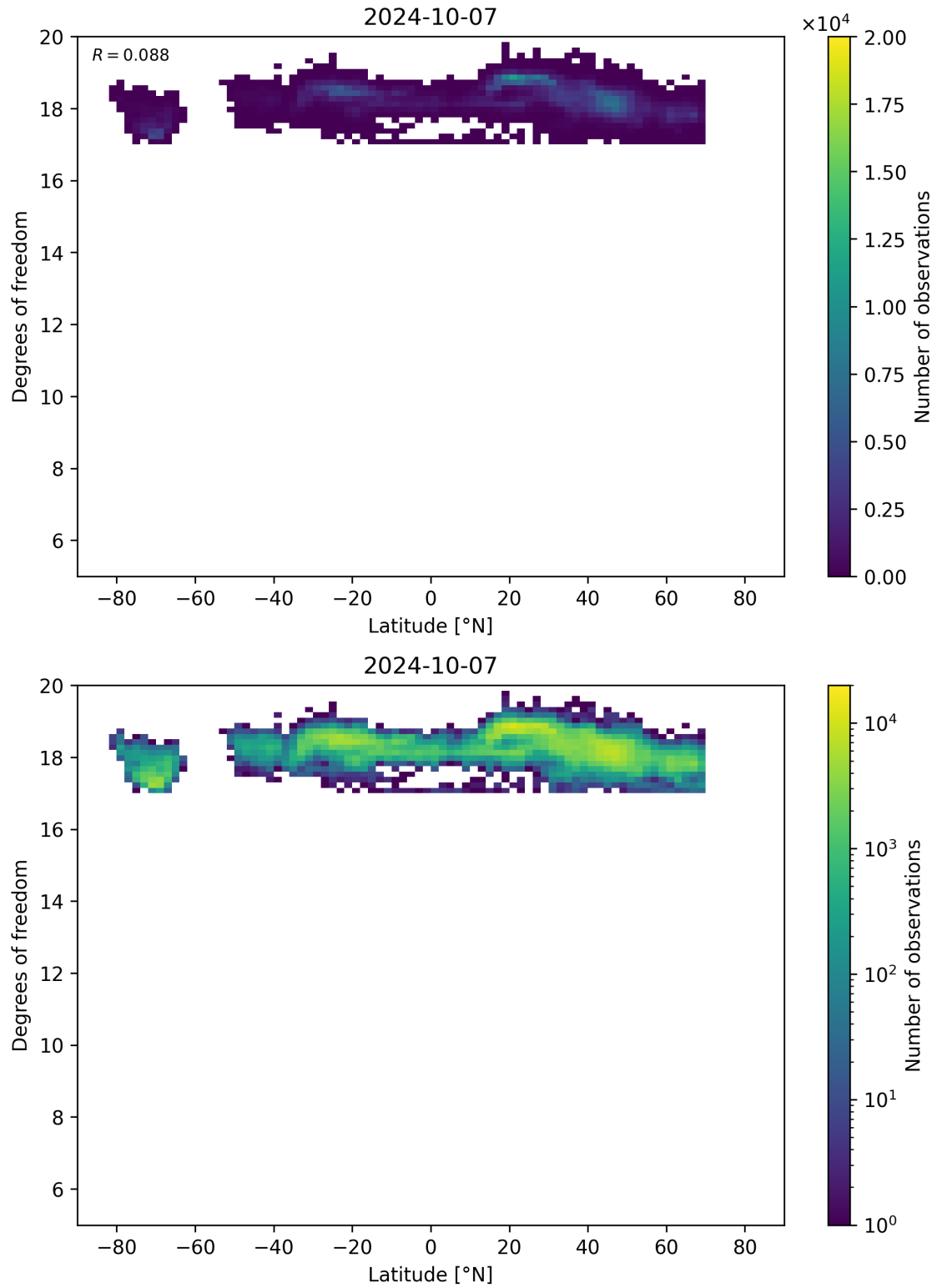
Figure 55: Scatter density plot of “Latitude” against “Degrees of freedom” for 2024-10-06 to 2024-10-08.
