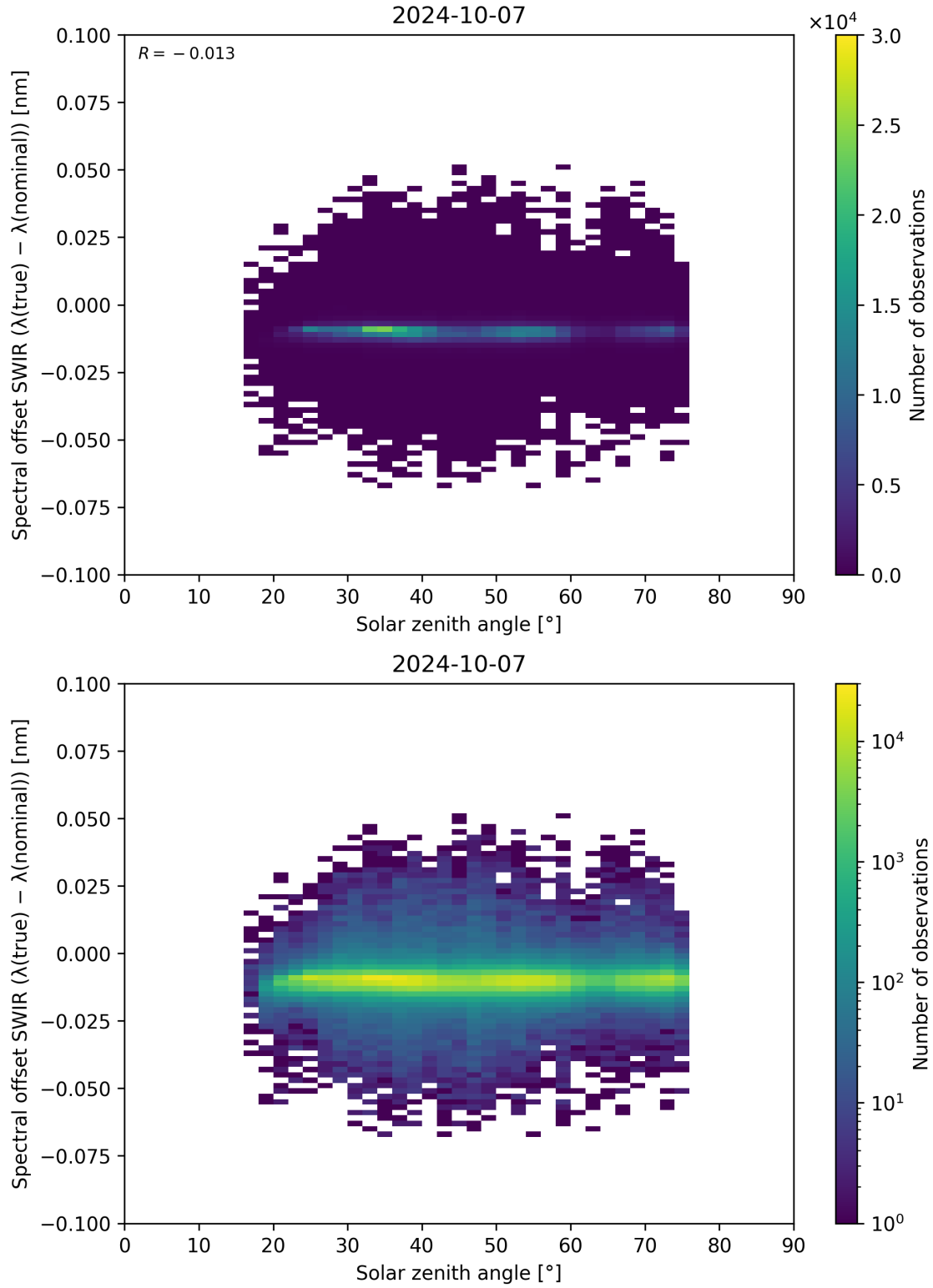
Figure 104: Scatter density plot of “Solar zenith angle” against “Spectral offset SWIR ( \lambda_{\text{true}} - \lambda_{\text{nominal}} )” for 2024-10-06 to 2024-10-08.
