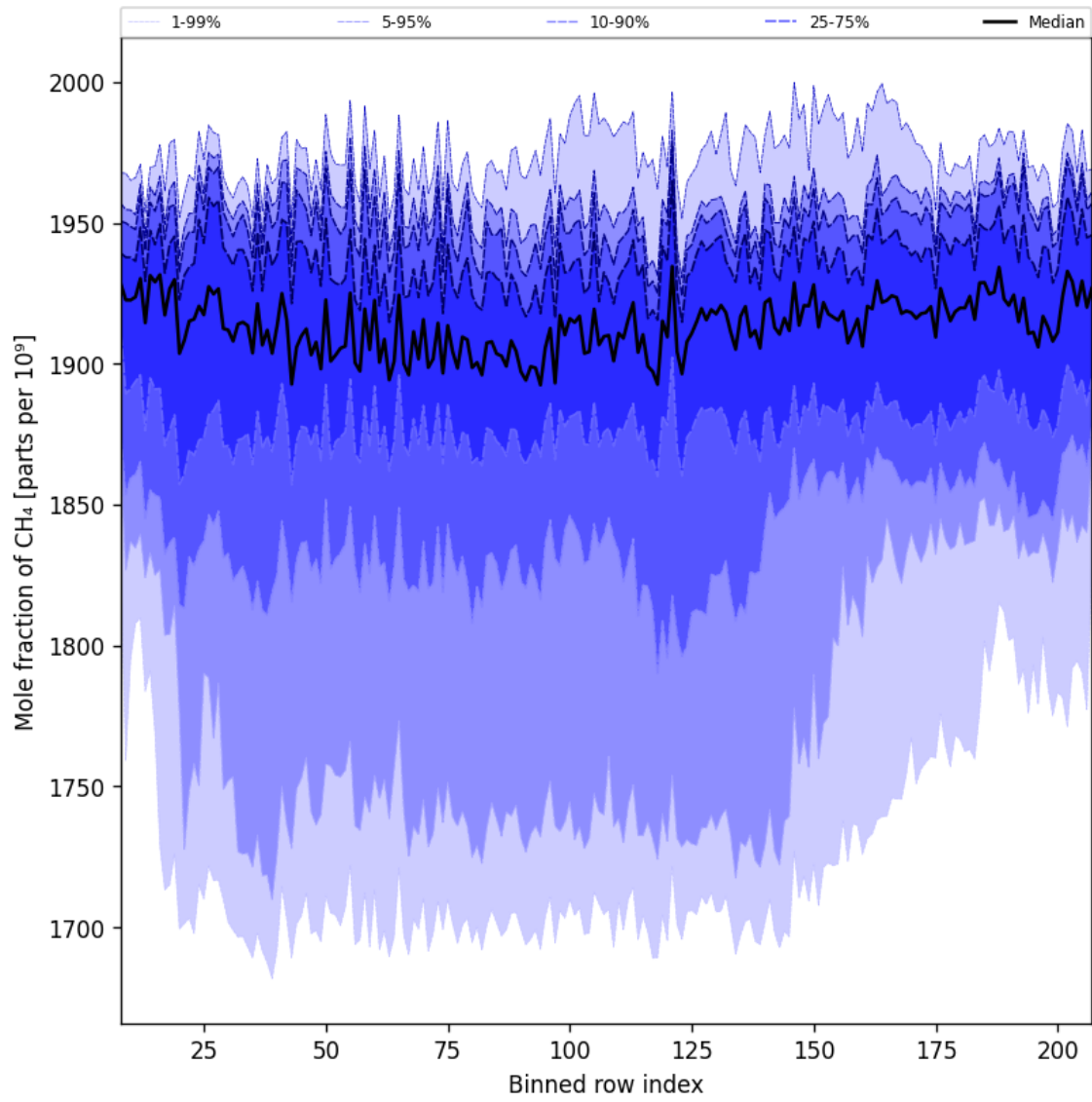
Figure 34: Along track statistics of “Mole fraction of CH 4 ” for 2024-10-06 to 2024-10-08
