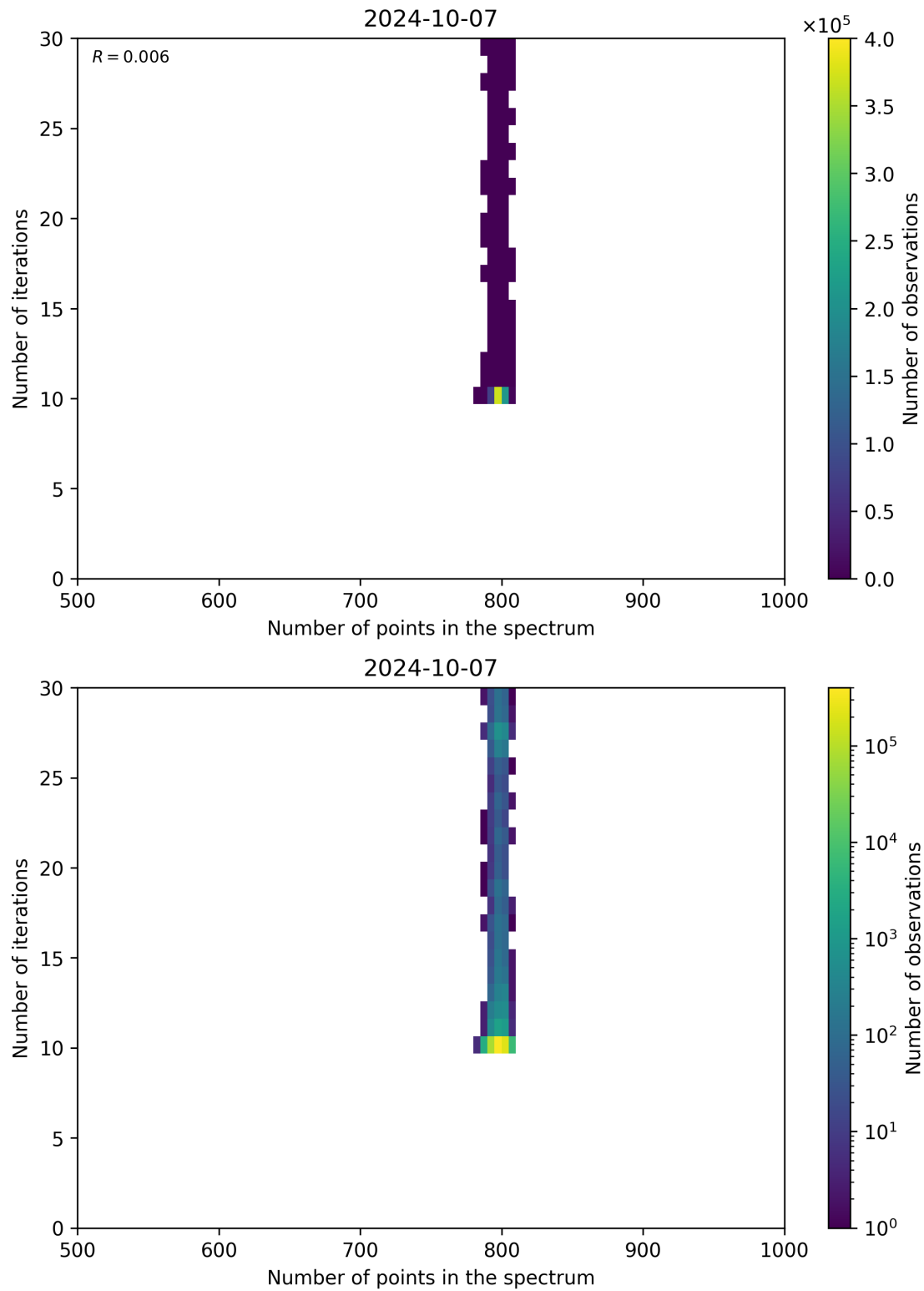
Figure 92: Scatter density plot of “Number of points in the spectrum” against “Number of iterations” for 2024-10-06 to 2024-10-08.
