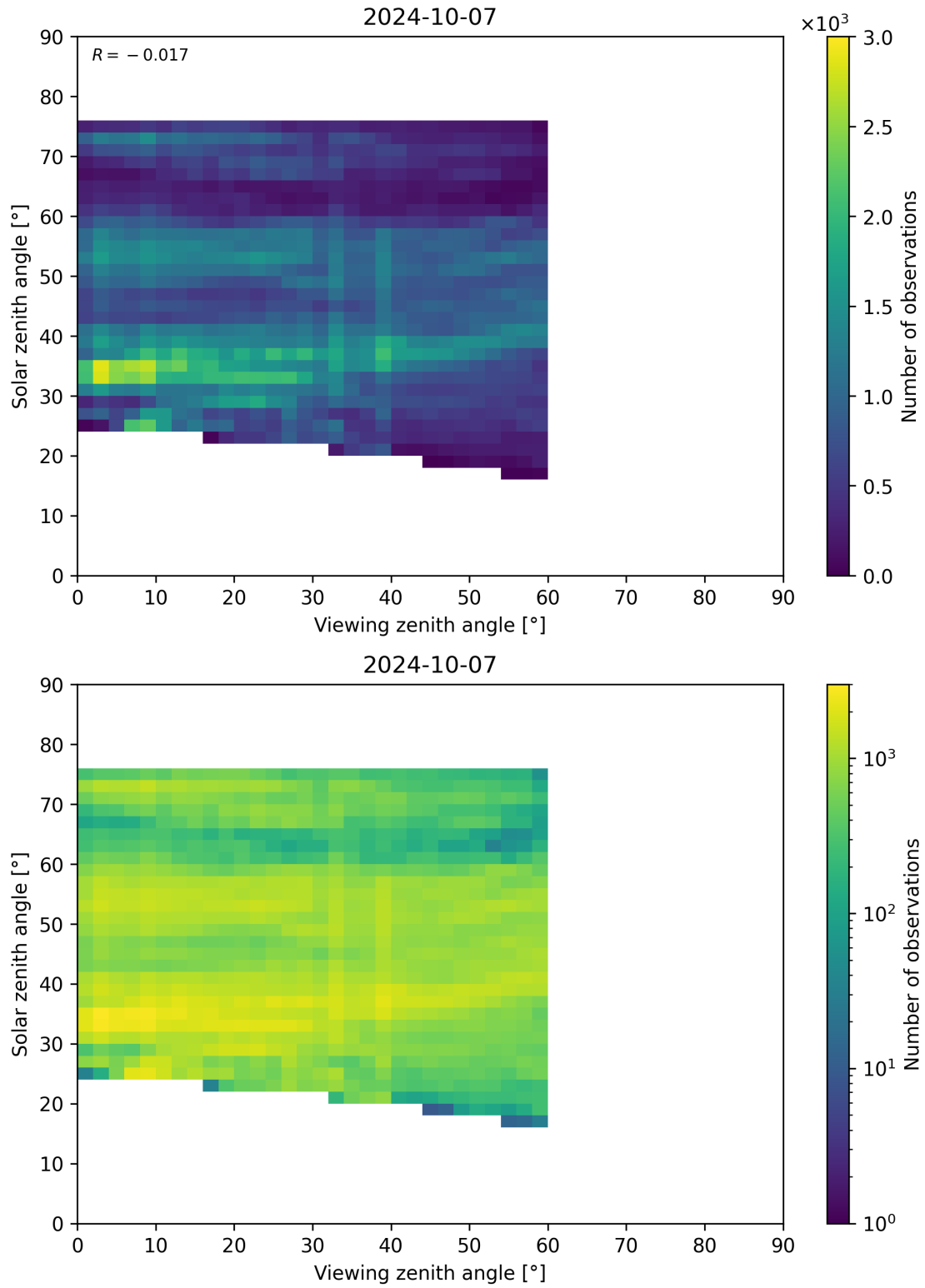
Figure 115: Scatter density plot of “Viewing zenith angle” against “Solar zenith angle” for 2024-10-06 to 2024-10-08.
