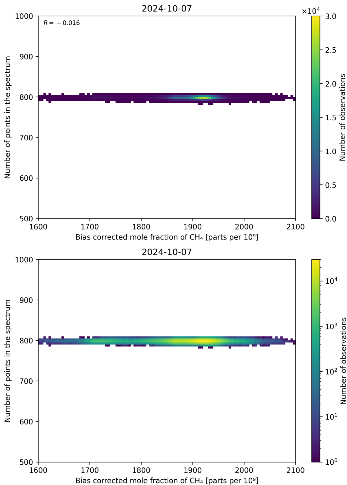
Figure 68: Scatter density plot of “Bias corrected mole fraction of CH 4 ” against “Number of points in the spectrum” for 2024-10-06 to 2024-10-08.
