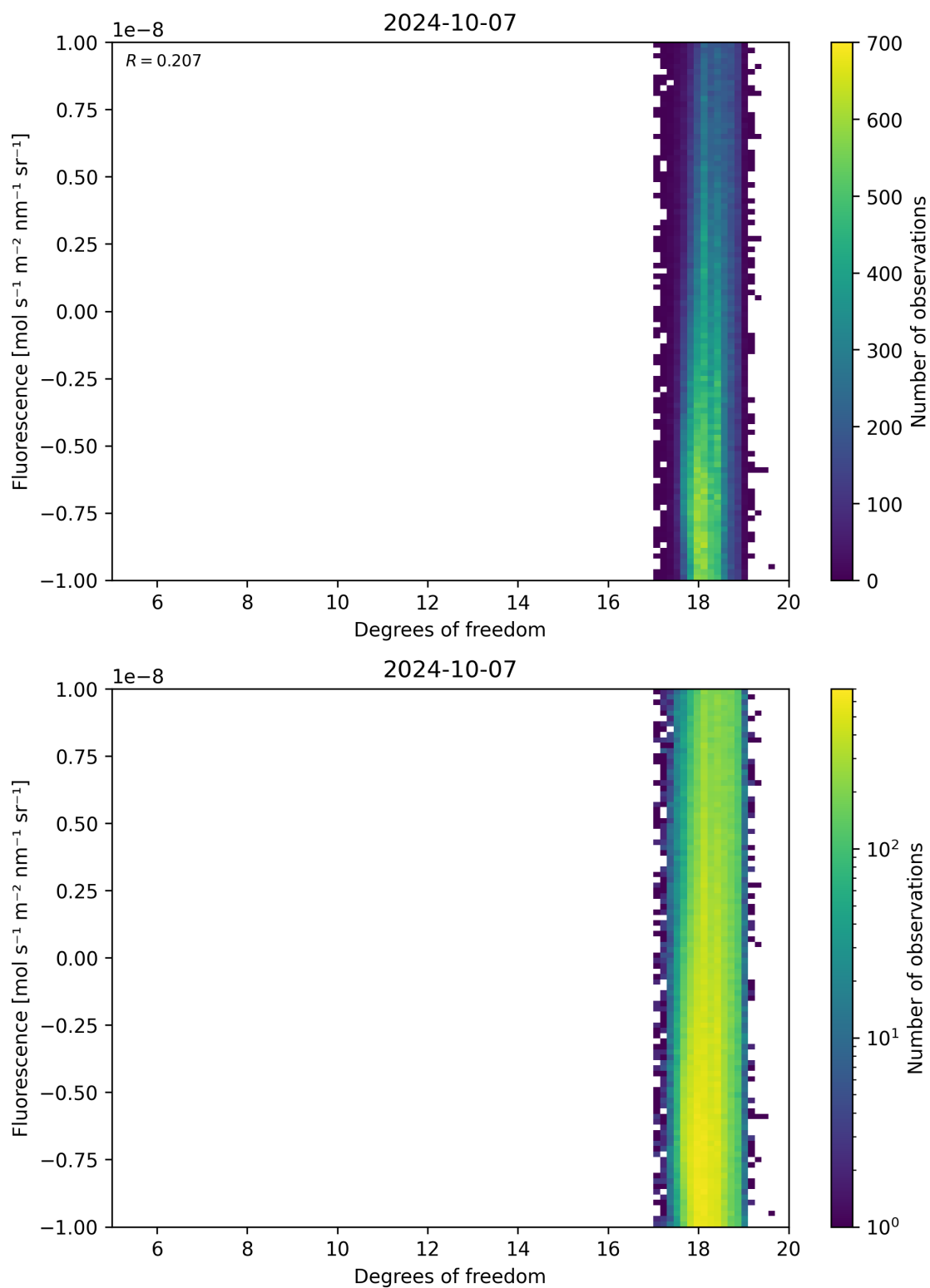
Figure 51: Scatter density plot of “Degrees of freedom” against “Fluorescence” for 2024-10-06 to 2024-10-08.
