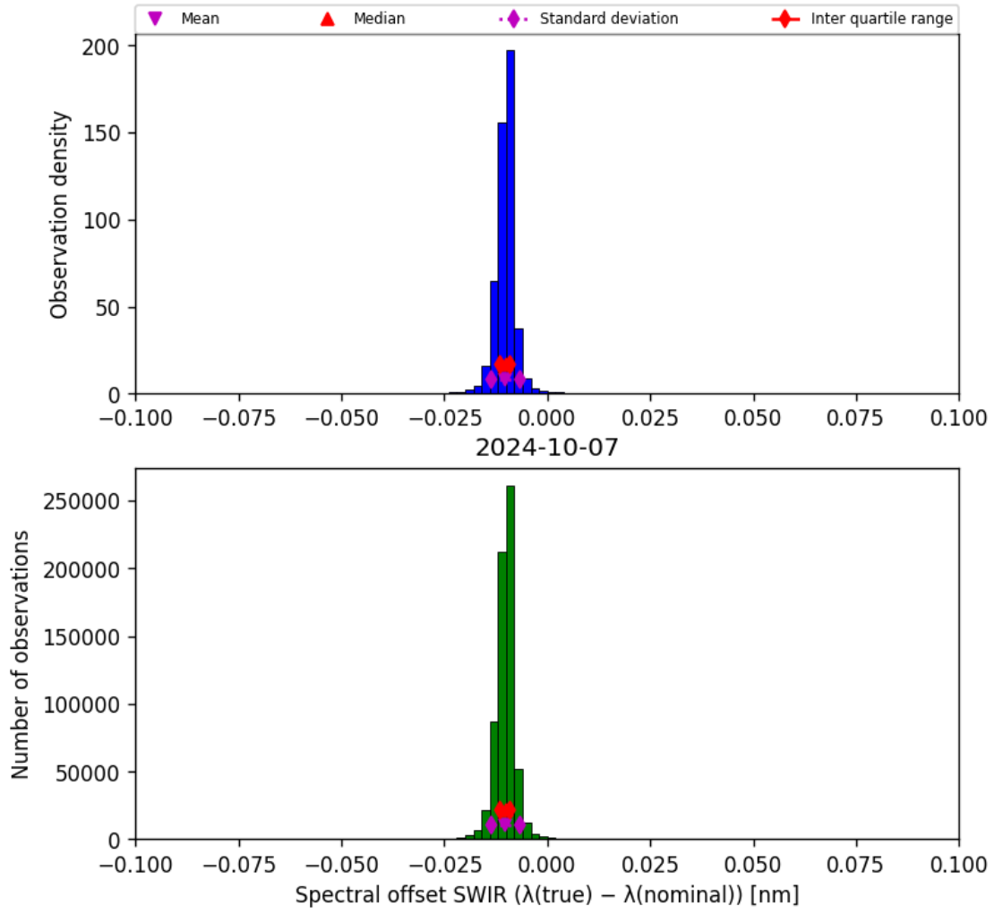
Figure 27: Histogram of “Spectral offset SWIR ( \lambda_{\text{true}} - \lambda_{\text{nominal}} )” for 2024-10-06 to 2024-10-08
