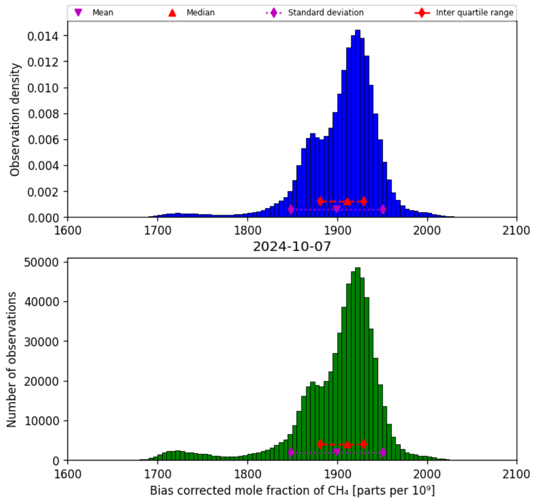
Figure 25: Histogram of “Bias corrected mole fraction of CH 4 ” for 2024-10-06 to 2024-10-08
