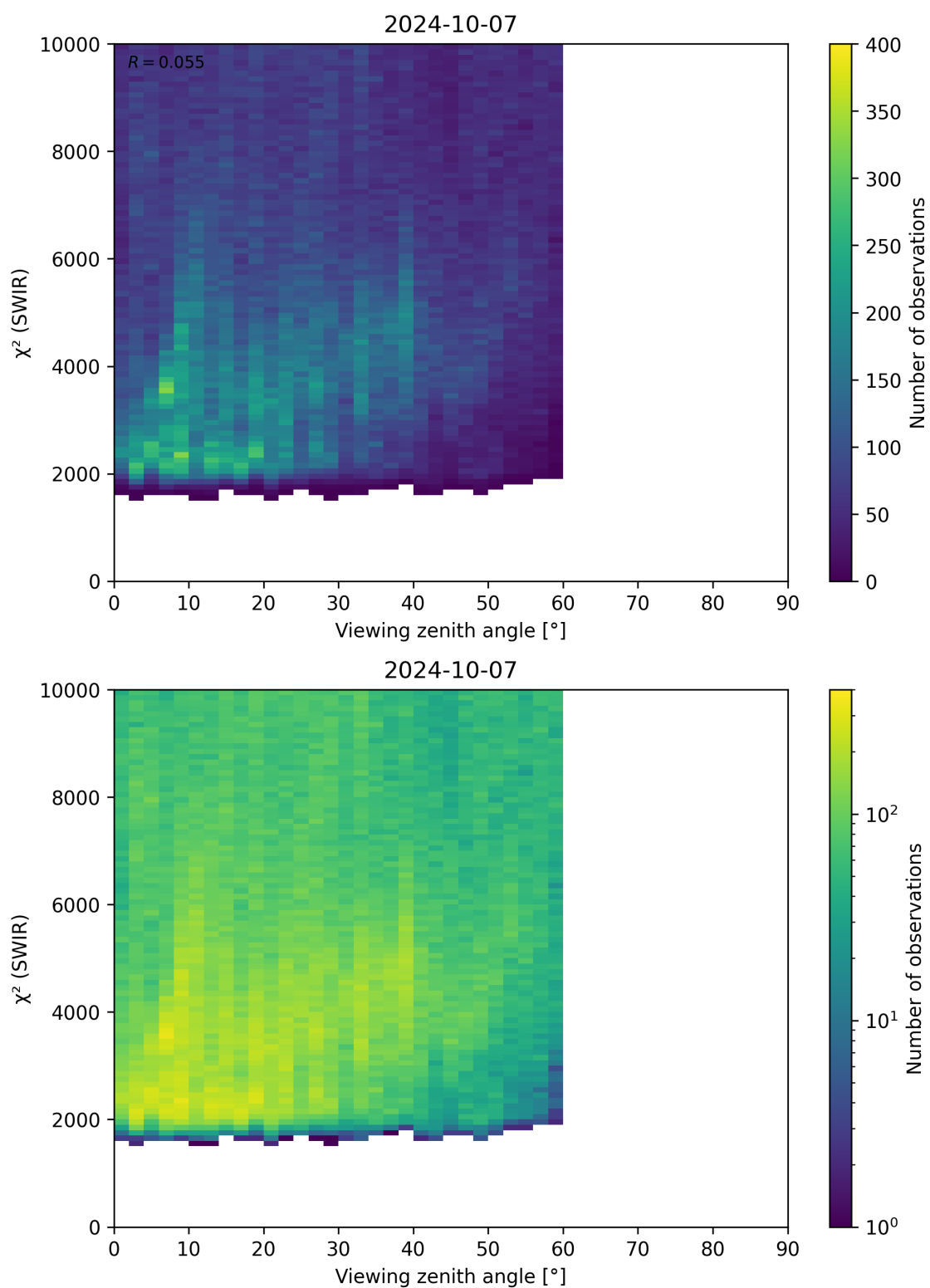
Figure 106: Scatter density plot of “Viewing zenith angle” against “ \chi^2 (SWIR)” for 2024-10-06 to 2024-10-08.
