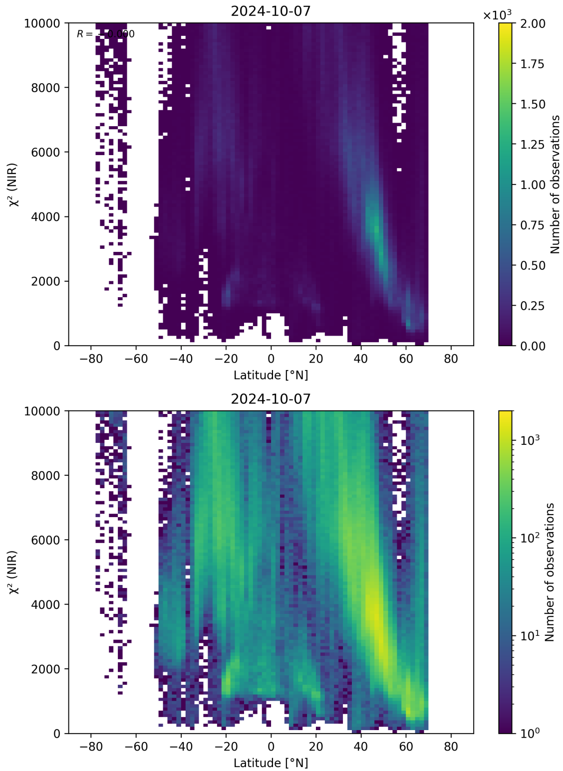
Figure 53: Scatter density plot of “Latitude” against “ \chi^2 (NIR)” for 2024-10-06 to 2024-10-08.
