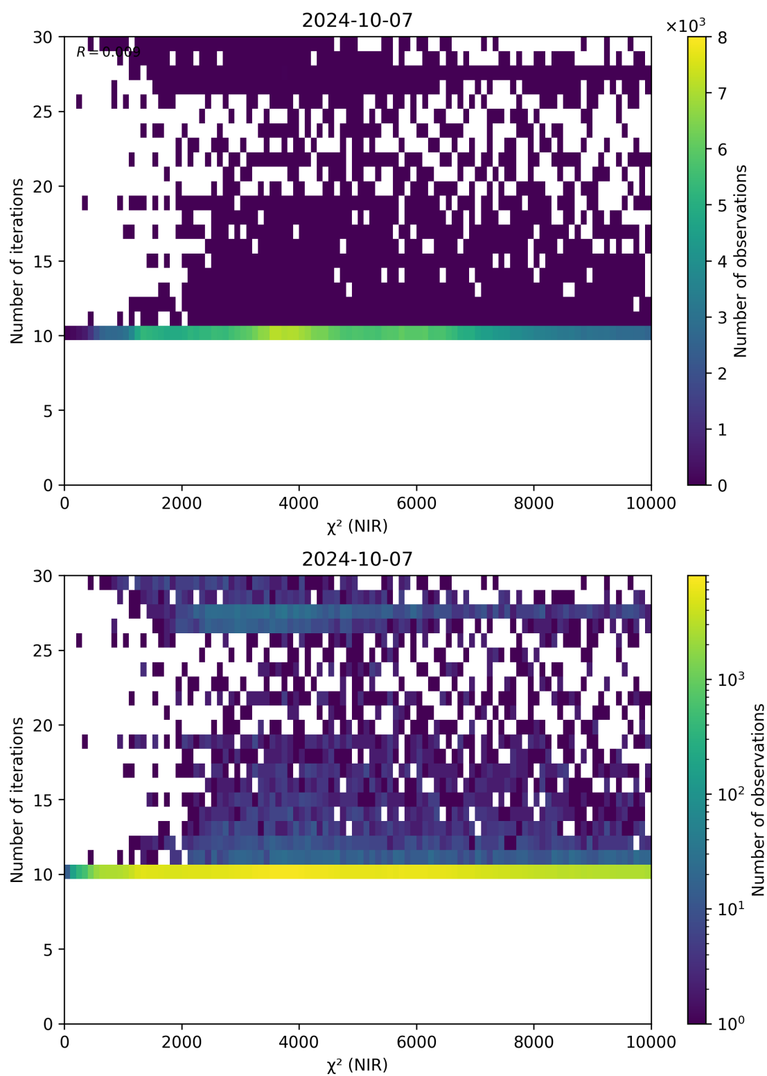
Figure 46: Scatter density plot of “ \chi^2 (NIR)” against “Number of iterations” for 2024-10-06 to 2024-10-08.
