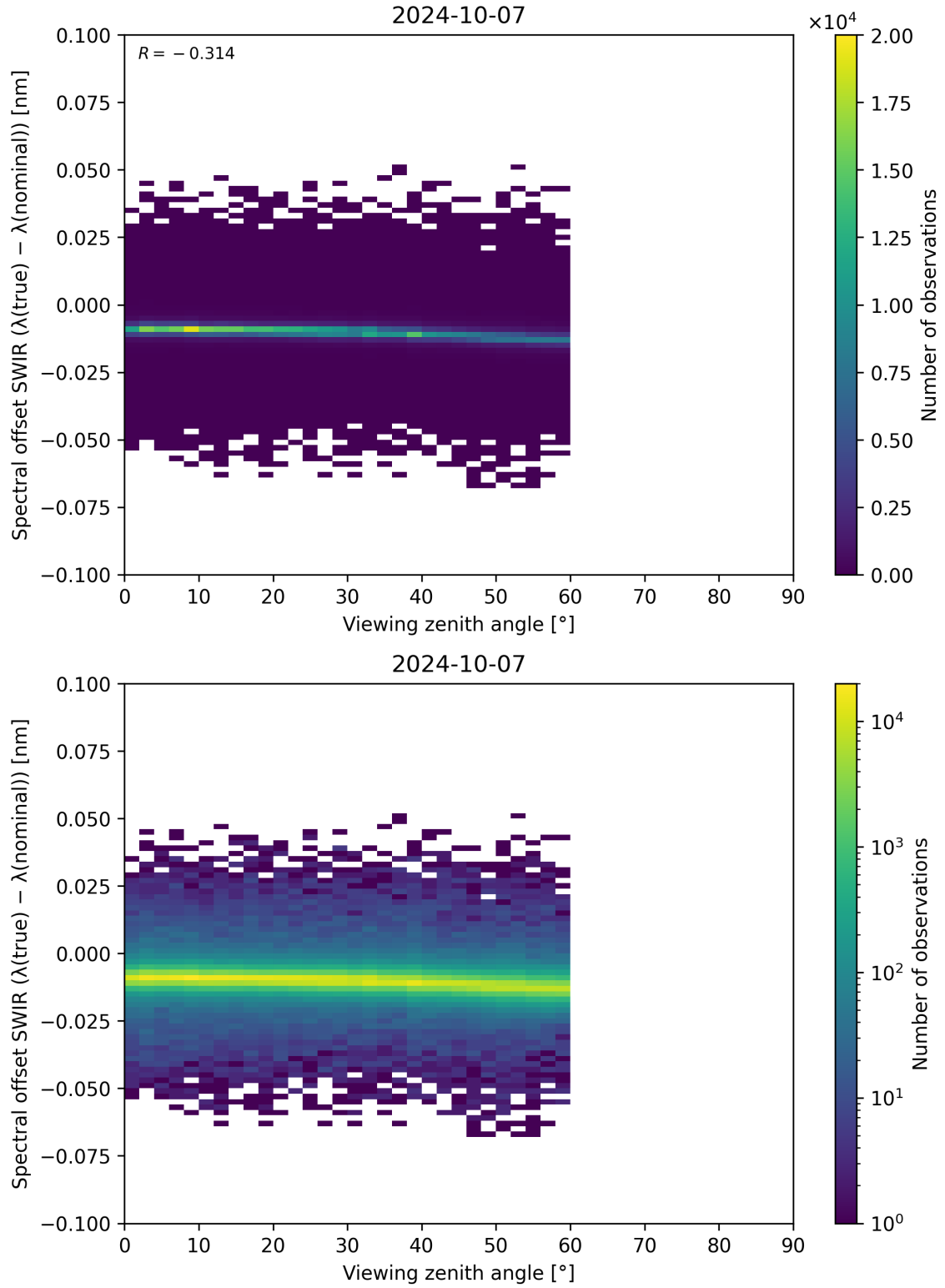
Figure 116: Scatter density plot of “Viewing zenith angle” against “Spectral offset SWIR ( \lambda_{\text{true}} - \lambda_{\text{nominal}} )” for 2024-10-06 to 2024-10-08.
