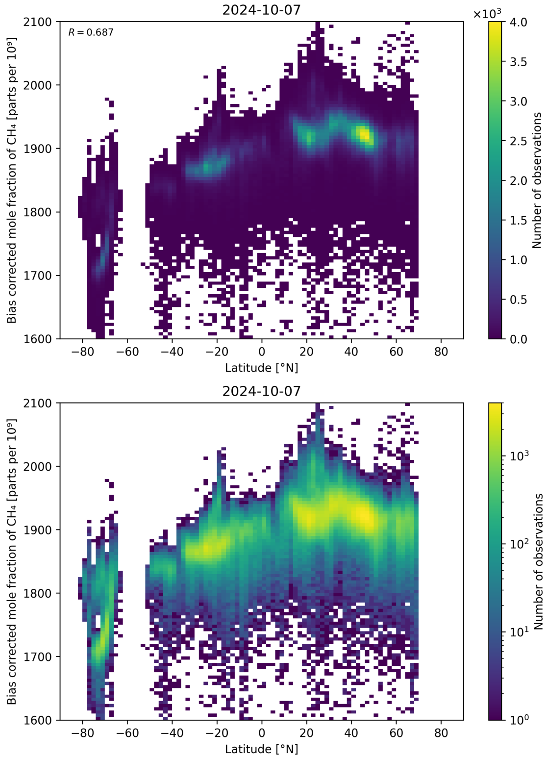
Figure 58: Scatter density plot of “Latitude” against “Bias corrected mole fraction of CH 4 ” for 2024-10-06 to 2024-10-08.
