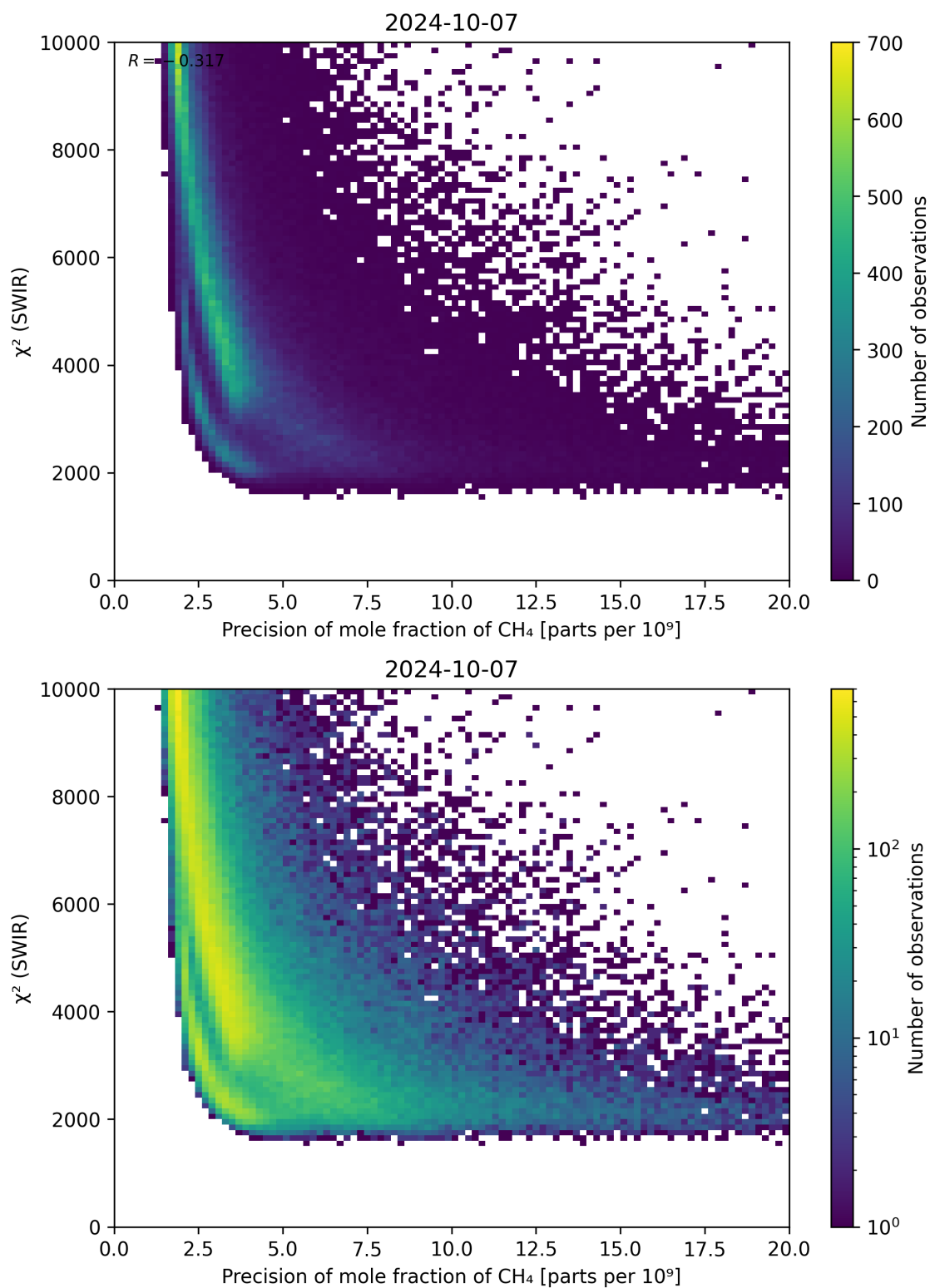
Figure 79: Scatter density plot of “Precision of mole fraction of CH 4 ” against “ \chi^2 (SWIR)” for 2024-10-06 to 2024-10-08.
