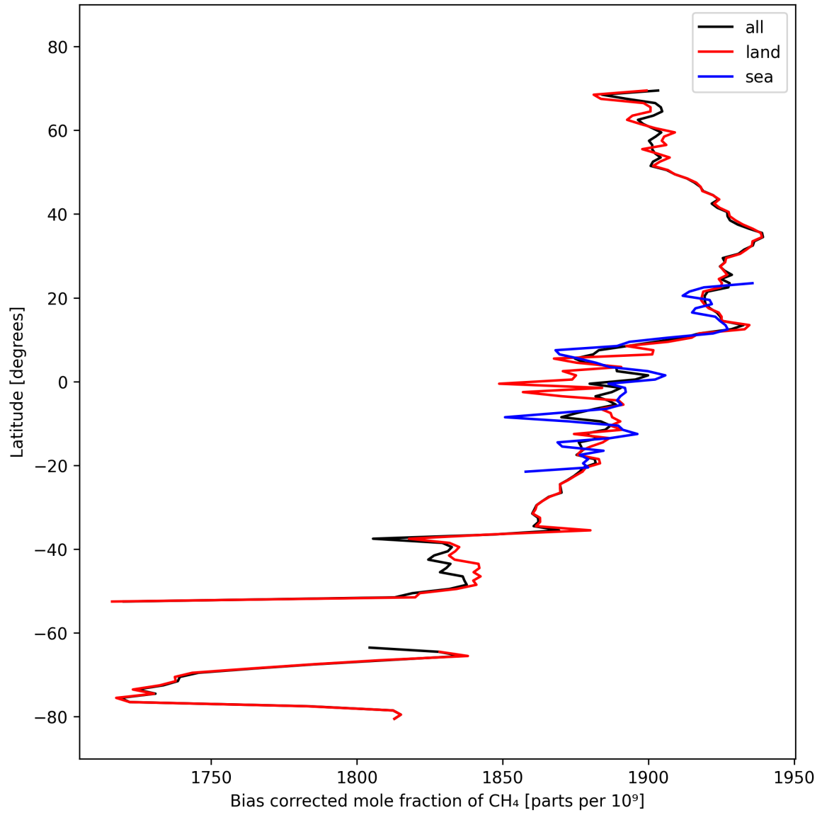
Figure 14: Zonal average of “Bias corrected mole fraction of CH 4 ” for 2024-10-06 to 2024-10-08.
