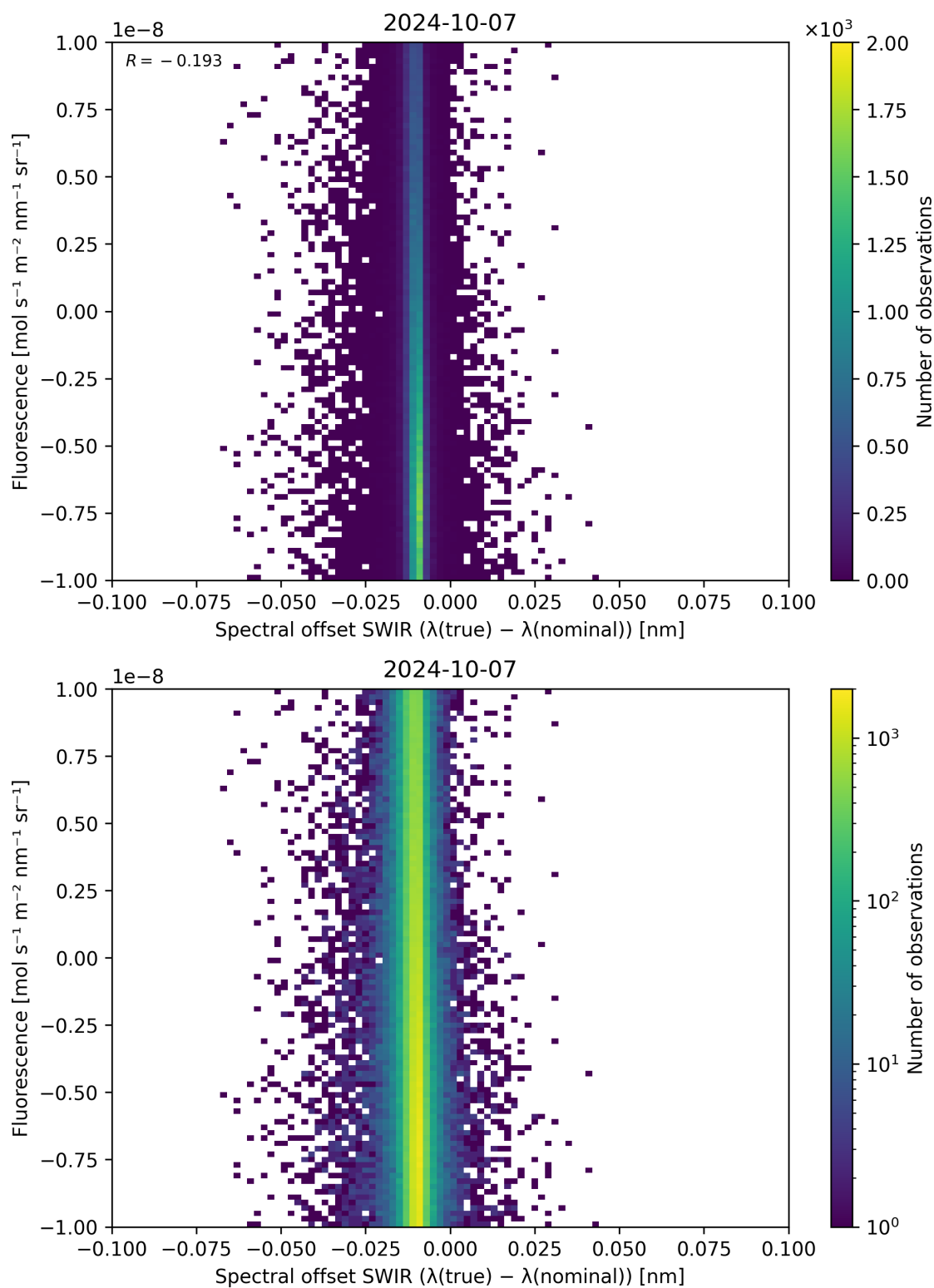
Figure 120: Scatter density plot of “Spectral offset SWIR ( \lambda_{\text{true}} - \lambda_{\text{nominal}} )” against “Fluorescence” for 2024-10-06 to 2024-10-08.
