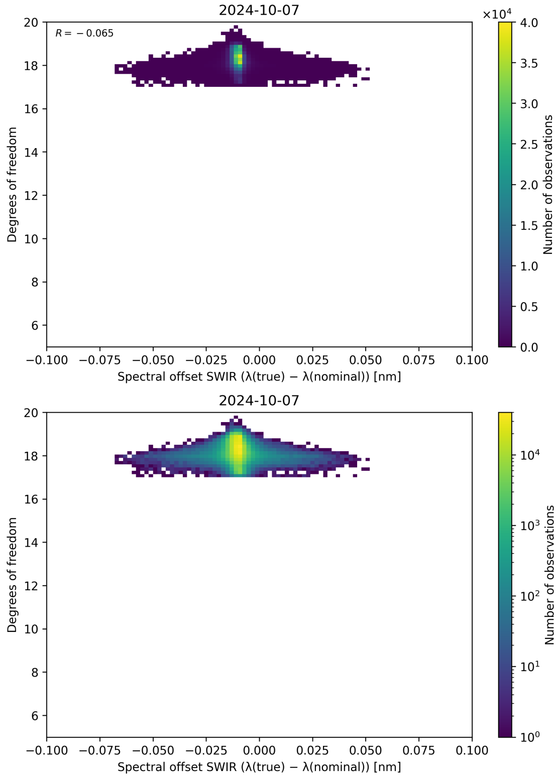
Figure 119: Scatter density plot of “Spectral offset SWIR ( \lambda_{\text{true}} - \lambda_{\text{nominal}} )” against “Degrees of freedom” for 2024-10-06 to 2024-10-08.
