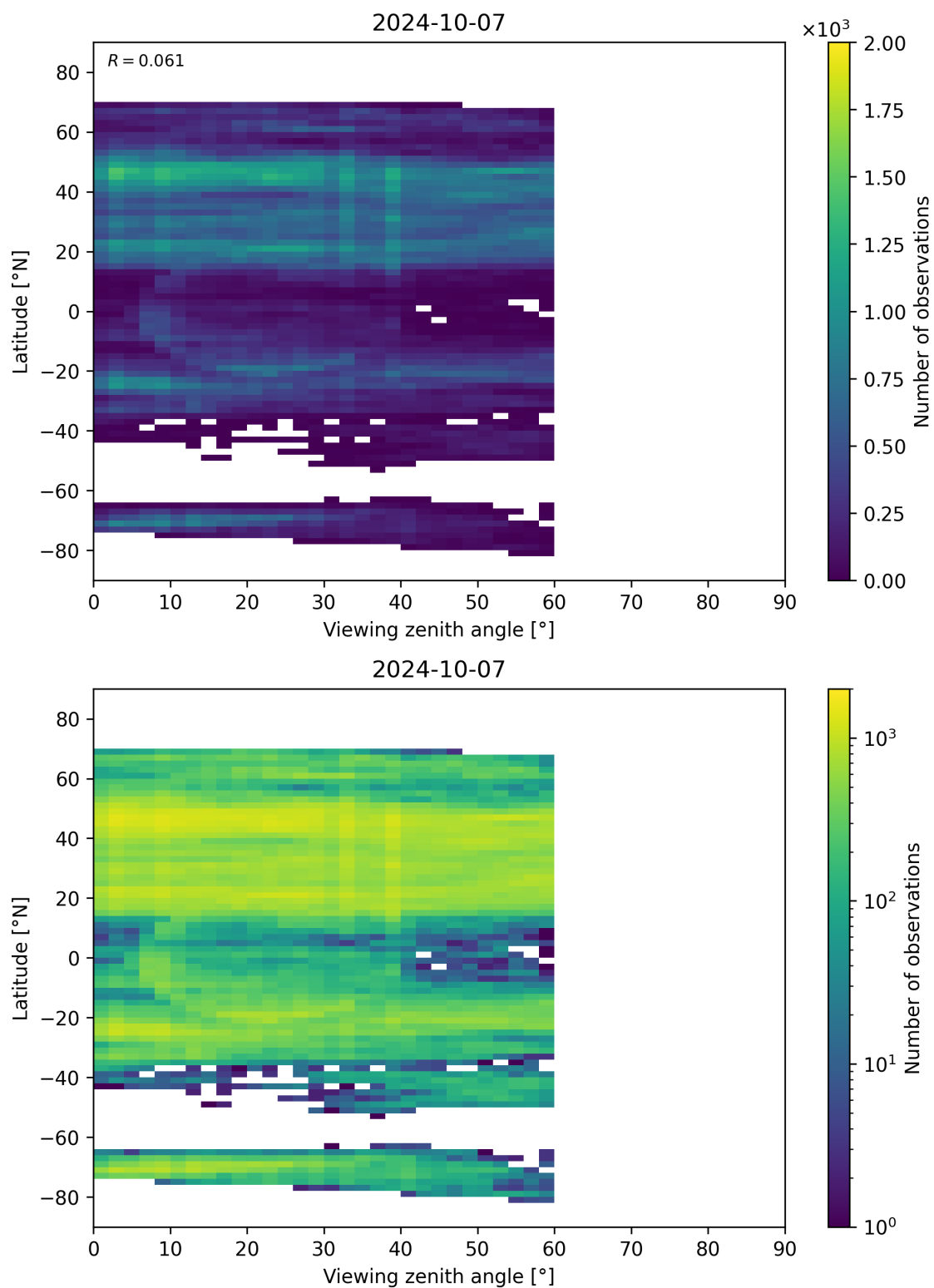
Figure 109: Scatter density plot of “Viewing zenith angle” against “Latitude” for 2024-10-06 to 2024-10-08.
