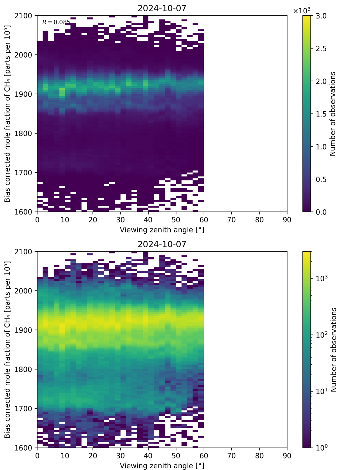
Figure 111: Scatter density plot of “Viewing zenith angle” against “Bias corrected mole fraction of CH 4 ” for 2024-10-06 to 2024-10-08.
