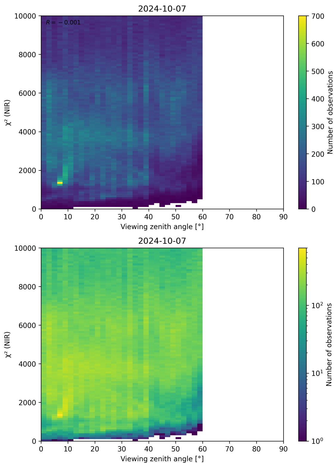
Figure 105: Scatter density plot of “Viewing zenith angle” against “ \chi^2 (NIR)” for 2024-10-06 to 2024-10-08.
