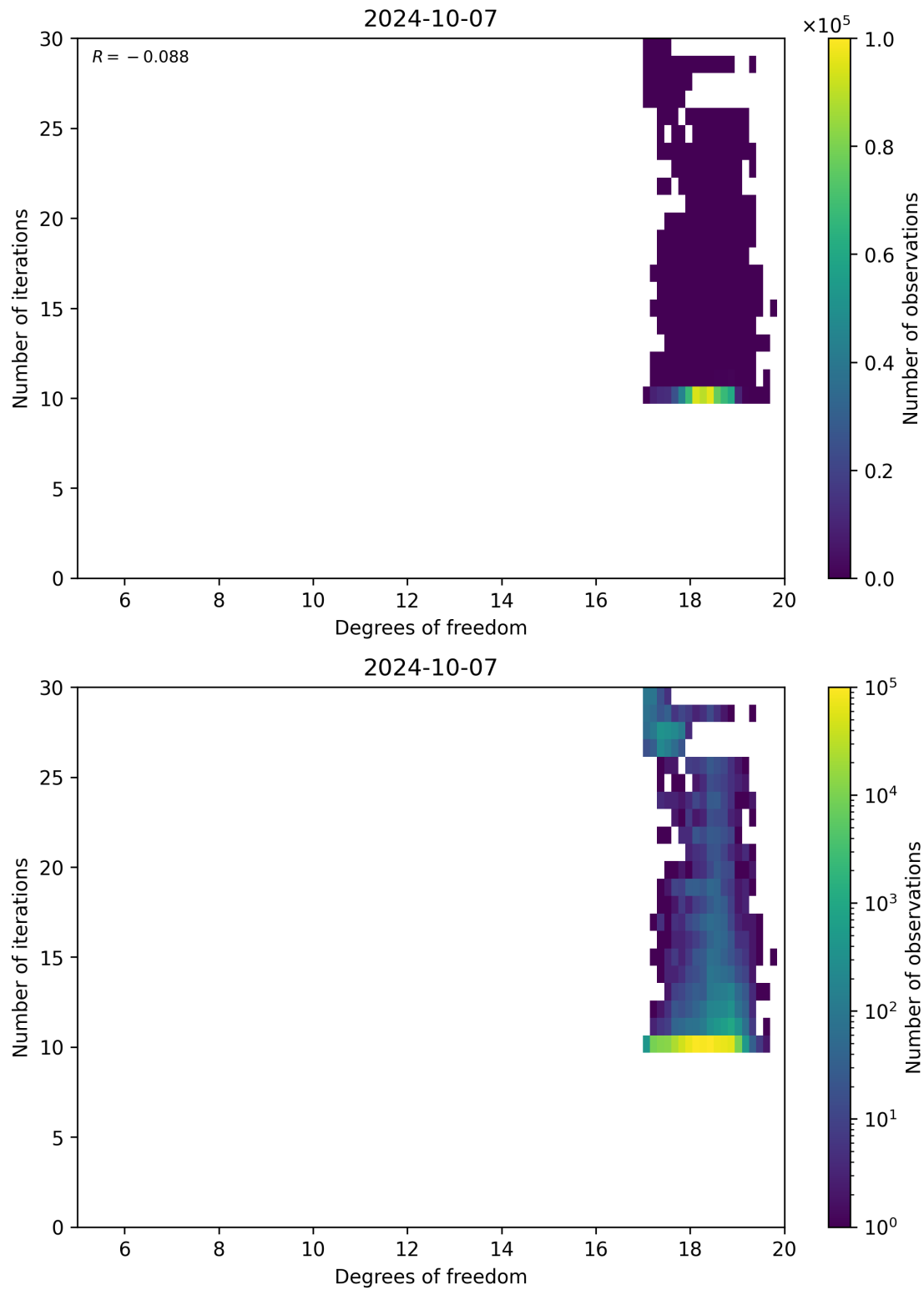
Figure 52: Scatter density plot of “Degrees of freedom” against “Number of iterations” for 2024-10-06 to 2024-10-08.
