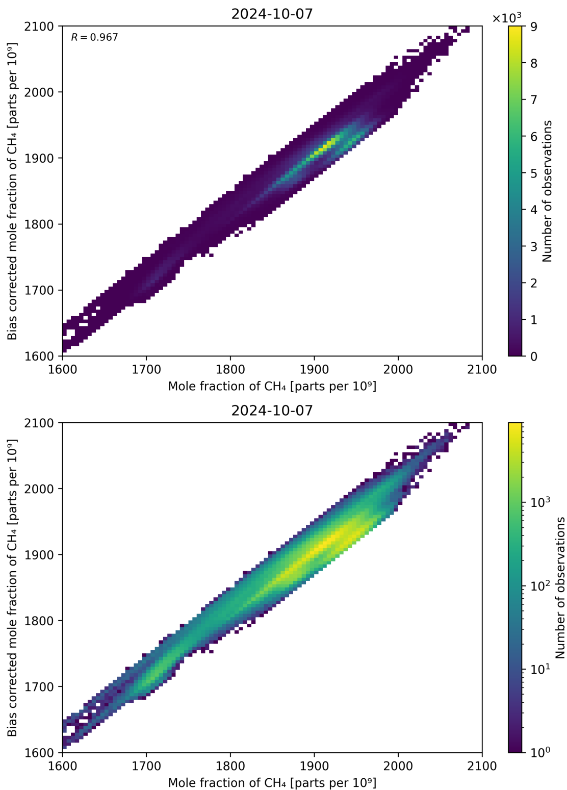
Figure 74: Scatter density plot of “Mole fraction of CH 4 ” against “Bias corrected mole fraction of CH 4 ” for 2024-10-06 to 2024-10-08.
