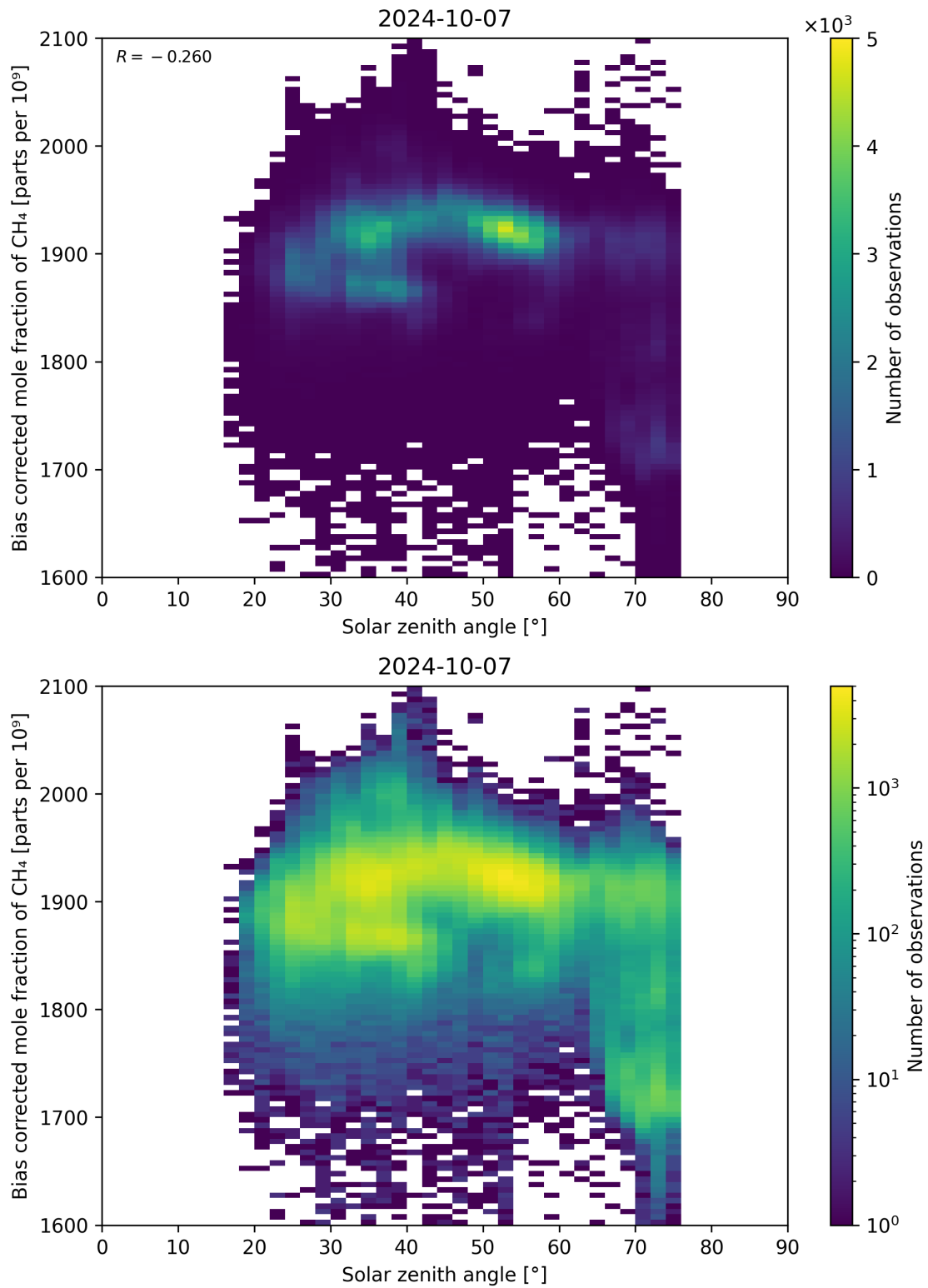
Figure 100: Scatter density plot of “Solar zenith angle” against “Bias corrected mole fraction of CH 4 ” for 2024-10-06 to 2024-10-08.
