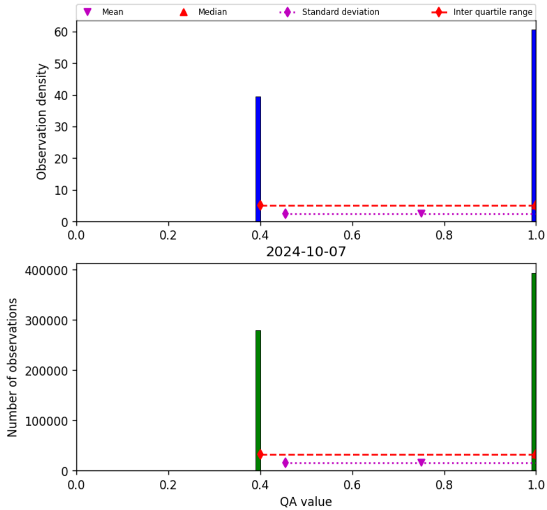
Figure 22: Histogram of “QA value” for 2024-10-06 to 2024-10-08
