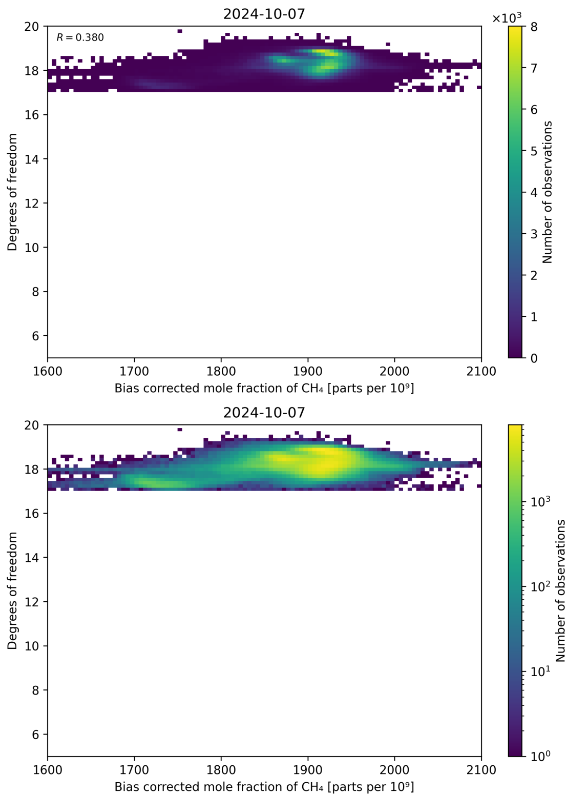
Figure 65: Scatter density plot of “Bias corrected mole fraction of CH 4 ” against “Degrees of freedom” for 2024-10-06 to 2024-10-08.
