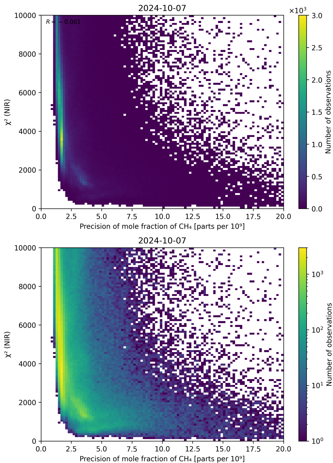
Figure 78: Scatter density plot of “Precision of mole fraction of CH 4 ” against “ \chi^2 (NIR)” for 2024-10-06 to 2024-10-08.
