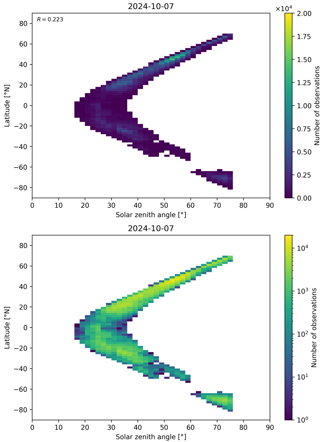
Figure 98: Scatter density plot of “Solar zenith angle” against “Latitude” for 2024-10-06 to 2024-10-08.
