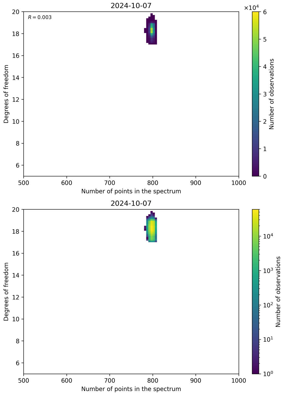
Figure 90: Scatter density plot of “Number of points in the spectrum” against “Degrees of freedom” for 2024-10-06 to 2024-10-08.
