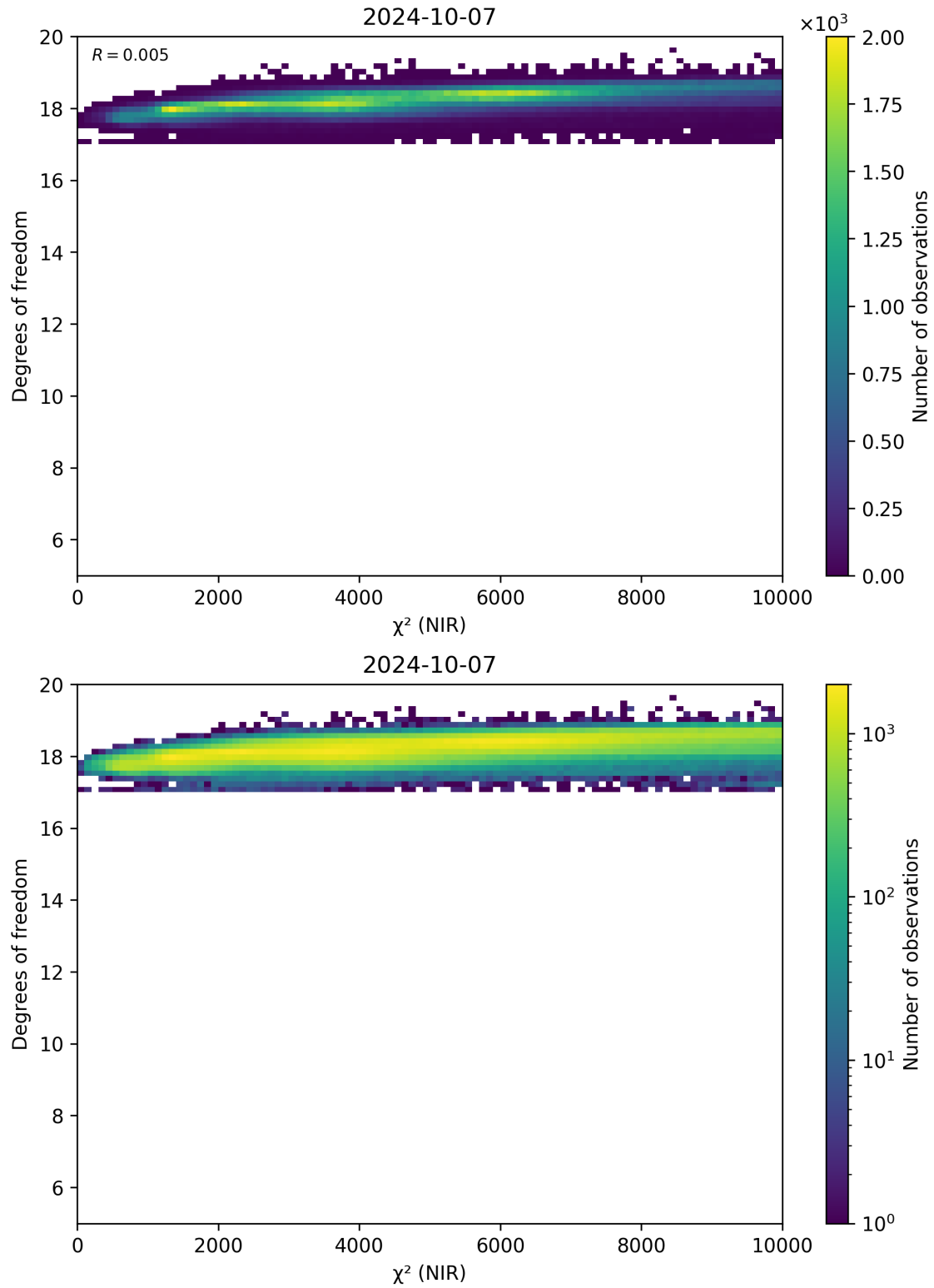
Figure 44: Scatter density plot of “ \chi^2 (NIR)” against “Degrees of freedom” for 2024-10-06 to 2024-10-08.
