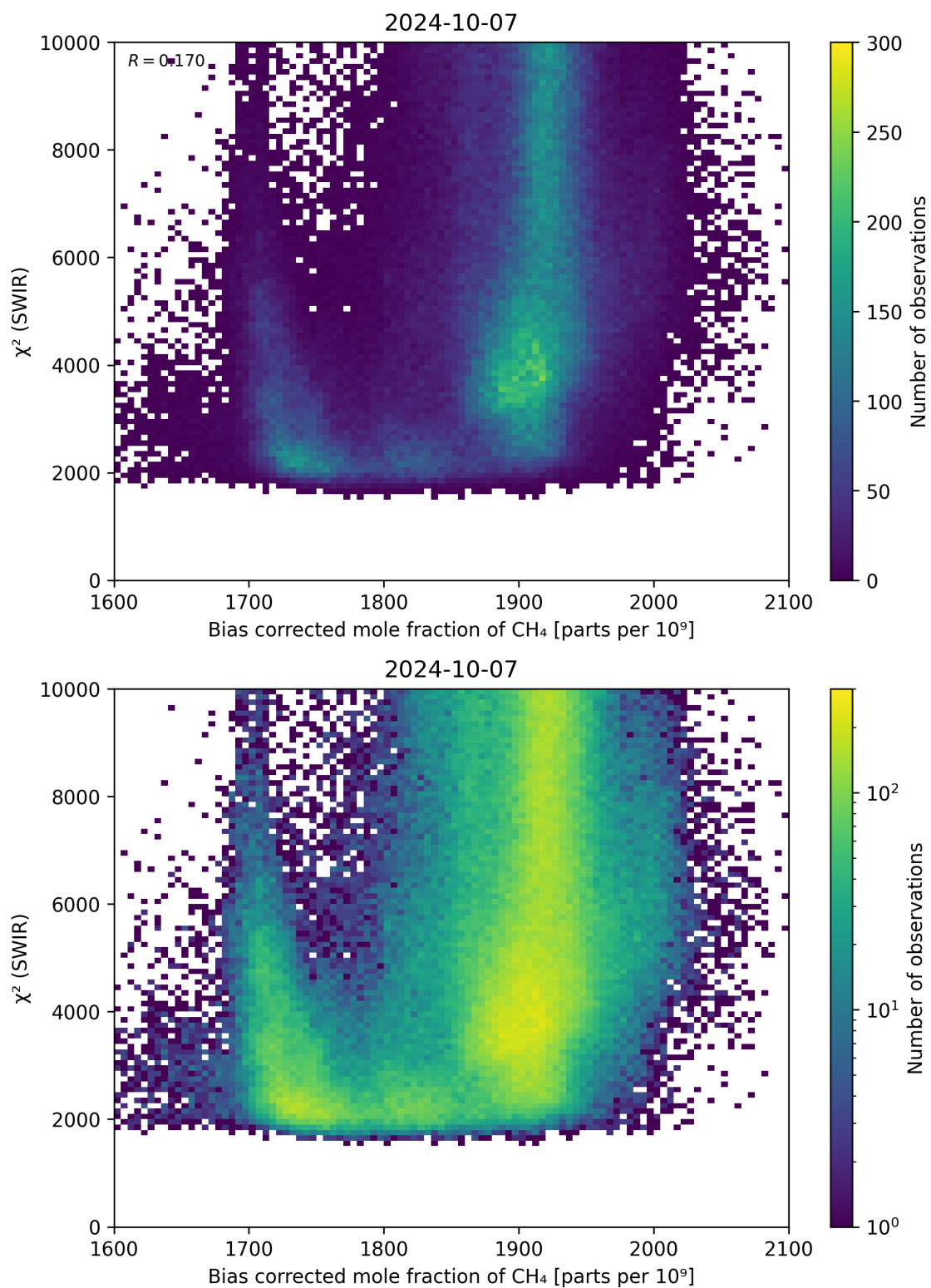
Figure 64: Scatter density plot of “Bias corrected mole fraction of \text{CH}_4 ” against “ \chi^2 (SWIR)” for 2024-10-06 to 2024-10-08.
