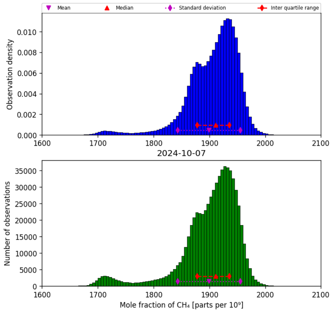
Figure 23: Histogram of “Mole fraction of CH 4 ” for 2024-10-06 to 2024-10-08
