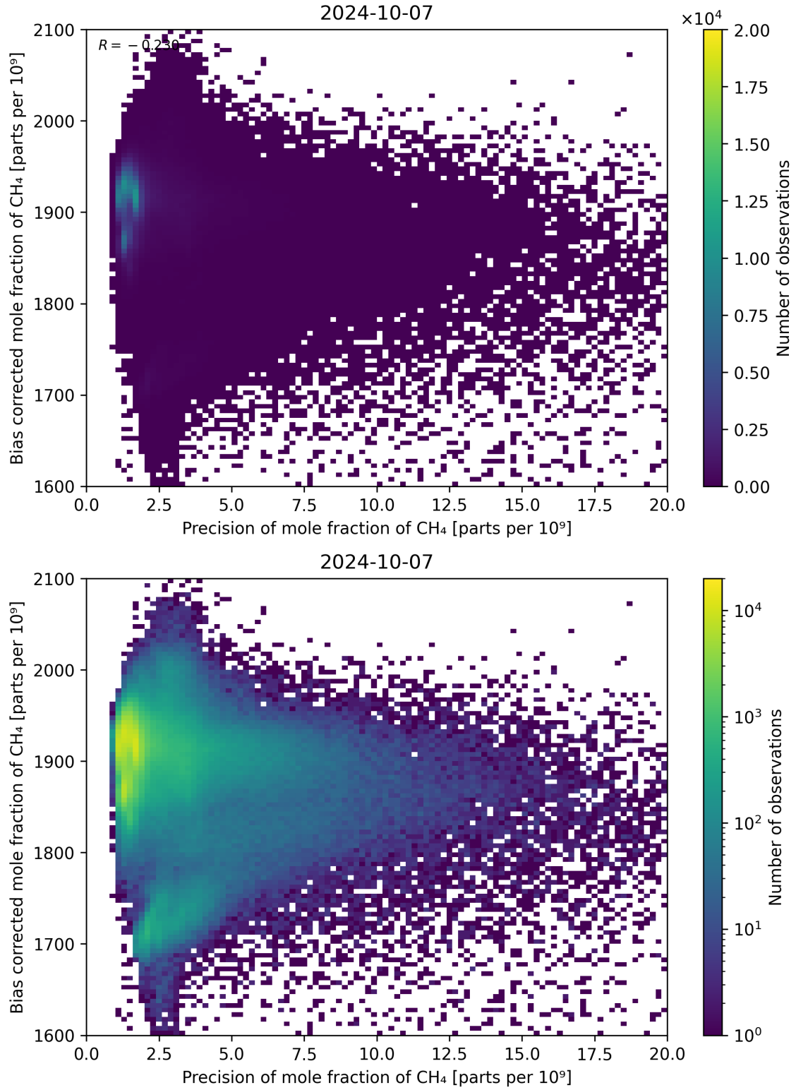
Figure 82: Scatter density plot of “Precision of mole fraction of CH 4 ” against “Bias corrected mole fraction of CH 4 ” for 2024-10-06 to 2024-10-08.
