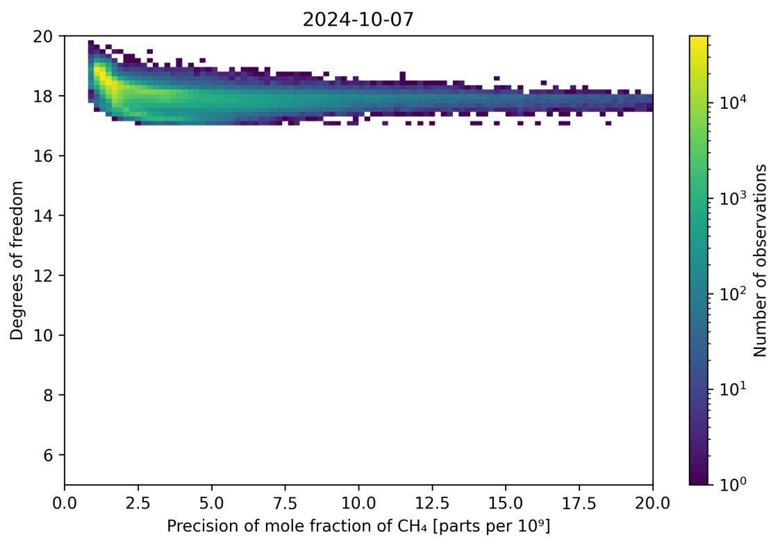
Figure 80: Scatter density plot of “Precision of mole fraction of CH 4 ” against “Degrees of freedom” for 2024-10-06 to 2024-10-08.
