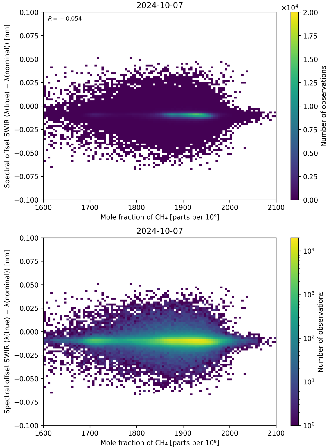
Figure 86: Scatter density plot of “Mole fraction of CH 4 ” against “Spectral offset SWIR ( \lambda_{\text{true}} - \lambda_{\text{nominal}} )” for 2024-10-06 to 2024-10-08.
