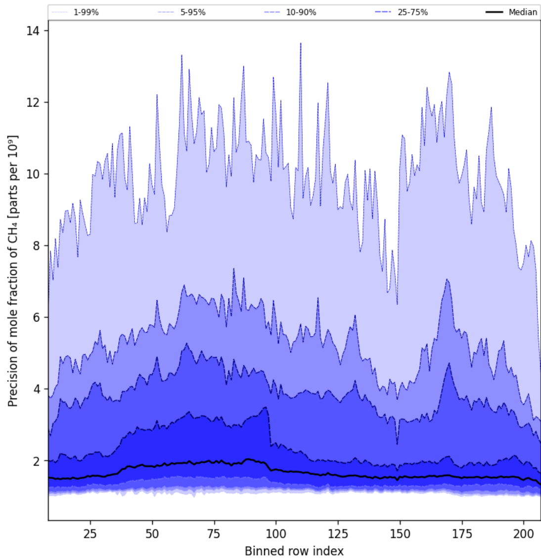
Figure 35: Along track statistics of “Precision of mole fraction of CH 4 ” for 2024-10-06 to 2024-10-08
