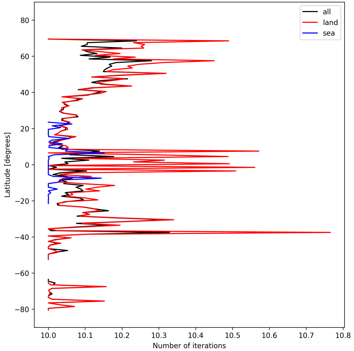
Figure 20: Zonal average of “Number of iterations” for 2024-10-06 to 2024-10-08.
