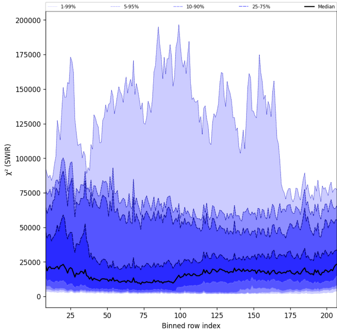
Figure 39: Along track statistics of " \chi^2 (SWIR)" for 2024-10-06 to 2024-10-08
