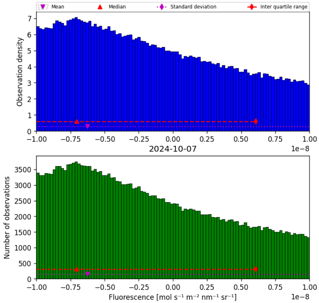
Figure 32: Histogram of “Fluorescence” for 2024-10-06 to 2024-10-08
