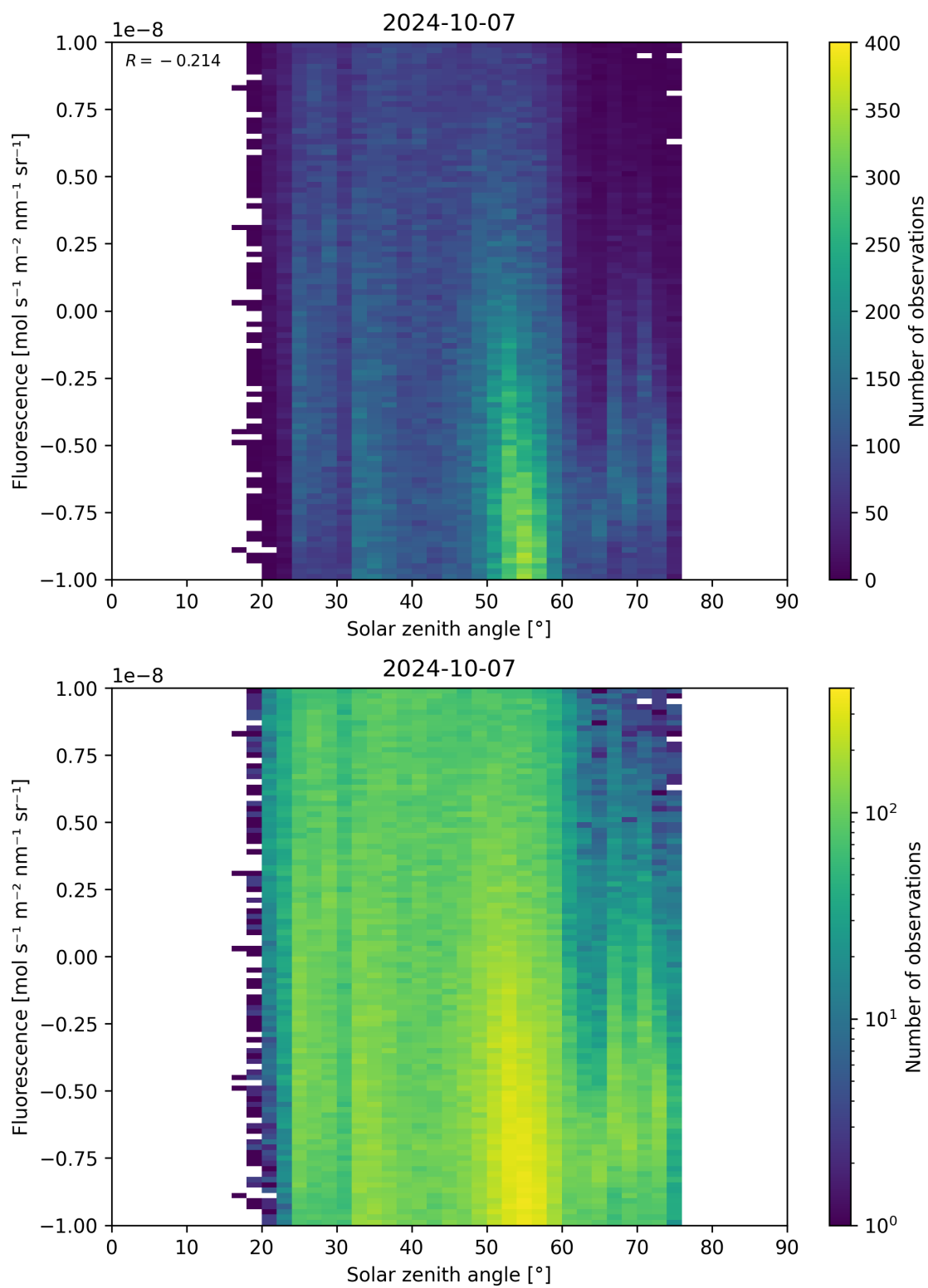
Figure 97: Scatter density plot of “Solar zenith angle” against “Fluorescence” for 2024-10-06 to 2024-10-08.
