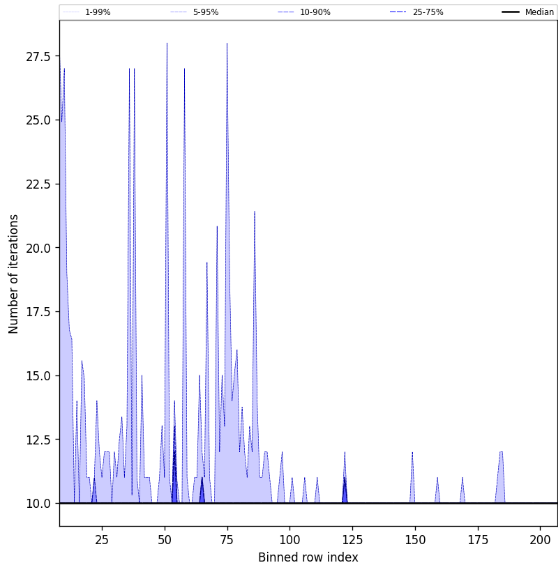
Figure 42: Along track statistics of “Number of iterations” for 2024-10-06 to 2024-10-08
