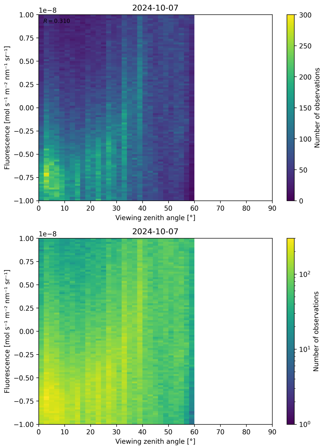
Figure 108: Scatter density plot of “Viewing zenith angle” against “Fluorescence” for 2024-10-06 to 2024-10-08.
