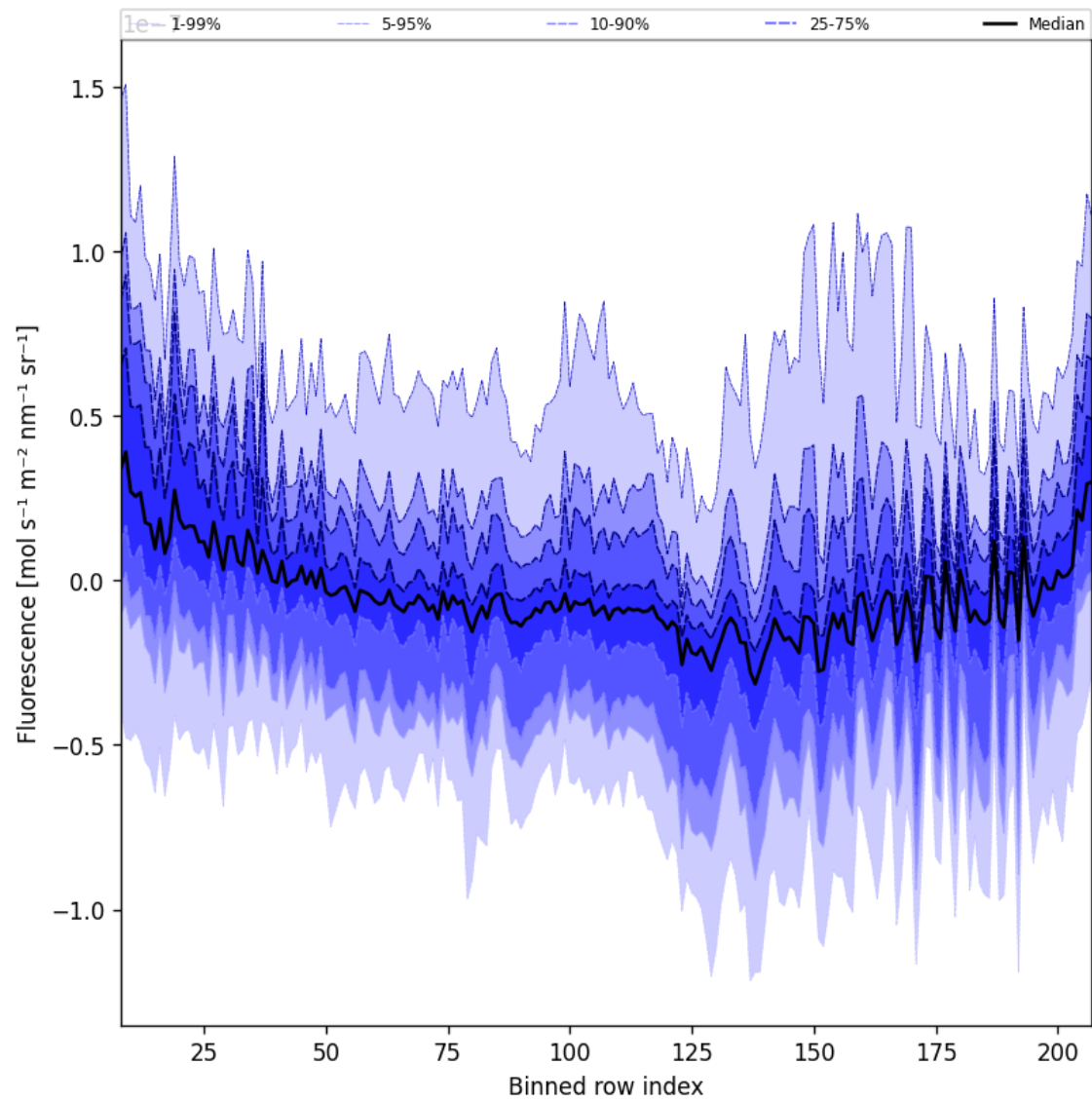
Figure 43: Along track statistics of “Fluorescence” for 2024-10-06 to 2024-10-08
