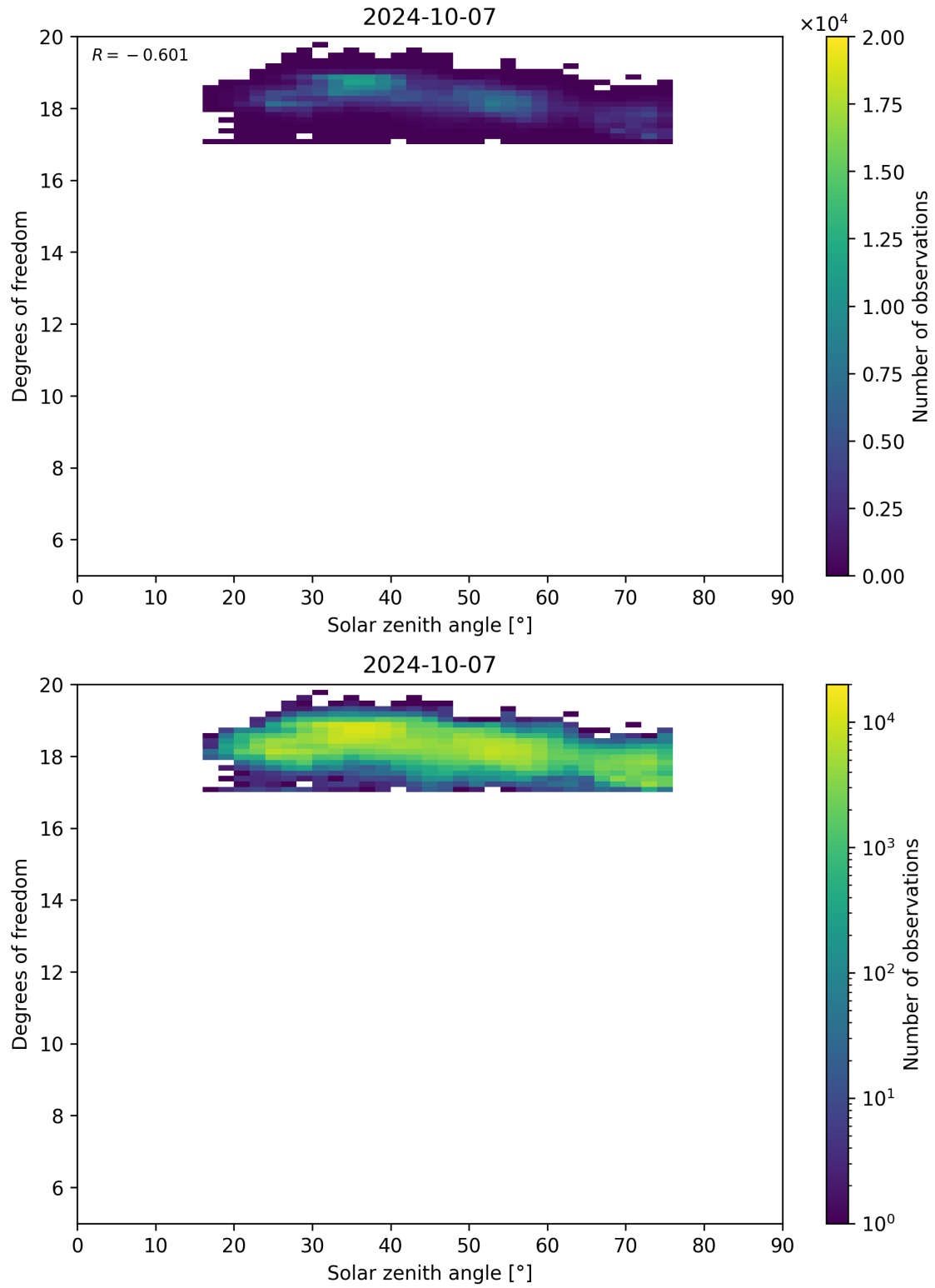
Figure 96: Scatter density plot of “Solar zenith angle” against “Degrees of freedom” for 2024-10-06 to 2024-10-08.
