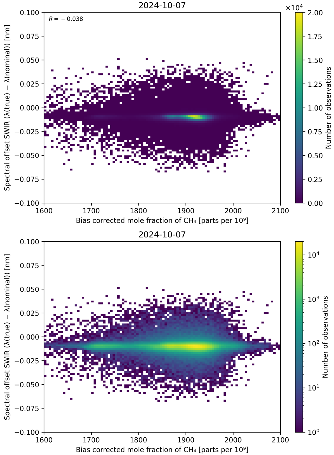
Figure 69: Scatter density plot of “Bias corrected mole fraction of \text{CH}_4 ” against “Spectral offset SWIR ( \lambda_{\text{true}} - \lambda_{\text{nominal}} )” for 2024-10-06 to 2024-10-08.
