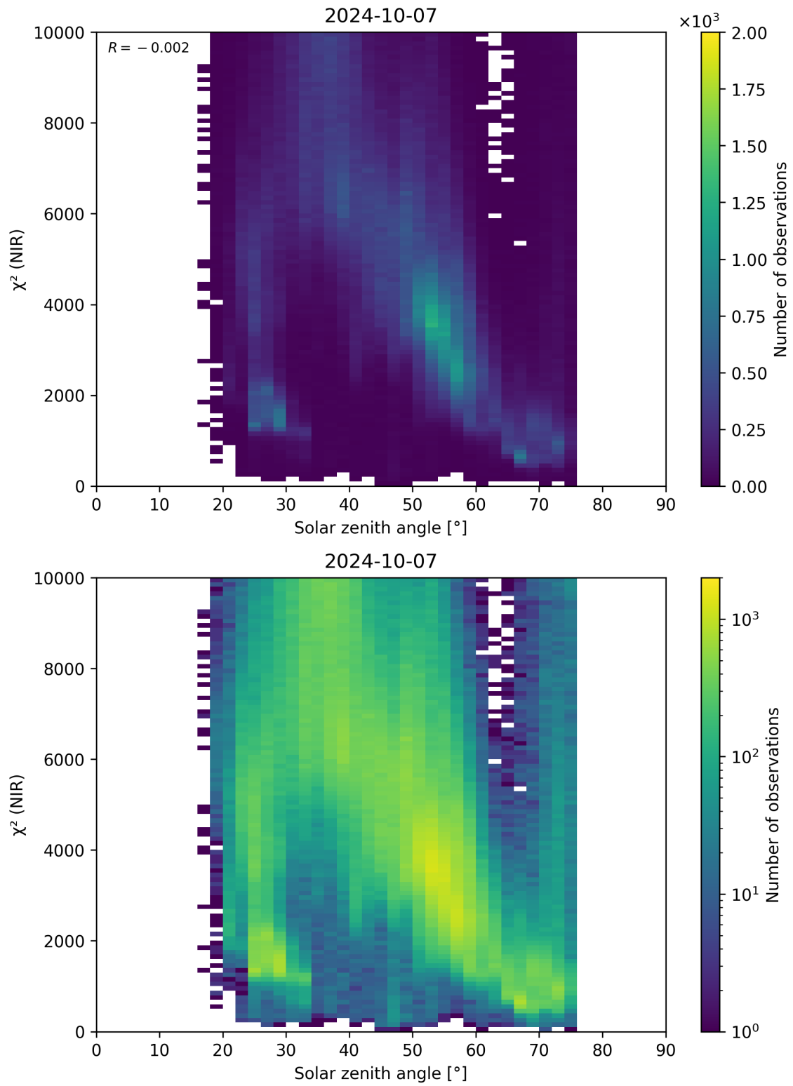
Figure 94: Scatter density plot of “Solar zenith angle” against “ \chi^2 (NIR)” for 2024-10-06 to 2024-10-08.
