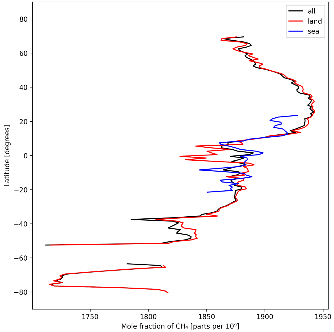
Figure 12: Zonal average of “Mole fraction of \text{CH}_4 ” for 2024-10-06 to 2024-10-08.
