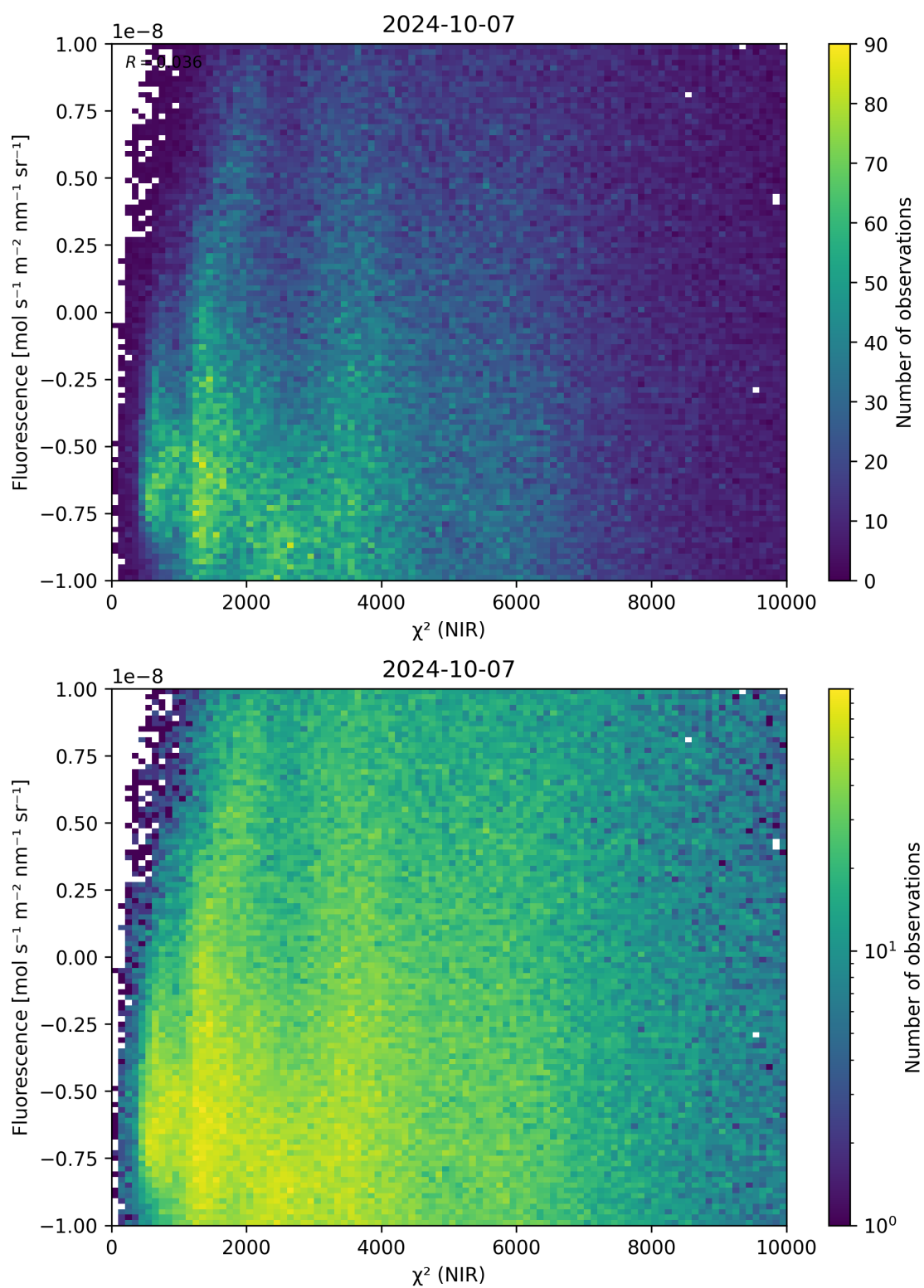
Figure 45: Scatter density plot of “ \chi^2 (NIR)” against “Fluorescence” for 2024-10-06 to 2024-10-08.
