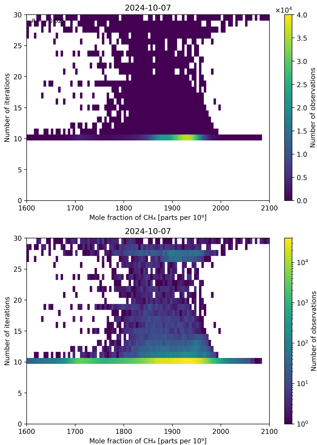
Figure 76: Scatter density plot of “Mole fraction of CH 4 ” against “Number of iterations” for 2024-10-06 to 2024-10-08.
