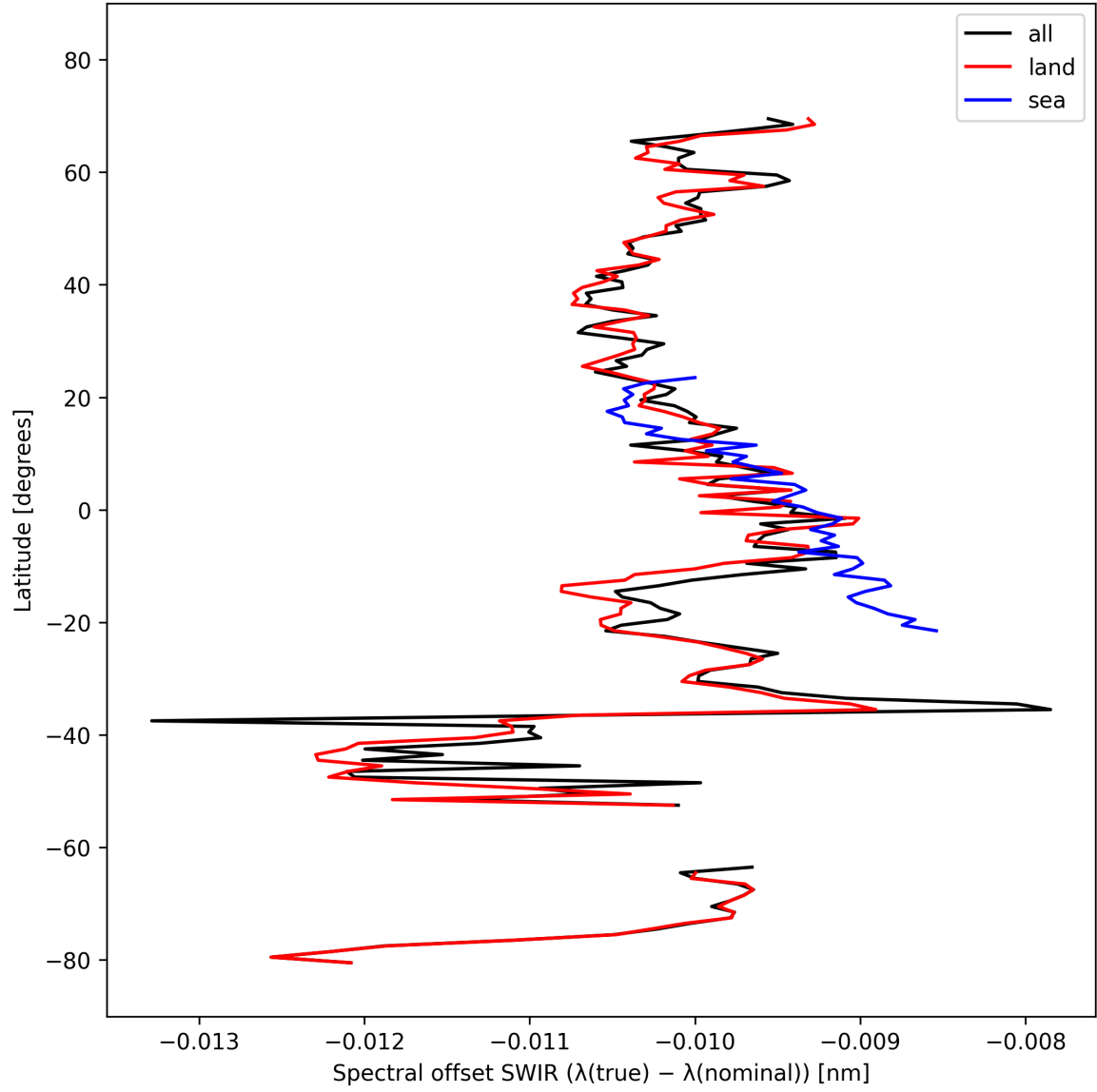
Figure 16: Zonal average of “Spectral offset SWIR ( \lambda_{\text{true}} - \lambda_{\text{nominal}} )” for 2024-10-06 to 2024-10-08.
