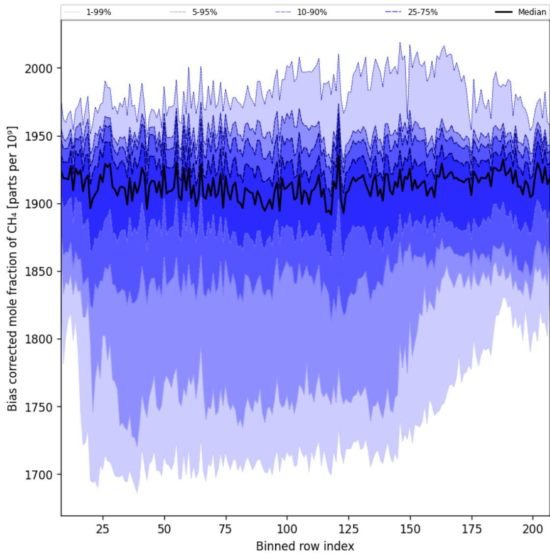
Figure 36: Along track statistics of “Bias corrected mole fraction of CH 4 ” for 2024-10-06 to 2024-10-08
