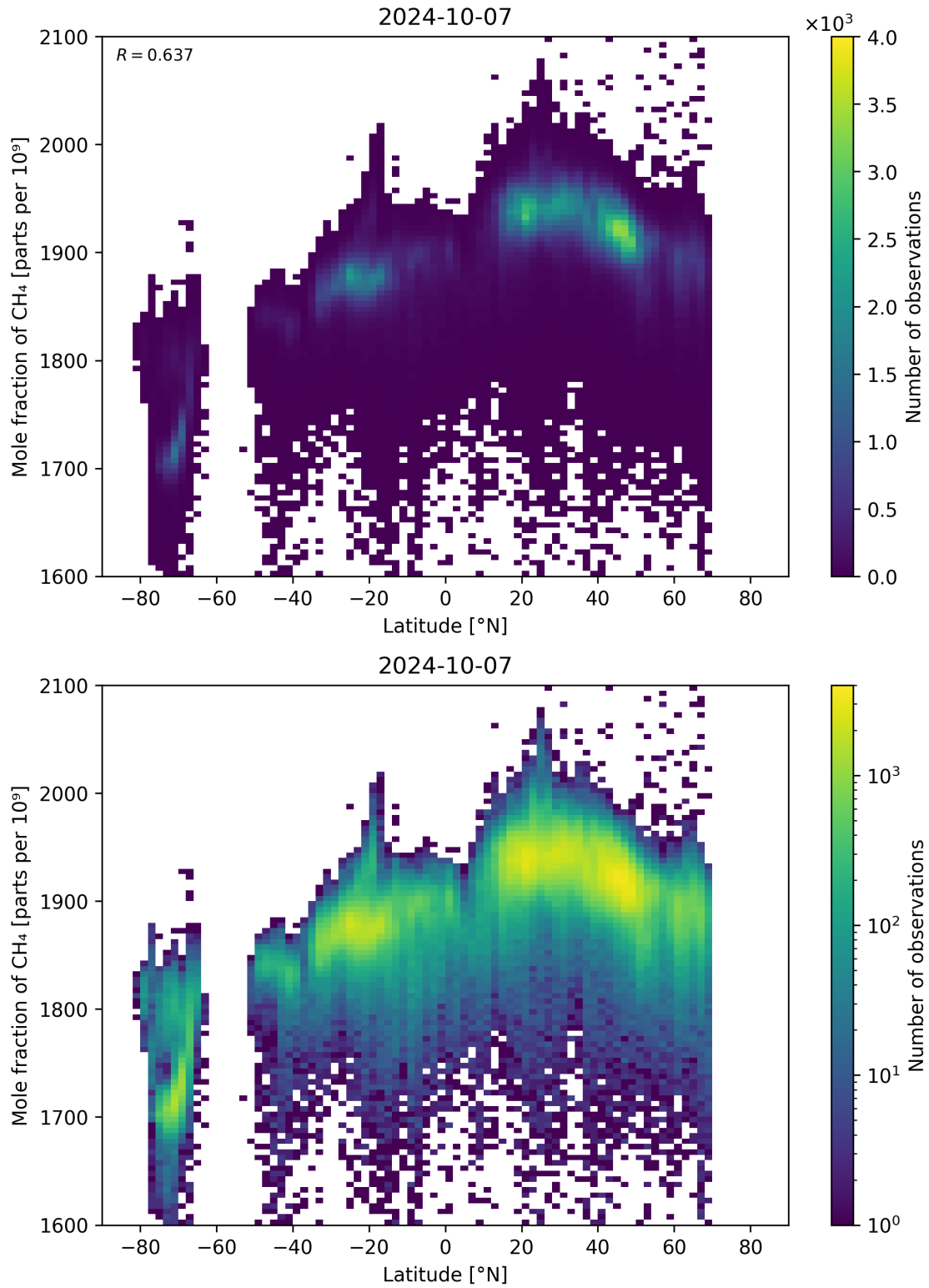
Figure 57: Scatter density plot of “Latitude” against “Mole fraction of CH 4 ” for 2024-10-06 to 2024-10-08.
