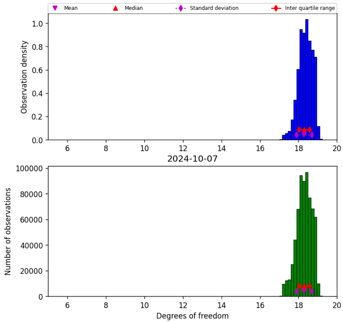
Figure 30: Histogram of “Degrees of freedom” for 2024-10-06 to 2024-10-08
