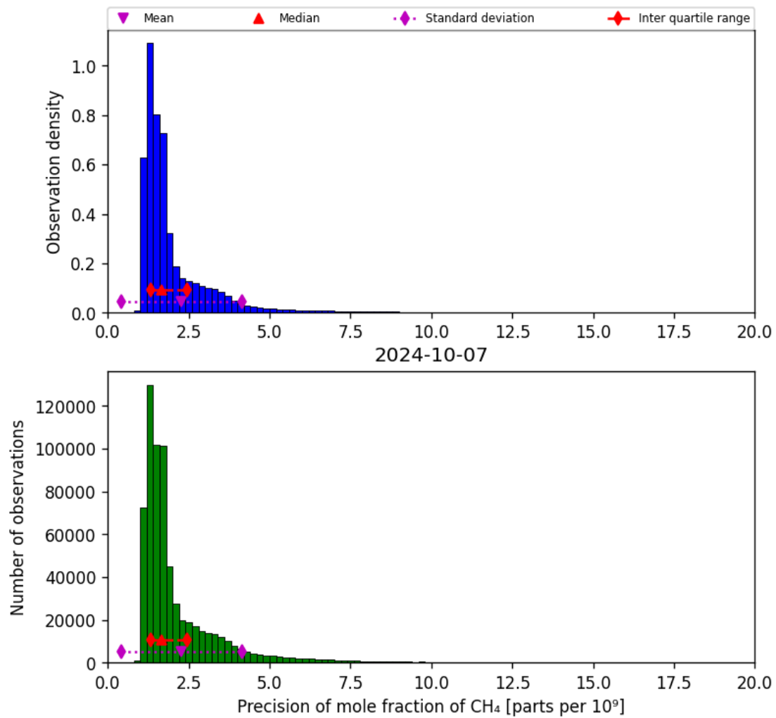
Figure 24: Histogram of “Precision of mole fraction of CH 4 ” for 2024-10-06 to 2024-10-08
