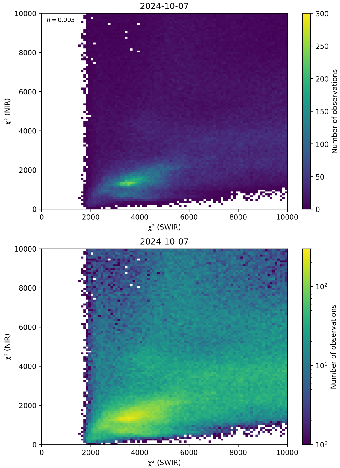
Figure 47: Scatter density plot of “ \chi^2 (SWIR)” against “ \chi^2 (NIR)” for 2024-10-06 to 2024-10-08.
