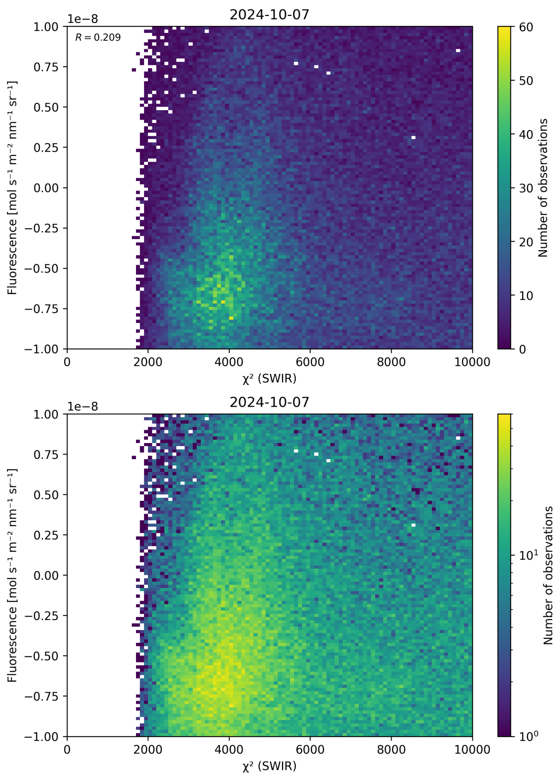
Figure 49: Scatter density plot of “ \chi^2 (SWIR)” against “Fluorescence” for 2024-10-06 to 2024-10-08.
