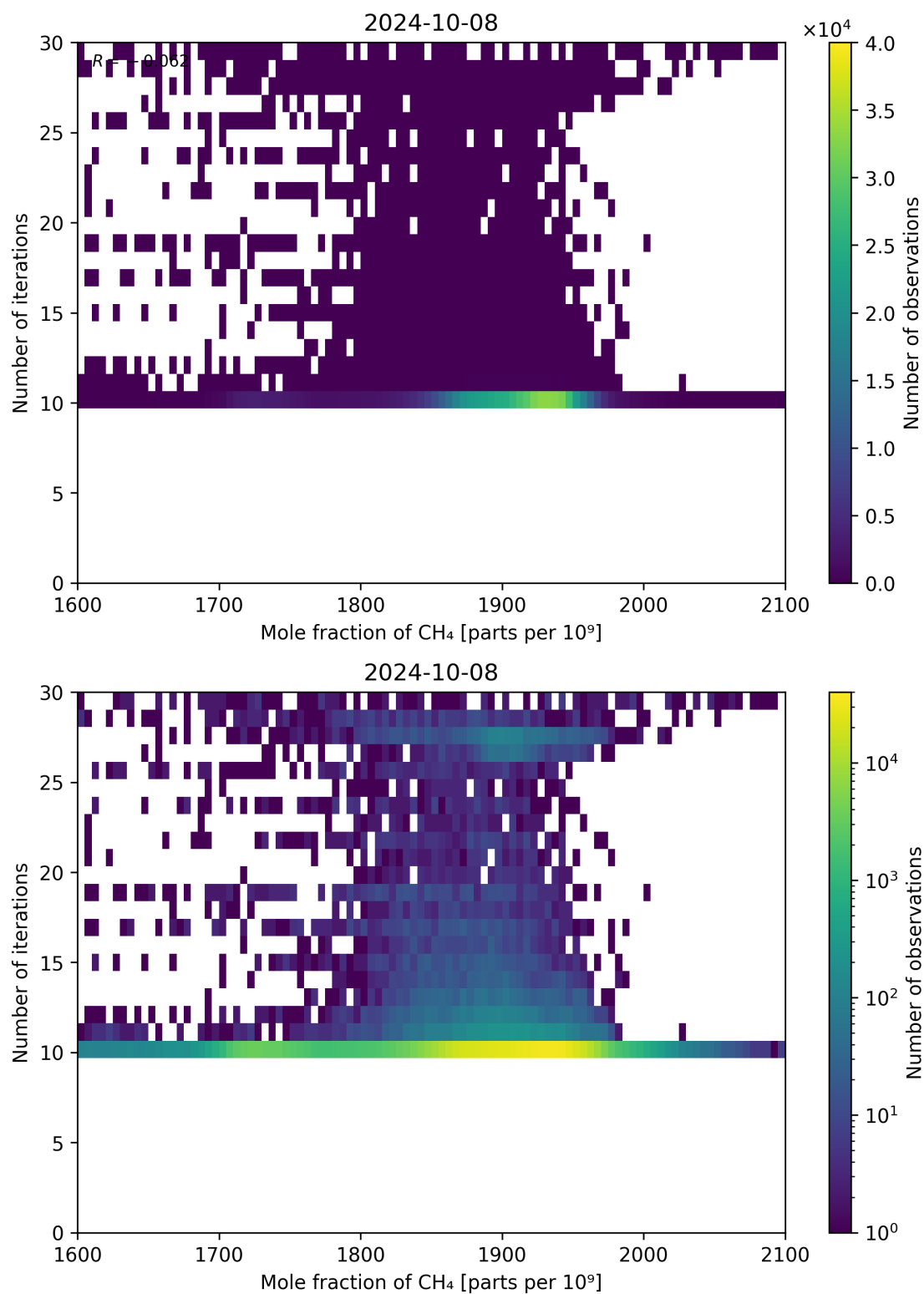
Figure 76: Scatter density plot of “Mole fraction of CH 4 ” against “Number of iterations” for 2024-10-08 to 2024-10-09.
