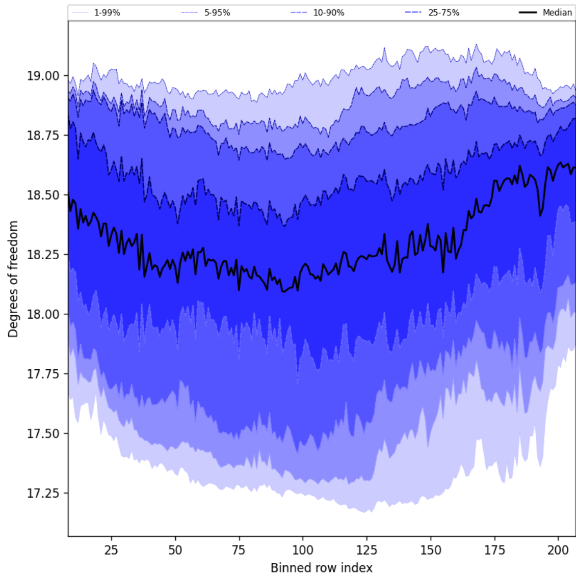
Figure 41: Along track statistics of “Degrees of freedom” for 2024-10-08 to 2024-10-09
