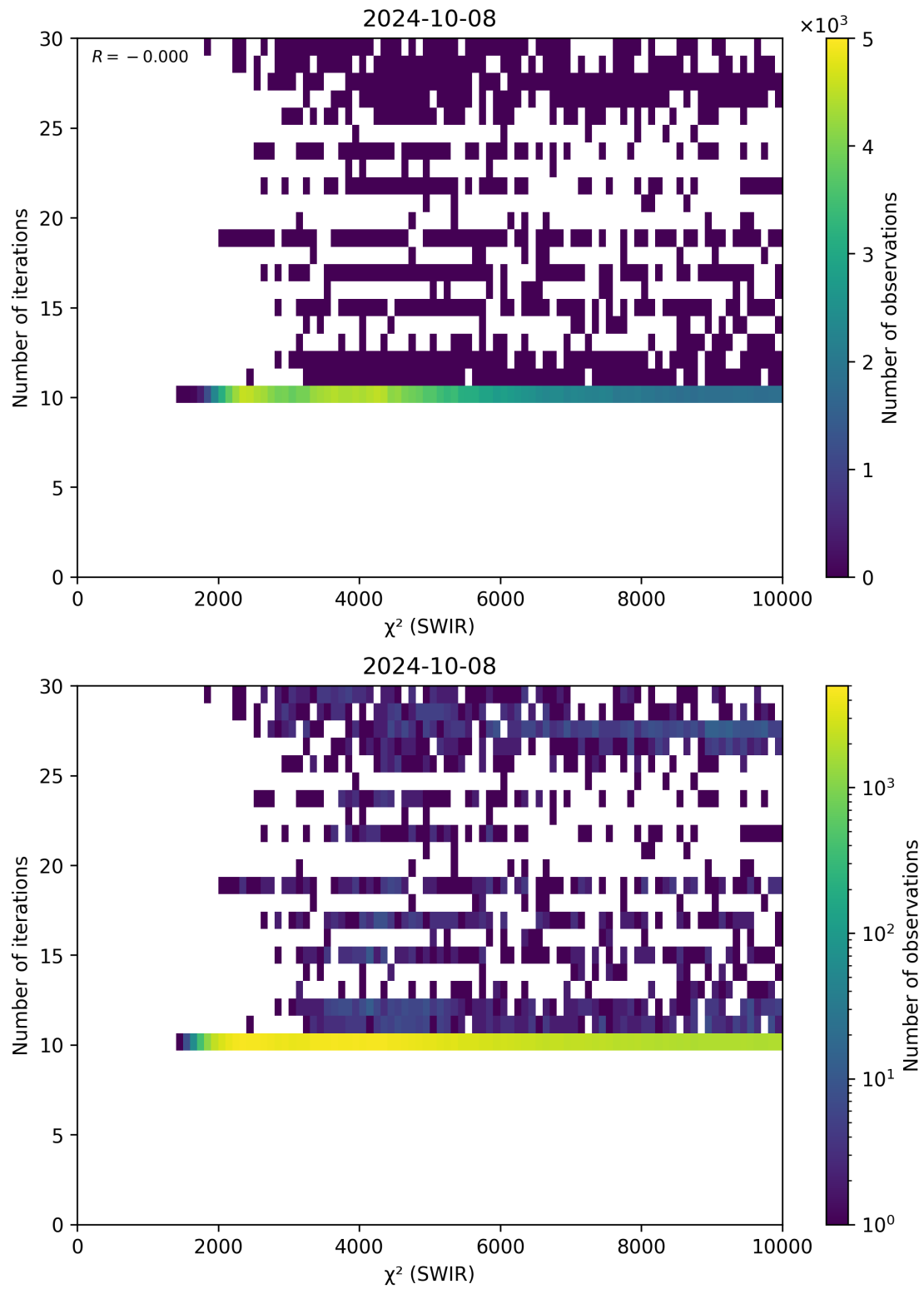
Figure 50: Scatter density plot of “ \chi^2 (SWIR)” against “Number of iterations” for 2024-10-08 to 2024-10-09.
