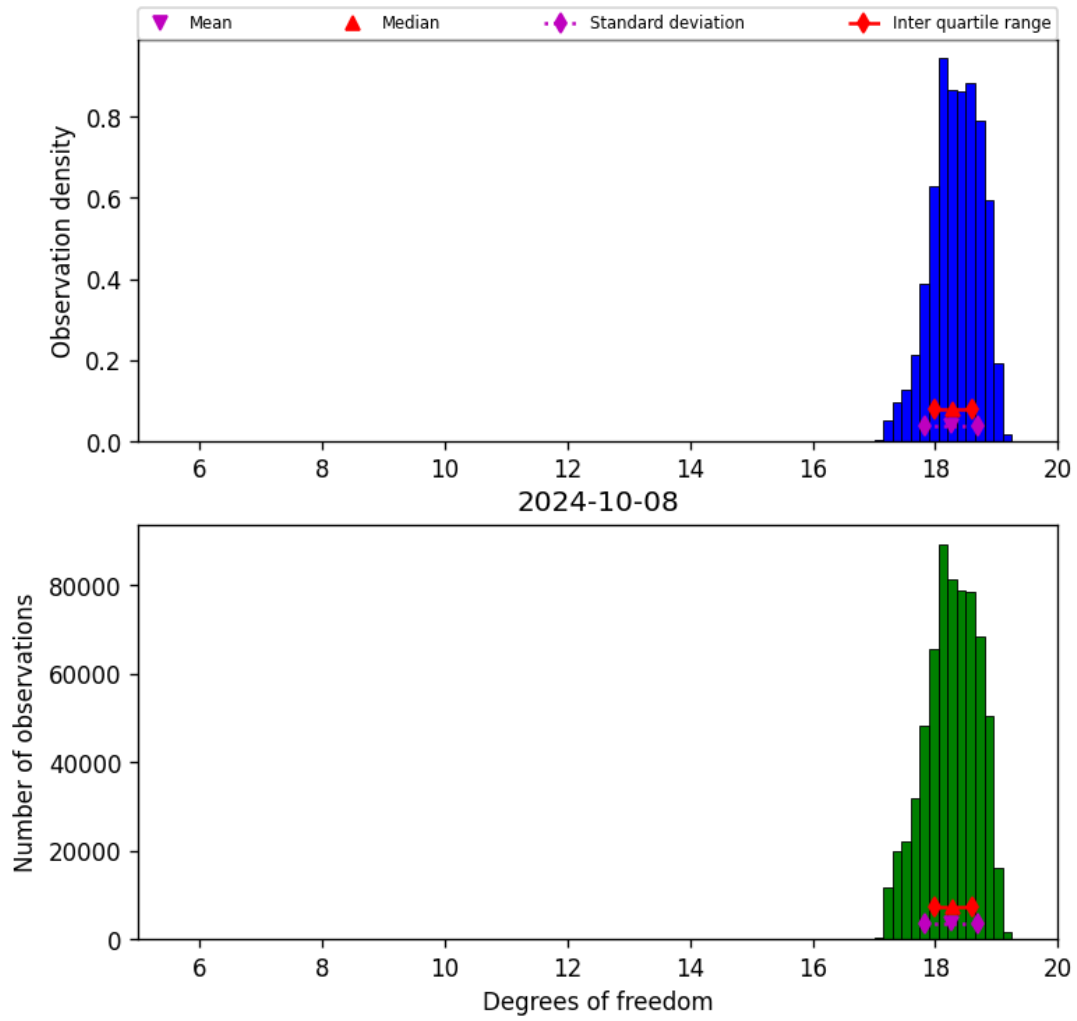
Figure 30: Histogram of “Degrees of freedom” for 2024-10-08 to 2024-10-09
