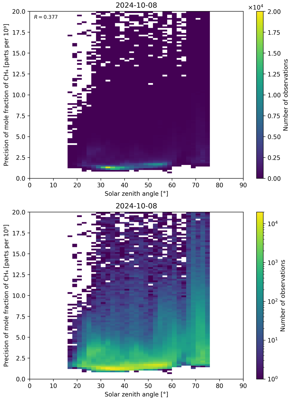
Figure 101: Scatter density plot of “Solar zenith angle” against “Precision of mole fraction of CH 4 ” for 2024-10-08 to 2024-10-09.
