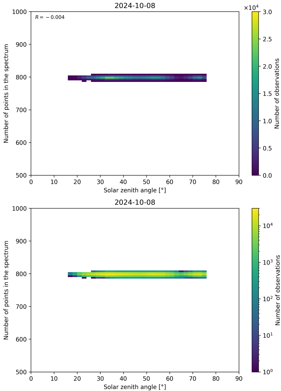
Figure 103: Scatter density plot of “Solar zenith angle” against “Number of points in the spectrum” for 2024-10-08 to 2024-10-09.
