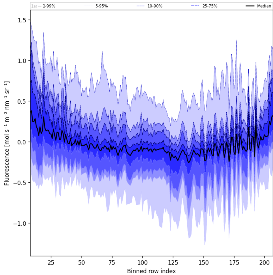
Figure 43: Along track statistics of “Fluorescence” for 2024-10-08 to 2024-10-09
