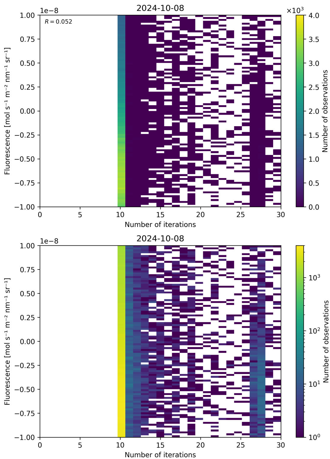
Figure 87: Scatter density plot of “Number of iterations” against “Fluorescence” for 2024-10-08 to 2024-10-09.
