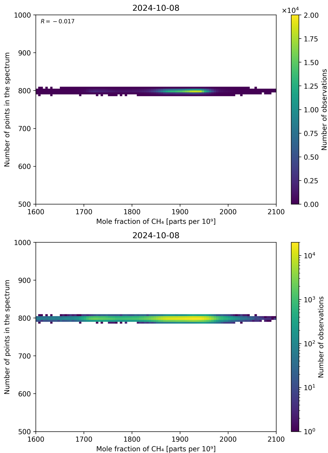
Figure 77: Scatter density plot of “Mole fraction of CH 4 ” against “Number of points in the spectrum” for 2024-10-08 to 2024-10-09.
