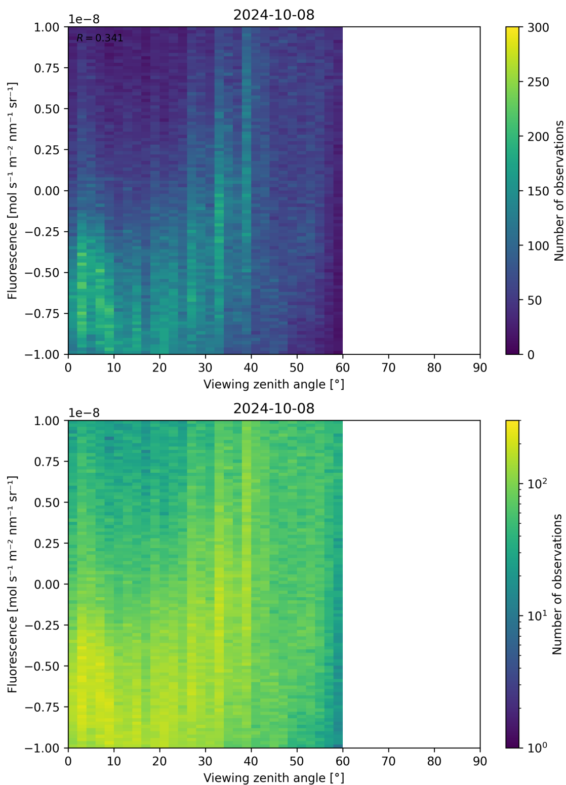
Figure 108: Scatter density plot of “Viewing zenith angle” against “Fluorescence” for 2024-10-08 to 2024-10-09.
