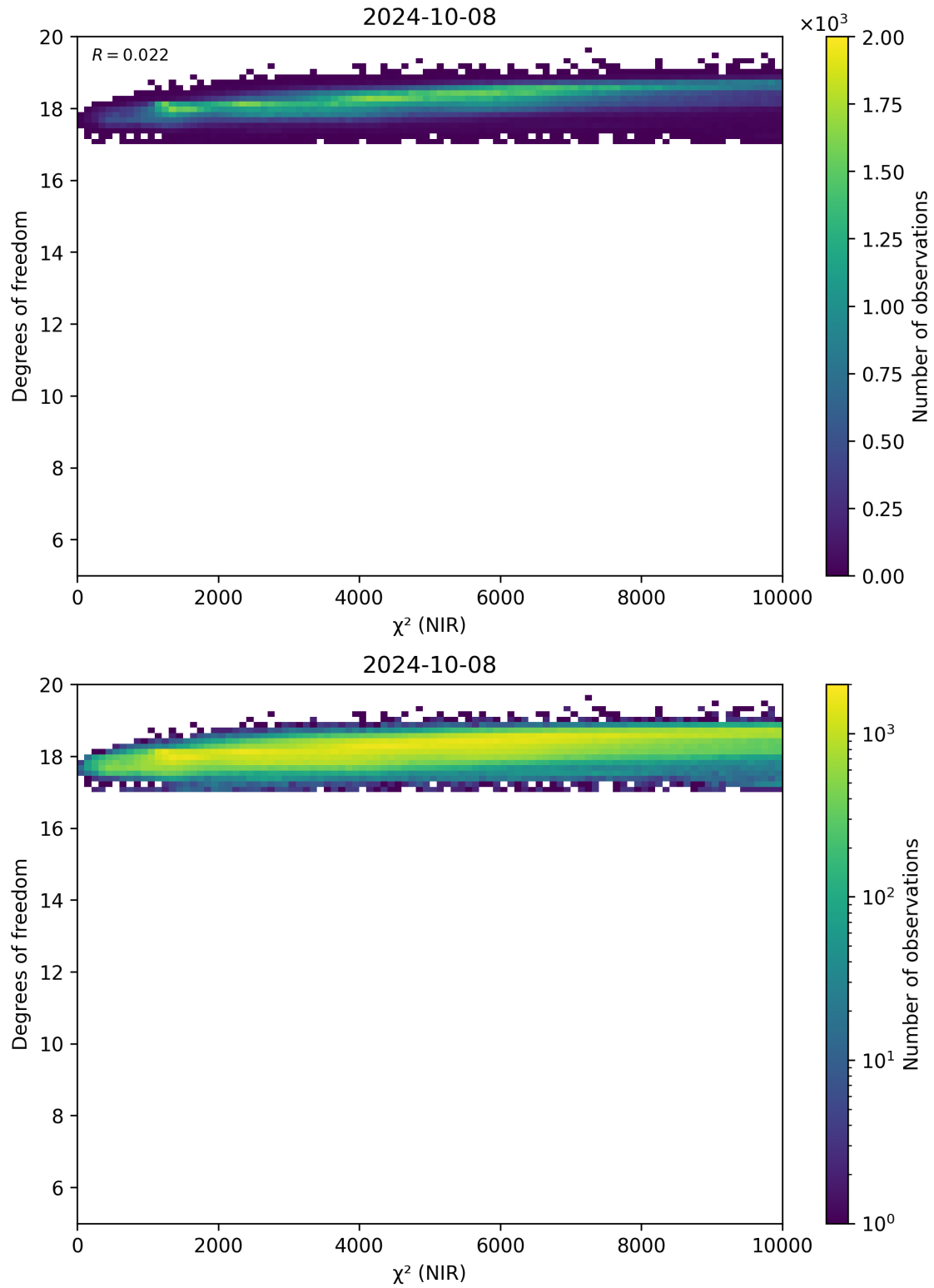
Figure 44: Scatter density plot of “ \chi^2 (NIR)” against “Degrees of freedom” for 2024-10-08 to 2024-10-09.
