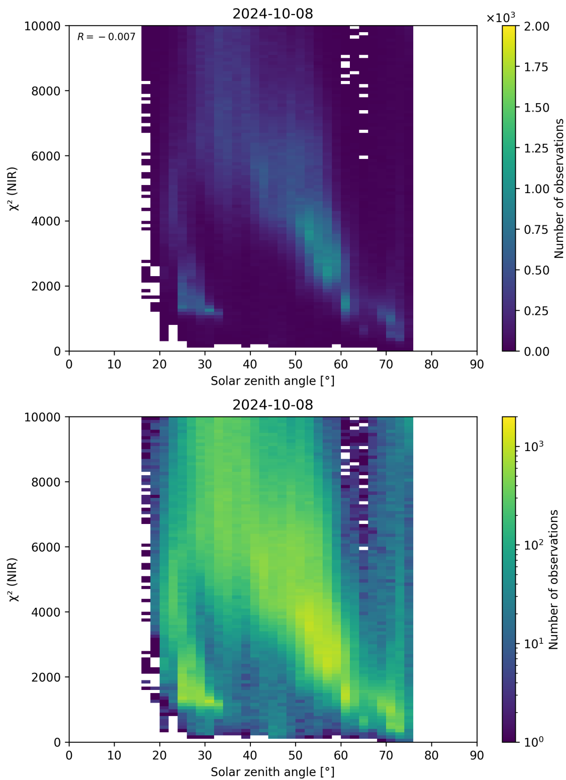
Figure 94: Scatter density plot of “Solar zenith angle” against “ \chi^2 (NIR)” for 2024-10-08 to 2024-10-09.
