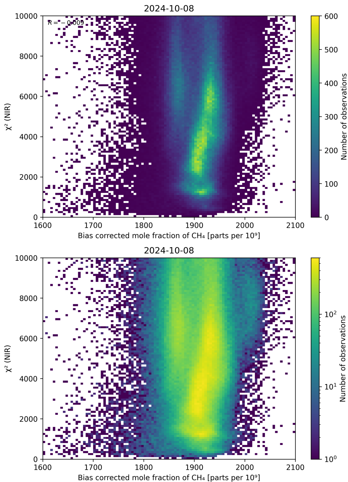
Figure 63: Scatter density plot of “Bias corrected mole fraction of CH 4 ” against “ \chi^2 (NIR)” for 2024-10-08 to 2024-10-09.
