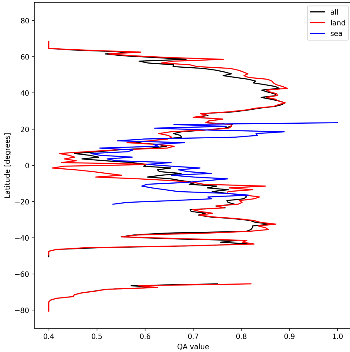
Figure 11: Zonal average of “QA value” for 2024-10-08 to 2024-10-09.
