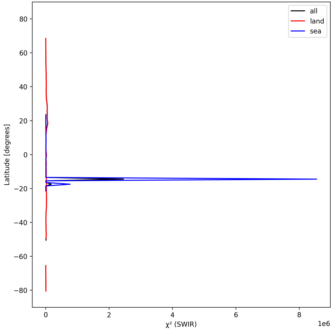
Figure 17: Zonal average of “ \chi^2 (SWIR)” for 2024-10-08 to 2024-10-09.
