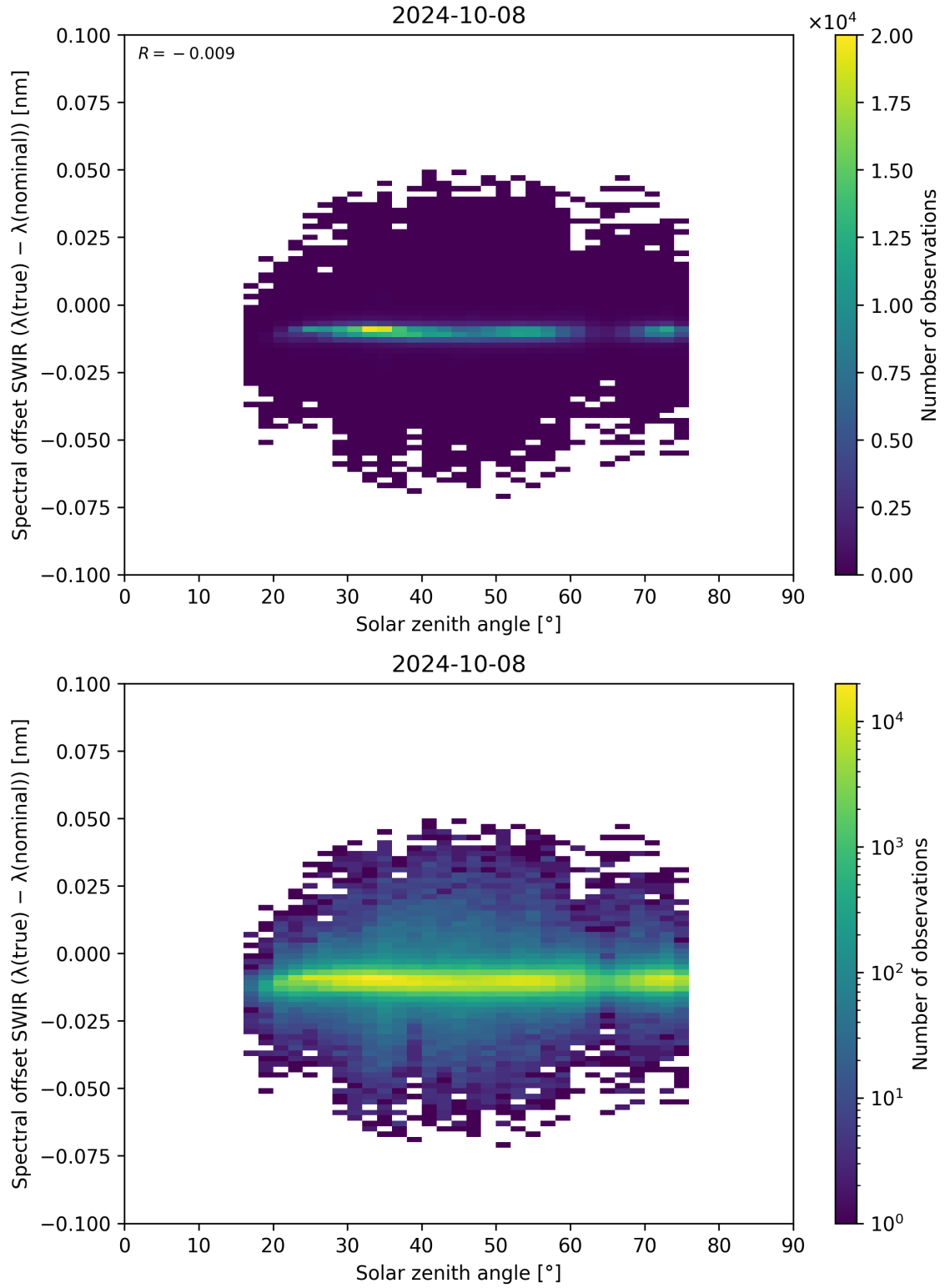
Figure 104: Scatter density plot of “Solar zenith angle” against “Spectral offset SWIR ( \lambda_{\text{true}} - \lambda_{\text{nominal}} )” for 2024-10-08 to 2024-10-09.
