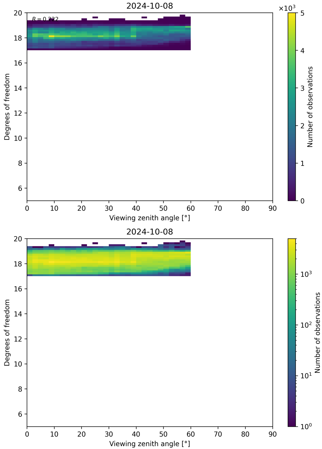
Figure 107: Scatter density plot of “Viewing zenith angle” against “Degrees of freedom” for 2024-10-08 to 2024-10-09.
