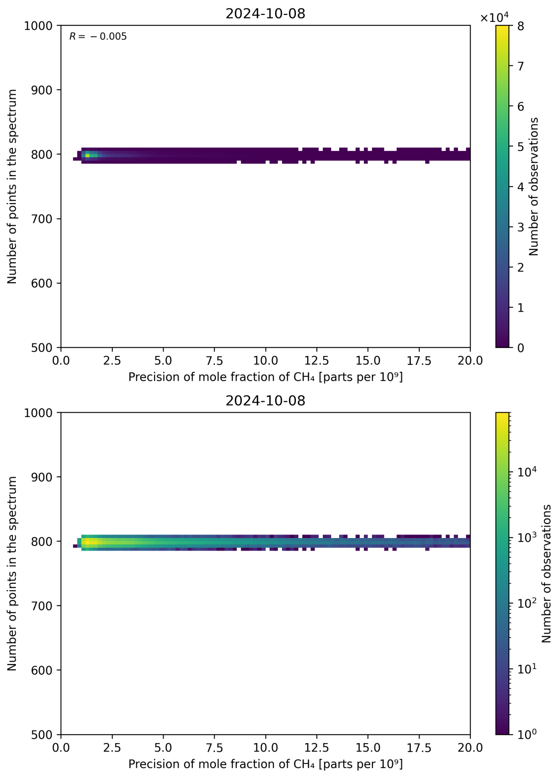
Figure 84: Scatter density plot of “Precision of mole fraction of CH 4 ” against “Number of points in the spectrum” for 2024-10-08 to 2024-10-09.
