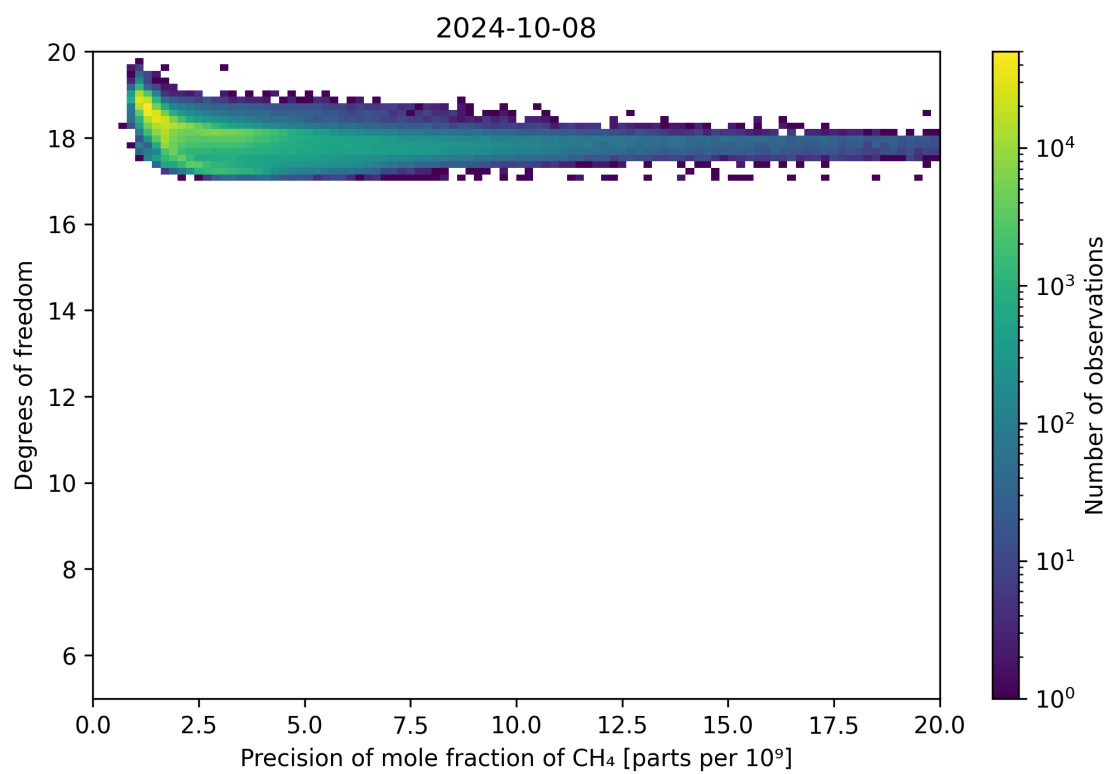
Figure 80: Scatter density plot of “Precision of mole fraction of CH 4 ” against “Degrees of freedom” for 2024-10-08 to 2024-10-09.
