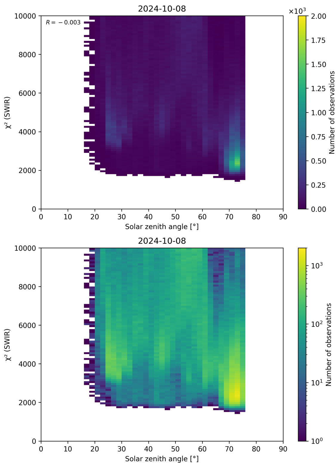
Figure 95: Scatter density plot of “Solar zenith angle” against “ \chi^2 (SWIR)” for 2024-10-08 to 2024-10-09.
