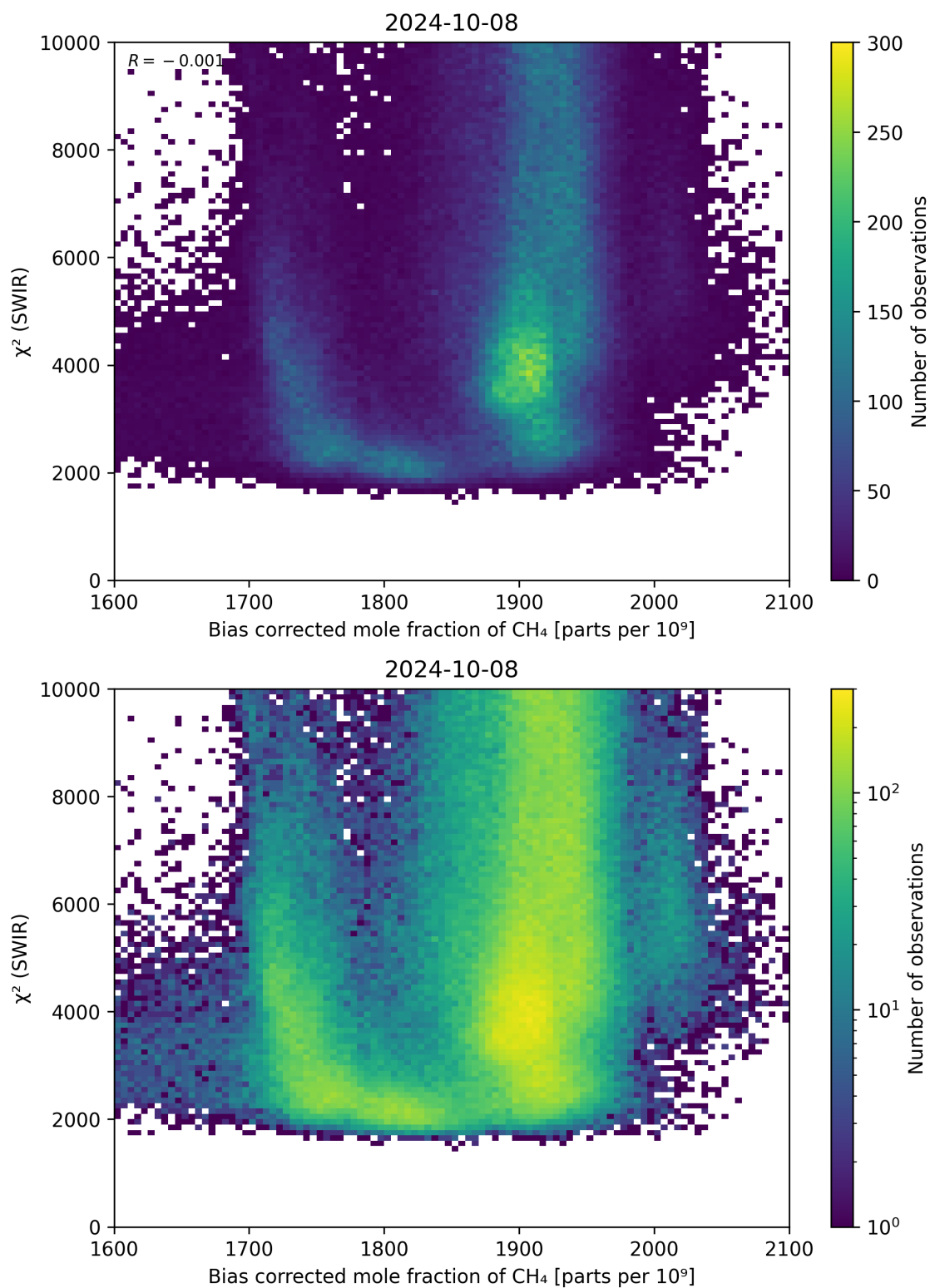
Figure 64: Scatter density plot of “Bias corrected mole fraction of \text{CH}_4 ” against “ \chi^2 (SWIR)” for 2024-10-08 to 2024-10-09.
