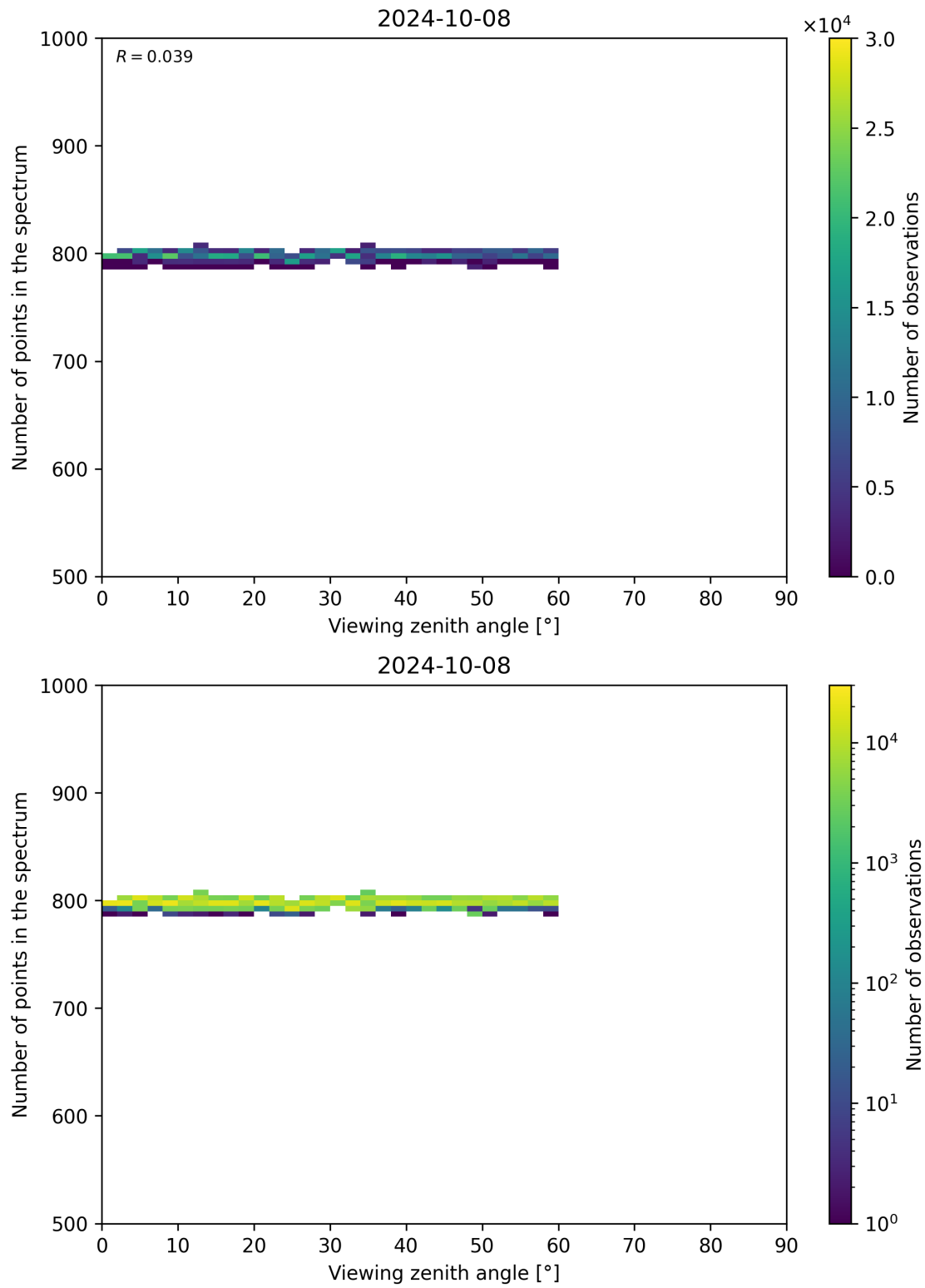
Figure 114: Scatter density plot of “Viewing zenith angle” against “Number of points in the spectrum” for 2024-10-08 to 2024-10-09.
