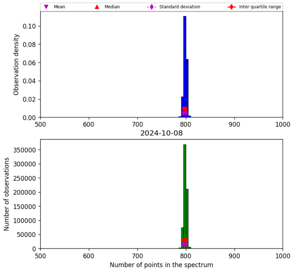
Figure 26: Histogram of “Number of points in the spectrum” for 2024-10-08 to 2024-10-09
