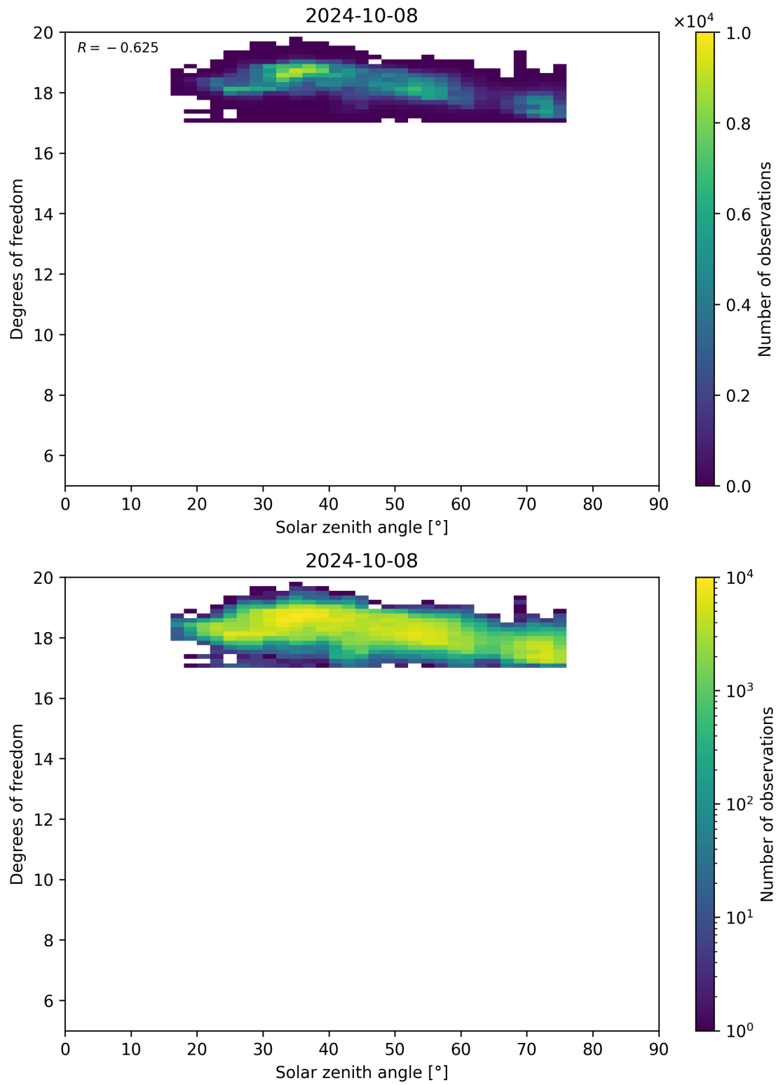
Figure 96: Scatter density plot of “Solar zenith angle” against “Degrees of freedom” for 2024-10-08 to 2024-10-09.
