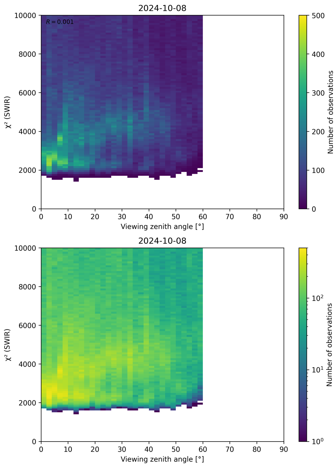
Figure 106: Scatter density plot of “Viewing zenith angle” against “ \chi^2 (SWIR)” for 2024-10-08 to 2024-10-09.
