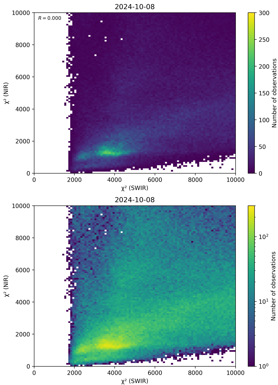
Figure 47: Scatter density plot of “ \chi^2 (SWIR)” against “ \chi^2 (NIR)” for 2024-10-08 to 2024-10-09.
