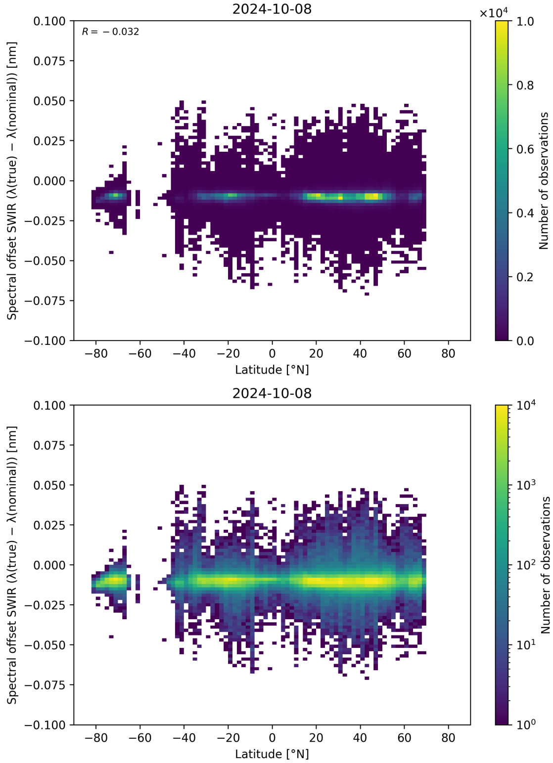
Figure 62: Scatter density plot of “Latitude” against “Spectral offset SWIR ( \lambda_{\text{true}} - \lambda_{\text{nominal}} )” for 2024-10-08 to 2024-10-09.
