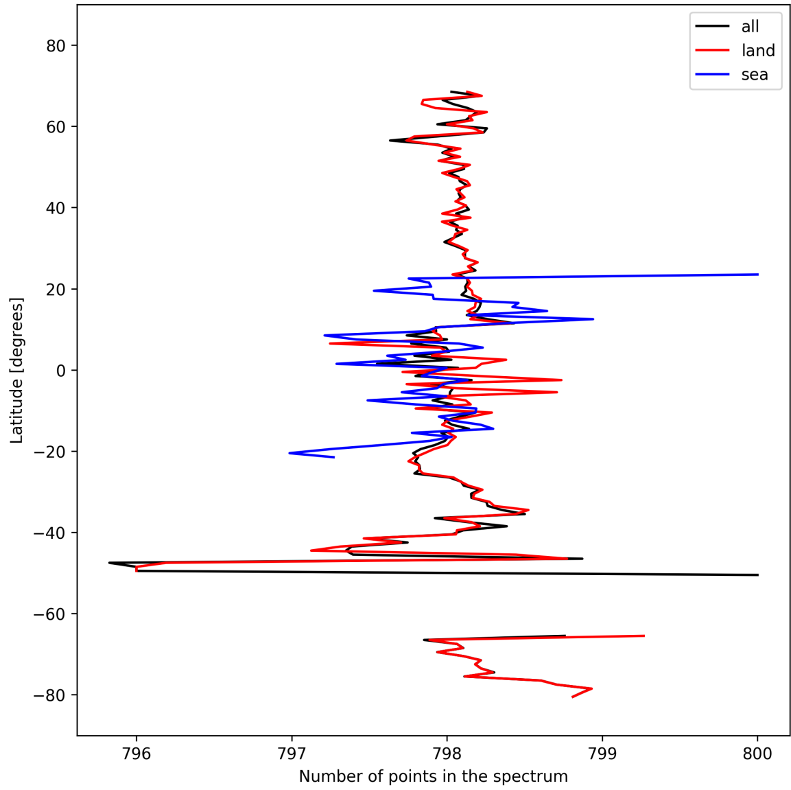
Figure 15: Zonal average of “Number of points in the spectrum” for 2024-10-08 to 2024-10-09.
