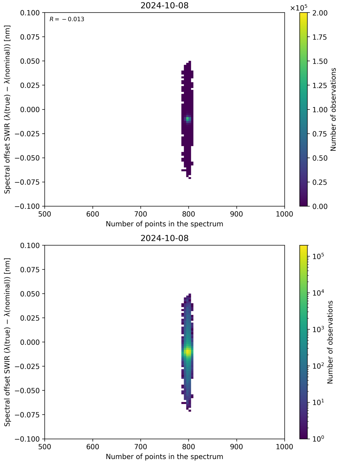
Figure 93: Scatter density plot of “Number of points in the spectrum” against “Spectral offset SWIR ( \lambda_{\text{true}} - \lambda_{\text{nominal}} )” for 2024-10-08 to 2024-10-09.
