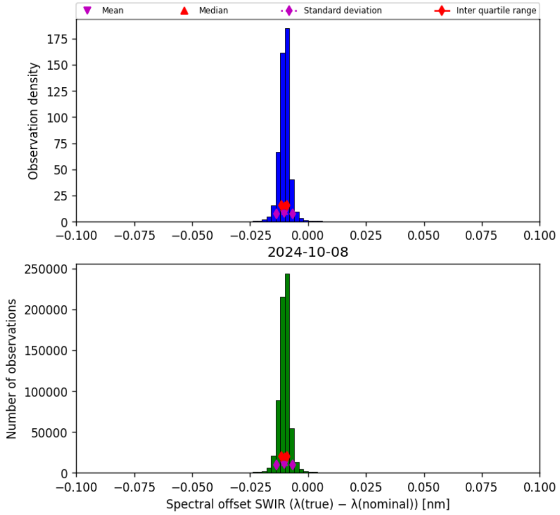
Figure 27: Histogram of “Spectral offset SWIR ( \lambda_{\text{true}} - \lambda_{\text{nominal}} )” for 2024-10-08 to 2024-10-09
