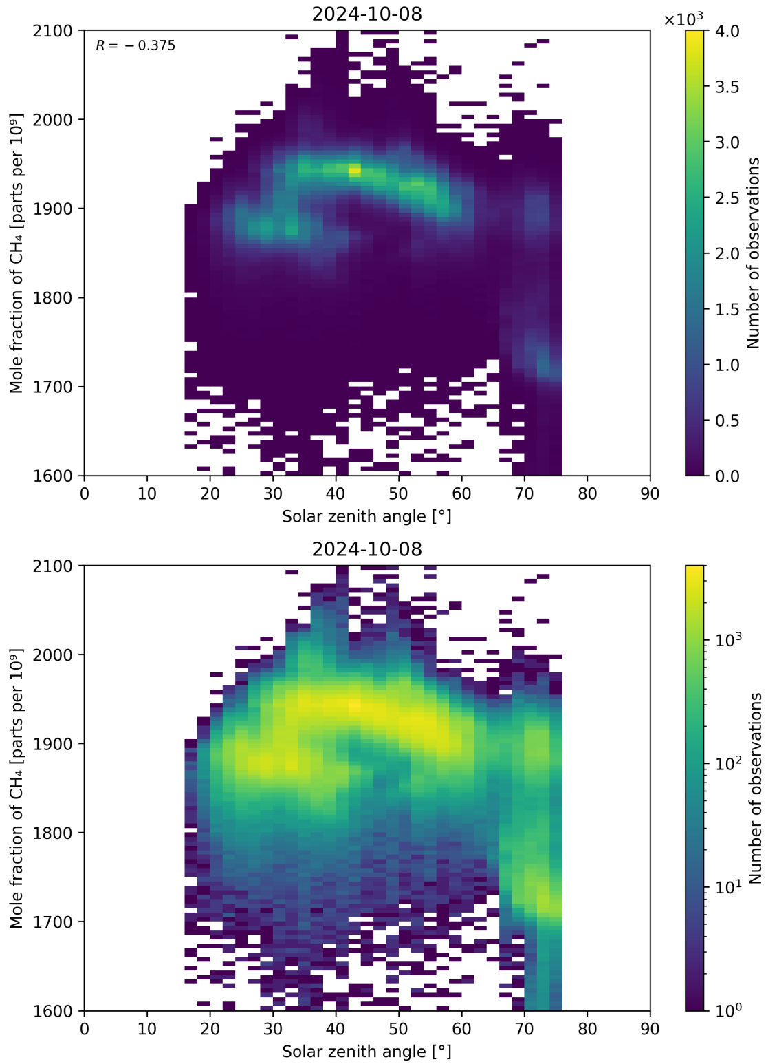
Figure 99: Scatter density plot of “Solar zenith angle” against “Mole fraction of \text{CH}_4 ” for 2024-10-08 to 2024-10-09.
