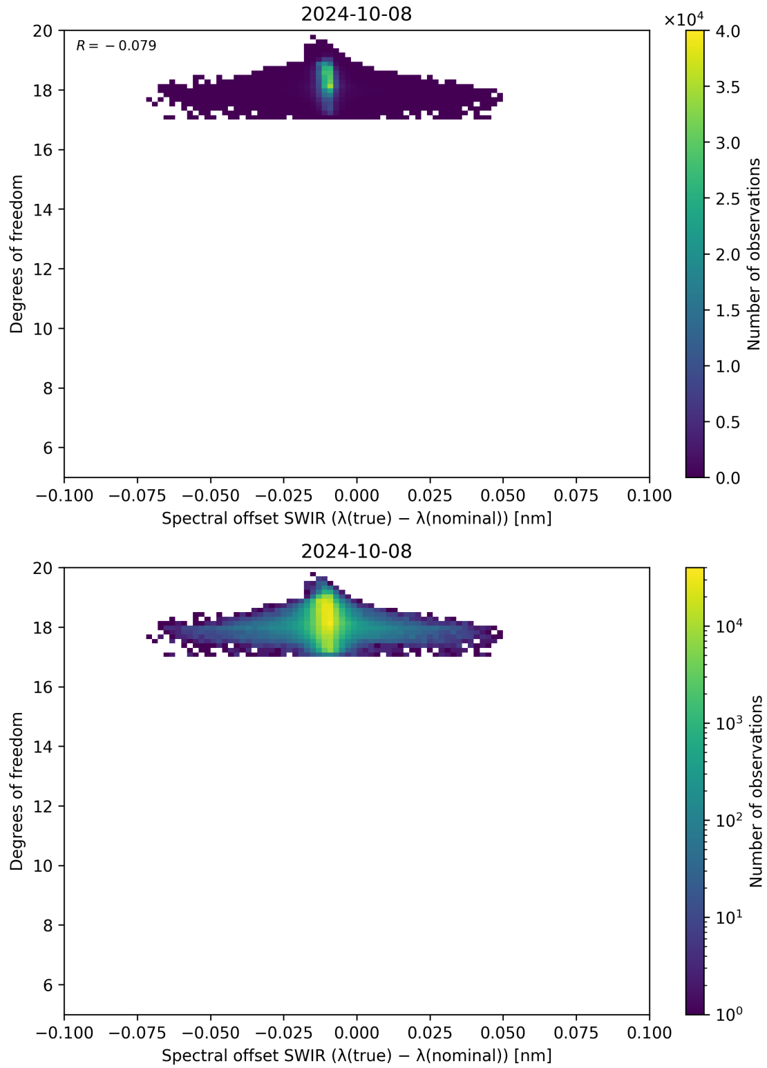
Figure 119: Scatter density plot of “Spectral offset SWIR ( \lambda_{\text{true}} - \lambda_{\text{nominal}} )” against “Degrees of freedom” for 2024-10-08 to 2024-10-09.
