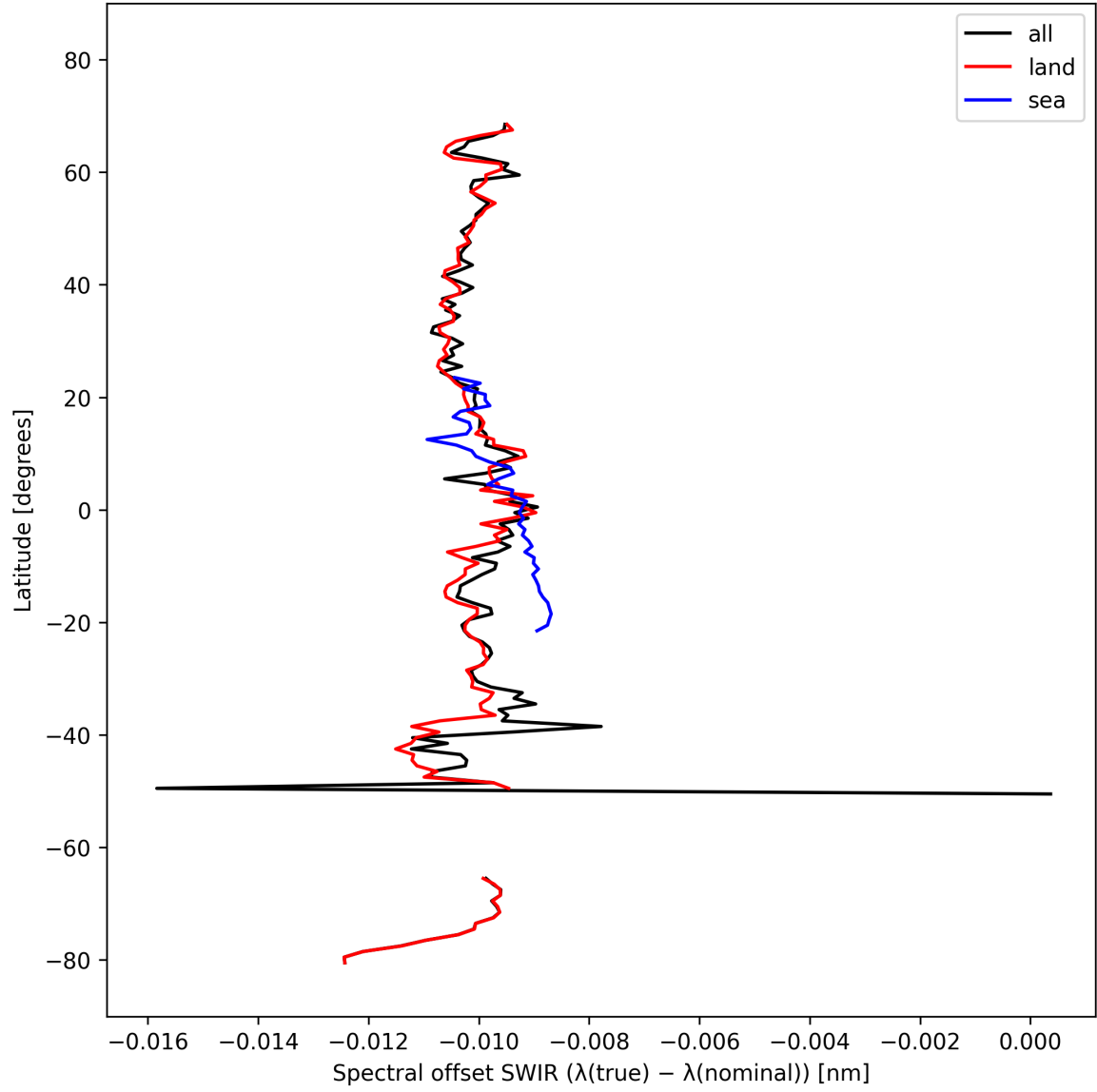
Figure 16: Zonal average of “Spectral offset SWIR ( \lambda_{\text{true}} - \lambda_{\text{nominal}} )” for 2024-10-08 to 2024-10-09.
