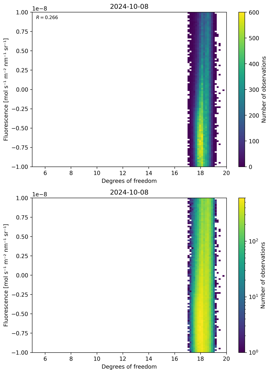
Figure 51: Scatter density plot of “Degrees of freedom” against “Fluorescence” for 2024-10-08 to 2024-10-09.
