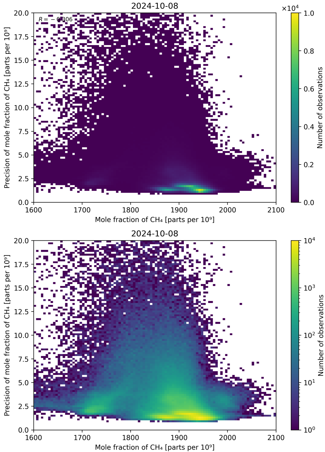
Figure 75: Scatter density plot of “Mole fraction of CH 4 ” against “Precision of mole fraction of CH 4 ” for 2024-10-08 to 2024-10-09.
