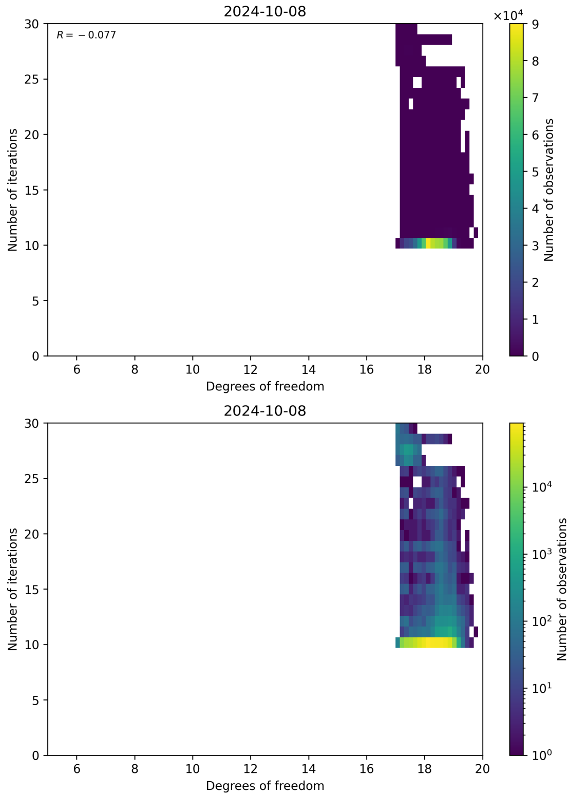
Figure 52: Scatter density plot of “Degrees of freedom” against “Number of iterations” for 2024-10-08 to 2024-10-09.
