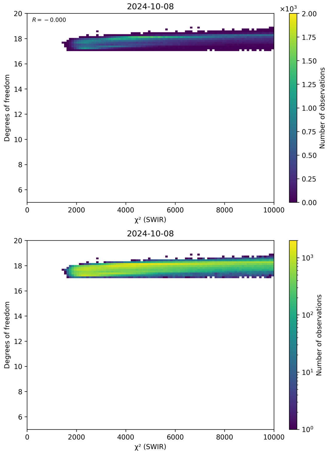
Figure 48: Scatter density plot of “ \chi^2 (SWIR)” against “Degrees of freedom” for 2024-10-08 to 2024-10-09.
