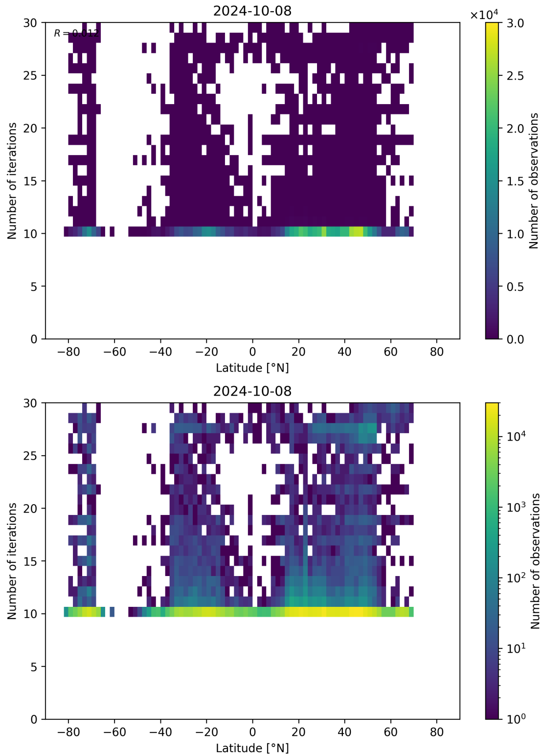
Figure 60: Scatter density plot of “Latitude” against “Number of iterations” for 2024-10-08 to 2024-10-09.
