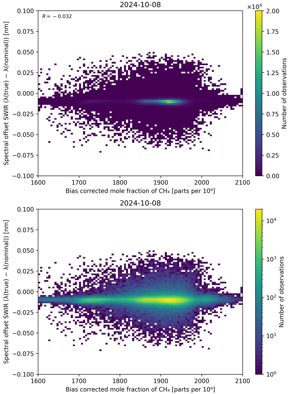
Figure 69: Scatter density plot of “Bias corrected mole fraction of \text{CH}_4 ” against “Spectral offset SWIR ( \lambda_{\text{true}} - \lambda_{\text{nominal}} )” for 2024-10-08 to 2024-10-09.
