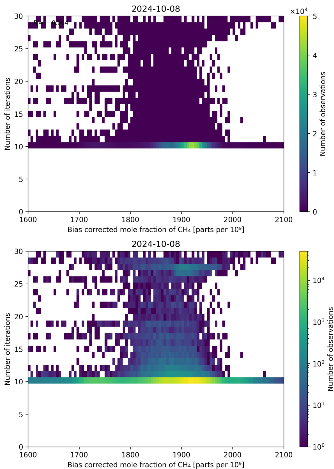
Figure 67: Scatter density plot of “Bias corrected mole fraction of CH 4 ” against “Number of iterations” for 2024-10-08 to 2024-10-09.
