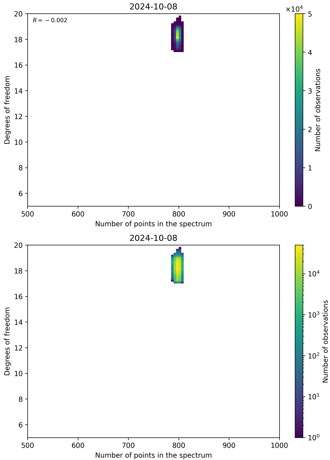
Figure 90: Scatter density plot of “Number of points in the spectrum” against “Degrees of freedom” for 2024-10-08 to 2024-10-09.
