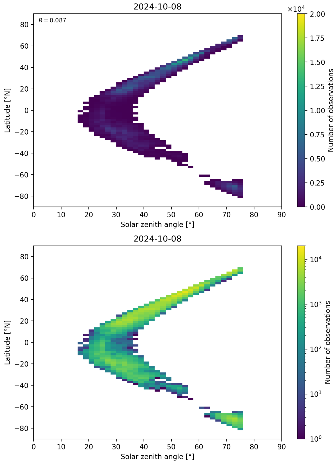
Figure 98: Scatter density plot of “Solar zenith angle” against “Latitude” for 2024-10-08 to 2024-10-09.
