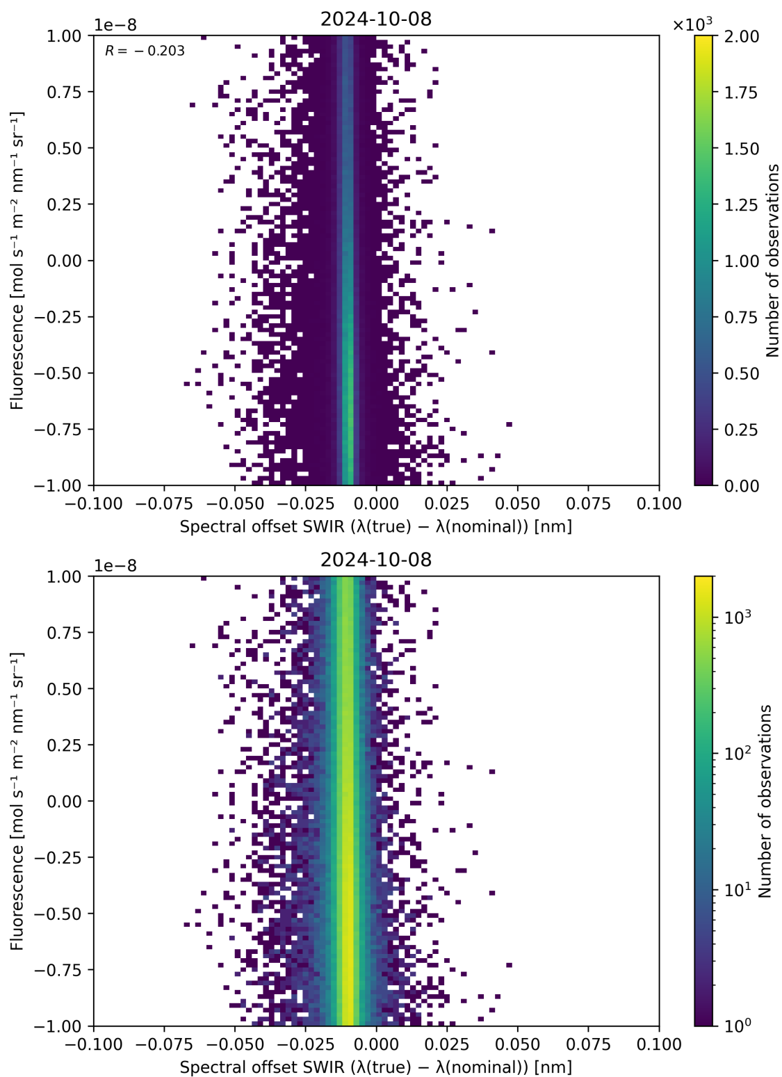
Figure 120: Scatter density plot of “Spectral offset SWIR ( \lambda_{\text{true}} - \lambda_{\text{nominal}} )” against “Fluorescence” for 2024-10-08 to 2024-10-09.
