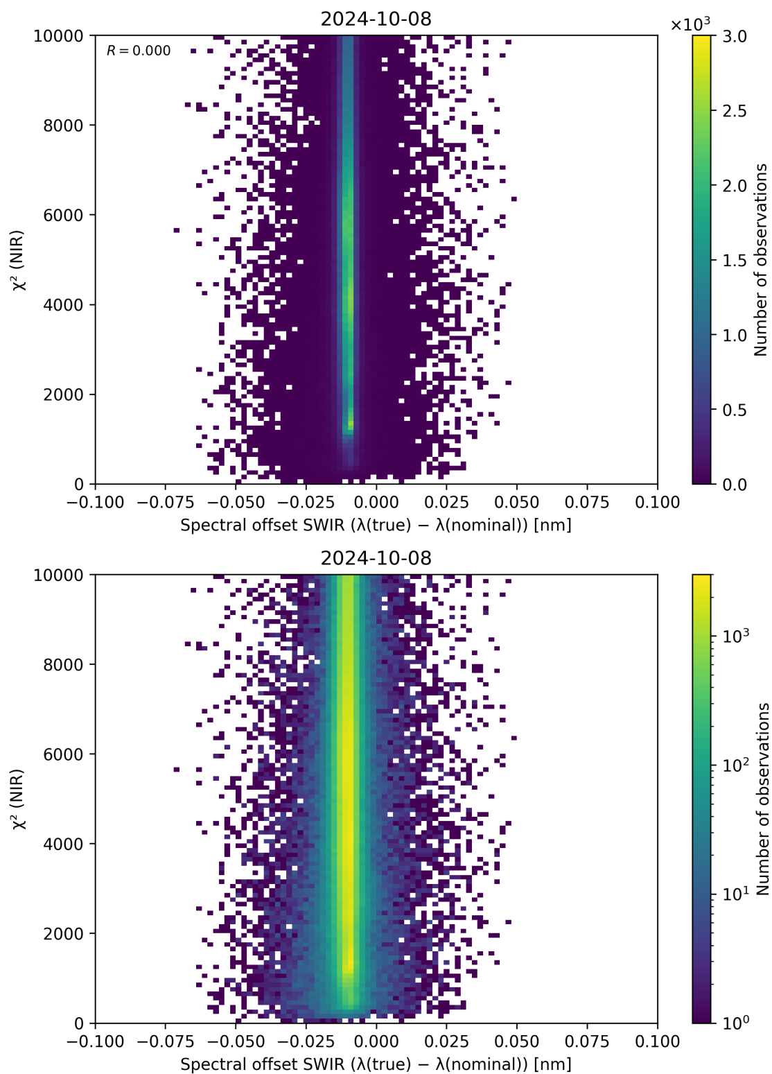
Figure 117: Scatter density plot of “Spectral offset SWIR ( \lambda_{\text{true}} - \lambda_{\text{nominal}} )” against “ \chi^2 (NIR)” for 2024-10-08 to 2024-10-09.
