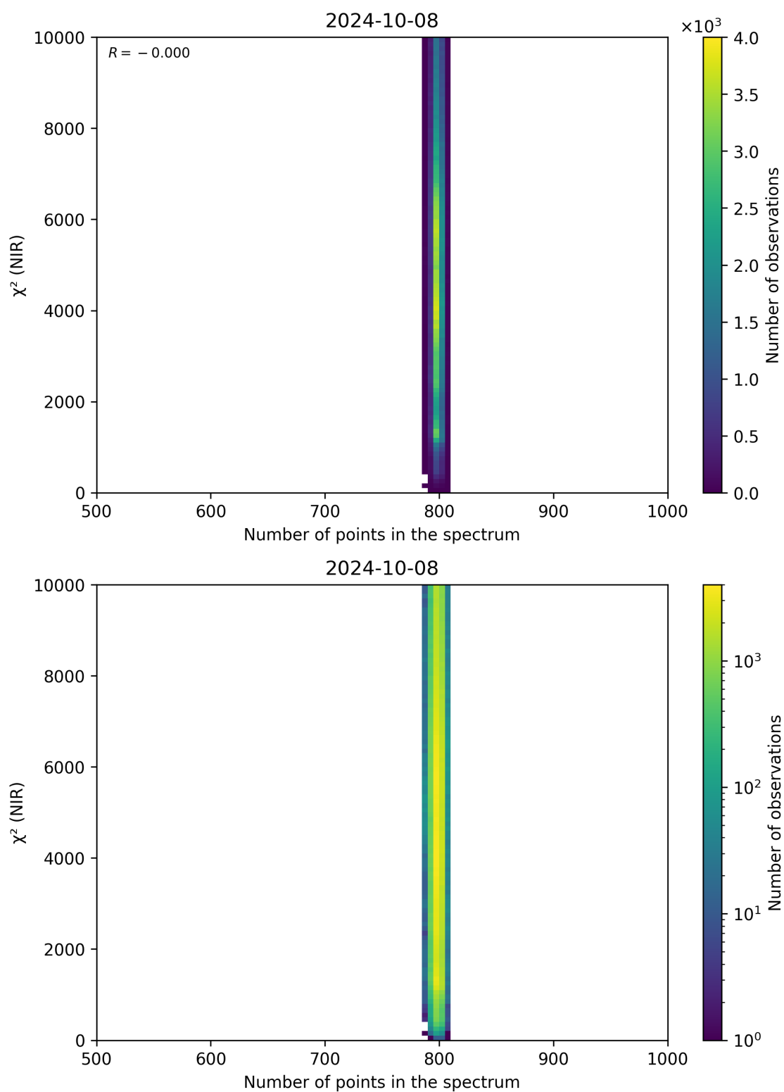
Figure 88: Scatter density plot of “Number of points in the spectrum” against “ \chi^2 (NIR)” for 2024-10-08 to 2024-10-09.
