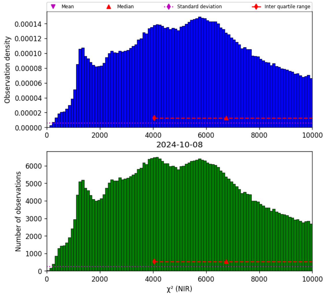
Figure 29: Histogram of “ \chi^2 (NIR)” for 2024-10-08 to 2024-10-09
