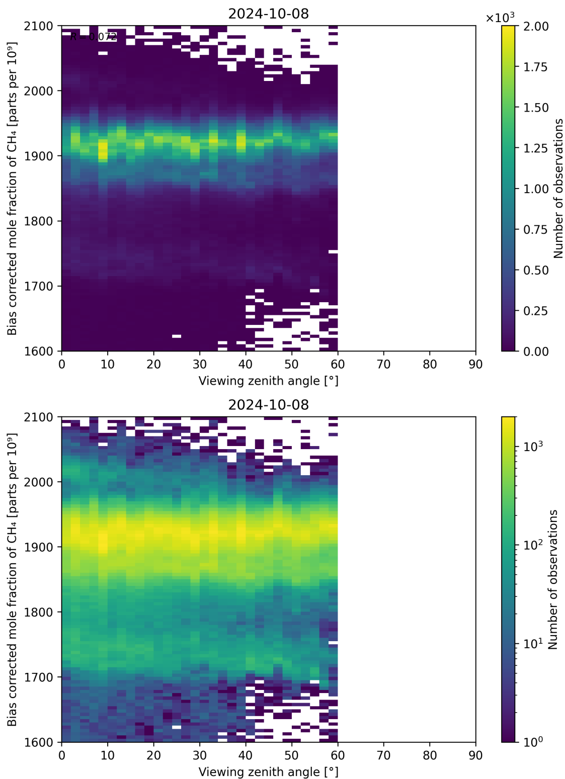
Figure 111: Scatter density plot of “Viewing zenith angle” against “Bias corrected mole fraction of CH 4 ” for 2024-10-08 to 2024-10-09.
