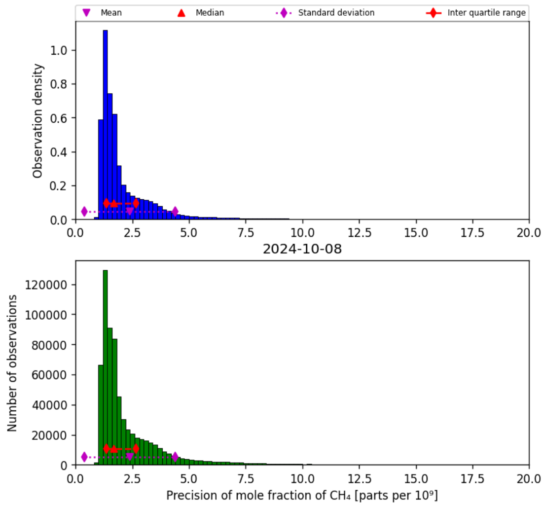
Figure 24: Histogram of “Precision of mole fraction of CH 4 ” for 2024-10-08 to 2024-10-09
