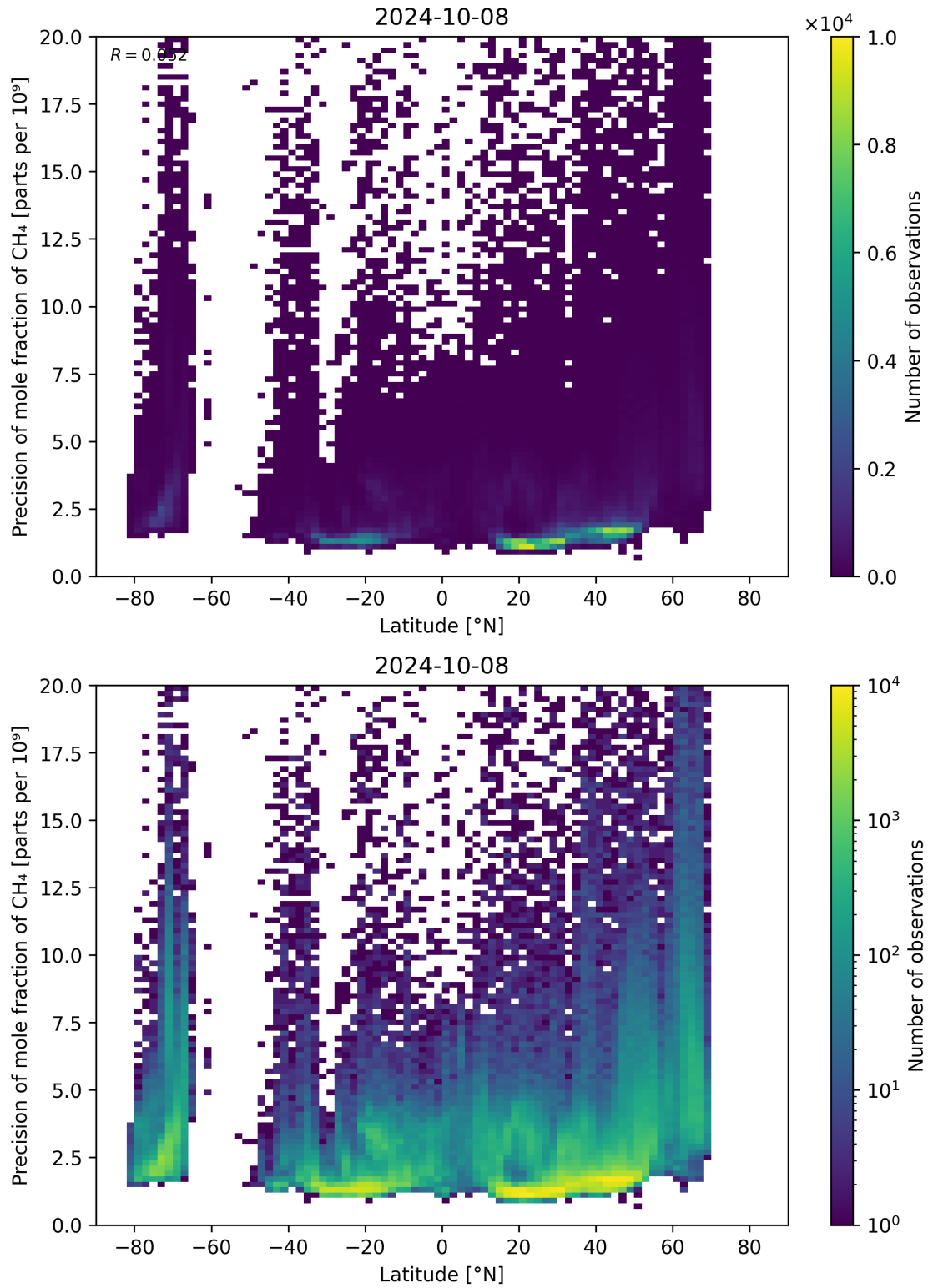
Figure 59: Scatter density plot of “Latitude” against “Precision of mole fraction of \text{CH}_4 ” for 2024-10-08 to 2024-10-09.
