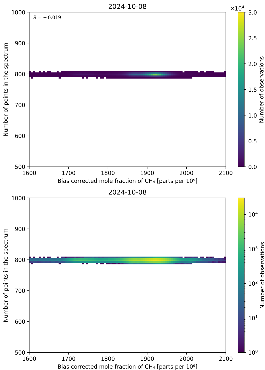
Figure 68: Scatter density plot of “Bias corrected mole fraction of CH 4 ” against “Number of points in the spectrum” for 2024-10-08 to 2024-10-09.
