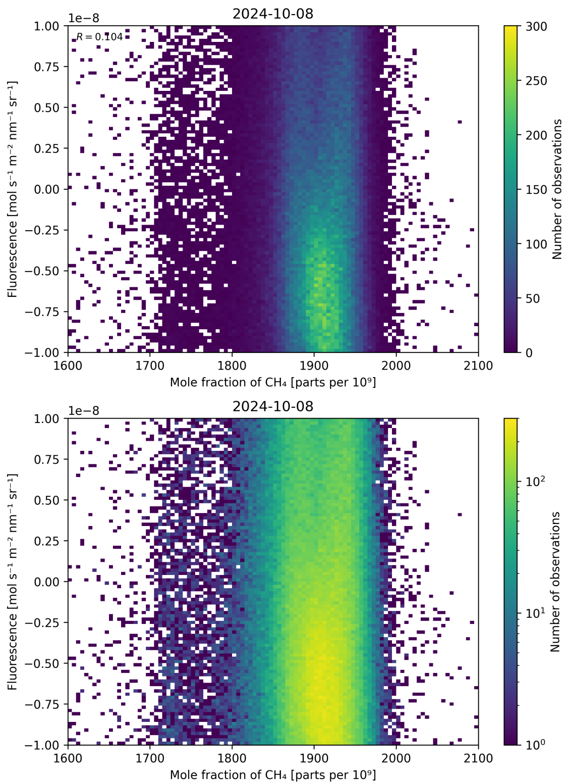
Figure 73: Scatter density plot of “Mole fraction of \text{CH}_4 ” against “Fluorescence” for 2024-10-08 to 2024-10-09.
