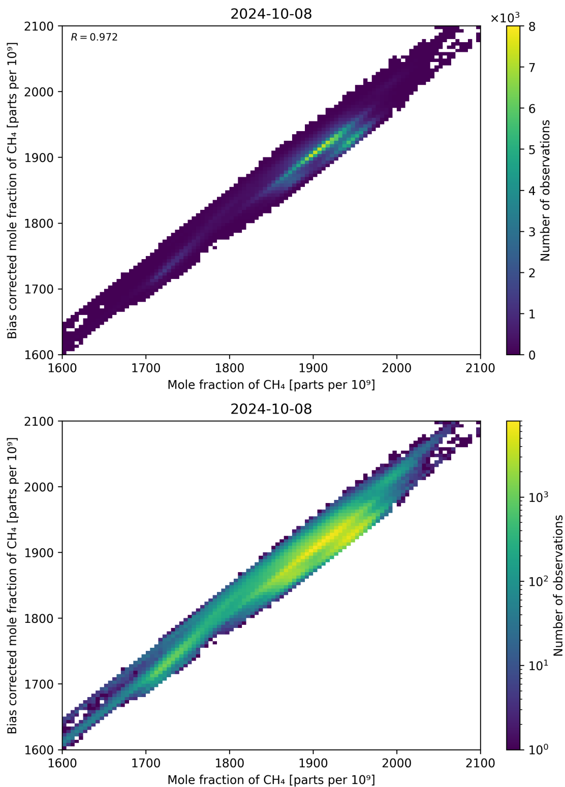
Figure 74: Scatter density plot of “Mole fraction of CH 4 ” against “Bias corrected mole fraction of CH 4 ” for 2024-10-08 to 2024-10-09.
