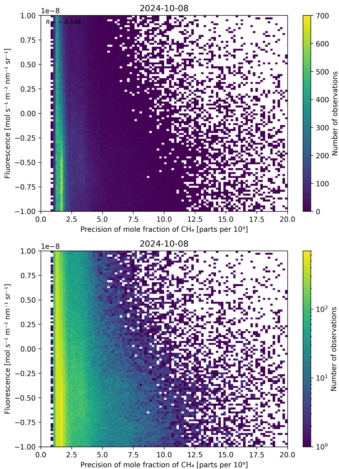
Figure 81: Scatter density plot of “Precision of mole fraction of \text{CH}_4 ” against “Fluorescence” for 2024-10-08 to 2024-10-09.
