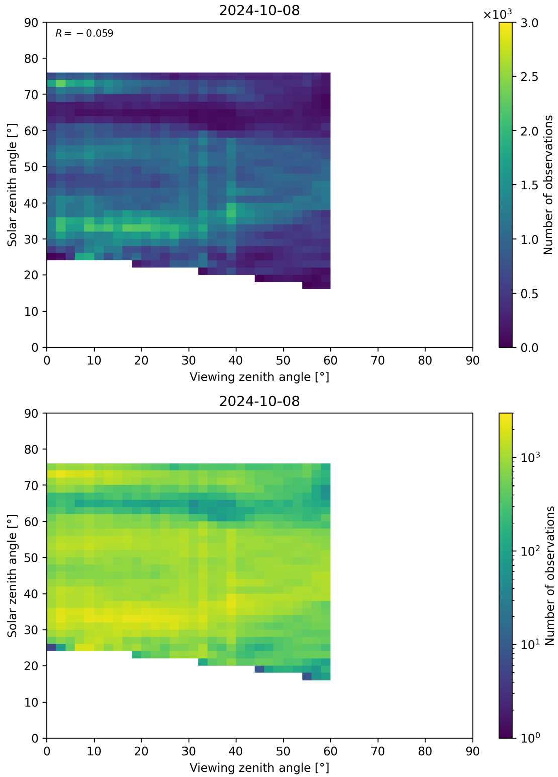
Figure 115: Scatter density plot of “Viewing zenith angle” against “Solar zenith angle” for 2024-10-08 to 2024-10-09.
