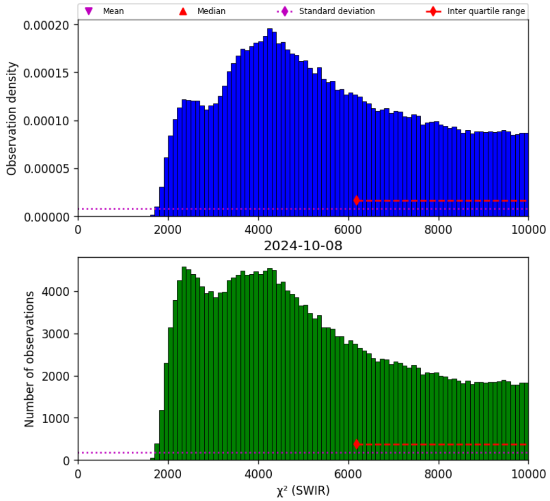
Figure 28: Histogram of " \chi^2 (SWIR)" for 2024-10-08 to 2024-10-09
