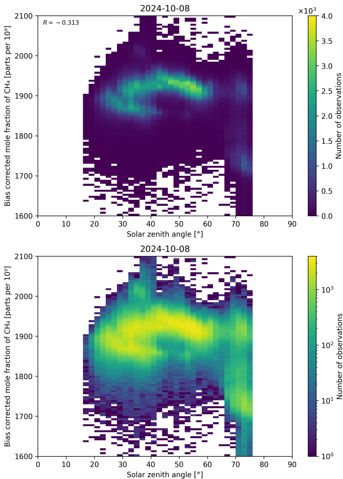
Figure 100: Scatter density plot of “Solar zenith angle” against “Bias corrected mole fraction of \text{CH}_4 ” for 2024-10-08 to 2024-10-09.
