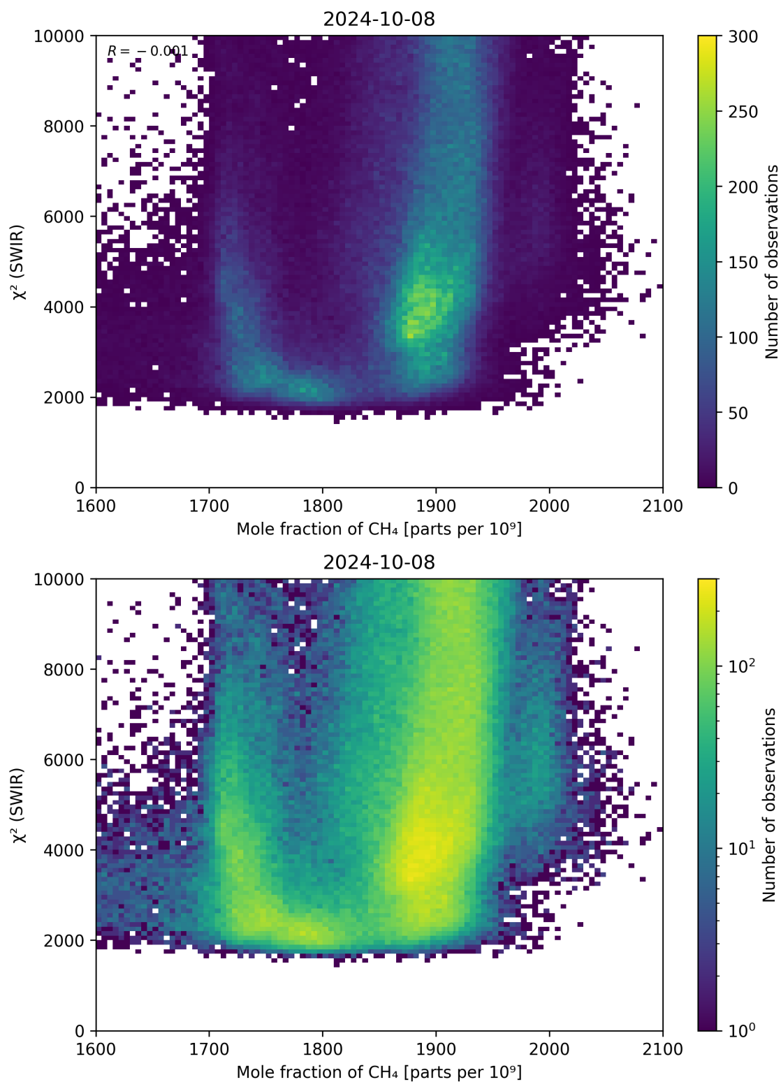
Figure 71: Scatter density plot of “Mole fraction of \text{CH}_4 ” against “ \chi^2 (SWIR)” for 2024-10-08 to 2024-10-09.
