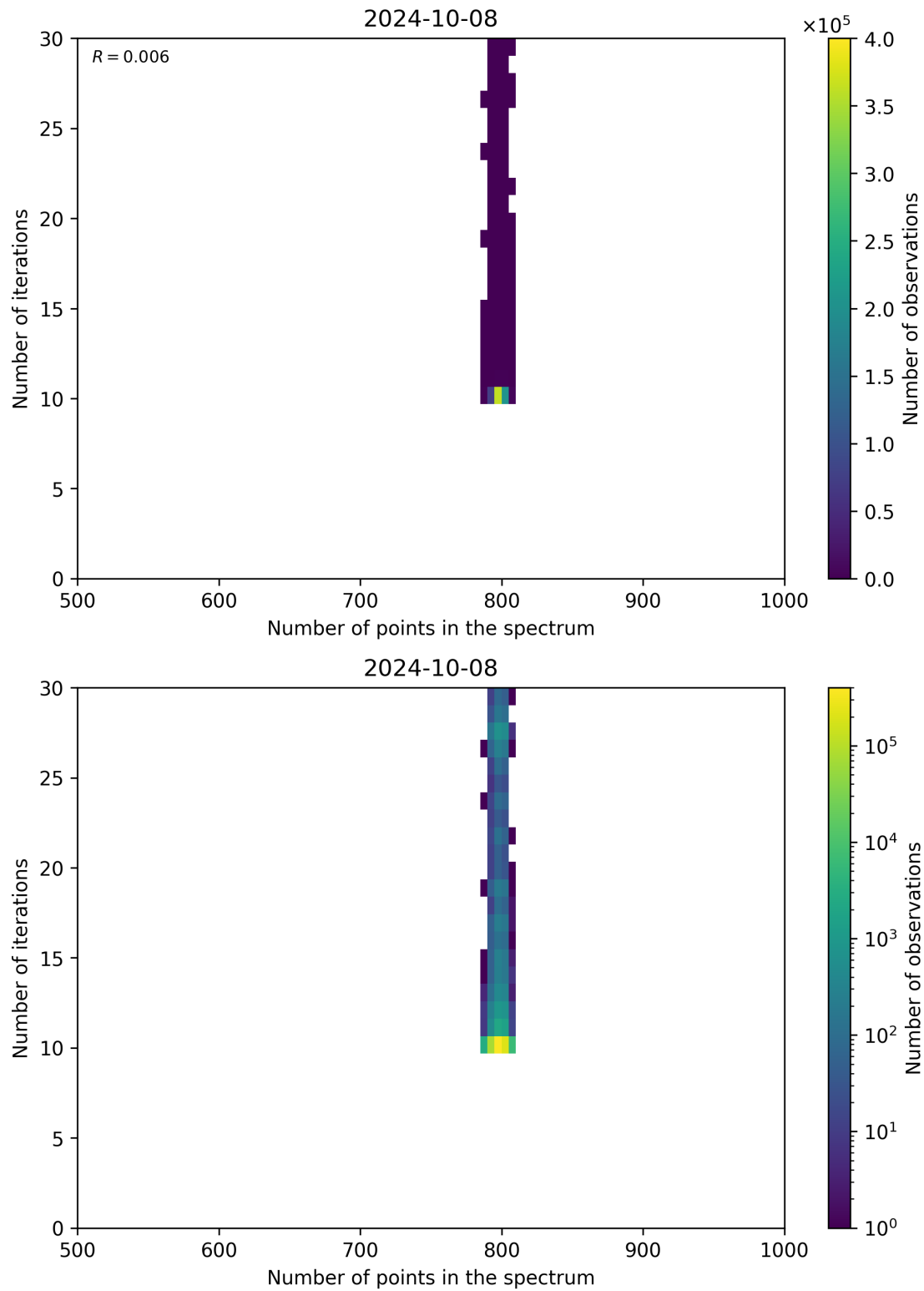
Figure 92: Scatter density plot of “Number of points in the spectrum” against “Number of iterations” for 2024-10-08 to 2024-10-09.
