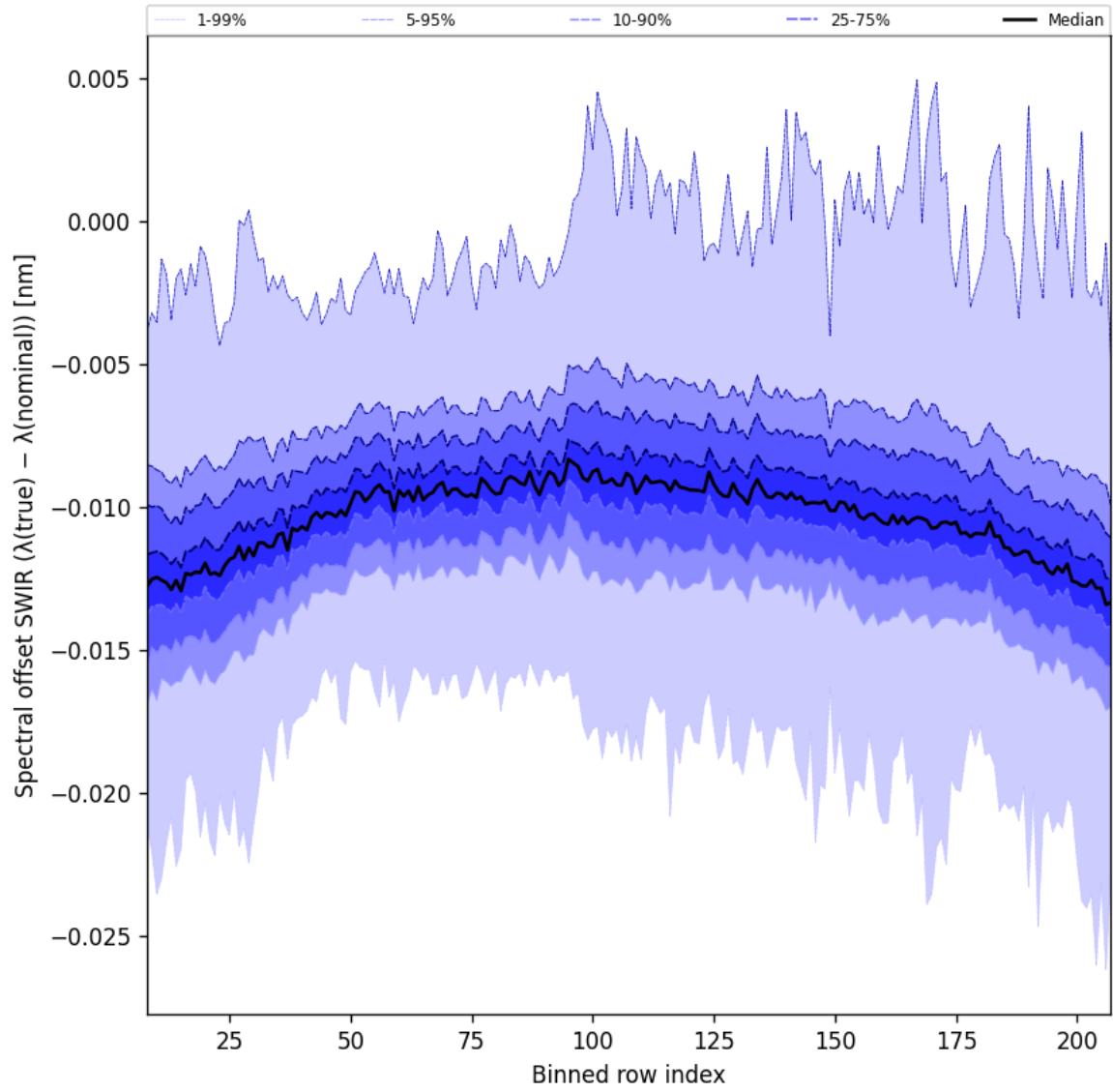
Figure 38: Along track statistics of “Spectral offset SWIR ( \lambda_{\text{true}} - \lambda_{\text{nominal}} )” for 2024-10-08 to 2024-10-09
