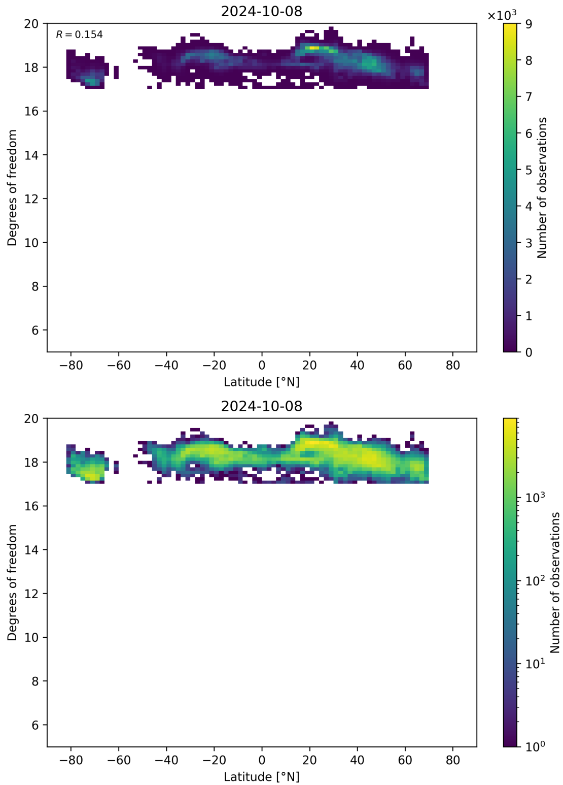
Figure 55: Scatter density plot of “Latitude” against “Degrees of freedom” for 2024-10-08 to 2024-10-09.
