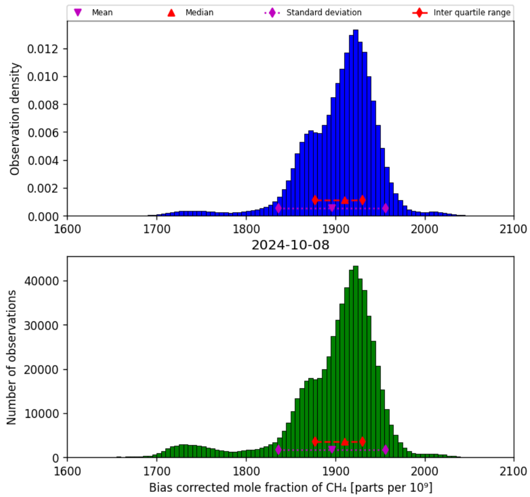
Figure 25: Histogram of “Bias corrected mole fraction of CH 4 ” for 2024-10-08 to 2024-10-09
