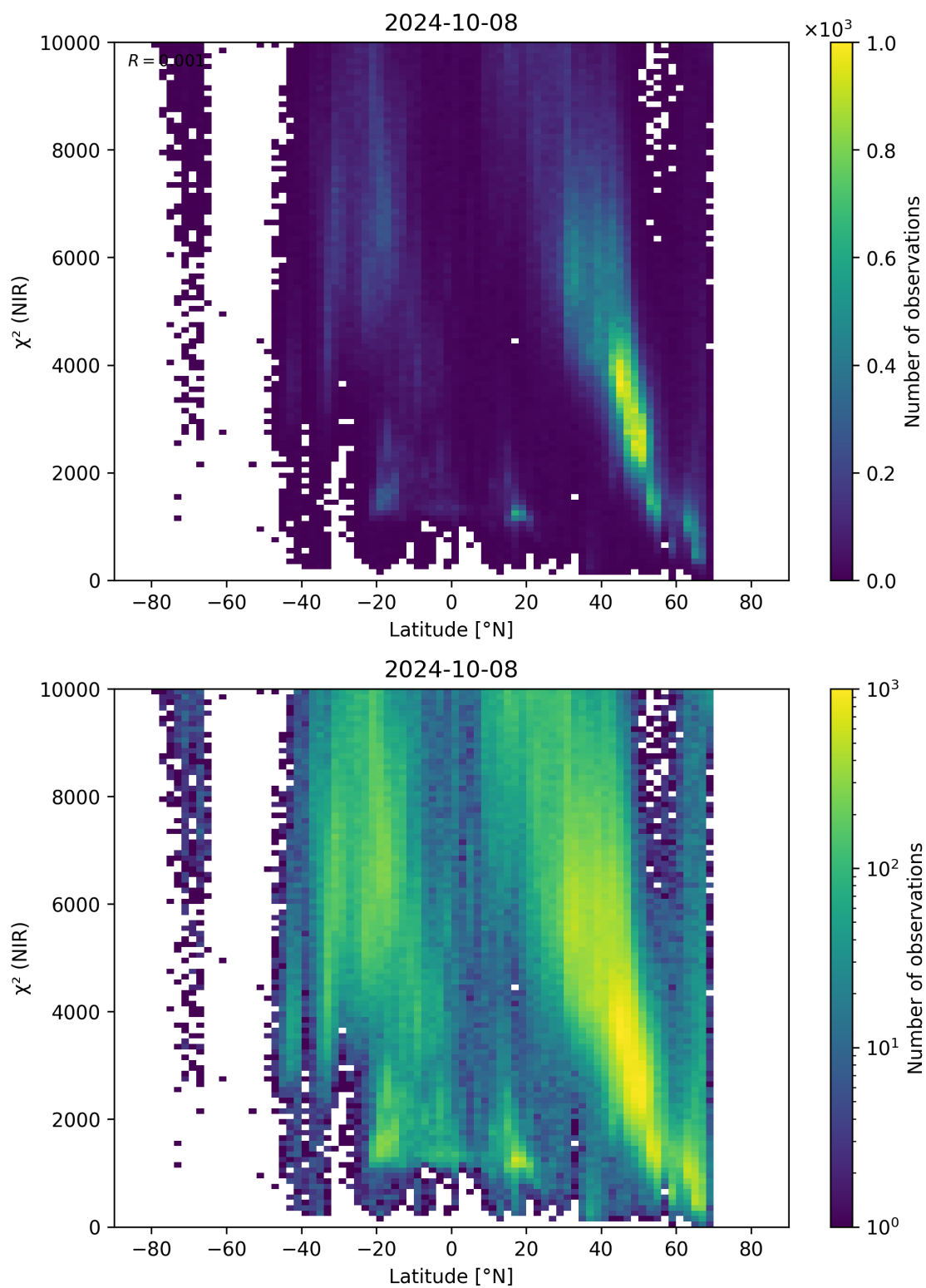
Figure 53: Scatter density plot of “Latitude” against “ \chi^2 (NIR)” for 2024-10-08 to 2024-10-09.
