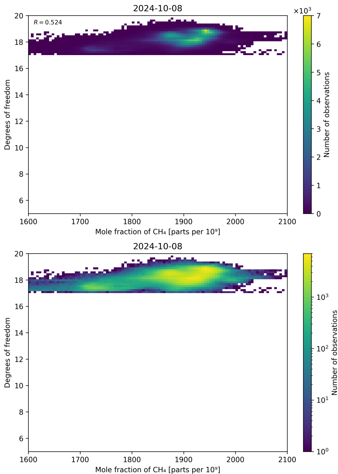
Figure 72: Scatter density plot of “Mole fraction of CH 4 ” against “Degrees of freedom” for 2024-10-08 to 2024-10-09.
