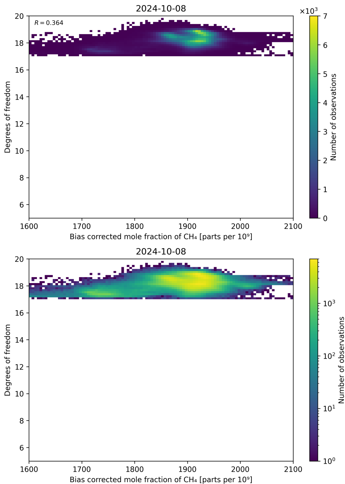
Figure 65: Scatter density plot of “Bias corrected mole fraction of CH 4 ” against “Degrees of freedom” for 2024-10-08 to 2024-10-09.
