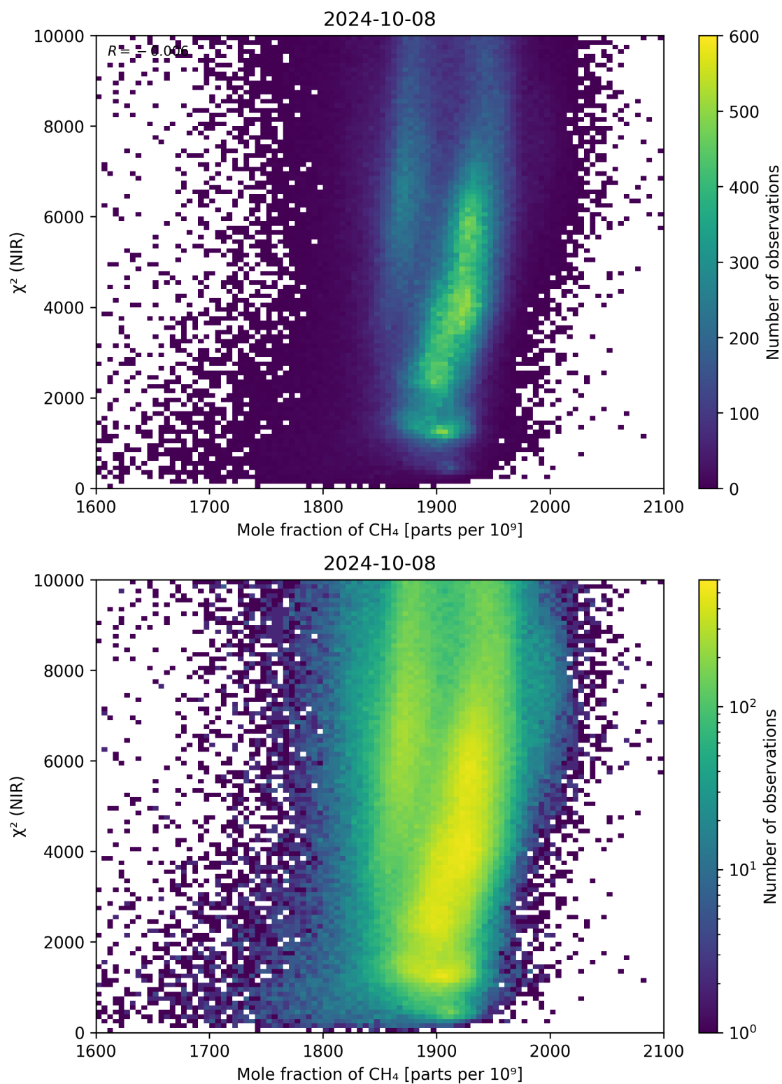
Figure 70: Scatter density plot of “Mole fraction of \text{CH}_4 ” against “ \chi^2 (NIR)” for 2024-10-08 to 2024-10-09.
