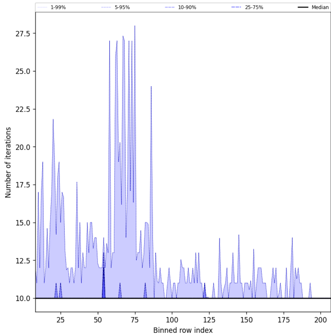
Figure 42: Along track statistics of “Number of iterations” for 2024-10-08 to 2024-10-09
