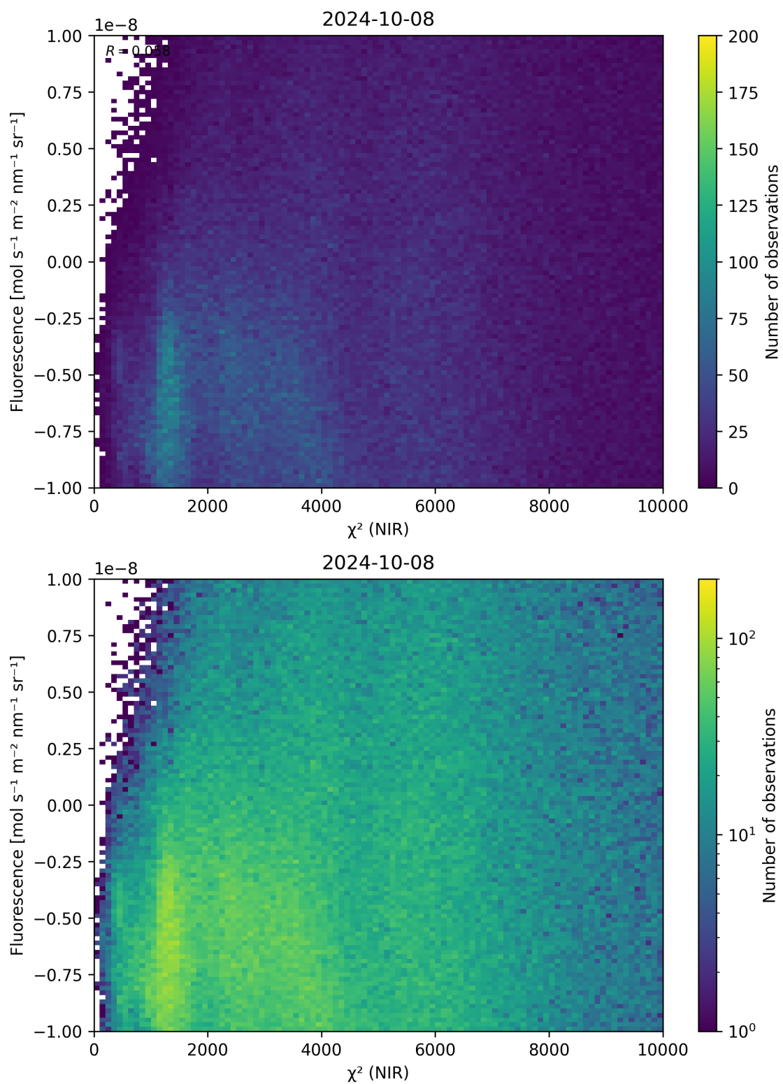
Figure 45: Scatter density plot of “ \chi^2 (NIR)” against “Fluorescence” for 2024-10-08 to 2024-10-09.
