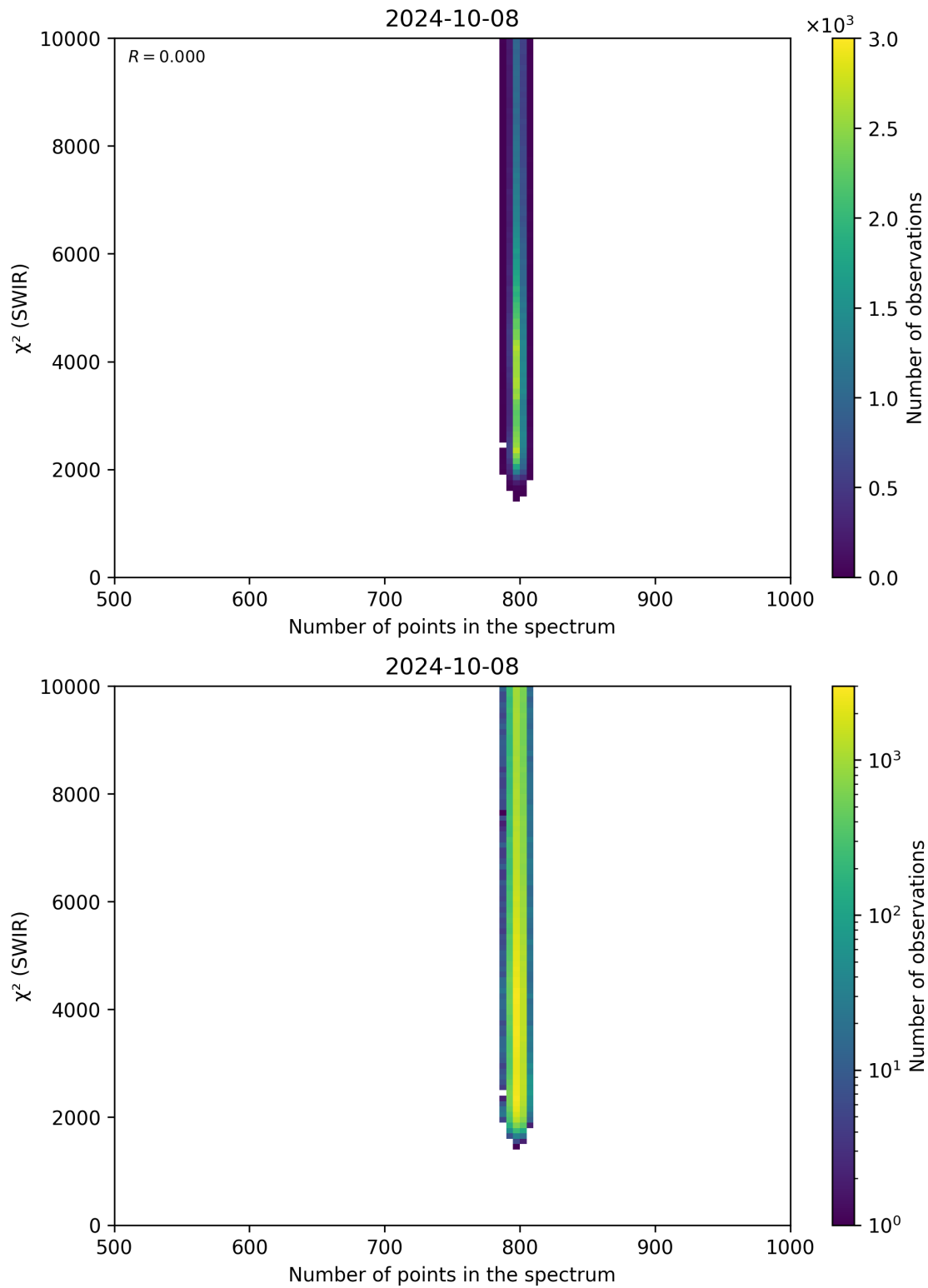
Figure 89: Scatter density plot of “Number of points in the spectrum” against “ \chi^2 (SWIR)” for 2024-10-08 to 2024-10-09.
