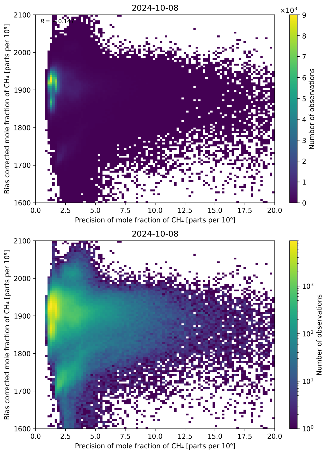
Figure 82: Scatter density plot of “Precision of mole fraction of CH 4 ” against “Bias corrected mole fraction of CH 4 ” for 2024-10-08 to 2024-10-09.
