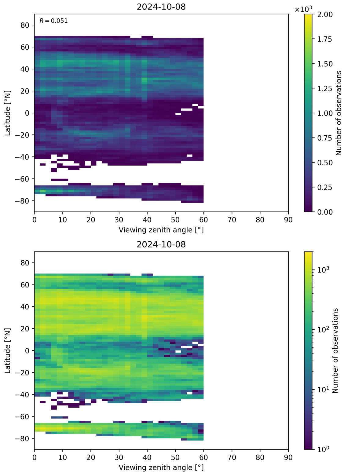
Figure 109: Scatter density plot of “Viewing zenith angle” against “Latitude” for 2024-10-08 to 2024-10-09.
