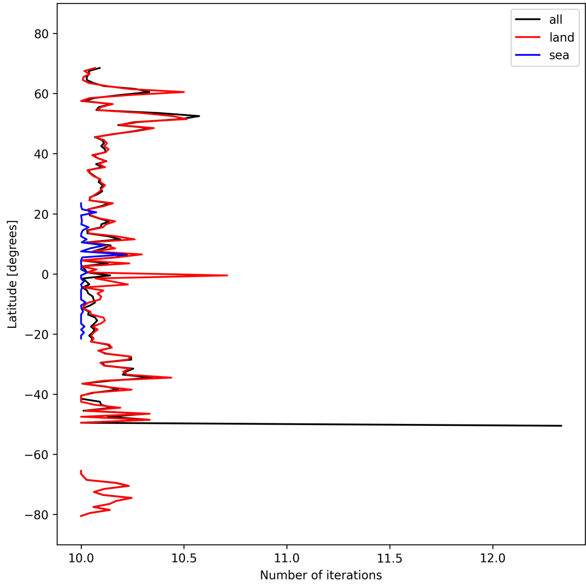
Figure 20: Zonal average of “Number of iterations” for 2024-10-08 to 2024-10-09.
