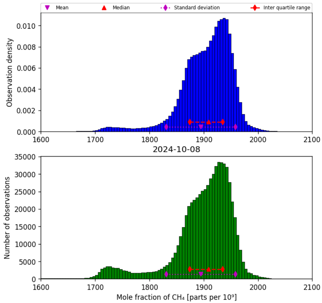
Figure 23: Histogram of “Mole fraction of CH 4 ” for 2024-10-08 to 2024-10-09
