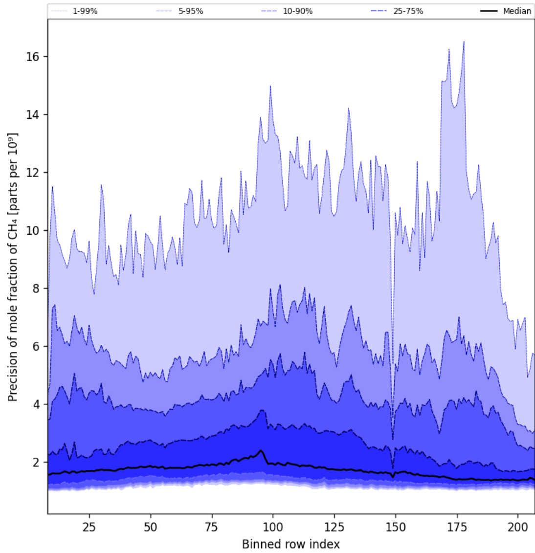
Figure 35: Along track statistics of “Precision of mole fraction of CH 4 ” for 2024-10-08 to 2024-10-09
