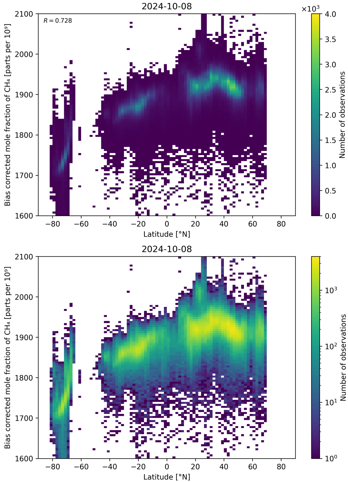
Figure 58: Scatter density plot of “Latitude” against “Bias corrected mole fraction of CH 4 ” for 2024-10-08 to 2024-10-09.
