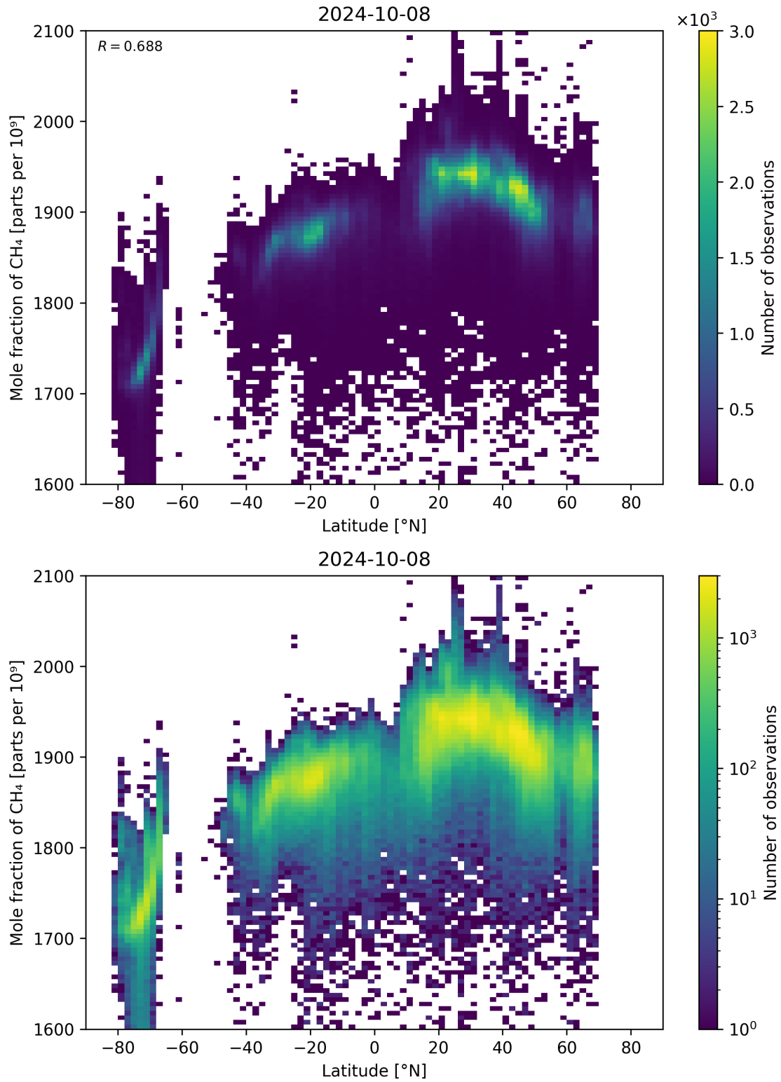
Figure 57: Scatter density plot of “Latitude” against “Mole fraction of CH 4 ” for 2024-10-08 to 2024-10-09.
