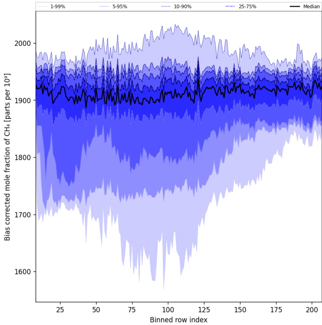
Figure 36: Along track statistics of “Bias corrected mole fraction of \text{CH}_4 ” for 2024-10-08 to 2024-10-09
