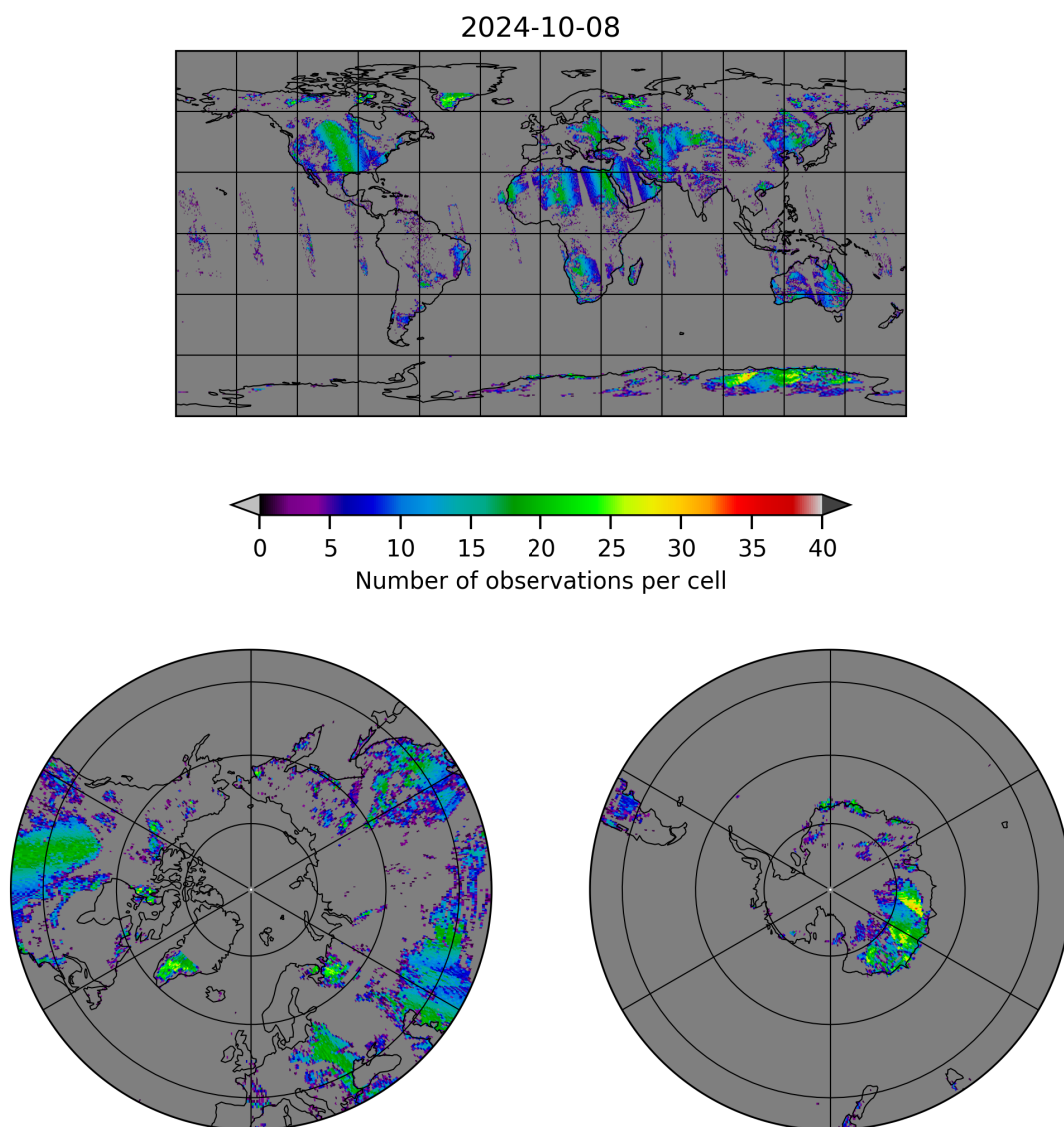
Figure 10: Map of the number of observations for 2024-10-08 to 2024-10-09
