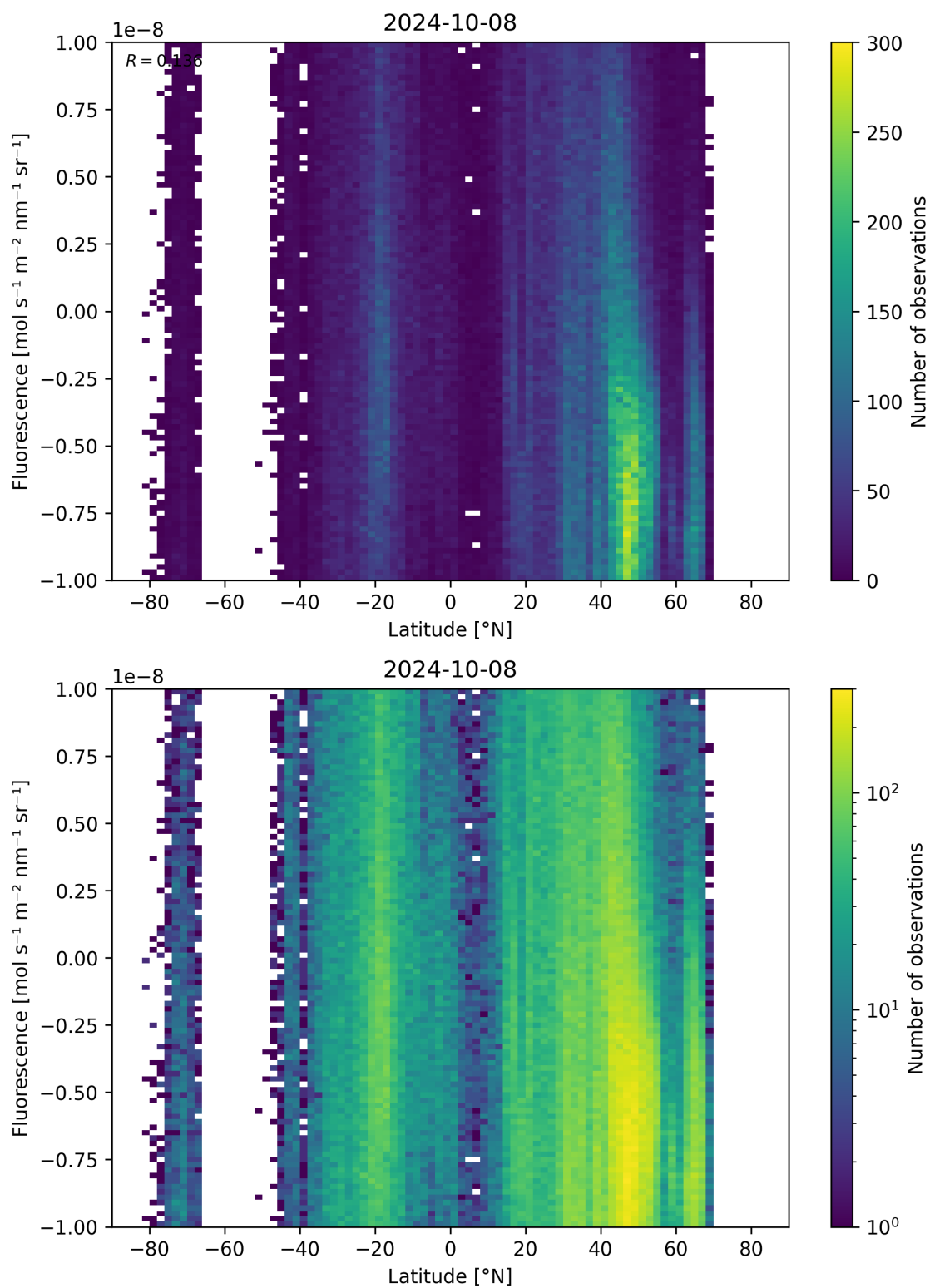
Figure 56: Scatter density plot of “Latitude” against “Fluorescence” for 2024-10-08 to 2024-10-09.
