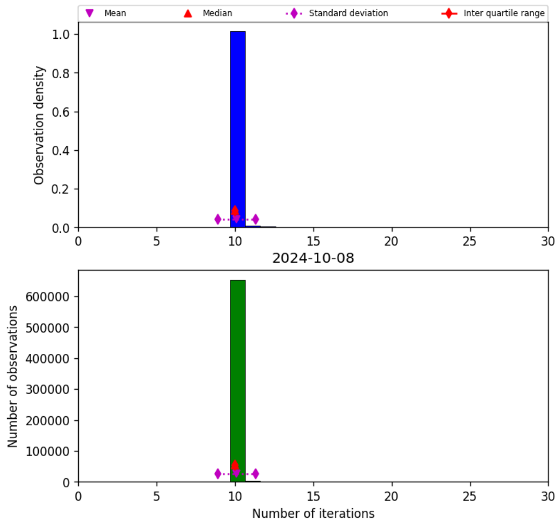
Figure 31: Histogram of “Number of iterations” for 2024-10-08 to 2024-10-09
