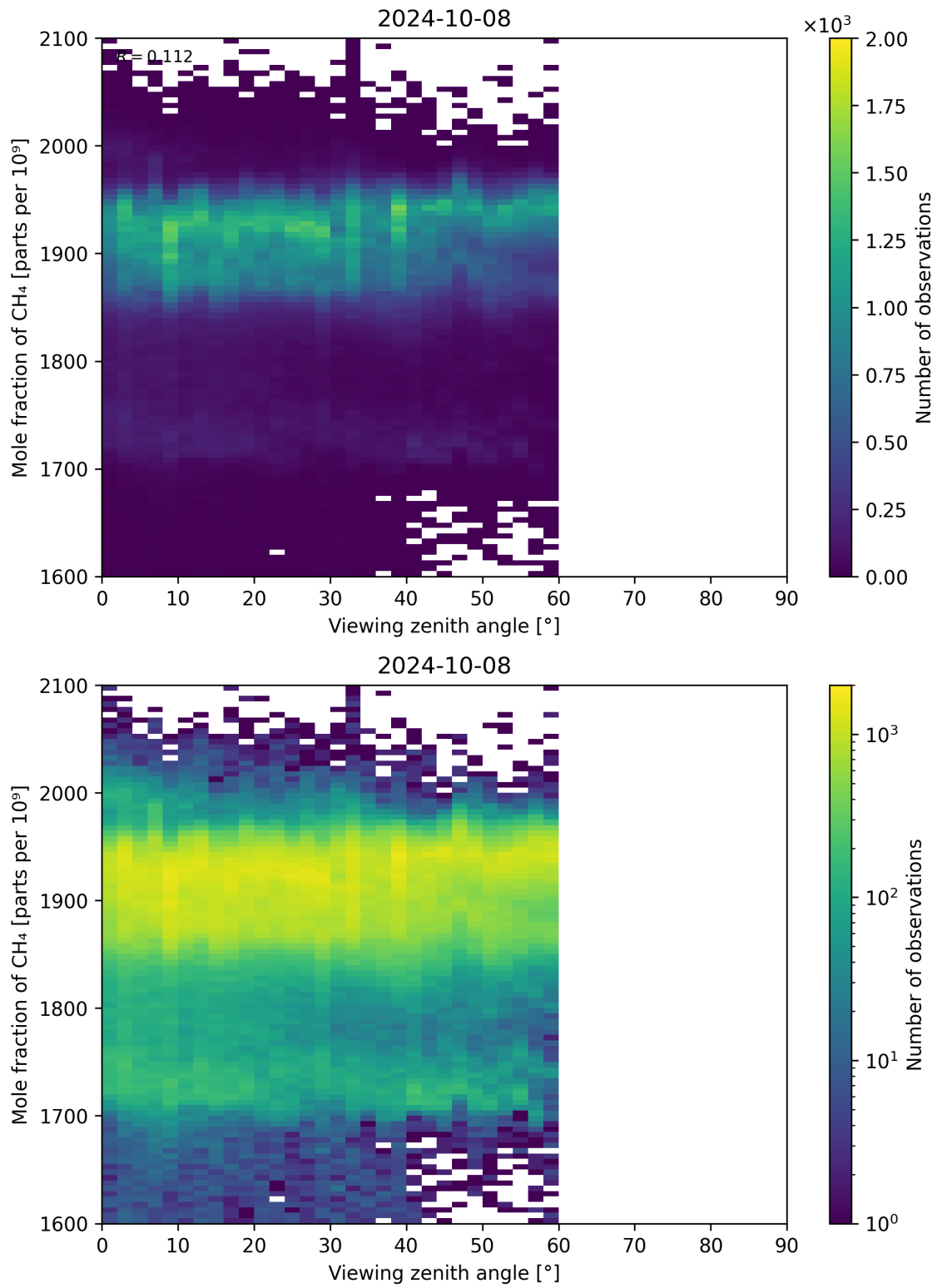
Figure 110: Scatter density plot of “Viewing zenith angle” against “Mole fraction of CH 4 ” for 2024-10-08 to 2024-10-09.
