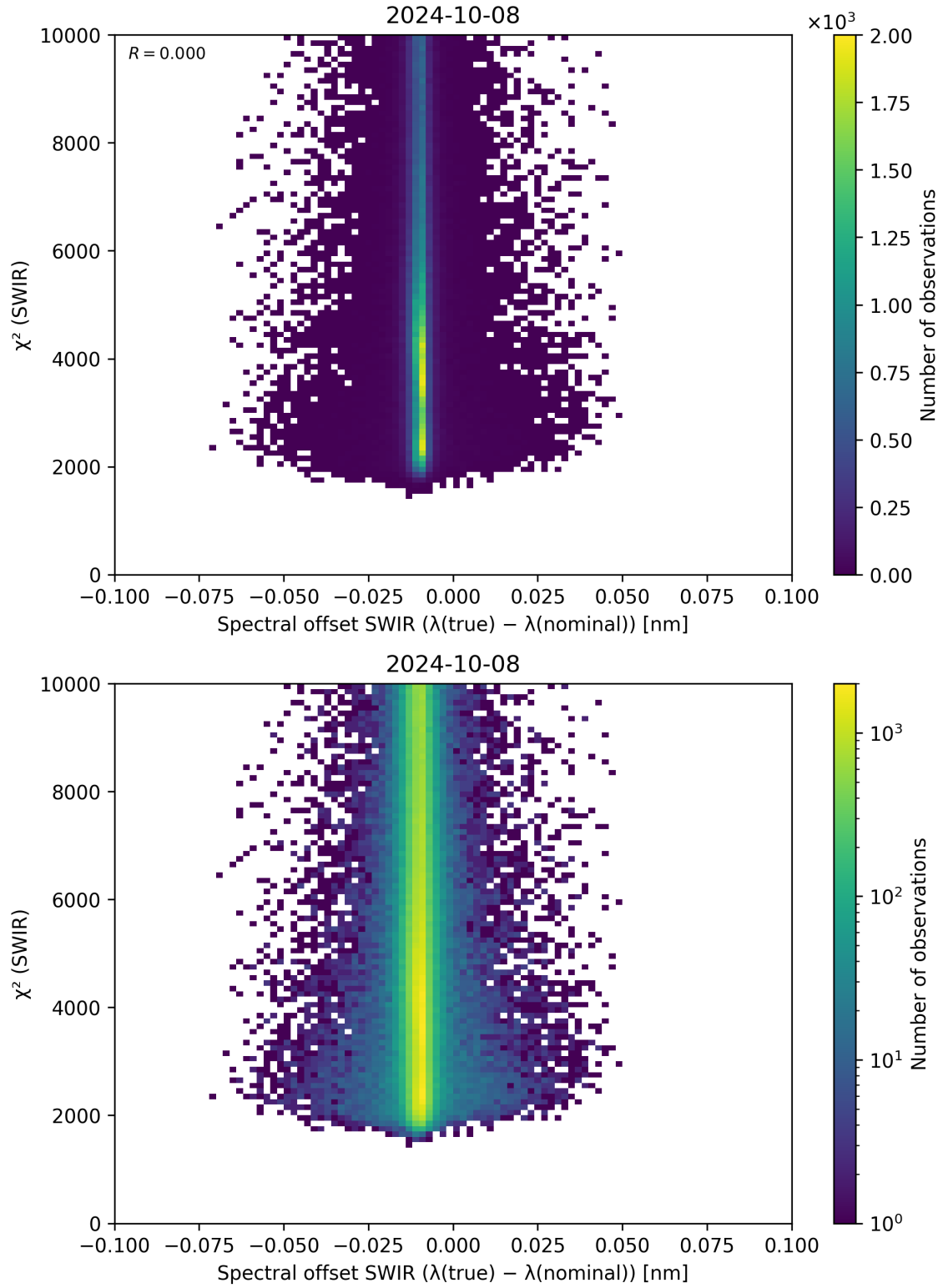
Figure 118: Scatter density plot of “Spectral offset SWIR ( \lambda_{\text{true}} - \lambda_{\text{nominal}} )” against “ \chi^2 (SWIR)” for 2024-10-08 to 2024-10-09.
