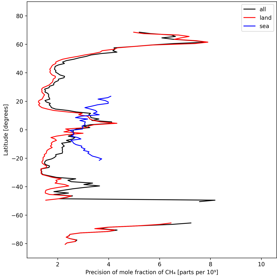
Figure 13: Zonal average of “Precision of mole fraction of CH 4 ” for 2024-10-08 to 2024-10-09.
