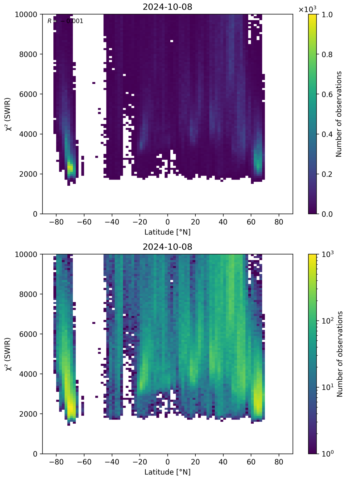
Figure 54: Scatter density plot of “Latitude” against “ \chi^2 (SWIR)” for 2024-10-08 to 2024-10-09.
