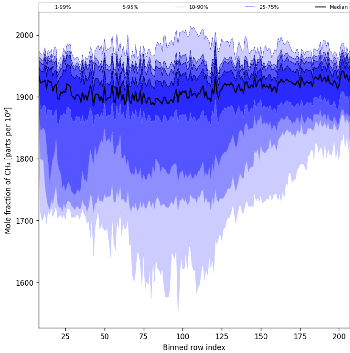
Figure 34: Along track statistics of “Mole fraction of CH 4 ” for 2024-10-08 to 2024-10-09
