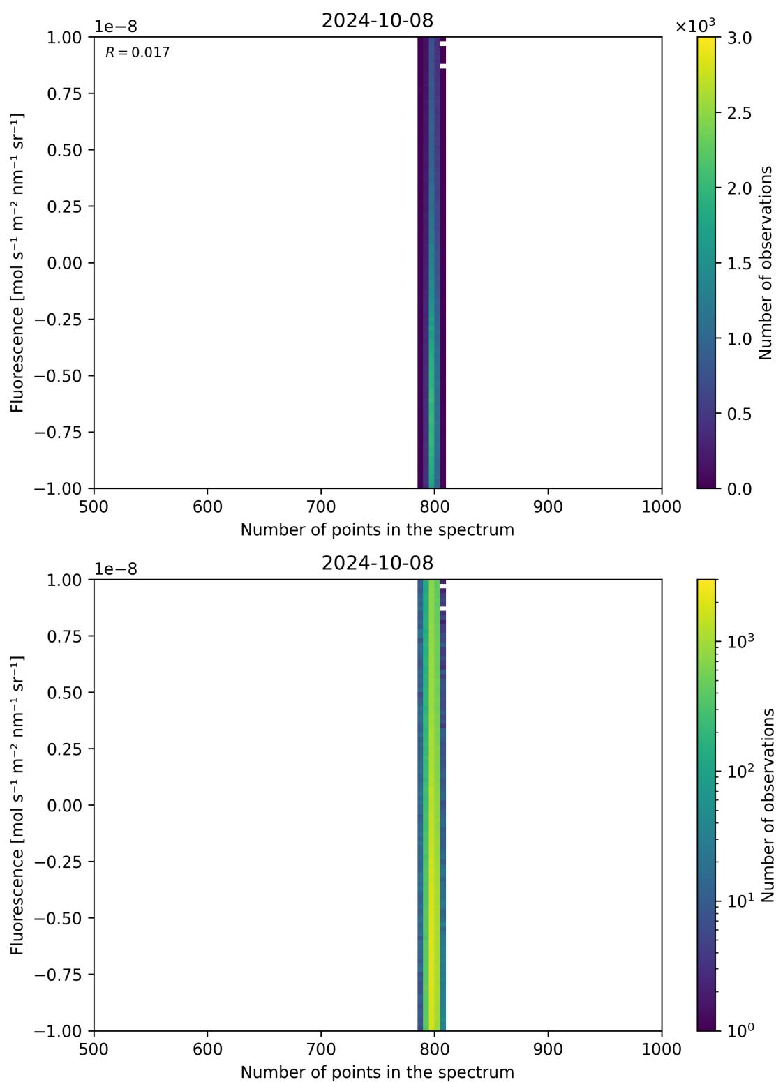
Figure 91: Scatter density plot of “Number of points in the spectrum” against “Fluorescence” for 2024-10-08 to 2024-10-09.
