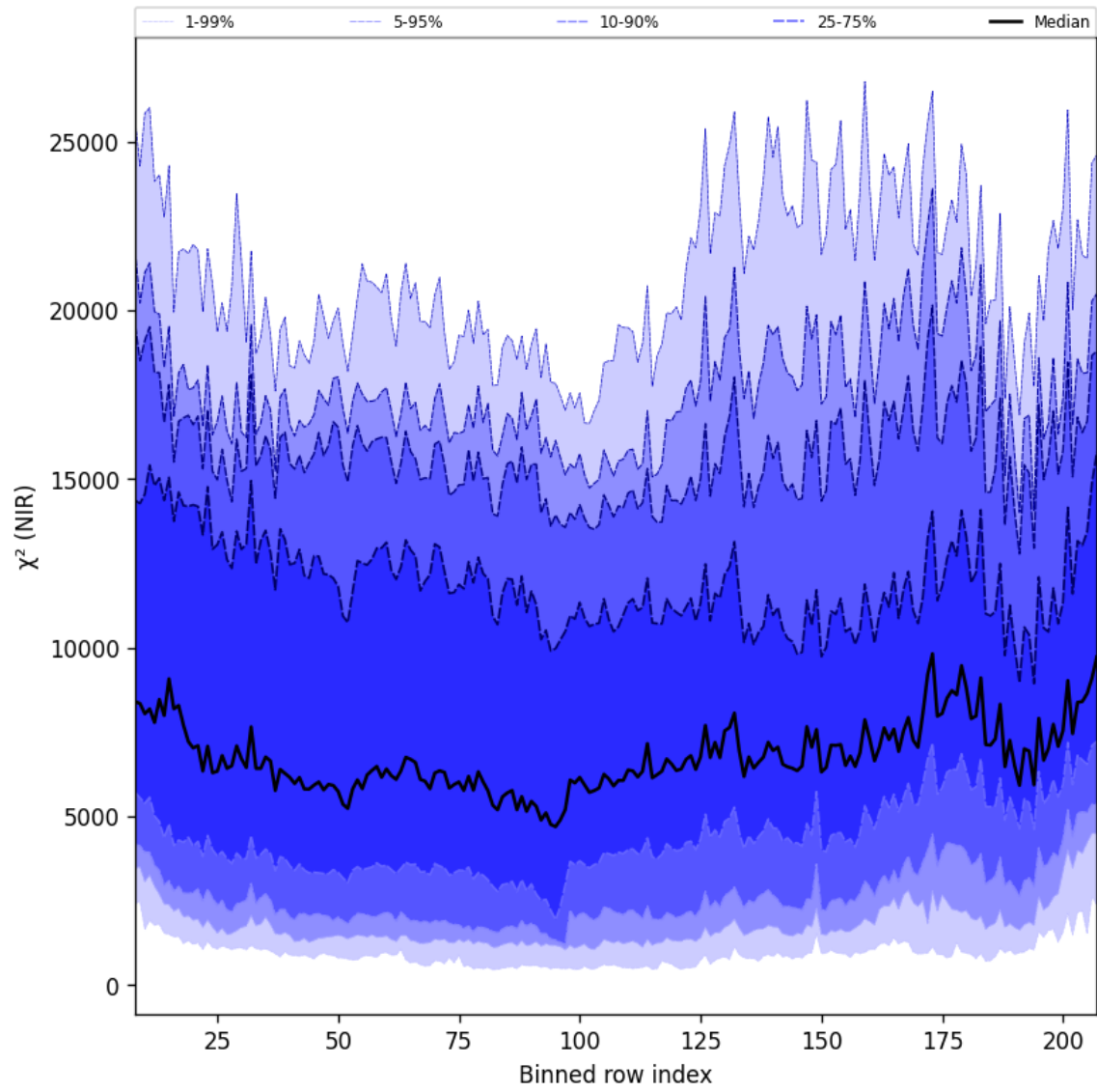
Figure 40: Along track statistics of “ \chi^2 (NIR)” for 2024-10-08 to 2024-10-09
