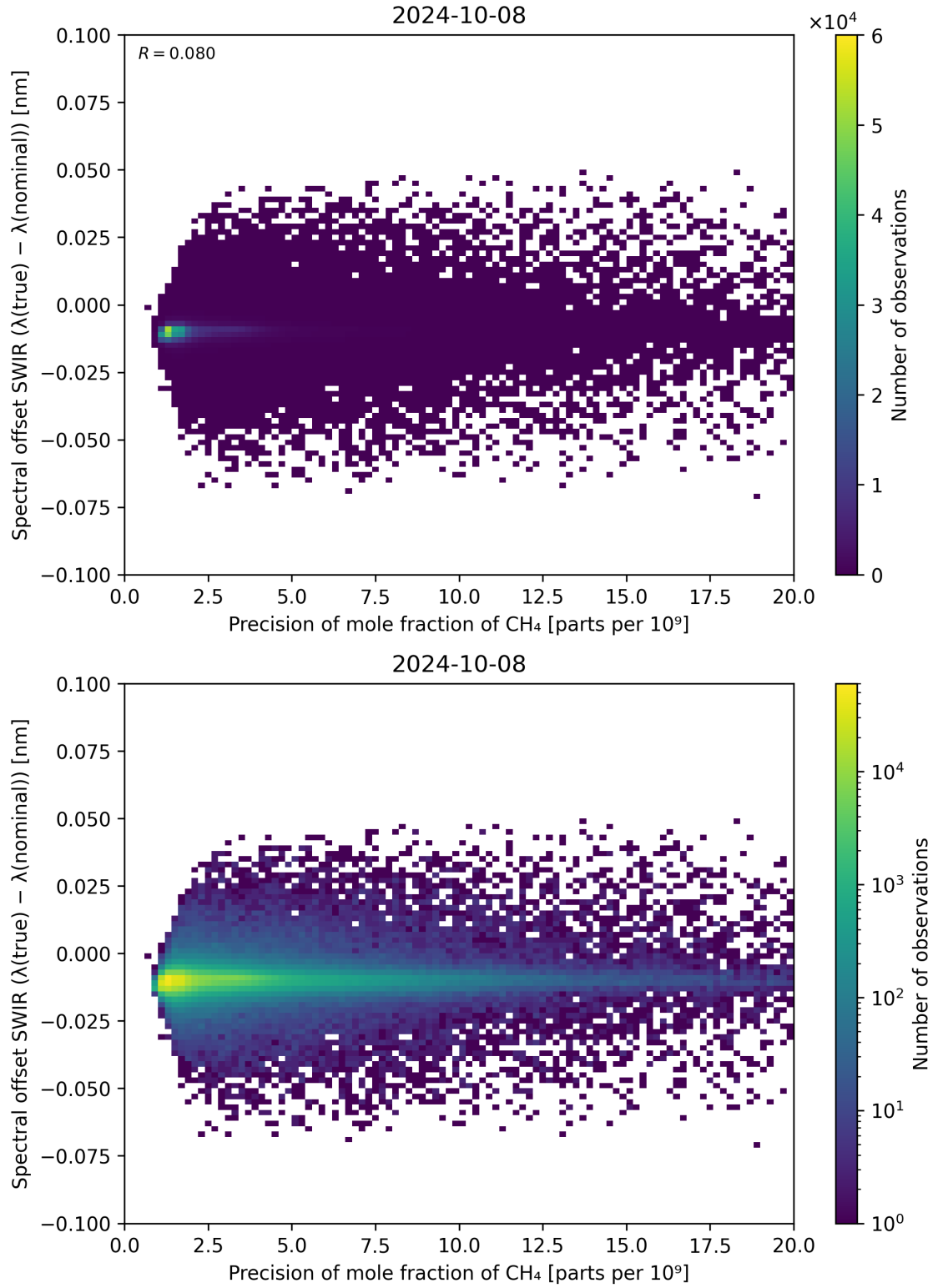
Figure 85: Scatter density plot of “Precision of mole fraction of \text{CH}_4 ” against “Spectral offset SWIR ( \lambda_{\text{true}} - \lambda_{\text{nominal}} )” for 2024-10-08 to 2024-10-09.
