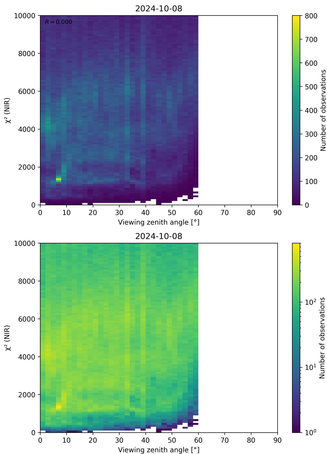
Figure 105: Scatter density plot of “Viewing zenith angle” against “ \chi^2 (NIR)” for 2024-10-08 to 2024-10-09.
