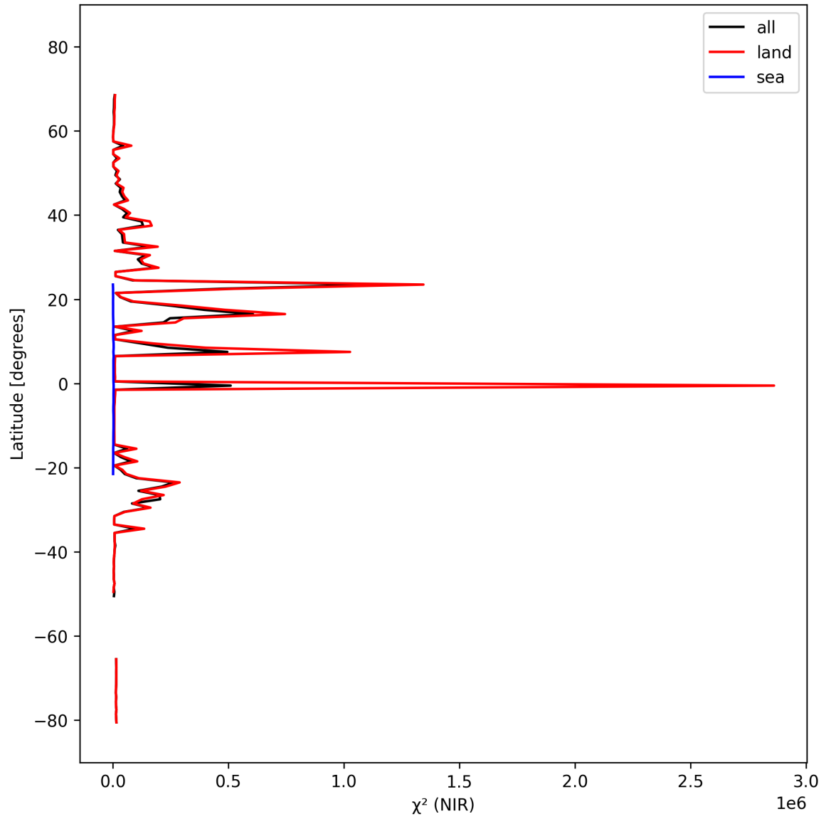
Figure 18: Zonal average of “ \chi^2 (NIR)” for 2024-10-08 to 2024-10-09.
