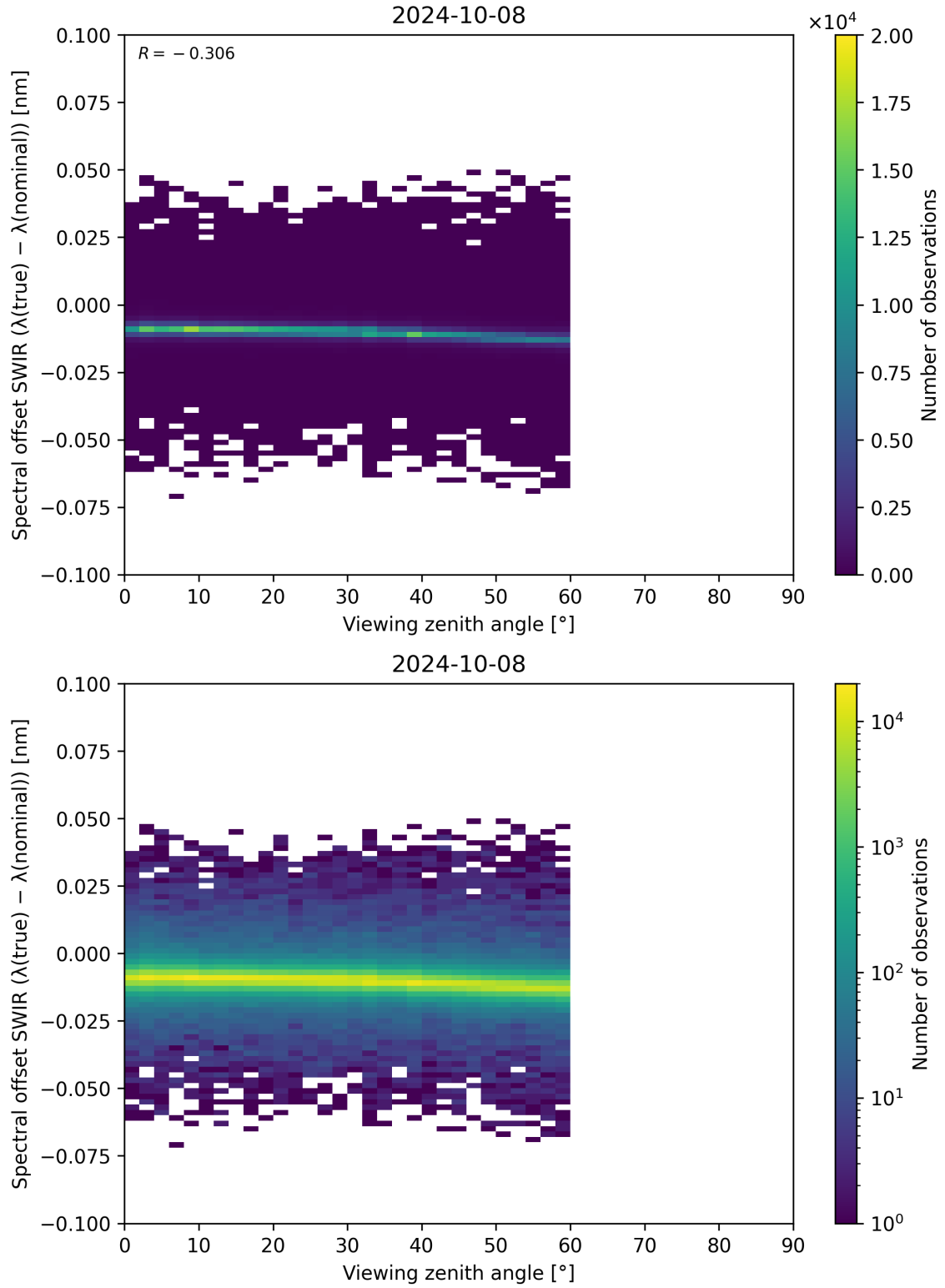
Figure 116: Scatter density plot of “Viewing zenith angle” against “Spectral offset SWIR ( \lambda_{\text{true}} - \lambda_{\text{nominal}} )” for 2024-10-08 to 2024-10-09.
