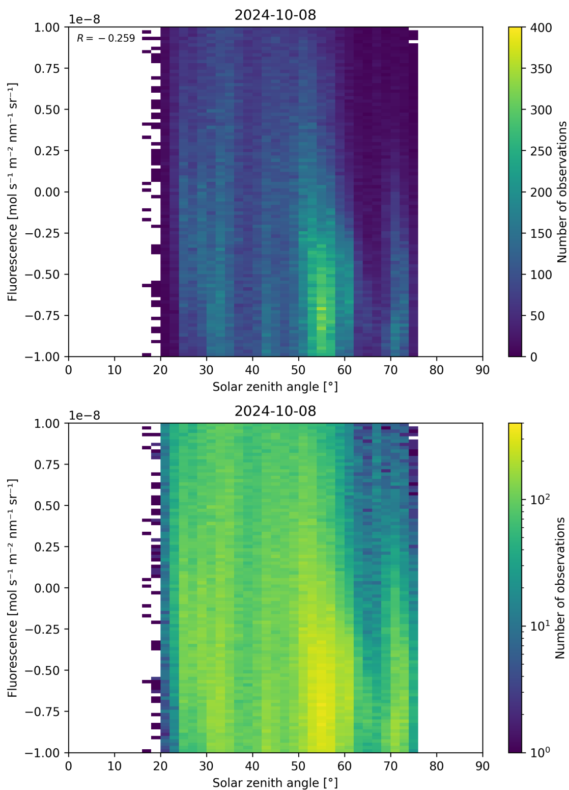
Figure 97: Scatter density plot of “Solar zenith angle” against “Fluorescence” for 2024-10-08 to 2024-10-09.
