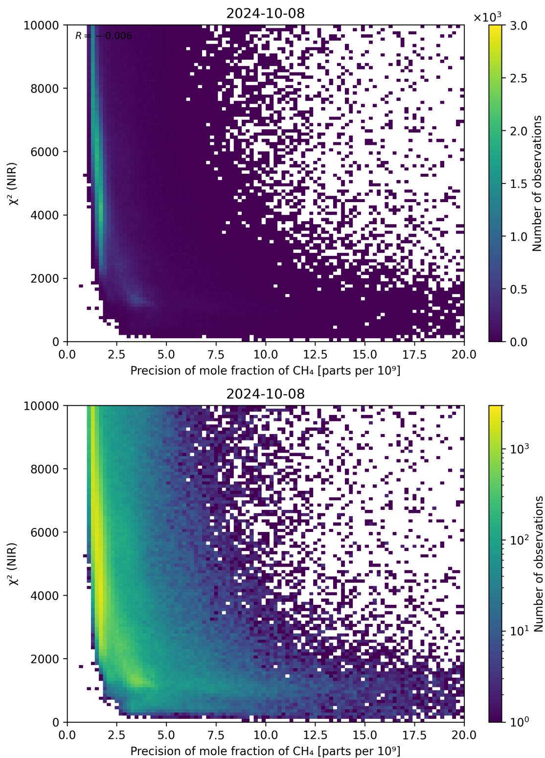
Figure 78: Scatter density plot of “Precision of mole fraction of CH 4 ” against “ \chi^2 (NIR)” for 2024-10-08 to 2024-10-09.
