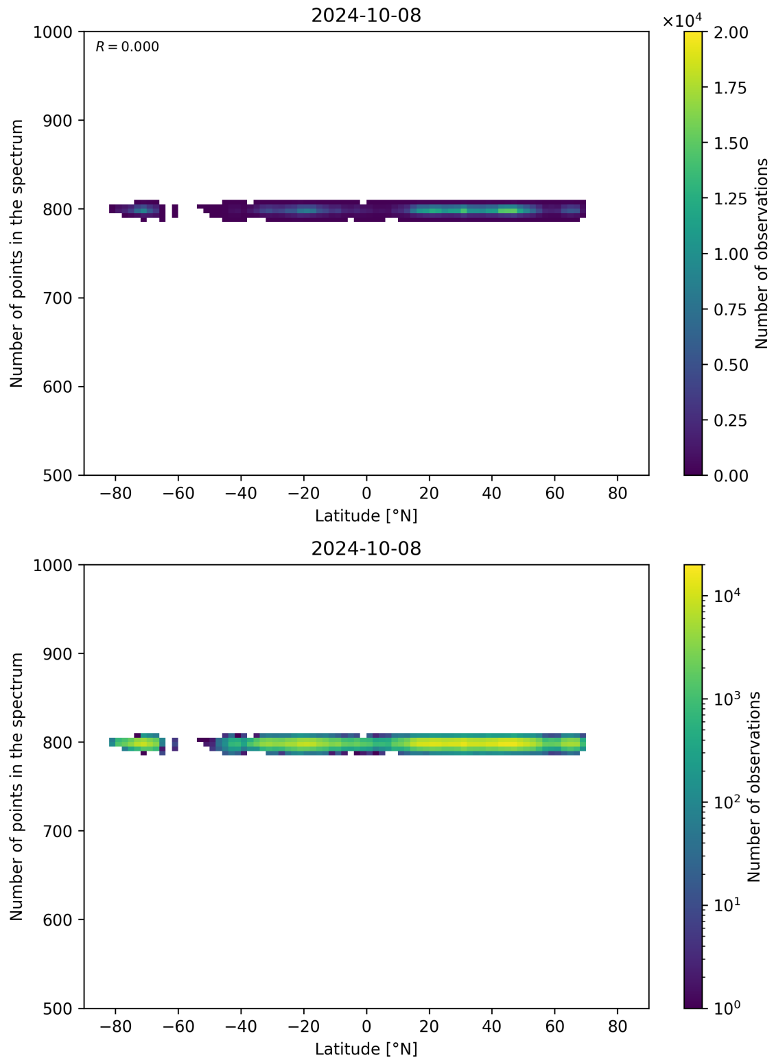
Figure 61: Scatter density plot of “Latitude” against “Number of points in the spectrum” for 2024-10-08 to 2024-10-09.
