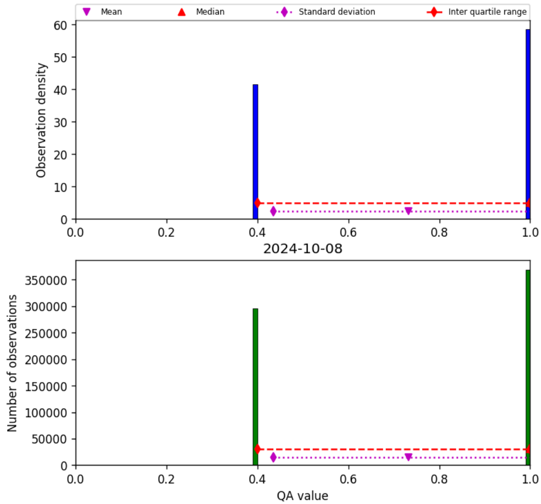
Figure 22: Histogram of “QA value” for 2024-10-08 to 2024-10-09
