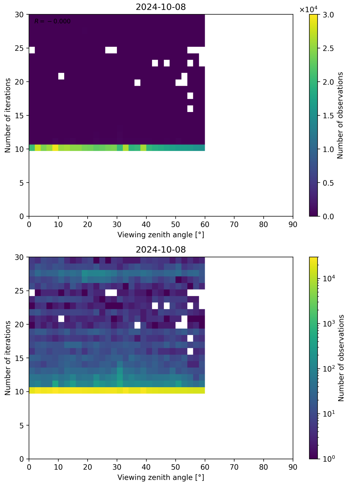
Figure 113: Scatter density plot of “Viewing zenith angle” against “Number of iterations” for 2024-10-08 to 2024-10-09.
