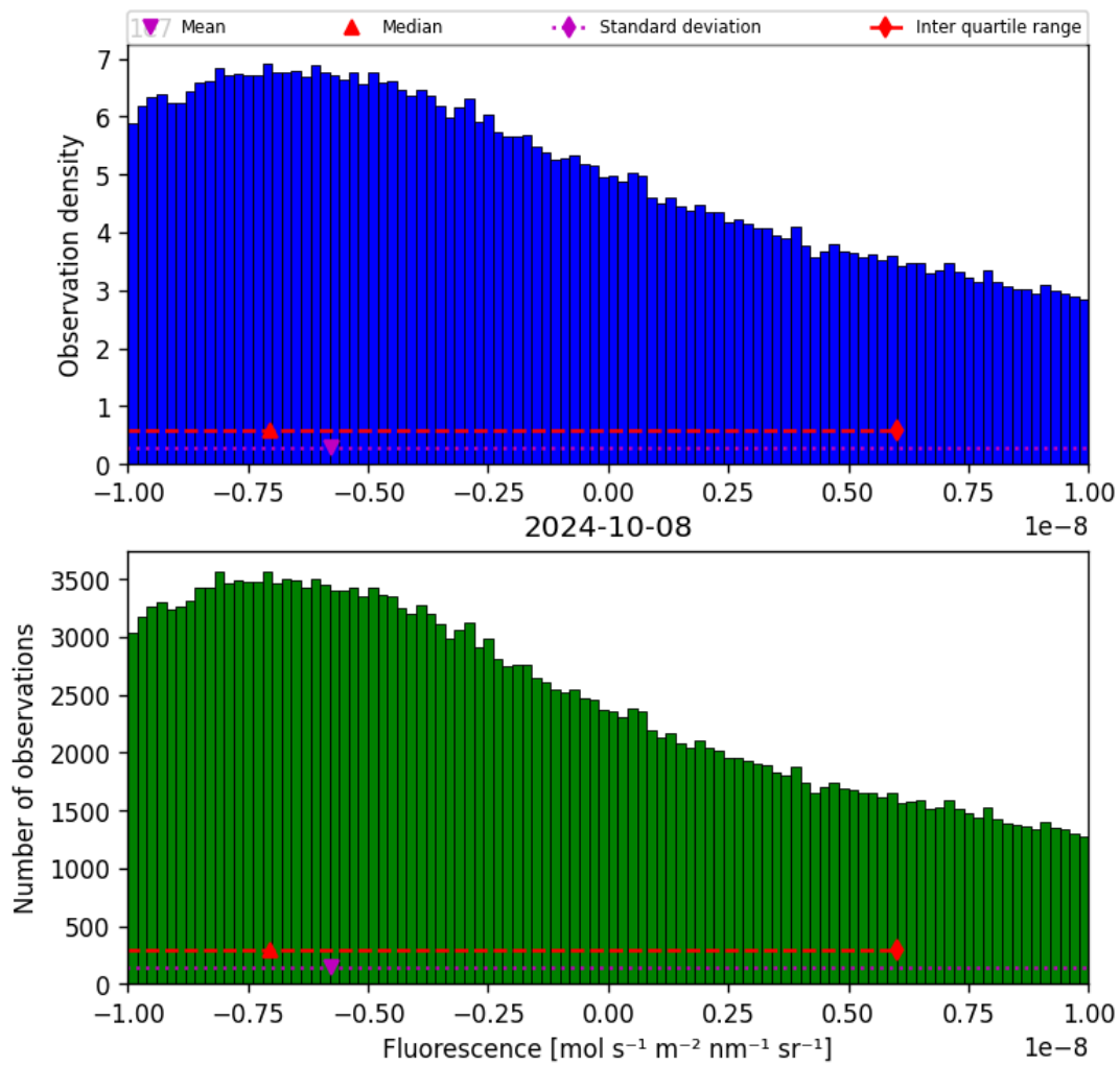
Figure 32: Histogram of “Fluorescence” for 2024-10-08 to 2024-10-09
