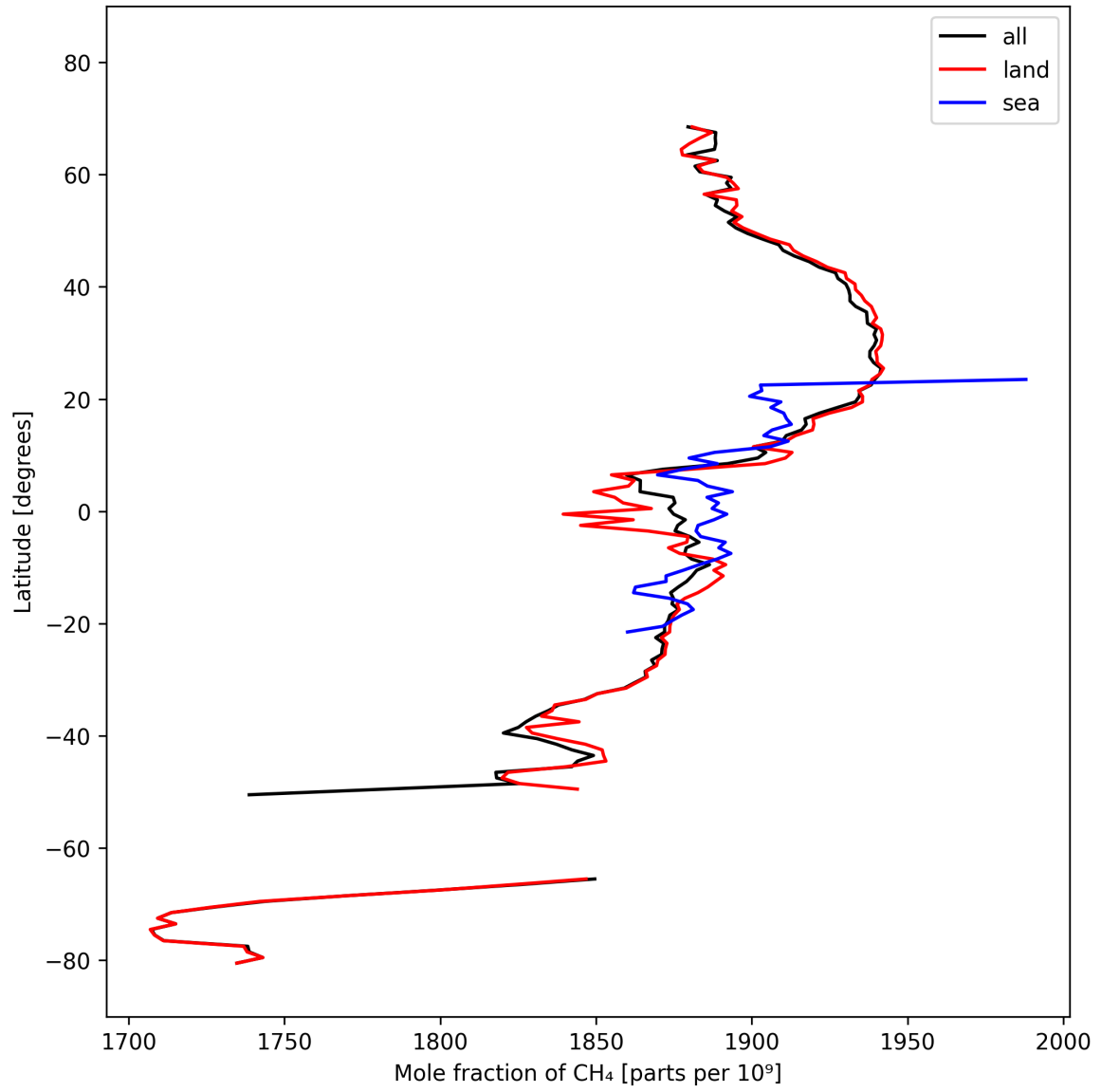
Figure 12: Zonal average of “Mole fraction of CH 4 ” for 2024-10-08 to 2024-10-09.
