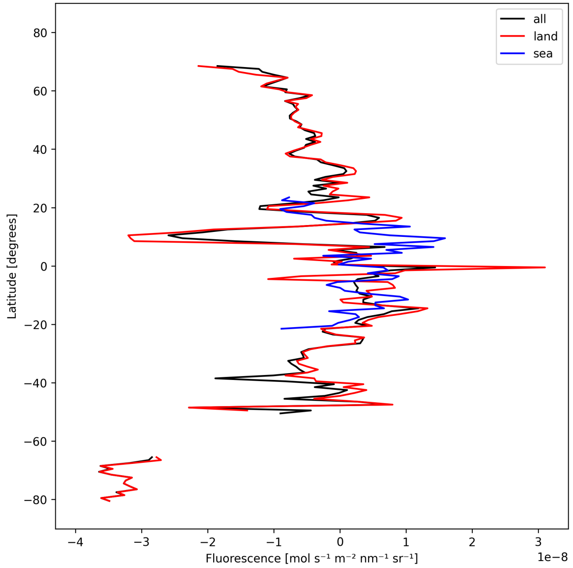
Figure 21: Zonal average of “Fluorescence” for 2024-10-08 to 2024-10-09.
