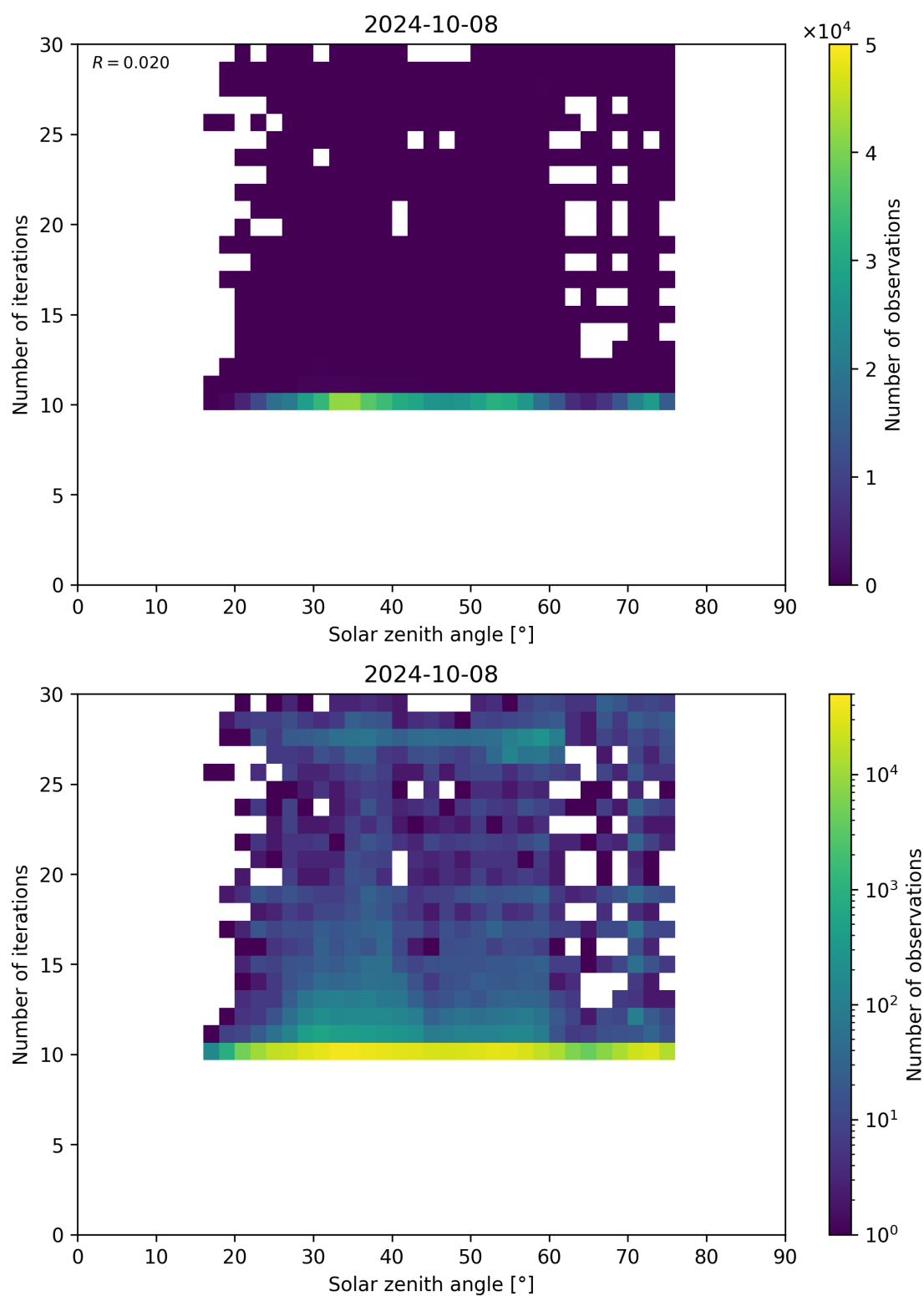
Figure 102: Scatter density plot of “Solar zenith angle” against “Number of iterations” for 2024-10-08 to 2024-10-09.
