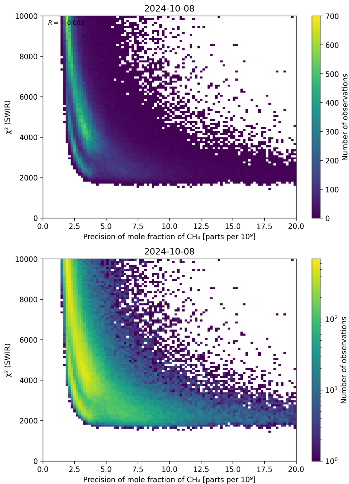
Figure 79: Scatter density plot of “Precision of mole fraction of \text{CH}_4 ” against “ \chi^2 (SWIR)” for 2024-10-08 to 2024-10-09.
