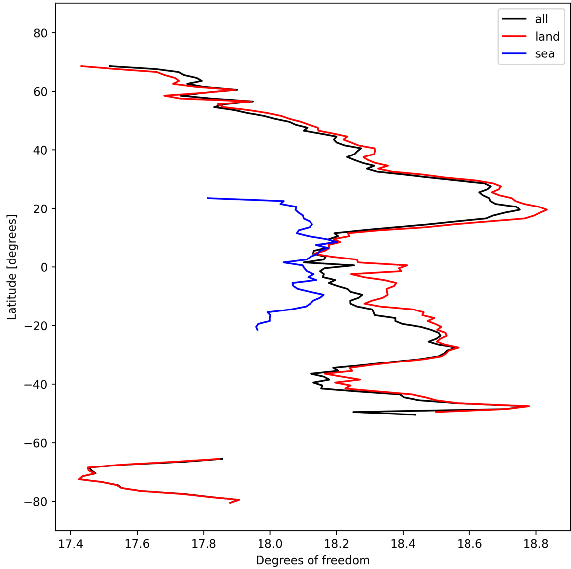
Figure 19: Zonal average of “Degrees of freedom” for 2024-10-08 to 2024-10-09.
