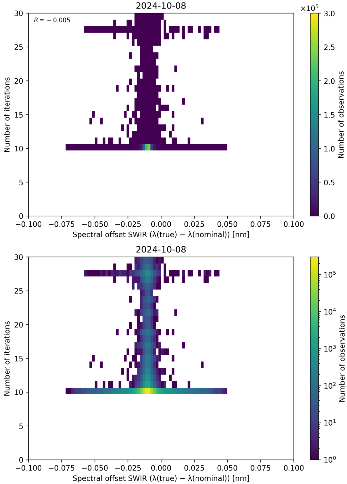
Figure 121: Scatter density plot of “Spectral offset SWIR ( \lambda_{\text{true}} - \lambda_{\text{nominal}} )” against “Number of iterations” for 2024-10-08 to 2024-10-09.
