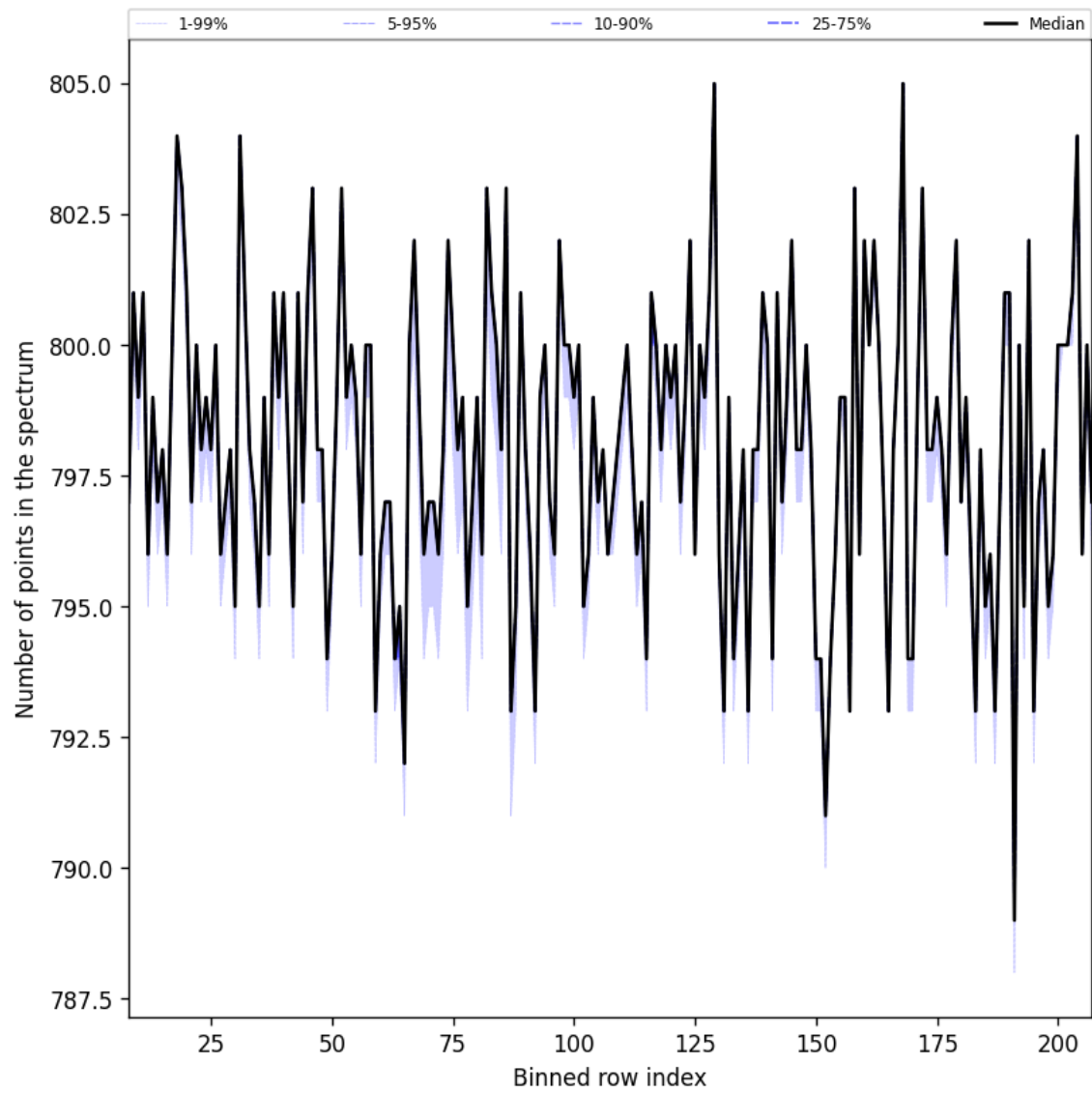
Figure 37: Along track statistics of “Number of points in the spectrum” for 2024-10-08 to 2024-10-09
