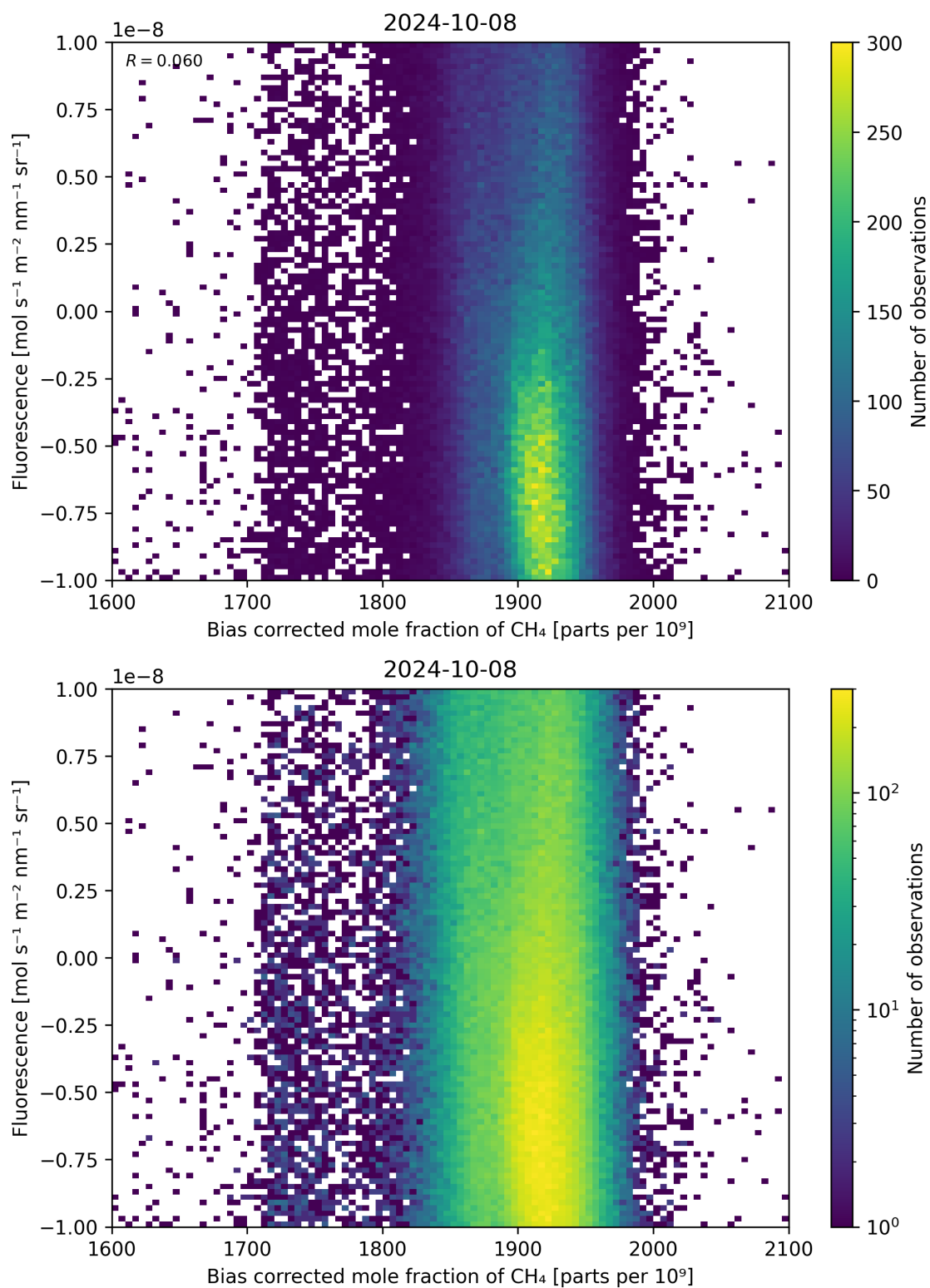
Figure 66: Scatter density plot of “Bias corrected mole fraction of \text{CH}_4 ” against “Fluorescence” for 2024-10-08 to 2024-10-09.
