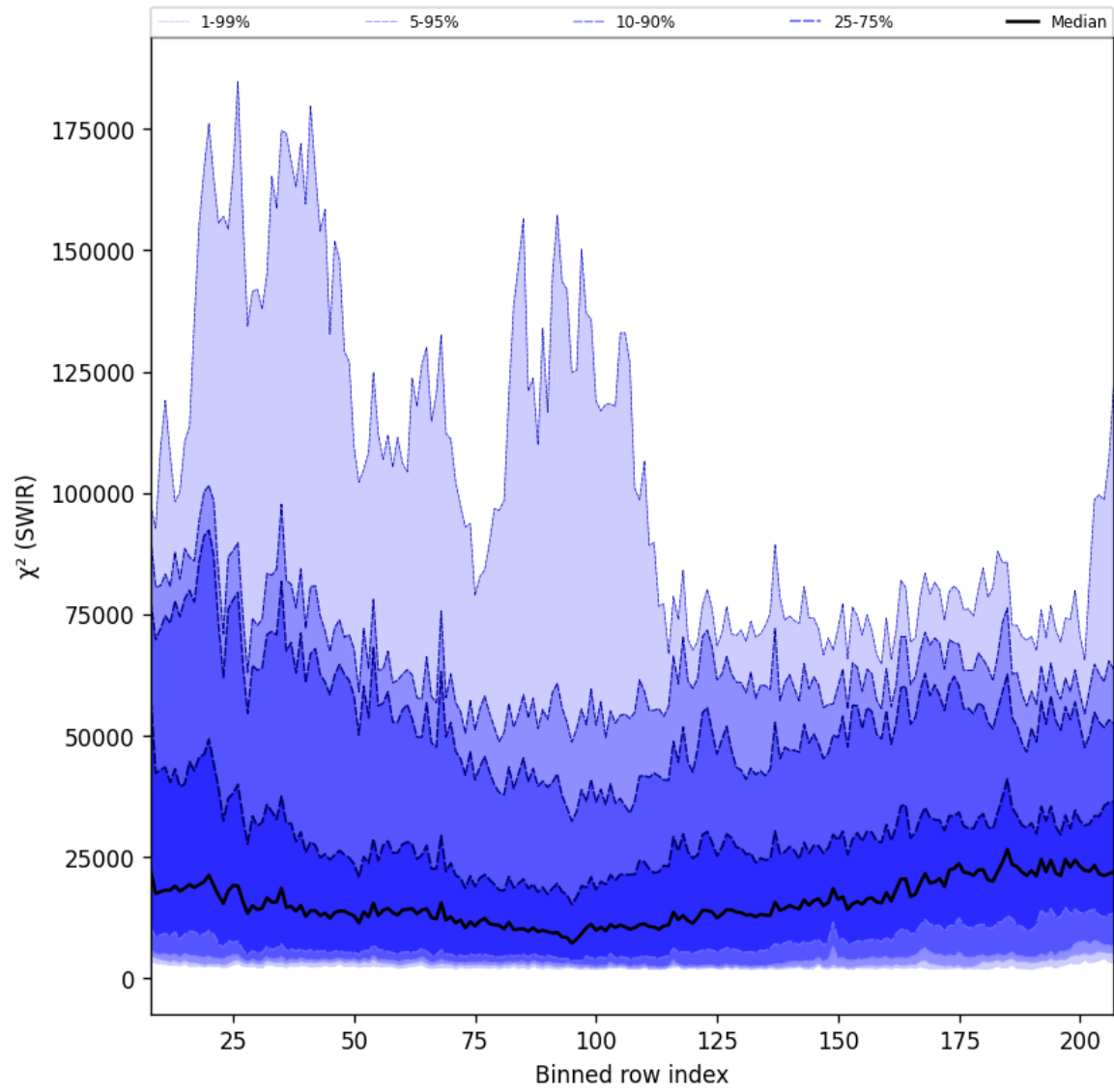
Figure 39: Along track statistics of " \chi^2 (SWIR)" for 2024-10-08 to 2024-10-09
