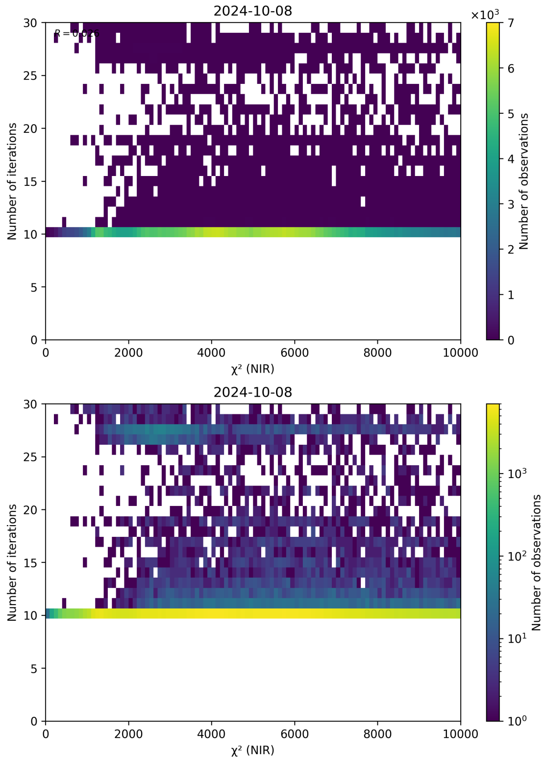
Figure 46: Scatter density plot of “ \chi^2 (NIR)” against “Number of iterations” for 2024-10-08 to 2024-10-09.
