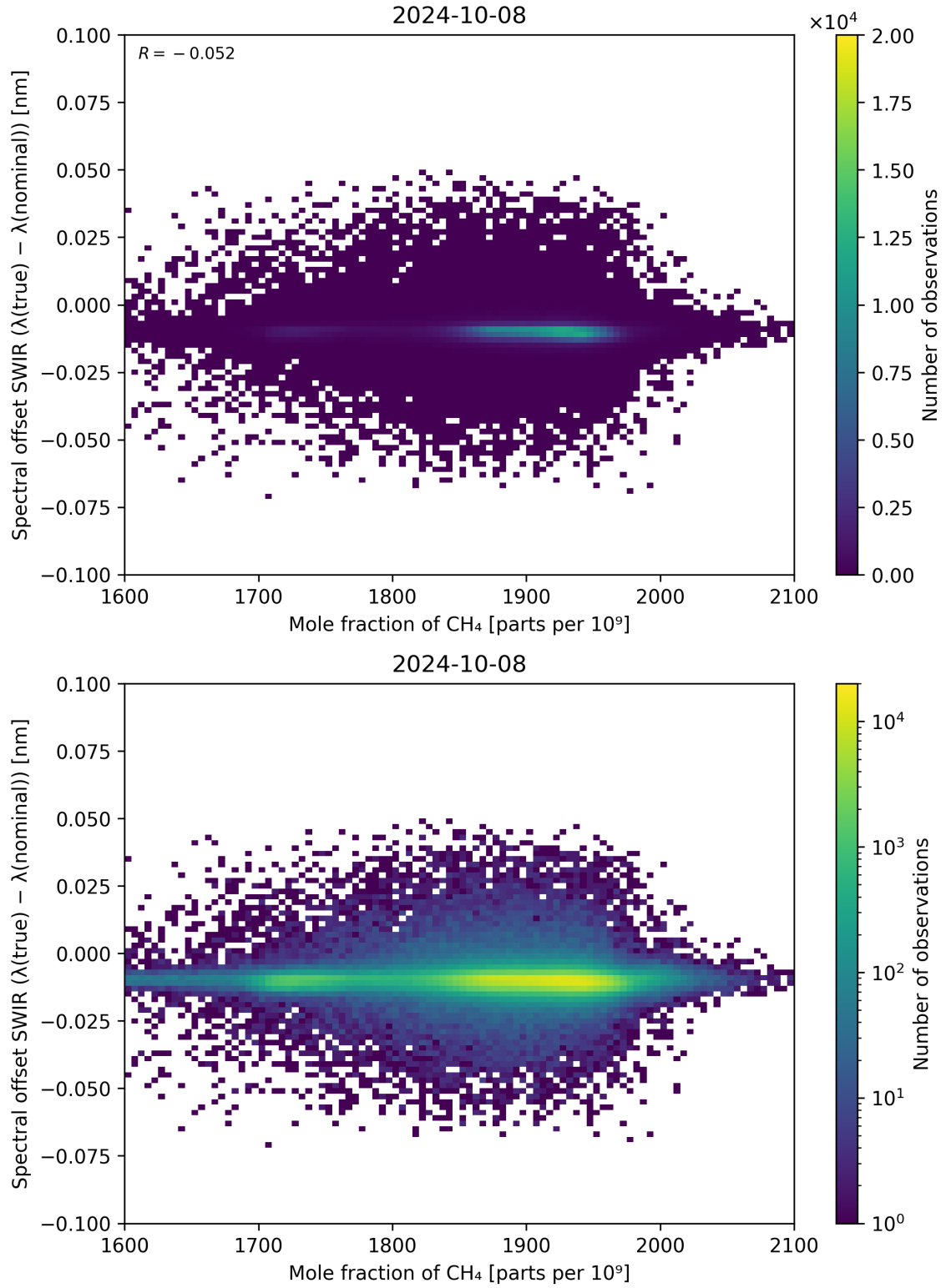
Figure 86: Scatter density plot of “Mole fraction of \text{CH}_4 ” against “Spectral offset SWIR ( \lambda_{\text{true}} - \lambda_{\text{nominal}} )” for 2024-10-08 to 2024-10-09.
