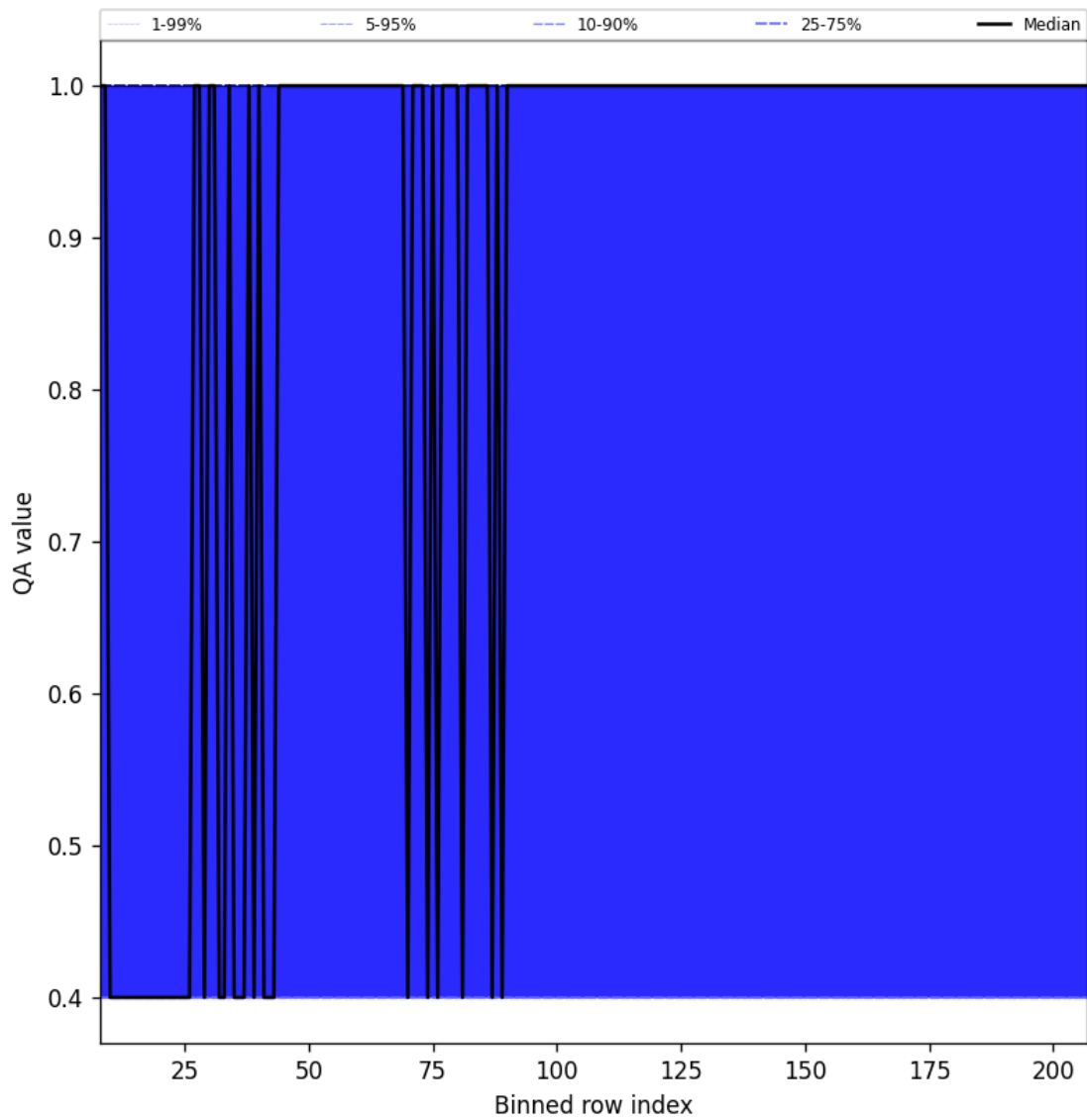
Figure 33: Along track statistics of “QA value” for 2024-10-08 to 2024-10-09
