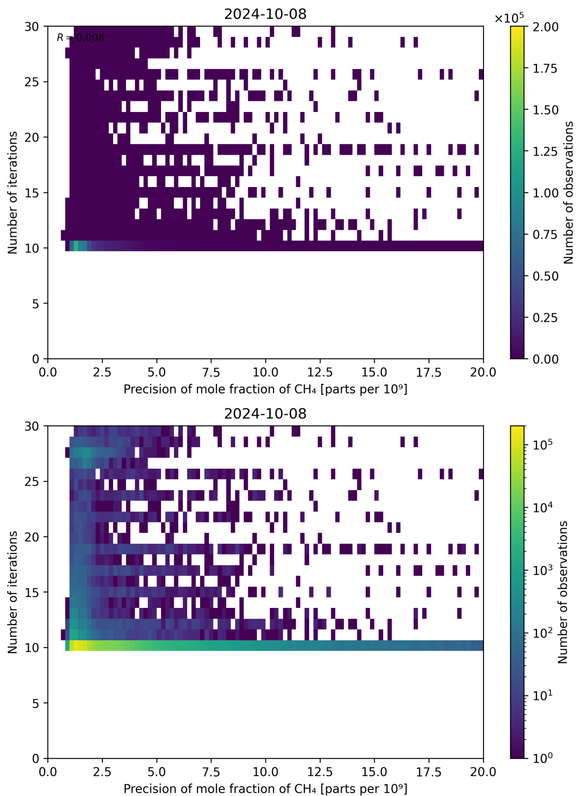
Figure 83: Scatter density plot of “Precision of mole fraction of CH 4 ” against “Number of iterations” for 2024-10-08 to 2024-10-09.
