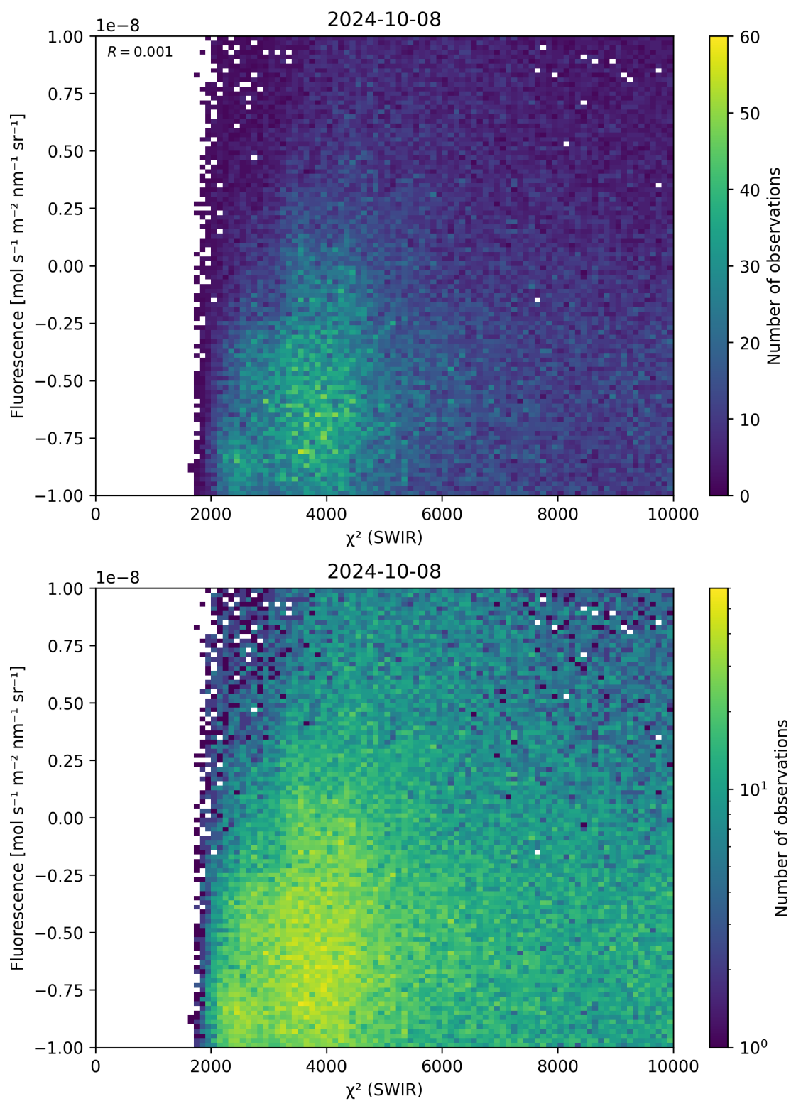
Figure 49: Scatter density plot of “ \chi^2 (SWIR)” against “Fluorescence” for 2024-10-08 to 2024-10-09.
