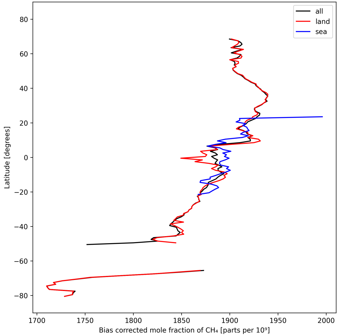
Figure 14: Zonal average of “Bias corrected mole fraction of CH 4 ” for 2024-10-08 to 2024-10-09.
