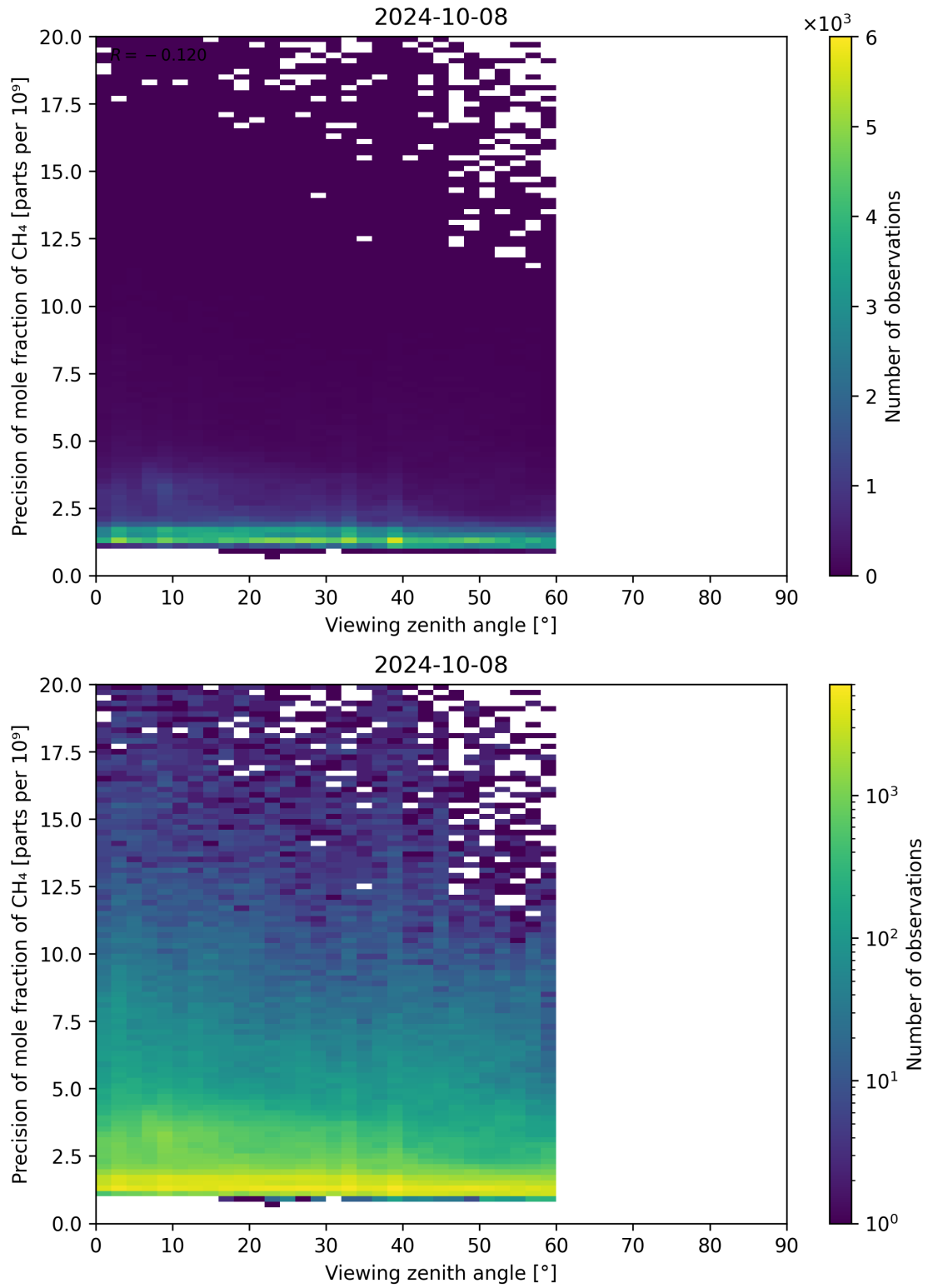
Figure 112: Scatter density plot of “Viewing zenith angle” against “Precision of mole fraction of \text{CH}_4 ” for 2024-10-08 to 2024-10-09.
