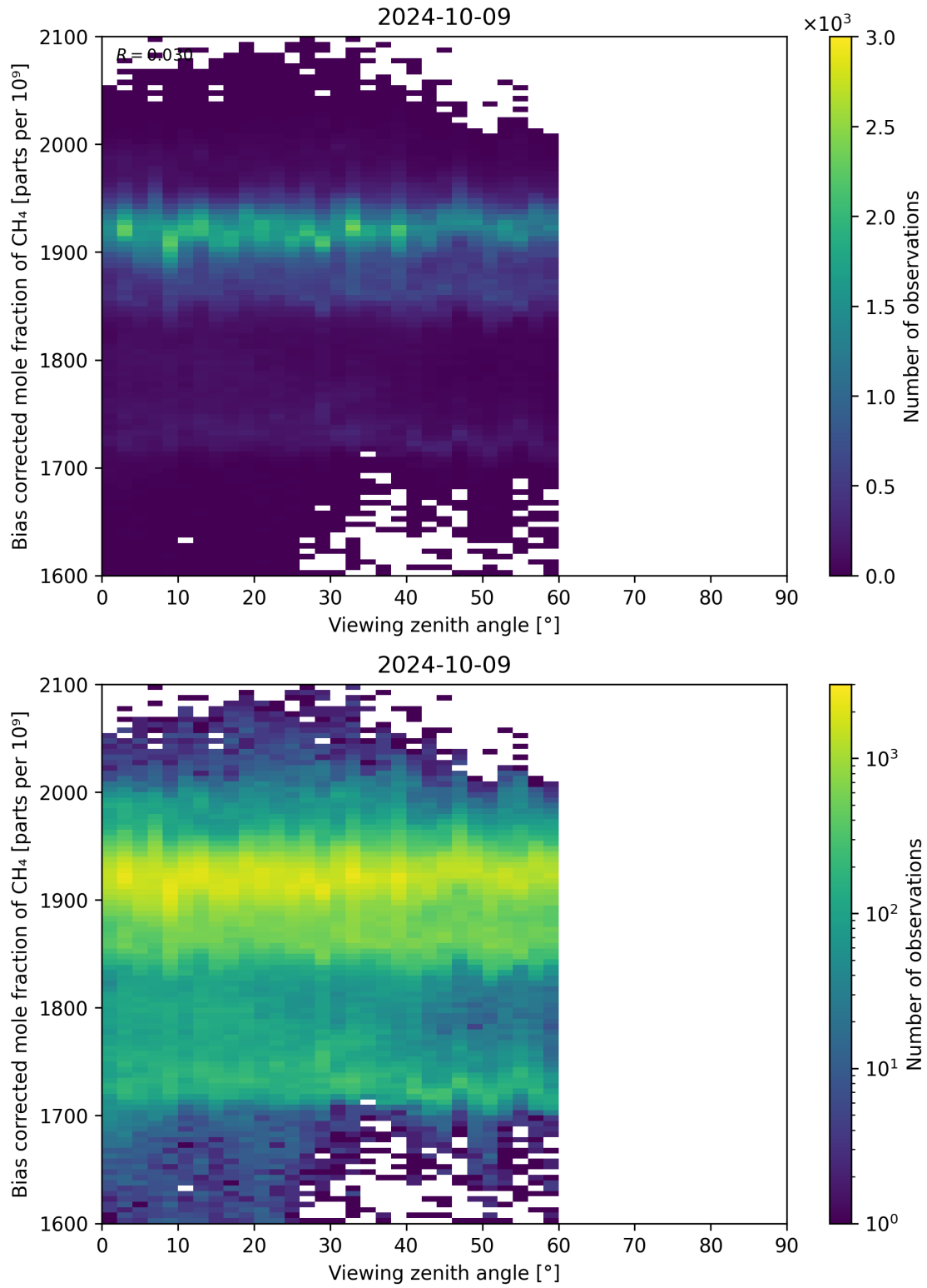
Figure 111: Scatter density plot of “Viewing zenith angle” against “Bias corrected mole fraction of CH 4 ” for 2024-10-08 to 2024-10-10.
