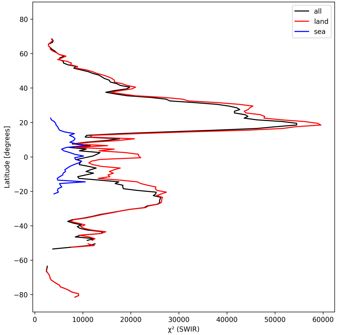
Figure 17: Zonal average of “ \chi^2 (SWIR)” for 2024-10-08 to 2024-10-10.
