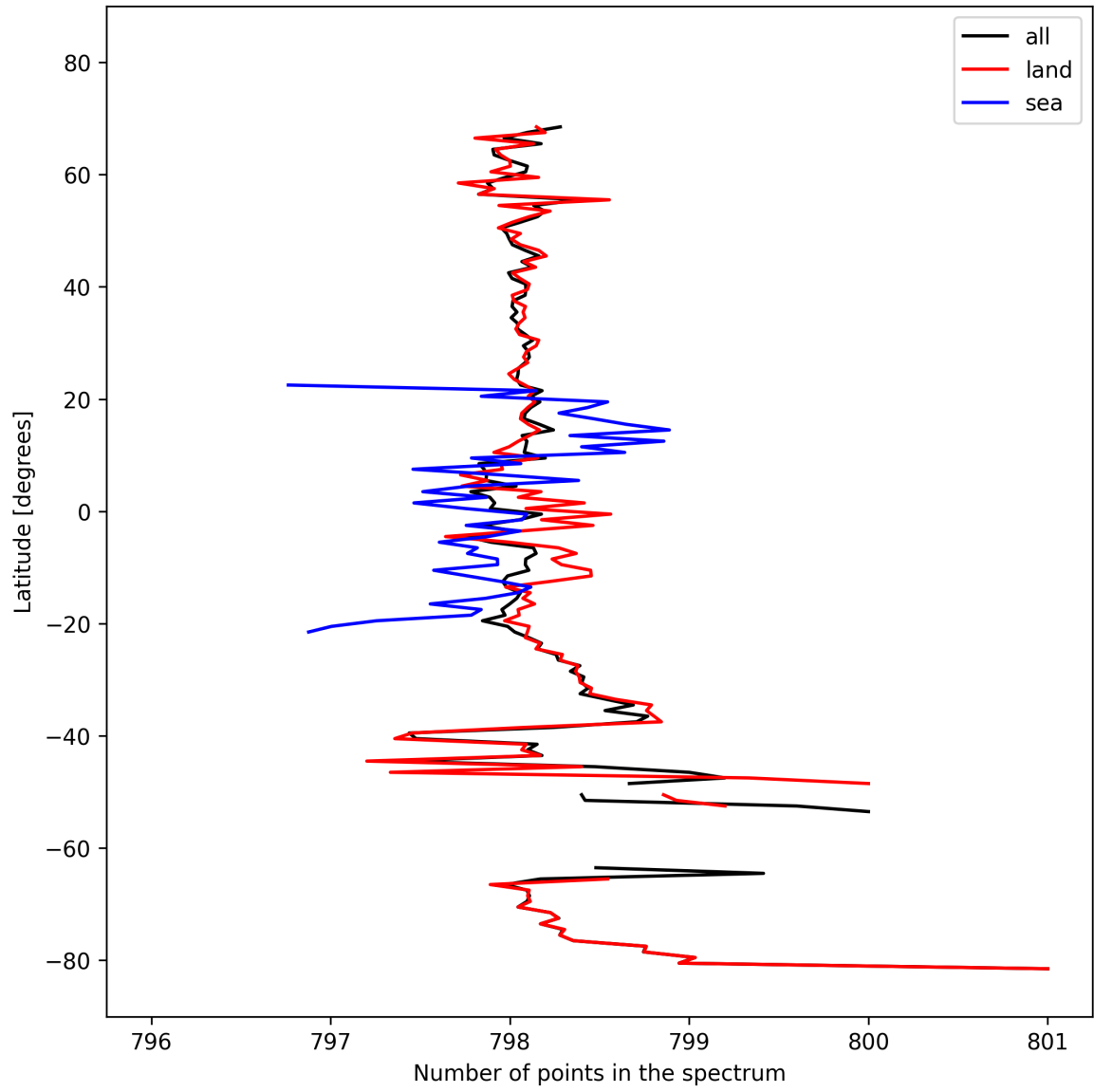
Figure 15: Zonal average of “Number of points in the spectrum” for 2024-10-08 to 2024-10-10.
