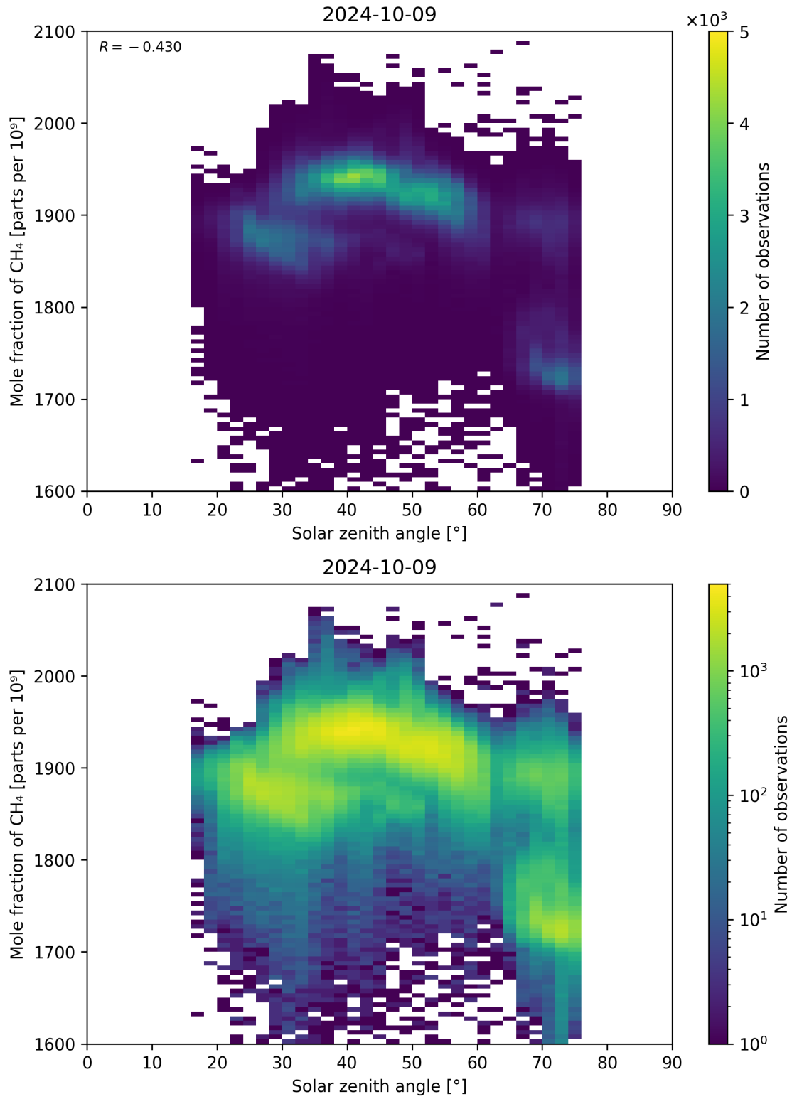
Figure 99: Scatter density plot of “Solar zenith angle” against “Mole fraction of \text{CH}_4 ” for 2024-10-08 to 2024-10-10.
