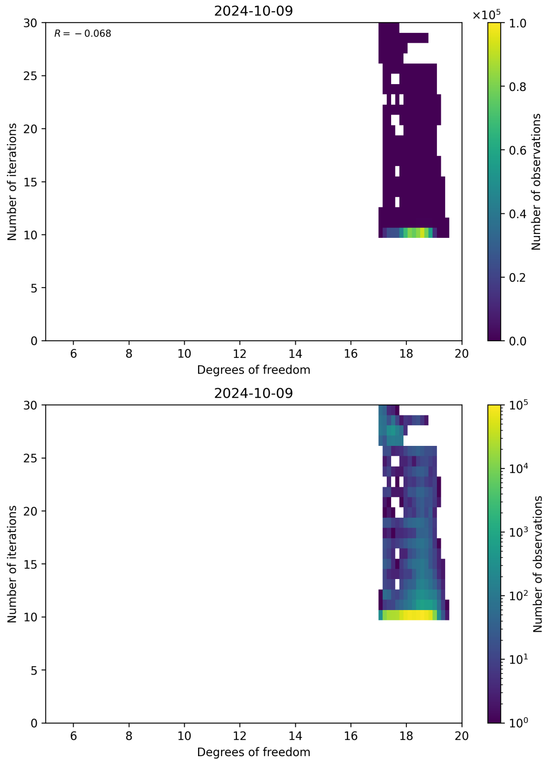
Figure 52: Scatter density plot of “Degrees of freedom” against “Number of iterations” for 2024-10-08 to 2024-10-10.
