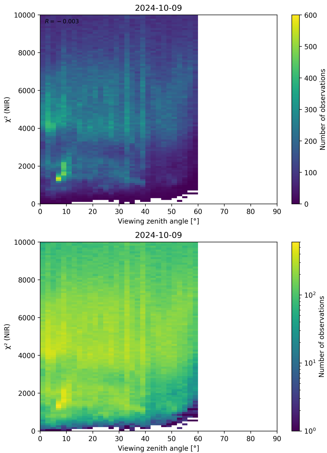
Figure 105: Scatter density plot of “Viewing zenith angle” against “ \chi^2 (NIR)” for 2024-10-08 to 2024-10-10.
