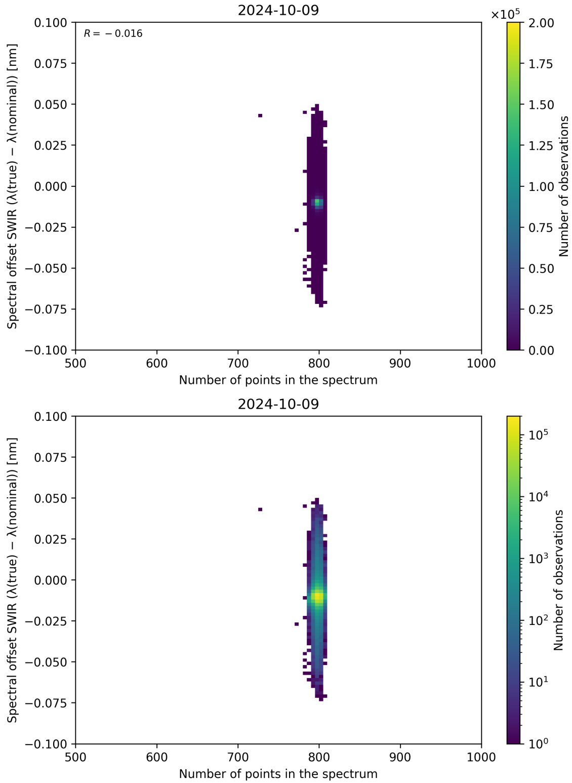
Figure 93: Scatter density plot of “Number of points in the spectrum” against “Spectral offset SWIR ( \lambda_{\text{true}} - \lambda_{\text{nominal}} )” for 2024-10-08 to 2024-10-10.
