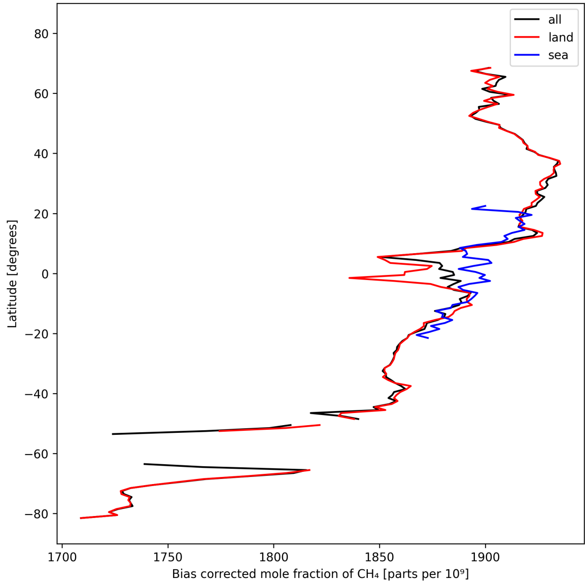
Figure 14: Zonal average of “Bias corrected mole fraction of CH 4 ” for 2024-10-08 to 2024-10-10.
