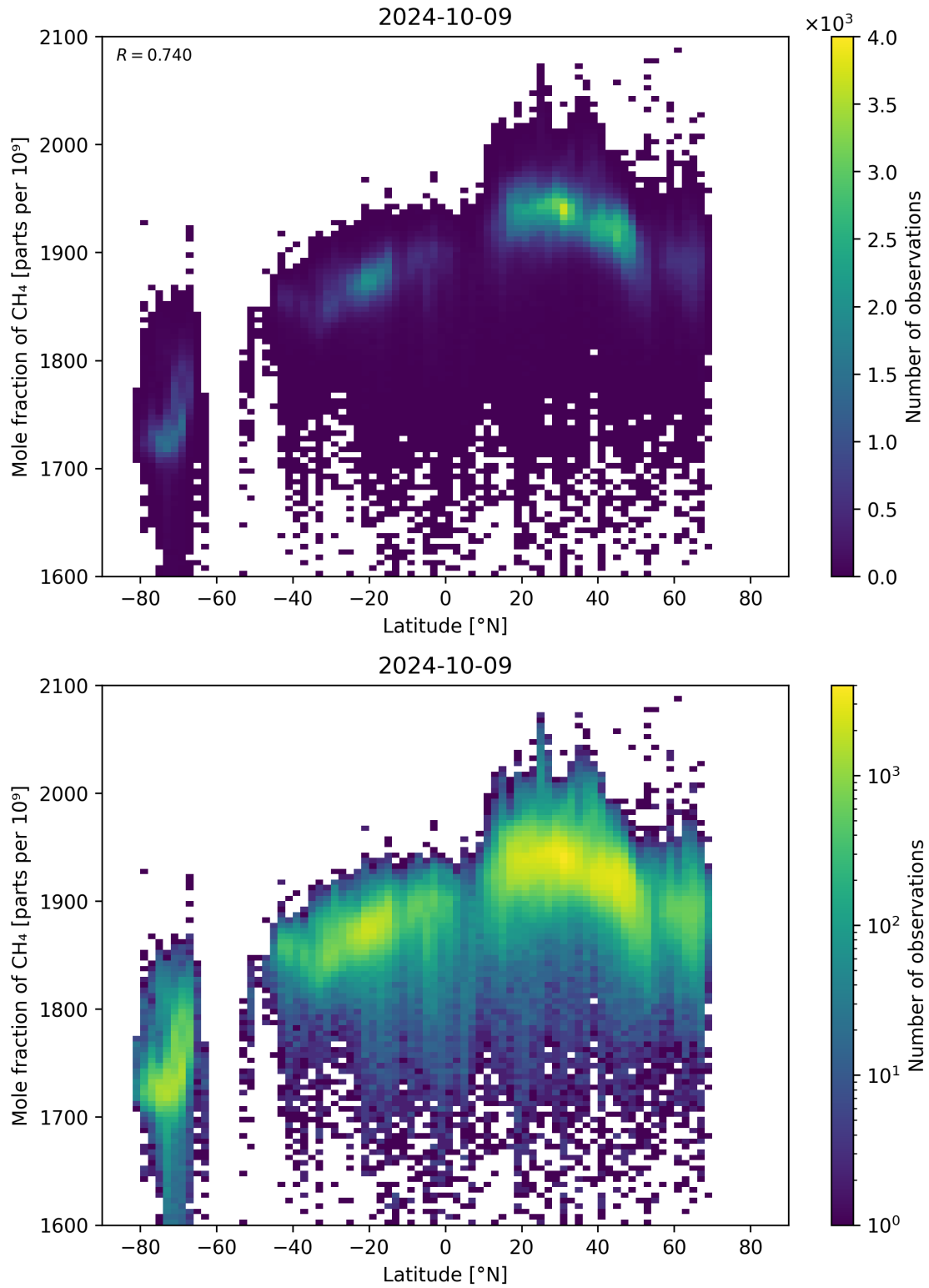
Figure 57: Scatter density plot of “Latitude” against “Mole fraction of CH 4 ” for 2024-10-08 to 2024-10-10.
