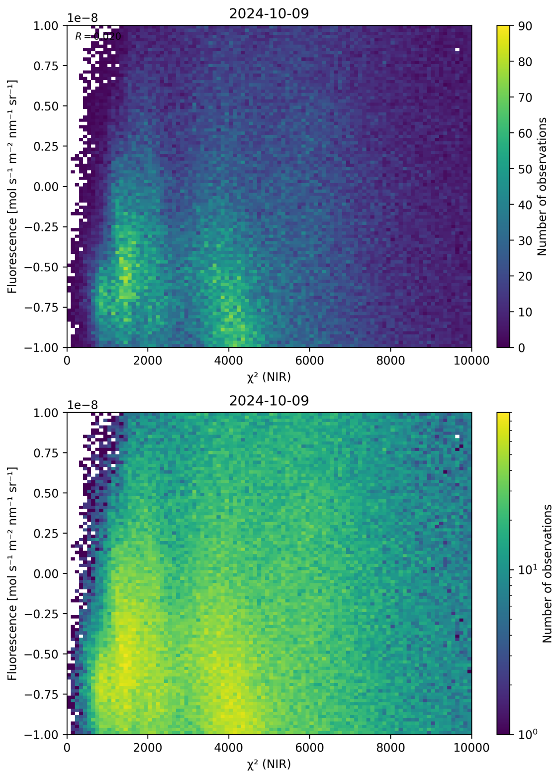
Figure 45: Scatter density plot of “ \chi^2 (NIR)” against “Fluorescence” for 2024-10-08 to 2024-10-10.
