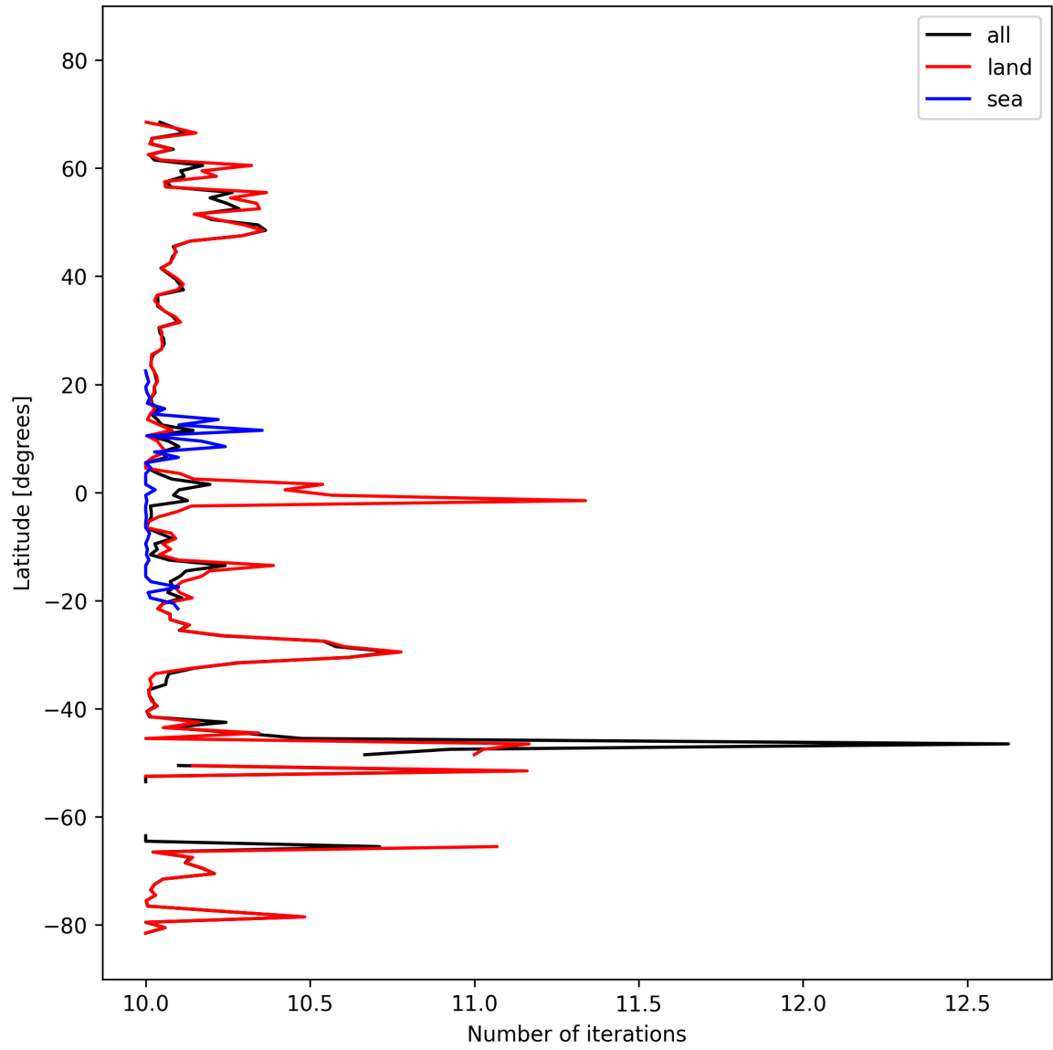
Figure 20: Zonal average of “Number of iterations” for 2024-10-08 to 2024-10-10.
