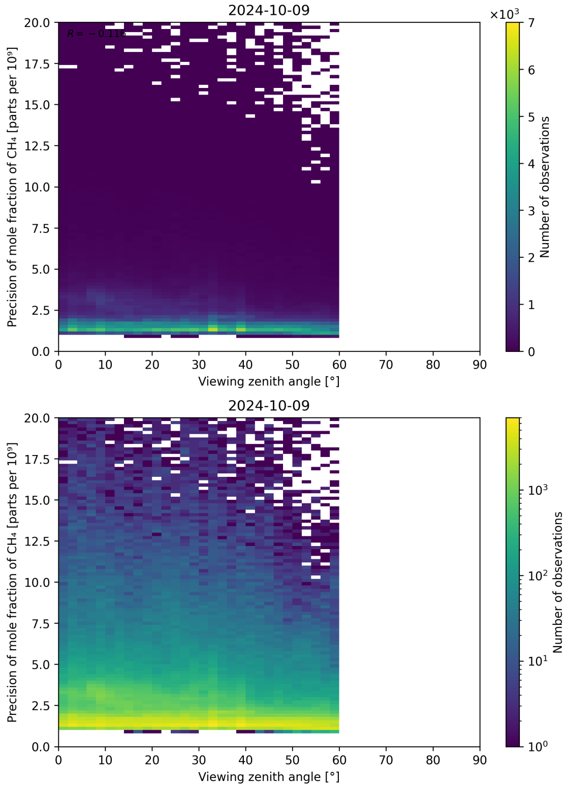
Figure 112: Scatter density plot of “Viewing zenith angle” against “Precision of mole fraction of CH 4 ” for 2024-10-08 to 2024-10-10.
