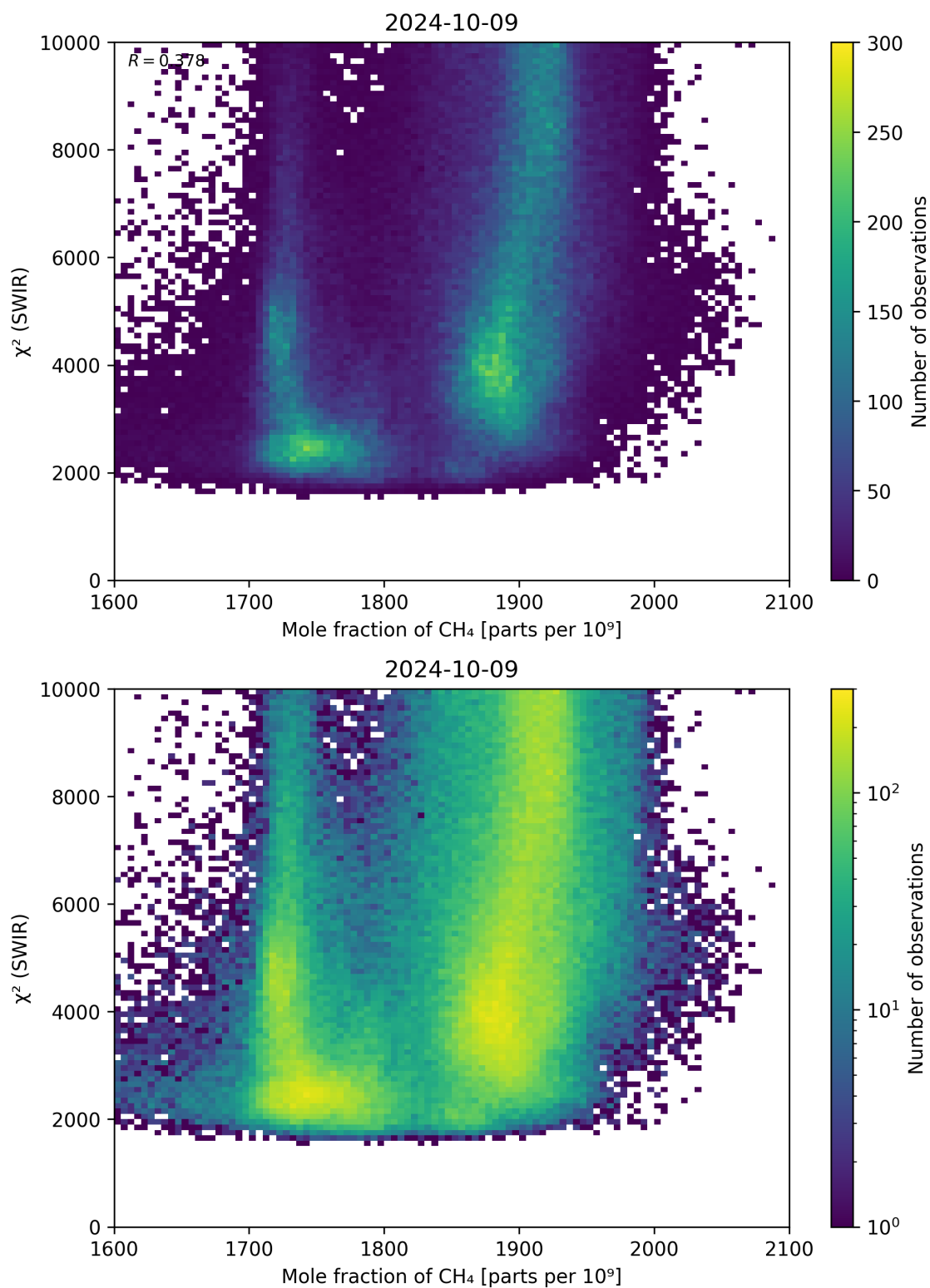
Figure 71: Scatter density plot of “Mole fraction of \text{CH}_4 ” against “ \chi^2 (SWIR)” for 2024-10-08 to 2024-10-10.
