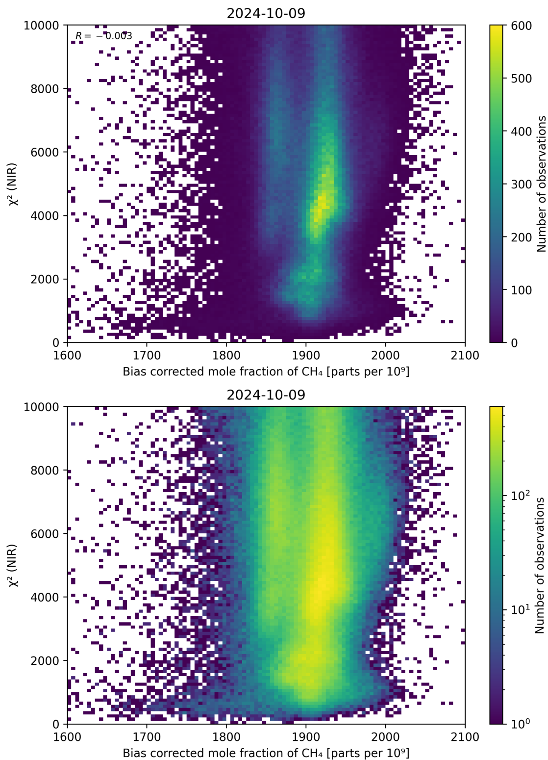
Figure 63: Scatter density plot of “Bias corrected mole fraction of CH 4 ” against “ \chi^2 (NIR)” for 2024-10-08 to 2024-10-10.
