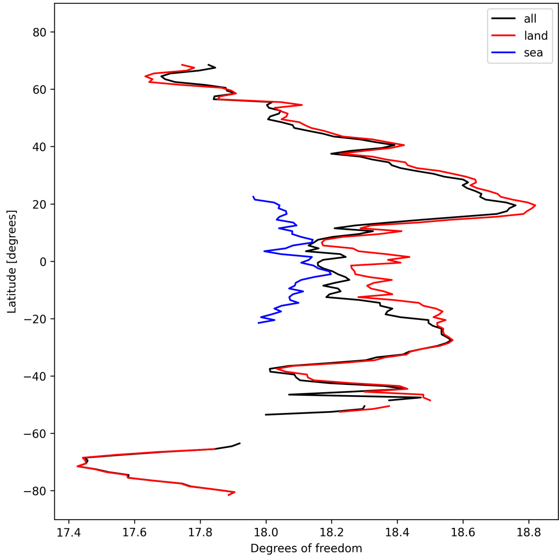
Figure 19: Zonal average of “Degrees of freedom” for 2024-10-08 to 2024-10-10.
