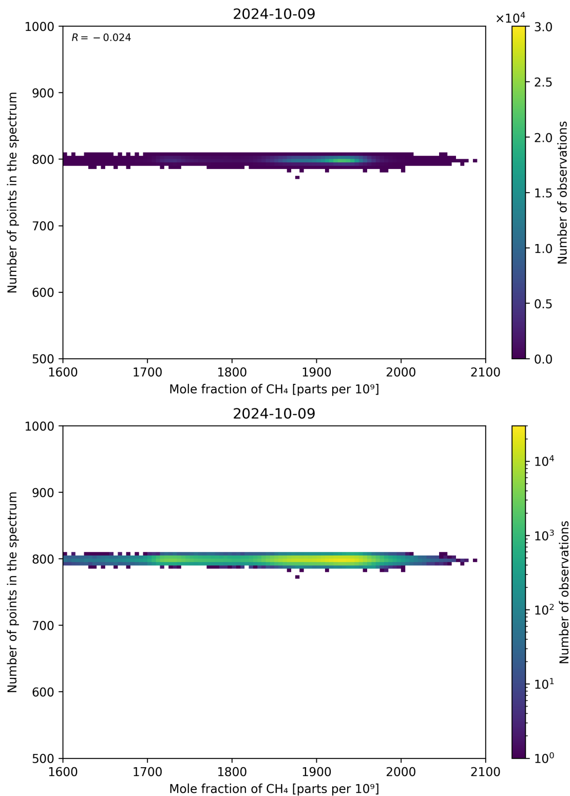
Figure 77: Scatter density plot of “Mole fraction of CH 4 ” against “Number of points in the spectrum” for 2024-10-08 to 2024-10-10.
