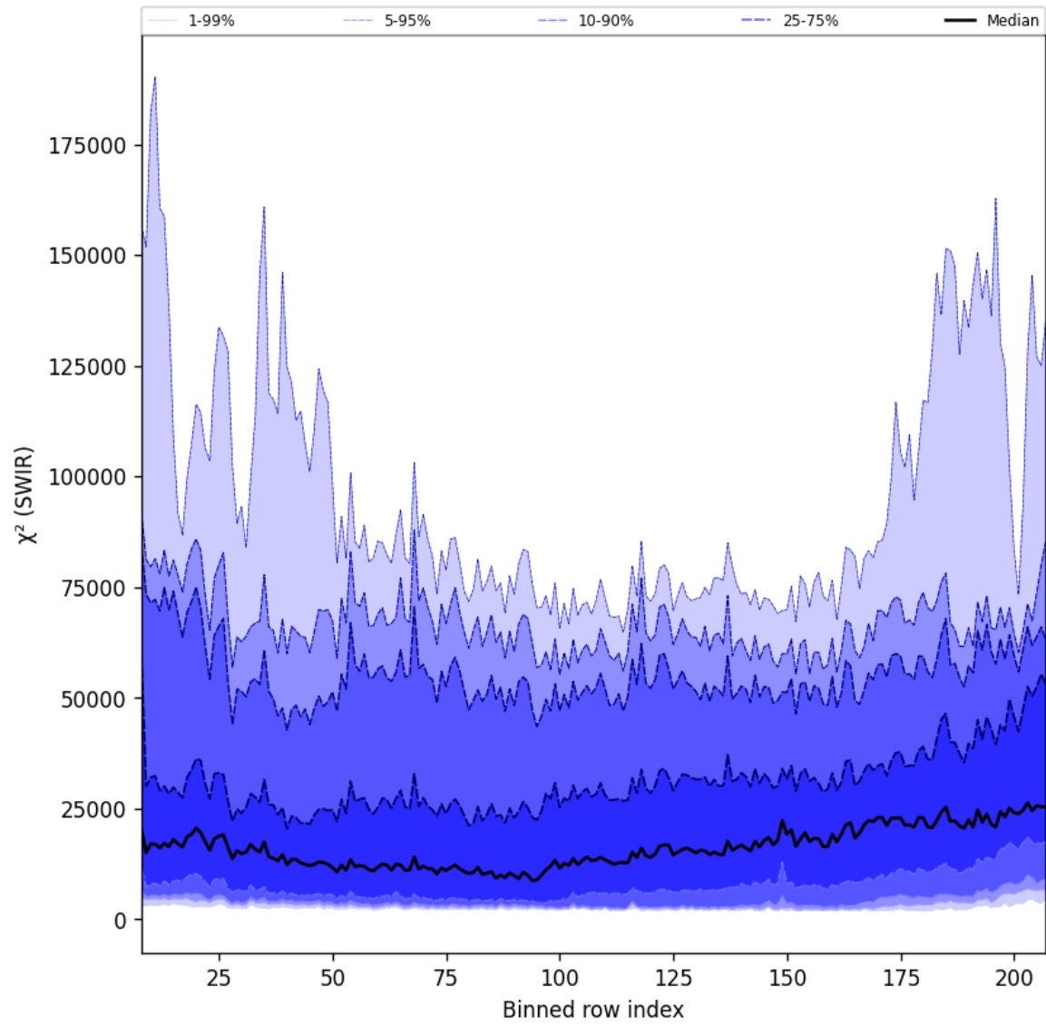
Figure 39: Along track statistics of “ \chi^2 (SWIR)” for 2024-10-08 to 2024-10-10
