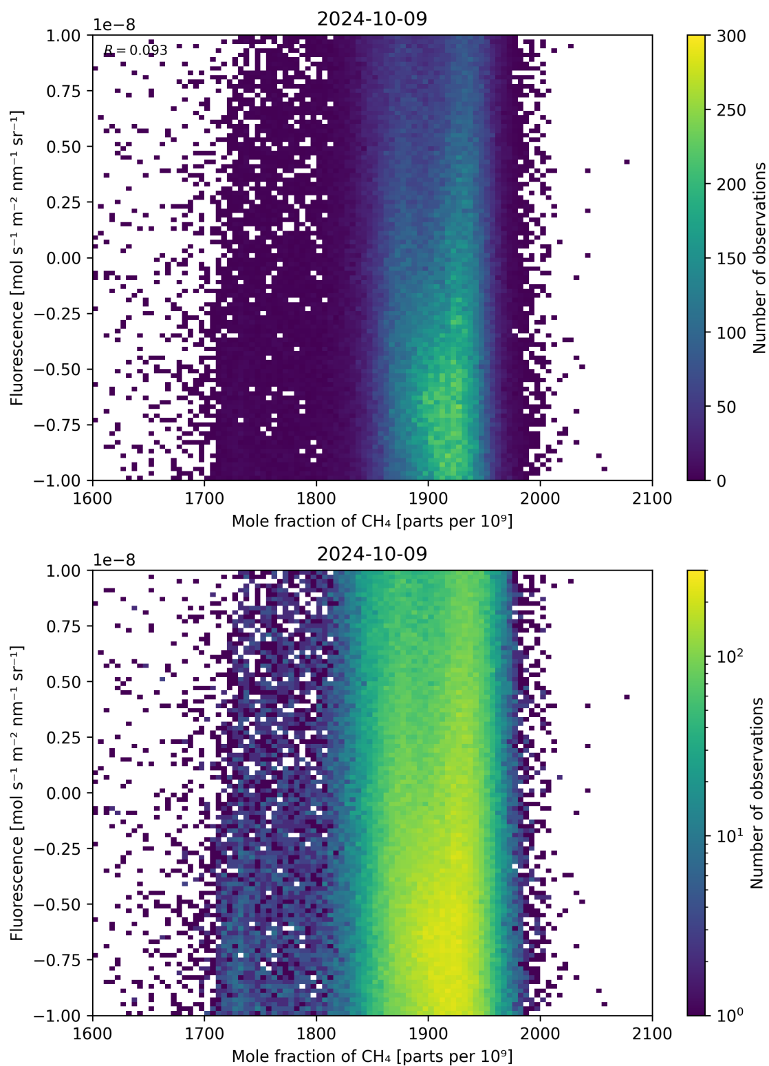
Figure 73: Scatter density plot of “Mole fraction of \text{CH}_4 ” against “Fluorescence” for 2024-10-08 to 2024-10-10.
