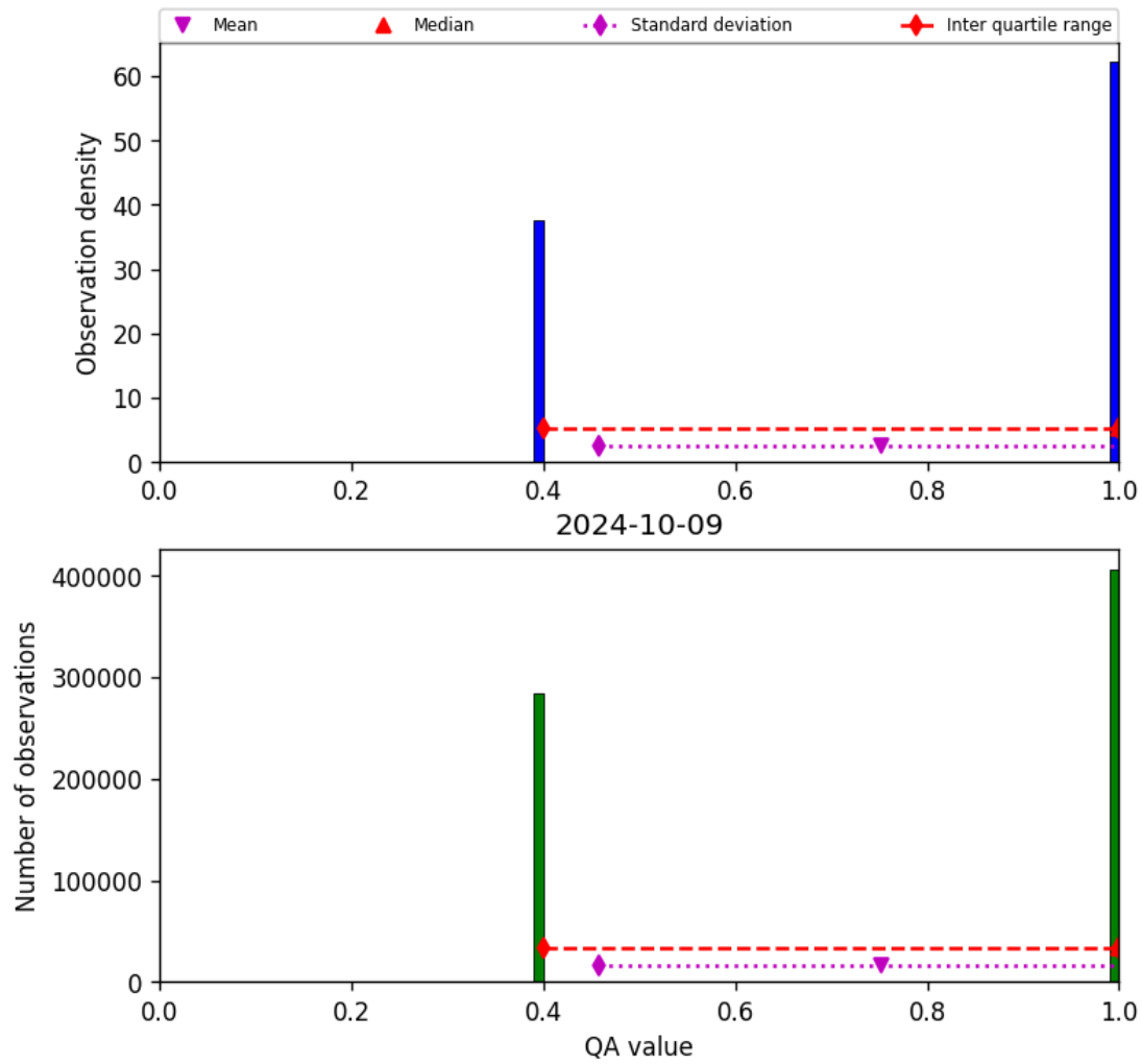
Figure 22: Histogram of “QA value” for 2024-10-08 to 2024-10-10
