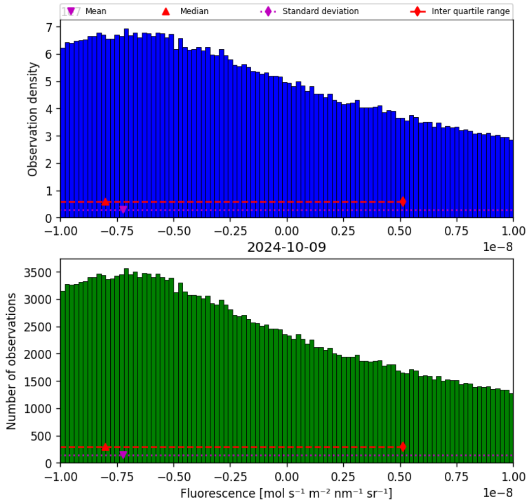
Figure 32: Histogram of “Fluorescence” for 2024-10-08 to 2024-10-10
