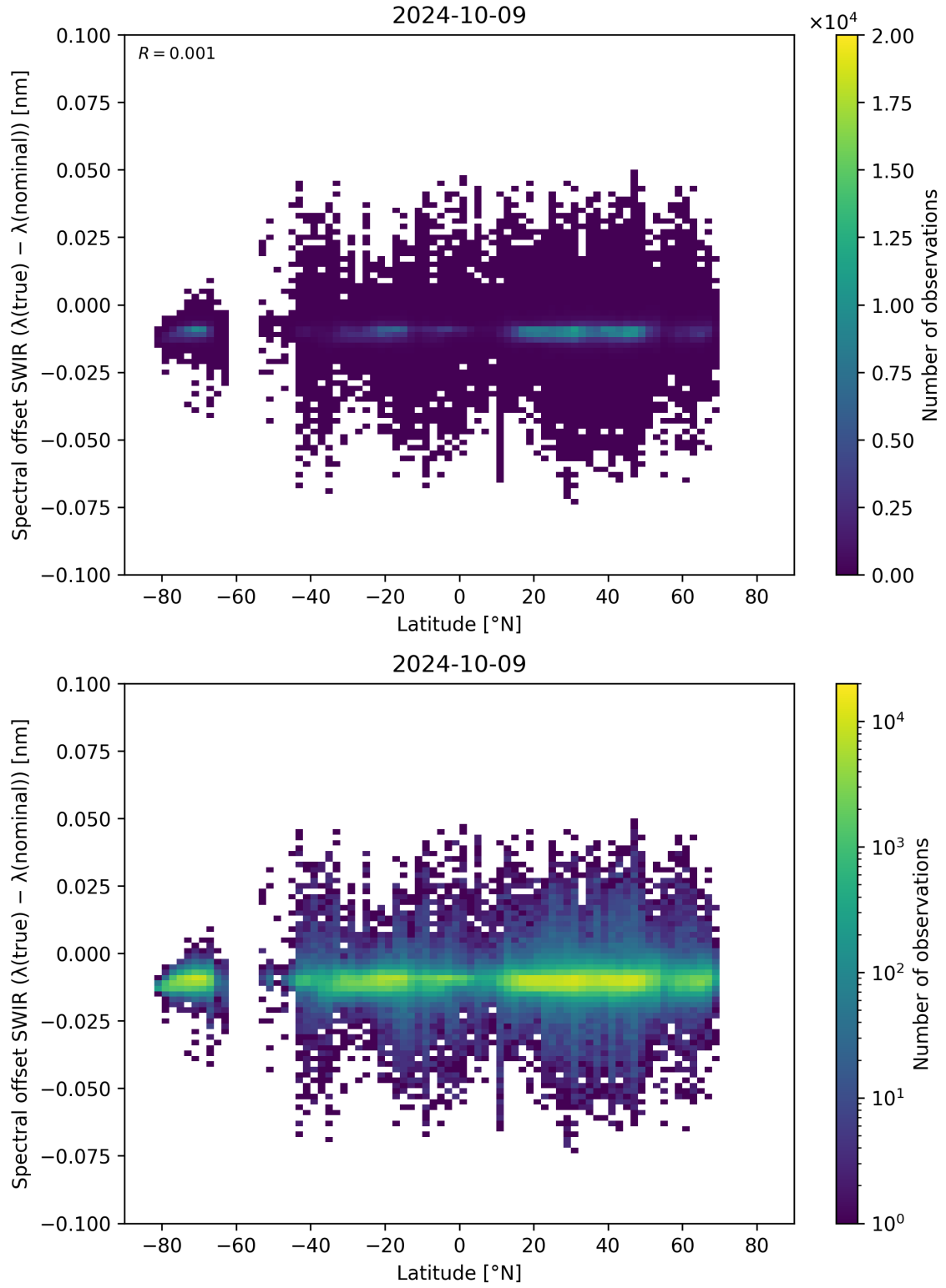
Figure 62: Scatter density plot of “Latitude” against “Spectral offset SWIR ( \lambda_{\text{true}} - \lambda_{\text{nominal}} )” for 2024-10-08 to 2024-10-10.
