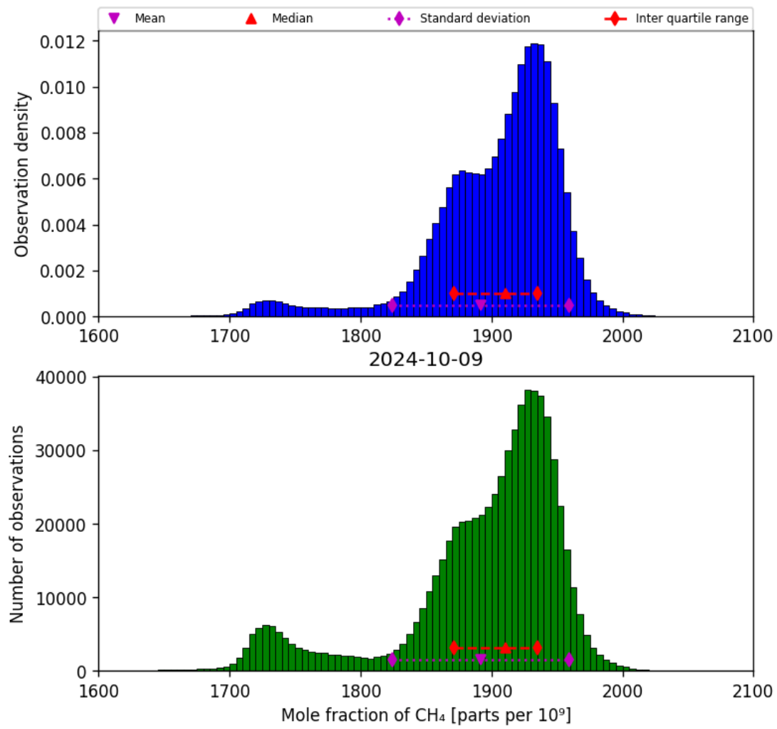
Figure 23: Histogram of “Mole fraction of CH 4 ” for 2024-10-08 to 2024-10-10
