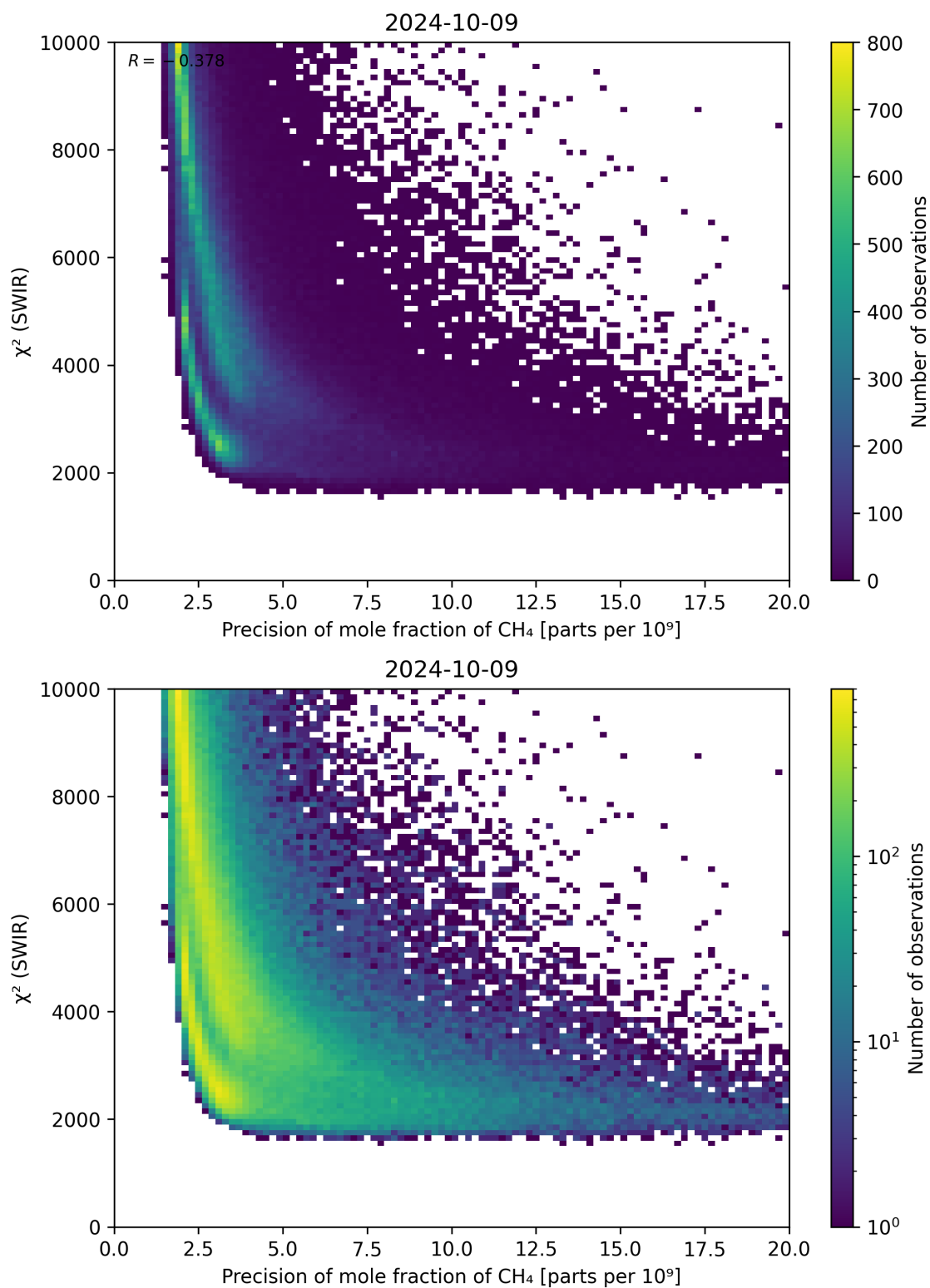
Figure 79: Scatter density plot of “Precision of mole fraction of CH 4 ” against “ \chi^2 (SWIR)” for 2024-10-08 to 2024-10-10.
