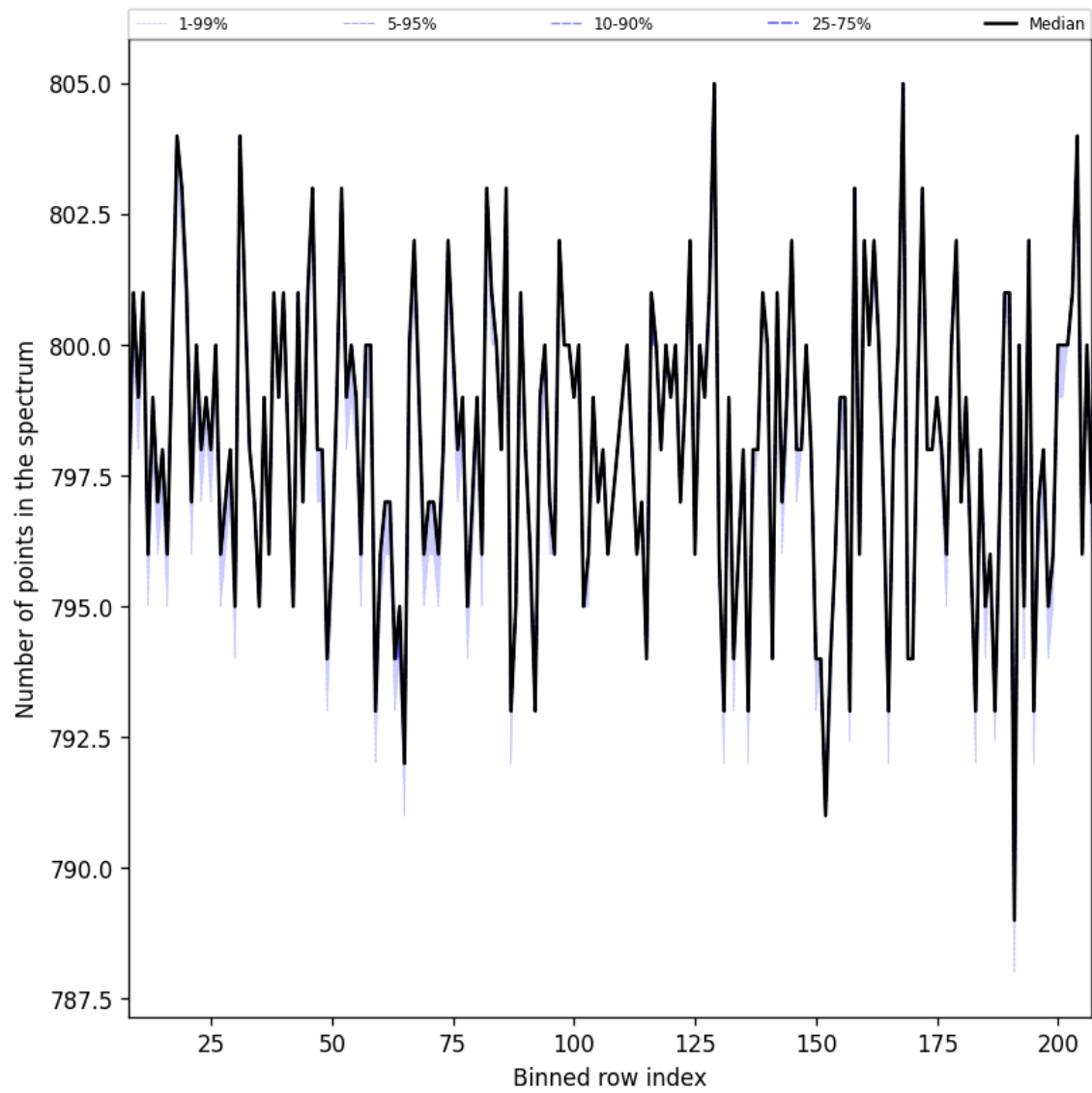
Figure 37: Along track statistics of “Number of points in the spectrum” for 2024-10-08 to 2024-10-10
