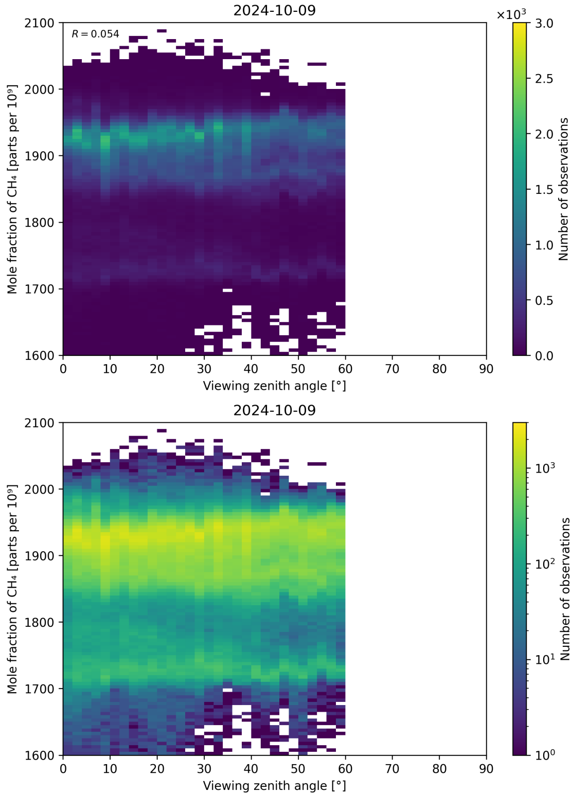
Figure 110: Scatter density plot of “Viewing zenith angle” against “Mole fraction of CH 4 ” for 2024-10-08 to 2024-10-10.
