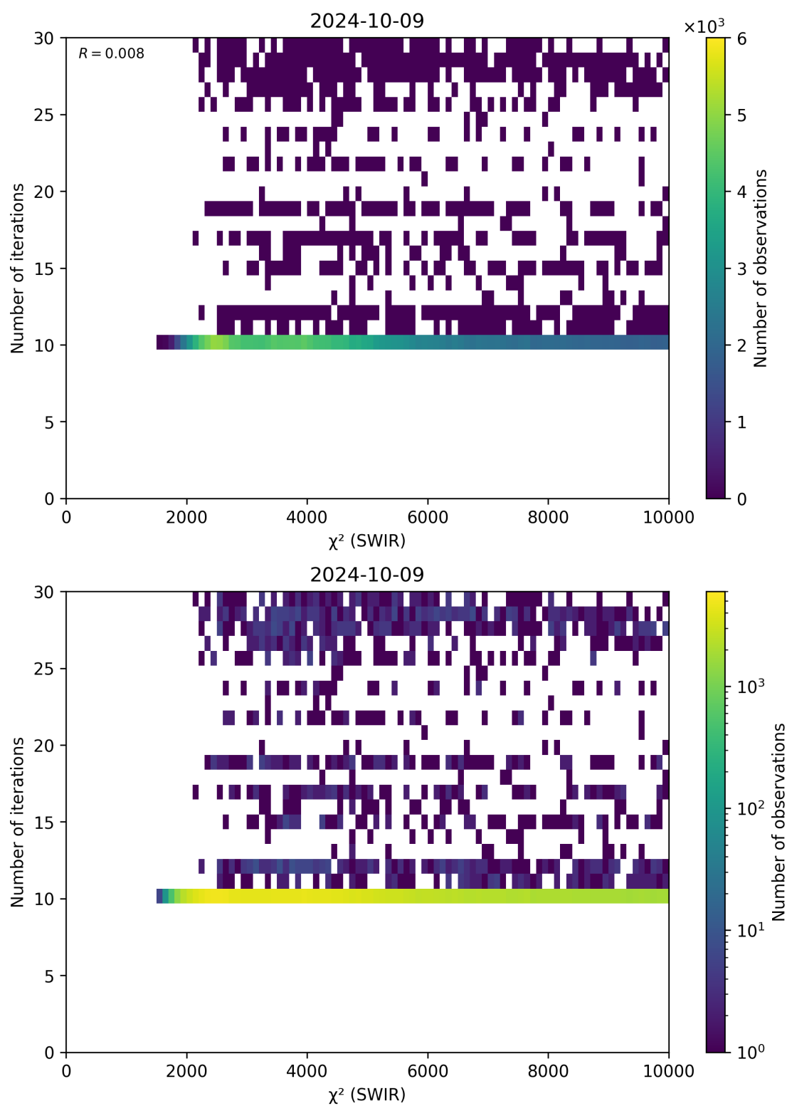
Figure 50: Scatter density plot of “ \chi^2 (SWIR)” against “Number of iterations” for 2024-10-08 to 2024-10-10.
