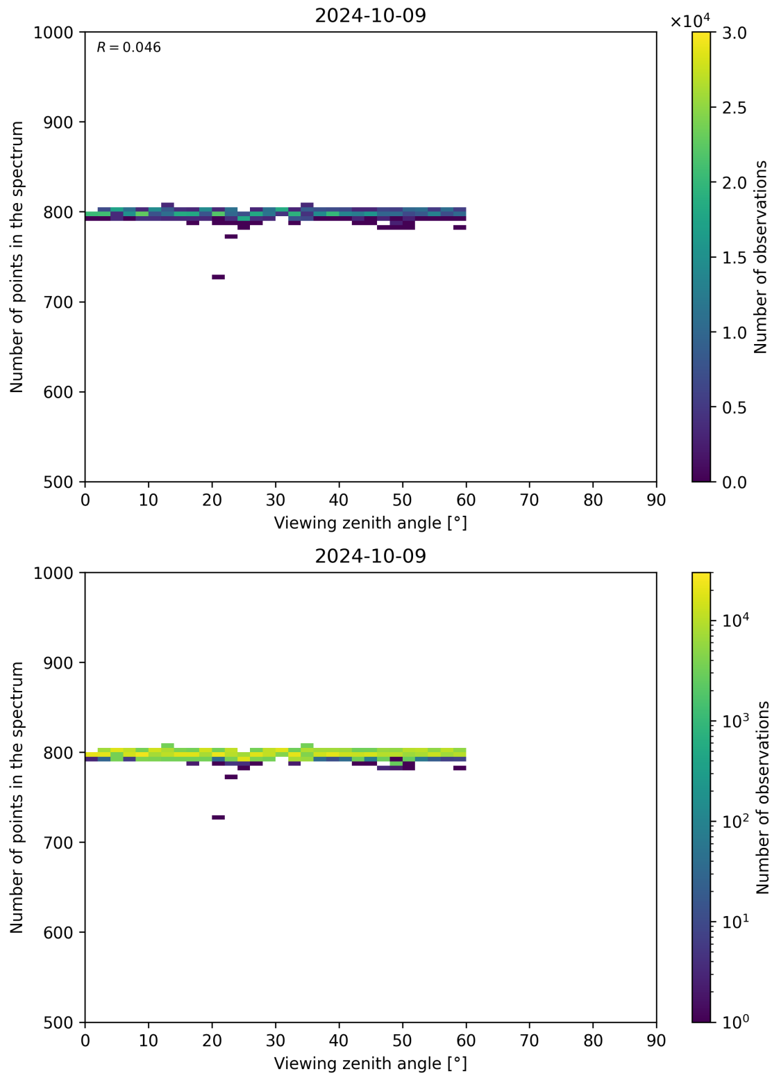
Figure 114: Scatter density plot of “Viewing zenith angle” against “Number of points in the spectrum” for 2024-10-08 to 2024-10-10.
