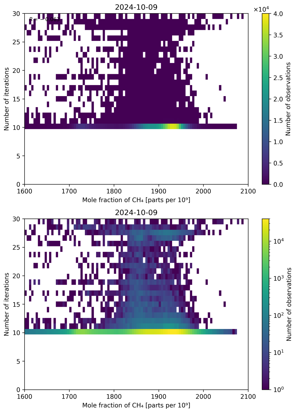
Figure 76: Scatter density plot of “Mole fraction of CH 4 ” against “Number of iterations” for 2024-10-08 to 2024-10-10.
