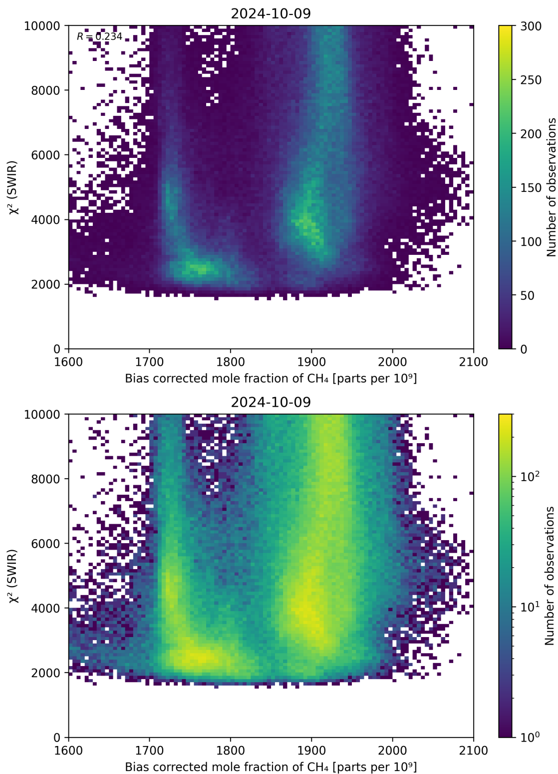
Figure 64: Scatter density plot of “Bias corrected mole fraction of \text{CH}_4 ” against “ \chi^2 (SWIR)” for 2024-10-08 to 2024-10-10.
