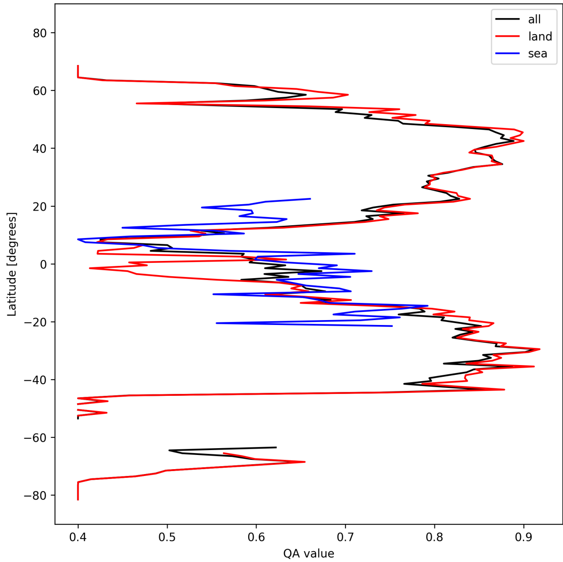
Figure 11: Zonal average of “QA value” for 2024-10-08 to 2024-10-10.
