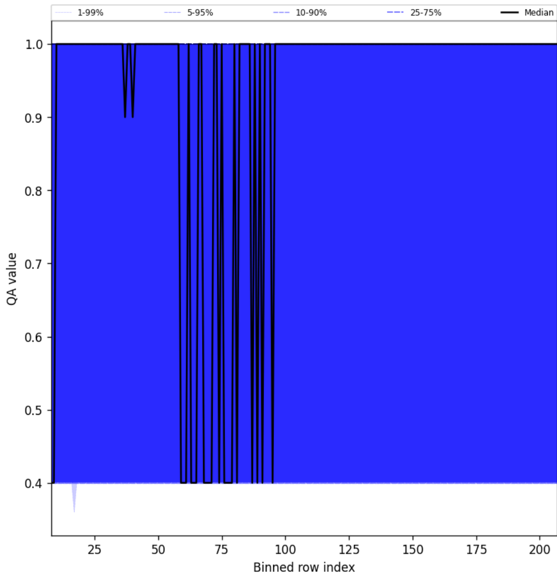
Figure 33: Along track statistics of “QA value” for 2024-10-08 to 2024-10-10
