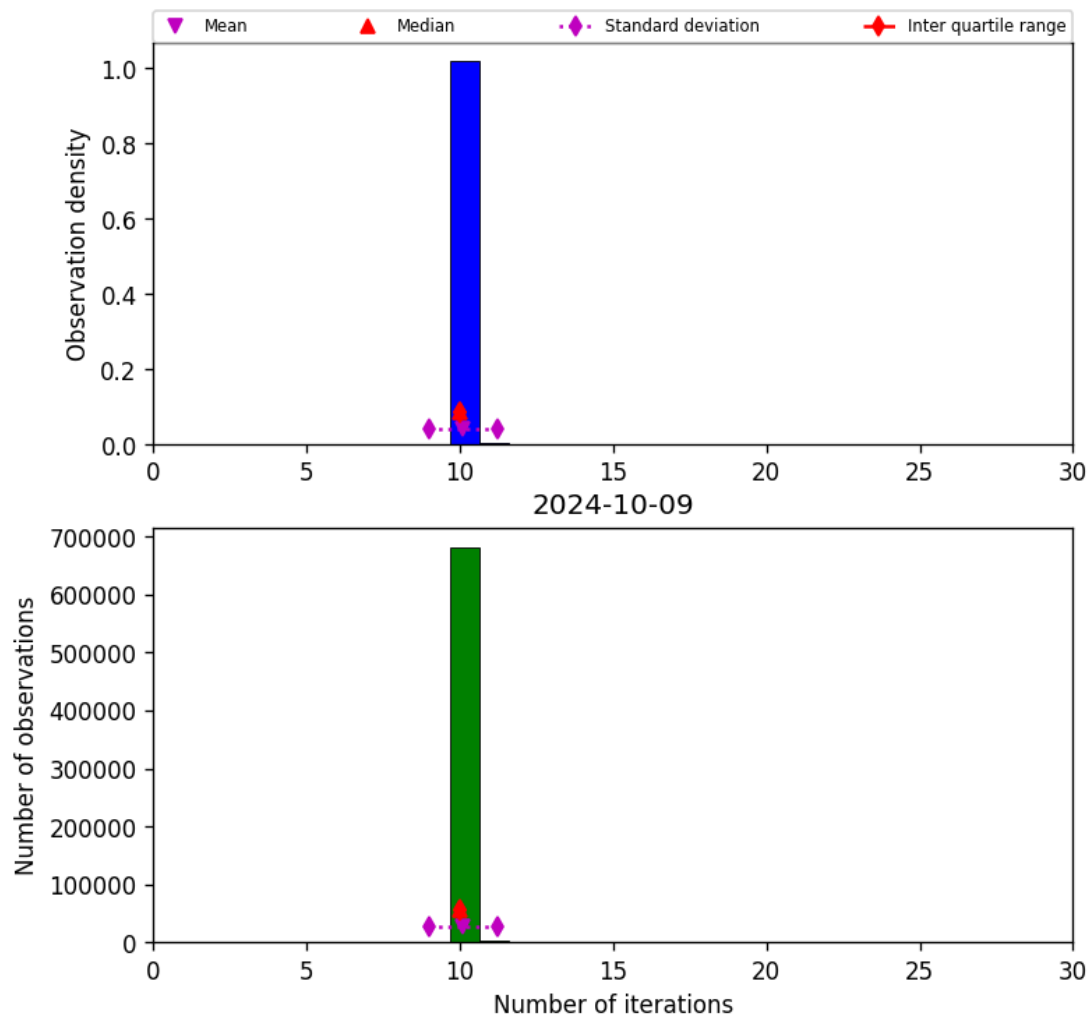
Figure 31: Histogram of “Number of iterations” for 2024-10-08 to 2024-10-10
