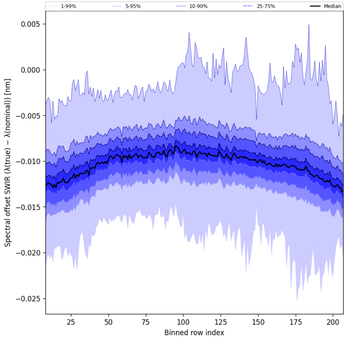
Figure 38: Along track statistics of “Spectral offset SWIR ( \lambda_{\text{true}} - \lambda_{\text{nominal}} )” for 2024-10-08 to 2024-10-10
