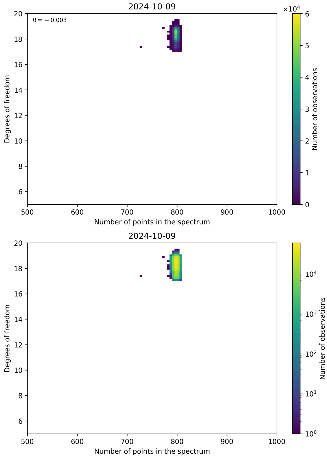
Figure 90: Scatter density plot of “Number of points in the spectrum” against “Degrees of freedom” for 2024-10-08 to 2024-10-10.
