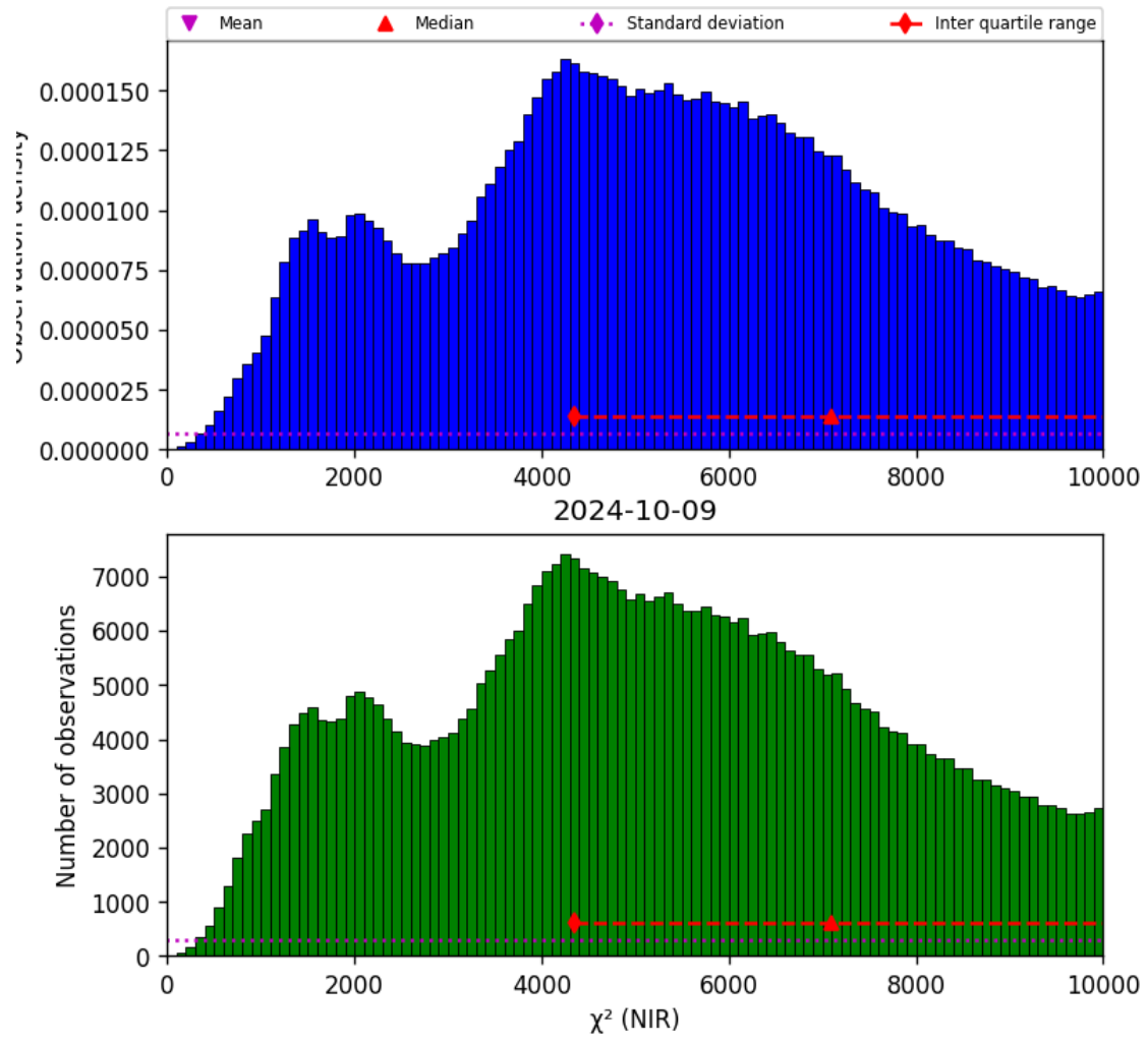
Figure 29: Histogram of “ \chi^2 (NIR)” for 2024-10-08 to 2024-10-10
