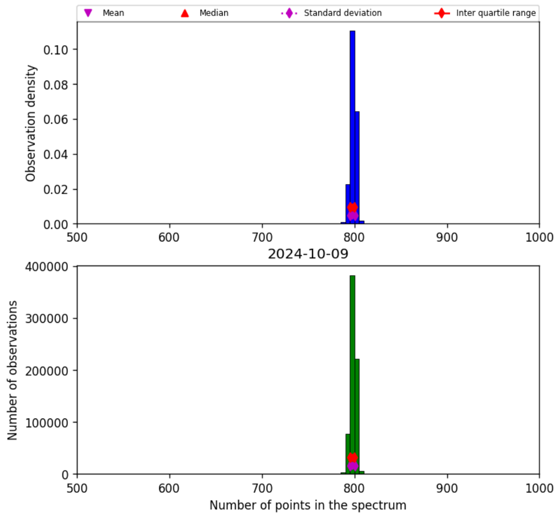
Figure 26: Histogram of “Number of points in the spectrum” for 2024-10-08 to 2024-10-10
