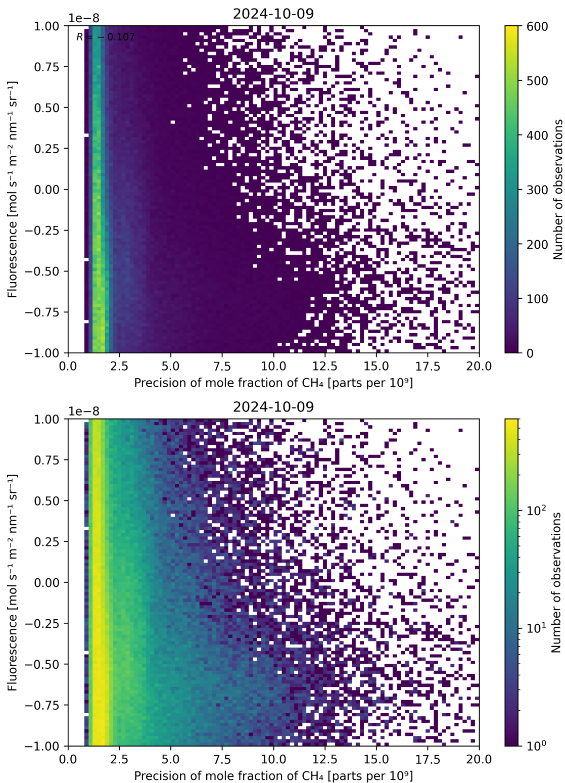
Figure 81: Scatter density plot of “Precision of mole fraction of \text{CH}_4 ” against “Fluorescence” for 2024-10-08 to 2024-10-10.
