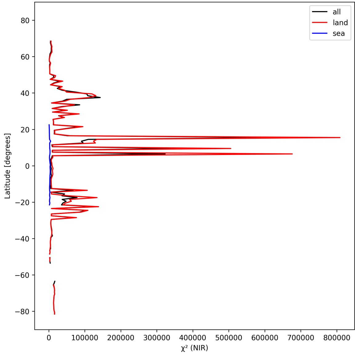
Figure 18: Zonal average of “ \chi^2 (NIR)” for 2024-10-08 to 2024-10-10.
