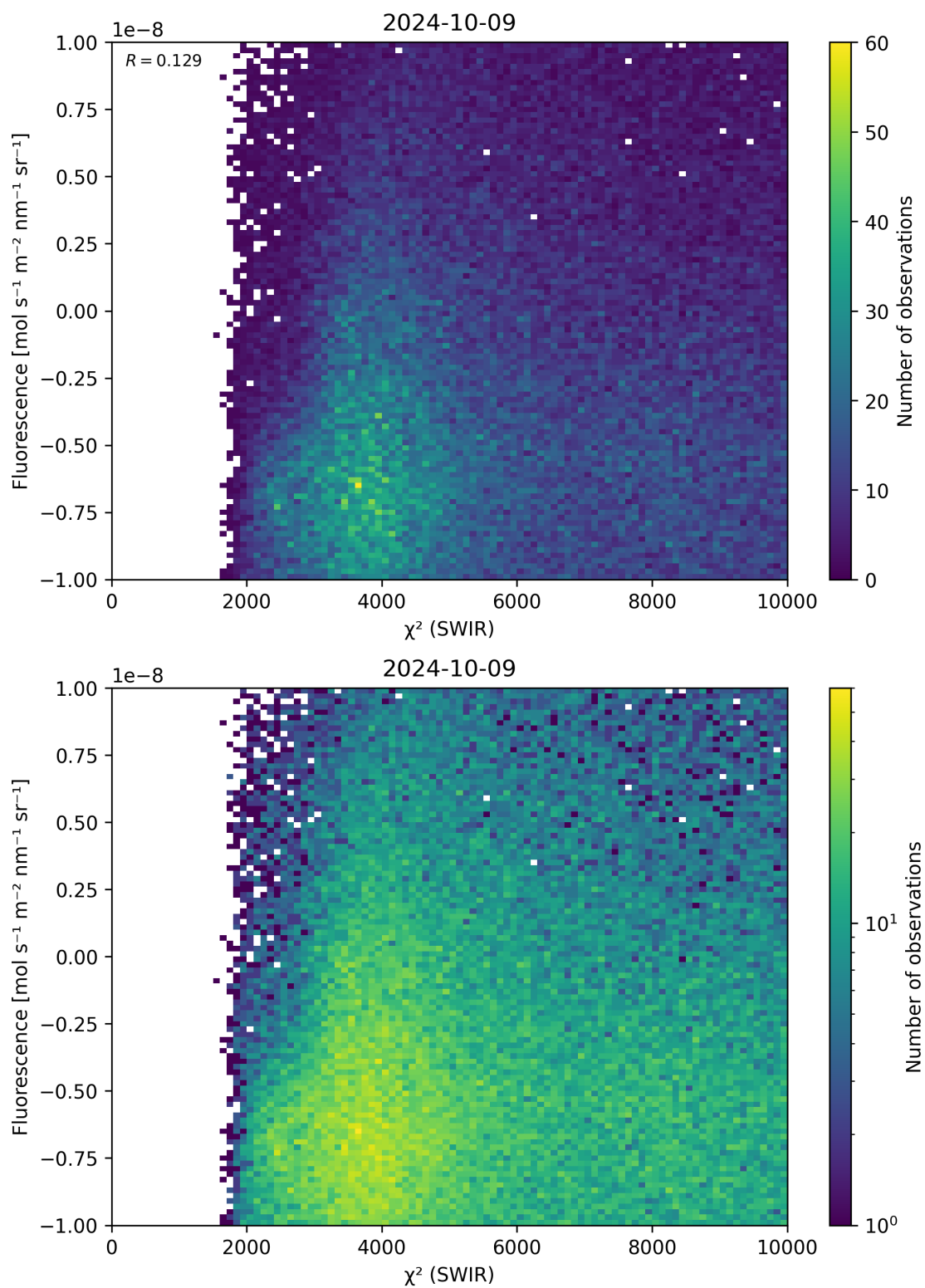
Figure 49: Scatter density plot of “ \chi^2 (SWIR)” against “Fluorescence” for 2024-10-08 to 2024-10-10.
