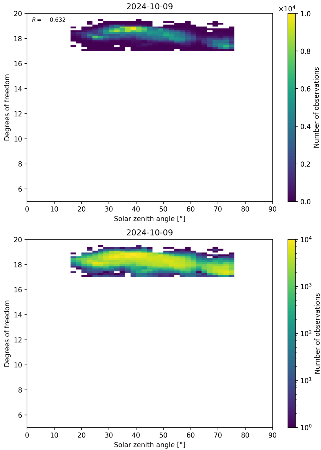
Figure 96: Scatter density plot of “Solar zenith angle” against “Degrees of freedom” for 2024-10-08 to 2024-10-10.
