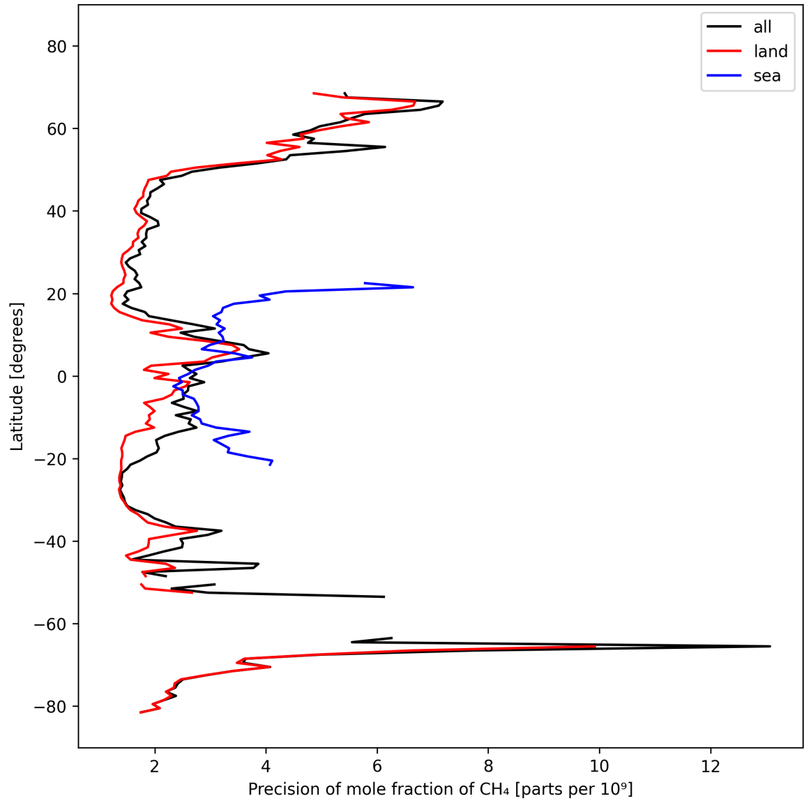
Figure 13: Zonal average of “Precision of mole fraction of CH 4 ” for 2024-10-08 to 2024-10-10.
