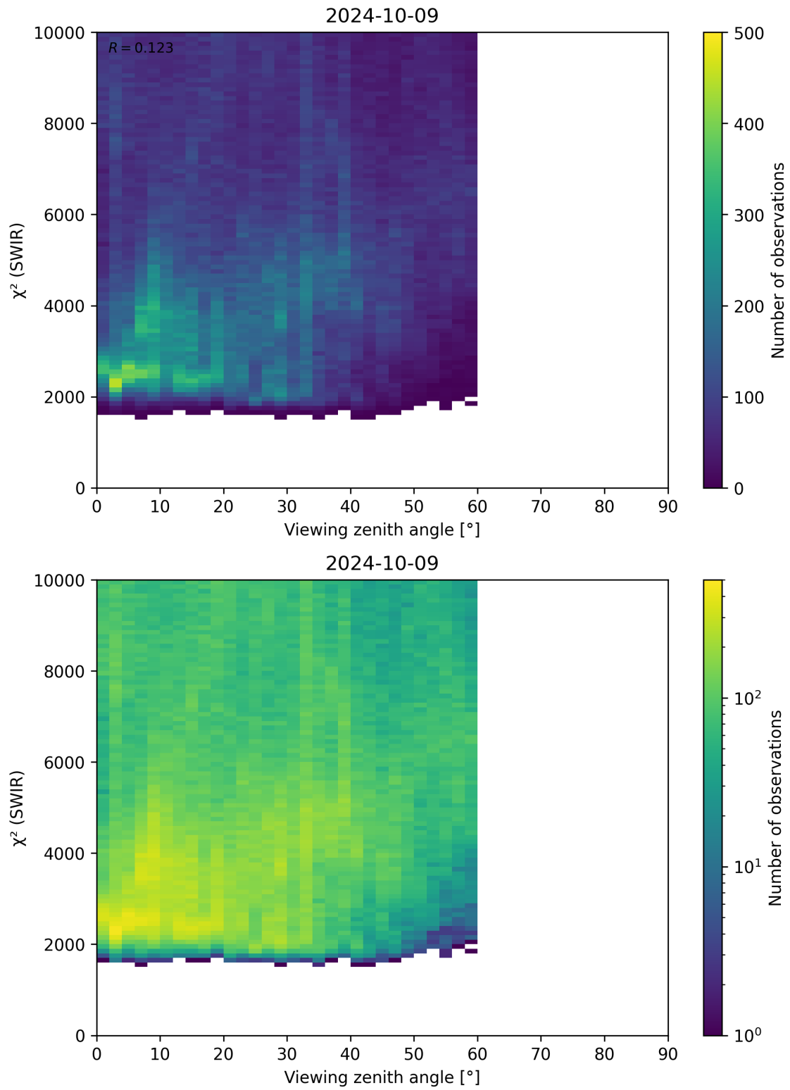
Figure 106: Scatter density plot of “Viewing zenith angle” against “ \chi^2 (SWIR)” for 2024-10-08 to 2024-10-10.
