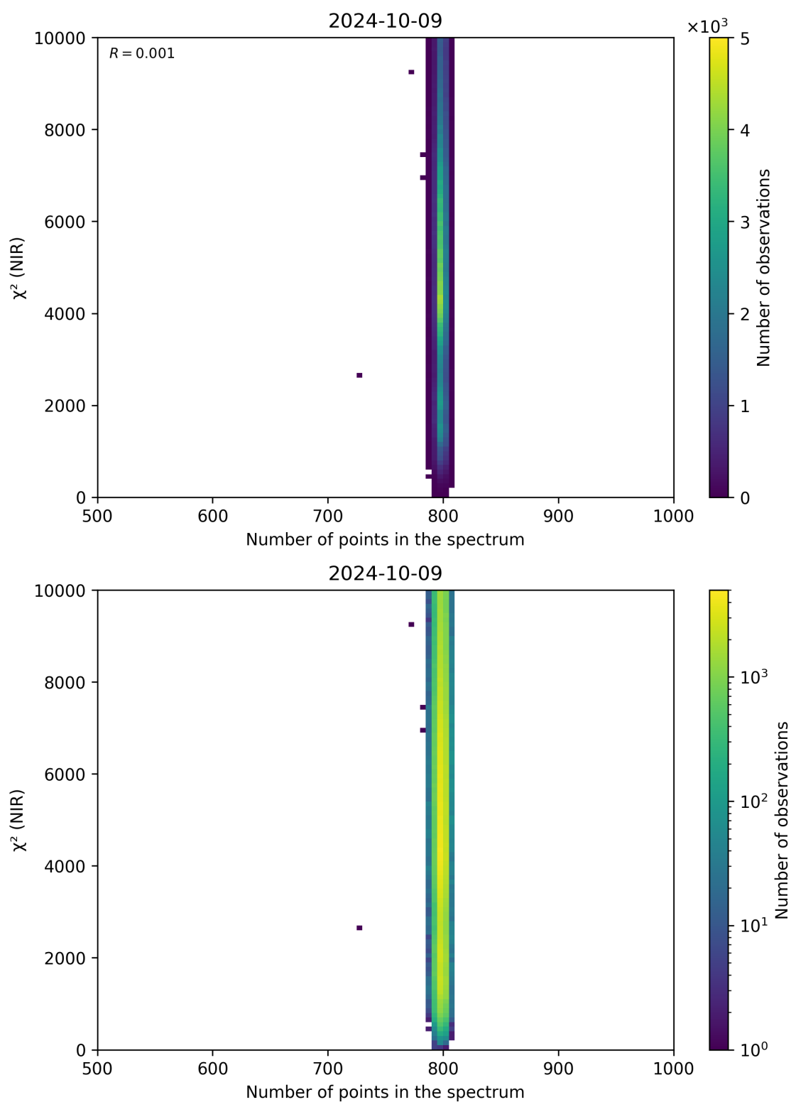
Figure 88: Scatter density plot of “Number of points in the spectrum” against “ \chi^2 (NIR)” for 2024-10-08 to 2024-10-10.
