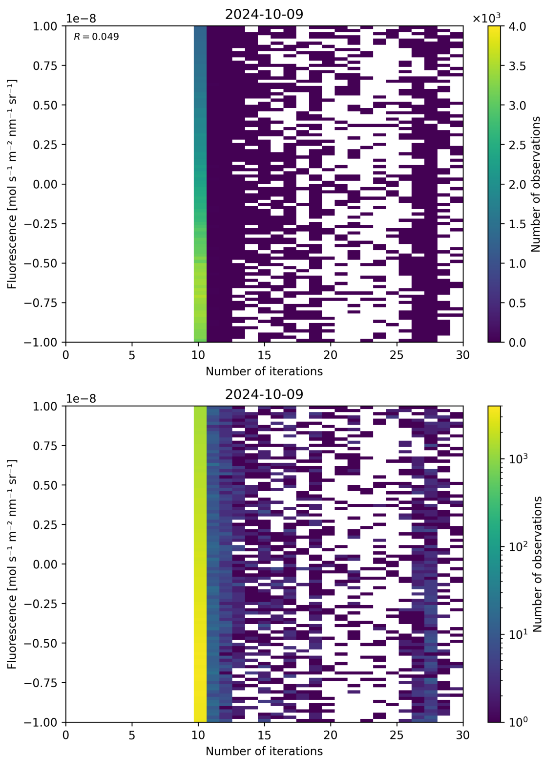
Figure 87: Scatter density plot of “Number of iterations” against “Fluorescence” for 2024-10-08 to 2024-10-10.
