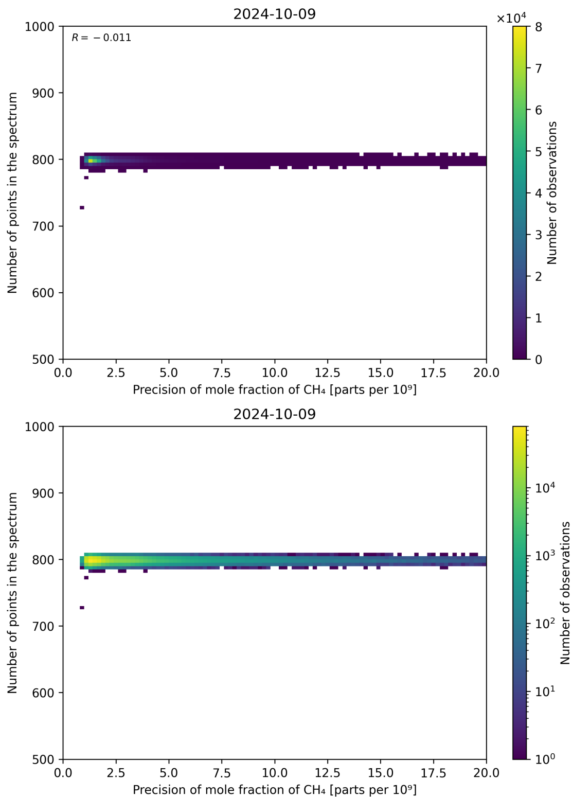
Figure 84: Scatter density plot of “Precision of mole fraction of CH 4 ” against “Number of points in the spectrum” for 2024-10-08 to 2024-10-10.
