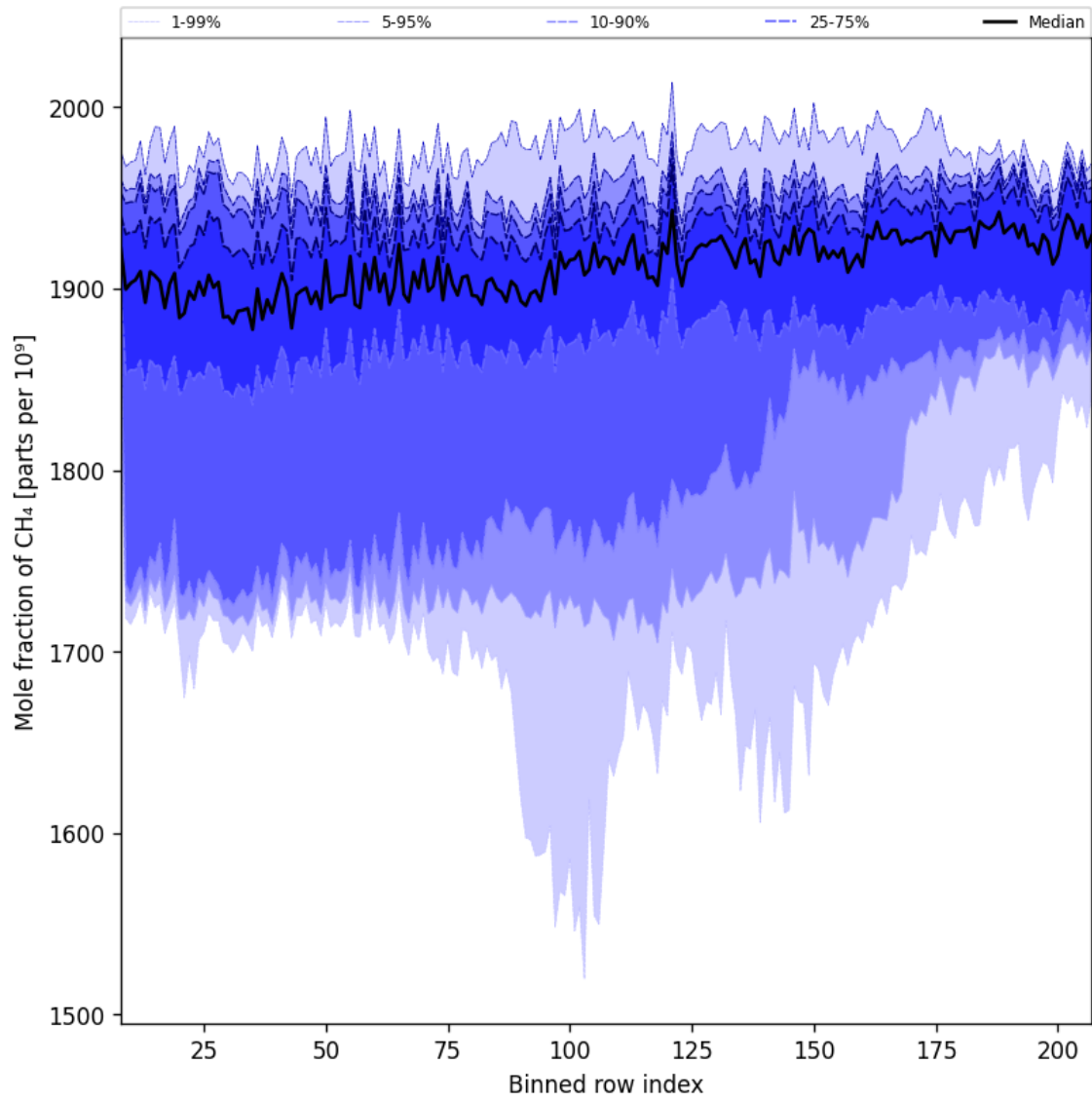
Figure 34: Along track statistics of “Mole fraction of CH 4 ” for 2024-10-08 to 2024-10-10
