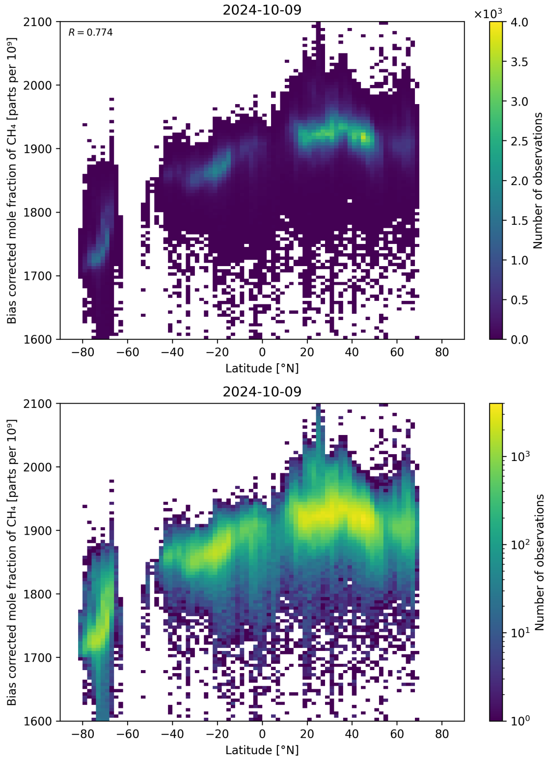
Figure 58: Scatter density plot of “Latitude” against “Bias corrected mole fraction of CH 4 ” for 2024-10-08 to 2024-10-10.
