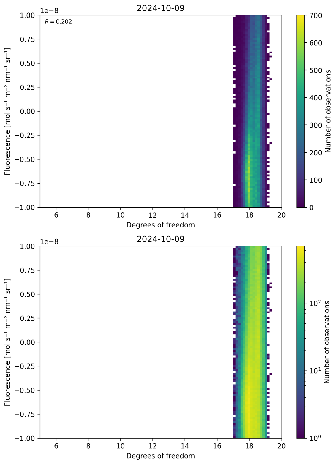
Figure 51: Scatter density plot of “Degrees of freedom” against “Fluorescence” for 2024-10-08 to 2024-10-10.
