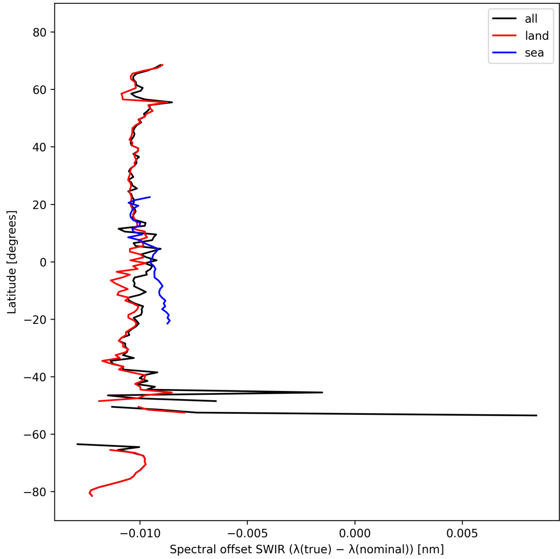
Figure 16: Zonal average of “Spectral offset SWIR ( \lambda_{\text{true}} - \lambda_{\text{nominal}} )” for 2024-10-08 to 2024-10-10.
