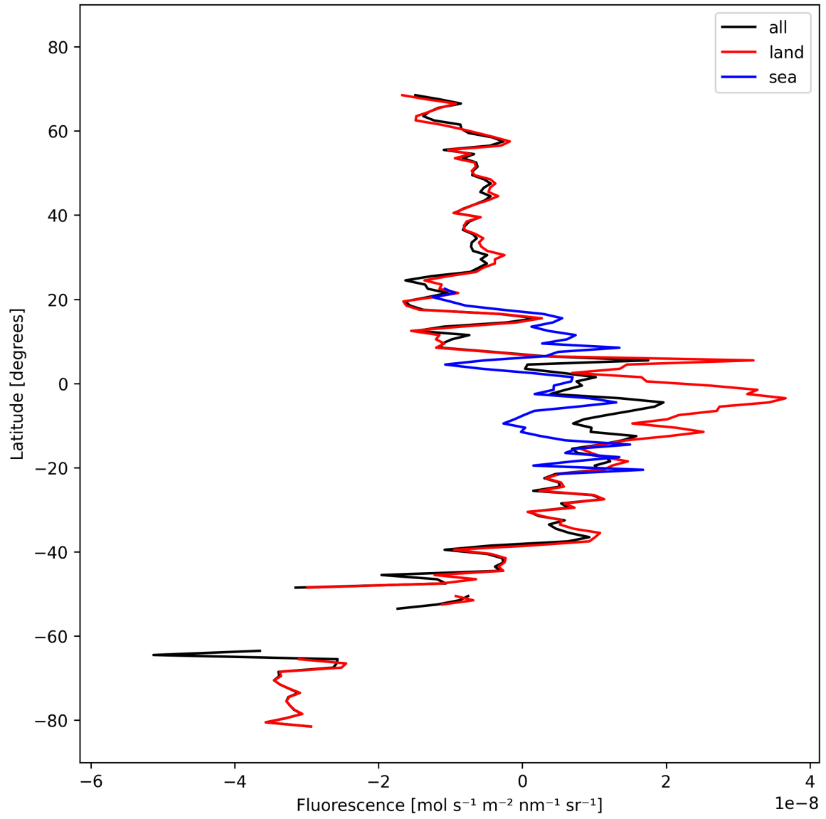
Figure 21: Zonal average of “Fluorescence” for 2024-10-08 to 2024-10-10.
