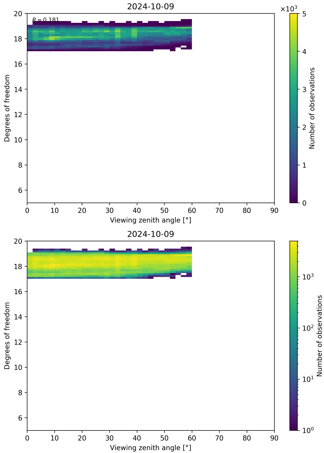
Figure 107: Scatter density plot of “Viewing zenith angle” against “Degrees of freedom” for 2024-10-08 to 2024-10-10.
