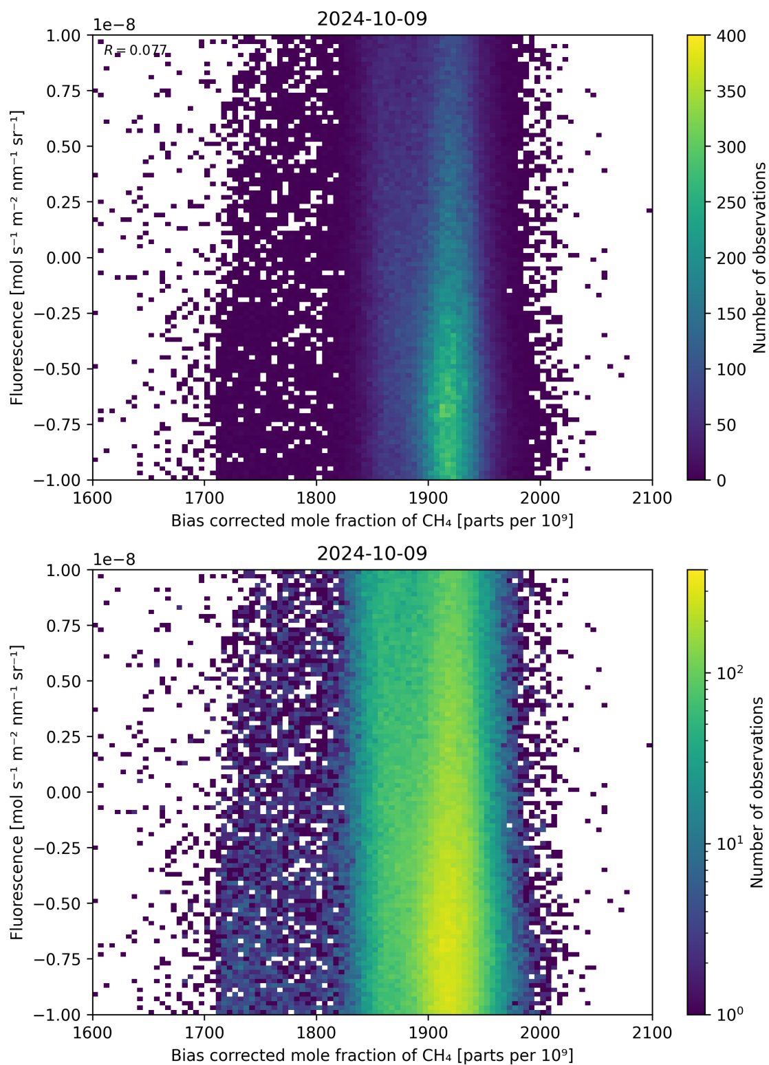
Figure 66: Scatter density plot of “Bias corrected mole fraction of \text{CH}_4 ” against “Fluorescence” for 2024-10-08 to 2024-10-10.
