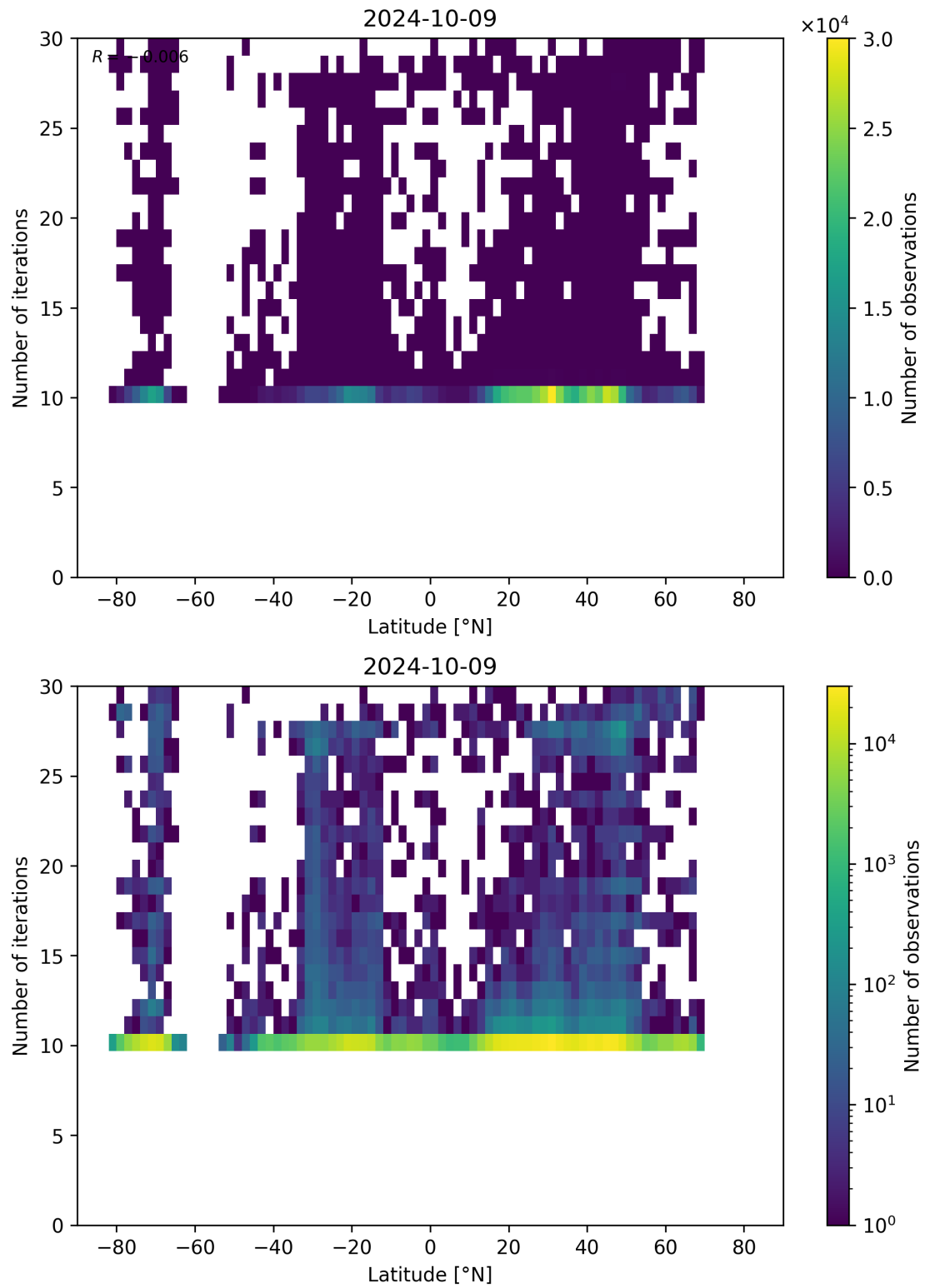
Figure 60: Scatter density plot of “Latitude” against “Number of iterations” for 2024-10-08 to 2024-10-10.
