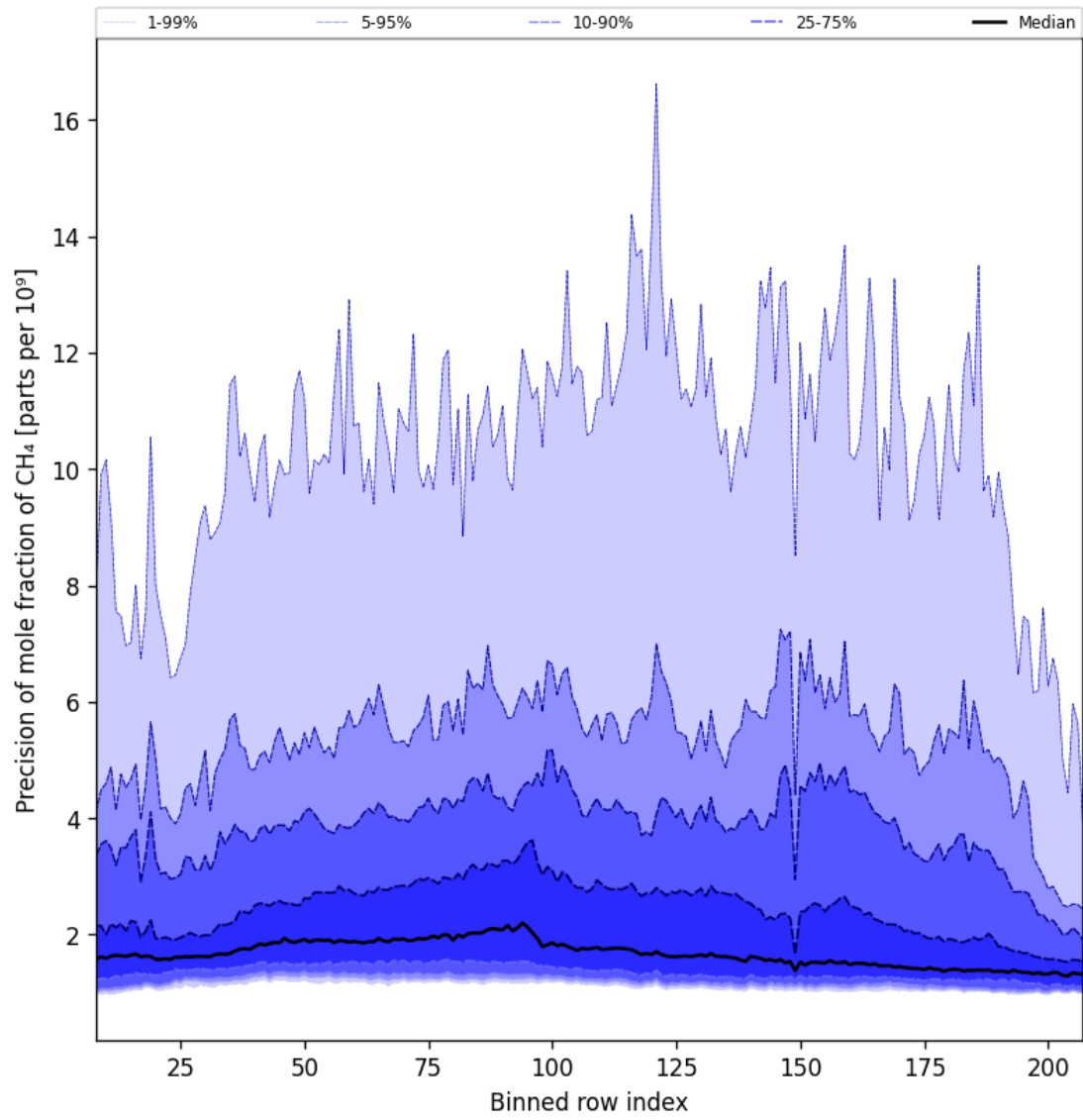
Figure 35: Along track statistics of “Precision of mole fraction of CH 4 ” for 2024-10-08 to 2024-10-10
