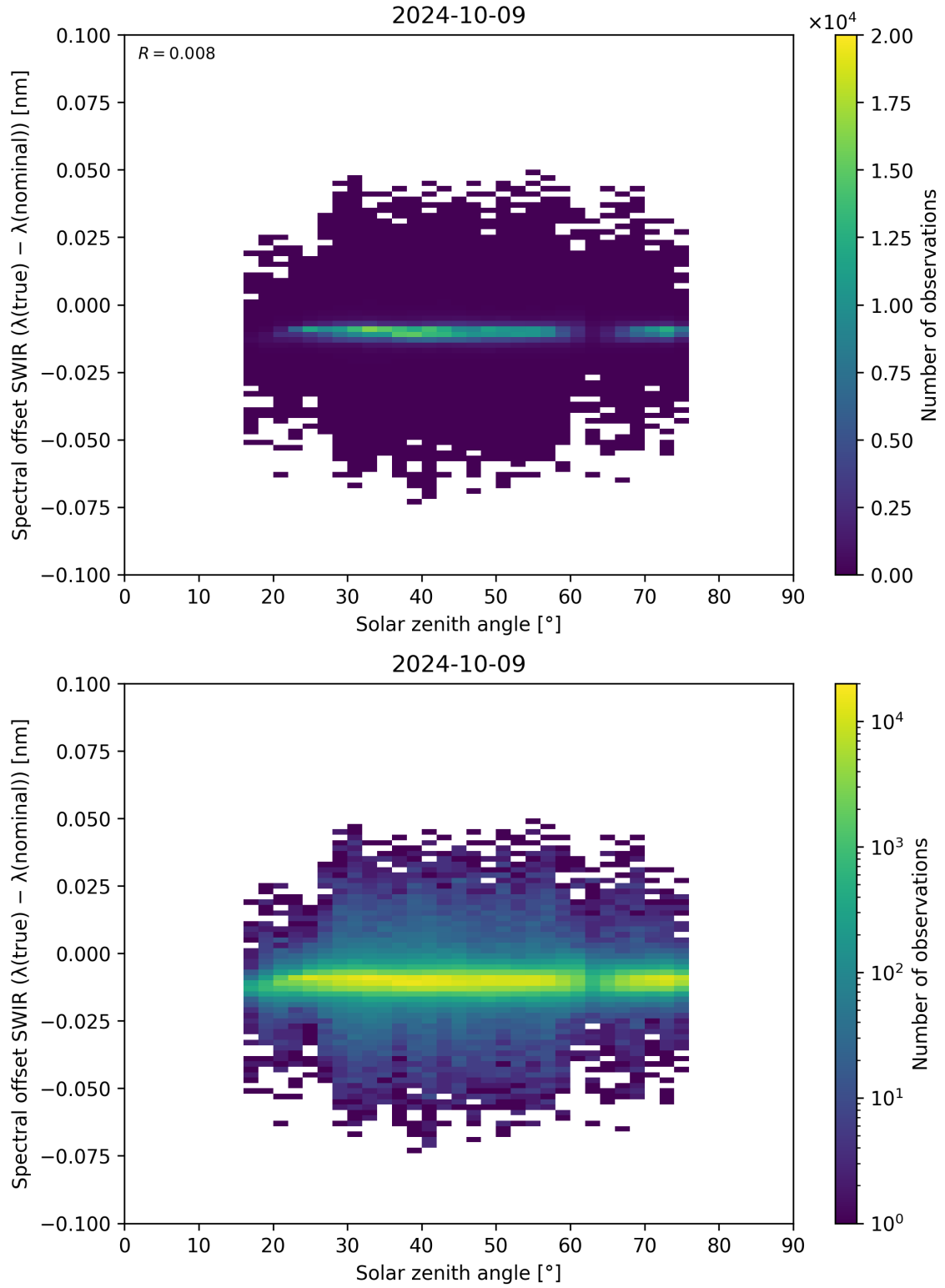
Figure 104: Scatter density plot of “Solar zenith angle” against “Spectral offset SWIR ( \lambda_{\text{true}} - \lambda_{\text{nominal}} )” for 2024-10-08 to 2024-10-10.
