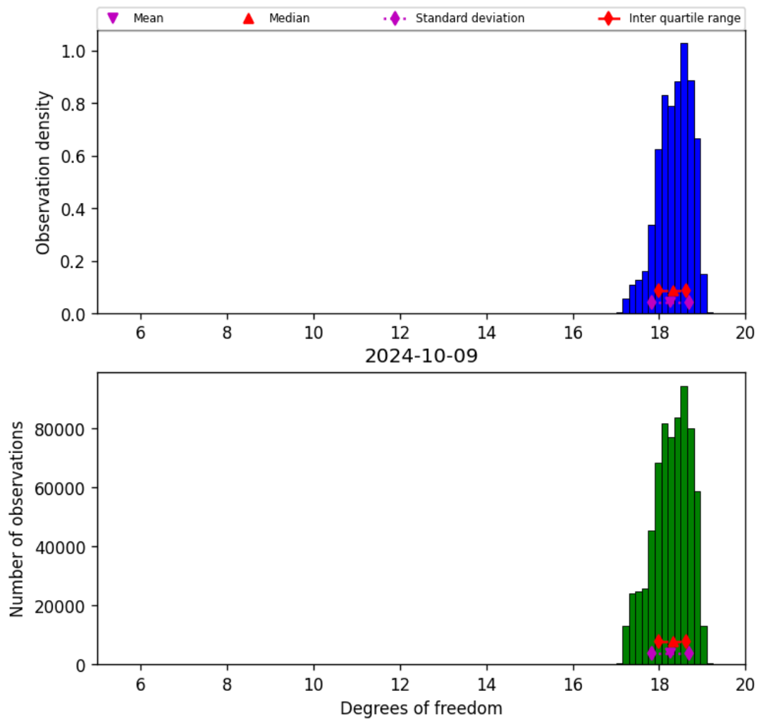
Figure 30: Histogram of “Degrees of freedom” for 2024-10-08 to 2024-10-10
