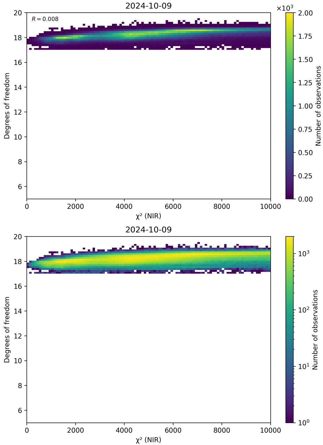
Figure 44: Scatter density plot of “ \chi^2 (NIR)” against “Degrees of freedom” for 2024-10-08 to 2024-10-10.
