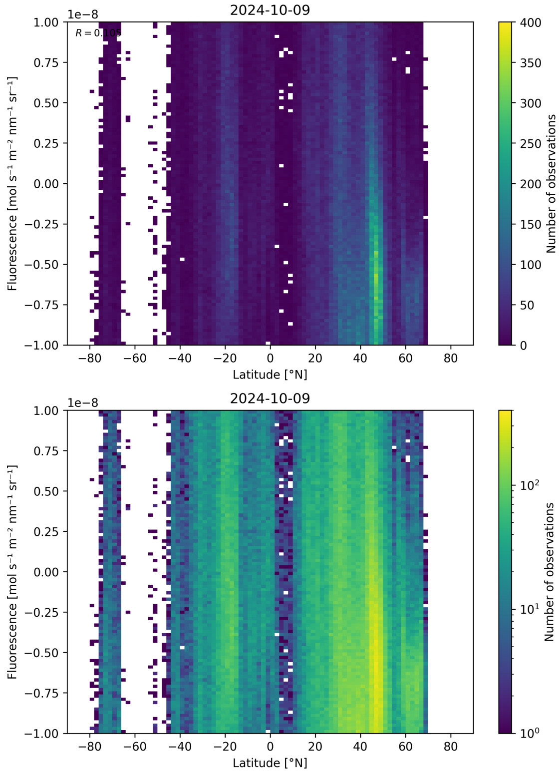
Figure 56: Scatter density plot of “Latitude” against “Fluorescence” for 2024-10-08 to 2024-10-10.
