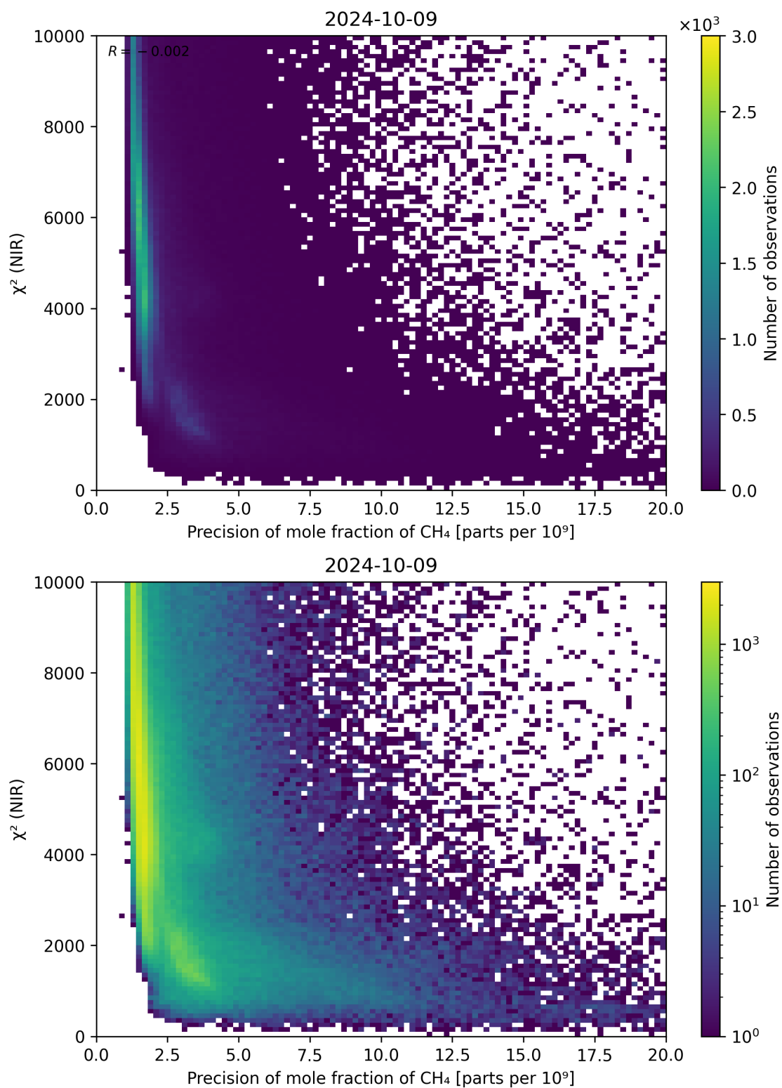
Figure 78: Scatter density plot of “Precision of mole fraction of CH 4 ” against “ \chi^2 (NIR)” for 2024-10-08 to 2024-10-10.
