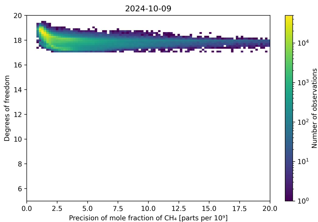
Figure 80: Scatter density plot of “Precision of mole fraction of CH 4 ” against “Degrees of freedom” for 2024-10-08 to 2024-10-10.
