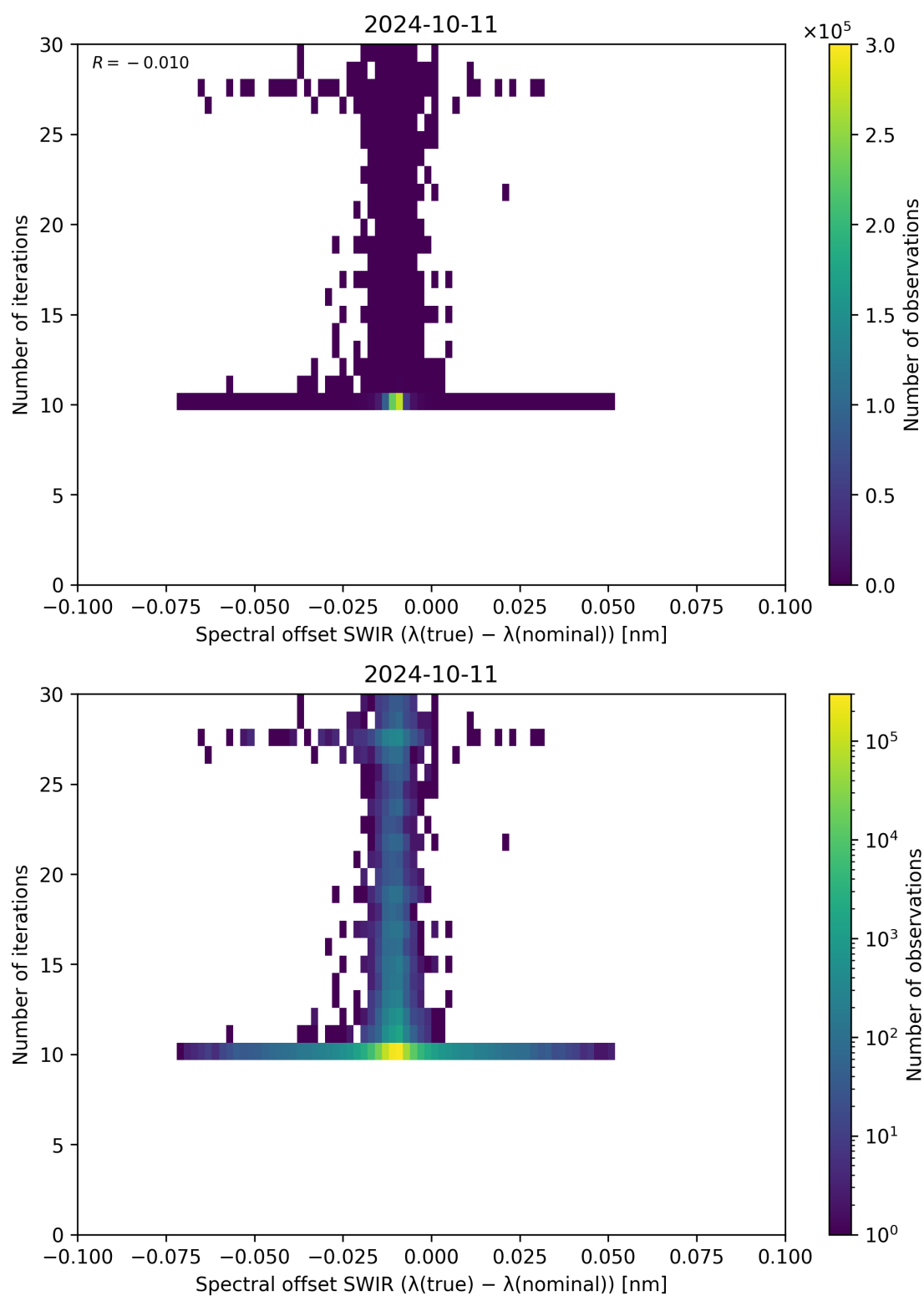
Figure 121: Scatter density plot of “Spectral offset SWIR ( \lambda_{\text{true}} - \lambda_{\text{nominal}} )” against “Number of iterations” for 2024-10-10 to 2024-10-12.
