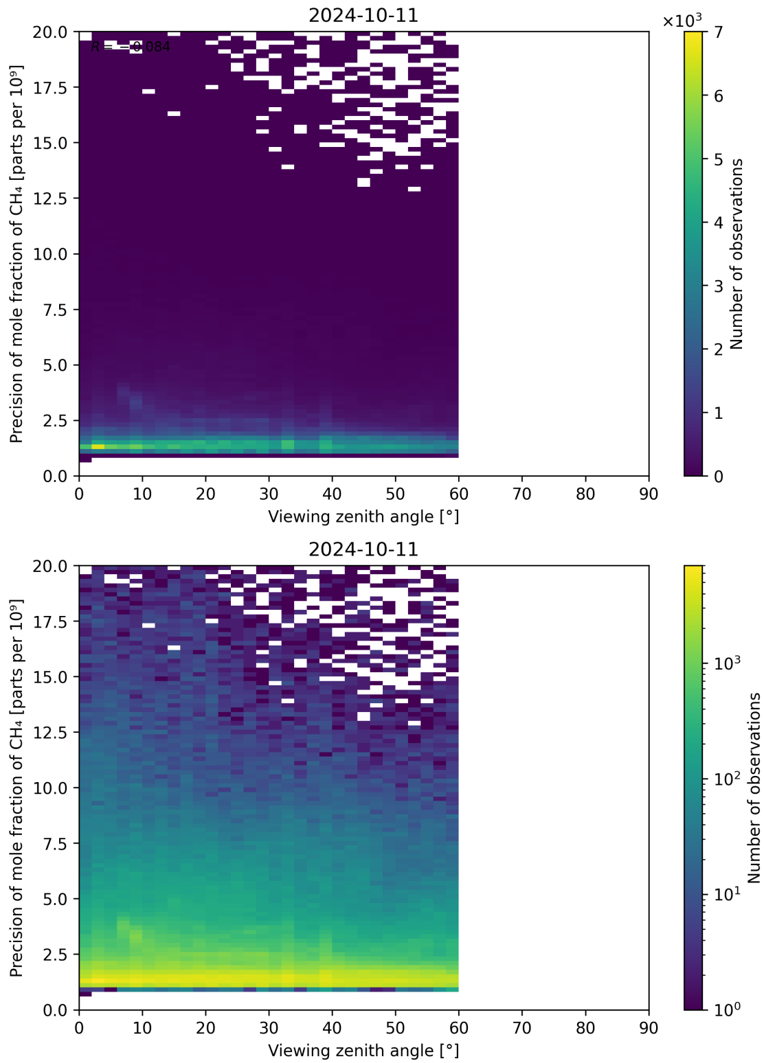
Figure 112: Scatter density plot of “Viewing zenith angle” against “Precision of mole fraction of CH 4 ” for 2024-10-10 to 2024-10-12.
