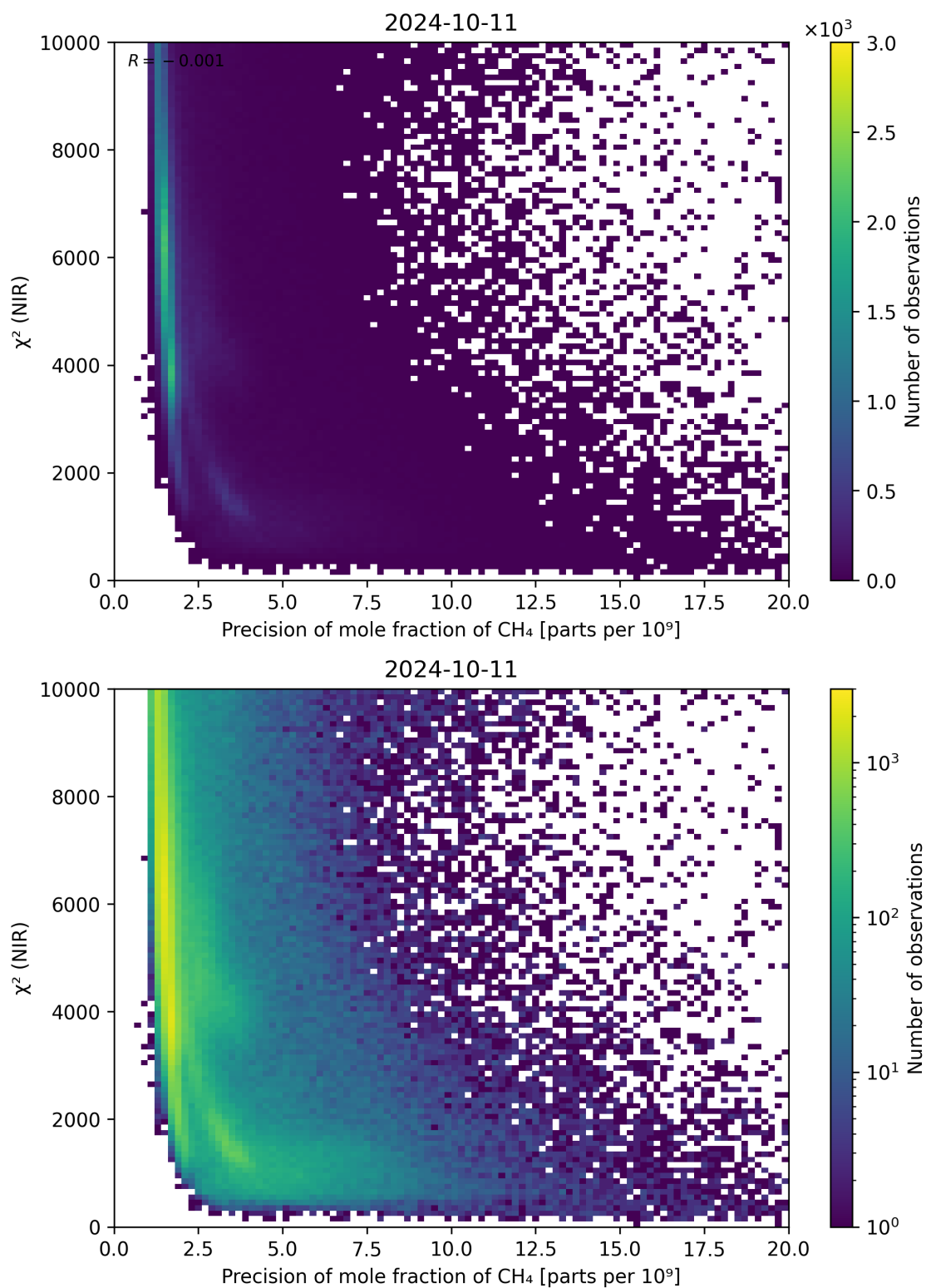
Figure 78: Scatter density plot of “Precision of mole fraction of CH 4 ” against “ \chi^2 (NIR)” for 2024-10-10 to 2024-10-12.
