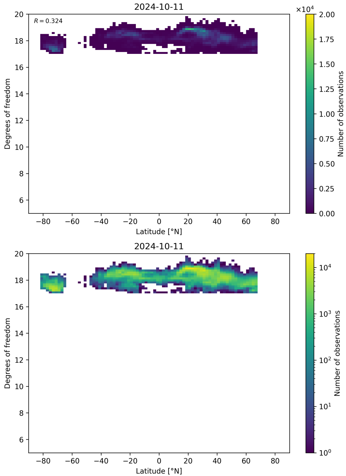
Figure 55: Scatter density plot of “Latitude” against “Degrees of freedom” for 2024-10-10 to 2024-10-12.
