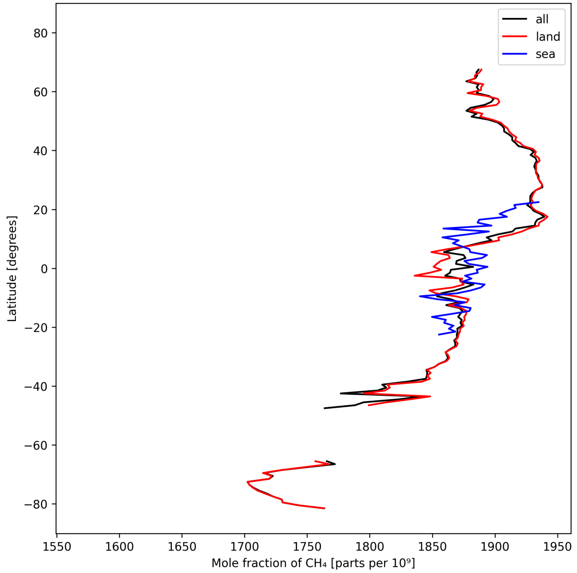
Figure 12: Zonal average of “Mole fraction of CH 4 ” for 2024-10-10 to 2024-10-12.
