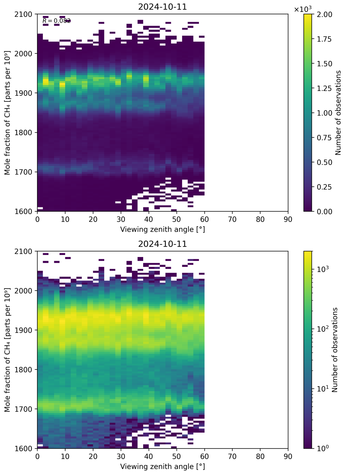
Figure 110: Scatter density plot of “Viewing zenith angle” against “Mole fraction of CH 4 ” for 2024-10-10 to 2024-10-12.
