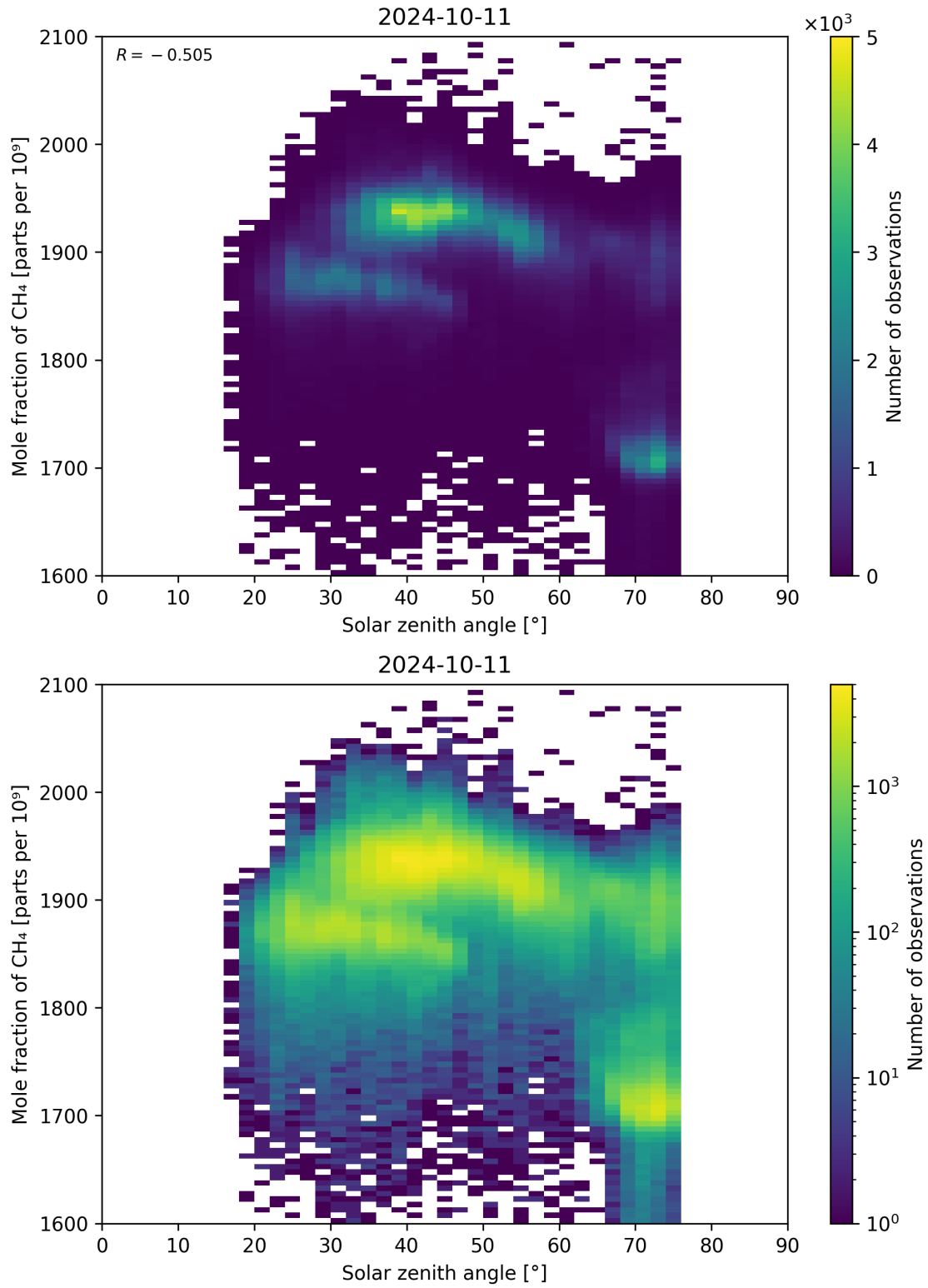
Figure 99: Scatter density plot of “Solar zenith angle” against “Mole fraction of CH 4 ” for 2024-10-10 to 2024-10-12.
