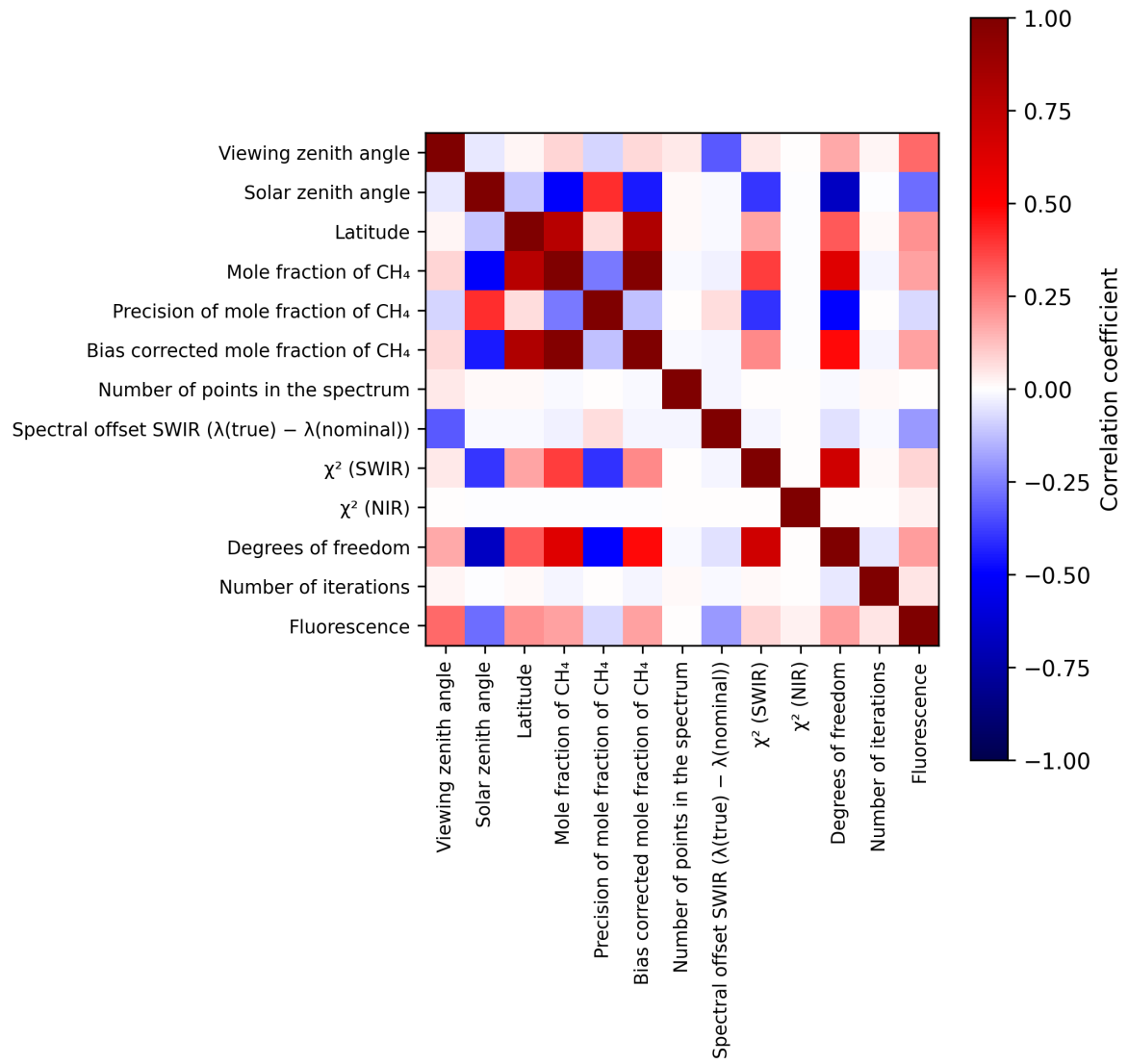
Figure 2: Map of correlation matrix for 2024-10-10 to 2024-10-12.
