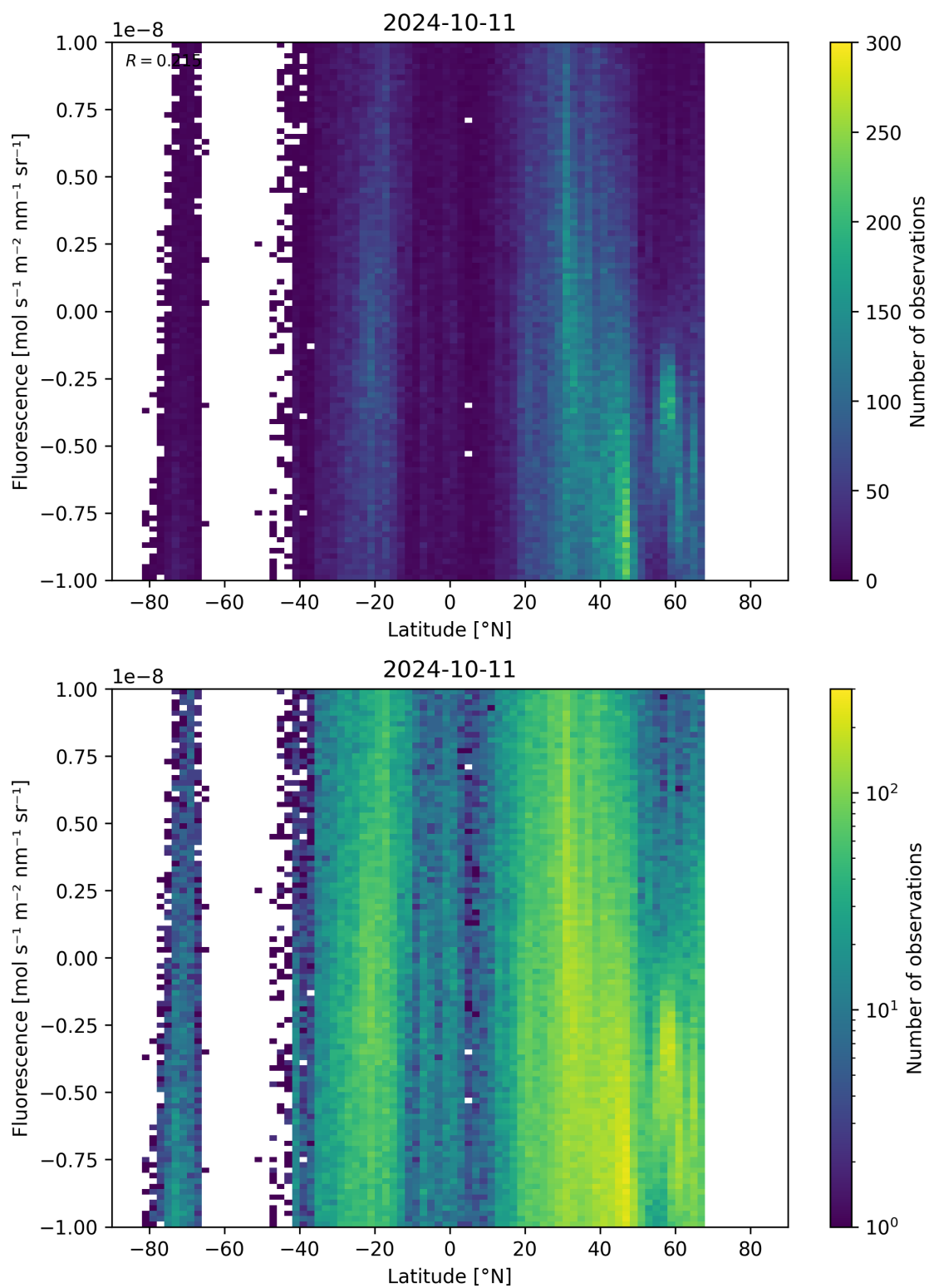
Figure 56: Scatter density plot of “Latitude” against “Fluorescence” for 2024-10-10 to 2024-10-12.
