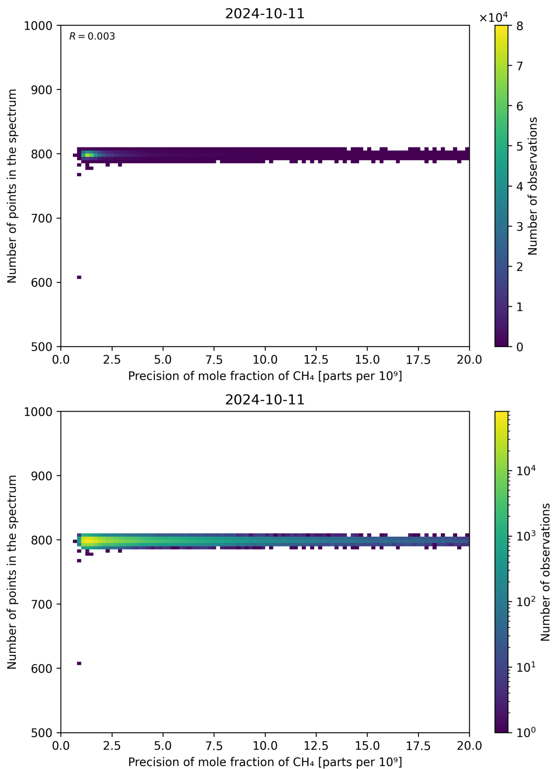
Figure 84: Scatter density plot of “Precision of mole fraction of CH 4 ” against “Number of points in the spectrum” for 2024-10-10 to 2024-10-12.
