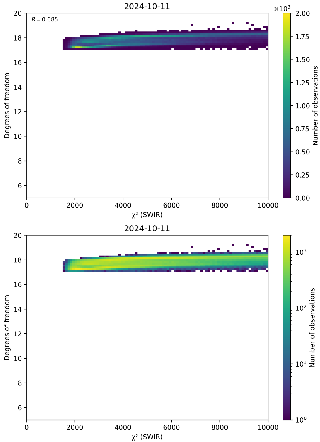
Figure 48: Scatter density plot of “ \chi^2 (SWIR)” against “Degrees of freedom” for 2024-10-10 to 2024-10-12.
