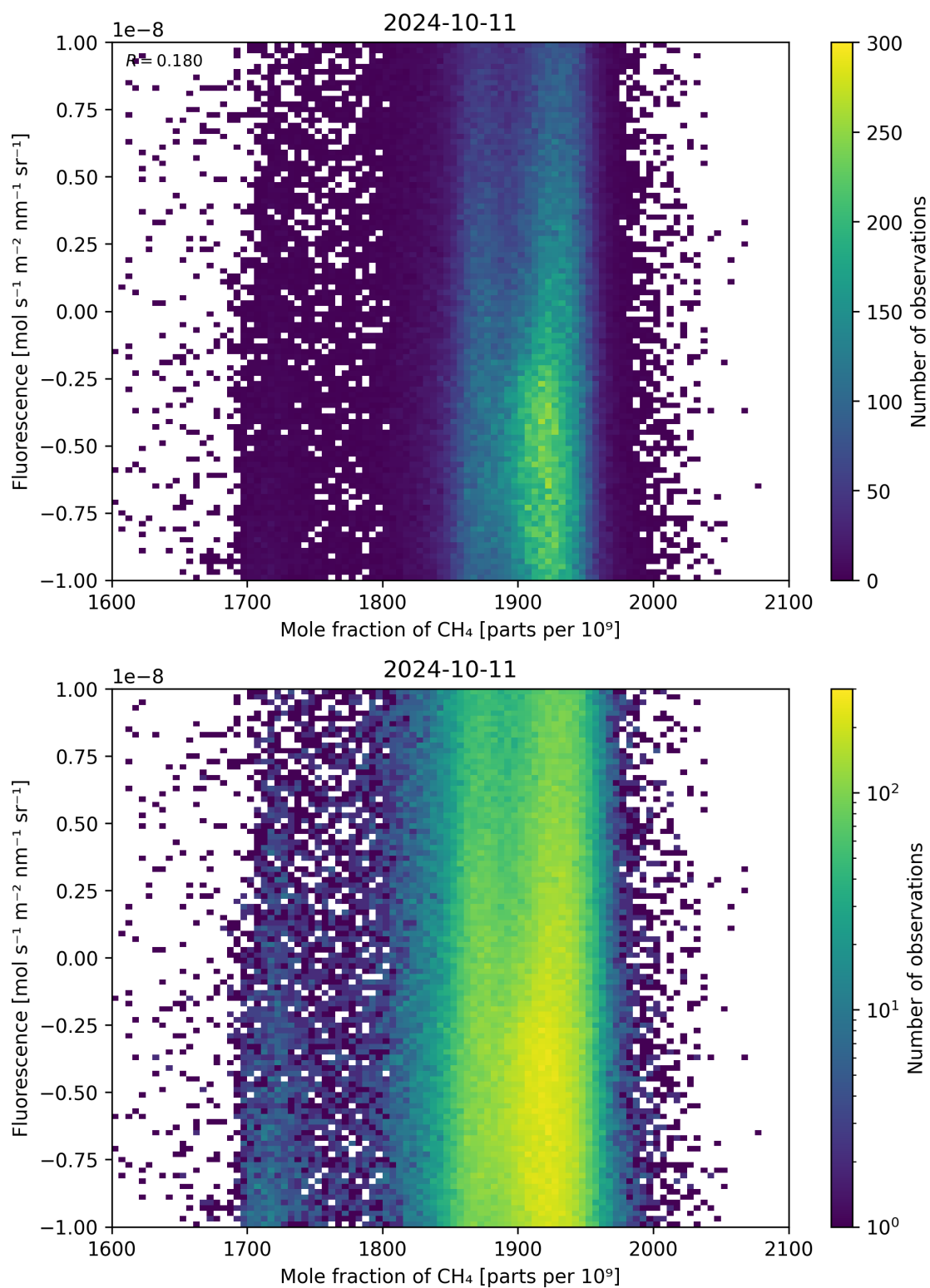
Figure 73: Scatter density plot of “Mole fraction of \text{CH}_4 ” against “Fluorescence” for 2024-10-10 to 2024-10-12.
