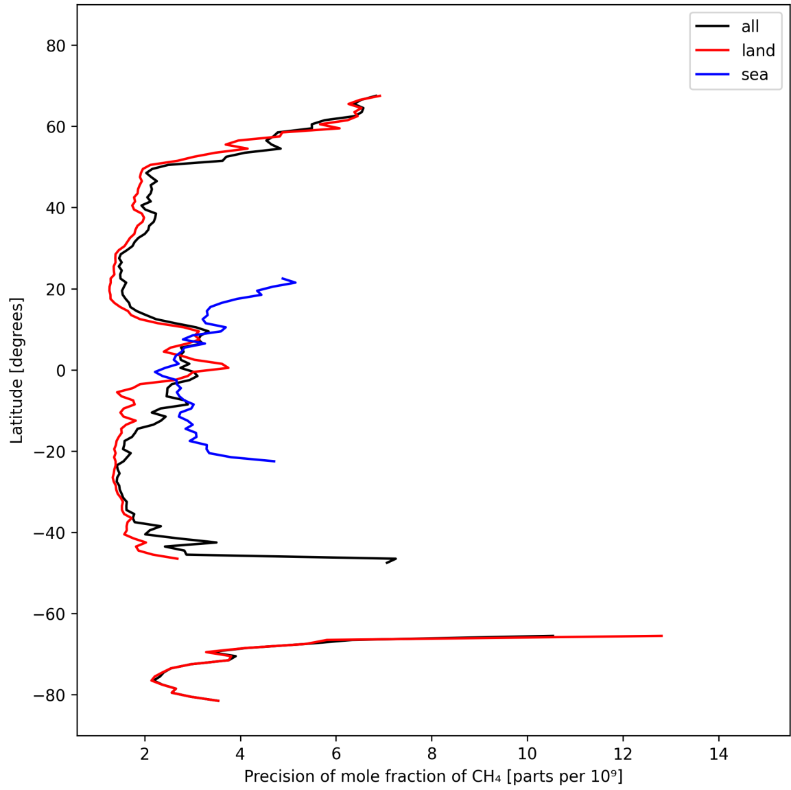
Figure 13: Zonal average of “Precision of mole fraction of CH 4 ” for 2024-10-10 to 2024-10-12.
