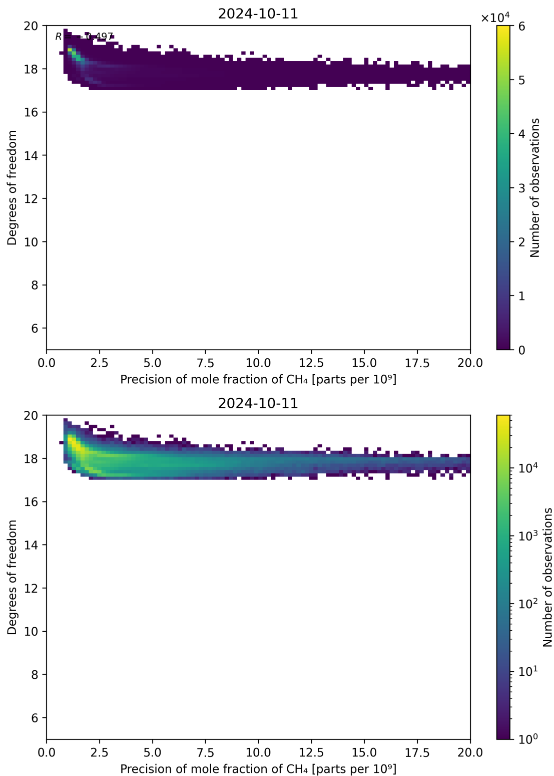
Figure 80: Scatter density plot of “Precision of mole fraction of CH 4 ” against “Degrees of freedom” for 2024-10-10 to 2024-10-12.
