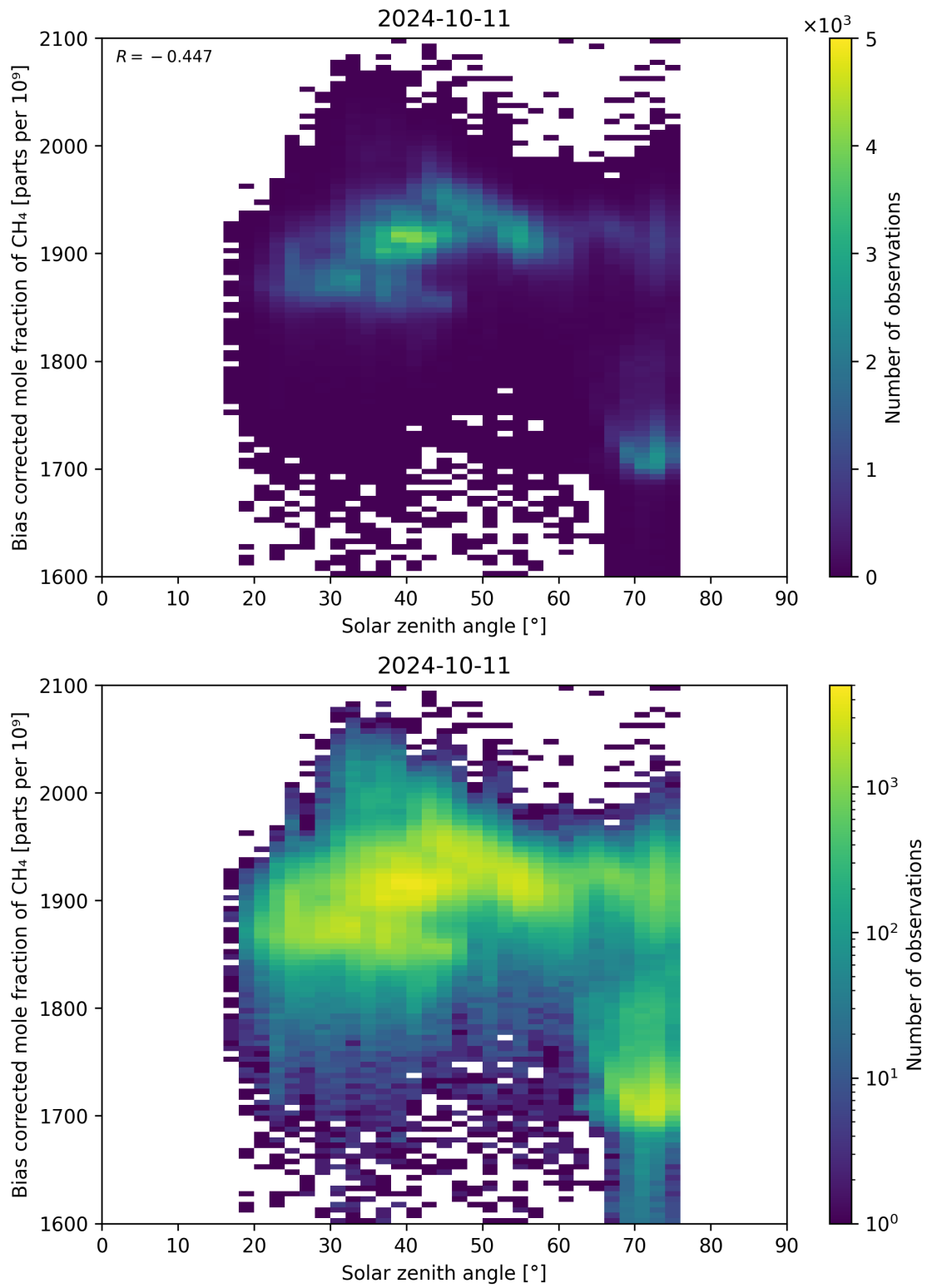
Figure 100: Scatter density plot of “Solar zenith angle” against “Bias corrected mole fraction of CH 4 ” for 2024-10-10 to 2024-10-12.
