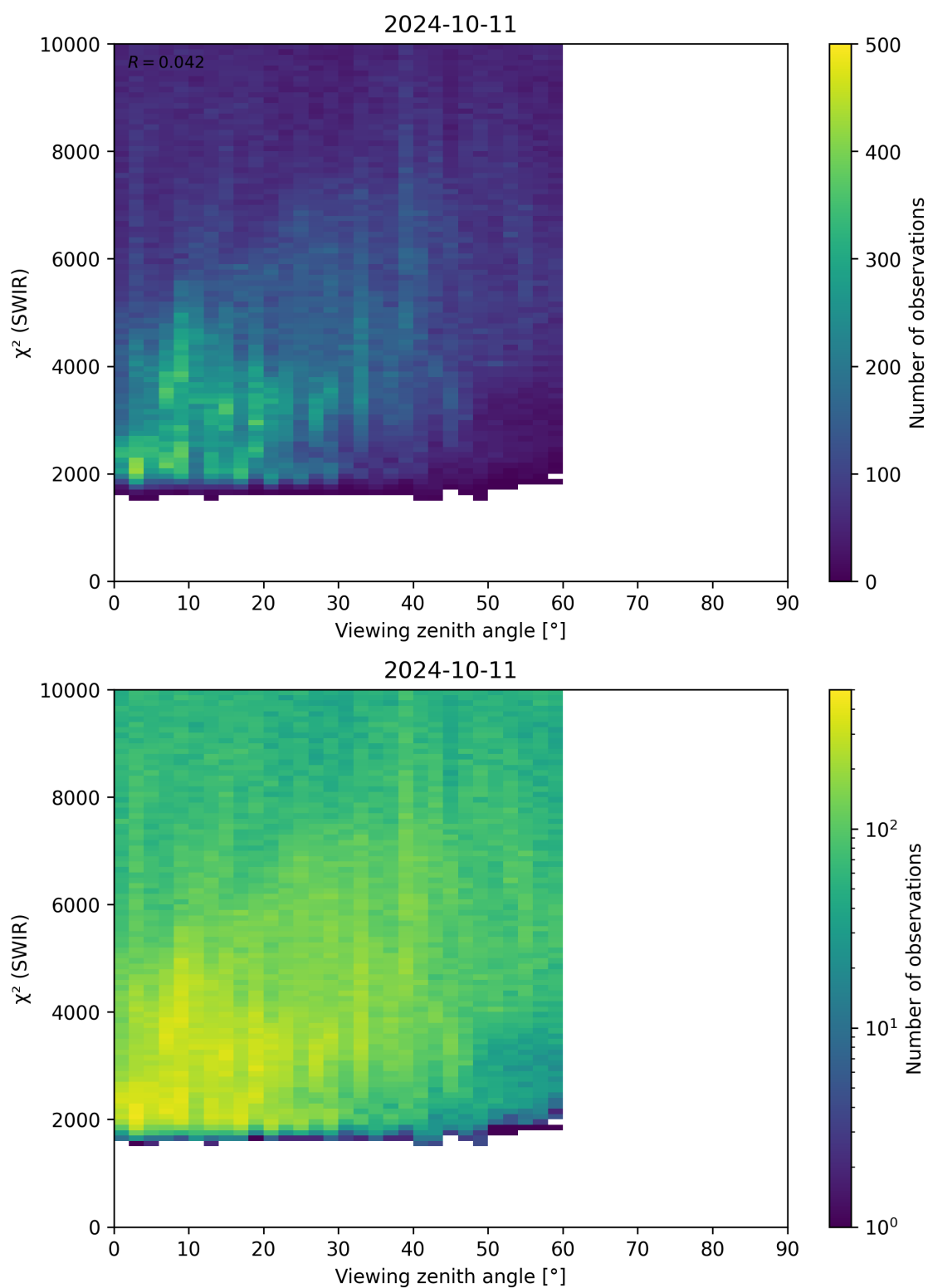
Figure 106: Scatter density plot of “Viewing zenith angle” against “ \chi^2 (SWIR)” for 2024-10-10 to 2024-10-12.
