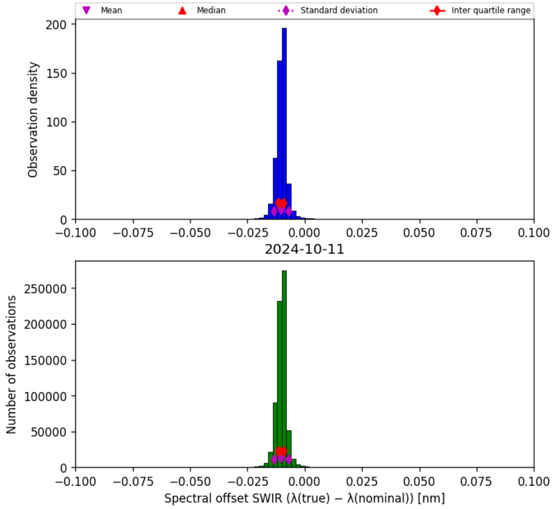
Figure 27: Histogram of “Spectral offset SWIR ( \lambda_{\text{true}} - \lambda_{\text{nominal}} )” for 2024-10-10 to 2024-10-12
