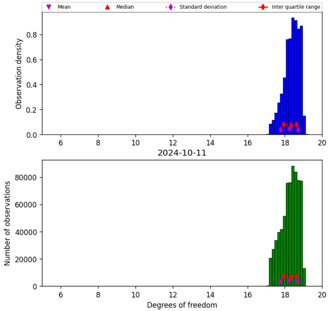
Figure 30: Histogram of “Degrees of freedom” for 2024-10-10 to 2024-10-12
