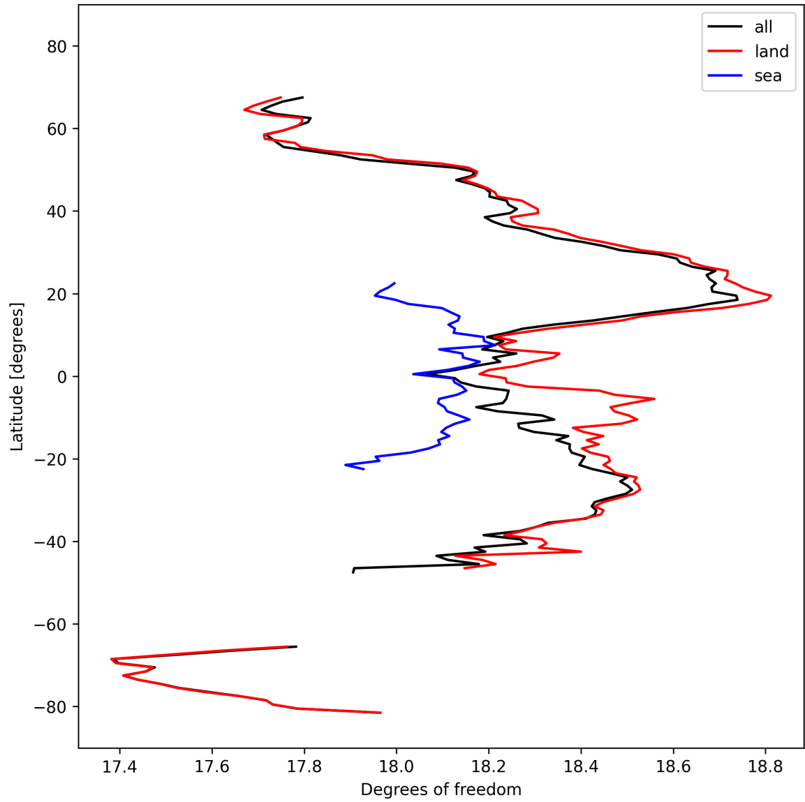
Figure 19: Zonal average of “Degrees of freedom” for 2024-10-10 to 2024-10-12.
