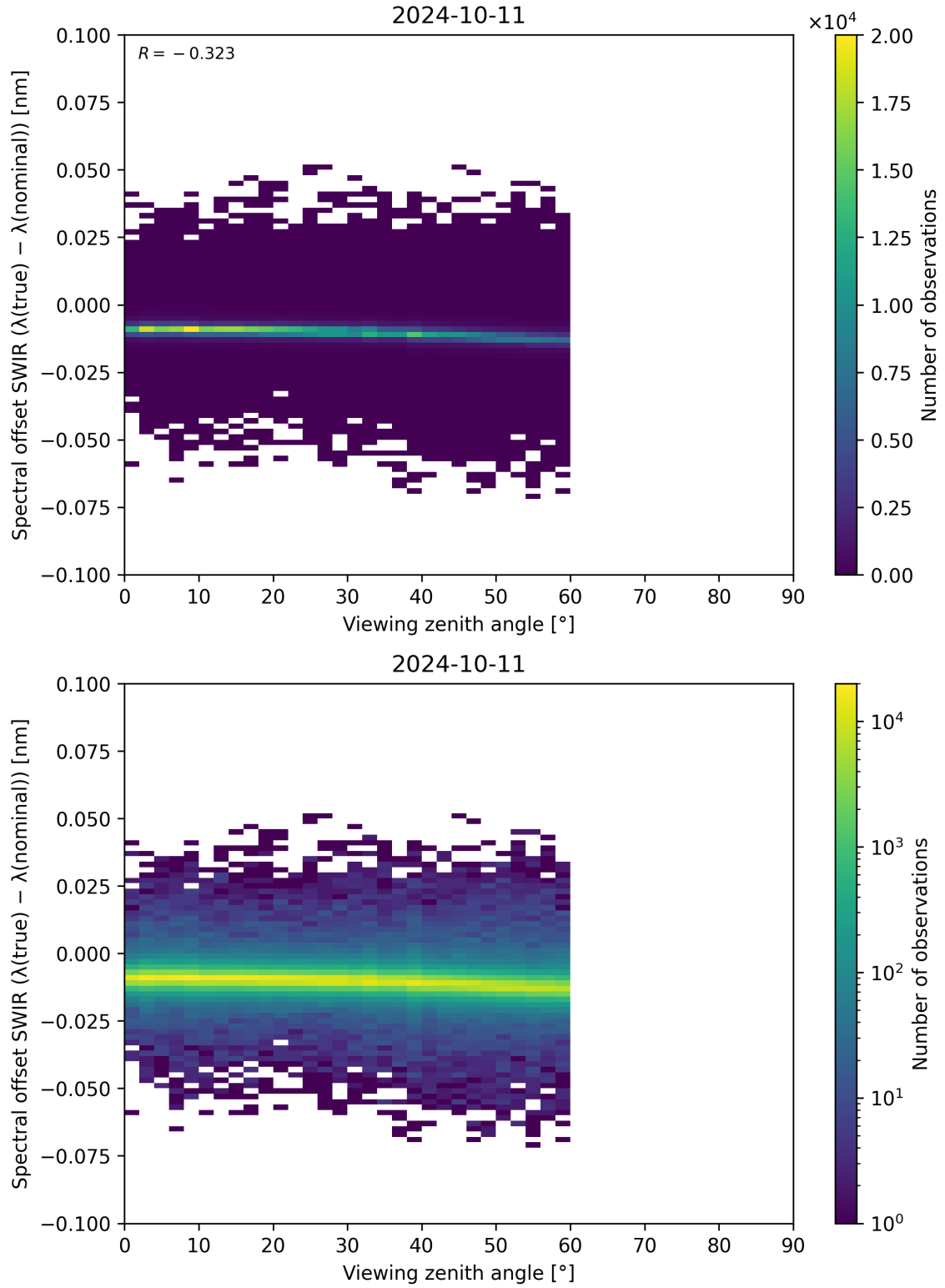
Figure 116: Scatter density plot of “Viewing zenith angle” against “Spectral offset SWIR ( \lambda_{\text{true}} - \lambda_{\text{nominal}} )” for 2024-10-10 to 2024-10-12.
