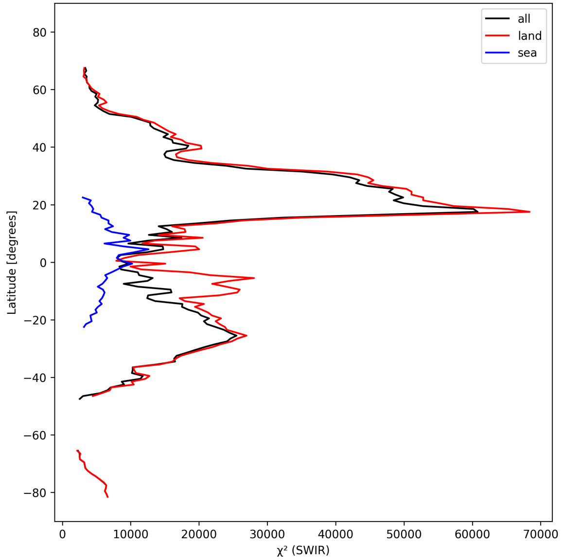
Figure 17: Zonal average of “ \chi^2 (SWIR)” for 2024-10-10 to 2024-10-12.
