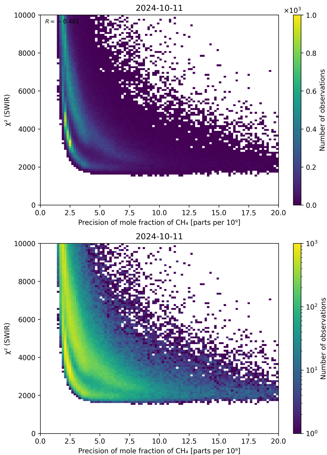
Figure 79: Scatter density plot of “Precision of mole fraction of \text{CH}_4 ” against “ \chi^2 (SWIR)” for 2024-10-10 to 2024-10-12.
