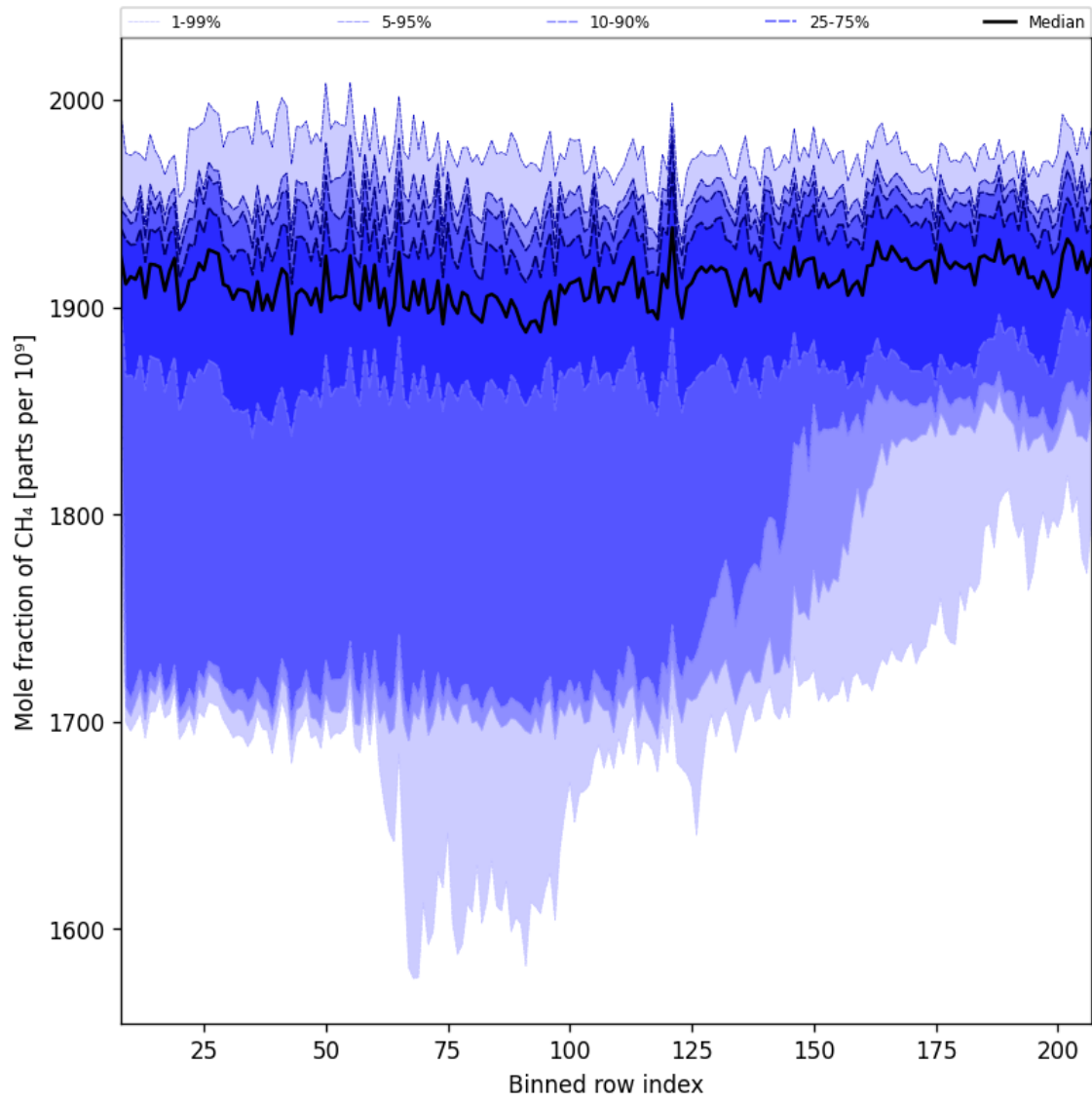
Figure 34: Along track statistics of “Mole fraction of CH 4 ” for 2024-10-10 to 2024-10-12
