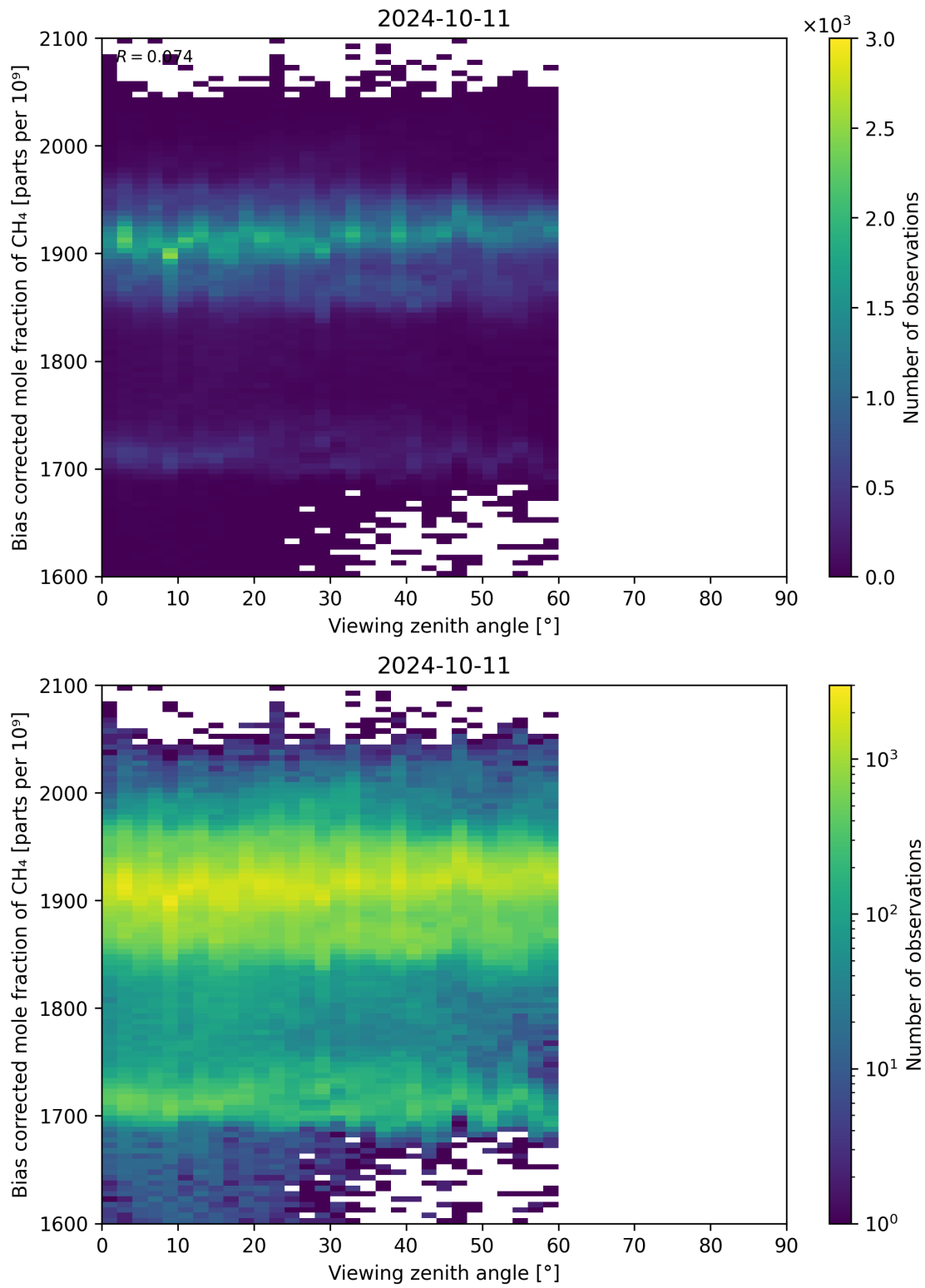
Figure 111: Scatter density plot of “Viewing zenith angle” against “Bias corrected mole fraction of CH 4 ” for 2024-10-10 to 2024-10-12.
