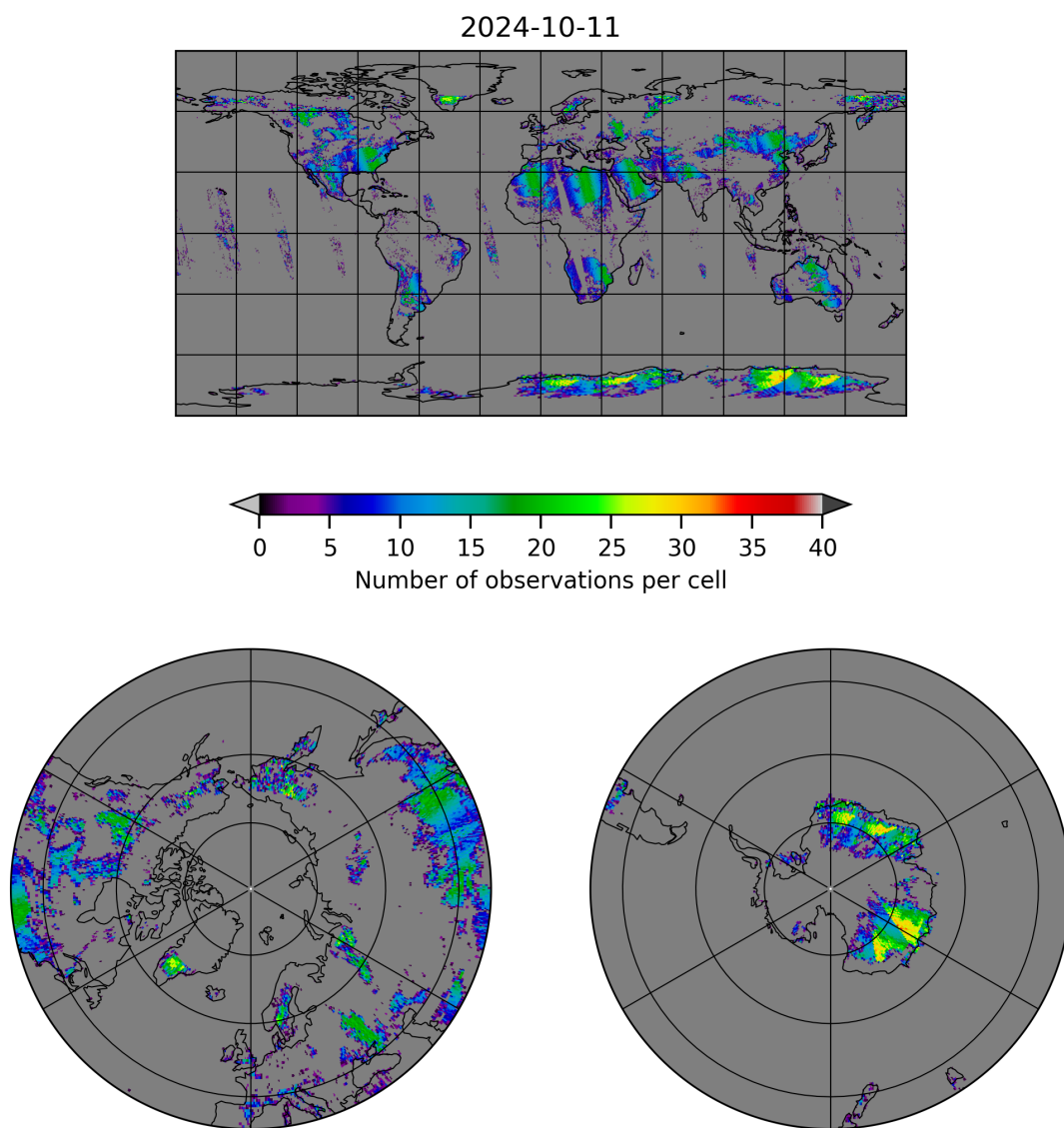
Figure 10: Map of the number of observations for 2024-10-10 to 2024-10-12
