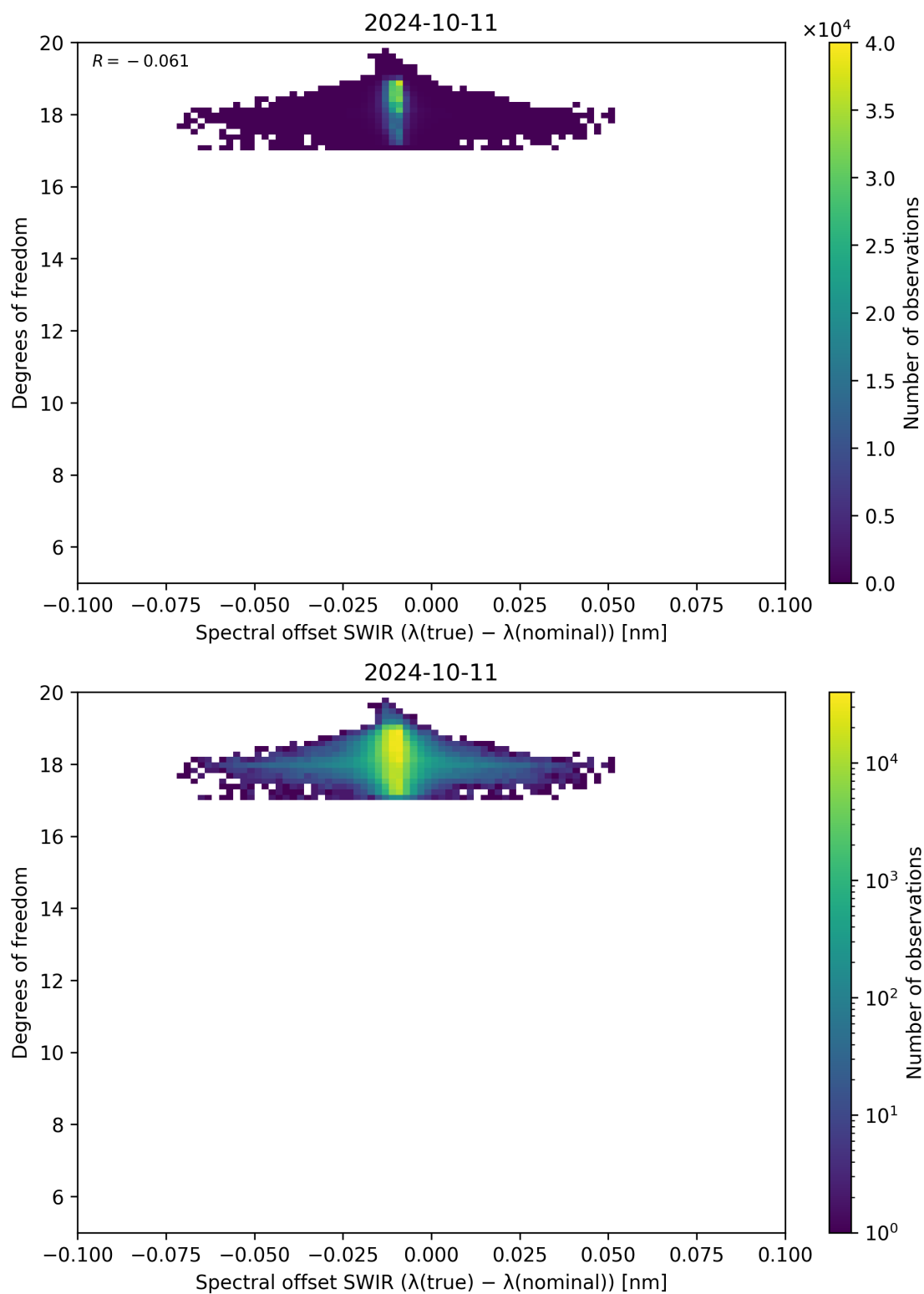
Figure 119: Scatter density plot of “Spectral offset SWIR ( \lambda_{\text{true}} - \lambda_{\text{nominal}} )” against “Degrees of freedom” for 2024-10-10 to 2024-10-12.
