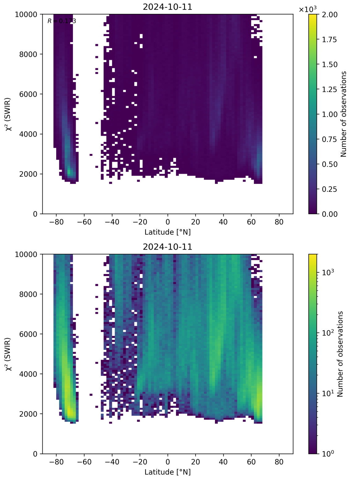
Figure 54: Scatter density plot of “Latitude” against “ \chi^2 (SWIR)” for 2024-10-10 to 2024-10-12.
