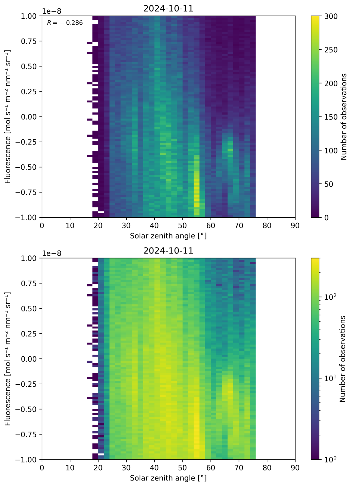
Figure 97: Scatter density plot of “Solar zenith angle” against “Fluorescence” for 2024-10-10 to 2024-10-12.
