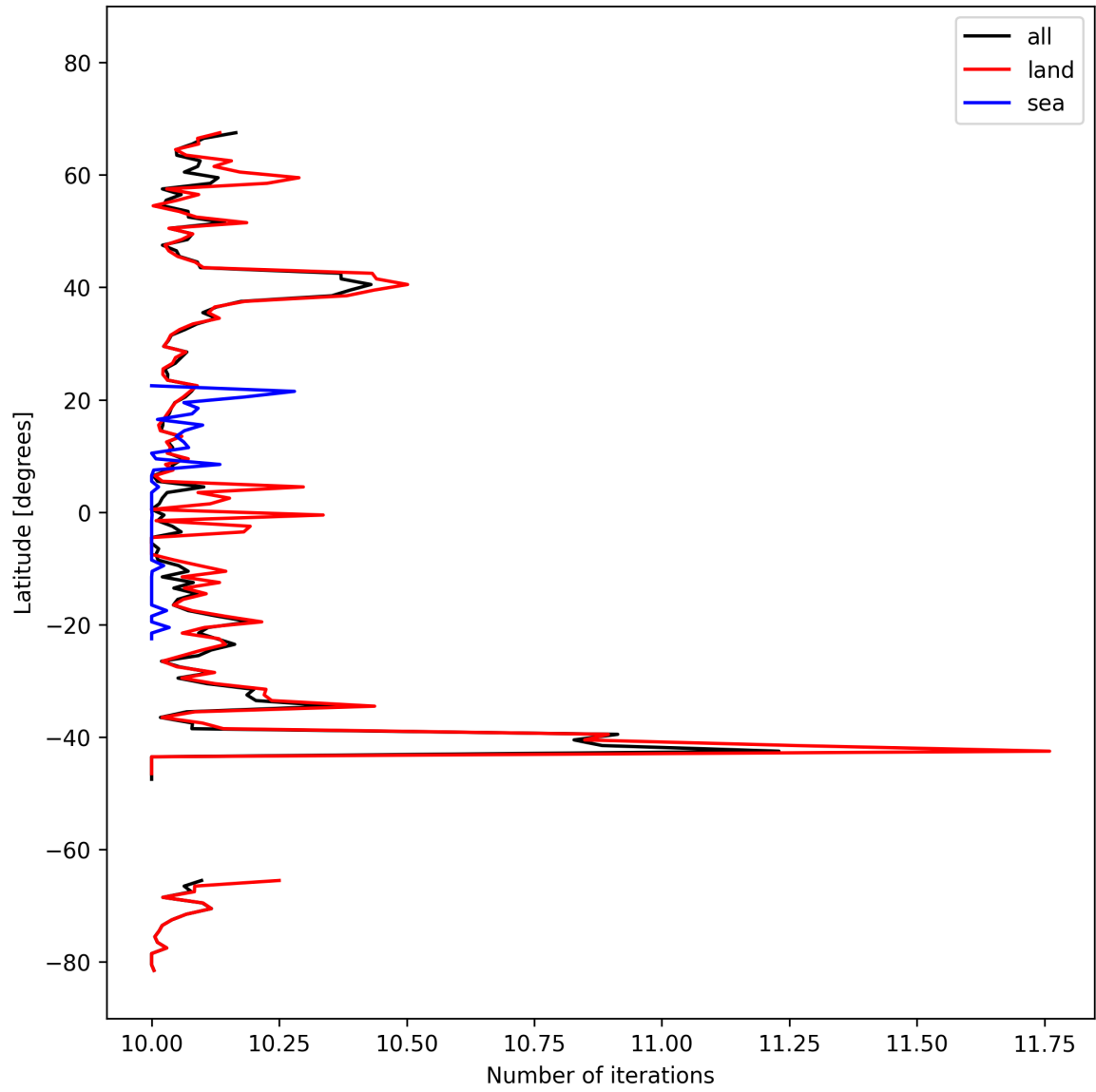
Figure 20: Zonal average of “Number of iterations” for 2024-10-10 to 2024-10-12.
