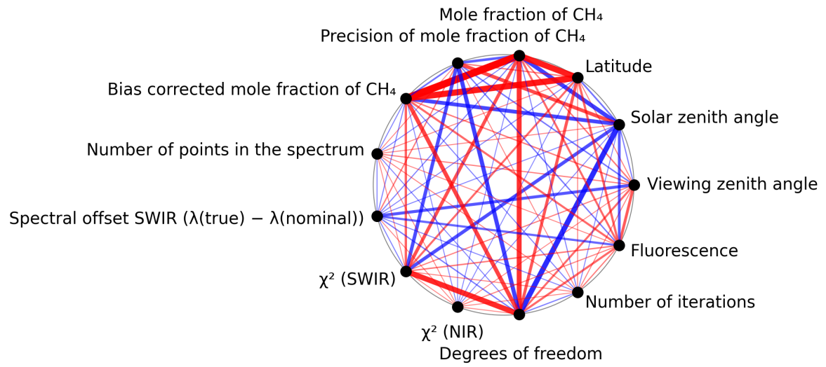
Figure 1: Map of correlation graph for 2024-10-10 to 2024-10-12.
