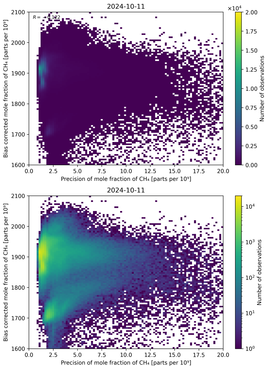
Figure 82: Scatter density plot of “Precision of mole fraction of CH 4 ” against “Bias corrected mole fraction of CH 4 ” for 2024-10-10 to 2024-10-12.
