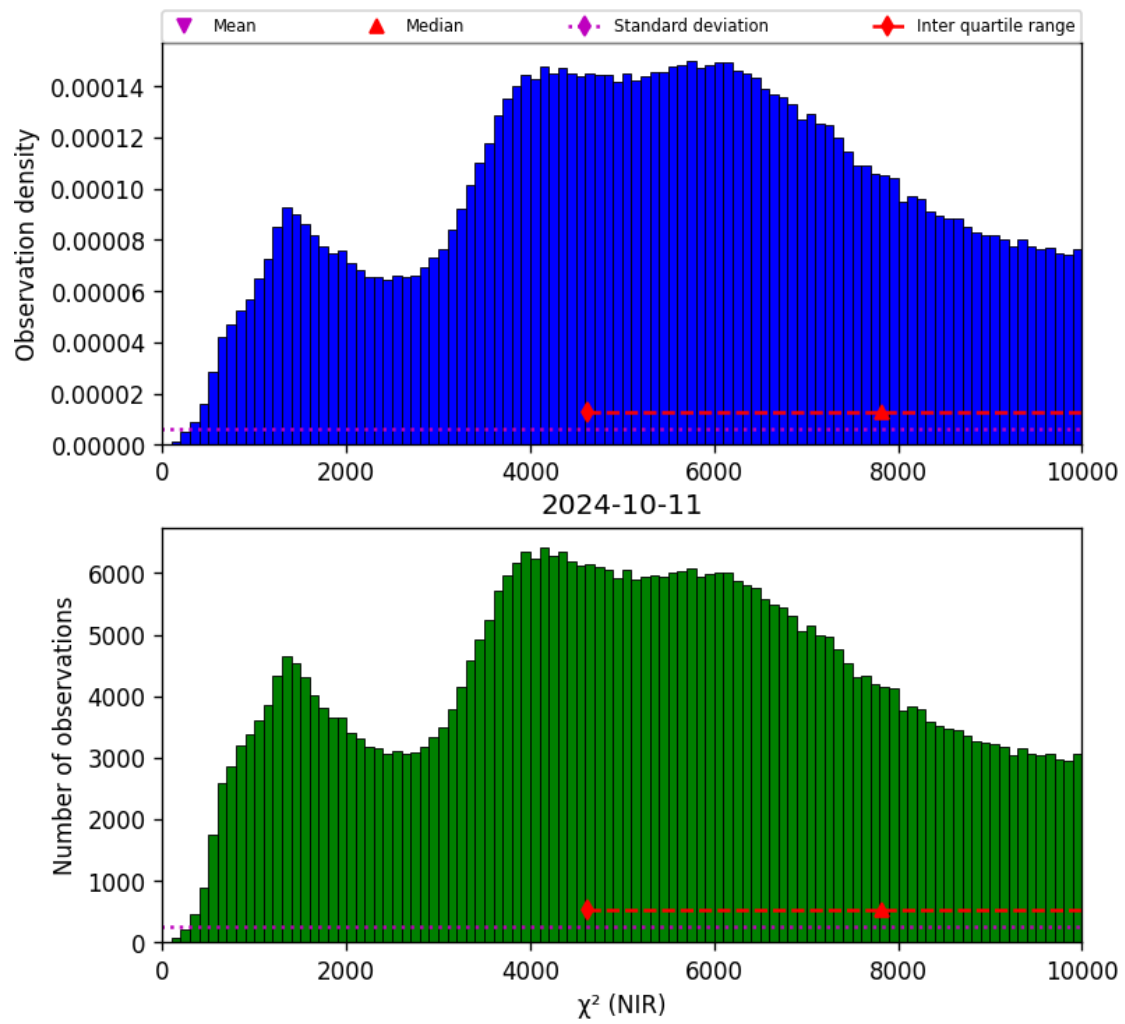
Figure 29: Histogram of “ \chi^2 (NIR)” for 2024-10-10 to 2024-10-12
