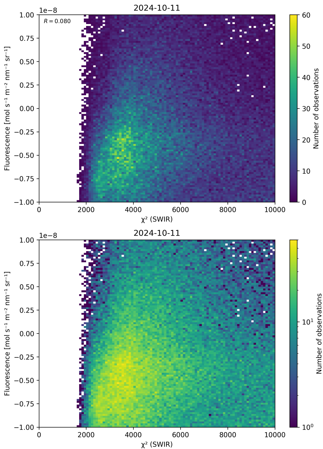
Figure 49: Scatter density plot of “ \chi^2 (SWIR)” against “Fluorescence” for 2024-10-10 to 2024-10-12.
