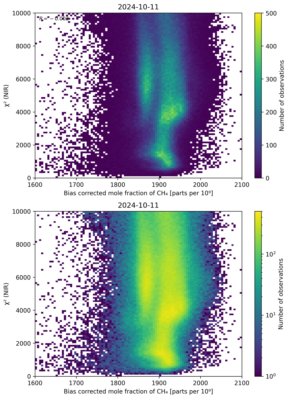
Figure 63: Scatter density plot of “Bias corrected mole fraction of CH 4 ” against “ \chi^2 (NIR)” for 2024-10-10 to 2024-10-12.
