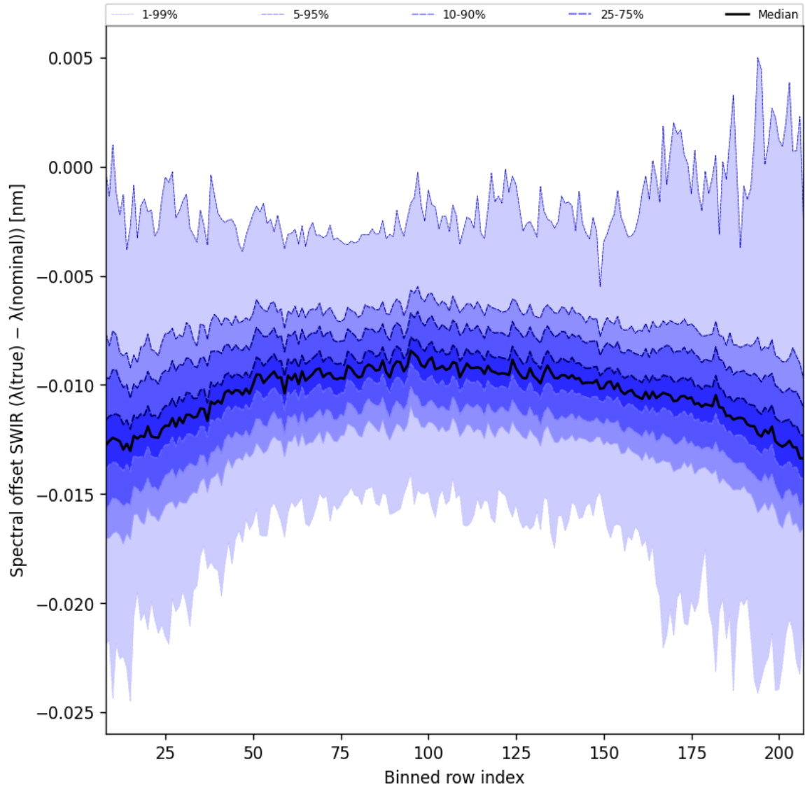
Figure 38: Along track statistics of “Spectral offset SWIR ( \lambda_{\text{true}} - \lambda_{\text{nominal}} )” for 2024-10-10 to 2024-10-12
