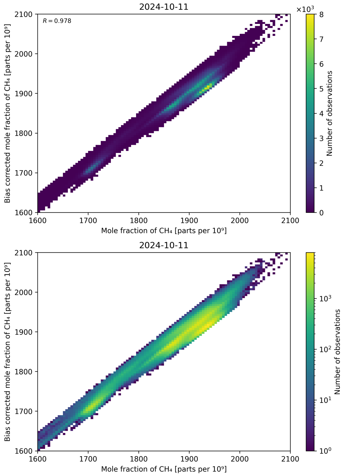
Figure 74: Scatter density plot of “Mole fraction of CH 4 ” against “Bias corrected mole fraction of CH 4 ” for 2024-10-10 to 2024-10-12.
