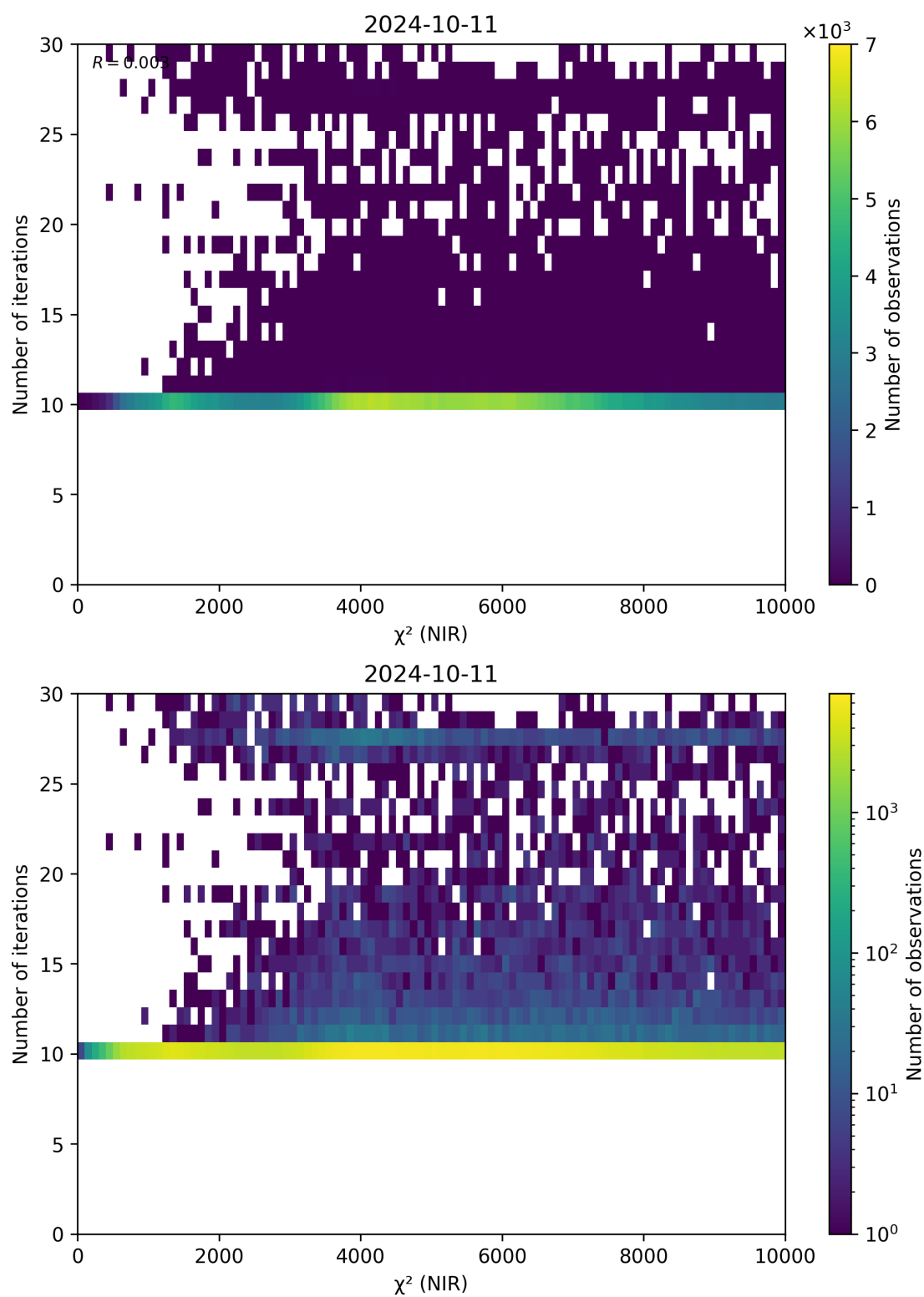
Figure 46: Scatter density plot of “ \chi^2 (NIR)” against “Number of iterations” for 2024-10-10 to 2024-10-12.
