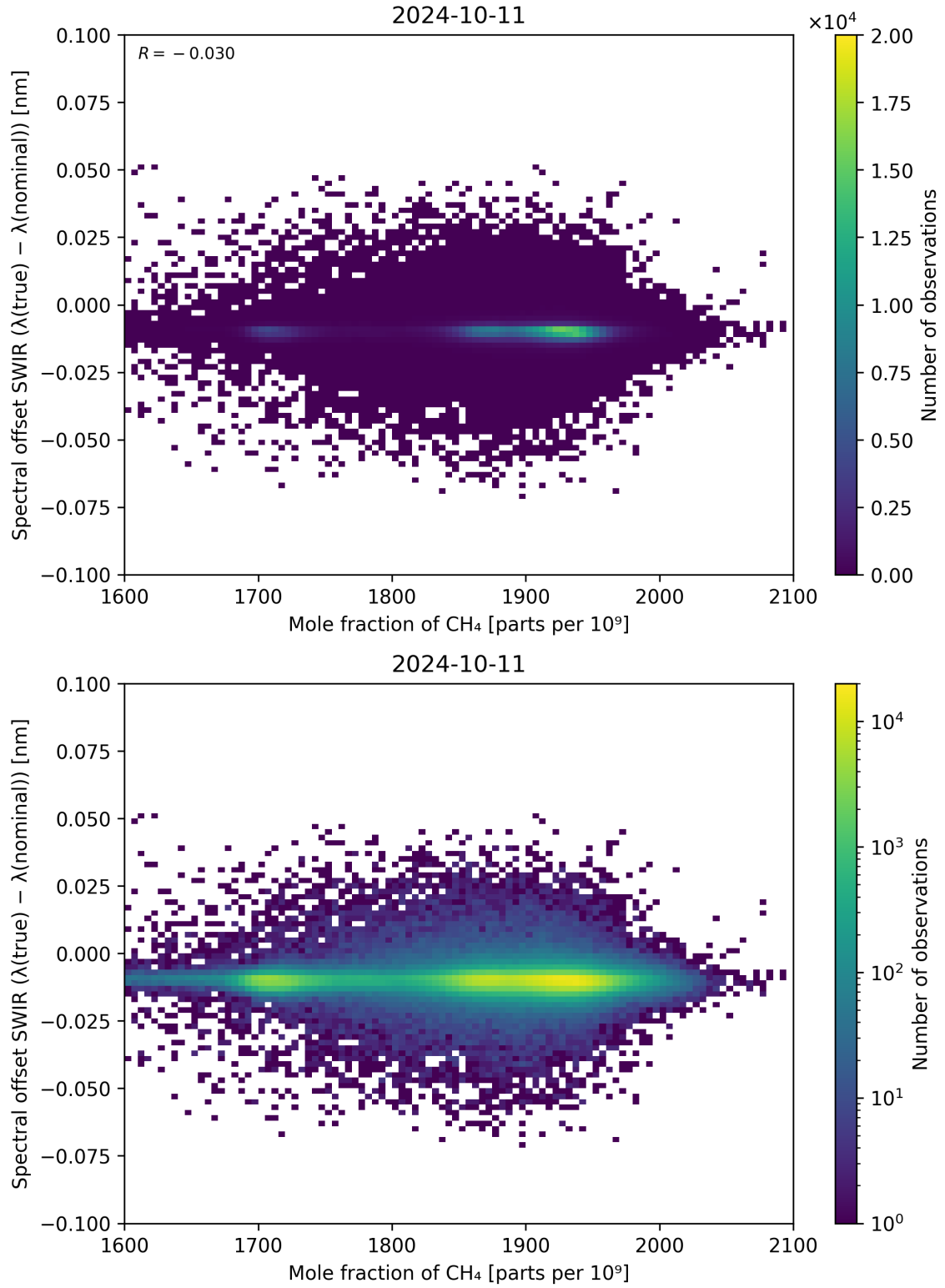
Figure 86: Scatter density plot of “Mole fraction of CH 4 ” against “Spectral offset SWIR ( \lambda_{\text{true}} - \lambda_{\text{nominal}} )” for 2024-10-10 to 2024-10-12.
