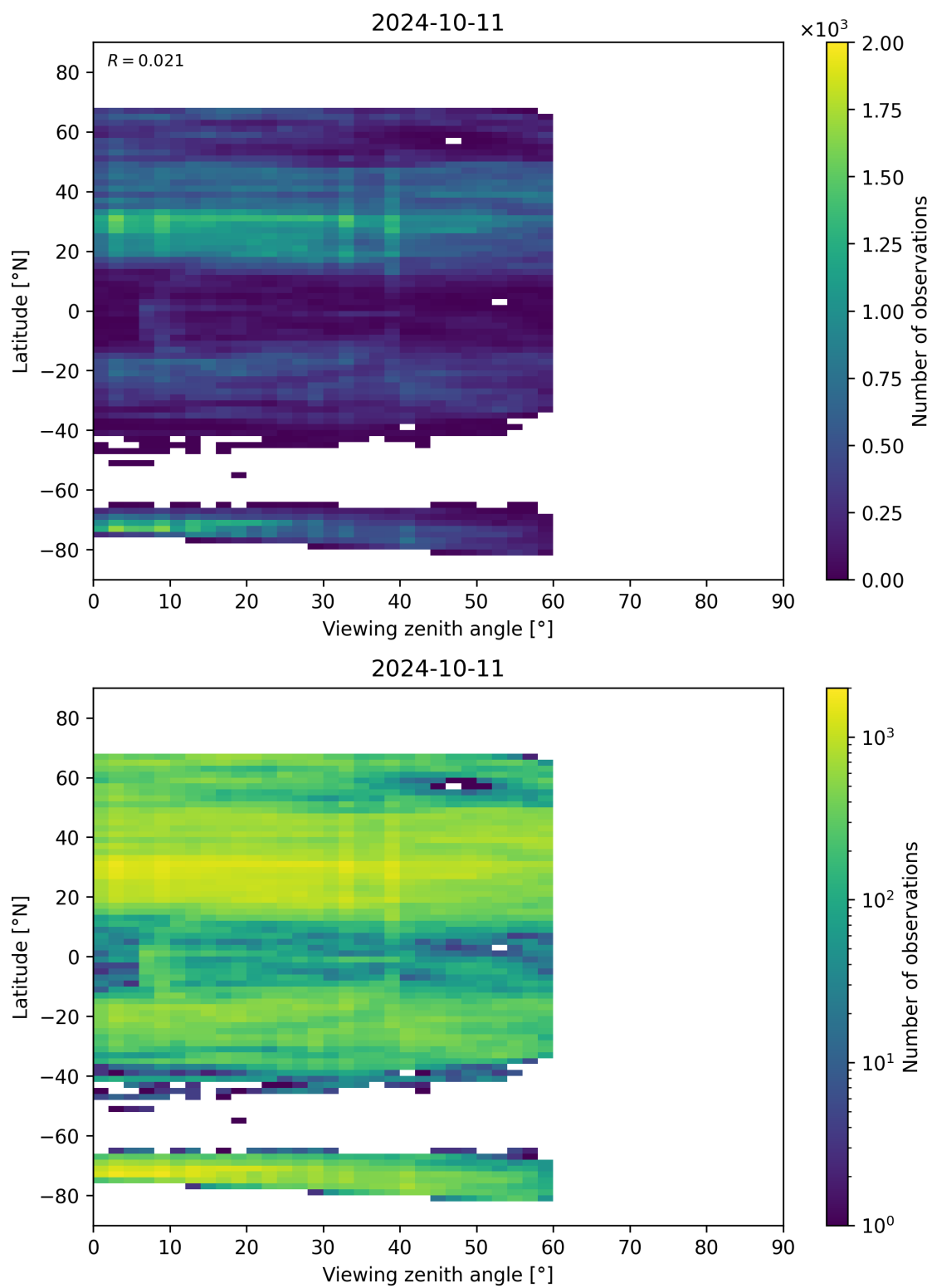
Figure 109: Scatter density plot of “Viewing zenith angle” against “Latitude” for 2024-10-10 to 2024-10-12.
