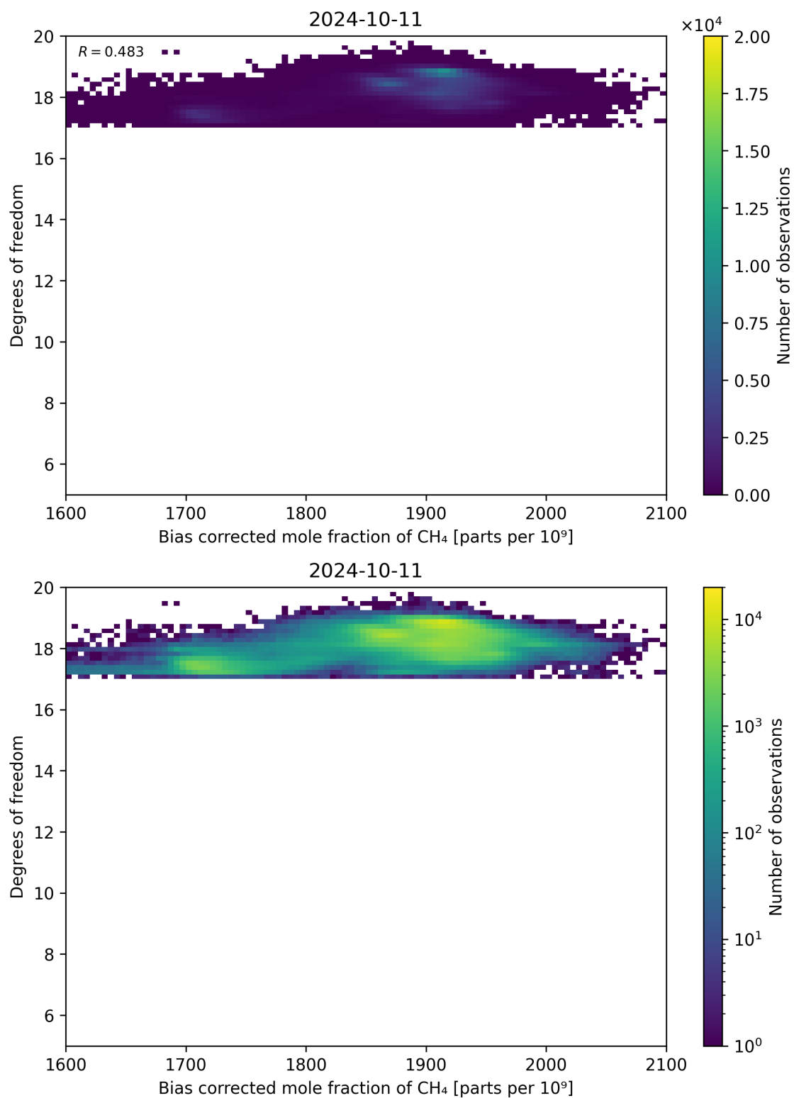
Figure 65: Scatter density plot of “Bias corrected mole fraction of CH 4 ” against “Degrees of freedom” for 2024-10-10 to 2024-10-12.
