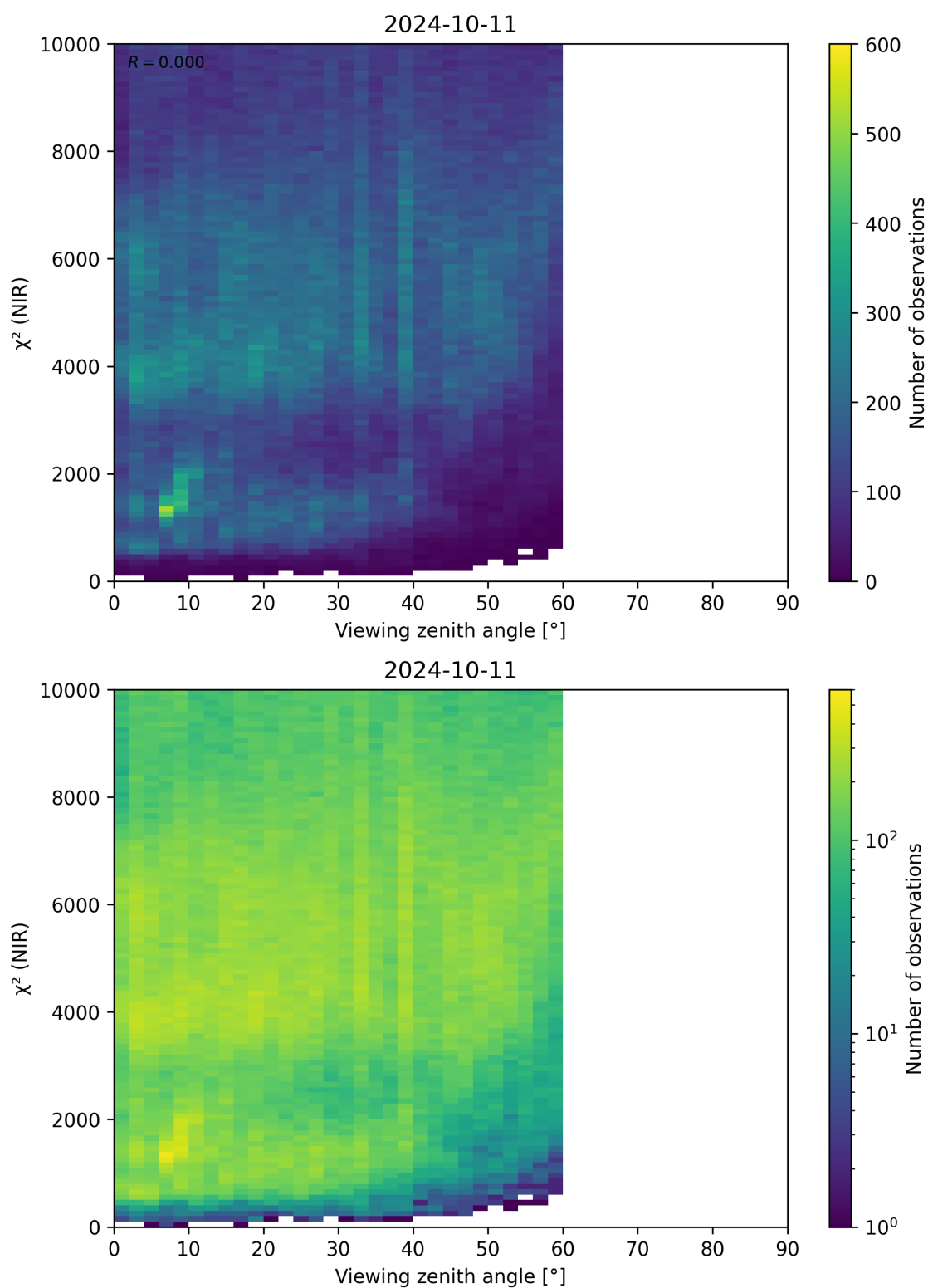
Figure 105: Scatter density plot of “Viewing zenith angle” against “ \chi^2 (NIR)” for 2024-10-10 to 2024-10-12.
