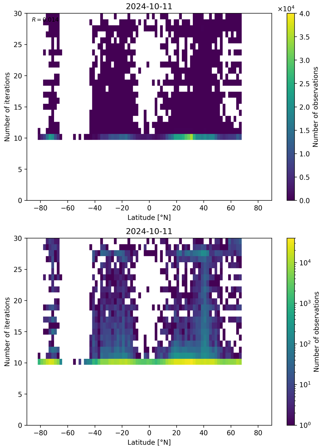
Figure 60: Scatter density plot of “Latitude” against “Number of iterations” for 2024-10-10 to 2024-10-12.
