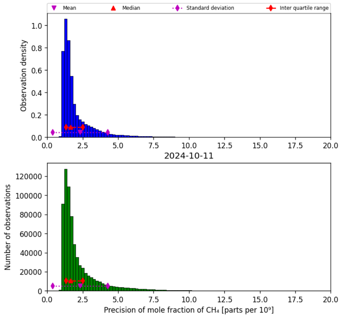
Figure 24: Histogram of “Precision of mole fraction of CH 4 ” for 2024-10-10 to 2024-10-12
