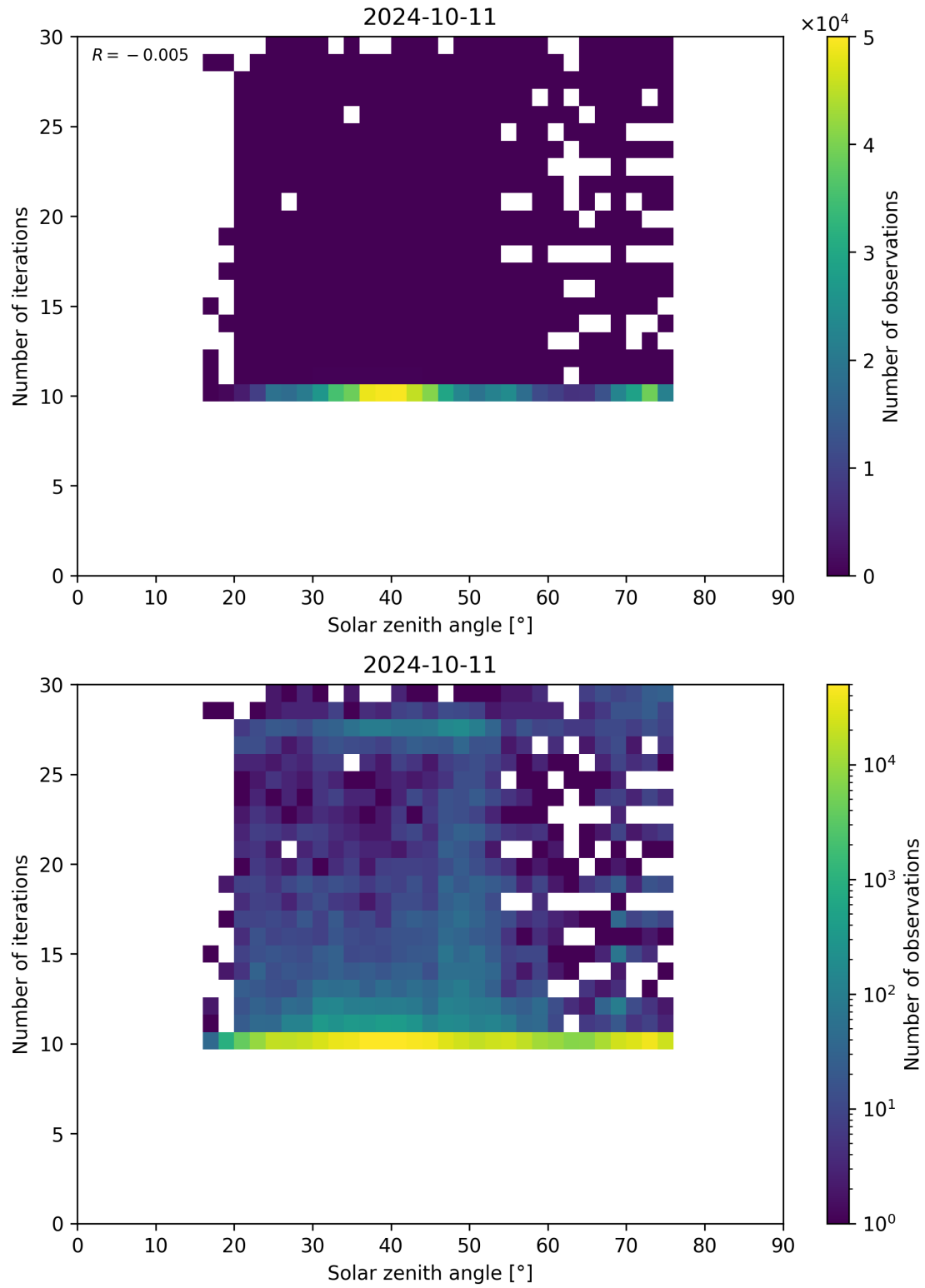
Figure 102: Scatter density plot of “Solar zenith angle” against “Number of iterations” for 2024-10-10 to 2024-10-12.
