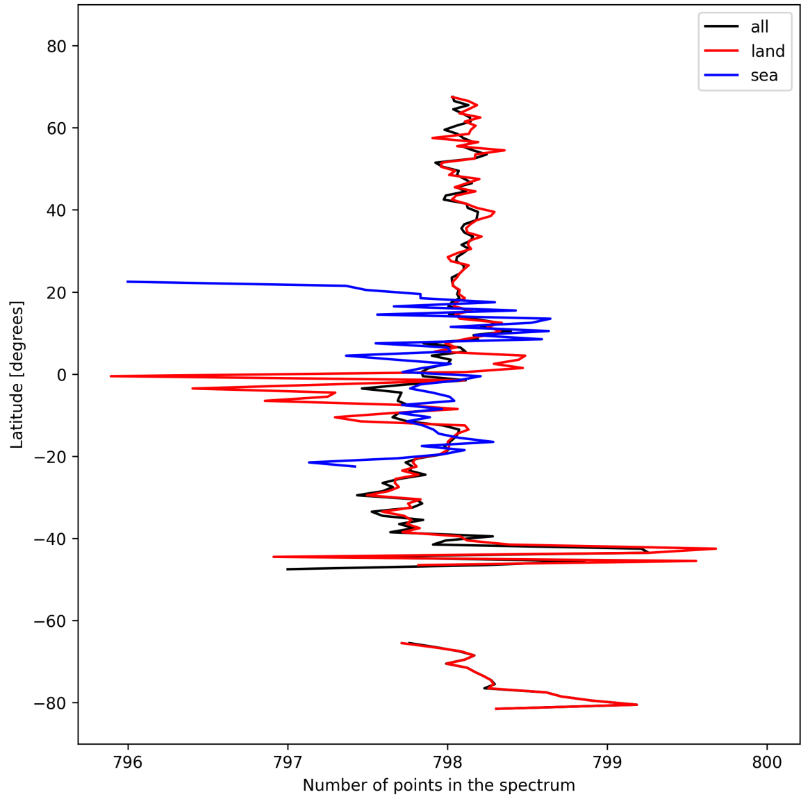
Figure 15: Zonal average of “Number of points in the spectrum” for 2024-10-10 to 2024-10-12.
