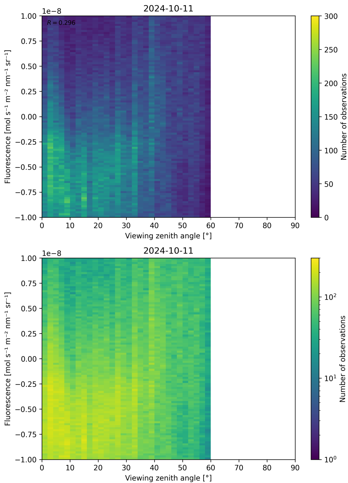
Figure 108: Scatter density plot of “Viewing zenith angle” against “Fluorescence” for 2024-10-10 to 2024-10-12.
