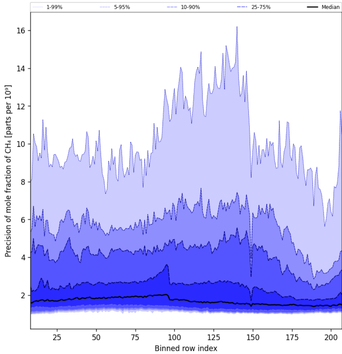
Figure 35: Along track statistics of “Precision of mole fraction of CH 4 ” for 2024-10-10 to 2024-10-12
