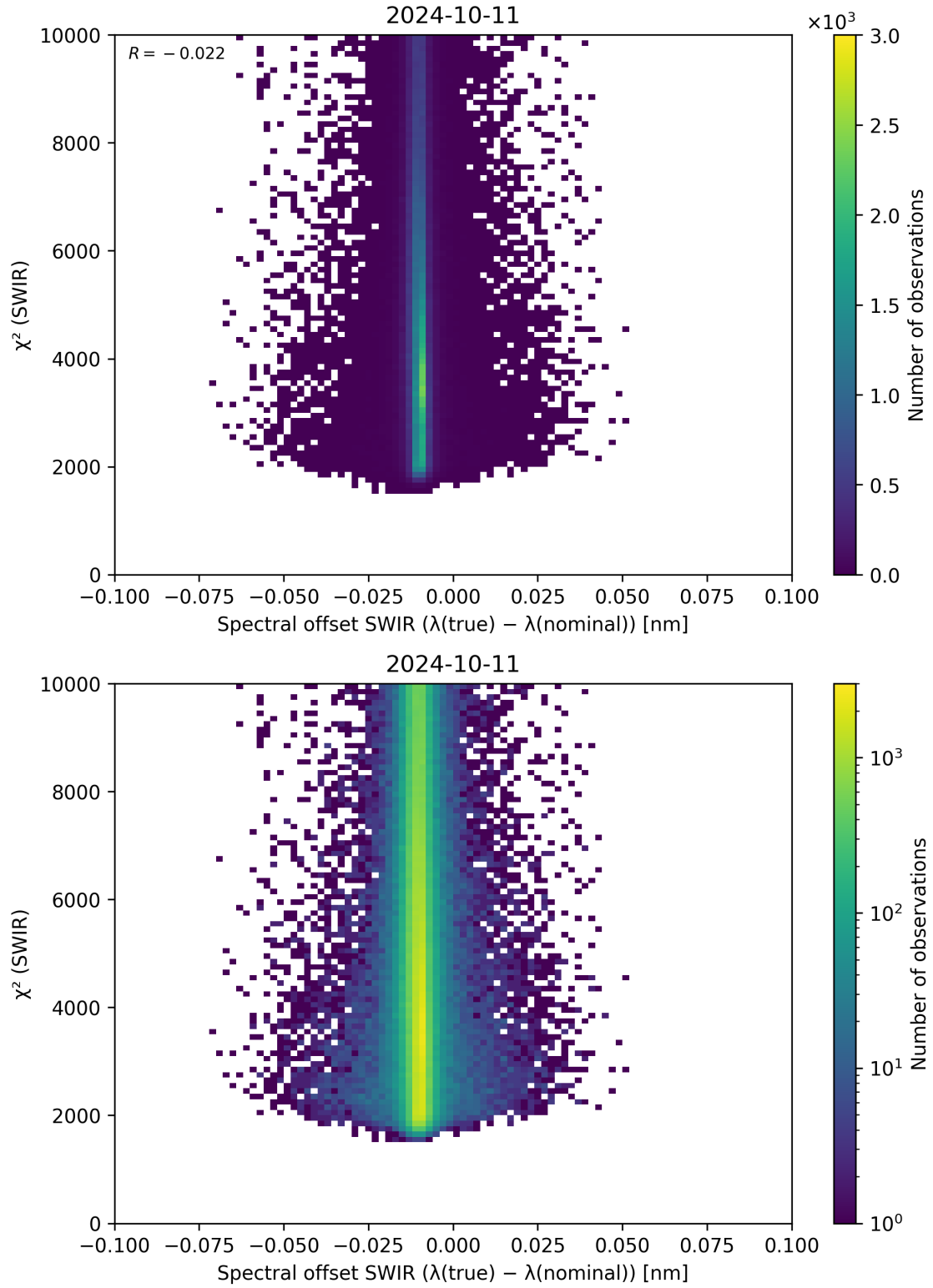
Figure 118: Scatter density plot of “Spectral offset SWIR ( \lambda_{\text{true}} - \lambda_{\text{nominal}} )” against “ \chi^2 (SWIR)” for 2024-10-10 to 2024-10-12.
