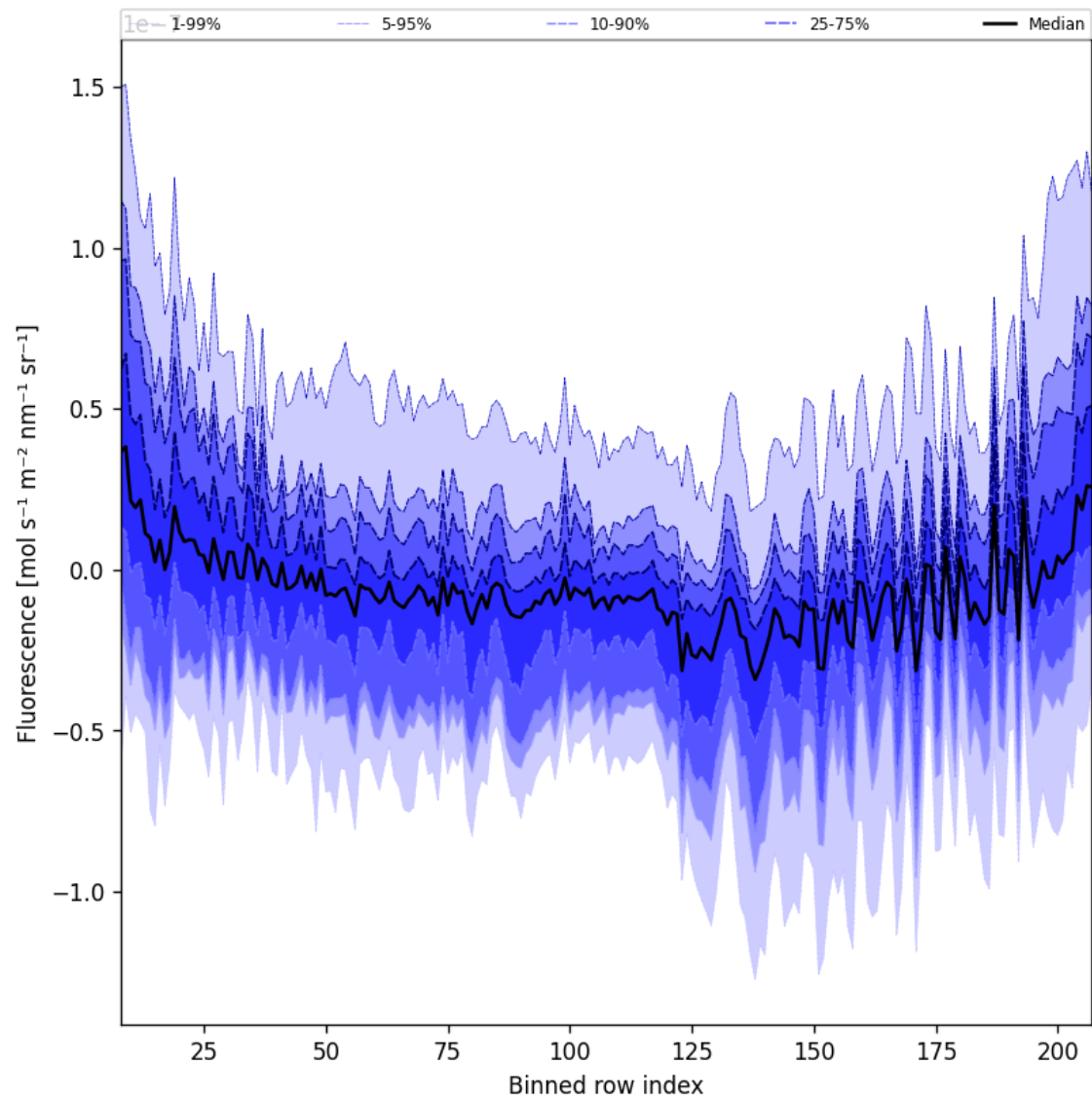
Figure 43: Along track statistics of “Fluorescence” for 2024-10-10 to 2024-10-12
