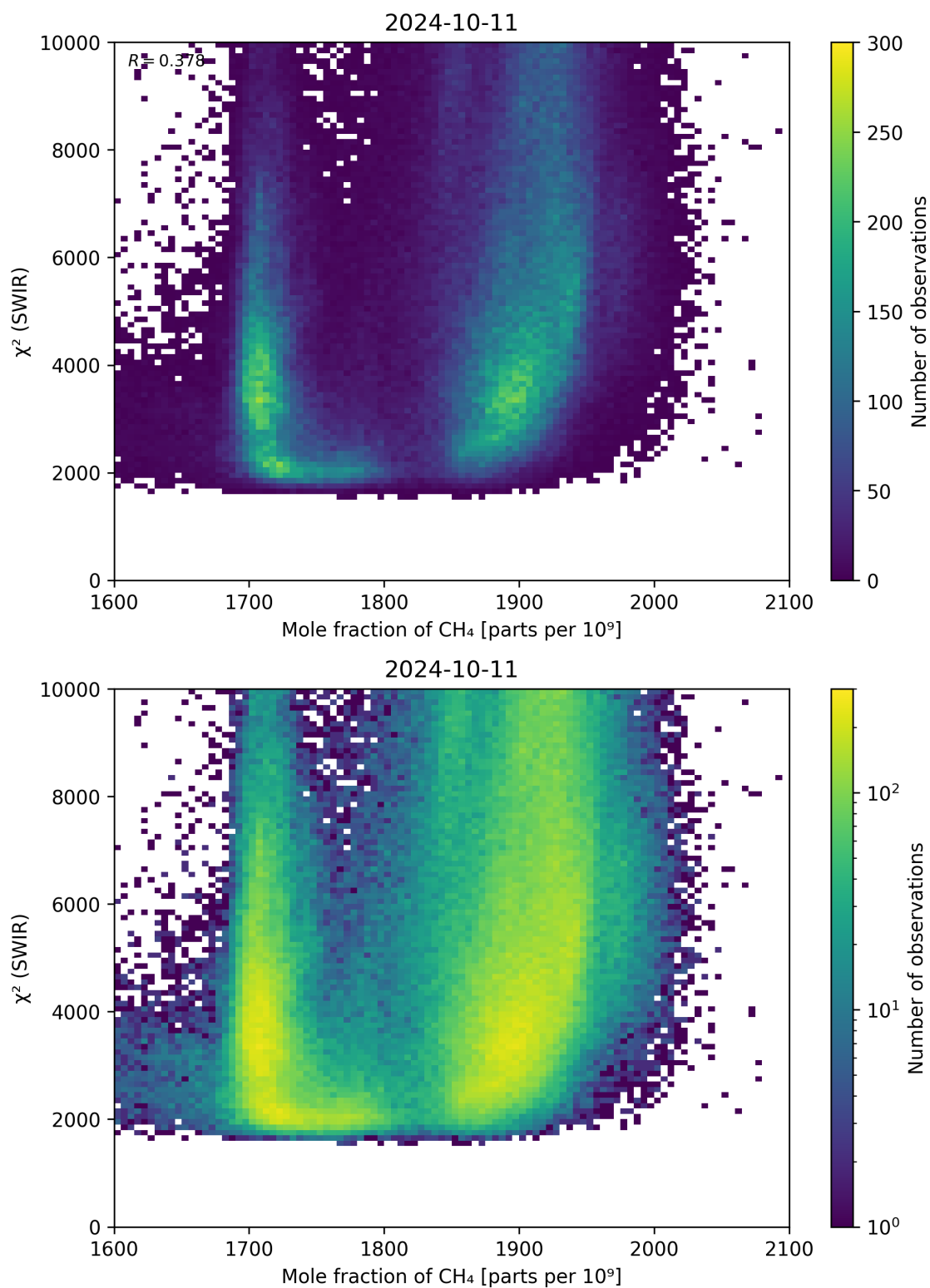
Figure 71: Scatter density plot of “Mole fraction of \text{CH}_4 ” against “ \chi^2 (SWIR)” for 2024-10-10 to 2024-10-12.
