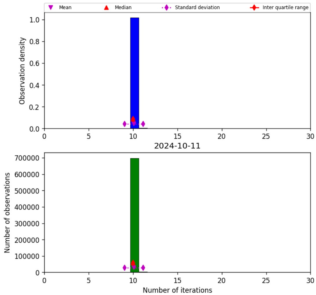
Figure 31: Histogram of “Number of iterations” for 2024-10-10 to 2024-10-12
