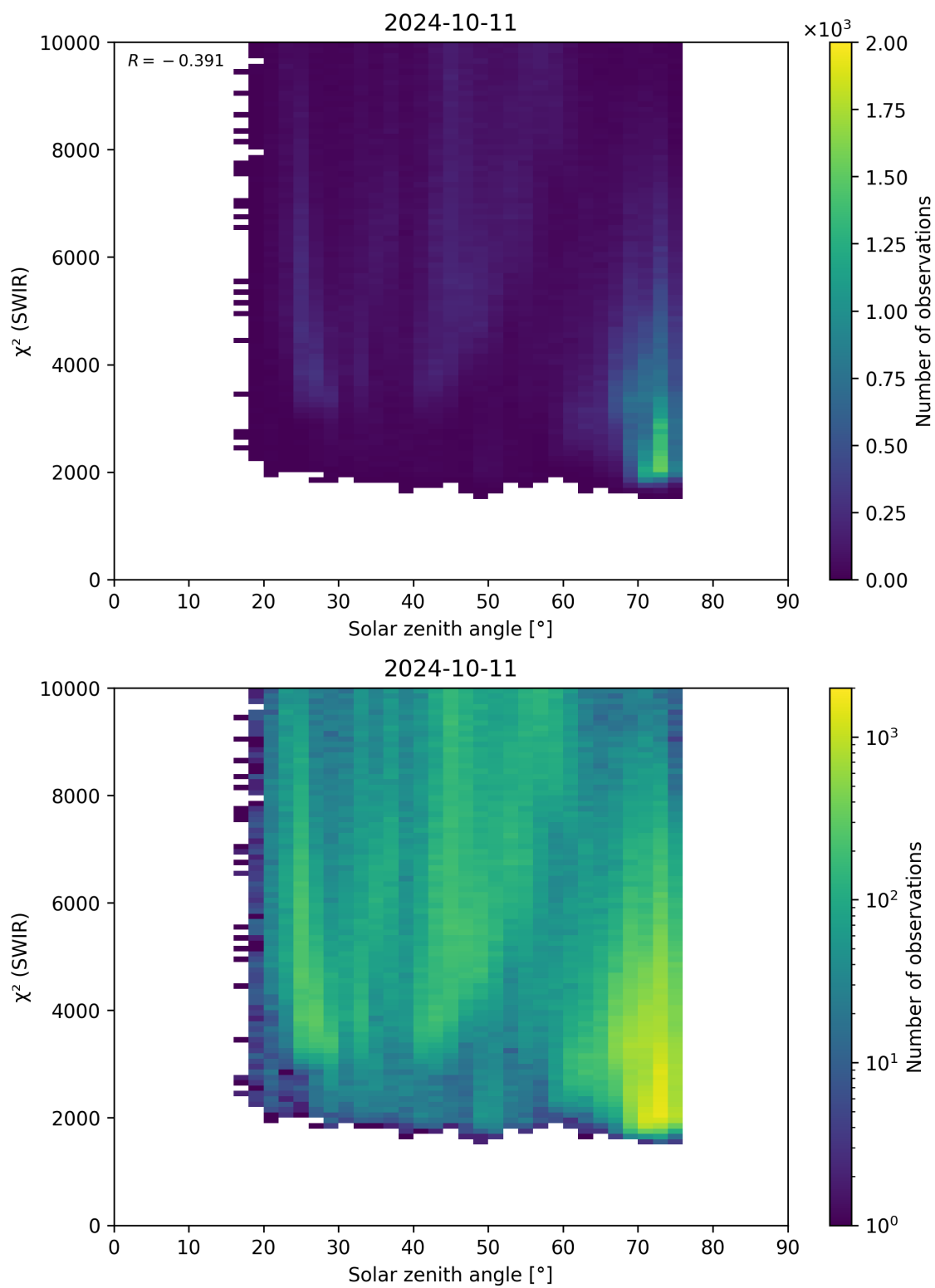
Figure 95: Scatter density plot of “Solar zenith angle” against “ \chi^2 (SWIR)” for 2024-10-10 to 2024-10-12.
