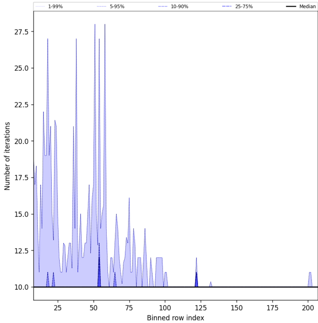
Figure 42: Along track statistics of “Number of iterations” for 2024-10-10 to 2024-10-12
