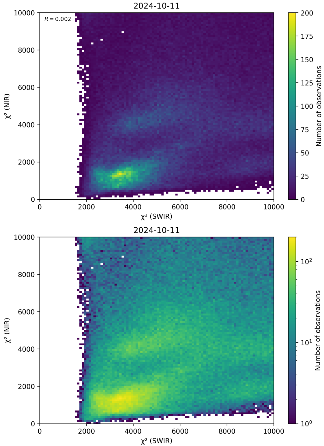
Figure 47: Scatter density plot of “ \chi^2 (SWIR)” against “ \chi^2 (NIR)” for 2024-10-10 to 2024-10-12.
