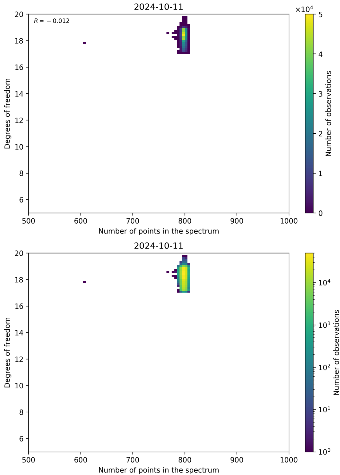
Figure 90: Scatter density plot of “Number of points in the spectrum” against “Degrees of freedom” for 2024-10-10 to 2024-10-12.
