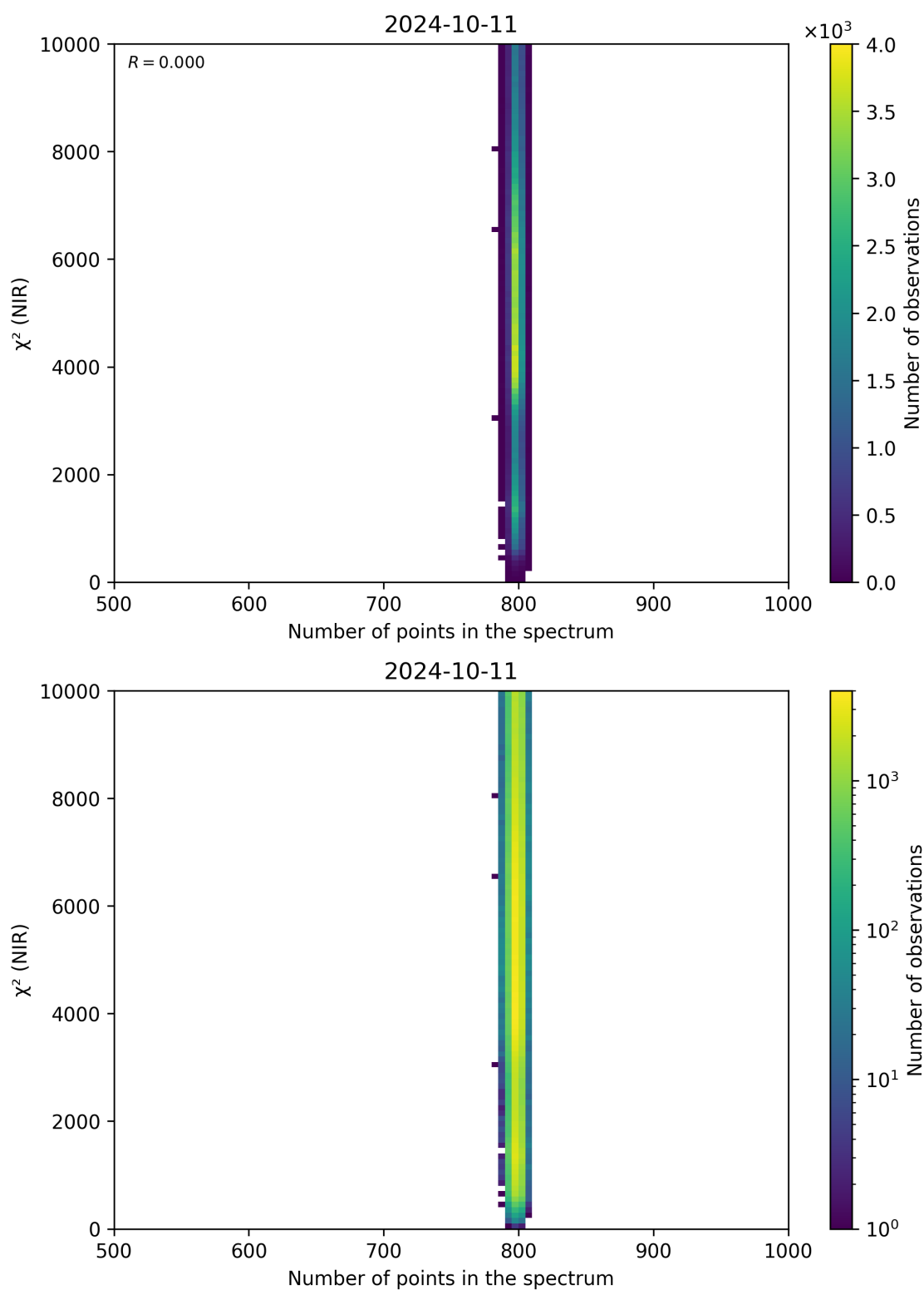
Figure 88: Scatter density plot of “Number of points in the spectrum” against “ \chi^2 (NIR)” for 2024-10-10 to 2024-10-12.
