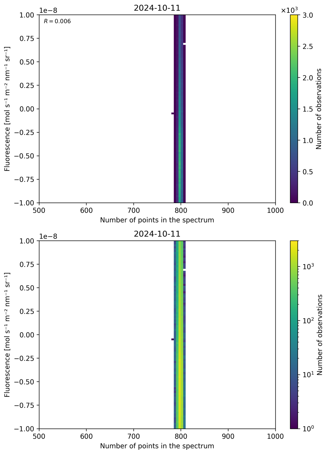
Figure 91: Scatter density plot of “Number of points in the spectrum” against “Fluorescence” for 2024-10-10 to 2024-10-12.
