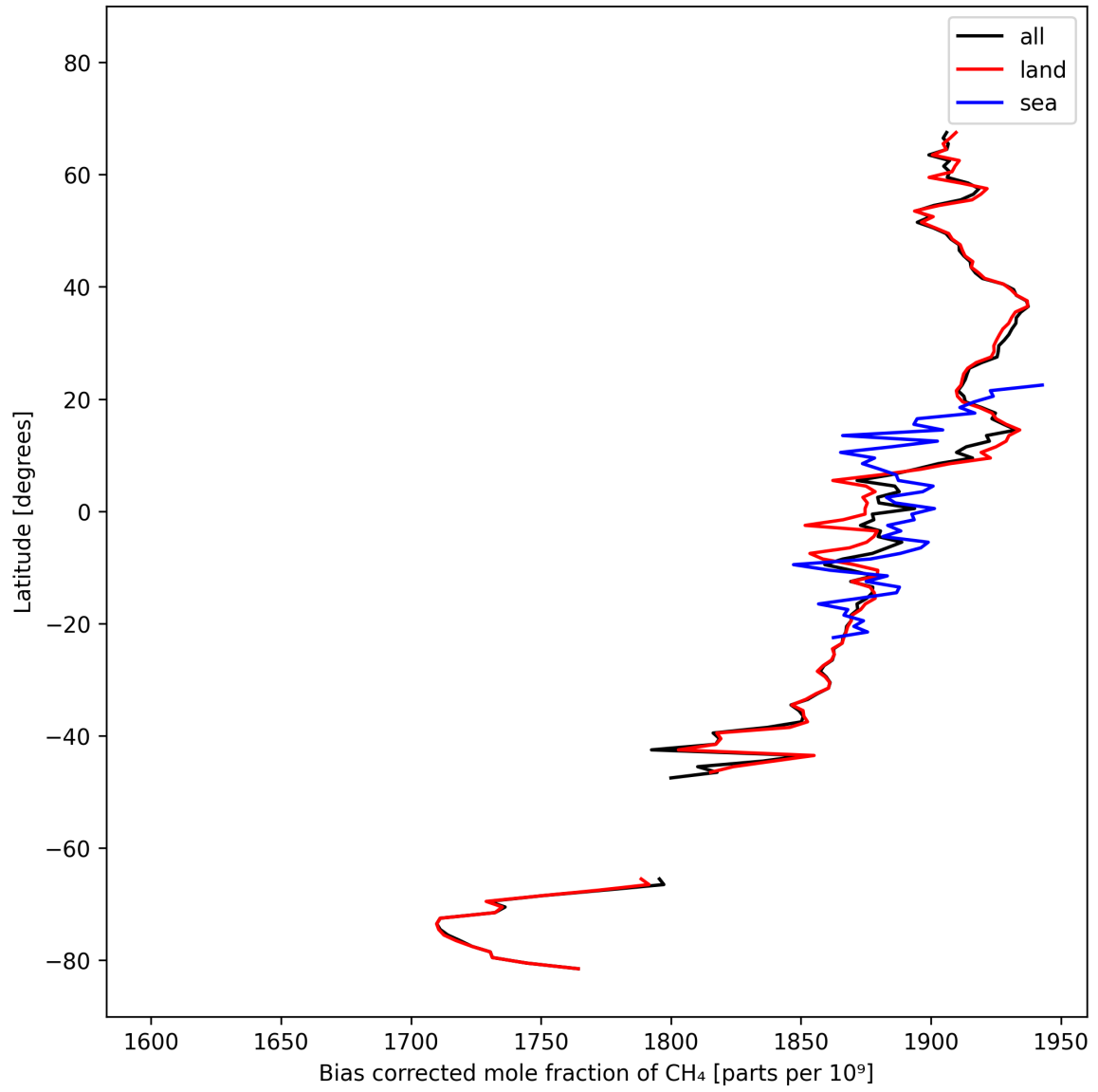
Figure 14: Zonal average of “Bias corrected mole fraction of CH 4 ” for 2024-10-10 to 2024-10-12.
