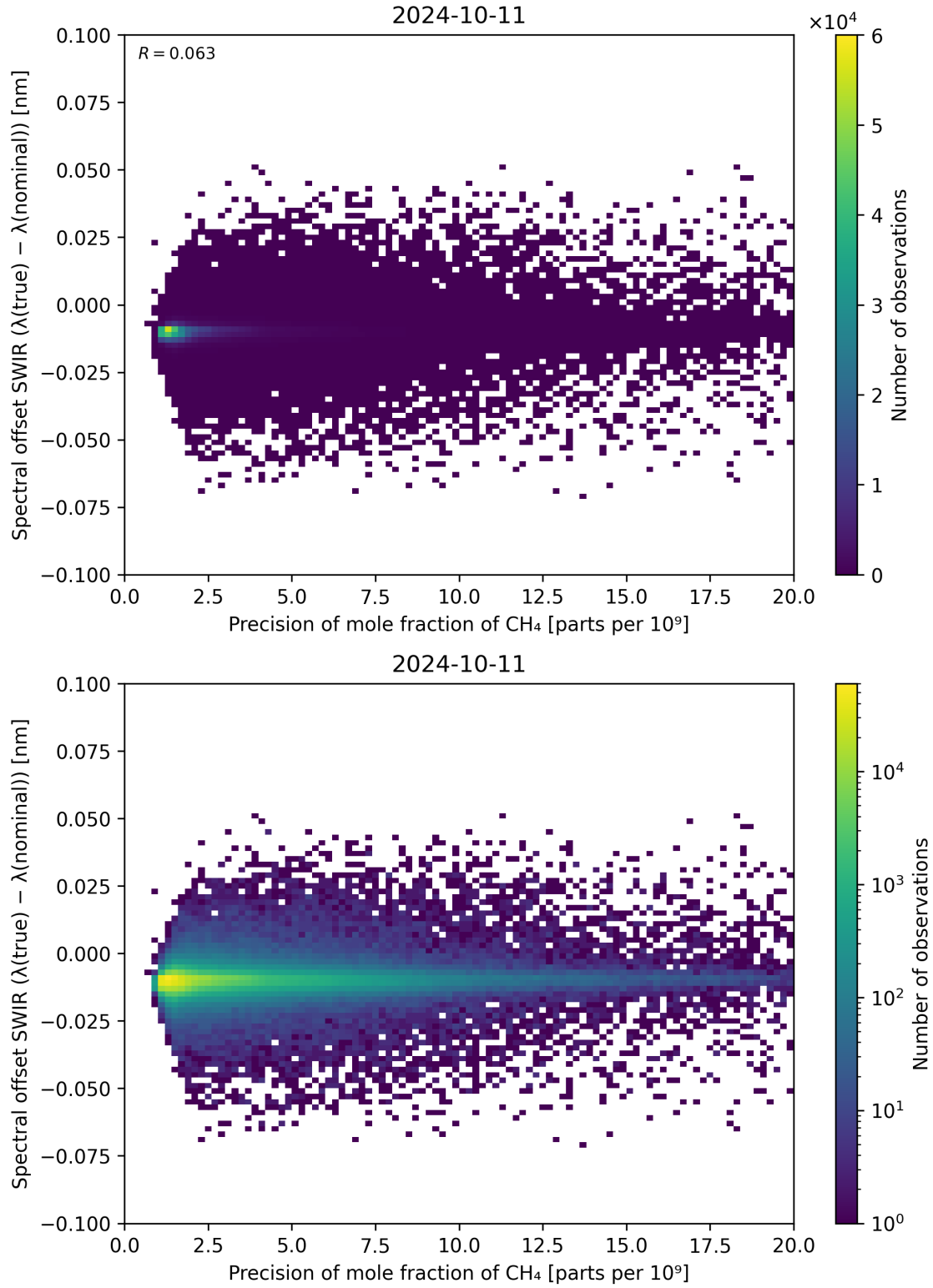
Figure 85: Scatter density plot of “Precision of mole fraction of CH 4 ” against “Spectral offset SWIR ( \lambda_{\text{true}} - \lambda_{\text{nominal}} )” for 2024-10-10 to 2024-10-12.
