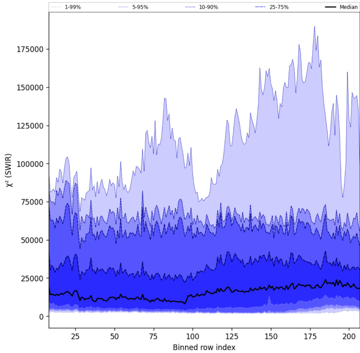
Figure 39: Along track statistics of “ \chi^2 (SWIR)” for 2024-10-10 to 2024-10-12
