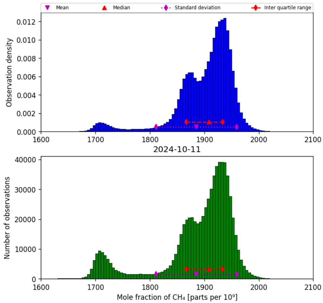
Figure 23: Histogram of “Mole fraction of CH 4 ” for 2024-10-10 to 2024-10-12
