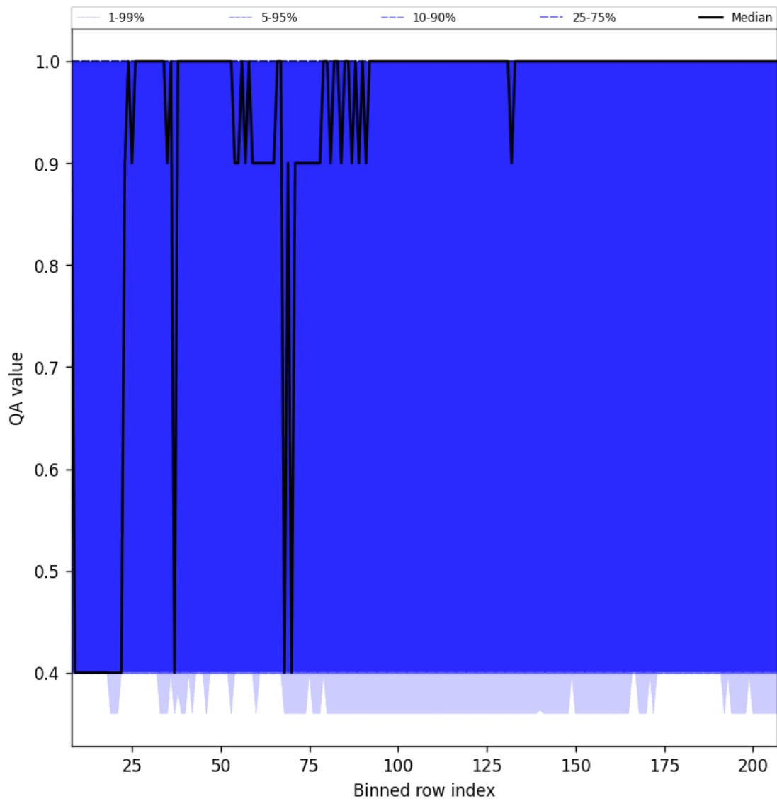
Figure 33: Along track statistics of “QA value” for 2024-10-10 to 2024-10-12
