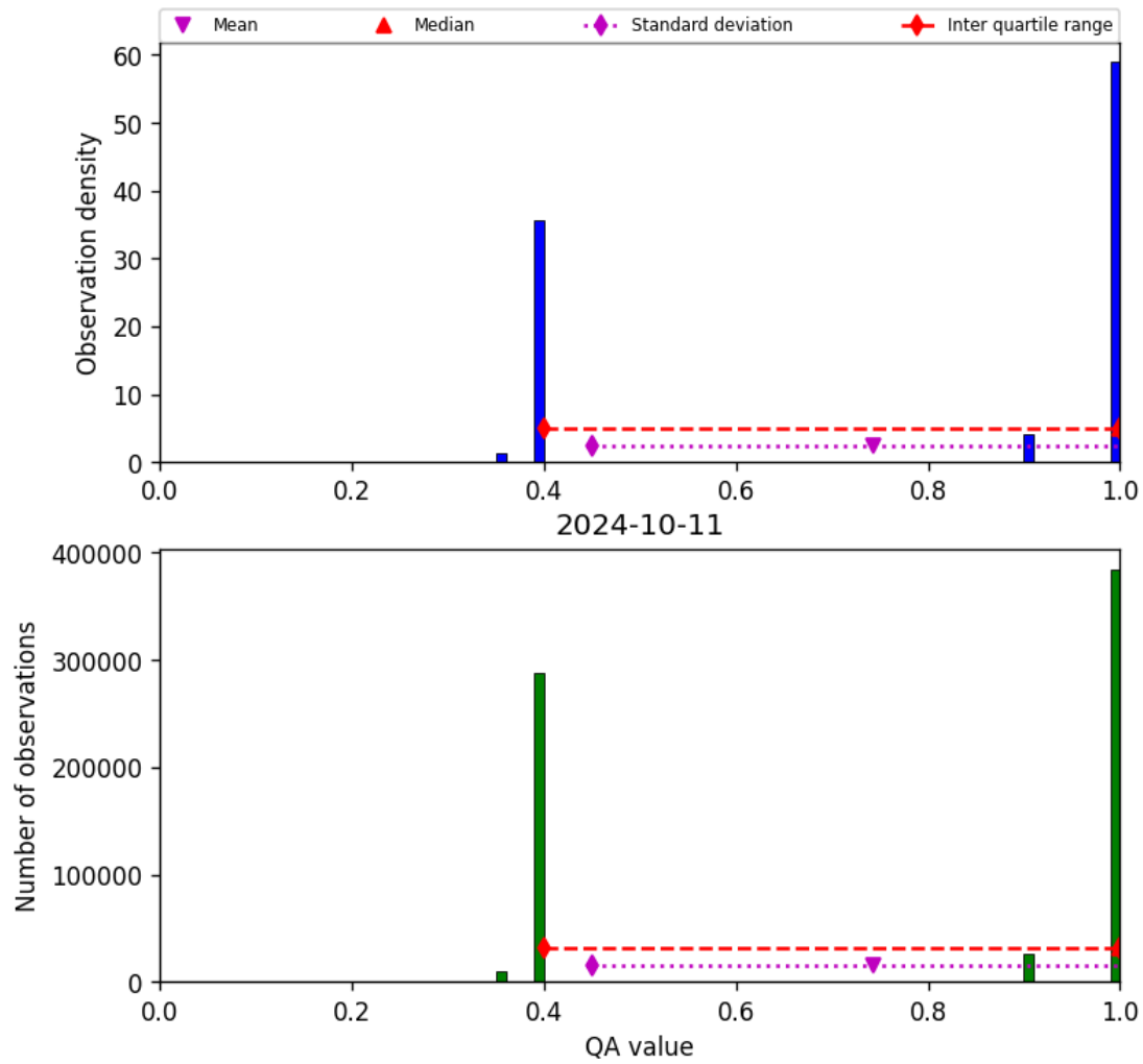
Figure 22: Histogram of “QA value” for 2024-10-10 to 2024-10-12
