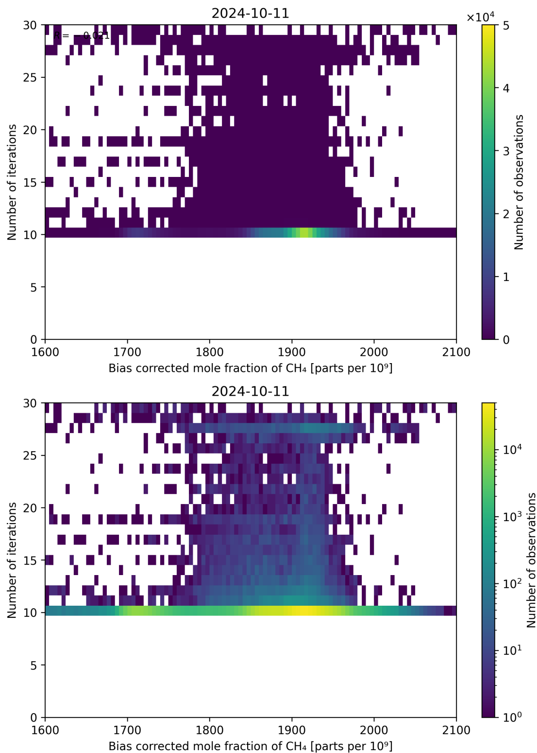
Figure 67: Scatter density plot of “Bias corrected mole fraction of CH 4 ” against “Number of iterations” for 2024-10-10 to 2024-10-12.
