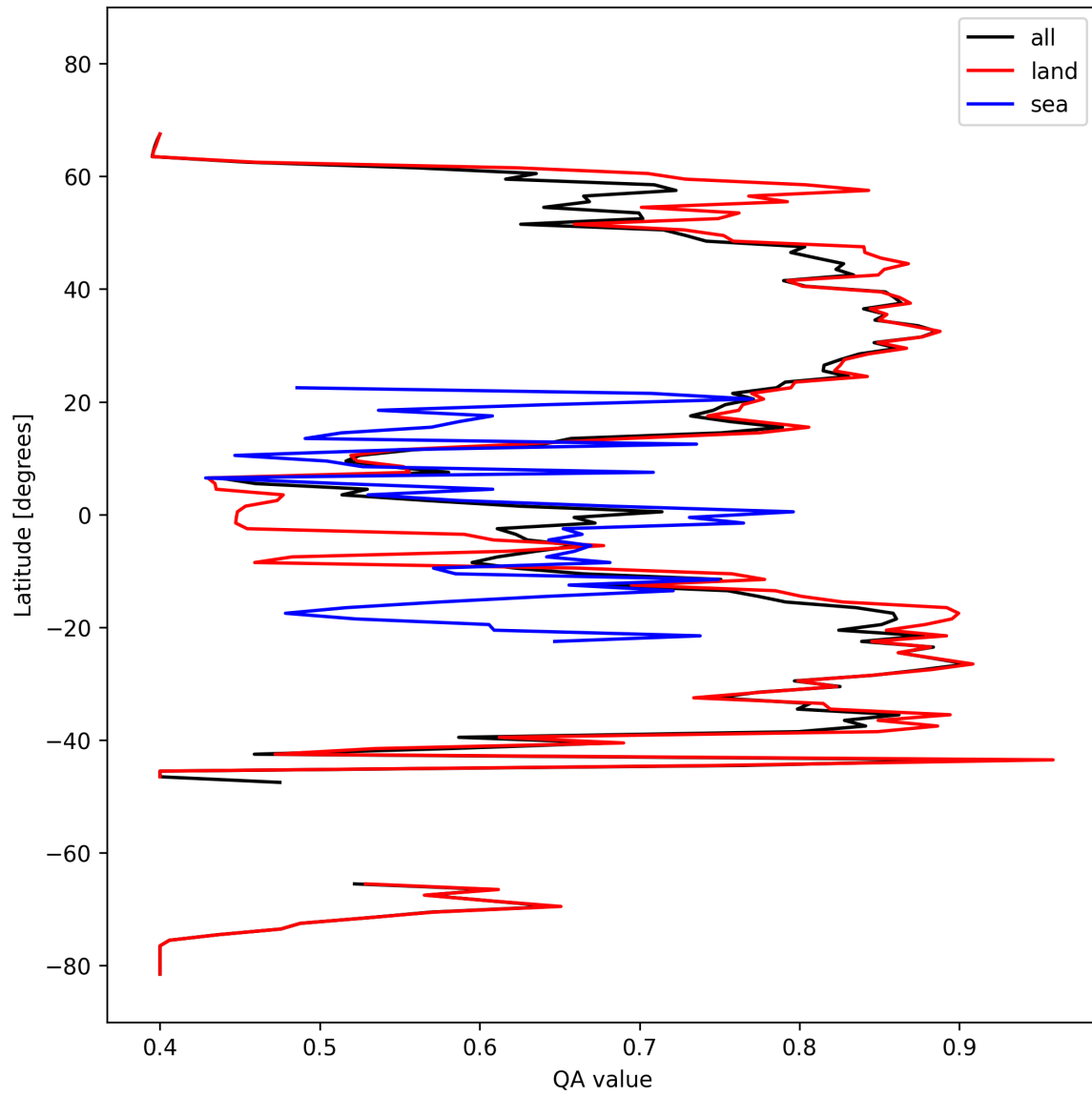
Figure 11: Zonal average of “QA value” for 2024-10-10 to 2024-10-12.
