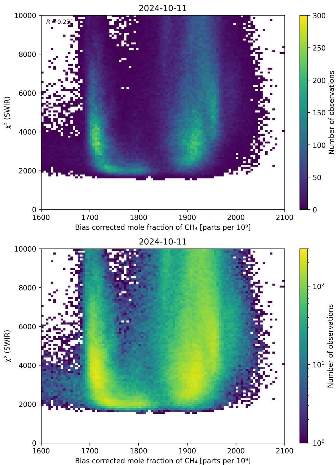
Figure 64: Scatter density plot of “Bias corrected mole fraction of CH 4 ” against “ \chi^2 (SWIR)” for 2024-10-10 to 2024-10-12.
