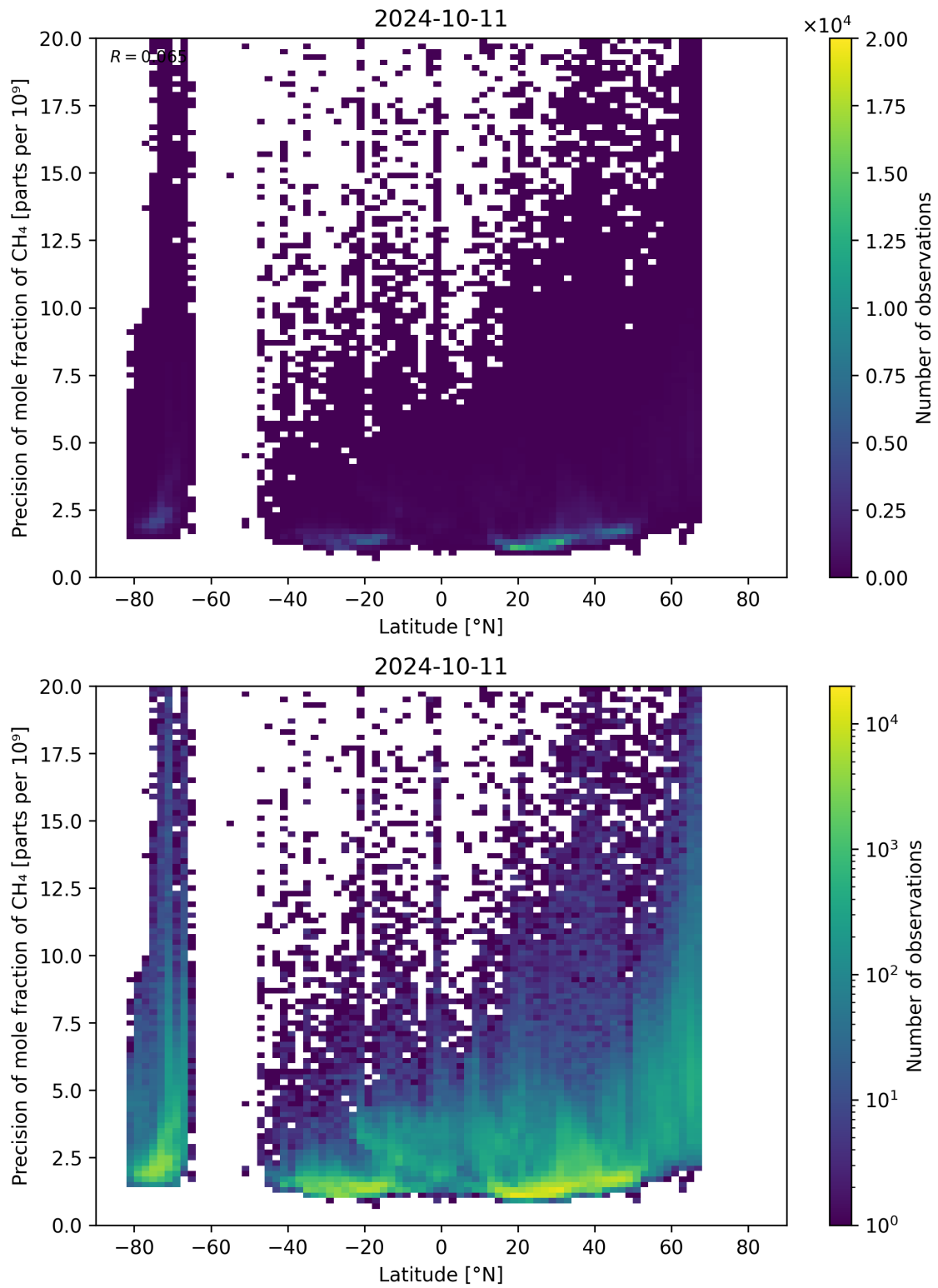
Figure 59: Scatter density plot of “Latitude” against “Precision of mole fraction of CH 4 ” for 2024-10-10 to 2024-10-12.
