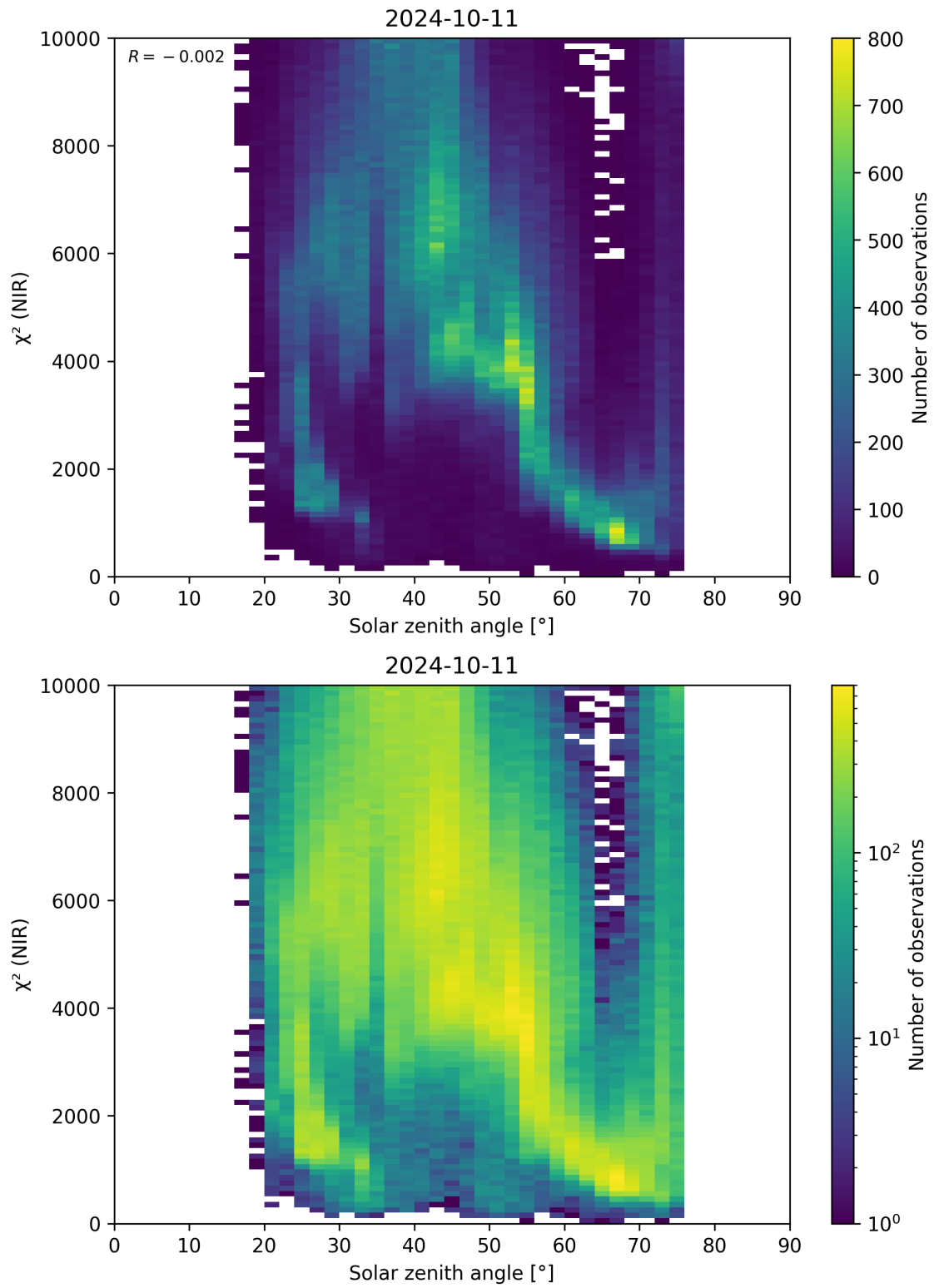
Figure 94: Scatter density plot of “Solar zenith angle” against “ \chi^2 (NIR)” for 2024-10-10 to 2024-10-12.
