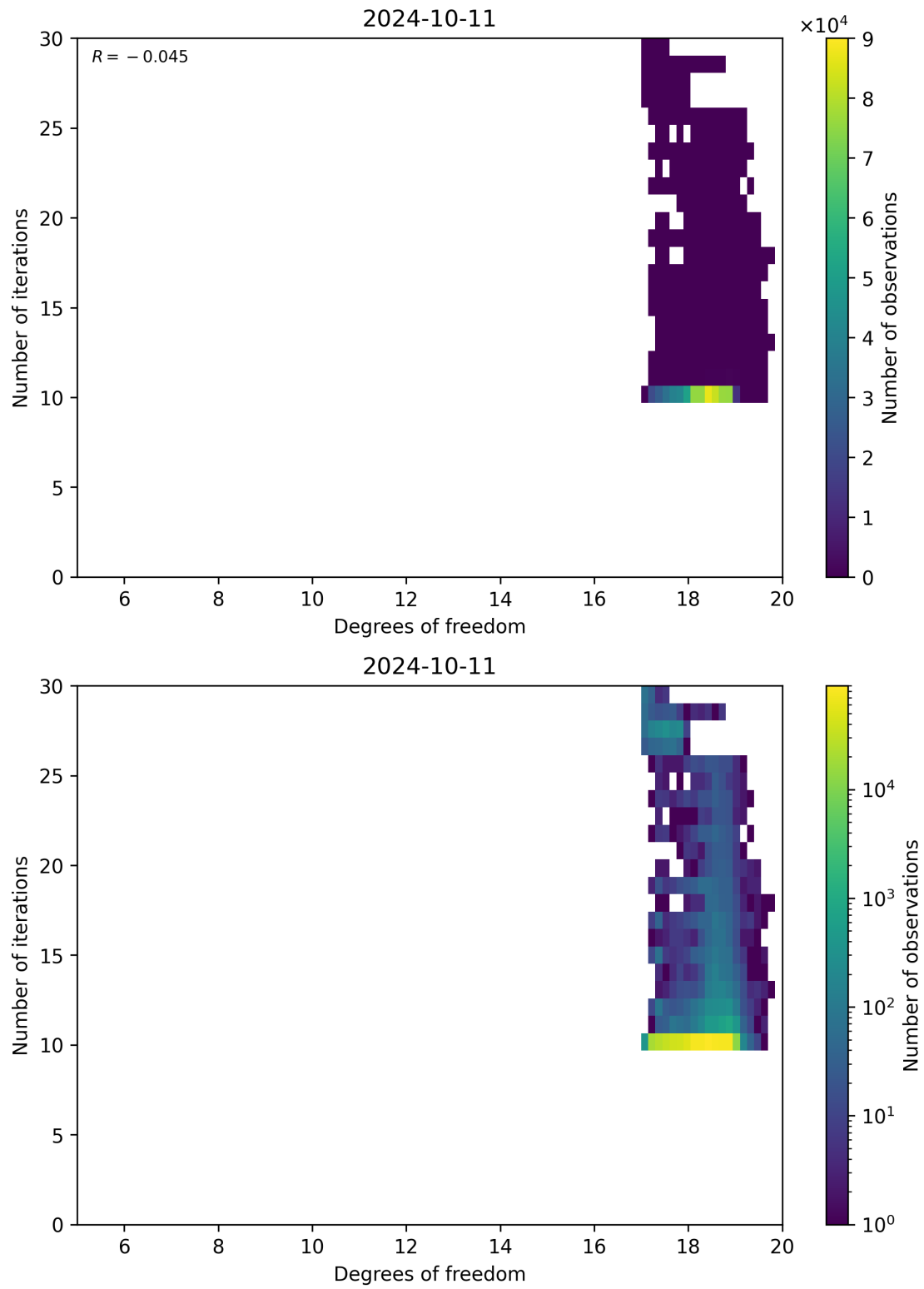
Figure 52: Scatter density plot of “Degrees of freedom” against “Number of iterations” for 2024-10-10 to 2024-10-12.
