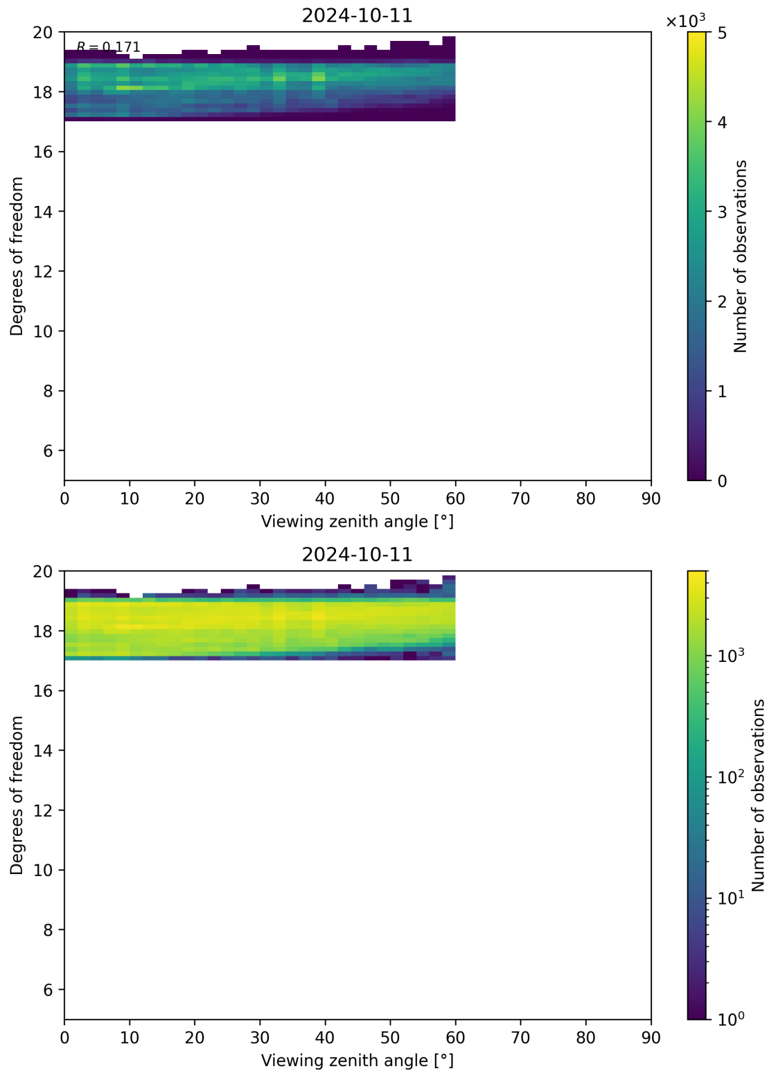
Figure 107: Scatter density plot of “Viewing zenith angle” against “Degrees of freedom” for 2024-10-10 to 2024-10-12.
