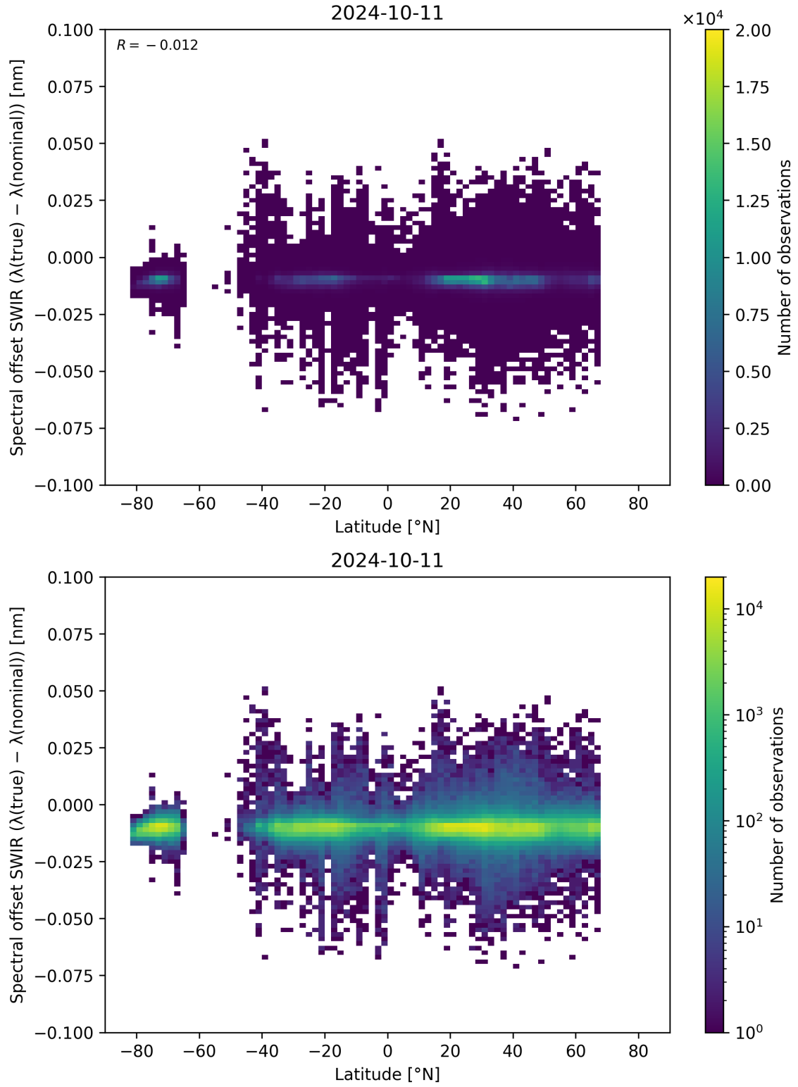
Figure 62: Scatter density plot of “Latitude” against “Spectral offset SWIR ( \lambda_{\text{true}} - \lambda_{\text{nominal}} )” for 2024-10-10 to 2024-10-12.
