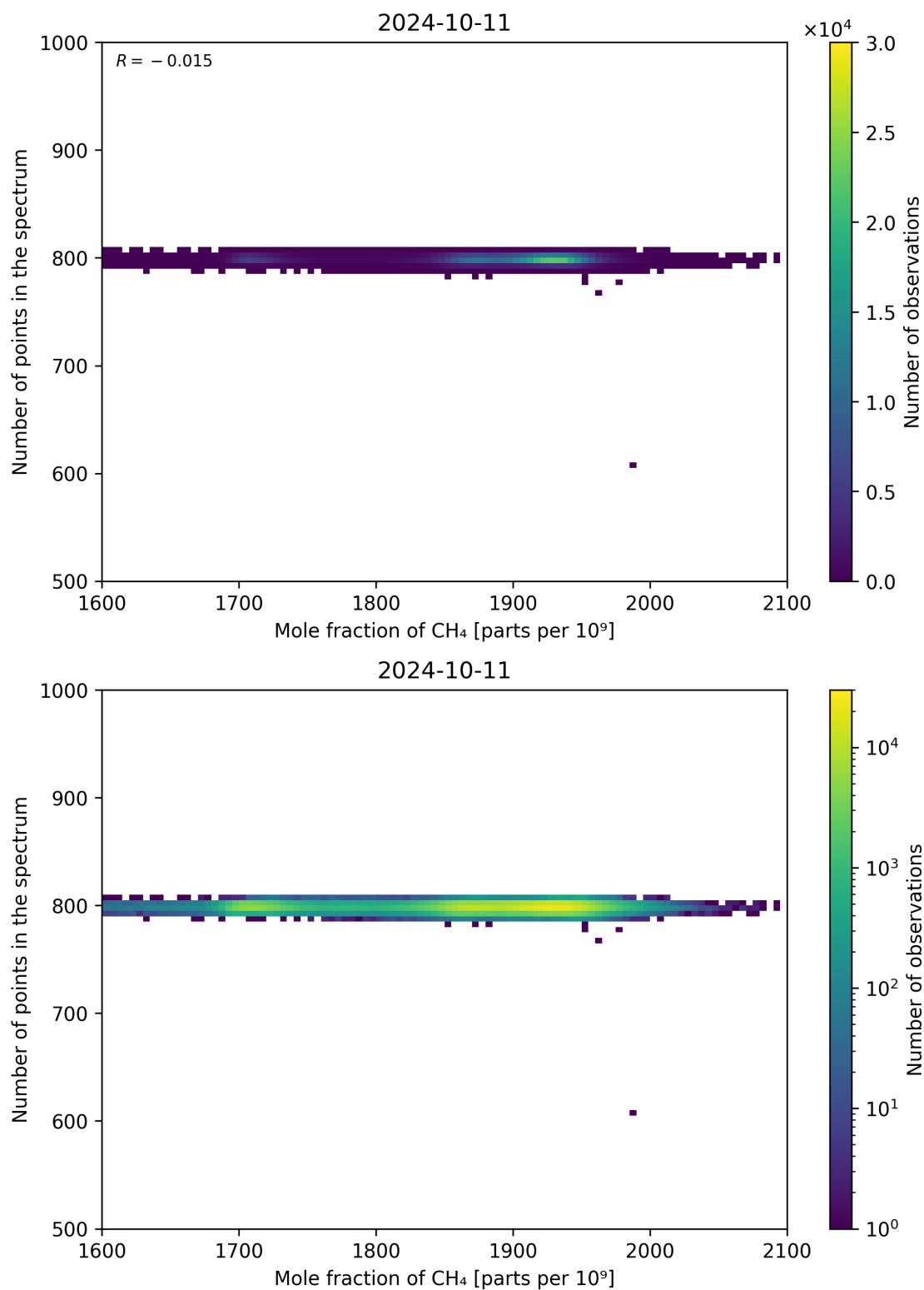
Figure 77: Scatter density plot of “Mole fraction of CH 4 ” against “Number of points in the spectrum” for 2024-10-10 to 2024-10-12.
