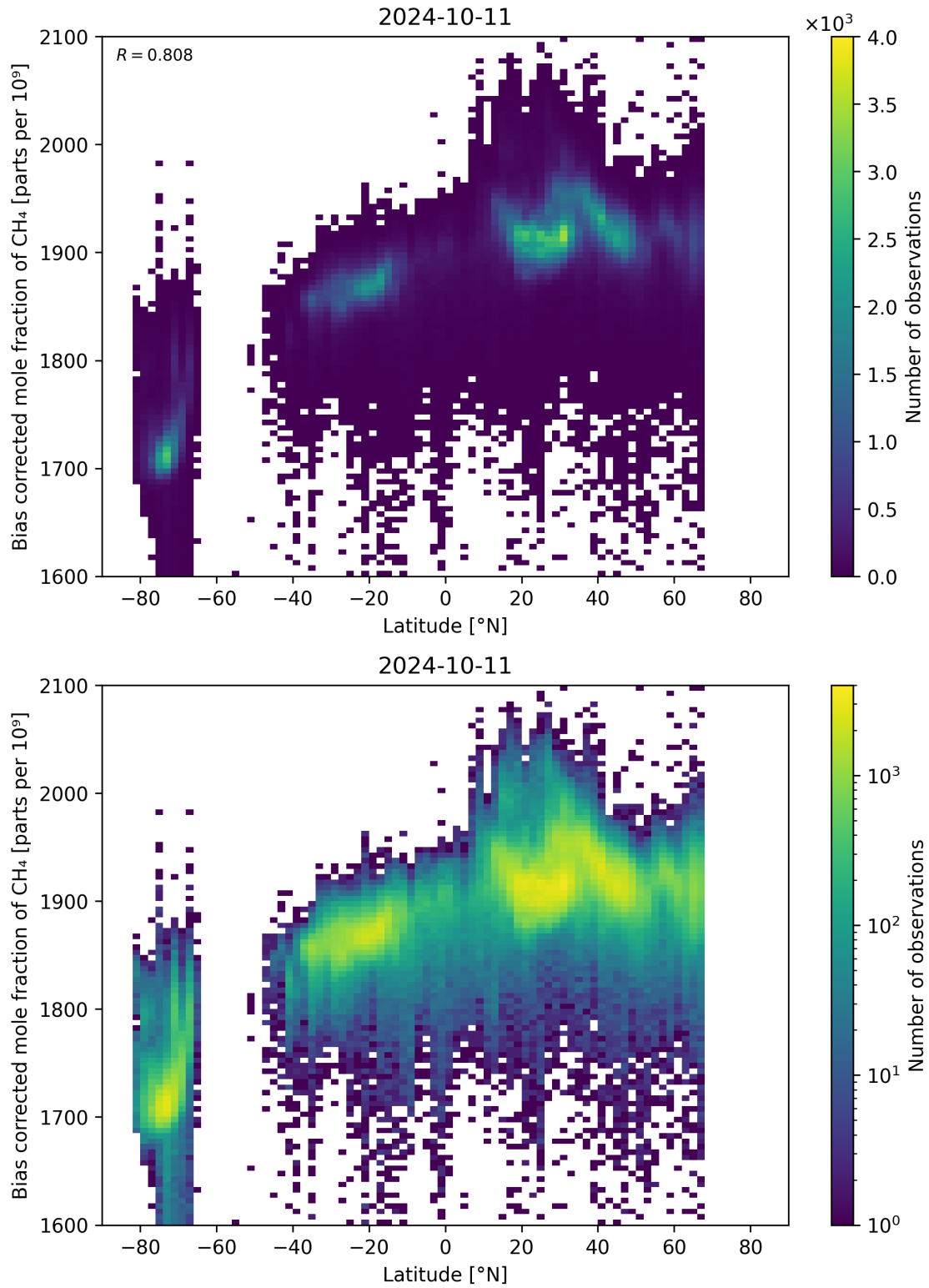
Figure 58: Scatter density plot of “Latitude” against “Bias corrected mole fraction of \text{CH}_4 ” for 2024-10-10 to 2024-10-12.
