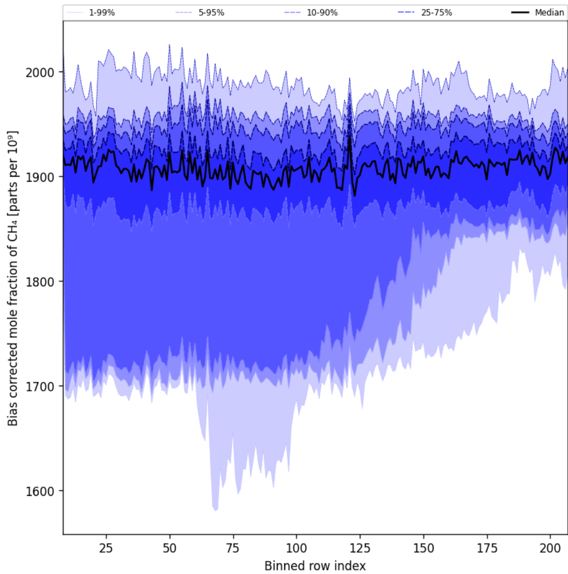
Figure 36: Along track statistics of “Bias corrected mole fraction of CH 4 ” for 2024-10-10 to 2024-10-12
