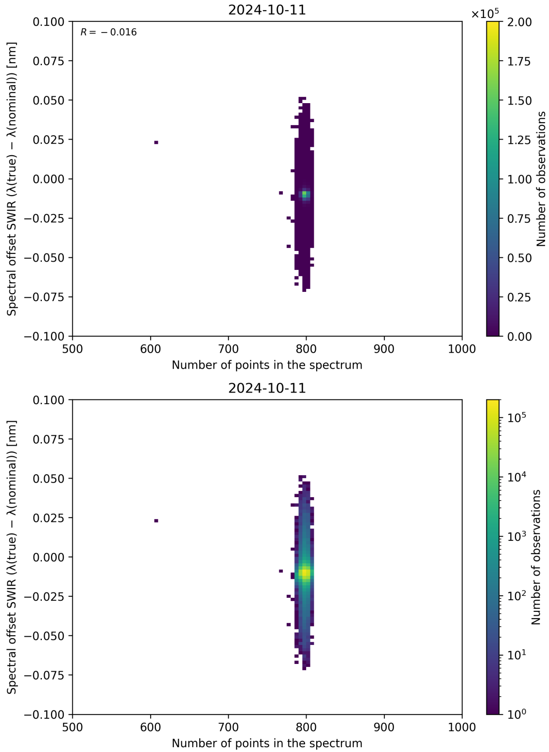
Figure 93: Scatter density plot of “Number of points in the spectrum” against “Spectral offset SWIR ( \lambda_{\text{true}} - \lambda_{\text{nominal}} )” for 2024-10-10 to 2024-10-12.
