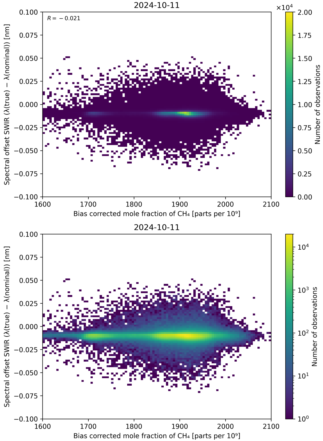
Figure 69: Scatter density plot of “Bias corrected mole fraction of \text{CH}_4 ” against “Spectral offset SWIR ( \lambda_{\text{true}} - \lambda_{\text{nominal}} )” for 2024-10-10 to 2024-10-12.
