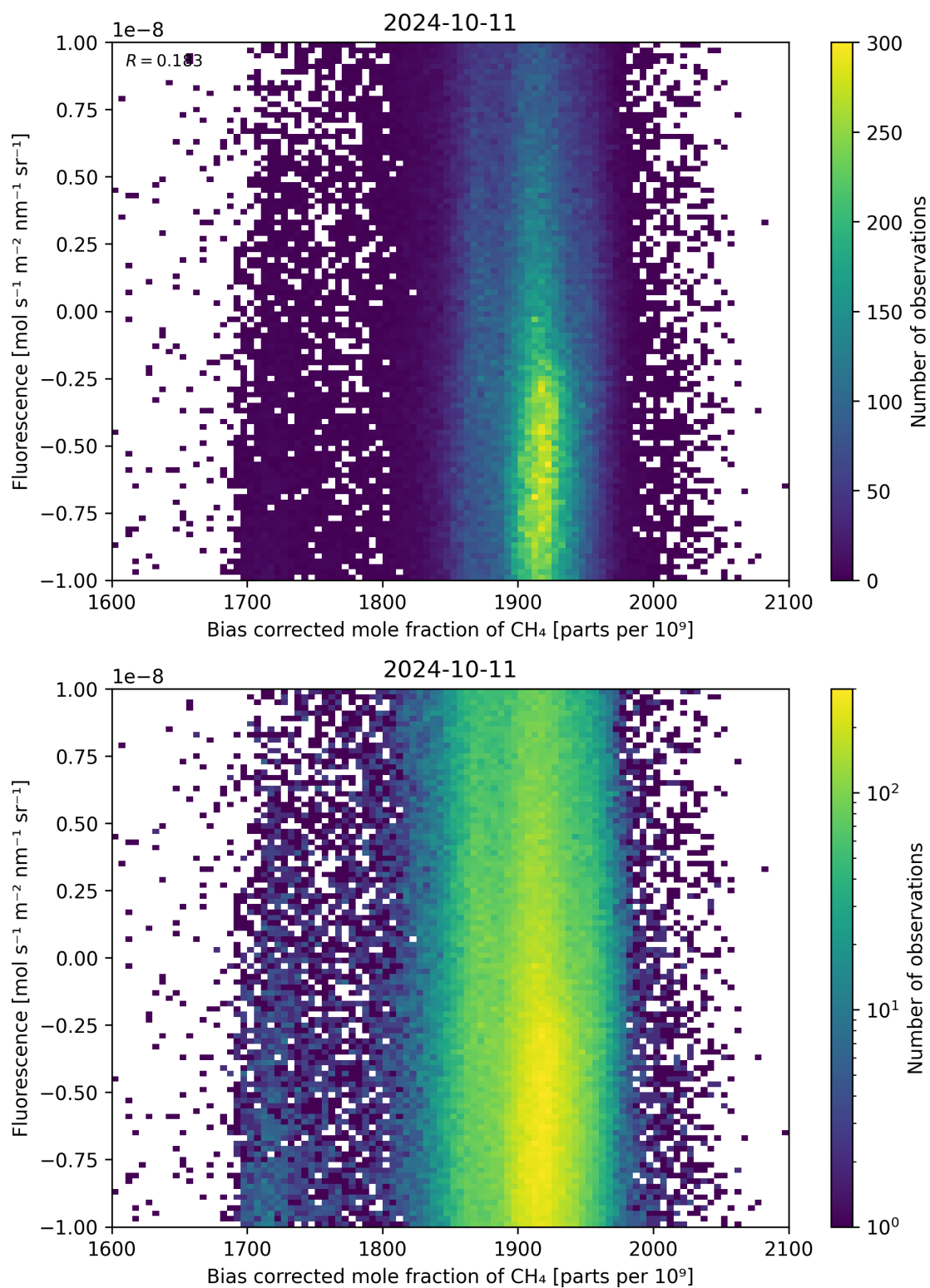
Figure 66: Scatter density plot of “Bias corrected mole fraction of CH 4 ” against “Fluorescence” for 2024-10-10 to 2024-10-12.
