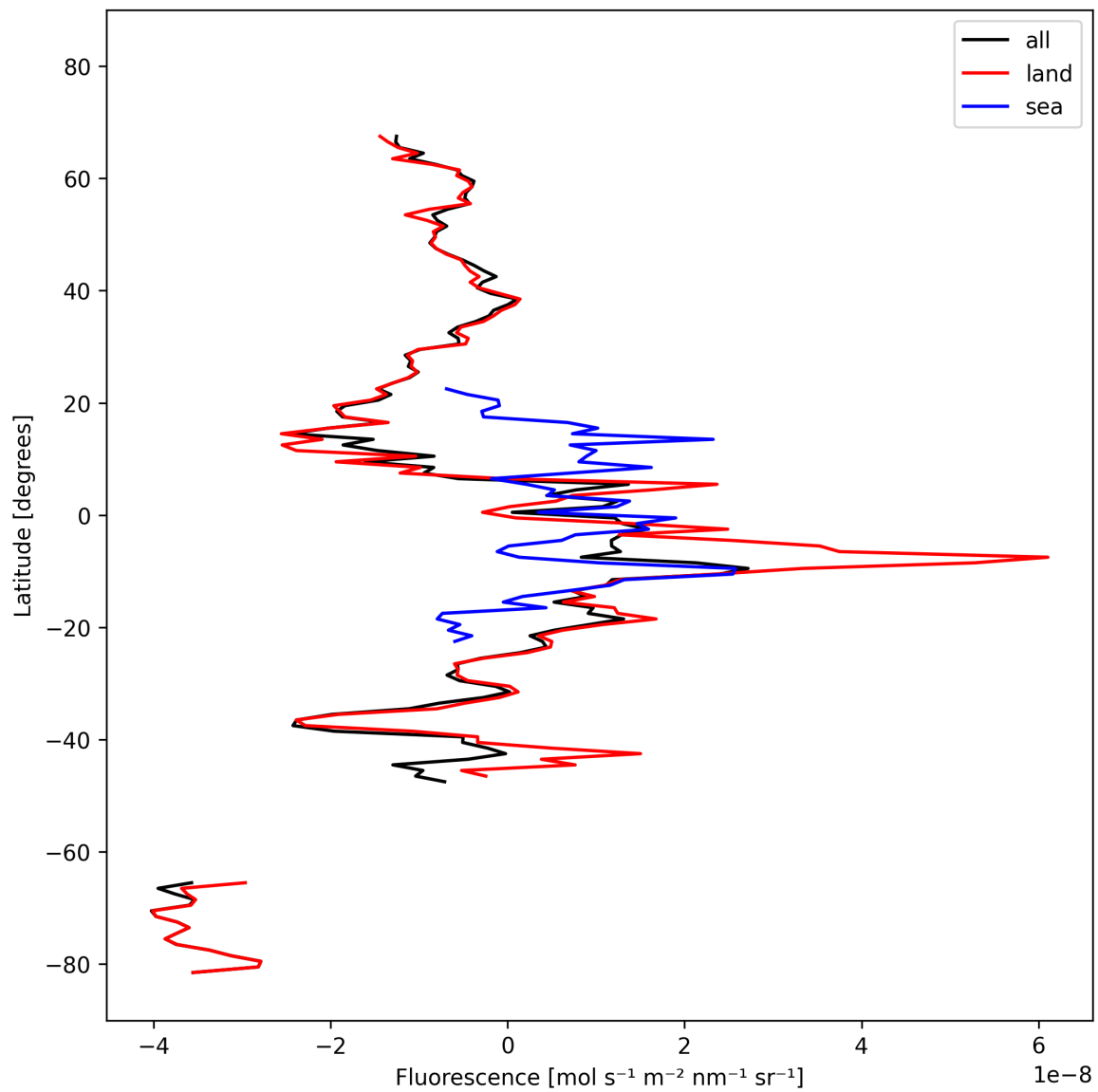
Figure 21: Zonal average of “Fluorescence” for 2024-10-10 to 2024-10-12.
