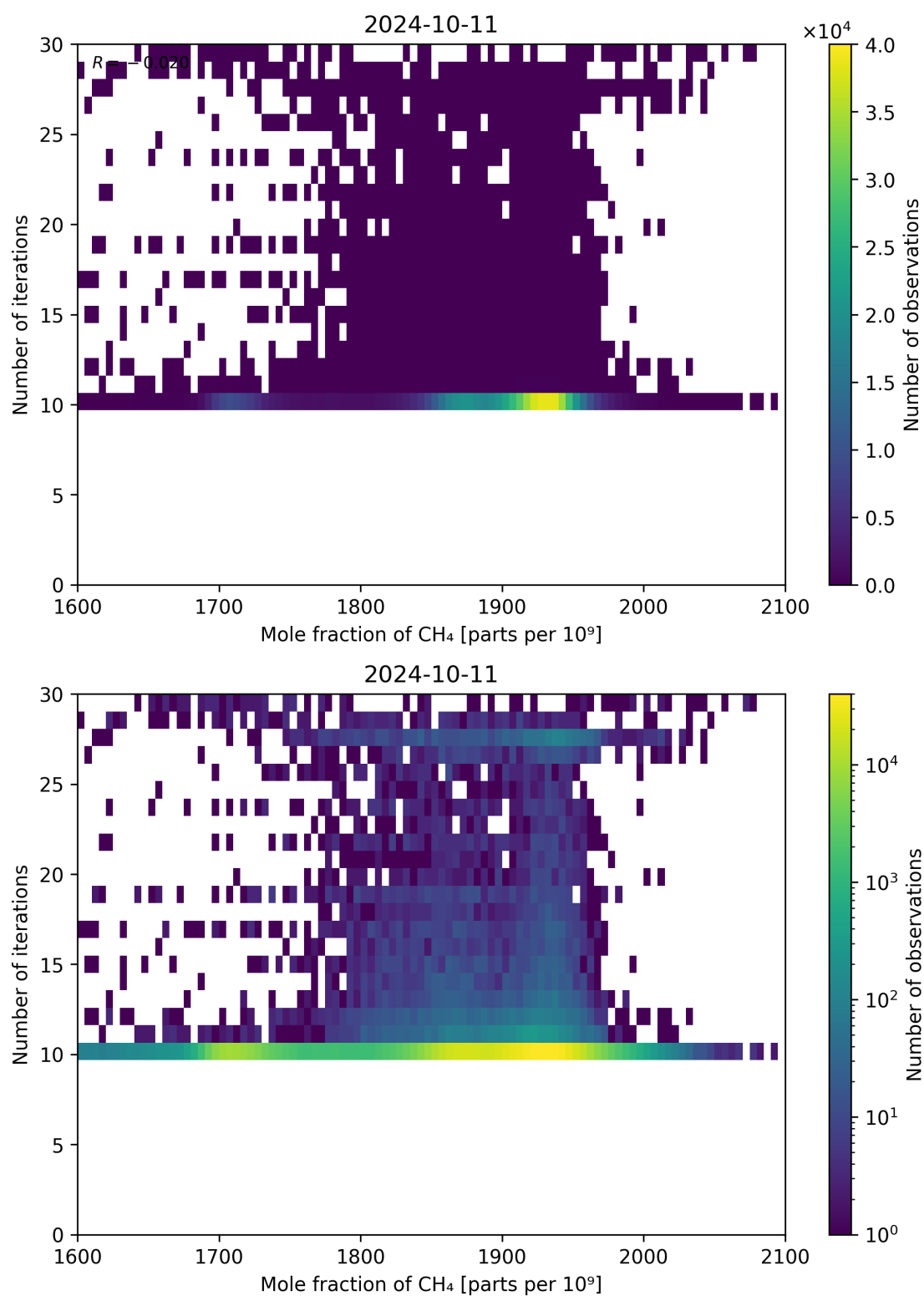
Figure 76: Scatter density plot of “Mole fraction of CH 4 ” against “Number of iterations” for 2024-10-10 to 2024-10-12.
