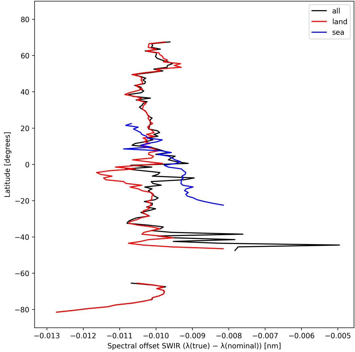
Figure 16: Zonal average of “Spectral offset SWIR ( \lambda_{\text{true}} - \lambda_{\text{nominal}} )” for 2024-10-10 to 2024-10-12.
