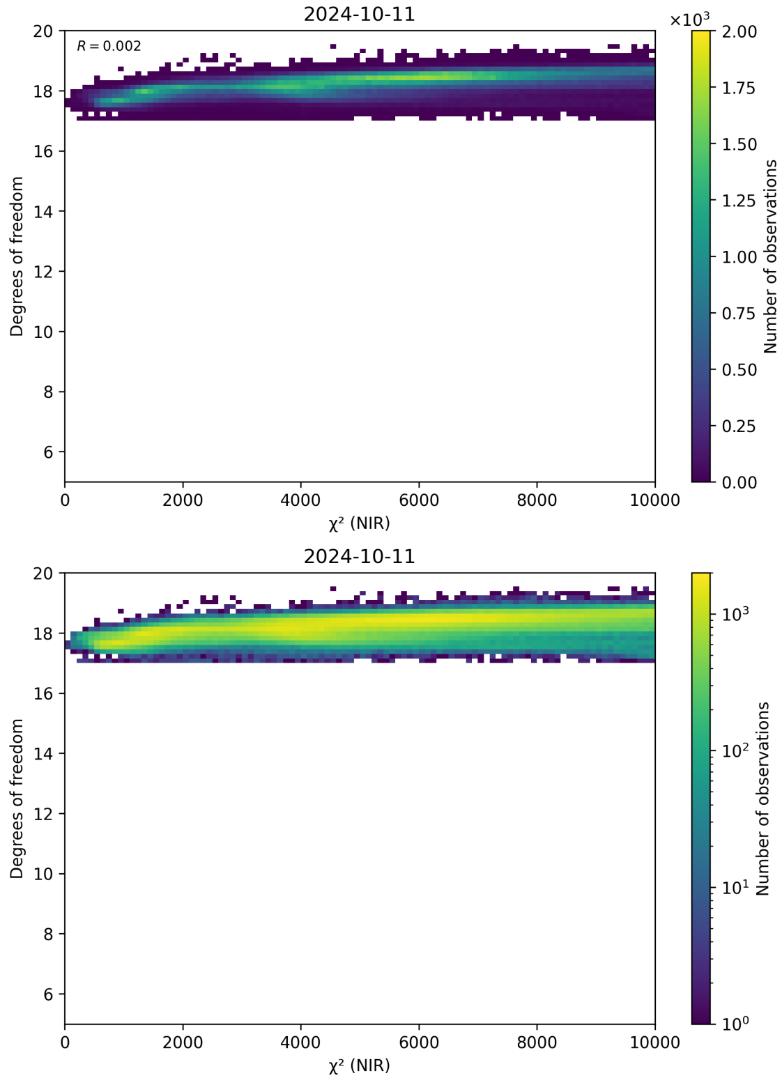
Figure 44: Scatter density plot of “ \chi^2 (NIR)” against “Degrees of freedom” for 2024-10-10 to 2024-10-12.
