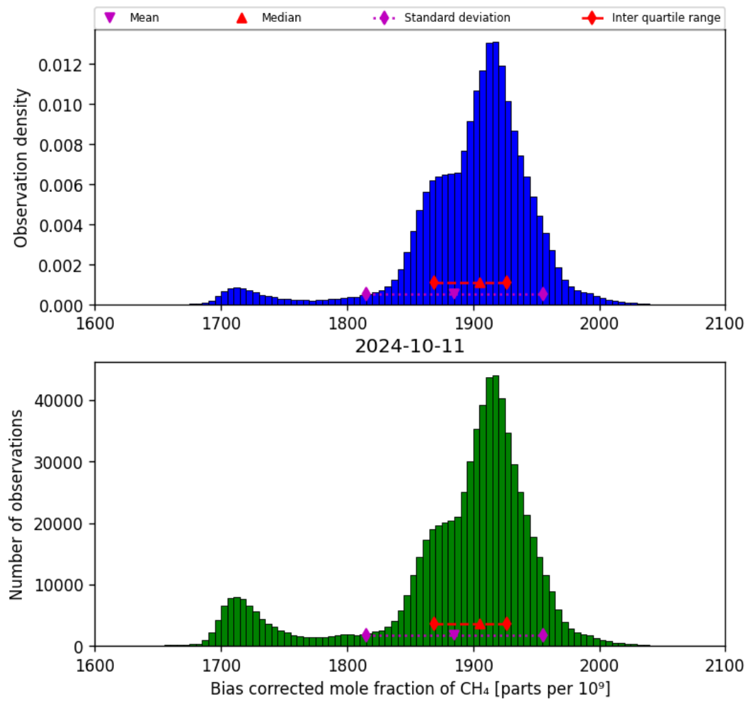
Figure 25: Histogram of “Bias corrected mole fraction of CH 4 ” for 2024-10-10 to 2024-10-12
