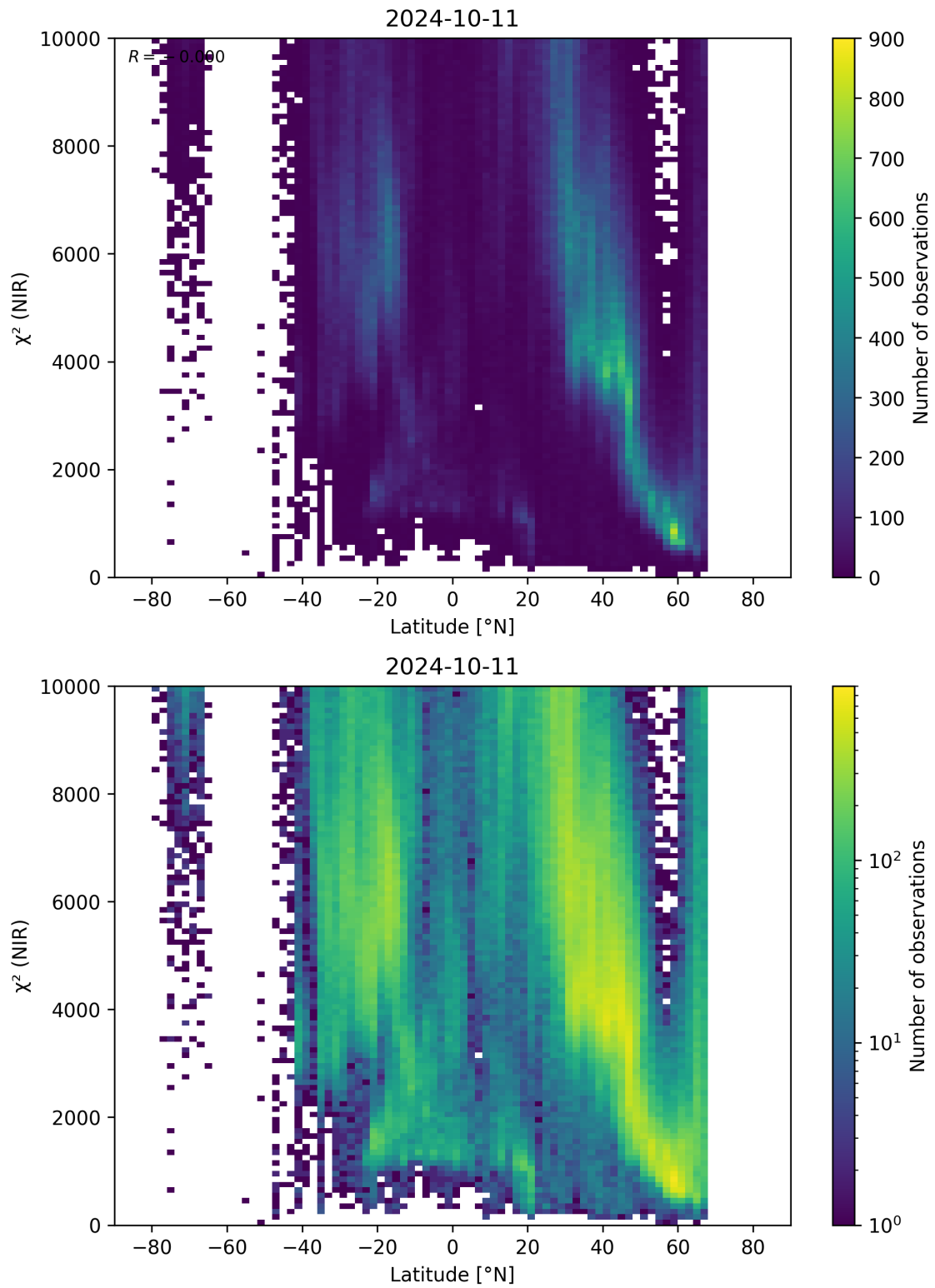
Figure 53: Scatter density plot of “Latitude” against “ \chi^2 (NIR)” for 2024-10-10 to 2024-10-12.
