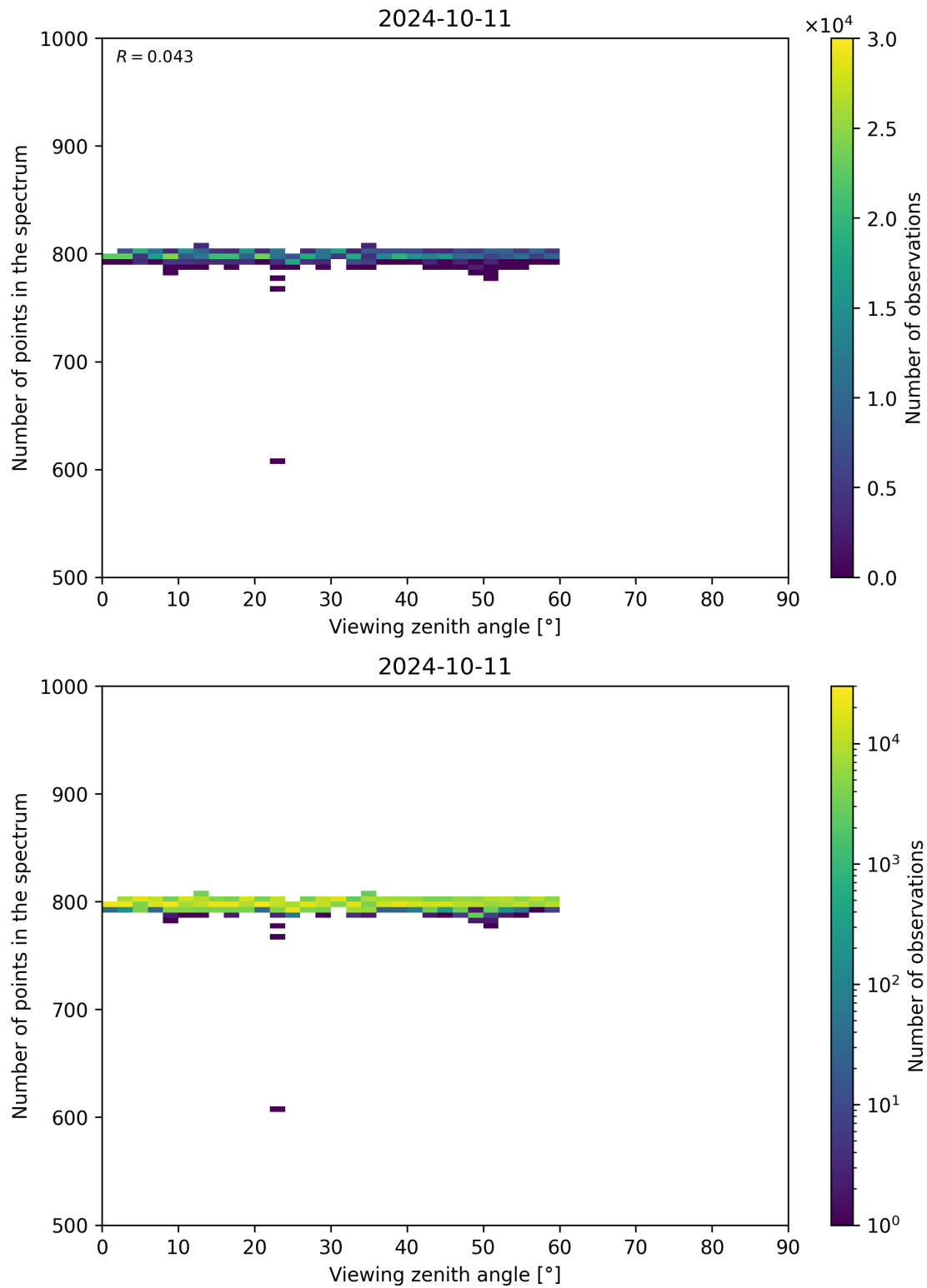
Figure 114: Scatter density plot of “Viewing zenith angle” against “Number of points in the spectrum” for 2024-10-10 to 2024-10-12.
