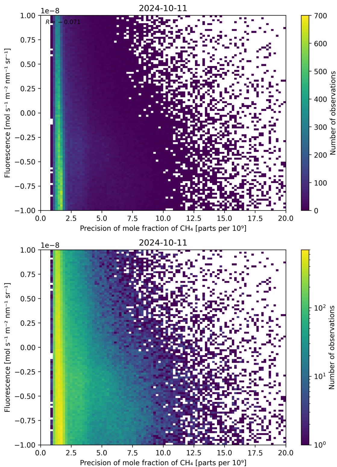
Figure 81: Scatter density plot of “Precision of mole fraction of CH 4 ” against “Fluorescence” for 2024-10-10 to 2024-10-12.
