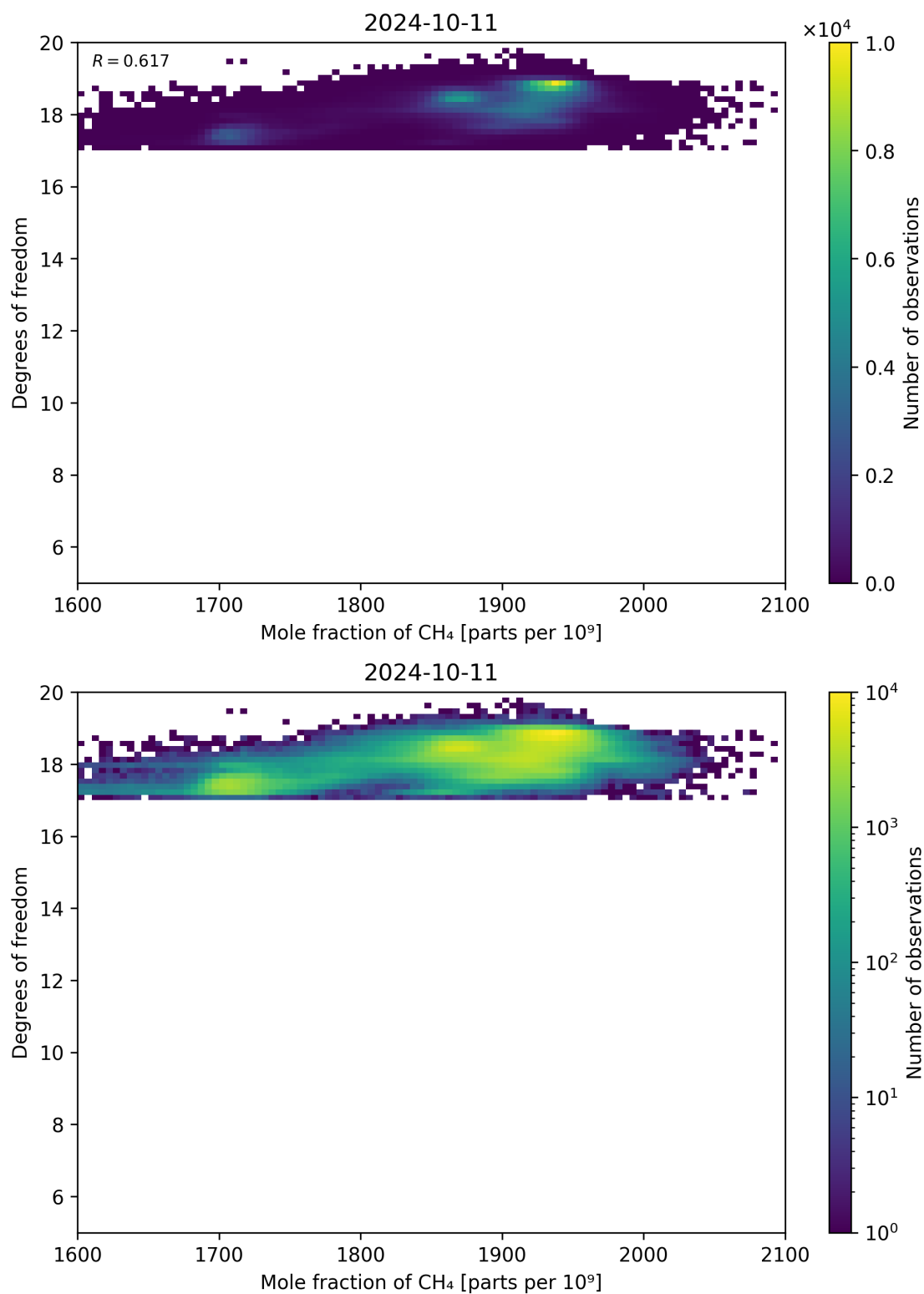
Figure 72: Scatter density plot of “Mole fraction of CH 4 ” against “Degrees of freedom” for 2024-10-10 to 2024-10-12.
