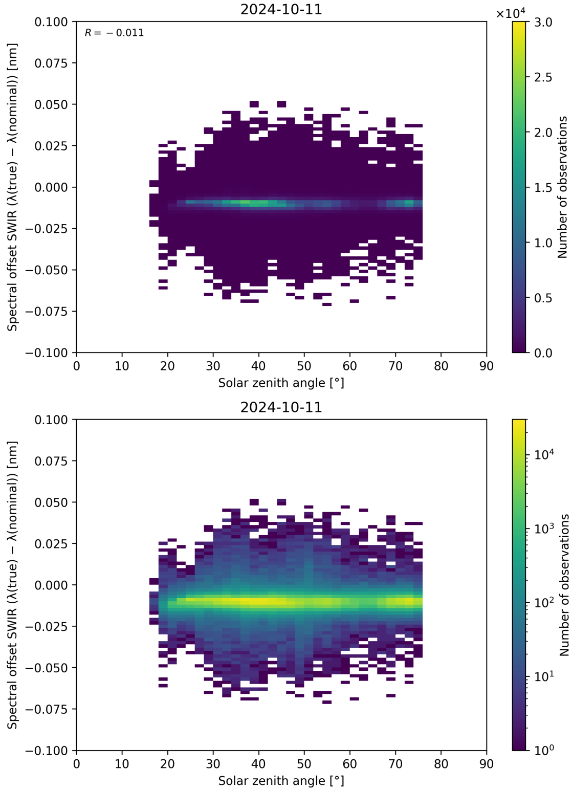
Figure 104: Scatter density plot of “Solar zenith angle” against “Spectral offset SWIR ( \lambda_{\text{true}} - \lambda_{\text{nominal}} )” for 2024-10-10 to 2024-10-12.
