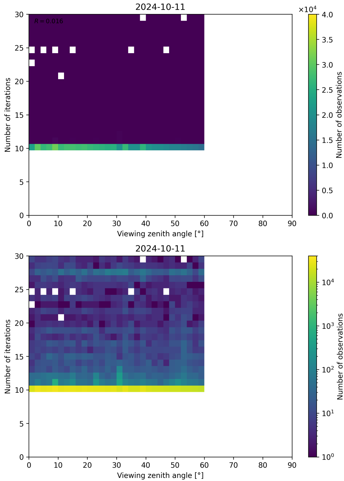
Figure 113: Scatter density plot of “Viewing zenith angle” against “Number of iterations” for 2024-10-10 to 2024-10-12.
