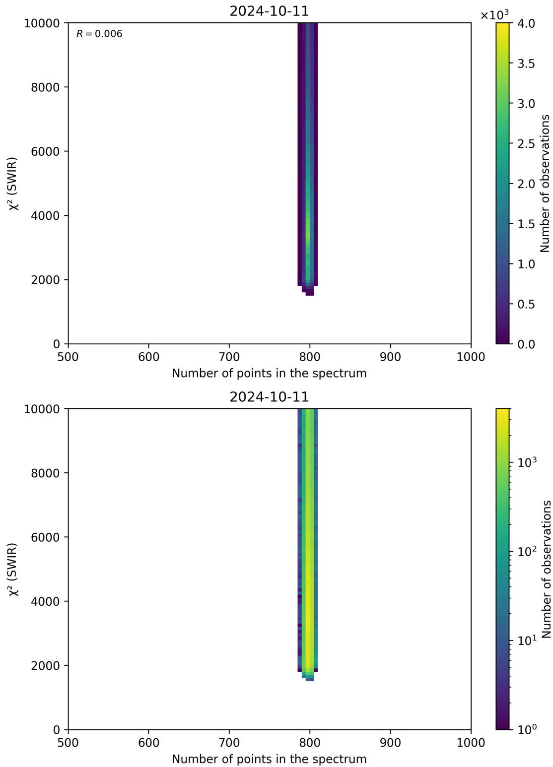
Figure 89: Scatter density plot of “Number of points in the spectrum” against “ \chi^2 (SWIR)” for 2024-10-10 to 2024-10-12.
