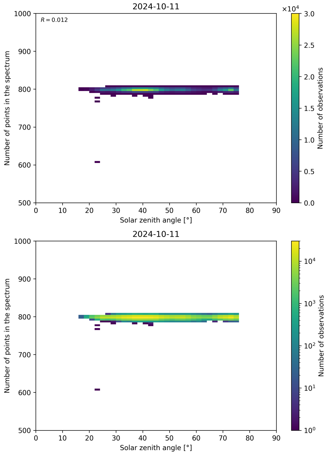
Figure 103: Scatter density plot of “Solar zenith angle” against “Number of points in the spectrum” for 2024-10-10 to 2024-10-12.
