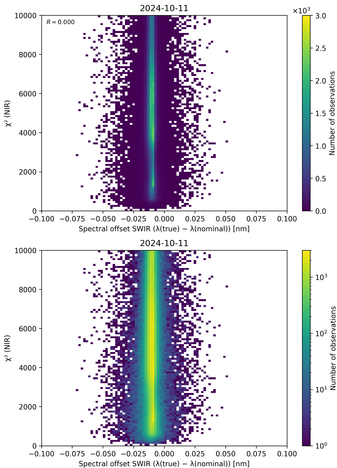
Figure 117: Scatter density plot of “Spectral offset SWIR ( \lambda_{\text{true}} - \lambda_{\text{nominal}} )” against “ \chi^2 (NIR)” for 2024-10-10 to 2024-10-12.
