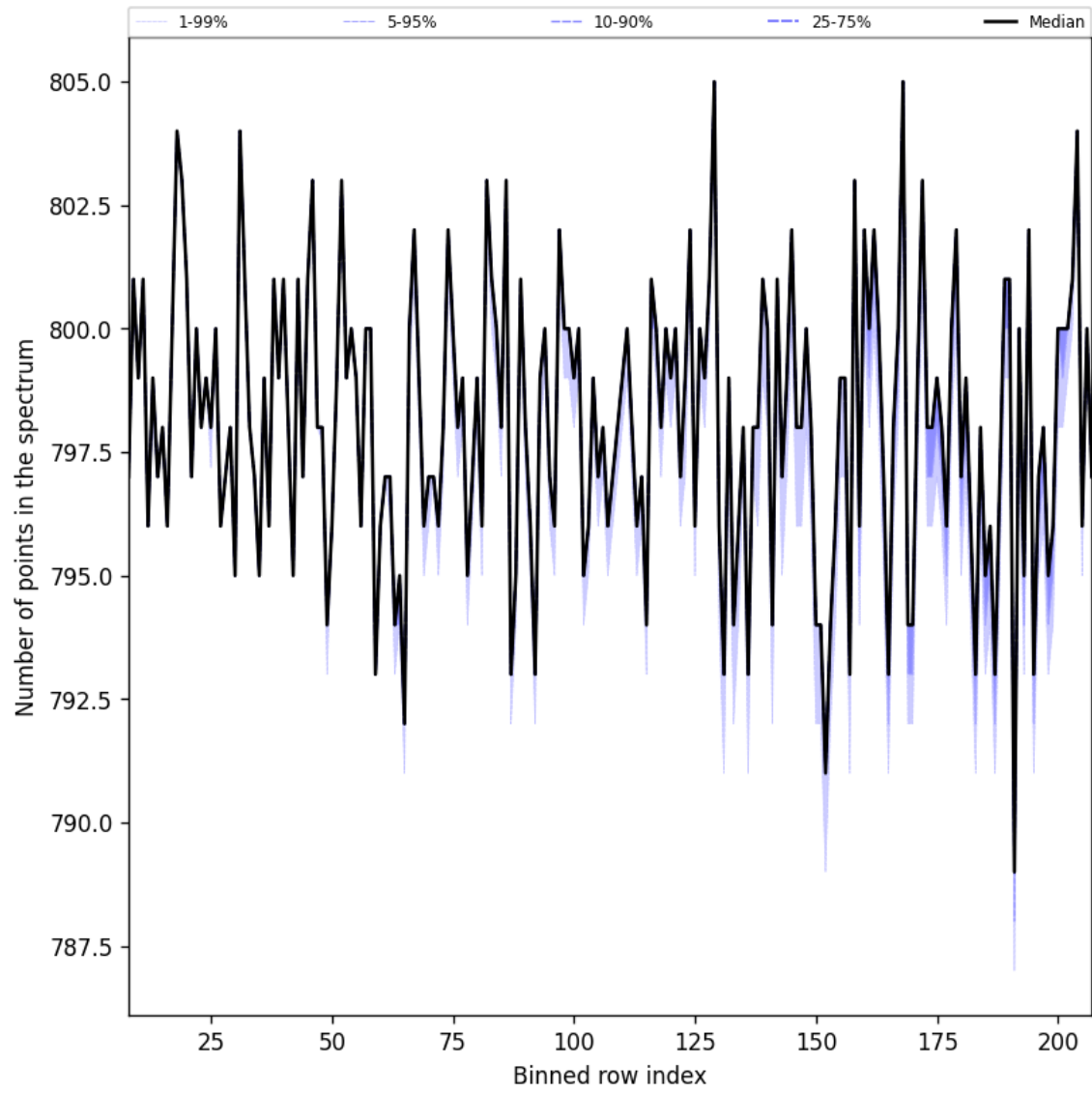
Figure 37: Along track statistics of “Number of points in the spectrum” for 2024-10-10 to 2024-10-12
