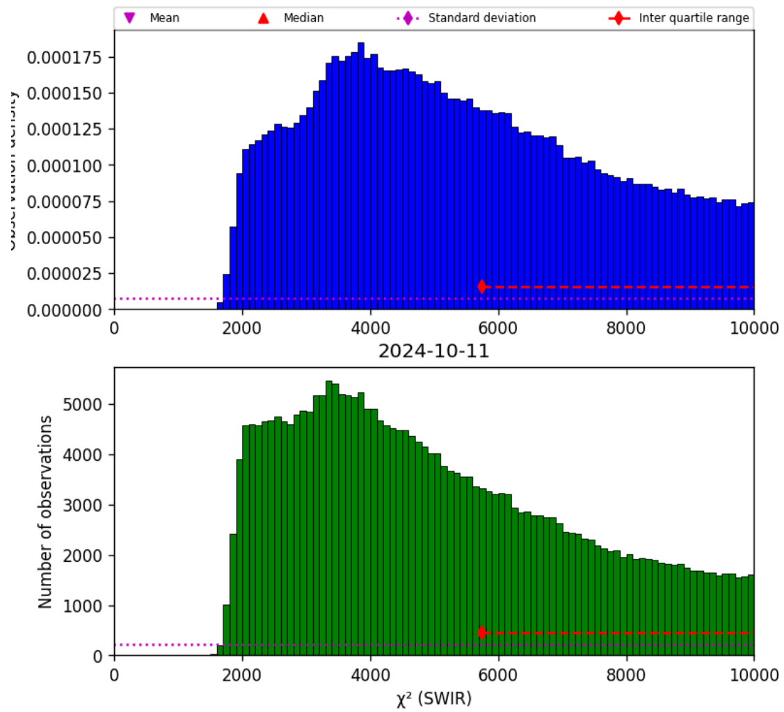
Figure 28: Histogram of “ \chi^2 (SWIR)” for 2024-10-10 to 2024-10-12
