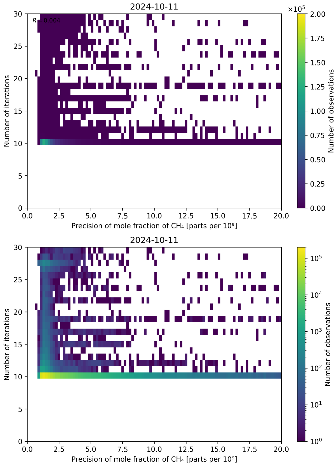
Figure 83: Scatter density plot of “Precision of mole fraction of CH 4 ” against “Number of iterations” for 2024-10-10 to 2024-10-12.
