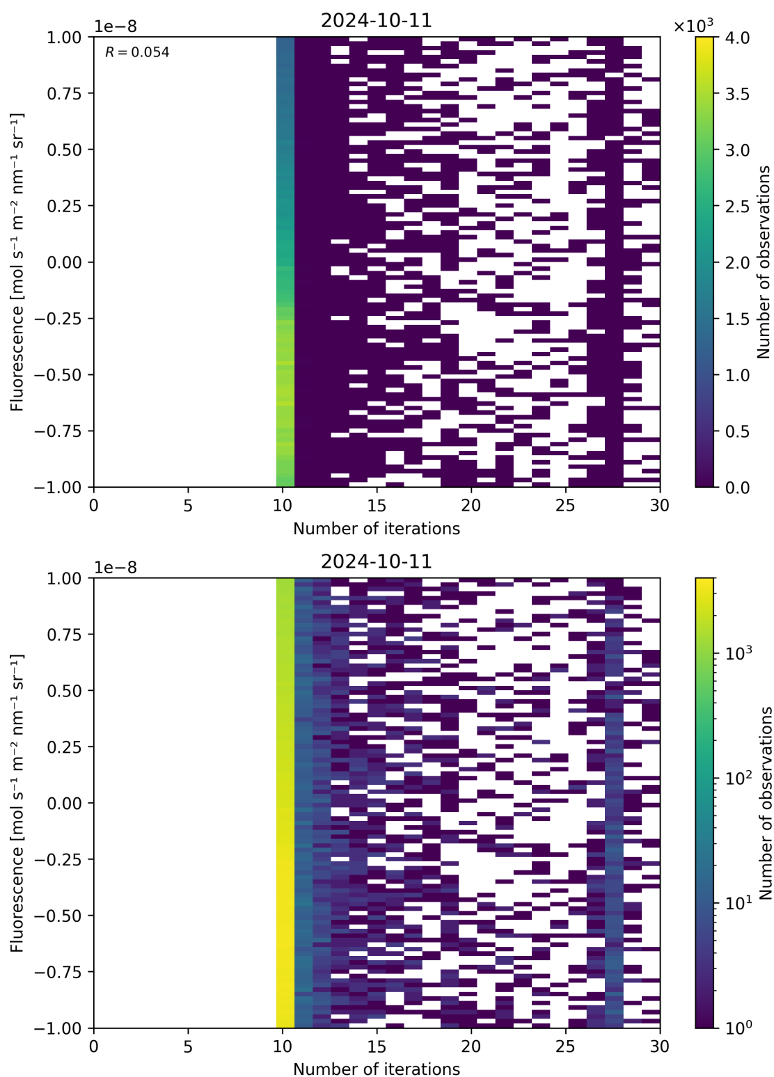
Figure 87: Scatter density plot of “Number of iterations” against “Fluorescence” for 2024-10-10 to 2024-10-12.
