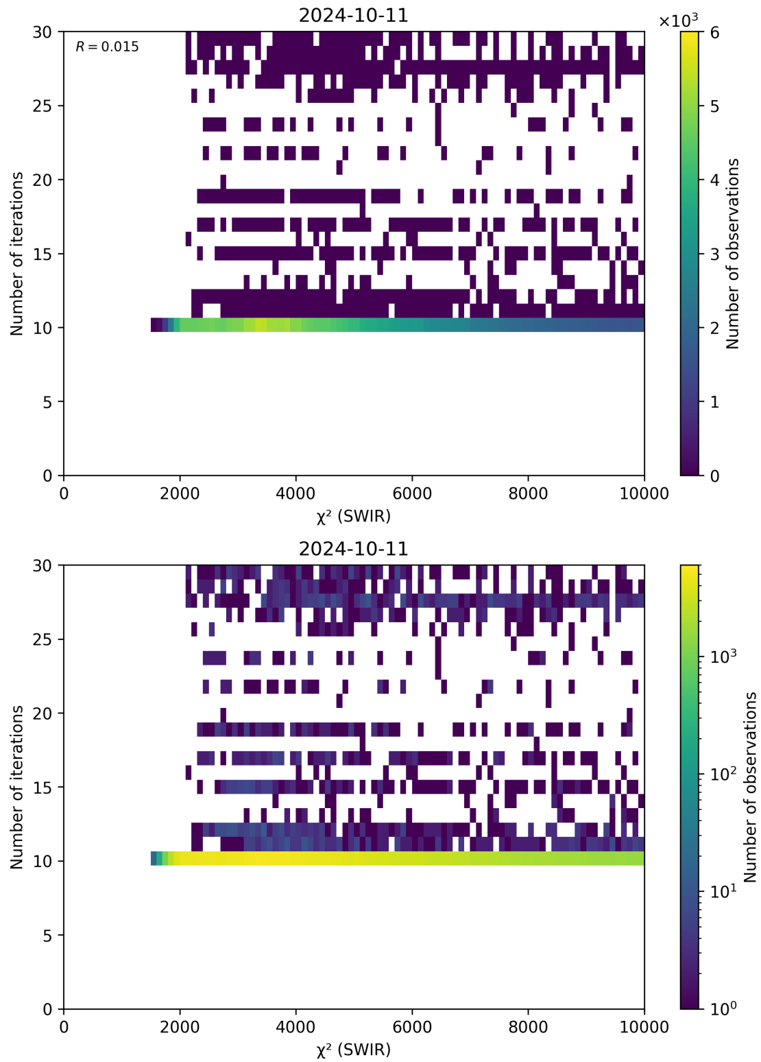
Figure 50: Scatter density plot of " \chi^2 (SWIR)" against "Number of iterations" for 2024-10-10 to 2024-10-12.
