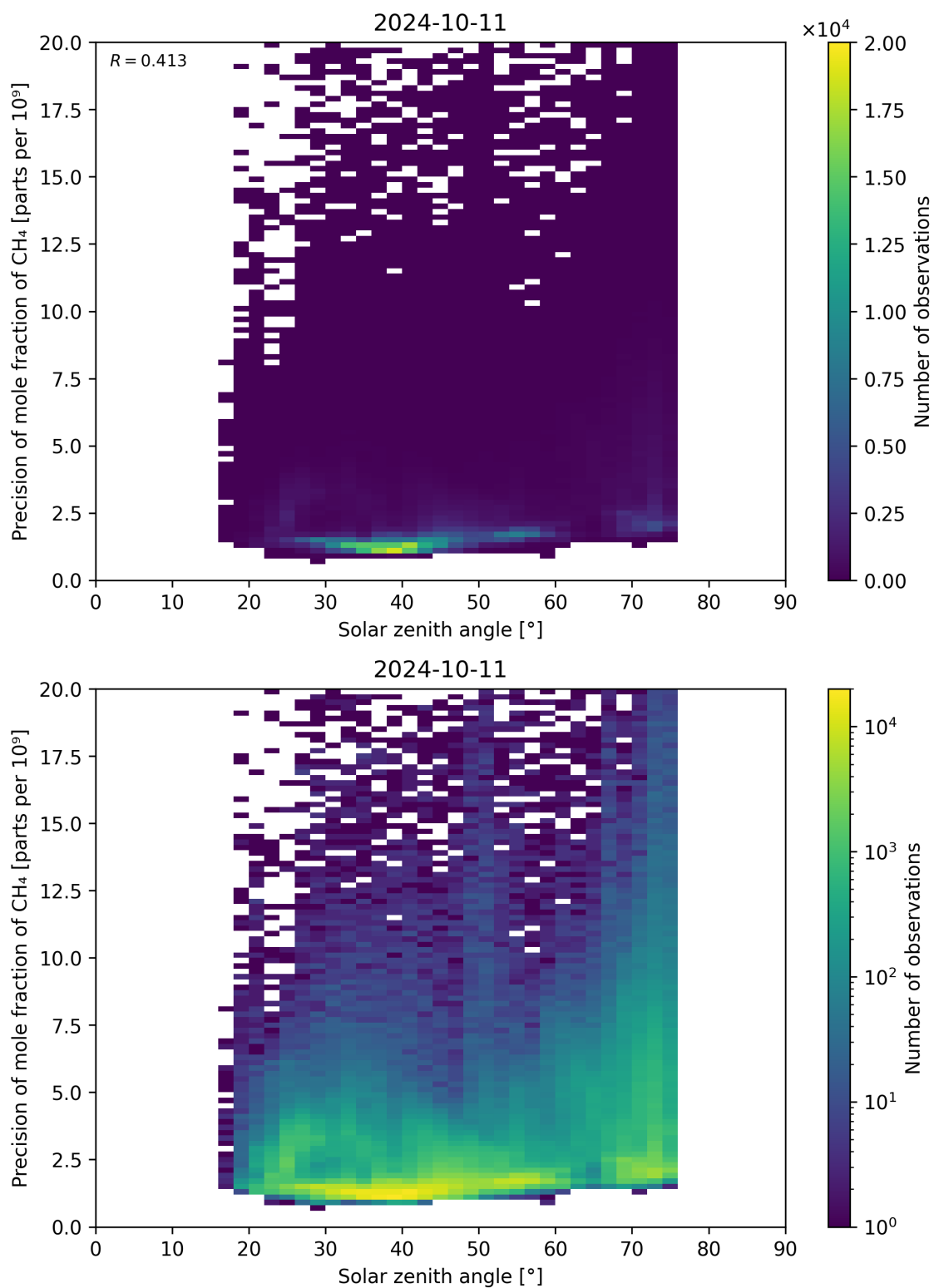
Figure 101: Scatter density plot of “Solar zenith angle” against “Precision of mole fraction of \text{CH}_4 ” for 2024-10-10 to 2024-10-12.
