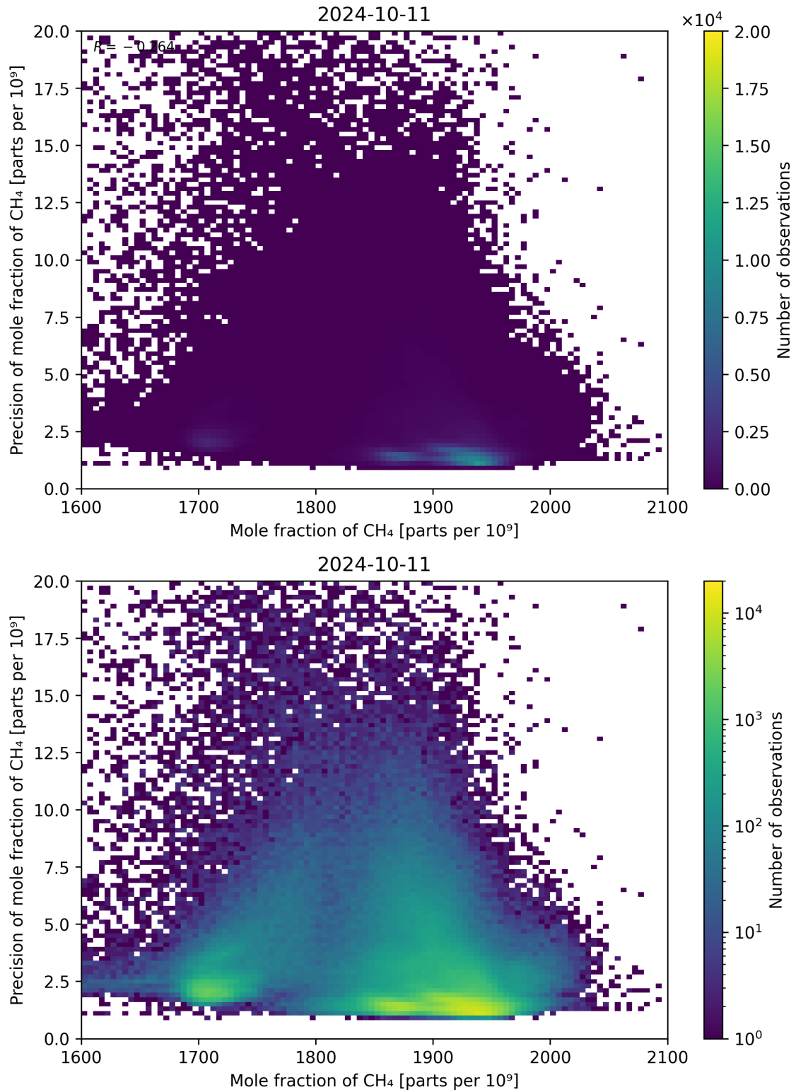
Figure 75: Scatter density plot of “Mole fraction of CH 4 ” against “Precision of mole fraction of CH 4 ” for 2024-10-10 to 2024-10-12.
