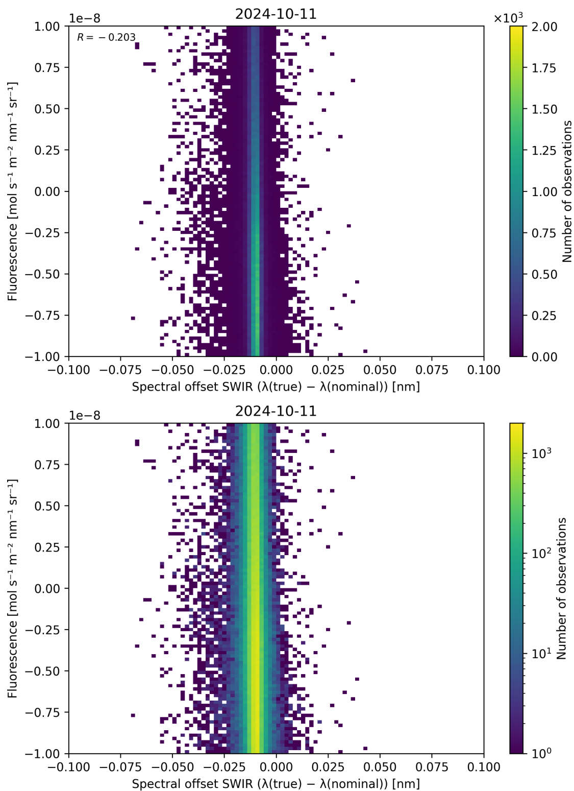
Figure 120: Scatter density plot of “Spectral offset SWIR ( \lambda_{\text{true}} - \lambda_{\text{nominal}} )” against “Fluorescence” for 2024-10-10 to 2024-10-12.
