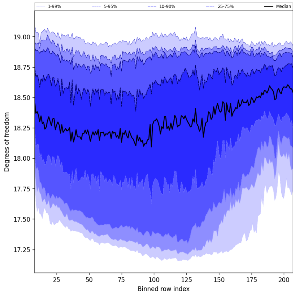
Figure 41: Along track statistics of “Degrees of freedom” for 2024-10-10 to 2024-10-12
