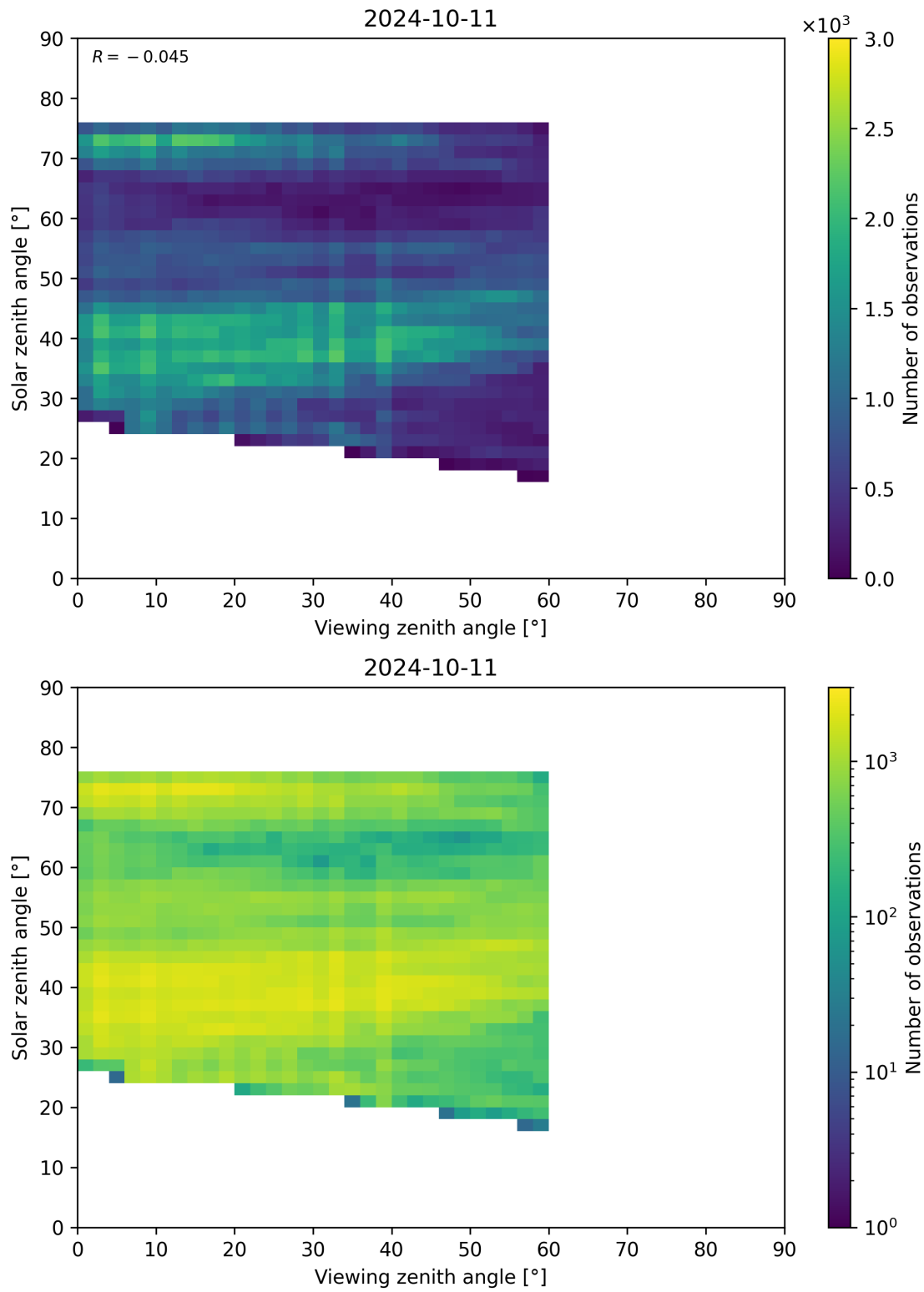
Figure 115: Scatter density plot of “Viewing zenith angle” against “Solar zenith angle” for 2024-10-10 to 2024-10-12.
