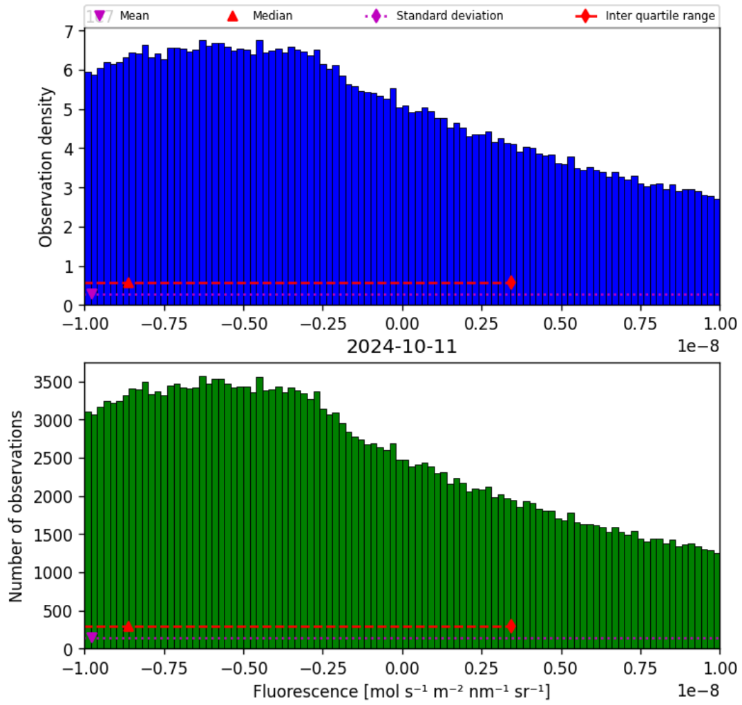
Figure 32: Histogram of “Fluorescence” for 2024-10-10 to 2024-10-12
