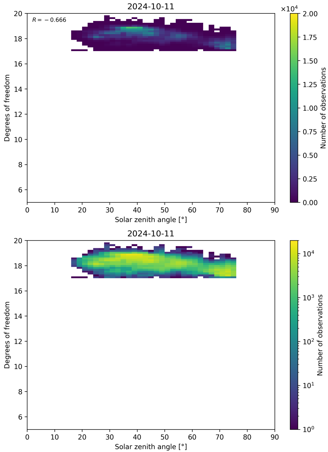
Figure 96: Scatter density plot of “Solar zenith angle” against “Degrees of freedom” for 2024-10-10 to 2024-10-12.
