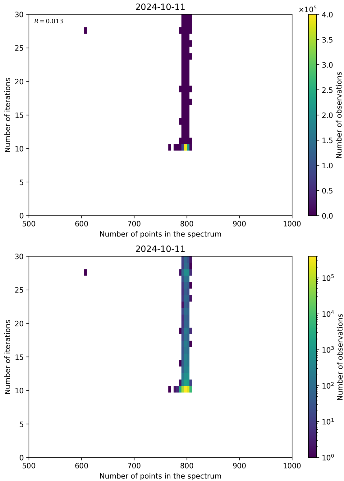
Figure 92: Scatter density plot of “Number of points in the spectrum” against “Number of iterations” for 2024-10-10 to 2024-10-12.
