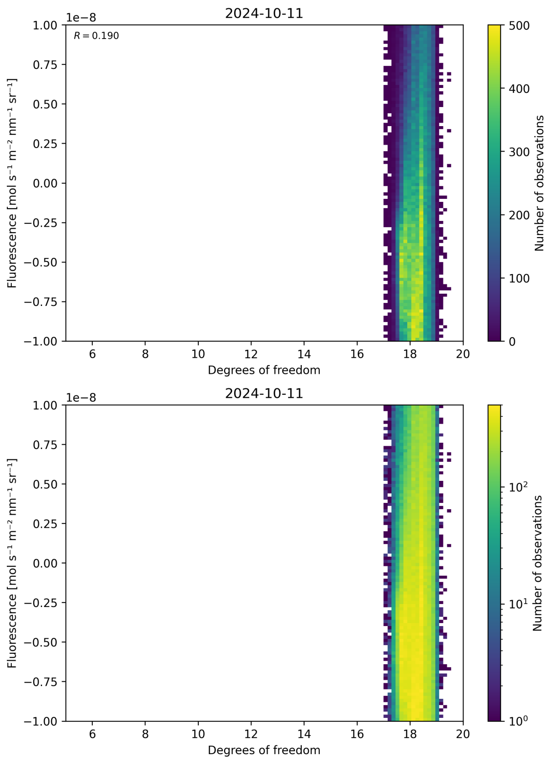
Figure 51: Scatter density plot of “Degrees of freedom” against “Fluorescence” for 2024-10-10 to 2024-10-12.
