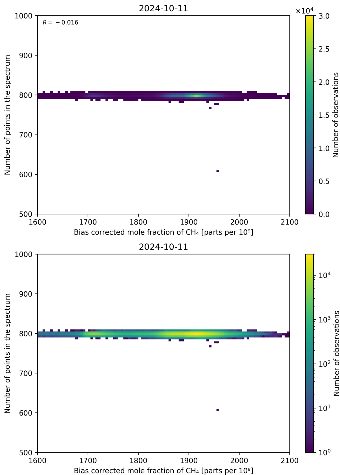
Figure 68: Scatter density plot of “Bias corrected mole fraction of CH 4 ” against “Number of points in the spectrum” for 2024-10-10 to 2024-10-12.
