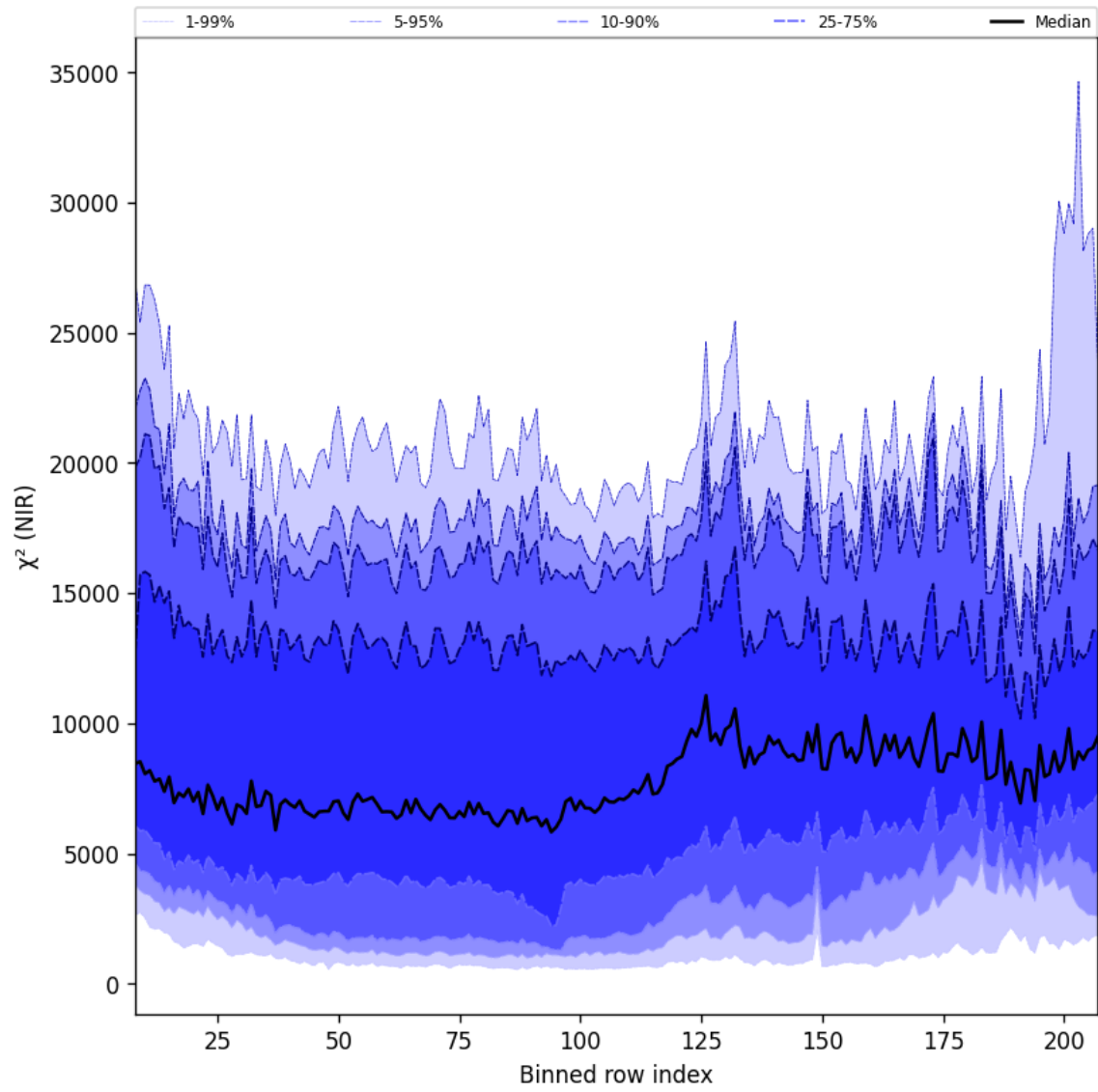
Figure 40: Along track statistics of “ \chi^2 (NIR)” for 2024-10-10 to 2024-10-12
