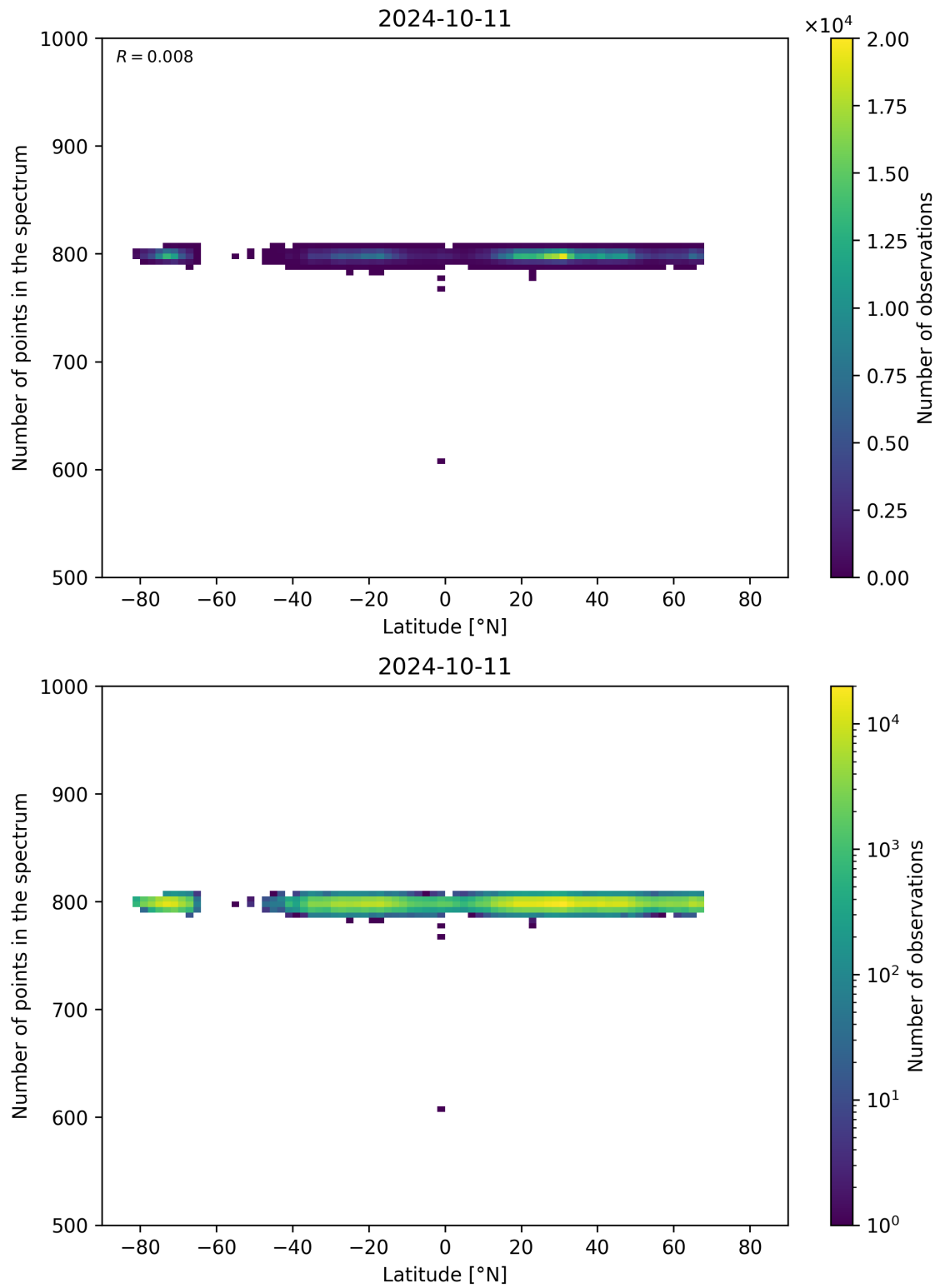
Figure 61: Scatter density plot of “Latitude” against “Number of points in the spectrum” for 2024-10-10 to 2024-10-12.
