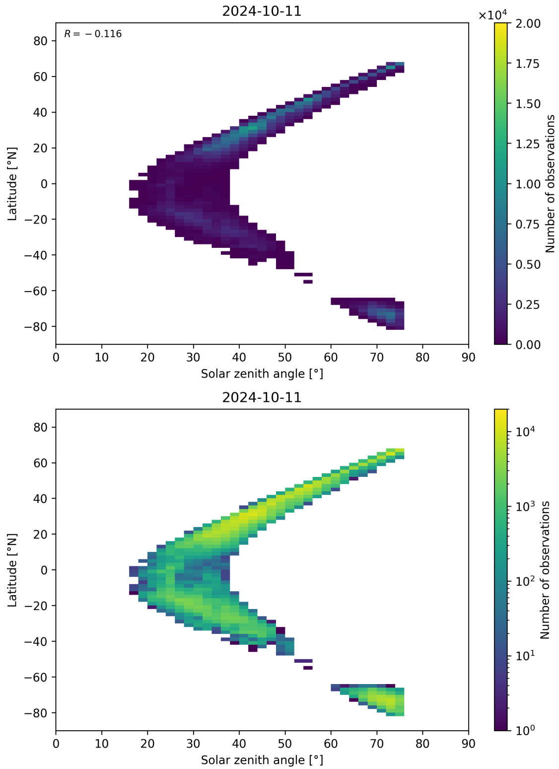
Figure 98: Scatter density plot of “Solar zenith angle” against “Latitude” for 2024-10-10 to 2024-10-12.
