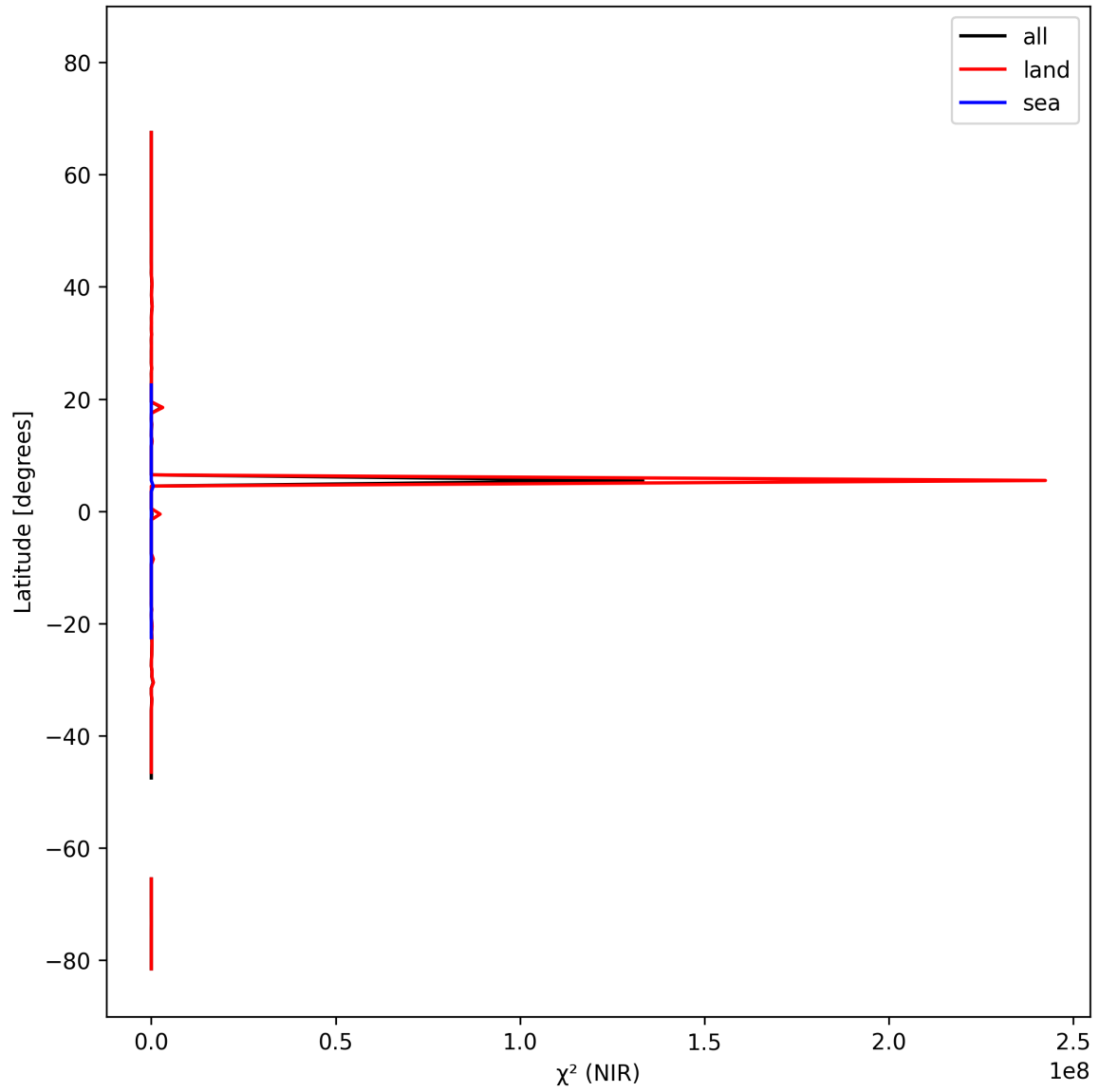
Figure 18: Zonal average of “ \chi^2 (NIR)” for 2024-10-10 to 2024-10-12.
