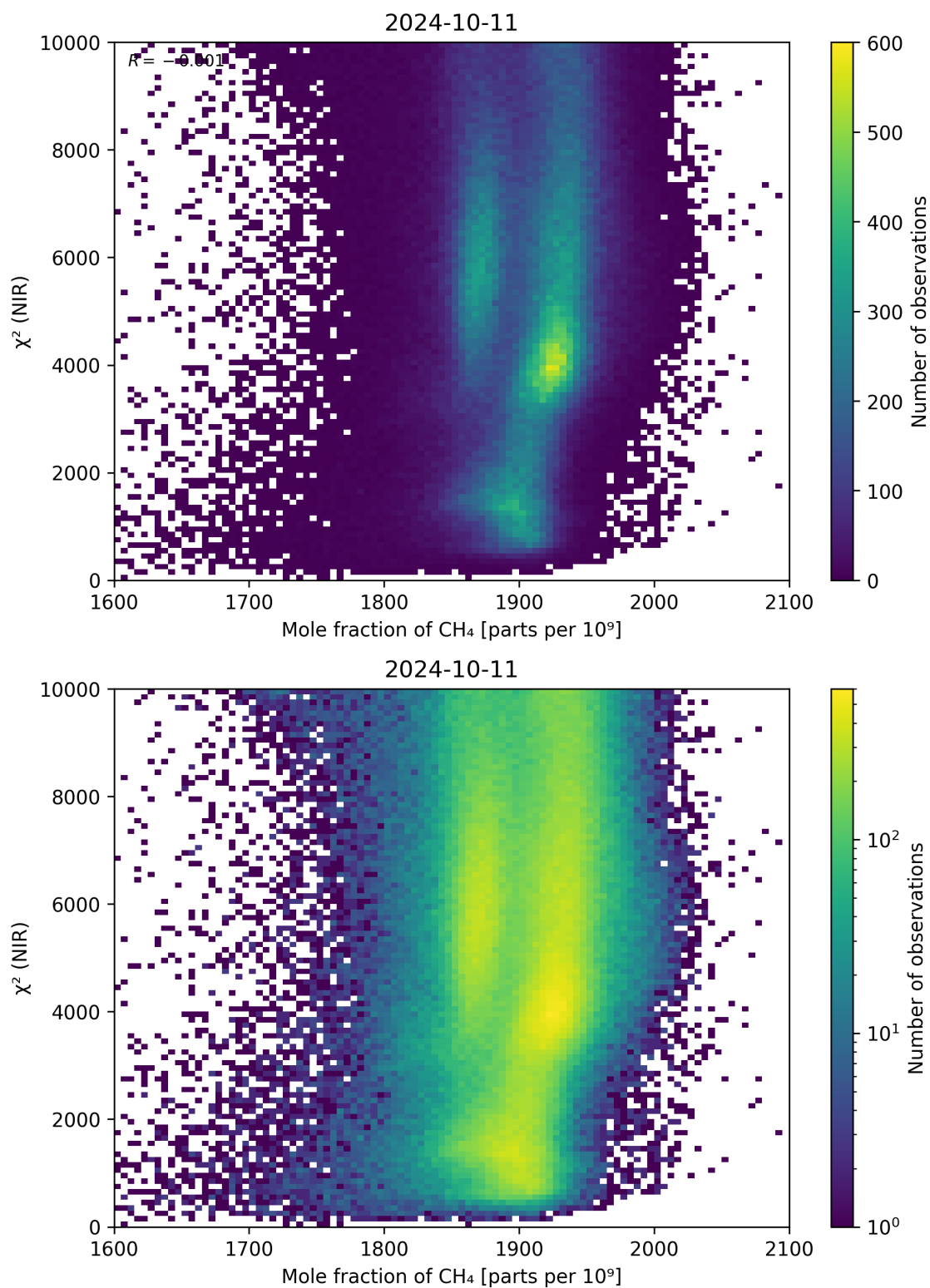
Figure 70: Scatter density plot of “Mole fraction of \text{CH}_4 ” against “ \chi^2 (NIR)” for 2024-10-10 to 2024-10-12.
