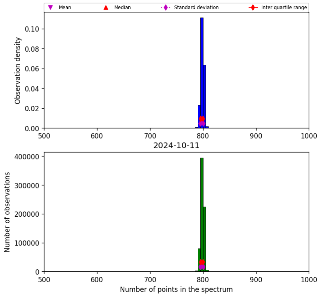
Figure 26: Histogram of “Number of points in the spectrum” for 2024-10-10 to 2024-10-12
