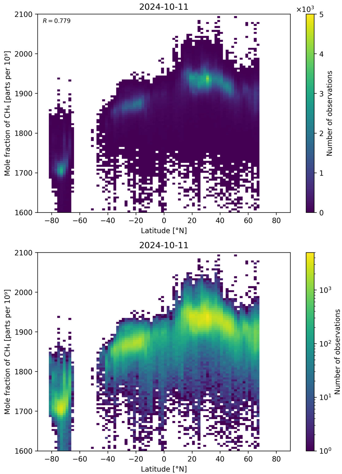
Figure 57: Scatter density plot of “Latitude” against “Mole fraction of \text{CH}_4 ” for 2024-10-10 to 2024-10-12.
