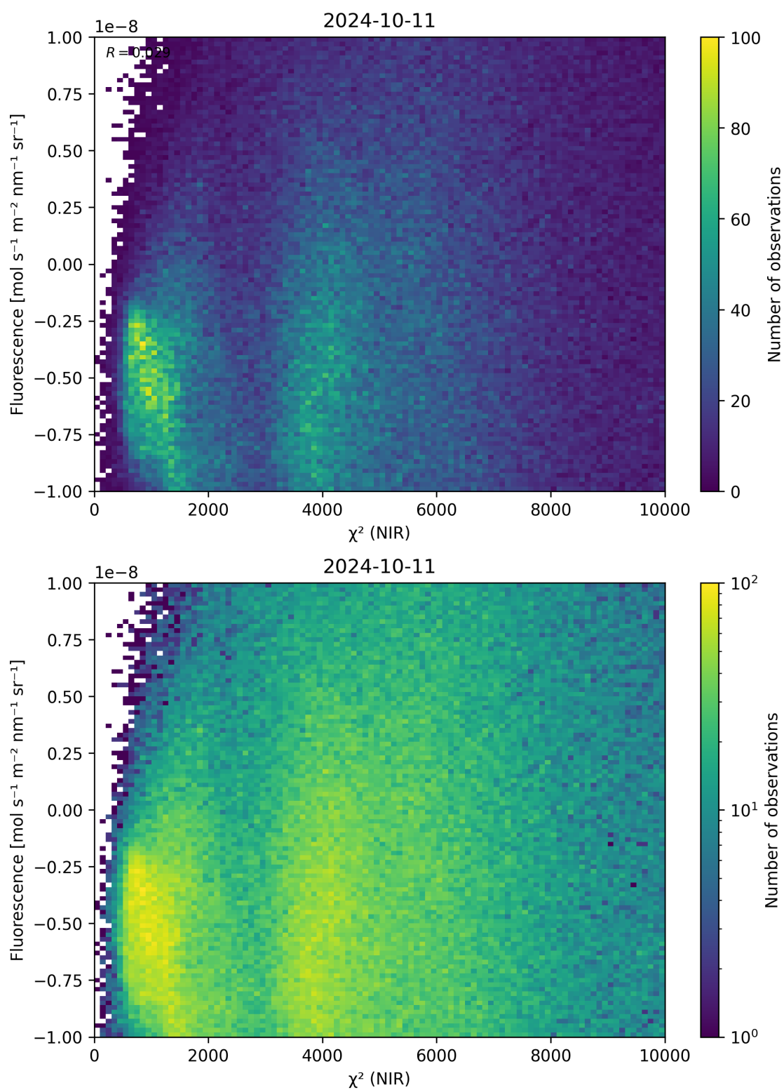
Figure 45: Scatter density plot of “ \chi^2 (NIR)” against “Fluorescence” for 2024-10-10 to 2024-10-12.
