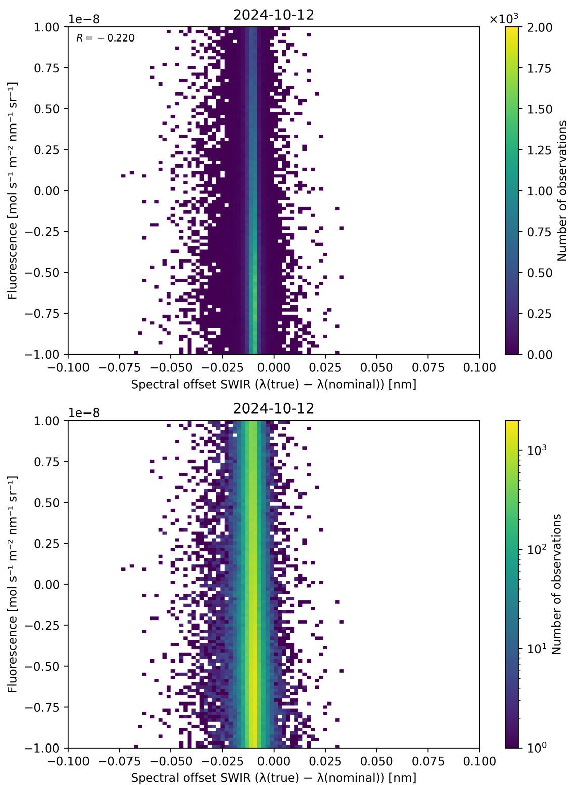
Figure 120: Scatter density plot of “Spectral offset SWIR ( \lambda_{\text{true}} - \lambda_{\text{nominal}} )” against “Fluorescence” for 2024-10-11 to 2024-10-13.
