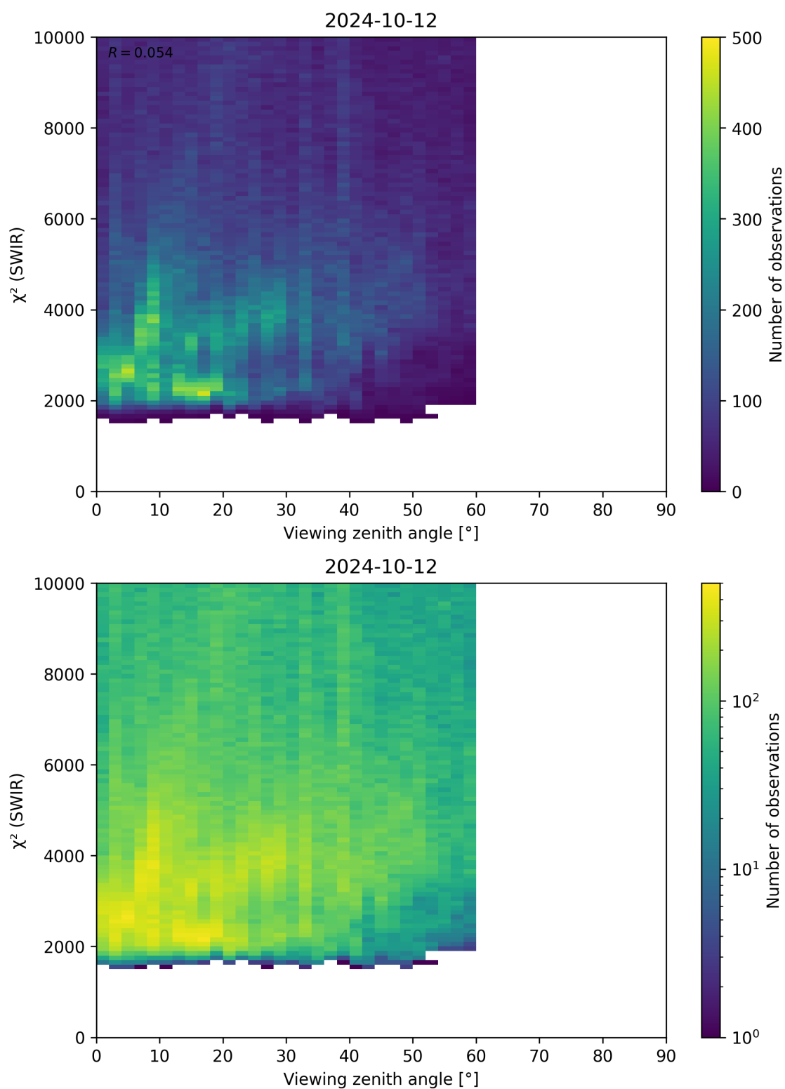
Figure 106: Scatter density plot of “Viewing zenith angle” against “ \chi^2 (SWIR)” for 2024-10-11 to 2024-10-13.
