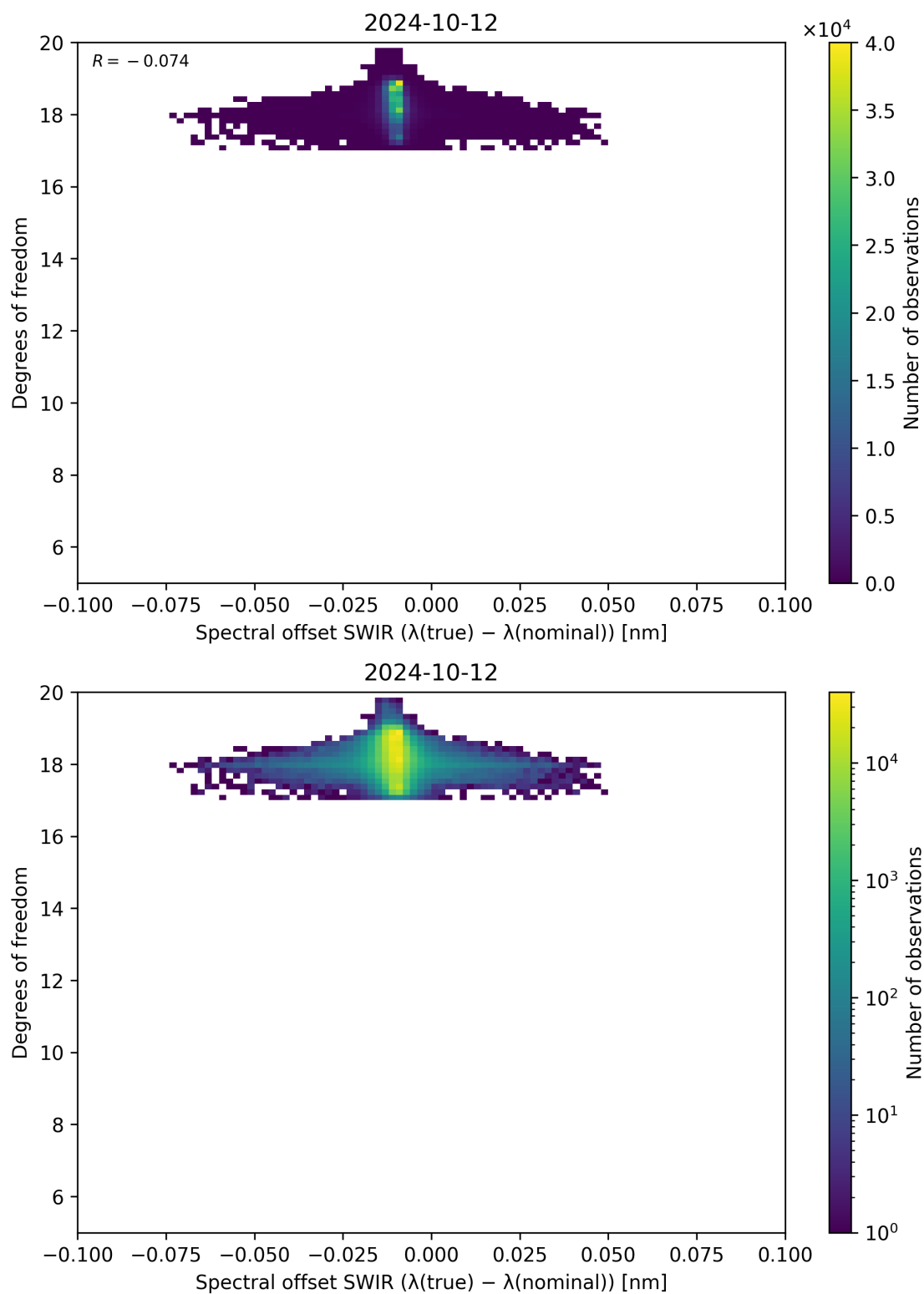
Figure 119: Scatter density plot of “Spectral offset SWIR ( \lambda_{\text{true}} - \lambda_{\text{nominal}} )” against “Degrees of freedom” for 2024-10-11 to 2024-10-13.
