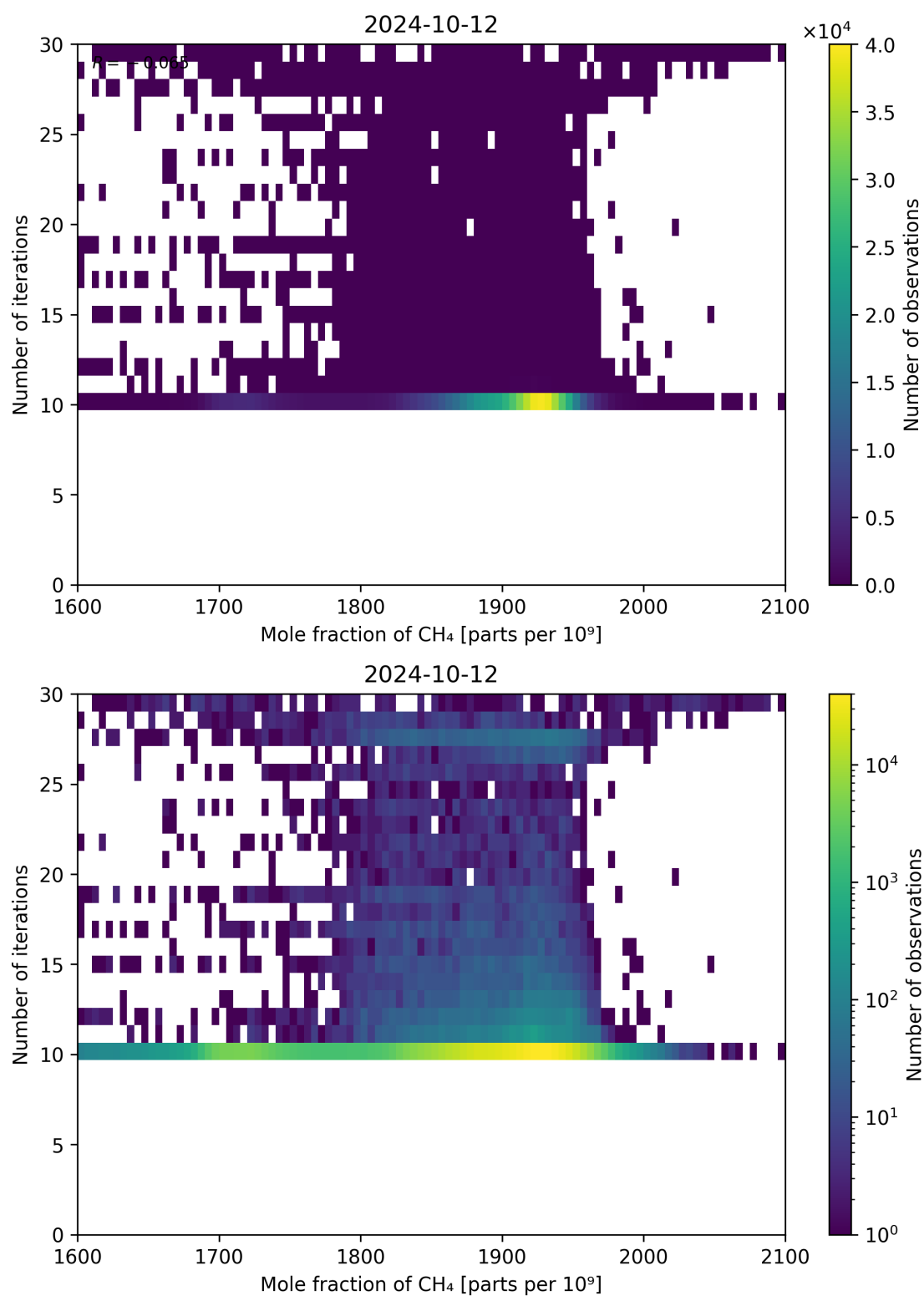
Figure 76: Scatter density plot of “Mole fraction of CH 4 ” against “Number of iterations” for 2024-10-11 to 2024-10-13.
