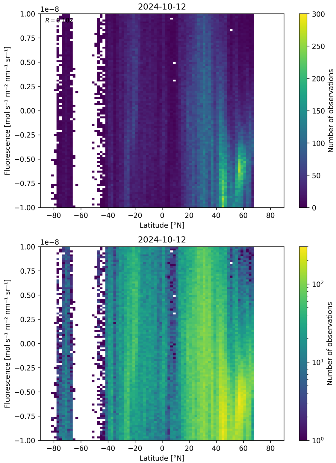
Figure 56: Scatter density plot of “Latitude” against “Fluorescence” for 2024-10-11 to 2024-10-13.
