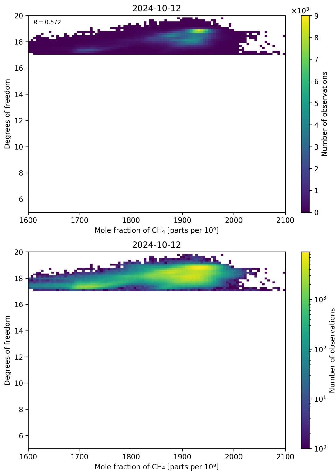
Figure 72: Scatter density plot of “Mole fraction of CH 4 ” against “Degrees of freedom” for 2024-10-11 to 2024-10-13.
