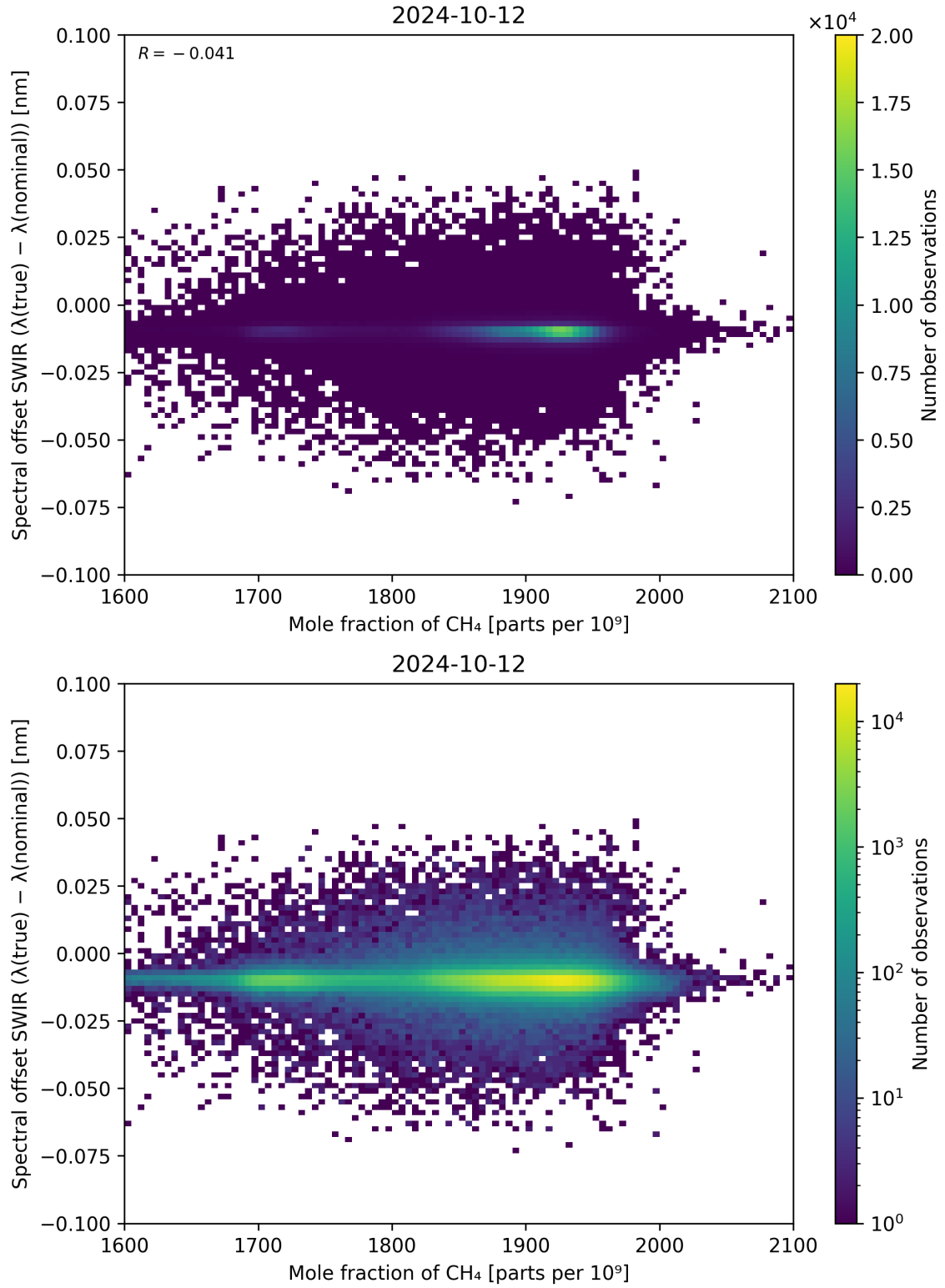
Figure 86: Scatter density plot of “Mole fraction of CH 4 ” against “Spectral offset SWIR ( \lambda_{\text{true}} - \lambda_{\text{nominal}} )” for 2024-10-11 to 2024-10-13.
