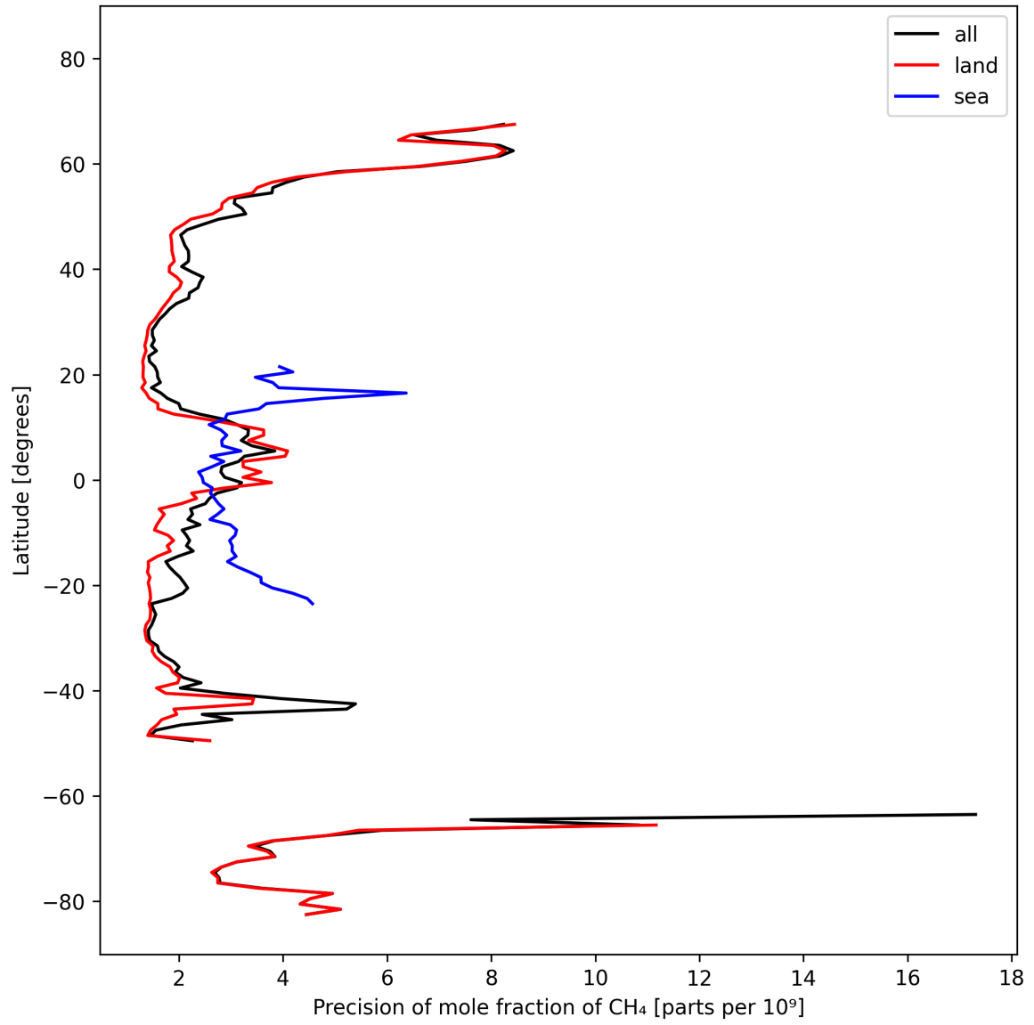
Figure 13: Zonal average of “Precision of mole fraction of CH 4 ” for 2024-10-11 to 2024-10-13.
