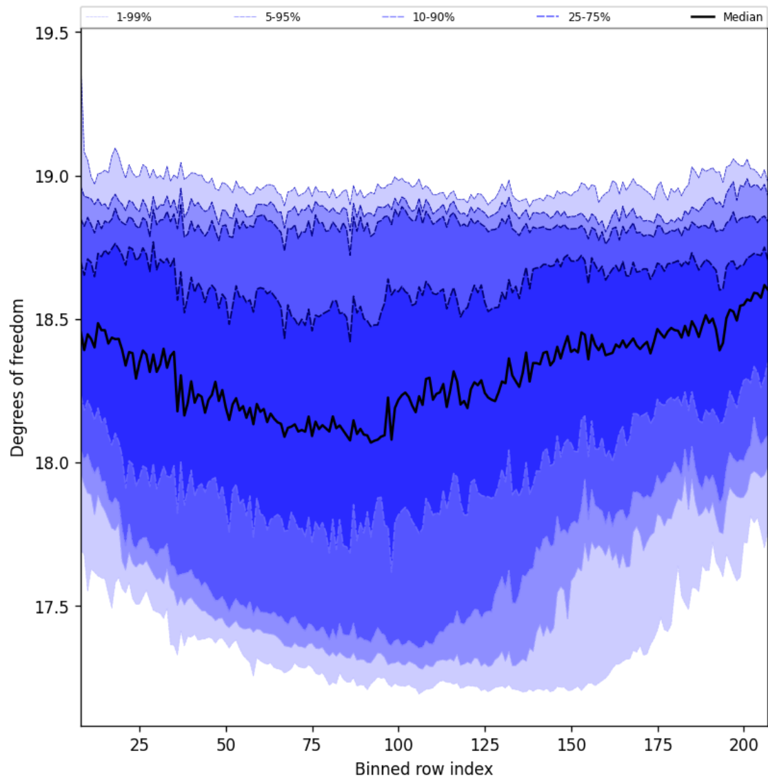
Figure 41: Along track statistics of “Degrees of freedom” for 2024-10-11 to 2024-10-13
