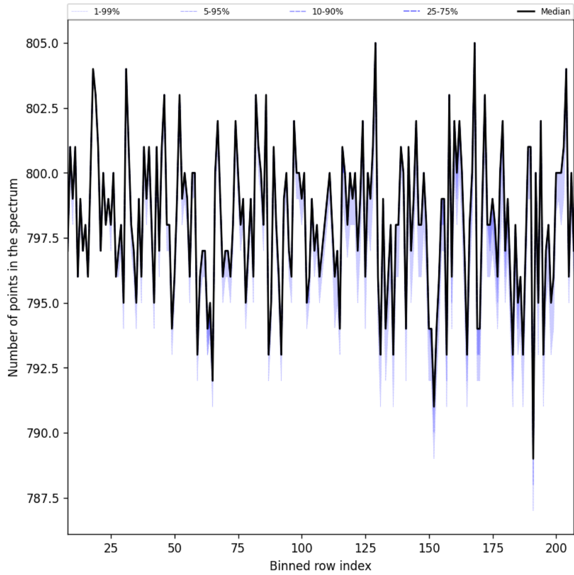
Figure 37: Along track statistics of “Number of points in the spectrum” for 2024-10-11 to 2024-10-13
