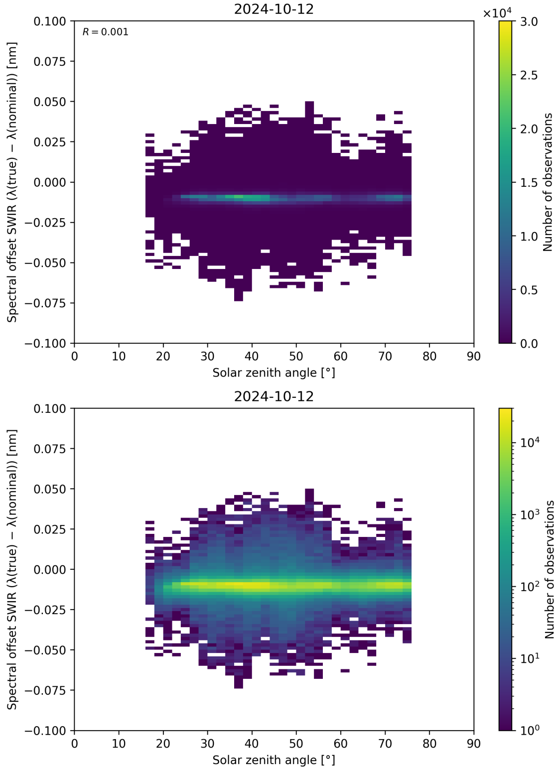
Figure 104: Scatter density plot of “Solar zenith angle” against “Spectral offset SWIR ( \lambda_{\text{true}} - \lambda_{\text{nominal}} )” for 2024-10-11 to 2024-10-13.
