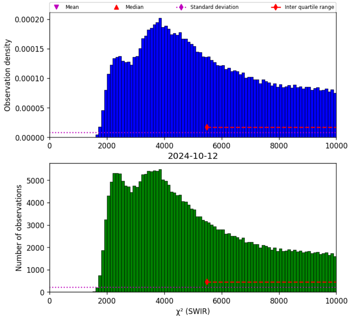
Figure 28: Histogram of “ \chi^2 (SWIR)” for 2024-10-11 to 2024-10-13
