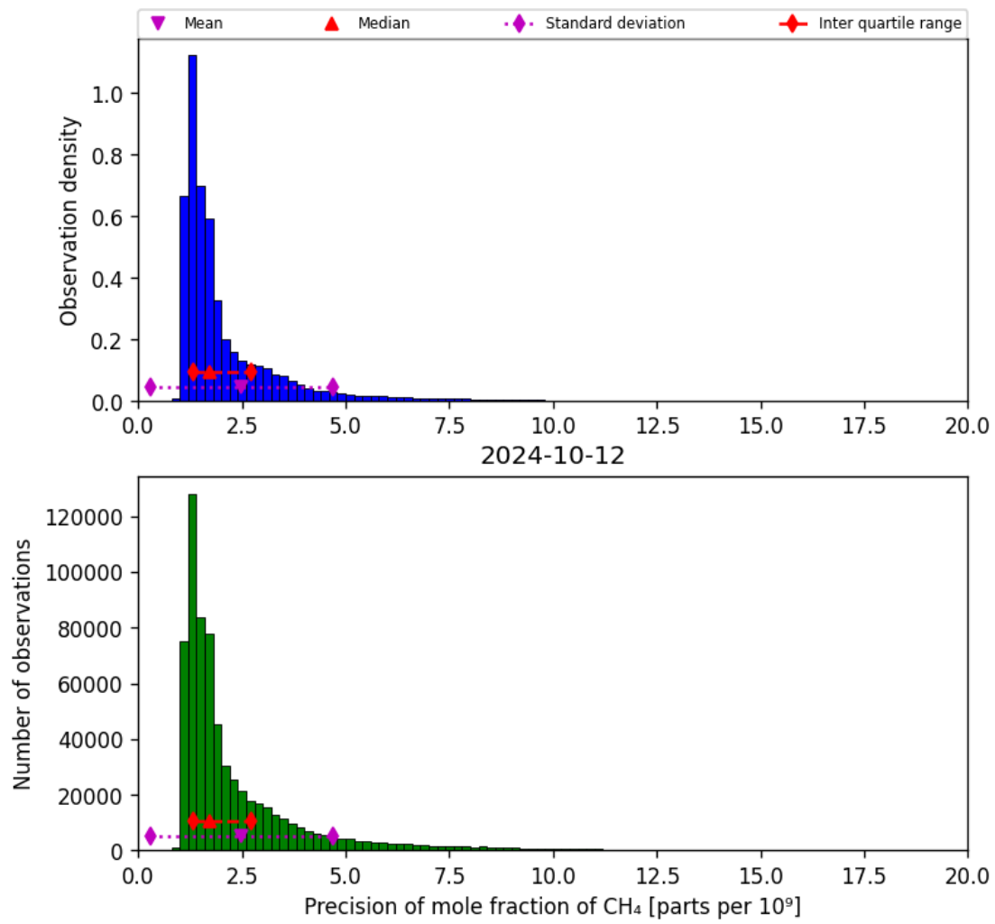
Figure 24: Histogram of “Precision of mole fraction of CH 4 ” for 2024-10-11 to 2024-10-13
