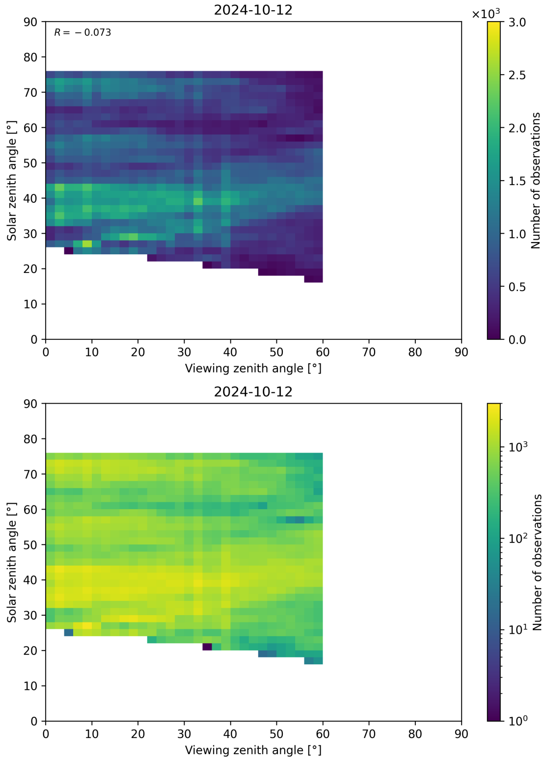
Figure 115: Scatter density plot of “Viewing zenith angle” against “Solar zenith angle” for 2024-10-11 to 2024-10-13.
