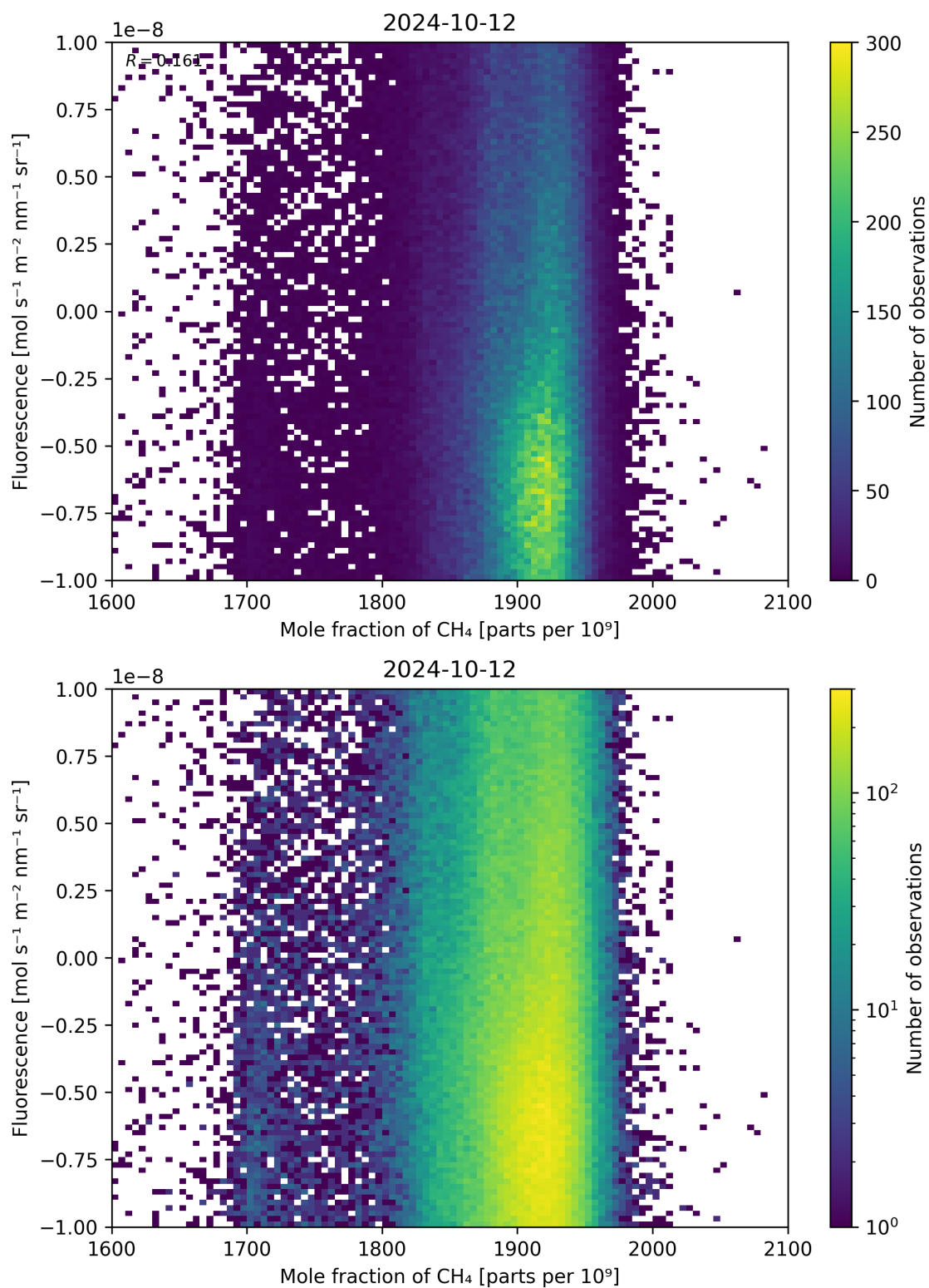
Figure 73: Scatter density plot of “Mole fraction of \text{CH}_4 ” against “Fluorescence” for 2024-10-11 to 2024-10-13.
