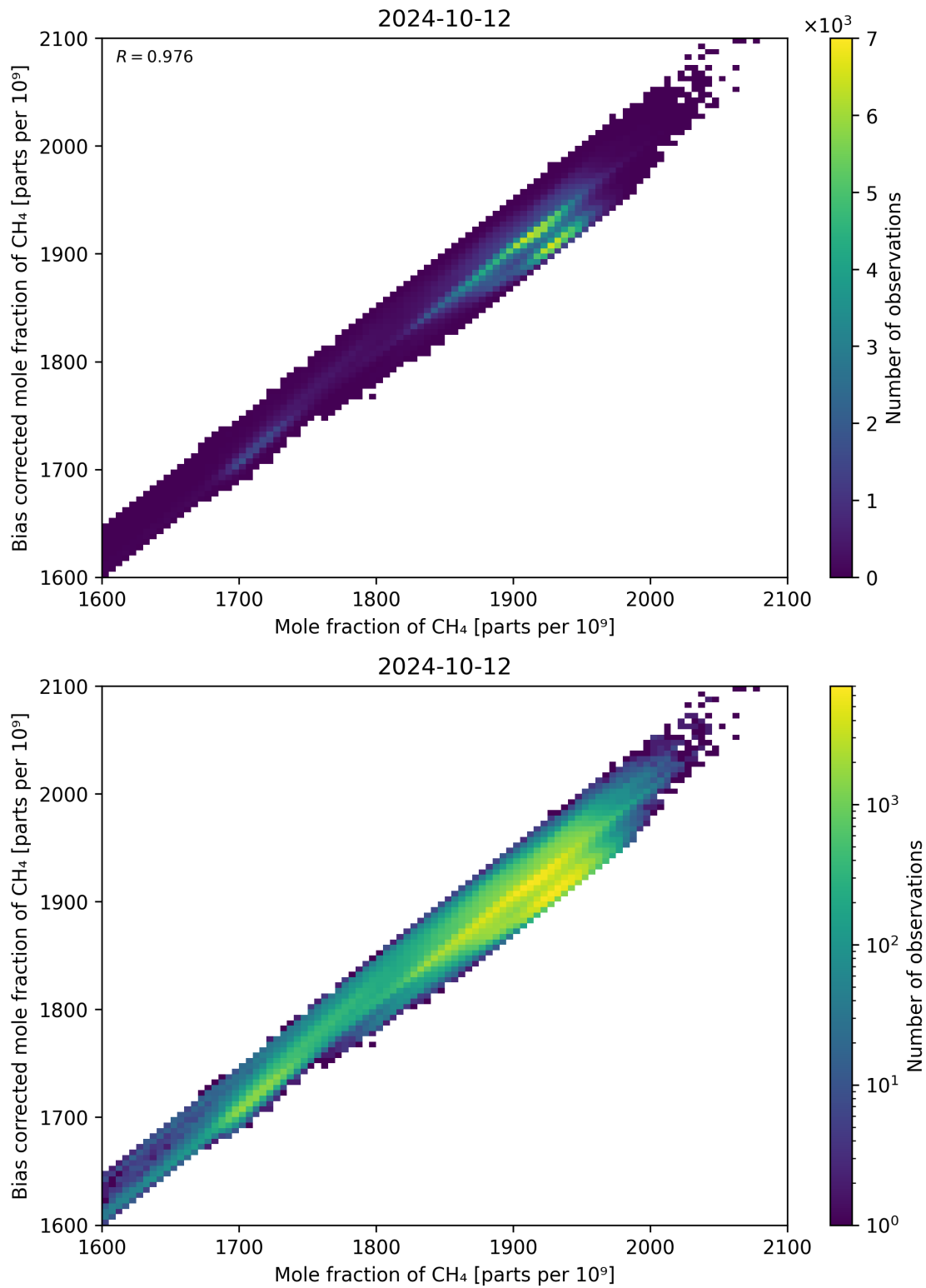
Figure 74: Scatter density plot of “Mole fraction of CH 4 ” against “Bias corrected mole fraction of CH 4 ” for 2024-10-11 to 2024-10-13.
