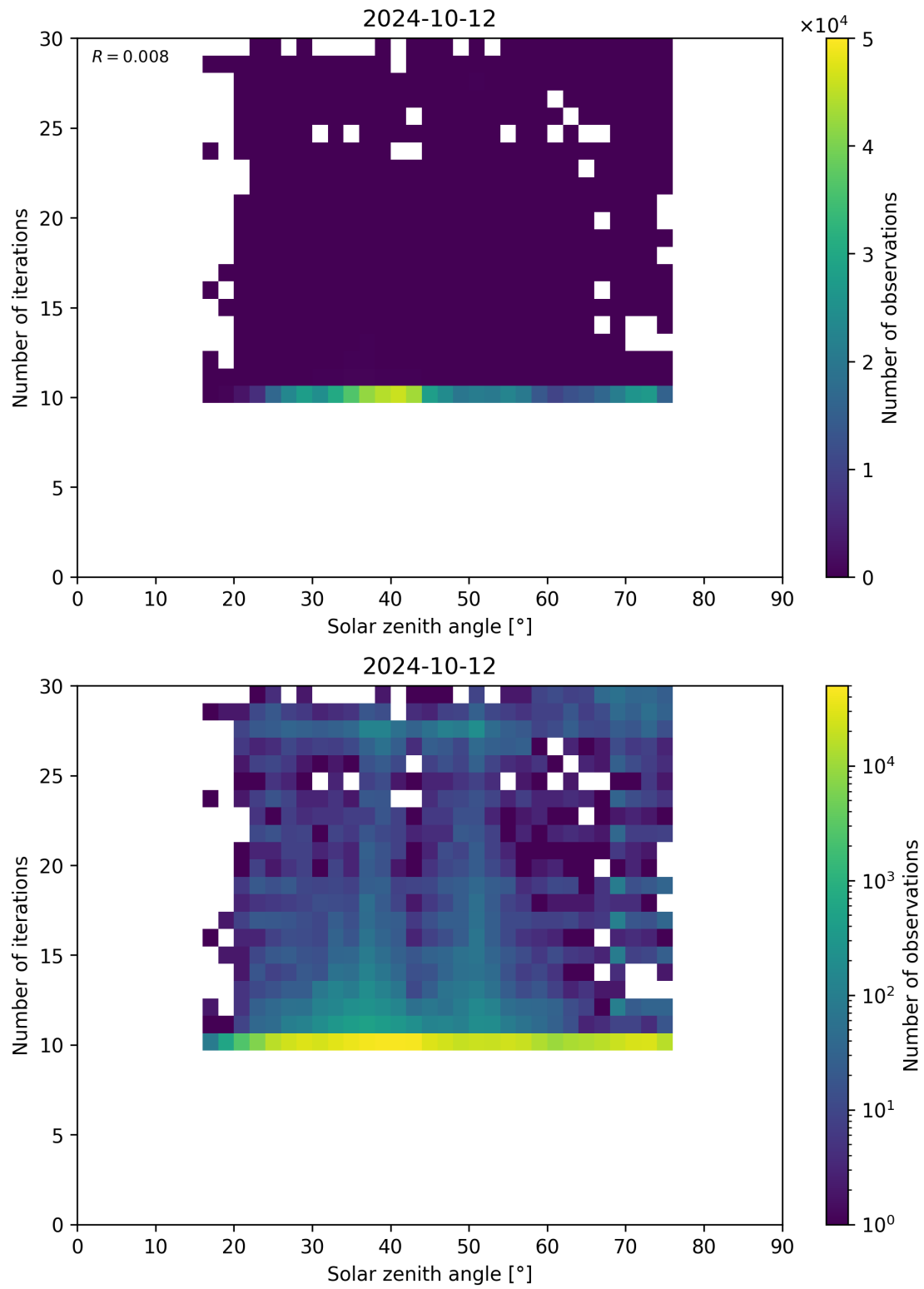
Figure 102: Scatter density plot of “Solar zenith angle” against “Number of iterations” for 2024-10-11 to 2024-10-13.
