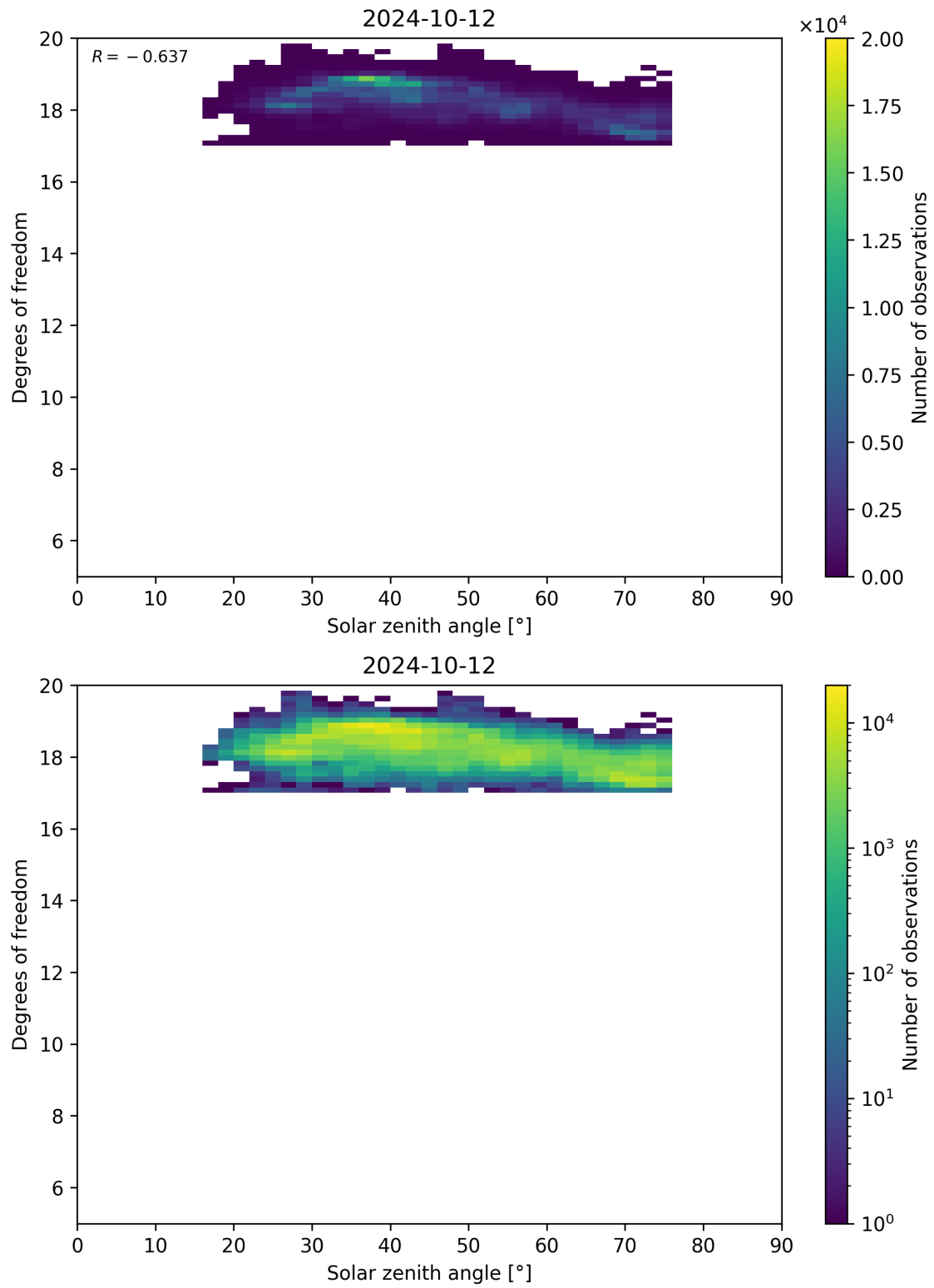
Figure 96: Scatter density plot of “Solar zenith angle” against “Degrees of freedom” for 2024-10-11 to 2024-10-13.
