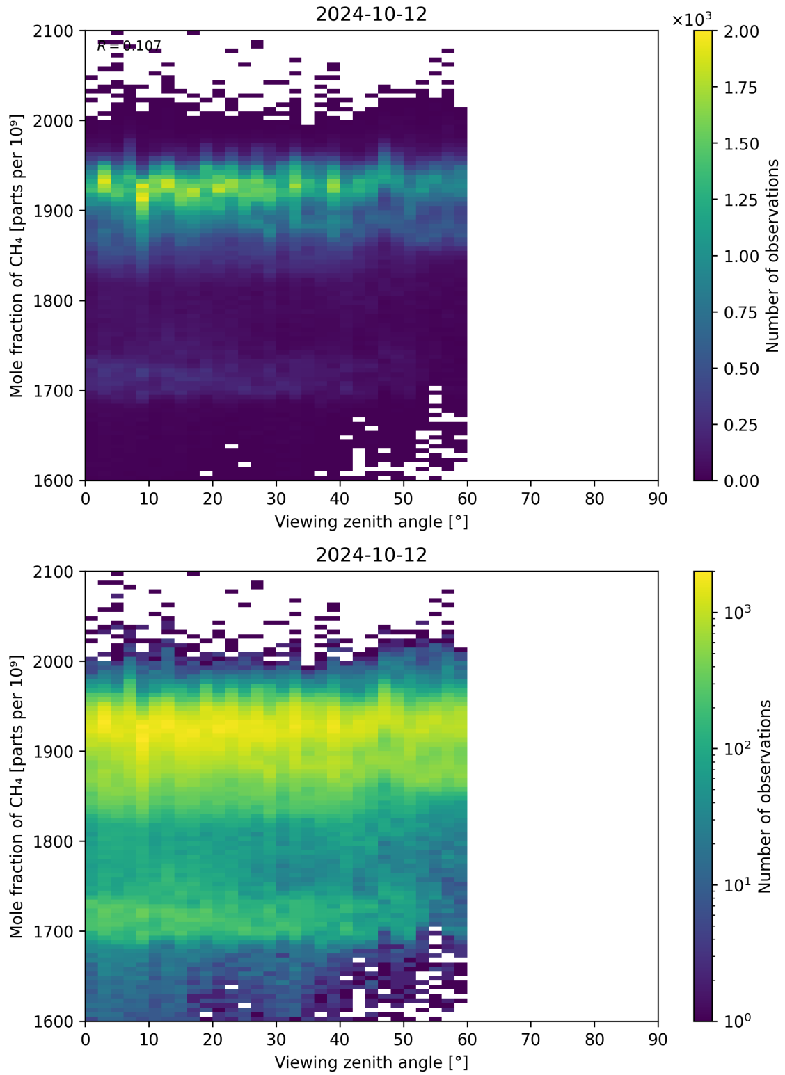
Figure 110: Scatter density plot of “Viewing zenith angle” against “Mole fraction of CH 4 ” for 2024-10-11 to 2024-10-13.
