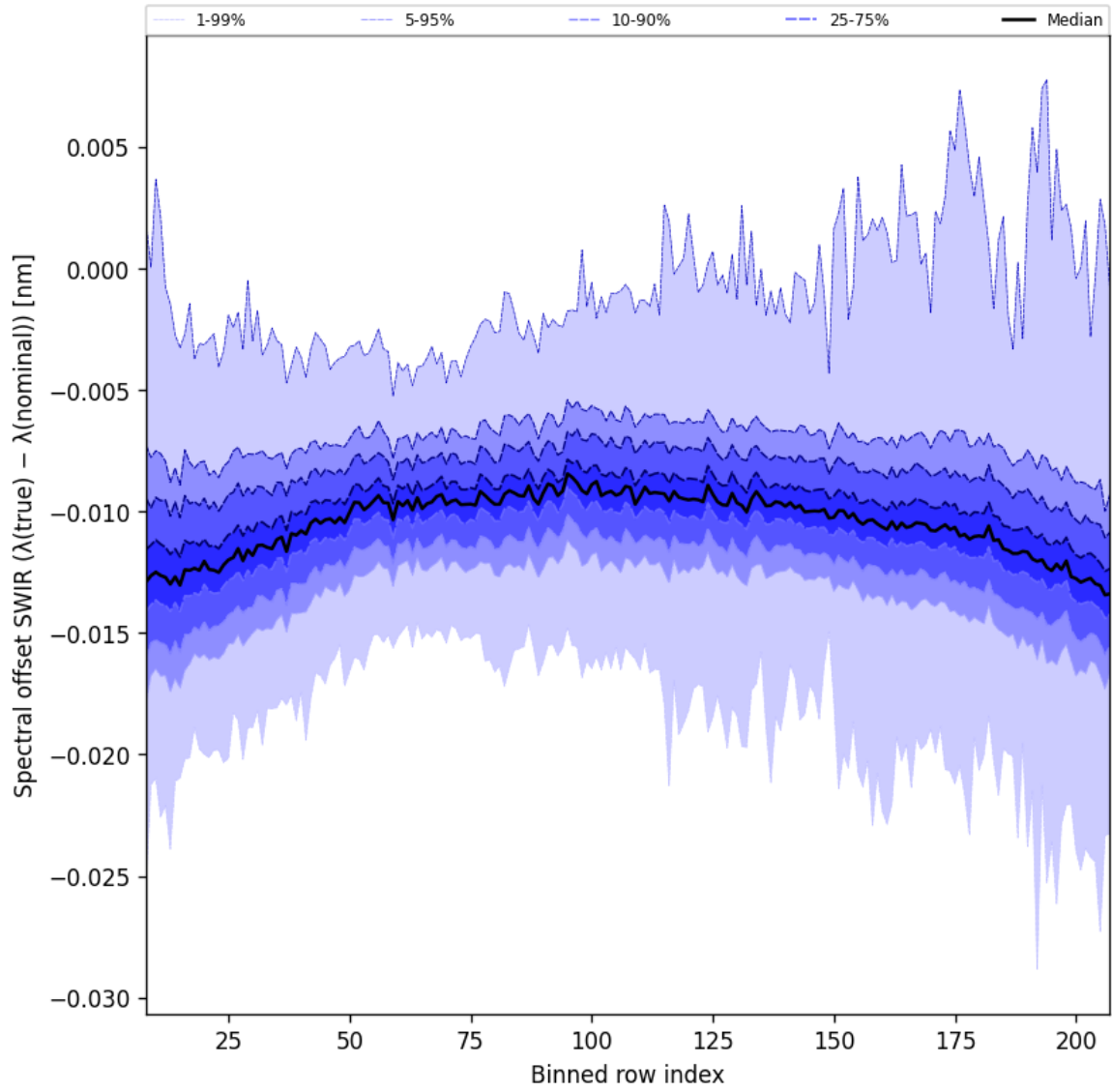
Figure 38: Along track statistics of “Spectral offset SWIR ( \lambda_{\text{true}} - \lambda_{\text{nominal}} )” for 2024-10-11 to 2024-10-13
