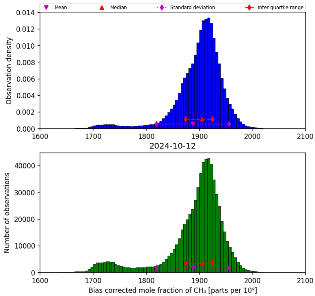
Figure 25: Histogram of “Bias corrected mole fraction of CH 4 ” for 2024-10-11 to 2024-10-13
