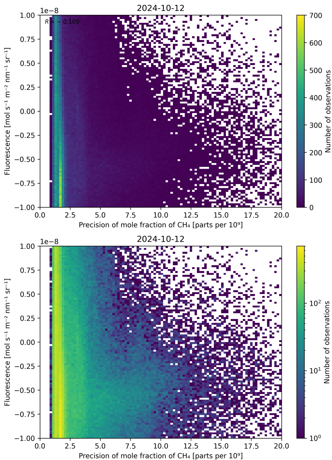
Figure 81: Scatter density plot of “Precision of mole fraction of CH 4 ” against “Fluorescence” for 2024-10-11 to 2024-10-13.
