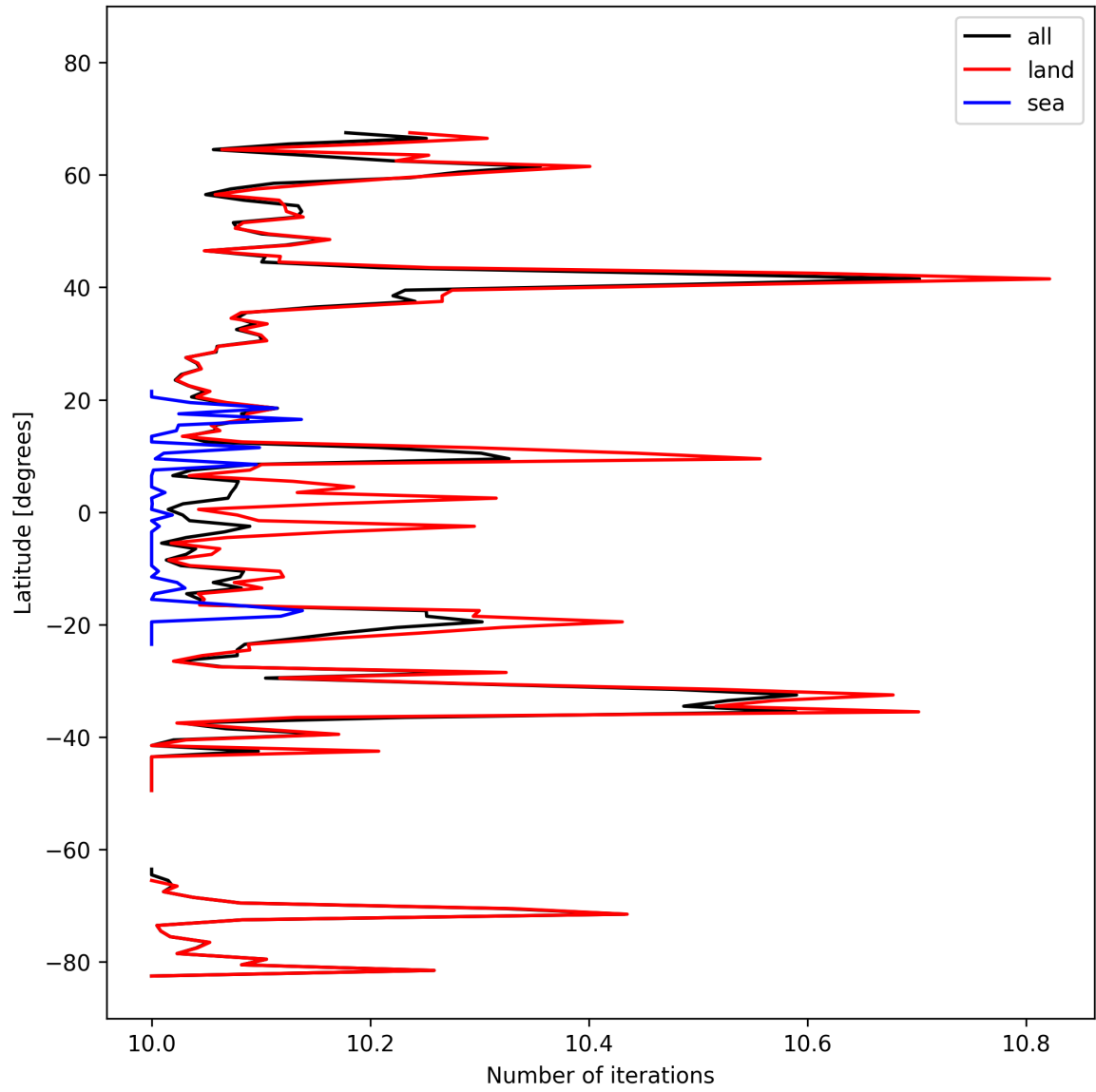
Figure 20: Zonal average of “Number of iterations” for 2024-10-11 to 2024-10-13.
