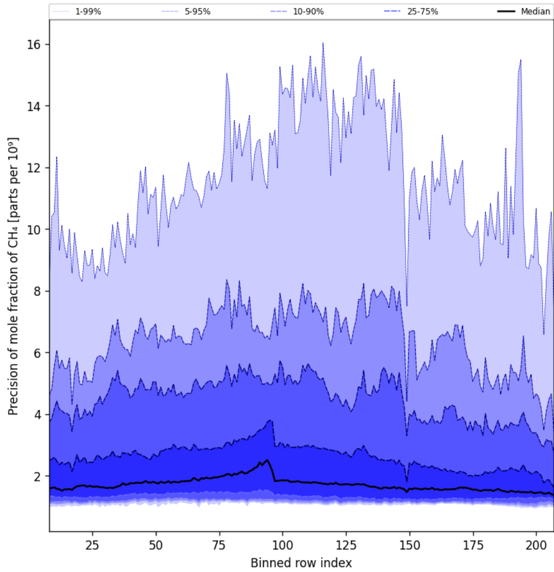
Figure 35: Along track statistics of “Precision of mole fraction of CH 4 ” for 2024-10-11 to 2024-10-13
