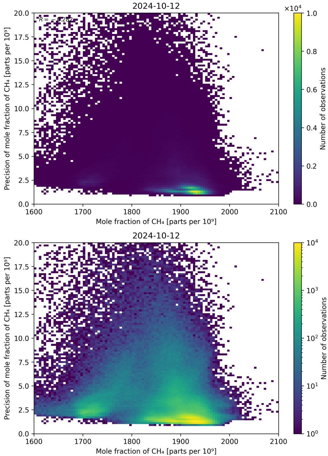
Figure 75: Scatter density plot of “Mole fraction of CH 4 ” against “Precision of mole fraction of CH 4 ” for 2024-10-11 to 2024-10-13.
