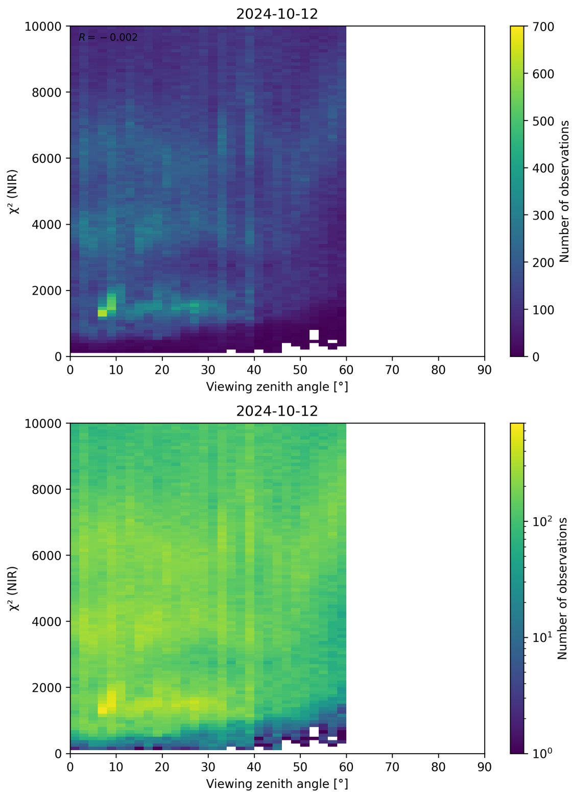
Figure 105: Scatter density plot of “Viewing zenith angle” against “ \chi^2 (NIR)” for 2024-10-11 to 2024-10-13.
