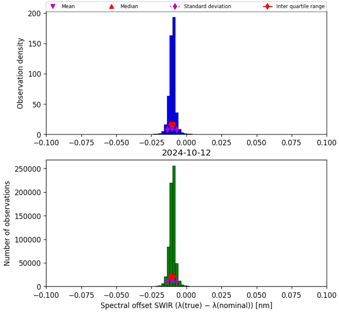
Figure 27: Histogram of “Spectral offset SWIR ( \lambda_{\text{true}} - \lambda_{\text{nominal}} )” for 2024-10-11 to 2024-10-13
