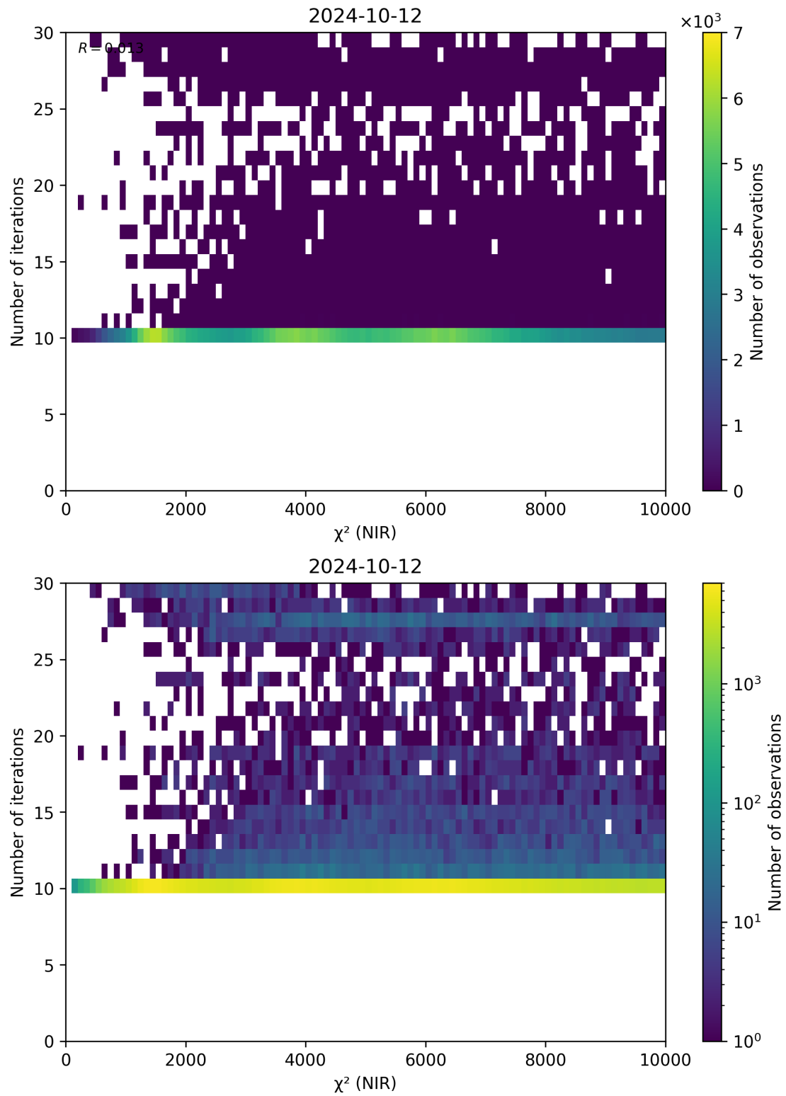
Figure 46: Scatter density plot of “ \chi^2 (NIR)” against “Number of iterations” for 2024-10-11 to 2024-10-13.
