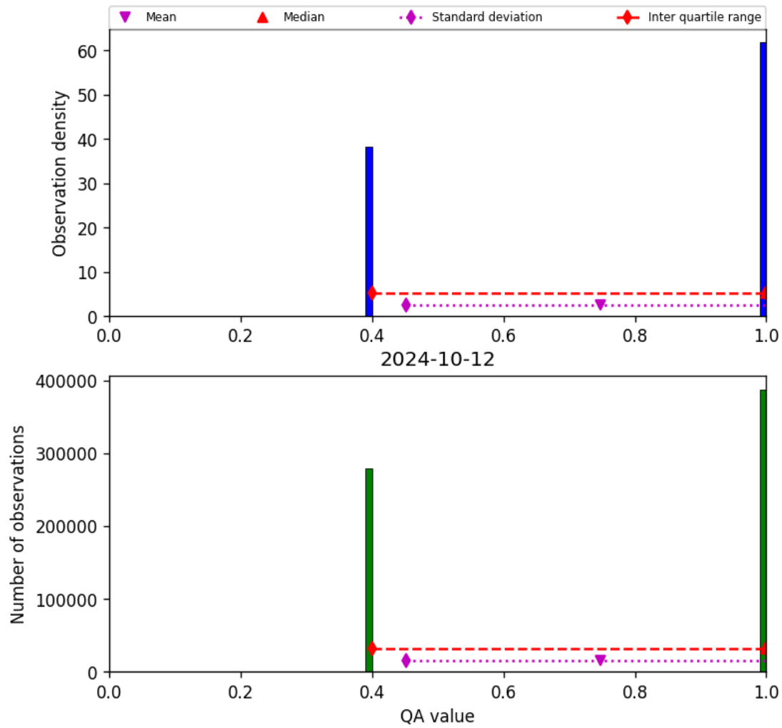
Figure 22: Histogram of “QA value” for 2024-10-11 to 2024-10-13
