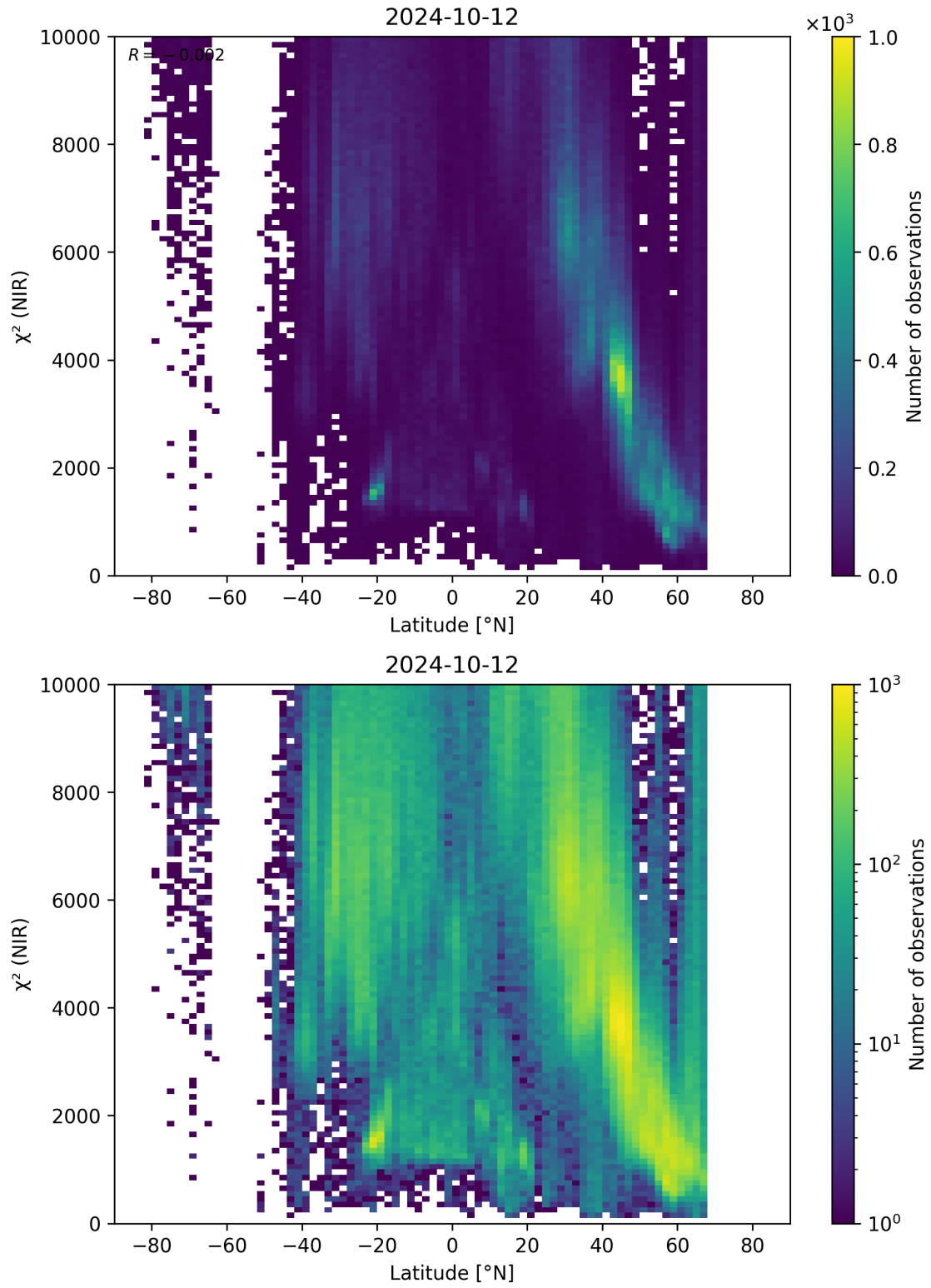
Figure 53: Scatter density plot of “Latitude” against “ \chi^2 (NIR)” for 2024-10-11 to 2024-10-13.
