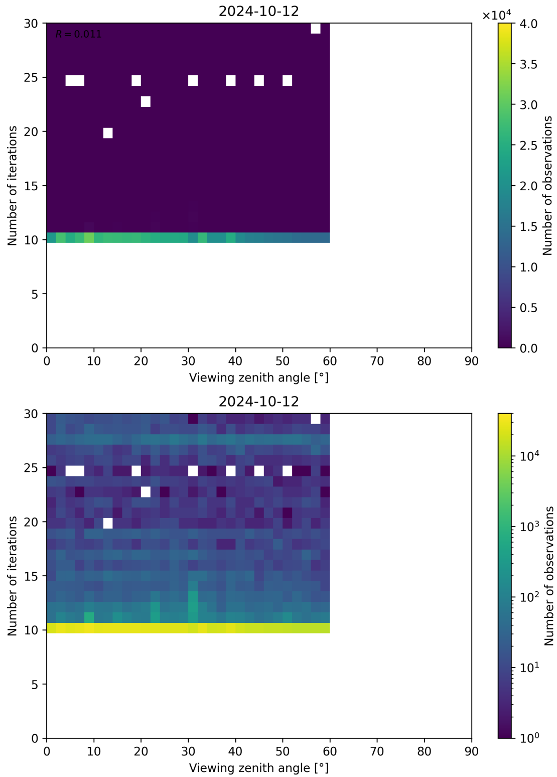
Figure 113: Scatter density plot of “Viewing zenith angle” against “Number of iterations” for 2024-10-11 to 2024-10-13.
