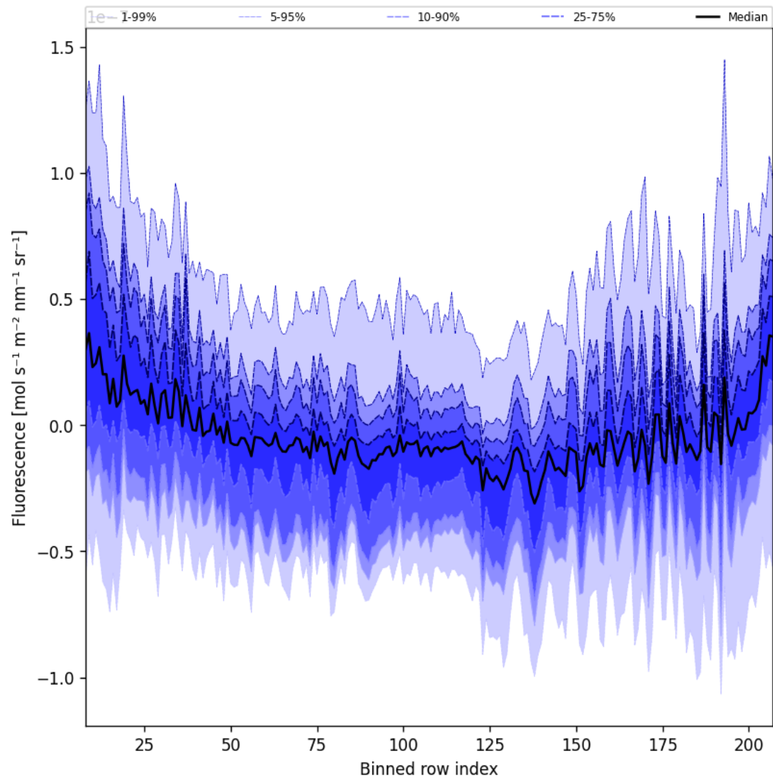
Figure 43: Along track statistics of “Fluorescence” for 2024-10-11 to 2024-10-13
