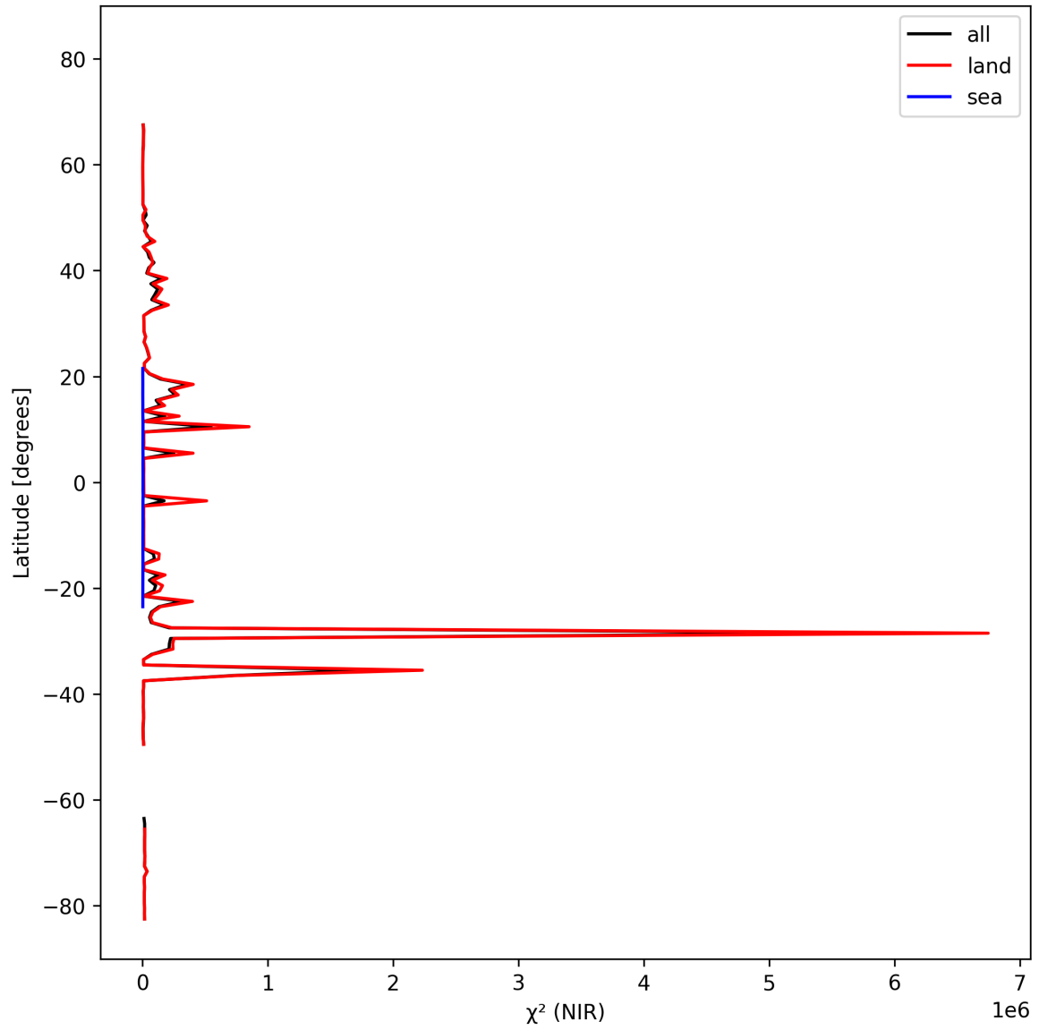
Figure 18: Zonal average of “ \chi^2 (NIR)” for 2024-10-11 to 2024-10-13.
