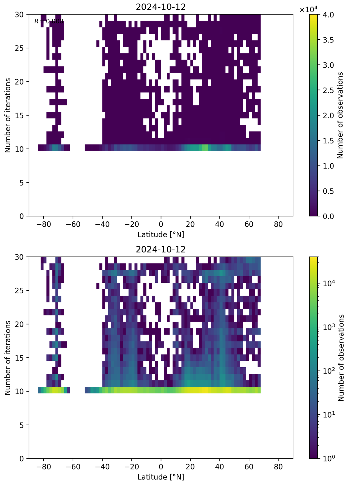
Figure 60: Scatter density plot of “Latitude” against “Number of iterations” for 2024-10-11 to 2024-10-13.
