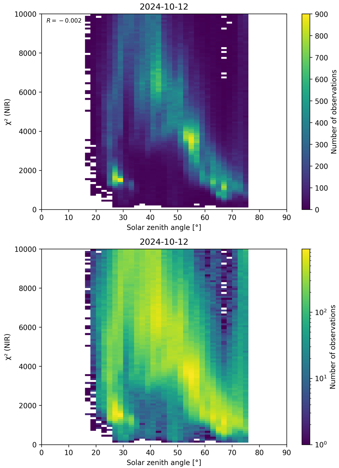
Figure 94: Scatter density plot of “Solar zenith angle” against “ \chi^2 (NIR)” for 2024-10-11 to 2024-10-13.
