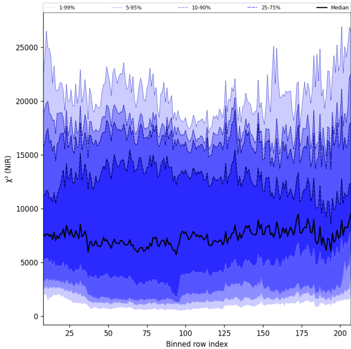
Figure 40: Along track statistics of " \chi^2 (NIR)" for 2024-10-11 to 2024-10-13
