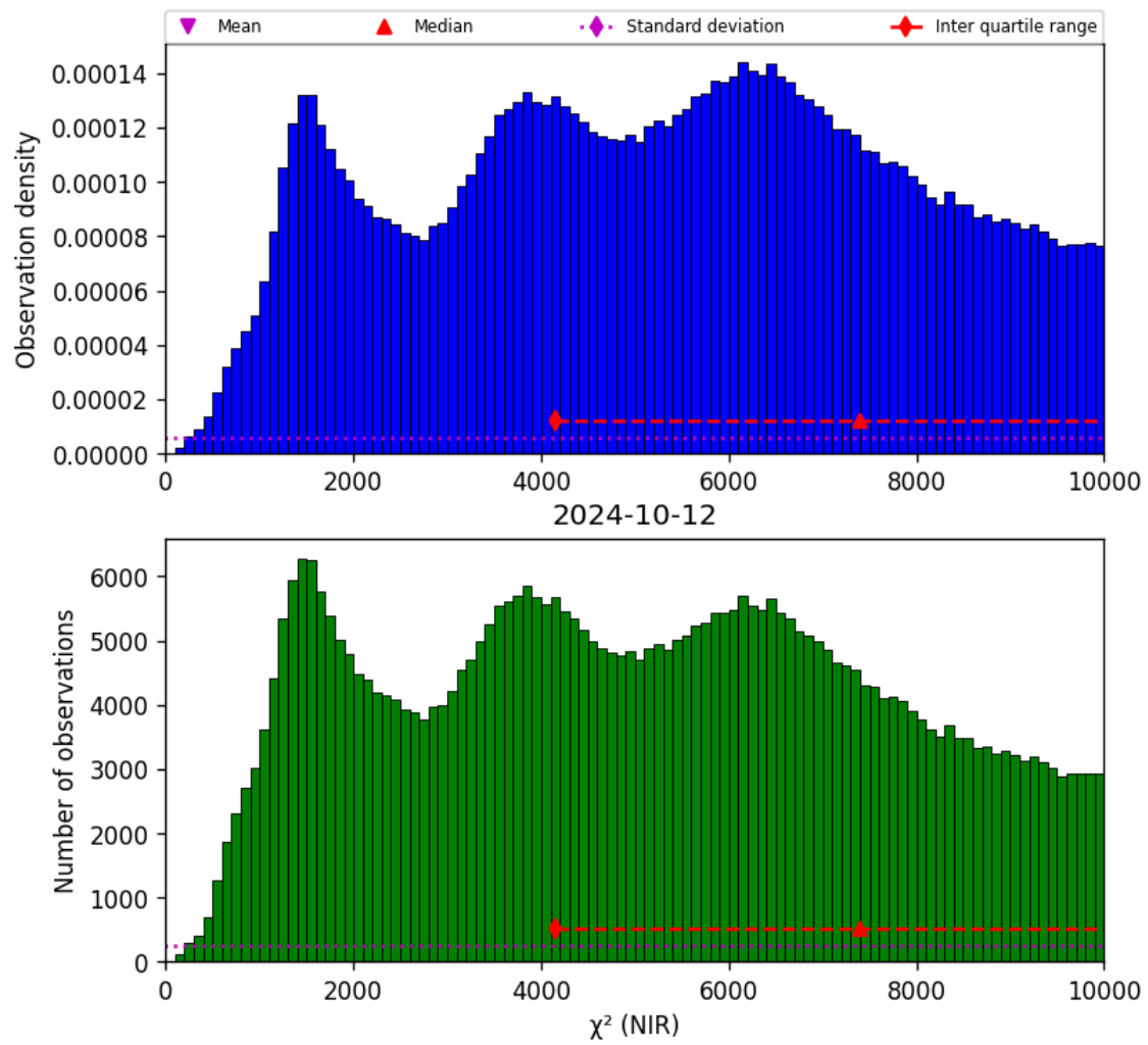
Figure 29: Histogram of “ \chi^2 (NIR)” for 2024-10-11 to 2024-10-13
