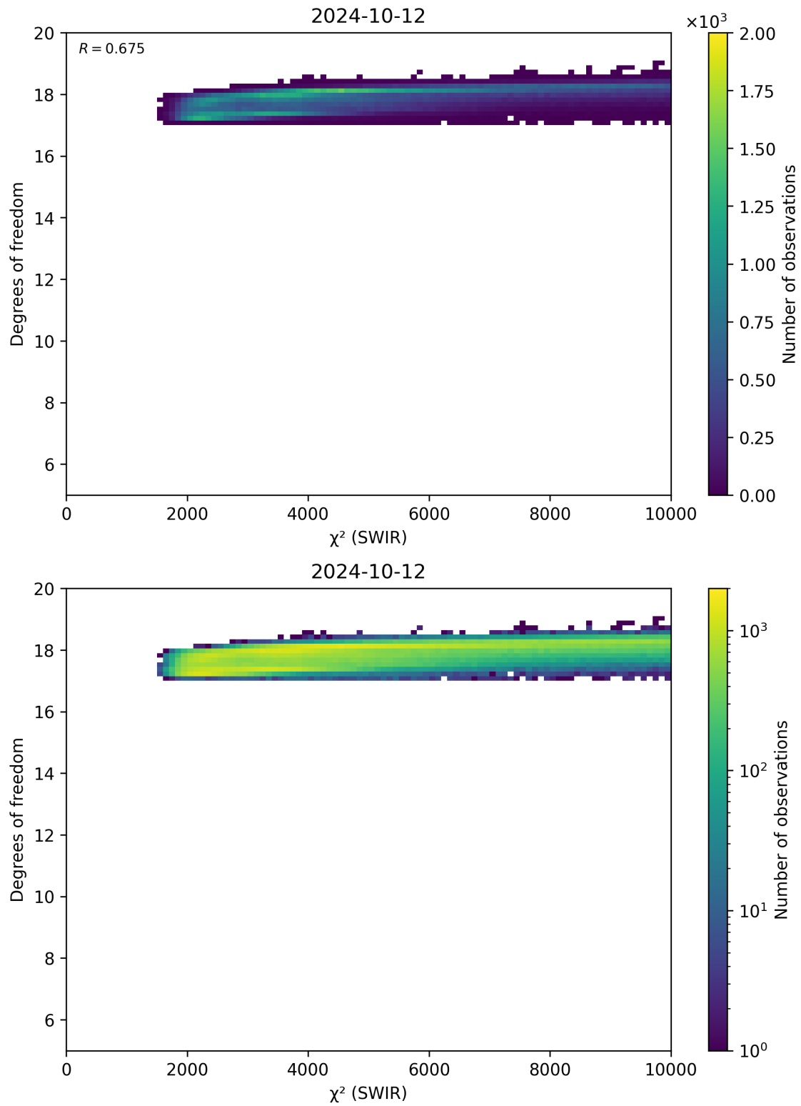
Figure 48: Scatter density plot of “ \chi^2 (SWIR)” against “Degrees of freedom” for 2024-10-11 to 2024-10-13.
