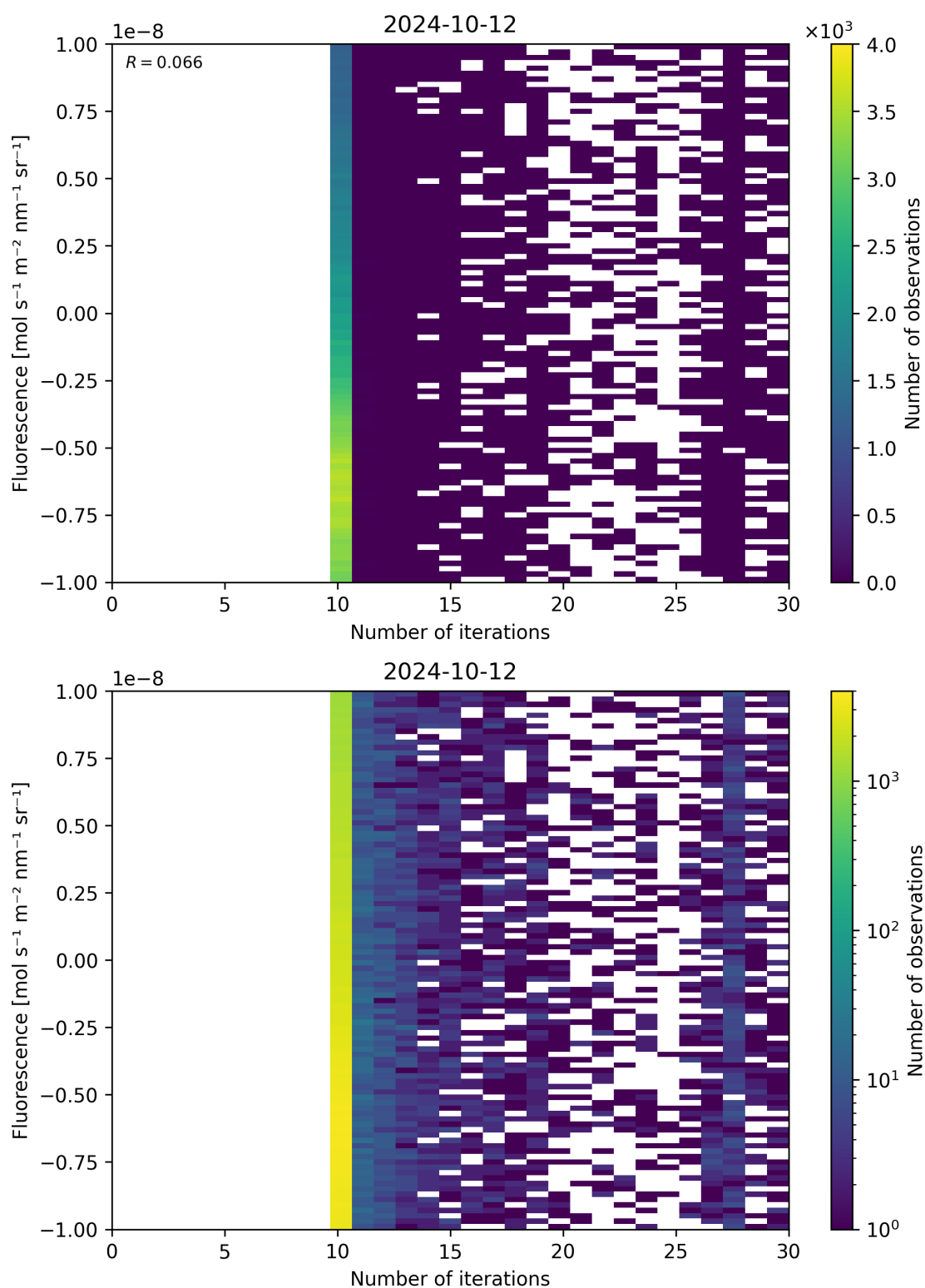
Figure 87: Scatter density plot of “Number of iterations” against “Fluorescence” for 2024-10-11 to 2024-10-13.
