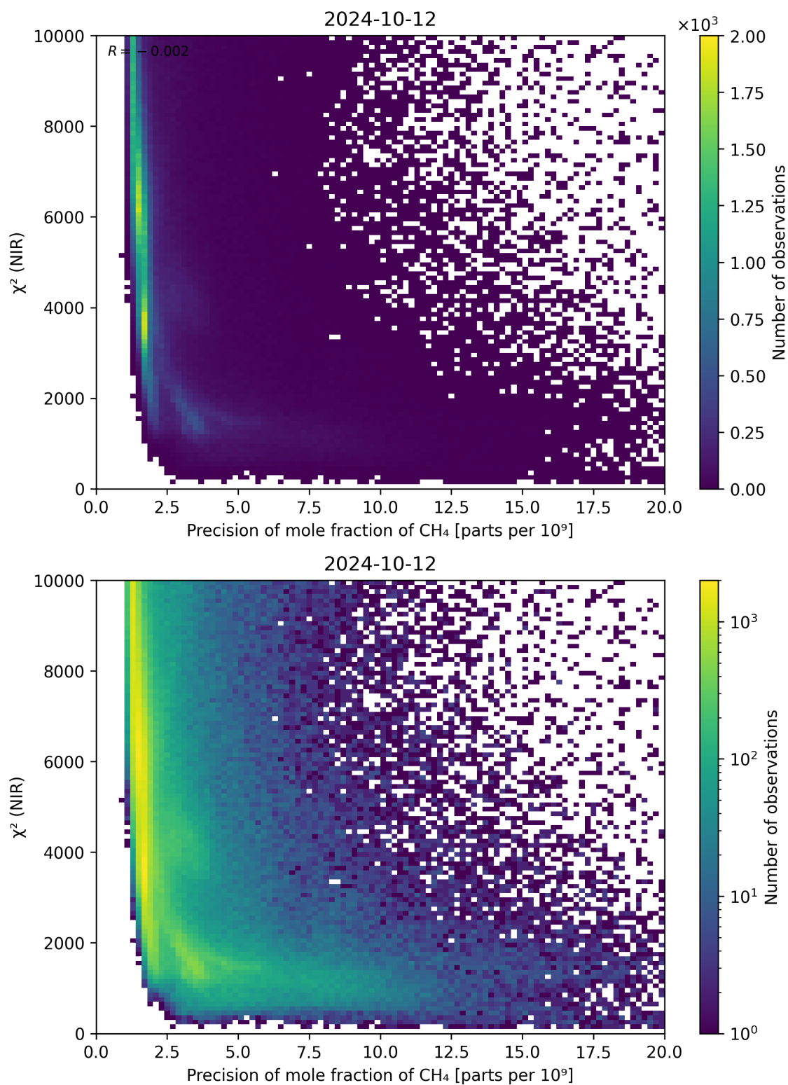
Figure 78: Scatter density plot of “Precision of mole fraction of \text{CH}_4 ” against “ \chi^2 (NIR)” for 2024-10-11 to 2024-10-13.
