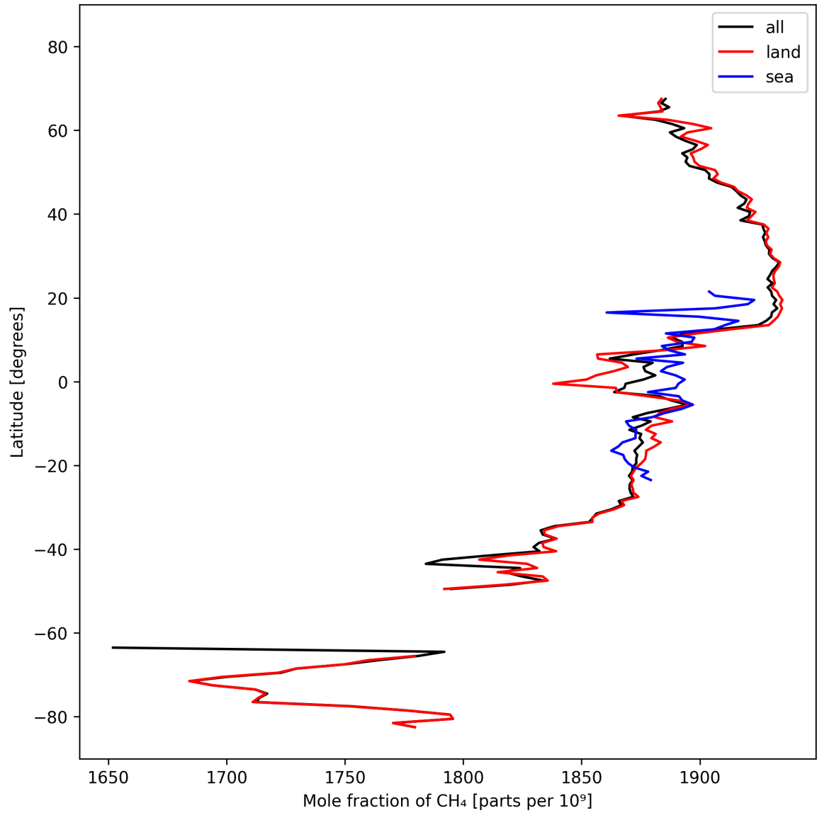
Figure 12: Zonal average of “Mole fraction of CH 4 ” for 2024-10-11 to 2024-10-13.
