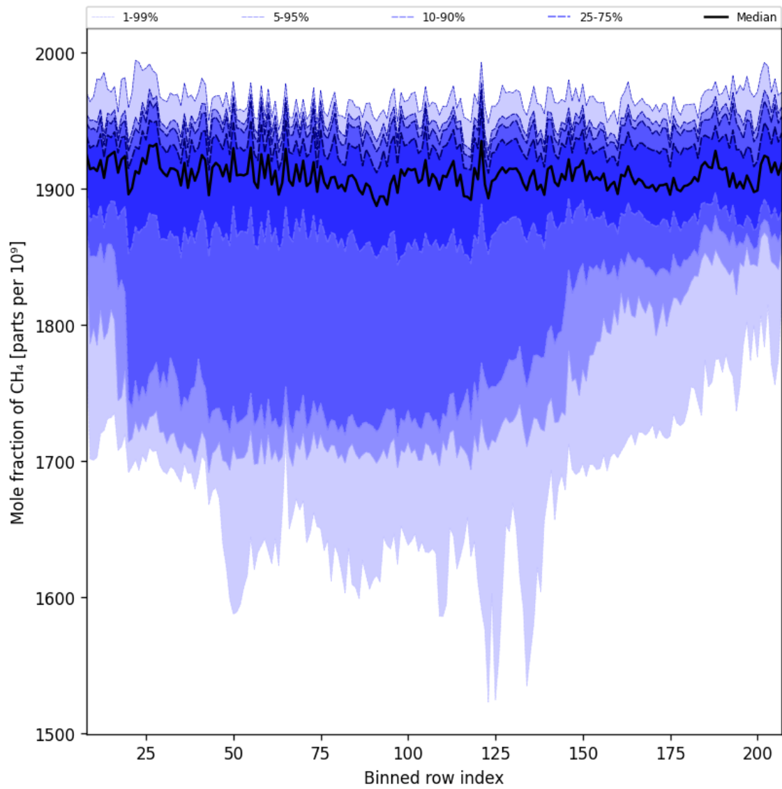
Figure 34: Along track statistics of “Mole fraction of CH 4 ” for 2024-10-11 to 2024-10-13
