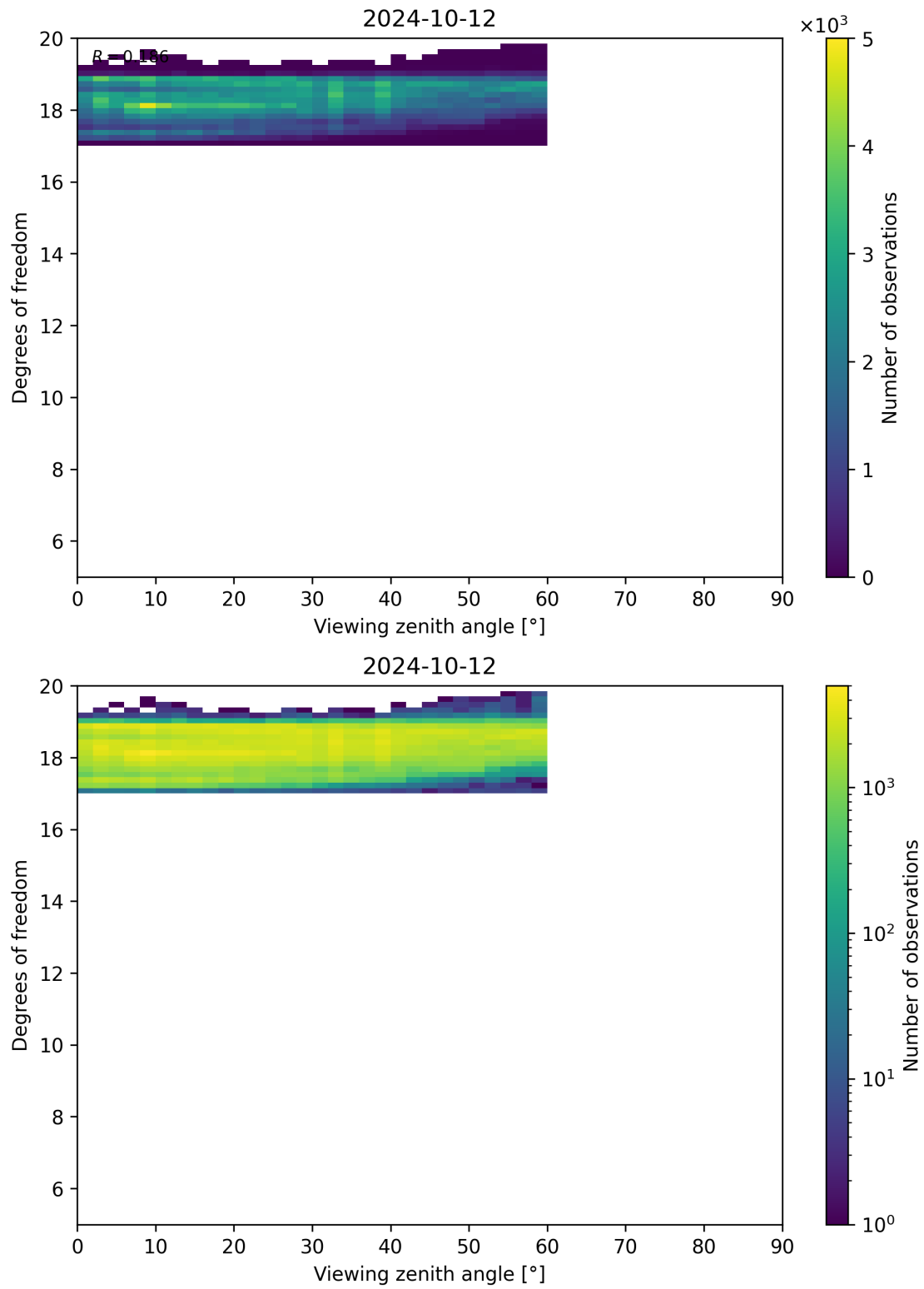
Figure 107: Scatter density plot of “Viewing zenith angle” against “Degrees of freedom” for 2024-10-11 to 2024-10-13.
