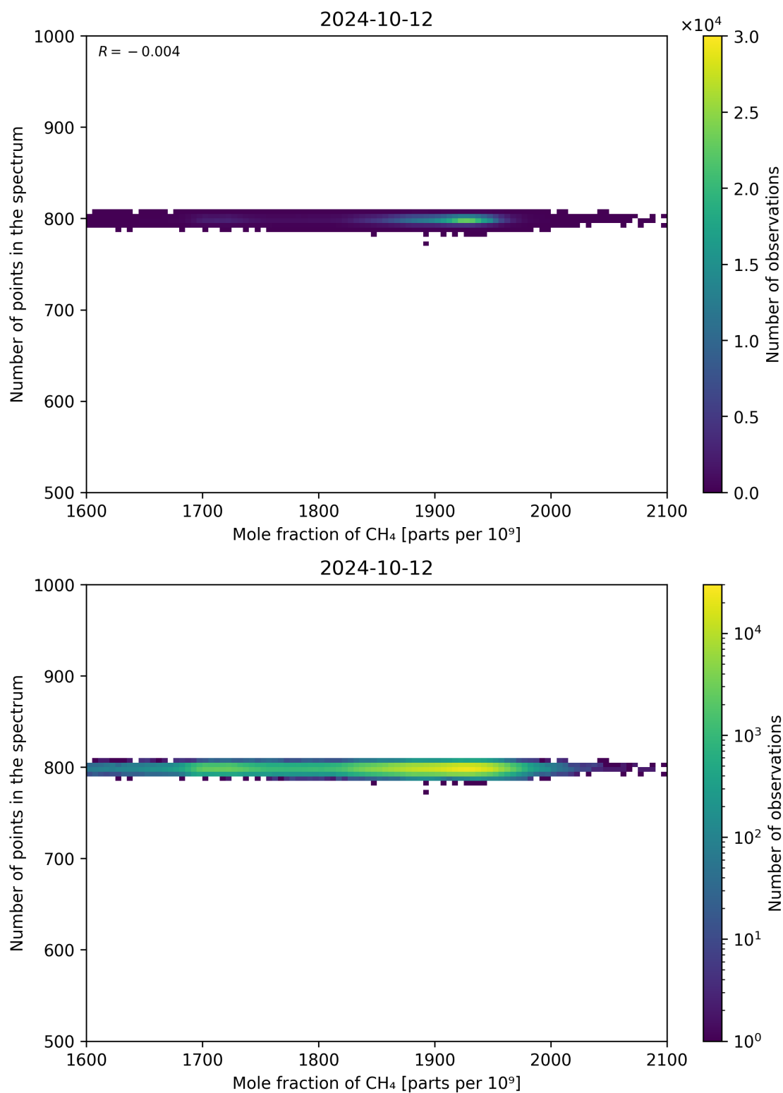
Figure 77: Scatter density plot of “Mole fraction of CH 4 ” against “Number of points in the spectrum” for 2024-10-11 to 2024-10-13.
