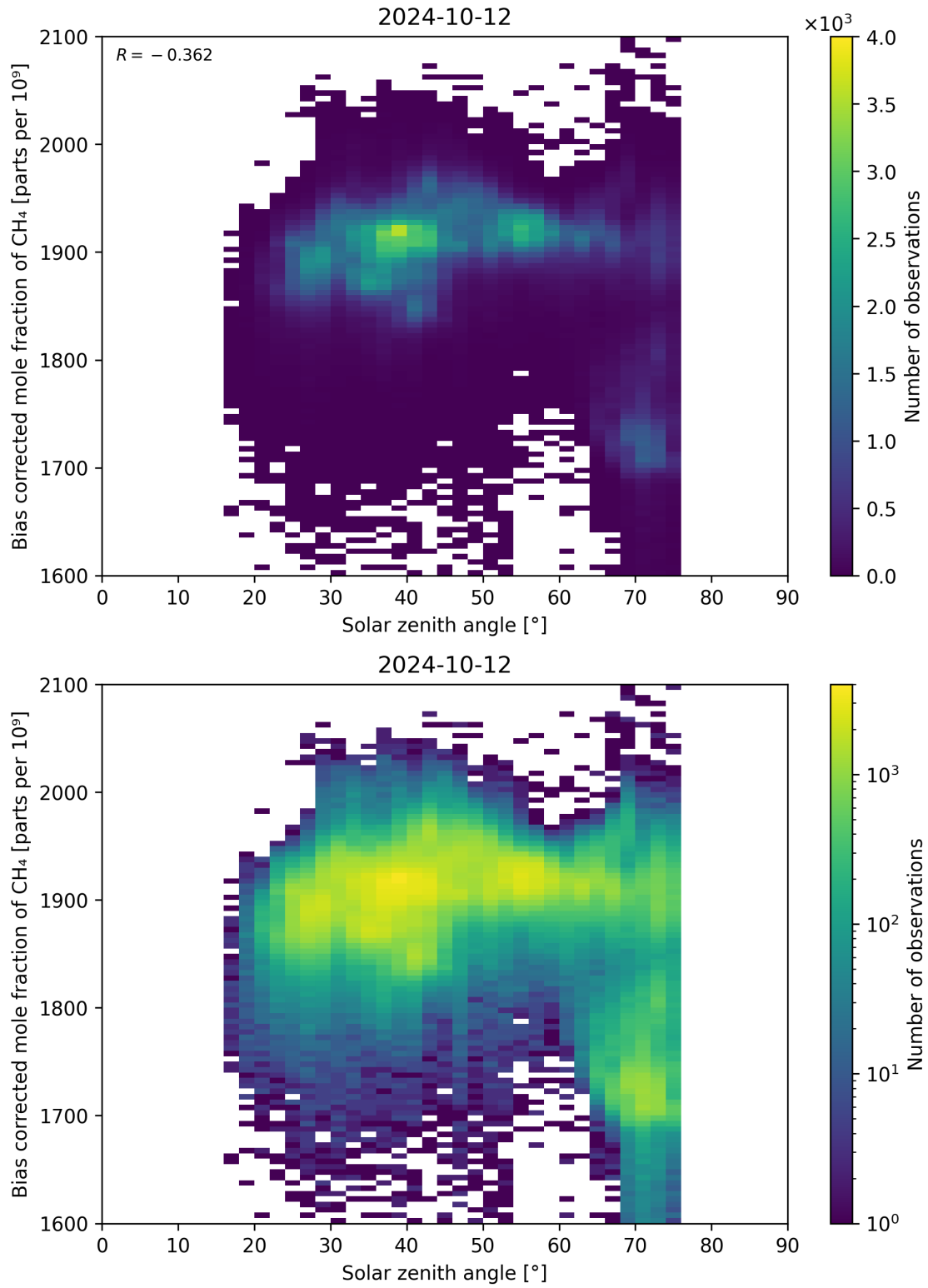
Figure 100: Scatter density plot of “Solar zenith angle” against “Bias corrected mole fraction of CH 4 ” for 2024-10-11 to 2024-10-13.
