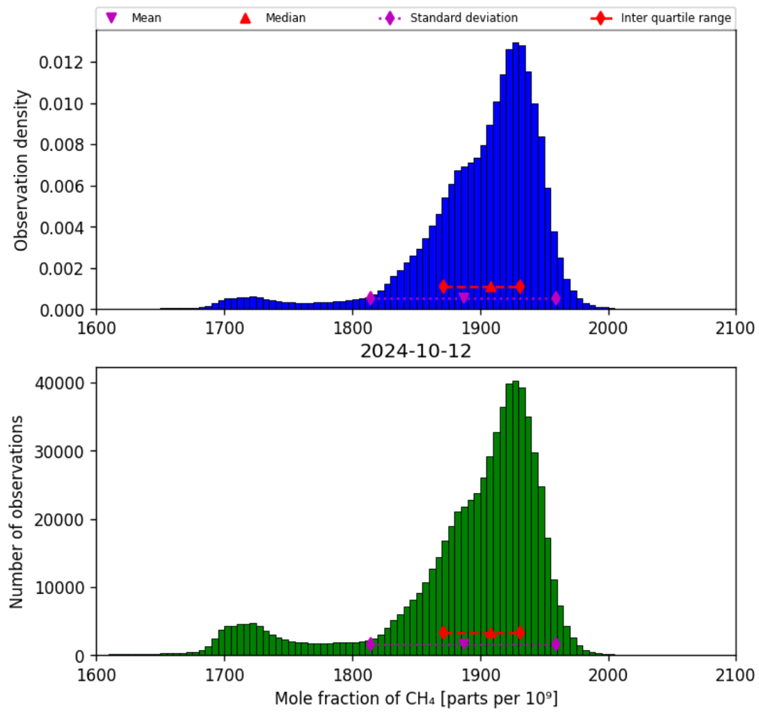
Figure 23: Histogram of “Mole fraction of CH 4 ” for 2024-10-11 to 2024-10-13
