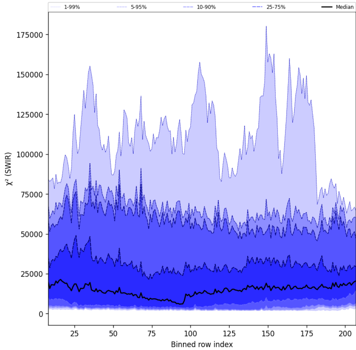
Figure 39: Along track statistics of “ \chi^2 (SWIR)” for 2024-10-11 to 2024-10-13
