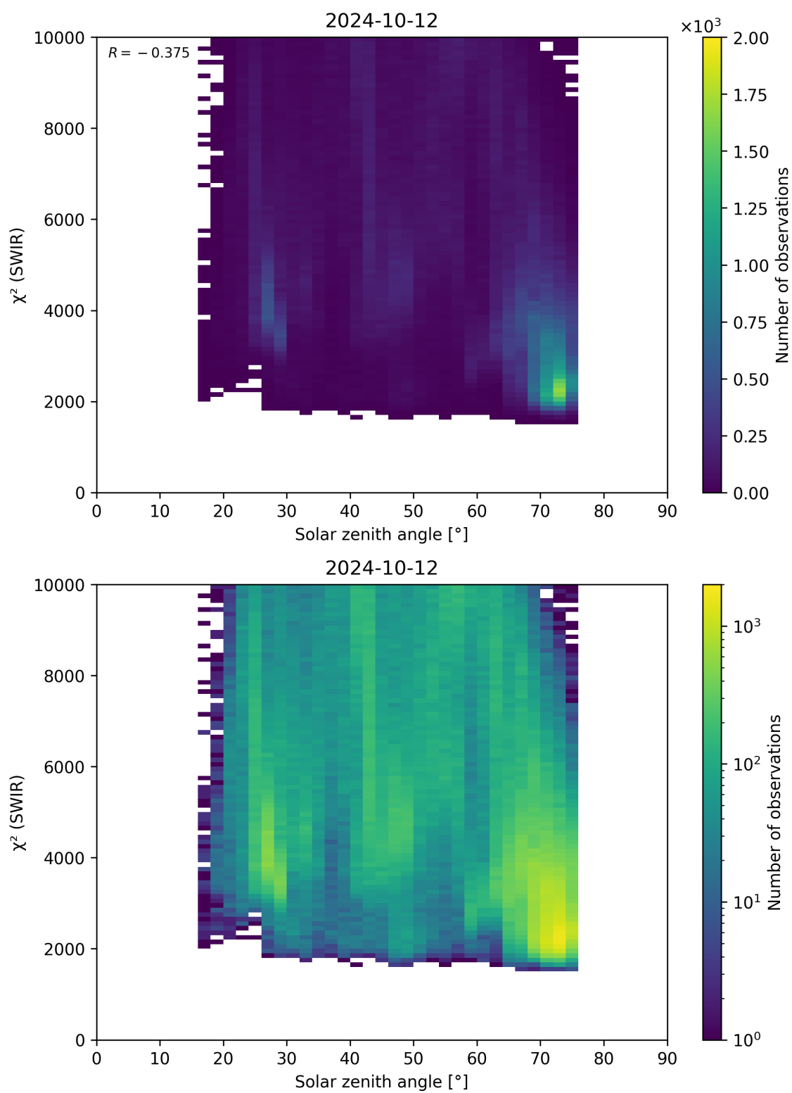
Figure 95: Scatter density plot of “Solar zenith angle” against “ \chi^2 (SWIR)” for 2024-10-11 to 2024-10-13.
