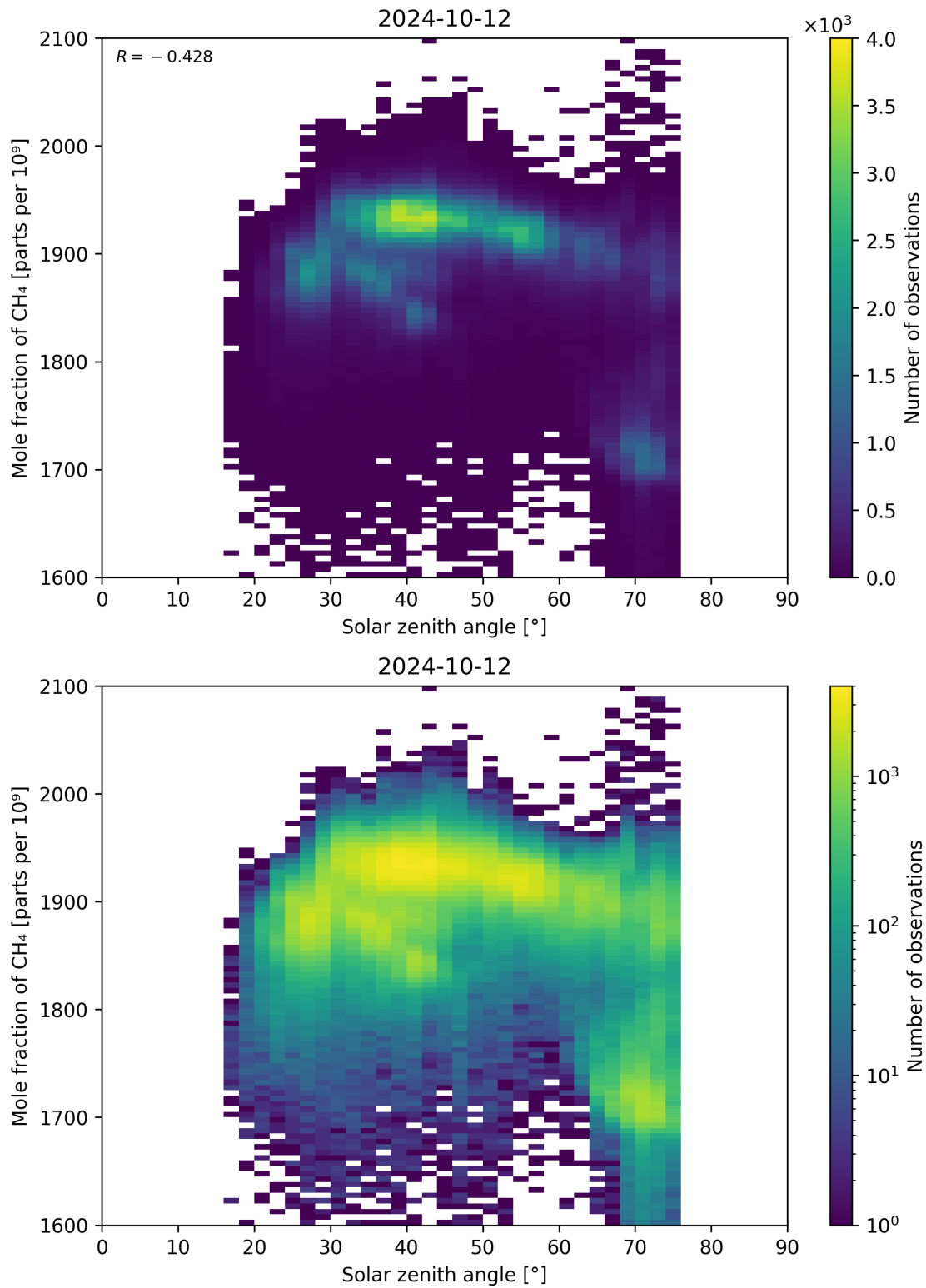
Figure 99: Scatter density plot of “Solar zenith angle” against “Mole fraction of \text{CH}_4 ” for 2024-10-11 to 2024-10-13.
