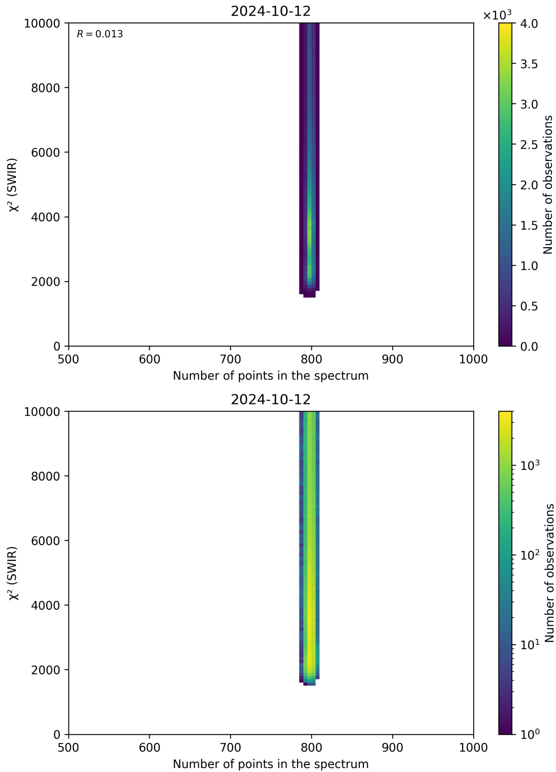
Figure 89: Scatter density plot of “Number of points in the spectrum” against “ \chi^2 (SWIR)” for 2024-10-11 to 2024-10-13.
