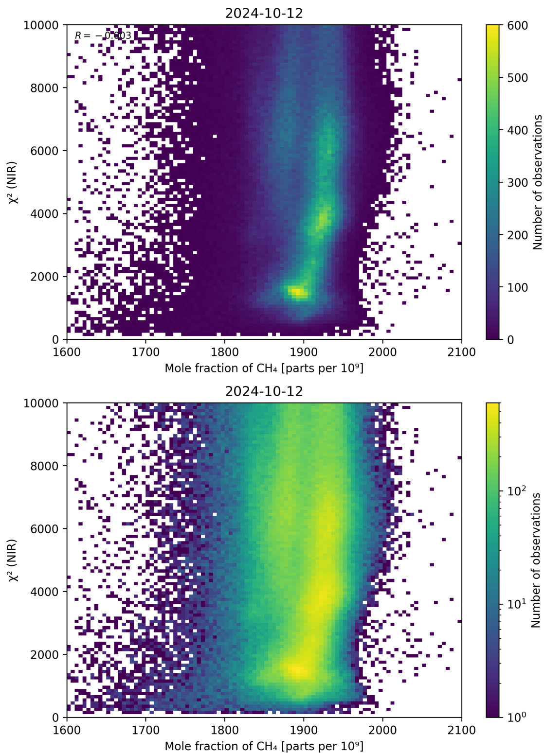
Figure 70: Scatter density plot of “Mole fraction of CH 4 ” against “ \chi^2 (NIR)” for 2024-10-11 to 2024-10-13.
