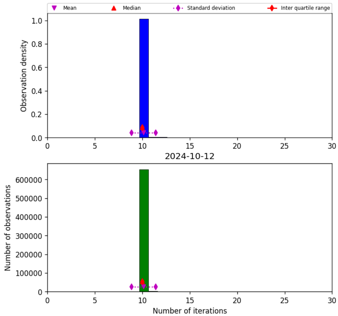
Figure 31: Histogram of “Number of iterations” for 2024-10-11 to 2024-10-13
