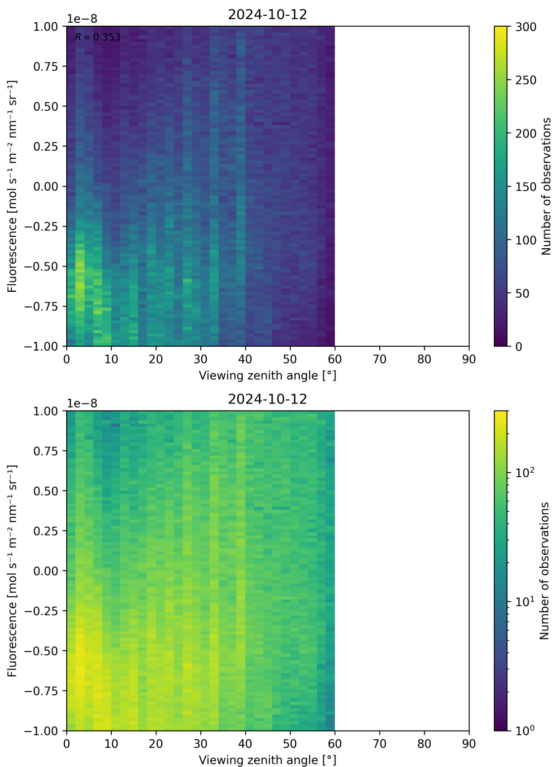
Figure 108: Scatter density plot of “Viewing zenith angle” against “Fluorescence” for 2024-10-11 to 2024-10-13.
