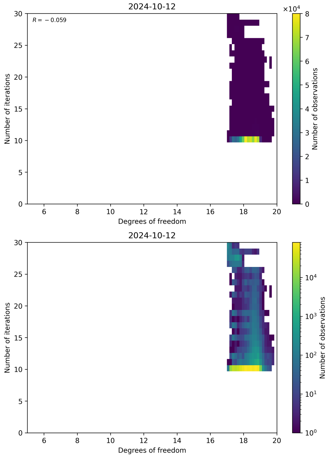
Figure 52: Scatter density plot of “Degrees of freedom” against “Number of iterations” for 2024-10-11 to 2024-10-13.
