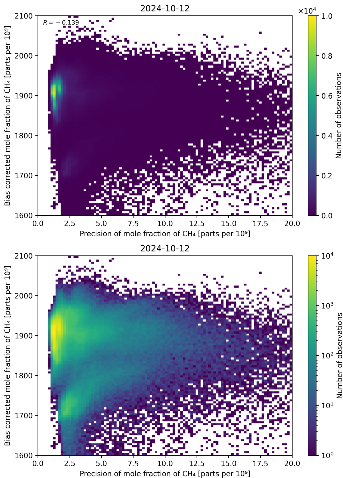
Figure 82: Scatter density plot of “Precision of mole fraction of CH 4 ” against “Bias corrected mole fraction of CH 4 ” for 2024-10-11 to 2024-10-13.
