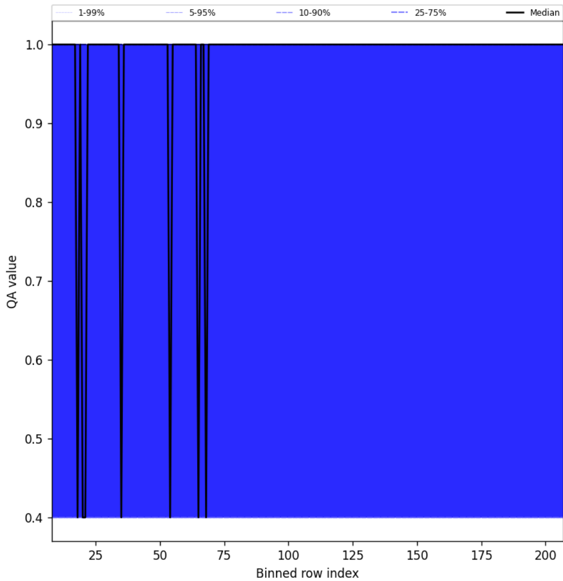
Figure 33: Along track statistics of “QA value” for 2024-10-11 to 2024-10-13
