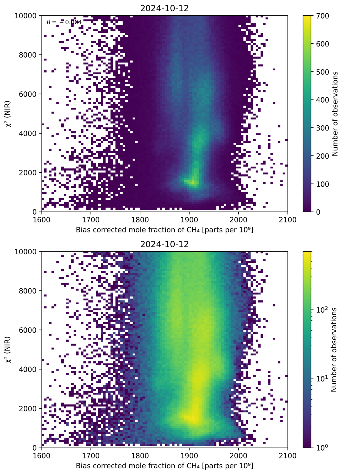
Figure 63: Scatter density plot of “Bias corrected mole fraction of \text{CH}_4 ” against “ \chi^2 (NIR)” for 2024-10-11 to 2024-10-13.
