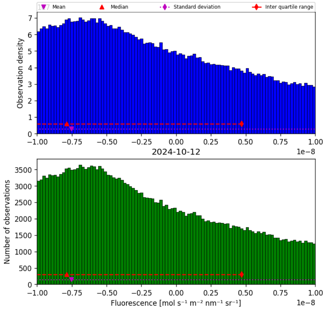
Figure 32: Histogram of “Fluorescence” for 2024-10-11 to 2024-10-13
