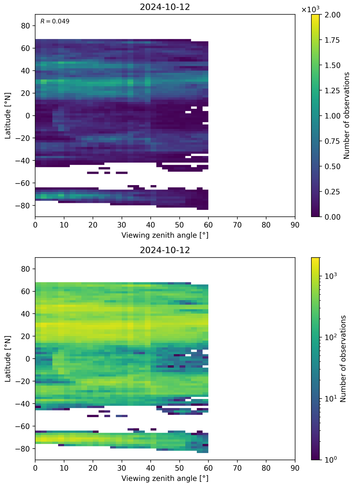
Figure 109: Scatter density plot of “Viewing zenith angle” against “Latitude” for 2024-10-11 to 2024-10-13.
