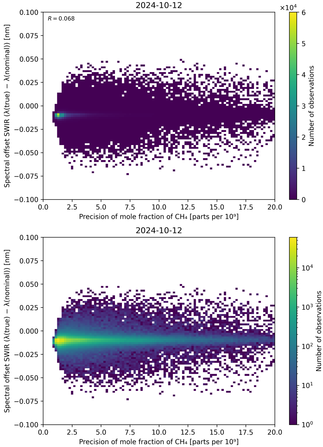
Figure 85: Scatter density plot of “Precision of mole fraction of CH 4 ” against “Spectral offset SWIR ( \lambda_{\text{true}} - \lambda_{\text{nominal}} )” for 2024-10-11 to 2024-10-13.
