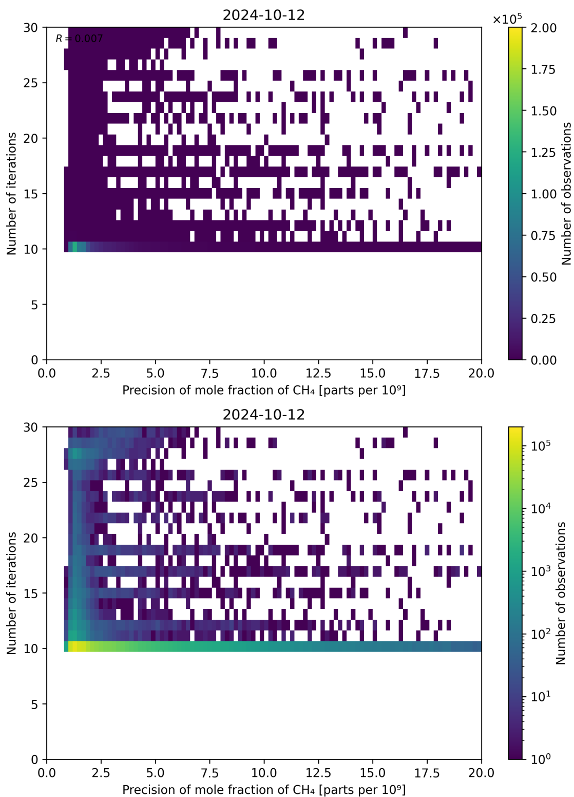
Figure 83: Scatter density plot of “Precision of mole fraction of CH 4 ” against “Number of iterations” for 2024-10-11 to 2024-10-13.
