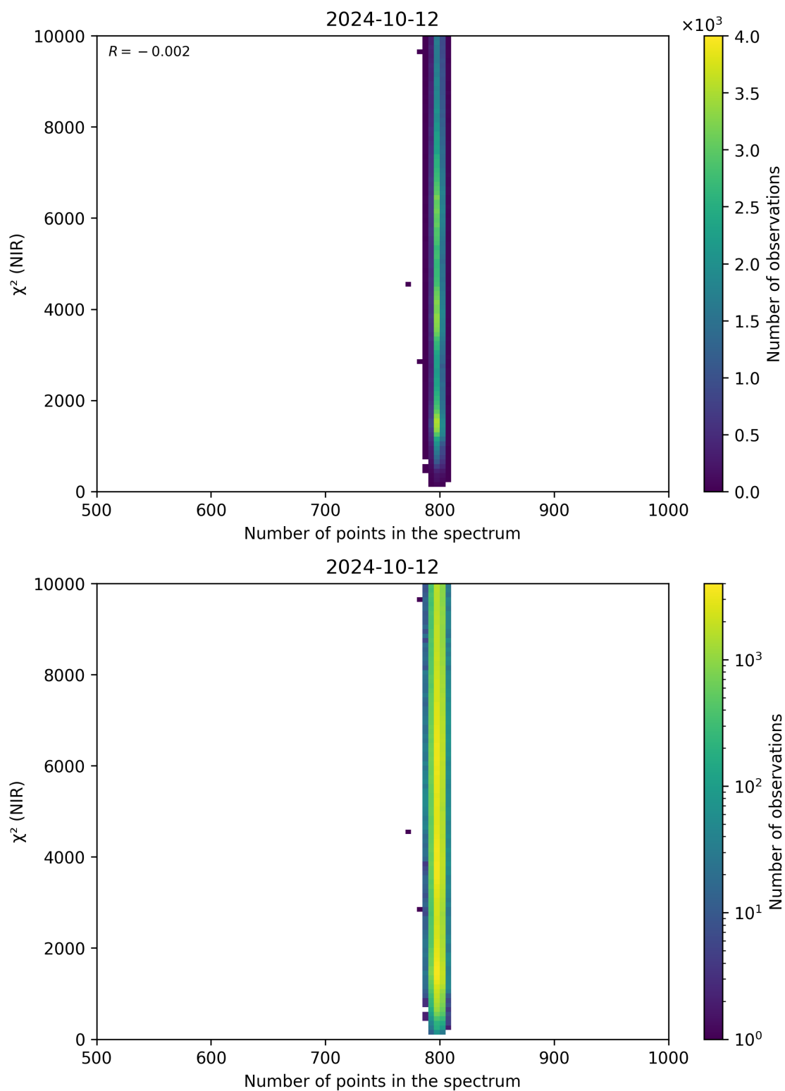
Figure 88: Scatter density plot of “Number of points in the spectrum” against “ \chi^2 (NIR)” for 2024-10-11 to 2024-10-13.
