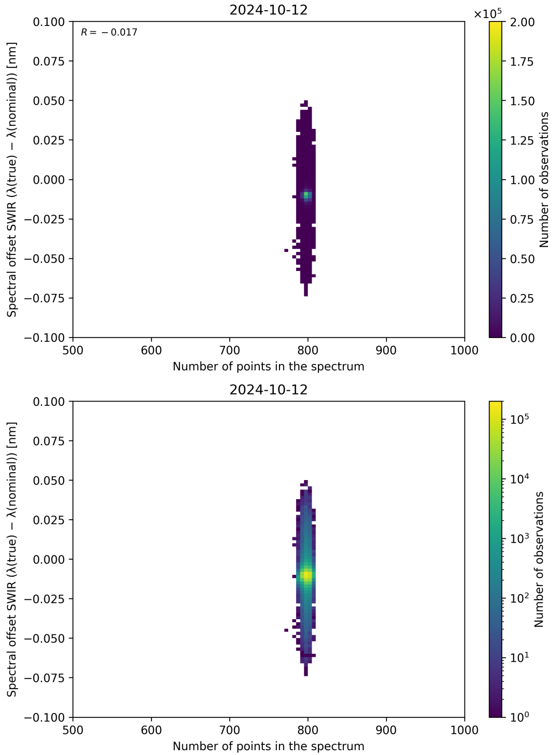
Figure 93: Scatter density plot of “Number of points in the spectrum” against “Spectral offset SWIR ( \lambda_{\text{true}} - \lambda_{\text{nominal}} )” for 2024-10-11 to 2024-10-13.
