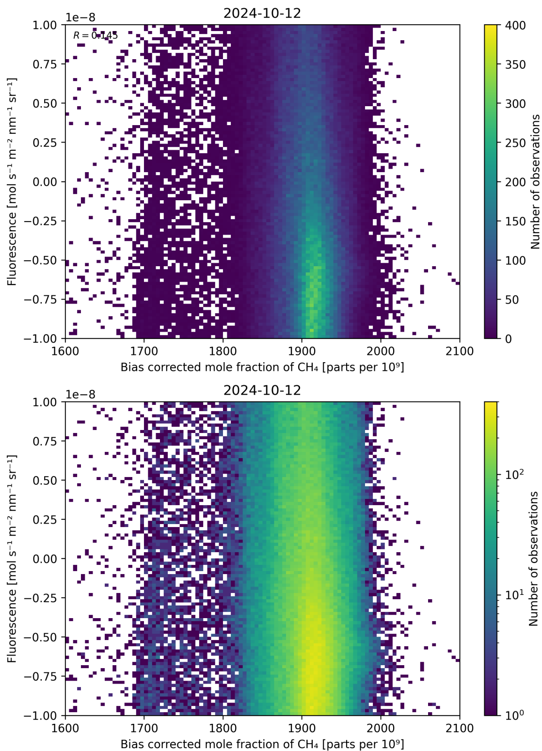
Figure 66: Scatter density plot of “Bias corrected mole fraction of \text{CH}_4 ” against “Fluorescence” for 2024-10-11 to 2024-10-13.
