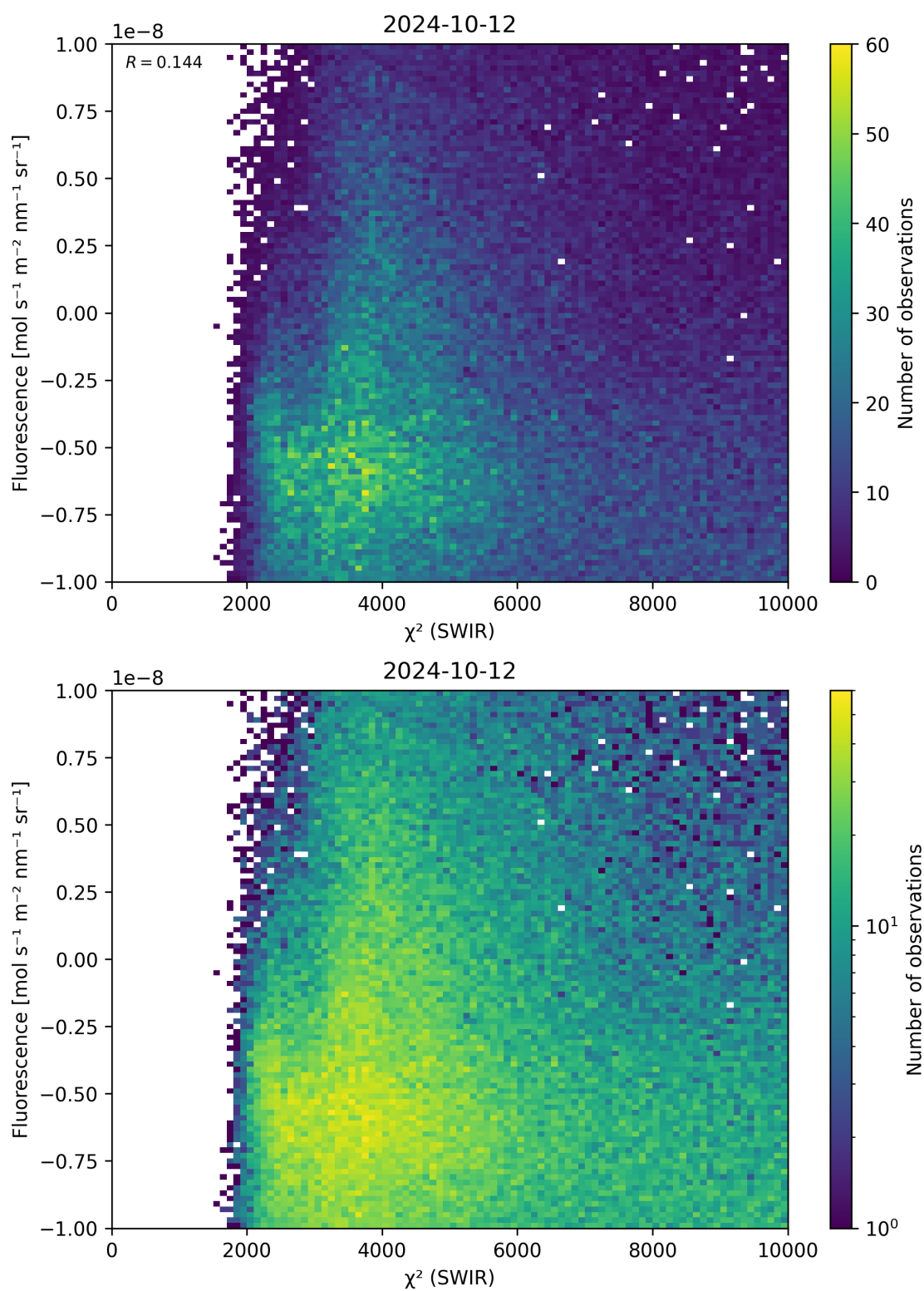
Figure 49: Scatter density plot of “ \chi^2 (SWIR)” against “Fluorescence” for 2024-10-11 to 2024-10-13.
