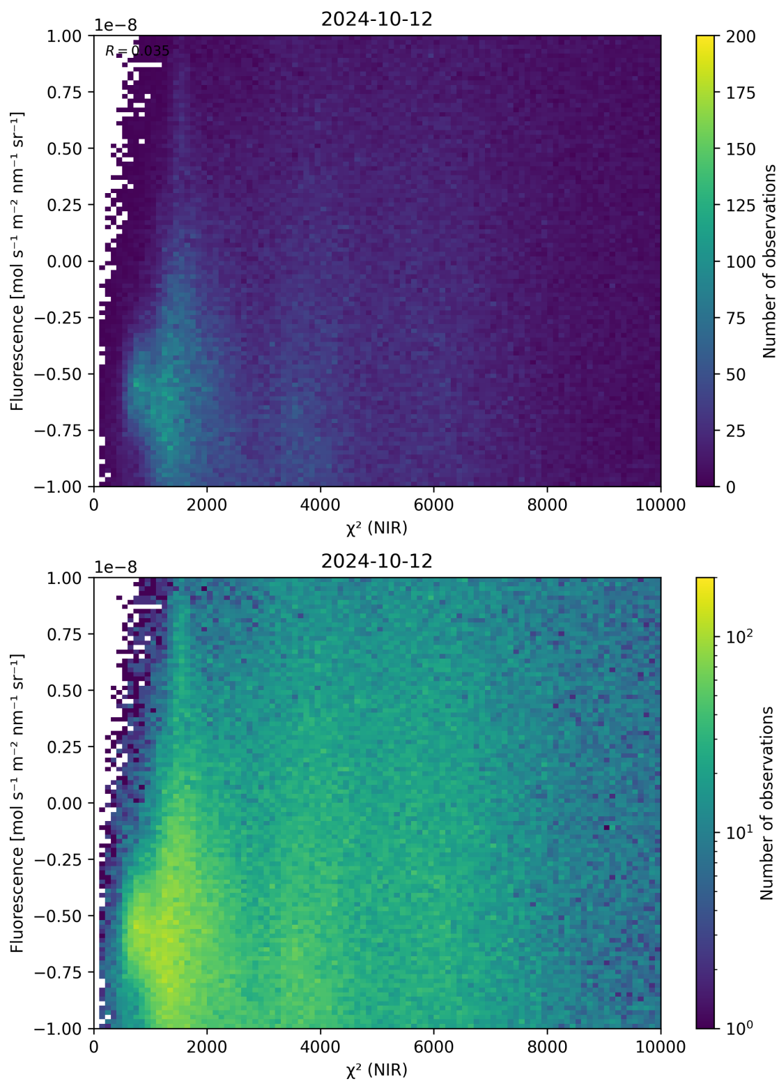
Figure 45: Scatter density plot of “ \chi^2 (NIR)” against “Fluorescence” for 2024-10-11 to 2024-10-13.
