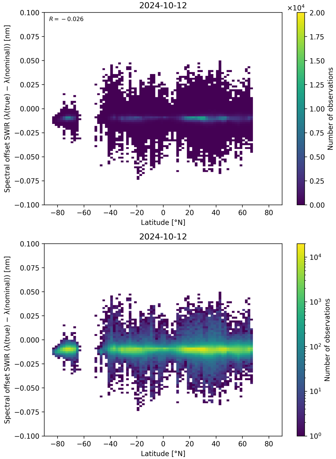
Figure 62: Scatter density plot of “Latitude” against “Spectral offset SWIR ( \lambda_{\text{true}} - \lambda_{\text{nominal}} )” for 2024-10-11 to 2024-10-13.
