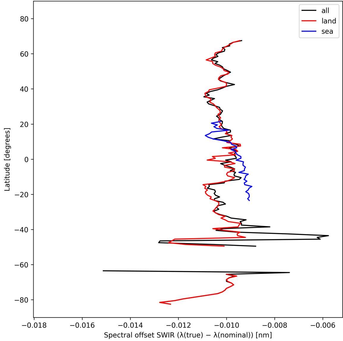
Figure 16: Zonal average of “Spectral offset SWIR ( \lambda_{\text{true}} - \lambda_{\text{nominal}} )” for 2024-10-11 to 2024-10-13.
