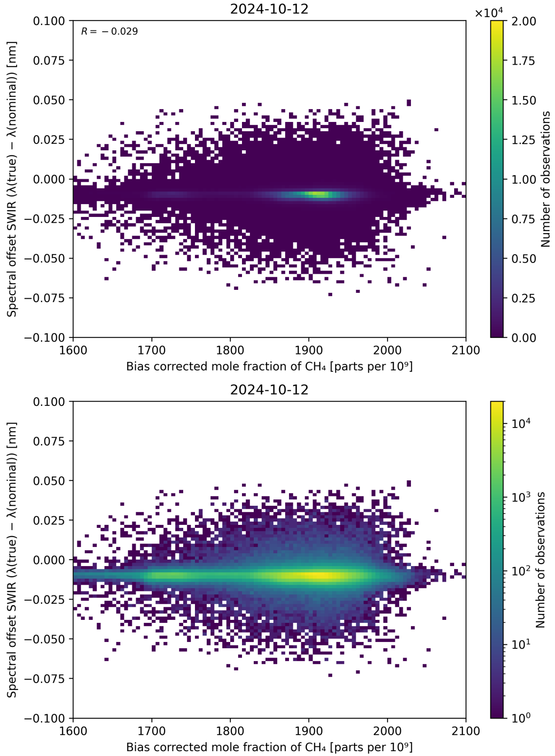
Figure 69: Scatter density plot of “Bias corrected mole fraction of CH 4 ” against “Spectral offset SWIR ( \lambda_{\text{true}} - \lambda_{\text{nominal}} )” for 2024-10-11 to 2024-10-13.
