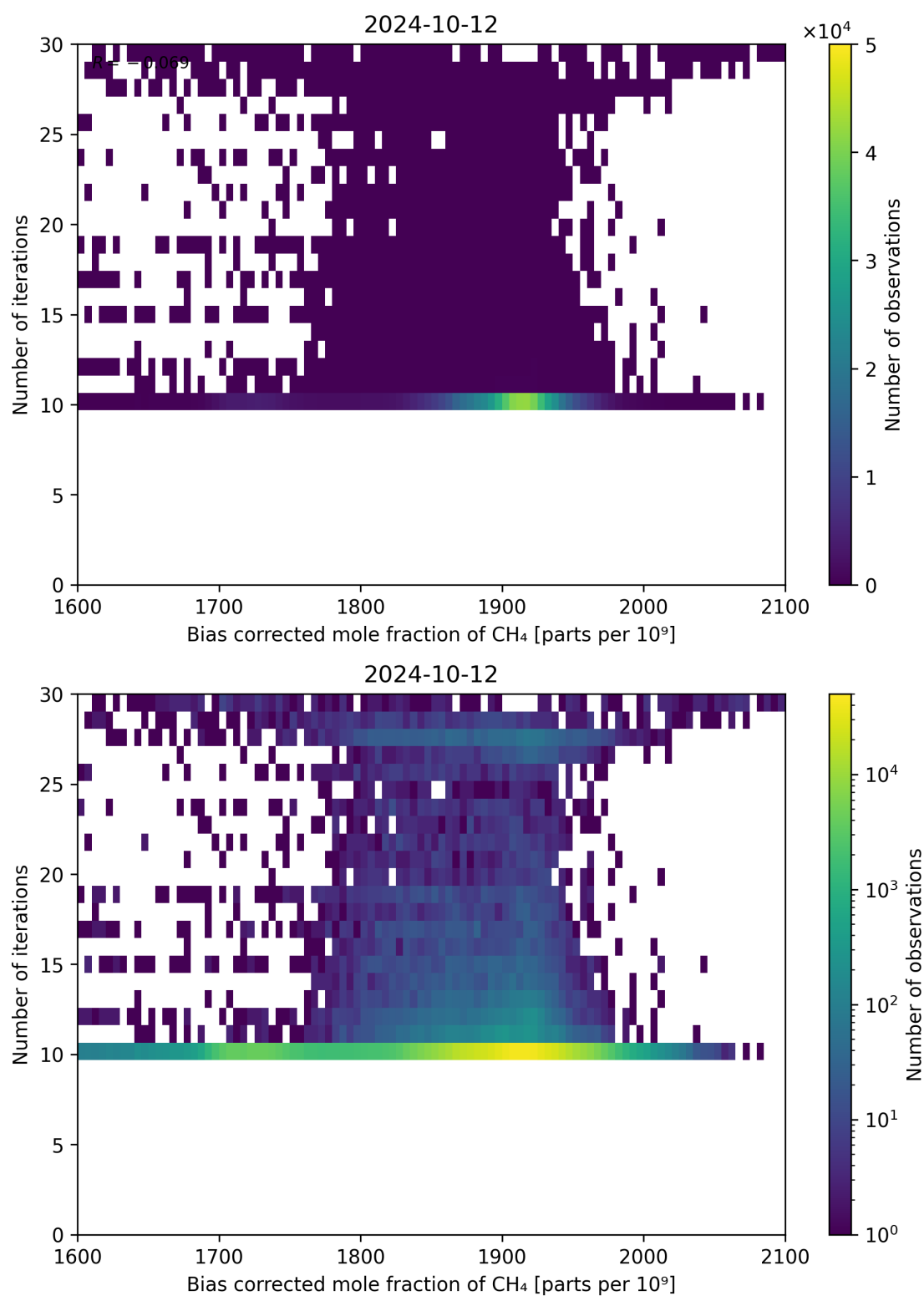
Figure 67: Scatter density plot of “Bias corrected mole fraction of \text{CH}_4 ” against “Number of iterations” for 2024-10-11 to 2024-10-13.
