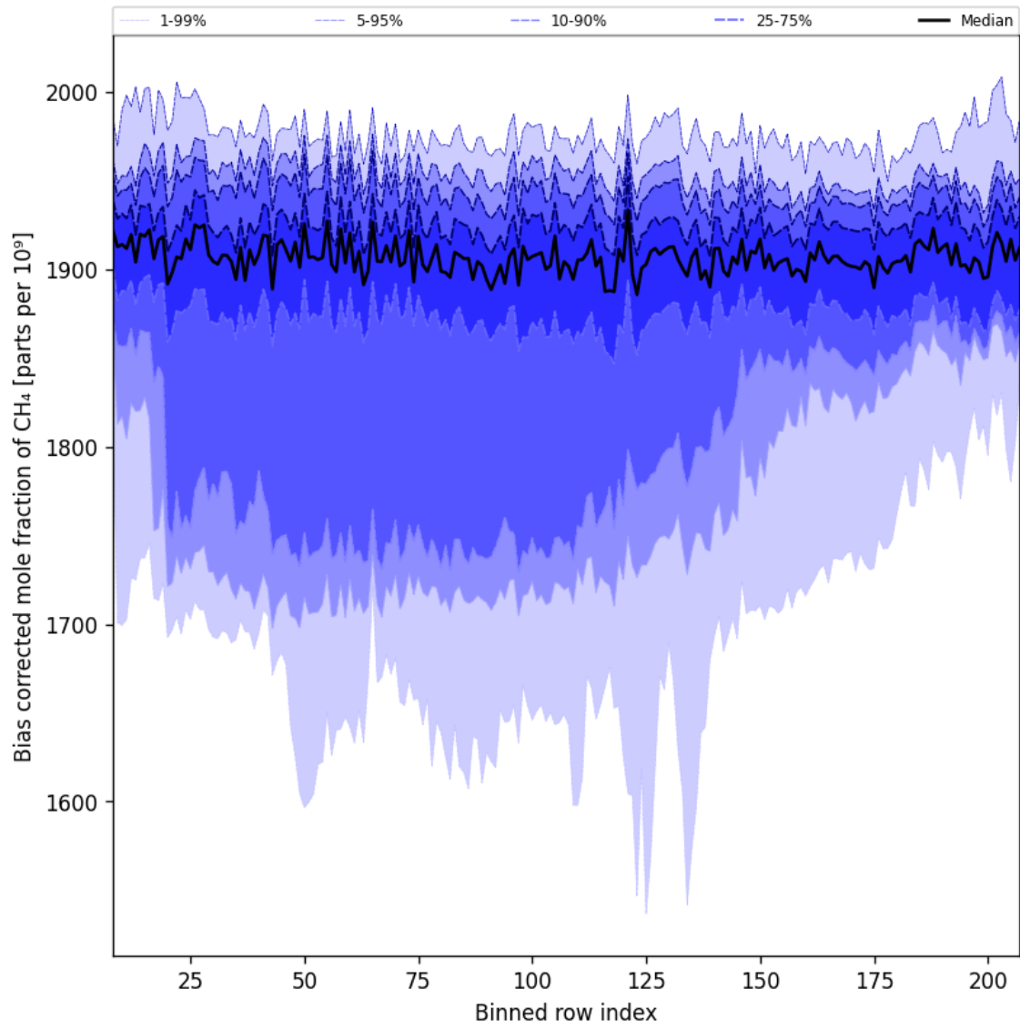
Figure 36: Along track statistics of “Bias corrected mole fraction of CH 4 ” for 2024-10-11 to 2024-10-13
