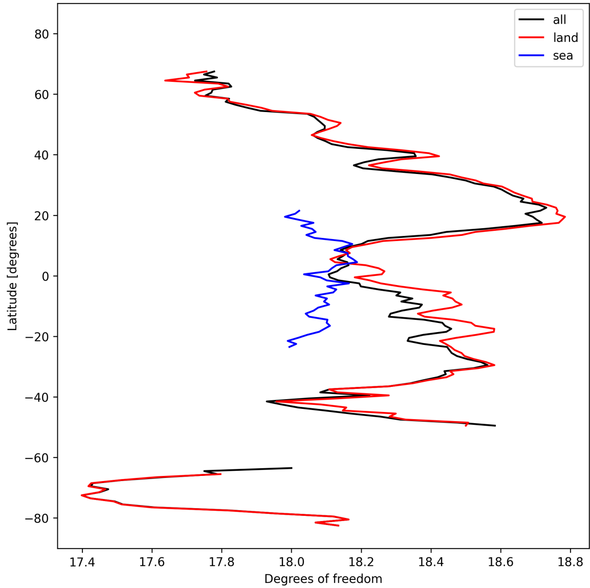
Figure 19: Zonal average of “Degrees of freedom” for 2024-10-11 to 2024-10-13.
