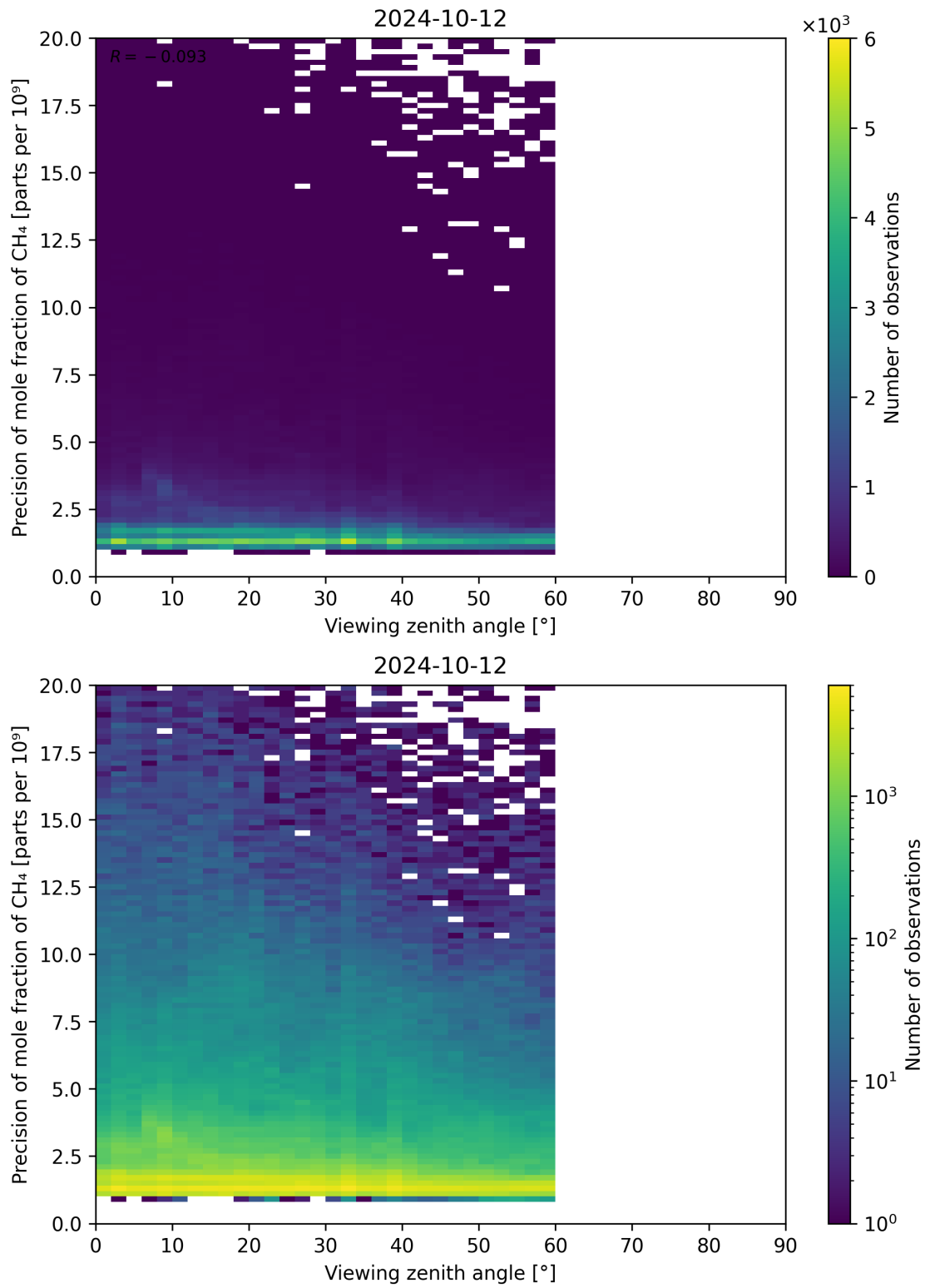
Figure 112: Scatter density plot of “Viewing zenith angle” against “Precision of mole fraction of CH 4 ” for 2024-10-11 to 2024-10-13.
