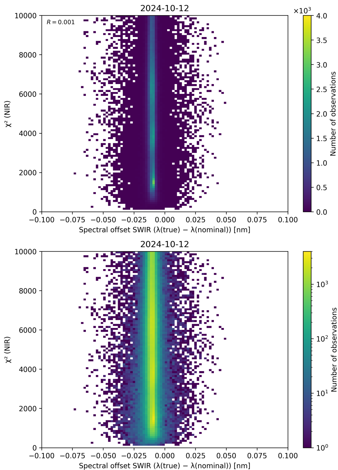
Figure 117: Scatter density plot of “Spectral offset SWIR ( \lambda_{\text{true}} - \lambda_{\text{nominal}} )” against “ \chi^2 (NIR)” for 2024-10-11 to 2024-10-13.
