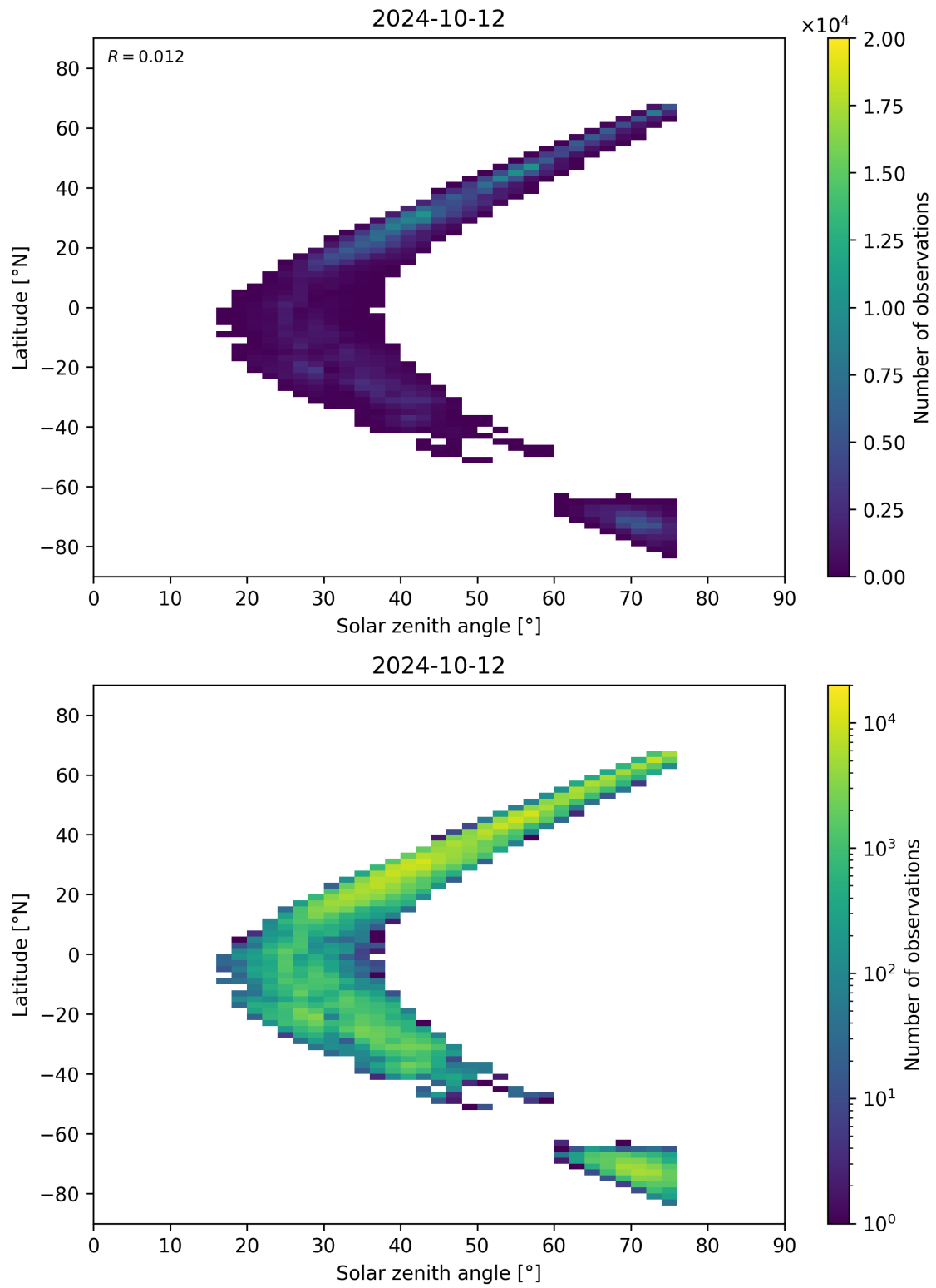
Figure 98: Scatter density plot of “Solar zenith angle” against “Latitude” for 2024-10-11 to 2024-10-13.
