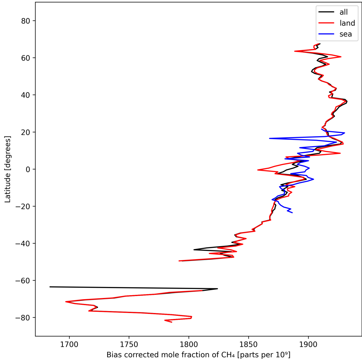
Figure 14: Zonal average of “Bias corrected mole fraction of CH 4 ” for 2024-10-11 to 2024-10-13.
