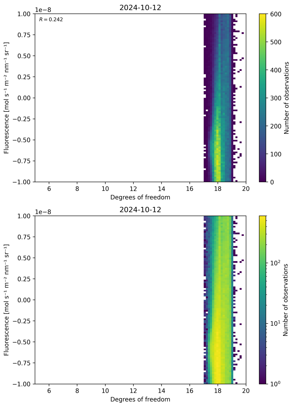
Figure 51: Scatter density plot of “Degrees of freedom” against “Fluorescence” for 2024-10-11 to 2024-10-13.
