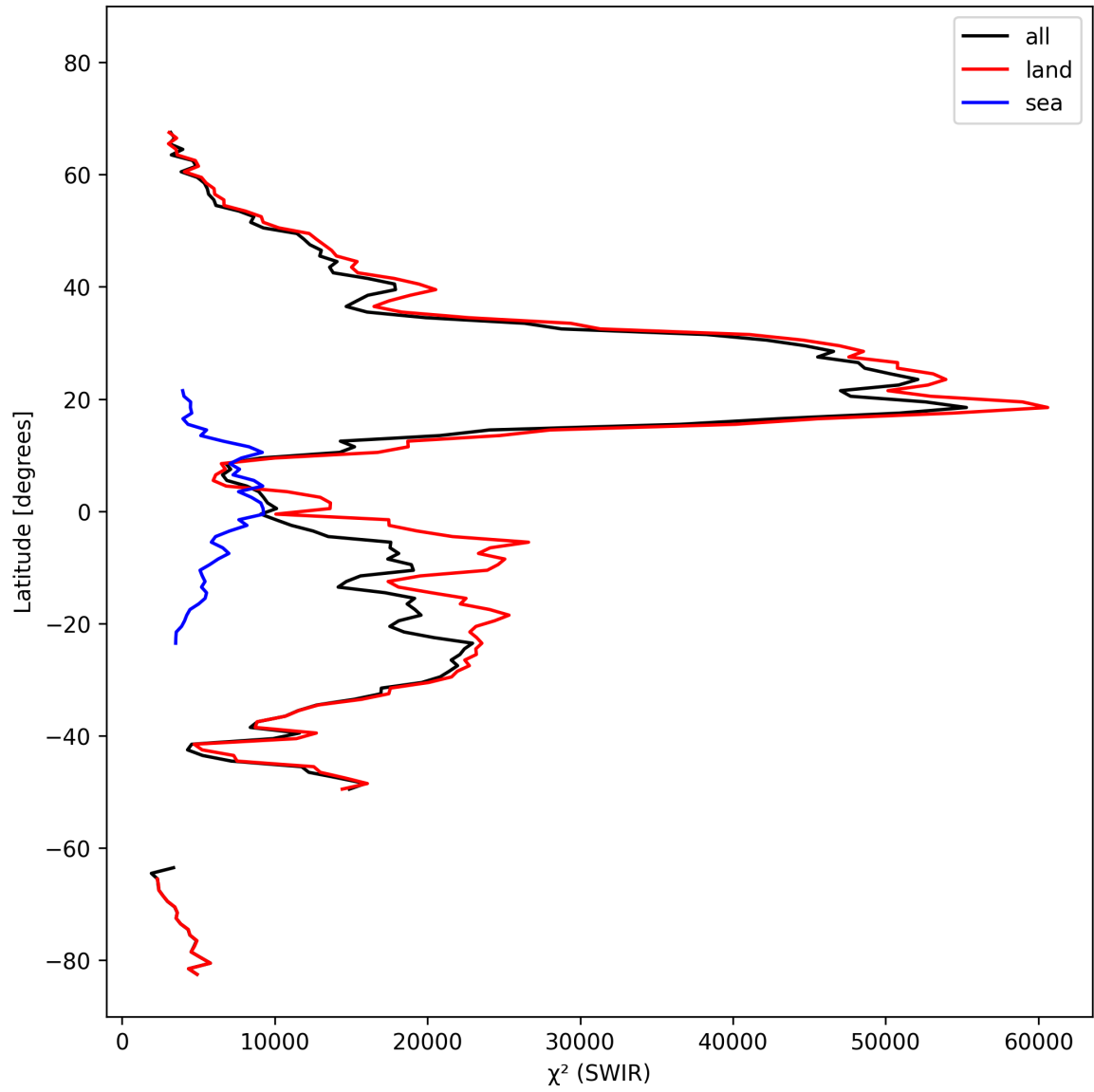
Figure 17: Zonal average of “ \chi^2 (SWIR)” for 2024-10-11 to 2024-10-13.
