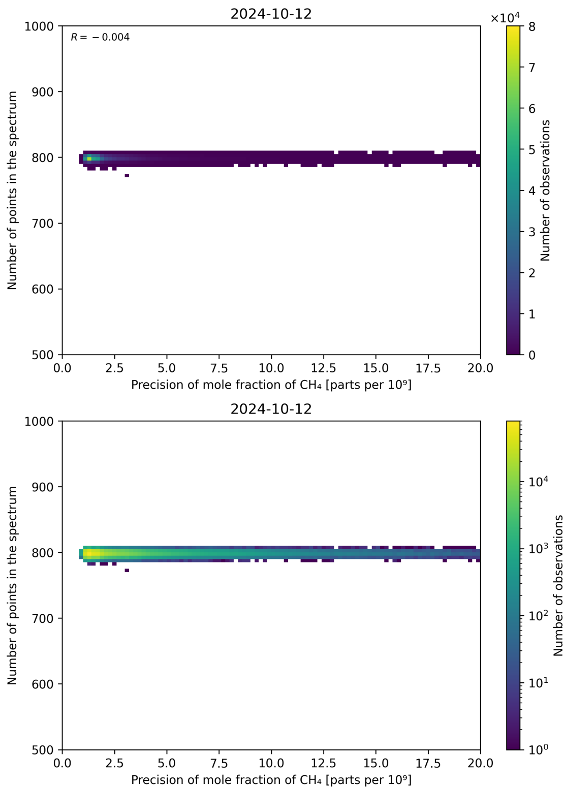
Figure 84: Scatter density plot of “Precision of mole fraction of CH 4 ” against “Number of points in the spectrum” for 2024-10-11 to 2024-10-13.
