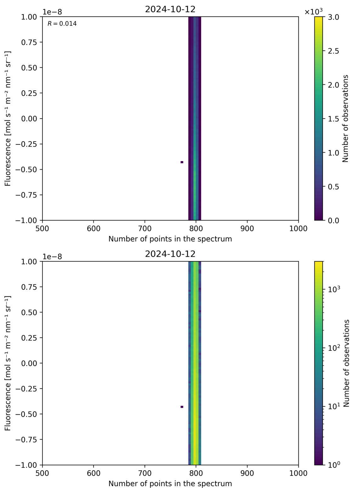
Figure 91: Scatter density plot of “Number of points in the spectrum” against “Fluorescence” for 2024-10-11 to 2024-10-13.
