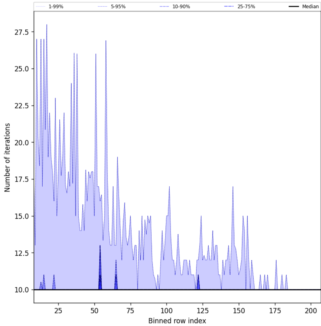
Figure 42: Along track statistics of “Number of iterations” for 2024-10-11 to 2024-10-13
