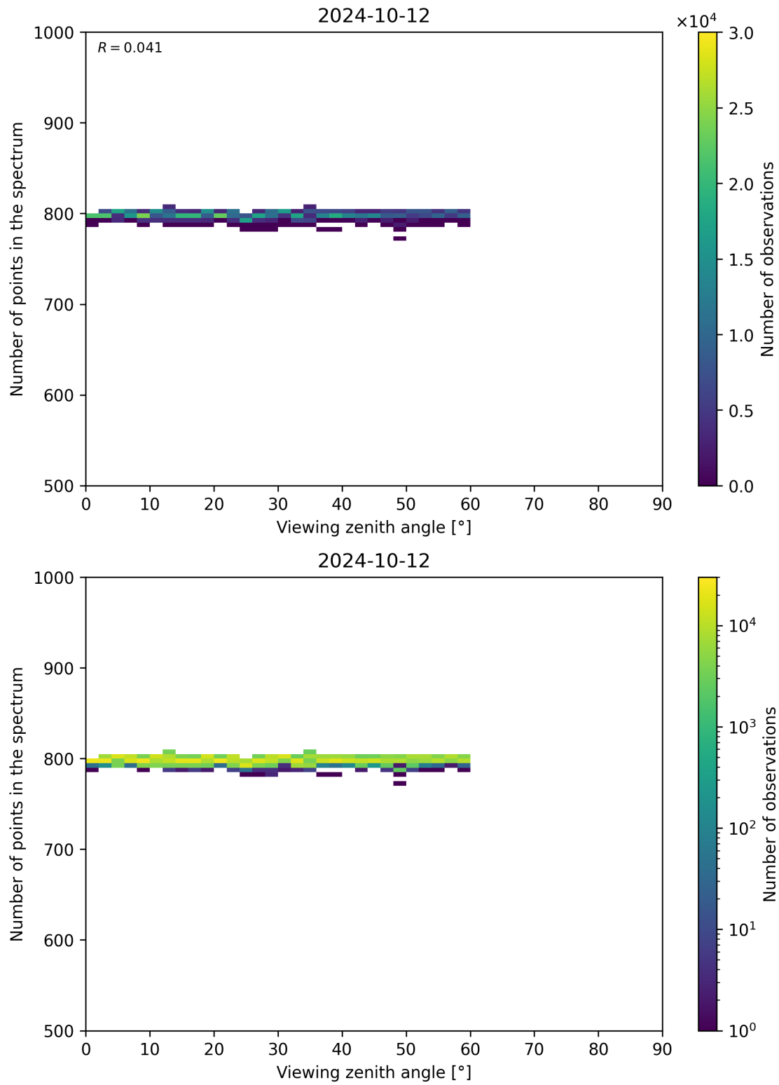
Figure 114: Scatter density plot of “Viewing zenith angle” against “Number of points in the spectrum” for 2024-10-11 to 2024-10-13.
