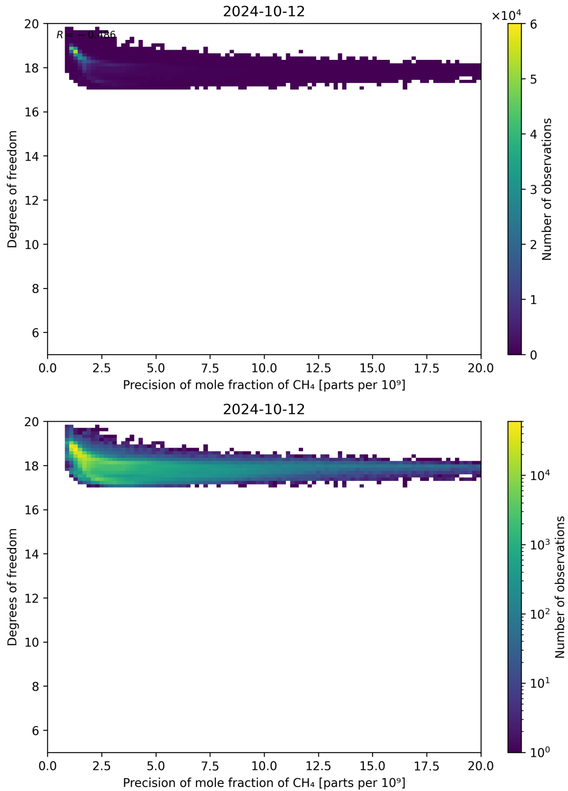
Figure 80: Scatter density plot of “Precision of mole fraction of CH 4 ” against “Degrees of freedom” for 2024-10-11 to 2024-10-13.
