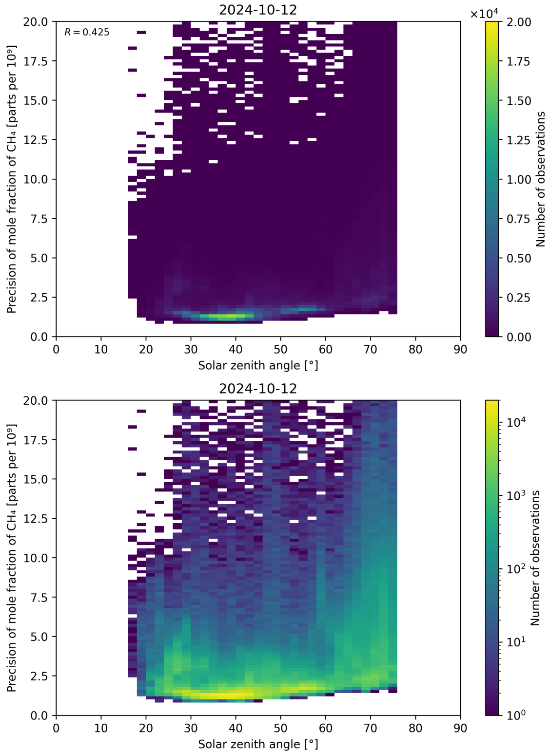
Figure 101: Scatter density plot of “Solar zenith angle” against “Precision of mole fraction of CH 4 ” for 2024-10-11 to 2024-10-13.
