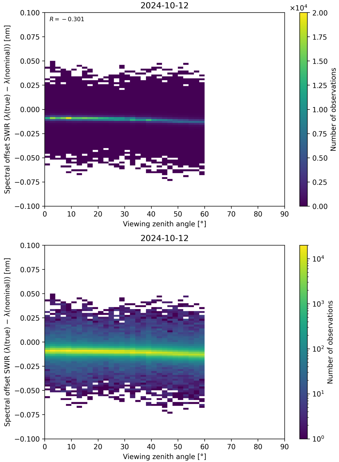
Figure 116: Scatter density plot of “Viewing zenith angle” against “Spectral offset SWIR ( \lambda_{\text{true}} - \lambda_{\text{nominal}} )” for 2024-10-11 to 2024-10-13.
