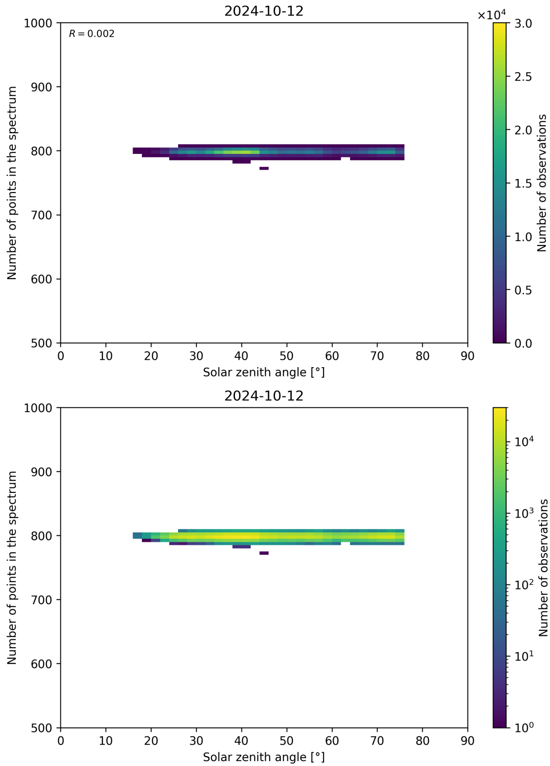
Figure 103: Scatter density plot of “Solar zenith angle” against “Number of points in the spectrum” for 2024-10-11 to 2024-10-13.
