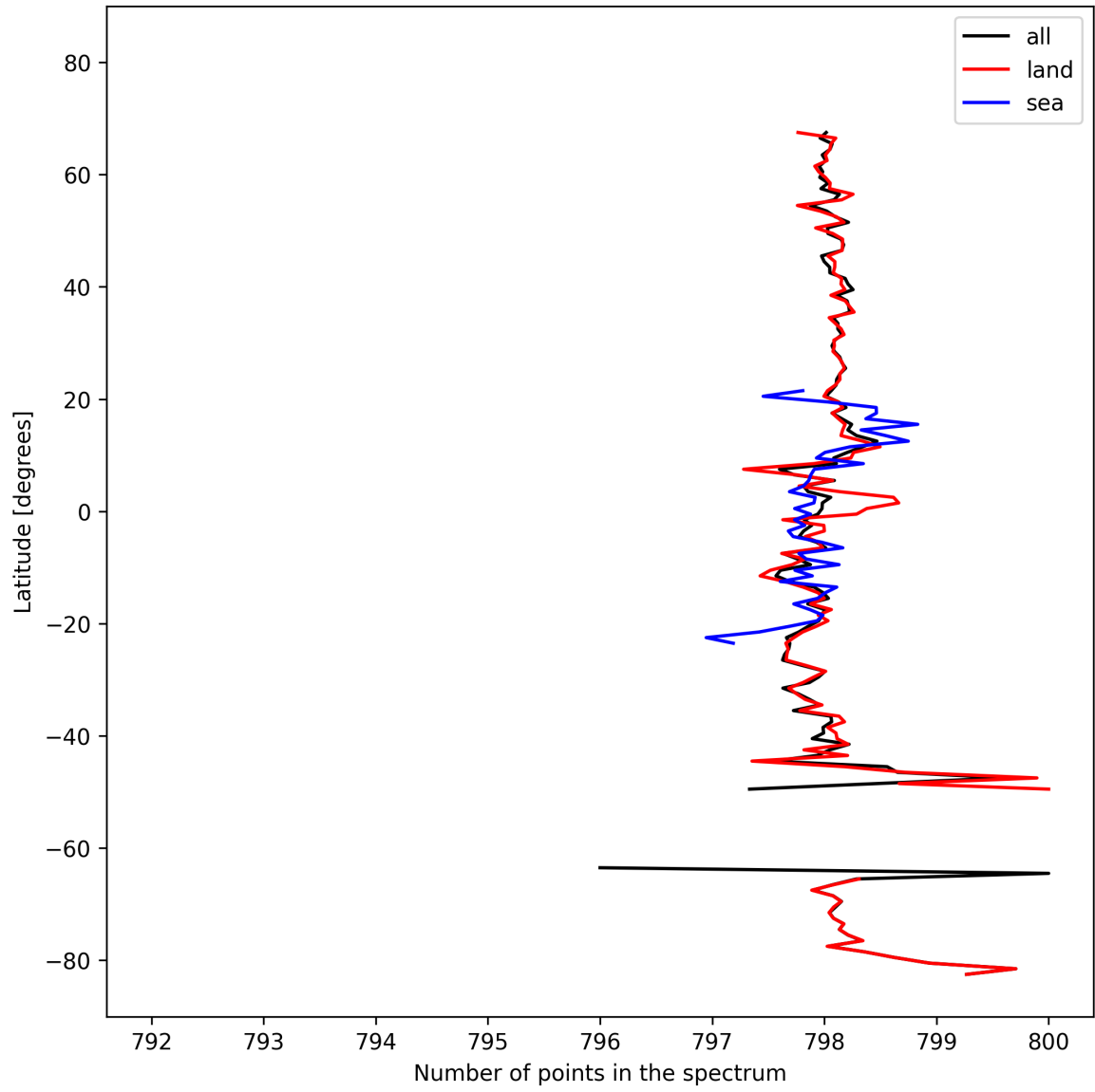
Figure 15: Zonal average of “Number of points in the spectrum” for 2024-10-11 to 2024-10-13.
