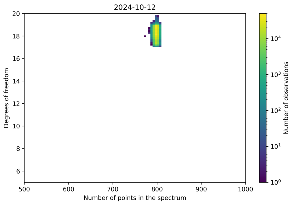
Figure 90: Scatter density plot of “Number of points in the spectrum” against “Degrees of freedom” for 2024-10-11 to 2024-10-13.
