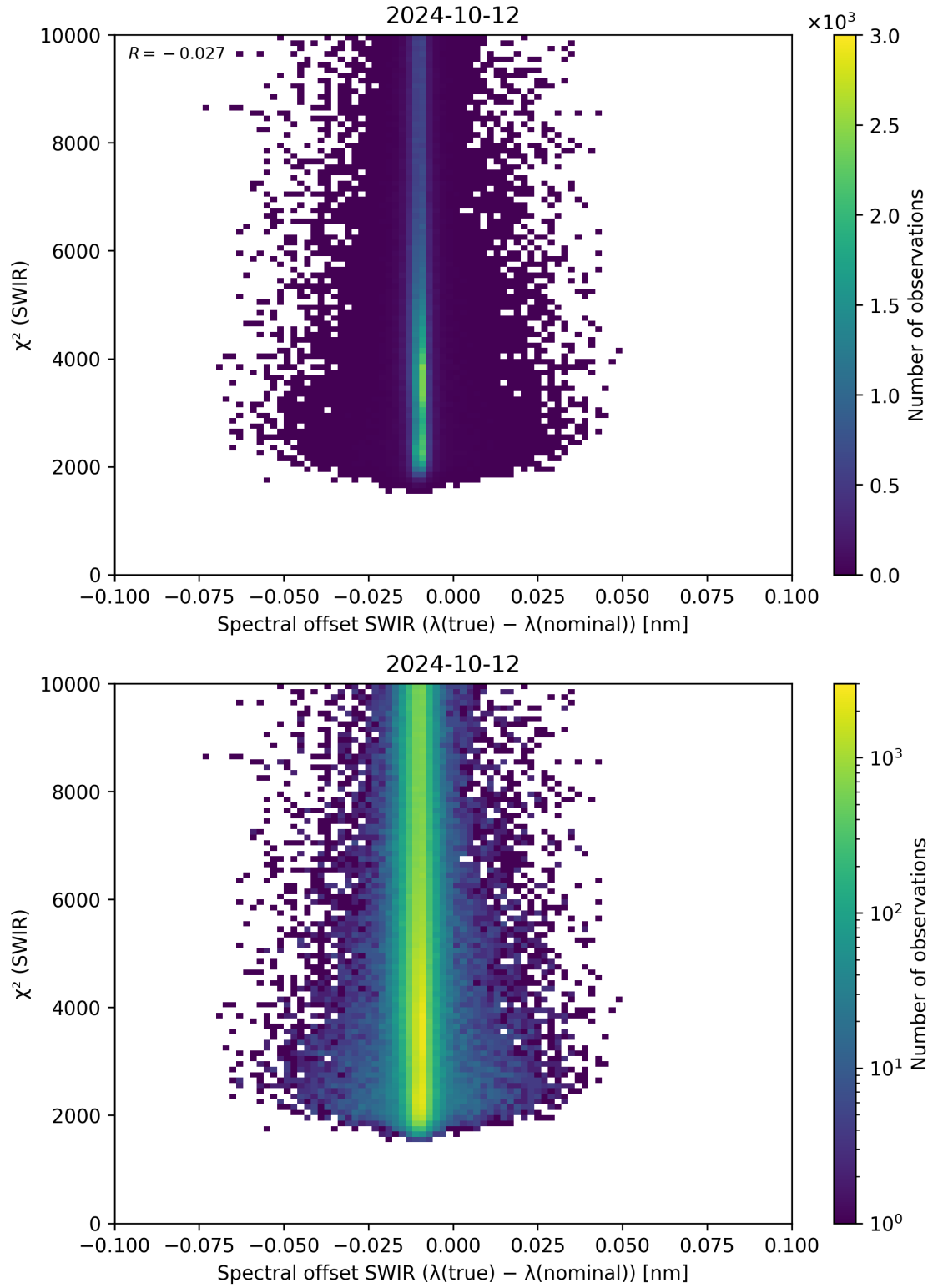
Figure 118: Scatter density plot of “Spectral offset SWIR ( \lambda_{\text{true}} - \lambda_{\text{nominal}} )” against “ \chi^2 (SWIR)” for 2024-10-11 to 2024-10-13.
