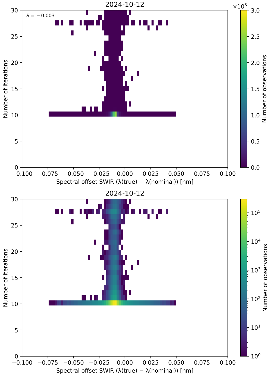
Figure 121: Scatter density plot of “Spectral offset SWIR ( \lambda_{\text{true}} - \lambda_{\text{nominal}} )” against “Number of iterations” for 2024-10-11 to 2024-10-13.
