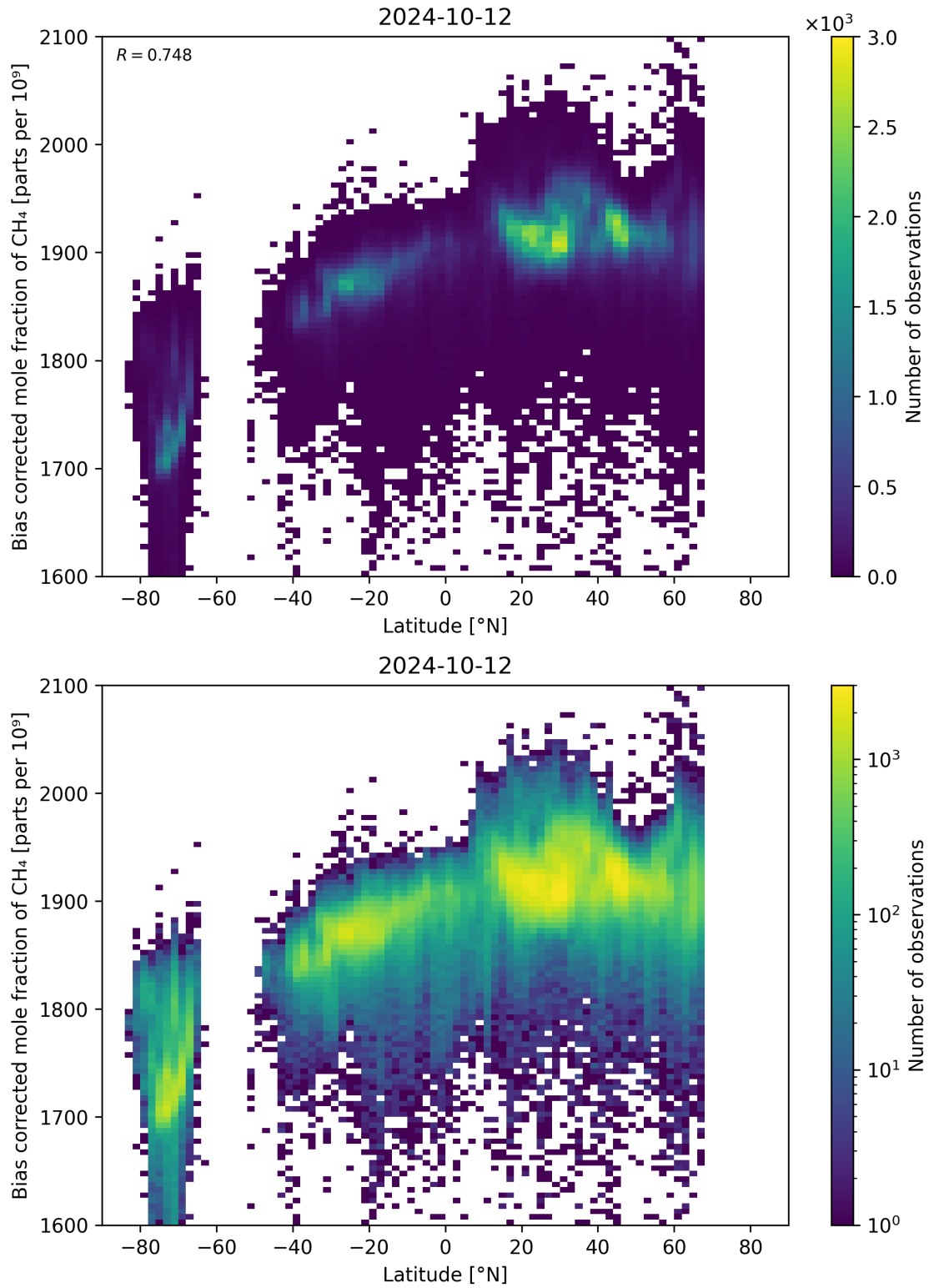
Figure 58: Scatter density plot of “Latitude” against “Bias corrected mole fraction of \text{CH}_4 ” for 2024-10-11 to 2024-10-13.
