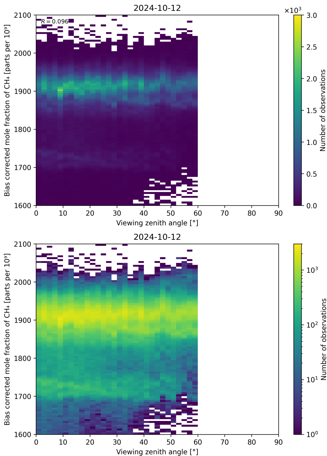
Figure 111: Scatter density plot of “Viewing zenith angle” against “Bias corrected mole fraction of CH 4 ” for 2024-10-11 to 2024-10-13.
