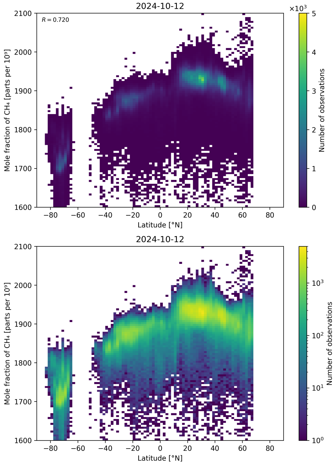
Figure 57: Scatter density plot of “Latitude” against “Mole fraction of \text{CH}_4 ” for 2024-10-11 to 2024-10-13.
