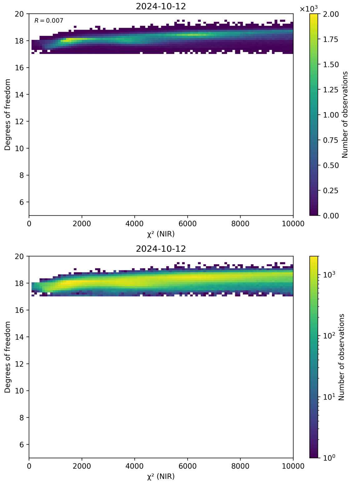
Figure 44: Scatter density plot of “ \chi^2 (NIR)” against “Degrees of freedom” for 2024-10-11 to 2024-10-13.
