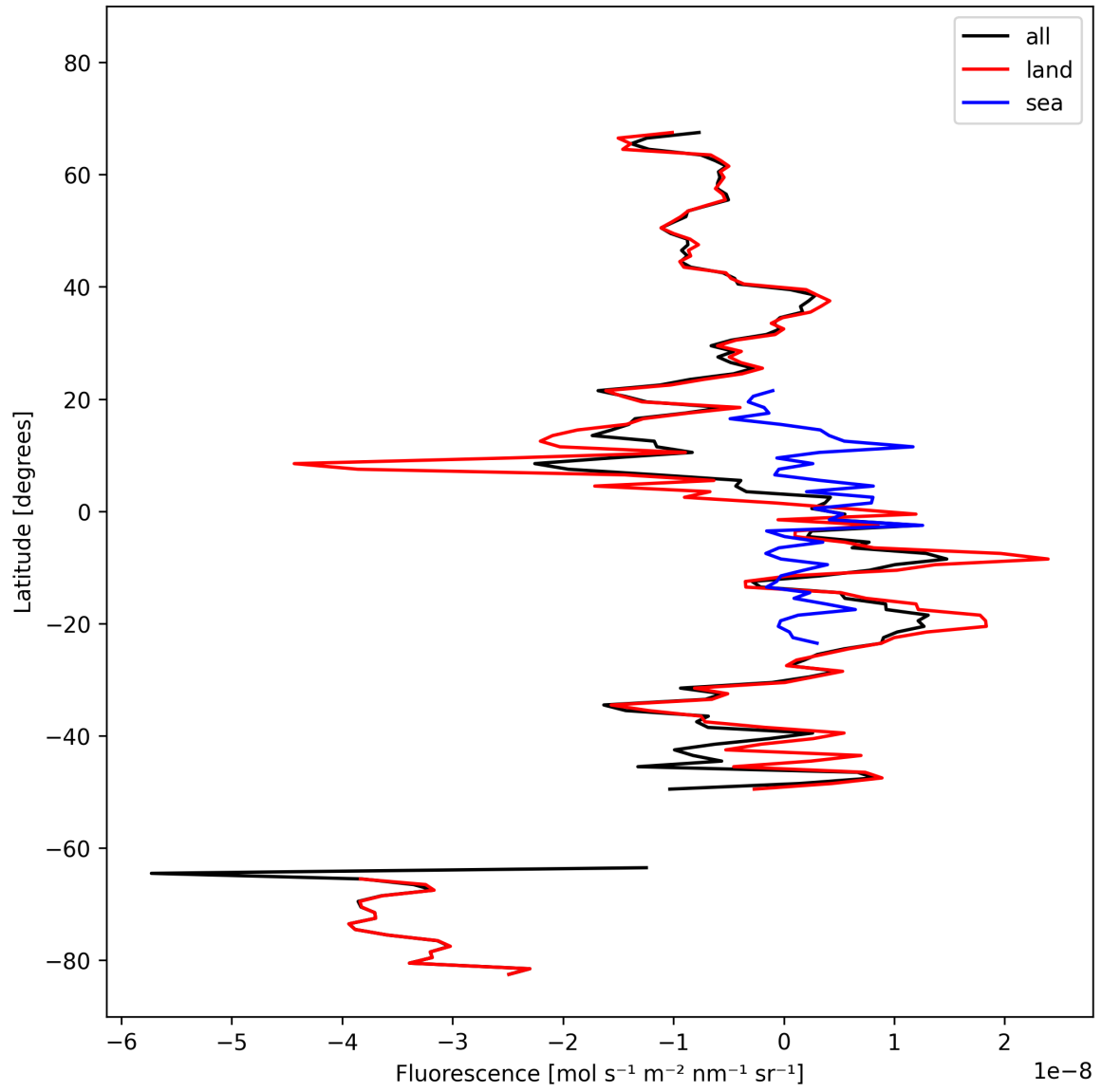
Figure 21: Zonal average of “Fluorescence” for 2024-10-11 to 2024-10-13.
