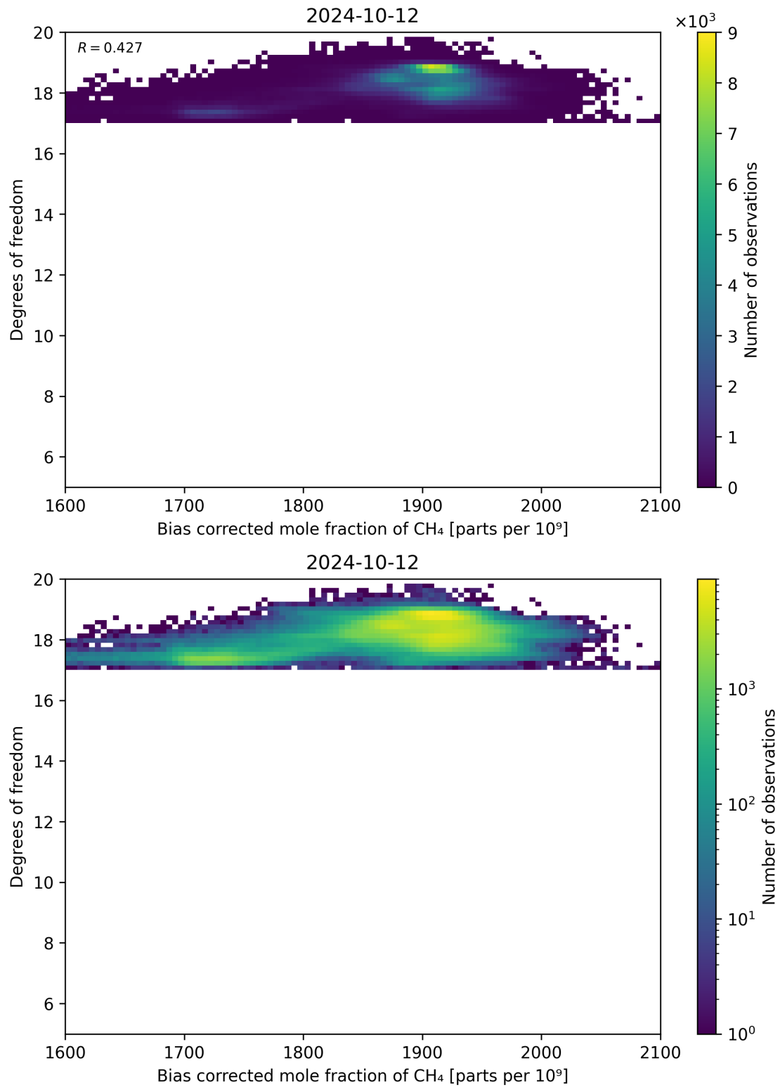
Figure 65: Scatter density plot of “Bias corrected mole fraction of CH 4 ” against “Degrees of freedom” for 2024-10-11 to 2024-10-13.
