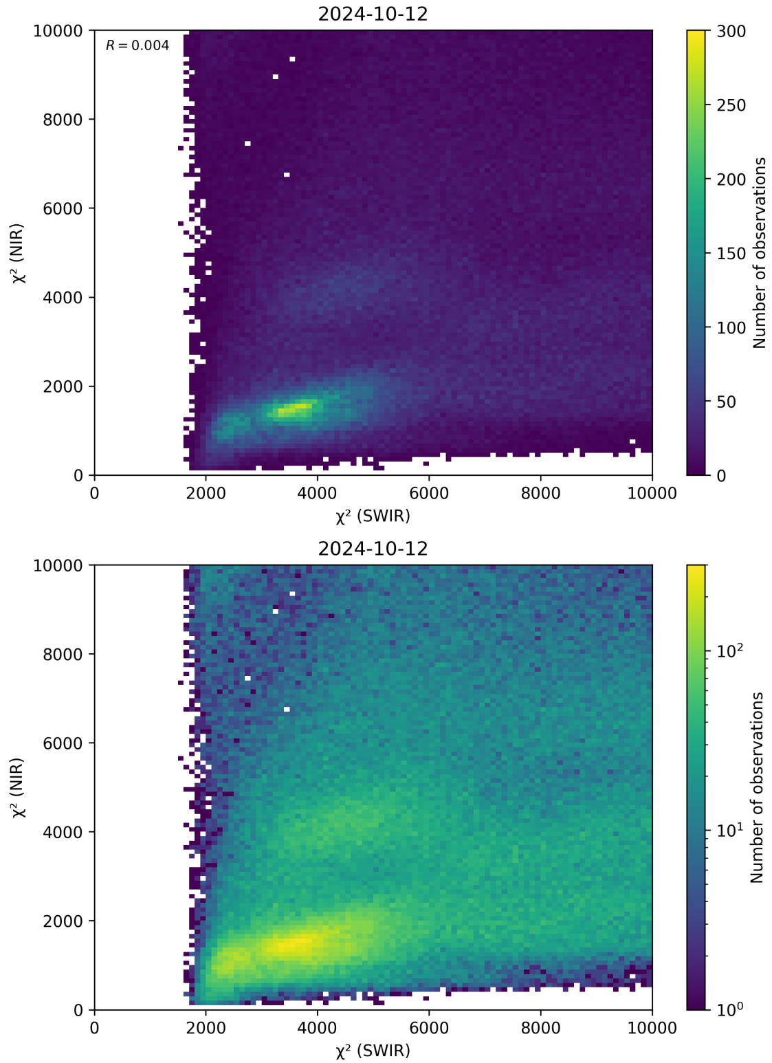
Figure 47: Scatter density plot of “ \chi^2 (SWIR)” against “ \chi^2 (NIR)” for 2024-10-11 to 2024-10-13.
