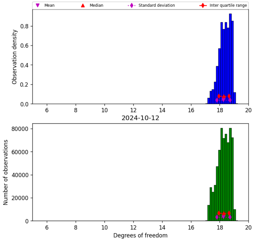
Figure 30: Histogram of “Degrees of freedom” for 2024-10-11 to 2024-10-13
