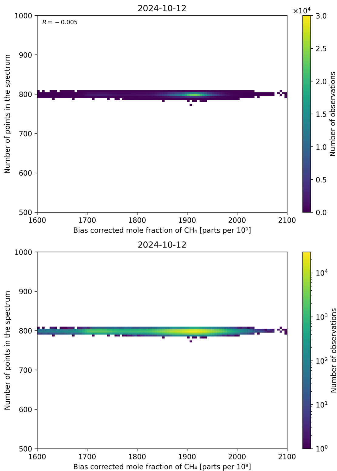
Figure 68: Scatter density plot of “Bias corrected mole fraction of CH 4 ” against “Number of points in the spectrum” for 2024-10-11 to 2024-10-13.
