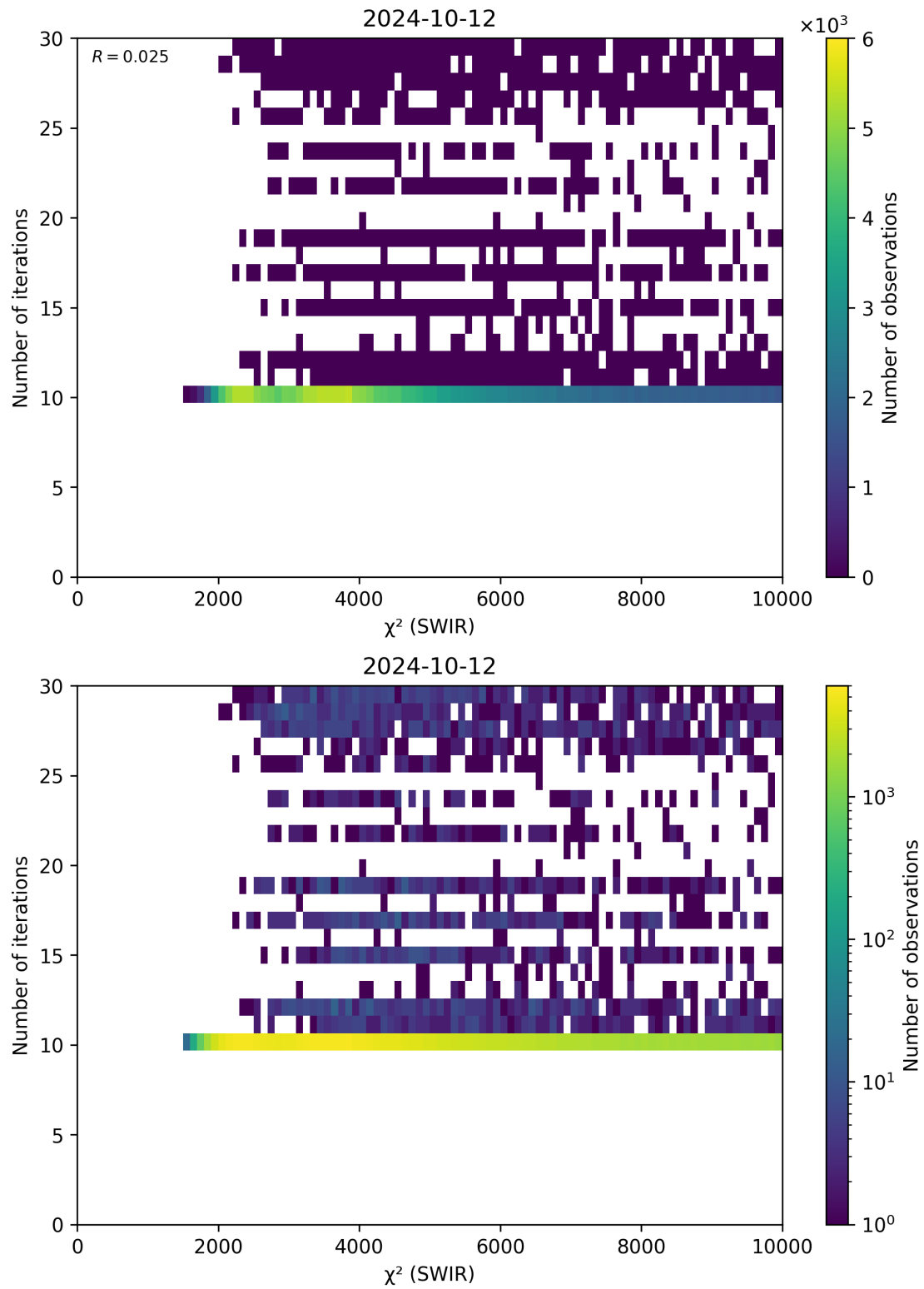
Figure 50: Scatter density plot of " \chi^2 (SWIR)" against "Number of iterations" for 2024-10-11 to 2024-10-13.
