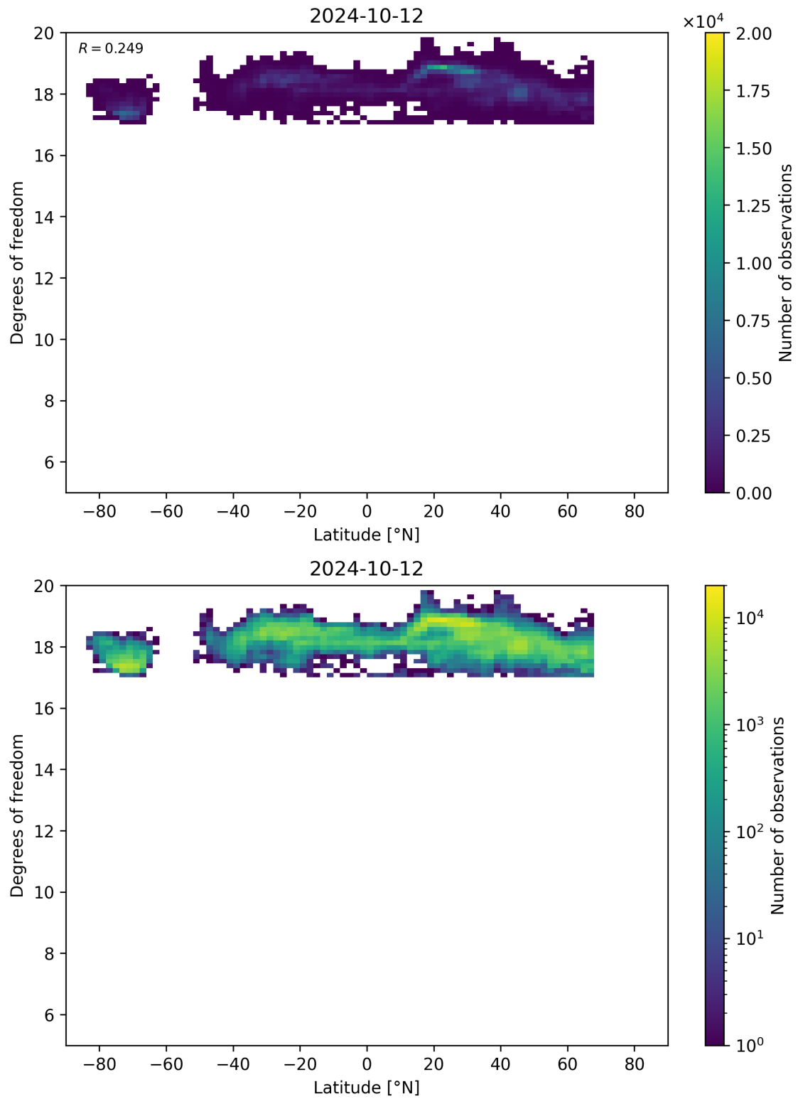
Figure 55: Scatter density plot of “Latitude” against “Degrees of freedom” for 2024-10-11 to 2024-10-13.
