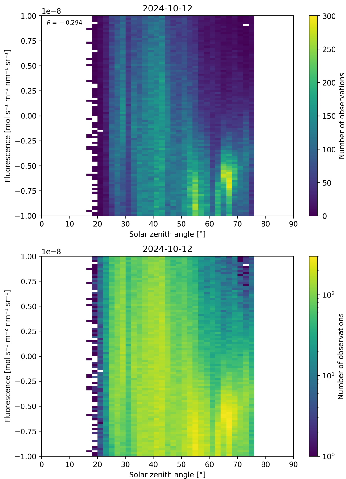
Figure 97: Scatter density plot of “Solar zenith angle” against “Fluorescence” for 2024-10-11 to 2024-10-13.
