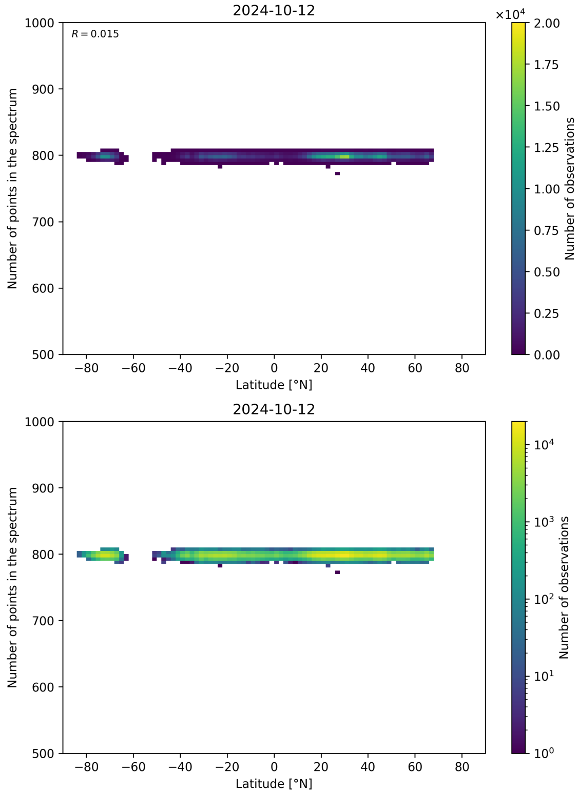
Figure 61: Scatter density plot of “Latitude” against “Number of points in the spectrum” for 2024-10-11 to 2024-10-13.
