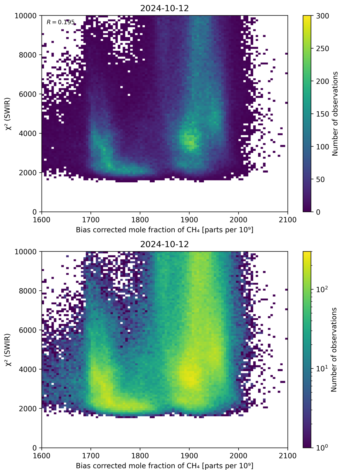
Figure 64: Scatter density plot of “Bias corrected mole fraction of \text{CH}_4 ” against “ \chi^2 (SWIR)” for 2024-10-11 to 2024-10-13.
