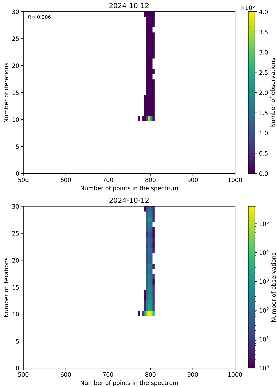
Figure 92: Scatter density plot of “Number of points in the spectrum” against “Number of iterations” for 2024-10-11 to 2024-10-13.
