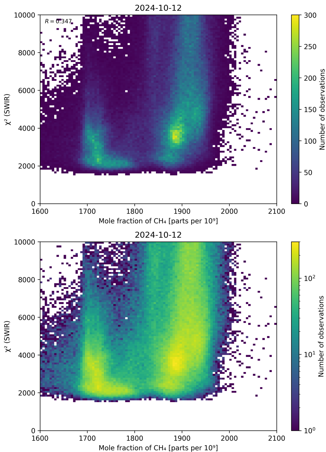
Figure 71: Scatter density plot of “Mole fraction of \text{CH}_4 ” against “ \chi^2 (SWIR)” for 2024-10-11 to 2024-10-13.
