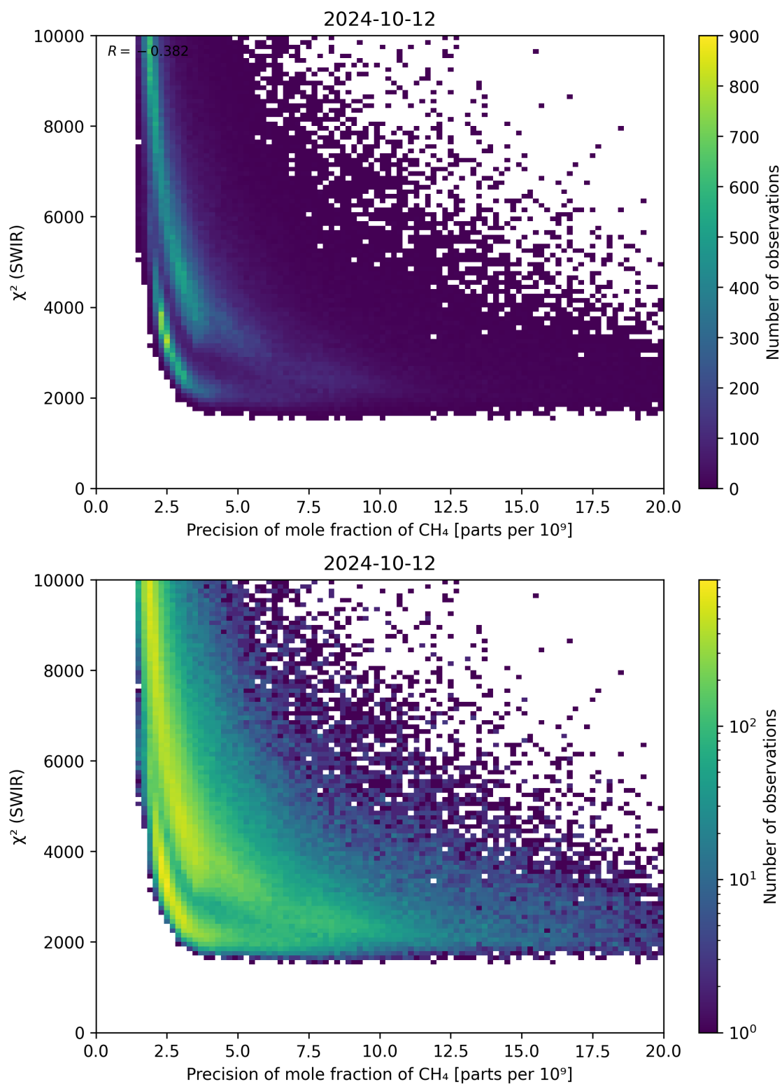
Figure 79: Scatter density plot of “Precision of mole fraction of \text{CH}_4 ” against “ \chi^2 (SWIR)” for 2024-10-11 to 2024-10-13.
