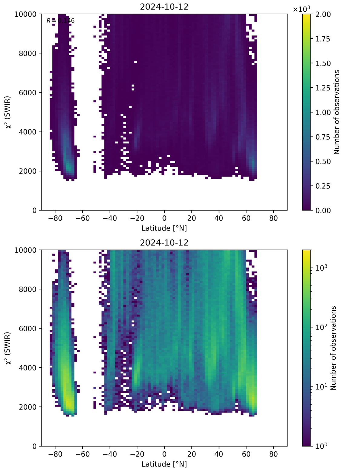
Figure 54: Scatter density plot of “Latitude” against “ \chi^2 (SWIR)” for 2024-10-11 to 2024-10-13.
