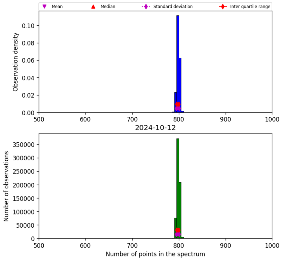
Figure 26: Histogram of “Number of points in the spectrum” for 2024-10-11 to 2024-10-13
