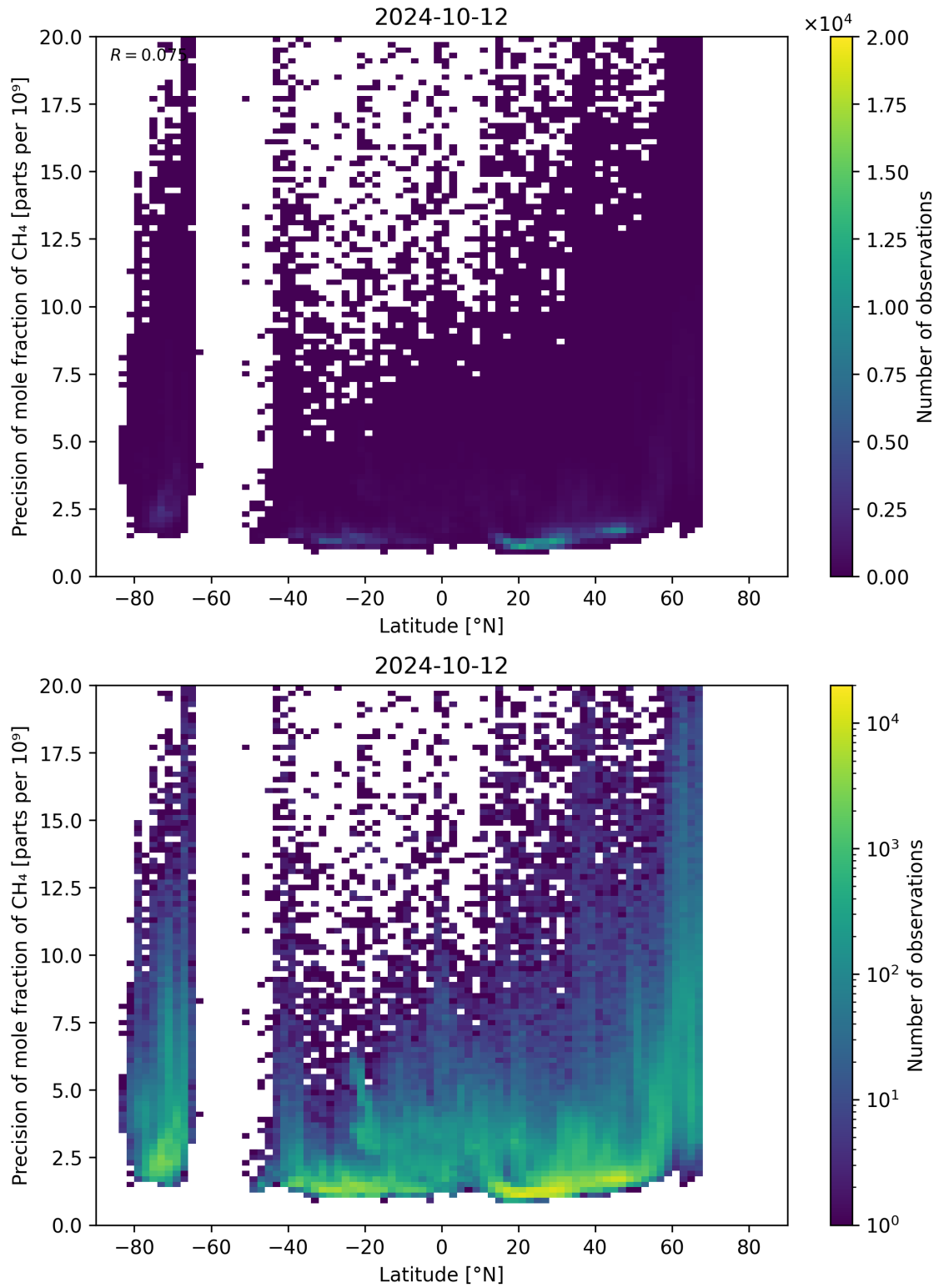
Figure 59: Scatter density plot of “Latitude” against “Precision of mole fraction of CH 4 ” for 2024-10-11 to 2024-10-13.
