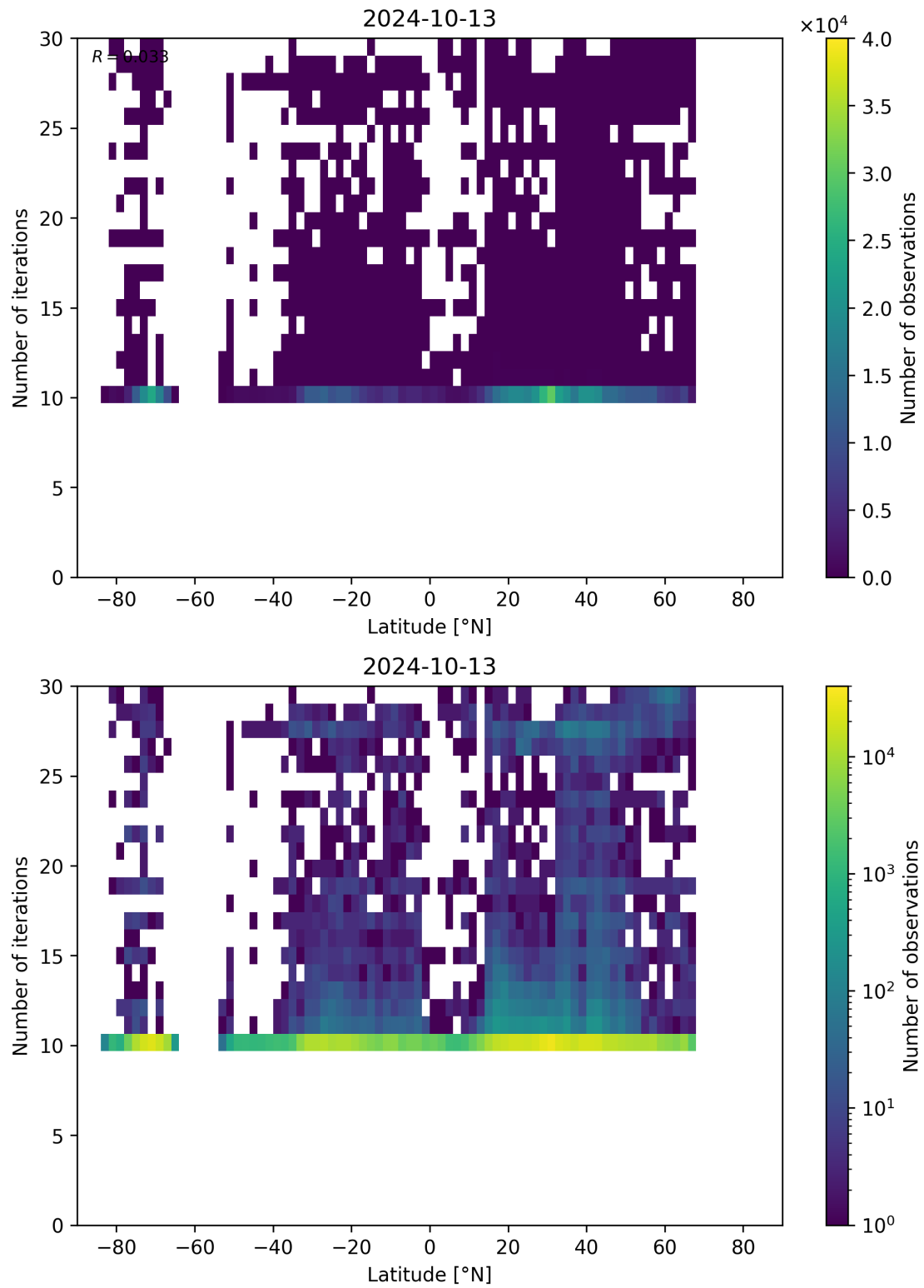
Figure 60: Scatter density plot of “Latitude” against “Number of iterations” for 2024-10-12 to 2024-10-14.
