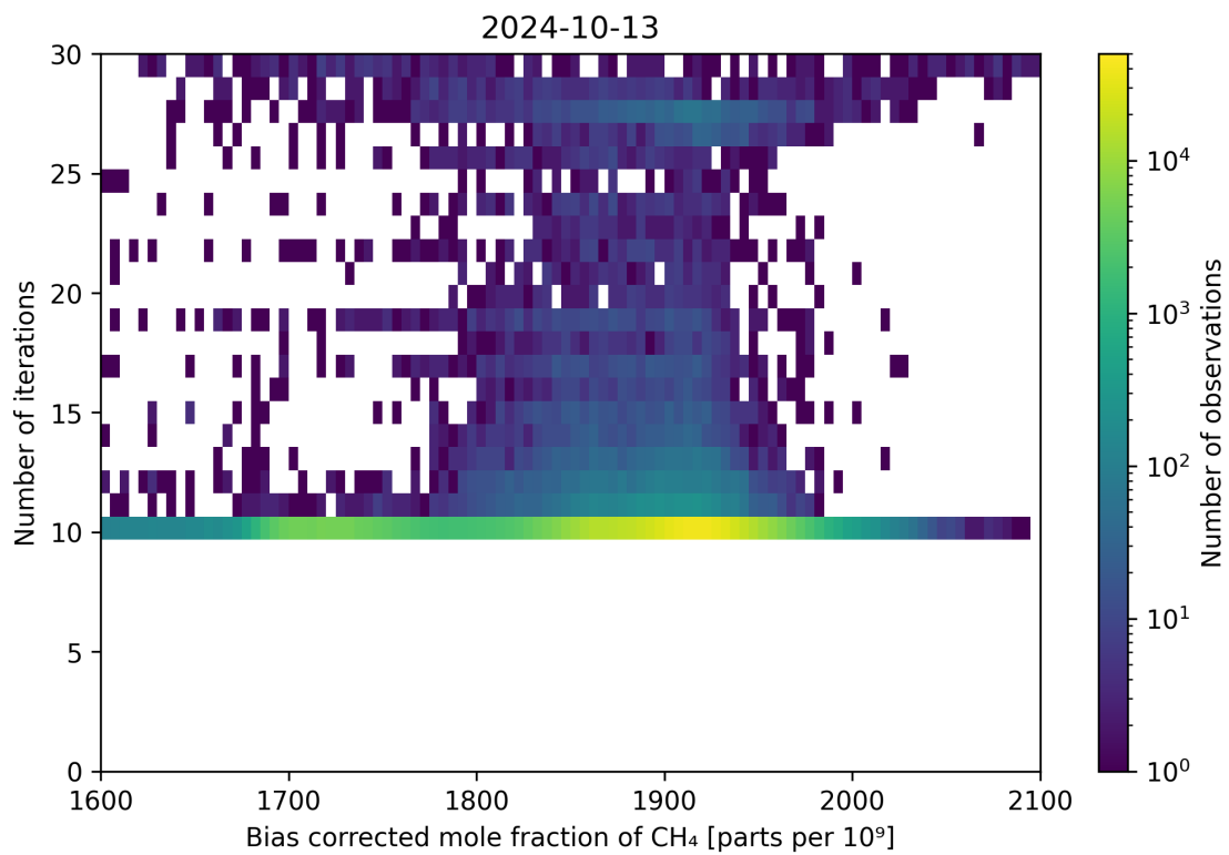
Figure 67: Scatter density plot of “Bias corrected mole fraction of CH 4 ” against “Number of iterations” for 2024-10-12 to 2024-10-14.
