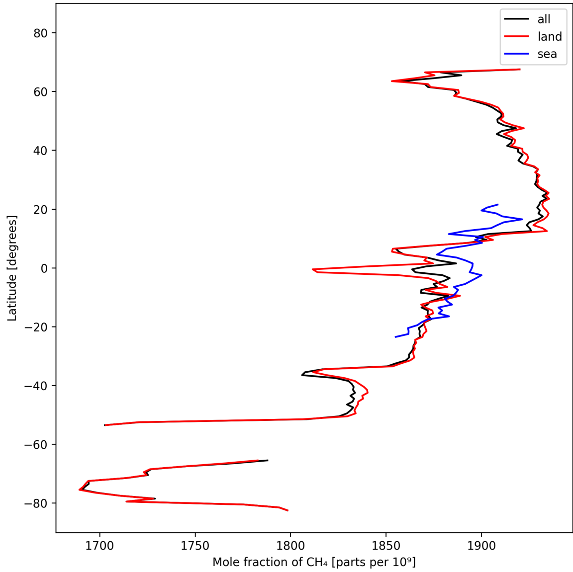
Figure 12: Zonal average of “Mole fraction of \text{CH}_4 ” for 2024-10-12 to 2024-10-14.
