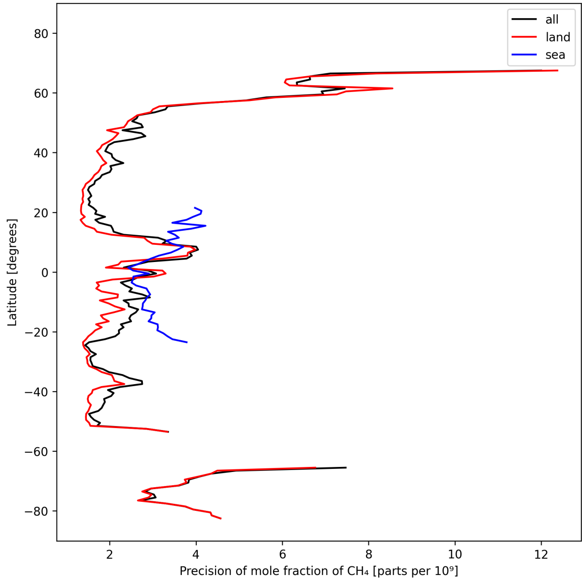
Figure 13: Zonal average of “Precision of mole fraction of CH 4 ” for 2024-10-12 to 2024-10-14.
