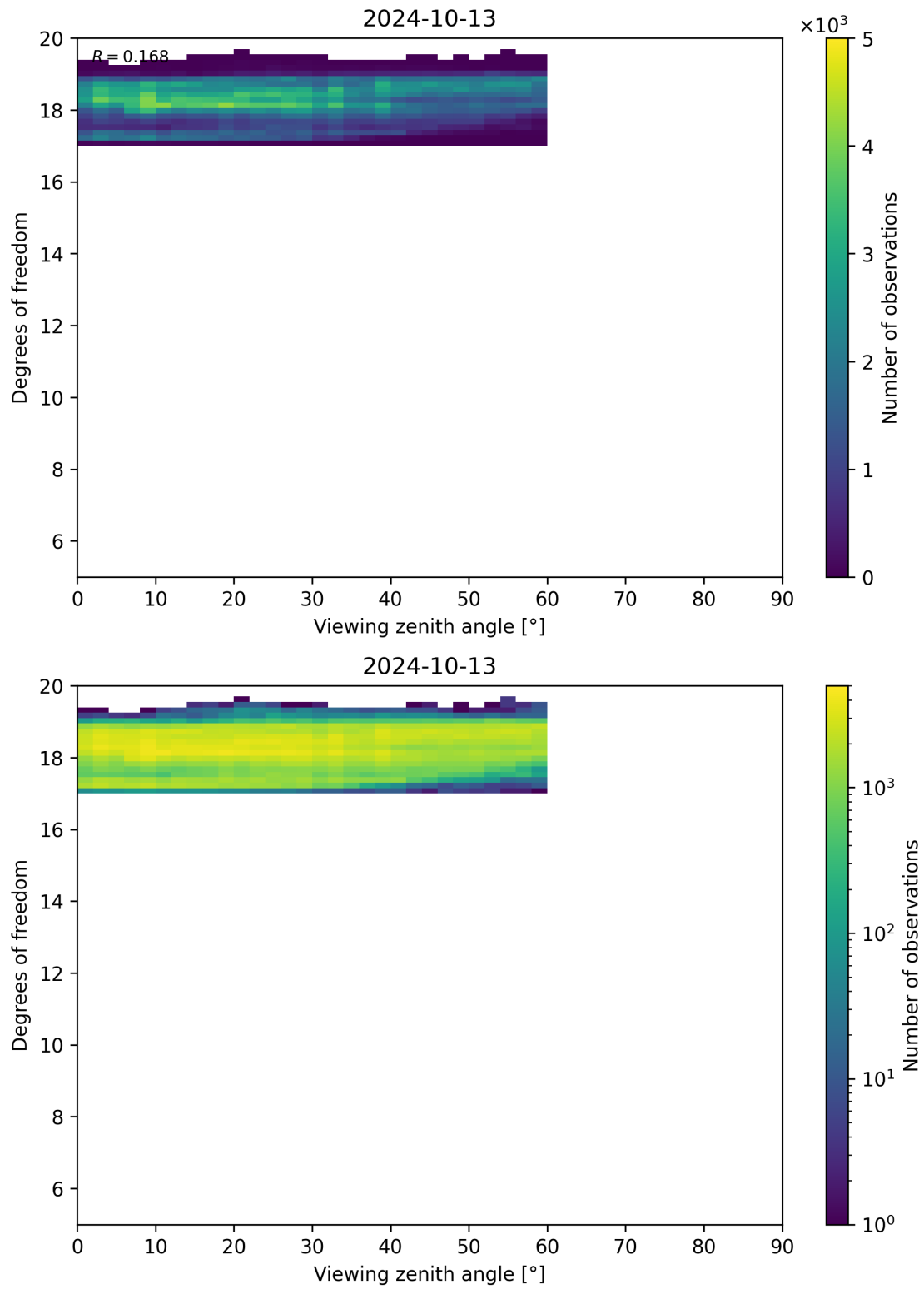
Figure 107: Scatter density plot of “Viewing zenith angle” against “Degrees of freedom” for 2024-10-12 to 2024-10-14.
