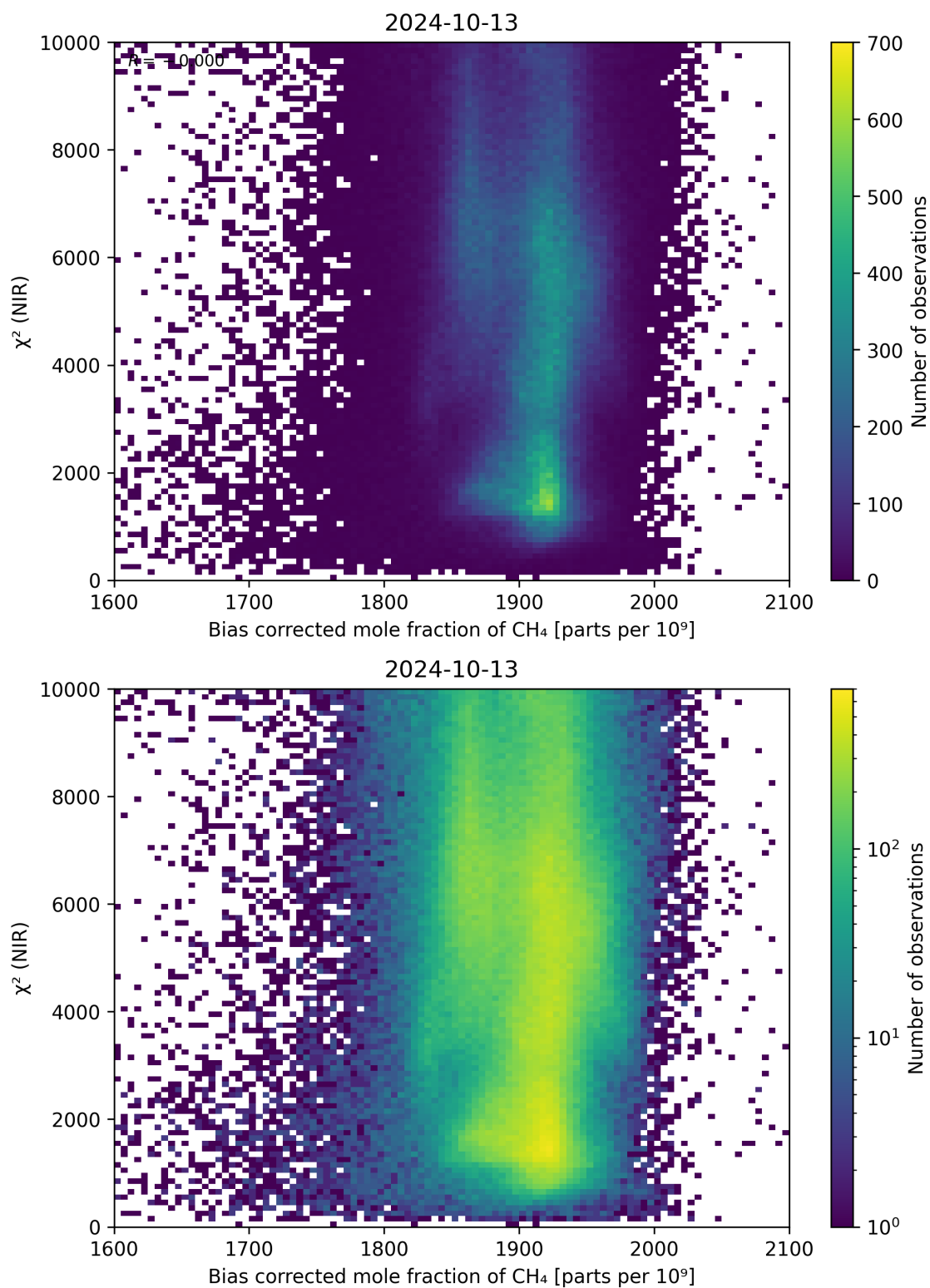
Figure 63: Scatter density plot of “Bias corrected mole fraction of \text{CH}_4 ” against “ \chi^2 (NIR)” for 2024-10-12 to 2024-10-14.
