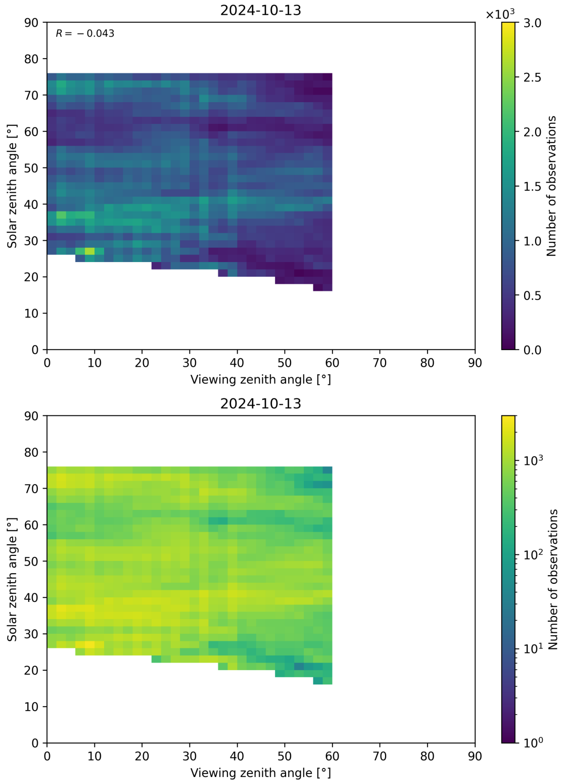
Figure 115: Scatter density plot of “Viewing zenith angle” against “Solar zenith angle” for 2024-10-12 to 2024-10-14.
