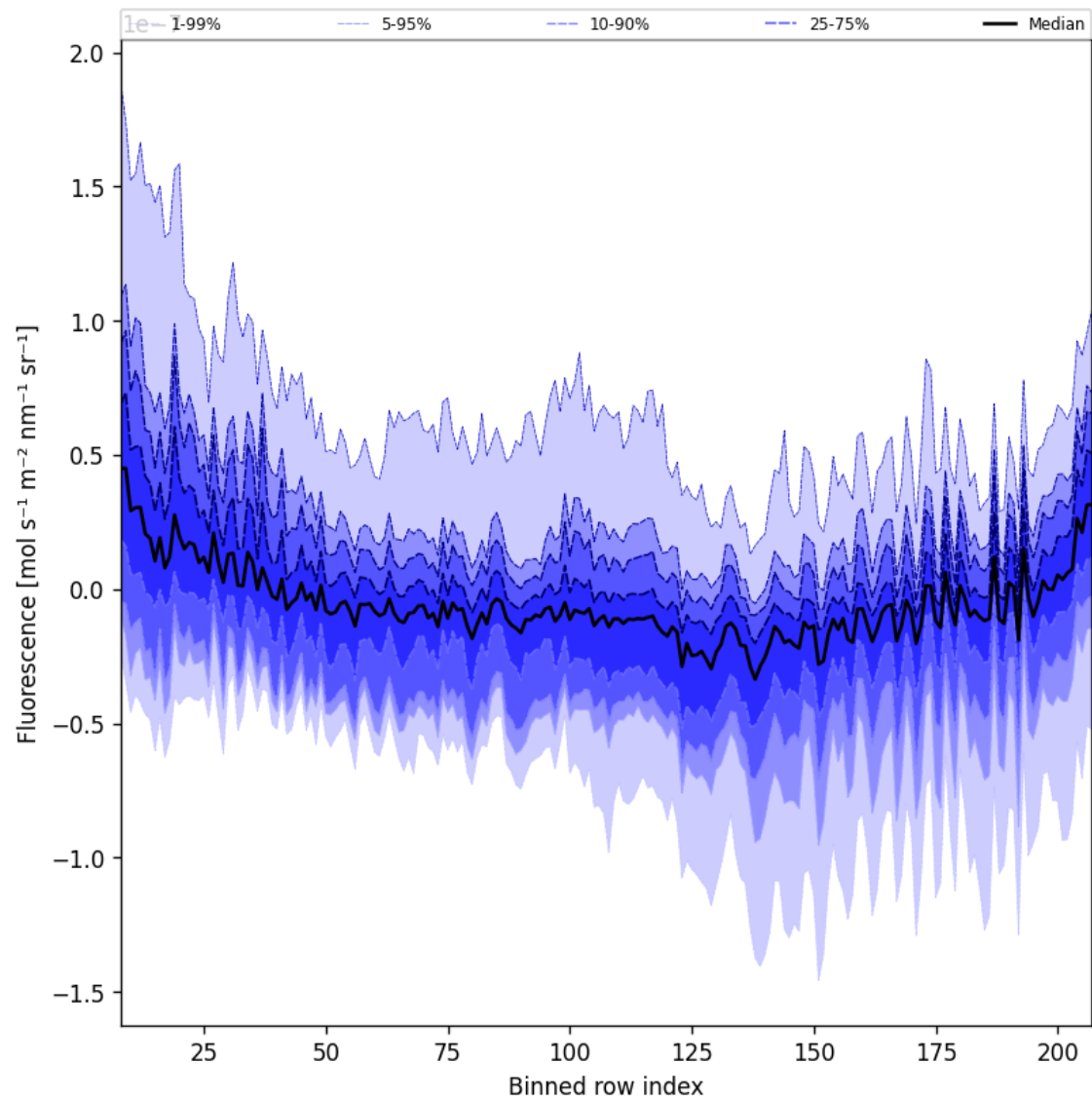
Figure 43: Along track statistics of “Fluorescence” for 2024-10-12 to 2024-10-14
