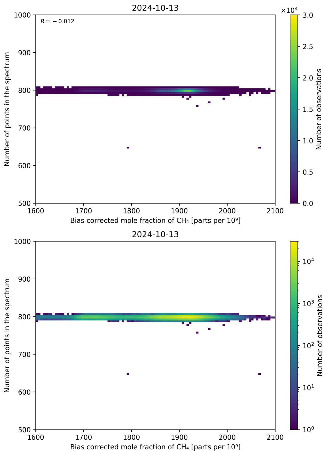
Figure 68: Scatter density plot of “Bias corrected mole fraction of CH 4 ” against “Number of points in the spectrum” for 2024-10-12 to 2024-10-14.
