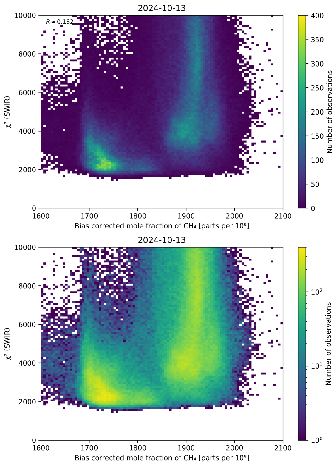
Figure 64: Scatter density plot of “Bias corrected mole fraction of CH 4 ” against “ \chi^2 (SWIR)” for 2024-10-12 to 2024-10-14.
