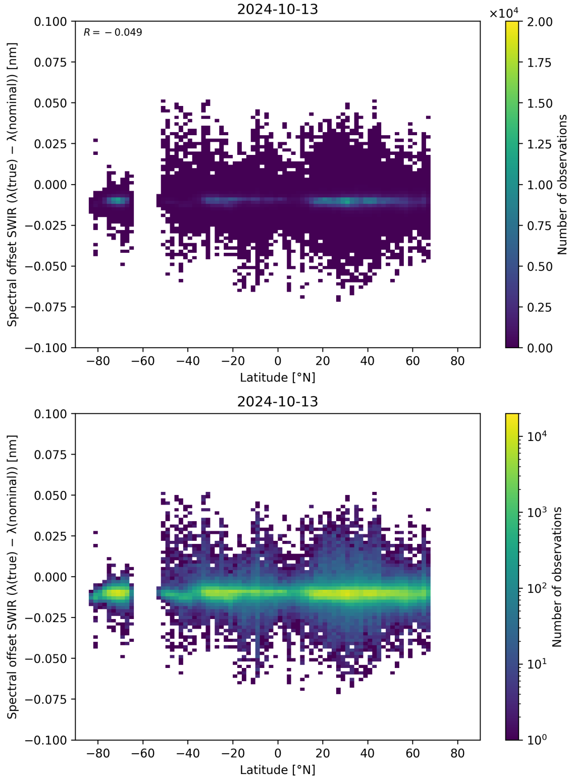
Figure 62: Scatter density plot of “Latitude” against “Spectral offset SWIR ( \lambda_{\text{true}} - \lambda_{\text{nominal}} )” for 2024-10-12 to 2024-10-14.
