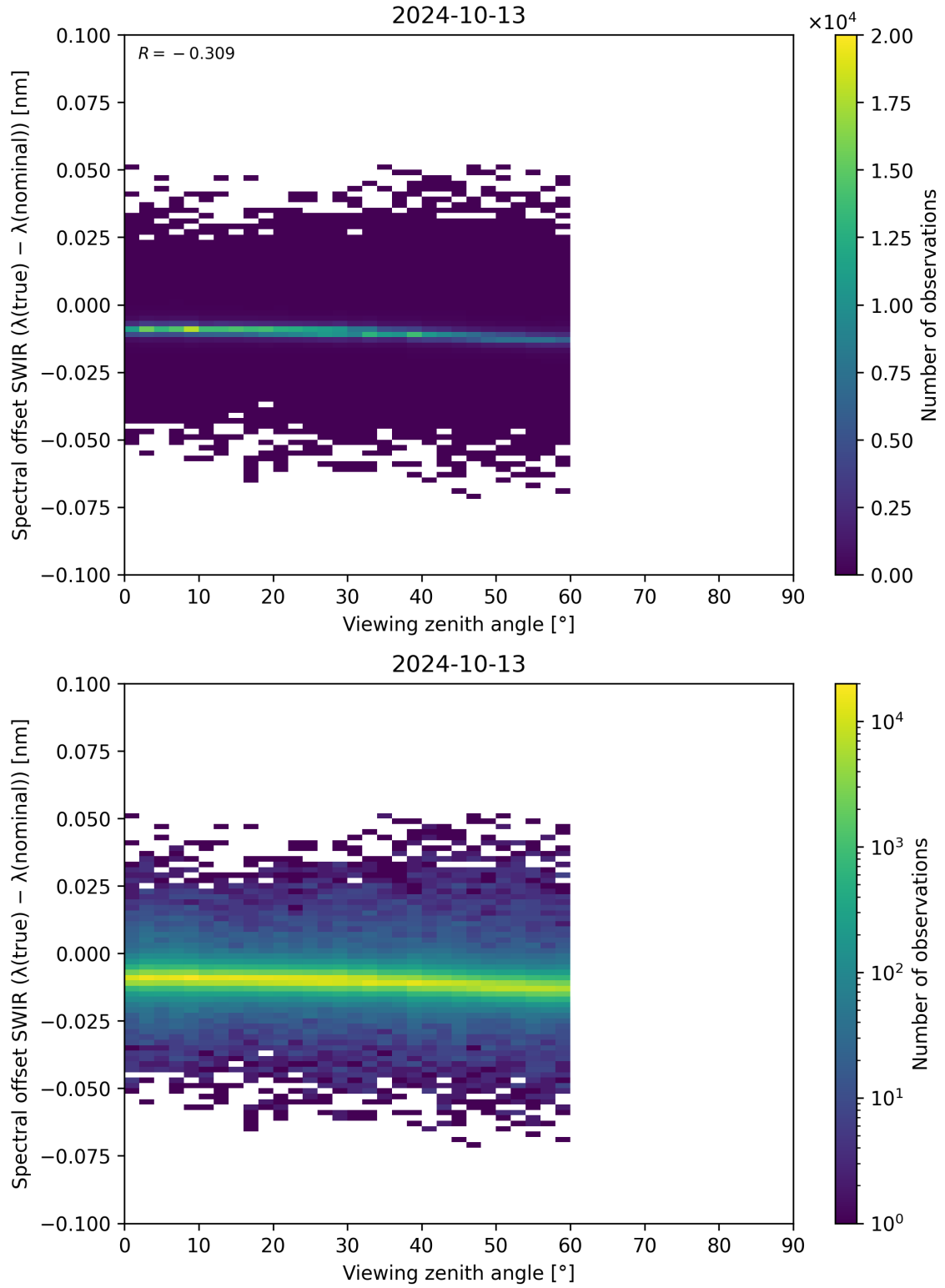
Figure 116: Scatter density plot of “Viewing zenith angle” against “Spectral offset SWIR ( \lambda_{\text{true}} - \lambda_{\text{nominal}} )” for 2024-10-12 to 2024-10-14.
