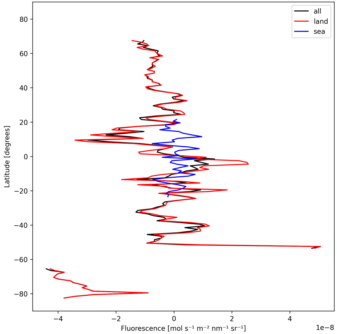
Figure 21: Zonal average of “Fluorescence” for 2024-10-12 to 2024-10-14.
