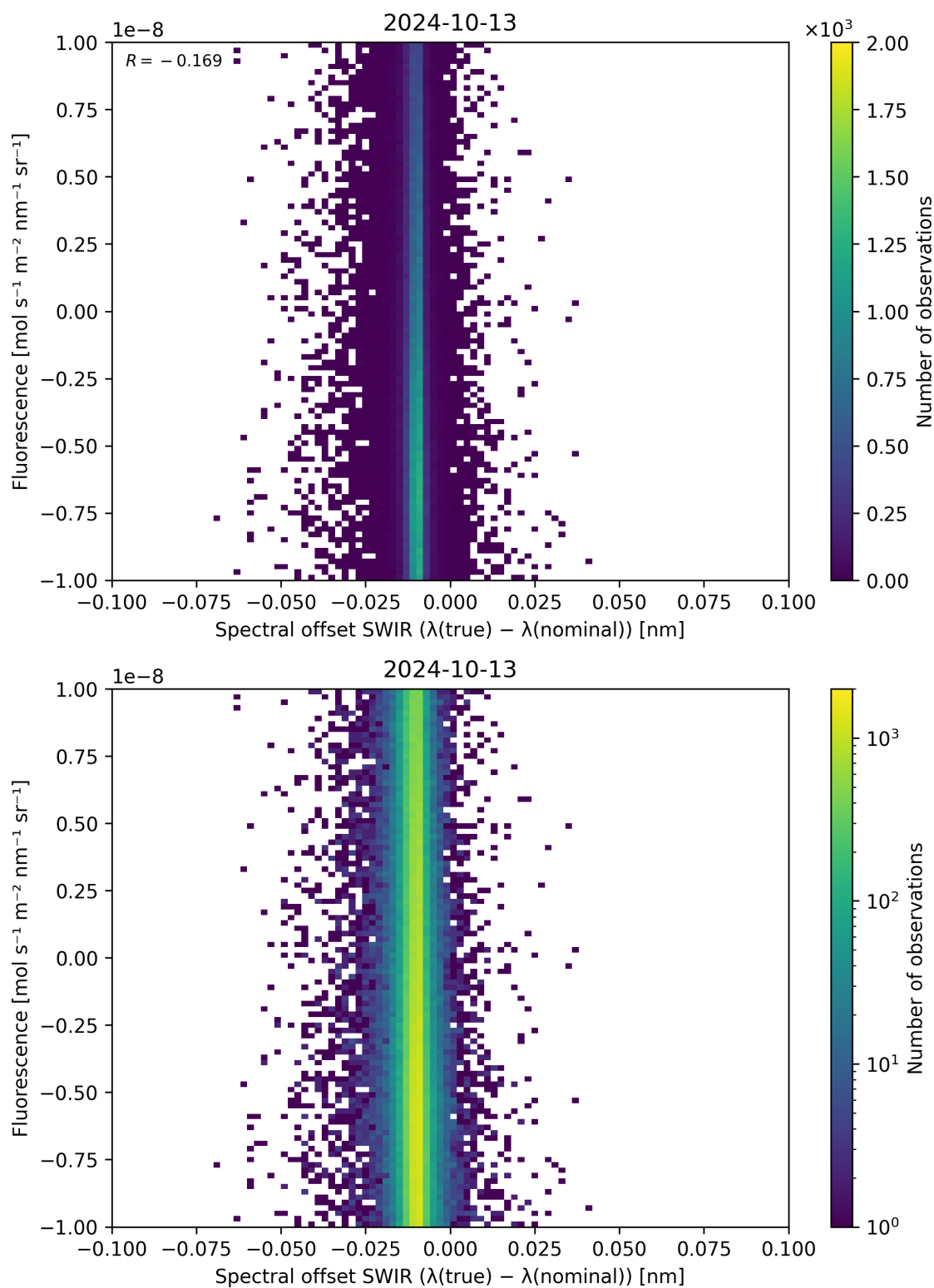
Figure 120: Scatter density plot of “Spectral offset SWIR ( \lambda_{\text{true}} - \lambda_{\text{nominal}} )” against “Fluorescence” for 2024-10-12 to 2024-10-14.
