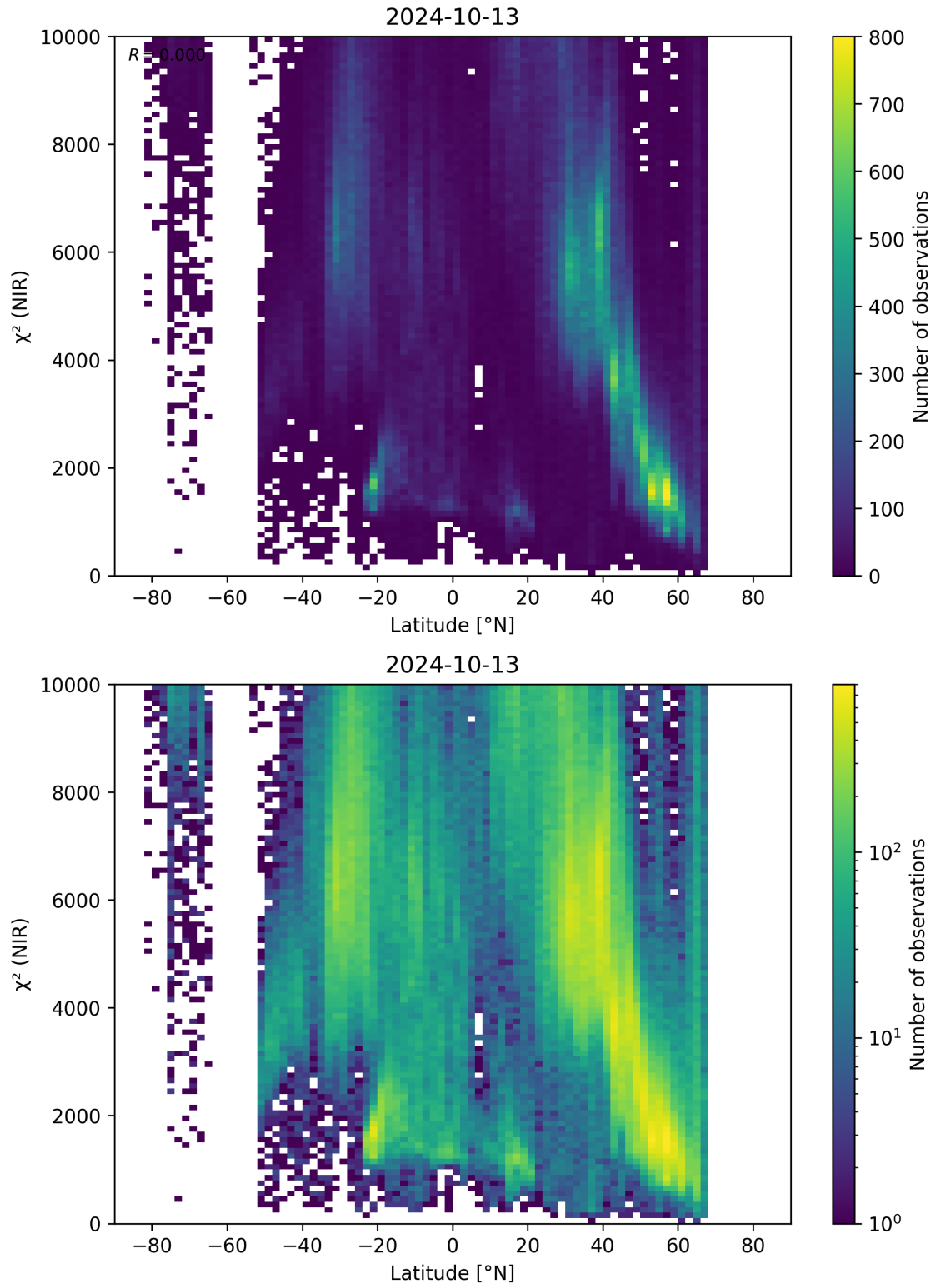
Figure 53: Scatter density plot of “Latitude” against “ \chi^2 (NIR)” for 2024-10-12 to 2024-10-14.
