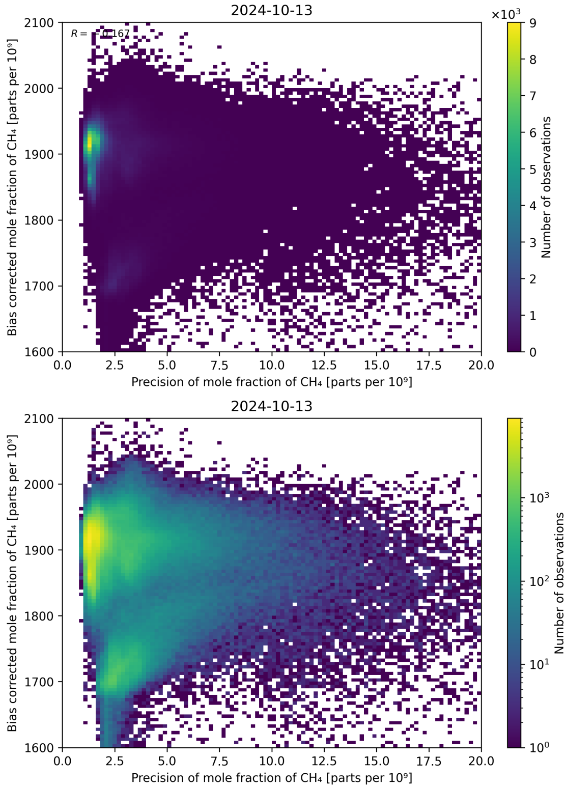
Figure 82: Scatter density plot of “Precision of mole fraction of CH 4 ” against “Bias corrected mole fraction of CH 4 ” for 2024-10-12 to 2024-10-14.
