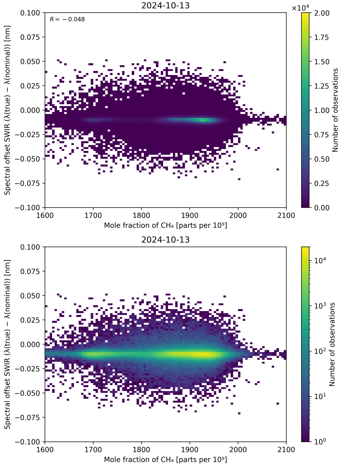
Figure 86: Scatter density plot of “Mole fraction of CH 4 ” against “Spectral offset SWIR ( \lambda_{\text{true}} - \lambda_{\text{nominal}} )” for 2024-10-12 to 2024-10-14.
