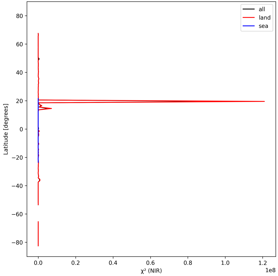
Figure 18: Zonal average of “ \chi^2 (NIR)” for 2024-10-12 to 2024-10-14.
