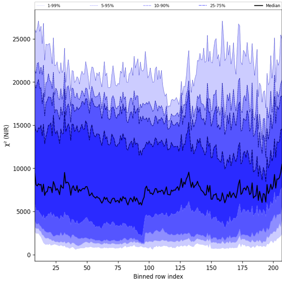
Figure 40: Along track statistics of " \chi^2 (NIR)" for 2024-10-12 to 2024-10-14
