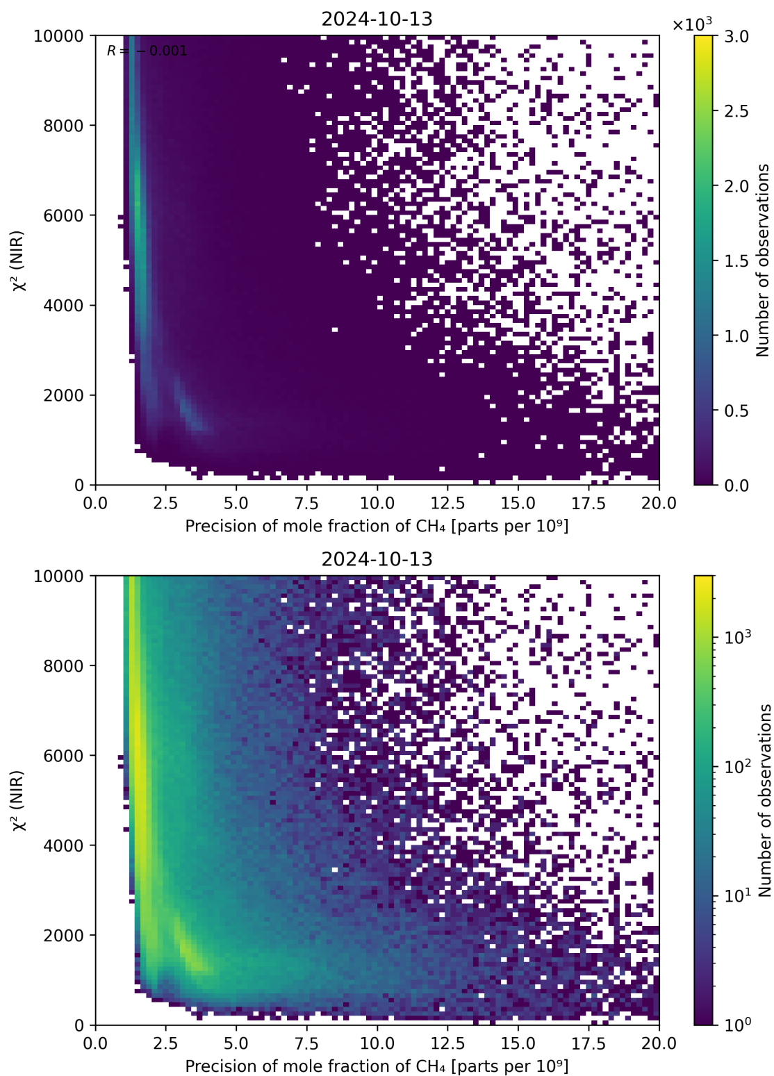
Figure 78: Scatter density plot of “Precision of mole fraction of CH 4 ” against “ \chi^2 (NIR)” for 2024-10-12 to 2024-10-14.
