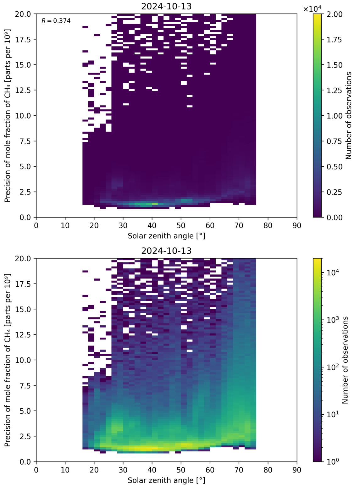
Figure 101: Scatter density plot of “Solar zenith angle” against “Precision of mole fraction of \text{CH}_4 ” for 2024-10-12 to 2024-10-14.
