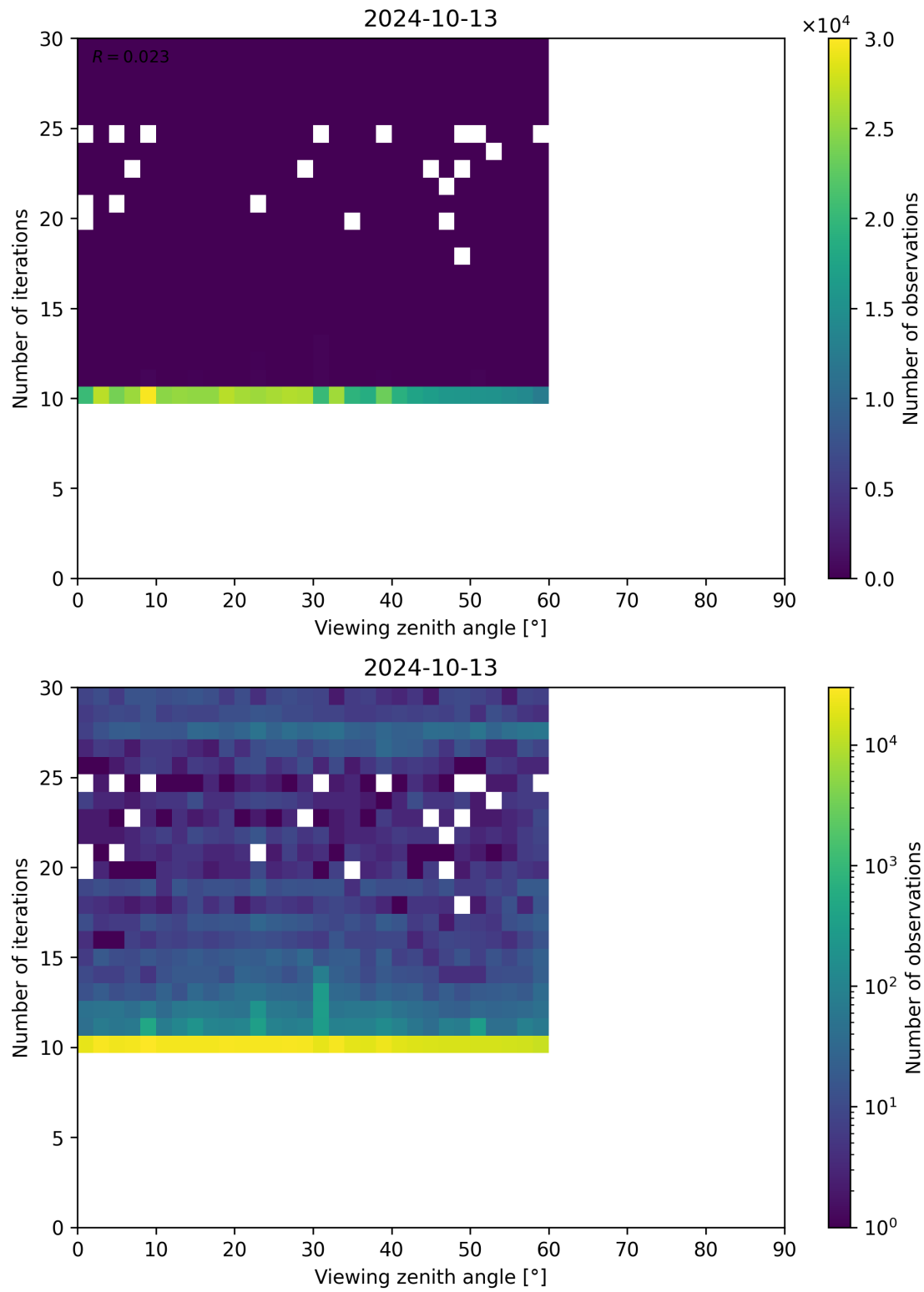
Figure 113: Scatter density plot of “Viewing zenith angle” against “Number of iterations” for 2024-10-12 to 2024-10-14.
