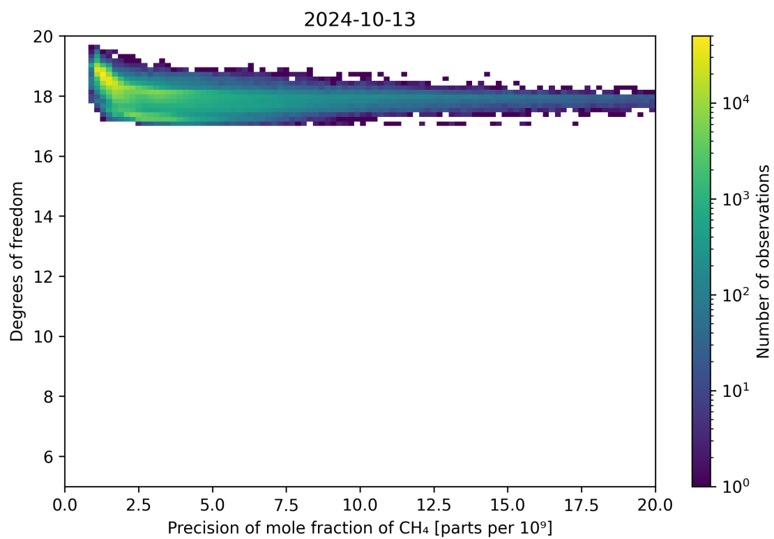
Figure 80: Scatter density plot of “Precision of mole fraction of CH 4 ” against “Degrees of freedom” for 2024-10-12 to 2024-10-14.
