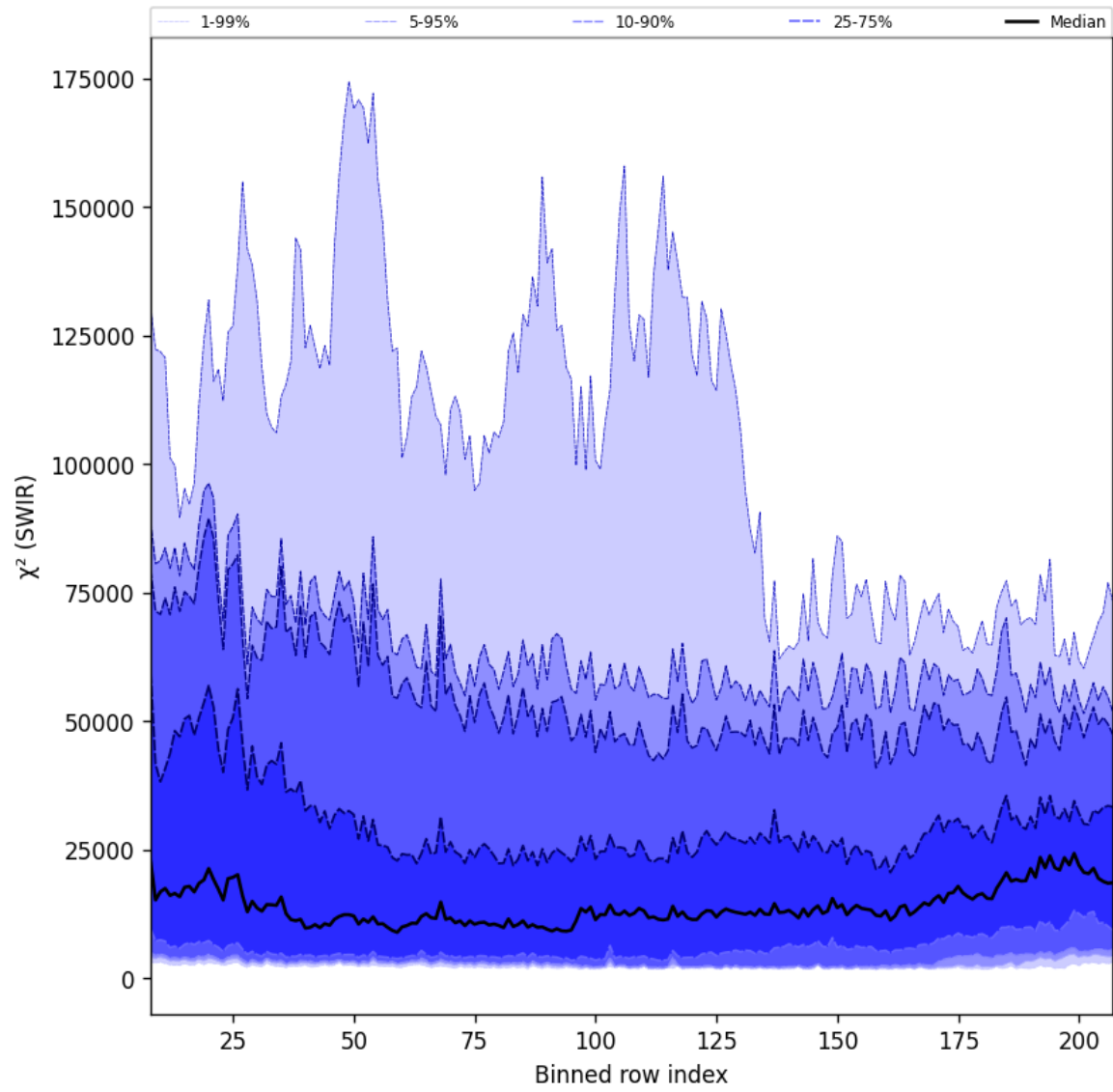
Figure 39: Along track statistics of “ \chi^2 (SWIR)” for 2024-10-12 to 2024-10-14
