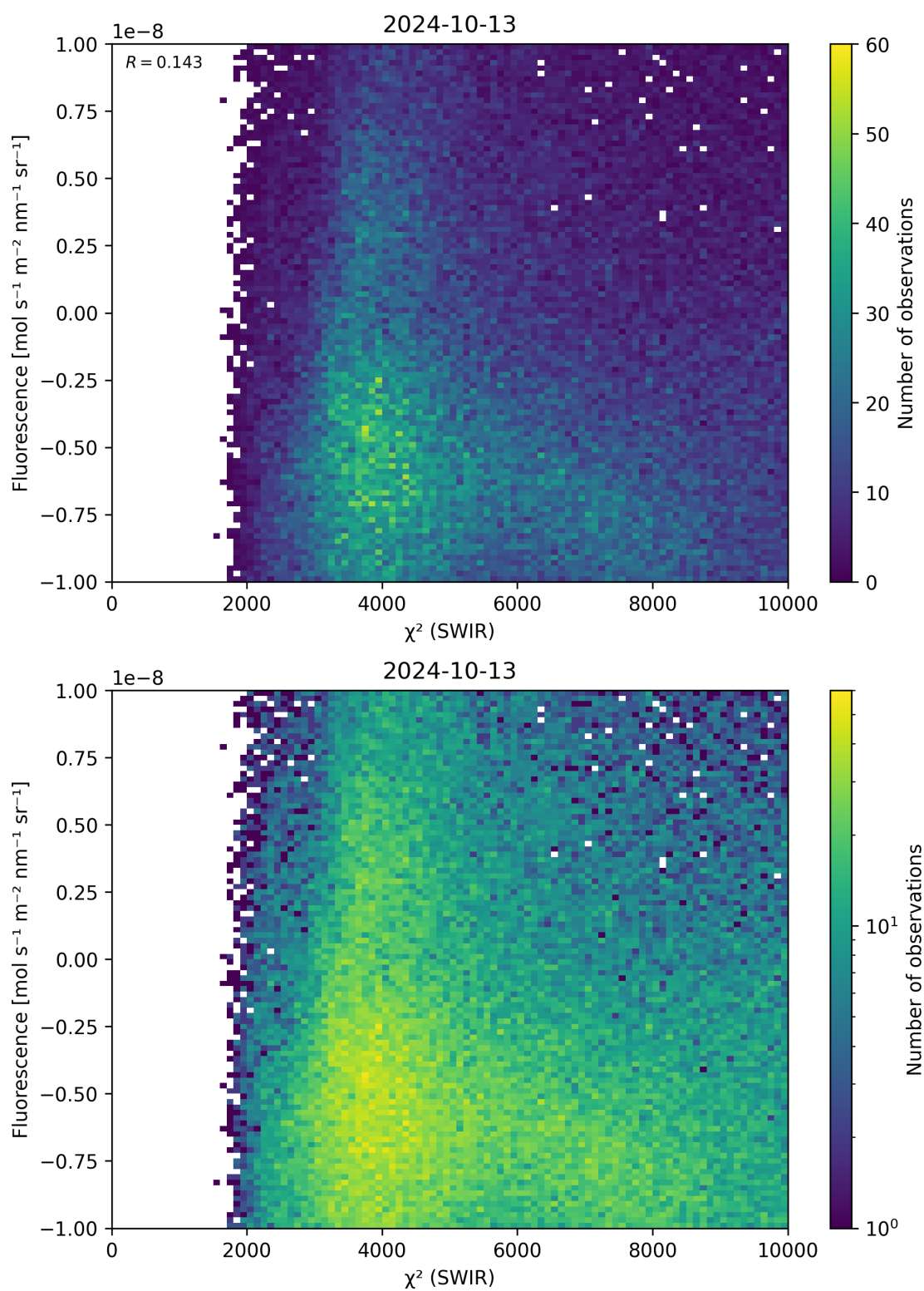
Figure 49: Scatter density plot of “ \chi^2 (SWIR)” against “Fluorescence” for 2024-10-12 to 2024-10-14.
