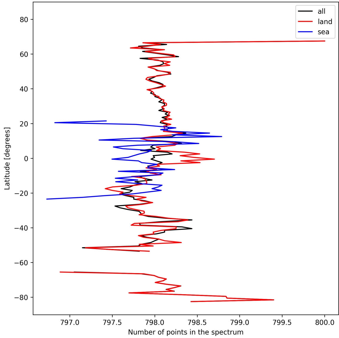
Figure 15: Zonal average of “Number of points in the spectrum” for 2024-10-12 to 2024-10-14.
