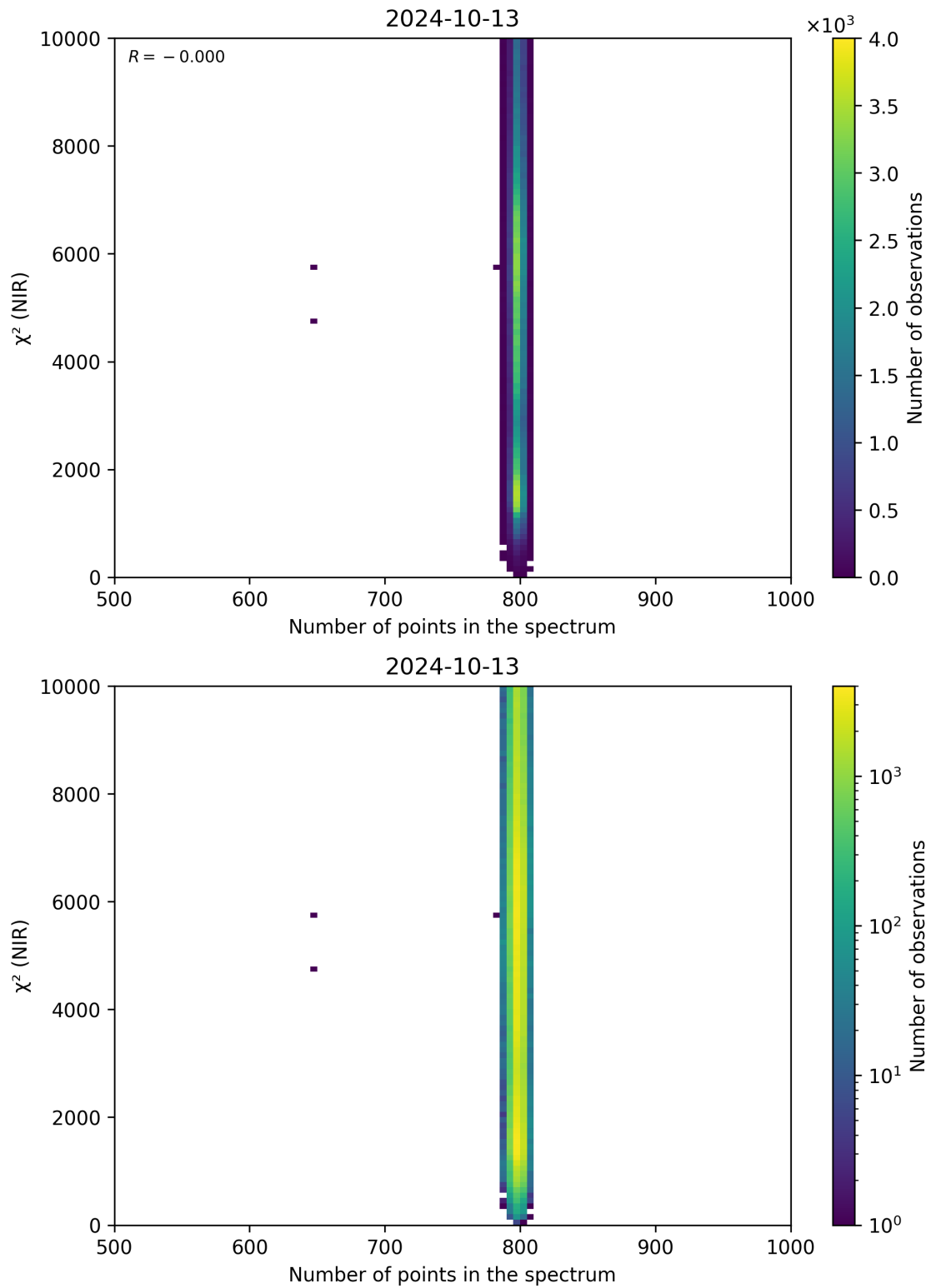
Figure 88: Scatter density plot of “Number of points in the spectrum” against “ \chi^2 (NIR)” for 2024-10-12 to 2024-10-14.
