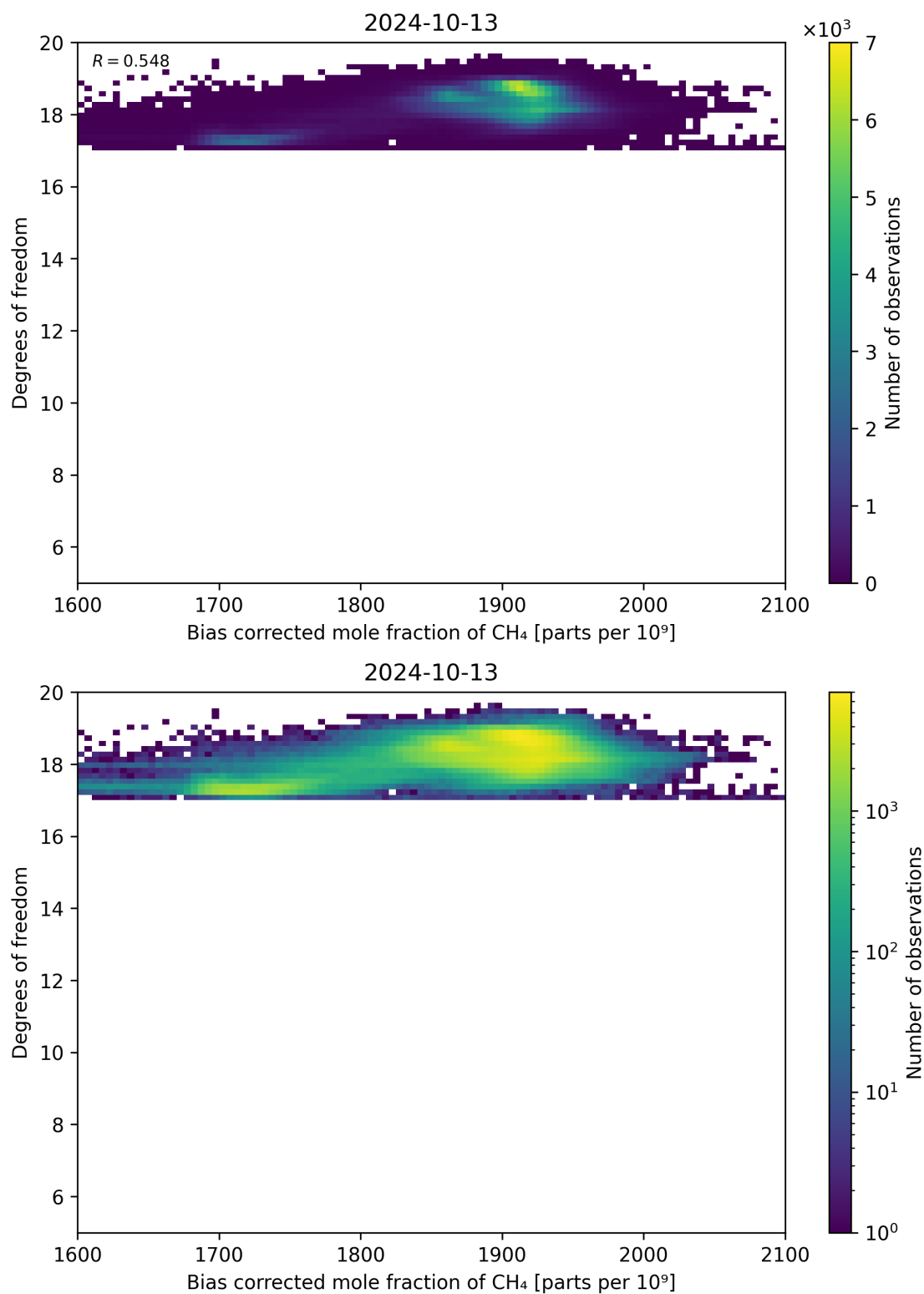
Figure 65: Scatter density plot of “Bias corrected mole fraction of CH 4 ” against “Degrees of freedom” for 2024-10-12 to 2024-10-14.
