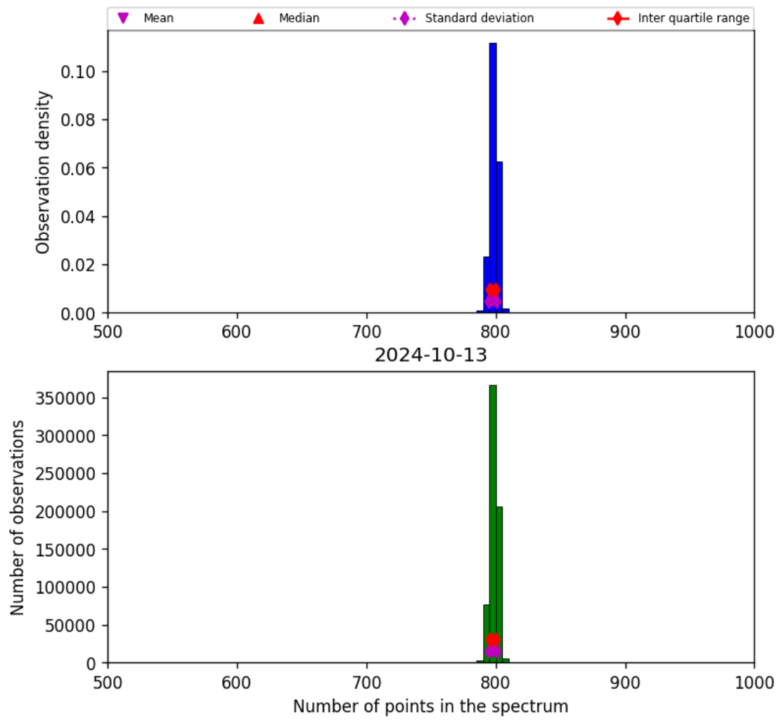
Figure 26: Histogram of “Number of points in the spectrum” for 2024-10-12 to 2024-10-14
