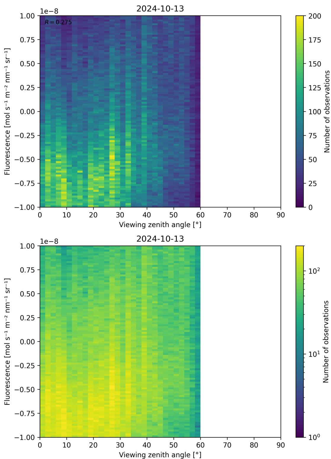
Figure 108: Scatter density plot of “Viewing zenith angle” against “Fluorescence” for 2024-10-12 to 2024-10-14.
