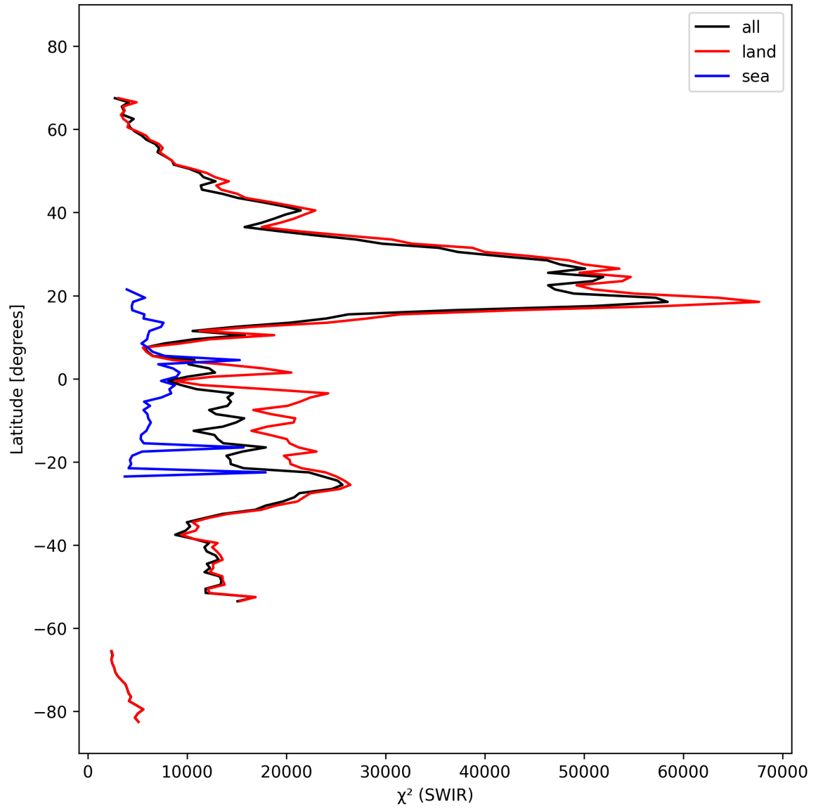
Figure 17: Zonal average of “ \chi^2 (SWIR)” for 2024-10-12 to 2024-10-14.
