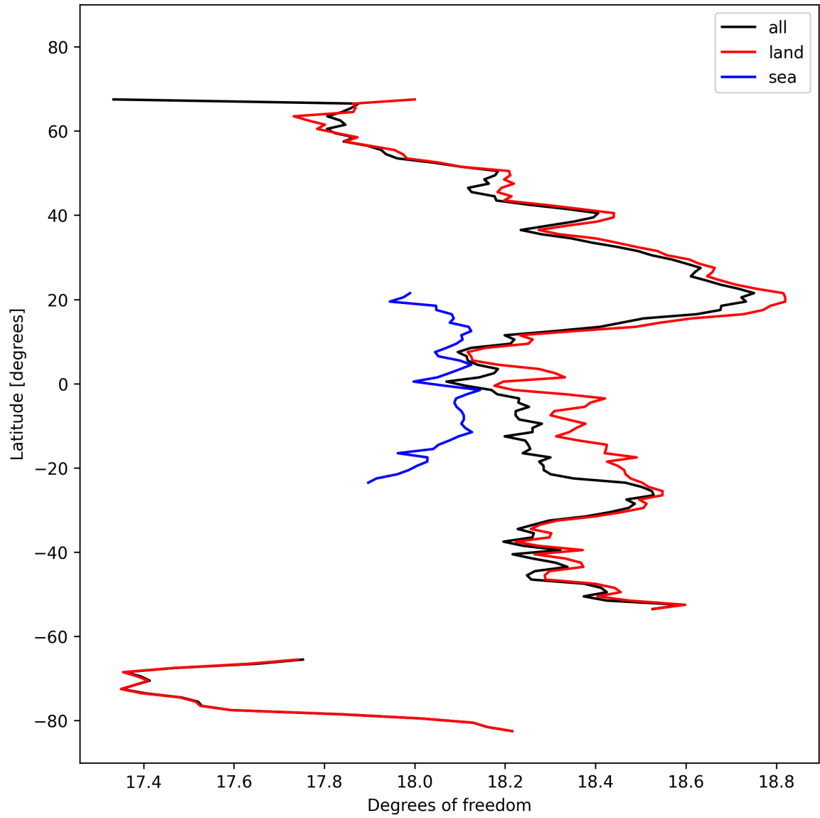
Figure 19: Zonal average of “Degrees of freedom” for 2024-10-12 to 2024-10-14.
