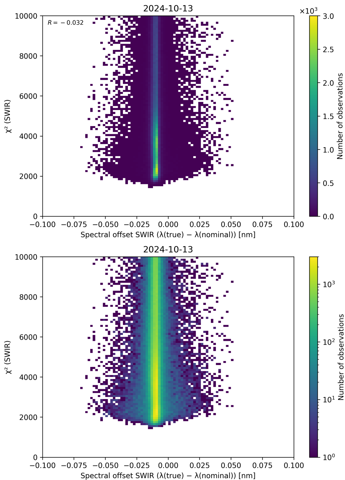
Figure 118: Scatter density plot of “Spectral offset SWIR ( \lambda_{\text{true}} - \lambda_{\text{nominal}} )” against “ \chi^2 (SWIR)” for 2024-10-12 to 2024-10-14.
