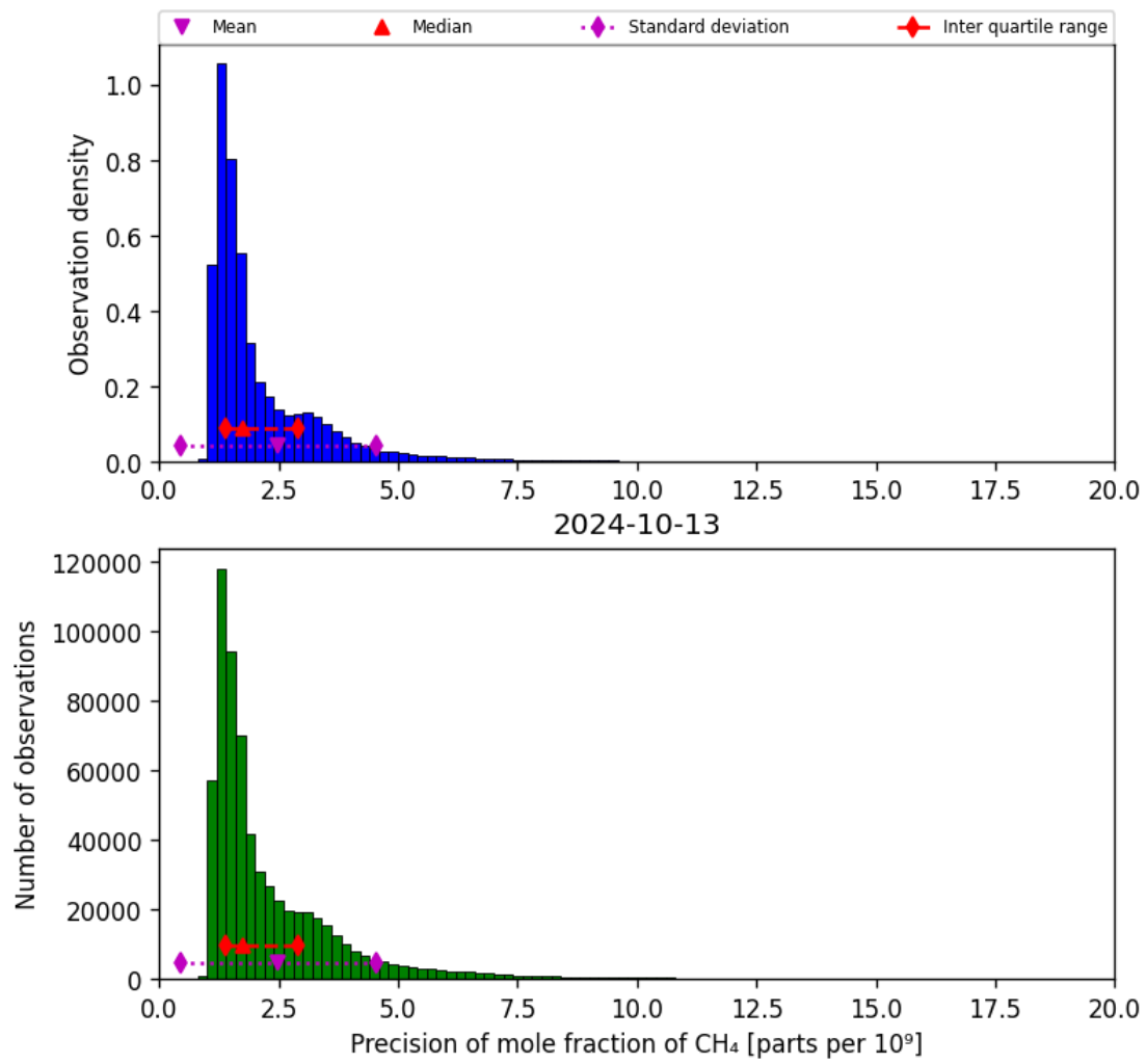
Figure 24: Histogram of “Precision of mole fraction of CH 4 ” for 2024-10-12 to 2024-10-14
