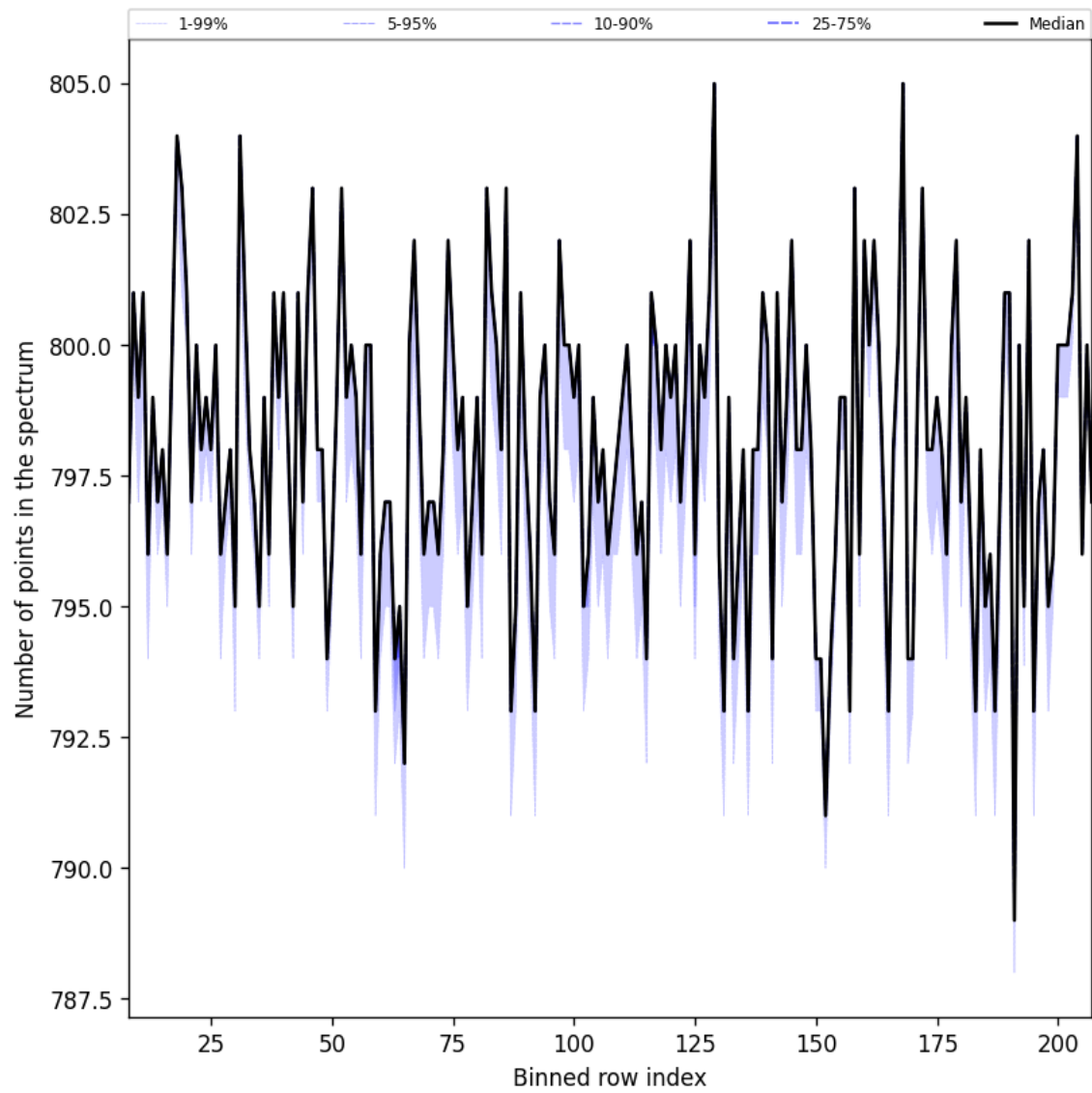
Figure 37: Along track statistics of “Number of points in the spectrum” for 2024-10-12 to 2024-10-14
