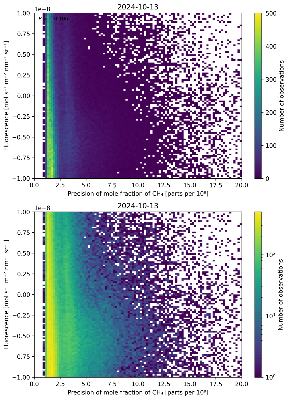
Figure 81: Scatter density plot of “Precision of mole fraction of \text{CH}_4 ” against “Fluorescence” for 2024-10-12 to 2024-10-14.
