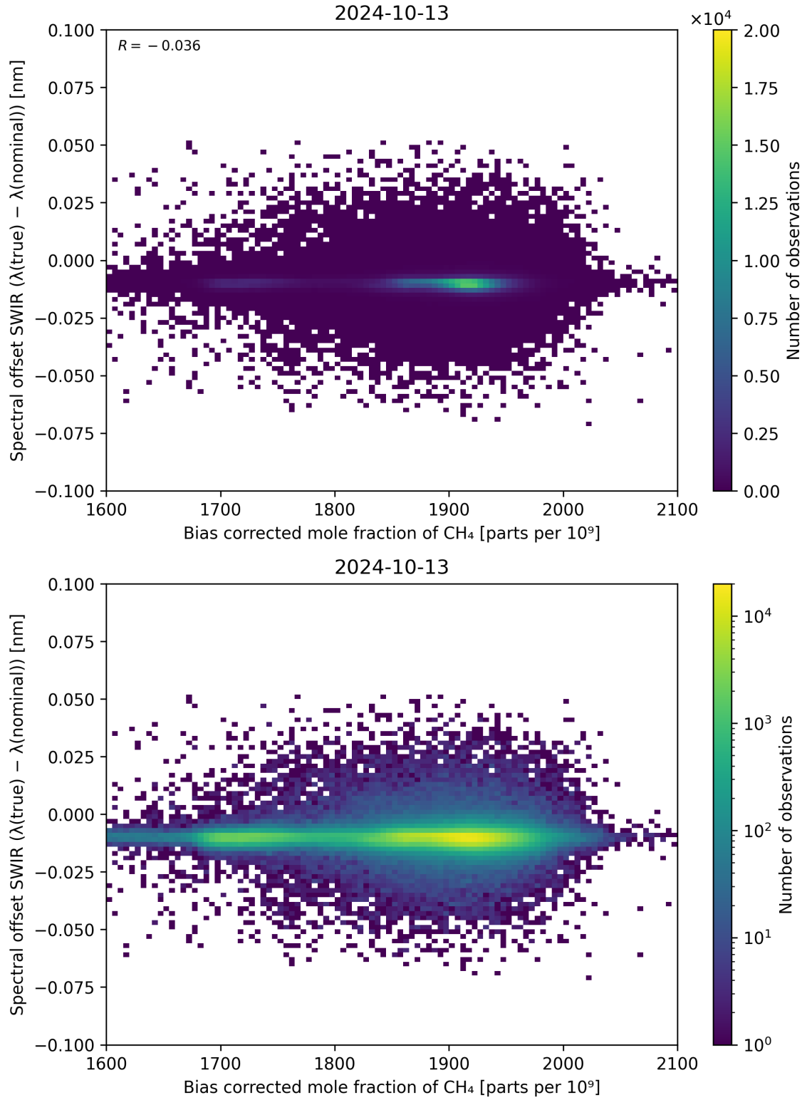
Figure 69: Scatter density plot of “Bias corrected mole fraction of CH 4 ” against “Spectral offset SWIR ( \lambda_{\text{true}} - \lambda_{\text{nominal}} )” for 2024-10-12 to 2024-10-14.
