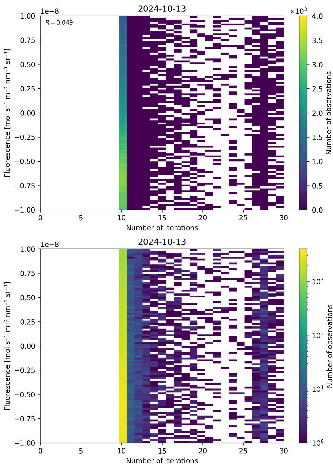
Figure 87: Scatter density plot of “Number of iterations” against “Fluorescence” for 2024-10-12 to 2024-10-14.
