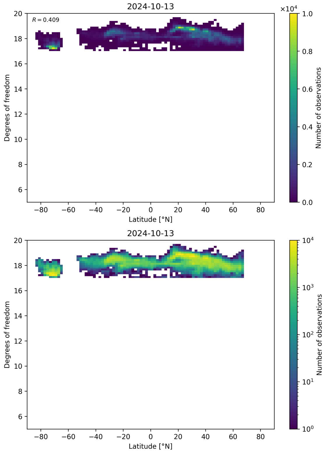
Figure 55: Scatter density plot of “Latitude” against “Degrees of freedom” for 2024-10-12 to 2024-10-14.
