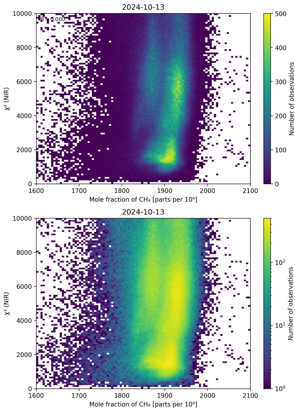
Figure 70: Scatter density plot of “Mole fraction of \text{CH}_4 ” against “ \chi^2 (NIR)” for 2024-10-12 to 2024-10-14.
