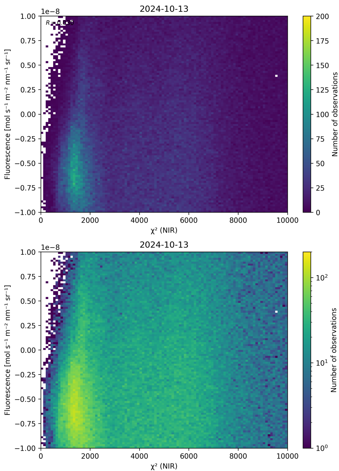
Figure 45: Scatter density plot of “ \chi^2 (NIR)” against “Fluorescence” for 2024-10-12 to 2024-10-14.
