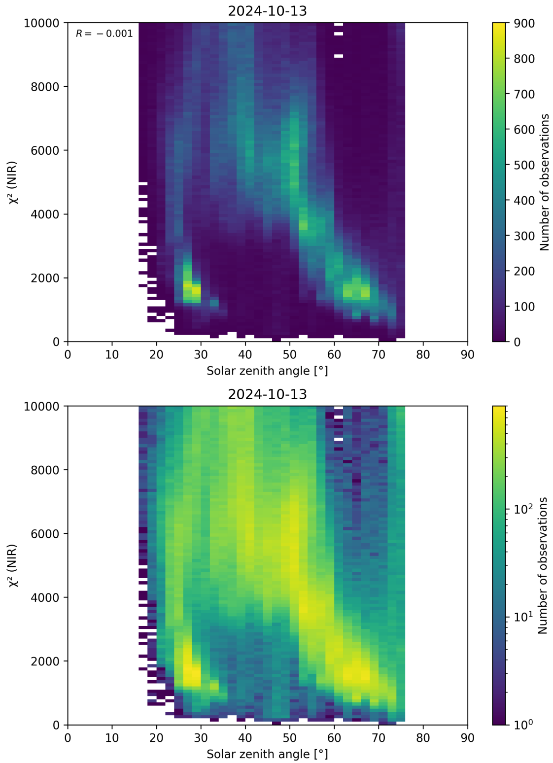
Figure 94: Scatter density plot of “Solar zenith angle” against “ \chi^2 (NIR)” for 2024-10-12 to 2024-10-14.
