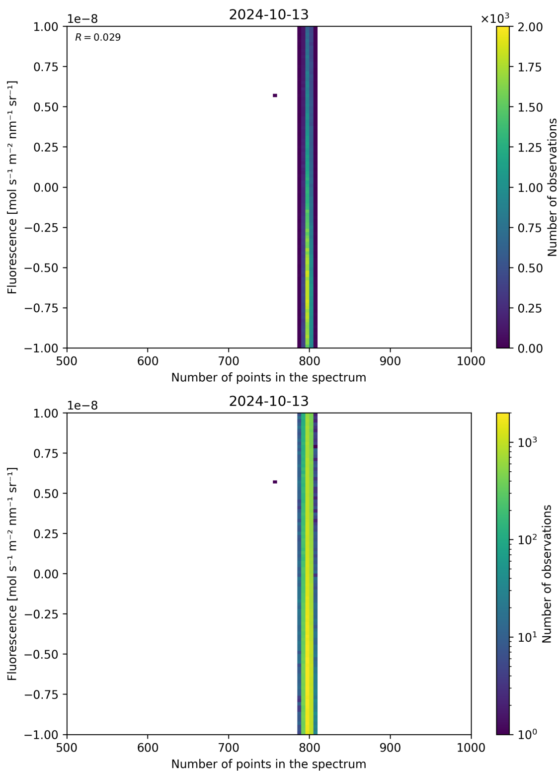
Figure 91: Scatter density plot of “Number of points in the spectrum” against “Fluorescence” for 2024-10-12 to 2024-10-14.
