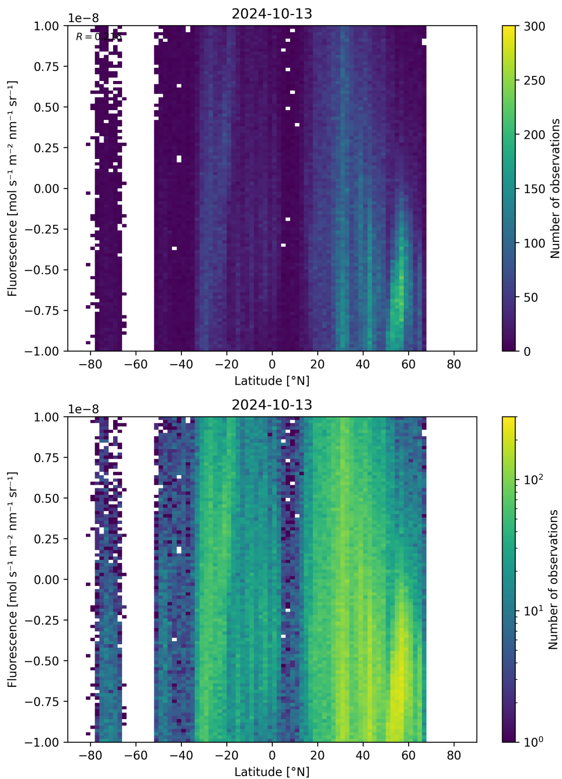
Figure 56: Scatter density plot of “Latitude” against “Fluorescence” for 2024-10-12 to 2024-10-14.
