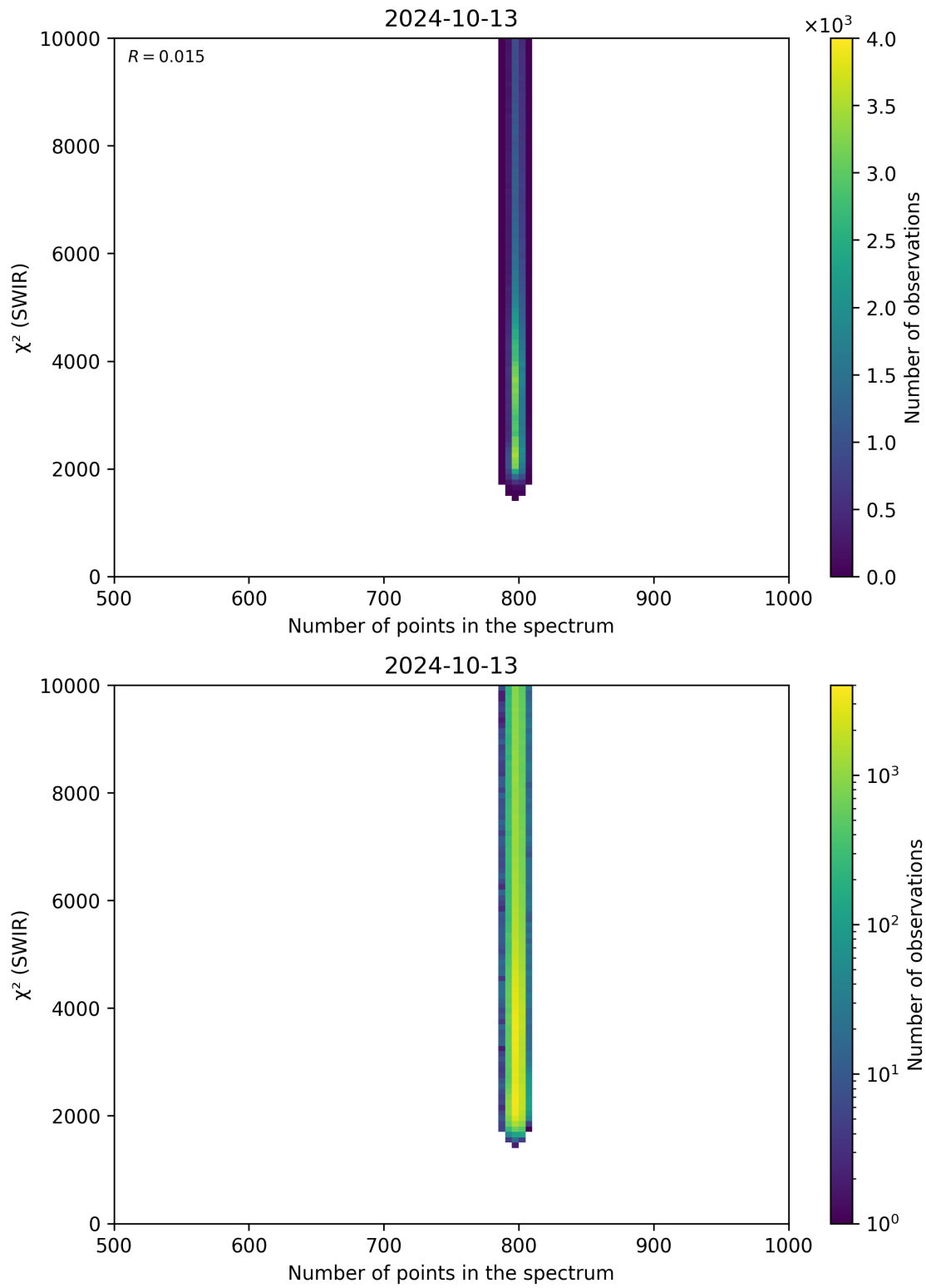
Figure 89: Scatter density plot of “Number of points in the spectrum” against “ \chi^2 (SWIR)” for 2024-10-12 to 2024-10-14.
