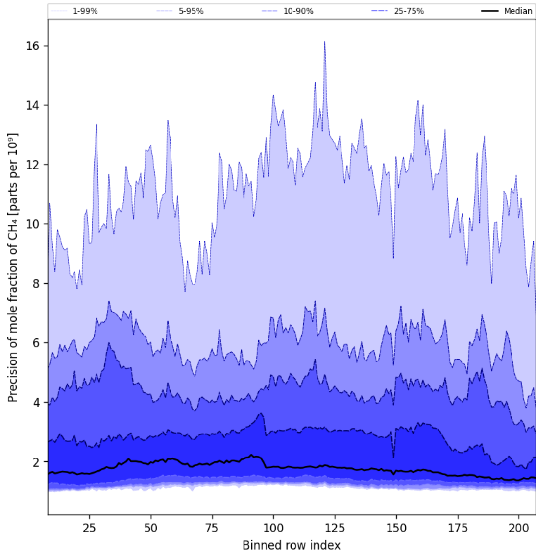
Figure 35: Along track statistics of “Precision of mole fraction of CH 4 ” for 2024-10-12 to 2024-10-14
