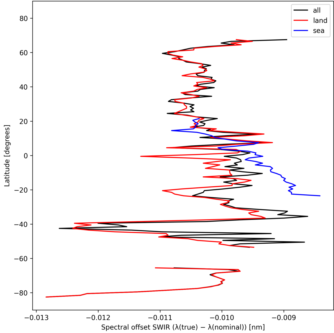
Figure 16: Zonal average of “Spectral offset SWIR ( \lambda_{\text{true}} - \lambda_{\text{nominal}} )” for 2024-10-12 to 2024-10-14.
