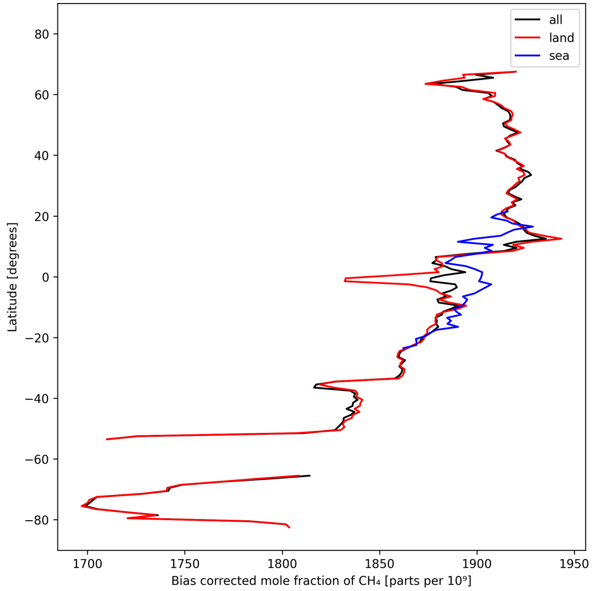
Figure 14: Zonal average of “Bias corrected mole fraction of CH 4 ” for 2024-10-12 to 2024-10-14.
