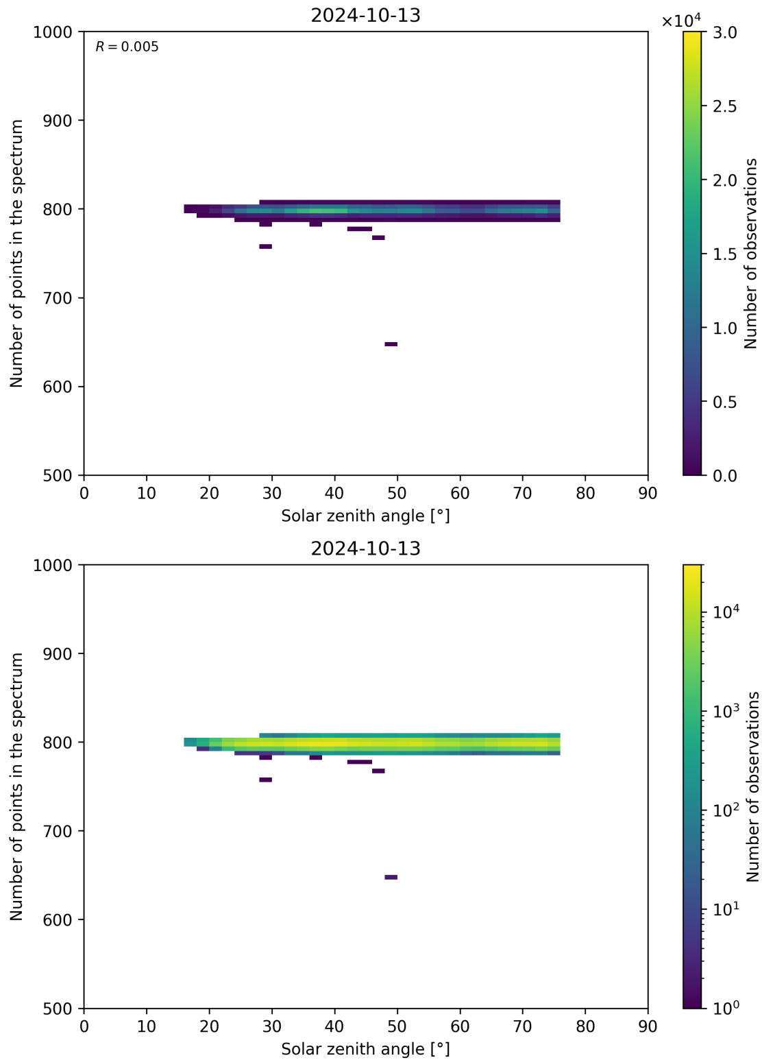
Figure 103: Scatter density plot of “Solar zenith angle” against “Number of points in the spectrum” for 2024-10-12 to 2024-10-14.
