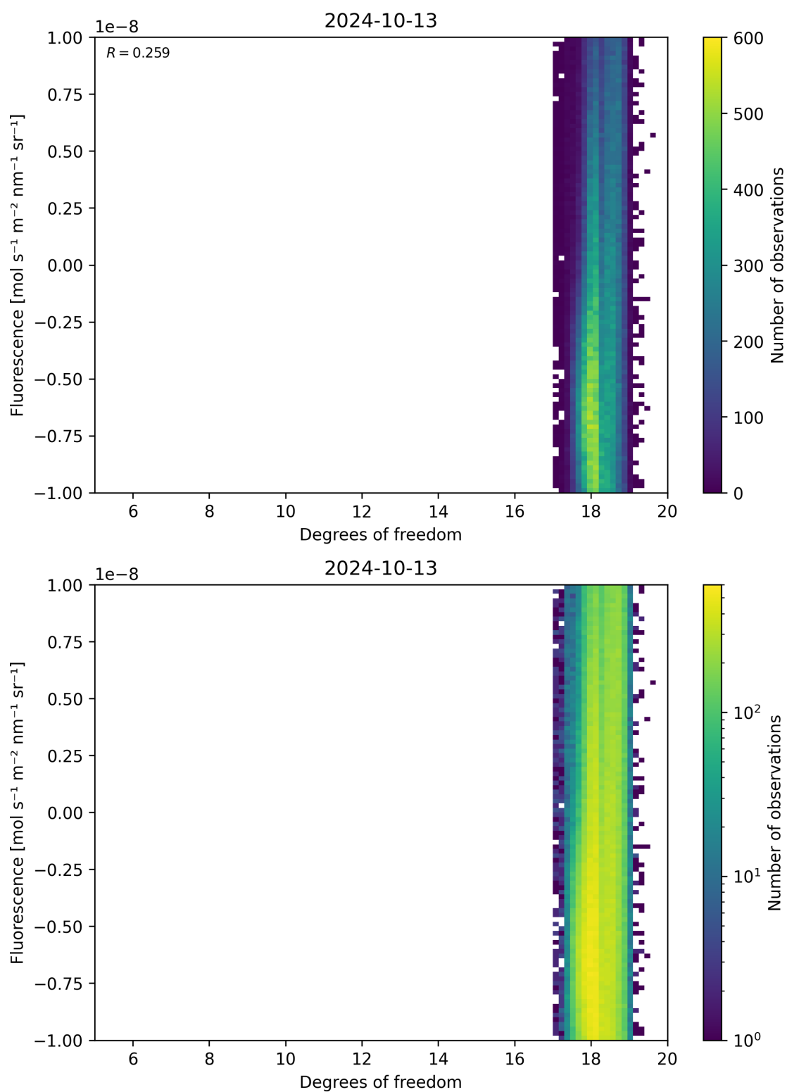
Figure 51: Scatter density plot of “Degrees of freedom” against “Fluorescence” for 2024-10-12 to 2024-10-14.
