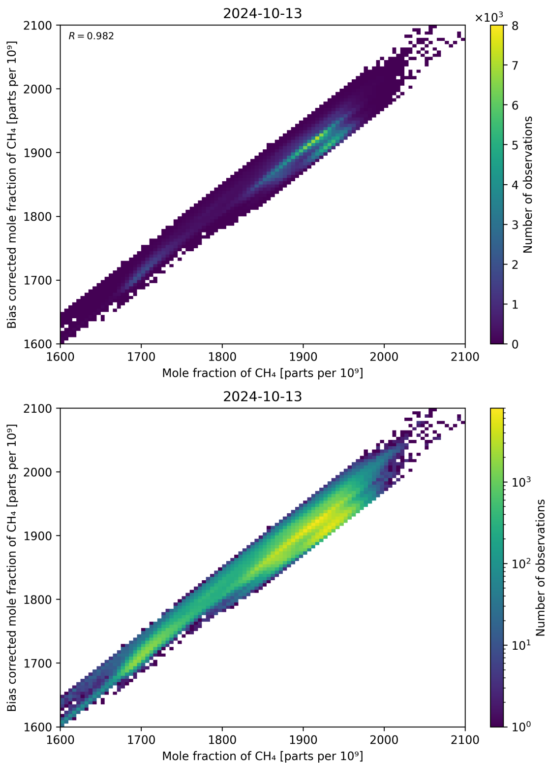
Figure 74: Scatter density plot of “Mole fraction of CH 4 ” against “Bias corrected mole fraction of CH 4 ” for 2024-10-12 to 2024-10-14.
