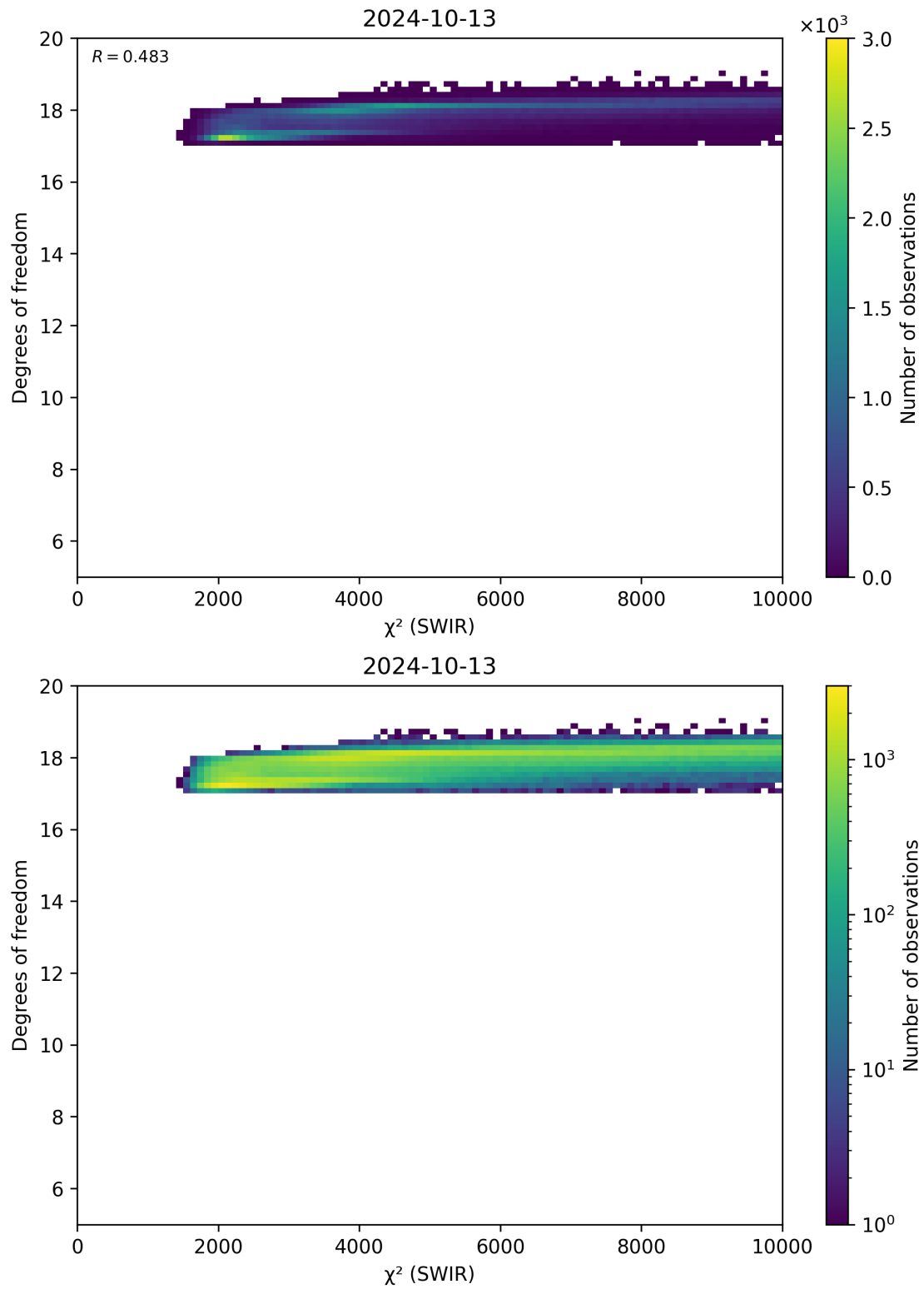
Figure 48: Scatter density plot of “ \chi^2 (SWIR)” against “Degrees of freedom” for 2024-10-12 to 2024-10-14.
