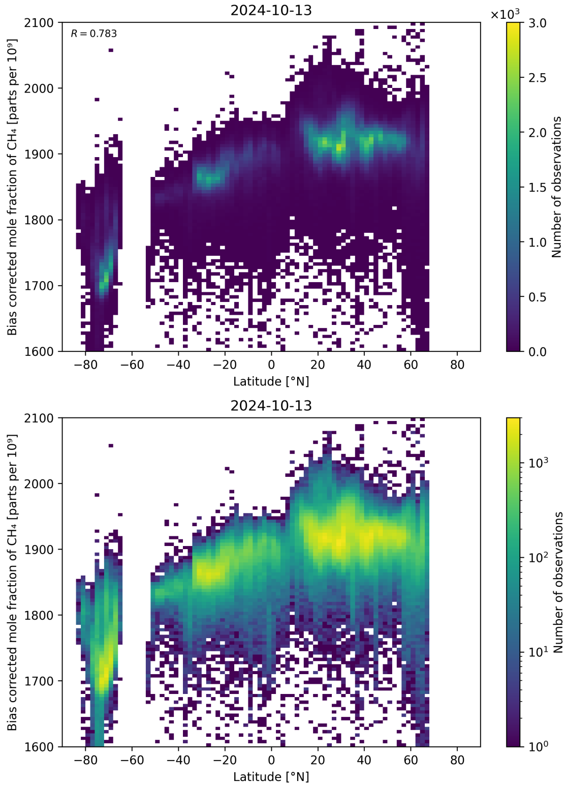
Figure 58: Scatter density plot of “Latitude” against “Bias corrected mole fraction of \text{CH}_4 ” for 2024-10-12 to 2024-10-14.
