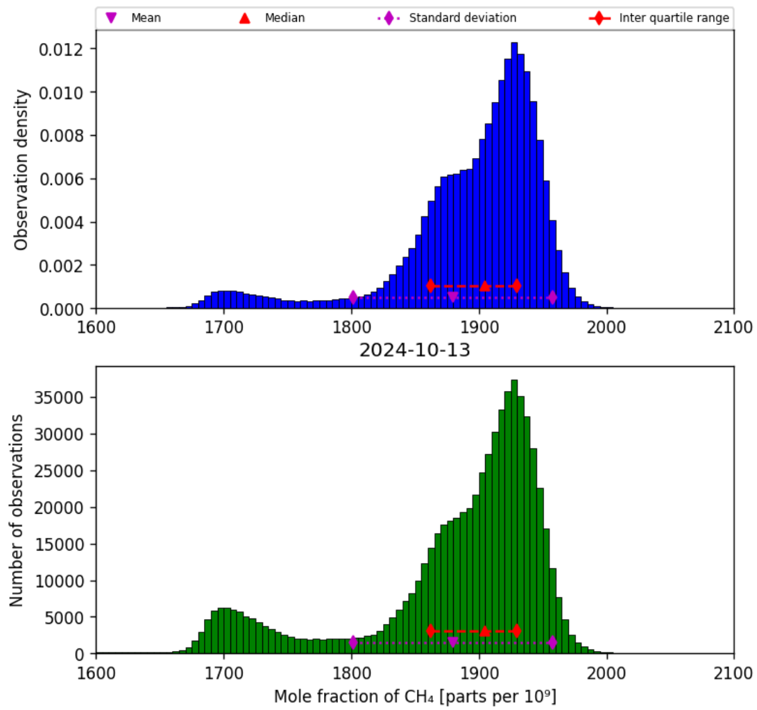
Figure 23: Histogram of “Mole fraction of CH 4 ” for 2024-10-12 to 2024-10-14
