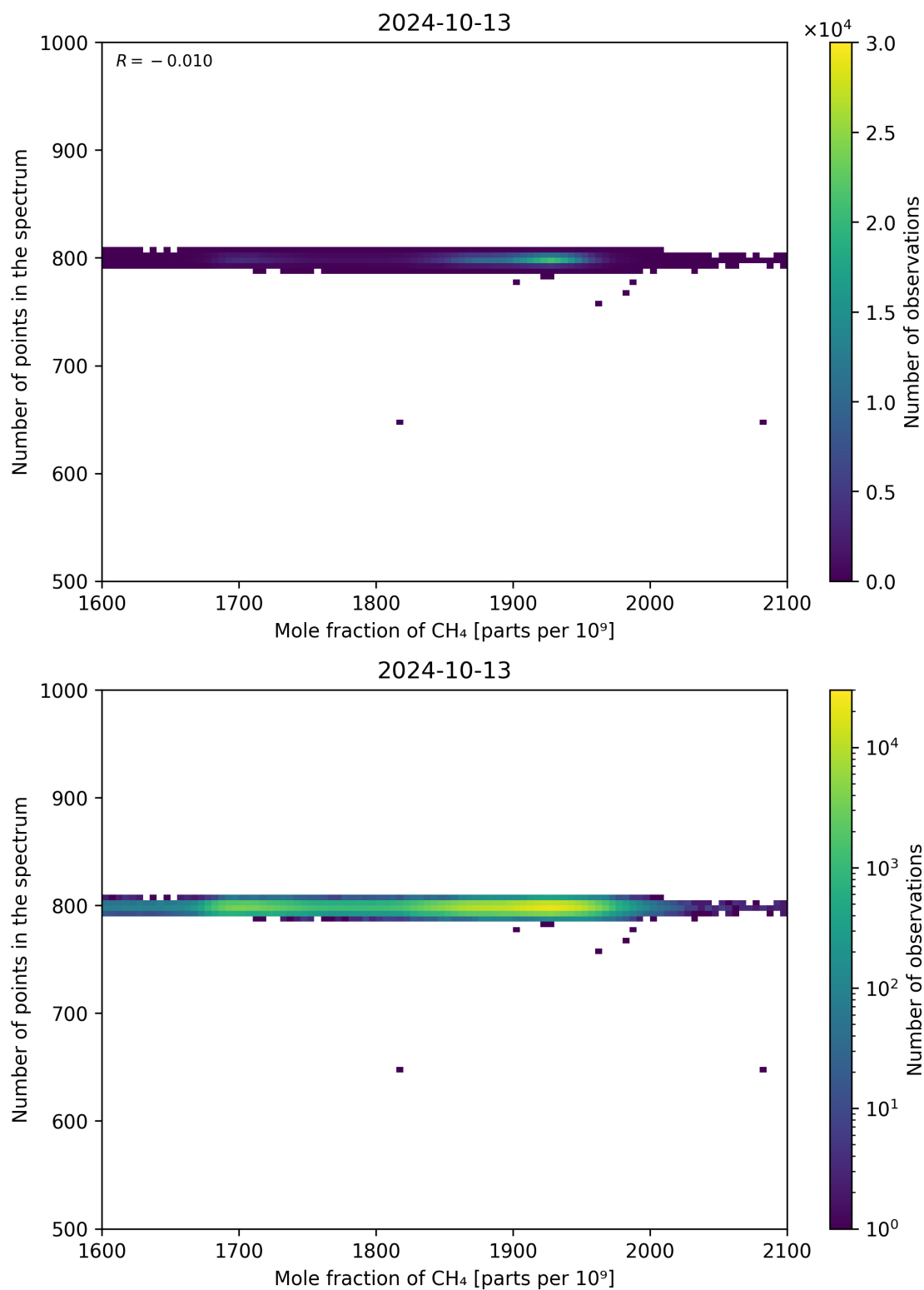
Figure 77: Scatter density plot of “Mole fraction of CH 4 ” against “Number of points in the spectrum” for 2024-10-12 to 2024-10-14.
