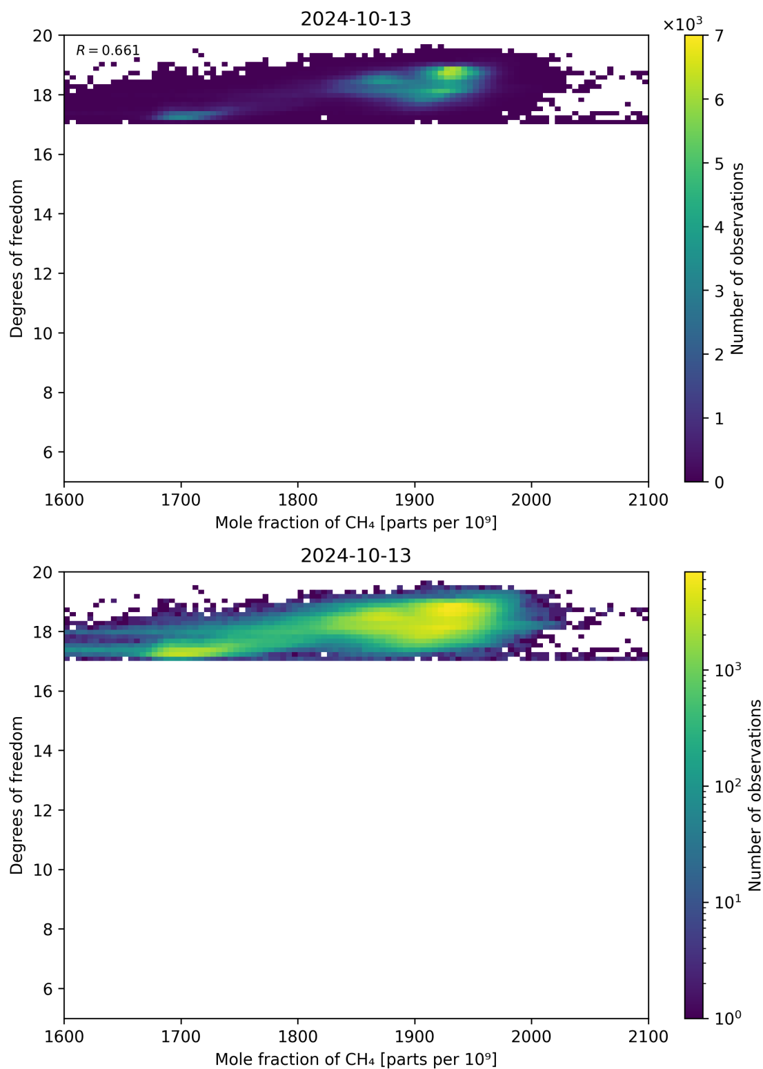
Figure 72: Scatter density plot of “Mole fraction of CH 4 ” against “Degrees of freedom” for 2024-10-12 to 2024-10-14.
