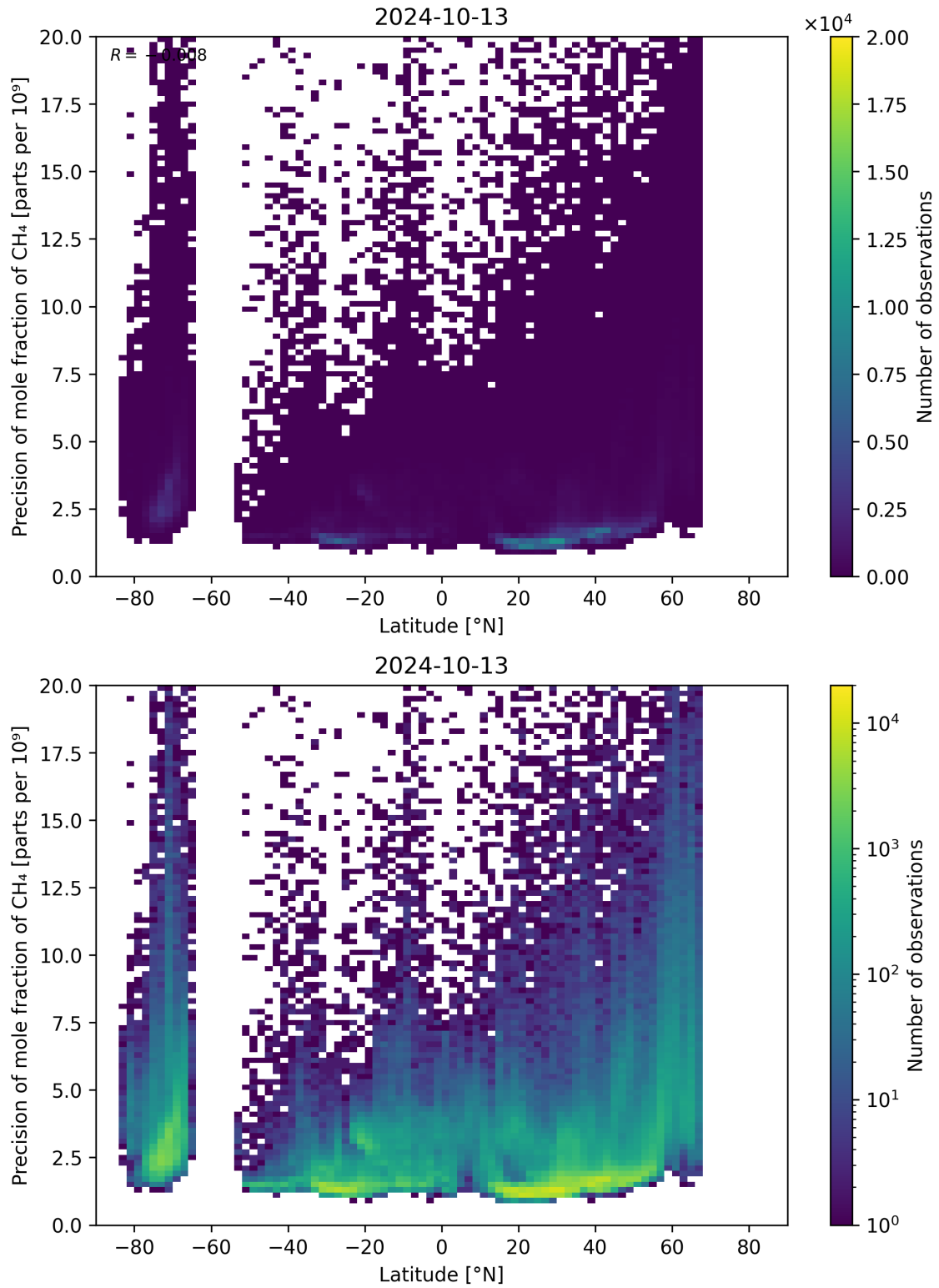
Figure 59: Scatter density plot of “Latitude” against “Precision of mole fraction of CH 4 ” for 2024-10-12 to 2024-10-14.
