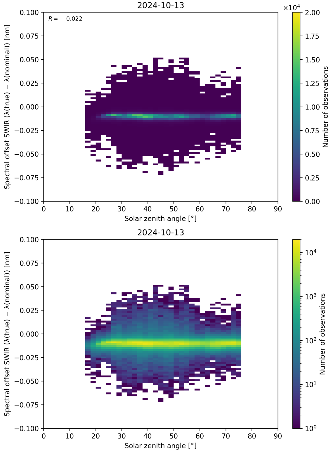
Figure 104: Scatter density plot of “Solar zenith angle” against “Spectral offset SWIR ( \lambda_{\text{true}} - \lambda_{\text{nominal}} )” for 2024-10-12 to 2024-10-14.
