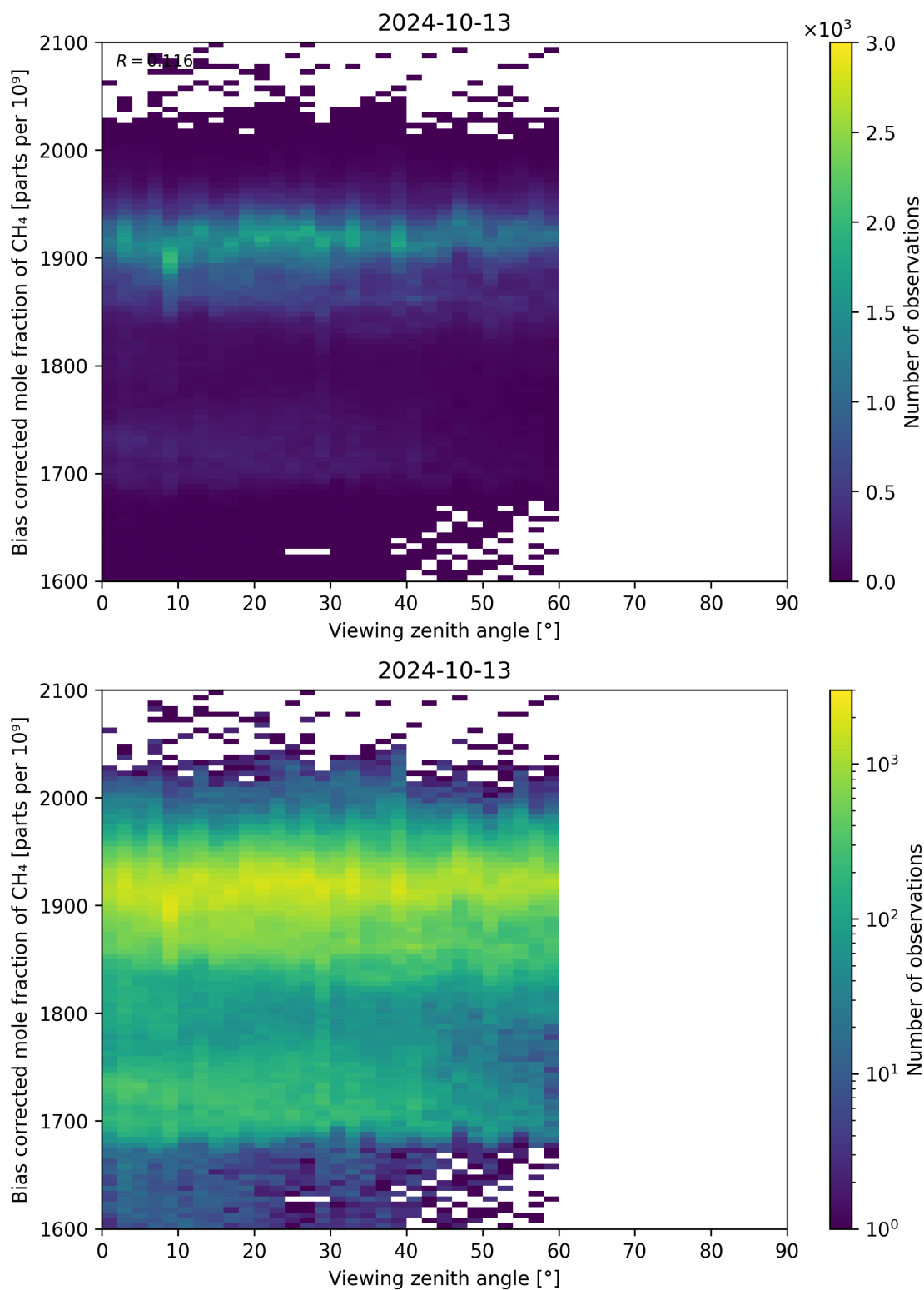
Figure 111: Scatter density plot of “Viewing zenith angle” against “Bias corrected mole fraction of CH 4 ” for 2024-10-12 to 2024-10-14.
