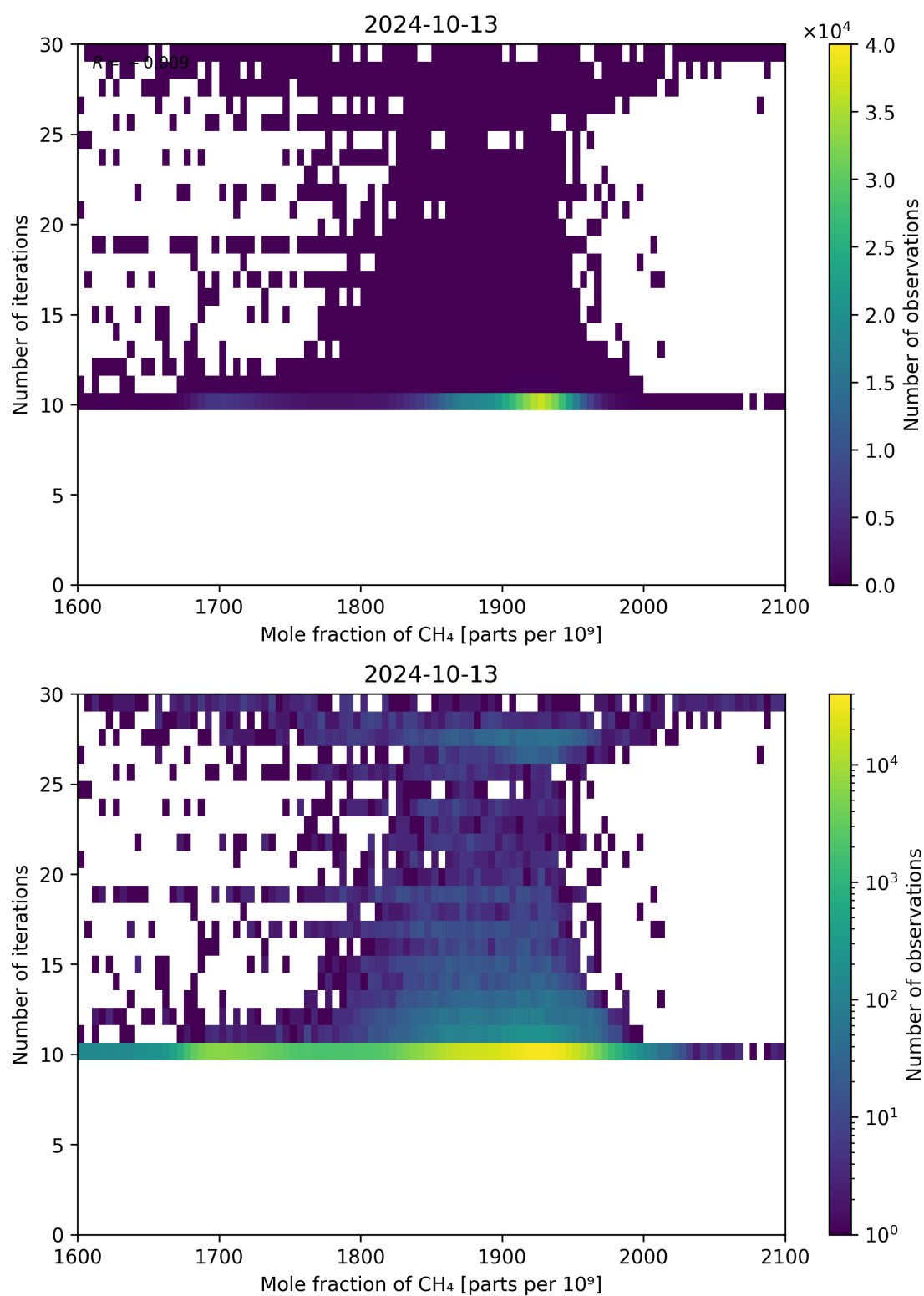
Figure 76: Scatter density plot of “Mole fraction of CH 4 ” against “Number of iterations” for 2024-10-12 to 2024-10-14.
