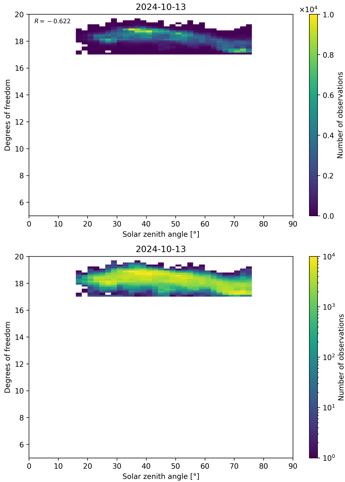
Figure 96: Scatter density plot of “Solar zenith angle” against “Degrees of freedom” for 2024-10-12 to 2024-10-14.
