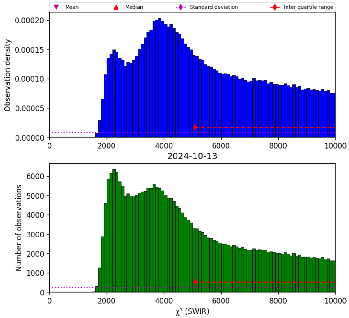
Figure 28: Histogram of “ \chi^2 (SWIR)” for 2024-10-12 to 2024-10-14
