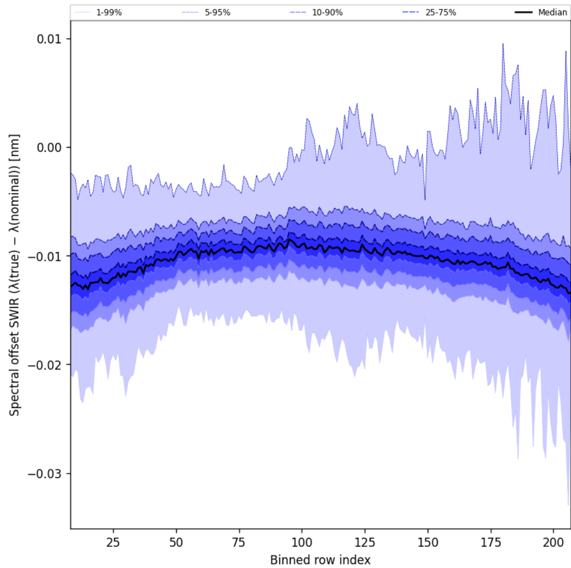
Figure 38: Along track statistics of “Spectral offset SWIR ( \lambda_{\text{true}} - \lambda_{\text{nominal}} )” for 2024-10-12 to 2024-10-14
