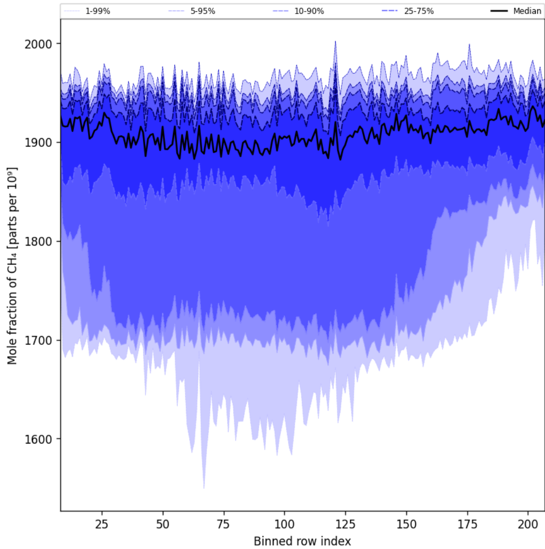
Figure 34: Along track statistics of “Mole fraction of CH 4 ” for 2024-10-12 to 2024-10-14
