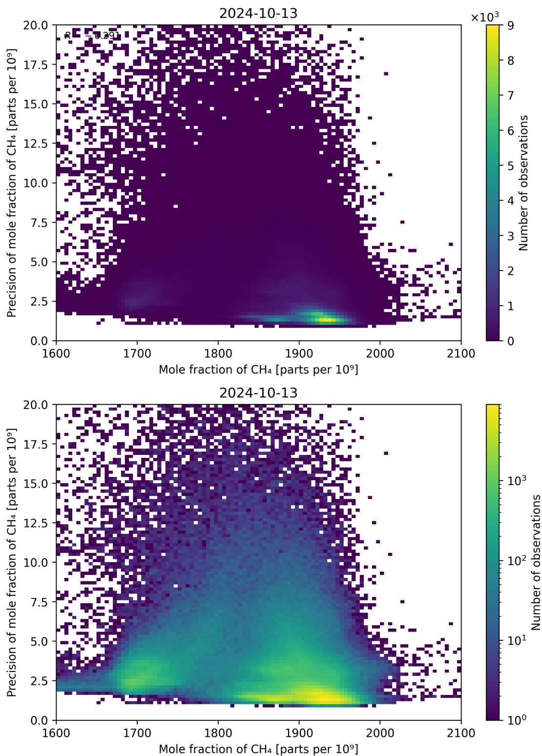
Figure 75: Scatter density plot of “Mole fraction of CH 4 ” against “Precision of mole fraction of CH 4 ” for 2024-10-12 to 2024-10-14.
