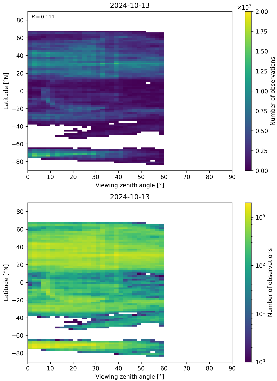
Figure 109: Scatter density plot of “Viewing zenith angle” against “Latitude” for 2024-10-12 to 2024-10-14.
