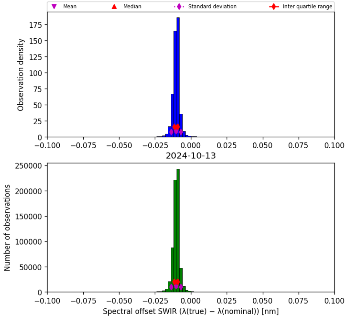
Figure 27: Histogram of “Spectral offset SWIR ( \lambda_{\text{true}} - \lambda_{\text{nominal}} )” for 2024-10-12 to 2024-10-14
