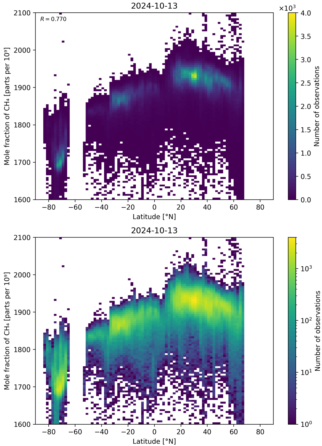
Figure 57: Scatter density plot of “Latitude” against “Mole fraction of \text{CH}_4 ” for 2024-10-12 to 2024-10-14.
