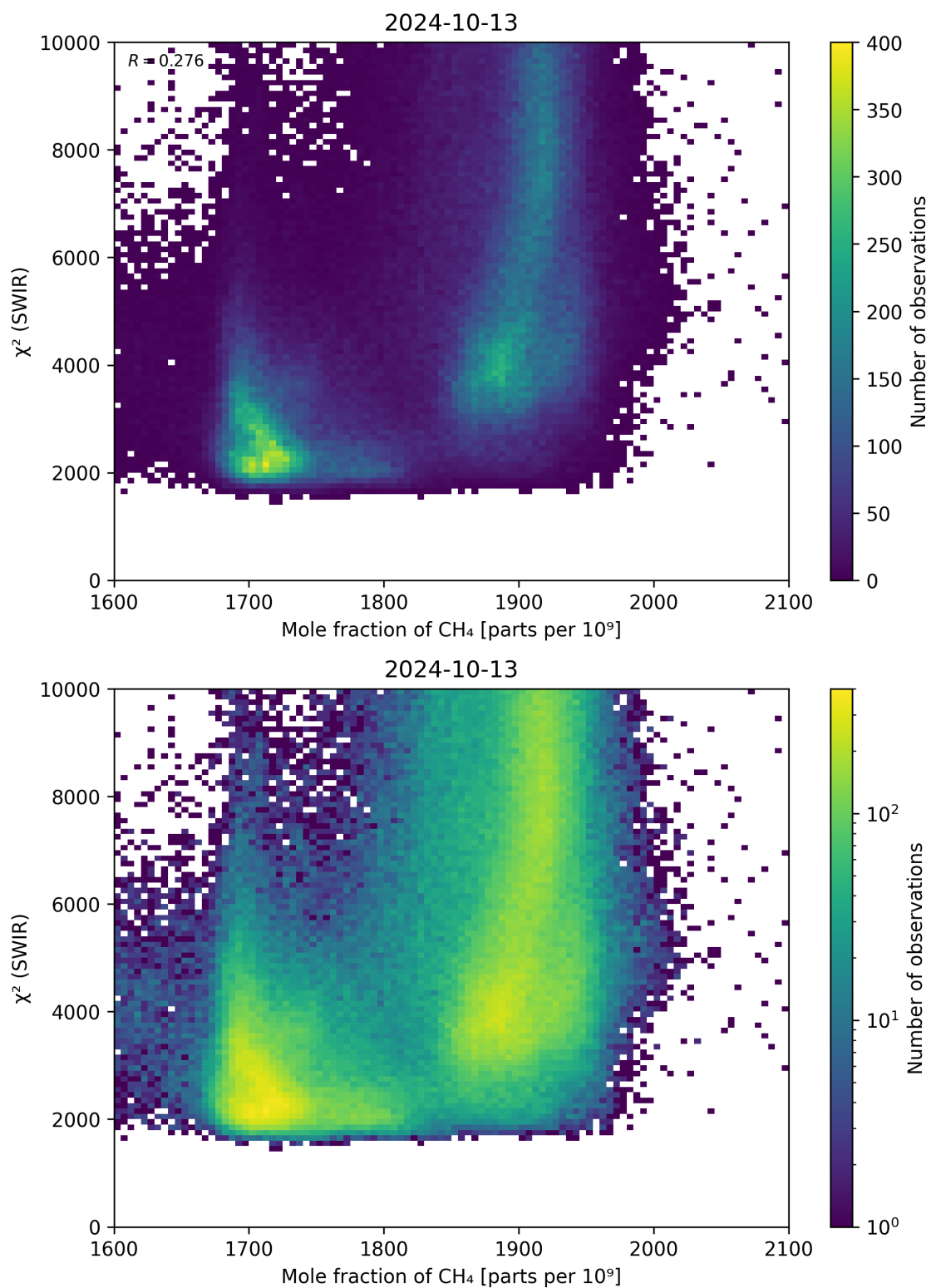
Figure 71: Scatter density plot of “Mole fraction of \text{CH}_4 ” against “ \chi^2 (SWIR)” for 2024-10-12 to 2024-10-14.
