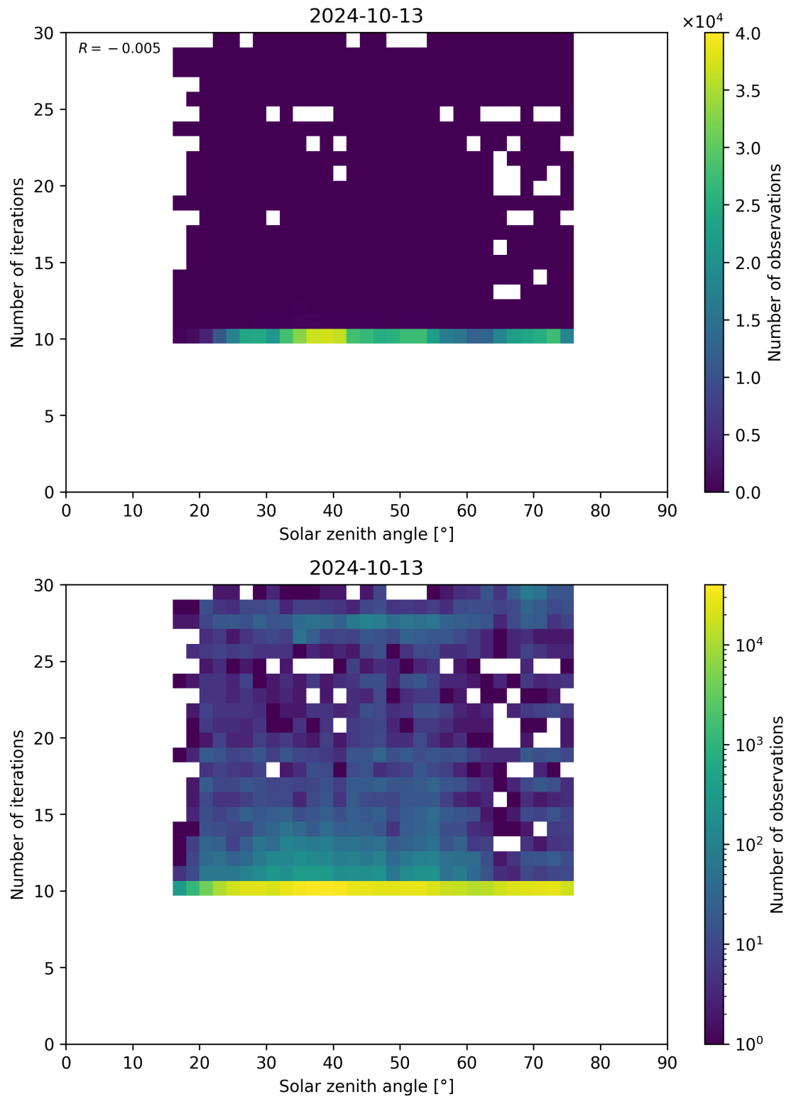
Figure 102: Scatter density plot of “Solar zenith angle” against “Number of iterations” for 2024-10-12 to 2024-10-14.
