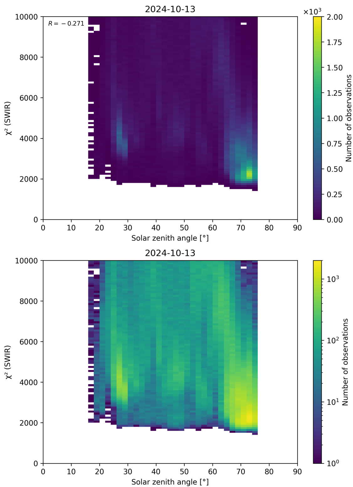
Figure 95: Scatter density plot of “Solar zenith angle” against “ \chi^2 (SWIR)” for 2024-10-12 to 2024-10-14.
