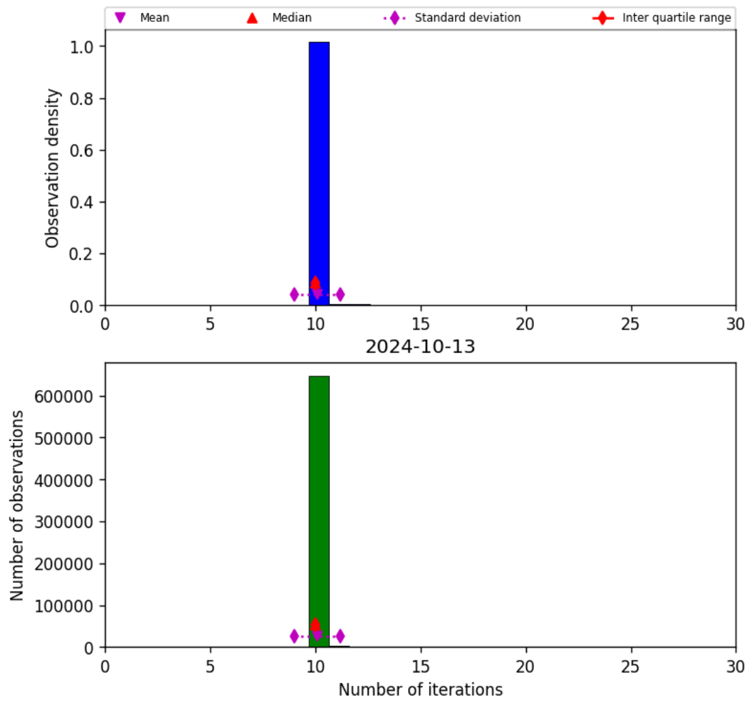
Figure 31: Histogram of “Number of iterations” for 2024-10-12 to 2024-10-14
