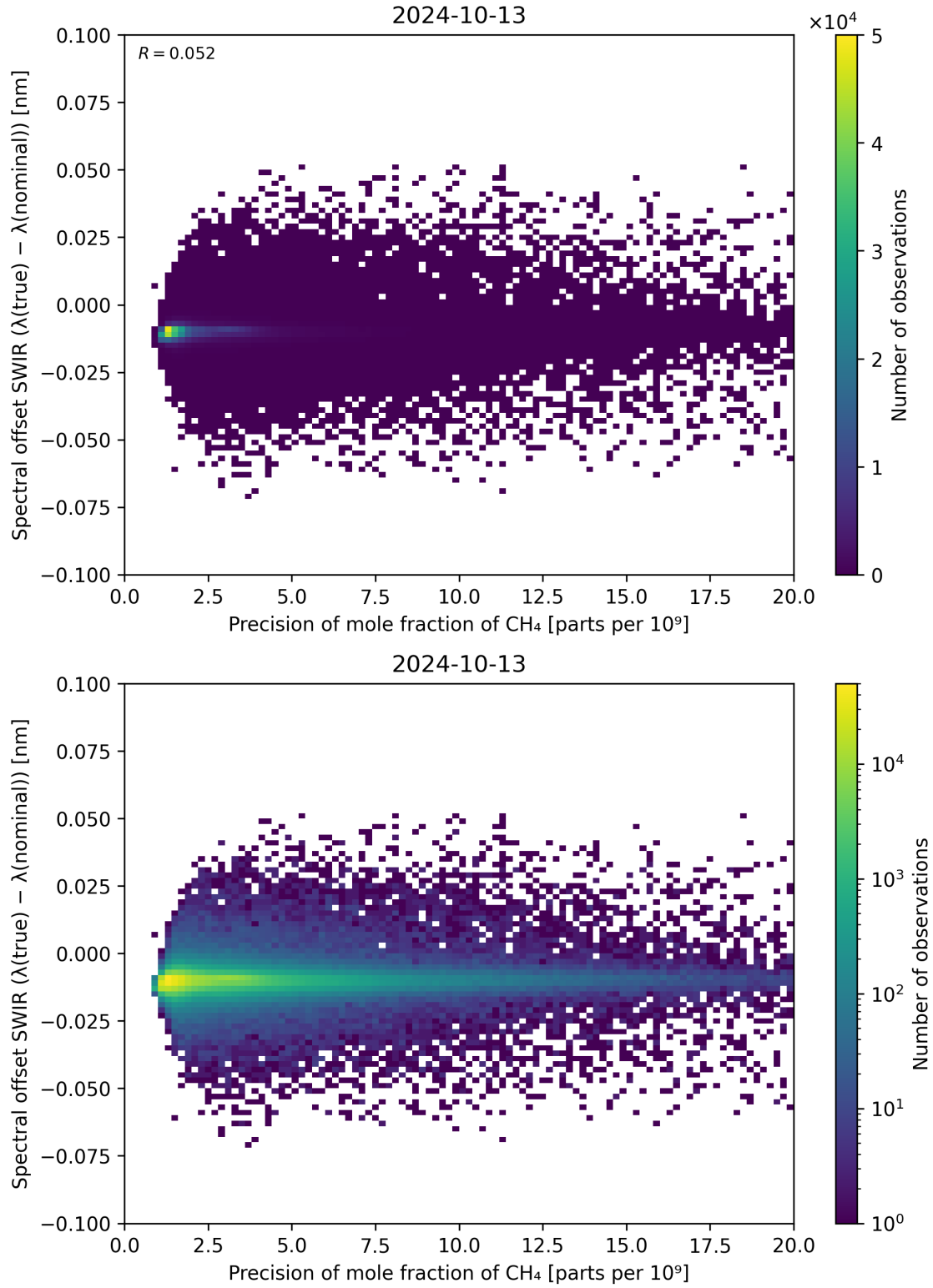
Figure 85: Scatter density plot of “Precision of mole fraction of \text{CH}_4 ” against “Spectral offset SWIR ( \lambda_{\text{true}} - \lambda_{\text{nominal}} )” for 2024-10-12 to 2024-10-14.
