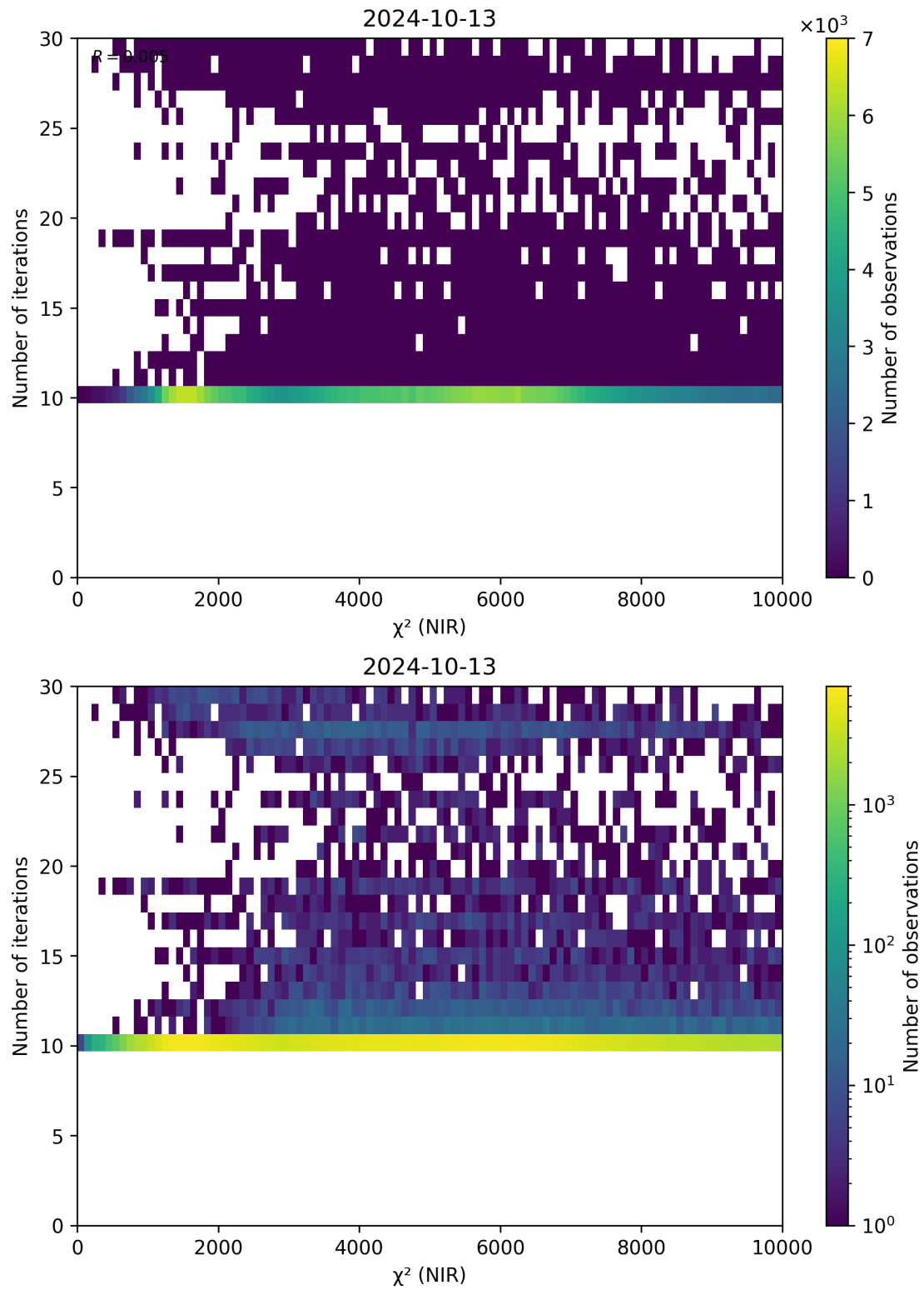
Figure 46: Scatter density plot of “ \chi^2 (NIR)” against “Number of iterations” for 2024-10-12 to 2024-10-14.
