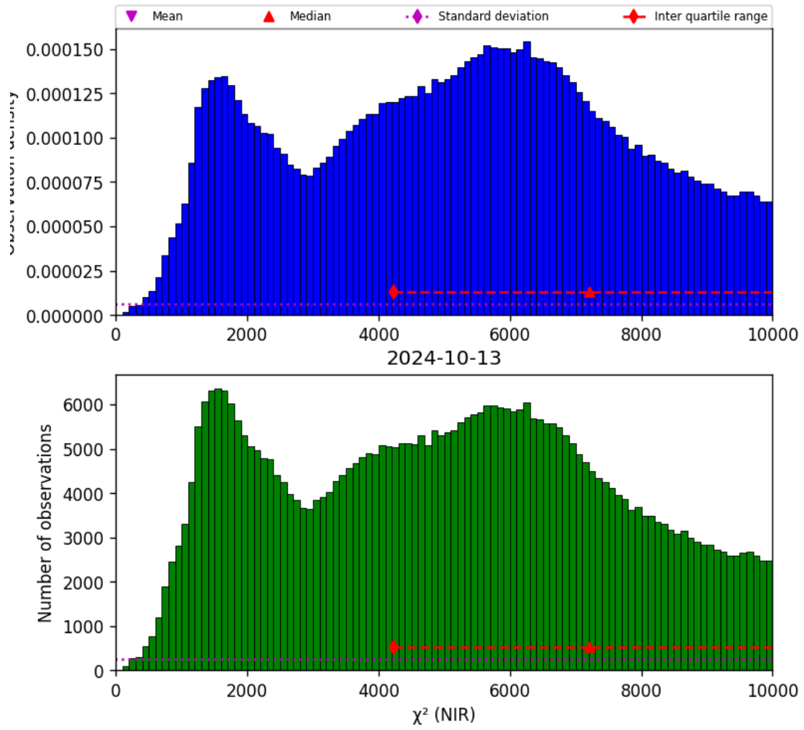
Figure 29: Histogram of “ \chi^2 (NIR)” for 2024-10-12 to 2024-10-14
