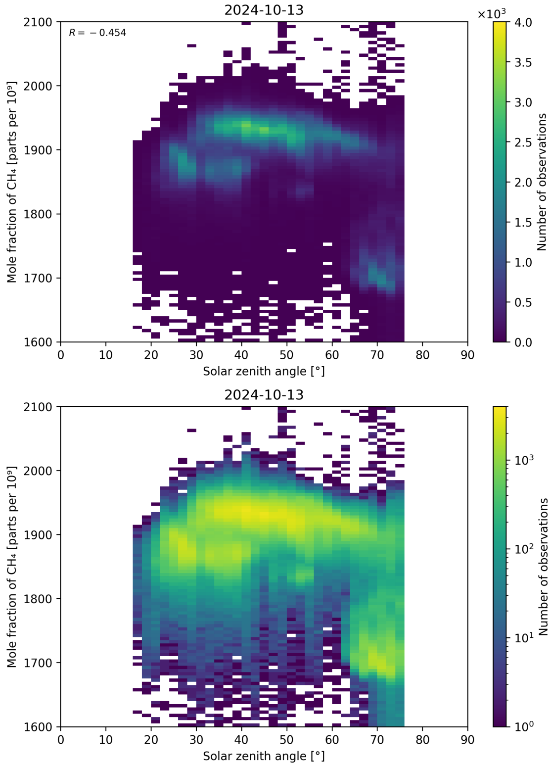
Figure 99: Scatter density plot of “Solar zenith angle” against “Mole fraction of \text{CH}_4 ” for 2024-10-12 to 2024-10-14.
