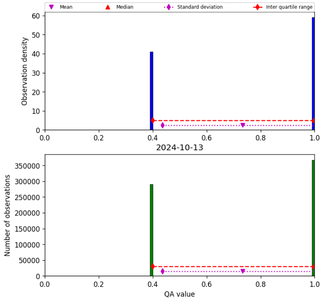
Figure 22: Histogram of “QA value” for 2024-10-12 to 2024-10-14
