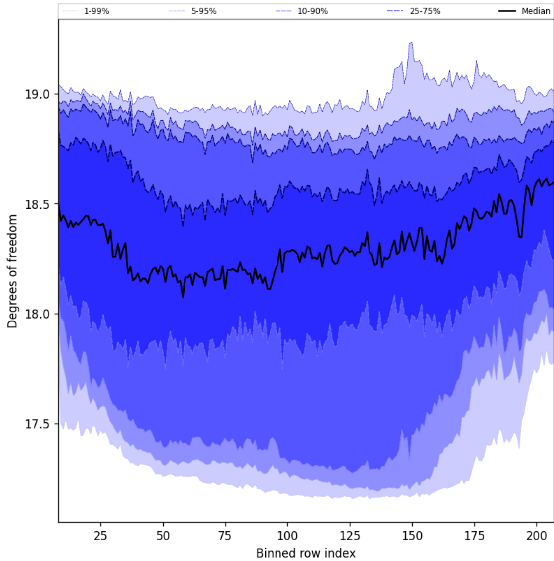
Figure 41: Along track statistics of “Degrees of freedom” for 2024-10-12 to 2024-10-14
