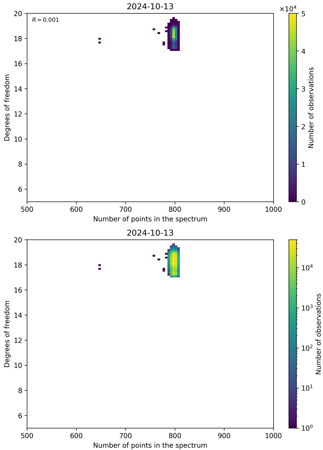
Figure 90: Scatter density plot of “Number of points in the spectrum” against “Degrees of freedom” for 2024-10-12 to 2024-10-14.
