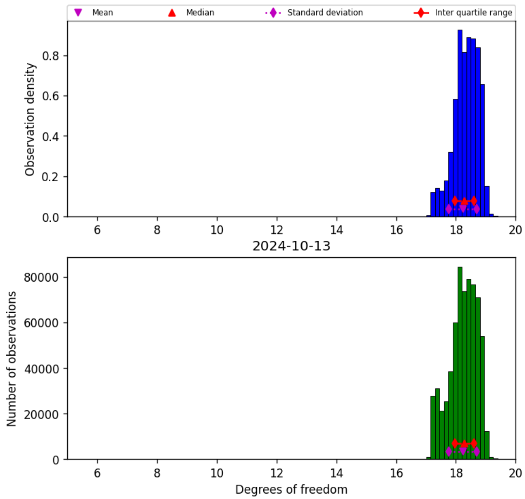
Figure 30: Histogram of “Degrees of freedom” for 2024-10-12 to 2024-10-14
