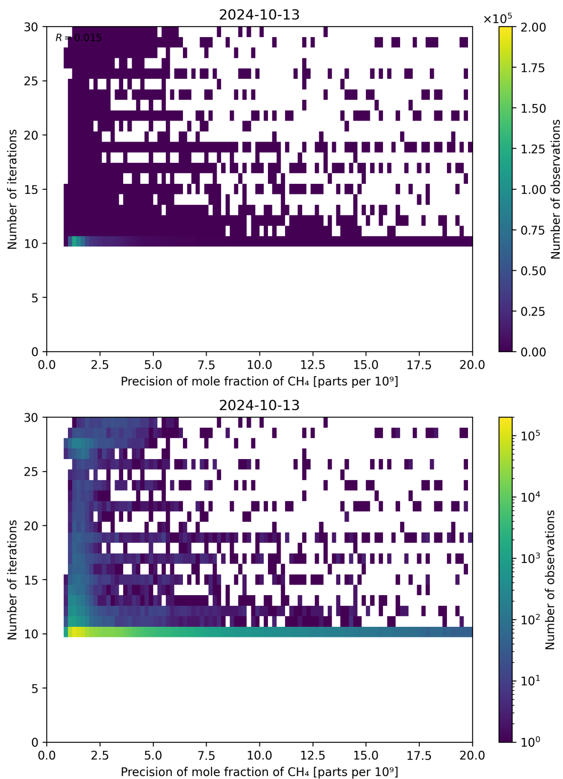
Figure 83: Scatter density plot of “Precision of mole fraction of CH 4 ” against “Number of iterations” for 2024-10-12 to 2024-10-14.
