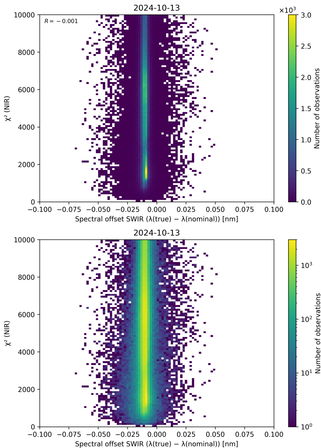
Figure 117: Scatter density plot of “Spectral offset SWIR ( \lambda_{\text{true}} - \lambda_{\text{nominal}} )” against “ \chi^2 (NIR)” for 2024-10-12 to 2024-10-14.
