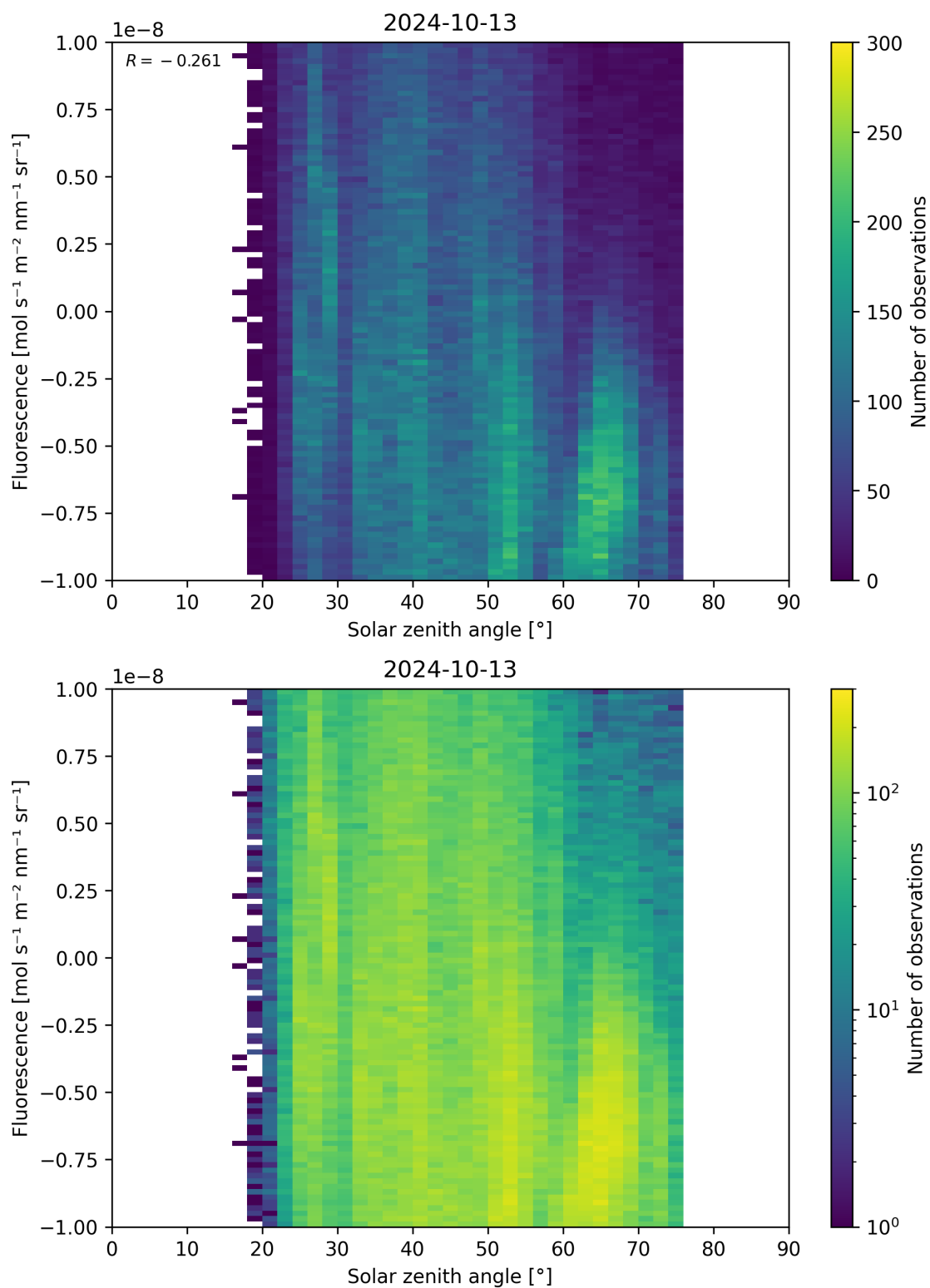
Figure 97: Scatter density plot of “Solar zenith angle” against “Fluorescence” for 2024-10-12 to 2024-10-14.
