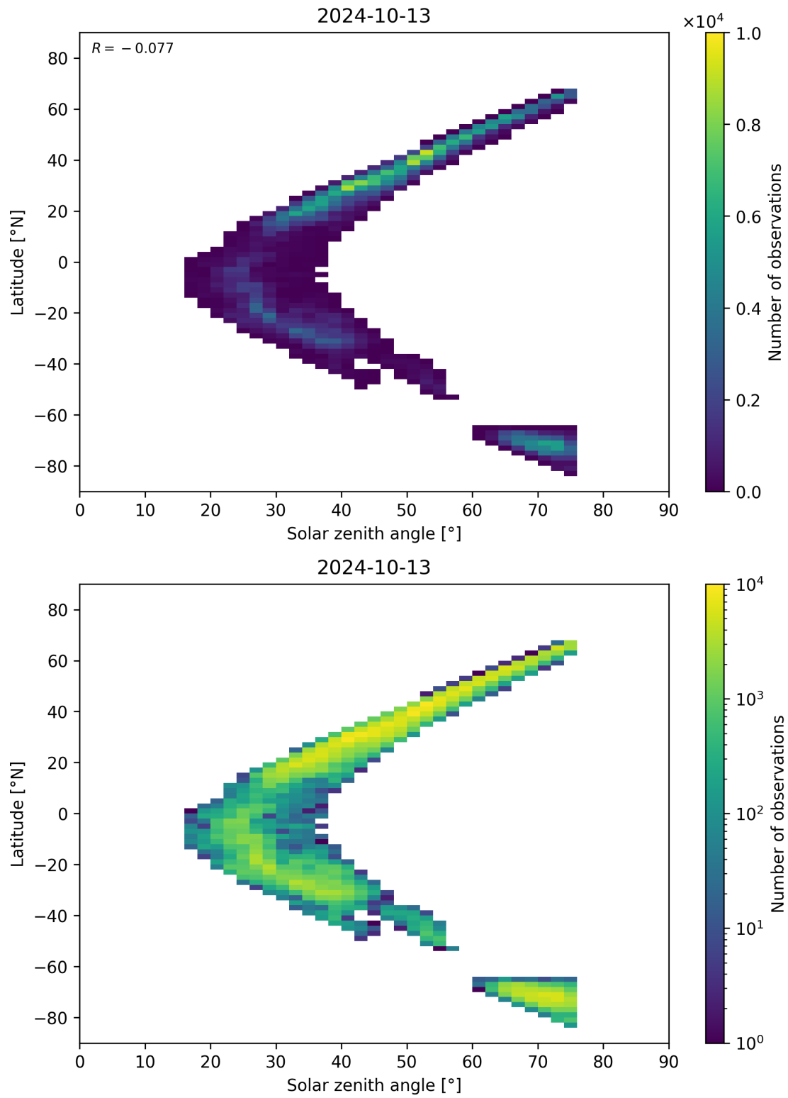
Figure 98: Scatter density plot of “Solar zenith angle” against “Latitude” for 2024-10-12 to 2024-10-14.
