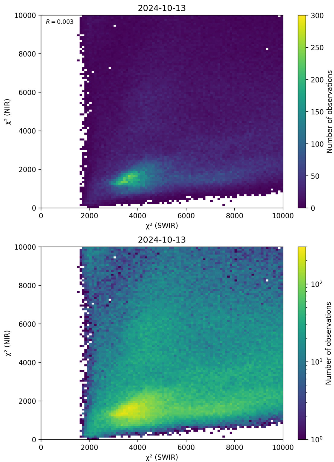
Figure 47: Scatter density plot of “ \chi^2 (SWIR)” against “ \chi^2 (NIR)” for 2024-10-12 to 2024-10-14.
