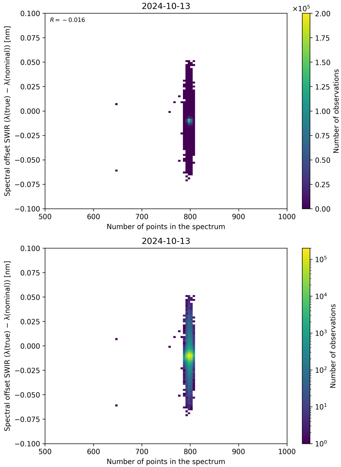
Figure 93: Scatter density plot of “Number of points in the spectrum” against “Spectral offset SWIR ( \lambda_{\text{true}} - \lambda_{\text{nominal}} )” for 2024-10-12 to 2024-10-14.
