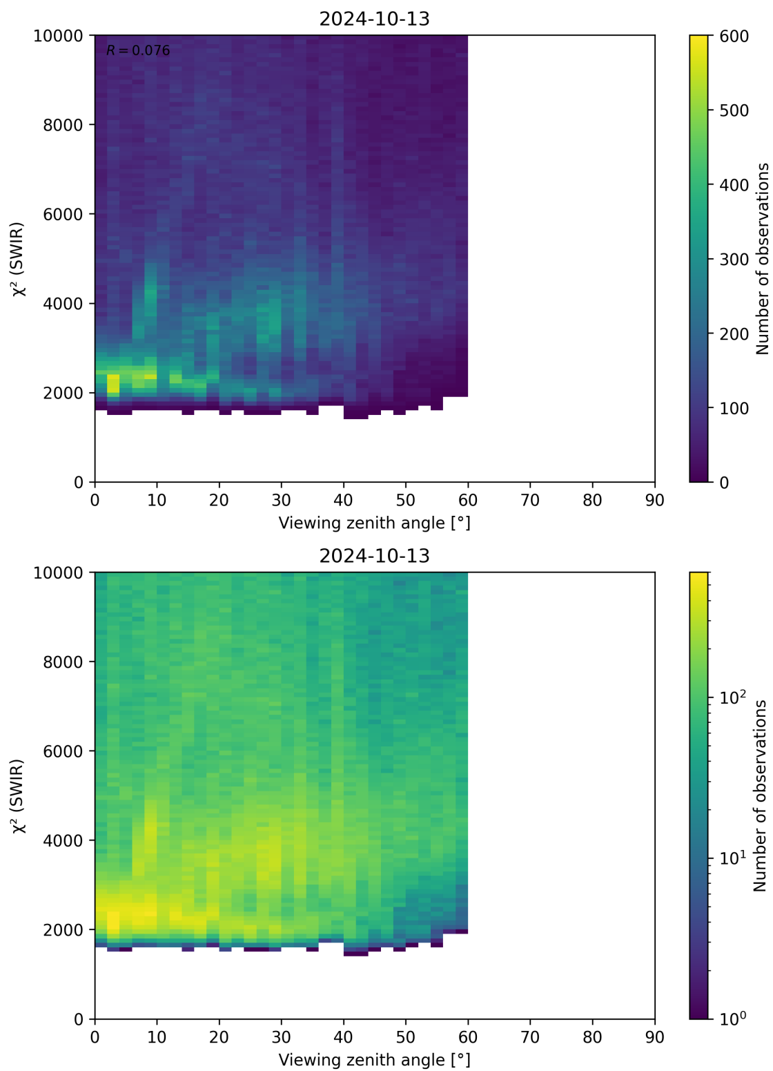
Figure 106: Scatter density plot of “Viewing zenith angle” against “ \chi^2 (SWIR)” for 2024-10-12 to 2024-10-14.
