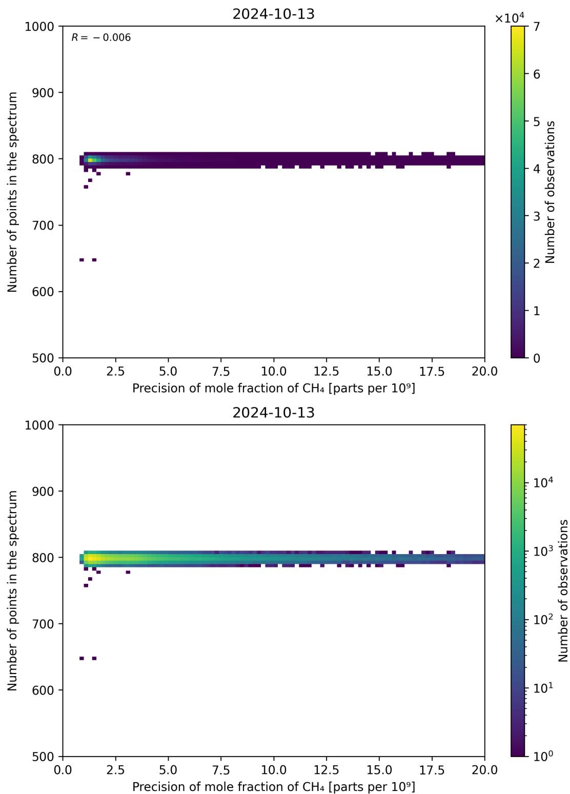
Figure 84: Scatter density plot of “Precision of mole fraction of CH 4 ” against “Number of points in the spectrum” for 2024-10-12 to 2024-10-14.
