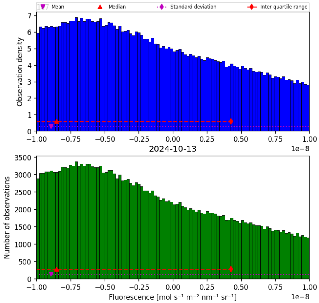
Figure 32: Histogram of “Fluorescence” for 2024-10-12 to 2024-10-14
