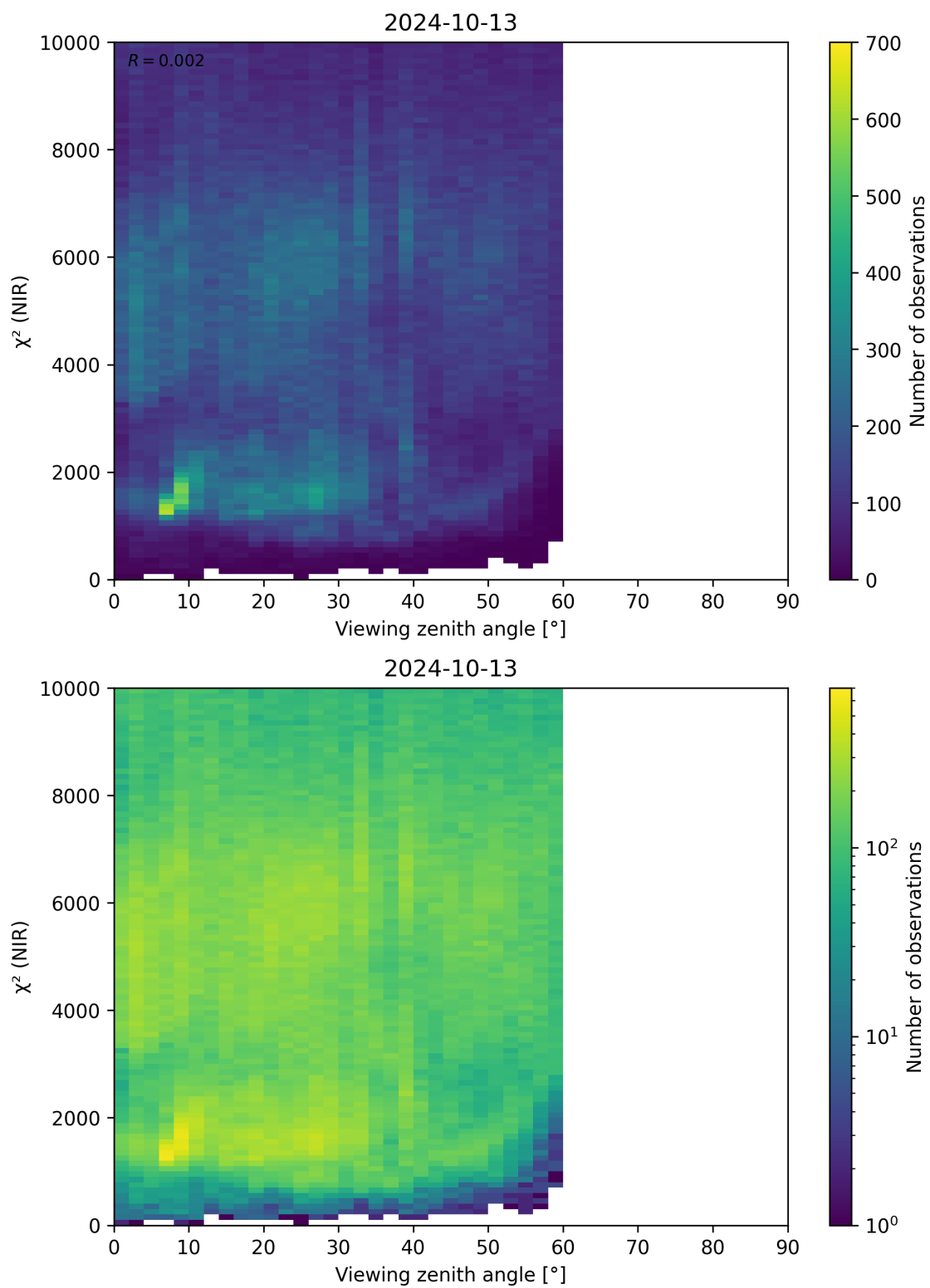
Figure 105: Scatter density plot of “Viewing zenith angle” against “ \chi^2 (NIR)” for 2024-10-12 to 2024-10-14.
