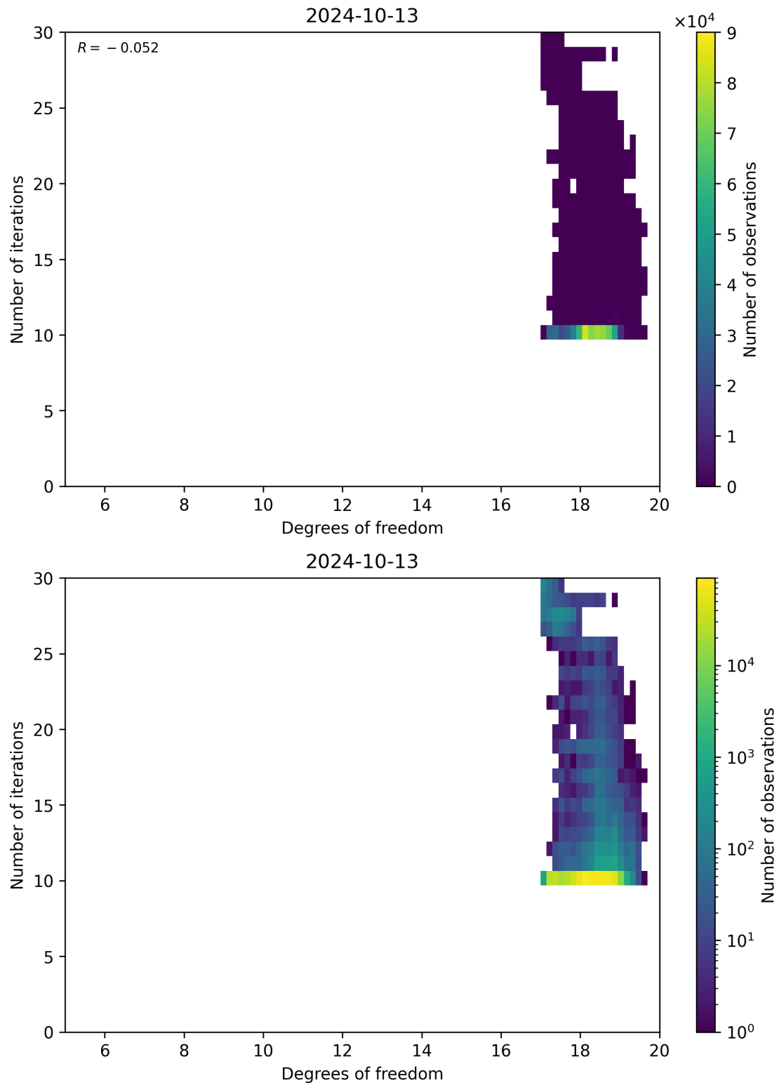
Figure 52: Scatter density plot of “Degrees of freedom” against “Number of iterations” for 2024-10-12 to 2024-10-14.
