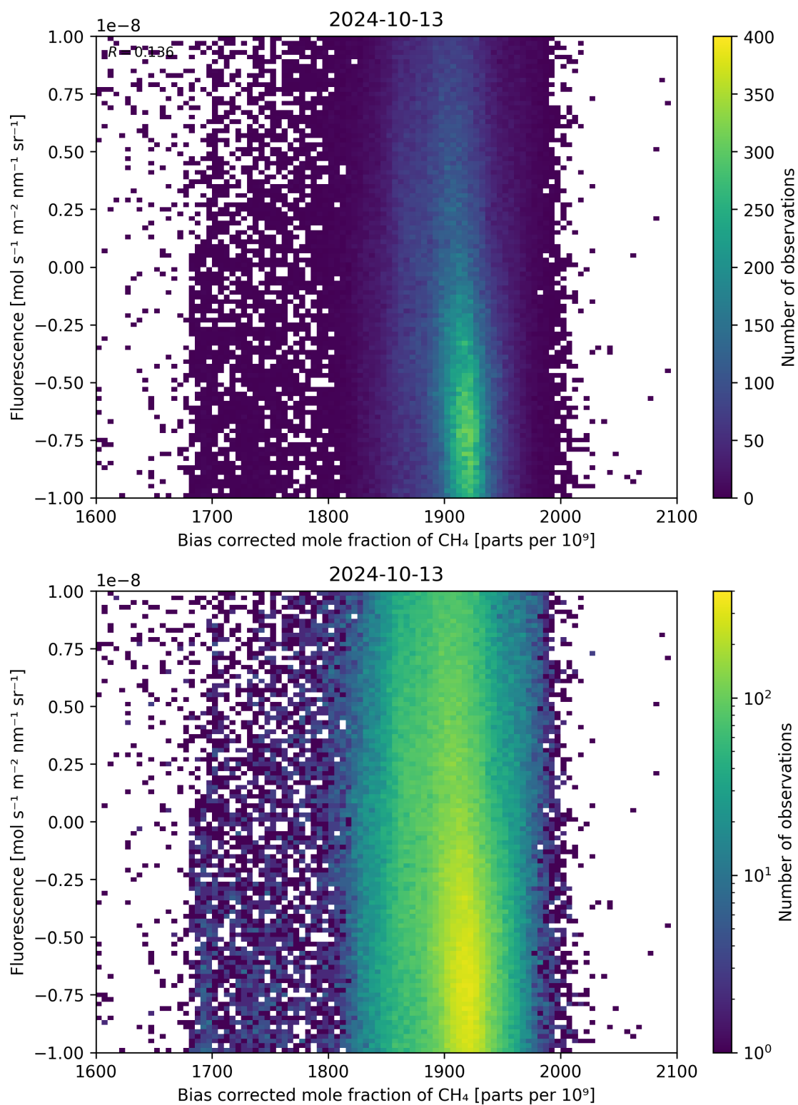
Figure 66: Scatter density plot of “Bias corrected mole fraction of \text{CH}_4 ” against “Fluorescence” for 2024-10-12 to 2024-10-14.
