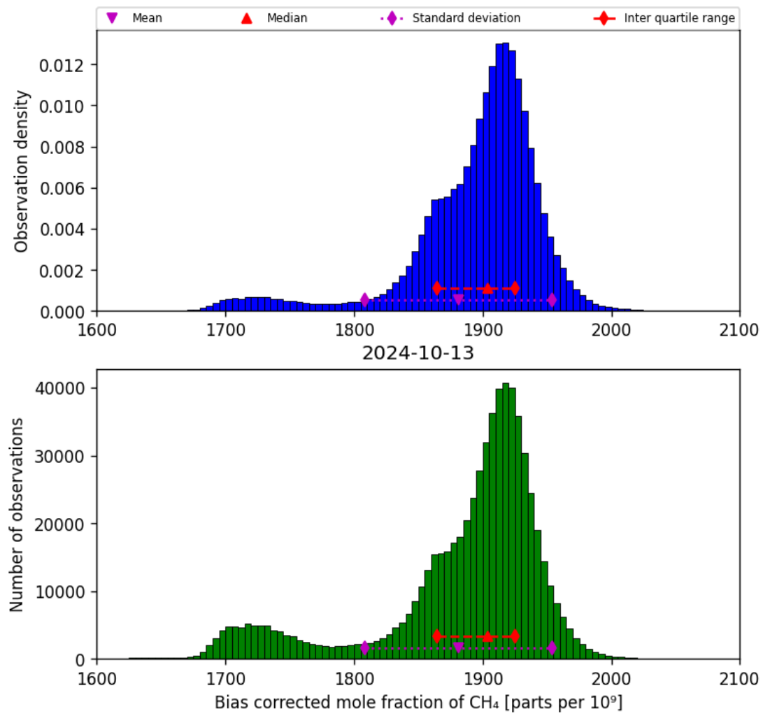
Figure 25: Histogram of “Bias corrected mole fraction of CH 4 ” for 2024-10-12 to 2024-10-14
