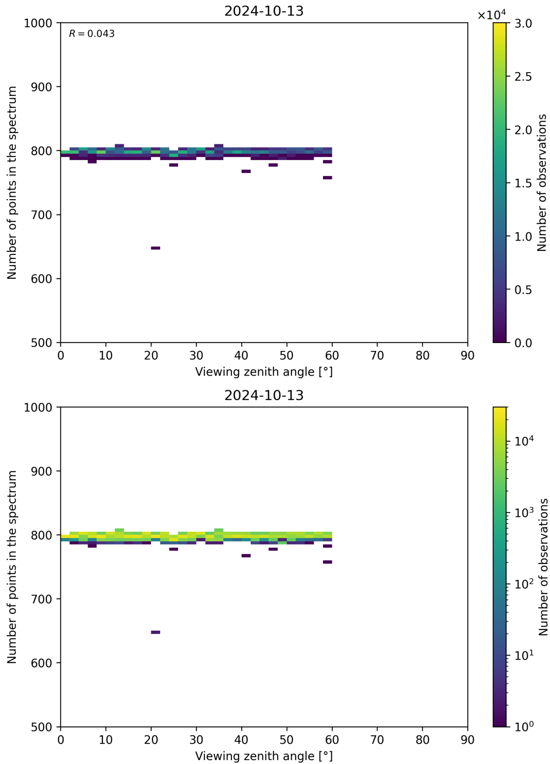
Figure 114: Scatter density plot of “Viewing zenith angle” against “Number of points in the spectrum” for 2024-10-12 to 2024-10-14.
