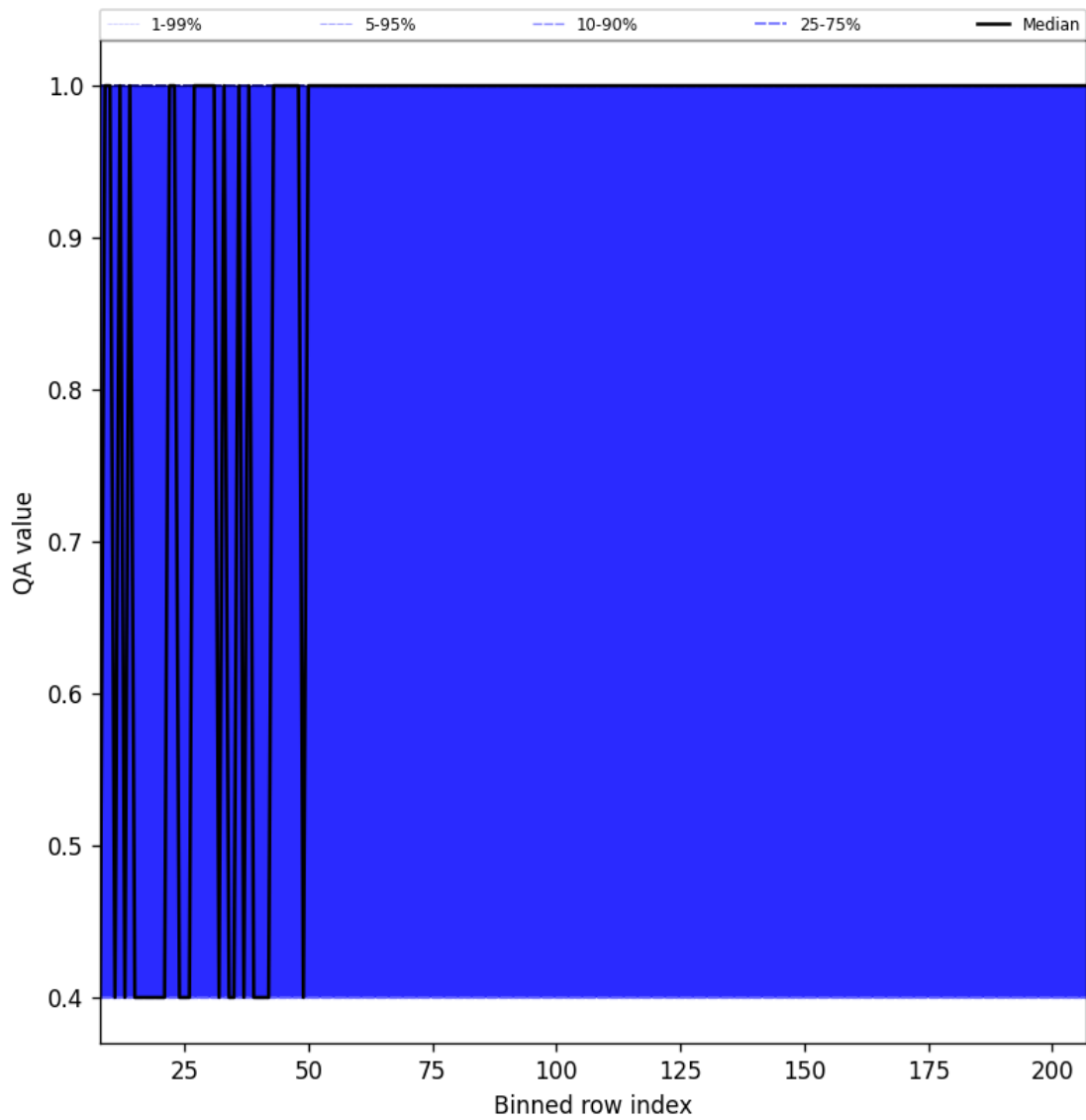
Figure 33: Along track statistics of “QA value” for 2024-10-12 to 2024-10-14
