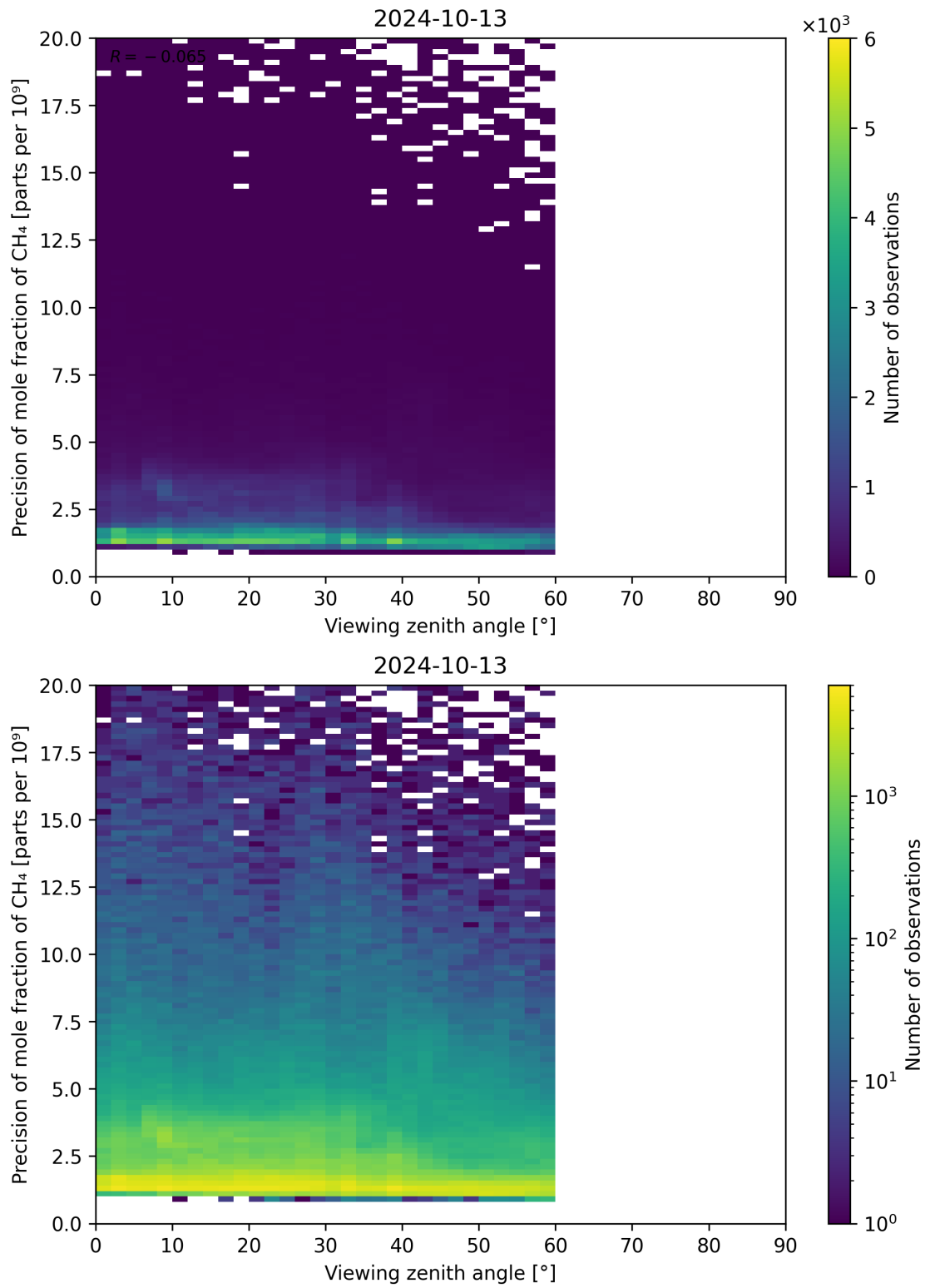
Figure 112: Scatter density plot of “Viewing zenith angle” against “Precision of mole fraction of CH 4 ” for 2024-10-12 to 2024-10-14.
