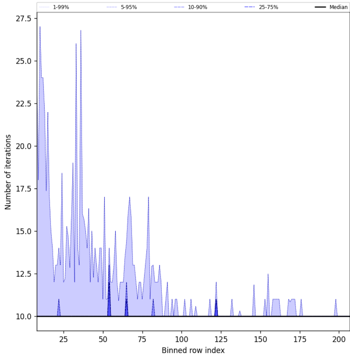
Figure 42: Along track statistics of “Number of iterations” for 2024-10-12 to 2024-10-14
