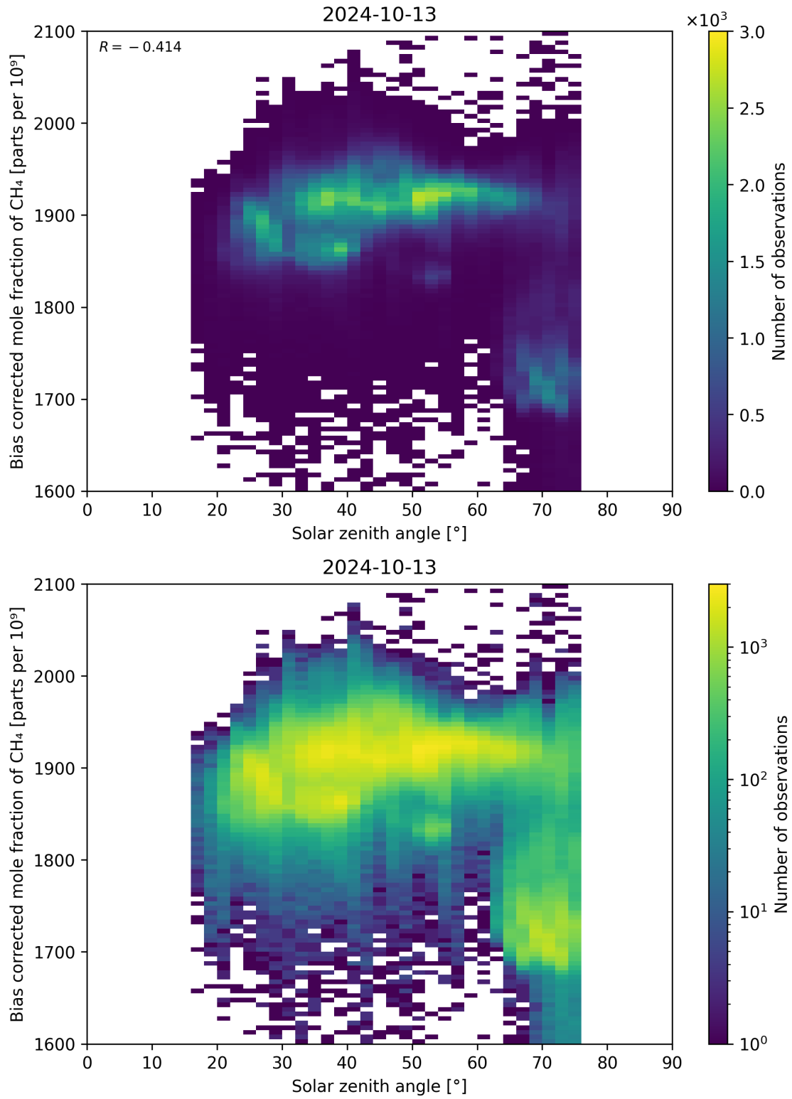
Figure 100: Scatter density plot of “Solar zenith angle” against “Bias corrected mole fraction of \text{CH}_4 ” for 2024-10-12 to 2024-10-14.
