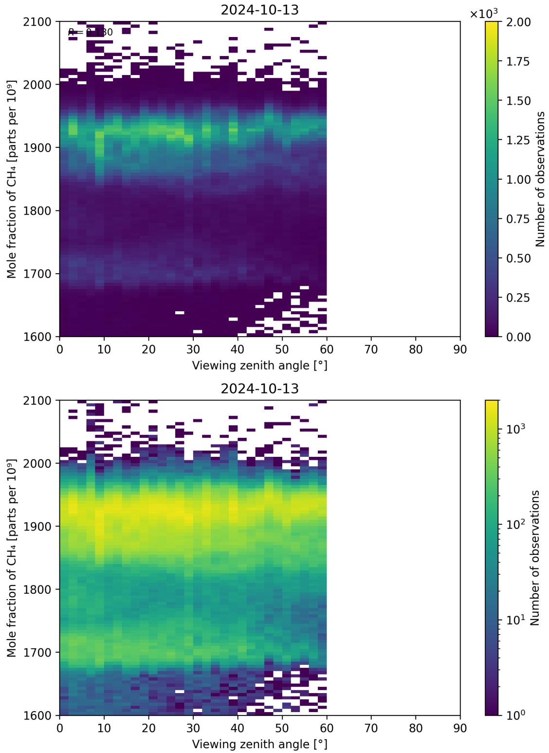
Figure 110: Scatter density plot of “Viewing zenith angle” against “Mole fraction of CH 4 ” for 2024-10-12 to 2024-10-14.
