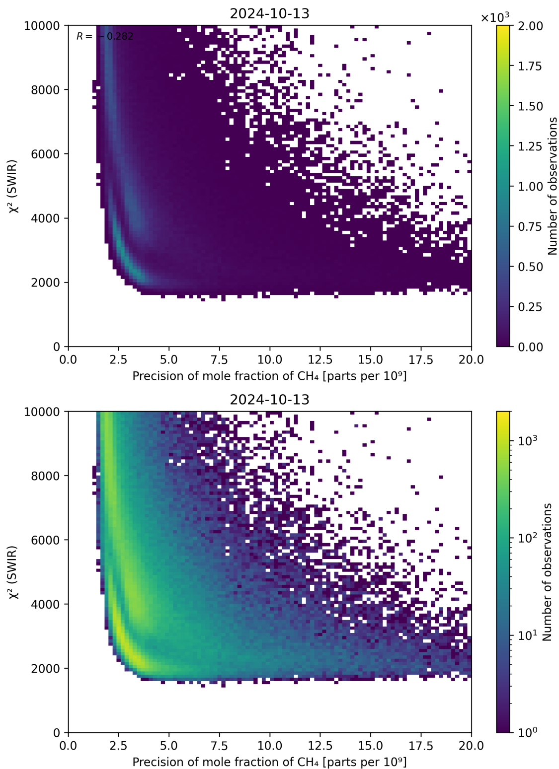
Figure 79: Scatter density plot of “Precision of mole fraction of CH 4 ” against “ \chi^2 (SWIR)” for 2024-10-12 to 2024-10-14.
