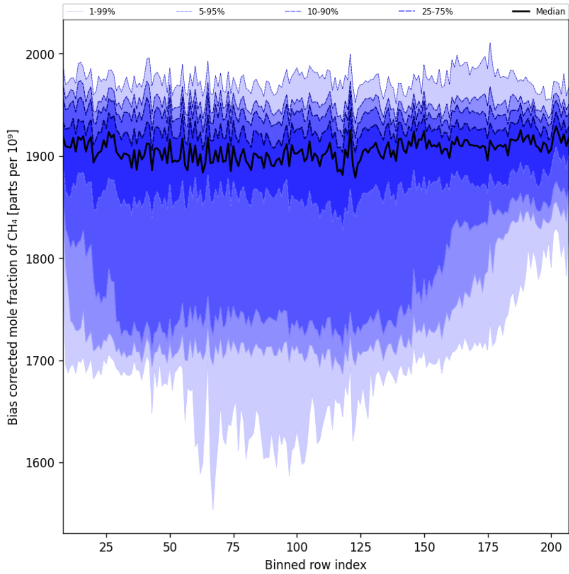
Figure 36: Along track statistics of “Bias corrected mole fraction of CH 4 ” for 2024-10-12 to 2024-10-14
