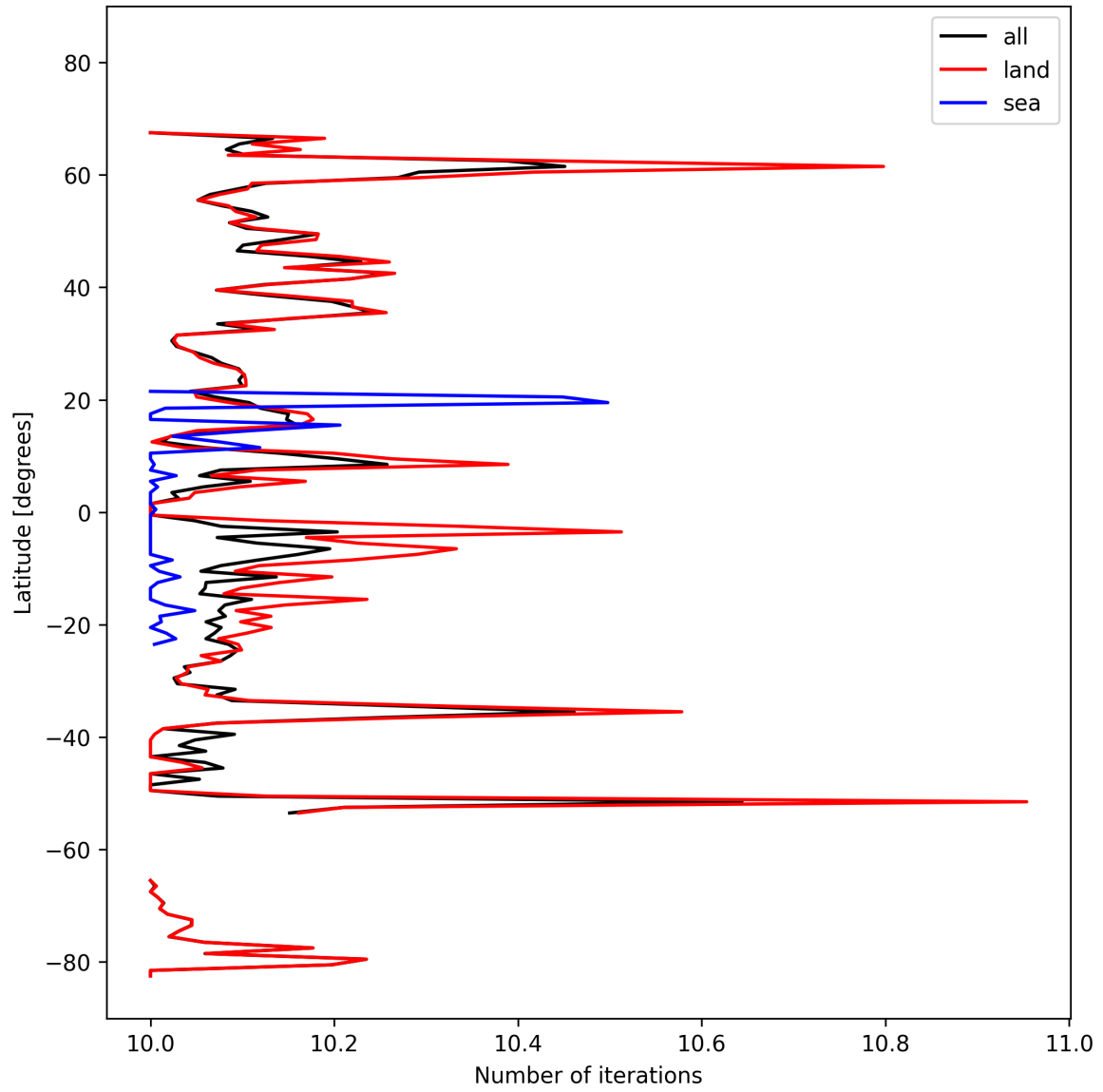
Figure 20: Zonal average of “Number of iterations” for 2024-10-12 to 2024-10-14.
