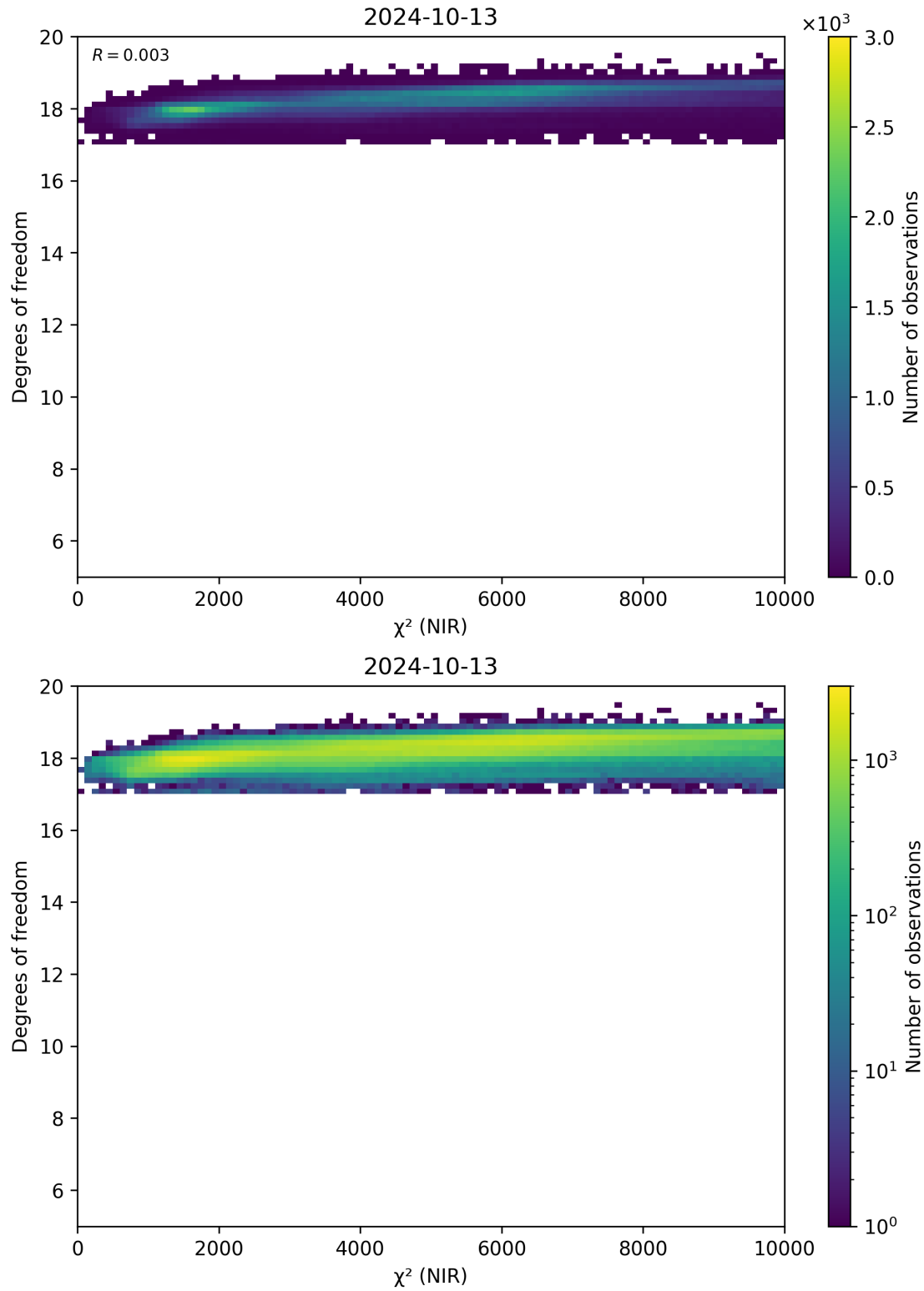
Figure 44: Scatter density plot of “ \chi^2 (NIR)” against “Degrees of freedom” for 2024-10-12 to 2024-10-14.
