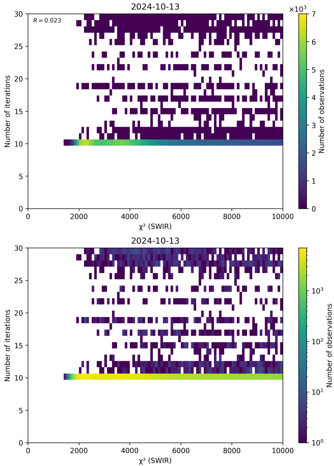
Figure 50: Scatter density plot of “ \chi^2 (SWIR)” against “Number of iterations” for 2024-10-12 to 2024-10-14.
