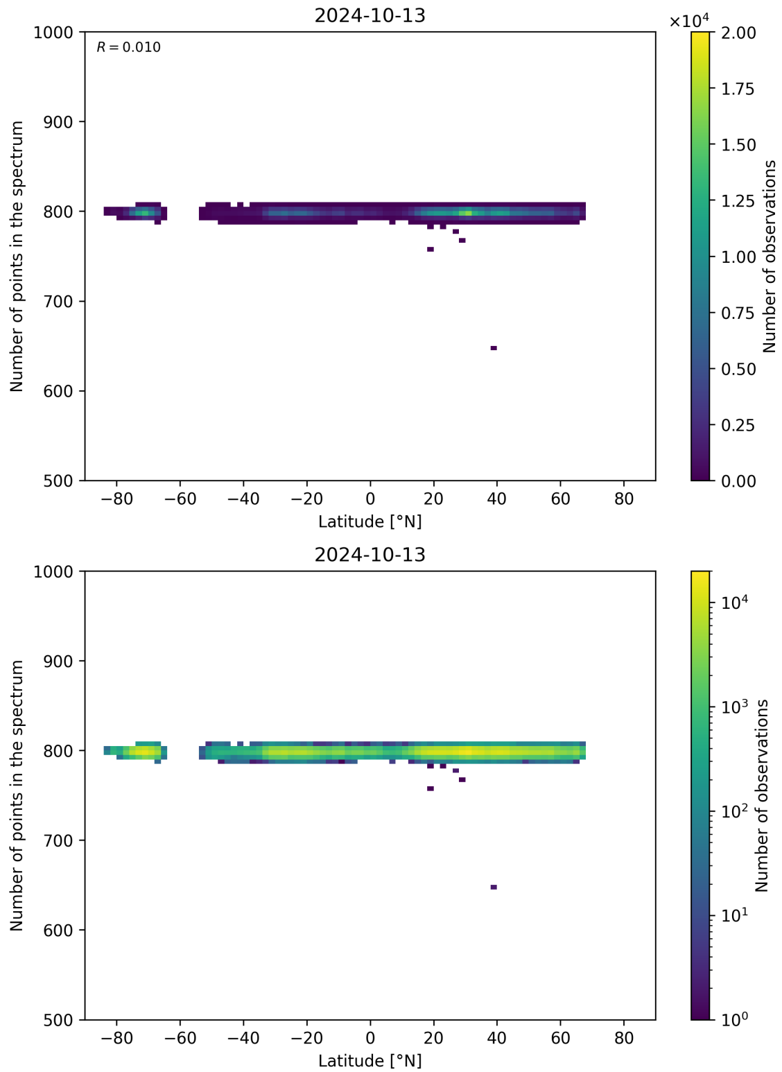
Figure 61: Scatter density plot of “Latitude” against “Number of points in the spectrum” for 2024-10-12 to 2024-10-14.
