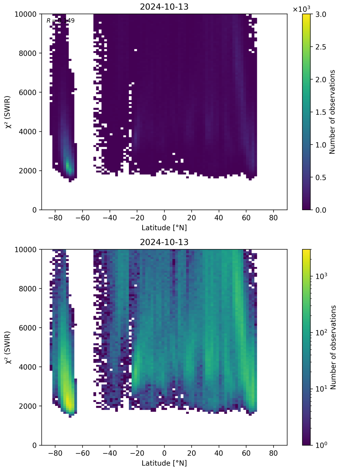
Figure 54: Scatter density plot of “Latitude” against “ \chi^2 (SWIR)” for 2024-10-12 to 2024-10-14.
