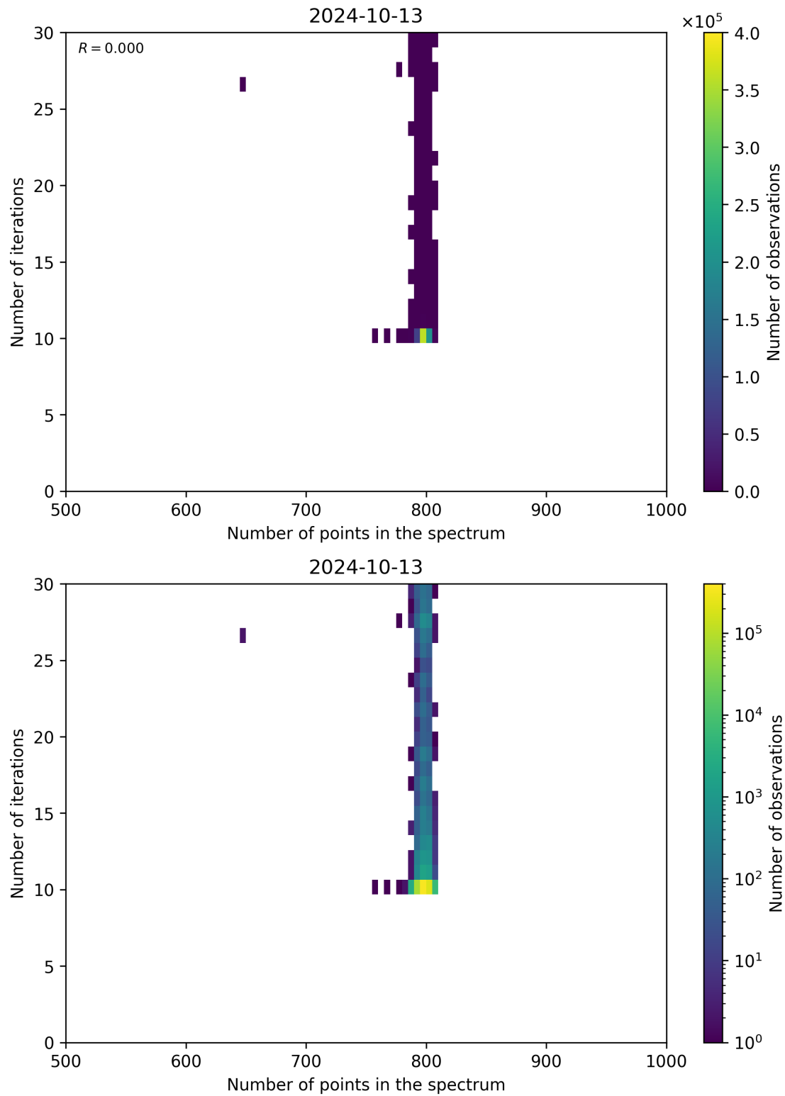
Figure 92: Scatter density plot of “Number of points in the spectrum” against “Number of iterations” for 2024-10-12 to 2024-10-14.
