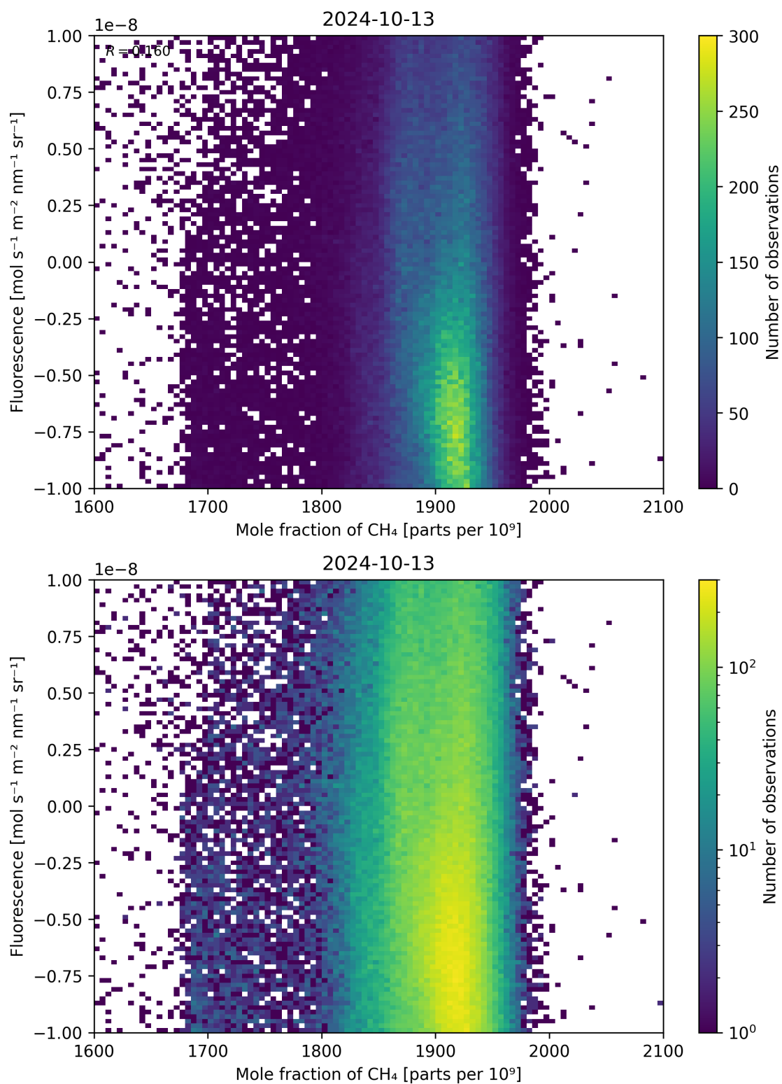
Figure 73: Scatter density plot of “Mole fraction of \text{CH}_4 ” against “Fluorescence” for 2024-10-12 to 2024-10-14.
