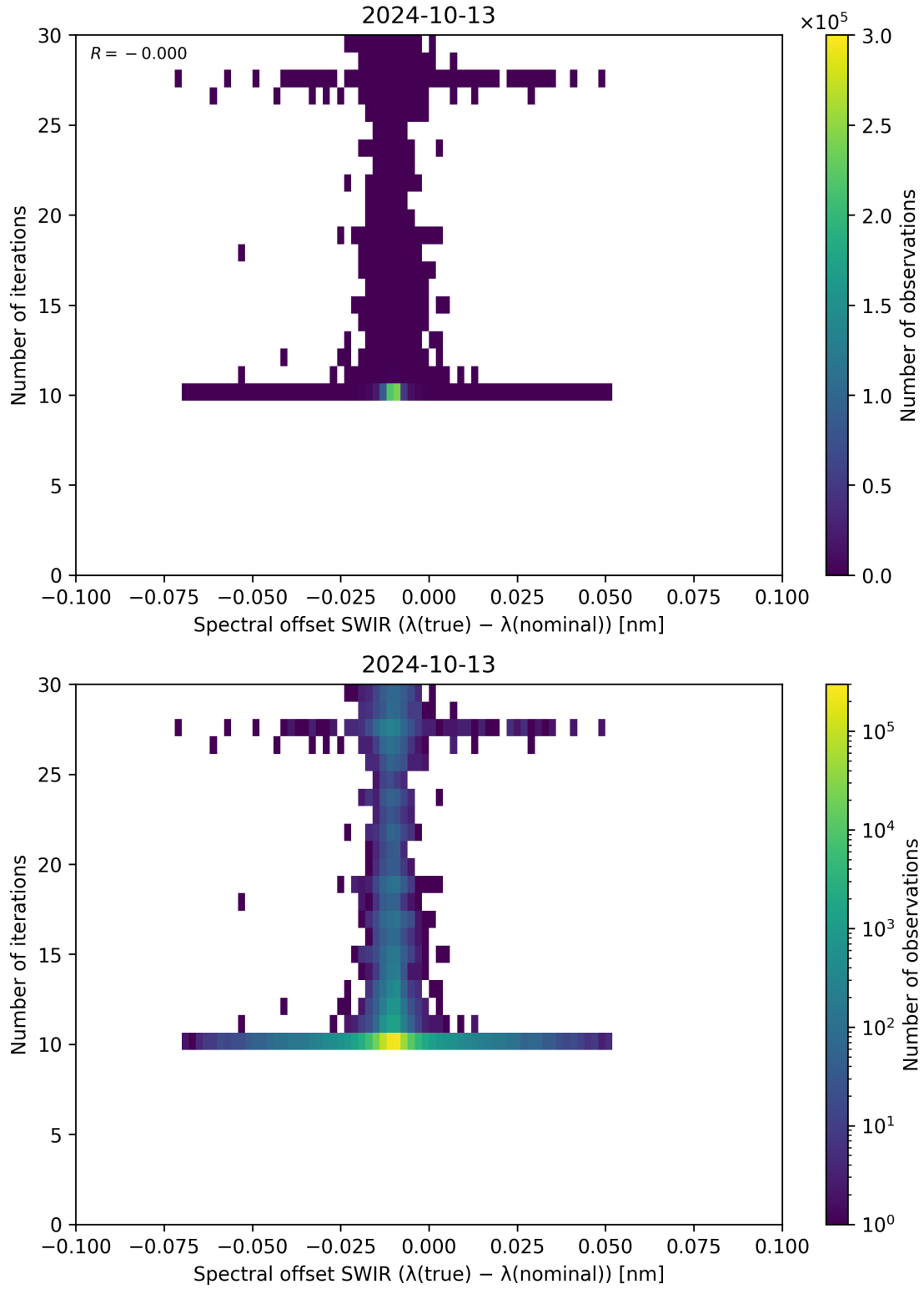
Figure 121: Scatter density plot of “Spectral offset SWIR ( \lambda_{\text{true}} - \lambda_{\text{nominal}} )” against “Number of iterations” for 2024-10-12 to 2024-10-14.
