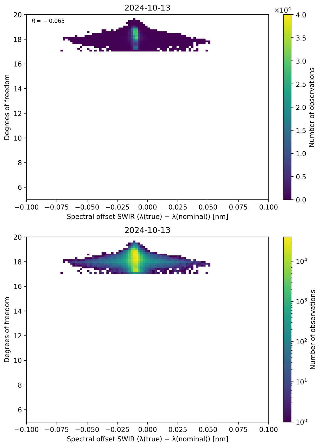
Figure 119: Scatter density plot of “Spectral offset SWIR ( \lambda_{\text{true}} - \lambda_{\text{nominal}} )” against “Degrees of freedom” for 2024-10-12 to 2024-10-14.
