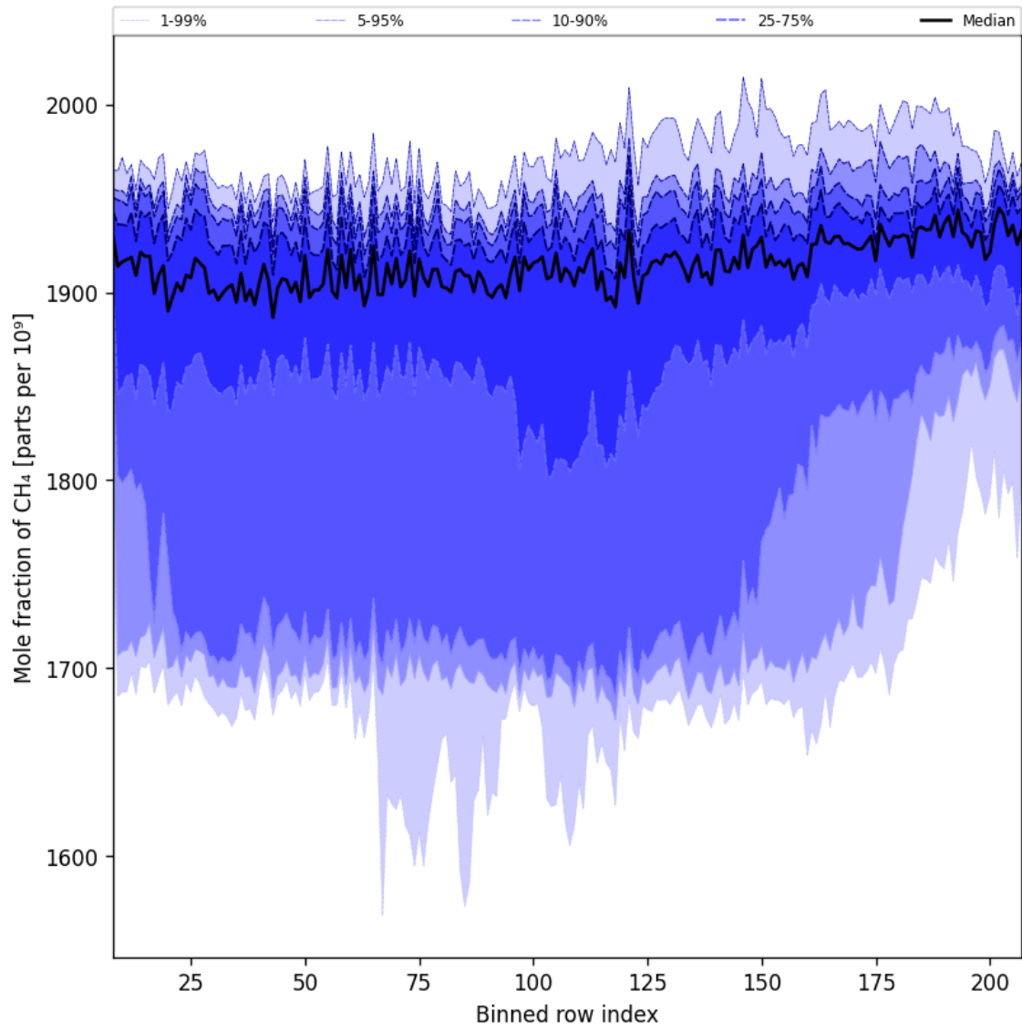
Figure 34: Along track statistics of “Mole fraction of CH 4 ” for 2024-10-14 to 2024-10-15
