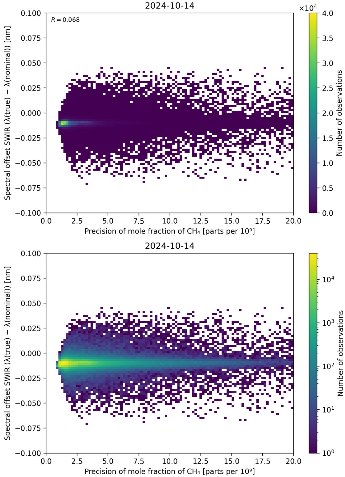
Figure 85: Scatter density plot of “Precision of mole fraction of CH 4 ” against “Spectral offset SWIR ( \lambda_{\text{true}} - \lambda_{\text{nominal}} )” for 2024-10-14 to 2024-10-15.
