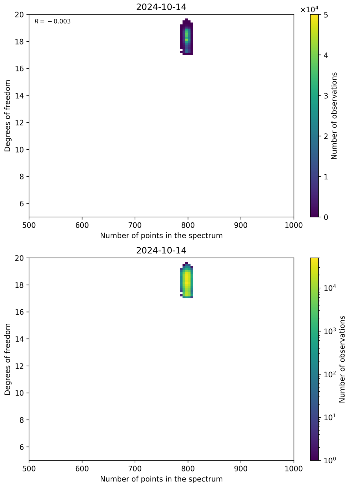
Figure 90: Scatter density plot of “Number of points in the spectrum” against “Degrees of freedom” for 2024-10-14 to 2024-10-15.
