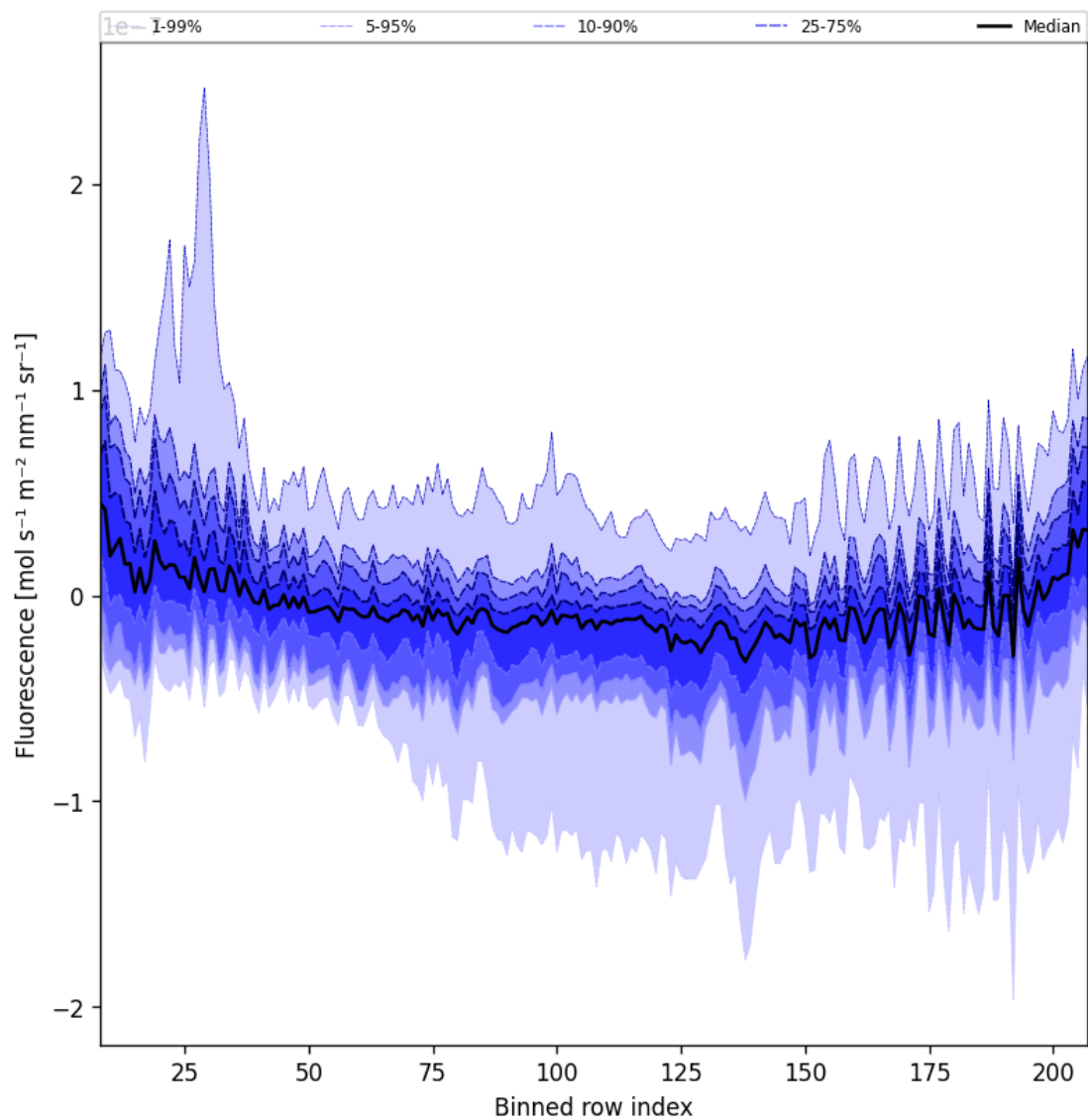
Figure 43: Along track statistics of “Fluorescence” for 2024-10-14 to 2024-10-15
