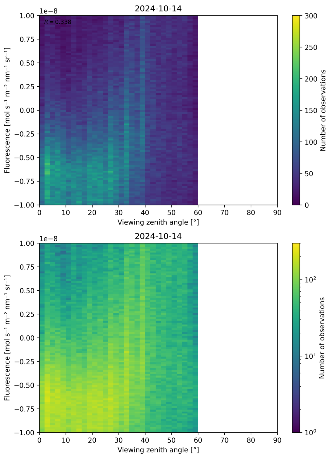
Figure 108: Scatter density plot of “Viewing zenith angle” against “Fluorescence” for 2024-10-14 to 2024-10-15.
