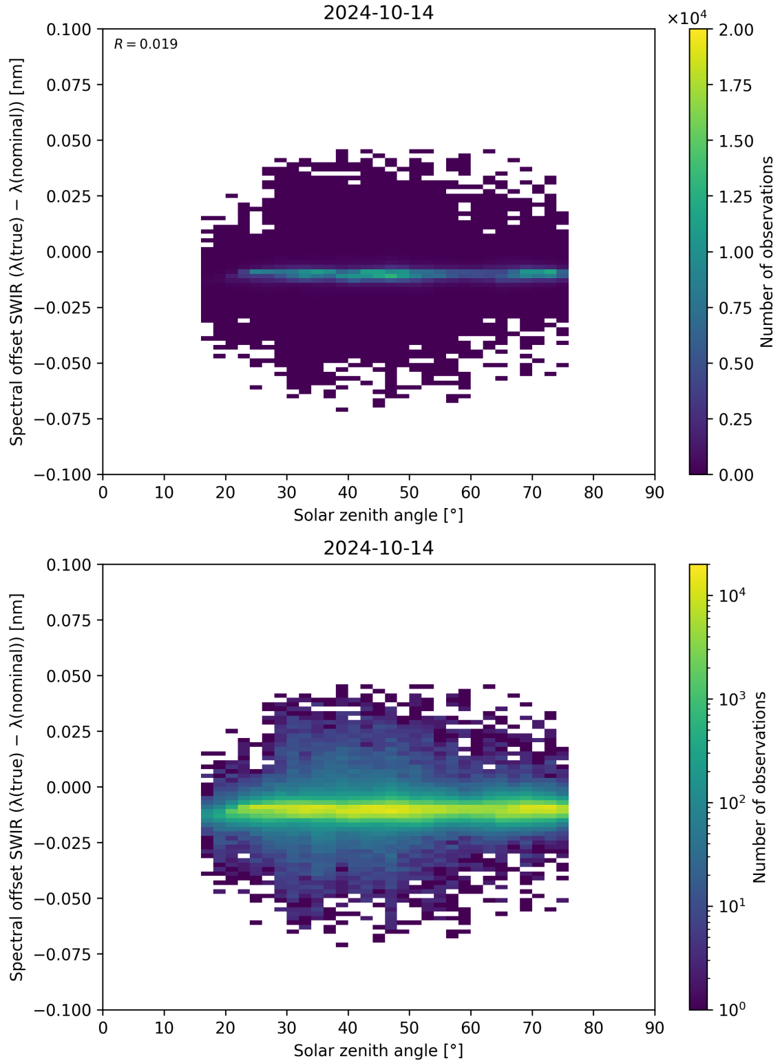
Figure 104: Scatter density plot of “Solar zenith angle” against “Spectral offset SWIR ( \lambda_{\text{true}} - \lambda_{\text{nominal}} )” for 2024-10-14 to 2024-10-15.
