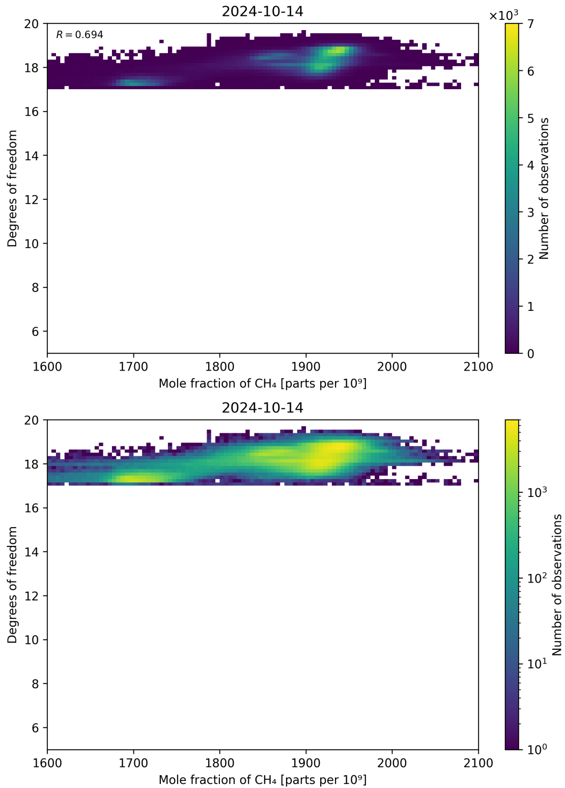
Figure 72: Scatter density plot of “Mole fraction of CH 4 ” against “Degrees of freedom” for 2024-10-14 to 2024-10-15.
