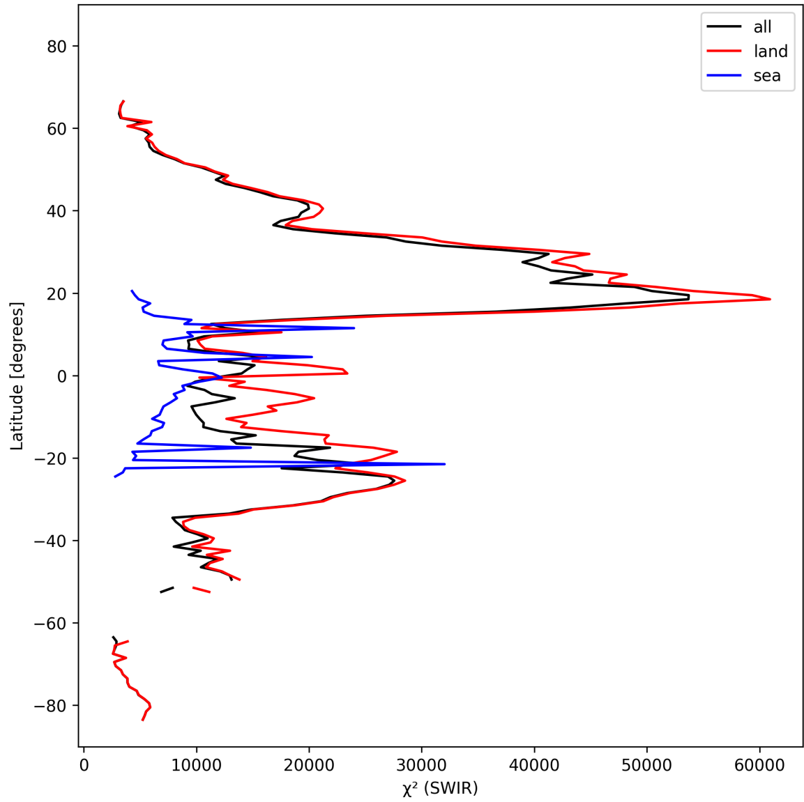
Figure 17: Zonal average of “ \chi^2 (SWIR)” for 2024-10-14 to 2024-10-15.
