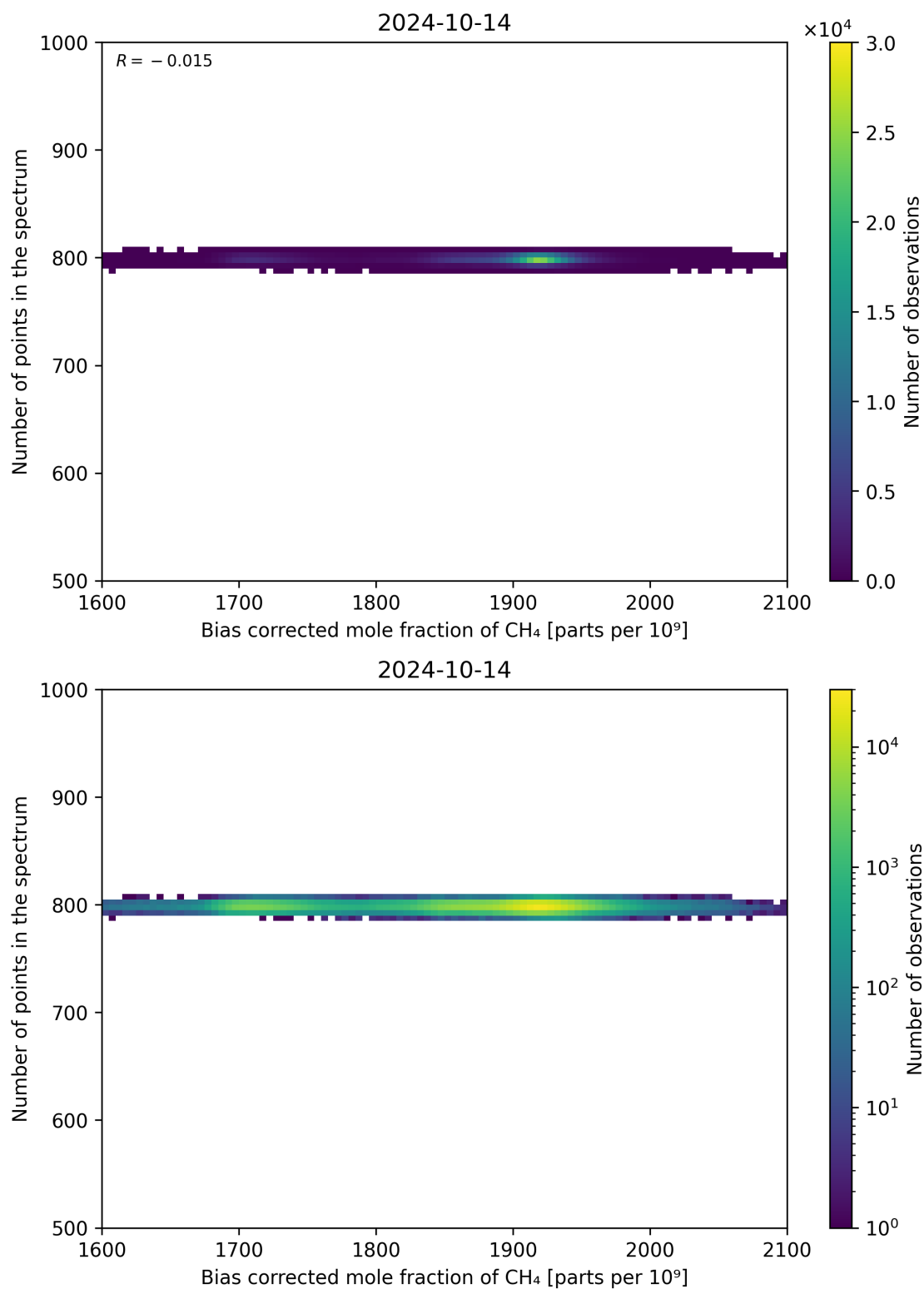
Figure 68: Scatter density plot of “Bias corrected mole fraction of CH 4 ” against “Number of points in the spectrum” for 2024-10-14 to 2024-10-15.
