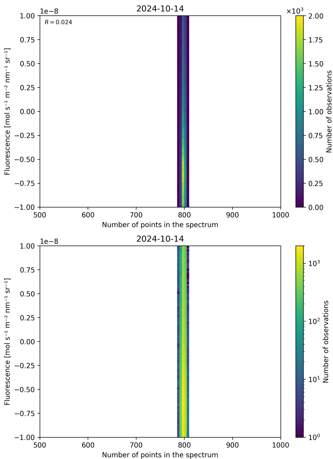
Figure 91: Scatter density plot of “Number of points in the spectrum” against “Fluorescence” for 2024-10-14 to 2024-10-15.
