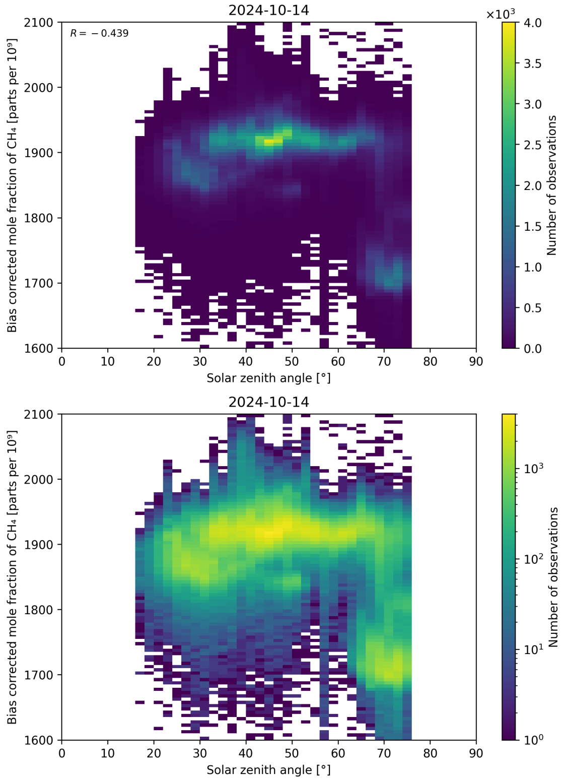
Figure 100: Scatter density plot of “Solar zenith angle” against “Bias corrected mole fraction of CH 4 ” for 2024-10-14 to 2024-10-15.
