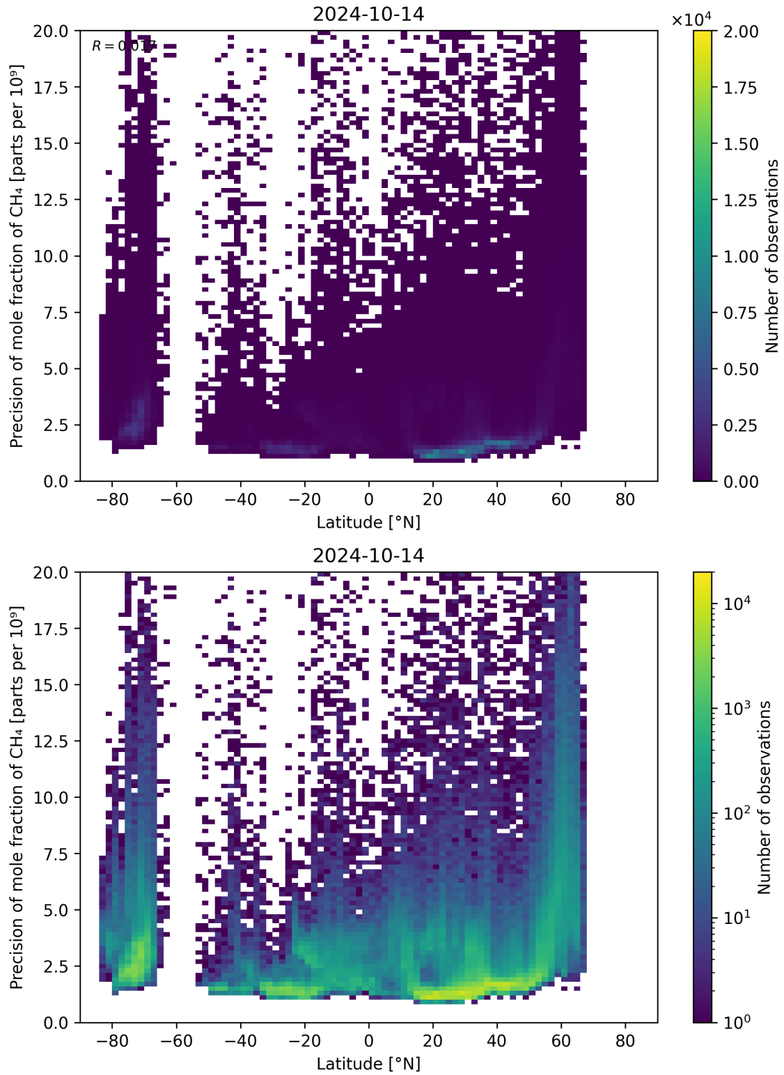
Figure 59: Scatter density plot of “Latitude” against “Precision of mole fraction of CH 4 ” for 2024-10-14 to 2024-10-15.
