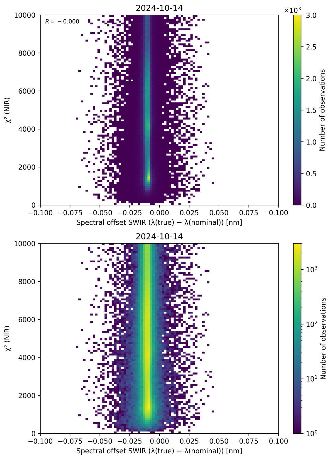
Figure 117: Scatter density plot of “Spectral offset SWIR ( \lambda_{\text{true}} - \lambda_{\text{nominal}} )” against “ \chi^2 (NIR)” for 2024-10-14 to 2024-10-15.
