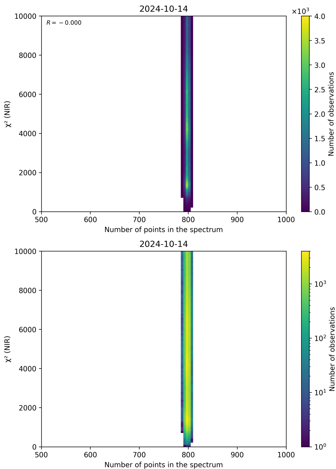
Figure 88: Scatter density plot of “Number of points in the spectrum” against “ \chi^2 (NIR)” for 2024-10-14 to 2024-10-15.
