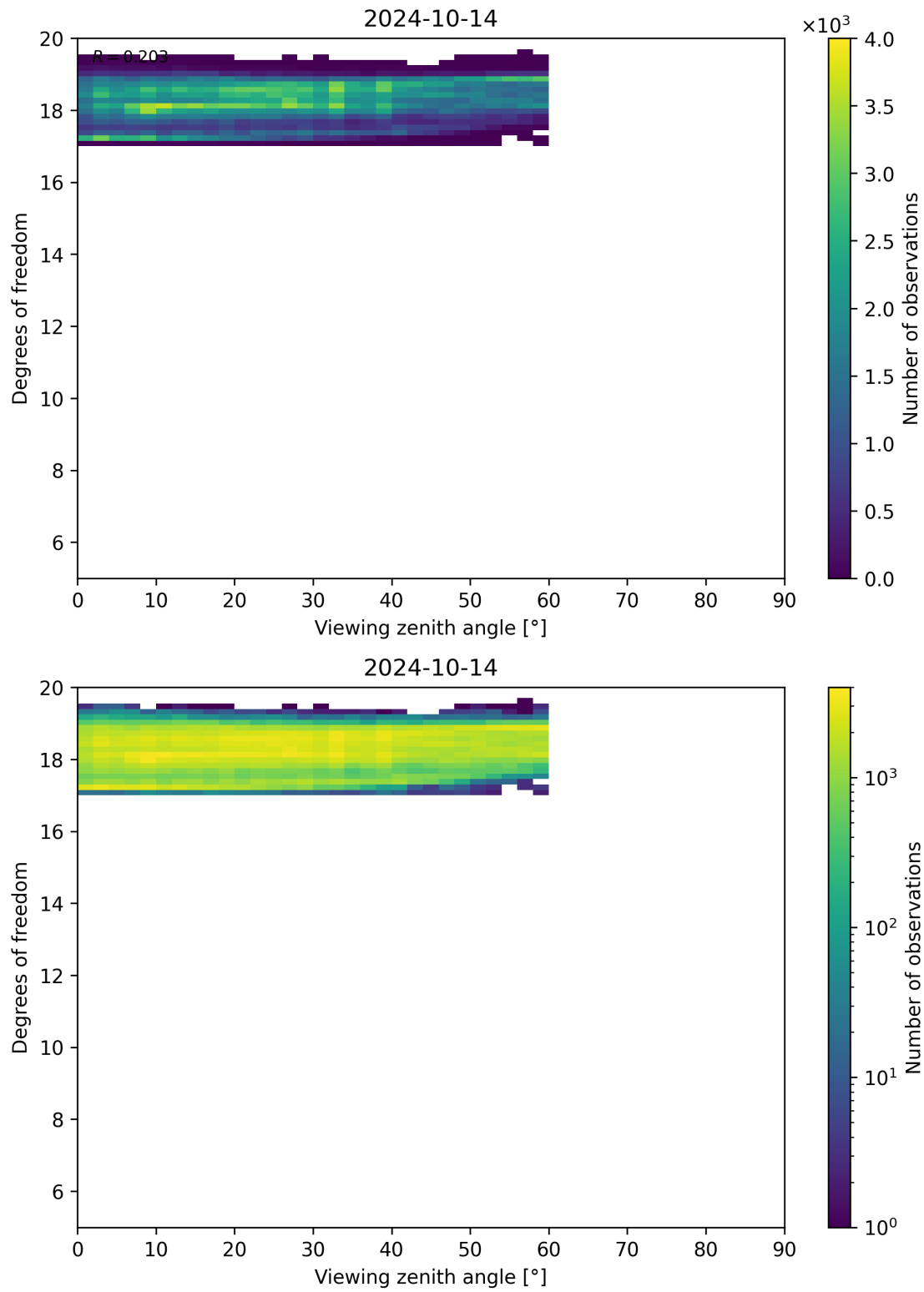
Figure 107: Scatter density plot of “Viewing zenith angle” against “Degrees of freedom” for 2024-10-14 to 2024-10-15.
