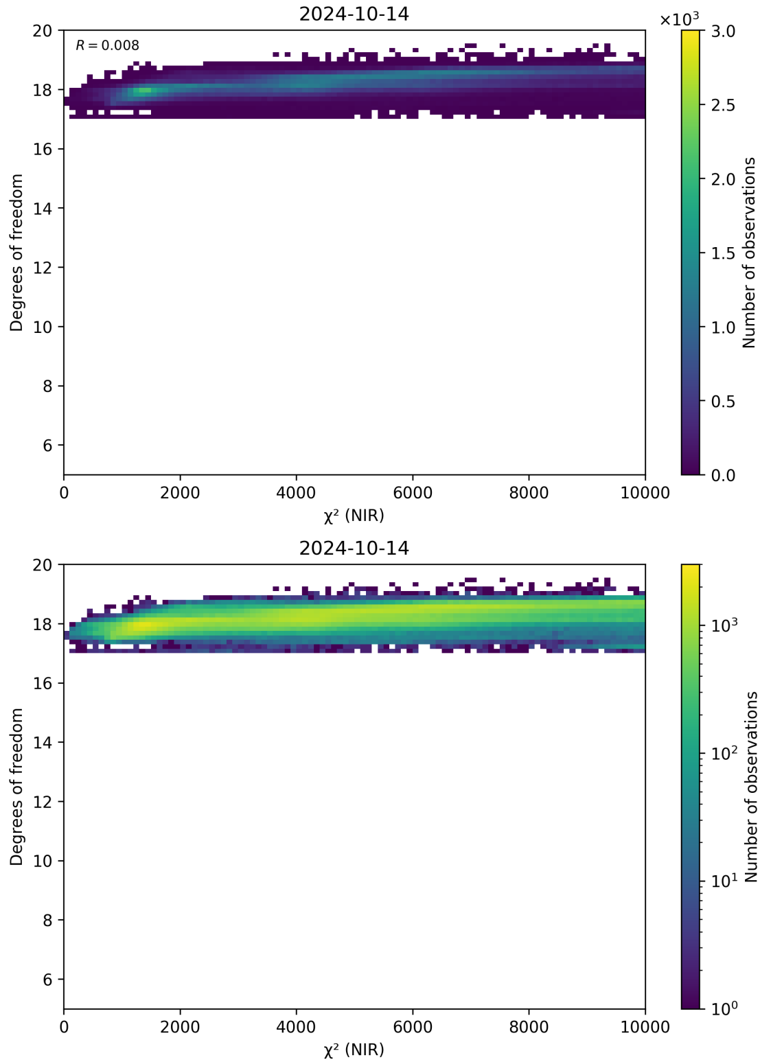
Figure 44: Scatter density plot of “ \chi^2 (NIR)” against “Degrees of freedom” for 2024-10-14 to 2024-10-15.
