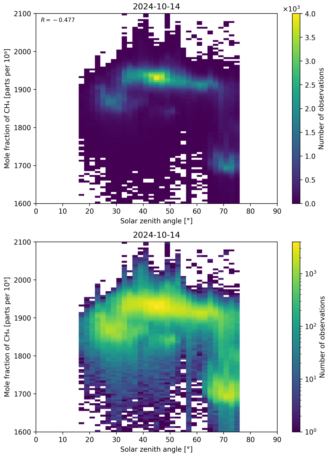
Figure 99: Scatter density plot of “Solar zenith angle” against “Mole fraction of CH 4 ” for 2024-10-14 to 2024-10-15.
