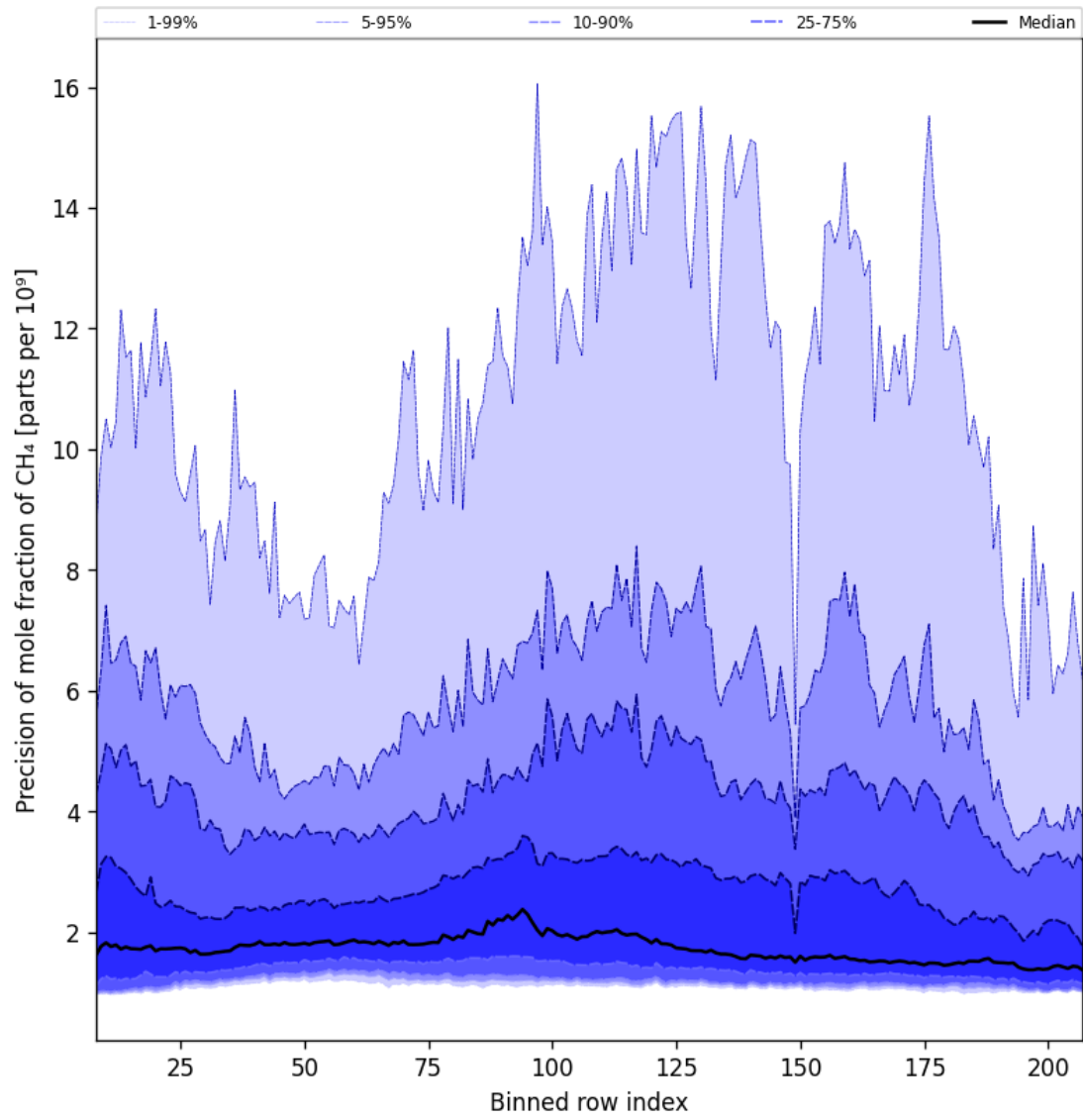
Figure 35: Along track statistics of “Precision of mole fraction of CH 4 ” for 2024-10-14 to 2024-10-15
