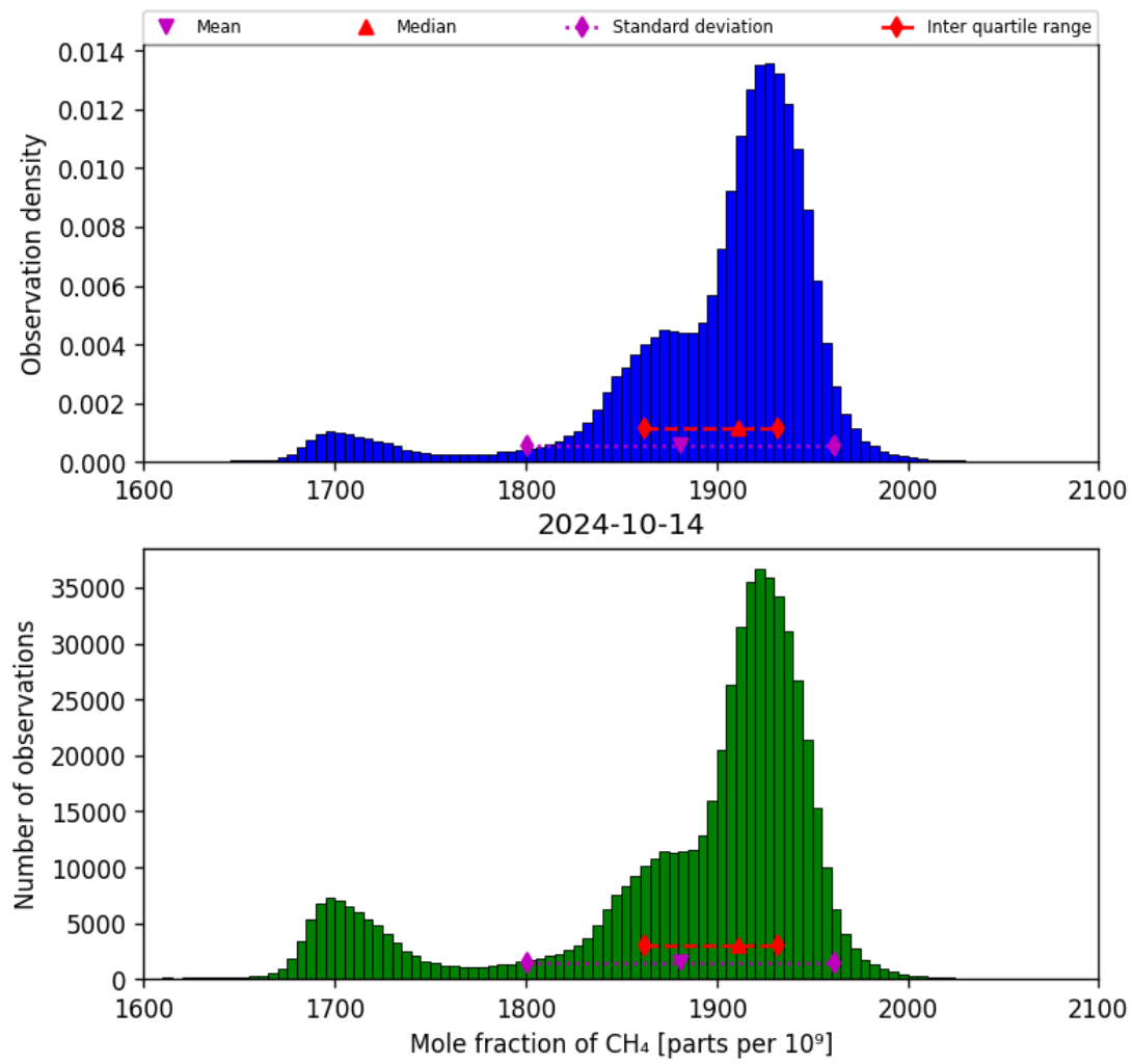
Figure 23: Histogram of “Mole fraction of CH 4 ” for 2024-10-14 to 2024-10-15
