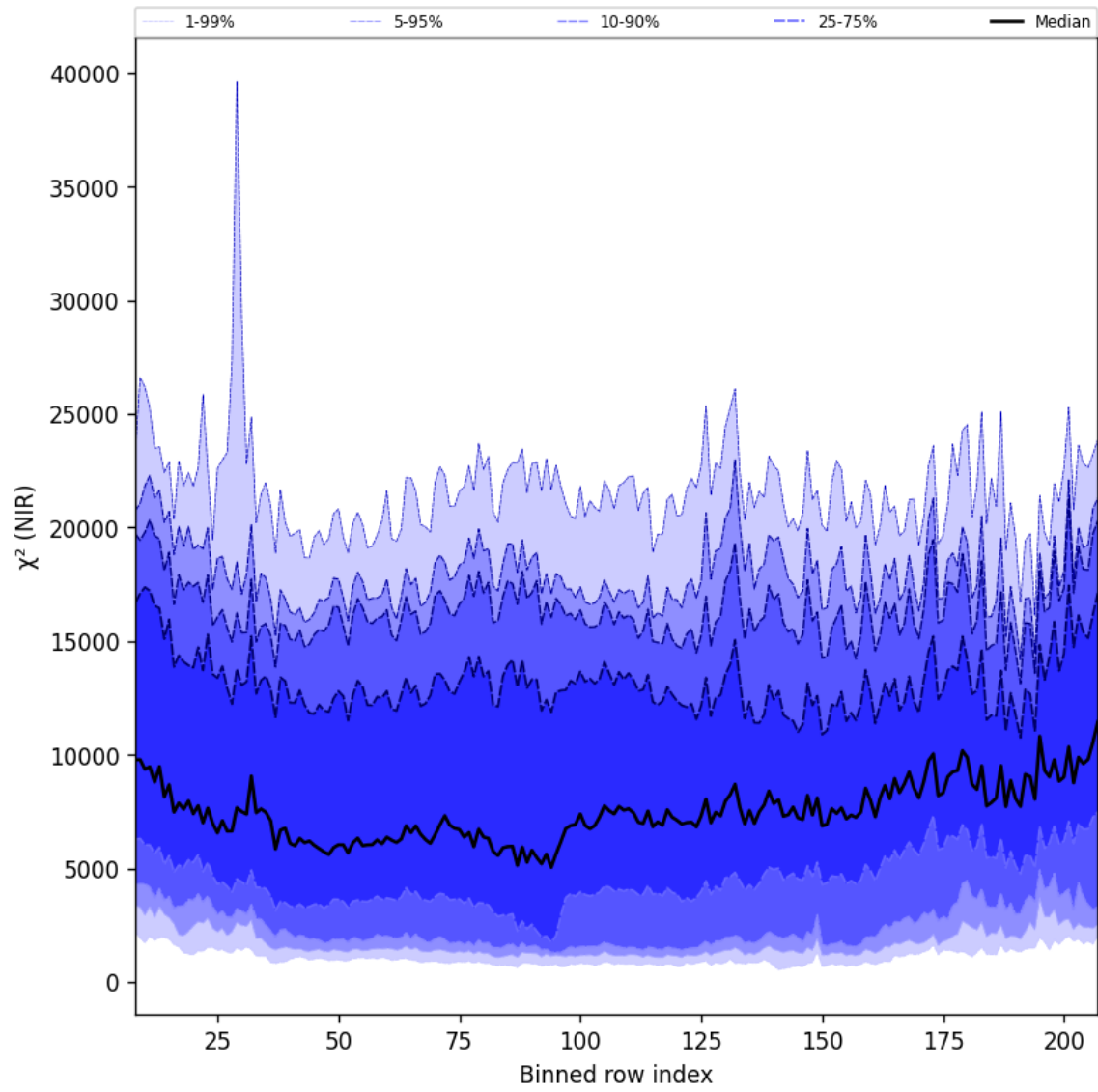
Figure 40: Along track statistics of “ \chi^2 (NIR)” for 2024-10-14 to 2024-10-15
