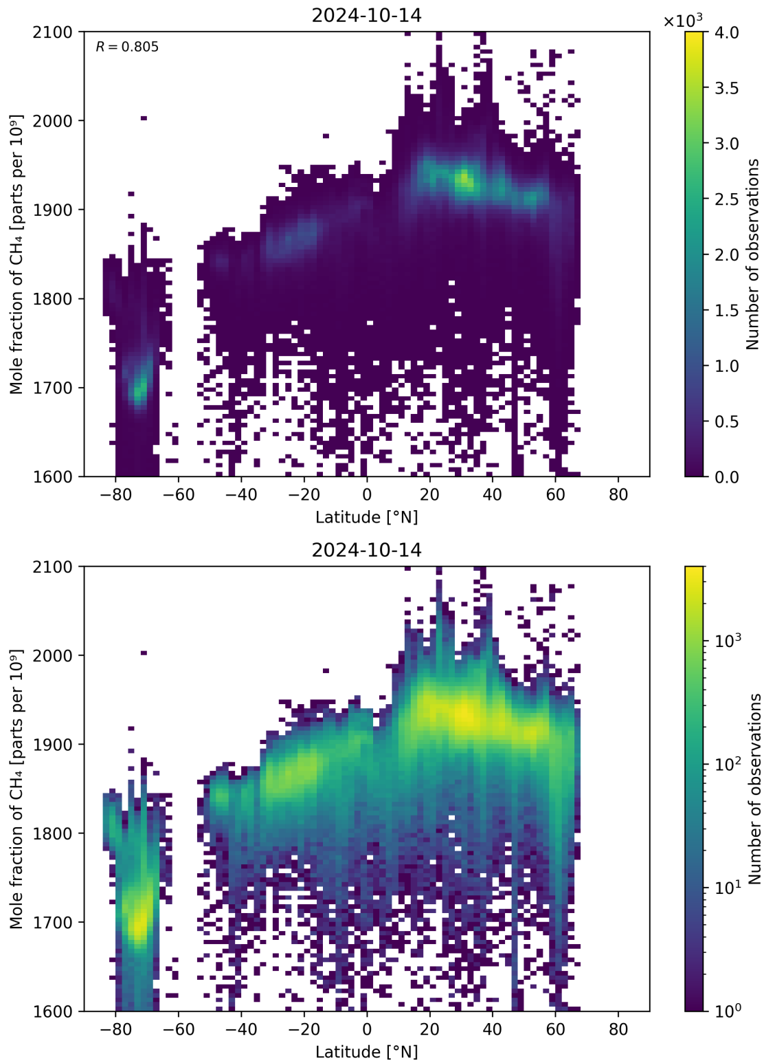
Figure 57: Scatter density plot of “Latitude” against “Mole fraction of \text{CH}_4 ” for 2024-10-14 to 2024-10-15.
