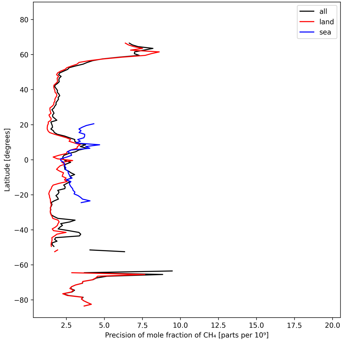
Figure 13: Zonal average of “Precision of mole fraction of CH 4 ” for 2024-10-14 to 2024-10-15.
