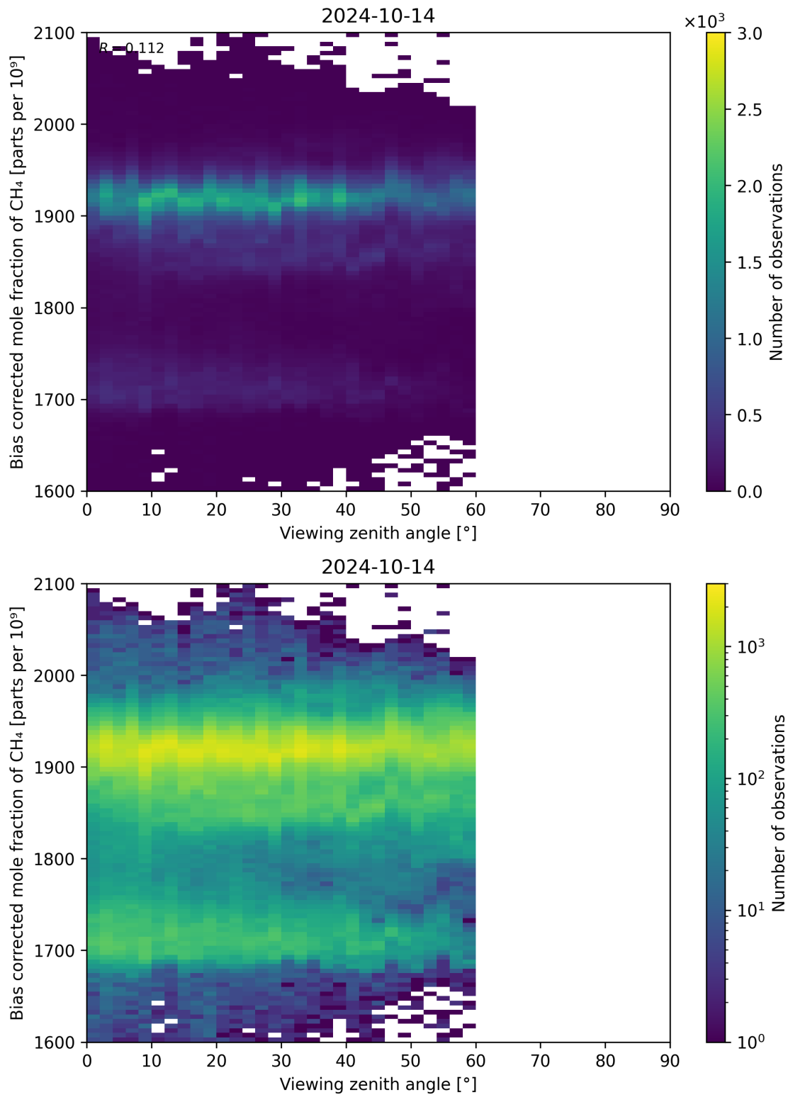
Figure 111: Scatter density plot of “Viewing zenith angle” against “Bias corrected mole fraction of CH 4 ” for 2024-10-14 to 2024-10-15.
