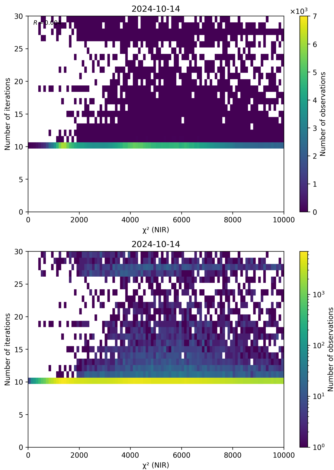
Figure 46: Scatter density plot of “ \chi^2 (NIR)” against “Number of iterations” for 2024-10-14 to 2024-10-15.
