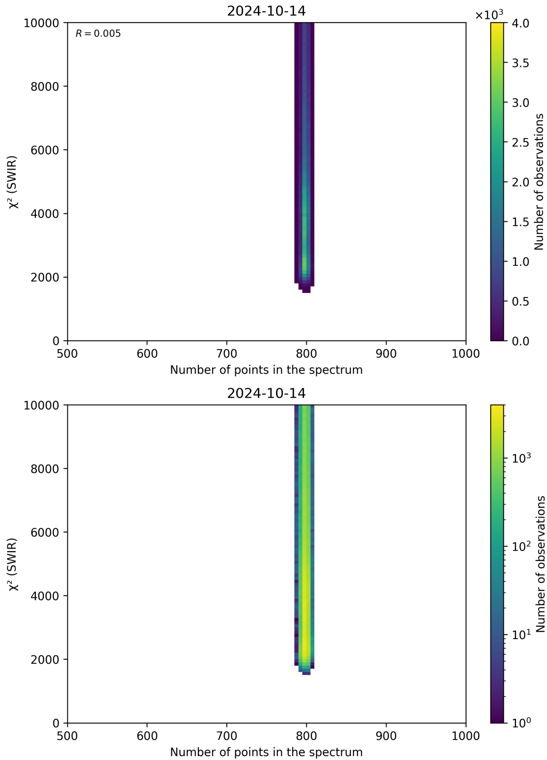
Figure 89: Scatter density plot of “Number of points in the spectrum” against “ \chi^2 (SWIR)” for 2024-10-14 to 2024-10-15.
