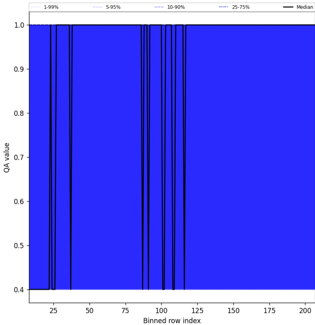
Figure 33: Along track statistics of “QA value” for 2024-10-14 to 2024-10-15
