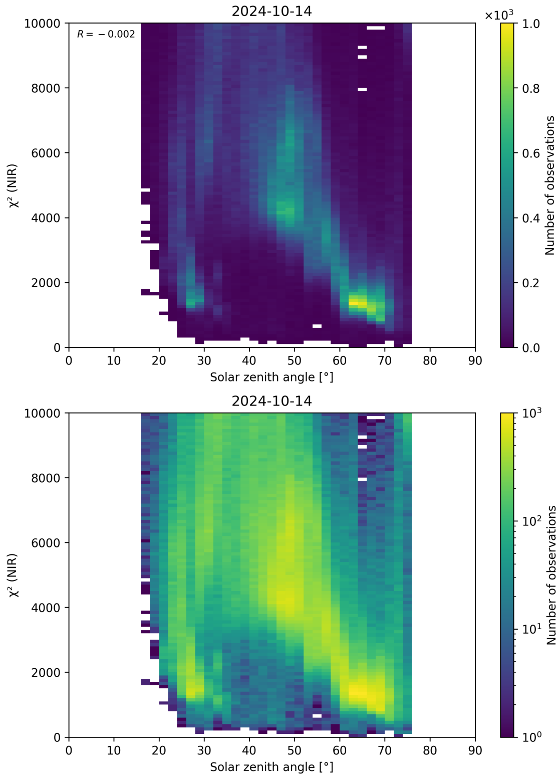
Figure 94: Scatter density plot of “Solar zenith angle” against “ \chi^2 (NIR)” for 2024-10-14 to 2024-10-15.
