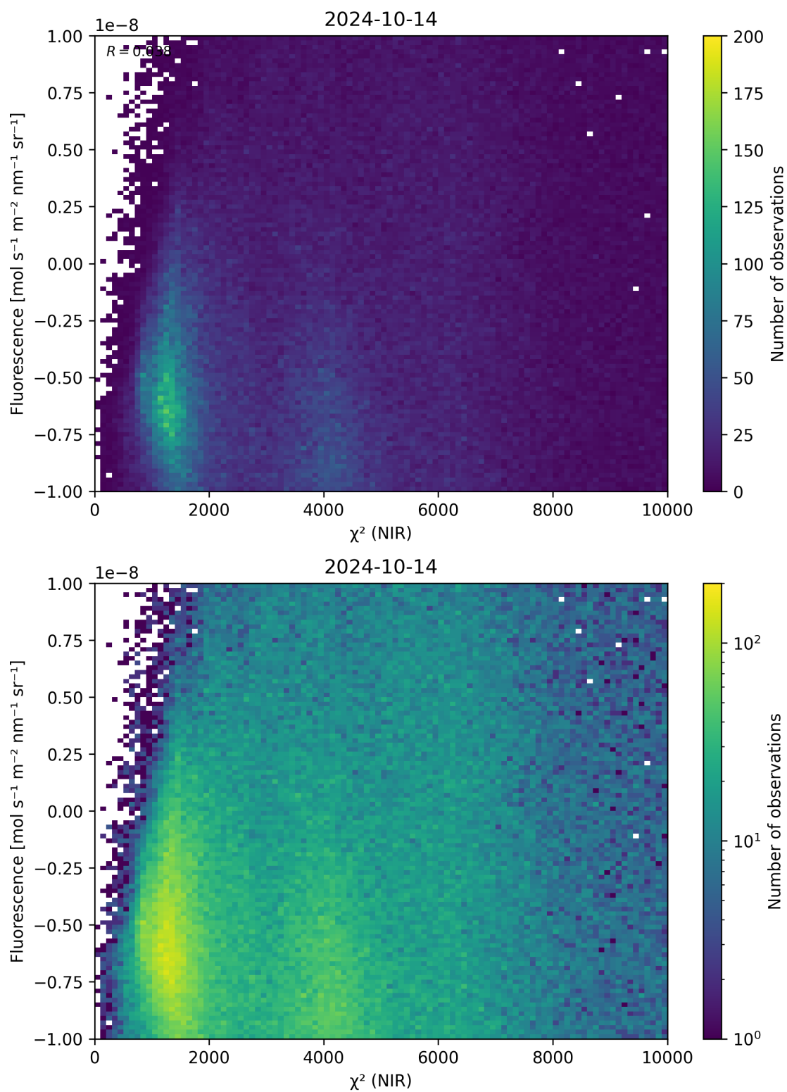
Figure 45: Scatter density plot of “ \chi^2 (NIR)” against “Fluorescence” for 2024-10-14 to 2024-10-15.
