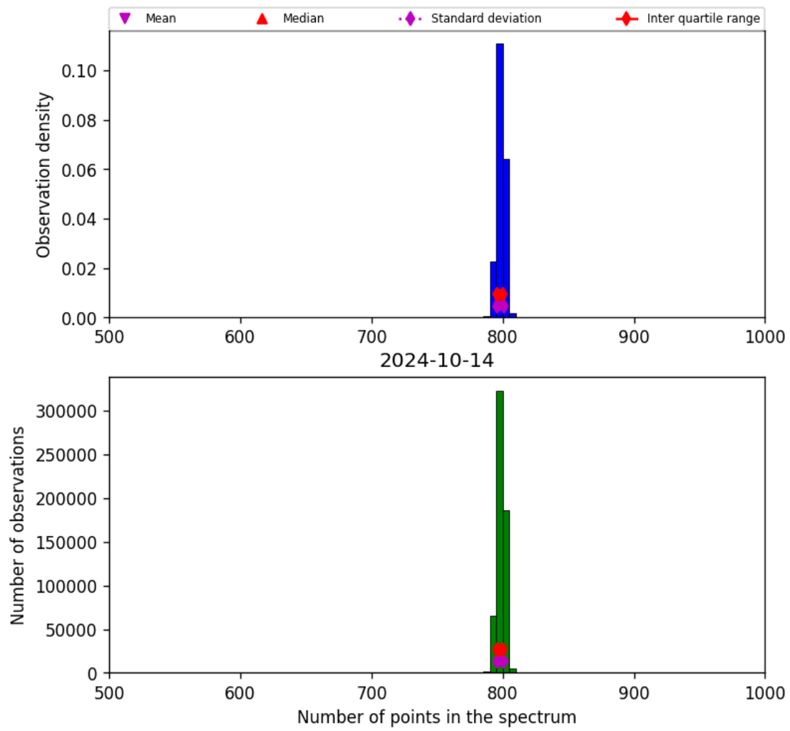
Figure 26: Histogram of “Number of points in the spectrum” for 2024-10-14 to 2024-10-15
