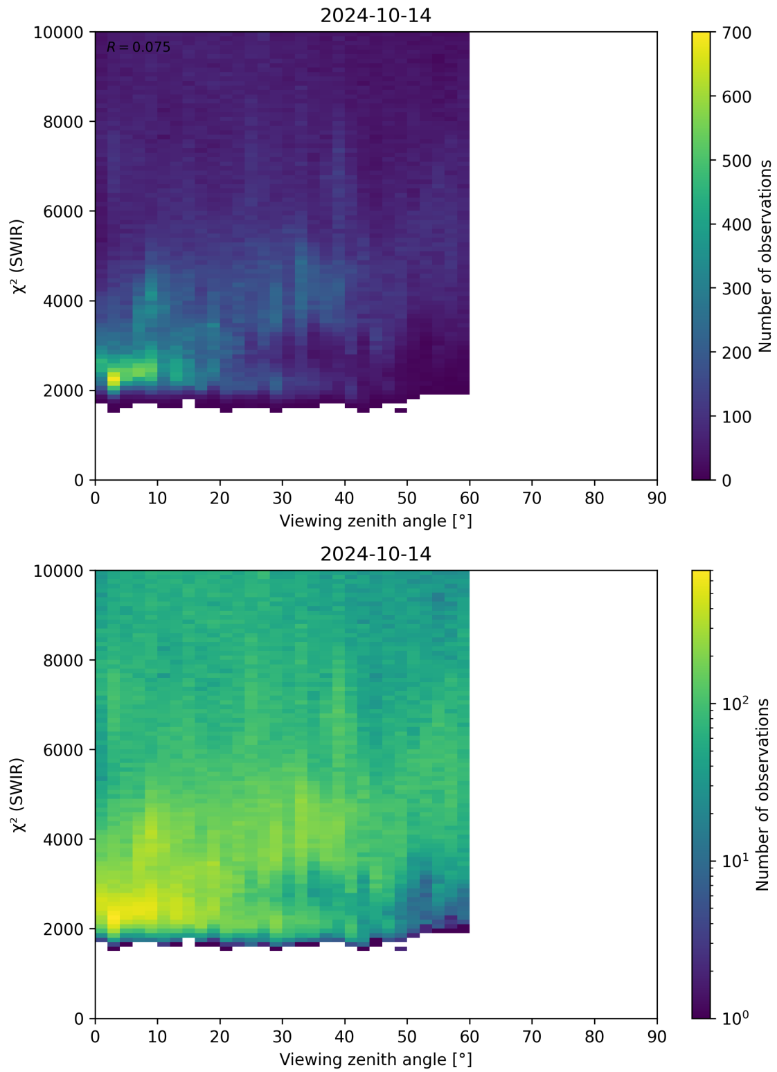
Figure 106: Scatter density plot of “Viewing zenith angle” against “ \chi^2 (SWIR)” for 2024-10-14 to 2024-10-15.
