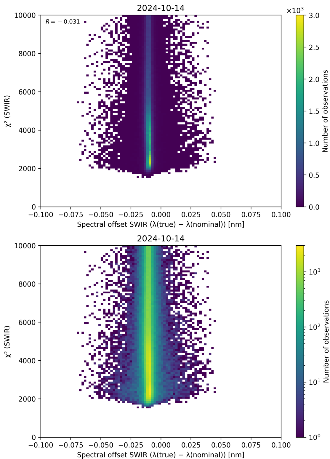
Figure 118: Scatter density plot of “Spectral offset SWIR ( \lambda_{\text{true}} - \lambda_{\text{nominal}} )” against “ \chi^2 (SWIR)” for 2024-10-14 to 2024-10-15.
