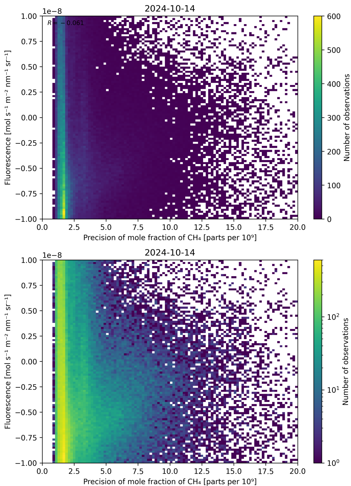
Figure 81: Scatter density plot of “Precision of mole fraction of \text{CH}_4 ” against “Fluorescence” for 2024-10-14 to 2024-10-15.
