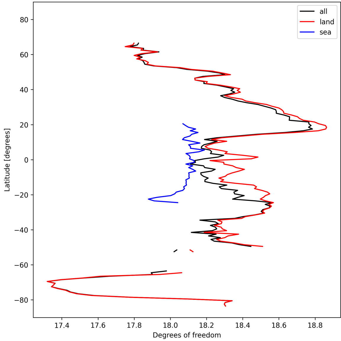
Figure 19: Zonal average of “Degrees of freedom” for 2024-10-14 to 2024-10-15.
