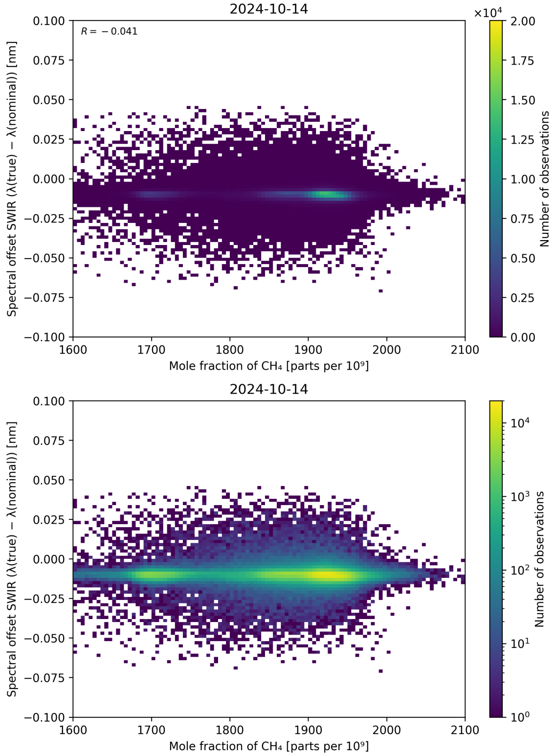
Figure 86: Scatter density plot of “Mole fraction of CH 4 ” against “Spectral offset SWIR ( \lambda_{\text{true}} - \lambda_{\text{nominal}} )” for 2024-10-14 to 2024-10-15.
