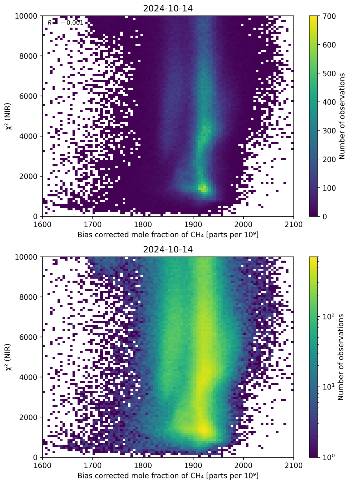
Figure 63: Scatter density plot of “Bias corrected mole fraction of CH 4 ” against “ \chi^2 (NIR)” for 2024-10-14 to 2024-10-15.
