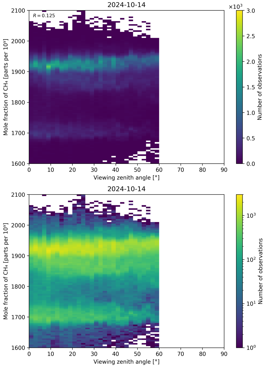
Figure 110: Scatter density plot of “Viewing zenith angle” against “Mole fraction of CH 4 ” for 2024-10-14 to 2024-10-15.
