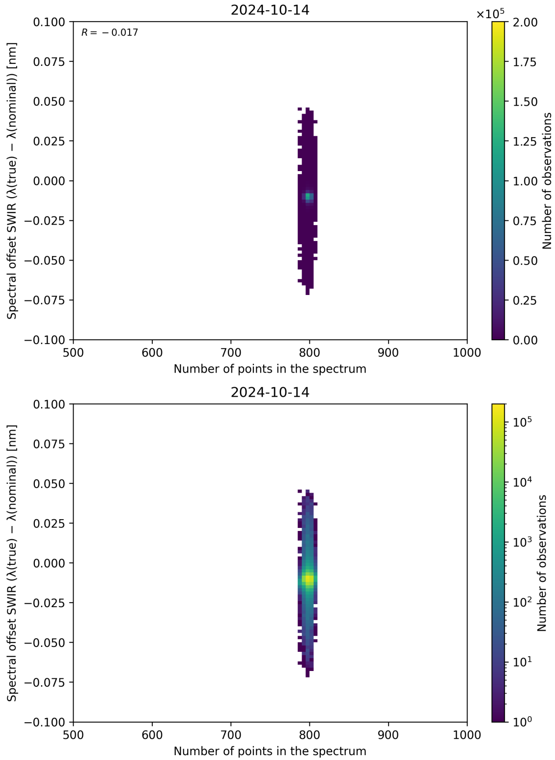
Figure 93: Scatter density plot of “Number of points in the spectrum” against “Spectral offset SWIR ( \lambda_{\text{true}} - \lambda_{\text{nominal}} )” for 2024-10-14 to 2024-10-15.
