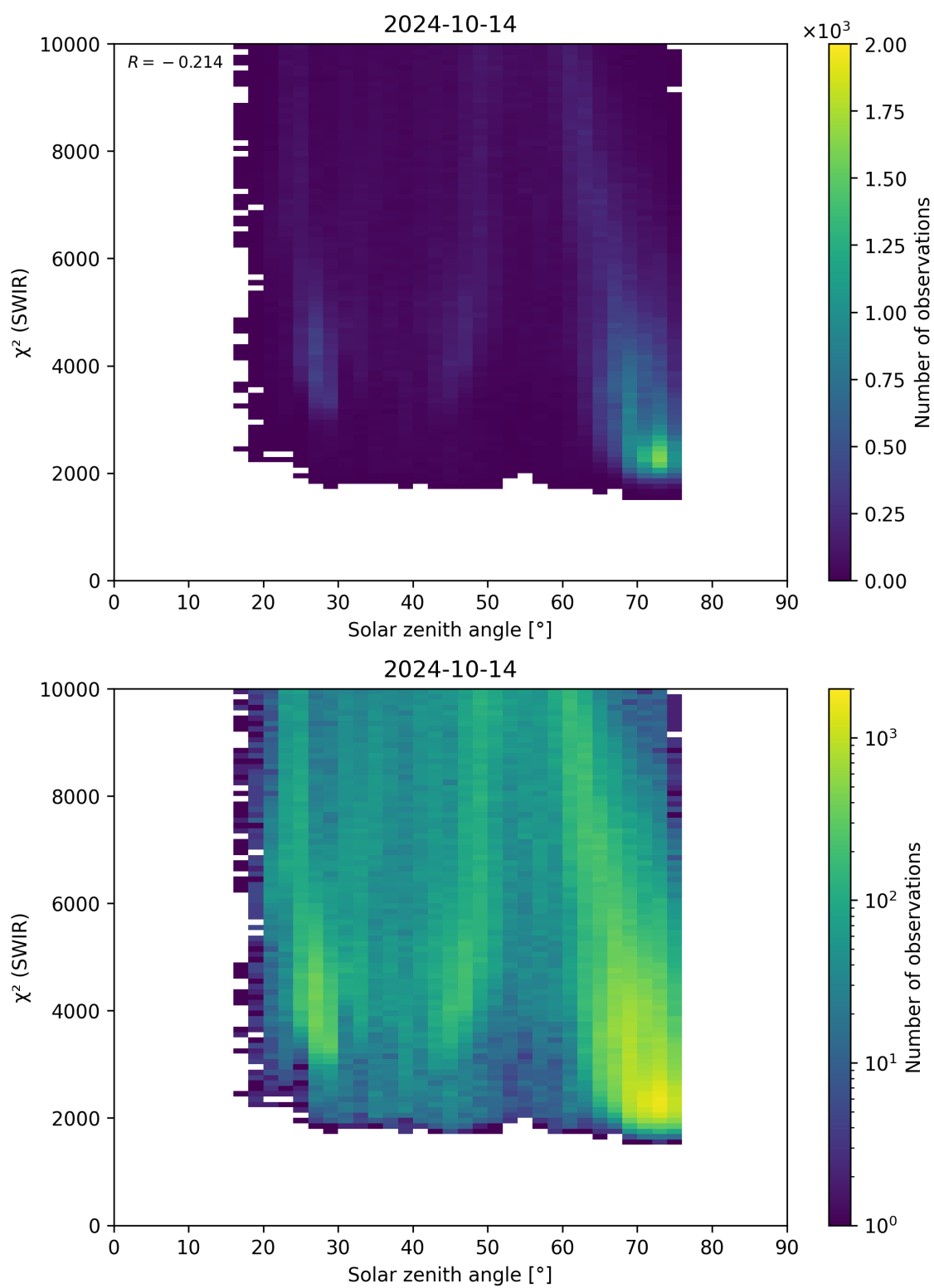
Figure 95: Scatter density plot of “Solar zenith angle” against “ \chi^2 (SWIR)” for 2024-10-14 to 2024-10-15.
