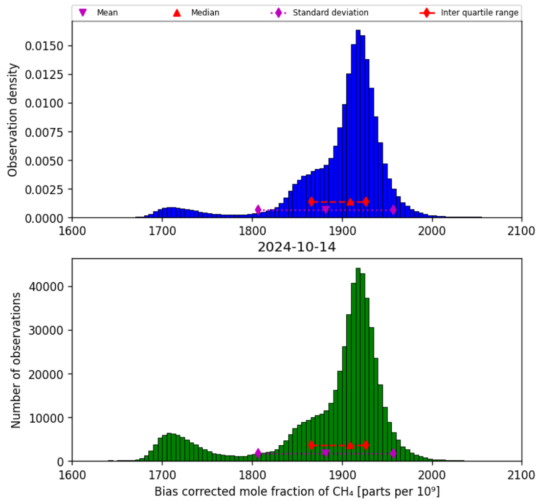
Figure 25: Histogram of “Bias corrected mole fraction of CH 4 ” for 2024-10-14 to 2024-10-15
