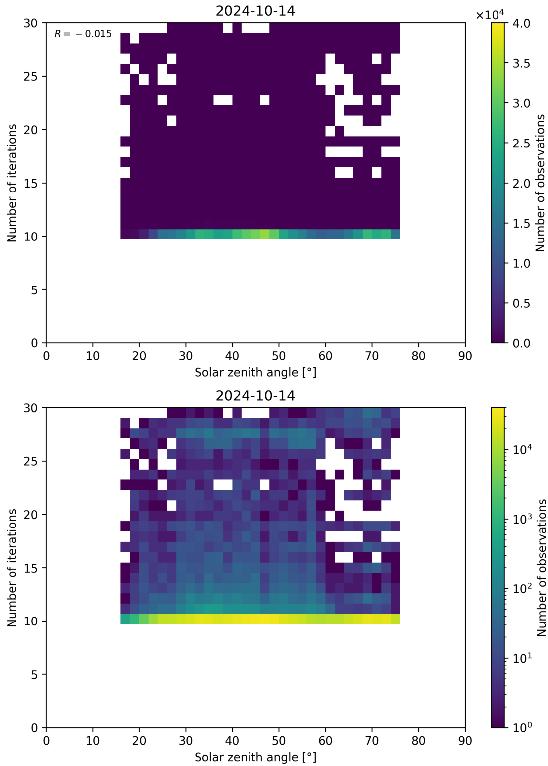
Figure 102: Scatter density plot of “Solar zenith angle” against “Number of iterations” for 2024-10-14 to 2024-10-15.
