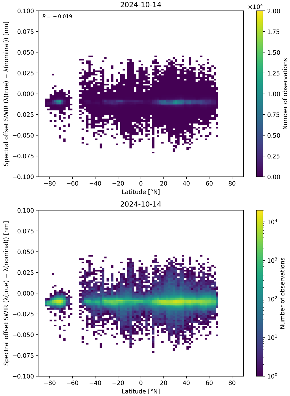
Figure 62: Scatter density plot of “Latitude” against “Spectral offset SWIR ( \lambda_{\text{true}} - \lambda_{\text{nominal}} )” for 2024-10-14 to 2024-10-15.
