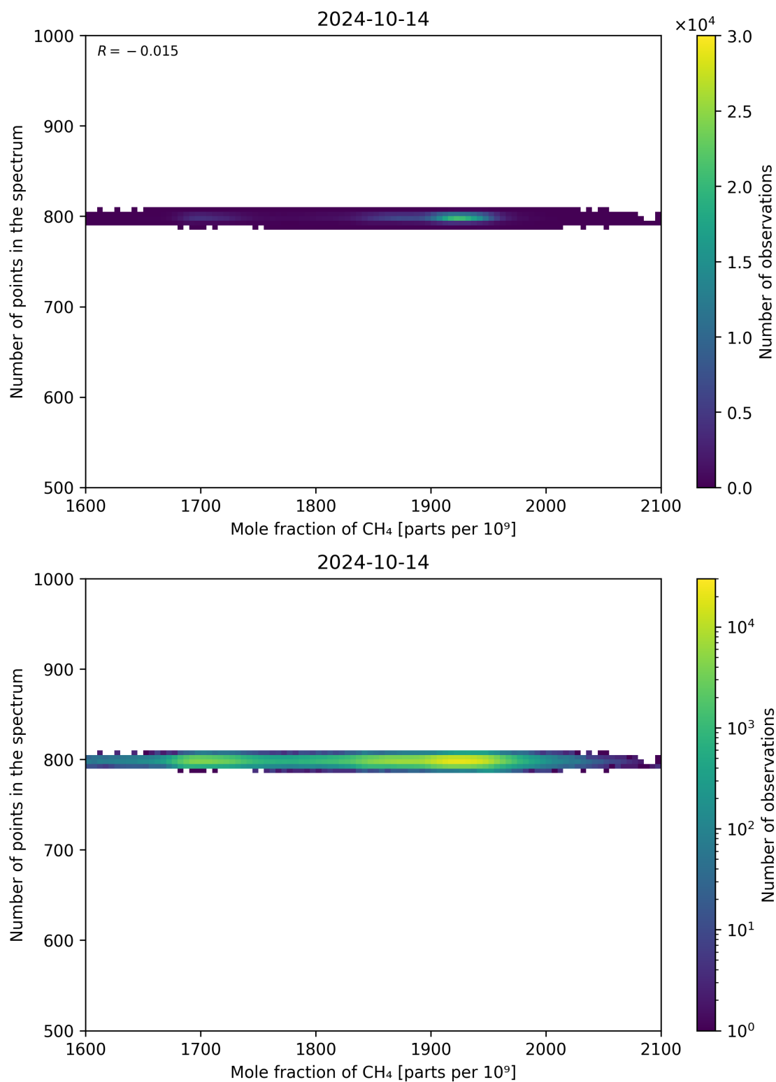
Figure 77: Scatter density plot of “Mole fraction of CH 4 ” against “Number of points in the spectrum” for 2024-10-14 to 2024-10-15.
