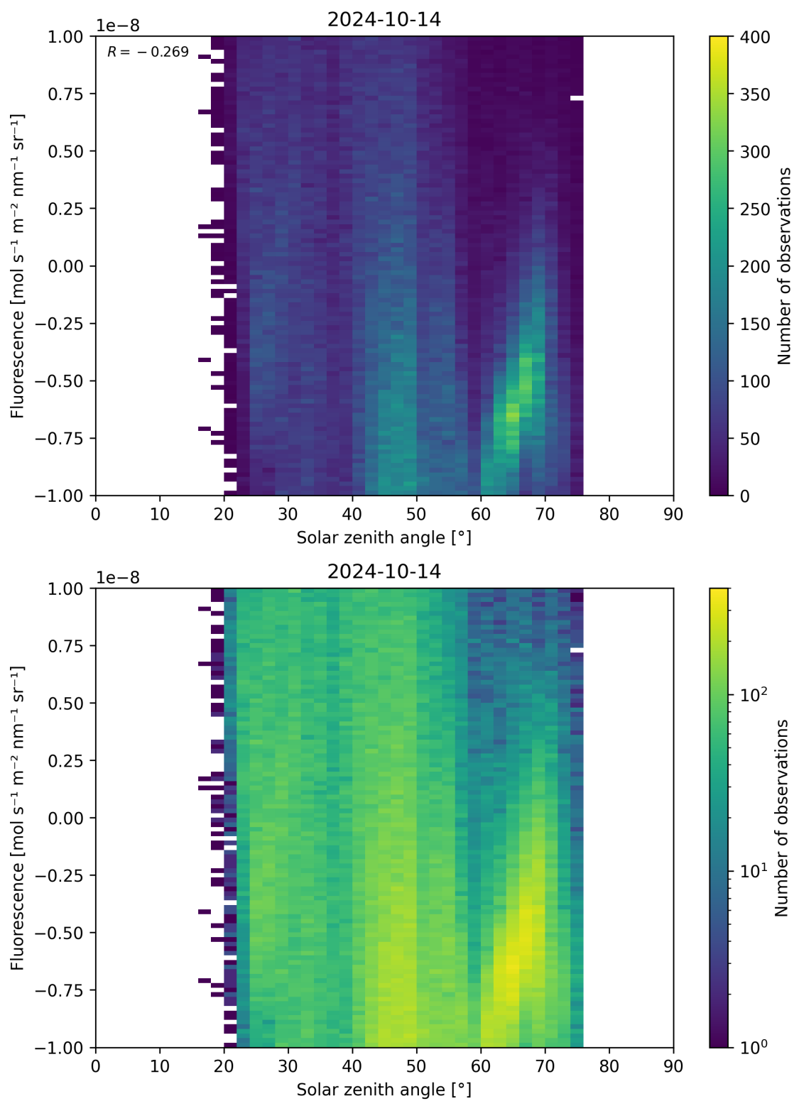
Figure 97: Scatter density plot of “Solar zenith angle” against “Fluorescence” for 2024-10-14 to 2024-10-15.
