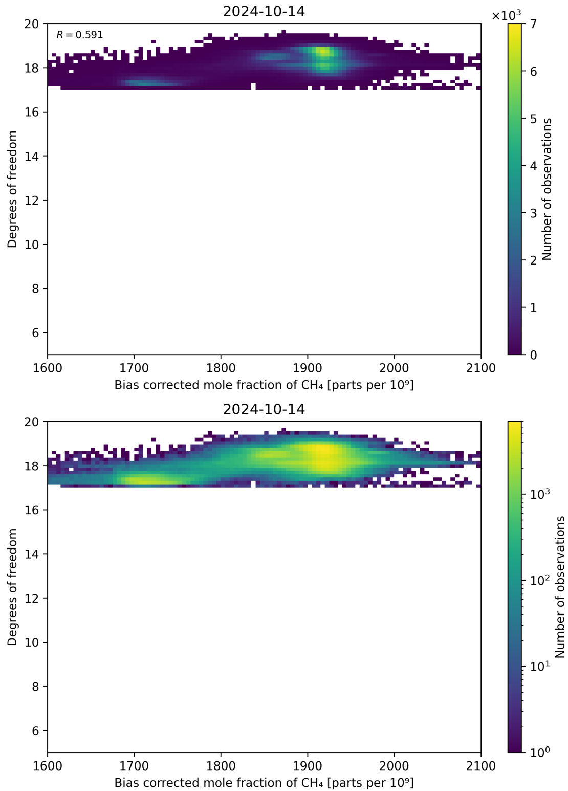
Figure 65: Scatter density plot of “Bias corrected mole fraction of CH 4 ” against “Degrees of freedom” for 2024-10-14 to 2024-10-15.
