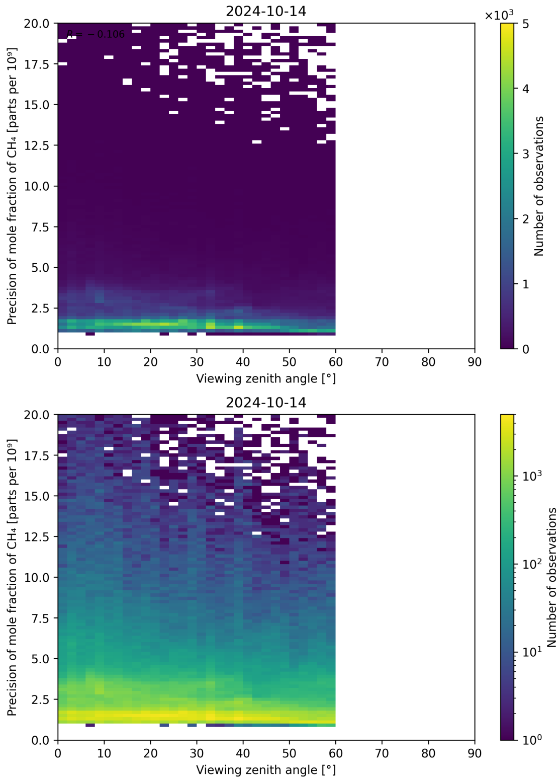
Figure 112: Scatter density plot of “Viewing zenith angle” against “Precision of mole fraction of CH 4 ” for 2024-10-14 to 2024-10-15.
