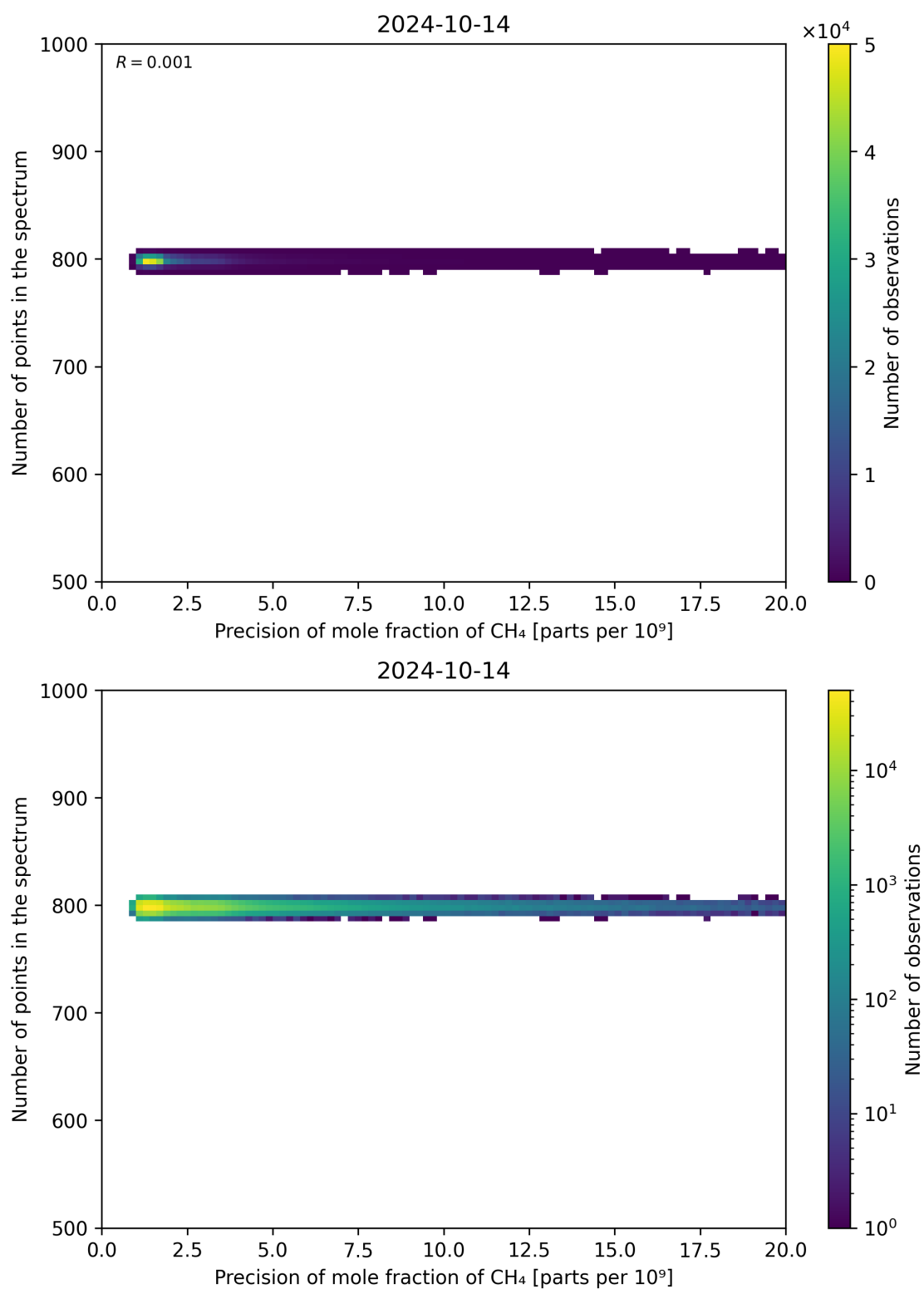
Figure 84: Scatter density plot of “Precision of mole fraction of CH 4 ” against “Number of points in the spectrum” for 2024-10-14 to 2024-10-15.
