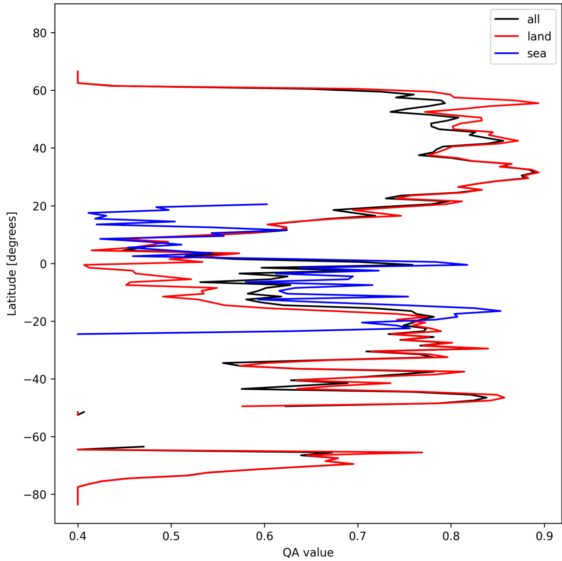
Figure 11: Zonal average of “QA value” for 2024-10-14 to 2024-10-15.
