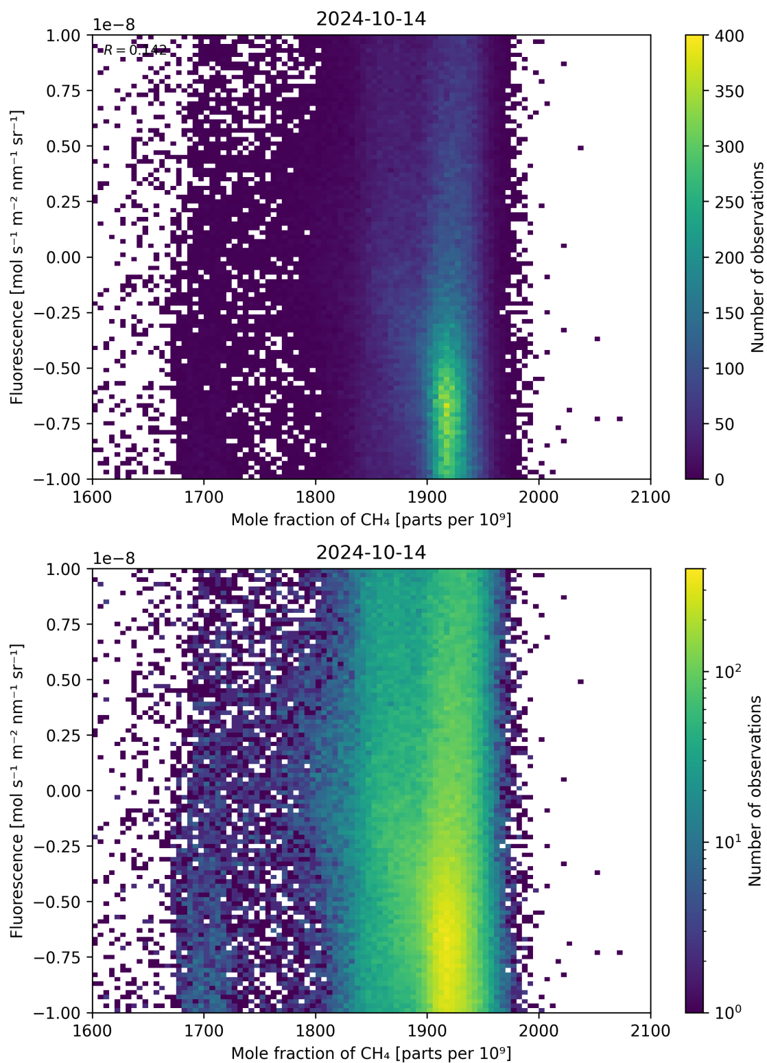
Figure 73: Scatter density plot of “Mole fraction of \text{CH}_4 ” against “Fluorescence” for 2024-10-14 to 2024-10-15.
