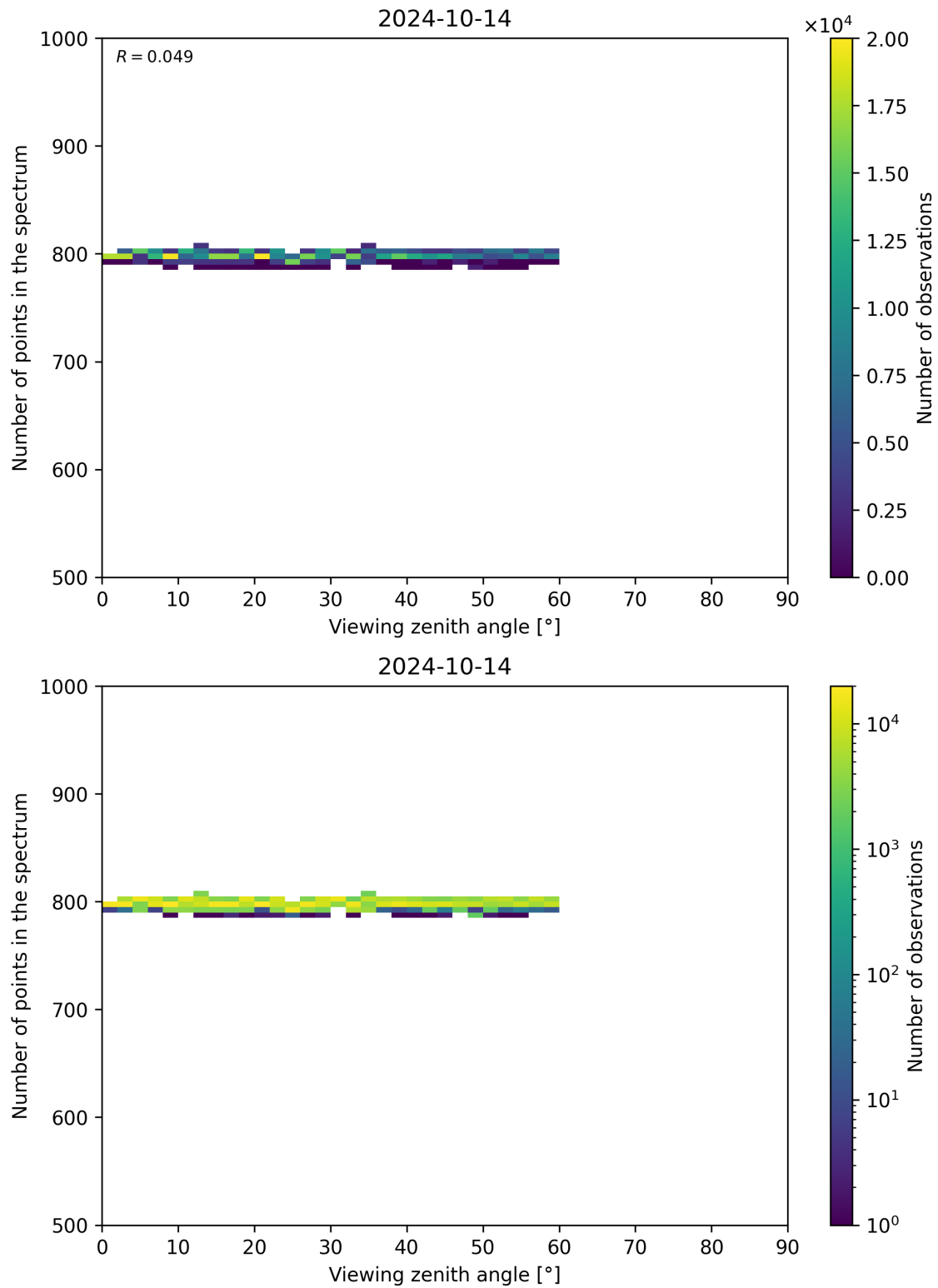
Figure 114: Scatter density plot of “Viewing zenith angle” against “Number of points in the spectrum” for 2024-10-14 to 2024-10-15.
