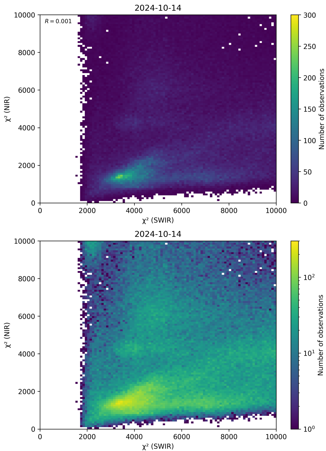
Figure 47: Scatter density plot of “ \chi^2 (SWIR)” against “ \chi^2 (NIR)” for 2024-10-14 to 2024-10-15.
