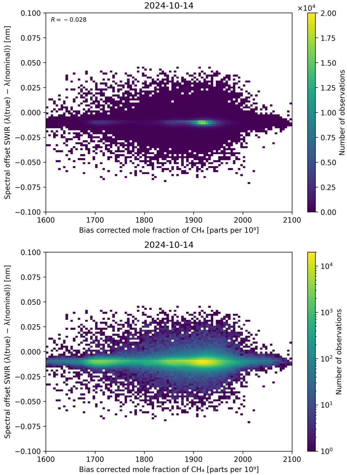
Figure 69: Scatter density plot of “Bias corrected mole fraction of \text{CH}_4 ” against “Spectral offset SWIR ( \lambda_{\text{true}} - \lambda_{\text{nominal}} )” for 2024-10-14 to 2024-10-15.
