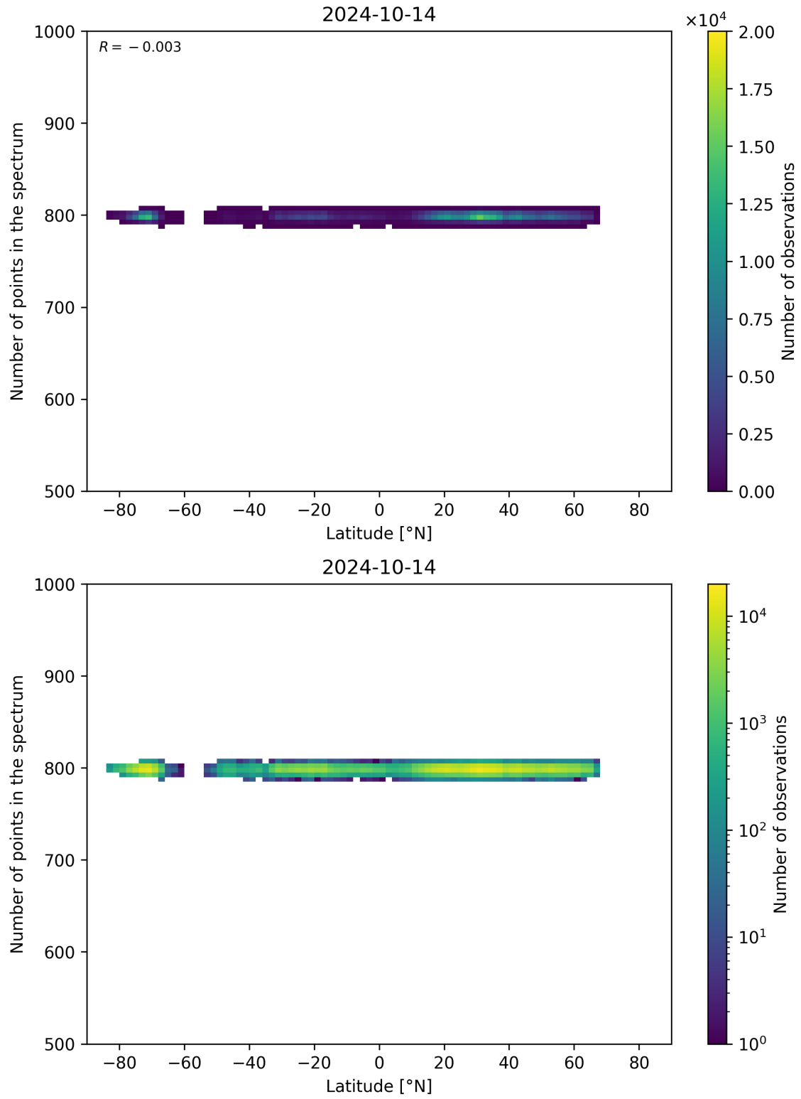
Figure 61: Scatter density plot of “Latitude” against “Number of points in the spectrum” for 2024-10-14 to 2024-10-15.
