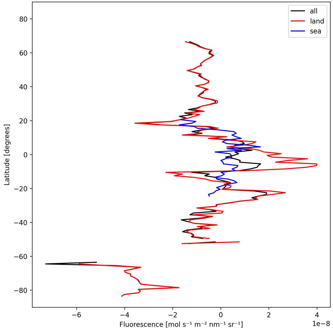
Figure 21: Zonal average of “Fluorescence” for 2024-10-14 to 2024-10-15.
