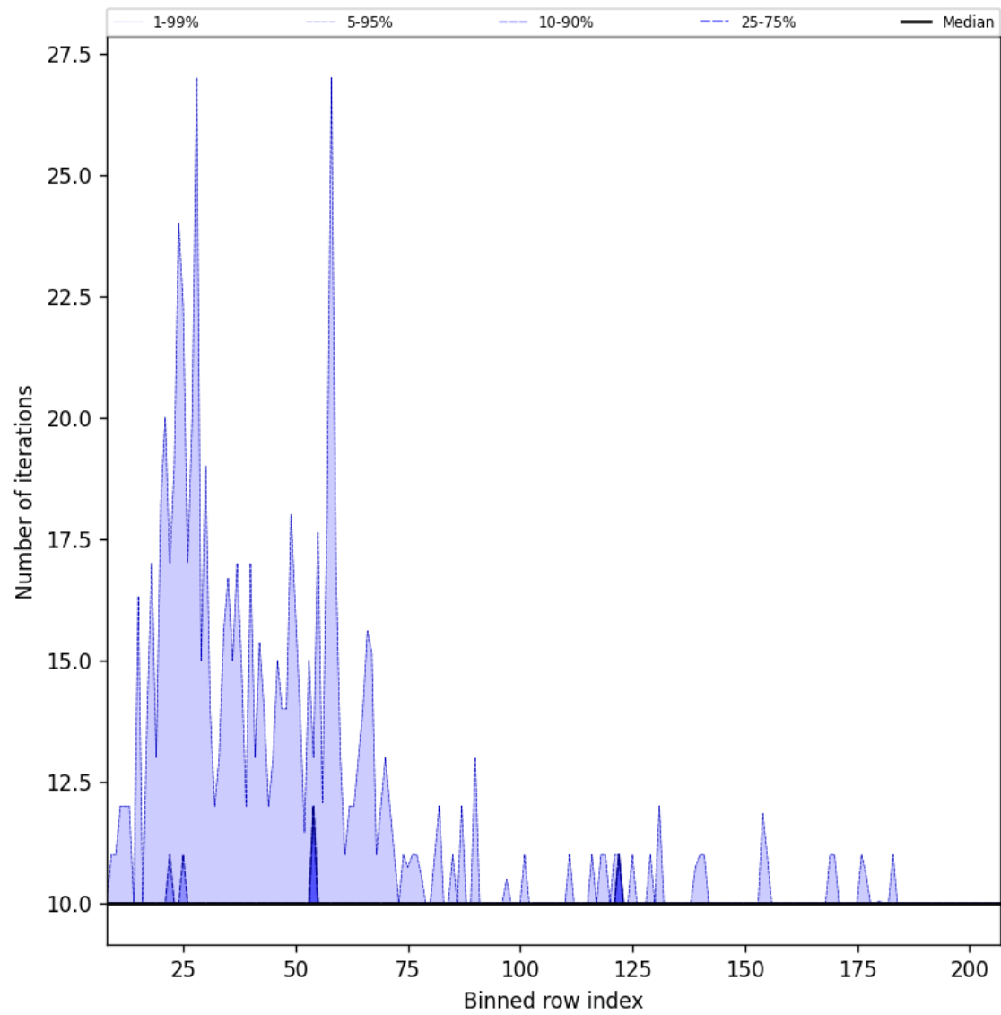
Figure 42: Along track statistics of “Number of iterations” for 2024-10-14 to 2024-10-15
