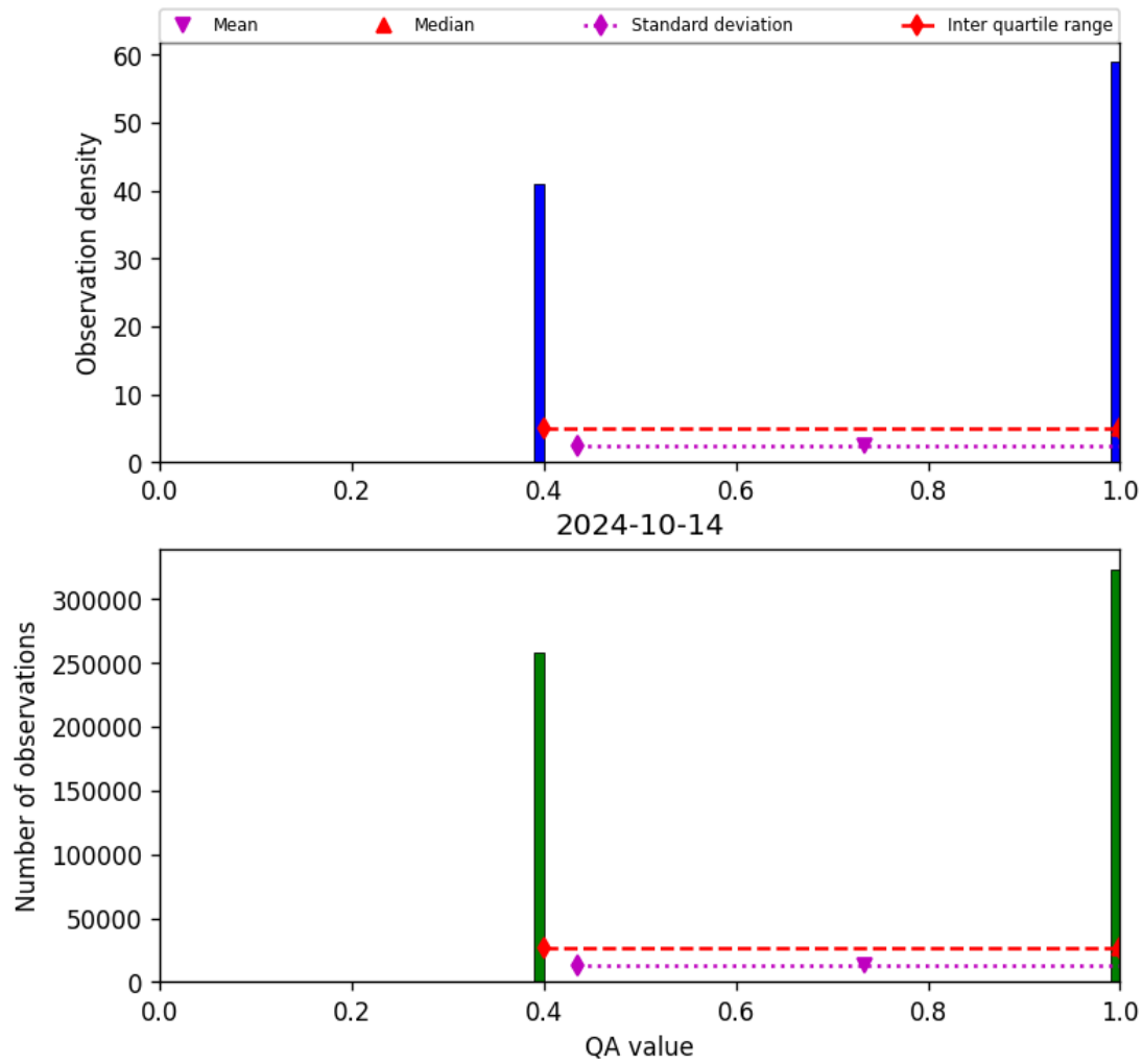
Figure 22: Histogram of “QA value” for 2024-10-14 to 2024-10-15
