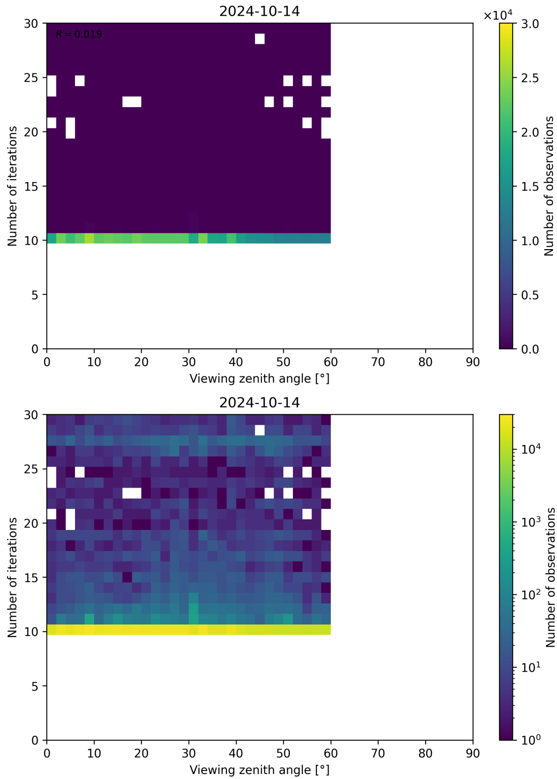
Figure 113: Scatter density plot of “Viewing zenith angle” against “Number of iterations” for 2024-10-14 to 2024-10-15.
