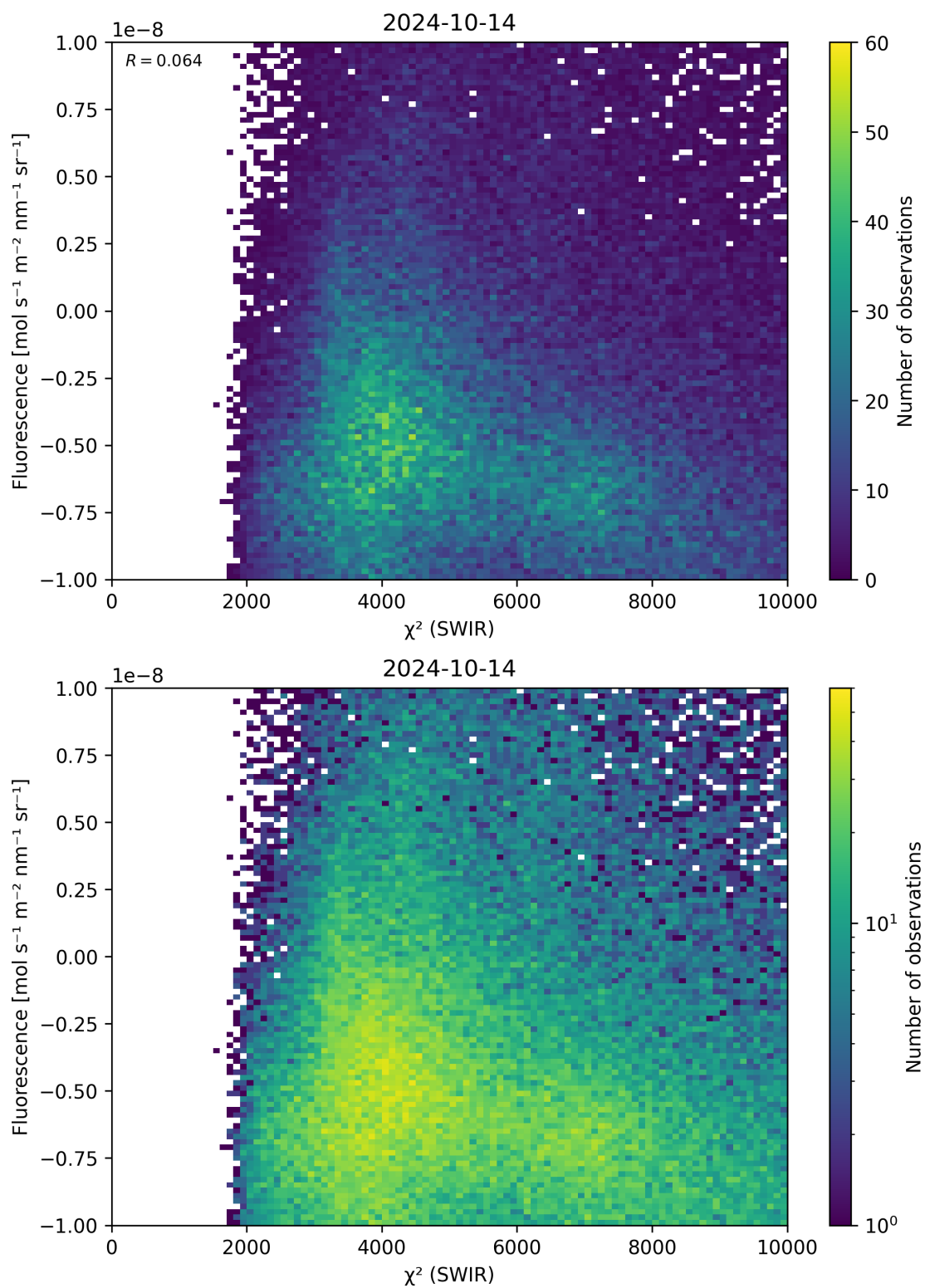
Figure 49: Scatter density plot of “ \chi^2 (SWIR)” against “Fluorescence” for 2024-10-14 to 2024-10-15.
