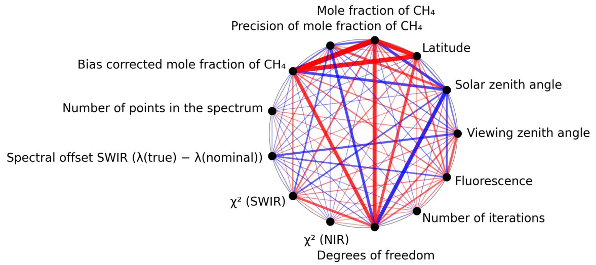
Figure 1: Map of correlation graph for 2024-10-14 to 2024-10-15.
