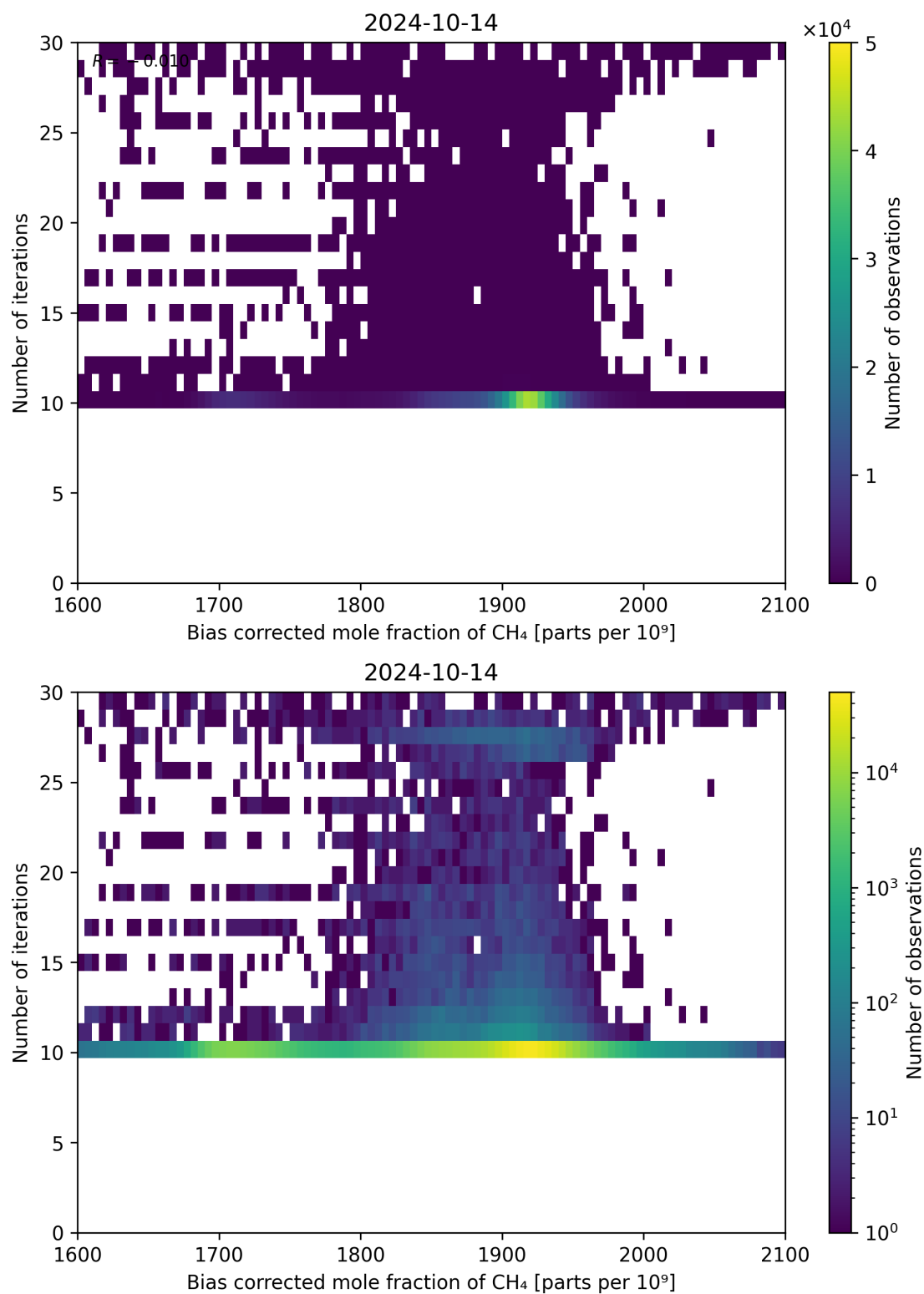
Figure 67: Scatter density plot of “Bias corrected mole fraction of CH 4 ” against “Number of iterations” for 2024-10-14 to 2024-10-15.
