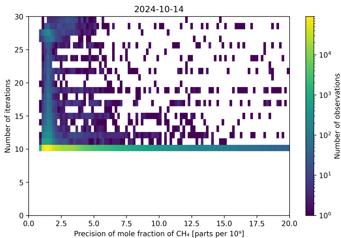
Figure 83: Scatter density plot of “Precision of mole fraction of \text{CH}_4 ” against “Number of iterations” for 2024-10-14 to 2024-10-15.
