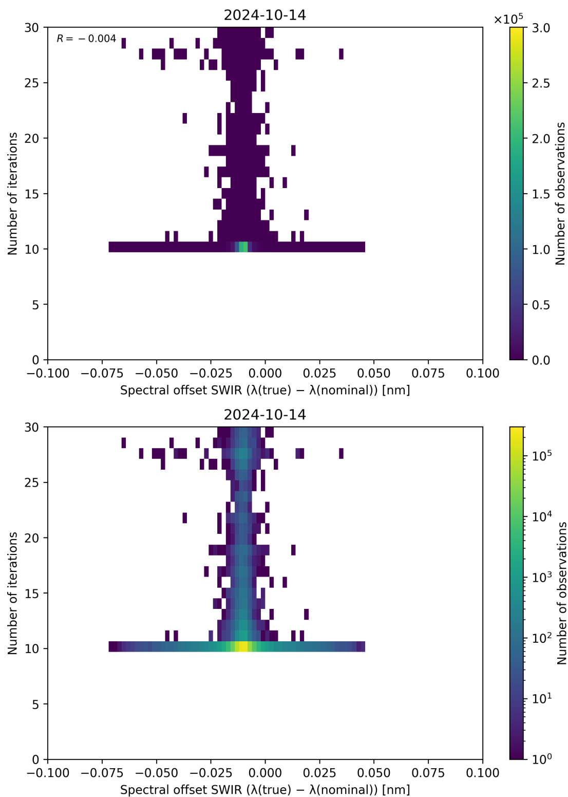
Figure 121: Scatter density plot of “Spectral offset SWIR ( \lambda_{\text{true}} - \lambda_{\text{nominal}} )” against “Number of iterations” for 2024-10-14 to 2024-10-15.
