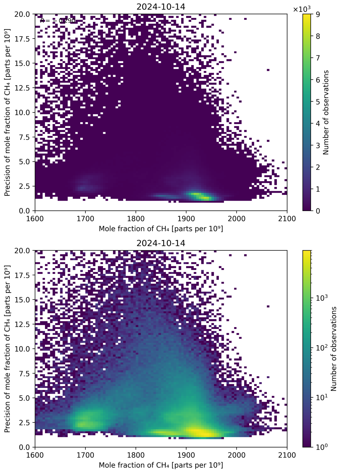
Figure 75: Scatter density plot of “Mole fraction of CH 4 ” against “Precision of mole fraction of CH 4 ” for 2024-10-14 to 2024-10-15.
