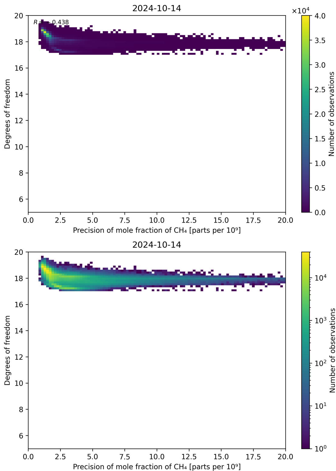
Figure 80: Scatter density plot of “Precision of mole fraction of CH 4 ” against “Degrees of freedom” for 2024-10-14 to 2024-10-15.
