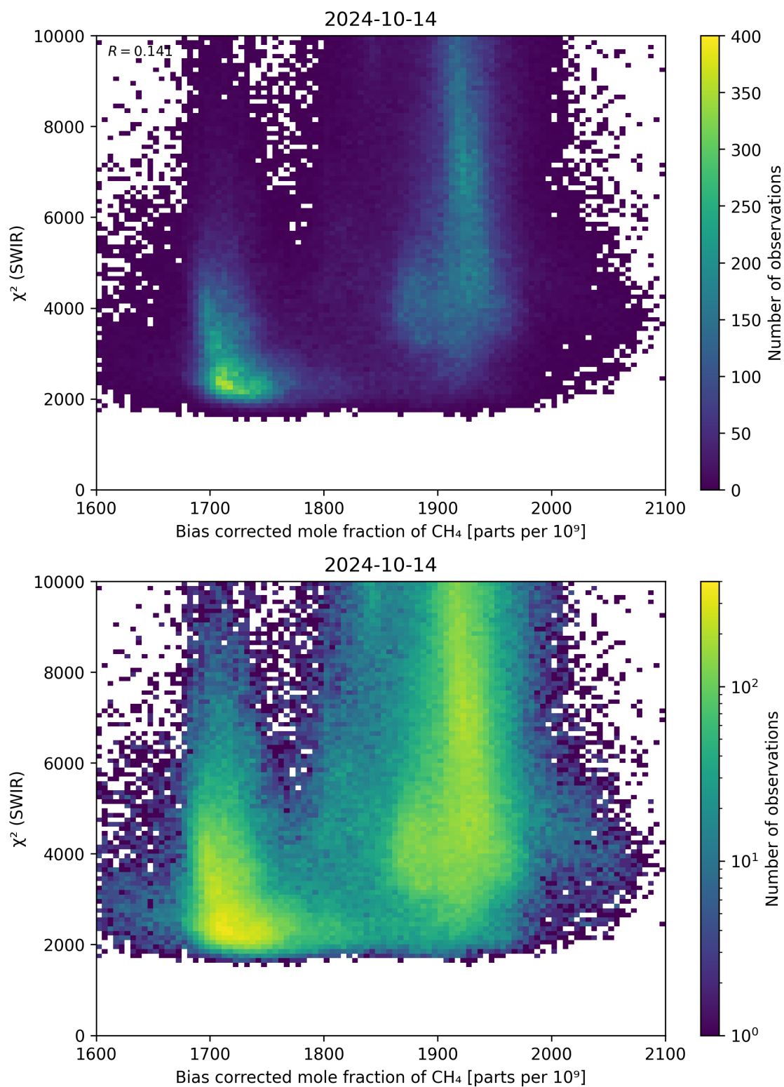
Figure 64: Scatter density plot of “Bias corrected mole fraction of \text{CH}_4 ” against “ \chi^2 (SWIR)” for 2024-10-14 to 2024-10-15.
