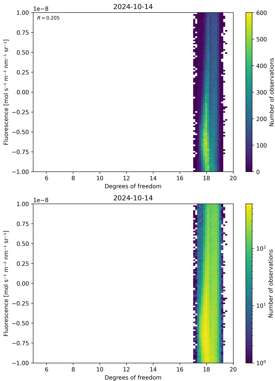
Figure 51: Scatter density plot of “Degrees of freedom” against “Fluorescence” for 2024-10-14 to 2024-10-15.
