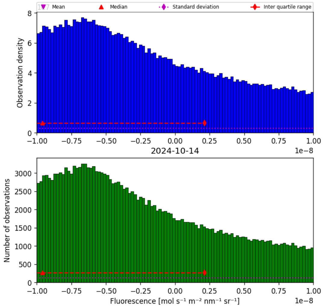
Figure 32: Histogram of “Fluorescence” for 2024-10-14 to 2024-10-15
