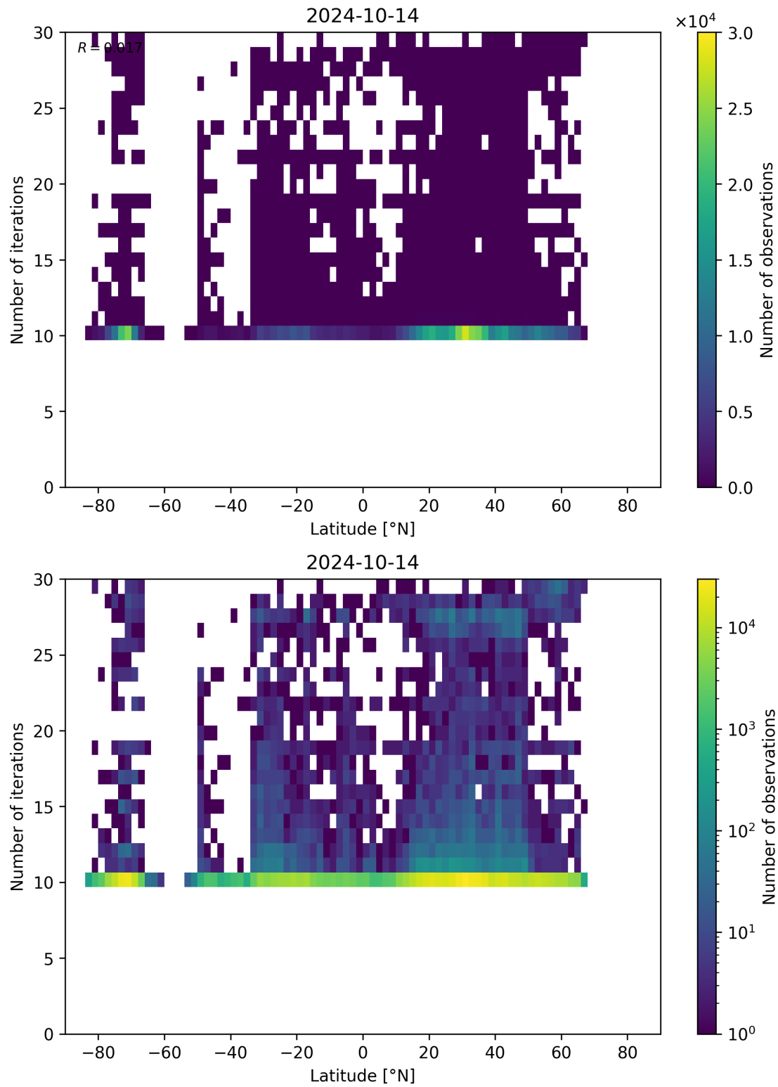
Figure 60: Scatter density plot of “Latitude” against “Number of iterations” for 2024-10-14 to 2024-10-15.
