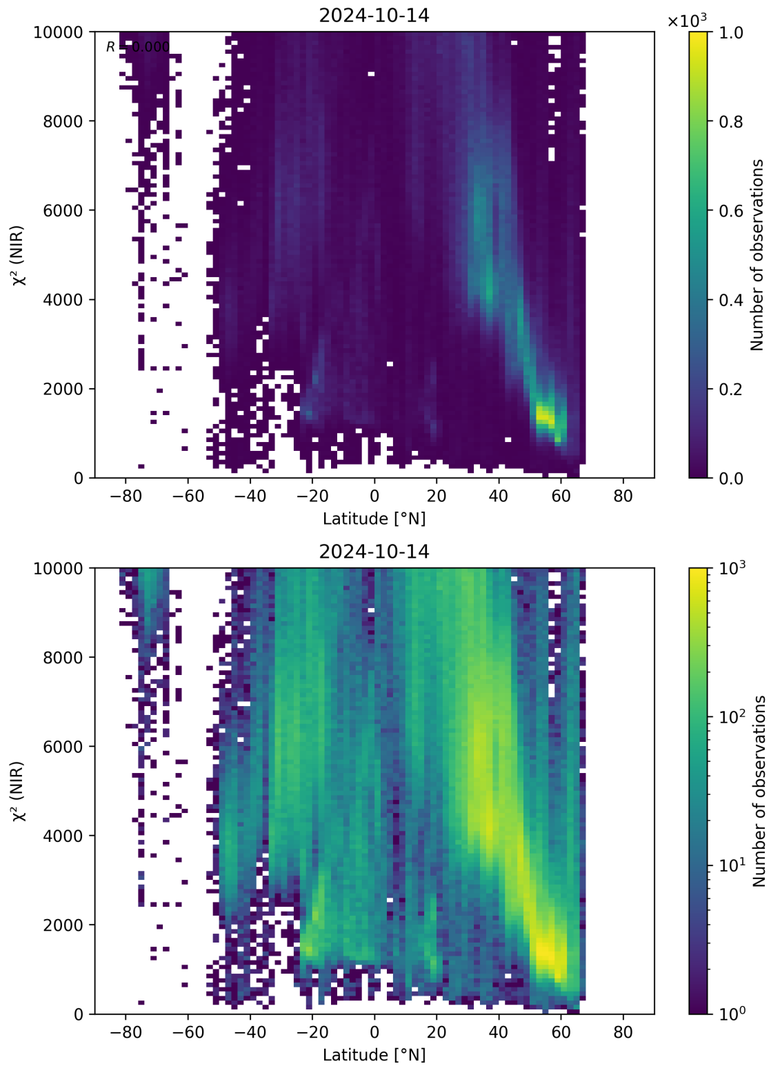
Figure 53: Scatter density plot of “Latitude” against “ \chi^2 (NIR)” for 2024-10-14 to 2024-10-15.
