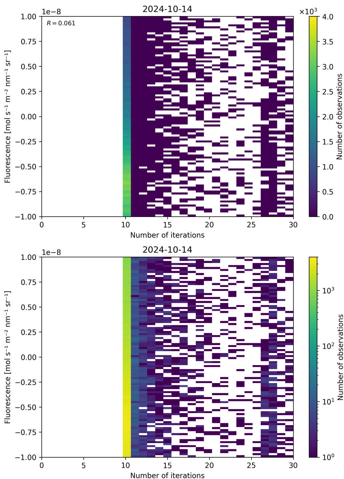
Figure 87: Scatter density plot of “Number of iterations” against “Fluorescence” for 2024-10-14 to 2024-10-15.
