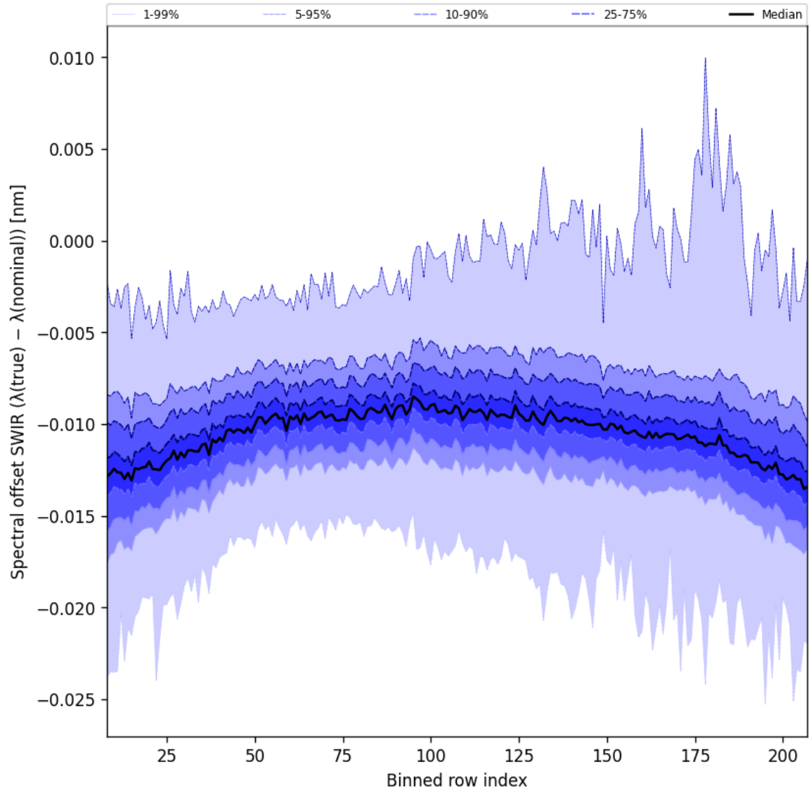
Figure 38: Along track statistics of “Spectral offset SWIR ( \lambda_{\text{true}} - \lambda_{\text{nominal}} )” for 2024-10-14 to 2024-10-15
