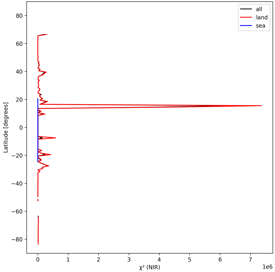
Figure 18: Zonal average of “ \chi^2 (NIR)” for 2024-10-14 to 2024-10-15.
