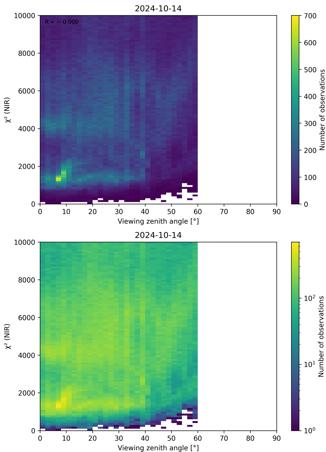
Figure 105: Scatter density plot of “Viewing zenith angle” against “ \chi^2 (NIR)” for 2024-10-14 to 2024-10-15.
