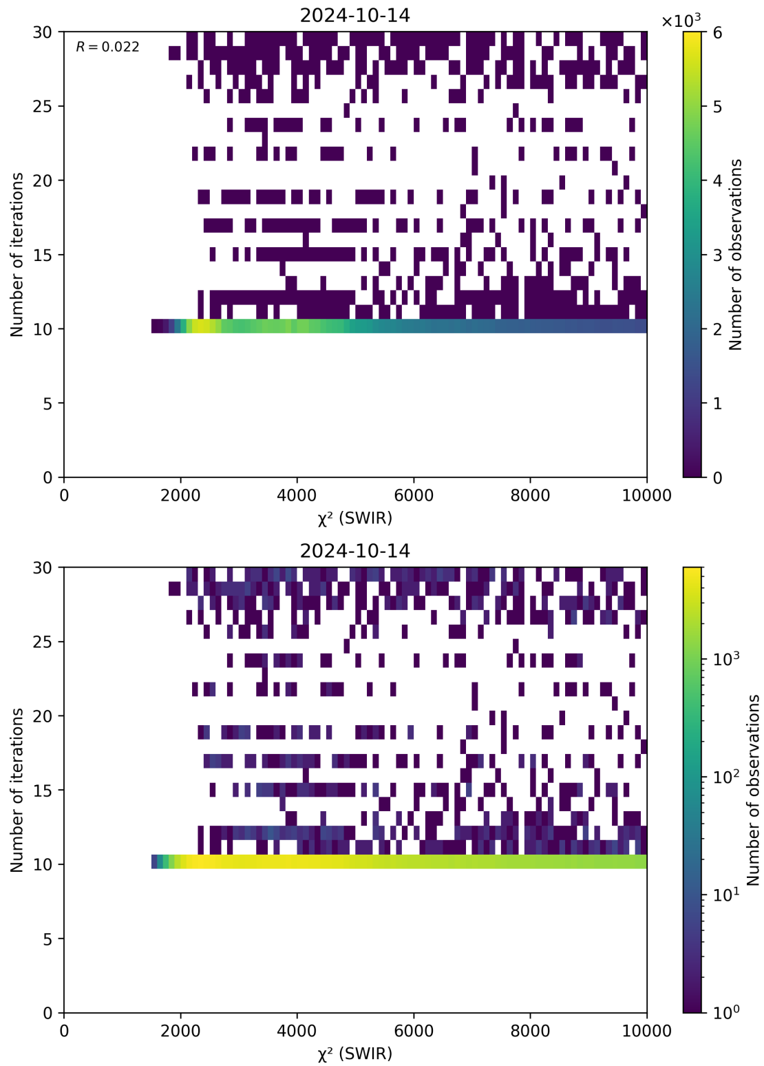
Figure 50: Scatter density plot of “ \chi^2 (SWIR)” against “Number of iterations” for 2024-10-14 to 2024-10-15.
