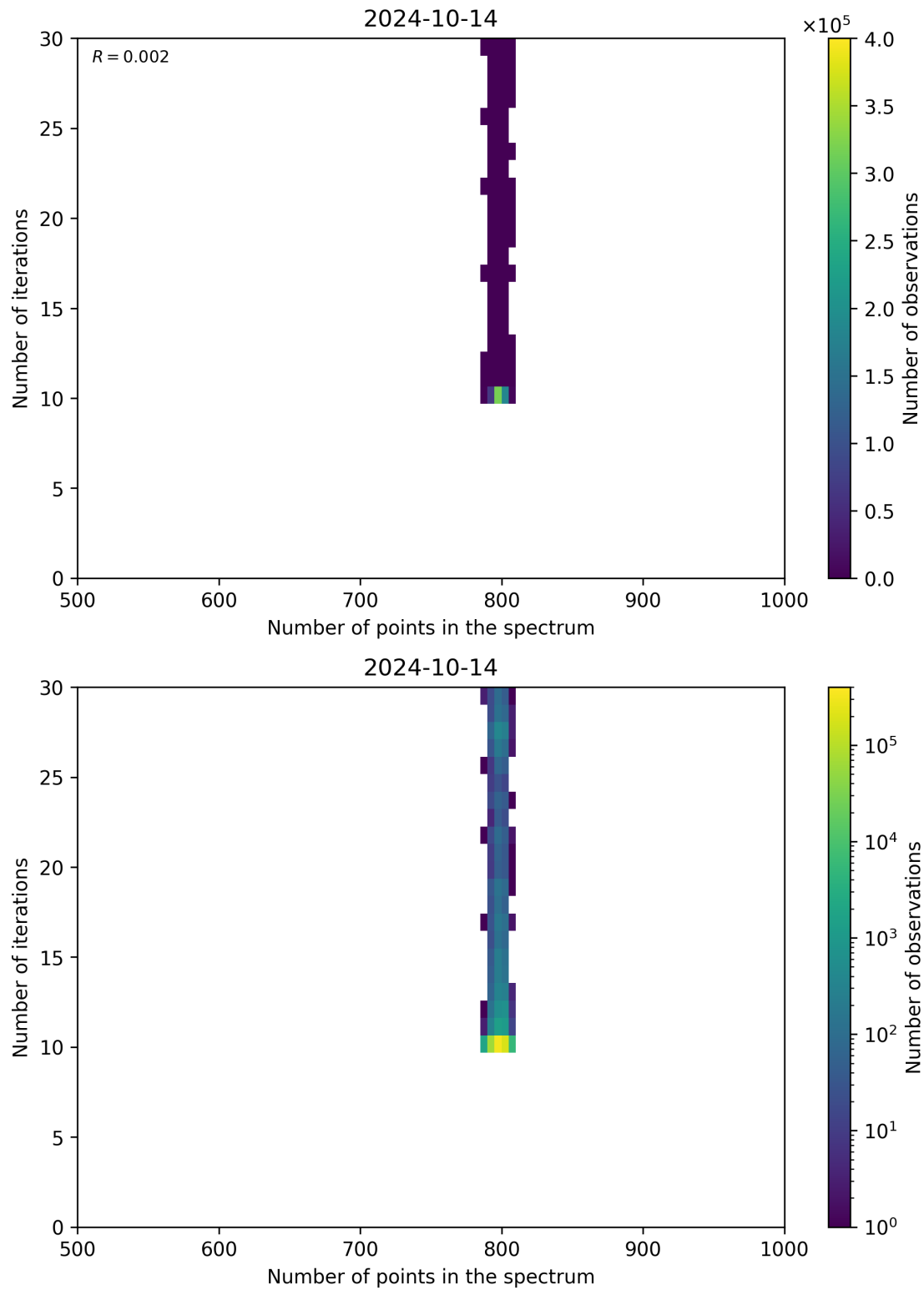
Figure 92: Scatter density plot of “Number of points in the spectrum” against “Number of iterations” for 2024-10-14 to 2024-10-15.
