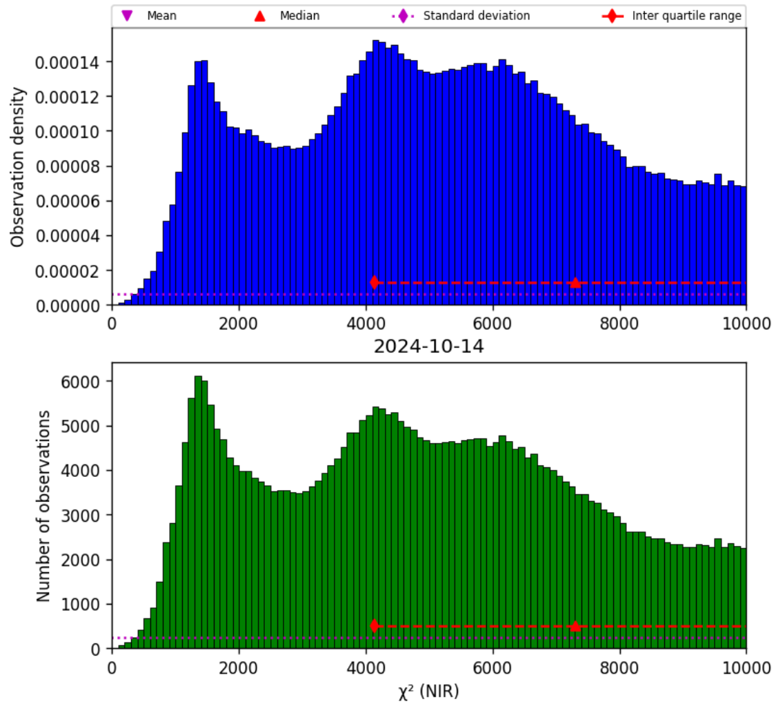
Figure 29: Histogram of “ \chi^2 (NIR)” for 2024-10-14 to 2024-10-15
