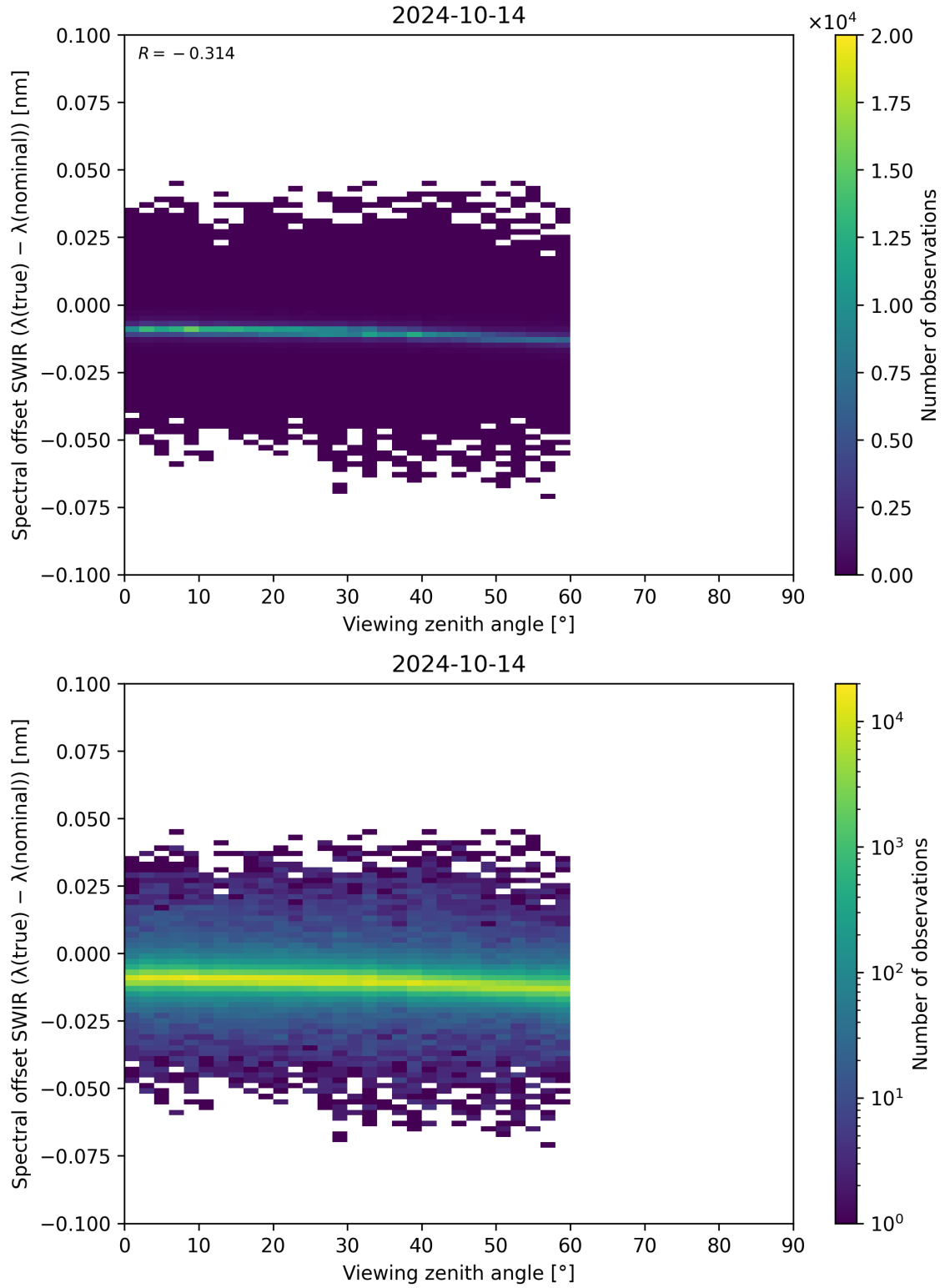
Figure 116: Scatter density plot of “Viewing zenith angle” against “Spectral offset SWIR ( \lambda_{\text{true}} - \lambda_{\text{nominal}} )” for 2024-10-14 to 2024-10-15.
