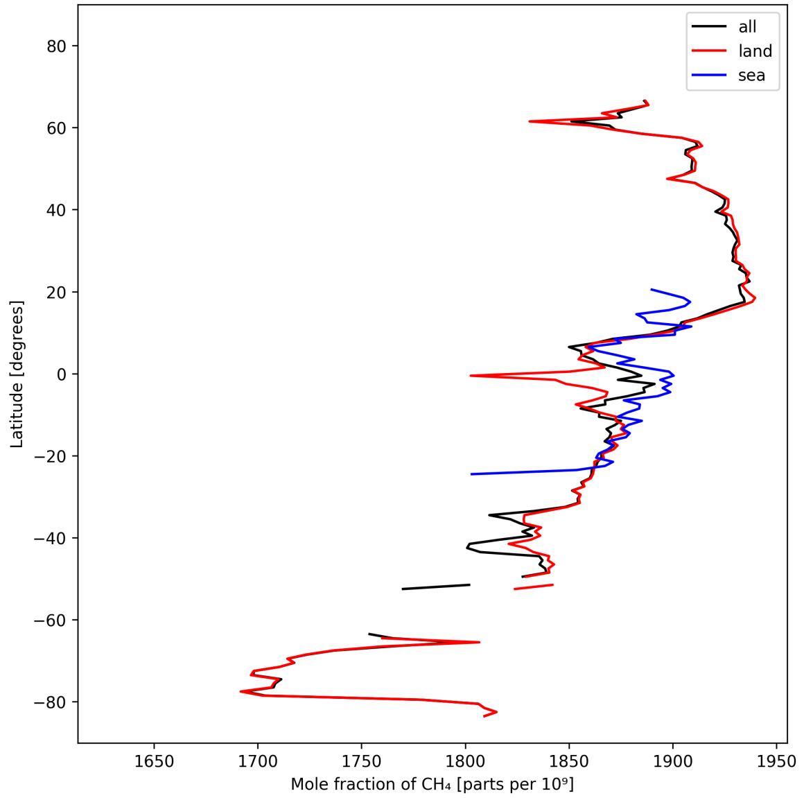
Figure 12: Zonal average of “Mole fraction of \text{CH}_4 ” for 2024-10-14 to 2024-10-15.
