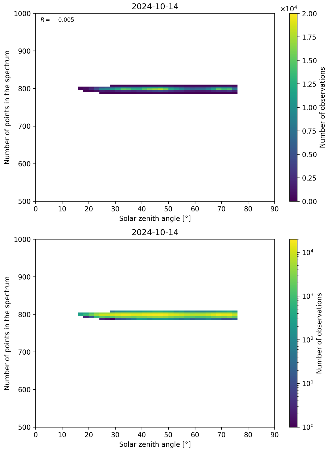
Figure 103: Scatter density plot of “Solar zenith angle” against “Number of points in the spectrum” for 2024-10-14 to 2024-10-15.
