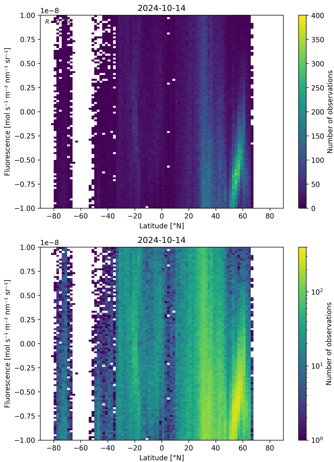
Figure 56: Scatter density plot of “Latitude” against “Fluorescence” for 2024-10-14 to 2024-10-15.
