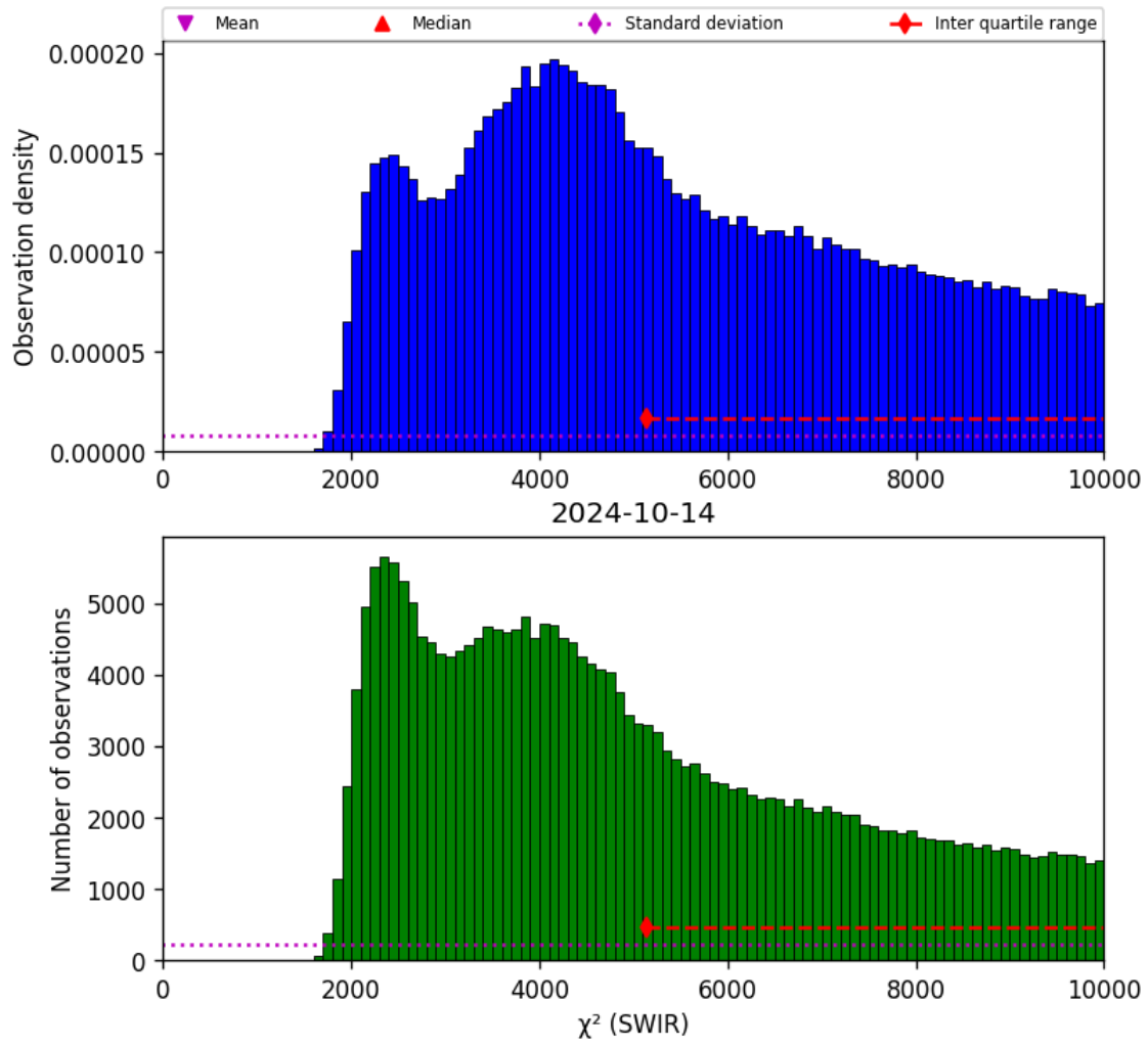
Figure 28: Histogram of “ \chi^2 (SWIR)” for 2024-10-14 to 2024-10-15
