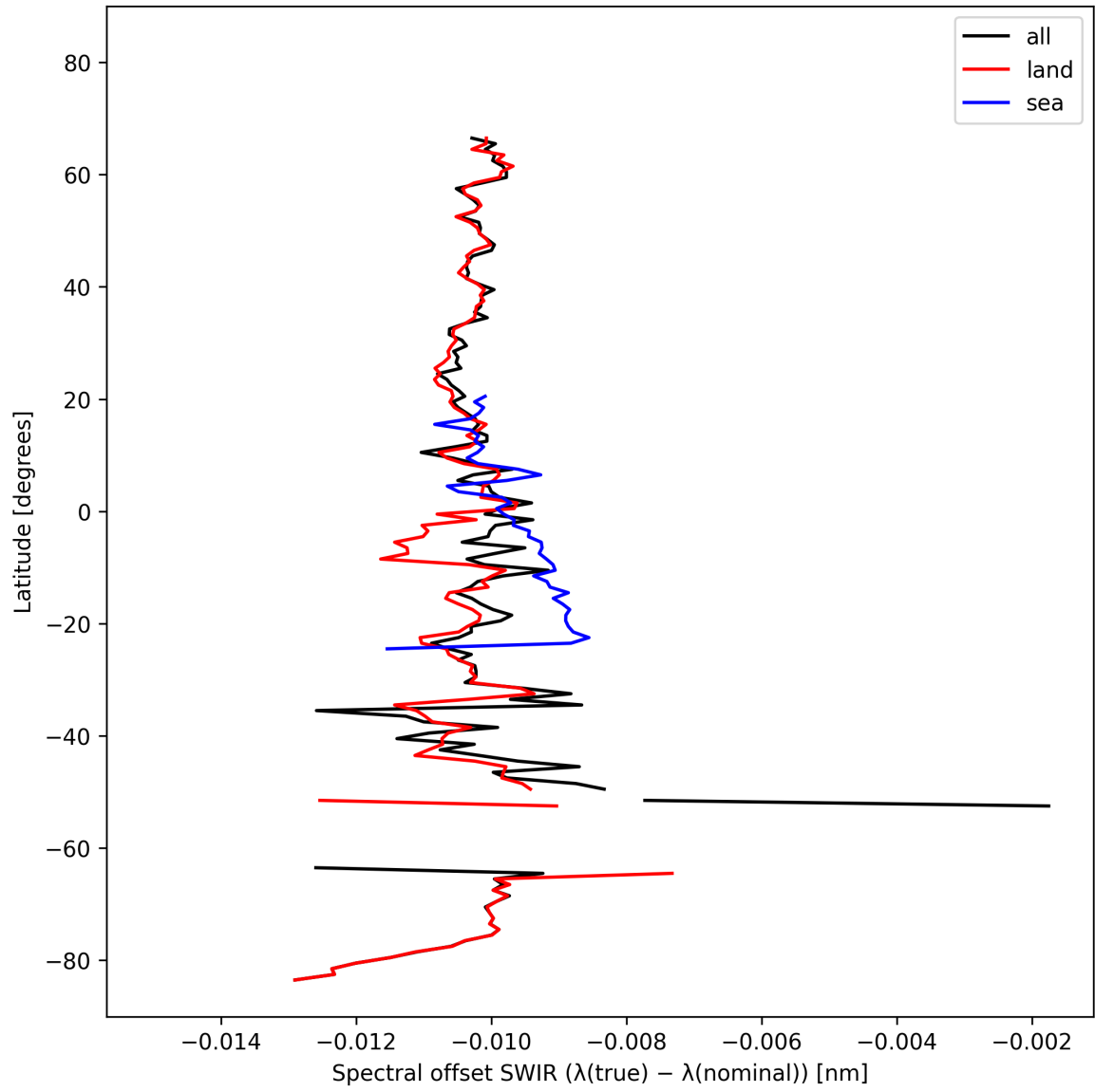
Figure 16: Zonal average of “Spectral offset SWIR ( \lambda_{\text{true}} - \lambda_{\text{nominal}} )” for 2024-10-14 to 2024-10-15.
