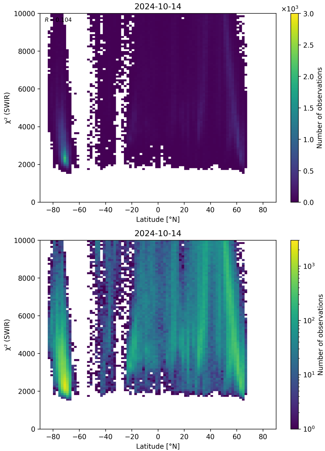
Figure 54: Scatter density plot of “Latitude” against “ \chi^2 (SWIR)” for 2024-10-14 to 2024-10-15.
