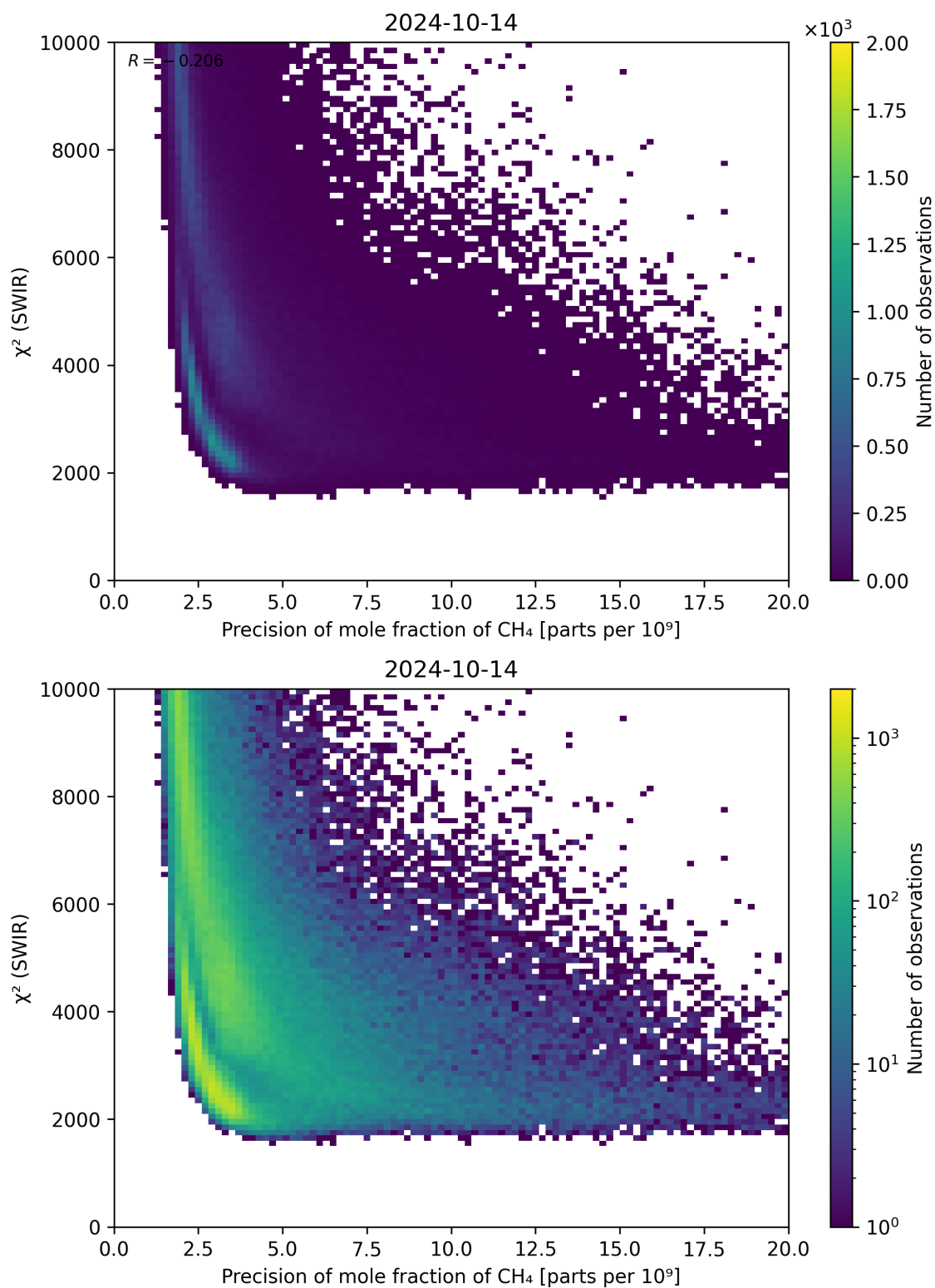
Figure 79: Scatter density plot of “Precision of mole fraction of \text{CH}_4 ” against “ \chi^2 (SWIR)” for 2024-10-14 to 2024-10-15.
