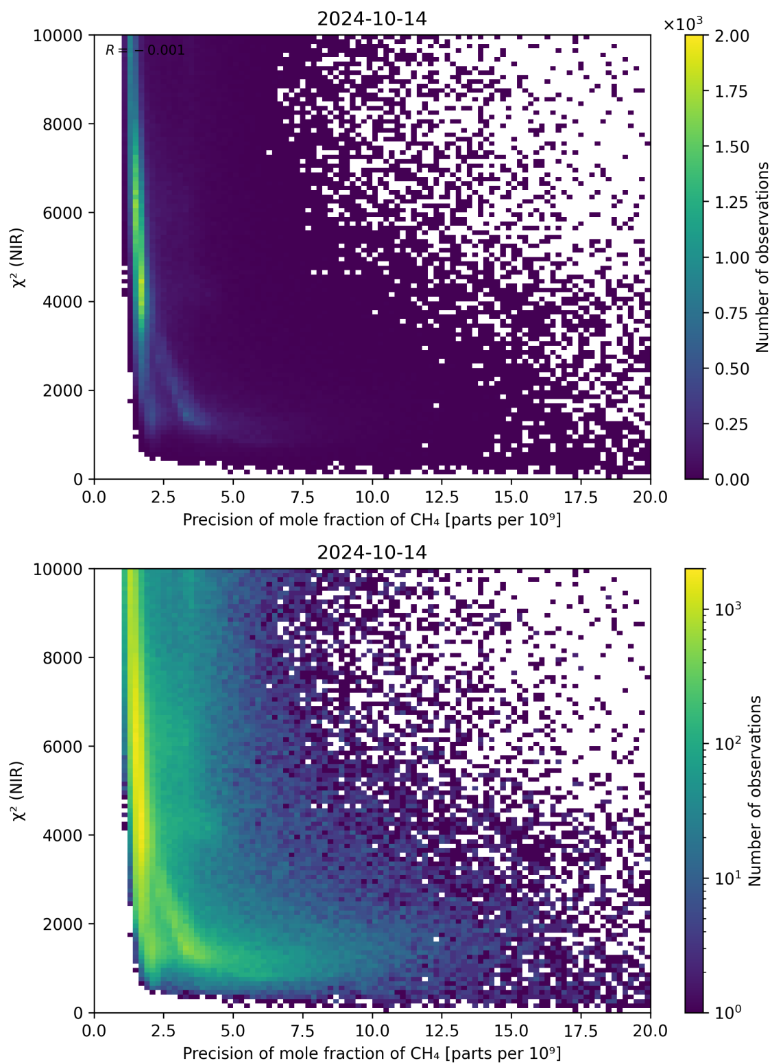
Figure 78: Scatter density plot of “Precision of mole fraction of \text{CH}_4 ” against “ \chi^2 (NIR)” for 2024-10-14 to 2024-10-15.
