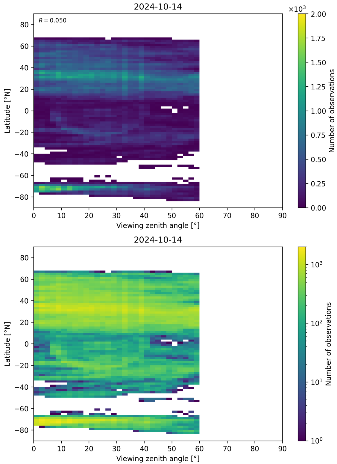
Figure 109: Scatter density plot of “Viewing zenith angle” against “Latitude” for 2024-10-14 to 2024-10-15.
