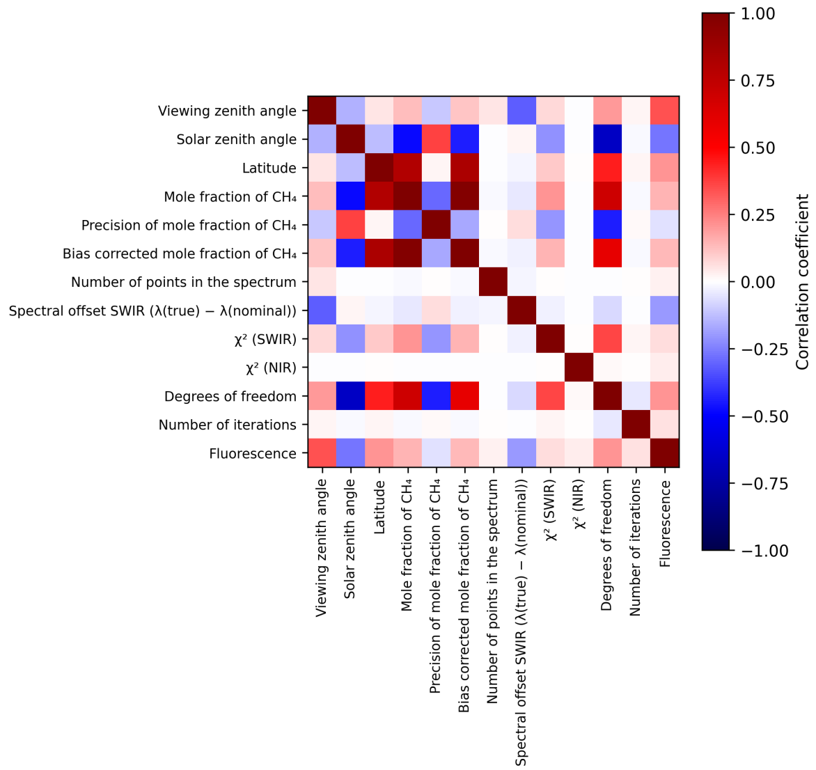
Figure 2: Map of correlation matrix for 2024-10-14 to 2024-10-15.
