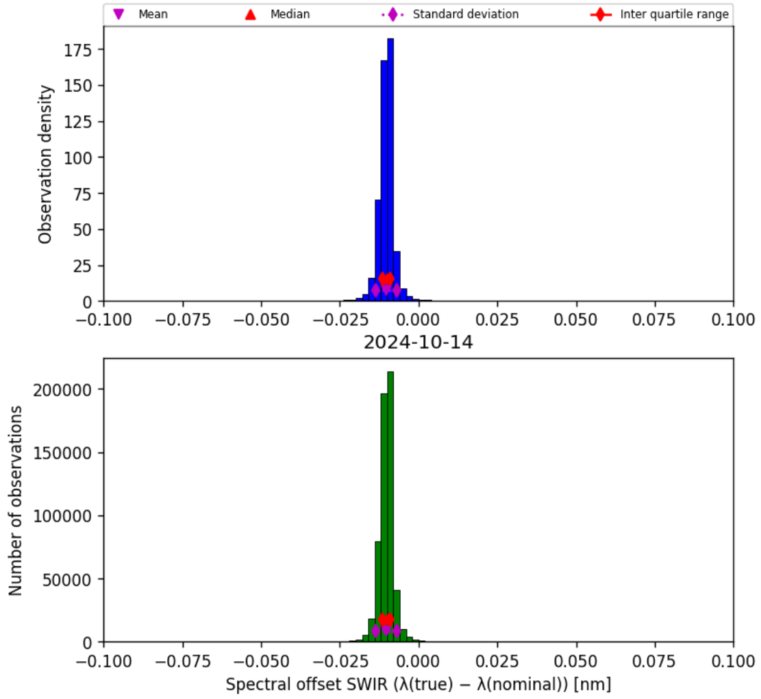
Figure 27: Histogram of “Spectral offset SWIR ( \lambda_{\text{true}} - \lambda_{\text{nominal}} )” for 2024-10-14 to 2024-10-15
