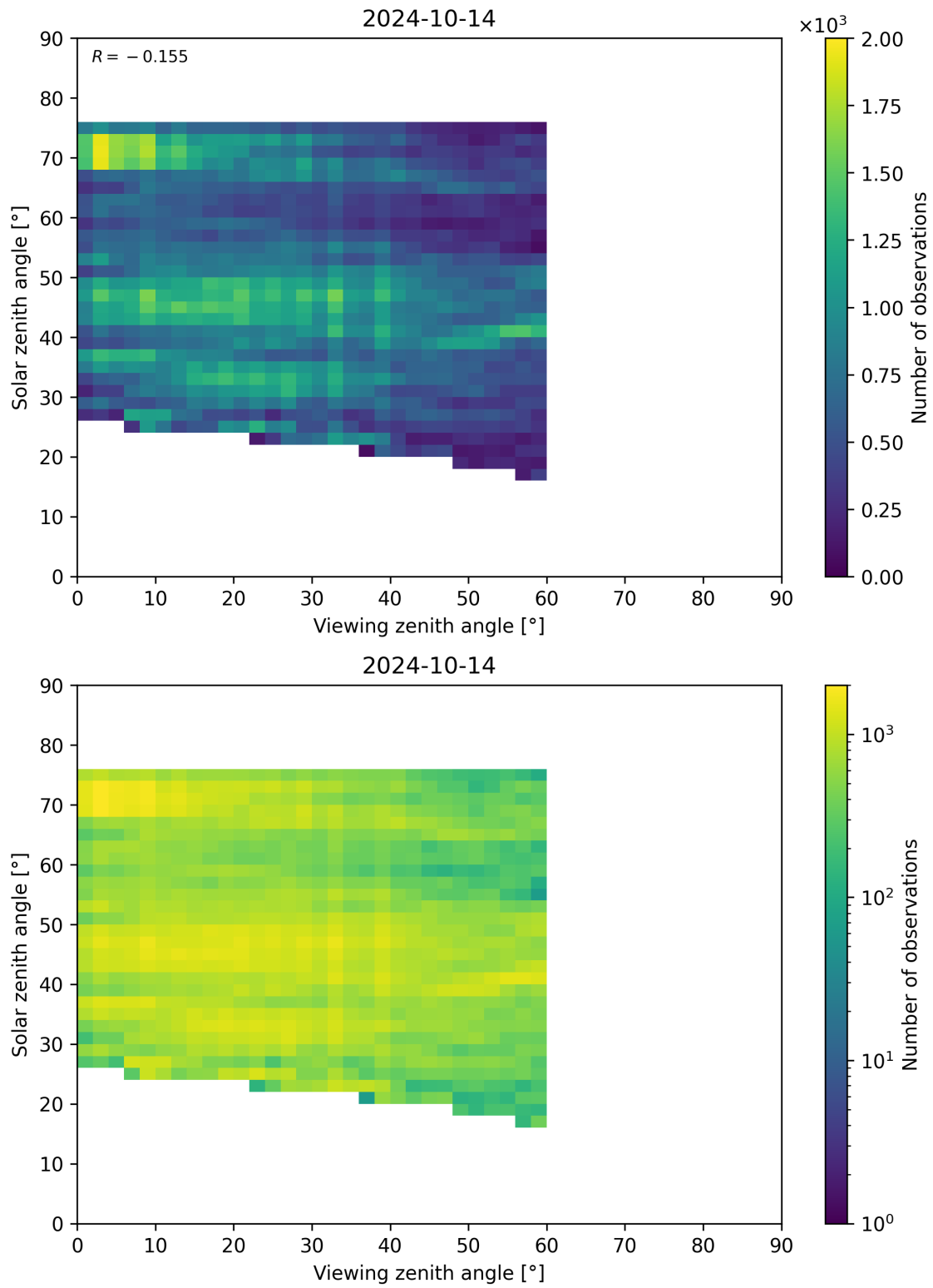
Figure 115: Scatter density plot of “Viewing zenith angle” against “Solar zenith angle” for 2024-10-14 to 2024-10-15.
