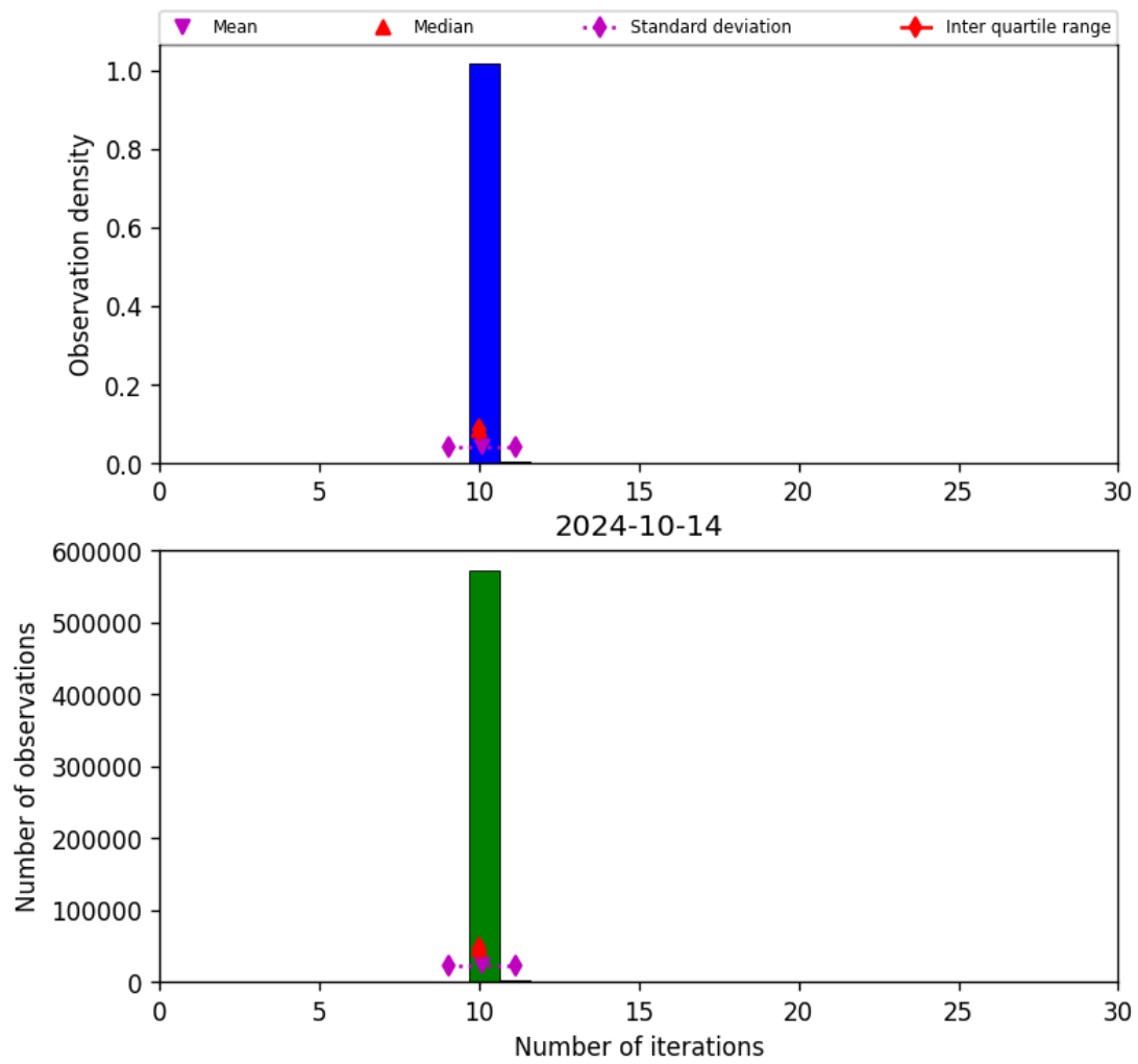
Figure 31: Histogram of “Number of iterations” for 2024-10-14 to 2024-10-15
