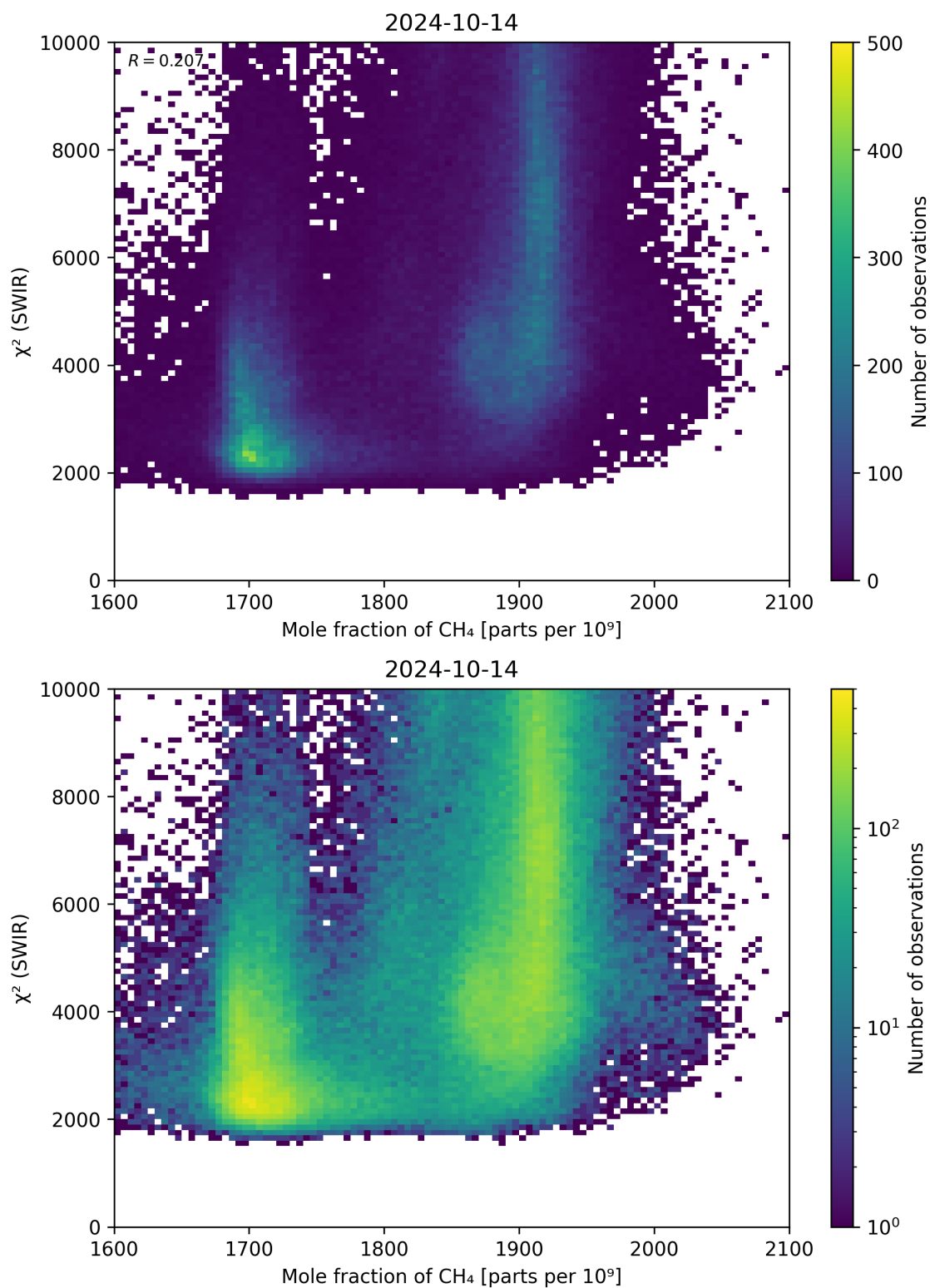
Figure 71: Scatter density plot of “Mole fraction of \text{CH}_4 ” against “ \chi^2 (SWIR)” for 2024-10-14 to 2024-10-15.
