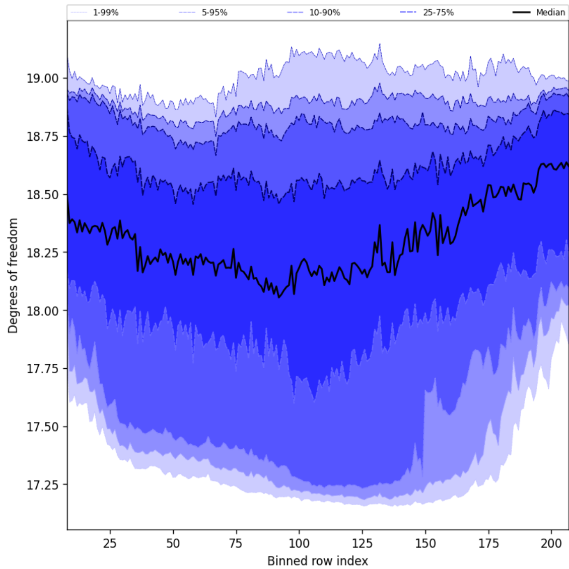
Figure 41: Along track statistics of “Degrees of freedom” for 2024-10-14 to 2024-10-15
