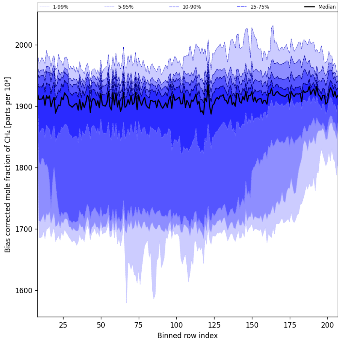
Figure 36: Along track statistics of “Bias corrected mole fraction of CH 4 ” for 2024-10-14 to 2024-10-15
