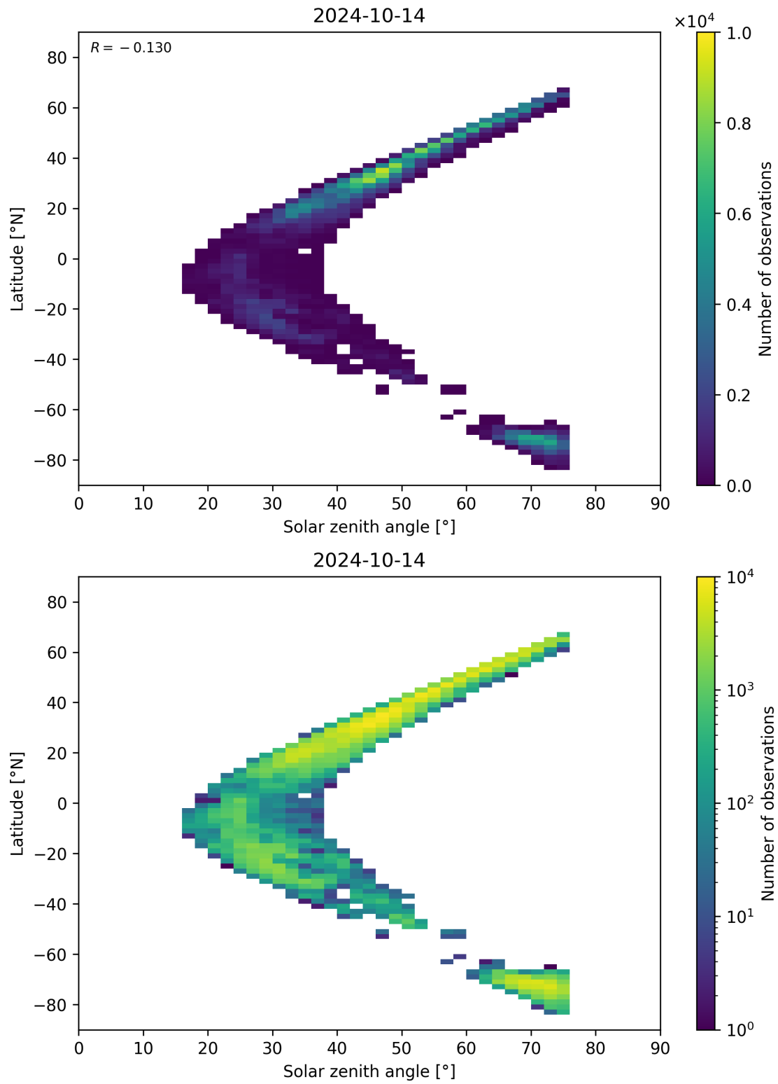
Figure 98: Scatter density plot of “Solar zenith angle” against “Latitude” for 2024-10-14 to 2024-10-15.
