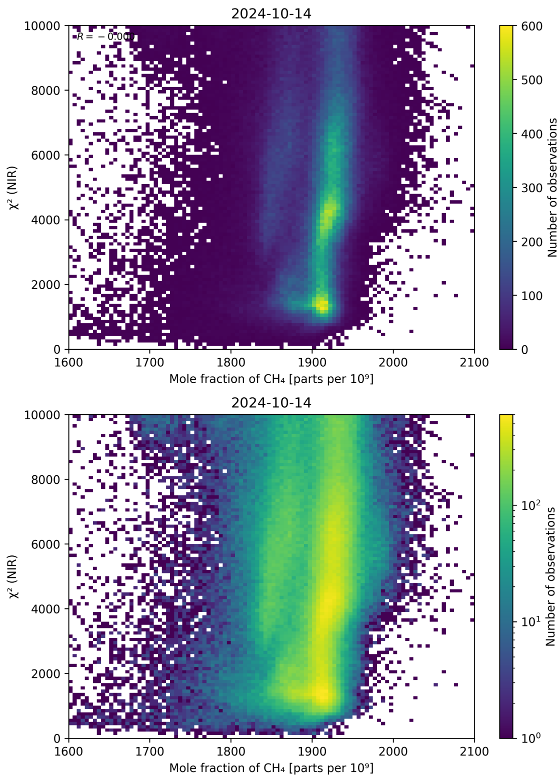
Figure 70: Scatter density plot of “Mole fraction of \text{CH}_4 ” against “ \chi^2 (NIR)” for 2024-10-14 to 2024-10-15.
