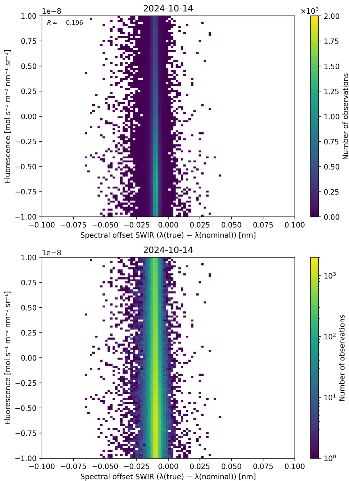
Figure 120: Scatter density plot of “Spectral offset SWIR ( \lambda_{\text{true}} - \lambda_{\text{nominal}} )” against “Fluorescence” for 2024-10-14 to 2024-10-15.
