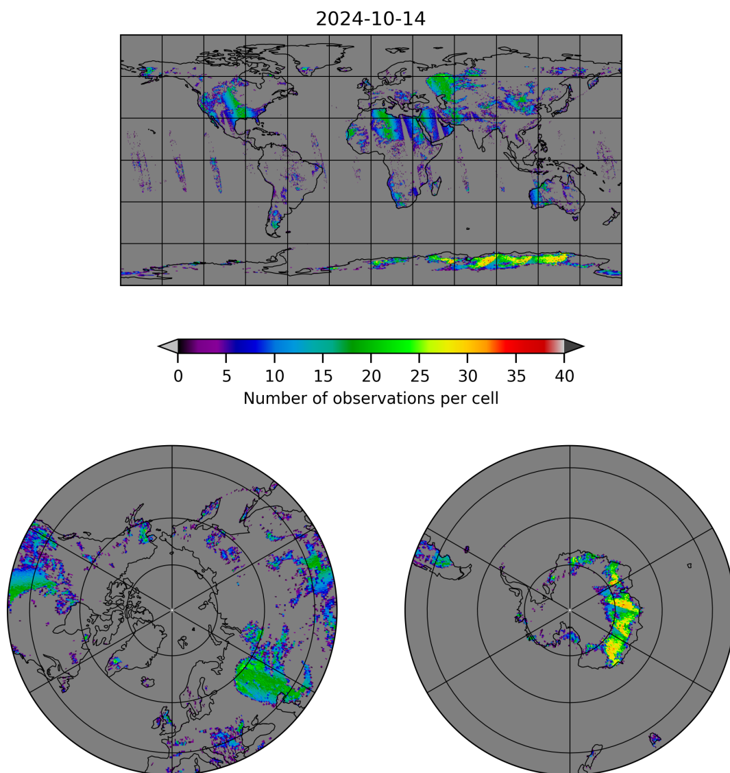
Figure 10: Map of the number of observations for 2024-10-14 to 2024-10-15
