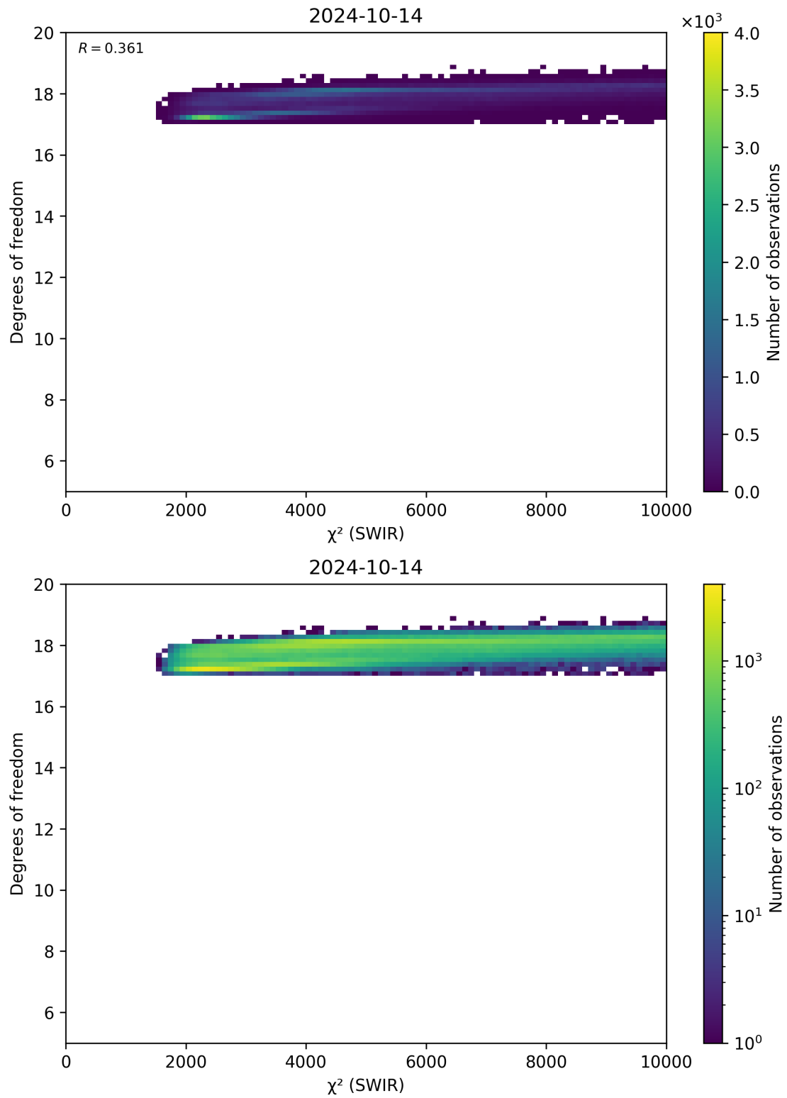
Figure 48: Scatter density plot of “ \chi^2 (SWIR)” against “Degrees of freedom” for 2024-10-14 to 2024-10-15.
