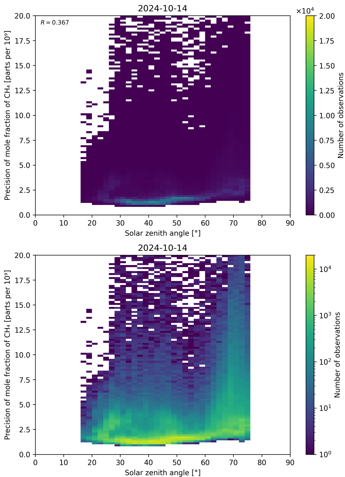
Figure 101: Scatter density plot of “Solar zenith angle” against “Precision of mole fraction of \text{CH}_4 ” for 2024-10-14 to 2024-10-15.
