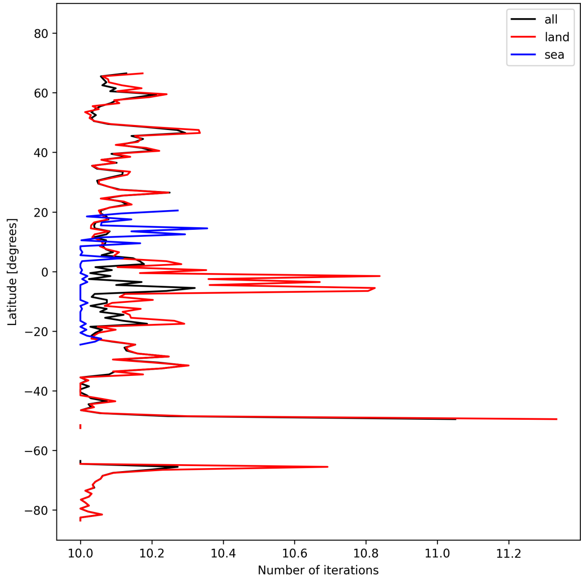
Figure 20: Zonal average of “Number of iterations” for 2024-10-14 to 2024-10-15.
