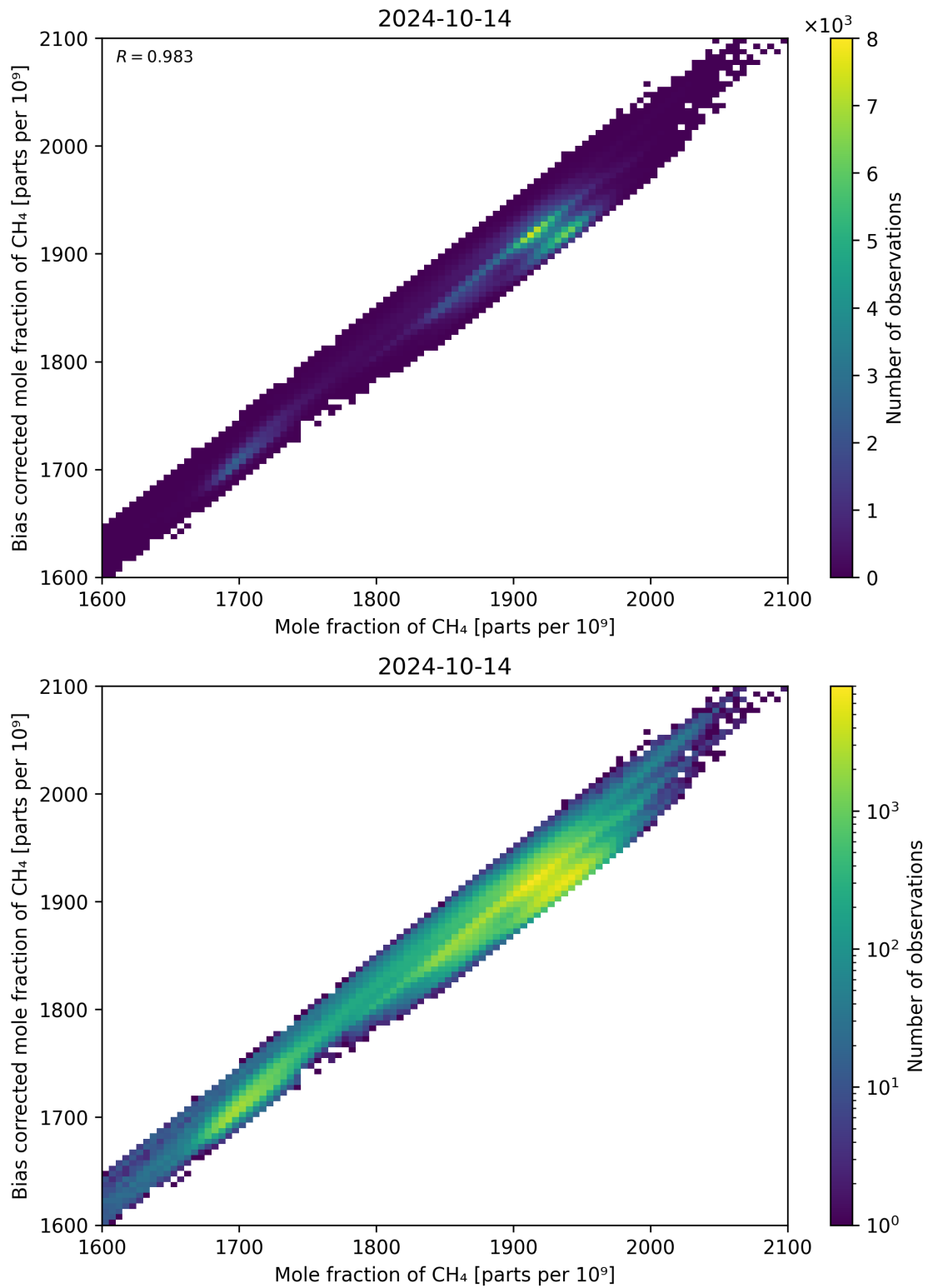
Figure 74: Scatter density plot of “Mole fraction of CH 4 ” against “Bias corrected mole fraction of CH 4 ” for 2024-10-14 to 2024-10-15.
