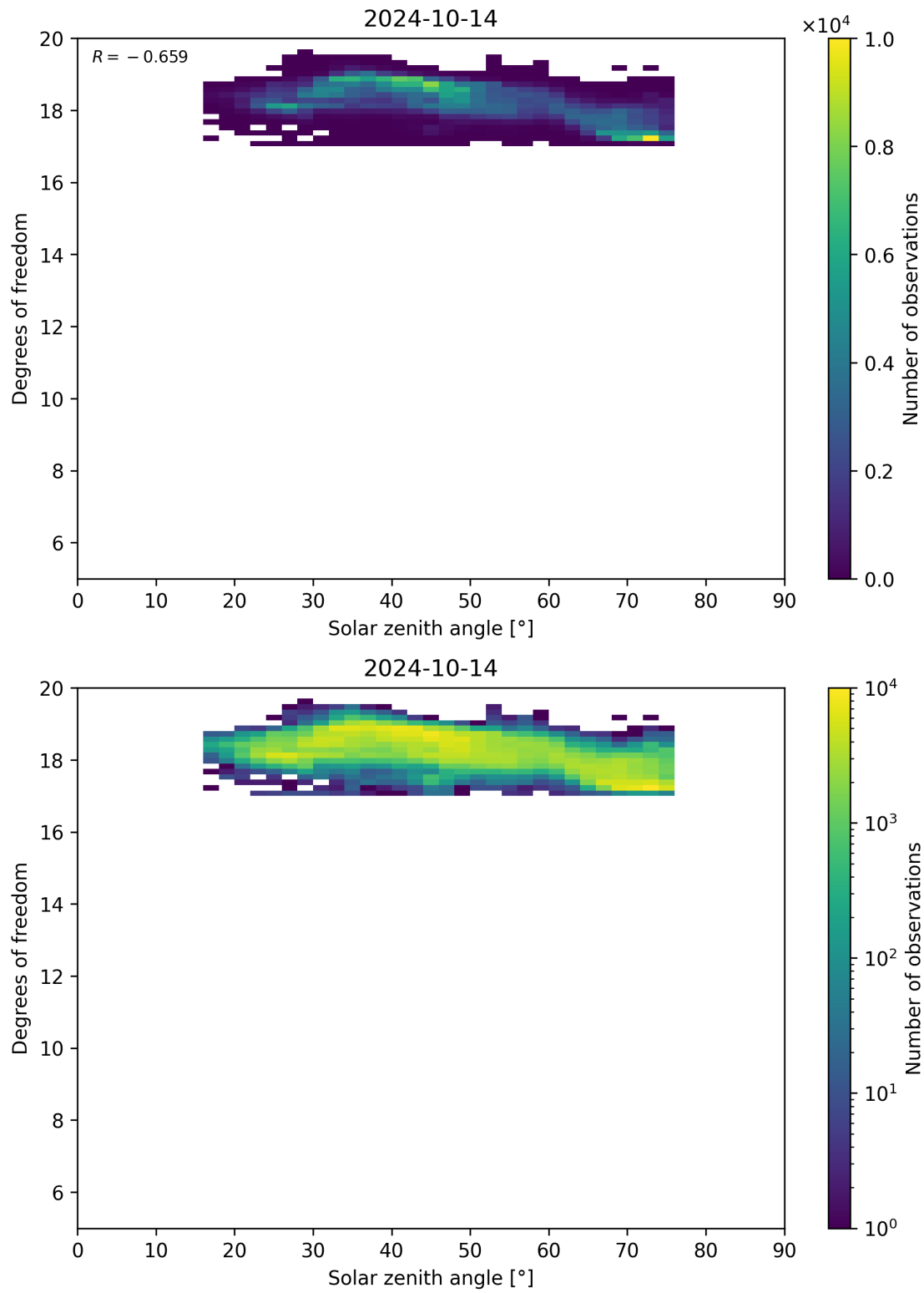
Figure 96: Scatter density plot of “Solar zenith angle” against “Degrees of freedom” for 2024-10-14 to 2024-10-15.
