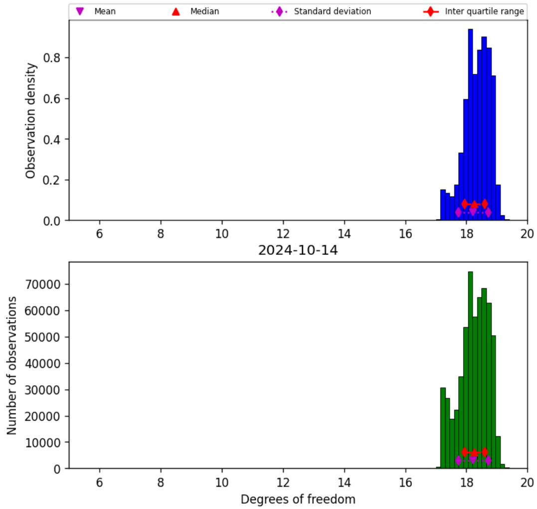
Figure 30: Histogram of “Degrees of freedom” for 2024-10-14 to 2024-10-15
