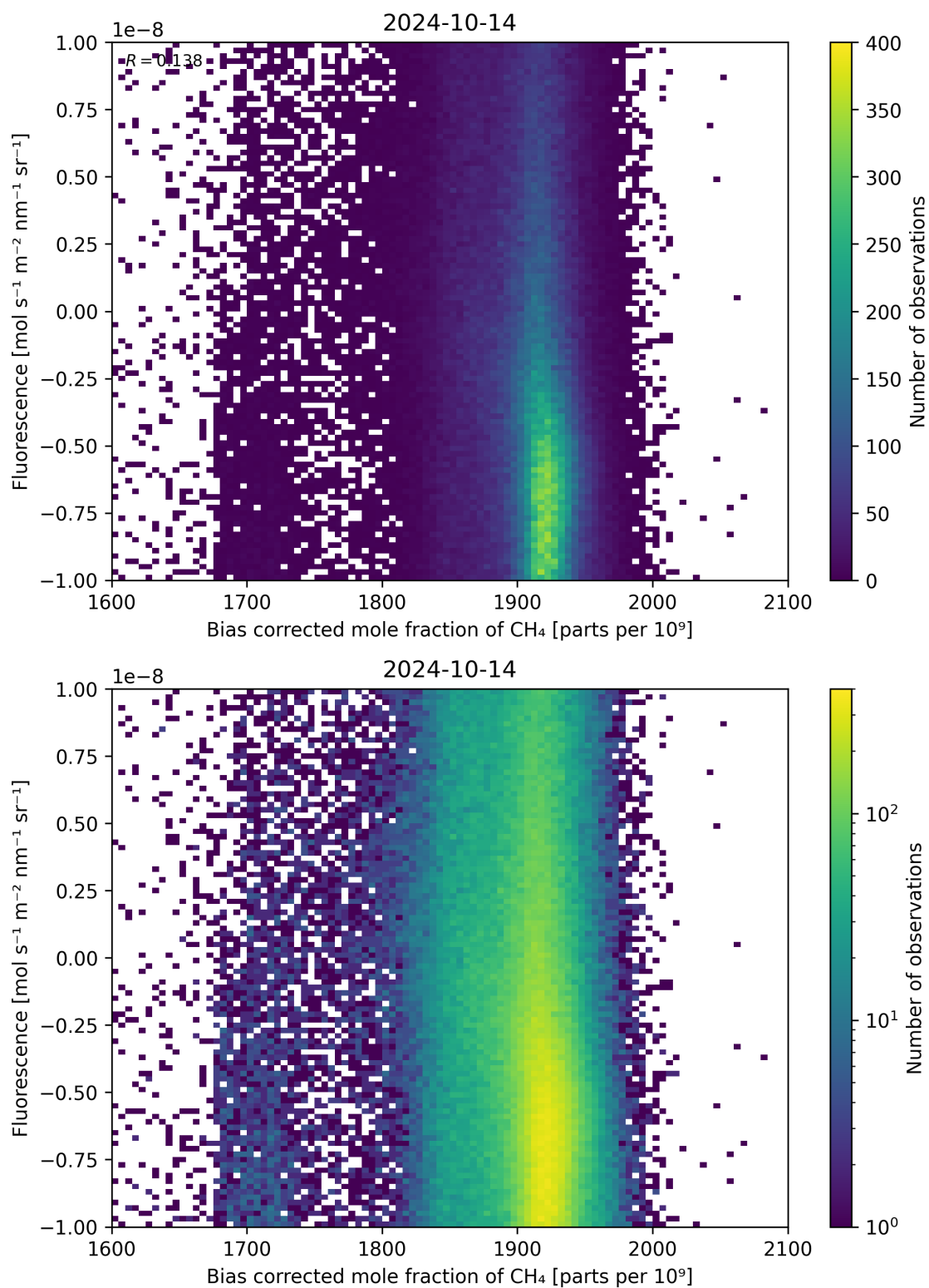
Figure 66: Scatter density plot of “Bias corrected mole fraction of \text{CH}_4 ” against “Fluorescence” for 2024-10-14 to 2024-10-15.
