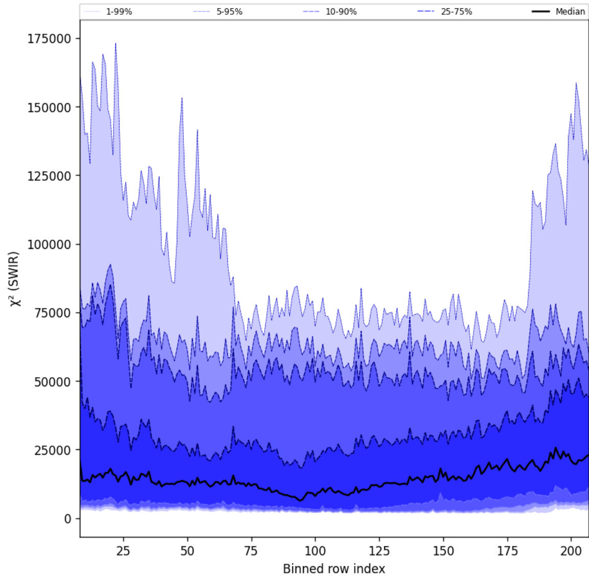
Figure 39: Along track statistics of " \chi^2 (SWIR)" for 2024-10-14 to 2024-10-15
