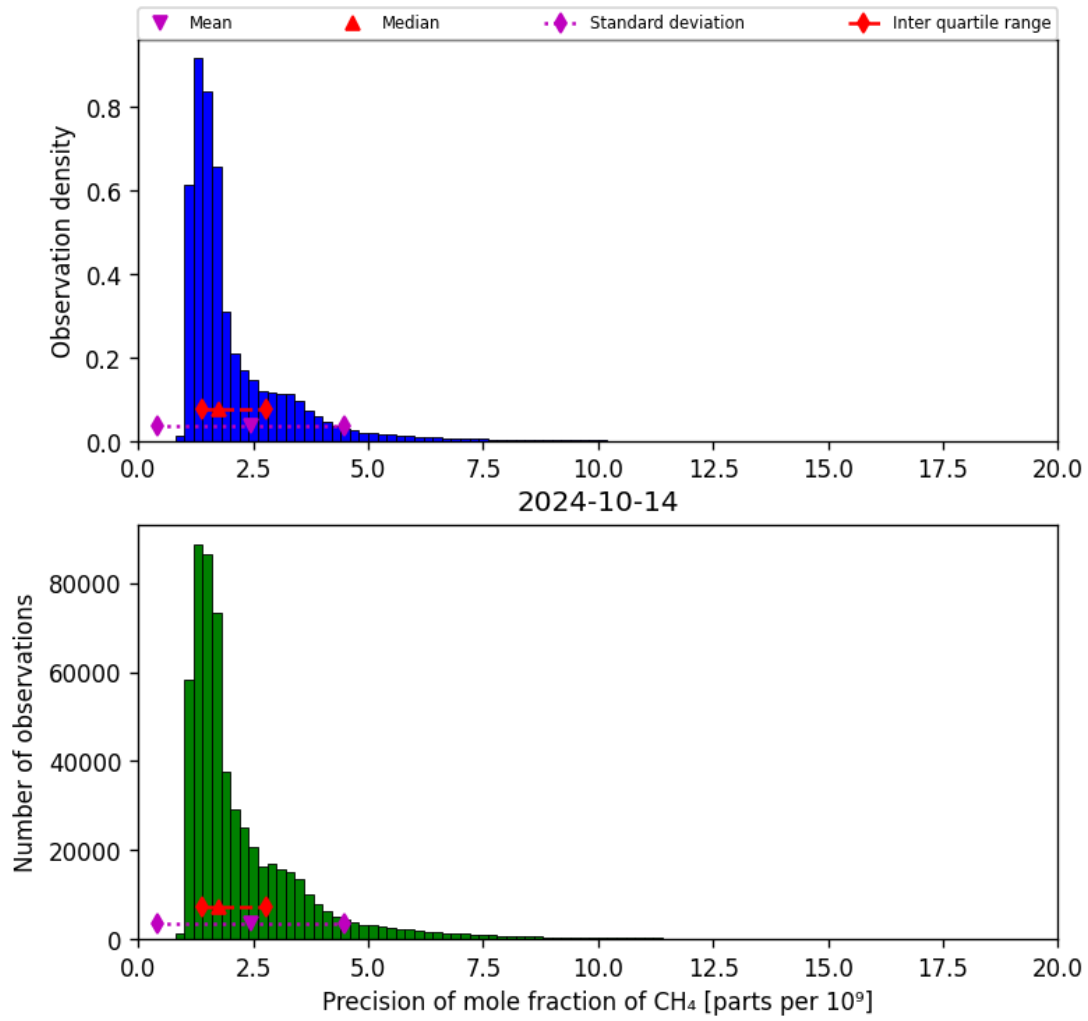
Figure 24: Histogram of “Precision of mole fraction of CH 4 ” for 2024-10-14 to 2024-10-15
