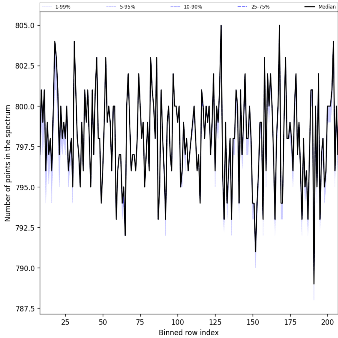
Figure 37: Along track statistics of “Number of points in the spectrum” for 2024-10-14 to 2024-10-15
