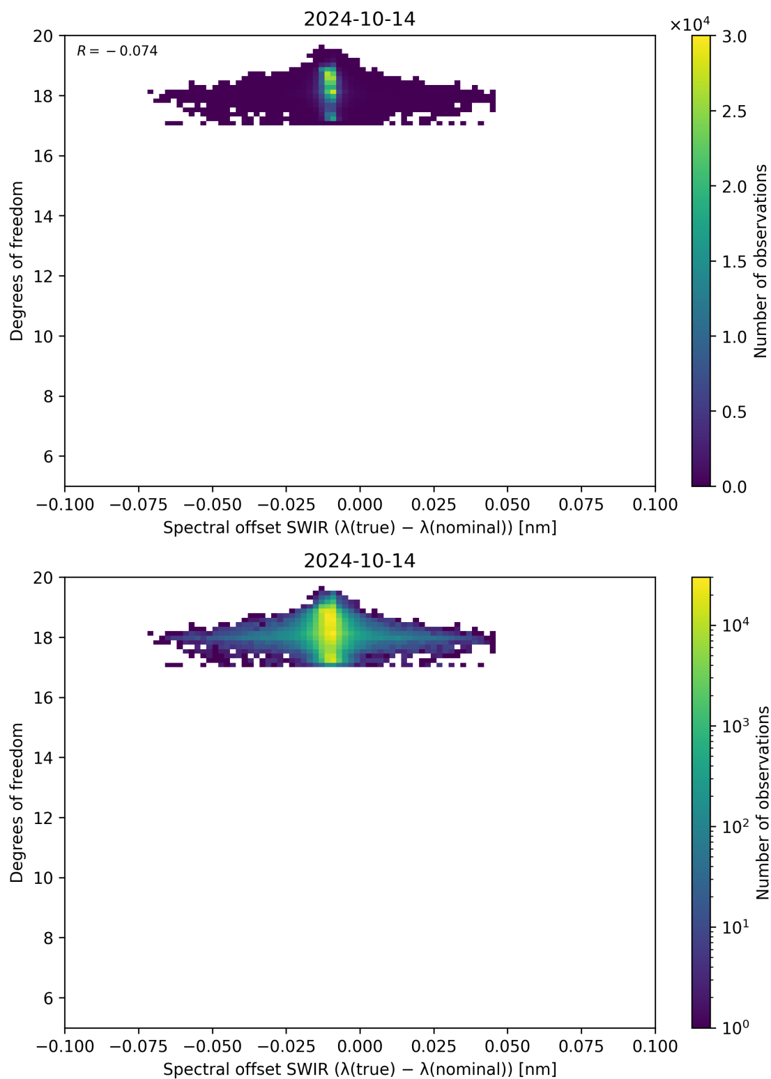
Figure 119: Scatter density plot of “Spectral offset SWIR ( \lambda_{\text{true}} - \lambda_{\text{nominal}} )” against “Degrees of freedom” for 2024-10-14 to 2024-10-15.
