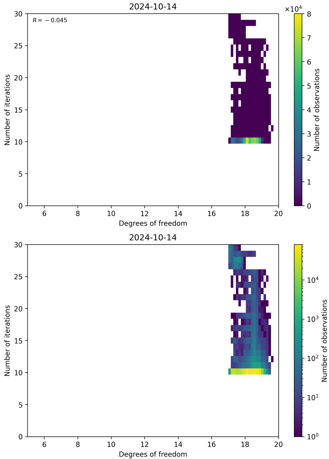
Figure 52: Scatter density plot of “Degrees of freedom” against “Number of iterations” for 2024-10-14 to 2024-10-15.
