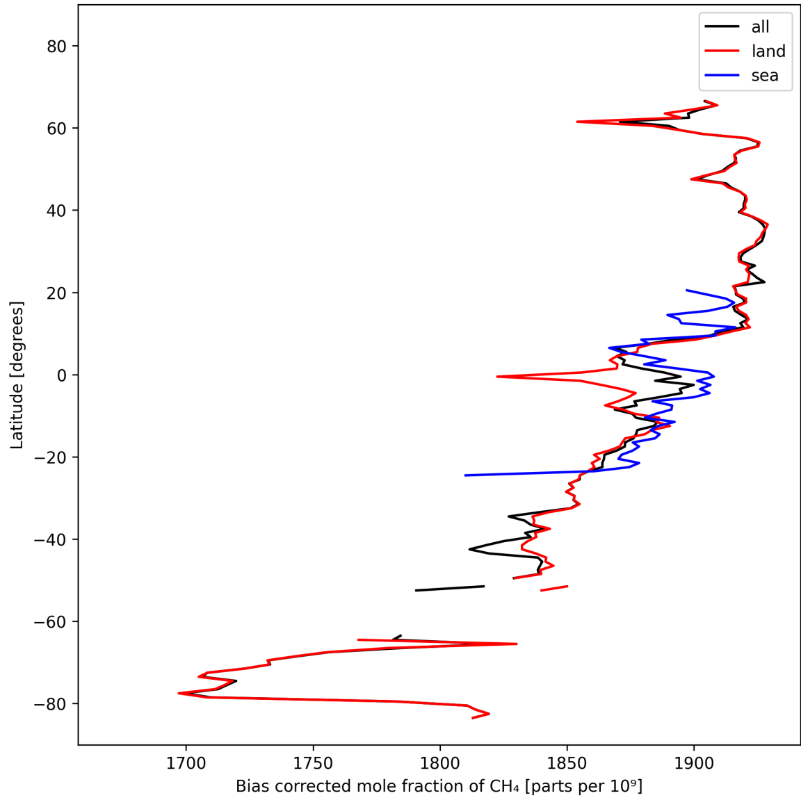
Figure 14: Zonal average of “Bias corrected mole fraction of CH 4 ” for 2024-10-14 to 2024-10-15.
