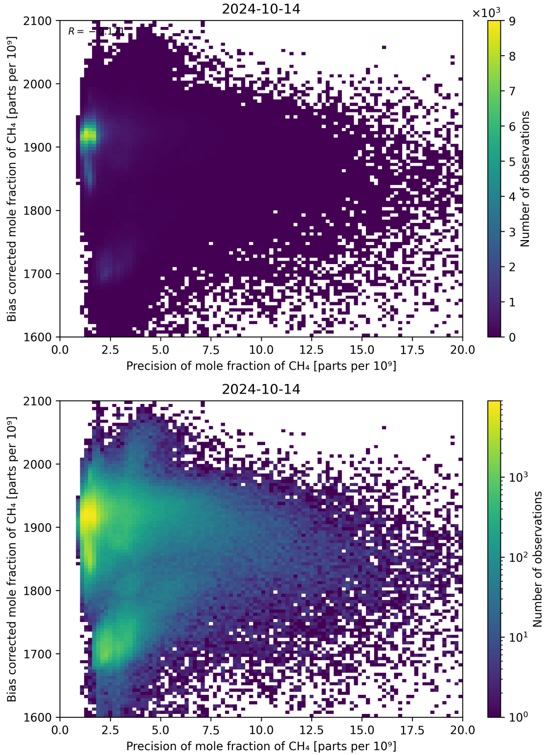
Figure 82: Scatter density plot of “Precision of mole fraction of CH 4 ” against “Bias corrected mole fraction of CH 4 ” for 2024-10-14 to 2024-10-15.
