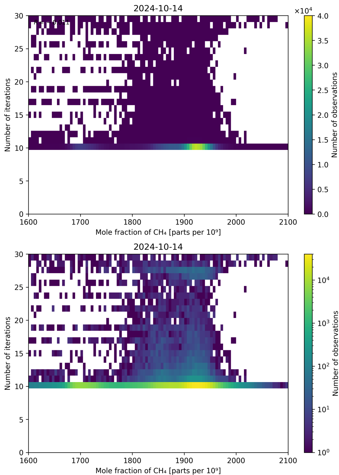
Figure 76: Scatter density plot of “Mole fraction of CH 4 ” against “Number of iterations” for 2024-10-14 to 2024-10-15.
