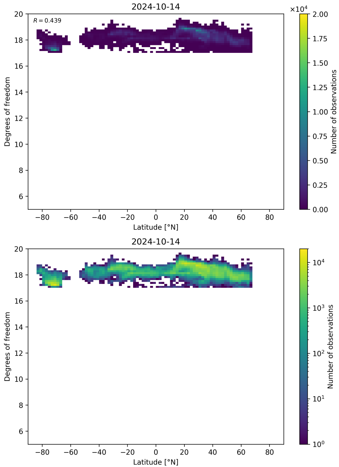
Figure 55: Scatter density plot of “Latitude” against “Degrees of freedom” for 2024-10-14 to 2024-10-15.
