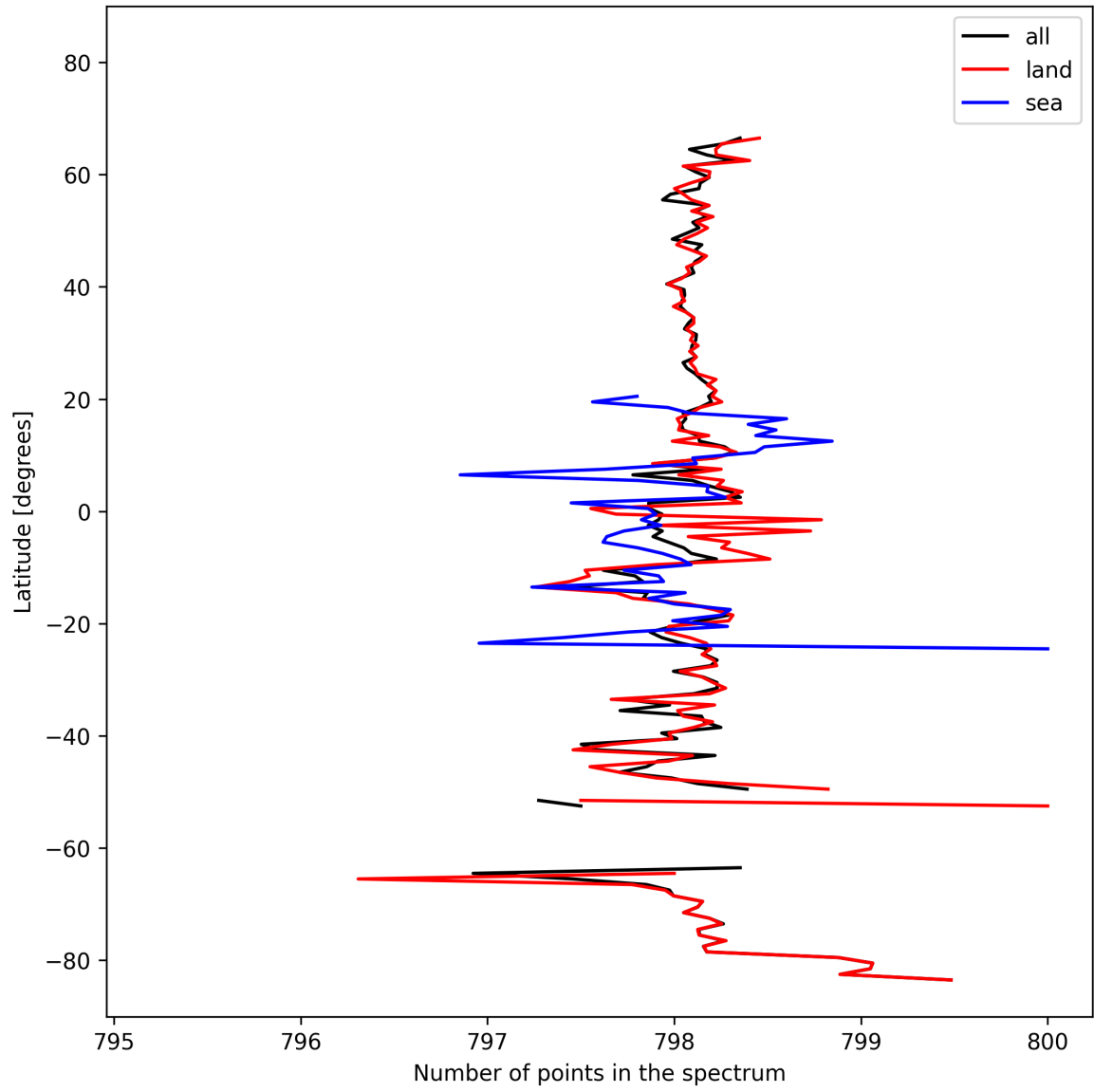
Figure 15: Zonal average of “Number of points in the spectrum” for 2024-10-14 to 2024-10-15.
