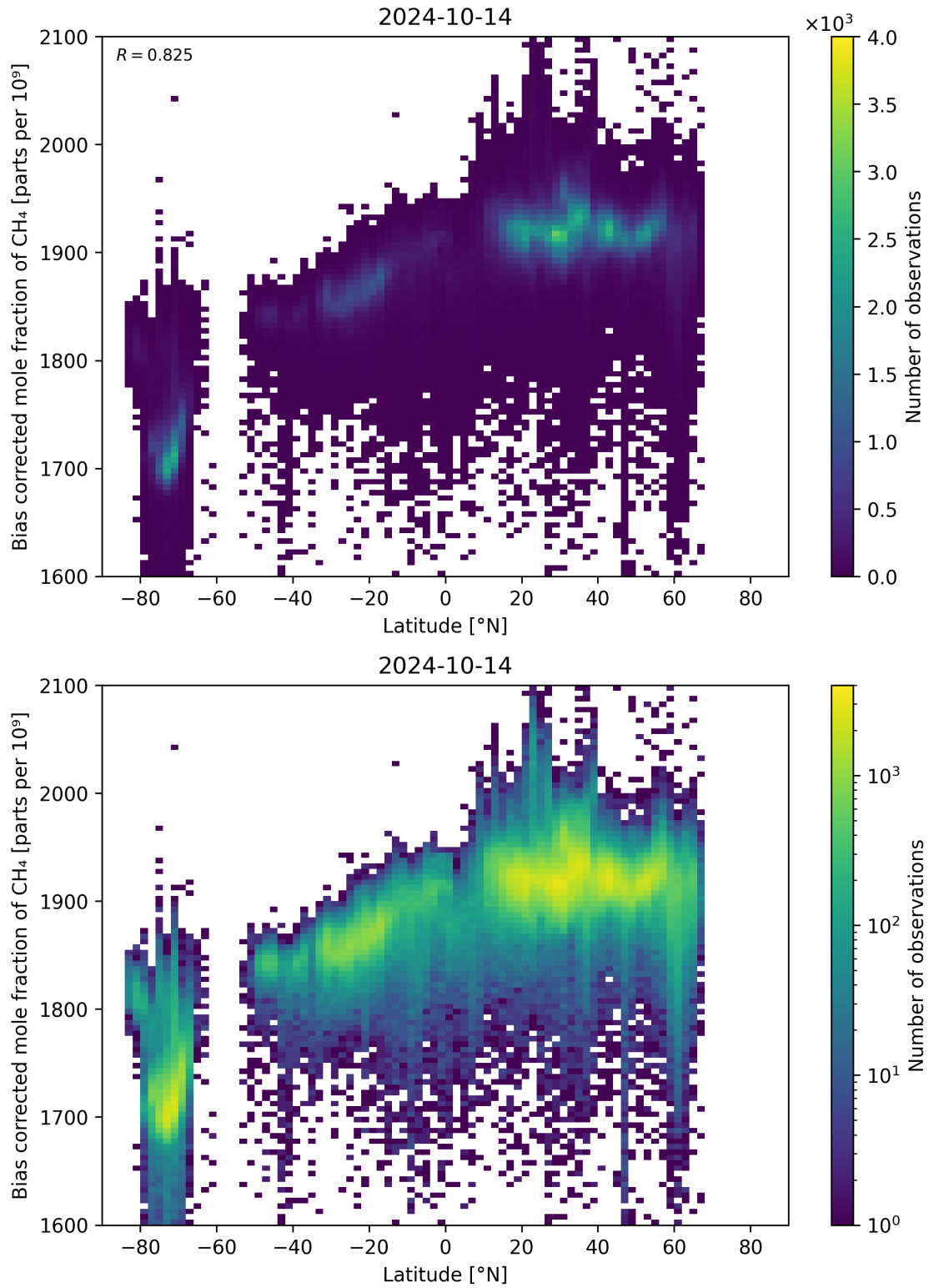
Figure 58: Scatter density plot of “Latitude” against “Bias corrected mole fraction of CH 4 ” for 2024-10-14 to 2024-10-15.
