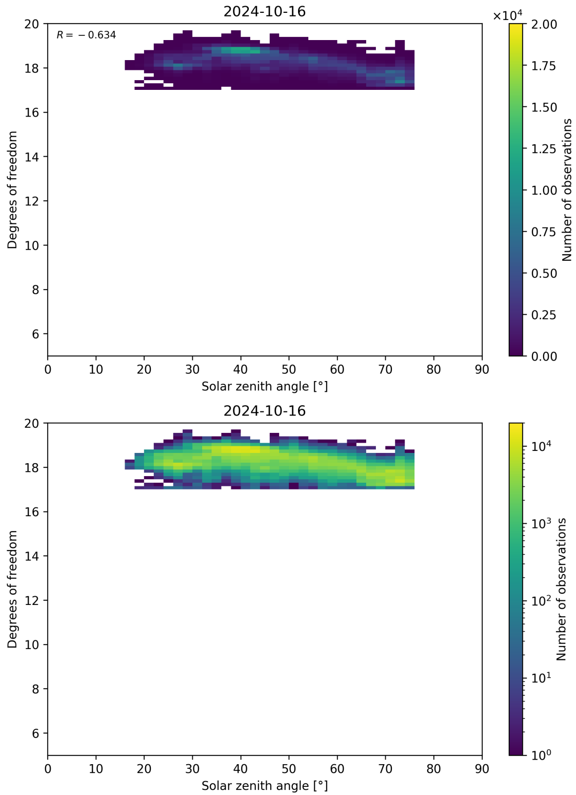
Figure 96: Scatter density plot of “Solar zenith angle” against “Degrees of freedom” for 2024-10-15 to 2024-10-17.
