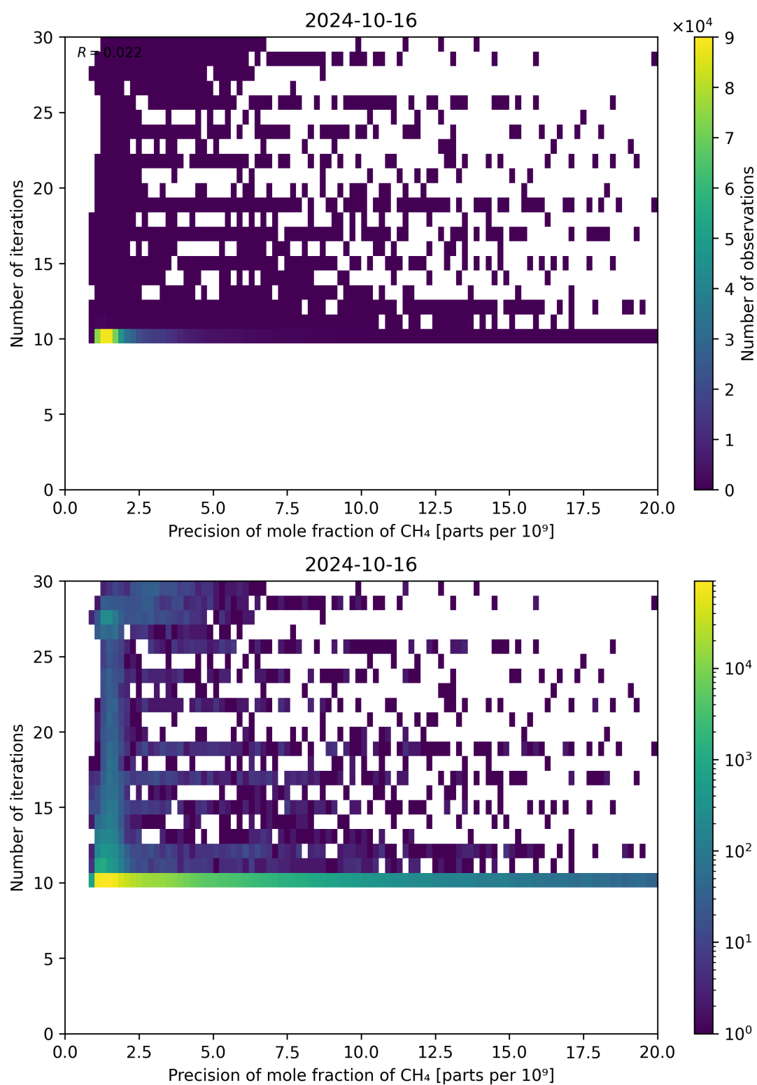
Figure 83: Scatter density plot of “Precision of mole fraction of CH 4 ” against “Number of iterations” for 2024-10-15 to 2024-10-17.
