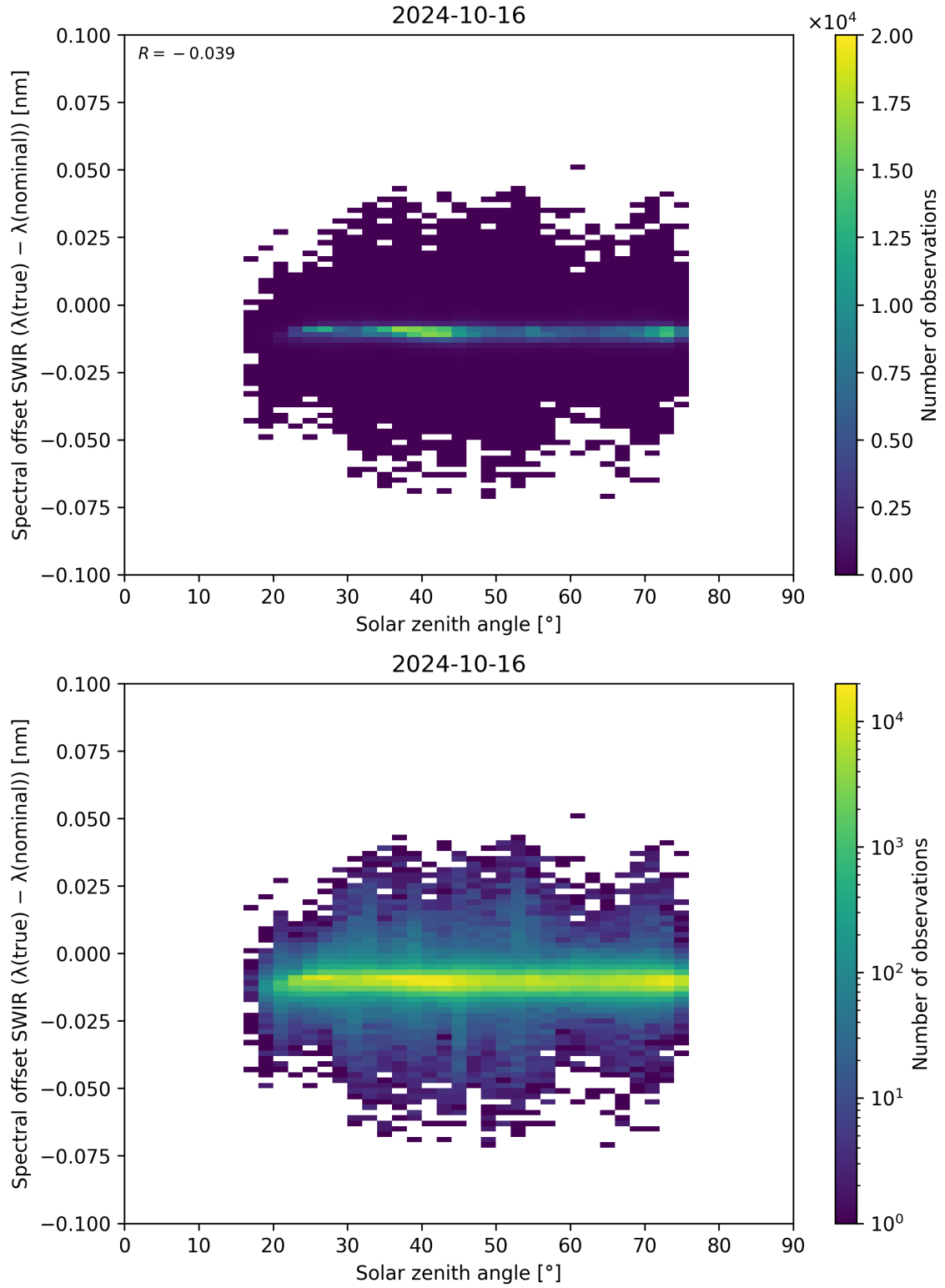
Figure 104: Scatter density plot of “Solar zenith angle” against “Spectral offset SWIR ( \lambda_{\text{true}} - \lambda_{\text{nominal}} )” for 2024-10-15 to 2024-10-17.
