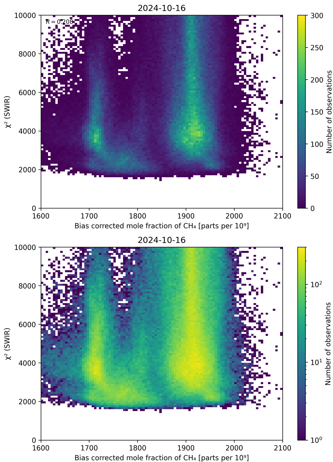
Figure 64: Scatter density plot of “Bias corrected mole fraction of \text{CH}_4 ” against “ \chi^2 (SWIR)” for 2024-10-15 to 2024-10-17.
