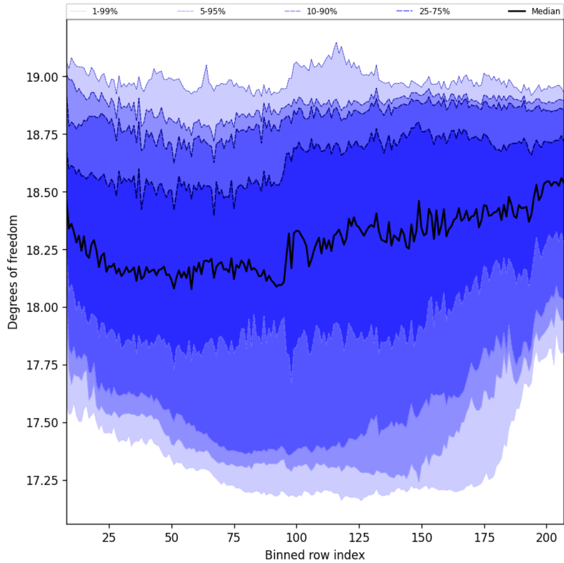
Figure 41: Along track statistics of “Degrees of freedom” for 2024-10-15 to 2024-10-17
