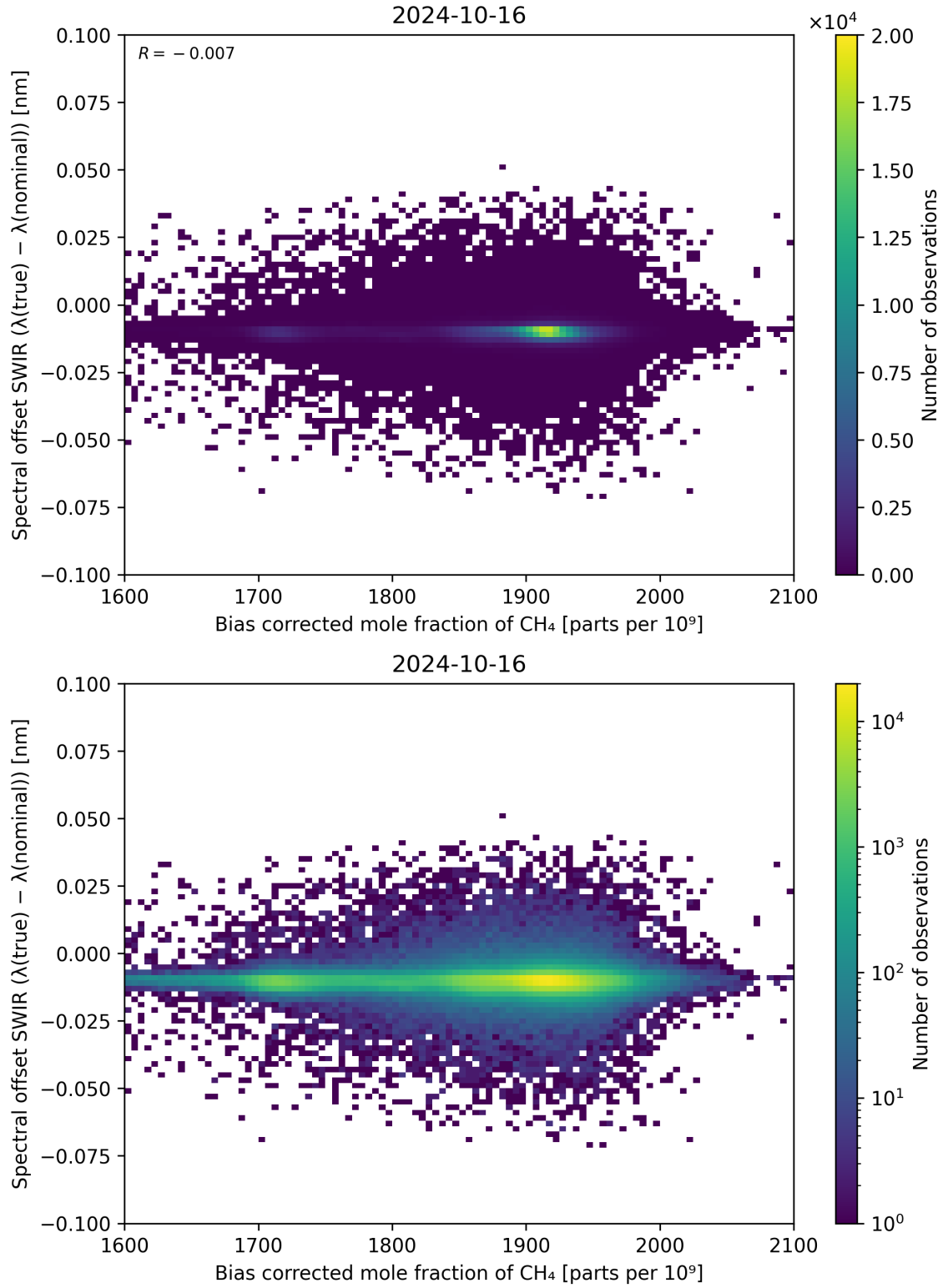
Figure 69: Scatter density plot of “Bias corrected mole fraction of \text{CH}_4 ” against “Spectral offset SWIR ( \lambda_{\text{true}} - \lambda_{\text{nominal}} )” for 2024-10-15 to 2024-10-17.
