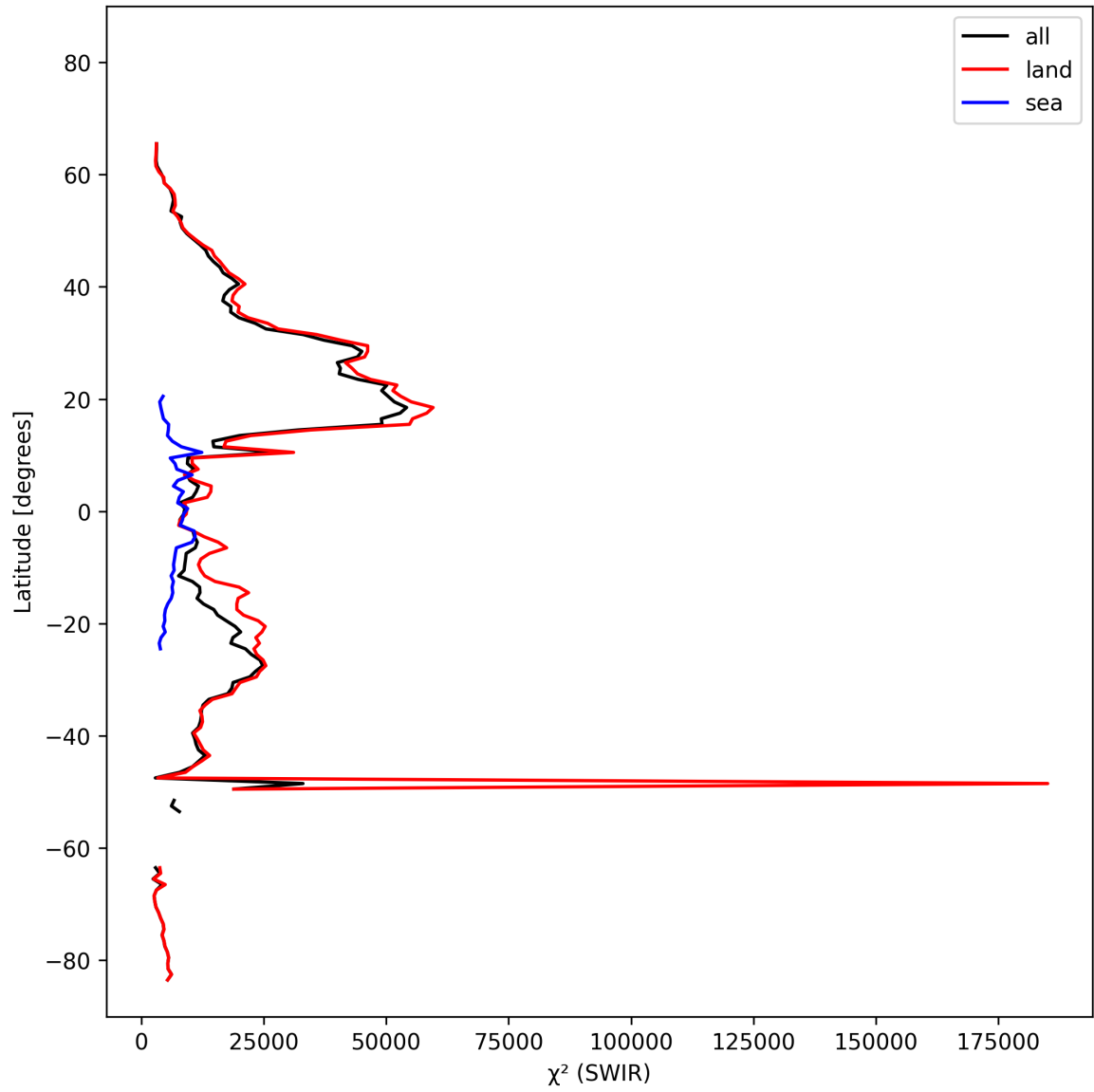
Figure 17: Zonal average of “ \chi^2 (SWIR)” for 2024-10-15 to 2024-10-17.
