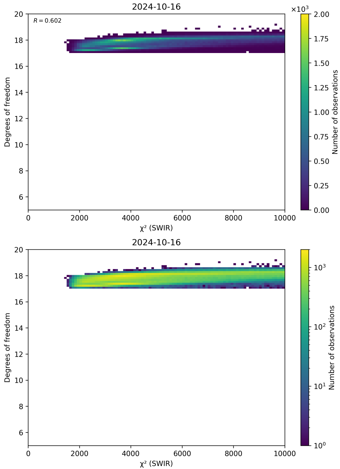
Figure 48: Scatter density plot of “ \chi^2 (SWIR)” against “Degrees of freedom” for 2024-10-15 to 2024-10-17.
