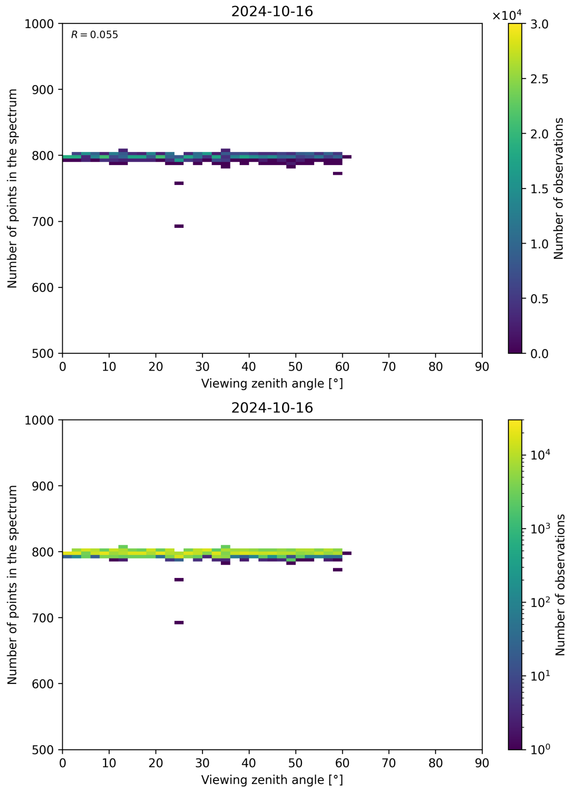
Figure 114: Scatter density plot of “Viewing zenith angle” against “Number of points in the spectrum” for 2024-10-15 to 2024-10-17.
