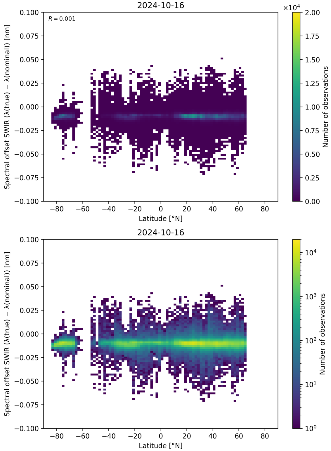
Figure 62: Scatter density plot of “Latitude” against “Spectral offset SWIR ( \lambda_{\text{true}} - \lambda_{\text{nominal}} )” for 2024-10-15 to 2024-10-17.
