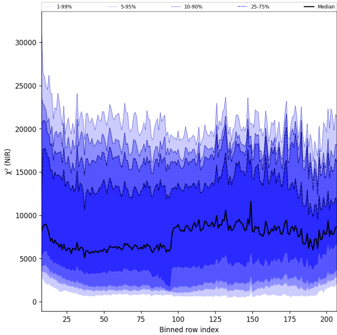
Figure 40: Along track statistics of “ \chi^2 (NIR)” for 2024-10-15 to 2024-10-17
