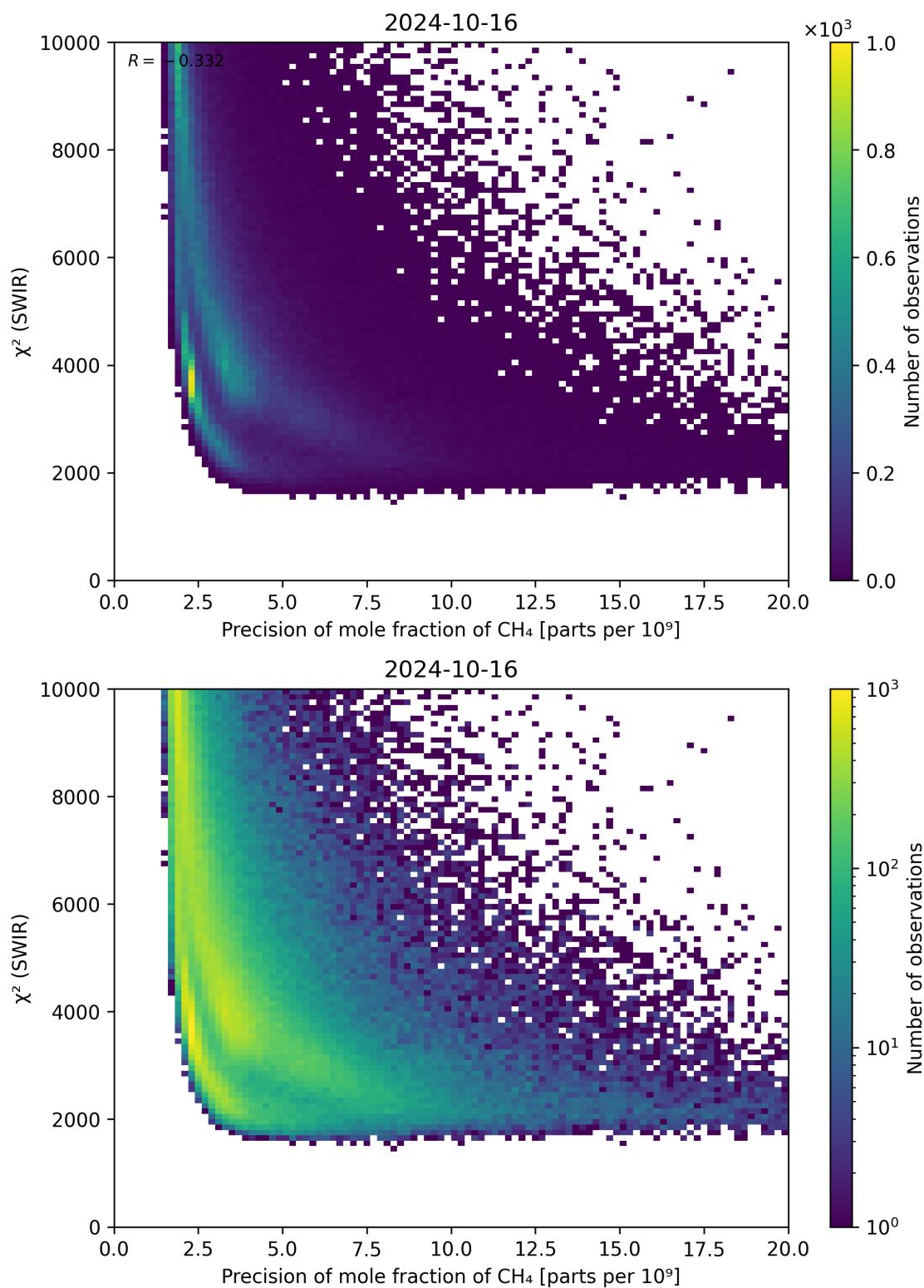
Figure 79: Scatter density plot of “Precision of mole fraction of CH 4 ” against “ \chi^2 (SWIR)” for 2024-10-15 to 2024-10-17.
