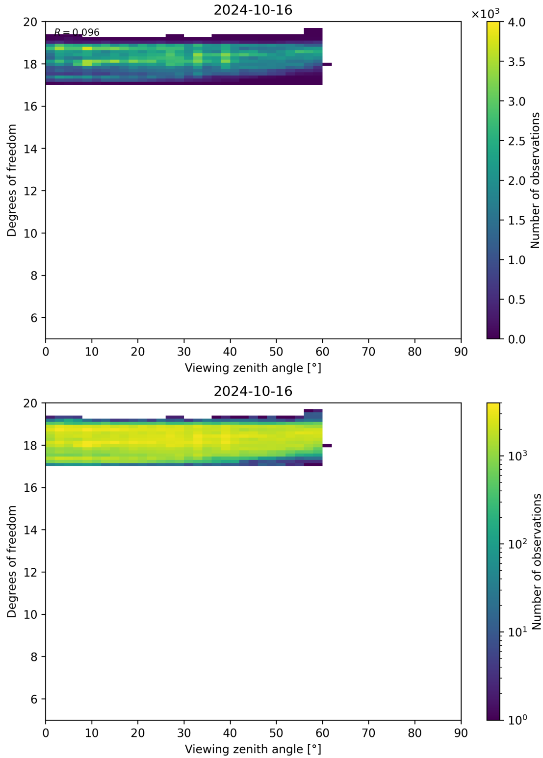
Figure 107: Scatter density plot of “Viewing zenith angle” against “Degrees of freedom” for 2024-10-15 to 2024-10-17.
