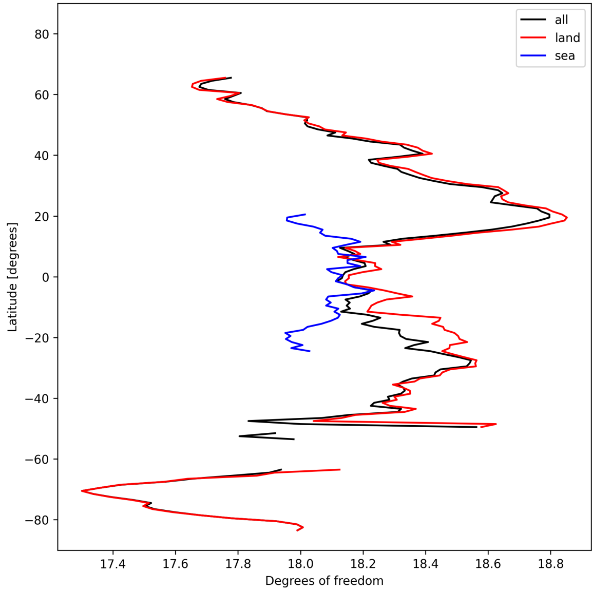
Figure 19: Zonal average of “Degrees of freedom” for 2024-10-15 to 2024-10-17.
