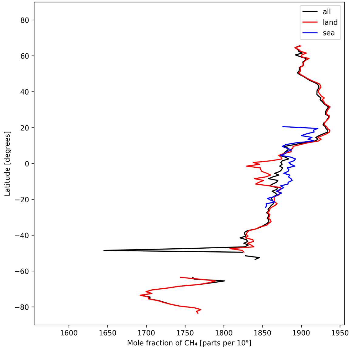
Figure 12: Zonal average of “Mole fraction of CH 4 ” for 2024-10-15 to 2024-10-17.
