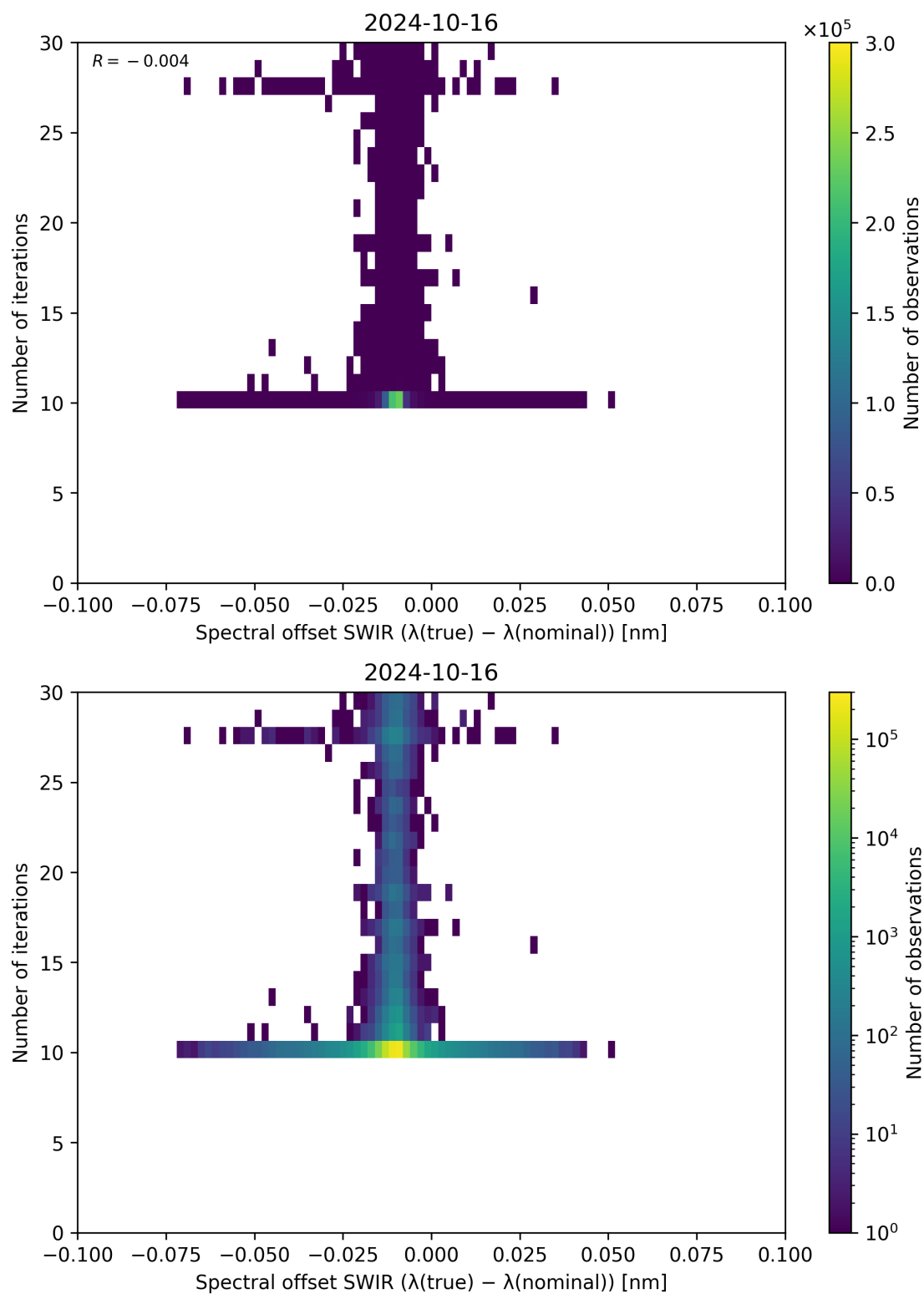
Figure 121: Scatter density plot of “Spectral offset SWIR ( \lambda_{\text{true}} - \lambda_{\text{nominal}} )” against “Number of iterations” for 2024-10-15 to 2024-10-17.
