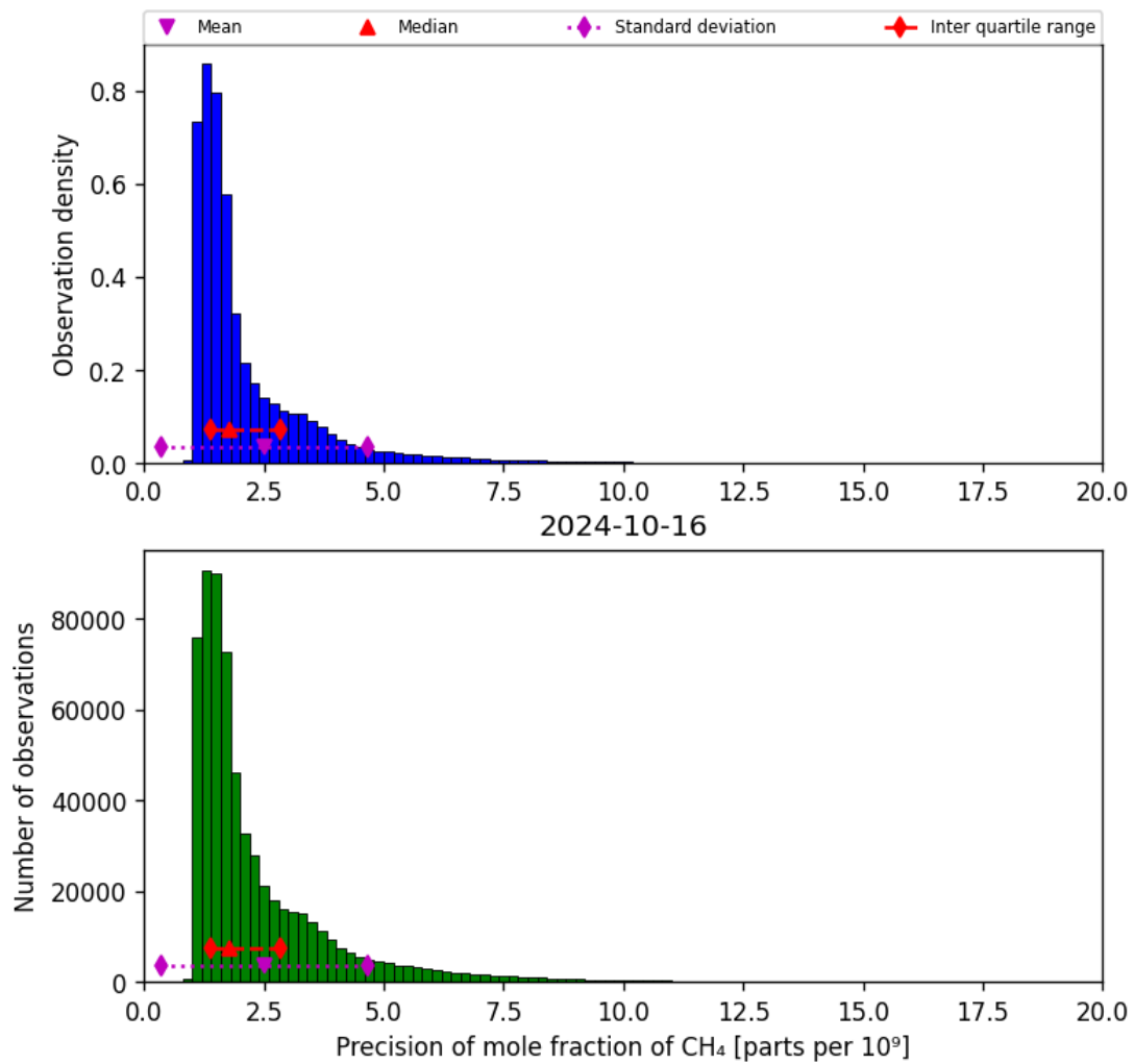
Figure 24: Histogram of “Precision of mole fraction of CH 4 ” for 2024-10-15 to 2024-10-17
