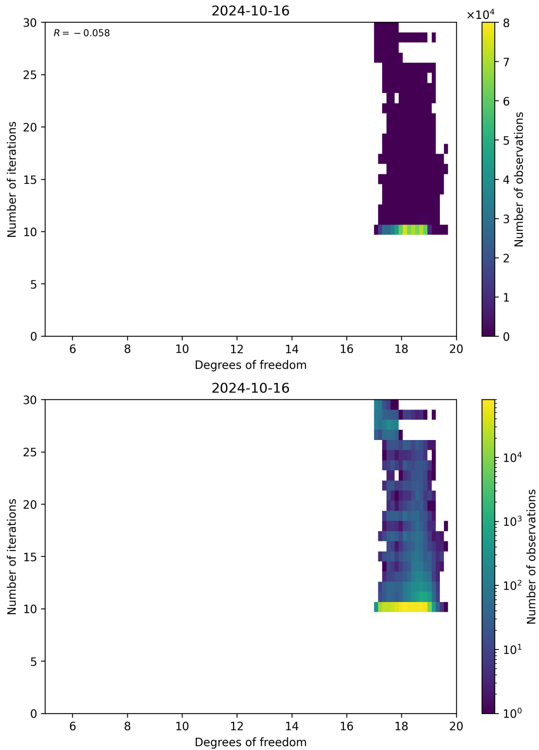
Figure 52: Scatter density plot of “Degrees of freedom” against “Number of iterations” for 2024-10-15 to 2024-10-17.
