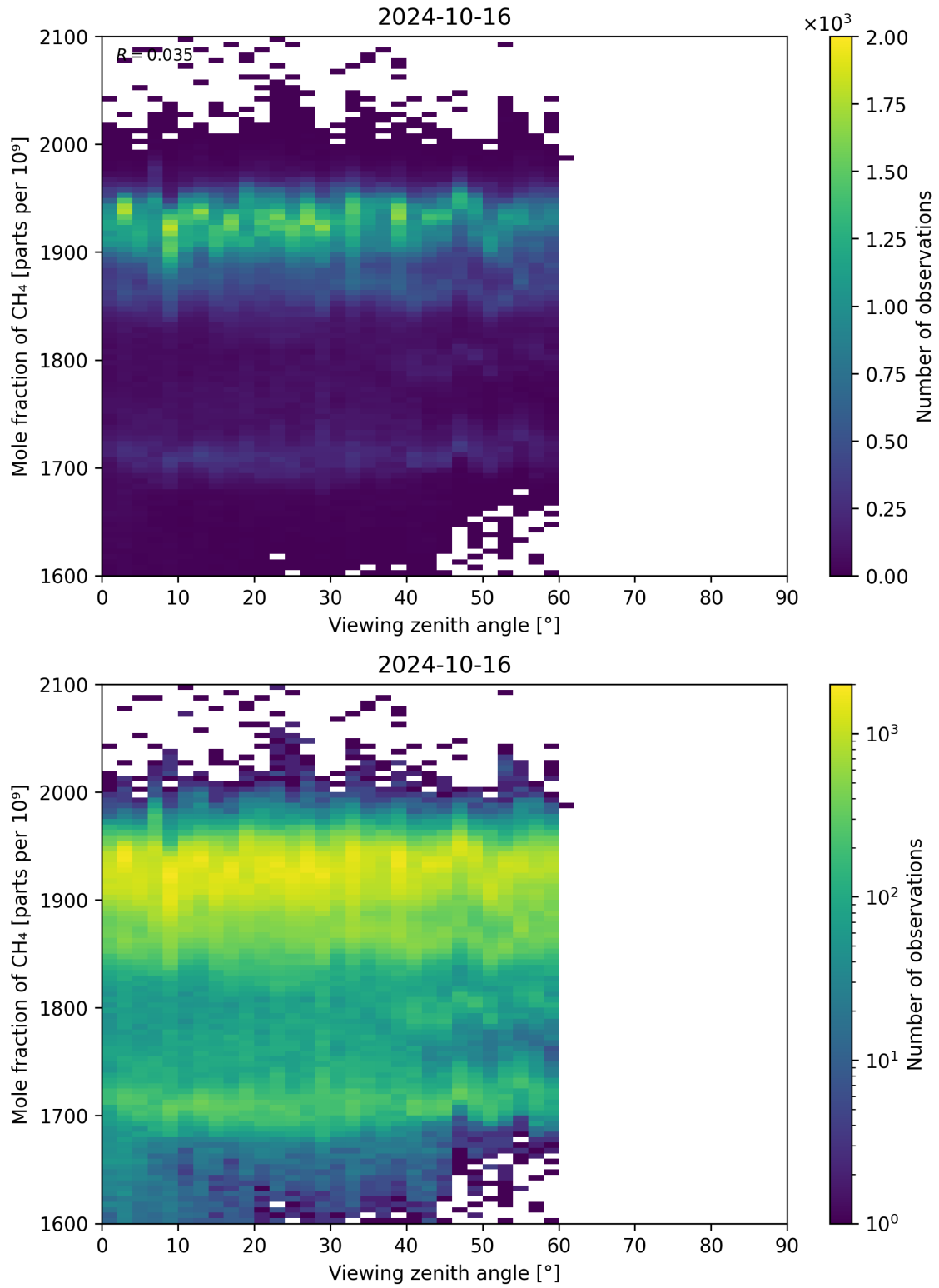
Figure 110: Scatter density plot of “Viewing zenith angle” against “Mole fraction of CH 4 ” for 2024-10-15 to 2024-10-17.
