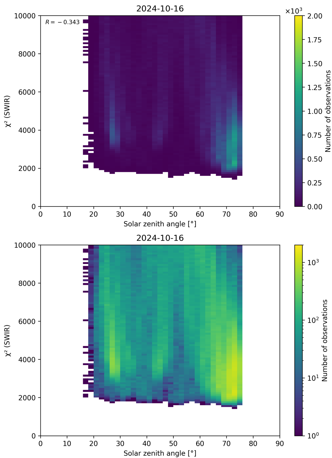
Figure 95: Scatter density plot of “Solar zenith angle” against “ \chi^2 (SWIR)” for 2024-10-15 to 2024-10-17.
