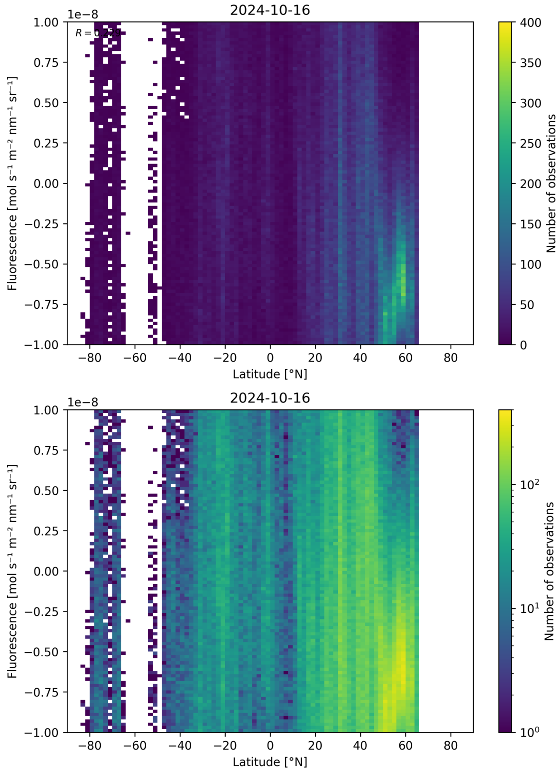
Figure 56: Scatter density plot of “Latitude” against “Fluorescence” for 2024-10-15 to 2024-10-17.
