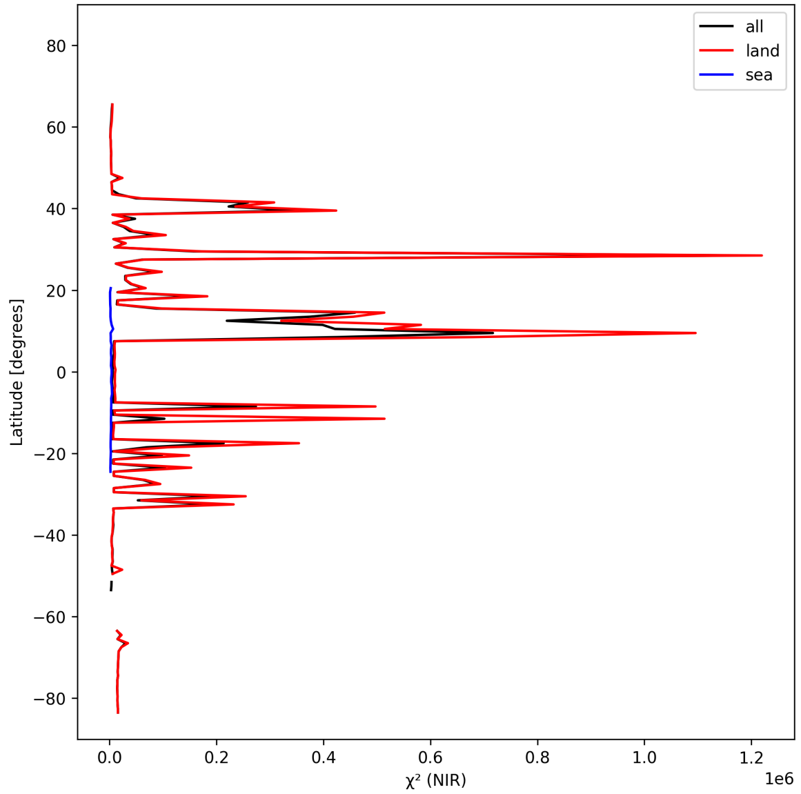
Figure 18: Zonal average of “ \chi^2 (NIR)” for 2024-10-15 to 2024-10-17.
