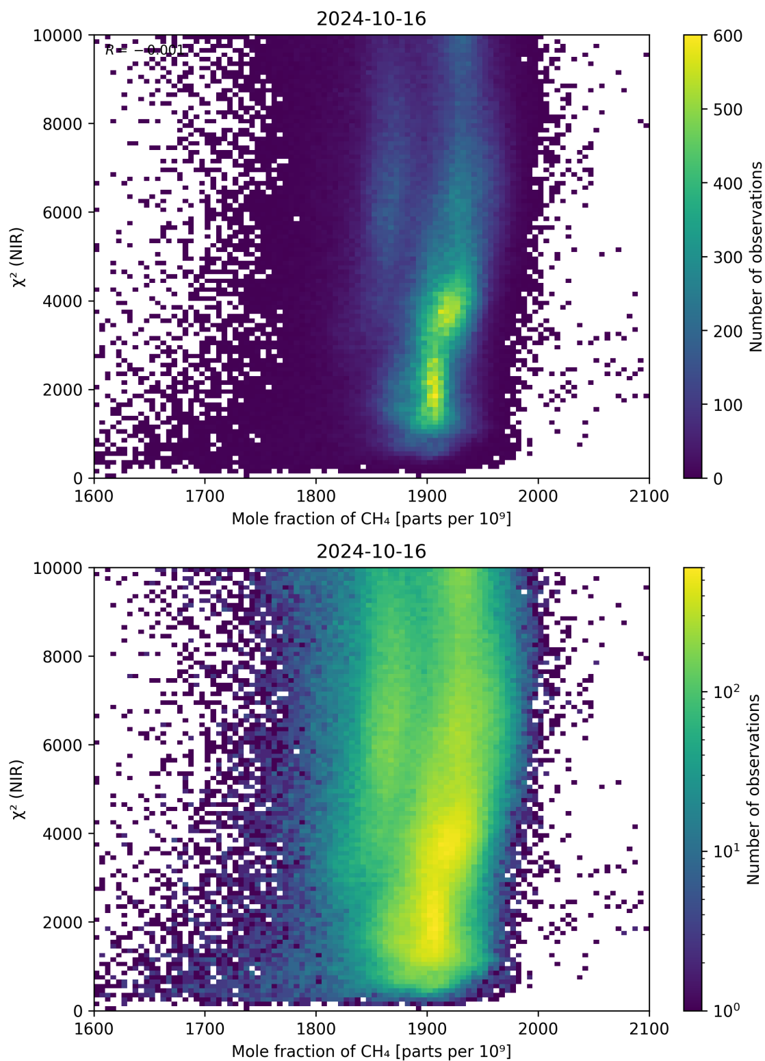
Figure 70: Scatter density plot of “Mole fraction of \text{CH}_4 ” against “ \chi^2 (NIR)” for 2024-10-15 to 2024-10-17.
