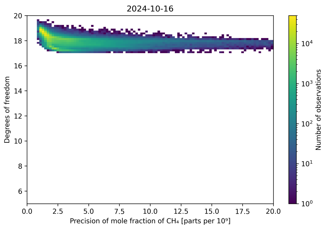
Figure 80: Scatter density plot of “Precision of mole fraction of CH 4 ” against “Degrees of freedom” for 2024-10-15 to 2024-10-17.
