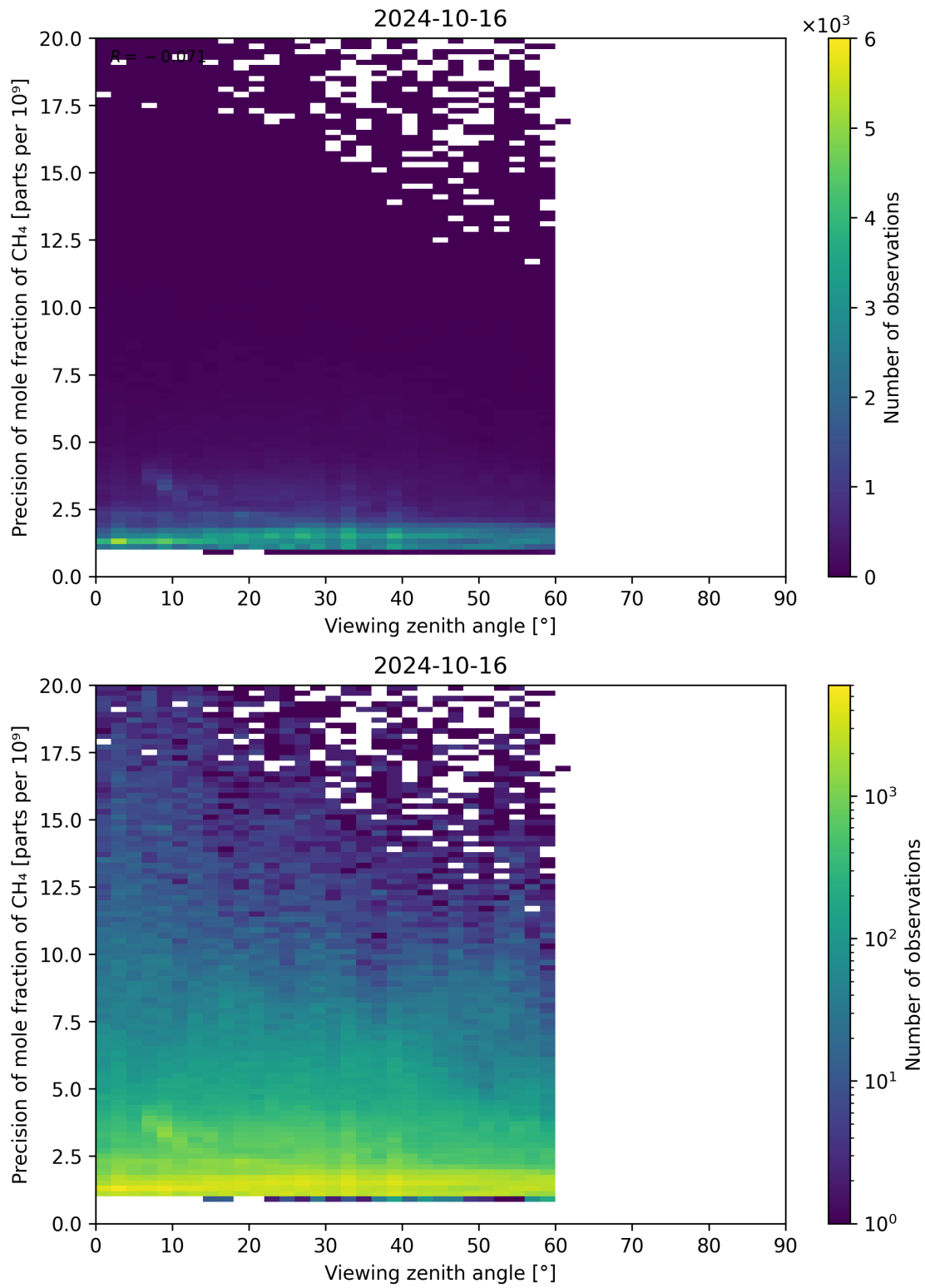
Figure 112: Scatter density plot of “Viewing zenith angle” against “Precision of mole fraction of CH 4 ” for 2024-10-15 to 2024-10-17.
