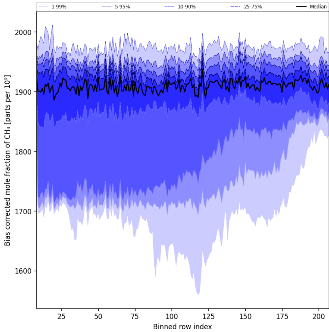
Figure 36: Along track statistics of “Bias corrected mole fraction of CH 4 ” for 2024-10-15 to 2024-10-17
