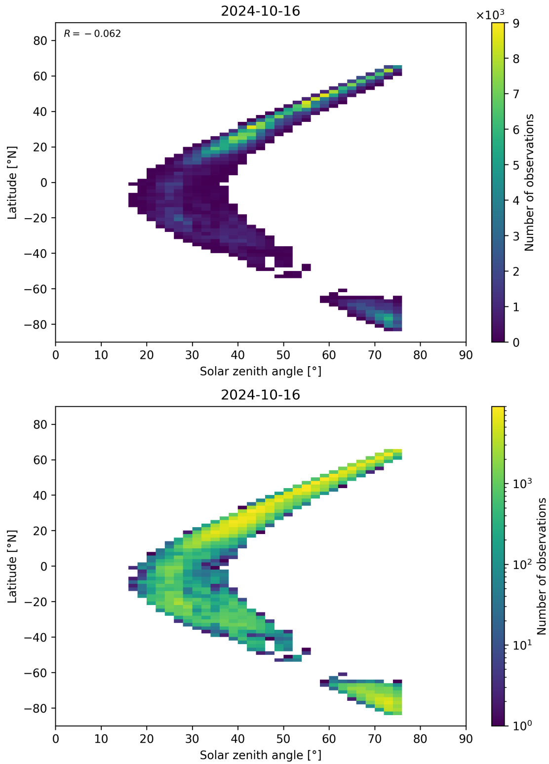
Figure 98: Scatter density plot of “Solar zenith angle” against “Latitude” for 2024-10-15 to 2024-10-17.
