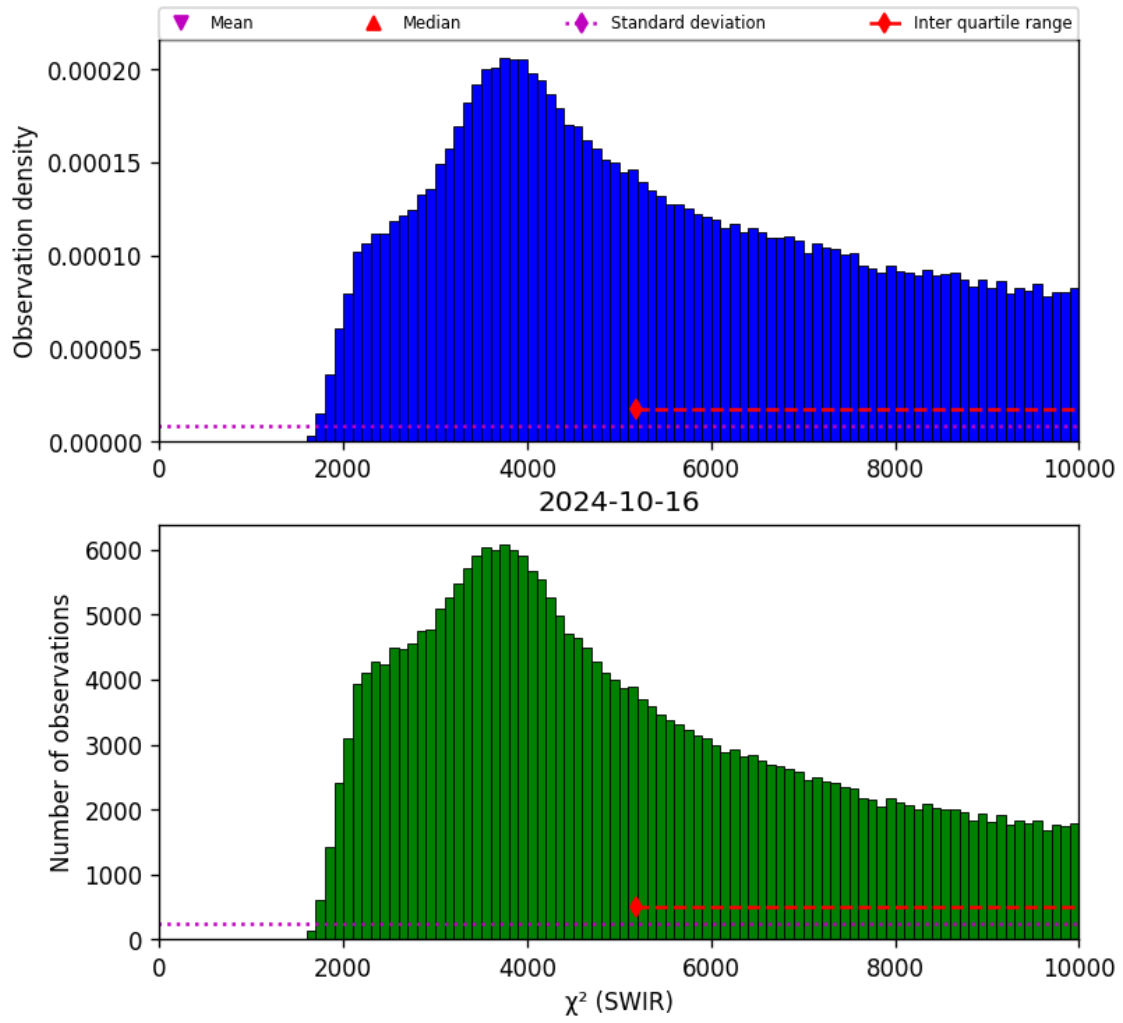
Figure 28: Histogram of “ \chi^2 (SWIR)” for 2024-10-15 to 2024-10-17
