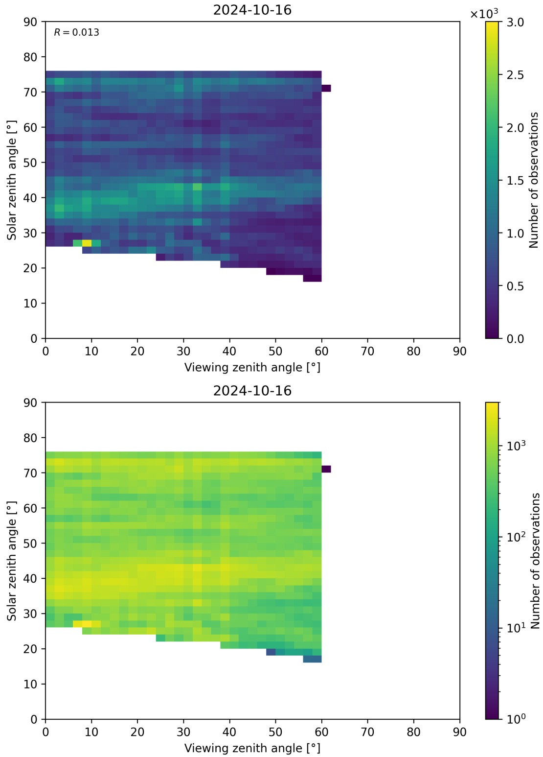
Figure 115: Scatter density plot of “Viewing zenith angle” against “Solar zenith angle” for 2024-10-15 to 2024-10-17.
