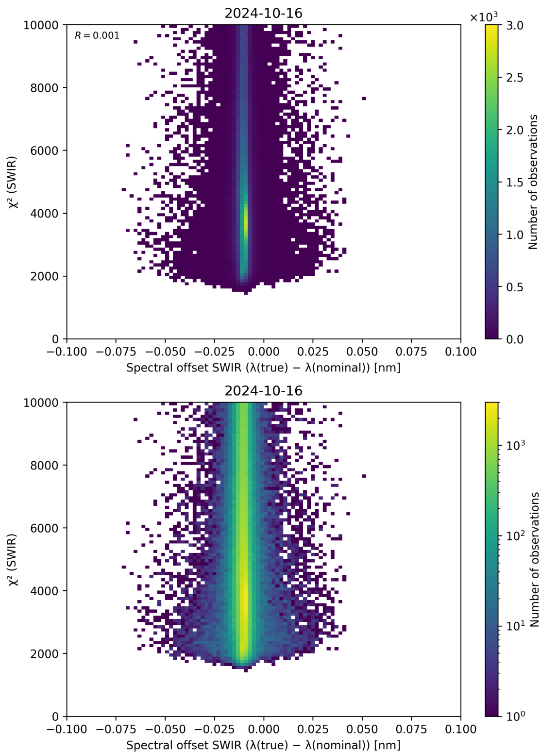
Figure 118: Scatter density plot of “Spectral offset SWIR ( \lambda_{\text{true}} - \lambda_{\text{nominal}} )” against “ \chi^2 (SWIR)” for 2024-10-15 to 2024-10-17.
