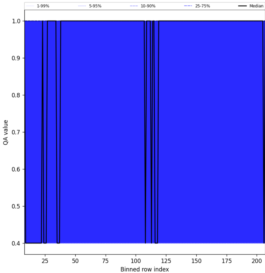
Figure 33: Along track statistics of “QA value” for 2024-10-15 to 2024-10-17
