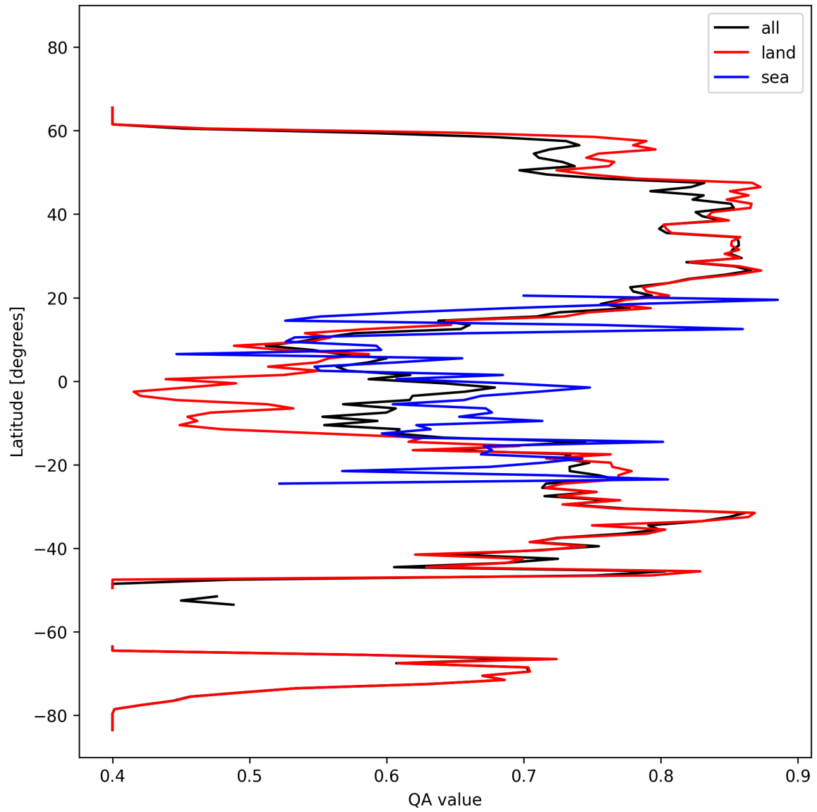
Figure 11: Zonal average of “QA value” for 2024-10-15 to 2024-10-17.
