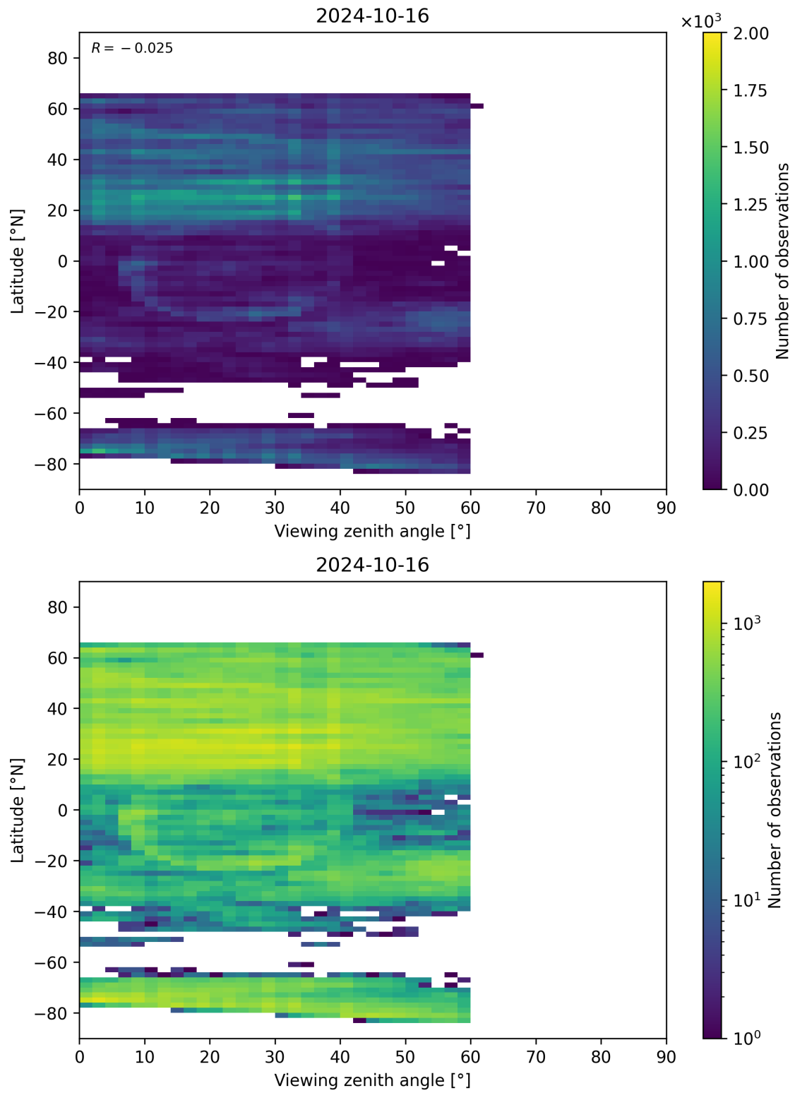
Figure 109: Scatter density plot of “Viewing zenith angle” against “Latitude” for 2024-10-15 to 2024-10-17.
