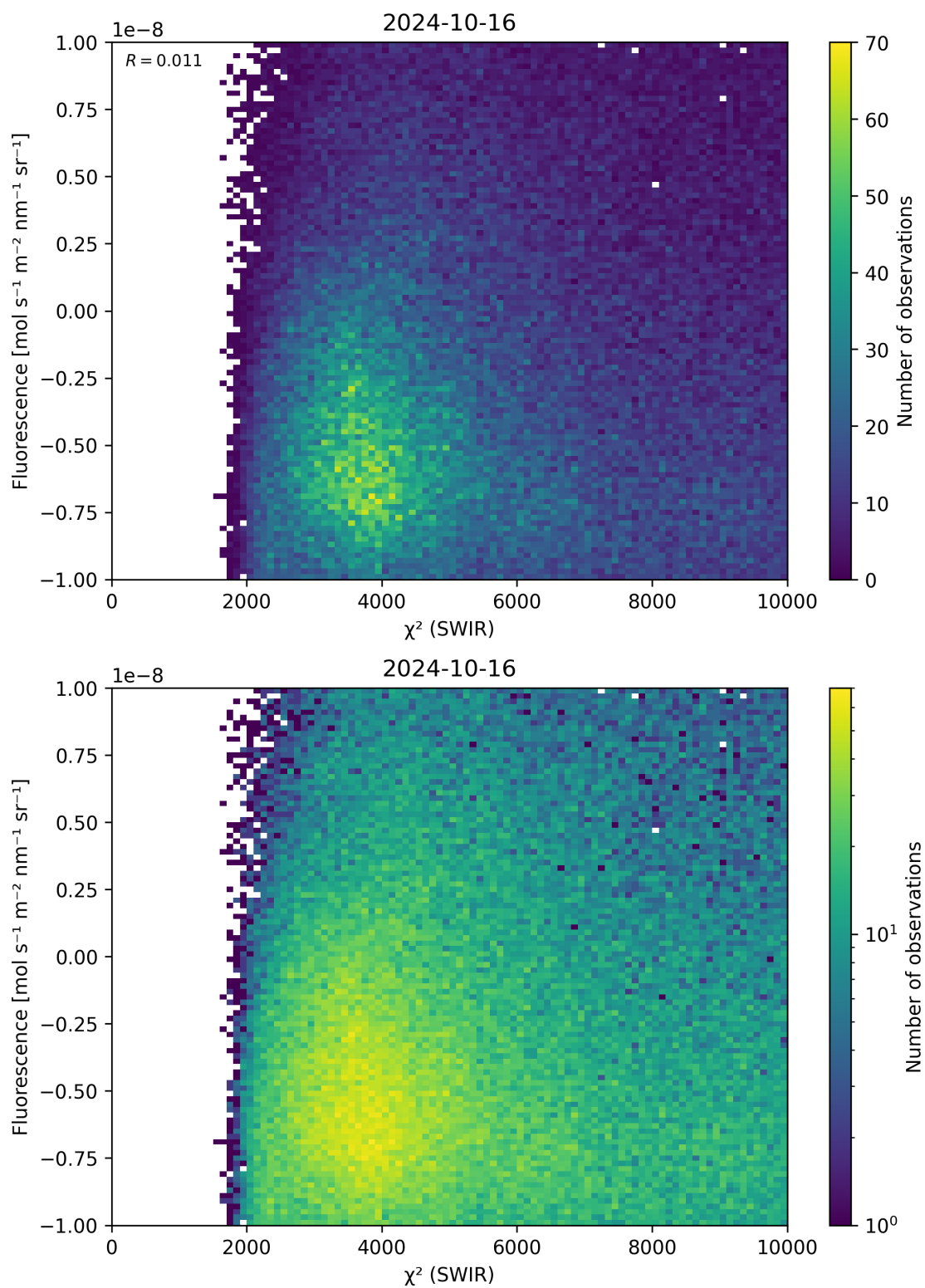
Figure 49: Scatter density plot of “ \chi^2 (SWIR)” against “Fluorescence” for 2024-10-15 to 2024-10-17.
