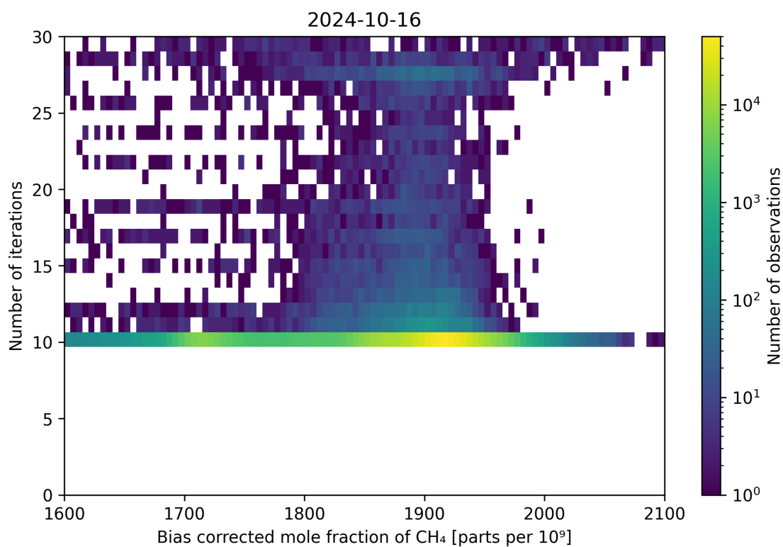
Figure 67: Scatter density plot of “Bias corrected mole fraction of CH 4 ” against “Number of iterations” for 2024-10-15 to 2024-10-17.
