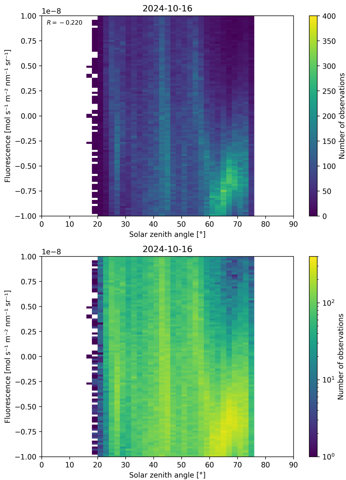
Figure 97: Scatter density plot of “Solar zenith angle” against “Fluorescence” for 2024-10-15 to 2024-10-17.
