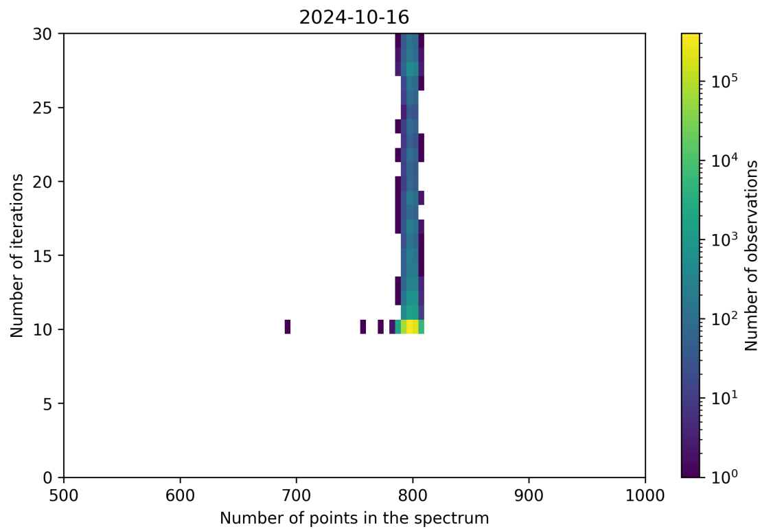
Figure 92: Scatter density plot of “Number of points in the spectrum” against “Number of iterations” for 2024-10-15 to 2024-10-17.
