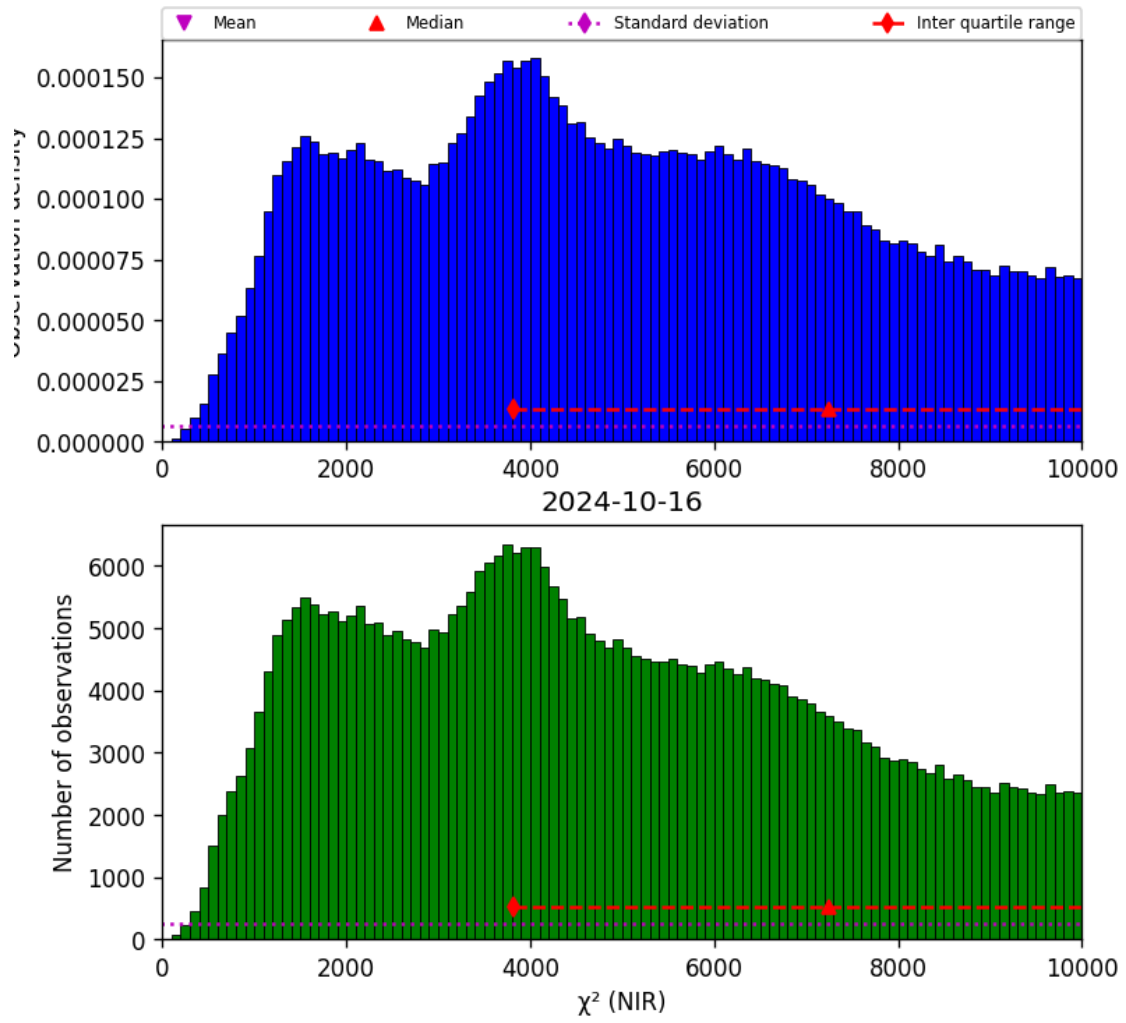
Figure 29: Histogram of “ \chi^2 (NIR)” for 2024-10-15 to 2024-10-17
