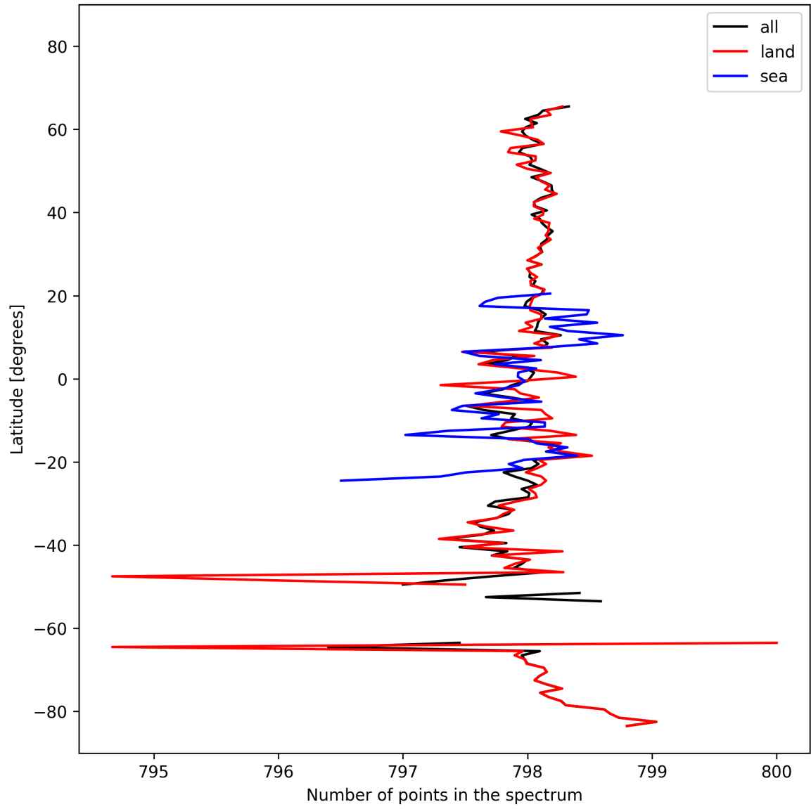
Figure 15: Zonal average of “Number of points in the spectrum” for 2024-10-15 to 2024-10-17.
