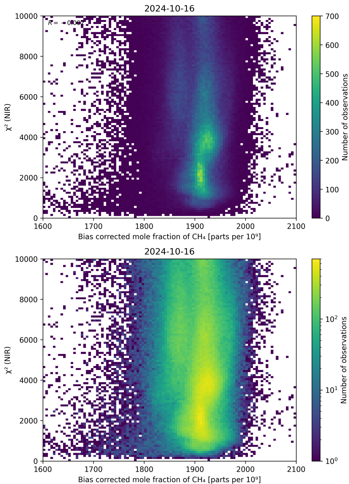
Figure 63: Scatter density plot of “Bias corrected mole fraction of \text{CH}_4 ” against “ \chi^2 (NIR)” for 2024-10-15 to 2024-10-17.
