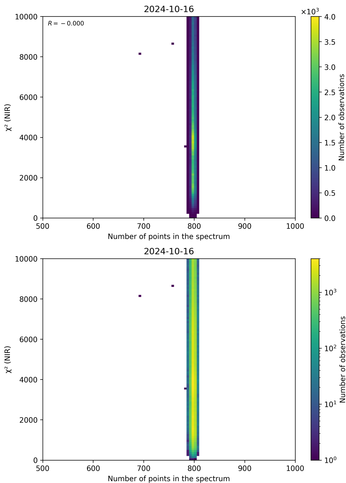
Figure 88: Scatter density plot of “Number of points in the spectrum” against “ \chi^2 (NIR)” for 2024-10-15 to 2024-10-17.
