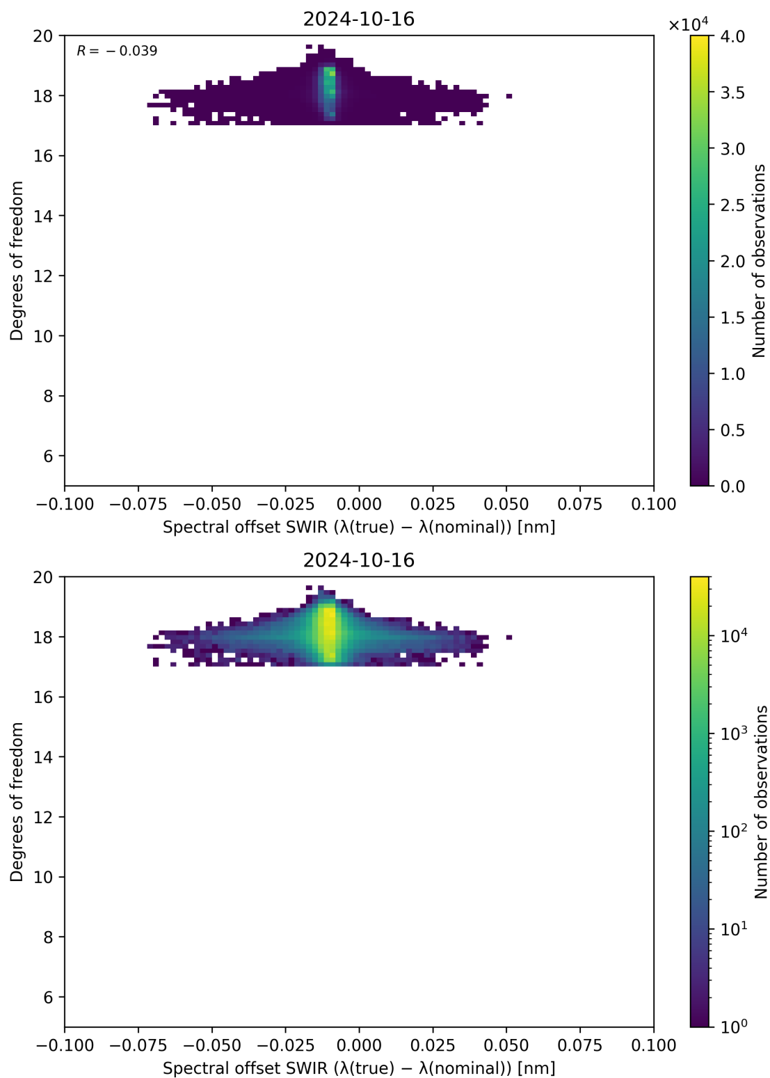
Figure 119: Scatter density plot of “Spectral offset SWIR ( \lambda_{\text{true}} - \lambda_{\text{nominal}} )” against “Degrees of freedom” for 2024-10-15 to 2024-10-17.
