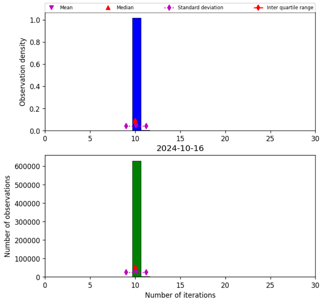
Figure 31: Histogram of “Number of iterations” for 2024-10-15 to 2024-10-17
