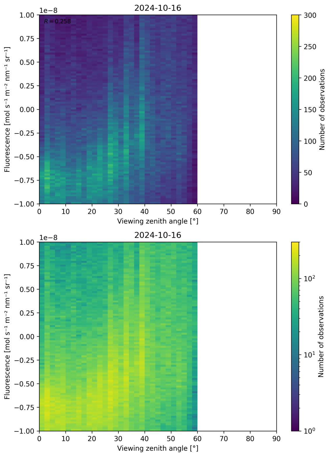
Figure 108: Scatter density plot of “Viewing zenith angle” against “Fluorescence” for 2024-10-15 to 2024-10-17.
