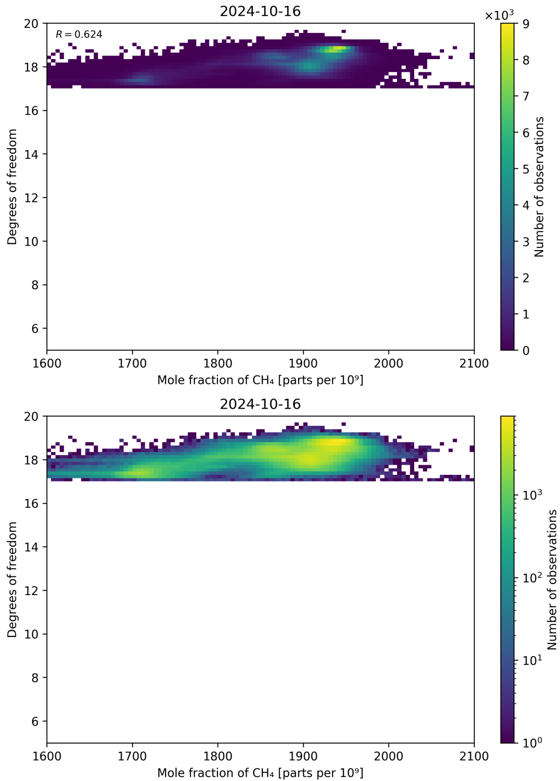
Figure 72: Scatter density plot of “Mole fraction of CH 4 ” against “Degrees of freedom” for 2024-10-15 to 2024-10-17.
