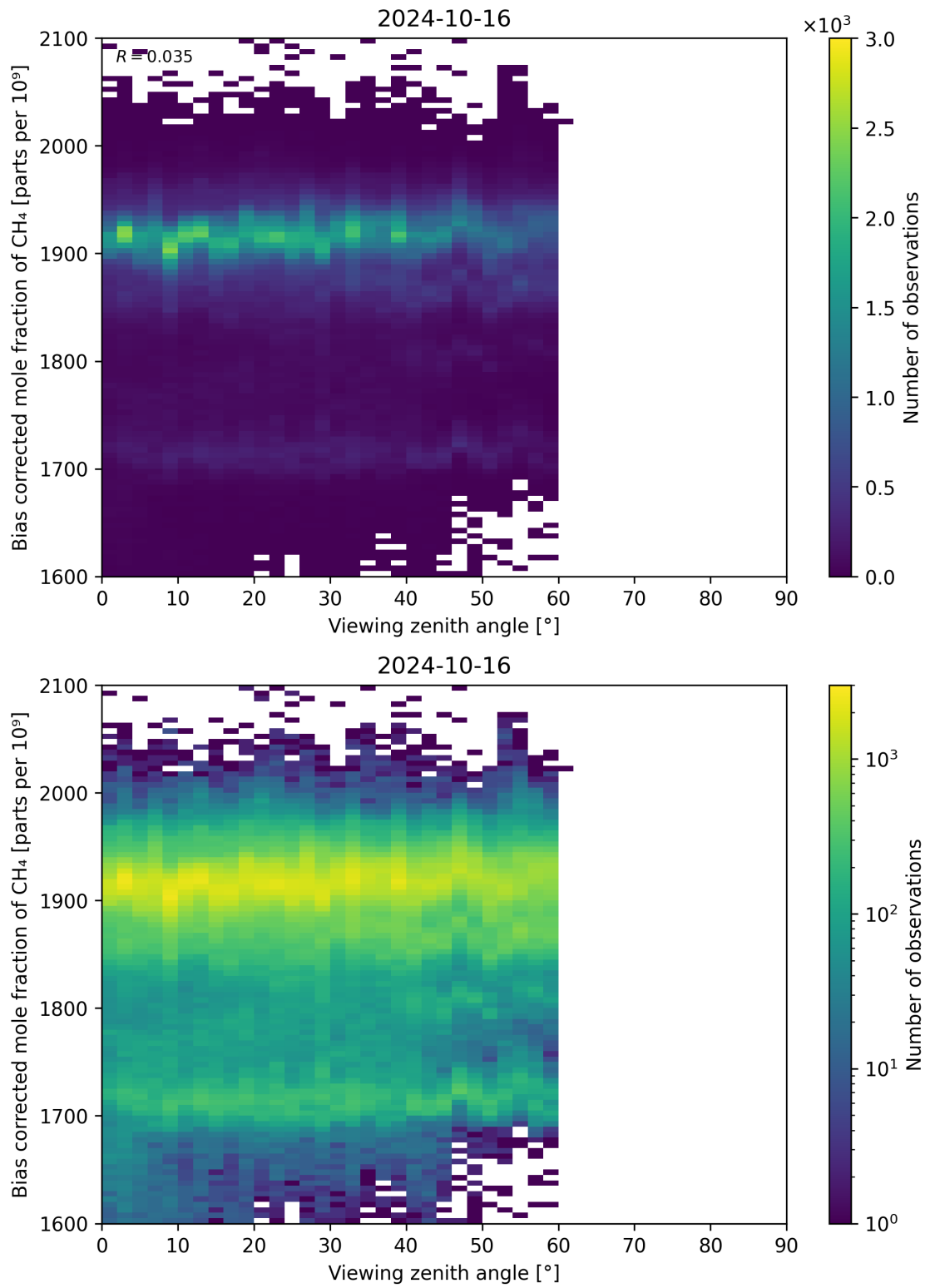
Figure 111: Scatter density plot of “Viewing zenith angle” against “Bias corrected mole fraction of CH 4 ” for 2024-10-15 to 2024-10-17.
