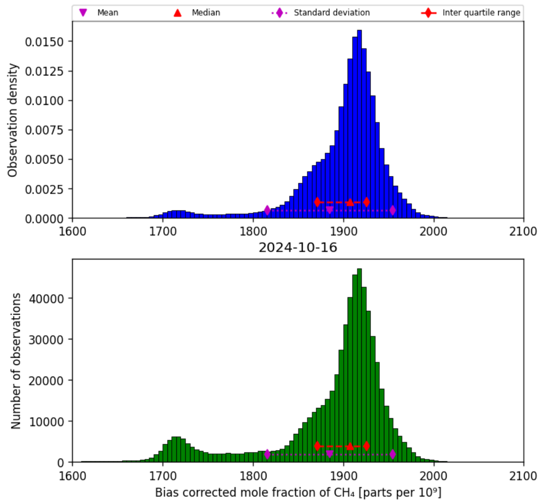
Figure 25: Histogram of “Bias corrected mole fraction of CH 4 ” for 2024-10-15 to 2024-10-17
