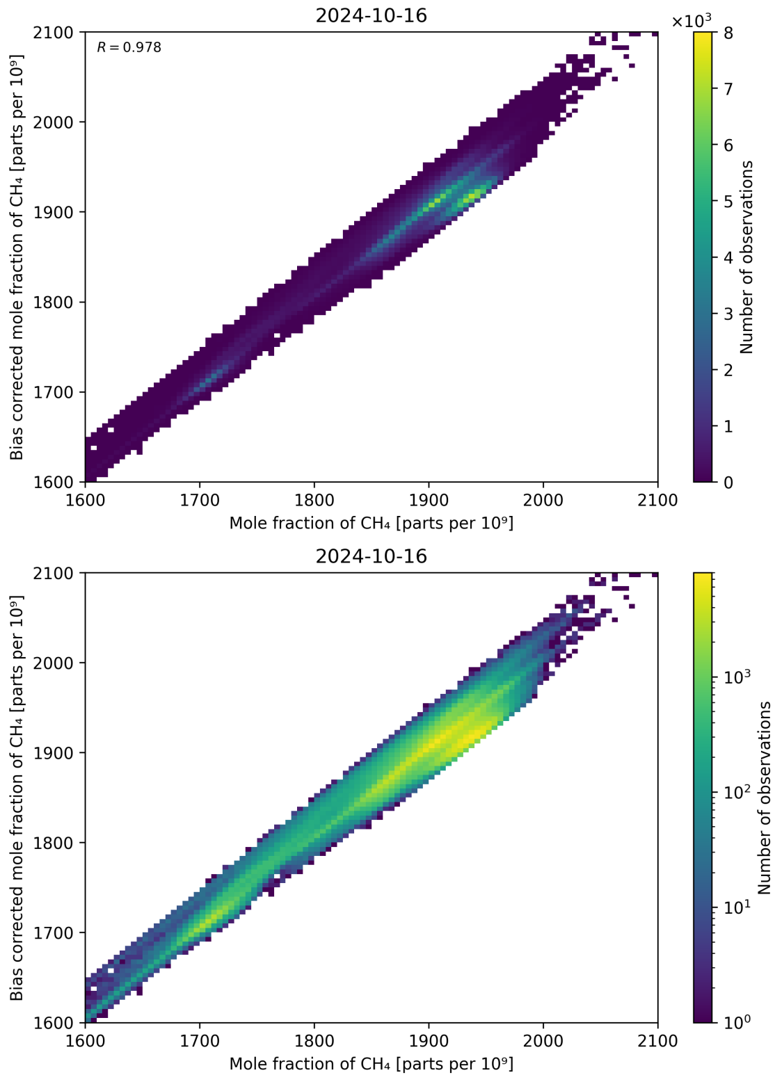
Figure 74: Scatter density plot of “Mole fraction of CH 4 ” against “Bias corrected mole fraction of CH 4 ” for 2024-10-15 to 2024-10-17.
