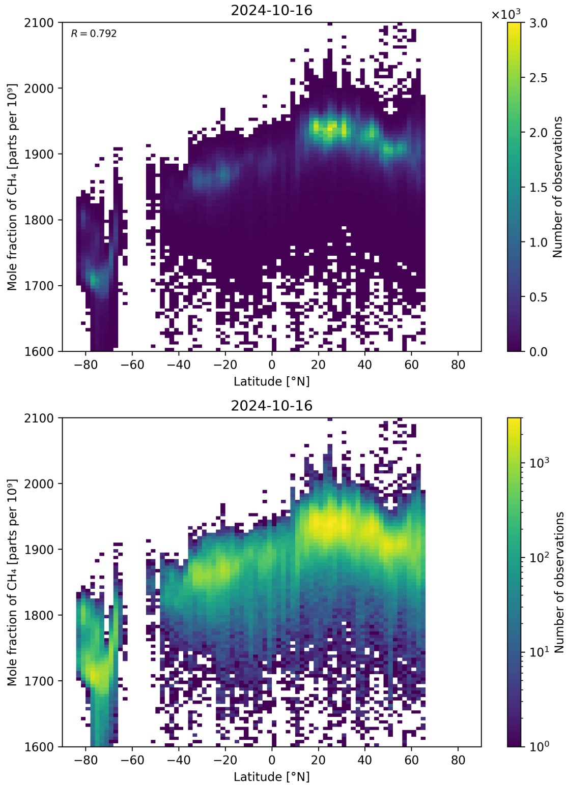
Figure 57: Scatter density plot of “Latitude” against “Mole fraction of CH 4 ” for 2024-10-15 to 2024-10-17.
