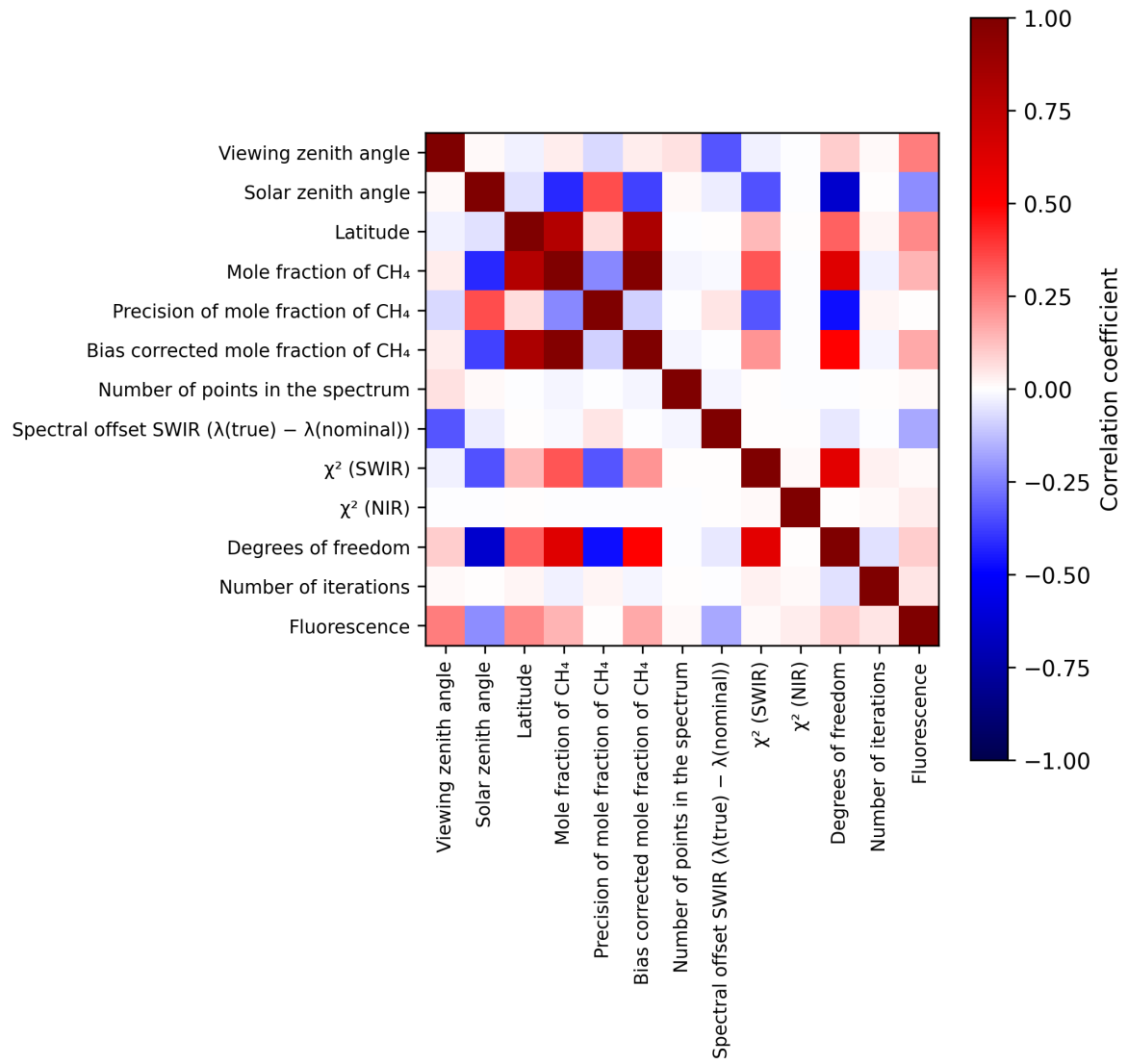
Figure 2: Map of correlation matrix for 2024-10-15 to 2024-10-17.
