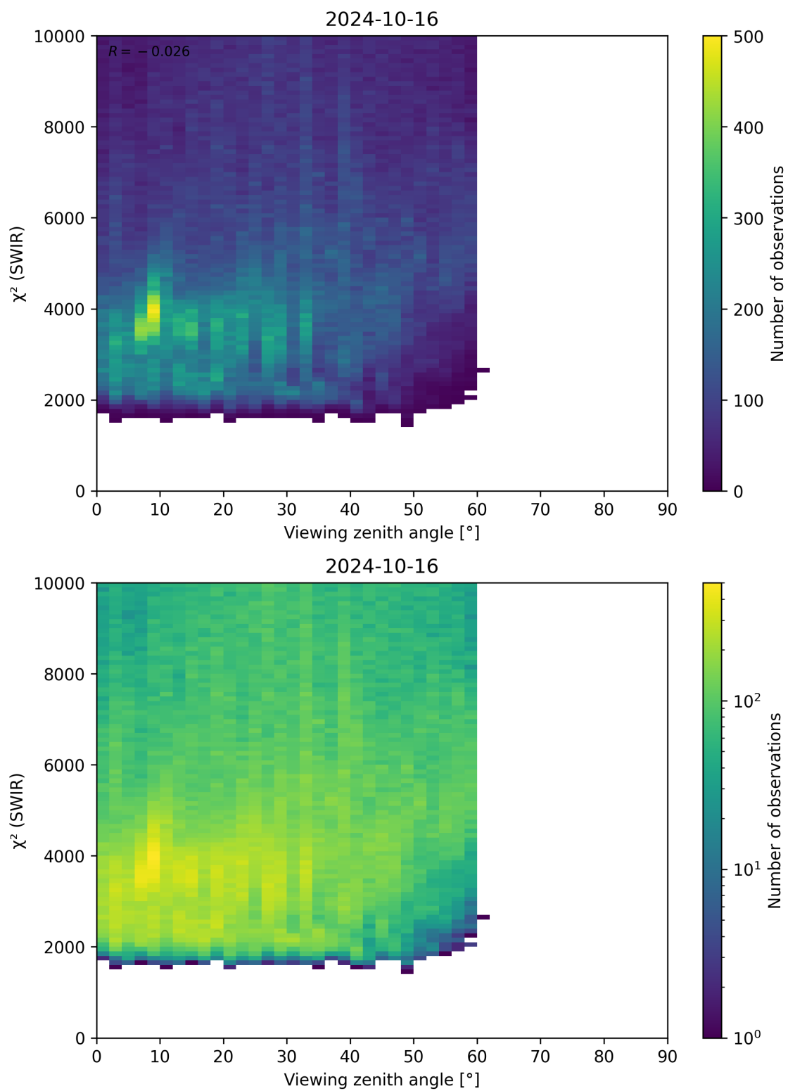
Figure 106: Scatter density plot of “Viewing zenith angle” against “ \chi^2 (SWIR)” for 2024-10-15 to 2024-10-17.
