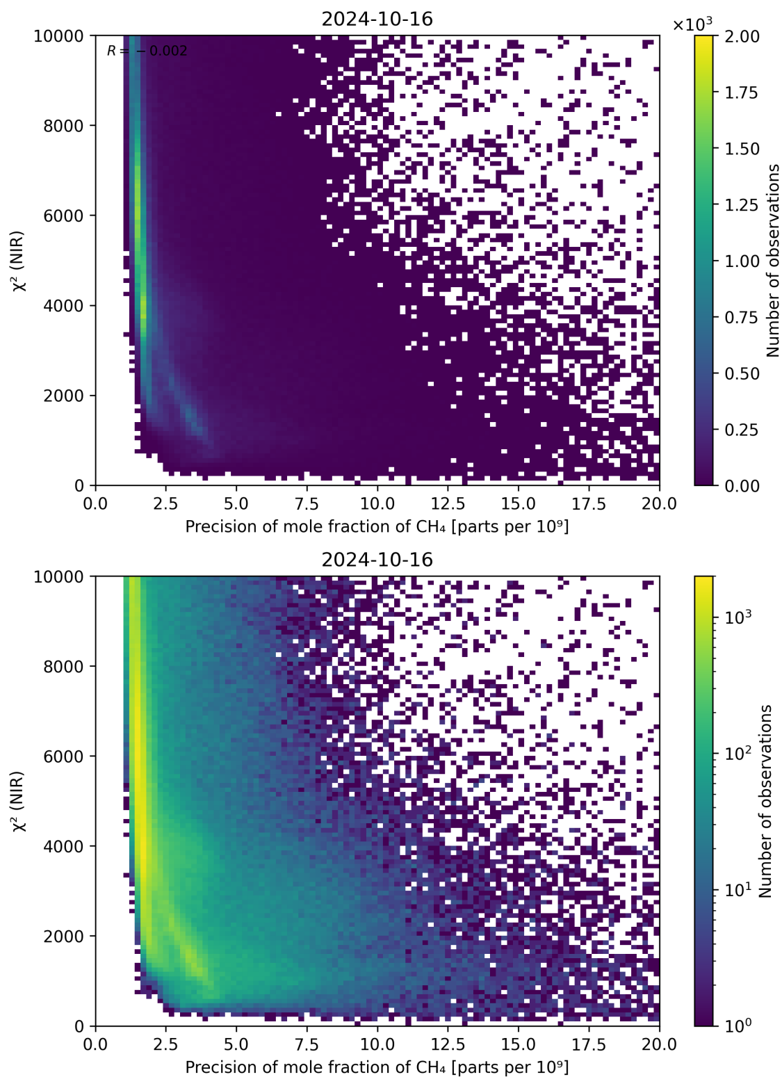
Figure 78: Scatter density plot of “Precision of mole fraction of CH 4 ” against “ \chi^2 (NIR)” for 2024-10-15 to 2024-10-17.
