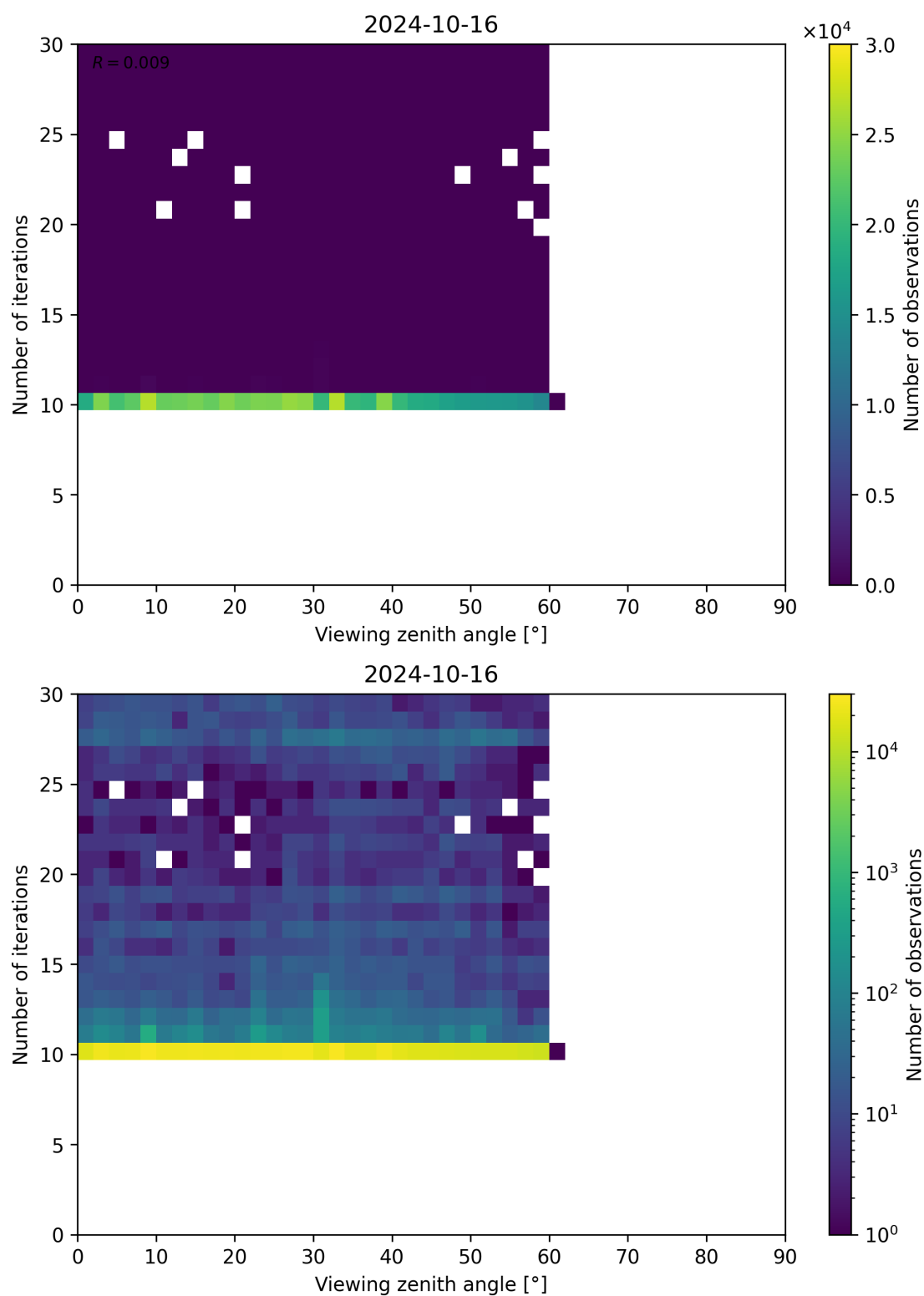
Figure 113: Scatter density plot of “Viewing zenith angle” against “Number of iterations” for 2024-10-15 to 2024-10-17.
