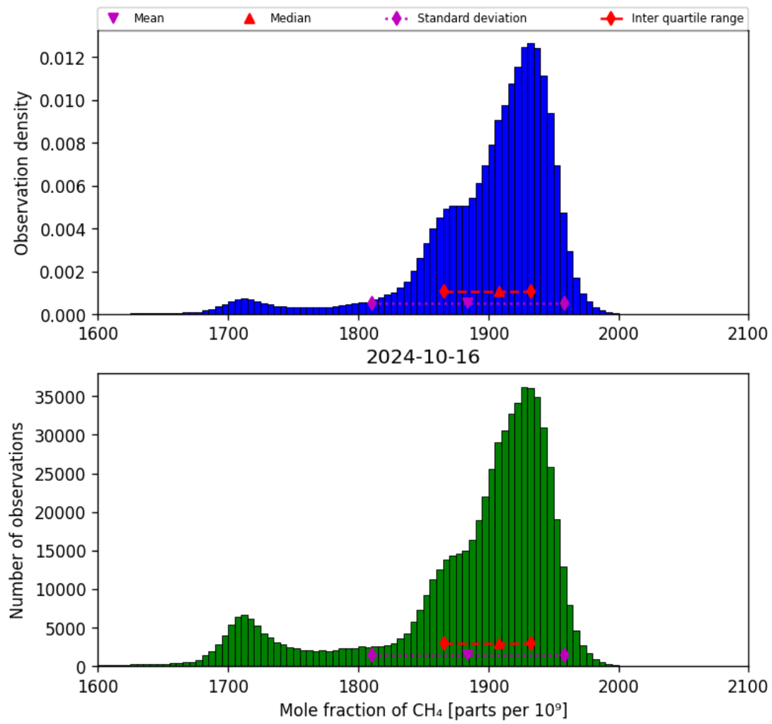
Figure 23: Histogram of “Mole fraction of CH 4 ” for 2024-10-15 to 2024-10-17
