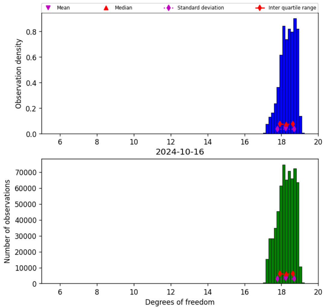
Figure 30: Histogram of “Degrees of freedom” for 2024-10-15 to 2024-10-17
