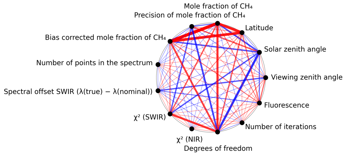
Figure 1: Map of correlation graph for 2024-10-15 to 2024-10-17.
