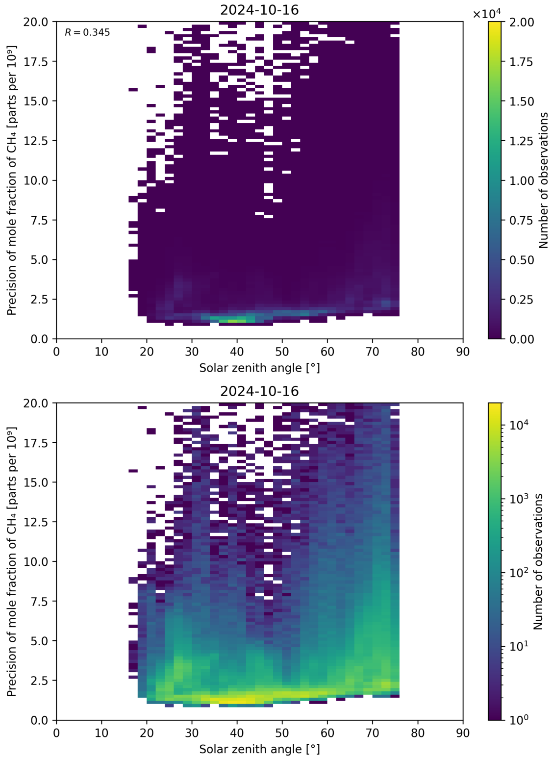
Figure 101: Scatter density plot of “Solar zenith angle” against “Precision of mole fraction of \text{CH}_4 ” for 2024-10-15 to 2024-10-17.
