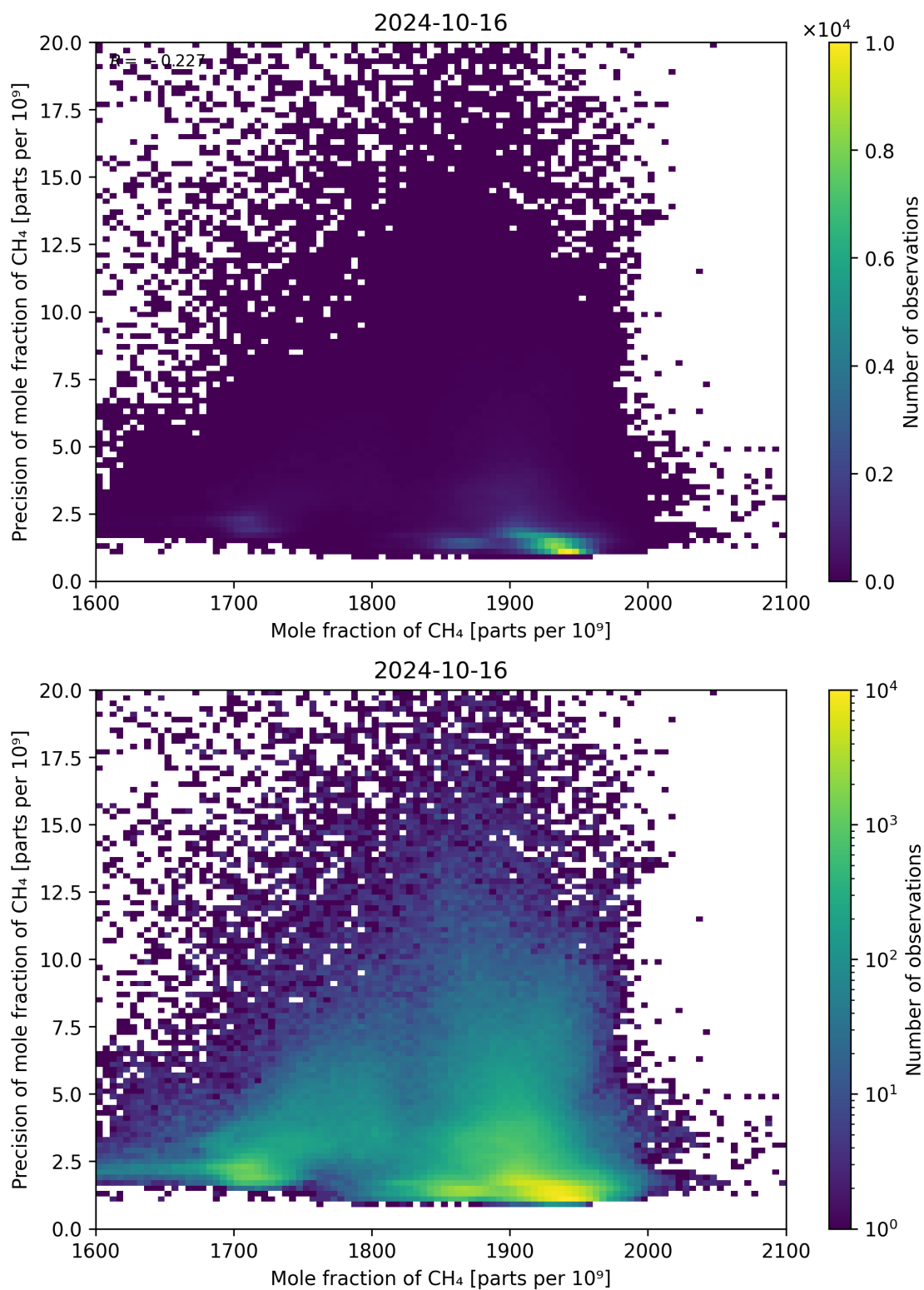
Figure 75: Scatter density plot of “Mole fraction of CH 4 ” against “Precision of mole fraction of CH 4 ” for 2024-10-15 to 2024-10-17.
