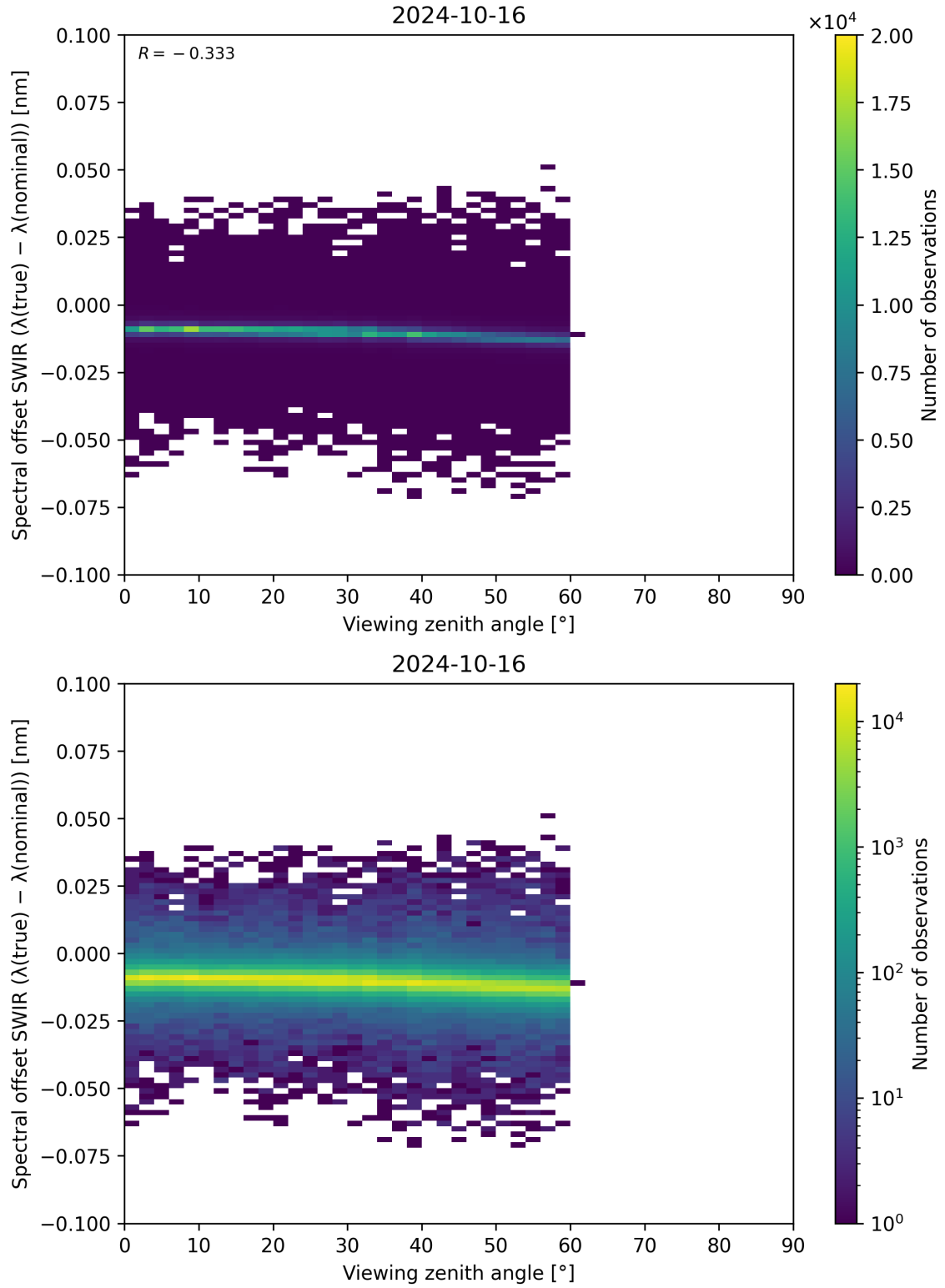
Figure 116: Scatter density plot of “Viewing zenith angle” against “Spectral offset SWIR ( \lambda_{\text{true}} - \lambda_{\text{nominal}} )” for 2024-10-15 to 2024-10-17.
