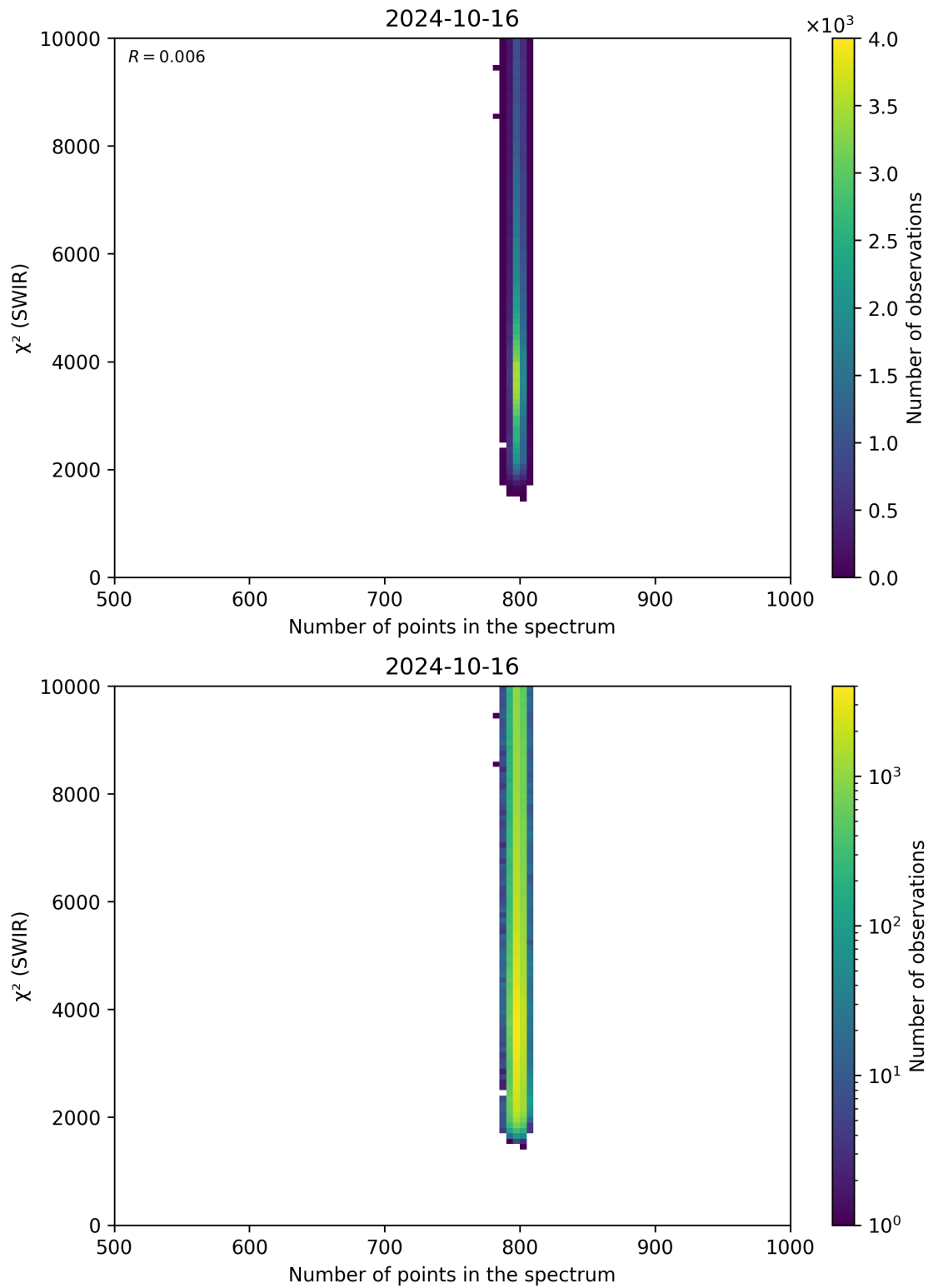
Figure 89: Scatter density plot of “Number of points in the spectrum” against “ \chi^2 (SWIR)” for 2024-10-15 to 2024-10-17.
