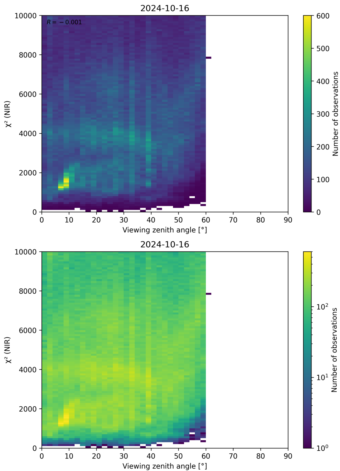
Figure 105: Scatter density plot of “Viewing zenith angle” against “ \chi^2 (NIR)” for 2024-10-15 to 2024-10-17.
