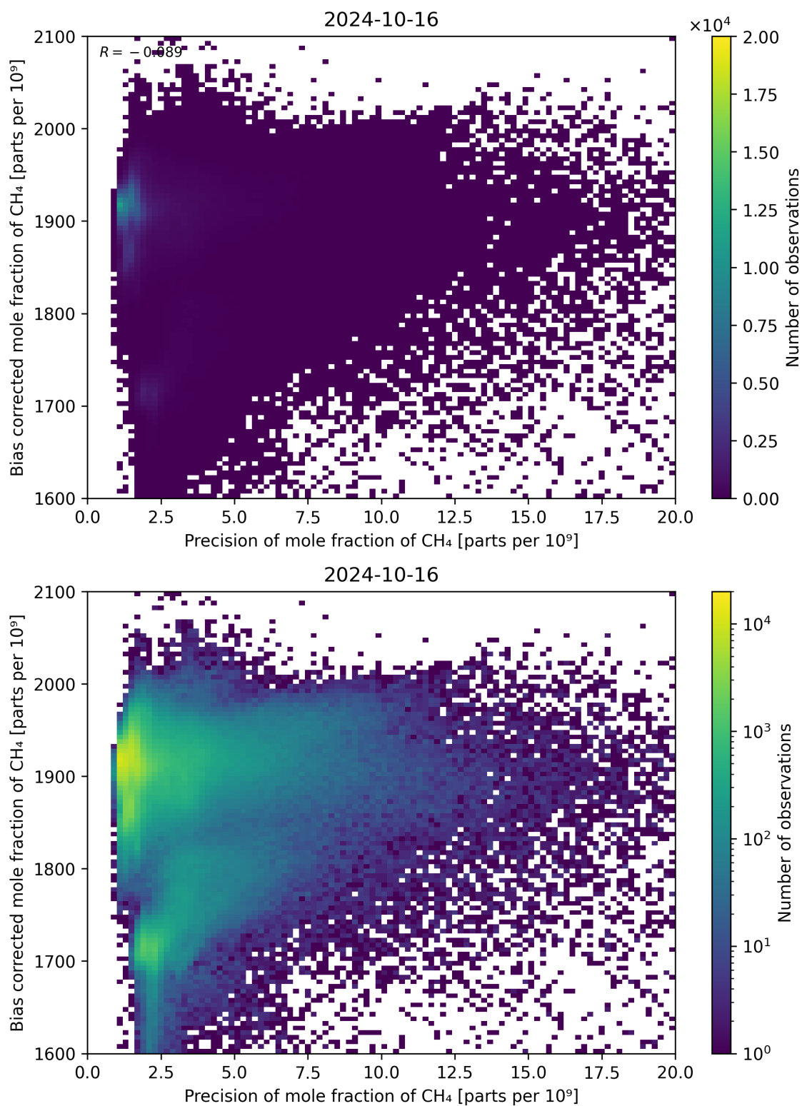
Figure 82: Scatter density plot of “Precision of mole fraction of CH 4 ” against “Bias corrected mole fraction of CH 4 ” for 2024-10-15 to 2024-10-17.
