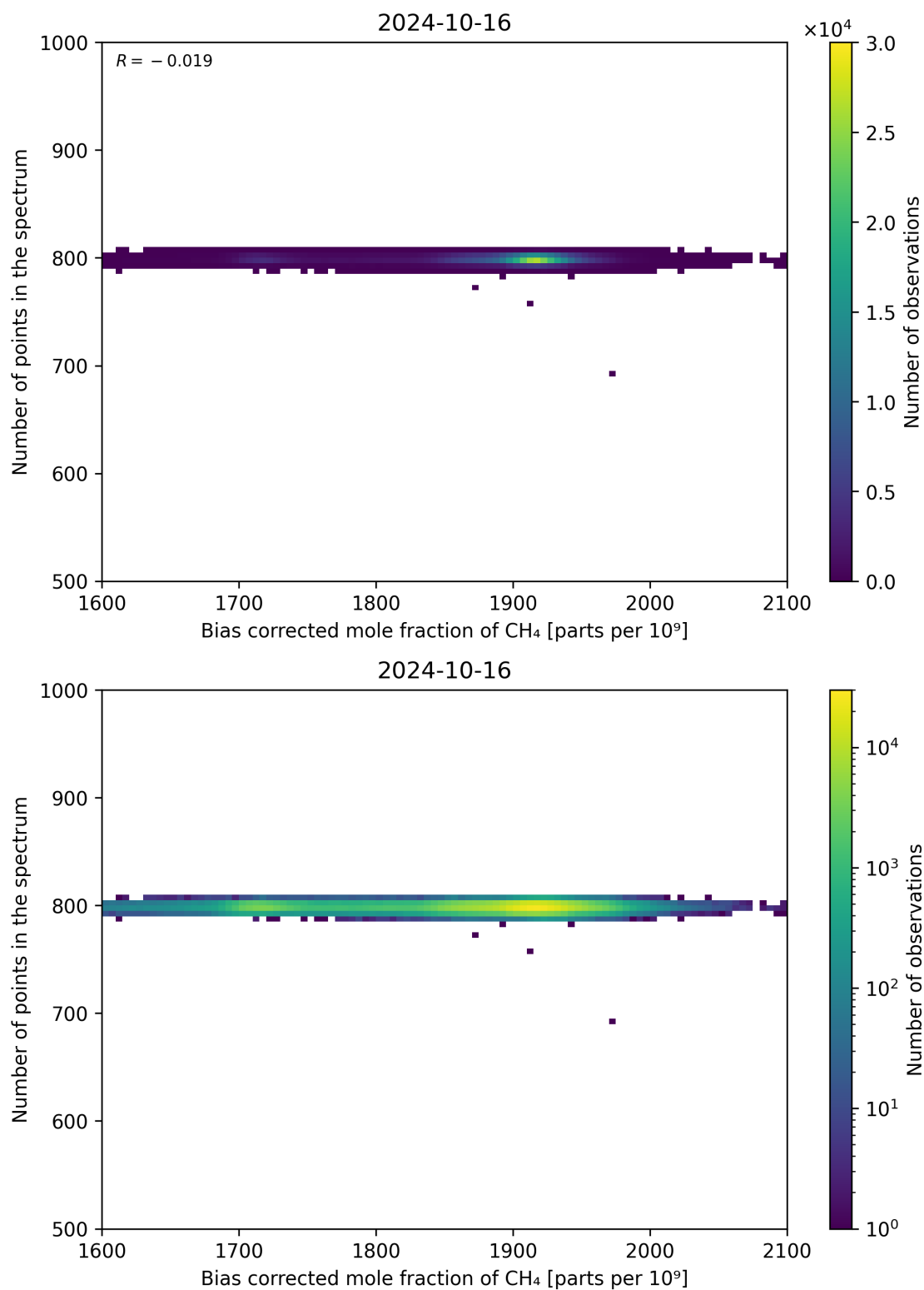
Figure 68: Scatter density plot of “Bias corrected mole fraction of CH 4 ” against “Number of points in the spectrum” for 2024-10-15 to 2024-10-17.
