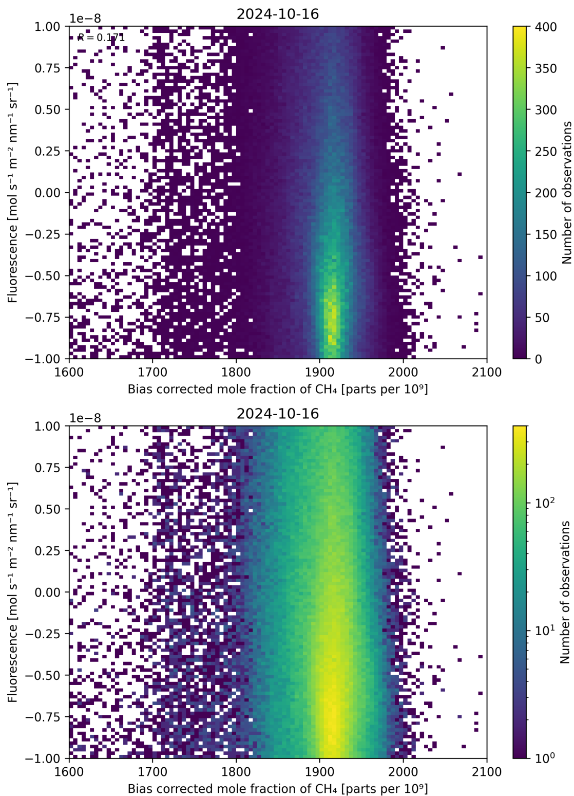
Figure 66: Scatter density plot of “Bias corrected mole fraction of \text{CH}_4 ” against “Fluorescence” for 2024-10-15 to 2024-10-17.
