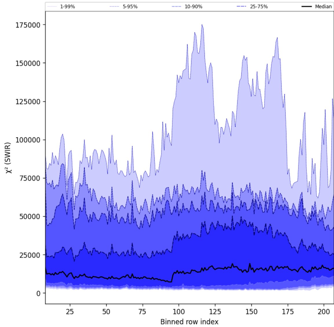
Figure 39: Along track statistics of “ \chi^2 (SWIR)” for 2024-10-15 to 2024-10-17
