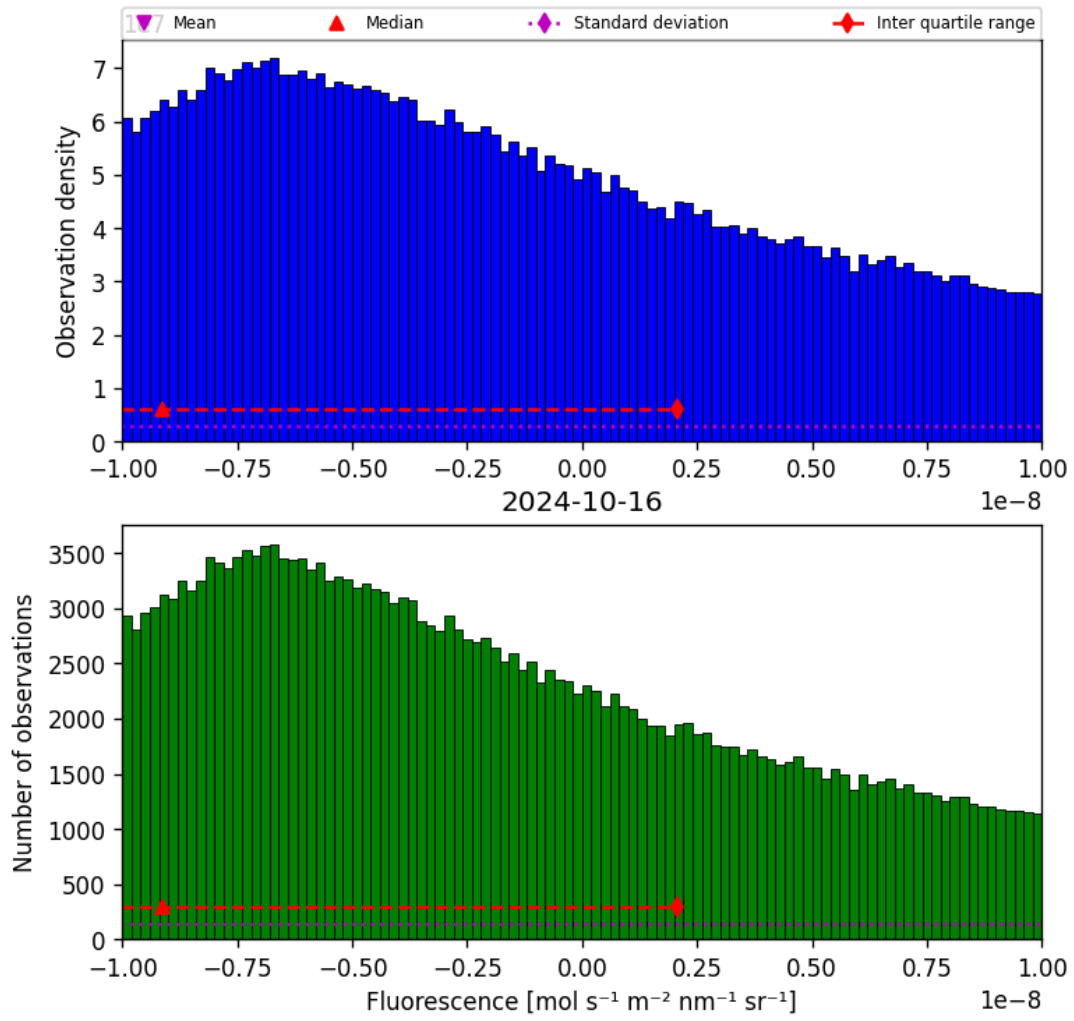
Figure 32: Histogram of “Fluorescence” for 2024-10-15 to 2024-10-17
