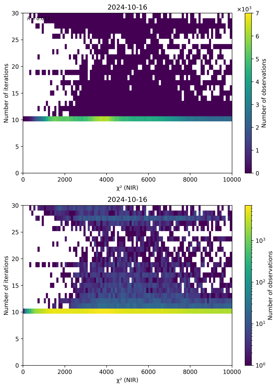
Figure 46: Scatter density plot of “ \chi^2 (NIR)” against “Number of iterations” for 2024-10-15 to 2024-10-17.
