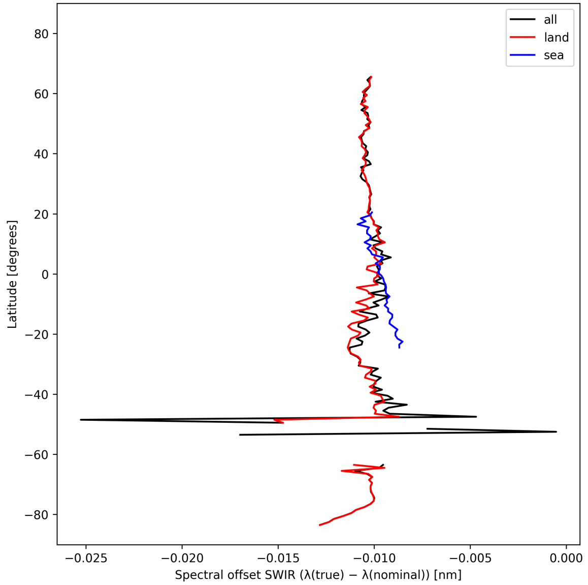
Figure 16: Zonal average of “Spectral offset SWIR ( \lambda_{\text{true}} - \lambda_{\text{nominal}} )” for 2024-10-15 to 2024-10-17.
