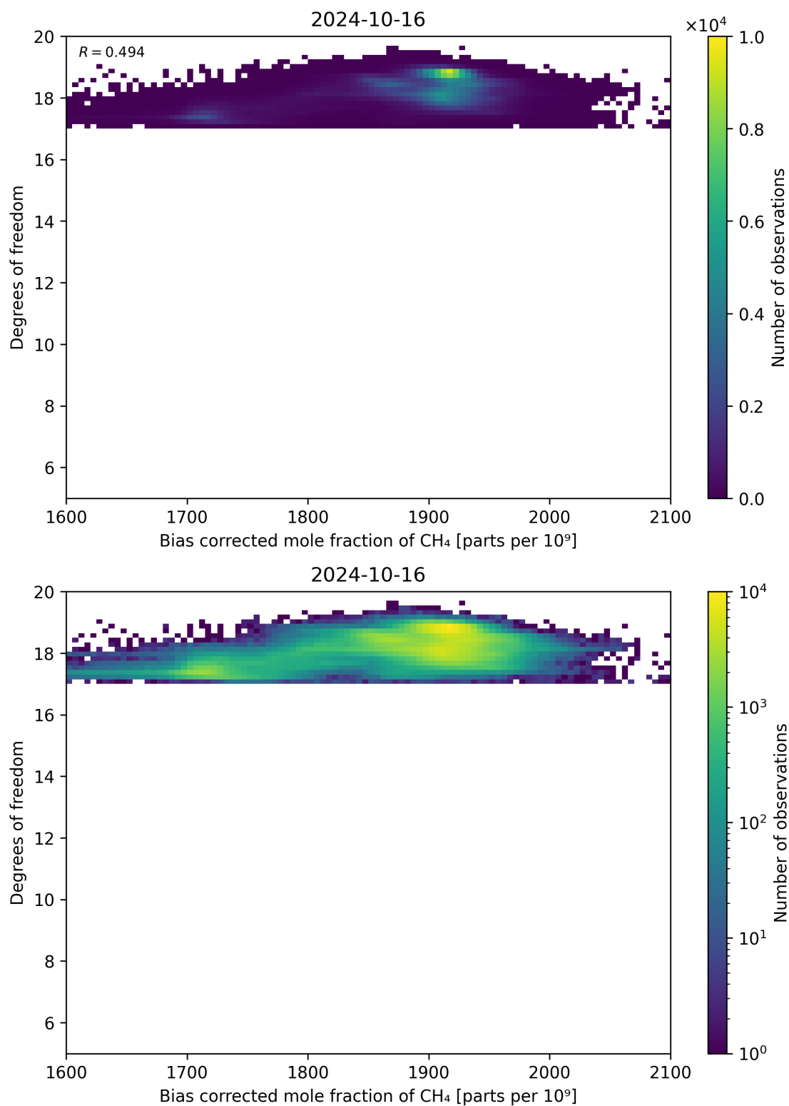
Figure 65: Scatter density plot of “Bias corrected mole fraction of \text{CH}_4 ” against “Degrees of freedom” for 2024-10-15 to 2024-10-17.
