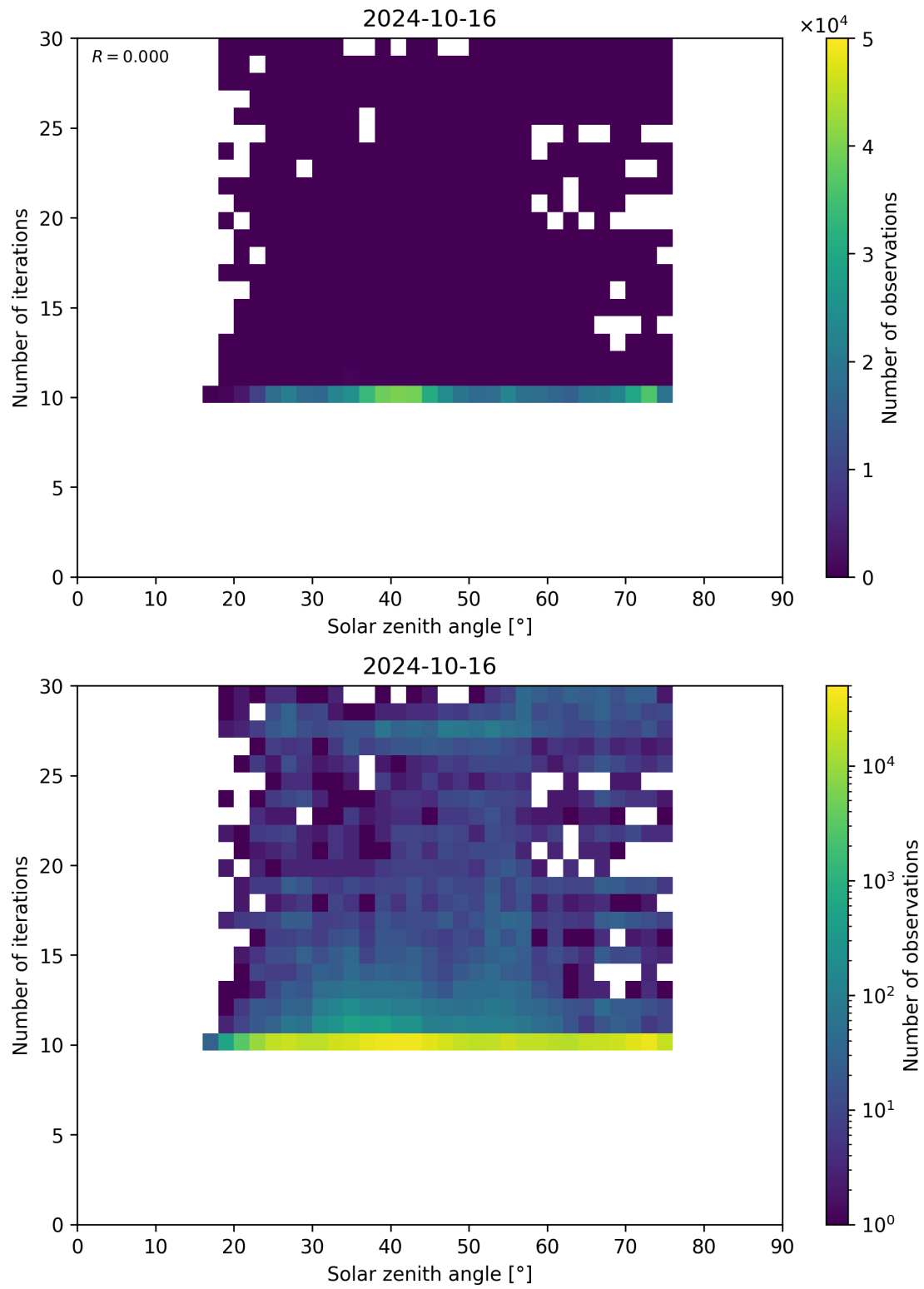
Figure 102: Scatter density plot of “Solar zenith angle” against “Number of iterations” for 2024-10-15 to 2024-10-17.
