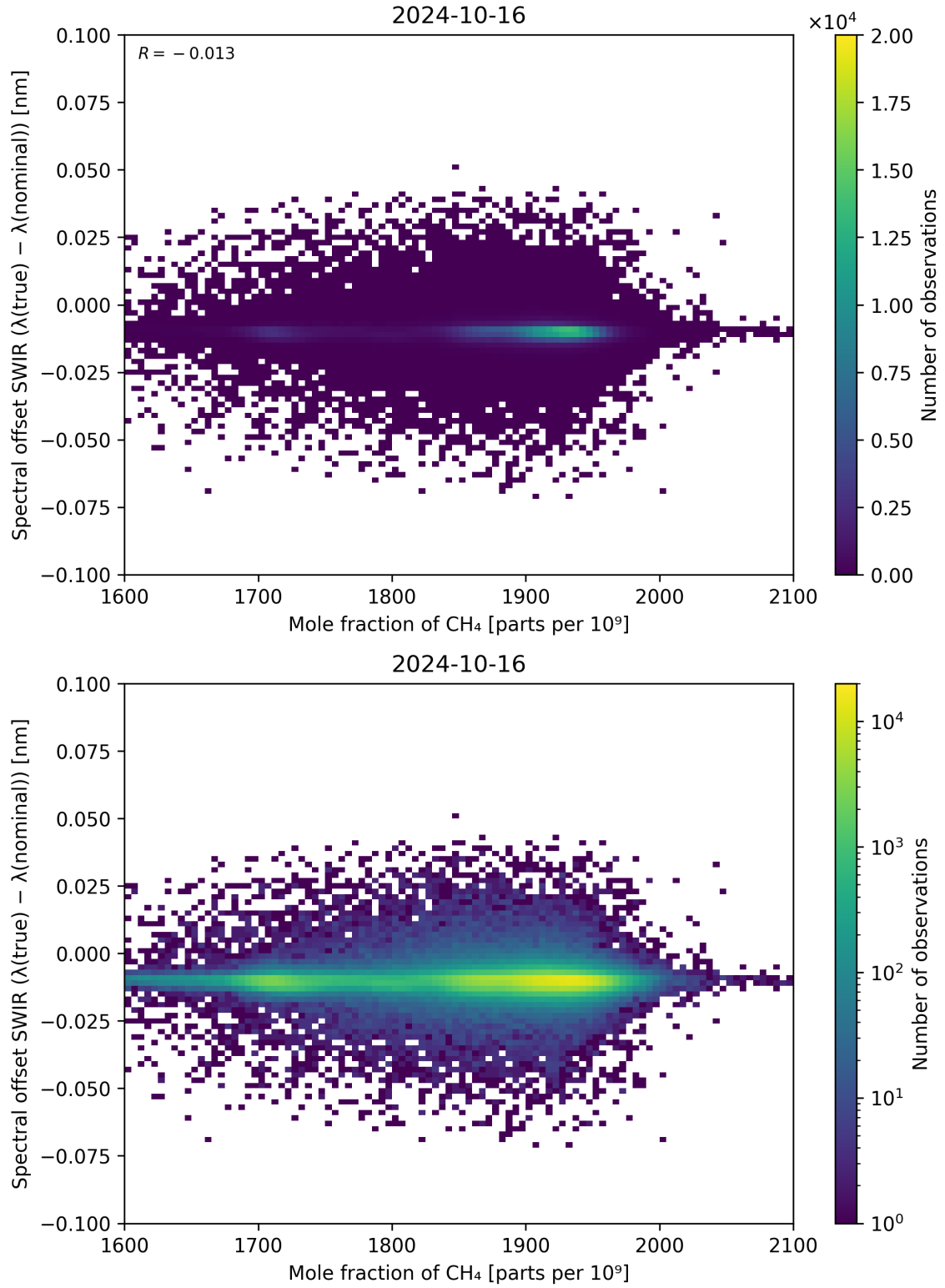
Figure 86: Scatter density plot of “Mole fraction of \text{CH}_4 ” against “Spectral offset SWIR ( \lambda_{\text{true}} - \lambda_{\text{nominal}} )” for 2024-10-15 to 2024-10-17.
