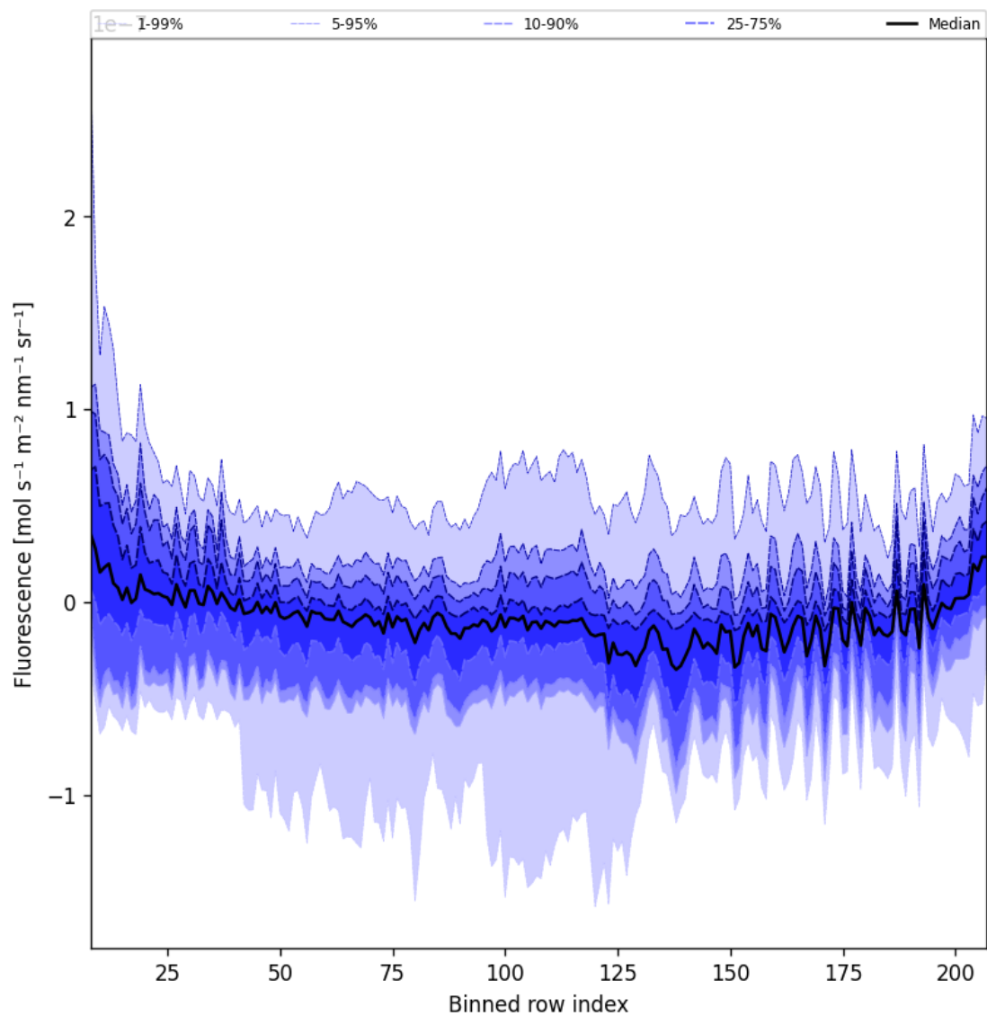
Figure 43: Along track statistics of “Fluorescence” for 2024-10-15 to 2024-10-17
