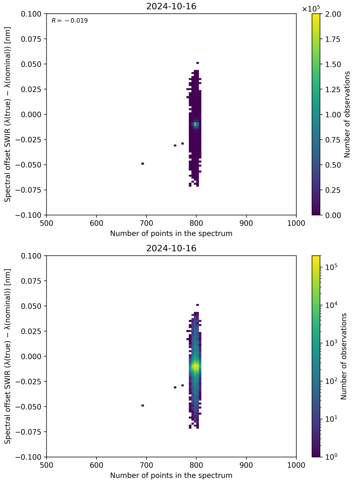
Figure 93: Scatter density plot of “Number of points in the spectrum” against “Spectral offset SWIR ( \lambda_{\text{true}} - \lambda_{\text{nominal}} )” for 2024-10-15 to 2024-10-17.
