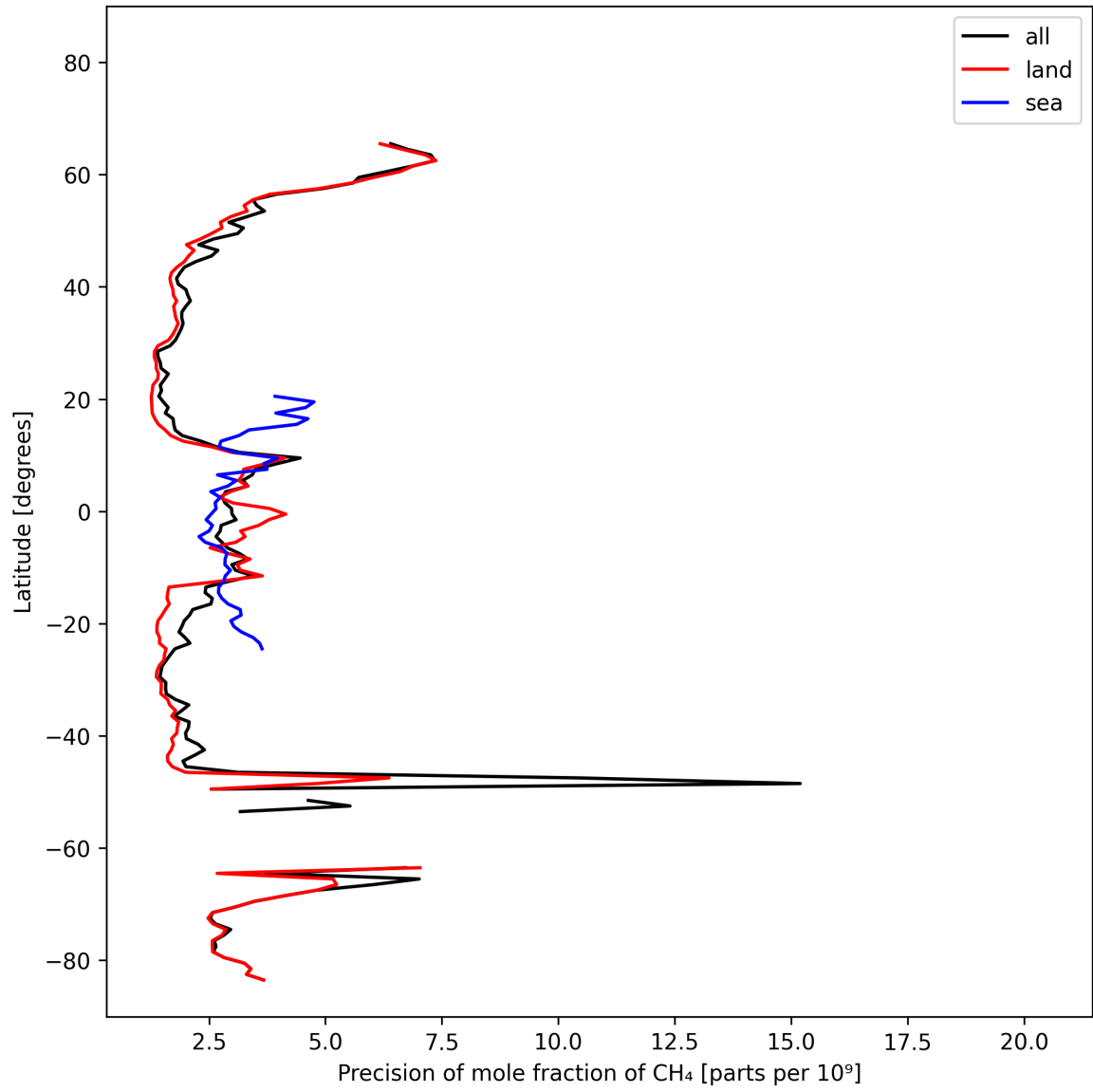
Figure 13: Zonal average of “Precision of mole fraction of CH 4 ” for 2024-10-15 to 2024-10-17.
