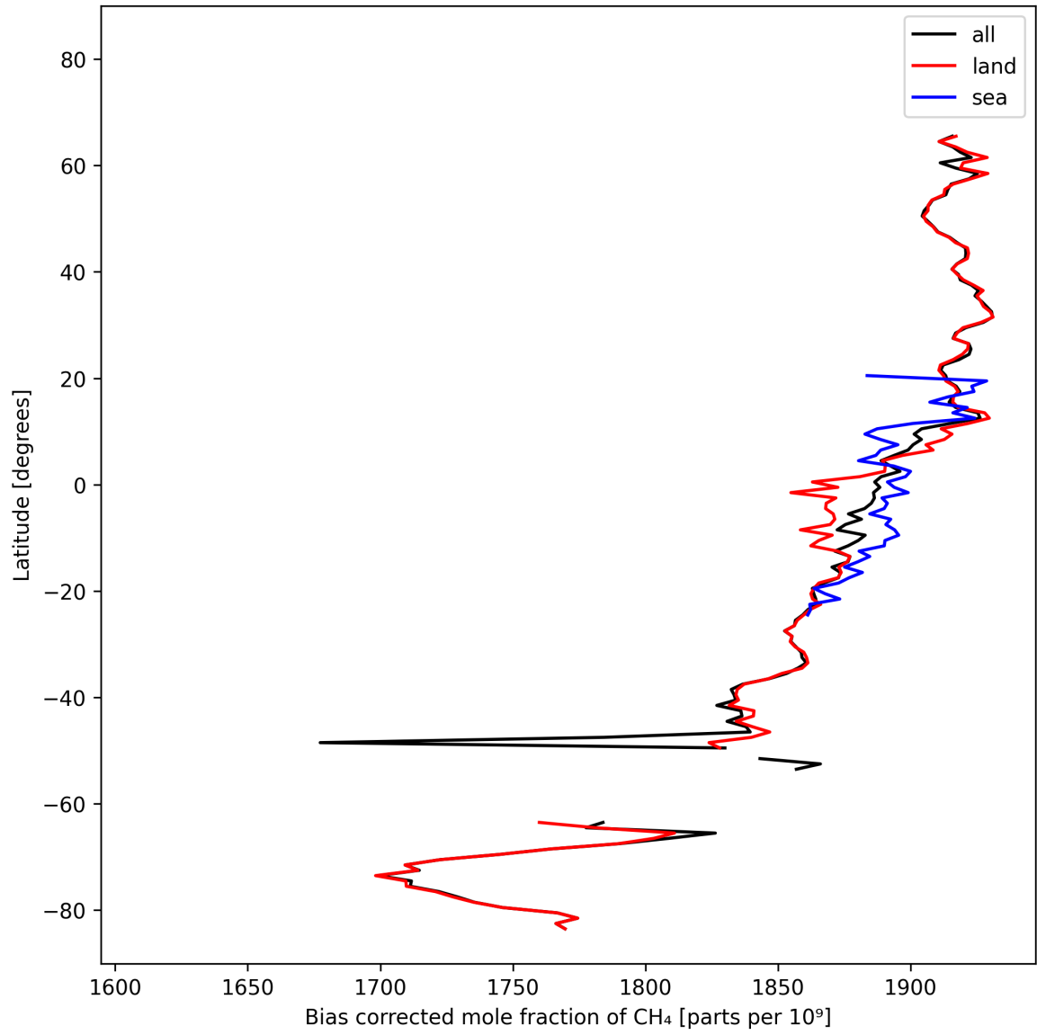
Figure 14: Zonal average of “Bias corrected mole fraction of CH 4 ” for 2024-10-15 to 2024-10-17.
