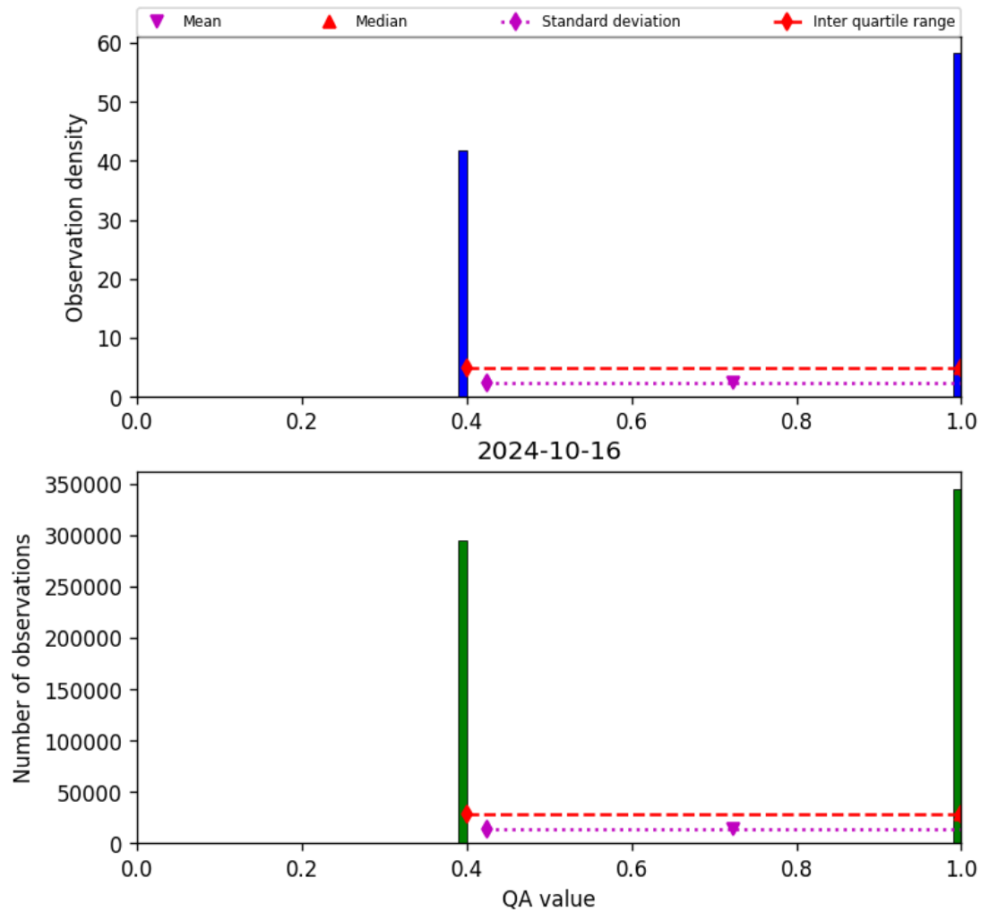
Figure 22: Histogram of “QA value” for 2024-10-15 to 2024-10-17
