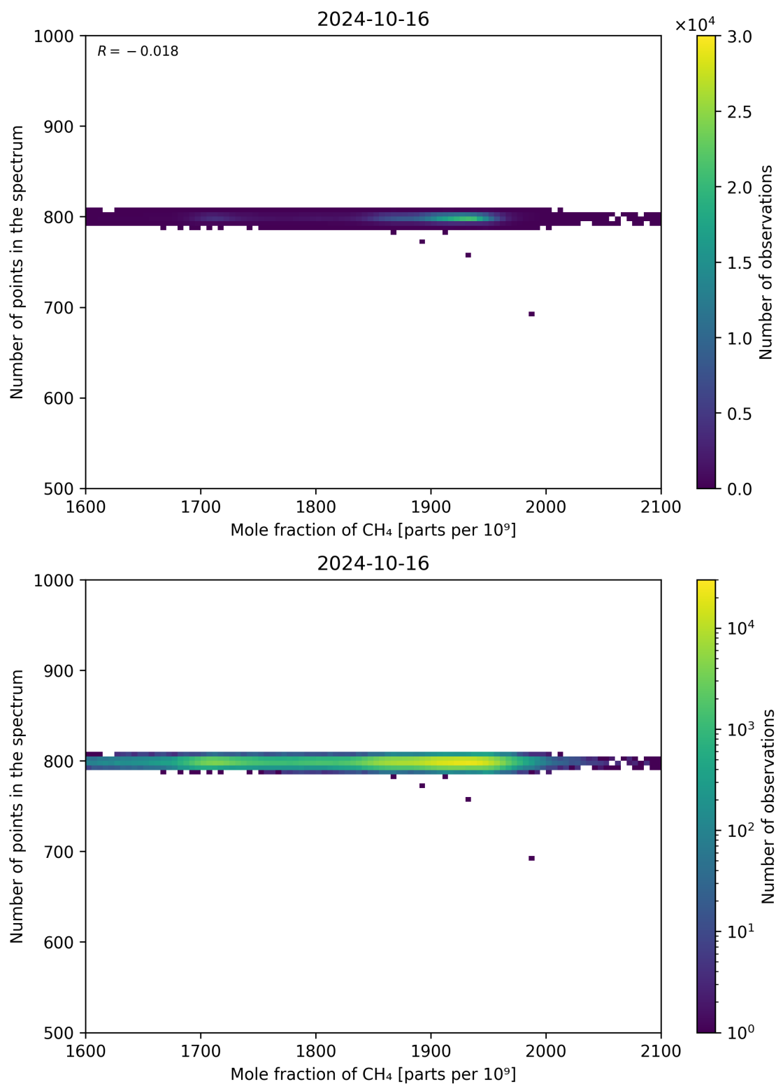
Figure 77: Scatter density plot of “Mole fraction of CH 4 ” against “Number of points in the spectrum” for 2024-10-15 to 2024-10-17.
