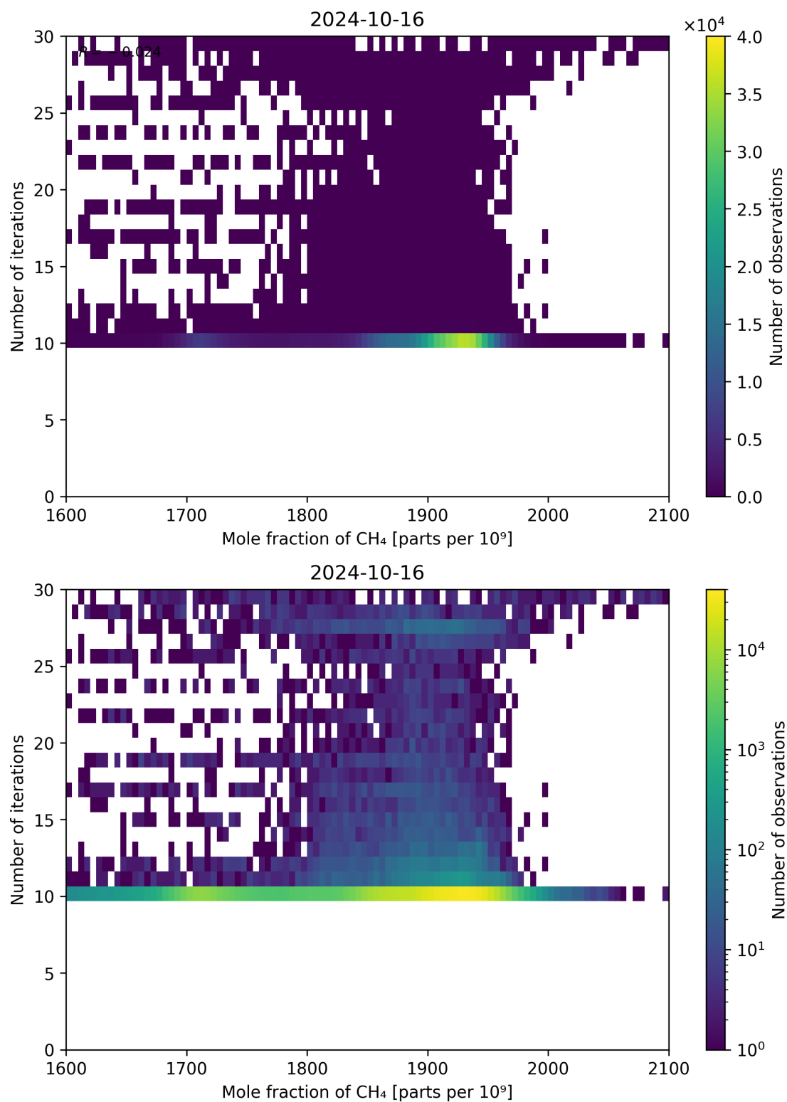
Figure 76: Scatter density plot of “Mole fraction of CH 4 ” against “Number of iterations” for 2024-10-15 to 2024-10-17.
