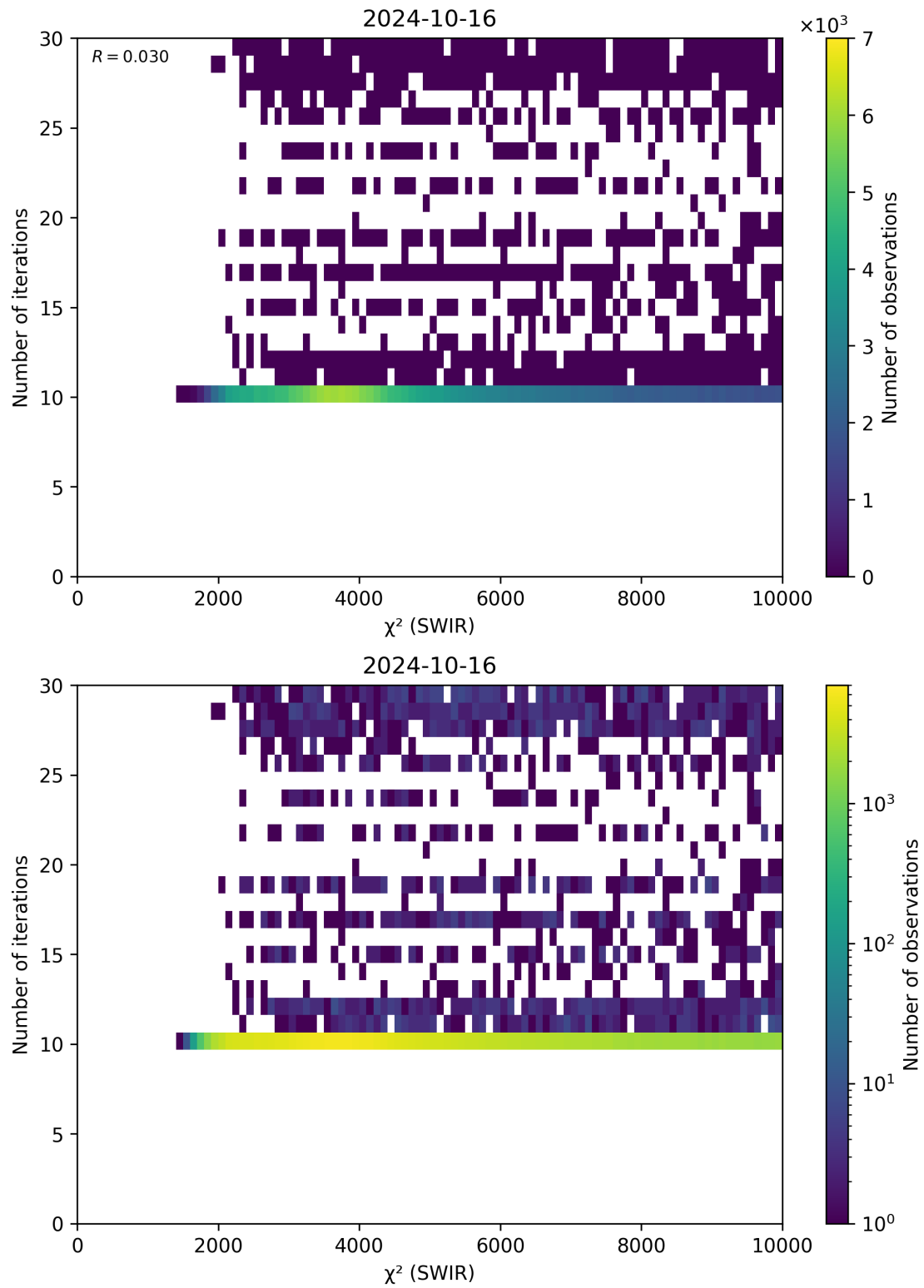
Figure 50: Scatter density plot of “ \chi^2 (SWIR)” against “Number of iterations” for 2024-10-15 to 2024-10-17.
