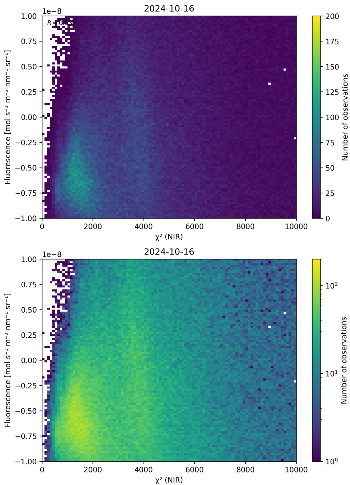
Figure 45: Scatter density plot of “ \chi^2 (NIR)” against “Fluorescence” for 2024-10-15 to 2024-10-17.
