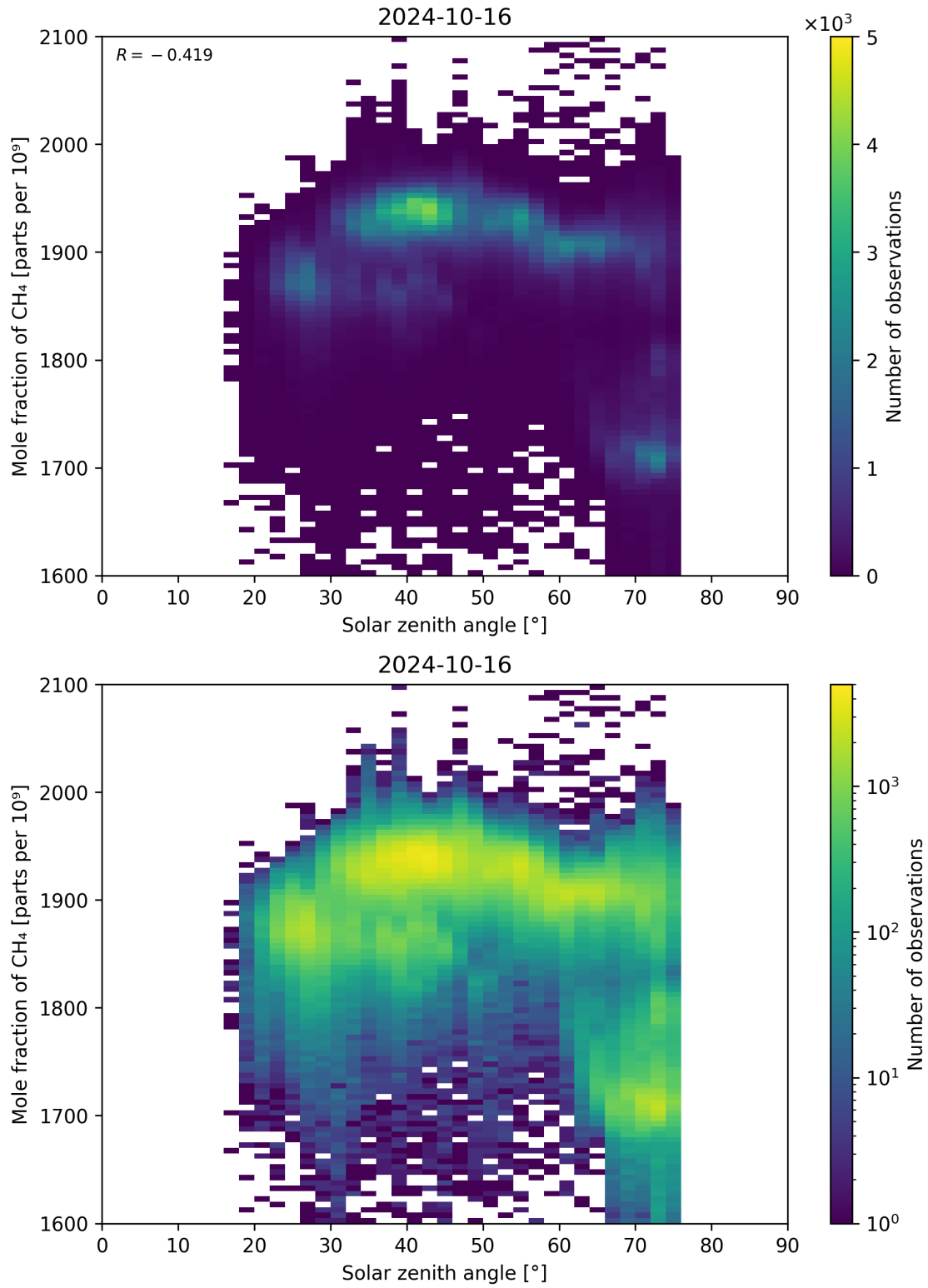
Figure 99: Scatter density plot of “Solar zenith angle” against “Mole fraction of CH 4 ” for 2024-10-15 to 2024-10-17.
