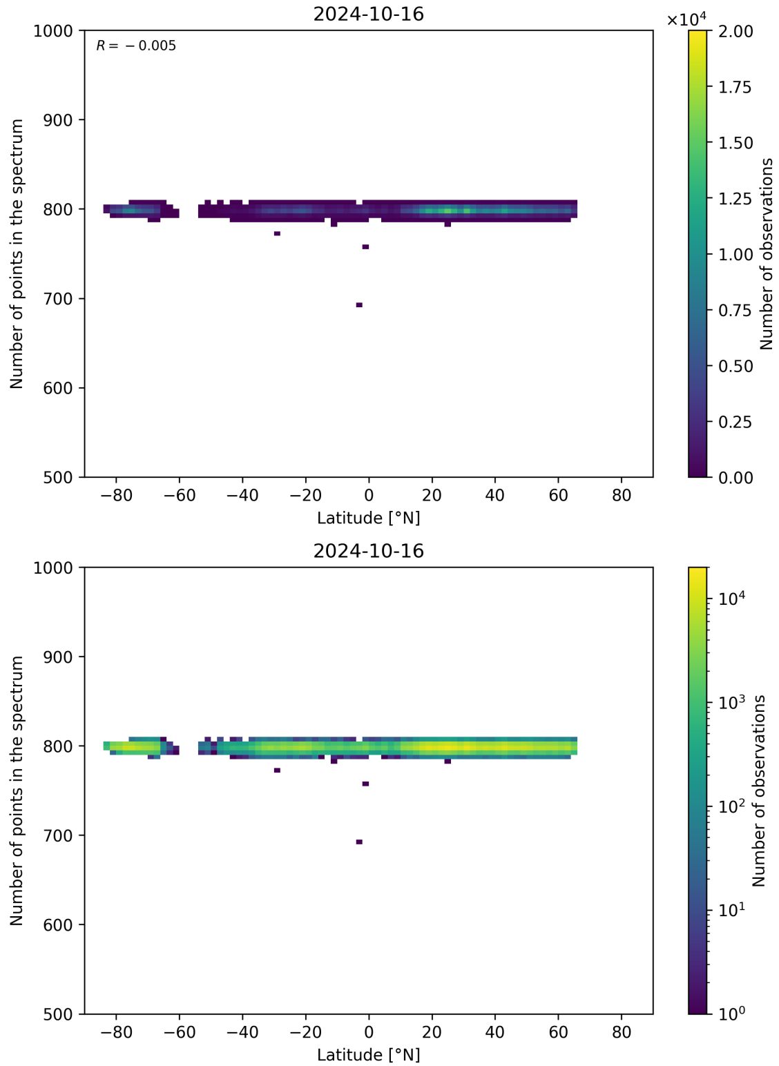
Figure 61: Scatter density plot of “Latitude” against “Number of points in the spectrum” for 2024-10-15 to 2024-10-17.
