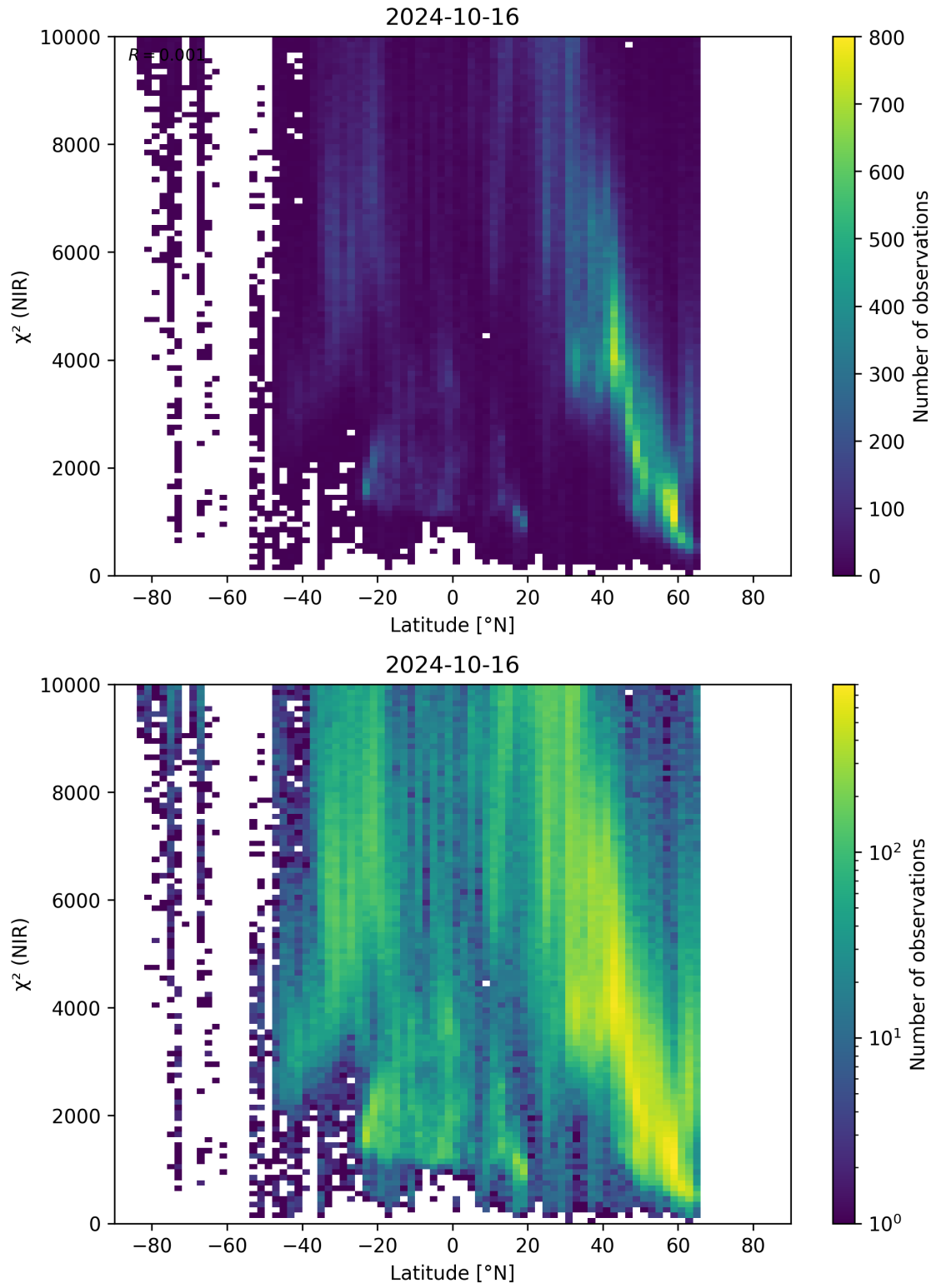
Figure 53: Scatter density plot of “Latitude” against “ \chi^2 (NIR)” for 2024-10-15 to 2024-10-17.
