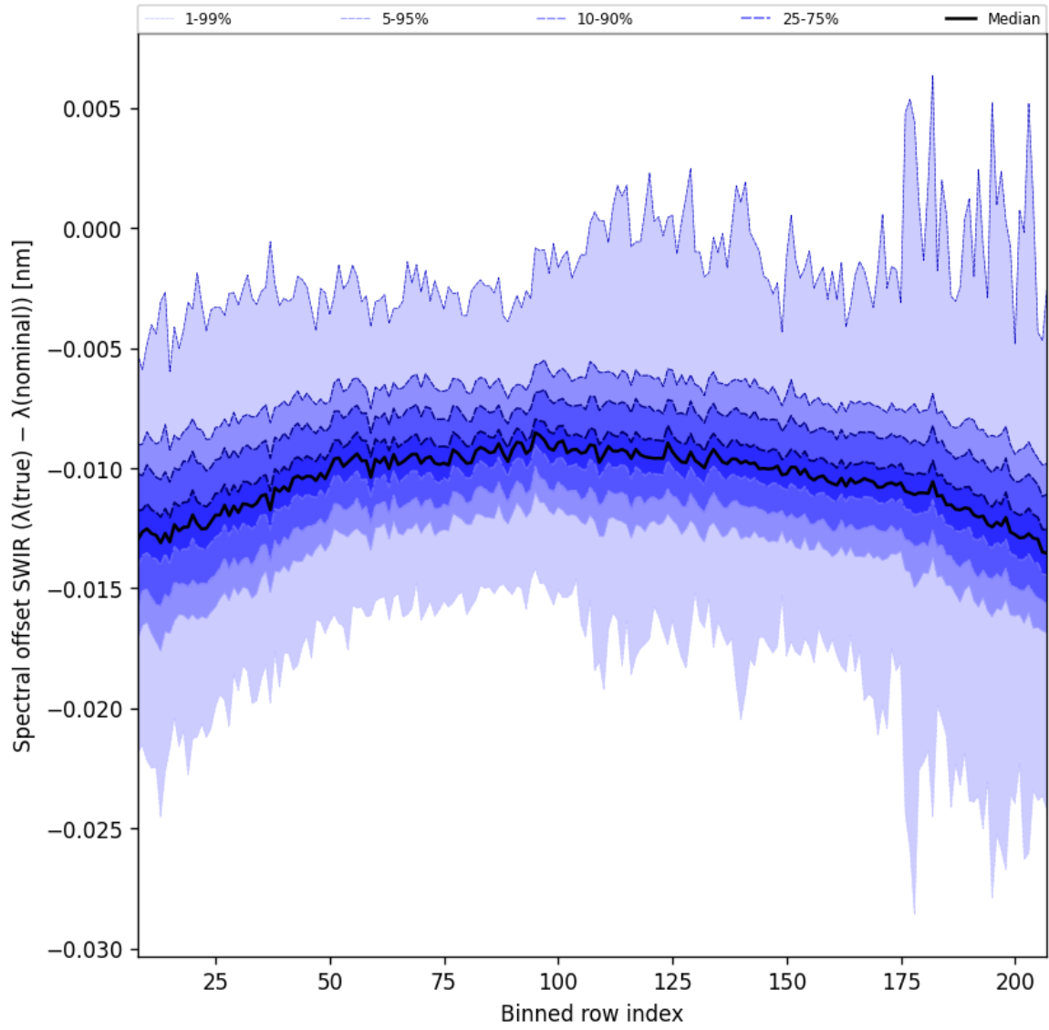
Figure 38: Along track statistics of “Spectral offset SWIR ( \lambda_{\text{true}} - \lambda_{\text{nominal}} )” for 2024-10-15 to 2024-10-17
