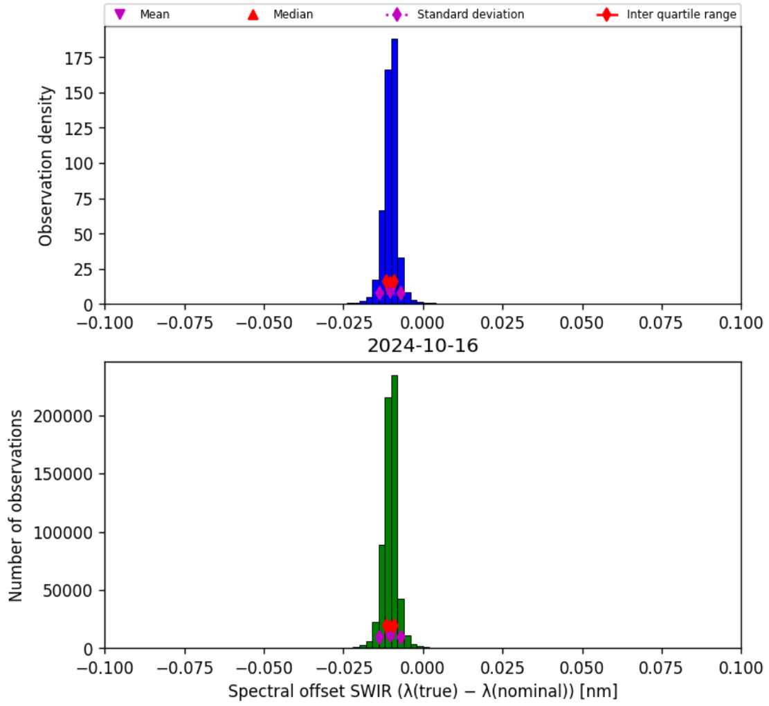
Figure 27: Histogram of “Spectral offset SWIR ( \lambda_{\text{true}} - \lambda_{\text{nominal}} )” for 2024-10-15 to 2024-10-17
