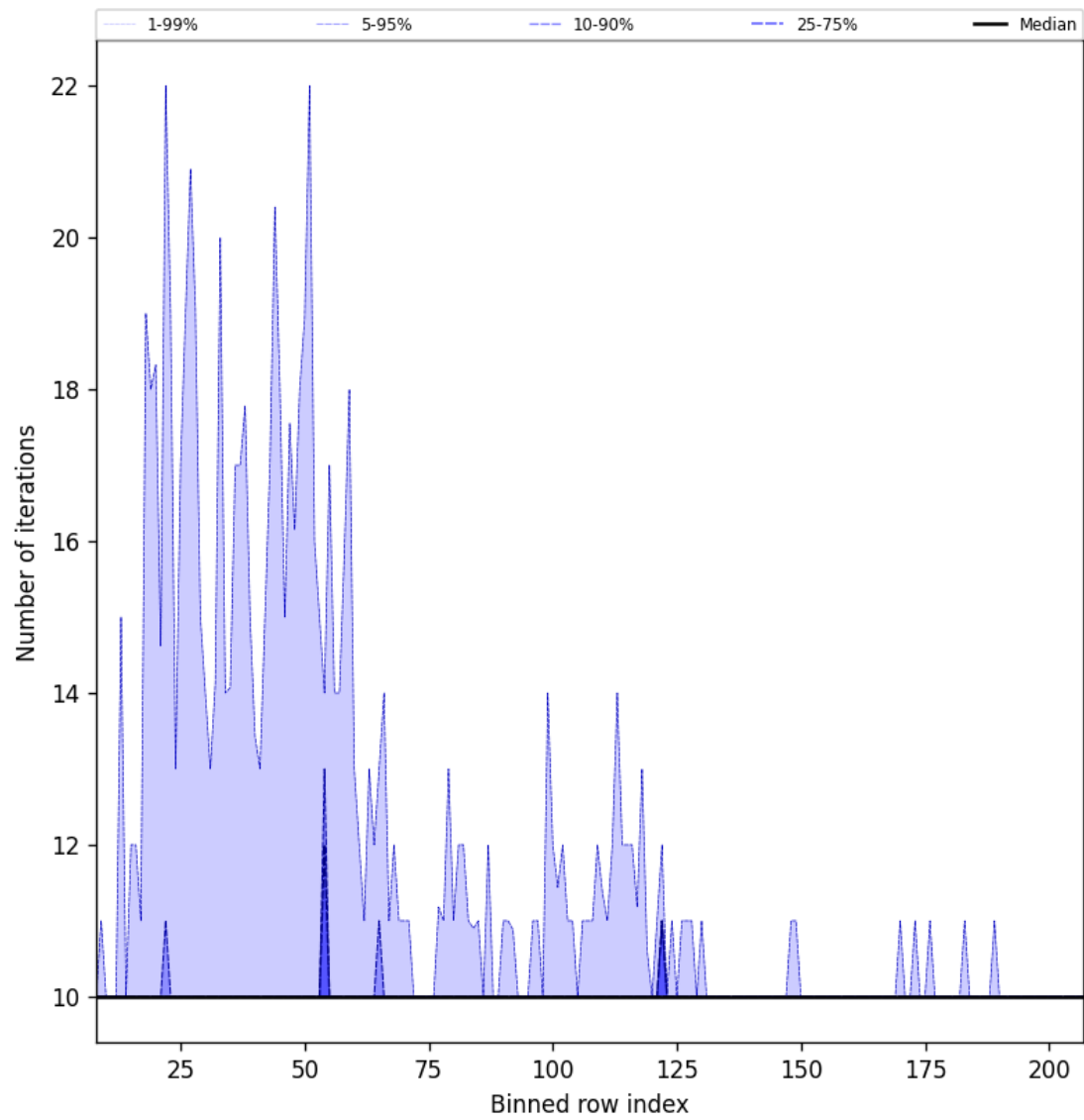
Figure 42: Along track statistics of “Number of iterations” for 2024-10-15 to 2024-10-17
