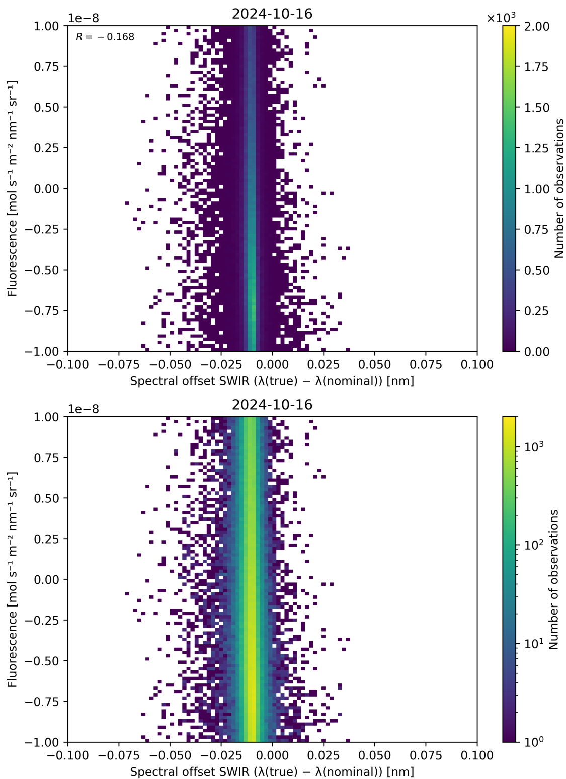
Figure 120: Scatter density plot of “Spectral offset SWIR ( \lambda_{\text{true}} - \lambda_{\text{nominal}} )” against “Fluorescence” for 2024-10-15 to 2024-10-17.
