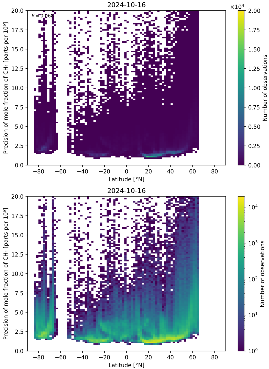
Figure 59: Scatter density plot of “Latitude” against “Precision of mole fraction of CH 4 ” for 2024-10-15 to 2024-10-17.
