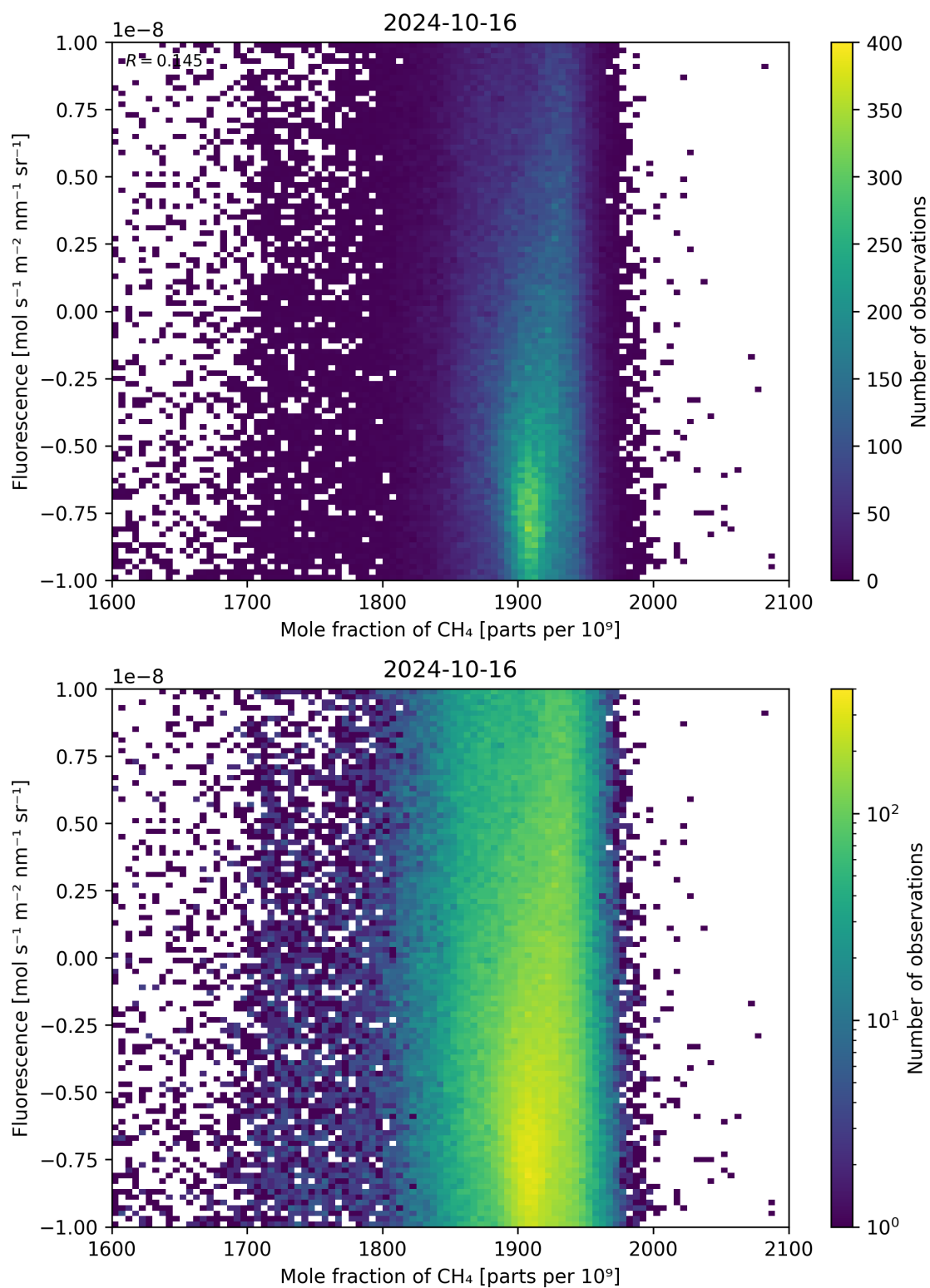
Figure 73: Scatter density plot of “Mole fraction of \text{CH}_4 ” against “Fluorescence” for 2024-10-15 to 2024-10-17.
