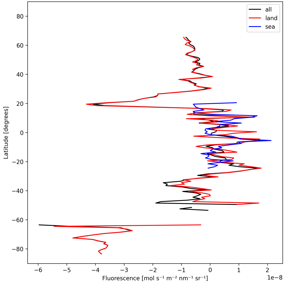
Figure 21: Zonal average of “Fluorescence” for 2024-10-15 to 2024-10-17.
