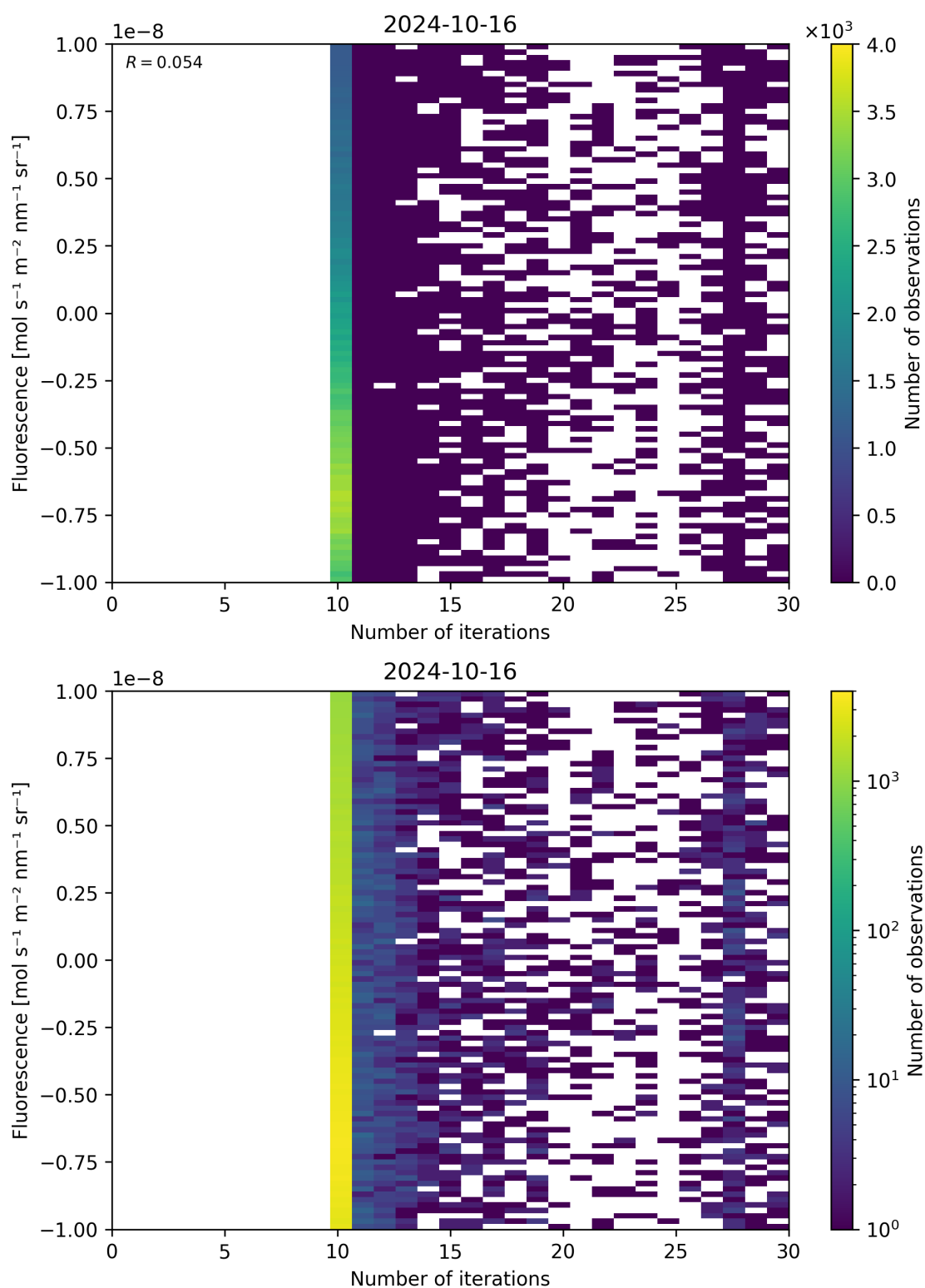
Figure 87: Scatter density plot of “Number of iterations” against “Fluorescence” for 2024-10-15 to 2024-10-17.
