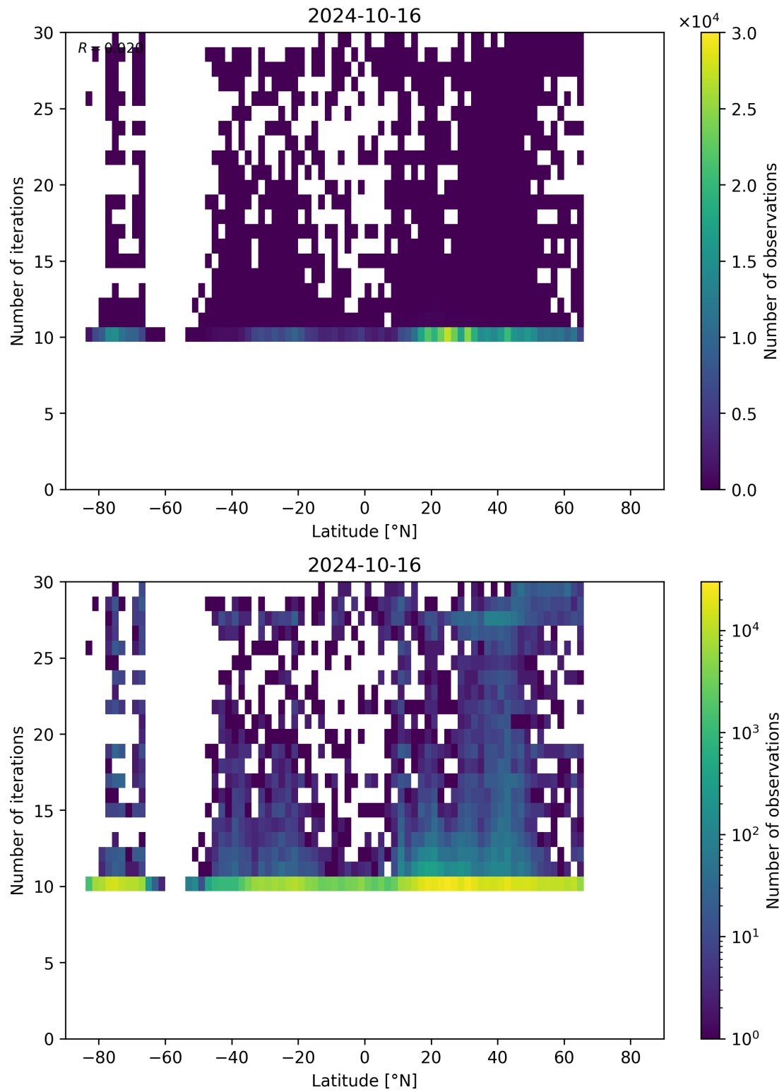
Figure 60: Scatter density plot of “Latitude” against “Number of iterations” for 2024-10-15 to 2024-10-17.
