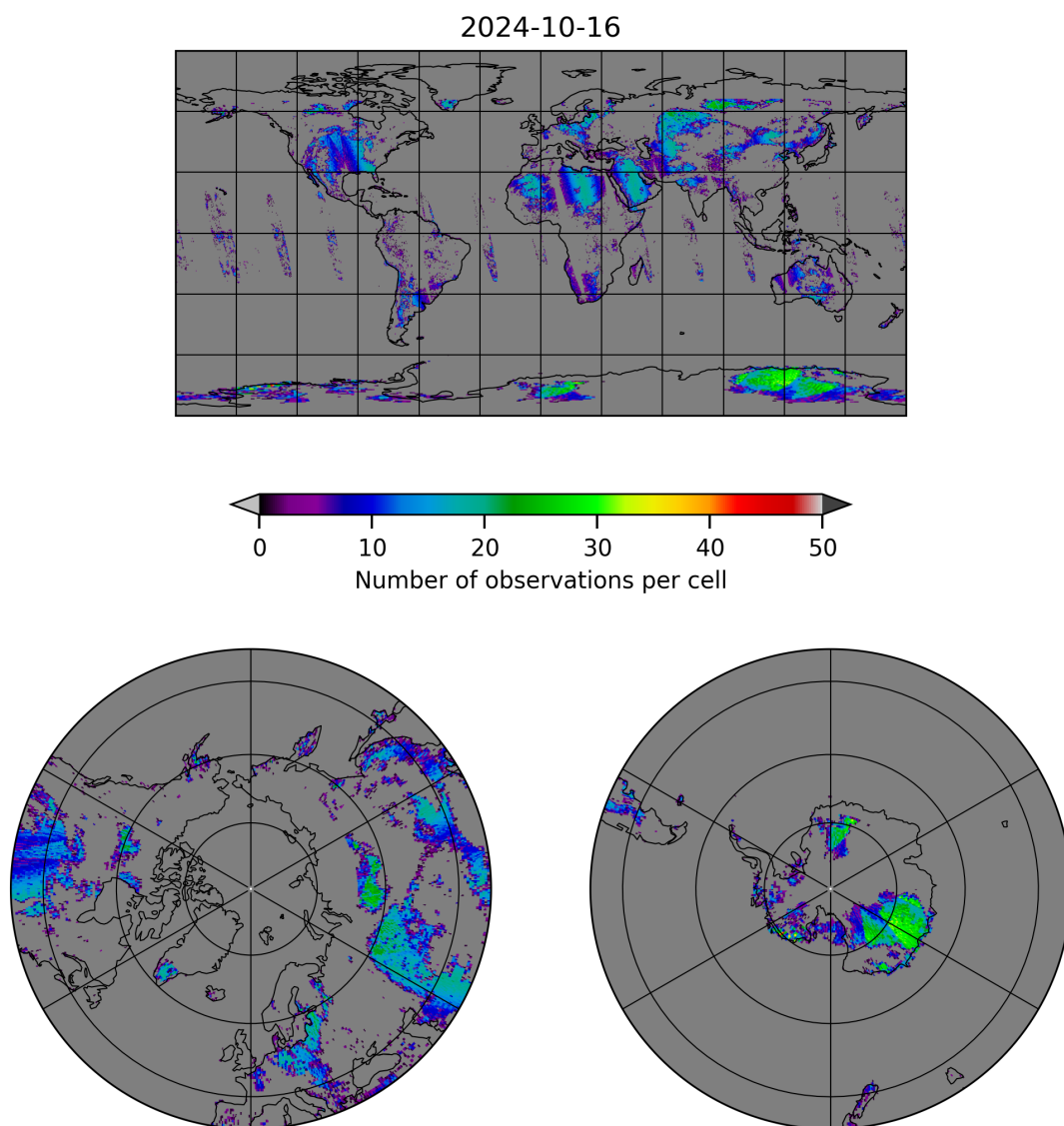
Figure 10: Map of the number of observations for 2024-10-15 to 2024-10-17
