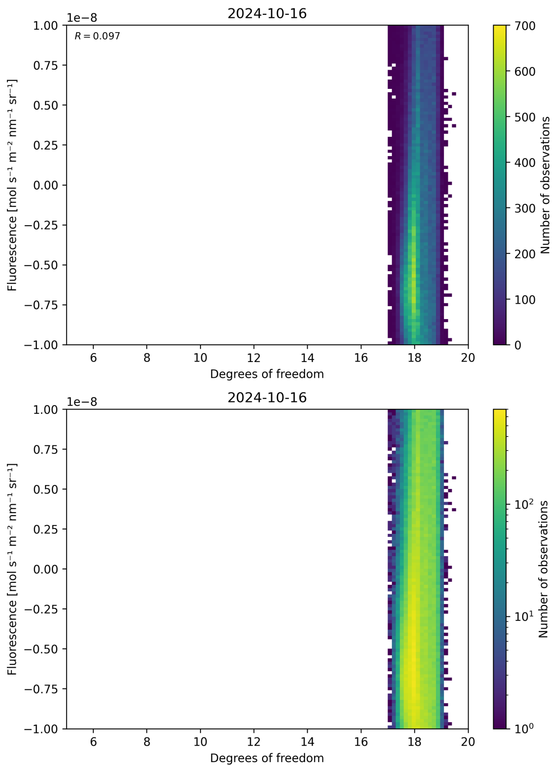
Figure 51: Scatter density plot of “Degrees of freedom” against “Fluorescence” for 2024-10-15 to 2024-10-17.
