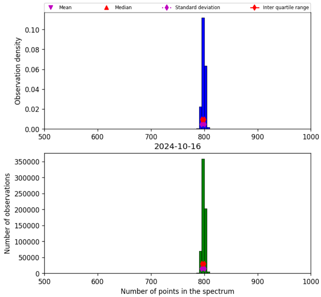
Figure 26: Histogram of “Number of points in the spectrum” for 2024-10-15 to 2024-10-17
