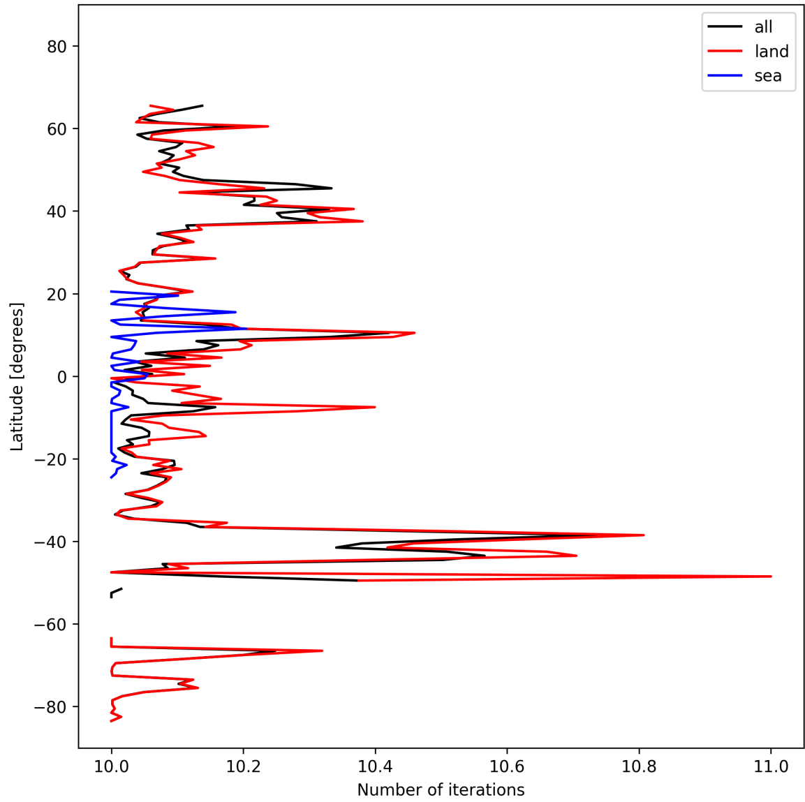
Figure 20: Zonal average of “Number of iterations” for 2024-10-15 to 2024-10-17.
