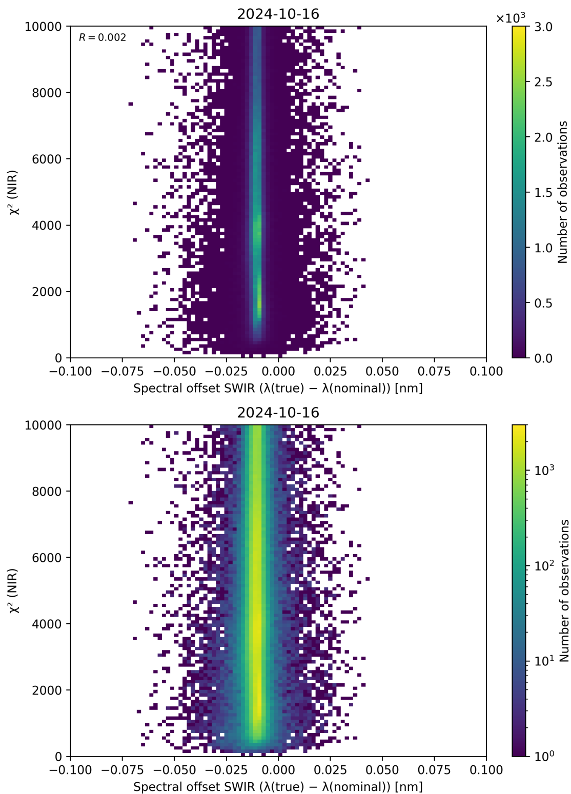
Figure 117: Scatter density plot of “Spectral offset SWIR ( \lambda_{\text{true}} - \lambda_{\text{nominal}} )” against “ \chi^2 (NIR)” for 2024-10-15 to 2024-10-17.
