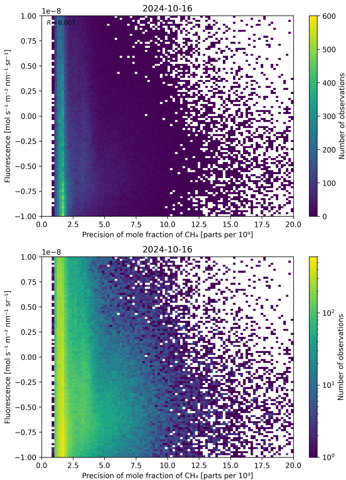
Figure 81: Scatter density plot of “Precision of mole fraction of \text{CH}_4 ” against “Fluorescence” for 2024-10-15 to 2024-10-17.
