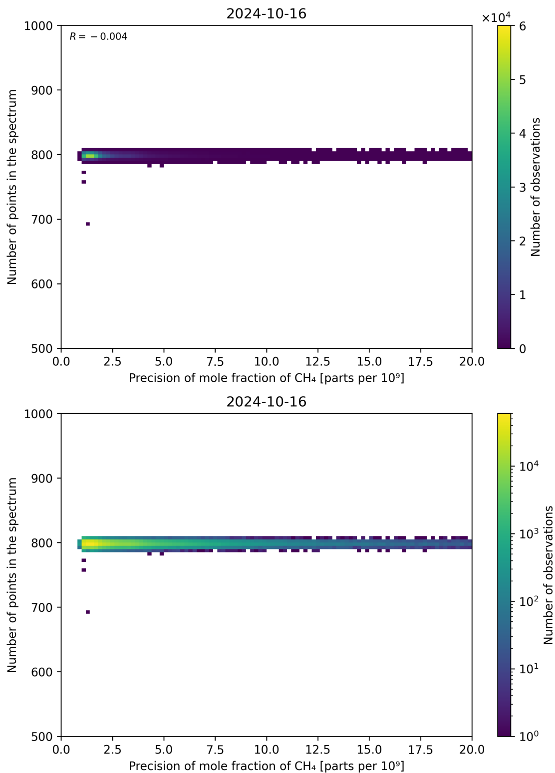
Figure 84: Scatter density plot of “Precision of mole fraction of CH 4 ” against “Number of points in the spectrum” for 2024-10-15 to 2024-10-17.
