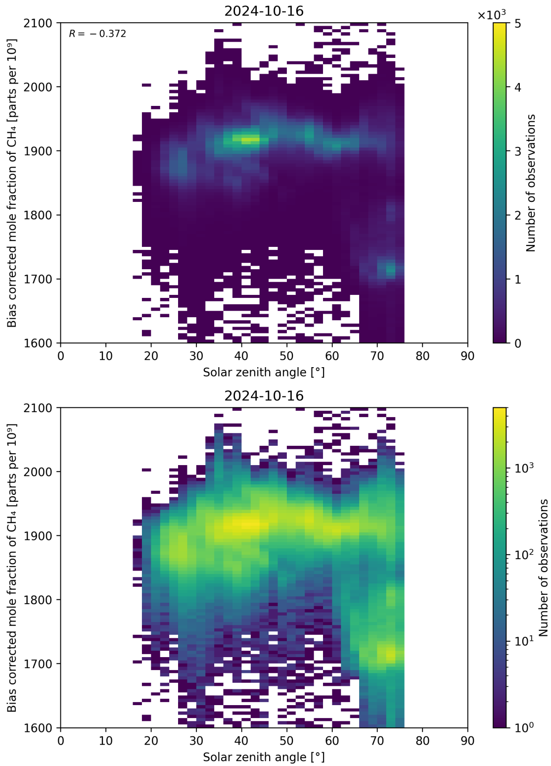
Figure 100: Scatter density plot of “Solar zenith angle” against “Bias corrected mole fraction of \text{CH}_4 ” for 2024-10-15 to 2024-10-17.
