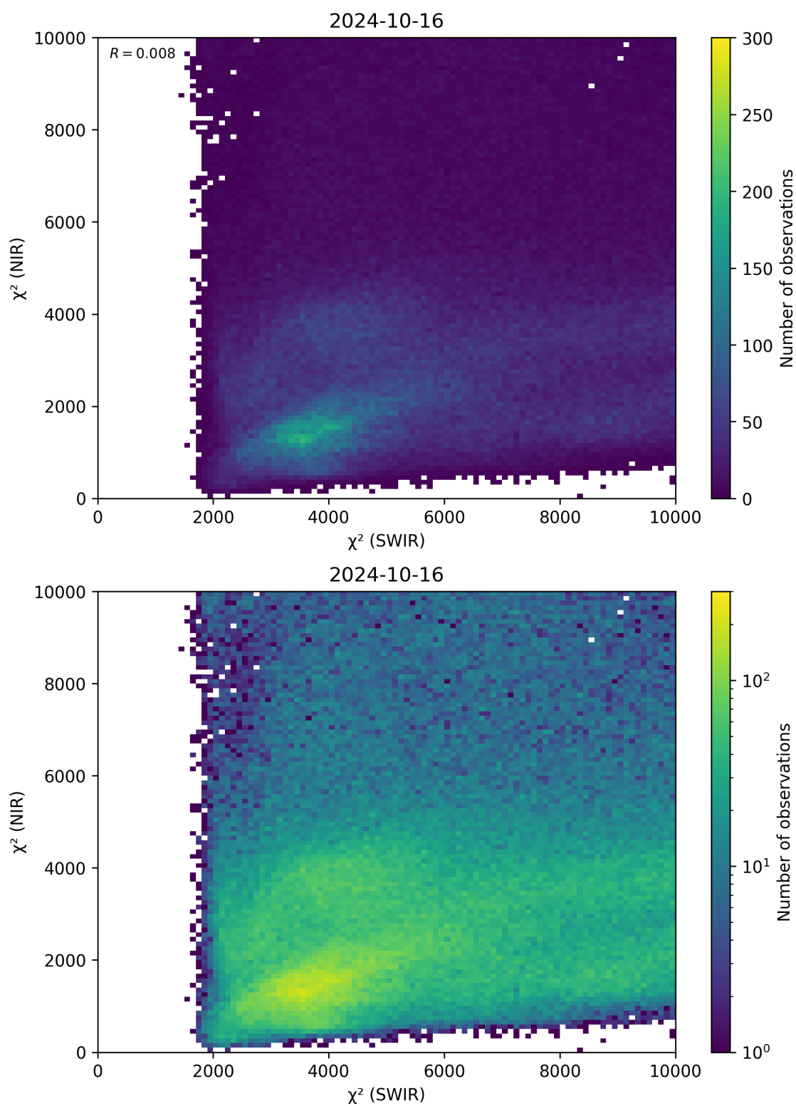
Figure 47: Scatter density plot of “ \chi^2 (SWIR)” against “ \chi^2 (NIR)” for 2024-10-15 to 2024-10-17.
