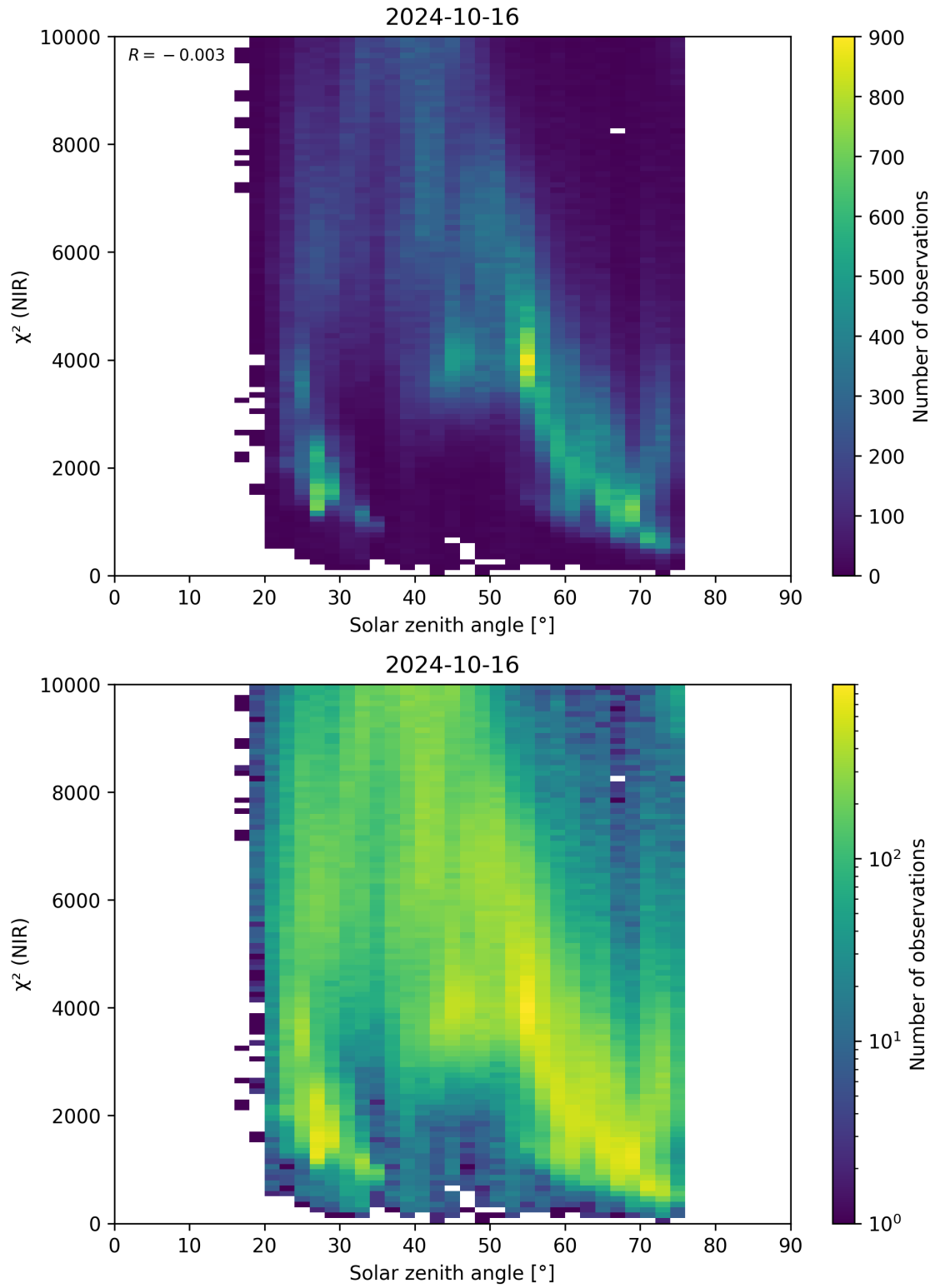
Figure 94: Scatter density plot of “Solar zenith angle” against “ \chi^2 (NIR)” for 2024-10-15 to 2024-10-17.
