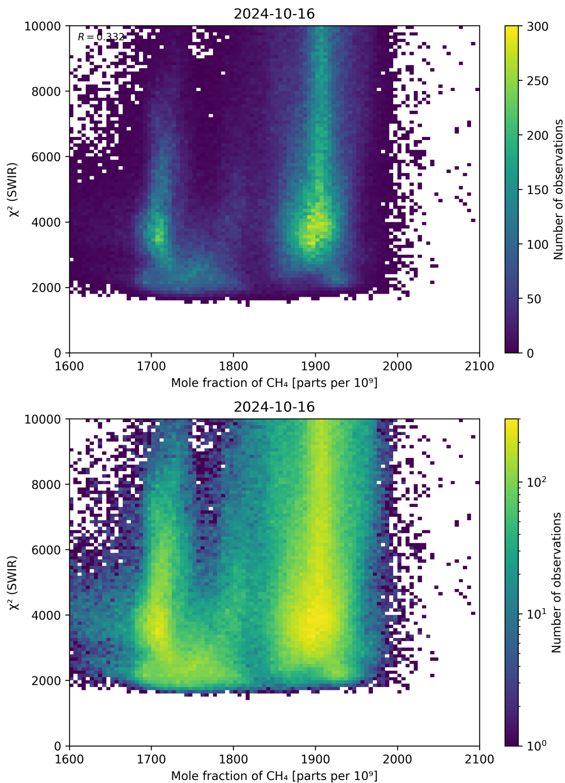
Figure 71: Scatter density plot of “Mole fraction of \text{CH}_4 ” against “ \chi^2 (SWIR)” for 2024-10-15 to 2024-10-17.
