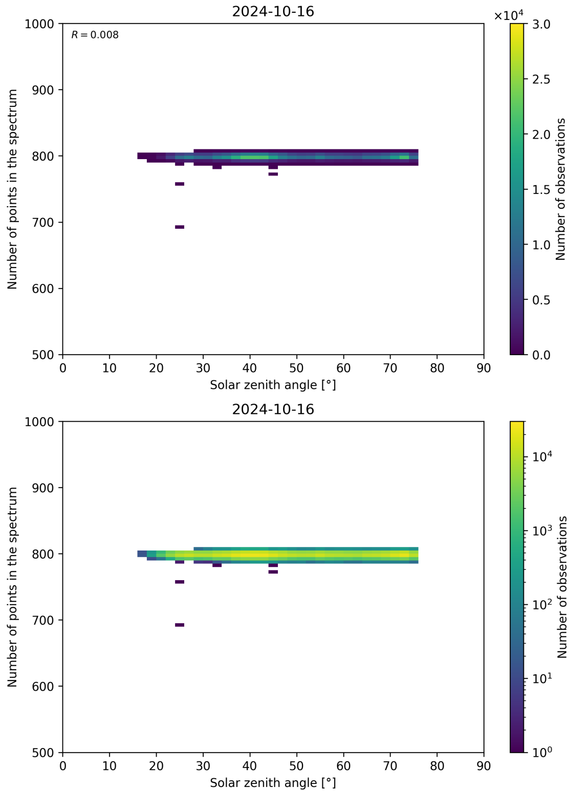
Figure 103: Scatter density plot of “Solar zenith angle” against “Number of points in the spectrum” for 2024-10-15 to 2024-10-17.
