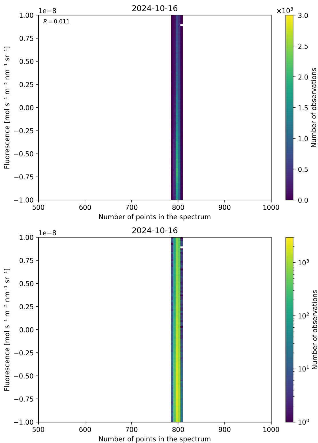
Figure 91: Scatter density plot of “Number of points in the spectrum” against “Fluorescence” for 2024-10-15 to 2024-10-17.
