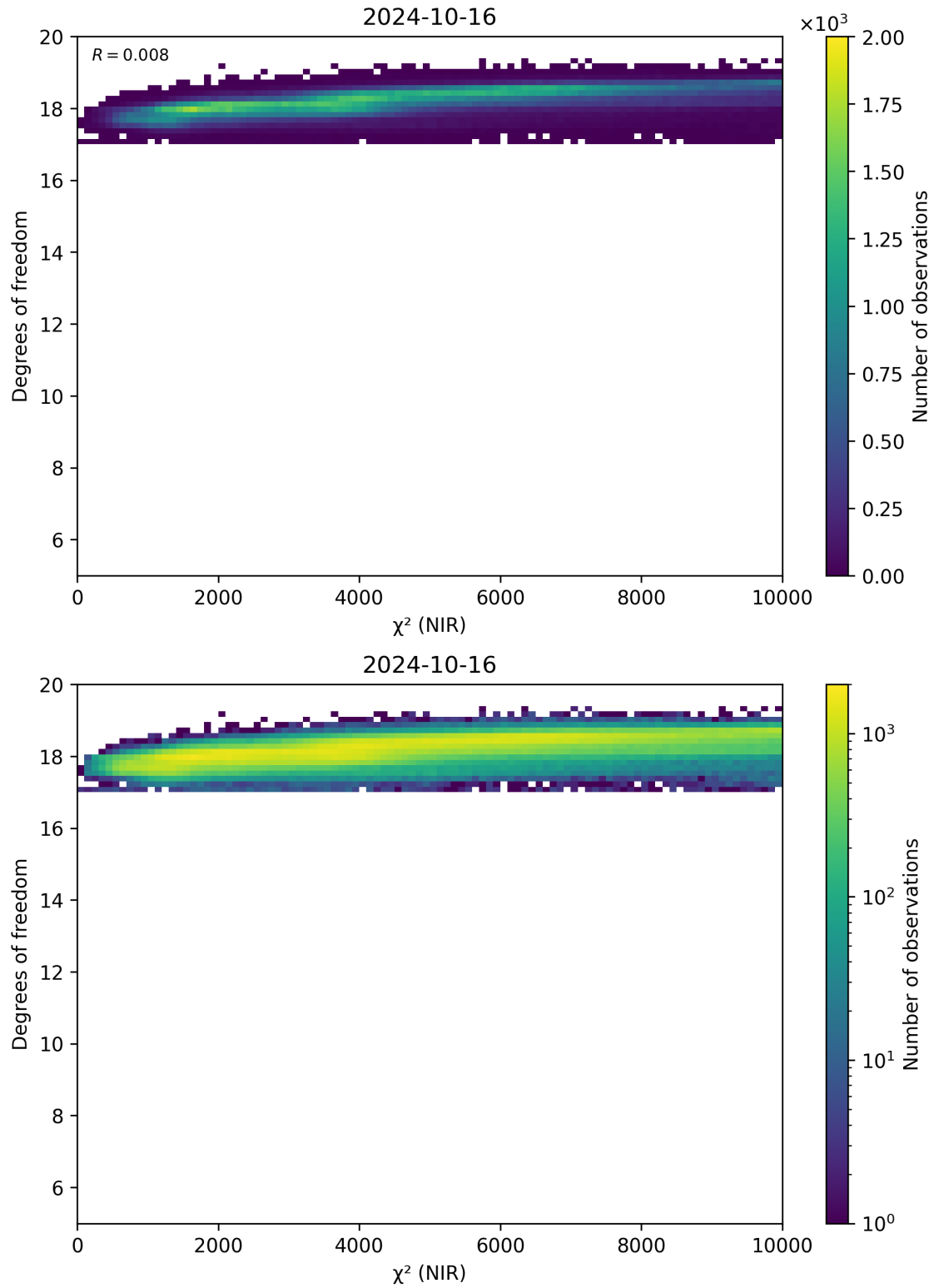
Figure 44: Scatter density plot of “ \chi^2 (NIR)” against “Degrees of freedom” for 2024-10-15 to 2024-10-17.
