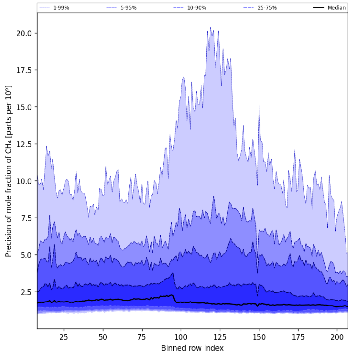
Figure 35: Along track statistics of “Precision of mole fraction of CH 4 ” for 2024-10-15 to 2024-10-17
