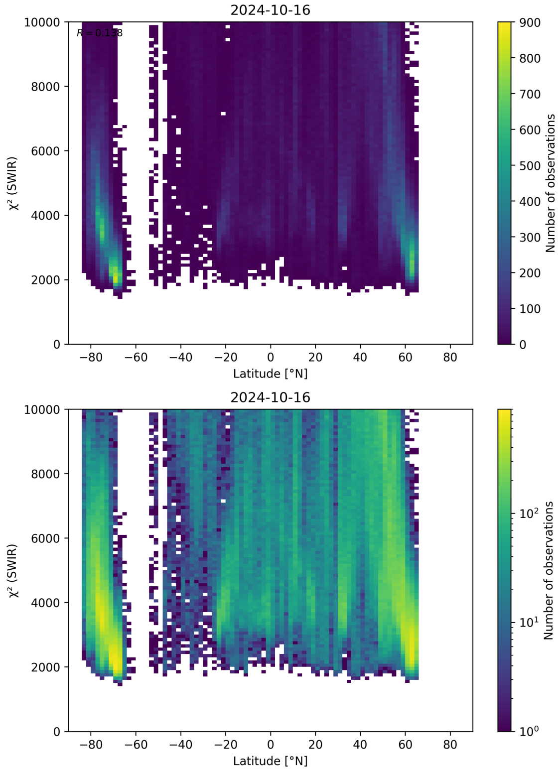
Figure 54: Scatter density plot of “Latitude” against “ \chi^2 (SWIR)” for 2024-10-15 to 2024-10-17.
