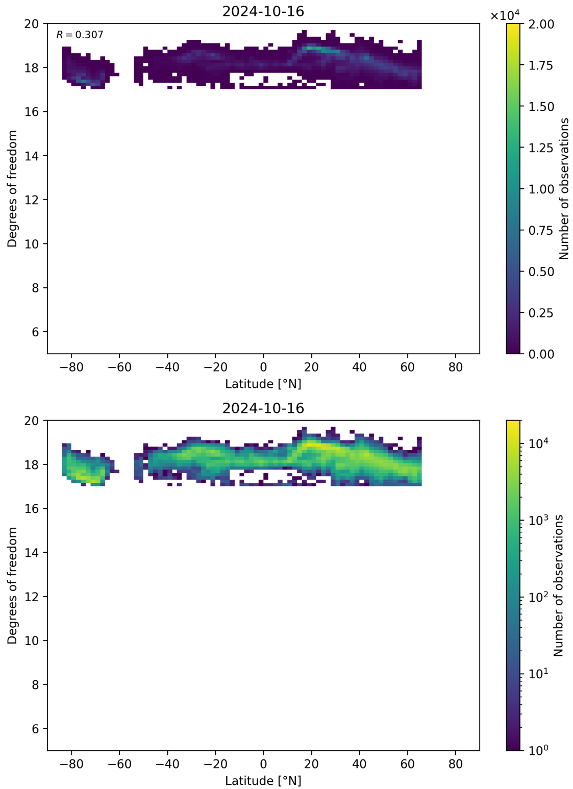
Figure 55: Scatter density plot of “Latitude” against “Degrees of freedom” for 2024-10-15 to 2024-10-17.
