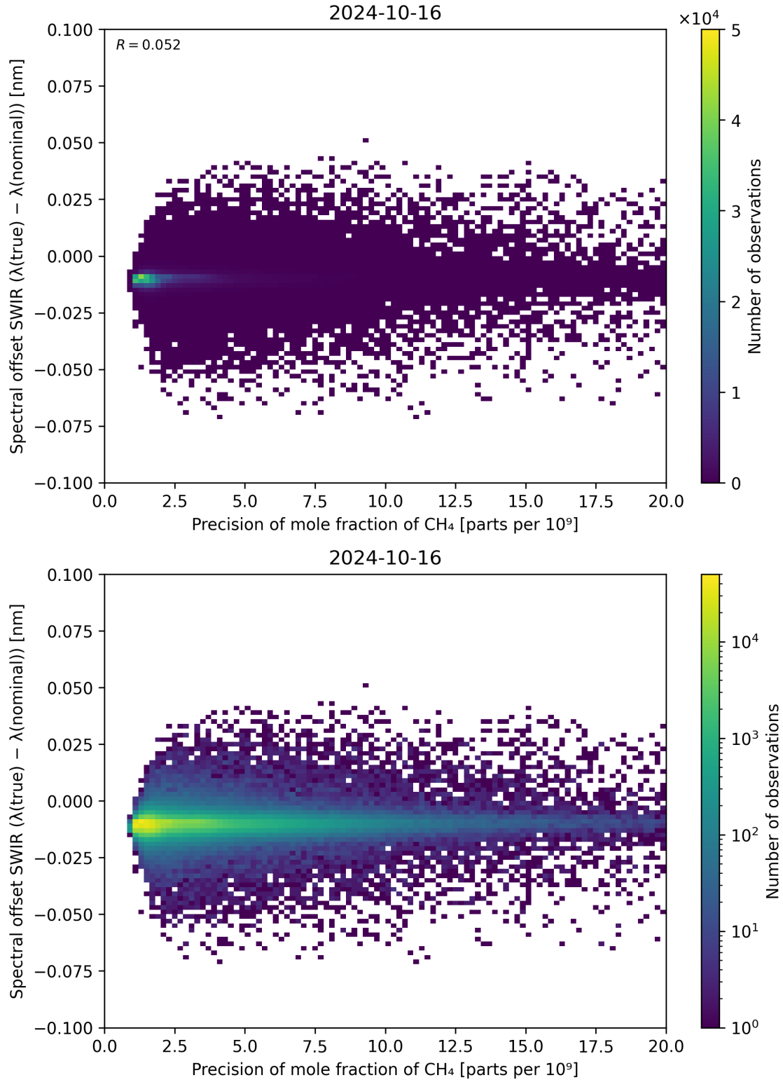
Figure 85: Scatter density plot of “Precision of mole fraction of CH 4 ” against “Spectral offset SWIR ( \lambda_{\text{true}} - \lambda_{\text{nominal}} )” for 2024-10-15 to 2024-10-17.
