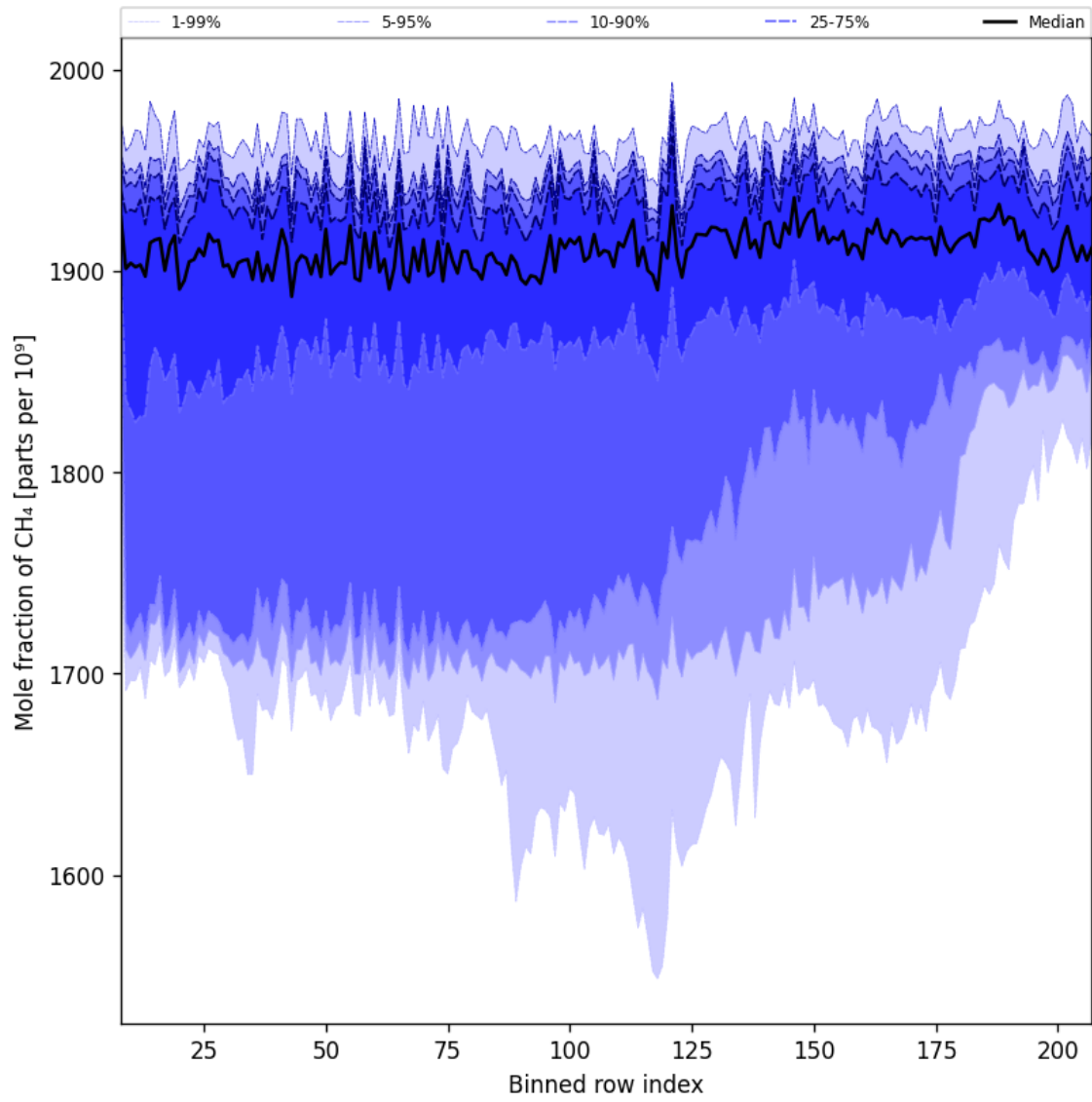
Figure 34: Along track statistics of “Mole fraction of CH 4 ” for 2024-10-15 to 2024-10-17
