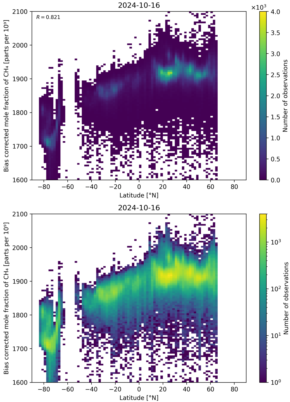
Figure 58: Scatter density plot of “Latitude” against “Bias corrected mole fraction of \text{CH}_4 ” for 2024-10-15 to 2024-10-17.
