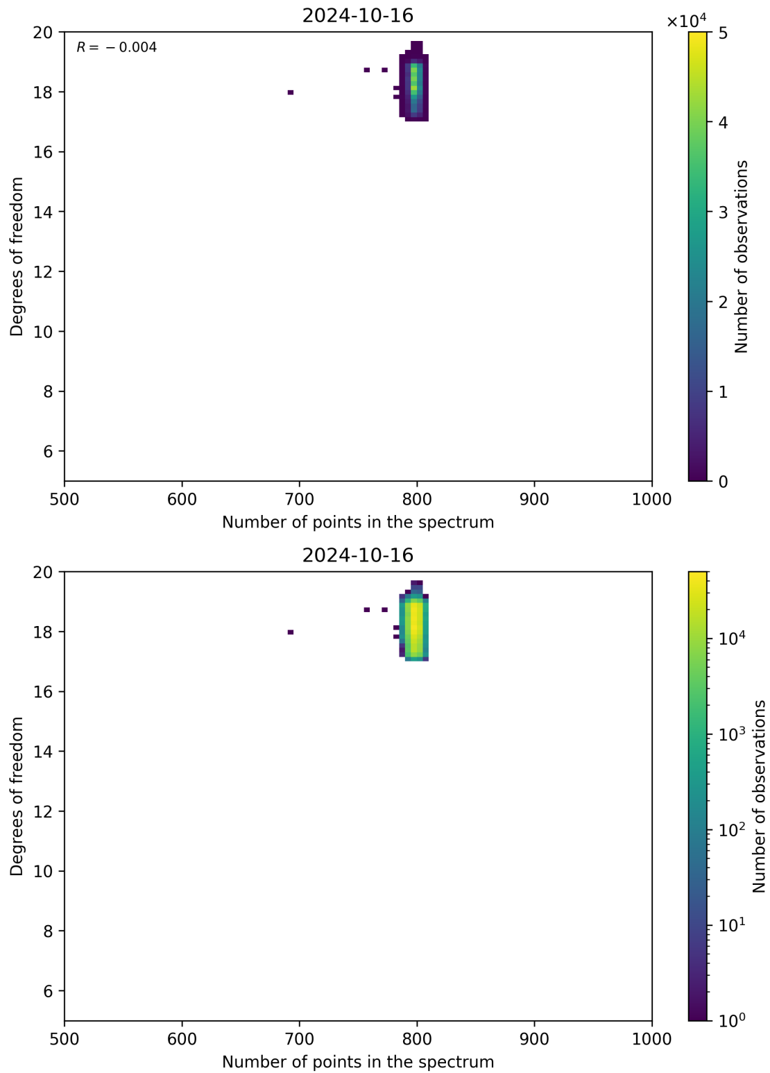
Figure 90: Scatter density plot of “Number of points in the spectrum” against “Degrees of freedom” for 2024-10-15 to 2024-10-17.
