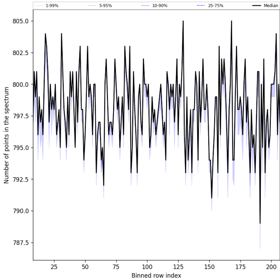
Figure 37: Along track statistics of “Number of points in the spectrum” for 2024-10-15 to 2024-10-17
