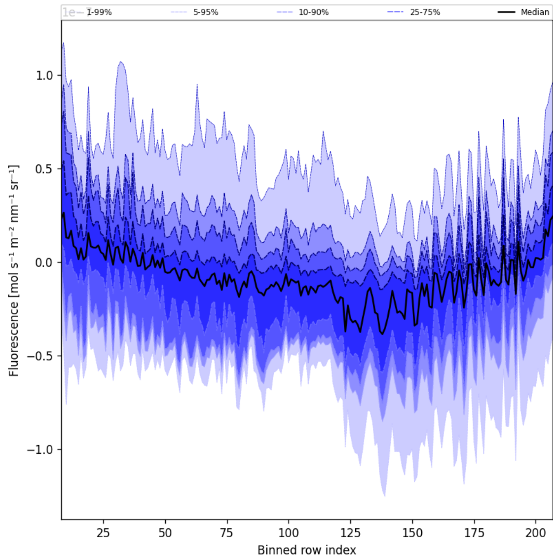
Figure 43: Along track statistics of “Fluorescence” for 2024-10-16 to 2024-10-18
