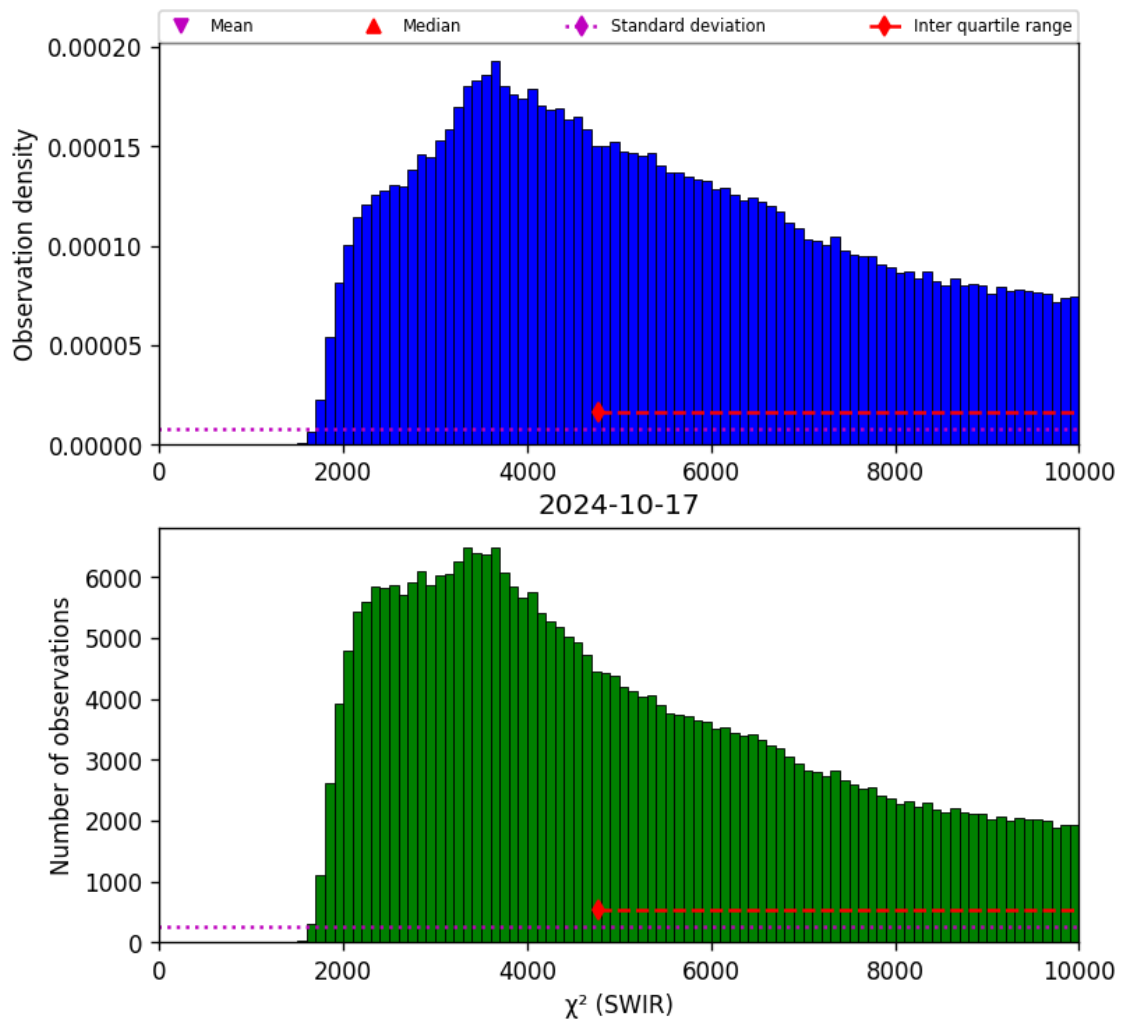
Figure 28: Histogram of “ \chi^2 (SWIR)” for 2024-10-16 to 2024-10-18
