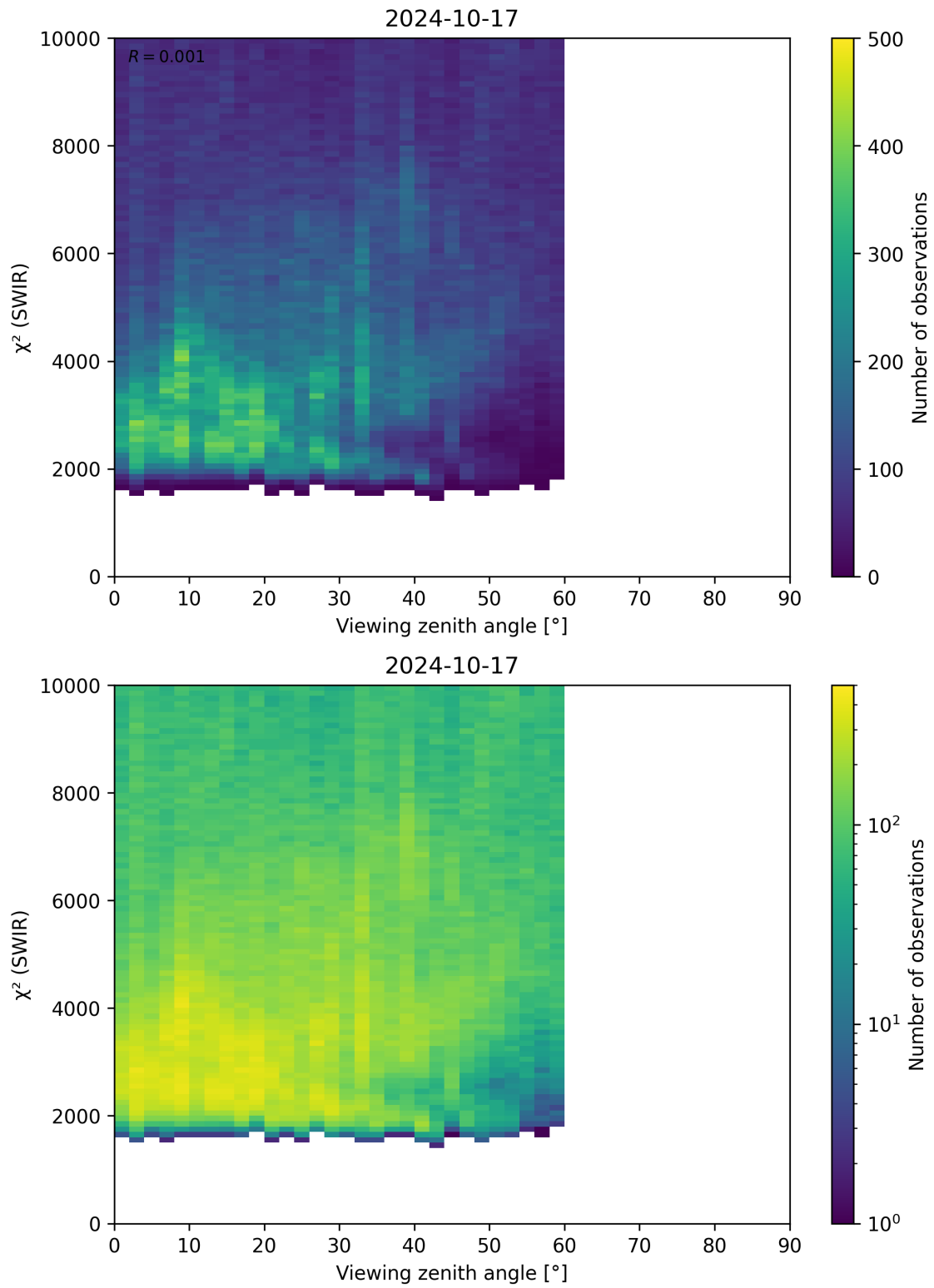
Figure 106: Scatter density plot of “Viewing zenith angle” against “ \chi^2 (SWIR)” for 2024-10-16 to 2024-10-18.
