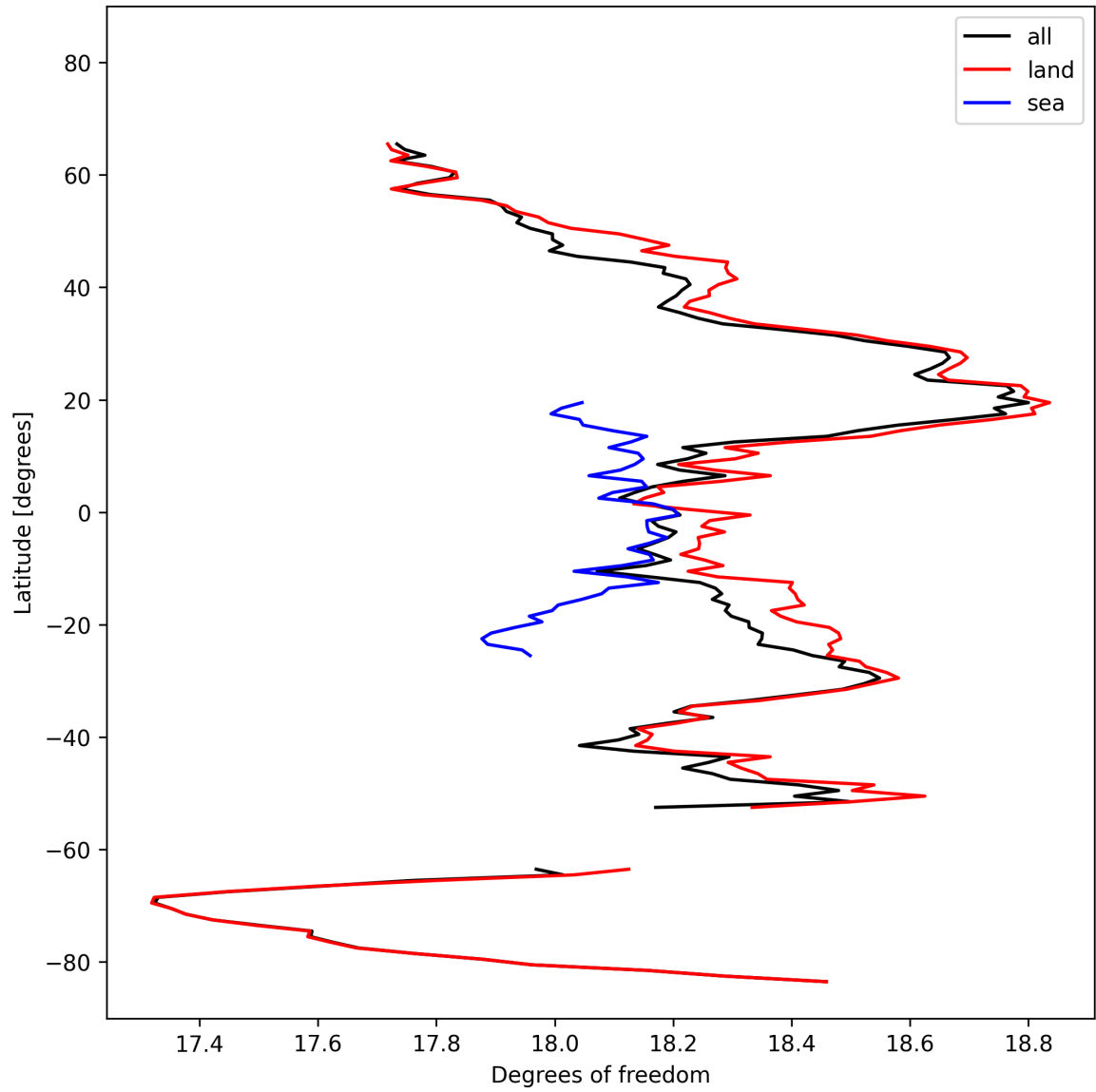
Figure 19: Zonal average of “Degrees of freedom” for 2024-10-16 to 2024-10-18.
