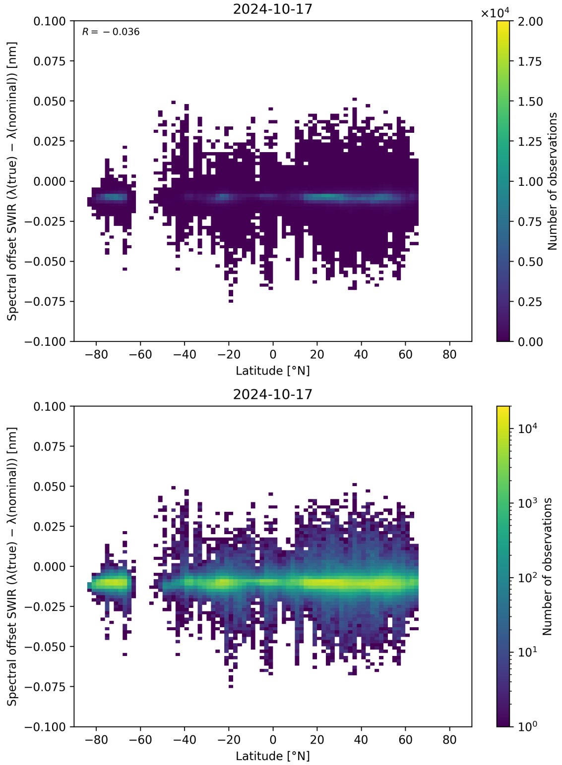
Figure 62: Scatter density plot of “Latitude” against “Spectral offset SWIR ( \lambda_{\text{true}} - \lambda_{\text{nominal}} )” for 2024-10-16 to 2024-10-18.
