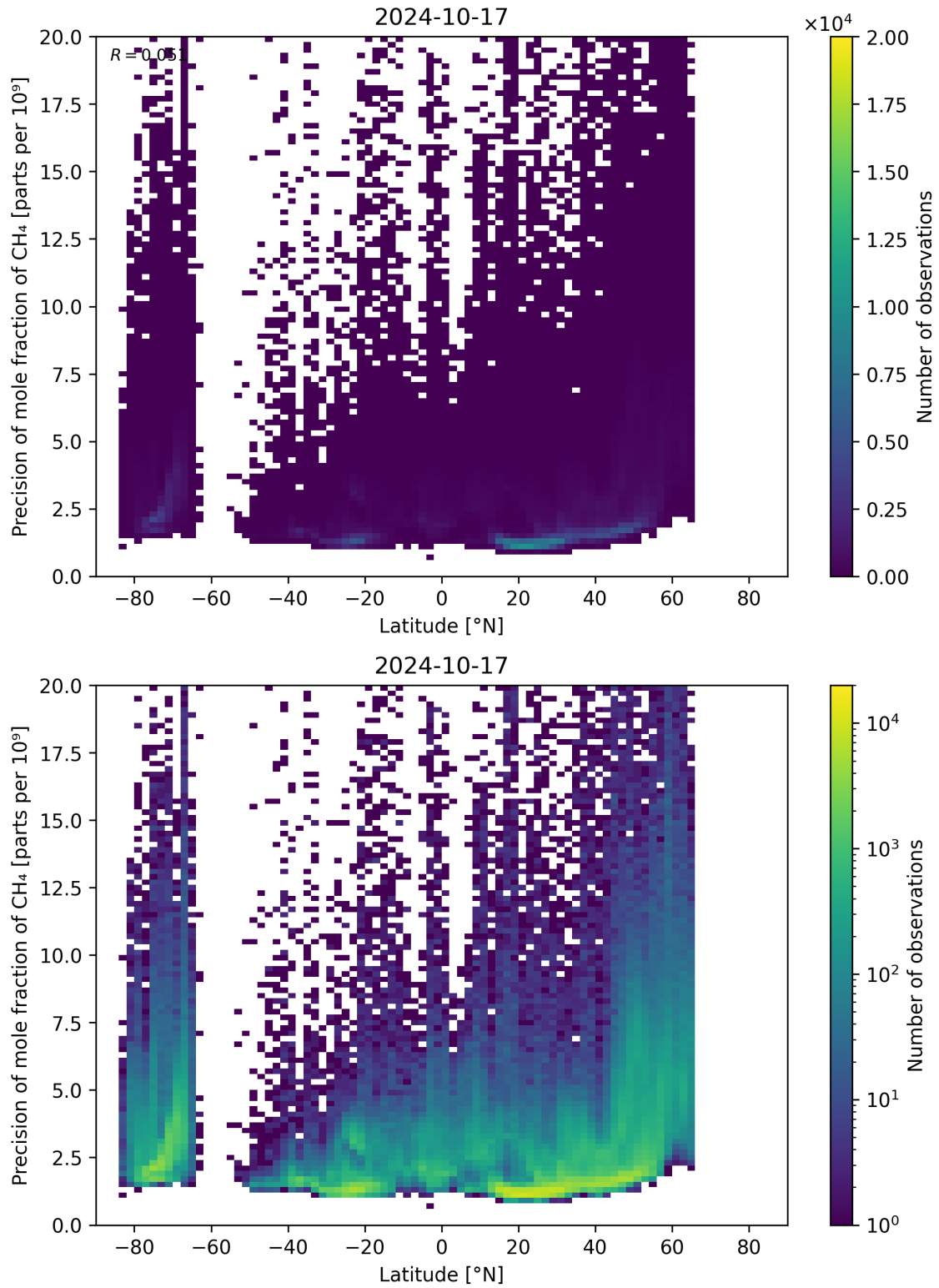
Figure 59: Scatter density plot of “Latitude” against “Precision of mole fraction of CH 4 ” for 2024-10-16 to 2024-10-18.
