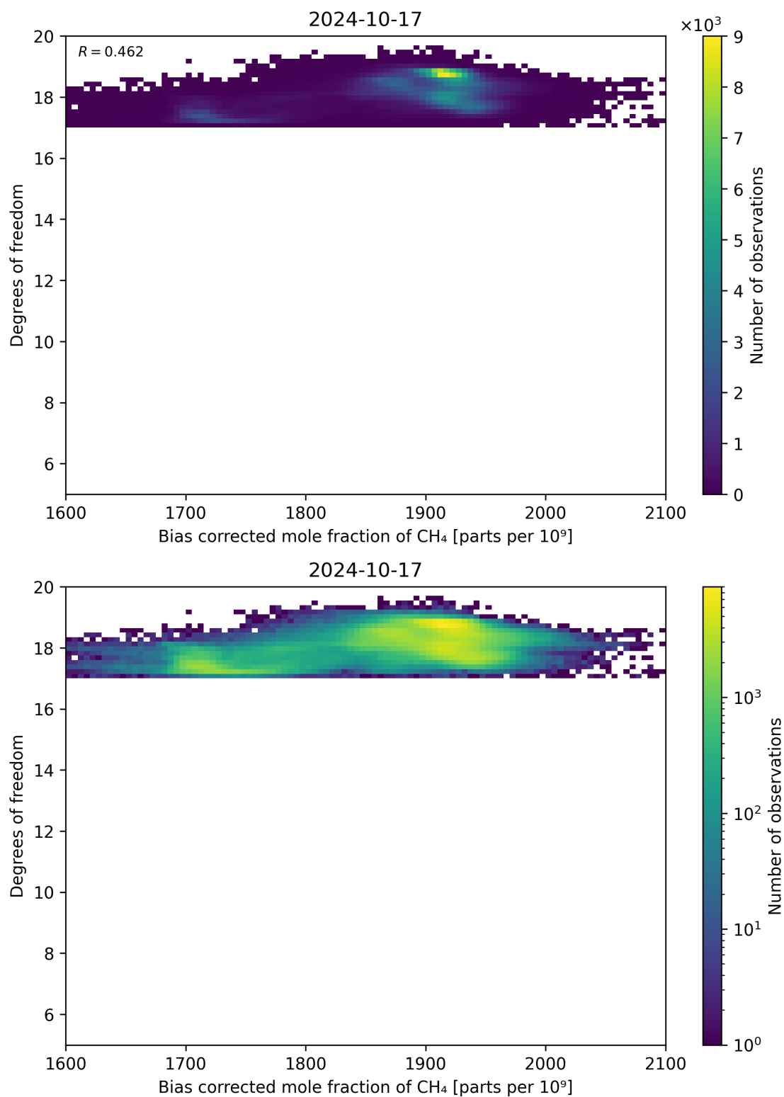
Figure 65: Scatter density plot of “Bias corrected mole fraction of CH 4 ” against “Degrees of freedom” for 2024-10-16 to 2024-10-18.
