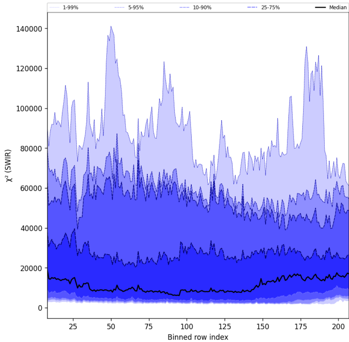
Figure 39: Along track statistics of " \chi^2 (SWIR)" for 2024-10-16 to 2024-10-18
