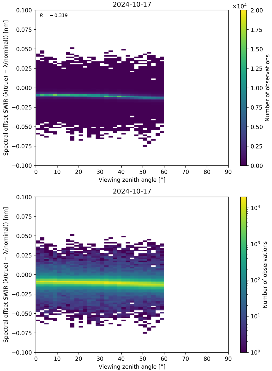
Figure 116: Scatter density plot of “Viewing zenith angle” against “Spectral offset SWIR ( \lambda_{\text{true}} - \lambda_{\text{nominal}} )” for 2024-10-16 to 2024-10-18.
