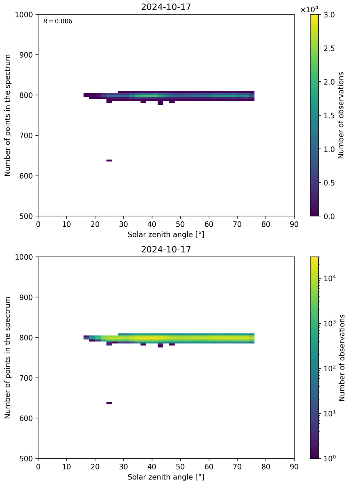
Figure 103: Scatter density plot of “Solar zenith angle” against “Number of points in the spectrum” for 2024-10-16 to 2024-10-18.
