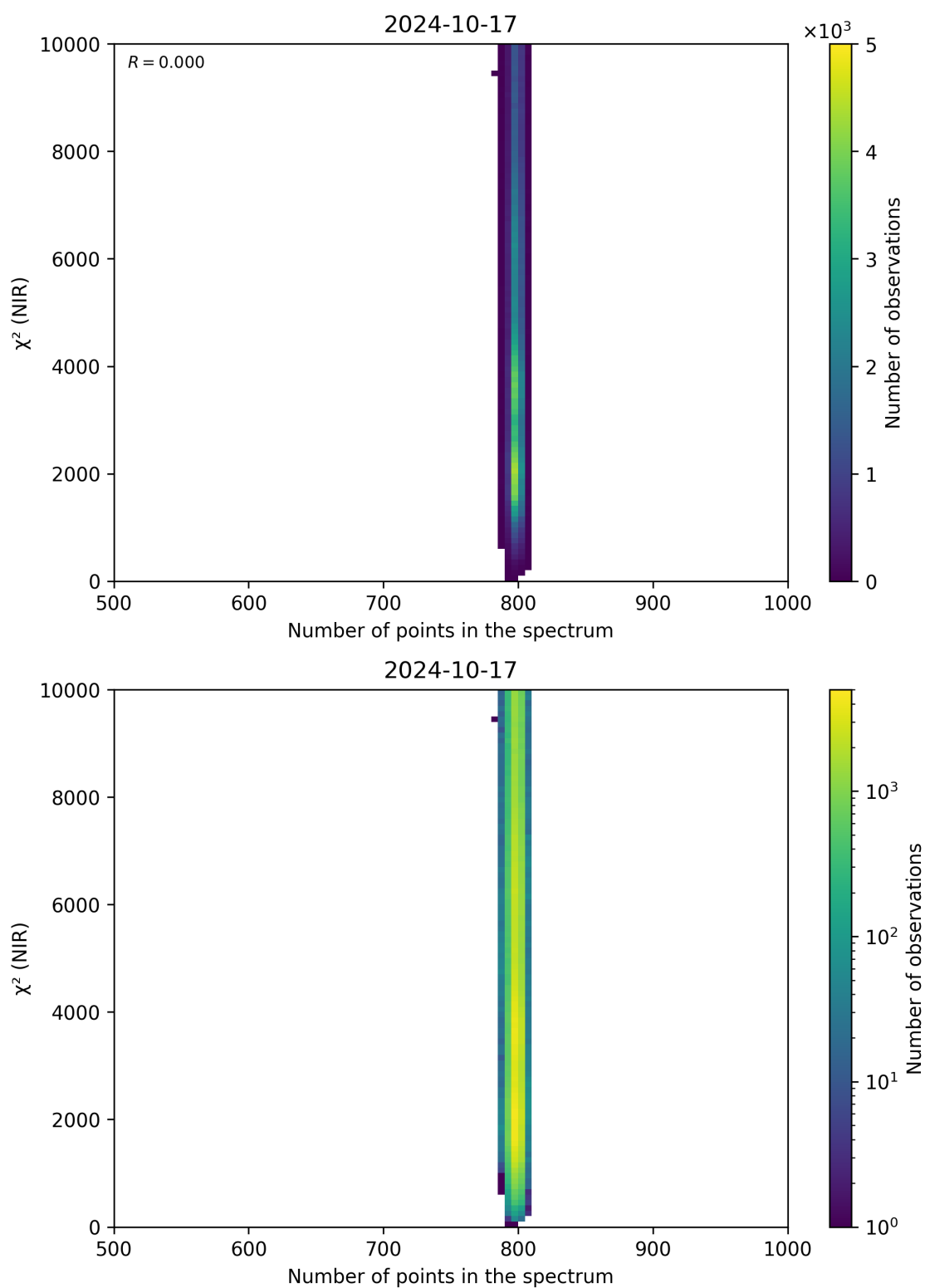
Figure 88: Scatter density plot of “Number of points in the spectrum” against “ \chi^2 (NIR)” for 2024-10-16 to 2024-10-18.
