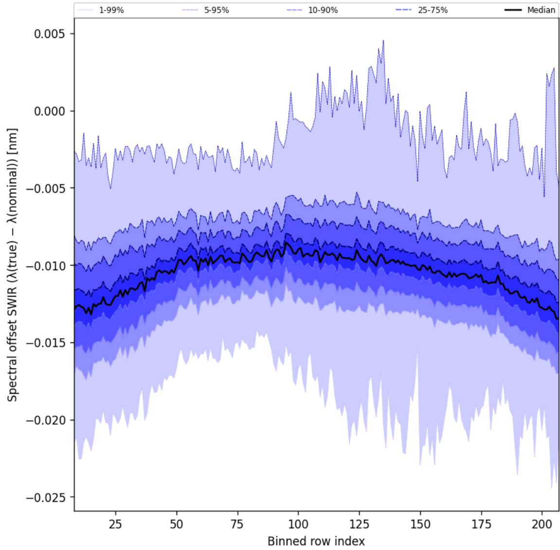
Figure 38: Along track statistics of “Spectral offset SWIR ( \lambda_{\text{true}} - \lambda_{\text{nominal}} )” for 2024-10-16 to 2024-10-18
