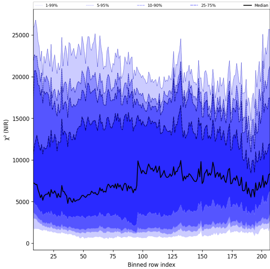
Figure 40: Along track statistics of “ \chi^2 (NIR)” for 2024-10-16 to 2024-10-18
