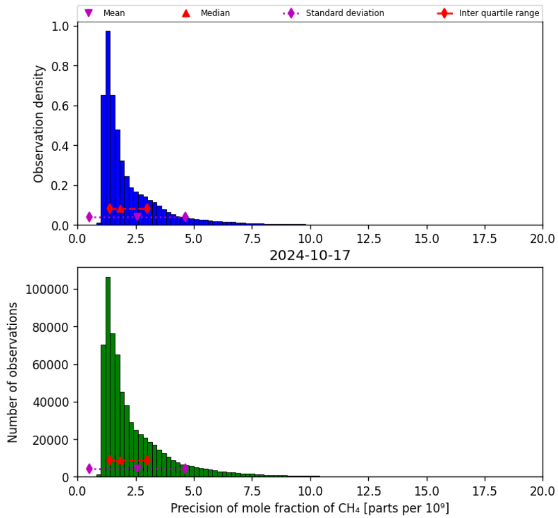
Figure 24: Histogram of “Precision of mole fraction of CH 4 ” for 2024-10-16 to 2024-10-18
