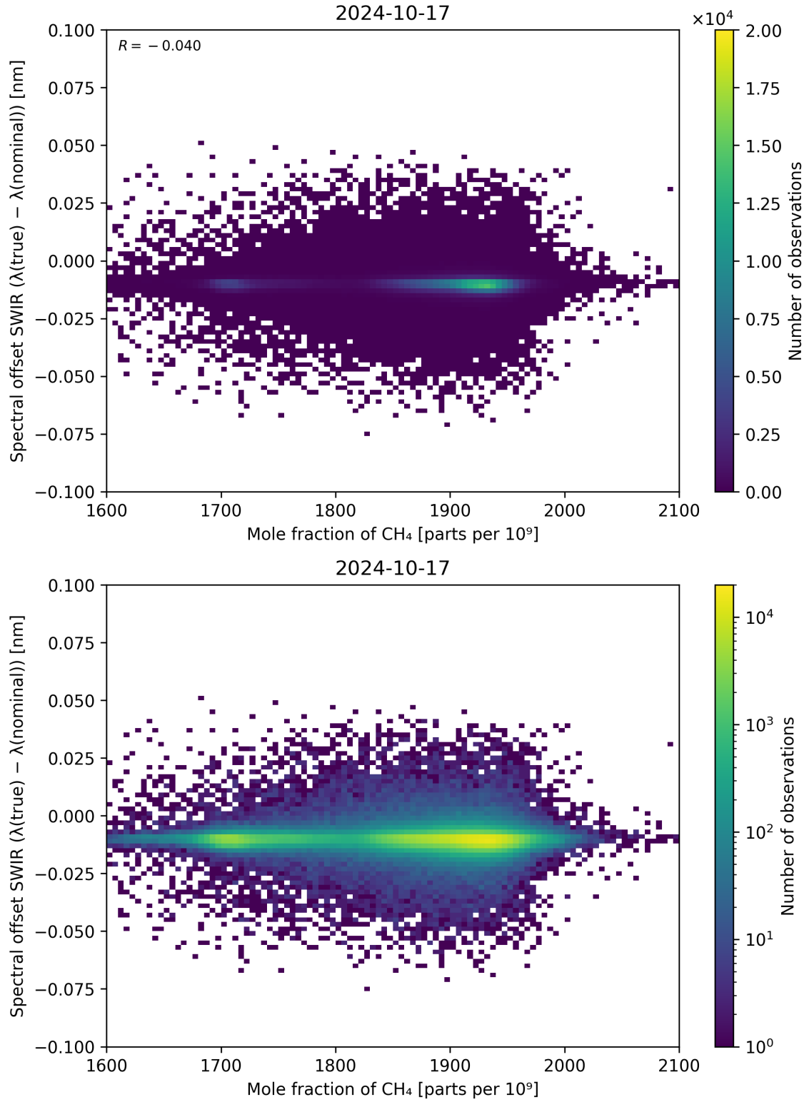
Figure 86: Scatter density plot of “Mole fraction of CH 4 ” against “Spectral offset SWIR ( \lambda_{\text{true}} - \lambda_{\text{nominal}} )” for 2024-10-16 to 2024-10-18.
