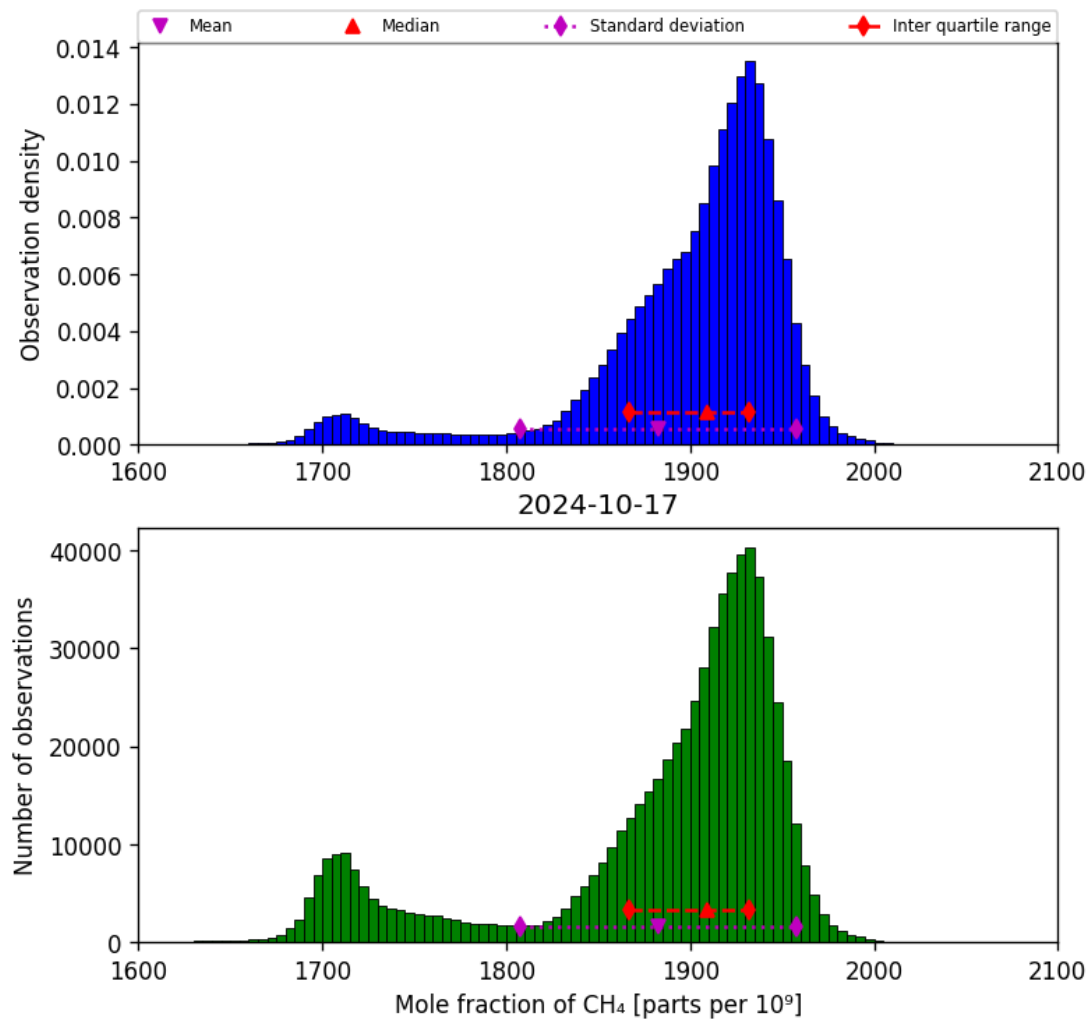
Figure 23: Histogram of “Mole fraction of CH 4 ” for 2024-10-16 to 2024-10-18
