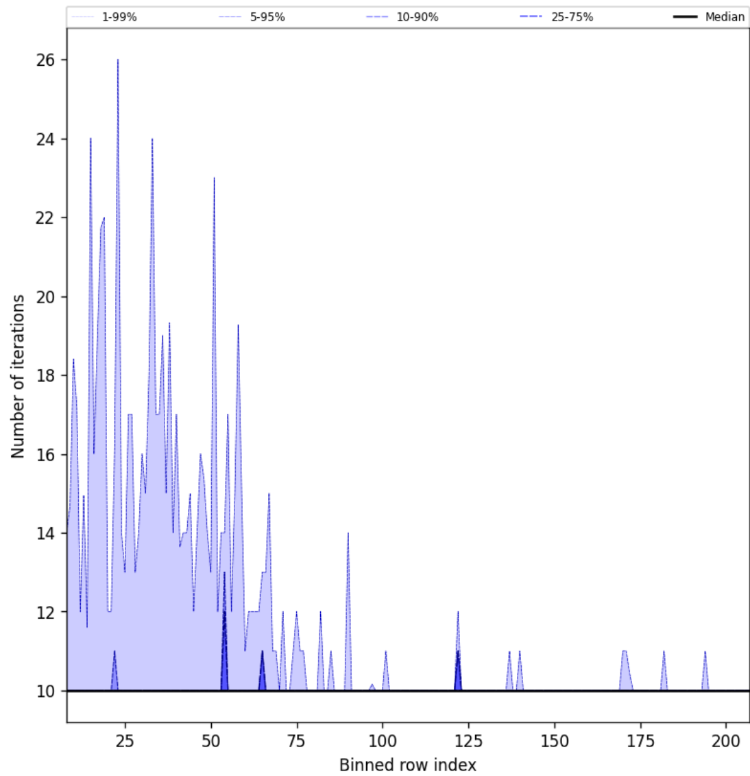
Figure 42: Along track statistics of “Number of iterations” for 2024-10-16 to 2024-10-18
