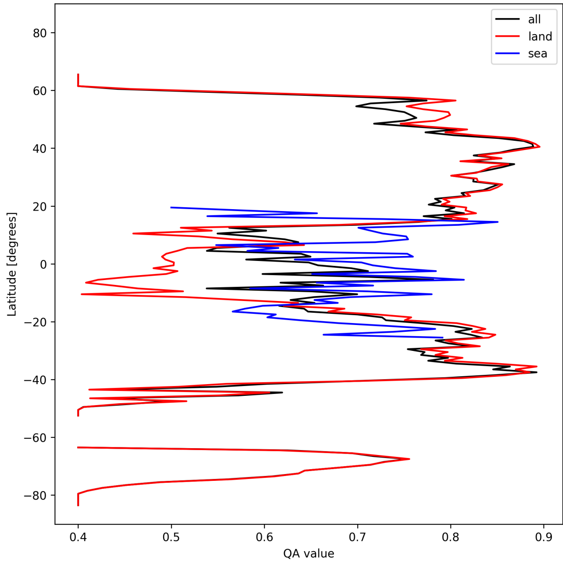
Figure 11: Zonal average of “QA value” for 2024-10-16 to 2024-10-18.
