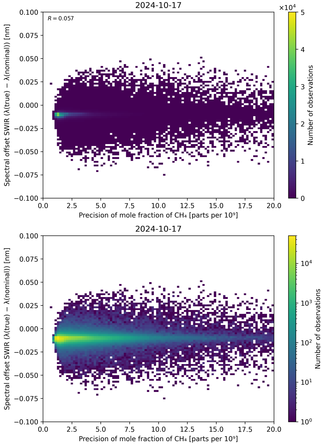
Figure 85: Scatter density plot of “Precision of mole fraction of CH 4 ” against “Spectral offset SWIR ( \lambda_{\text{true}} - \lambda_{\text{nominal}} )” for 2024-10-16 to 2024-10-18.
