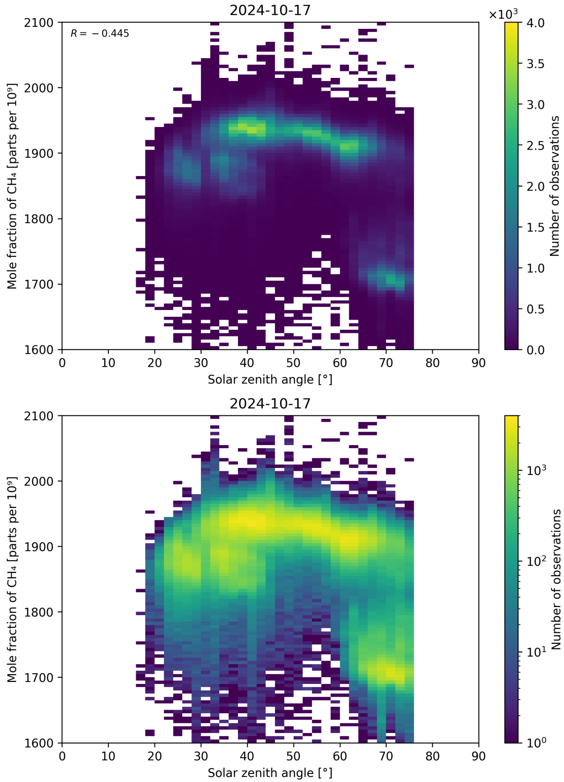
Figure 99: Scatter density plot of “Solar zenith angle” against “Mole fraction of \text{CH}_4 ” for 2024-10-16 to 2024-10-18.
