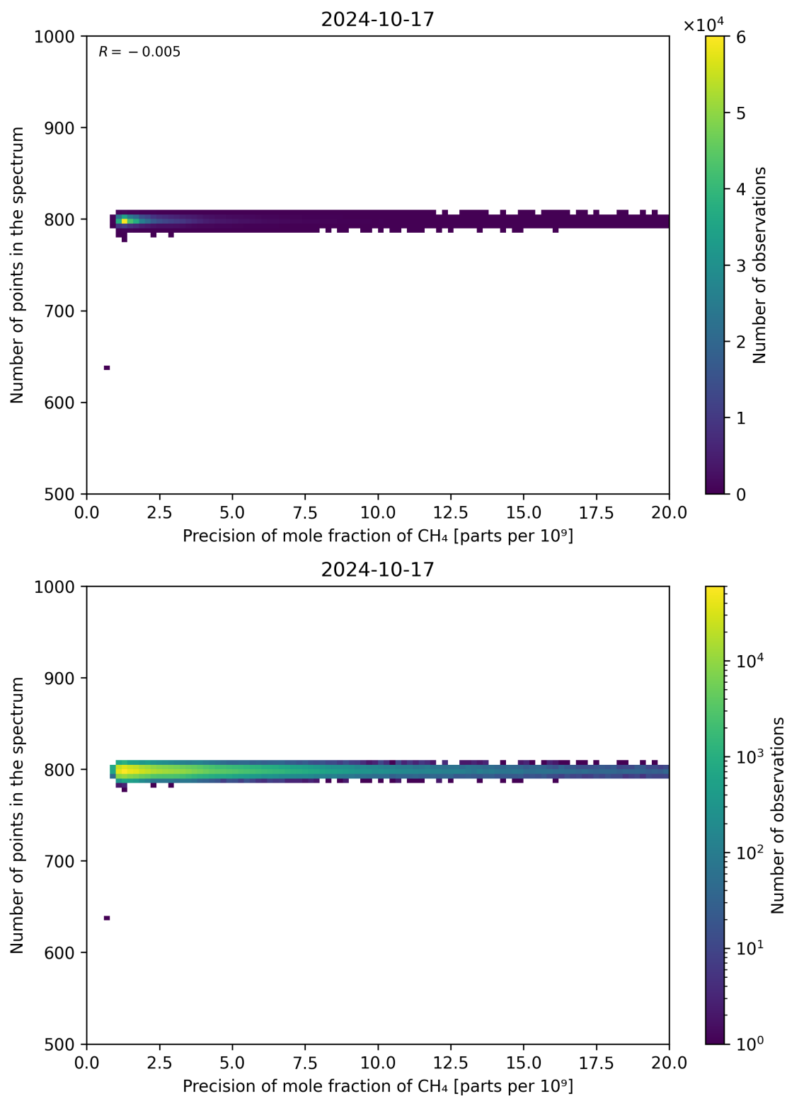
Figure 84: Scatter density plot of “Precision of mole fraction of CH 4 ” against “Number of points in the spectrum” for 2024-10-16 to 2024-10-18.
