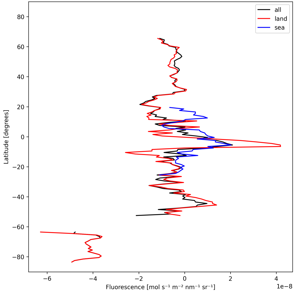
Figure 21: Zonal average of “Fluorescence” for 2024-10-16 to 2024-10-18.
