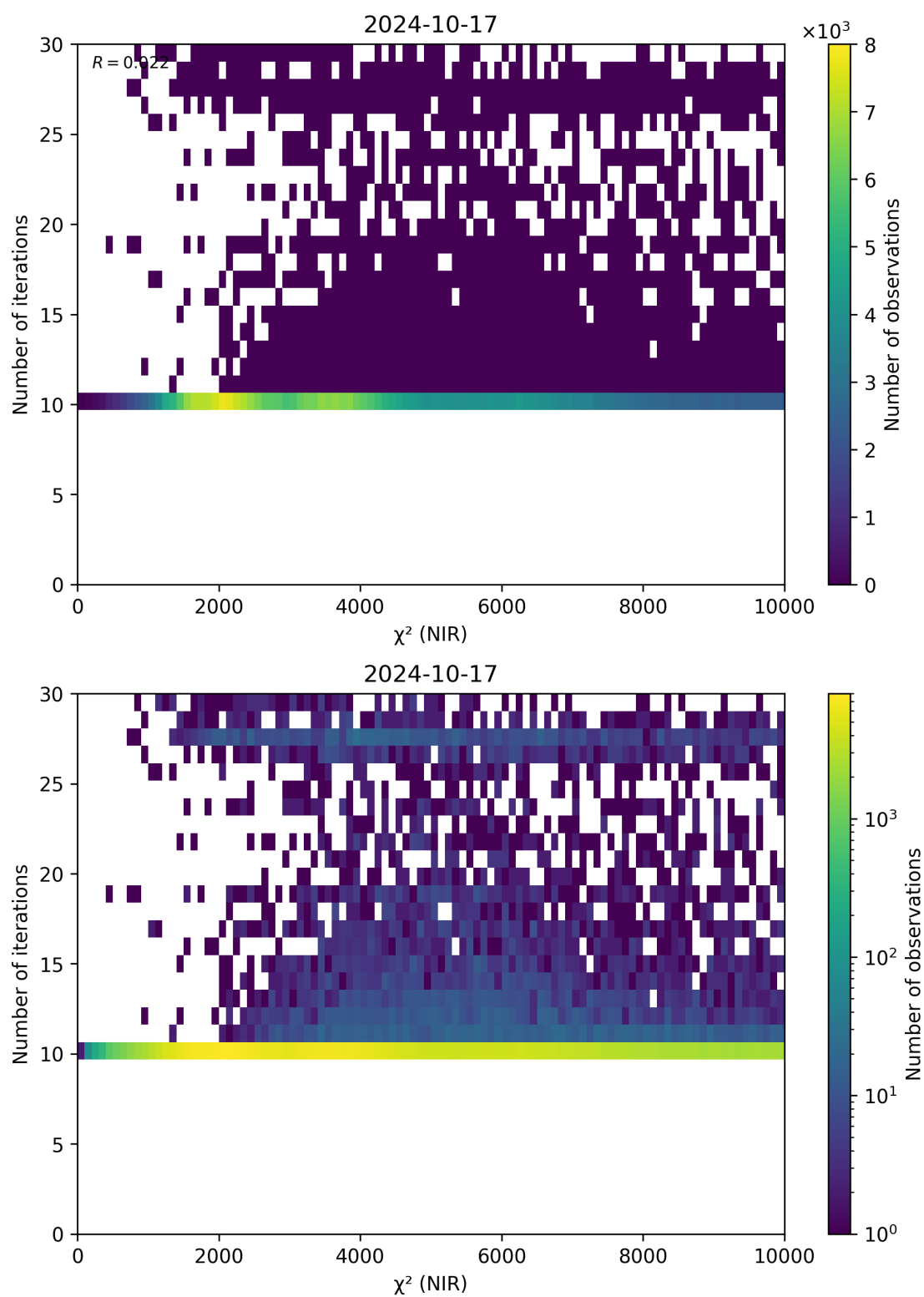
Figure 46: Scatter density plot of “ \chi^2 (NIR)” against “Number of iterations” for 2024-10-16 to 2024-10-18.
