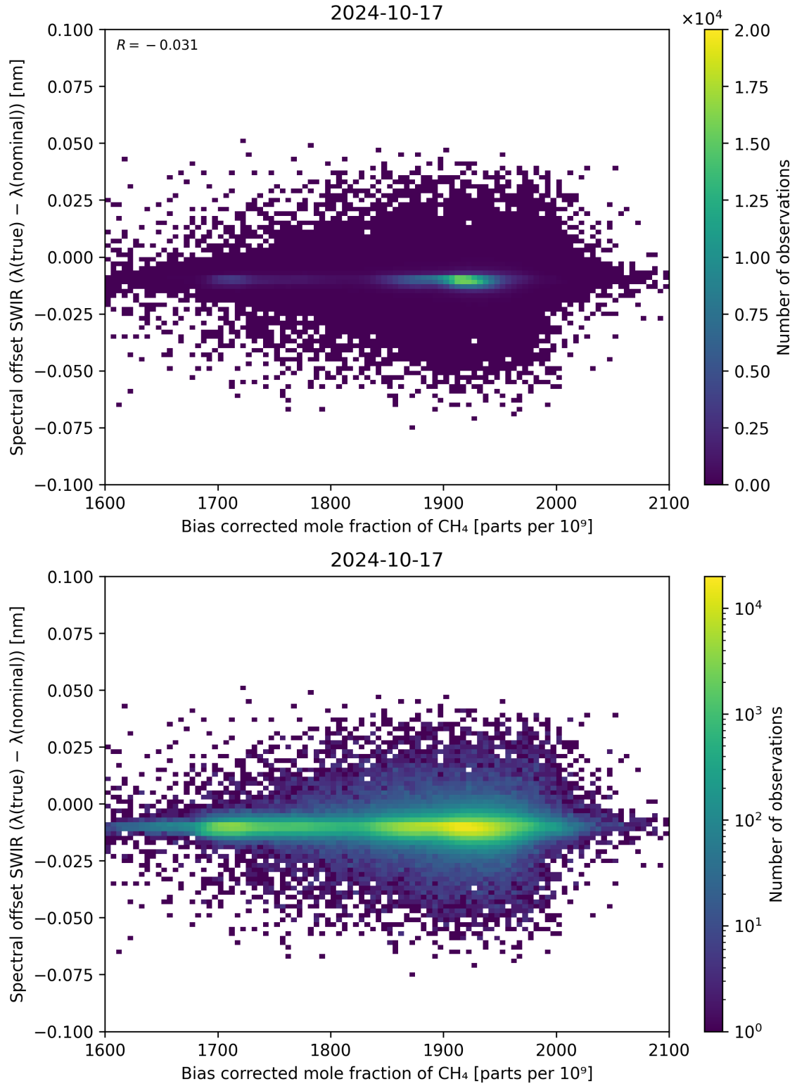
Figure 69: Scatter density plot of “Bias corrected mole fraction of \text{CH}_4 ” against “Spectral offset SWIR ( \lambda_{\text{true}} - \lambda_{\text{nominal}} )” for 2024-10-16 to 2024-10-18.
