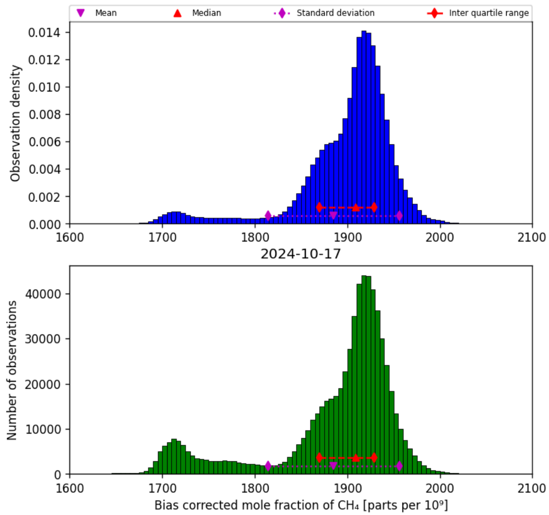
Figure 25: Histogram of “Bias corrected mole fraction of CH 4 ” for 2024-10-16 to 2024-10-18
