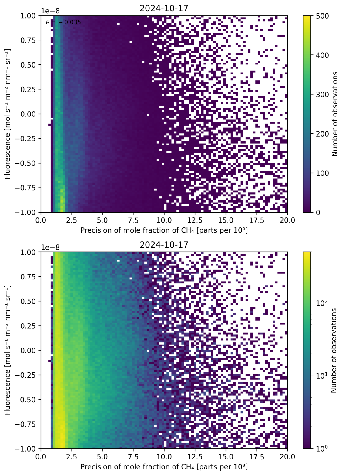
Figure 81: Scatter density plot of “Precision of mole fraction of \text{CH}_4 ” against “Fluorescence” for 2024-10-16 to 2024-10-18.
