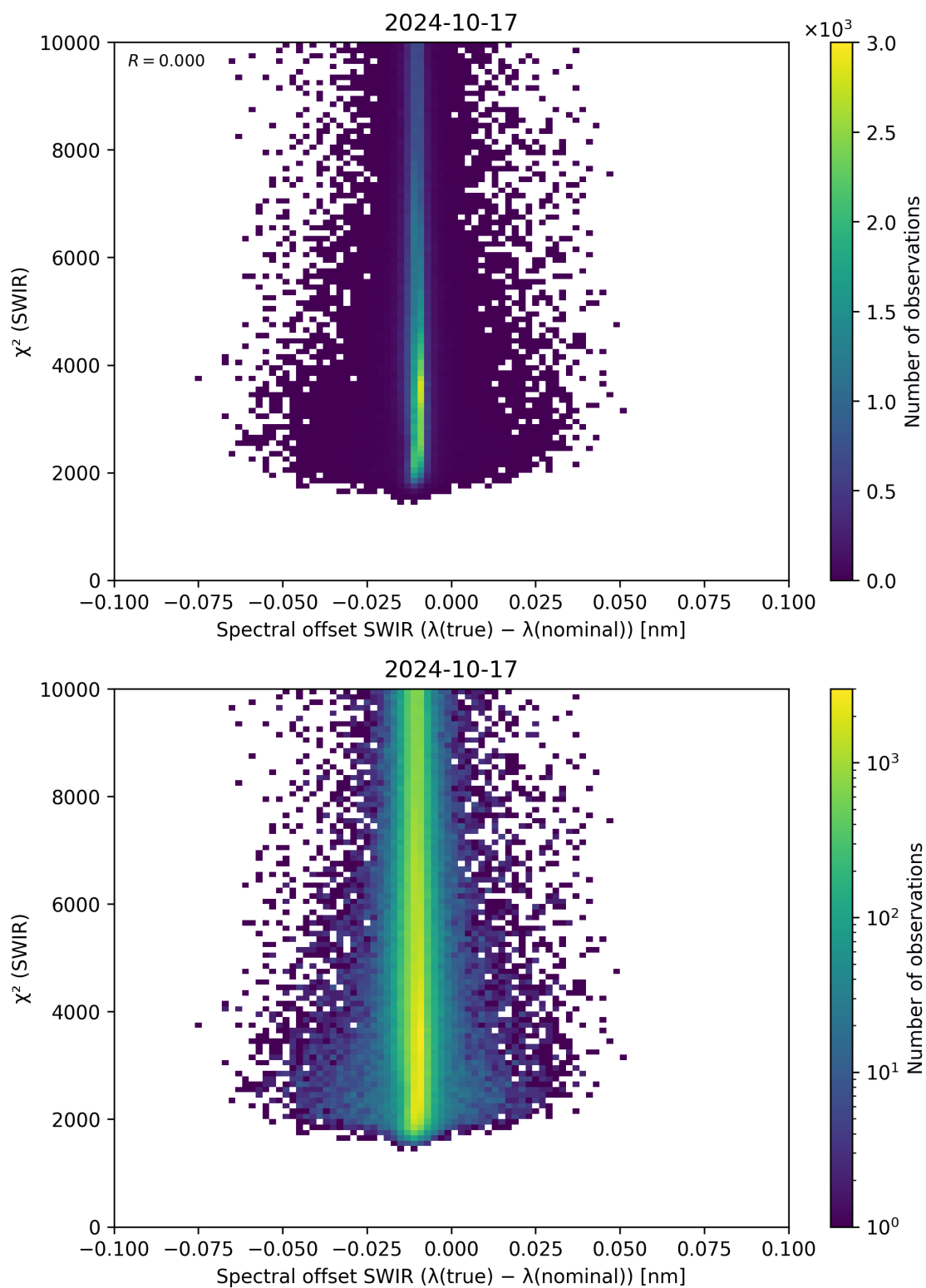
Figure 118: Scatter density plot of “Spectral offset SWIR ( \lambda_{\text{true}} - \lambda_{\text{nominal}} )” against “ \chi^2 (SWIR)” for 2024-10-16 to 2024-10-18.
