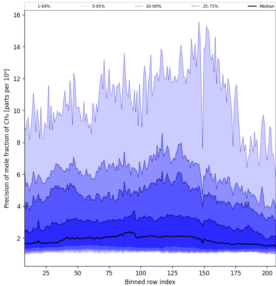
Figure 35: Along track statistics of “Precision of mole fraction of CH 4 ” for 2024-10-16 to 2024-10-18
