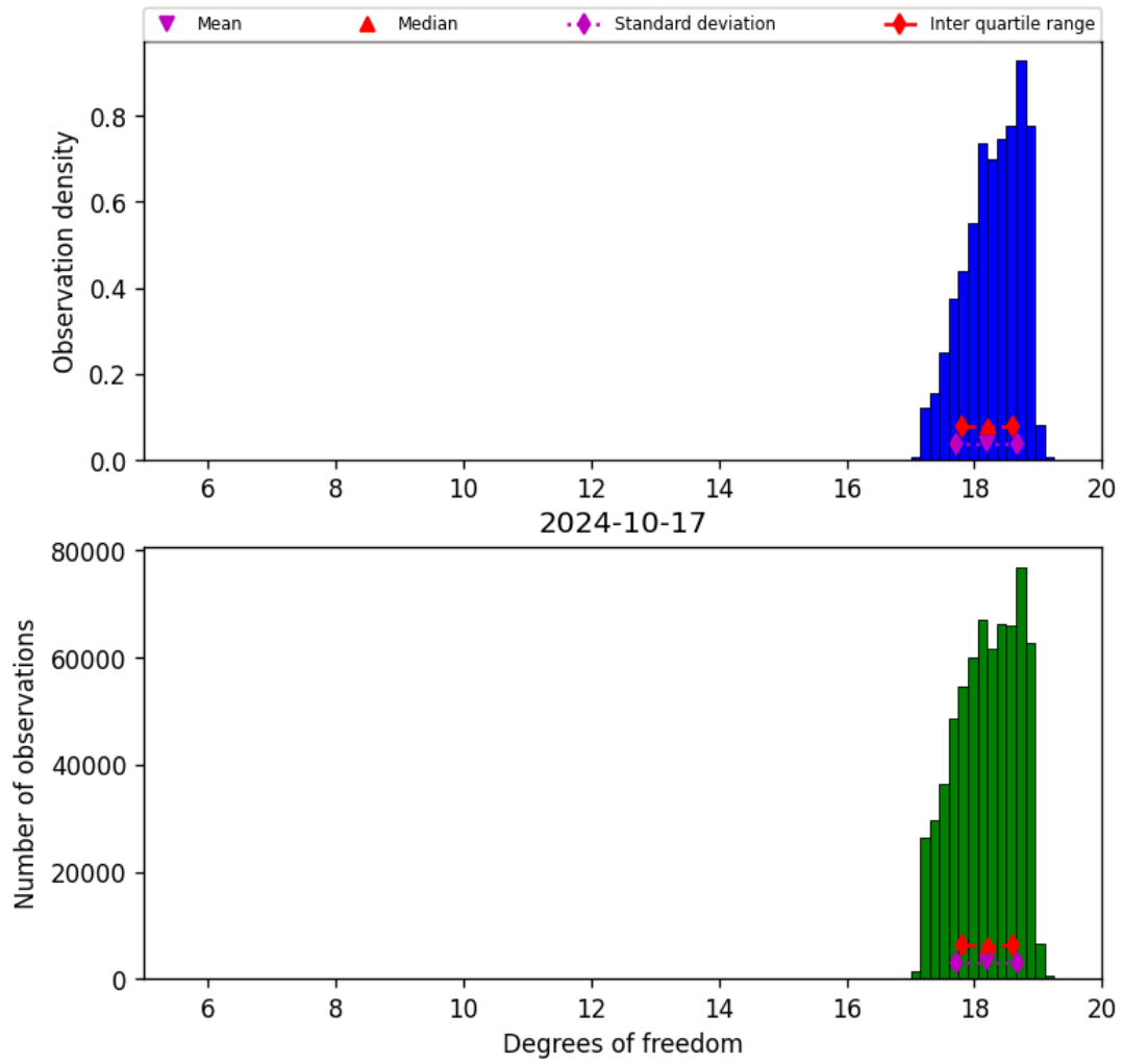
Figure 30: Histogram of “Degrees of freedom” for 2024-10-16 to 2024-10-18
