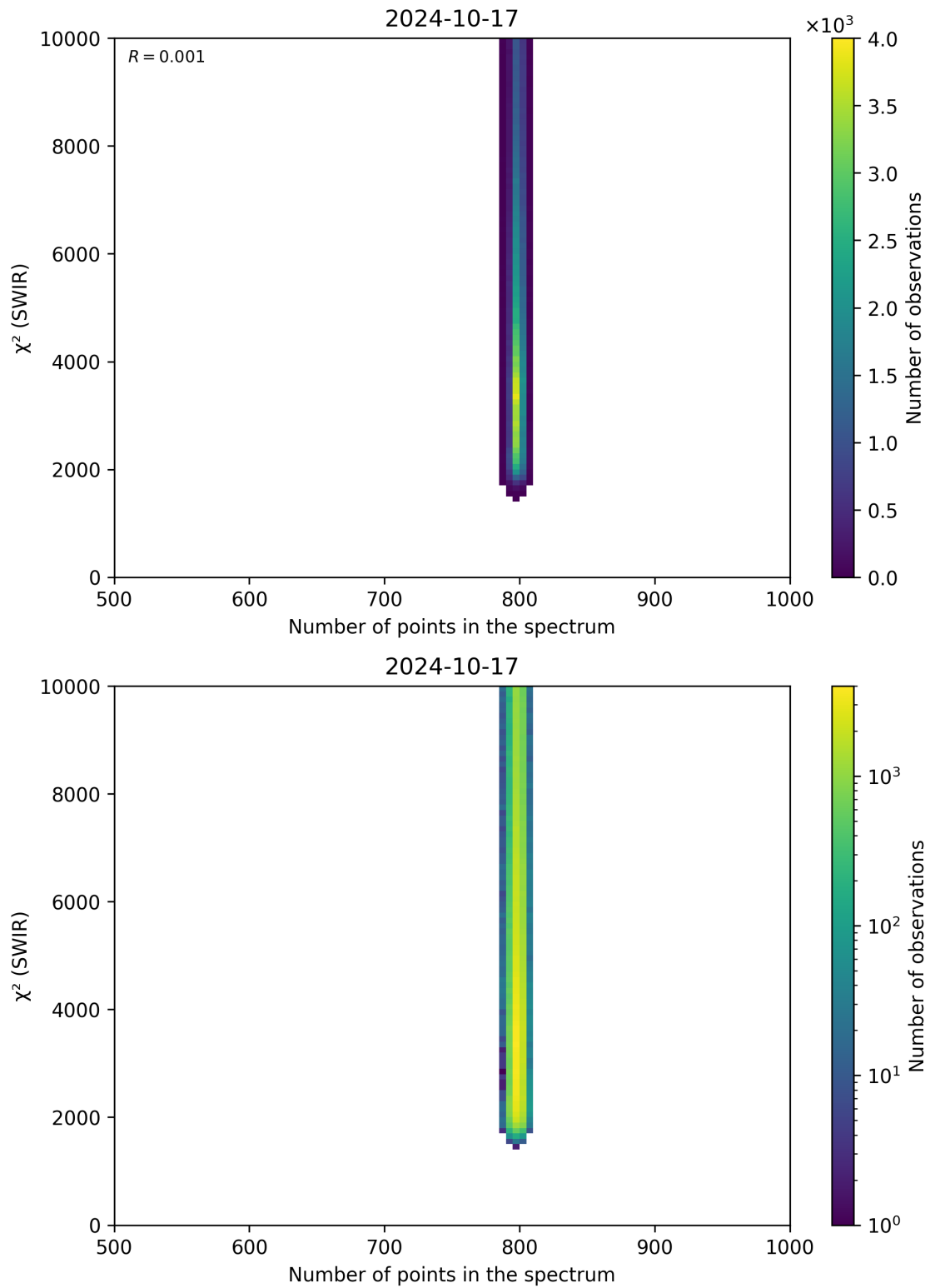
Figure 89: Scatter density plot of “Number of points in the spectrum” against “ \chi^2 (SWIR)” for 2024-10-16 to 2024-10-18.
