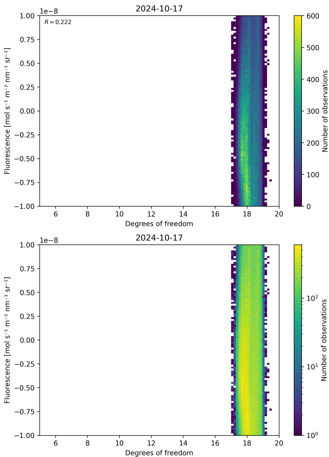
Figure 51: Scatter density plot of “Degrees of freedom” against “Fluorescence” for 2024-10-16 to 2024-10-18.
