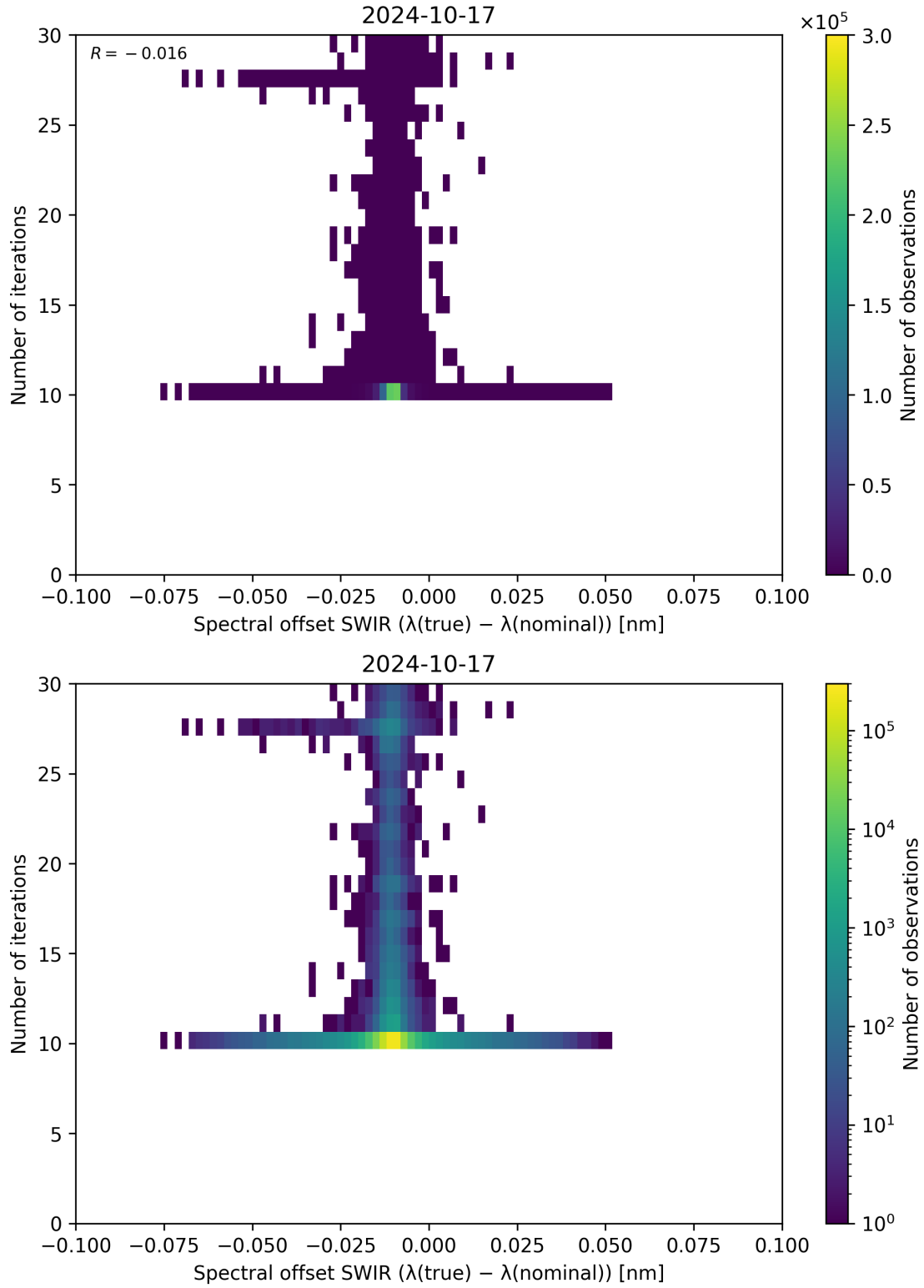
Figure 121: Scatter density plot of “Spectral offset SWIR ( \lambda_{\text{true}} - \lambda_{\text{nominal}} )” against “Number of iterations” for 2024-10-16 to 2024-10-18.
