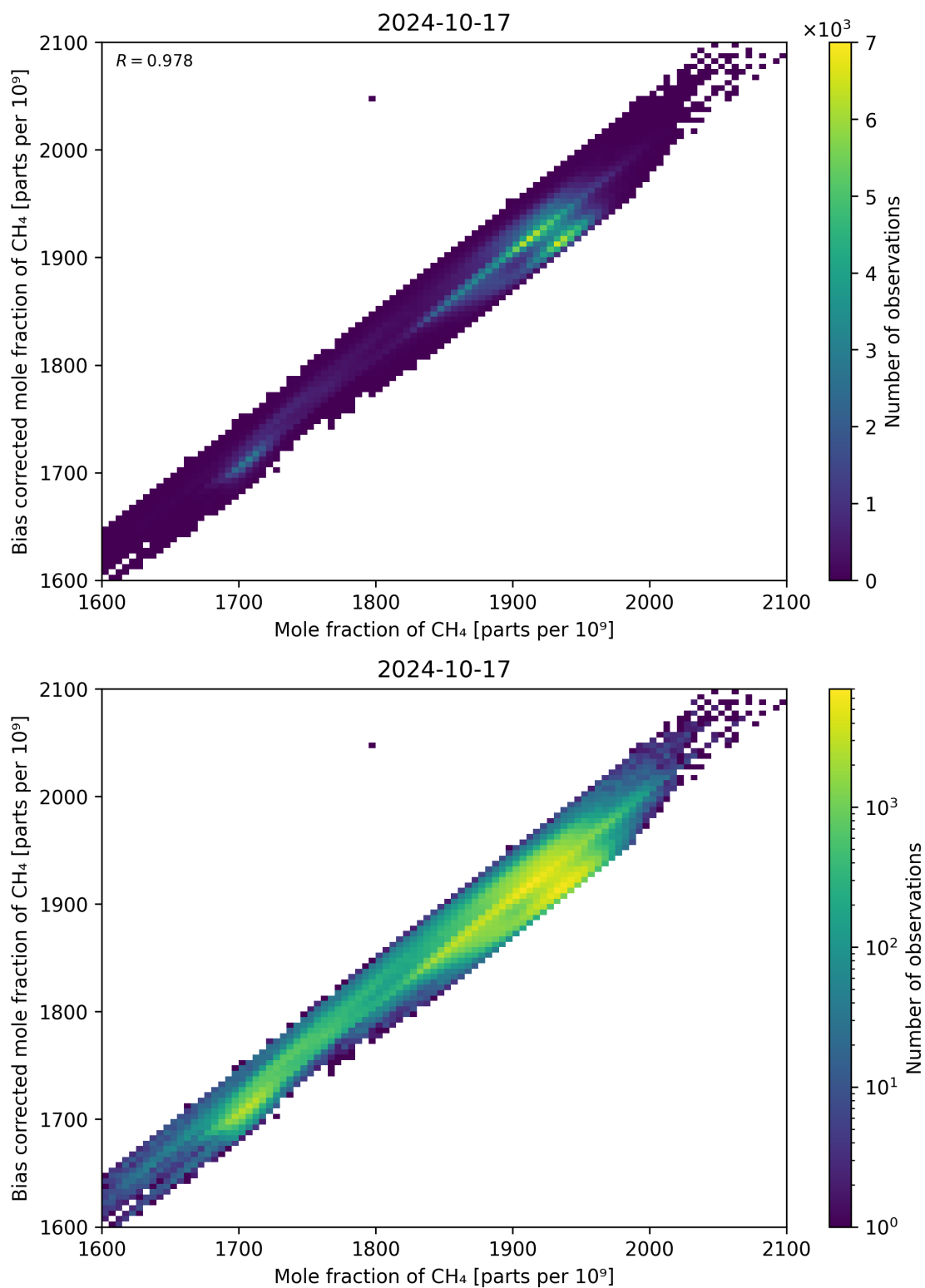
Figure 74: Scatter density plot of “Mole fraction of CH 4 ” against “Bias corrected mole fraction of CH 4 ” for 2024-10-16 to 2024-10-18.
