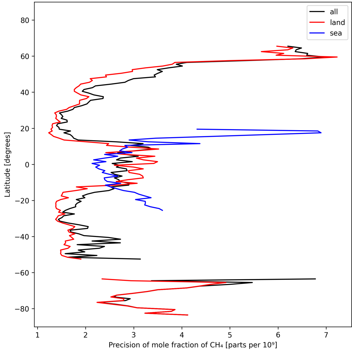
Figure 13: Zonal average of “Precision of mole fraction of CH 4 ” for 2024-10-16 to 2024-10-18.
