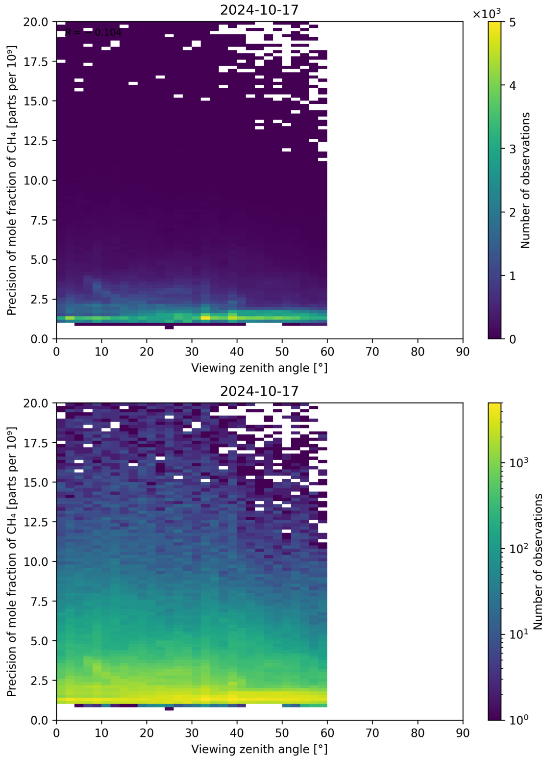
Figure 112: Scatter density plot of “Viewing zenith angle” against “Precision of mole fraction of CH 4 ” for 2024-10-16 to 2024-10-18.
