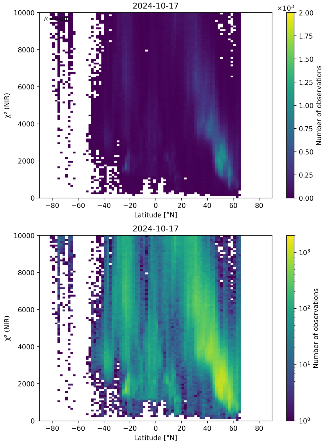
Figure 53: Scatter density plot of “Latitude” against “ \chi^2 (NIR)” for 2024-10-16 to 2024-10-18.
