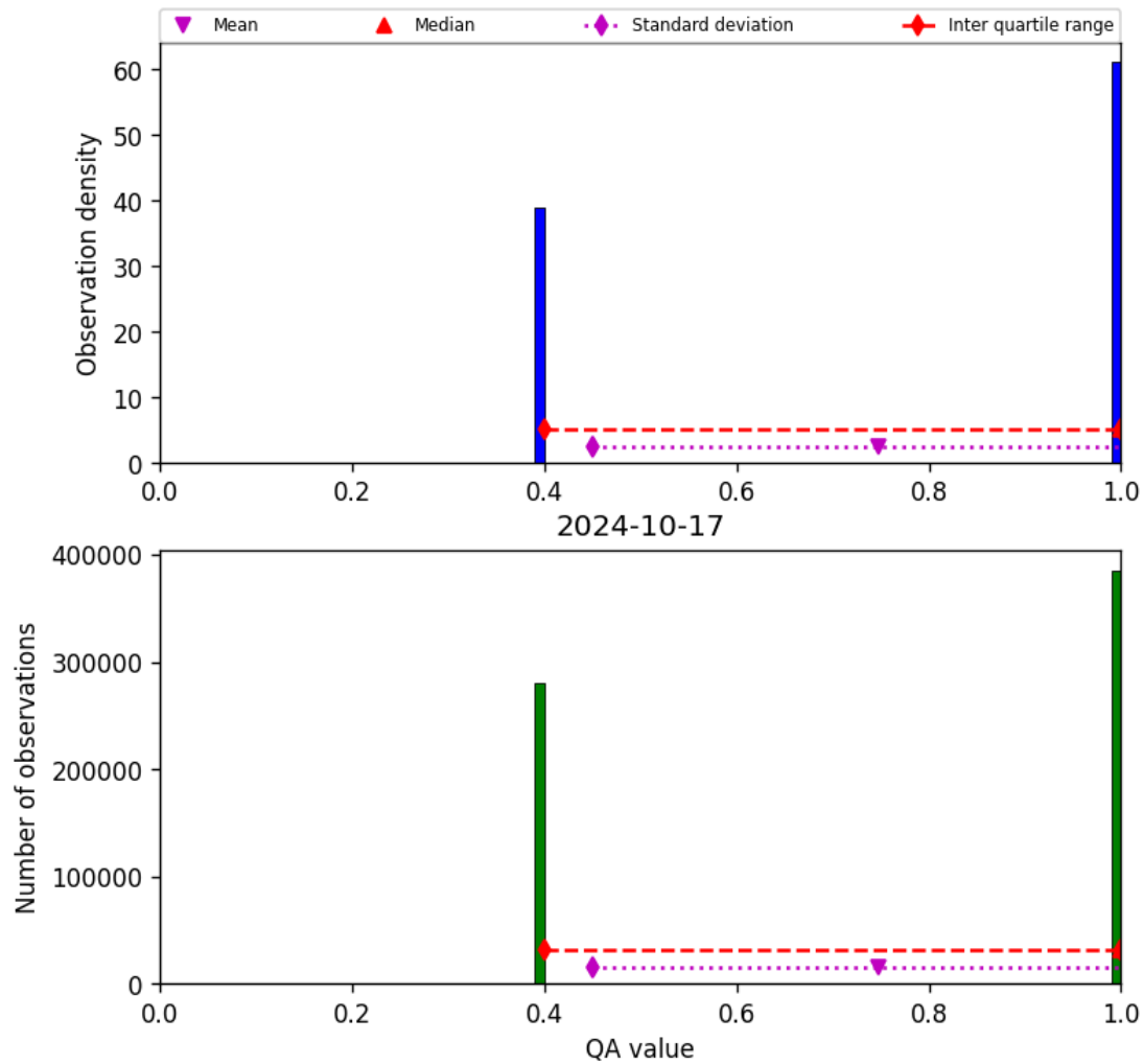
Figure 22: Histogram of “QA value” for 2024-10-16 to 2024-10-18
