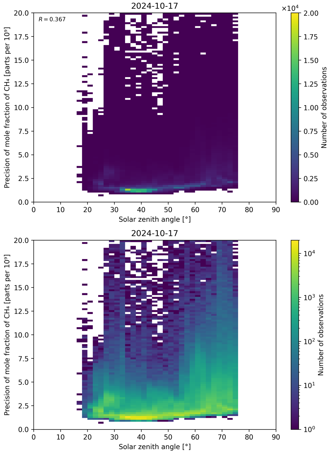
Figure 101: Scatter density plot of “Solar zenith angle” against “Precision of mole fraction of CH 4 ” for 2024-10-16 to 2024-10-18.
