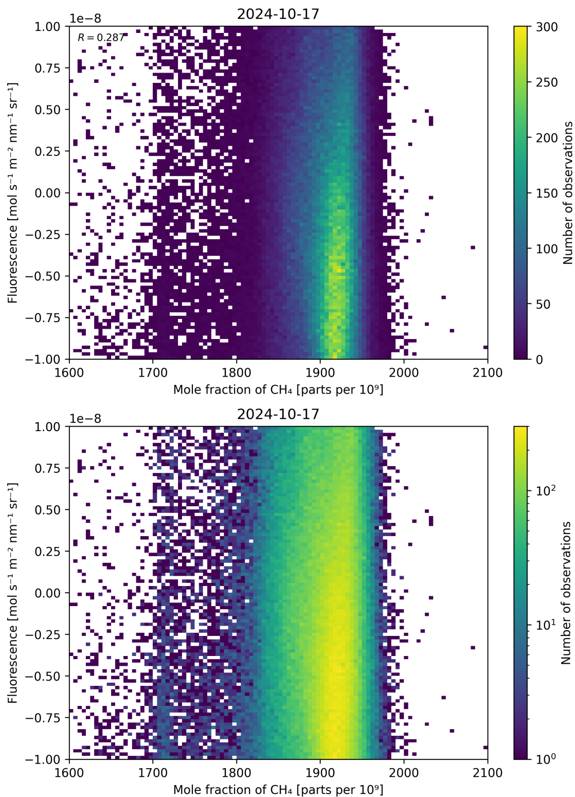
Figure 73: Scatter density plot of “Mole fraction of \text{CH}_4 ” against “Fluorescence” for 2024-10-16 to 2024-10-18.
