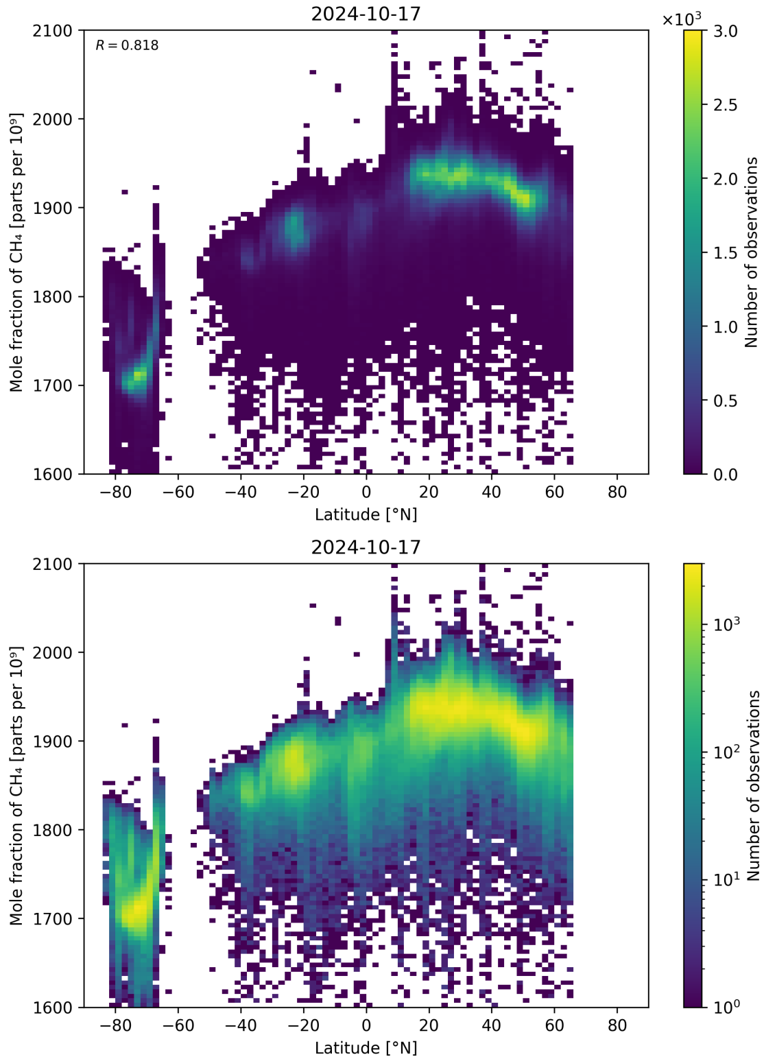
Figure 57: Scatter density plot of “Latitude” against “Mole fraction of \text{CH}_4 ” for 2024-10-16 to 2024-10-18.
