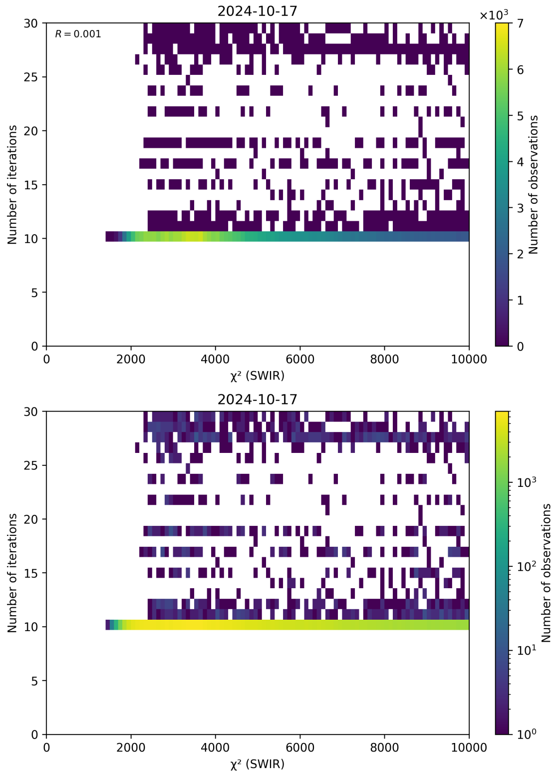
Figure 50: Scatter density plot of “ \chi^2 (SWIR)” against “Number of iterations” for 2024-10-16 to 2024-10-18.
