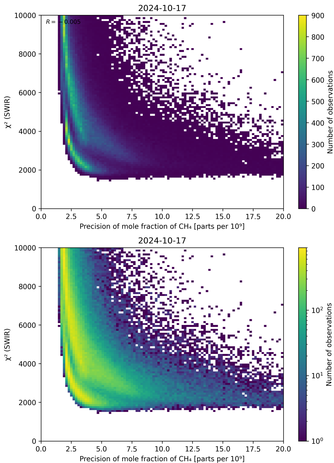
Figure 79: Scatter density plot of “Precision of mole fraction of \text{CH}_4 ” against “ \chi^2 (SWIR)” for 2024-10-16 to 2024-10-18.
