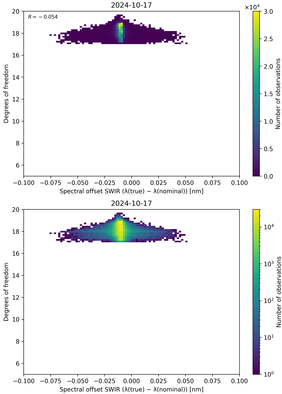
Figure 119: Scatter density plot of “Spectral offset SWIR ( \lambda_{\text{true}} - \lambda_{\text{nominal}} )” against “Degrees of freedom” for 2024-10-16 to 2024-10-18.
