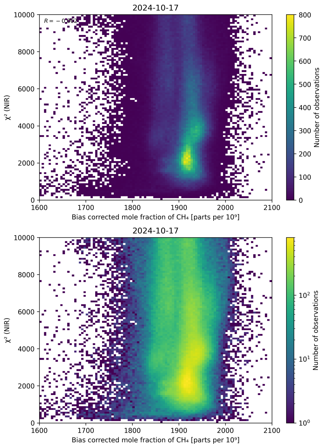
Figure 63: Scatter density plot of “Bias corrected mole fraction of \text{CH}_4 ” against “ \chi^2 (NIR)” for 2024-10-16 to 2024-10-18.
