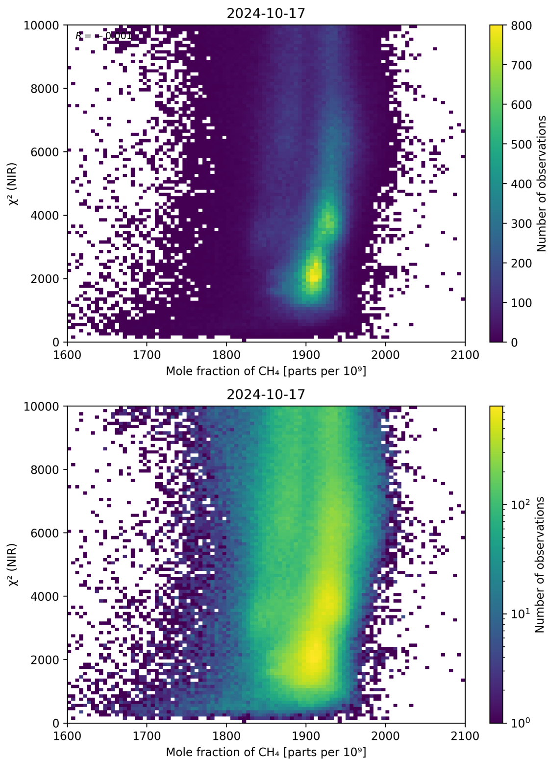
Figure 70: Scatter density plot of “Mole fraction of \text{CH}_4 ” against “ \chi^2 (NIR)” for 2024-10-16 to 2024-10-18.
