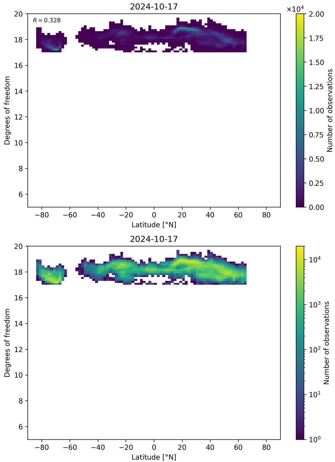
Figure 55: Scatter density plot of “Latitude” against “Degrees of freedom” for 2024-10-16 to 2024-10-18.
