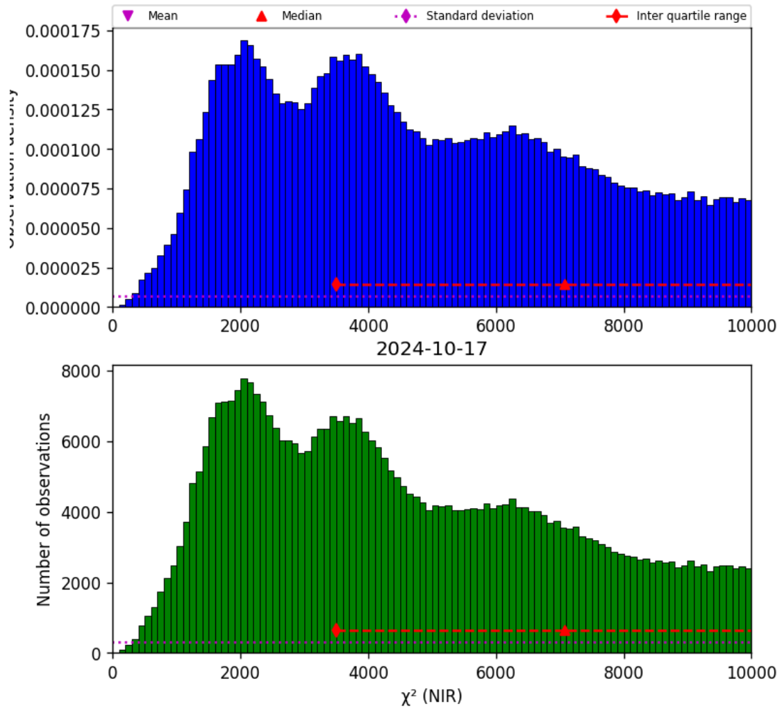
Figure 29: Histogram of “ \chi^2 (NIR)” for 2024-10-16 to 2024-10-18
