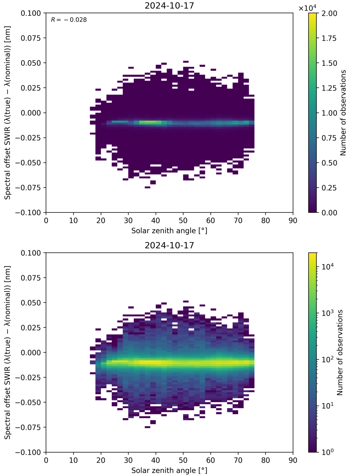
Figure 104: Scatter density plot of “Solar zenith angle” against “Spectral offset SWIR ( \lambda_{\text{true}} - \lambda_{\text{nominal}} )” for 2024-10-16 to 2024-10-18.
