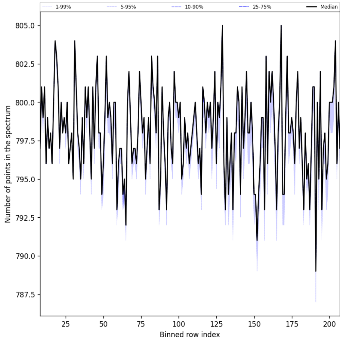
Figure 37: Along track statistics of “Number of points in the spectrum” for 2024-10-16 to 2024-10-18
