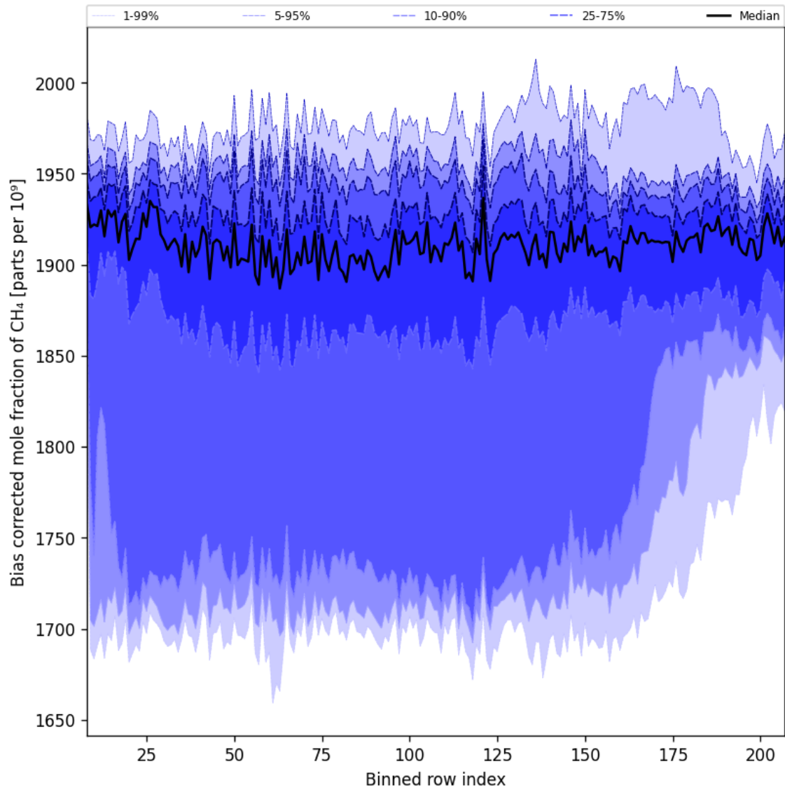
Figure 36: Along track statistics of “Bias corrected mole fraction of CH 4 ” for 2024-10-16 to 2024-10-18
