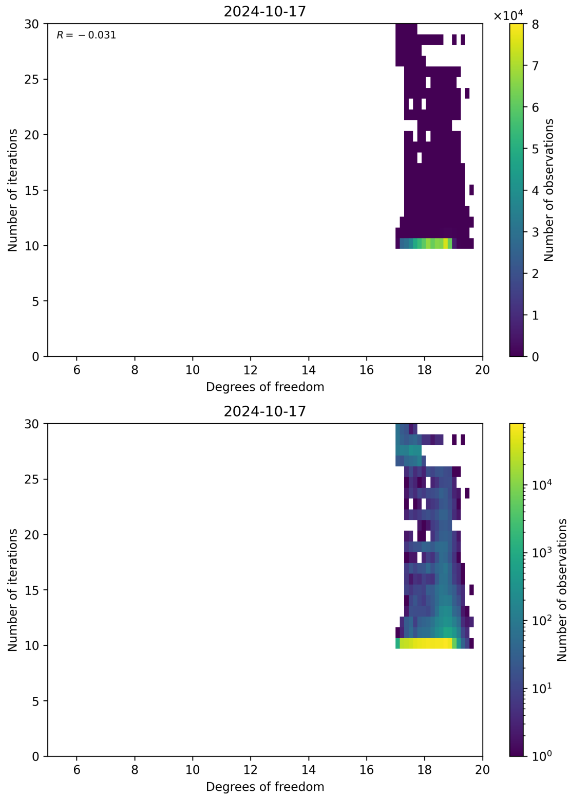
Figure 52: Scatter density plot of “Degrees of freedom” against “Number of iterations” for 2024-10-16 to 2024-10-18.
