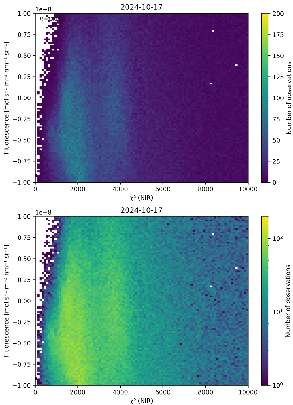
Figure 45: Scatter density plot of “ \chi^2 (NIR)” against “Fluorescence” for 2024-10-16 to 2024-10-18.
