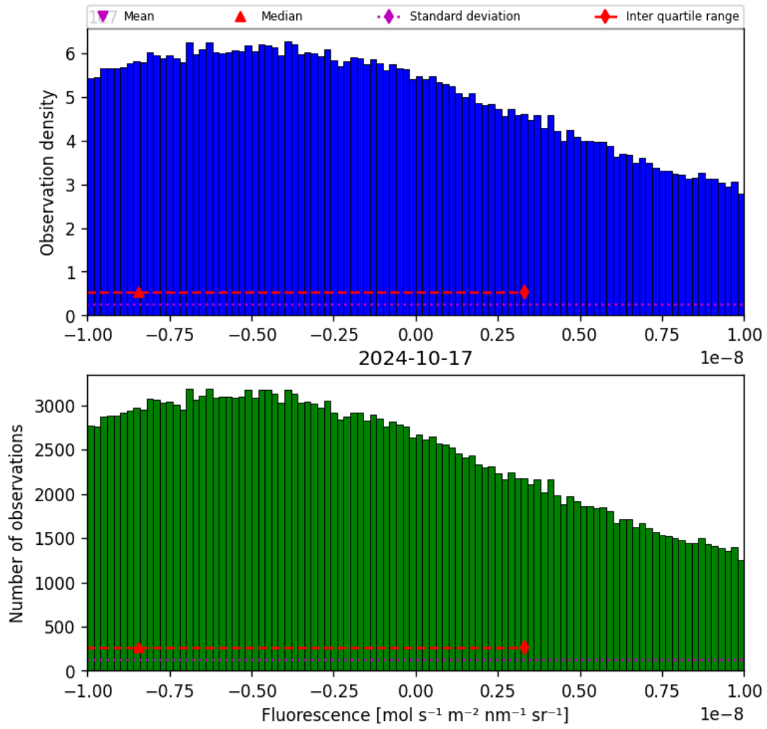
Figure 32: Histogram of “Fluorescence” for 2024-10-16 to 2024-10-18
