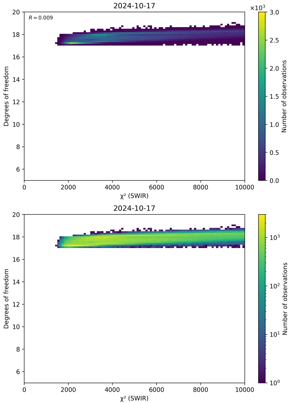
Figure 48: Scatter density plot of “ \chi^2 (SWIR)” against “Degrees of freedom” for 2024-10-16 to 2024-10-18.
