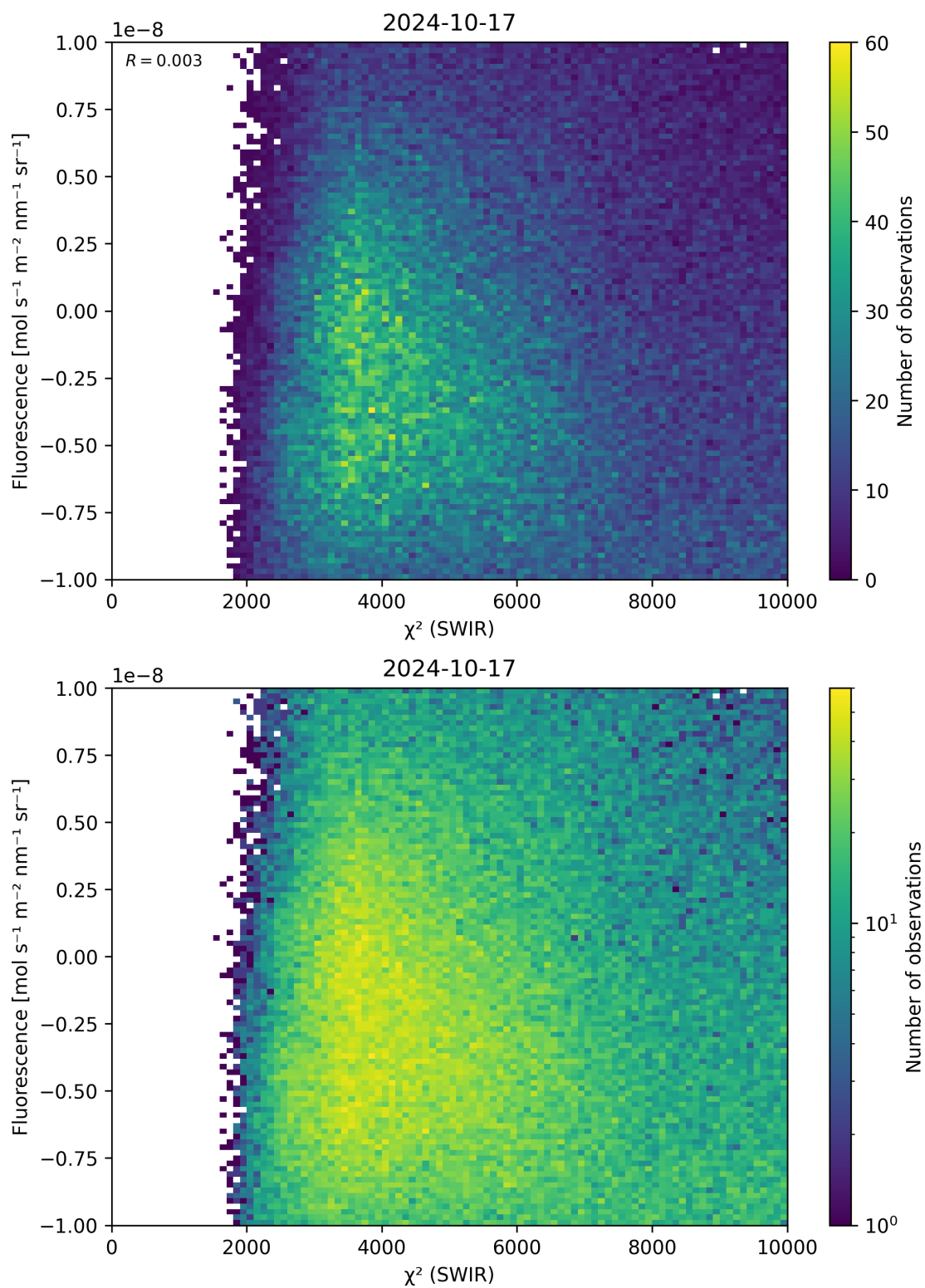
Figure 49: Scatter density plot of “ \chi^2 (SWIR)” against “Fluorescence” for 2024-10-16 to 2024-10-18.
