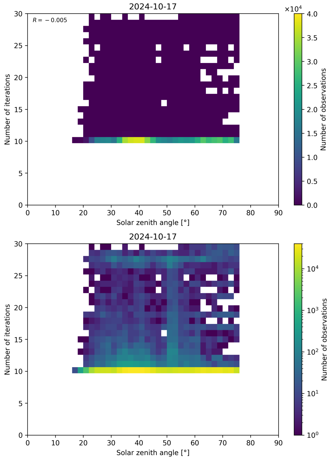
Figure 102: Scatter density plot of “Solar zenith angle” against “Number of iterations” for 2024-10-16 to 2024-10-18.
