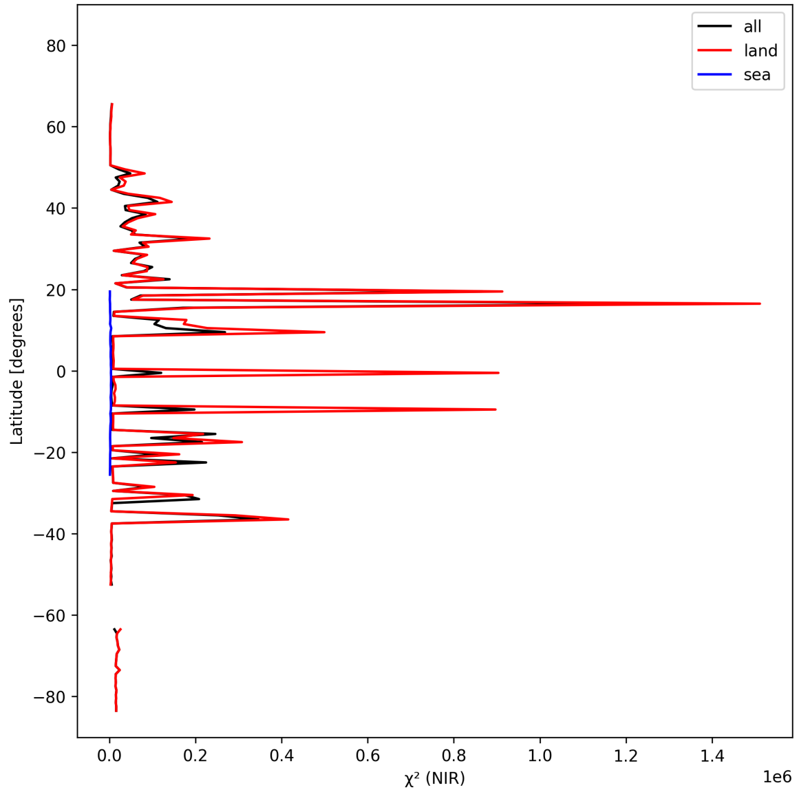
Figure 18: Zonal average of “ \chi^2 (NIR)” for 2024-10-16 to 2024-10-18.
