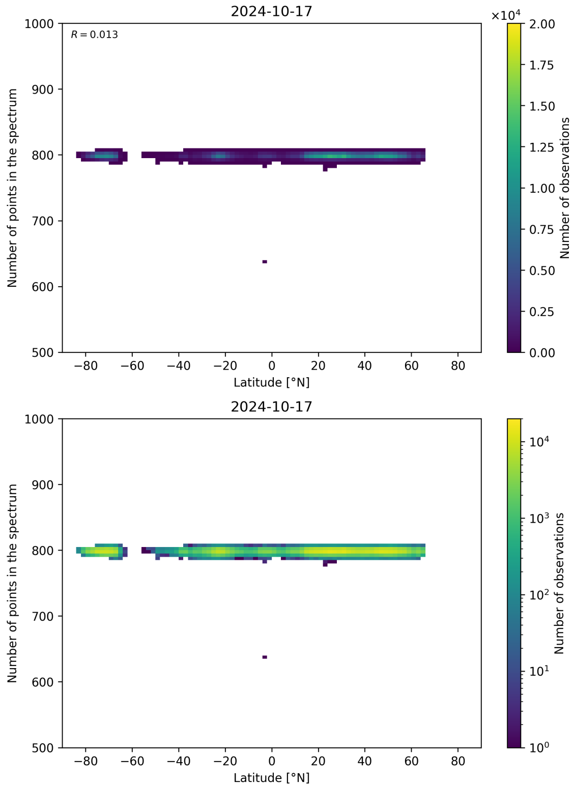
Figure 61: Scatter density plot of “Latitude” against “Number of points in the spectrum” for 2024-10-16 to 2024-10-18.
