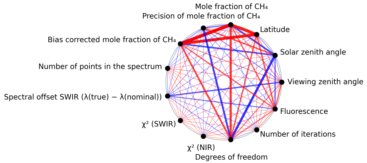
Figure 1: Map of correlation graph for 2024-10-16 to 2024-10-18.
