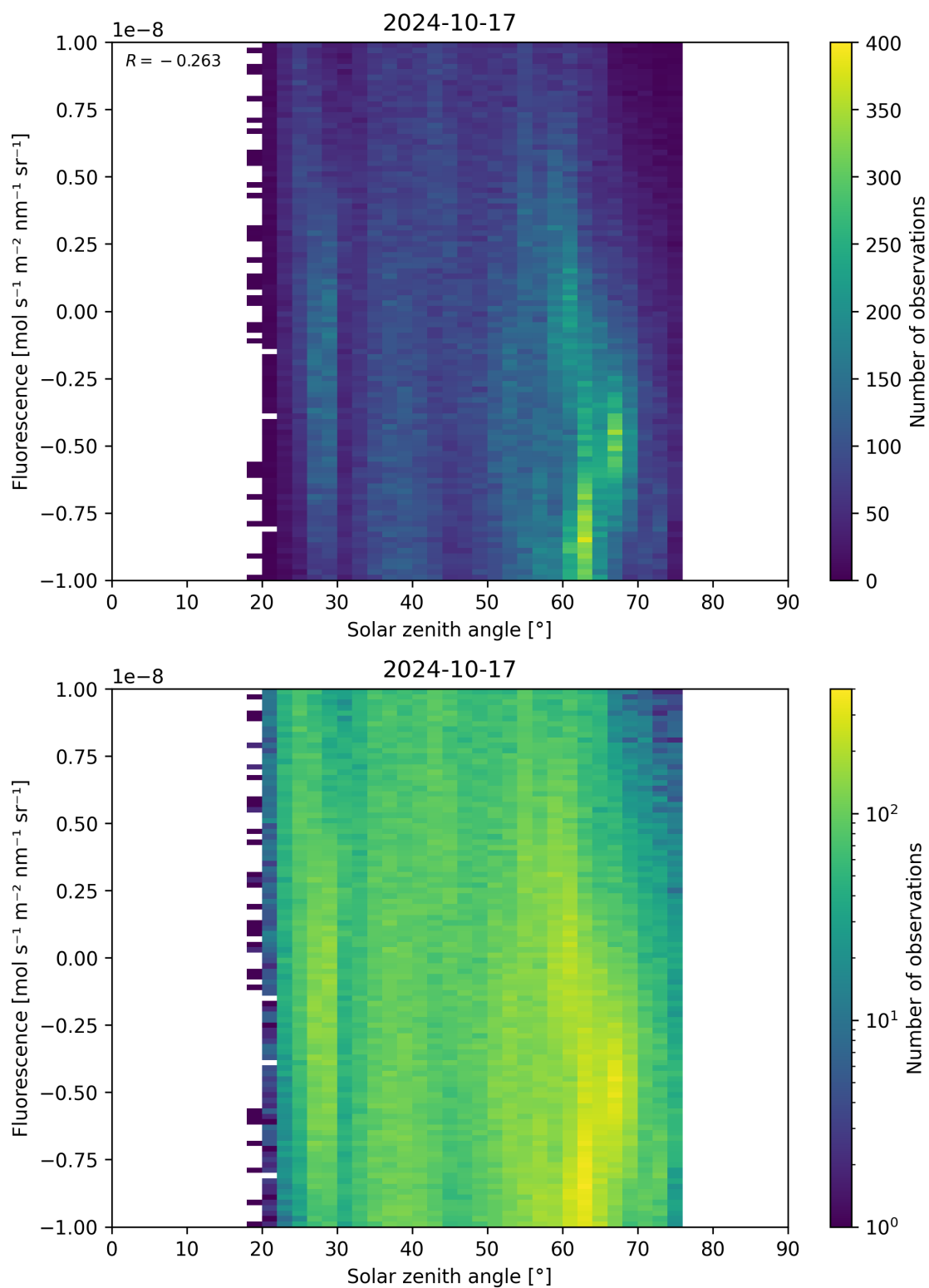
Figure 97: Scatter density plot of “Solar zenith angle” against “Fluorescence” for 2024-10-16 to 2024-10-18.
