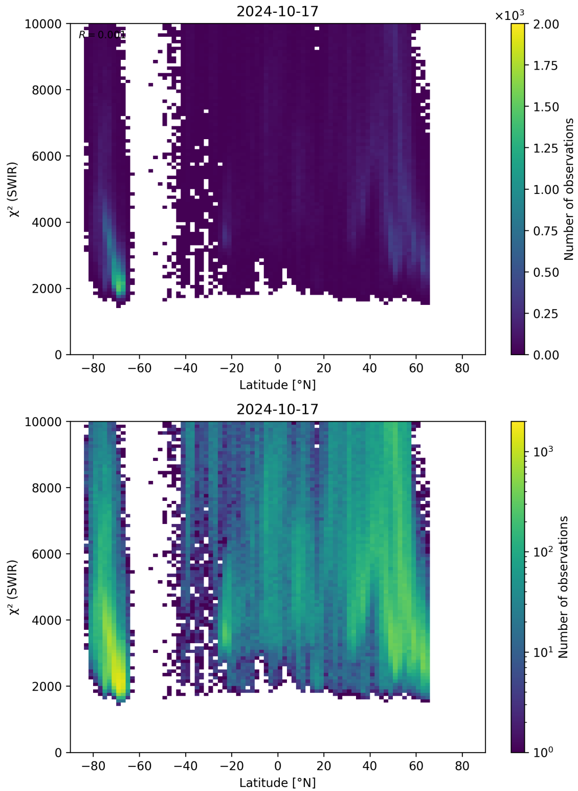
Figure 54: Scatter density plot of “Latitude” against “ \chi^2 (SWIR)” for 2024-10-16 to 2024-10-18.
