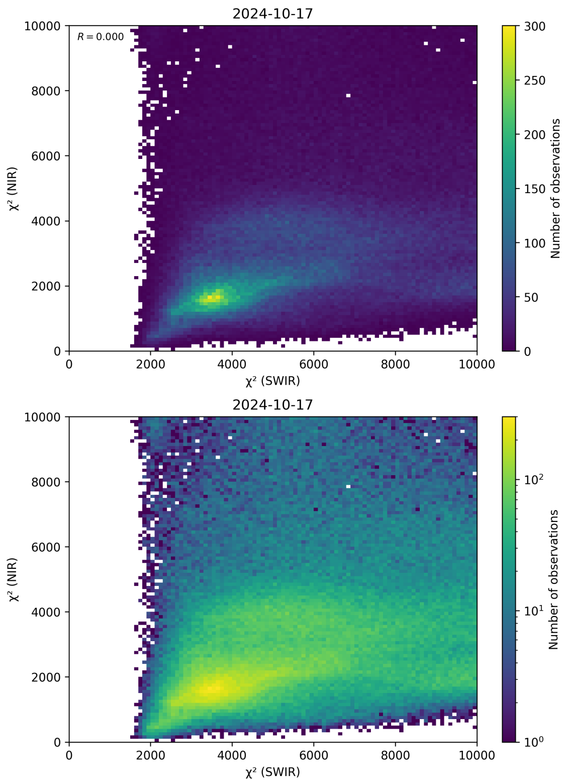
Figure 47: Scatter density plot of “ \chi^2 (SWIR)” against “ \chi^2 (NIR)” for 2024-10-16 to 2024-10-18.
