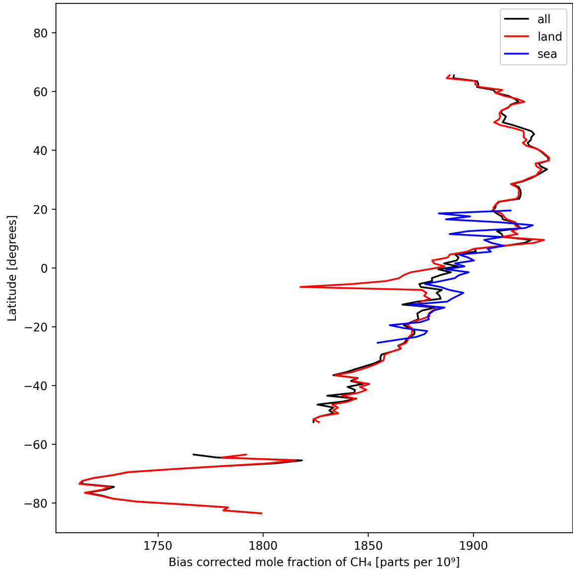
Figure 14: Zonal average of “Bias corrected mole fraction of CH 4 ” for 2024-10-16 to 2024-10-18.
