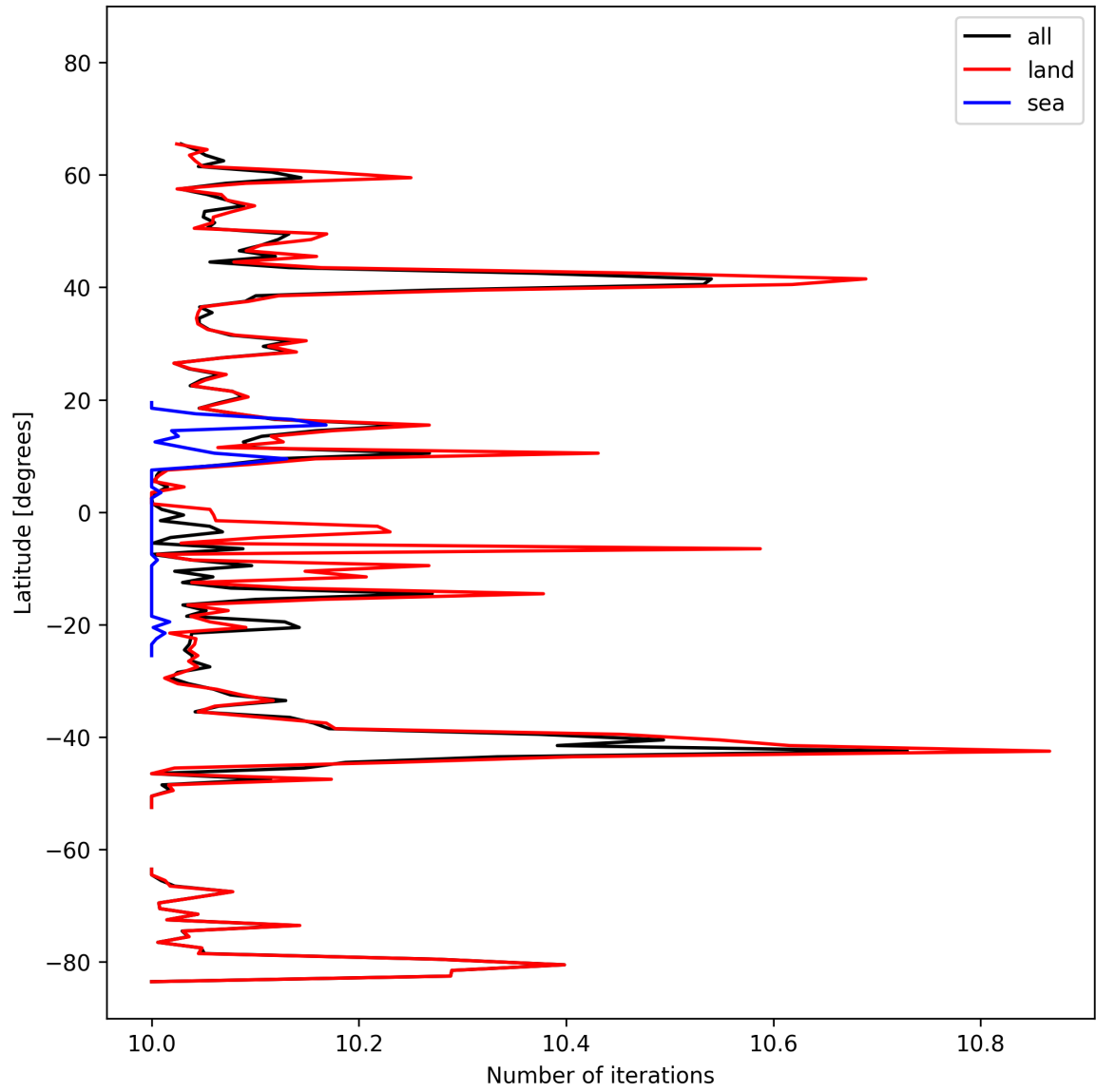
Figure 20: Zonal average of “Number of iterations” for 2024-10-16 to 2024-10-18.
