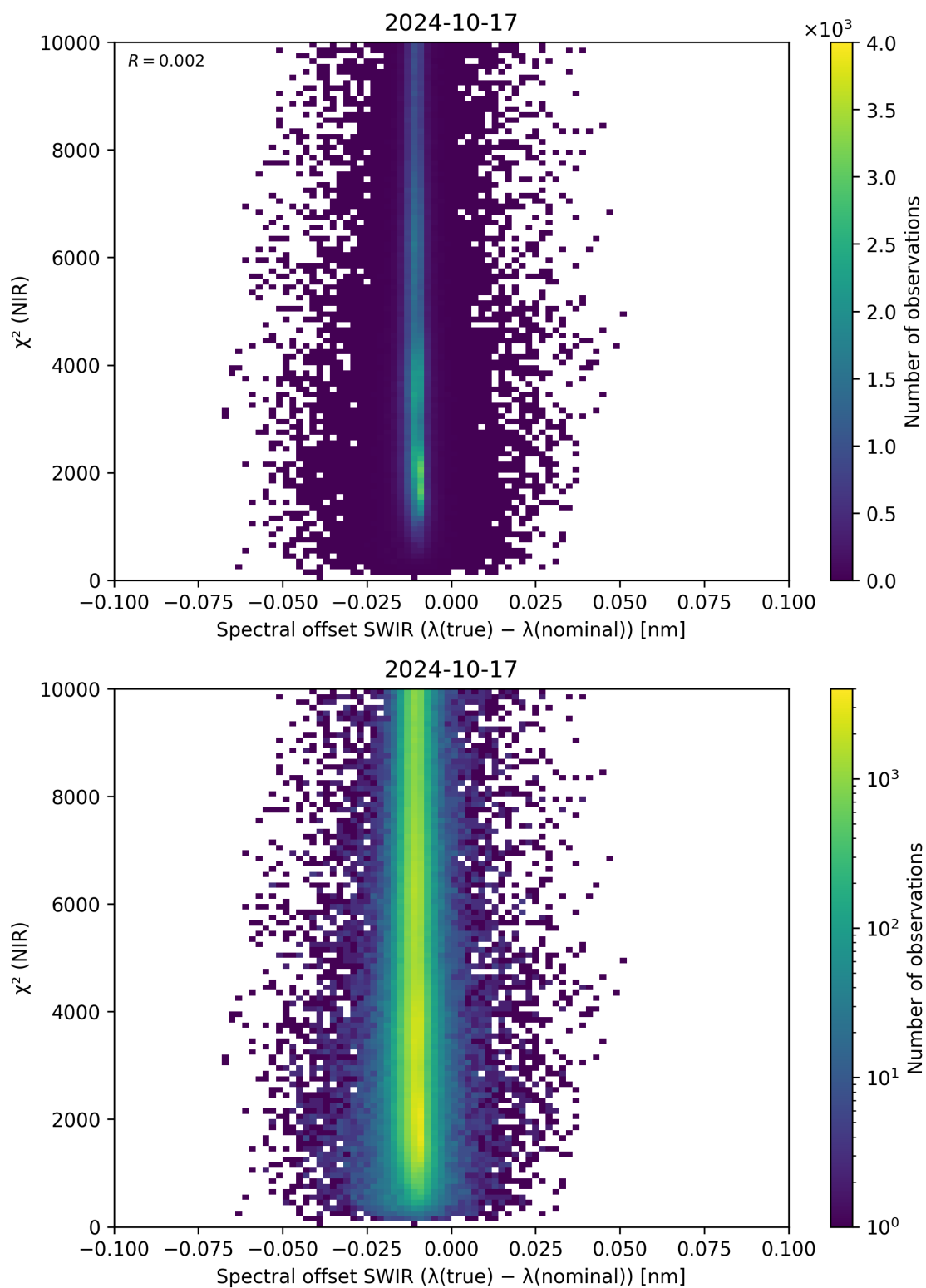
Figure 117: Scatter density plot of “Spectral offset SWIR ( \lambda_{\text{true}} - \lambda_{\text{nominal}} )” against “ \chi^2 (NIR)” for 2024-10-16 to 2024-10-18.
