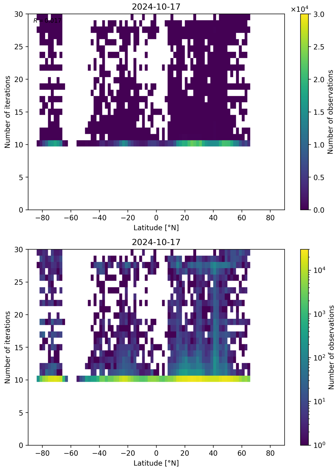
Figure 60: Scatter density plot of “Latitude” against “Number of iterations” for 2024-10-16 to 2024-10-18.
