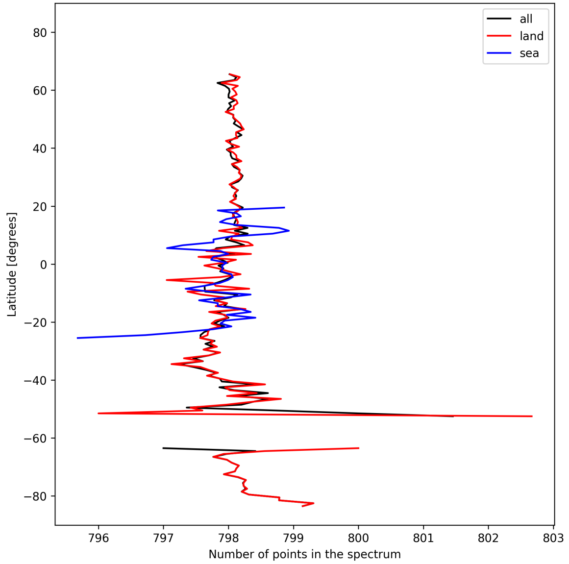
Figure 15: Zonal average of “Number of points in the spectrum” for 2024-10-16 to 2024-10-18.
