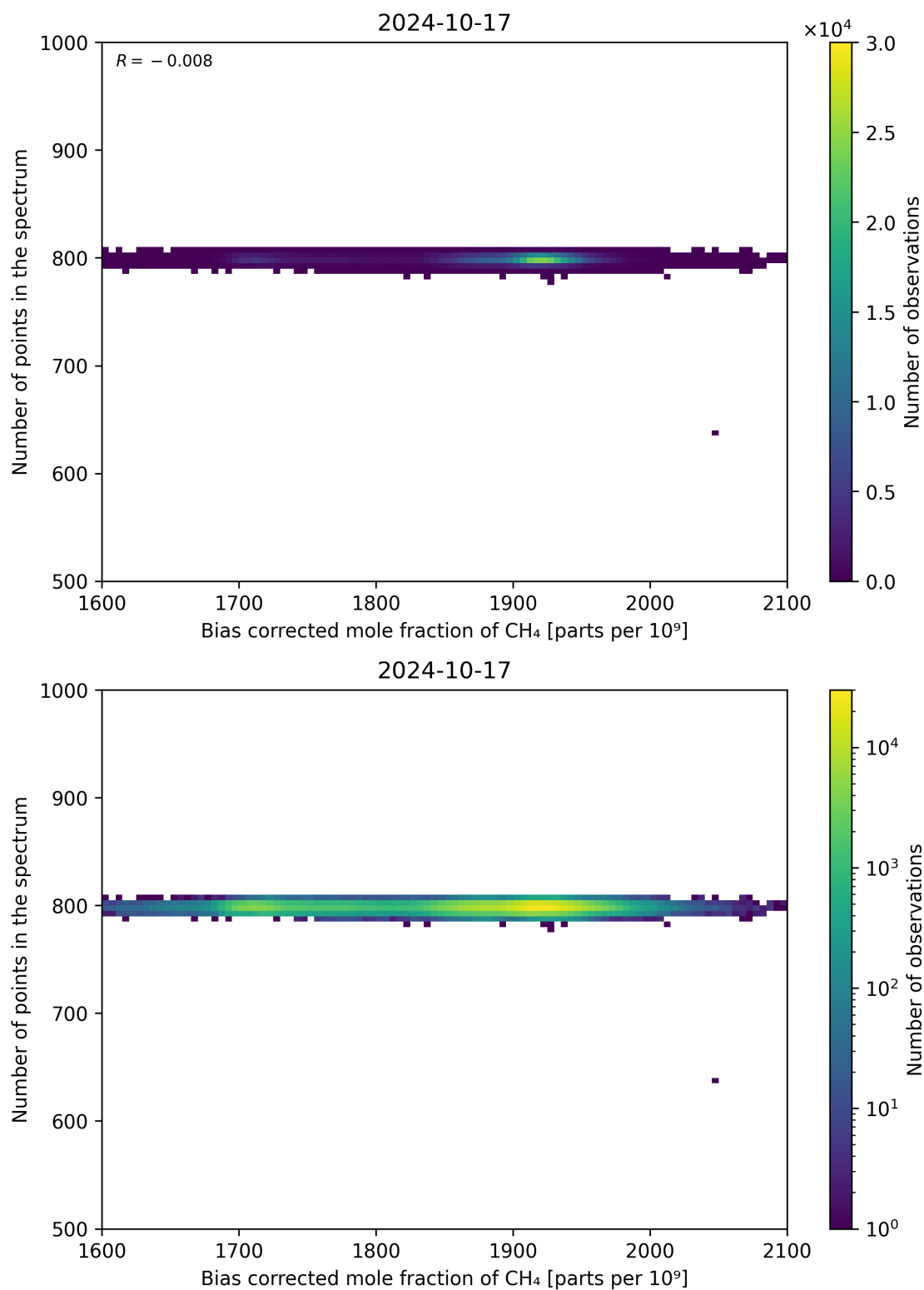
Figure 68: Scatter density plot of “Bias corrected mole fraction of CH 4 ” against “Number of points in the spectrum” for 2024-10-16 to 2024-10-18.
