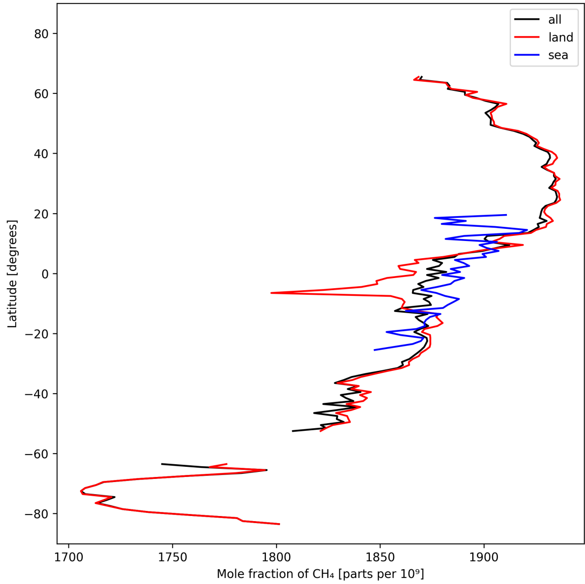
Figure 12: Zonal average of “Mole fraction of \text{CH}_4 ” for 2024-10-16 to 2024-10-18.
