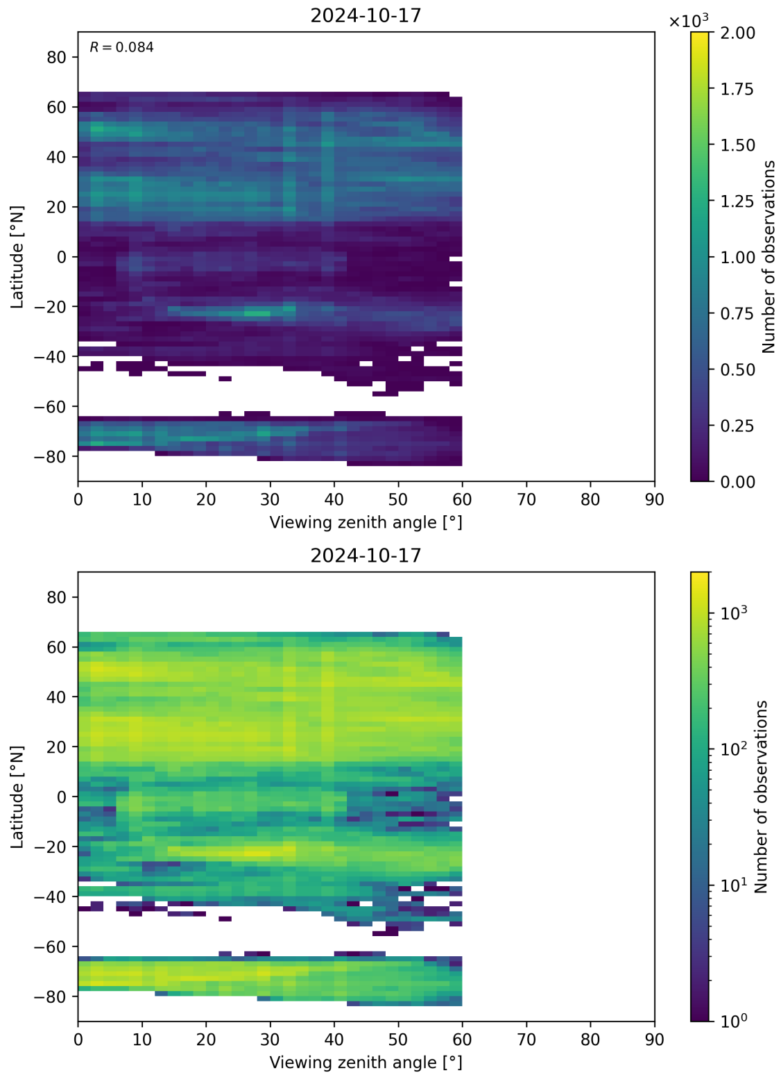
Figure 109: Scatter density plot of “Viewing zenith angle” against “Latitude” for 2024-10-16 to 2024-10-18.
