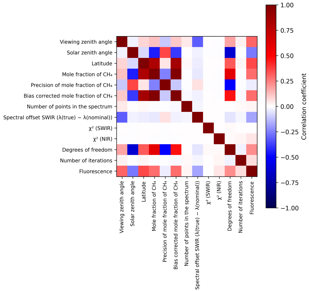
Figure 2: Map of correlation matrix for 2024-10-16 to 2024-10-18.
