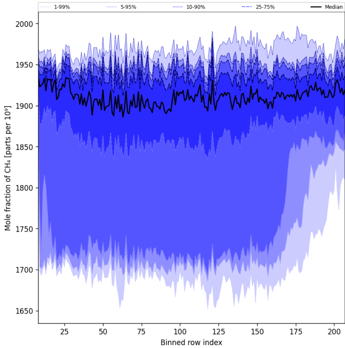
Figure 34: Along track statistics of “Mole fraction of CH 4 ” for 2024-10-16 to 2024-10-18
