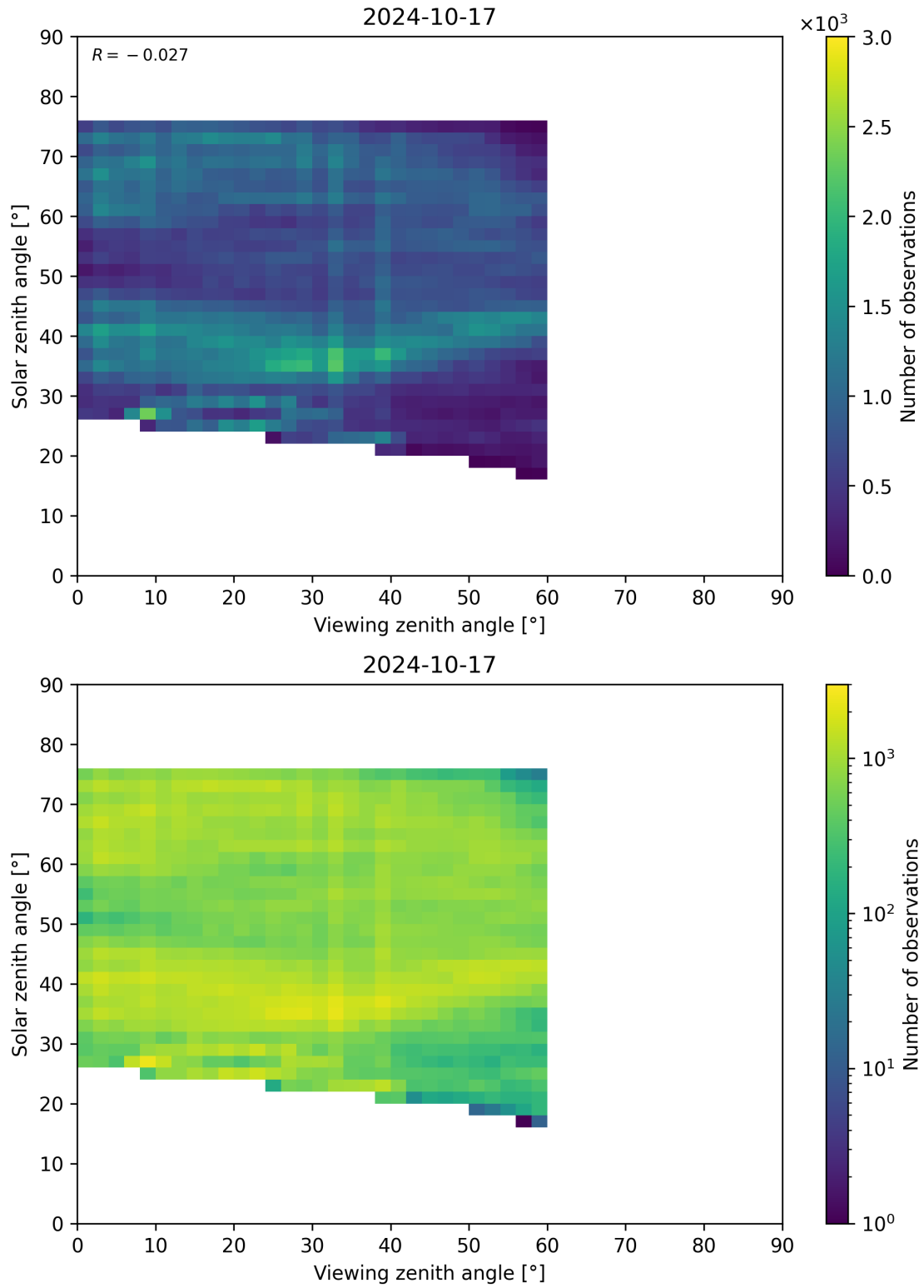
Figure 115: Scatter density plot of “Viewing zenith angle” against “Solar zenith angle” for 2024-10-16 to 2024-10-18.
