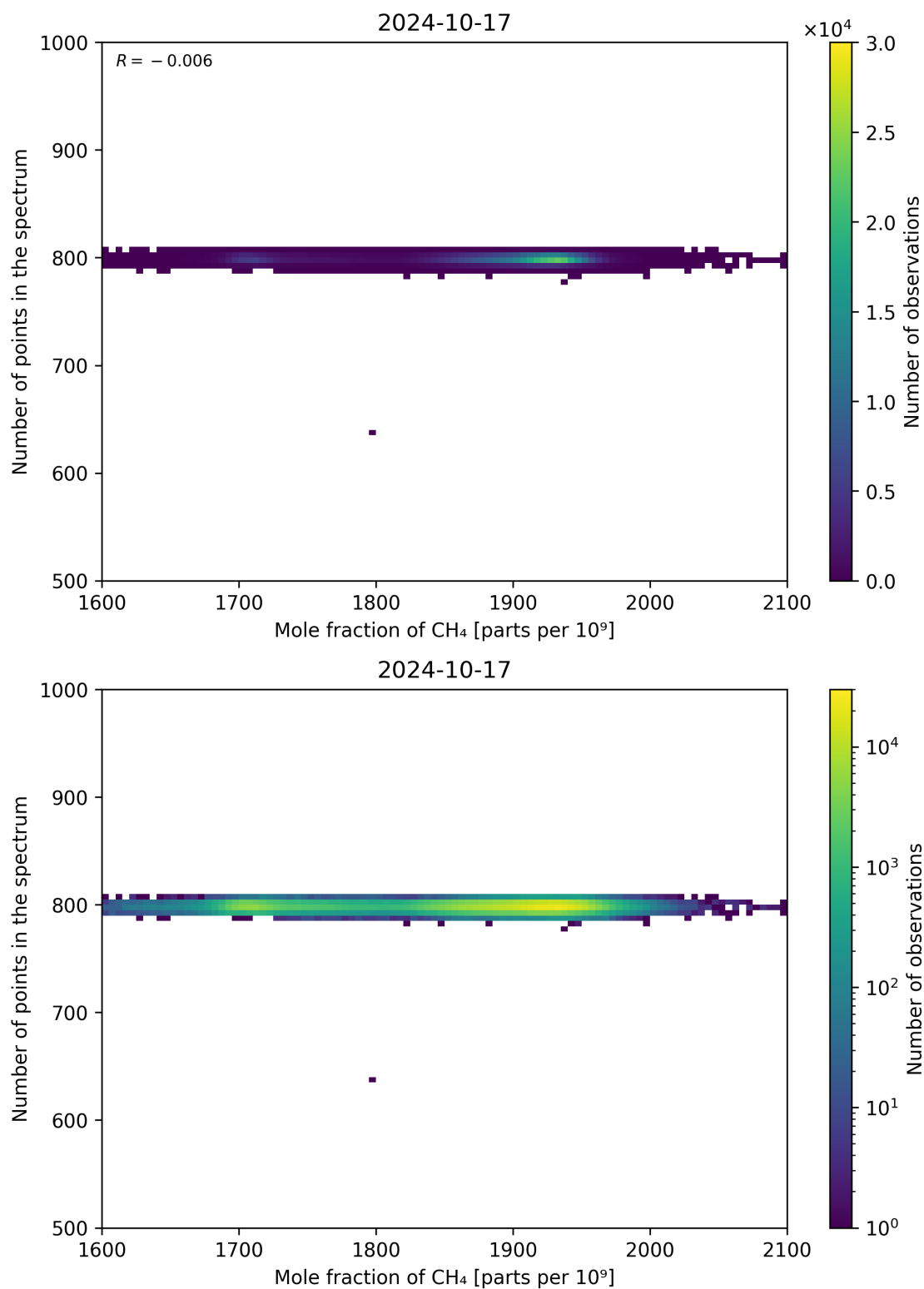
Figure 77: Scatter density plot of “Mole fraction of CH 4 ” against “Number of points in the spectrum” for 2024-10-16 to 2024-10-18.
