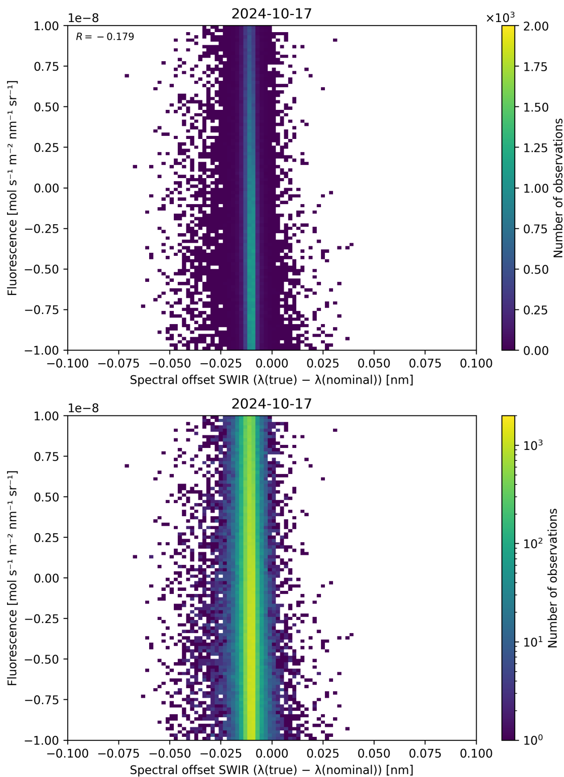
Figure 120: Scatter density plot of “Spectral offset SWIR ( \lambda_{\text{true}} - \lambda_{\text{nominal}} )” against “Fluorescence” for 2024-10-16 to 2024-10-18.
