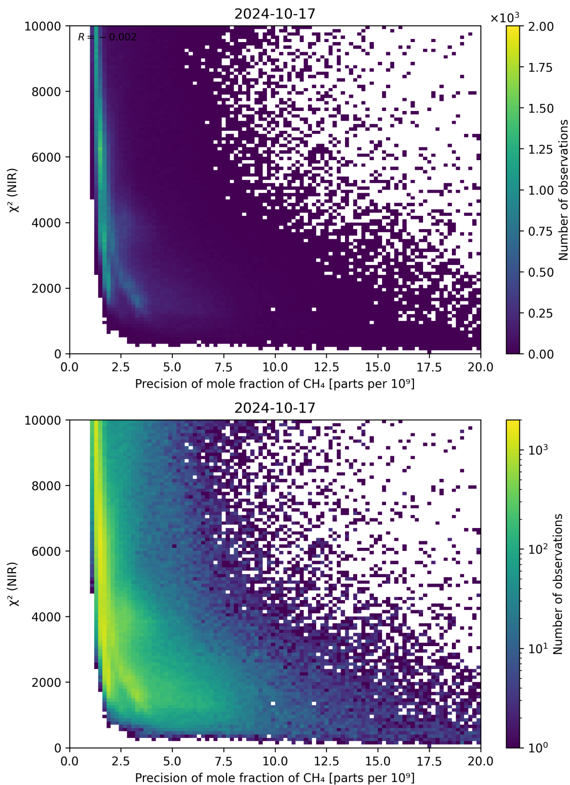
Figure 78: Scatter density plot of “Precision of mole fraction of CH 4 ” against “ \chi^2 (NIR)” for 2024-10-16 to 2024-10-18.
