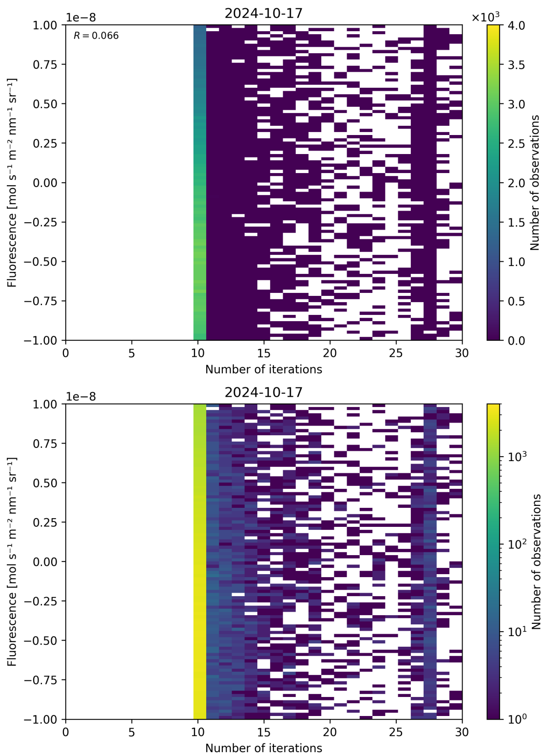
Figure 87: Scatter density plot of “Number of iterations” against “Fluorescence” for 2024-10-16 to 2024-10-18.
