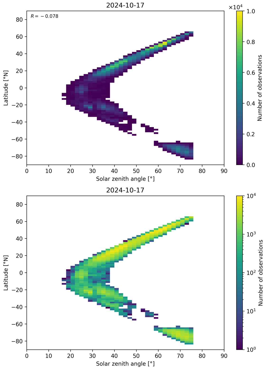
Figure 98: Scatter density plot of “Solar zenith angle” against “Latitude” for 2024-10-16 to 2024-10-18.
