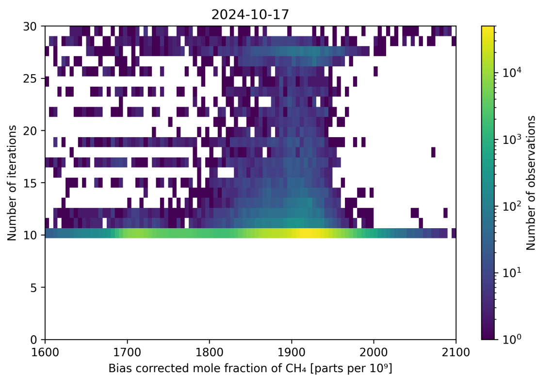
Figure 67: Scatter density plot of “Bias corrected mole fraction of CH 4 ” against “Number of iterations” for 2024-10-16 to 2024-10-18.
