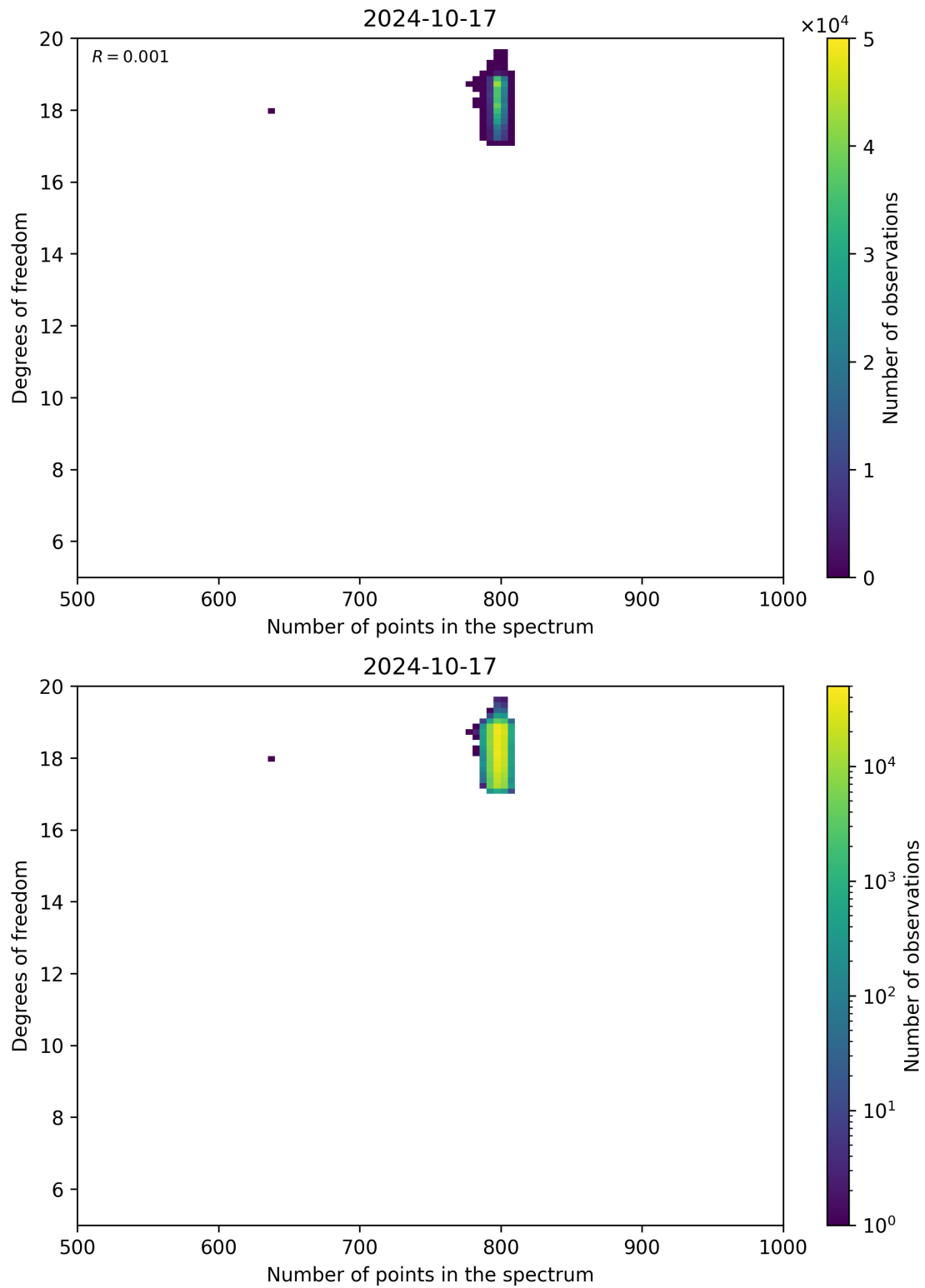
Figure 90: Scatter density plot of “Number of points in the spectrum” against “Degrees of freedom” for 2024-10-16 to 2024-10-18.
