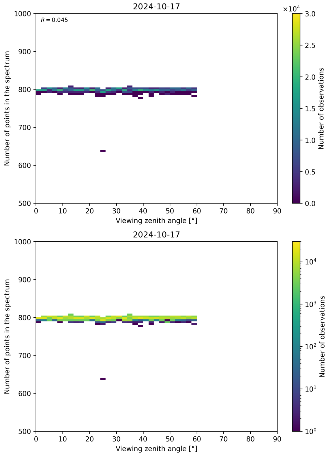
Figure 114: Scatter density plot of “Viewing zenith angle” against “Number of points in the spectrum” for 2024-10-16 to 2024-10-18.
