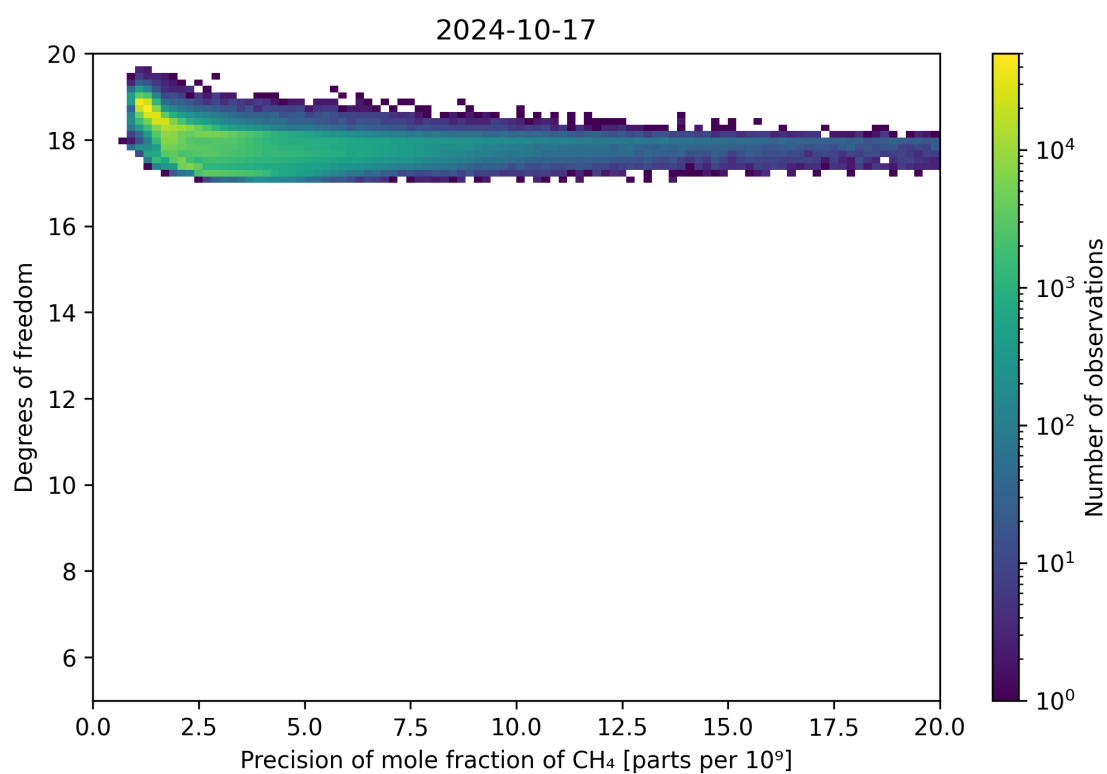
Figure 80: Scatter density plot of “Precision of mole fraction of CH 4 ” against “Degrees of freedom” for 2024-10-16 to 2024-10-18.
