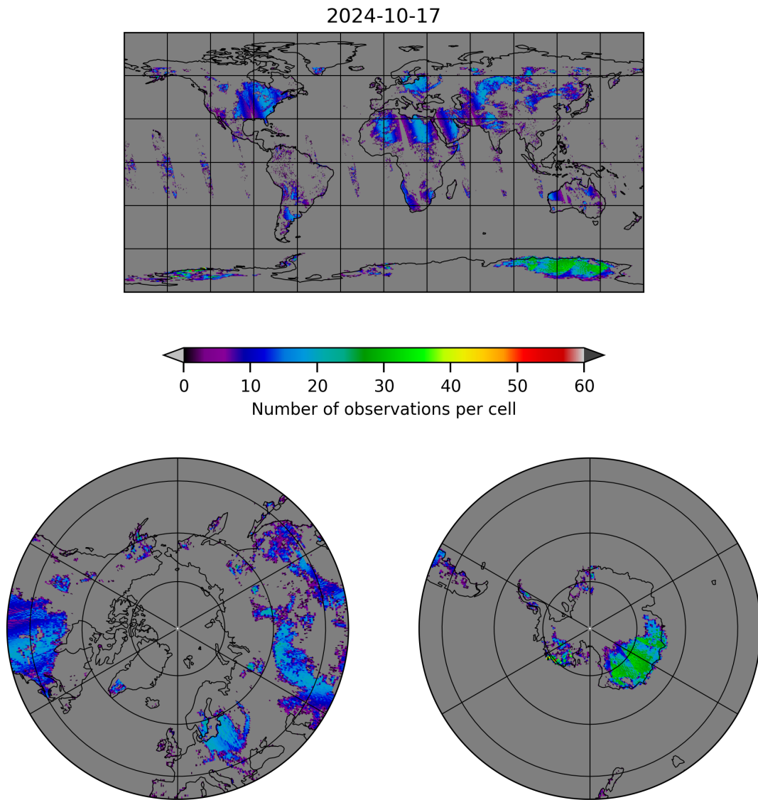
Figure 10: Map of the number of observations for 2024-10-16 to 2024-10-18
