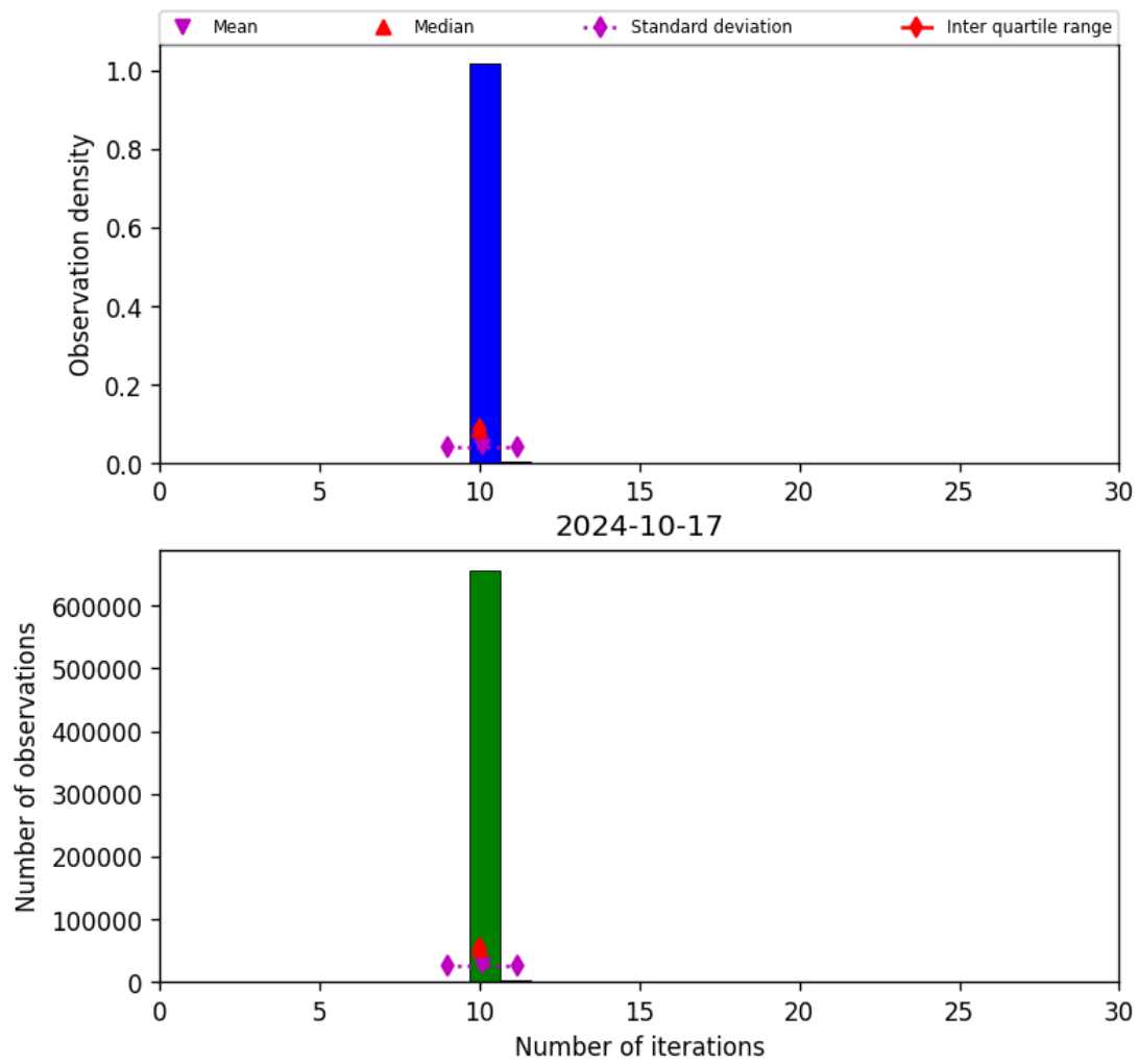
Figure 31: Histogram of “Number of iterations” for 2024-10-16 to 2024-10-18
