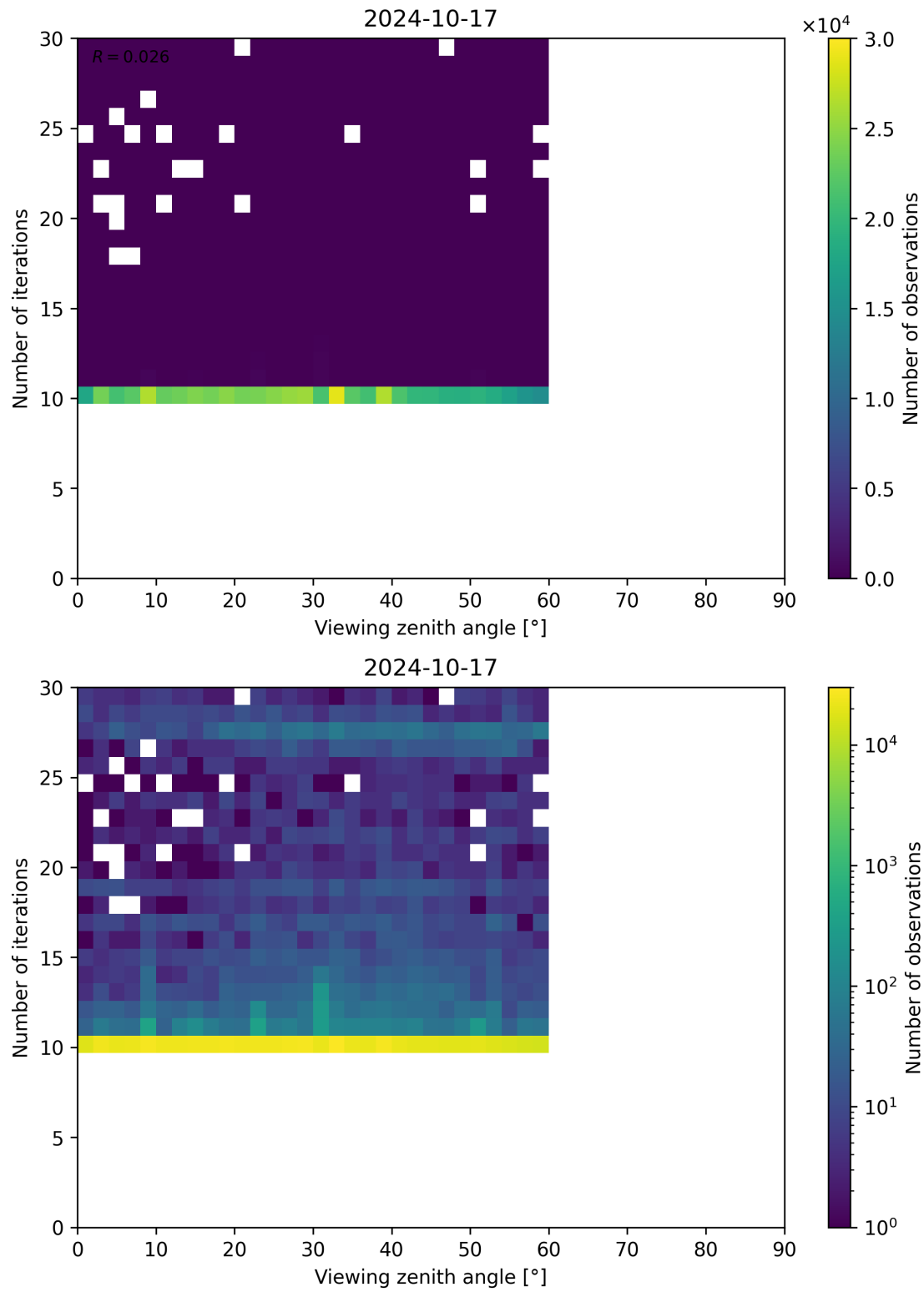
Figure 113: Scatter density plot of “Viewing zenith angle” against “Number of iterations” for 2024-10-16 to 2024-10-18.
