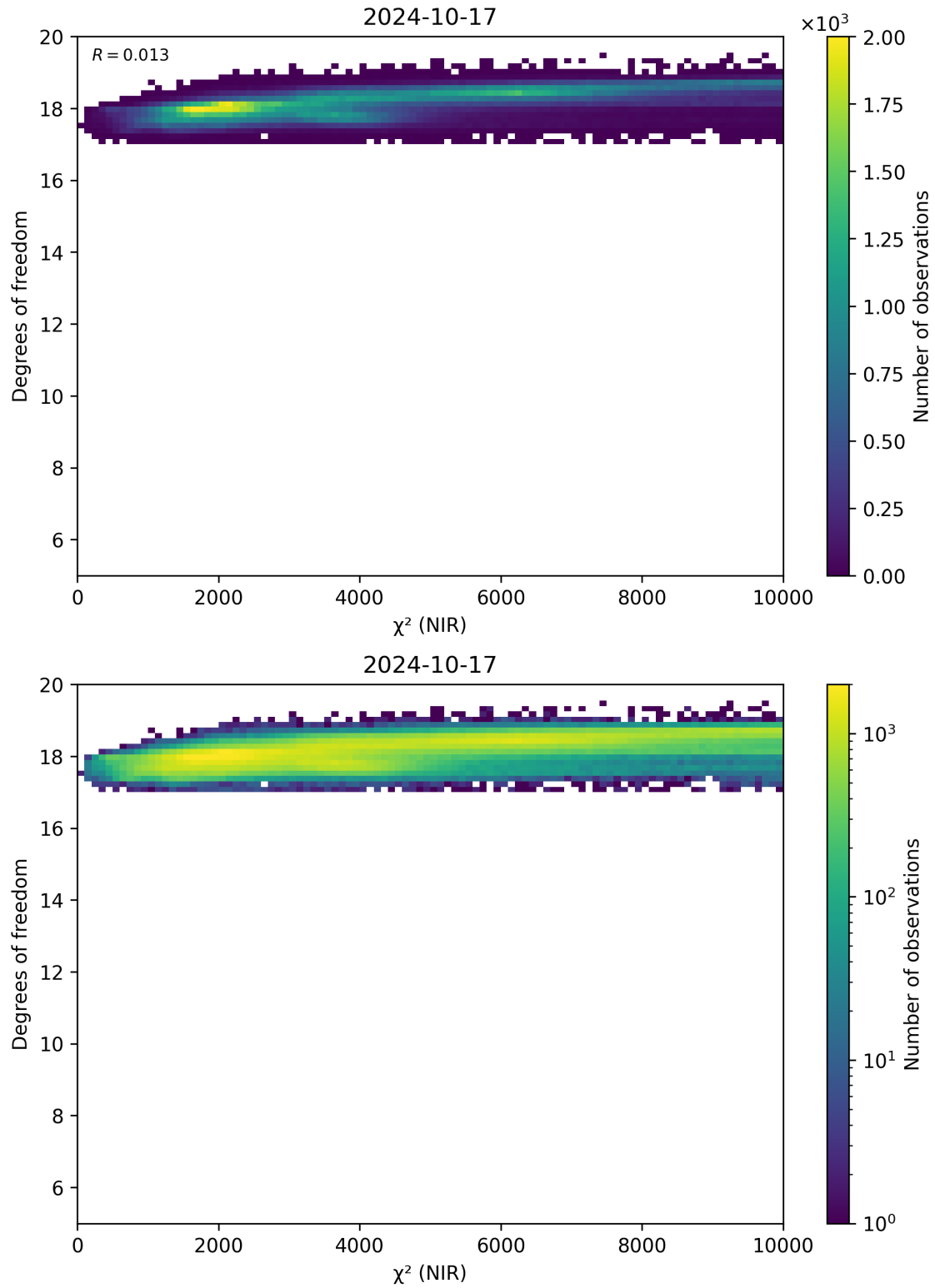
Figure 44: Scatter density plot of “ \chi^2 (NIR)” against “Degrees of freedom” for 2024-10-16 to 2024-10-18.
