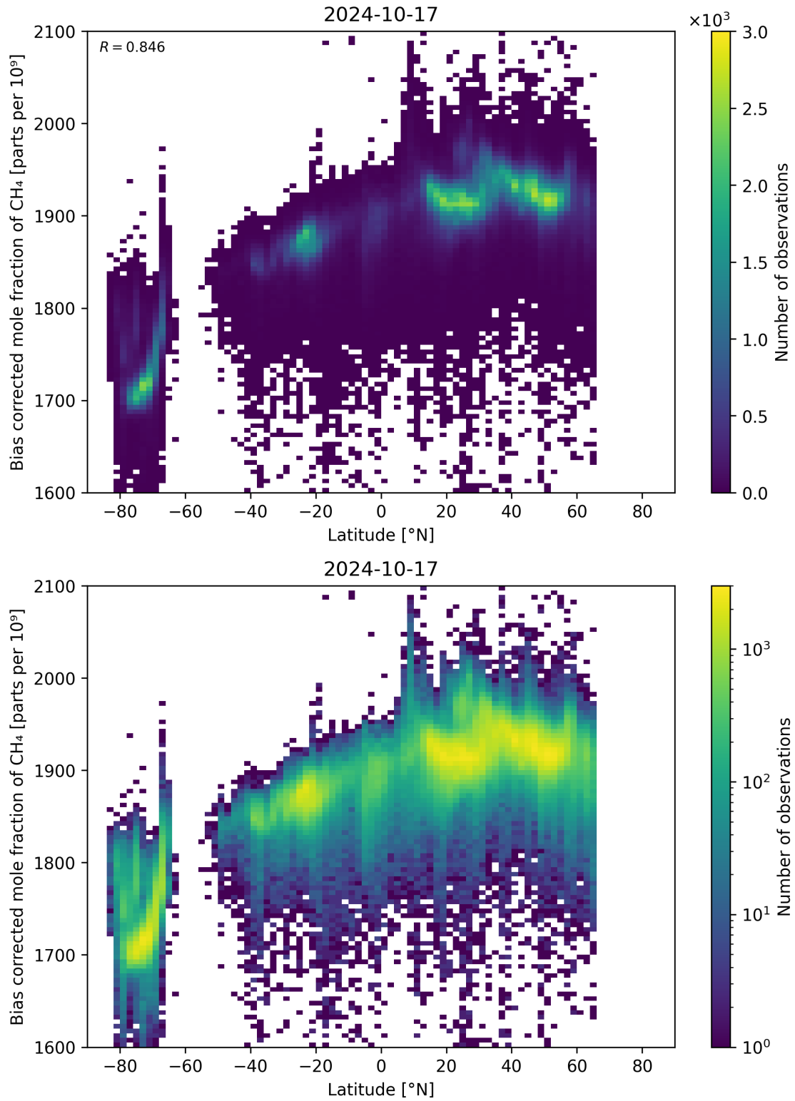
Figure 58: Scatter density plot of “Latitude” against “Bias corrected mole fraction of \text{CH}_4 ” for 2024-10-16 to 2024-10-18.
