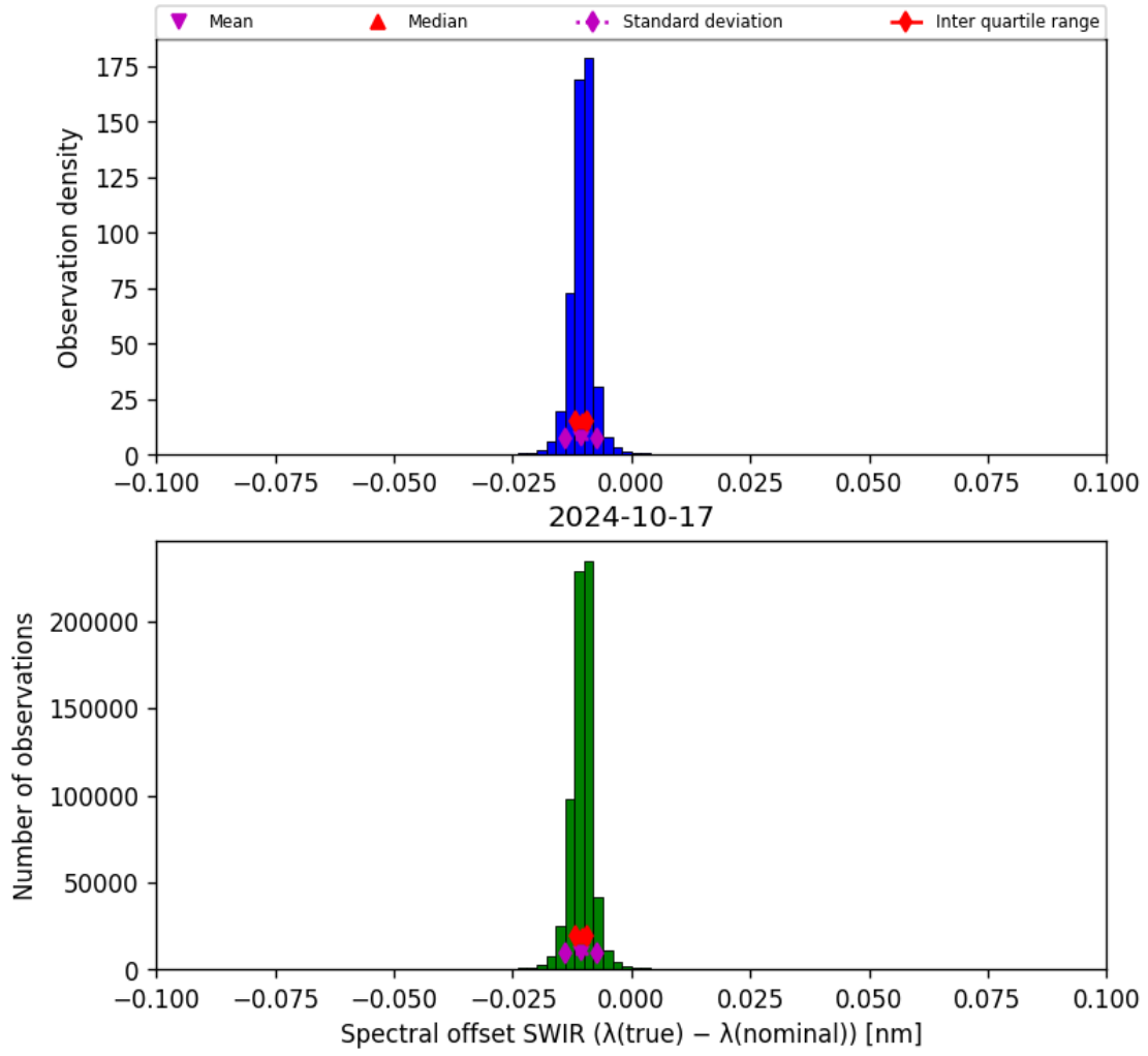
Figure 27: Histogram of “Spectral offset SWIR ( \lambda_{\text{true}} - \lambda_{\text{nominal}} )” for 2024-10-16 to 2024-10-18
