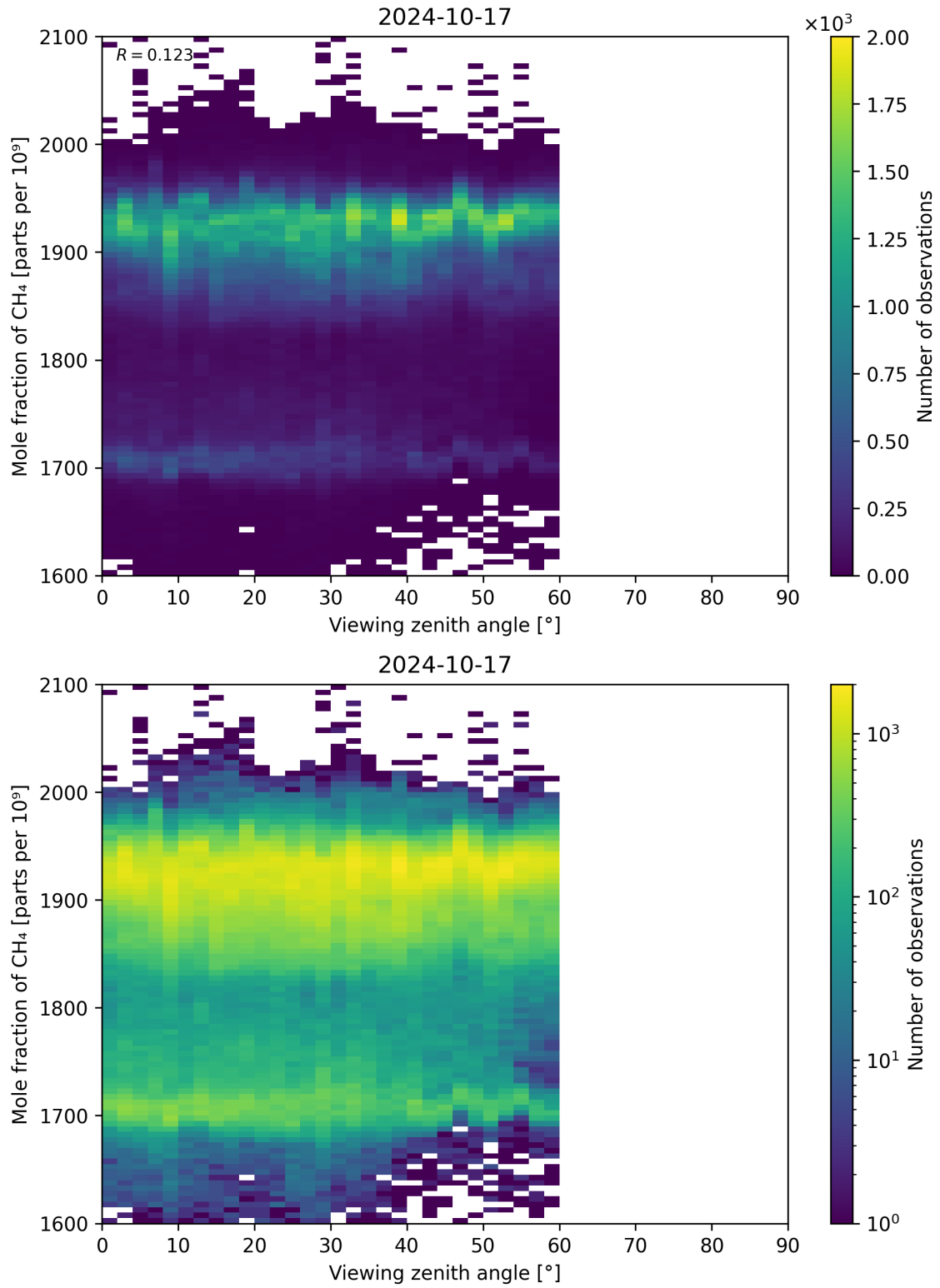
Figure 110: Scatter density plot of “Viewing zenith angle” against “Mole fraction of \text{CH}_4 ” for 2024-10-16 to 2024-10-18.
