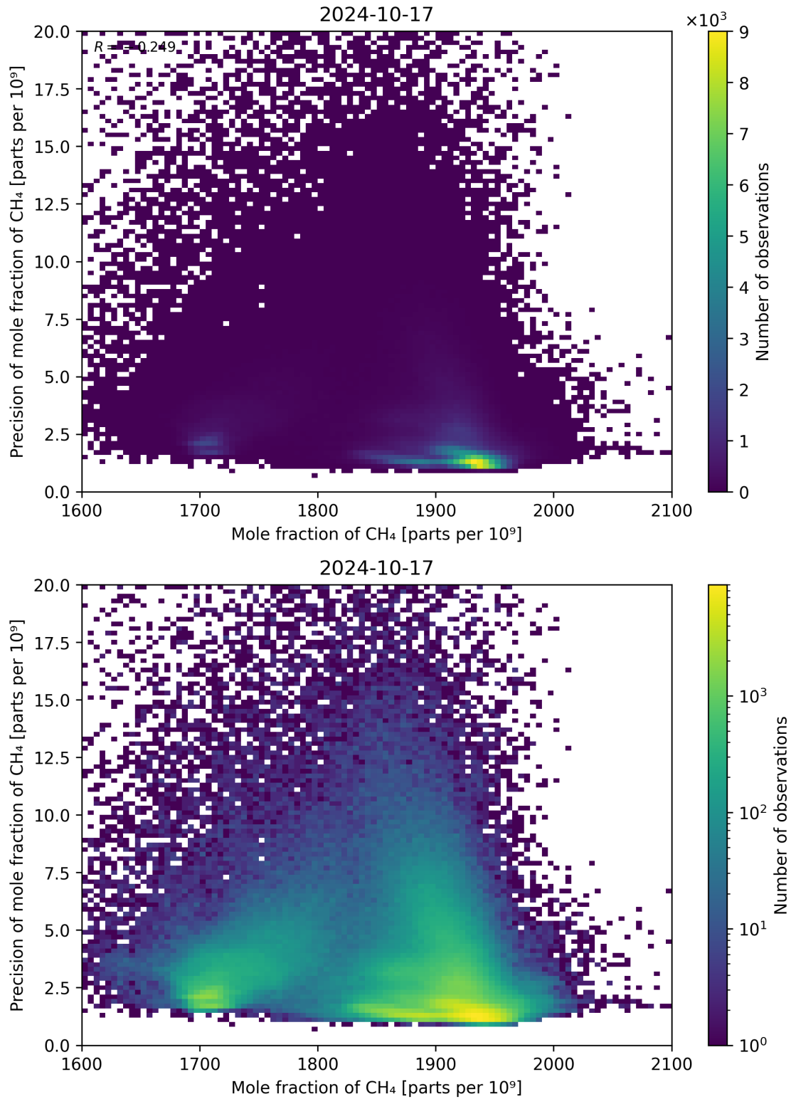
Figure 75: Scatter density plot of “Mole fraction of CH 4 ” against “Precision of mole fraction of CH 4 ” for 2024-10-16 to 2024-10-18.
