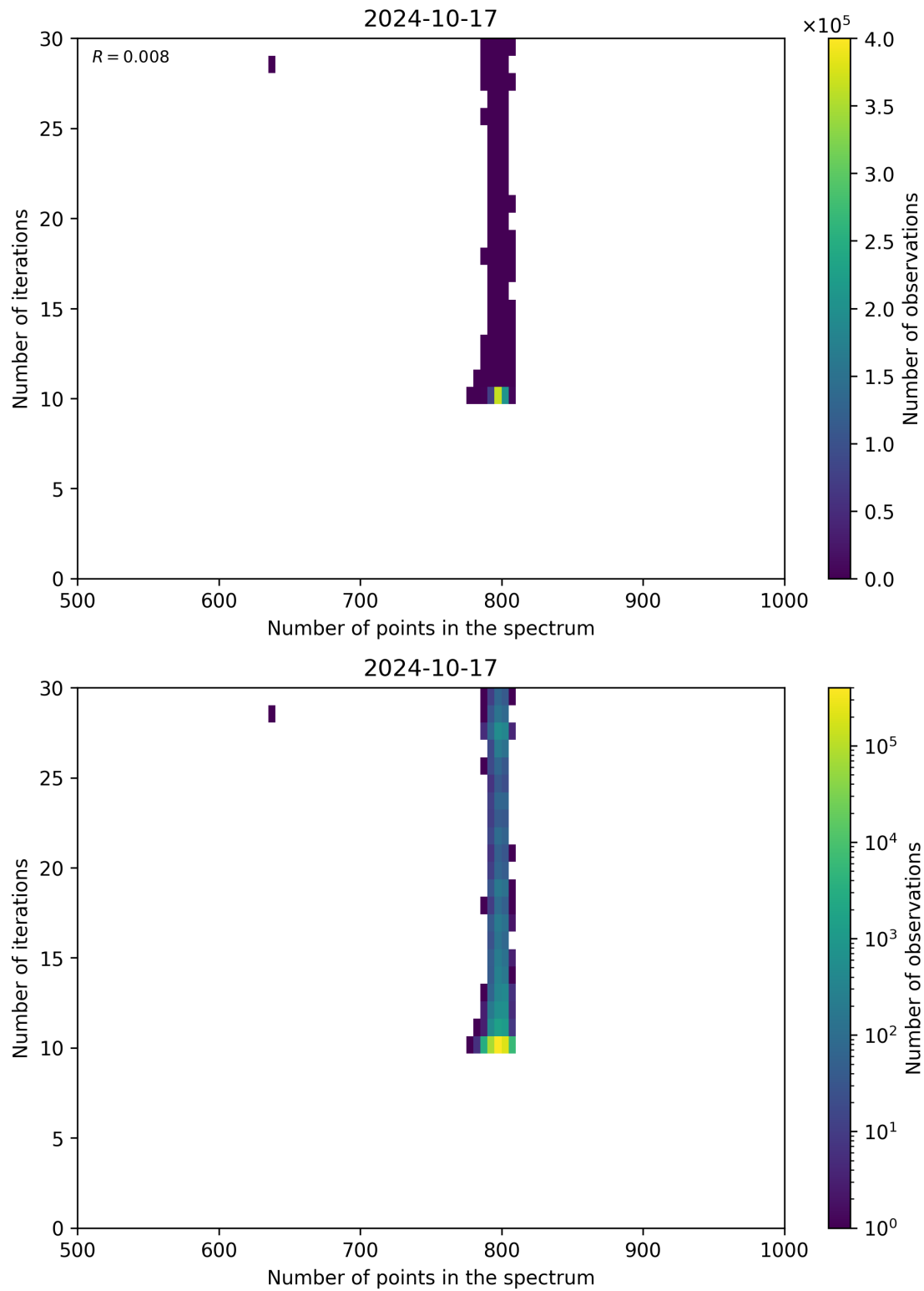
Figure 92: Scatter density plot of “Number of points in the spectrum” against “Number of iterations” for 2024-10-16 to 2024-10-18.
