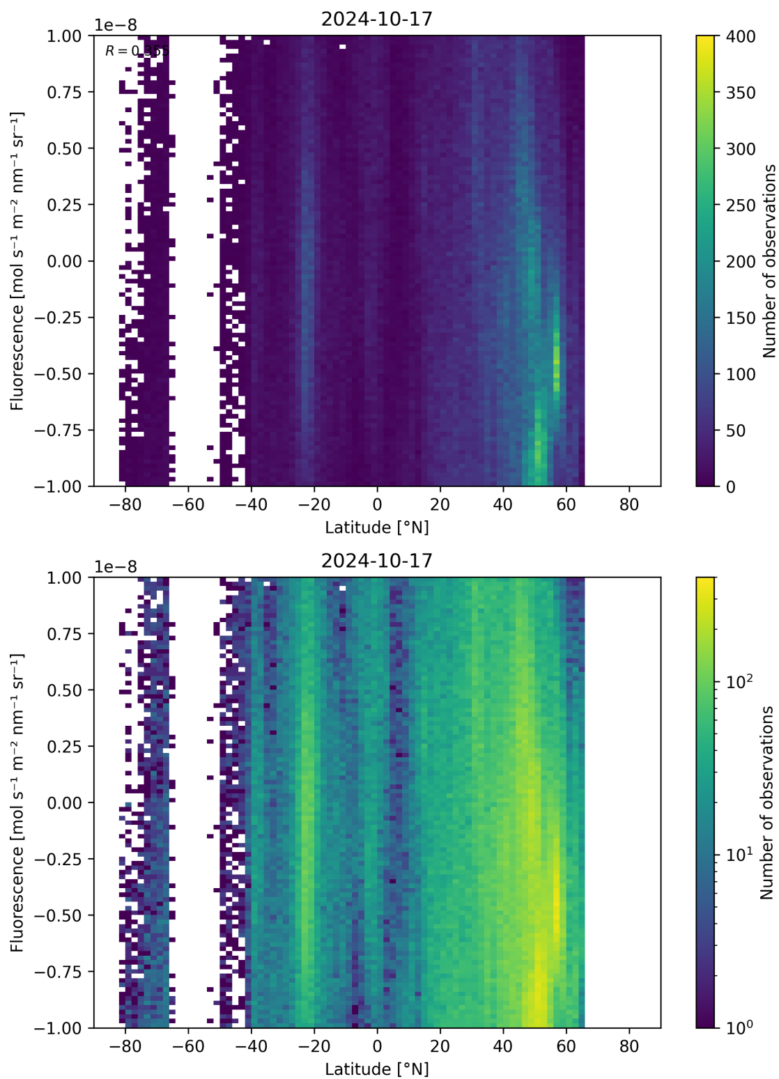
Figure 56: Scatter density plot of “Latitude” against “Fluorescence” for 2024-10-16 to 2024-10-18.
