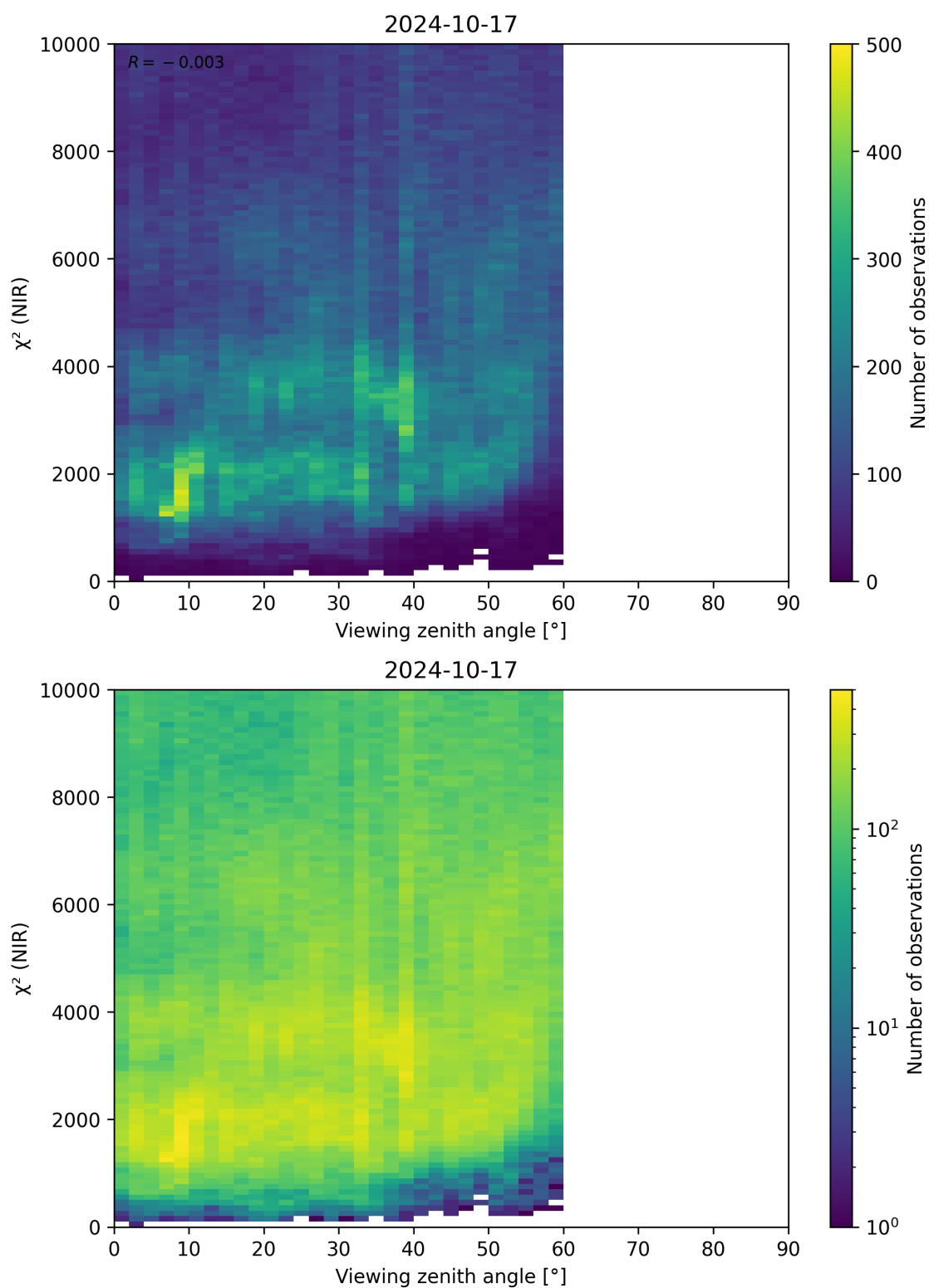
Figure 105: Scatter density plot of “Viewing zenith angle” against “ \chi^2 (NIR)” for 2024-10-16 to 2024-10-18.
