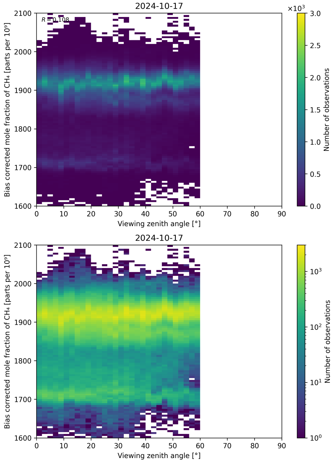
Figure 111: Scatter density plot of “Viewing zenith angle” against “Bias corrected mole fraction of CH 4 ” for 2024-10-16 to 2024-10-18.
