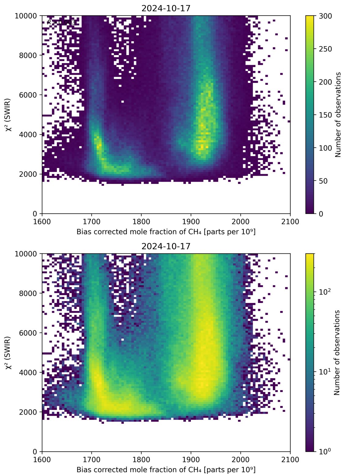
Figure 64: Scatter density plot of “Bias corrected mole fraction of \text{CH}_4 ” against “ \chi^2 (SWIR)” for 2024-10-16 to 2024-10-18.
