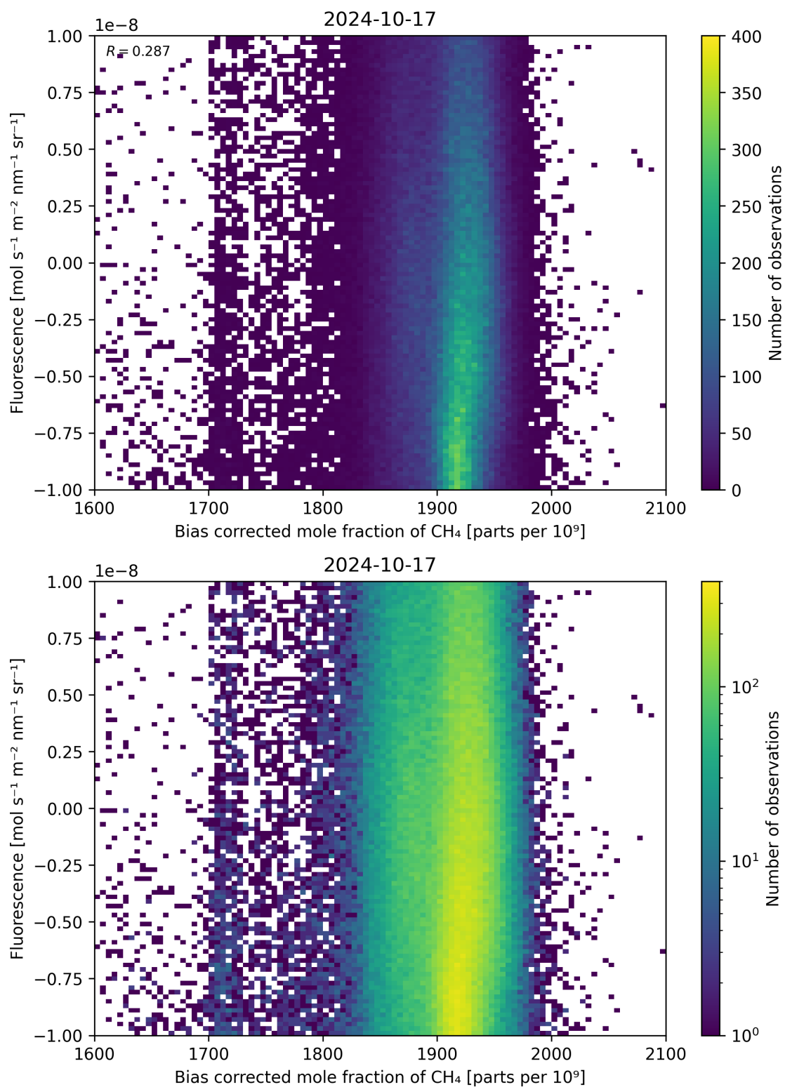
Figure 66: Scatter density plot of “Bias corrected mole fraction of \text{CH}_4 ” against “Fluorescence” for 2024-10-16 to 2024-10-18.
