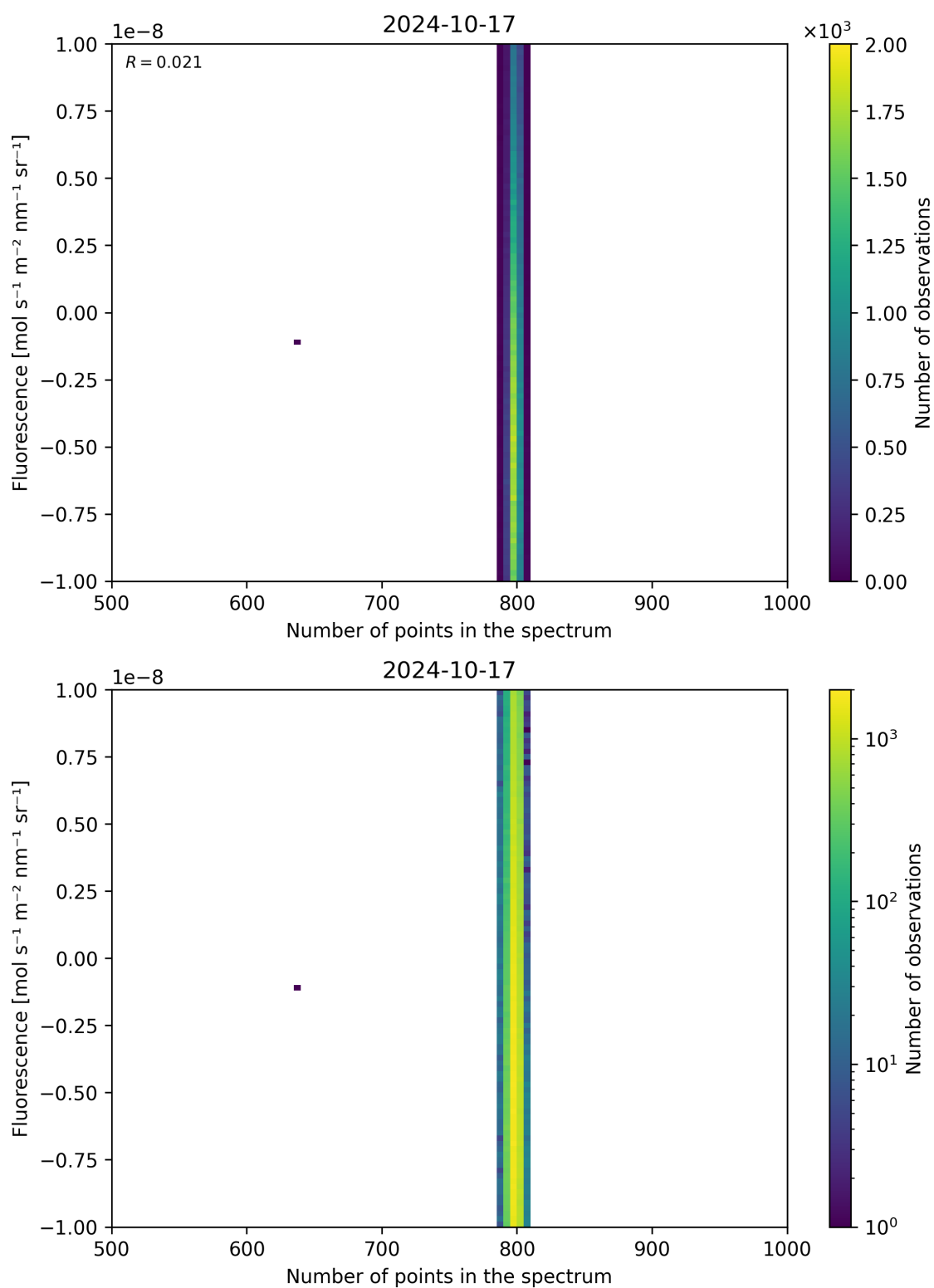
Figure 91: Scatter density plot of “Number of points in the spectrum” against “Fluorescence” for 2024-10-16 to 2024-10-18.
