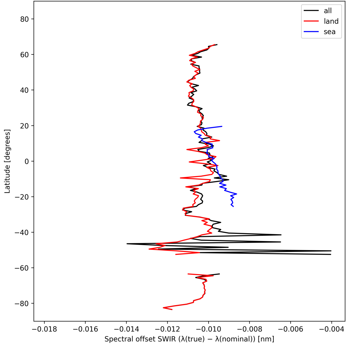
Figure 16: Zonal average of “Spectral offset SWIR ( \lambda_{\text{true}} - \lambda_{\text{nominal}} )” for 2024-10-16 to 2024-10-18.
