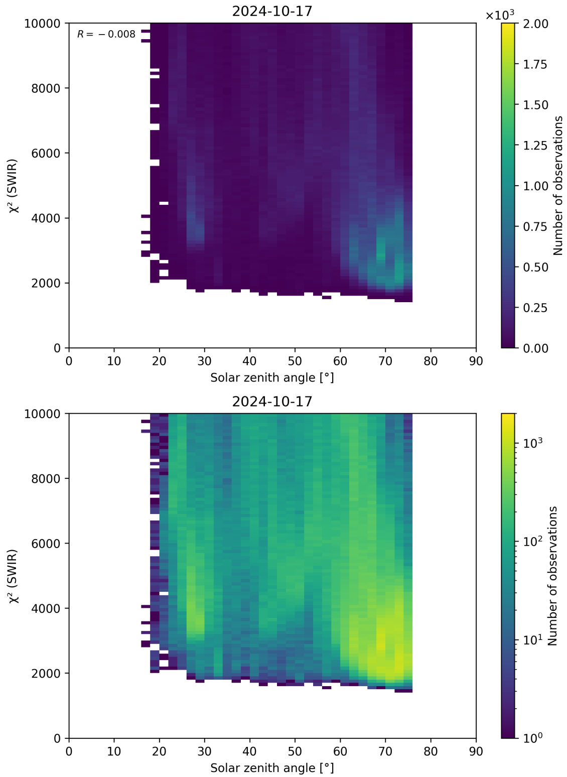
Figure 95: Scatter density plot of “Solar zenith angle” against “ \chi^2 (SWIR)” for 2024-10-16 to 2024-10-18.
