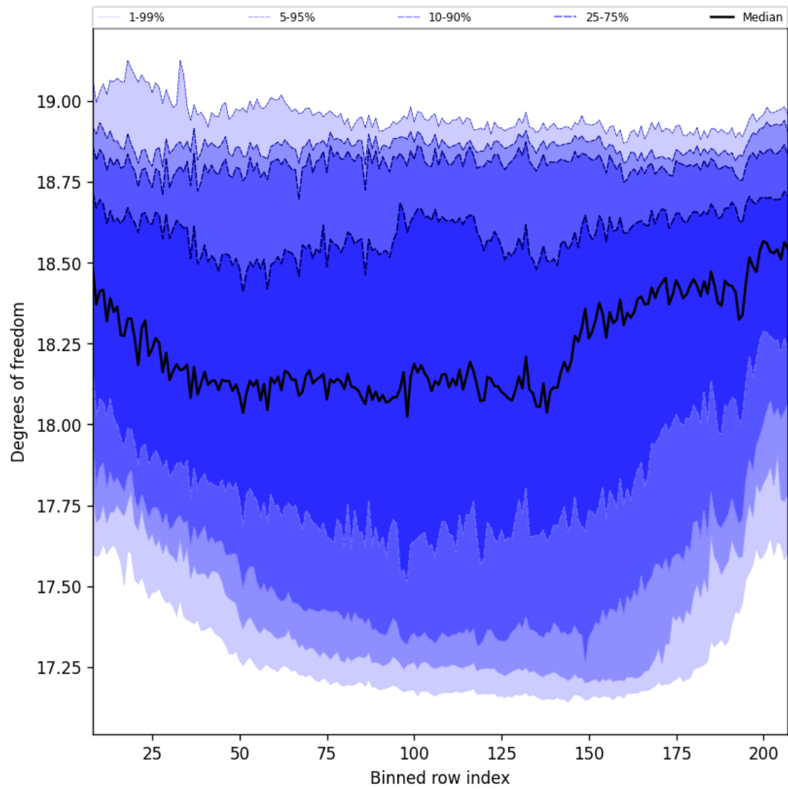
Figure 41: Along track statistics of “Degrees of freedom” for 2024-10-16 to 2024-10-18
