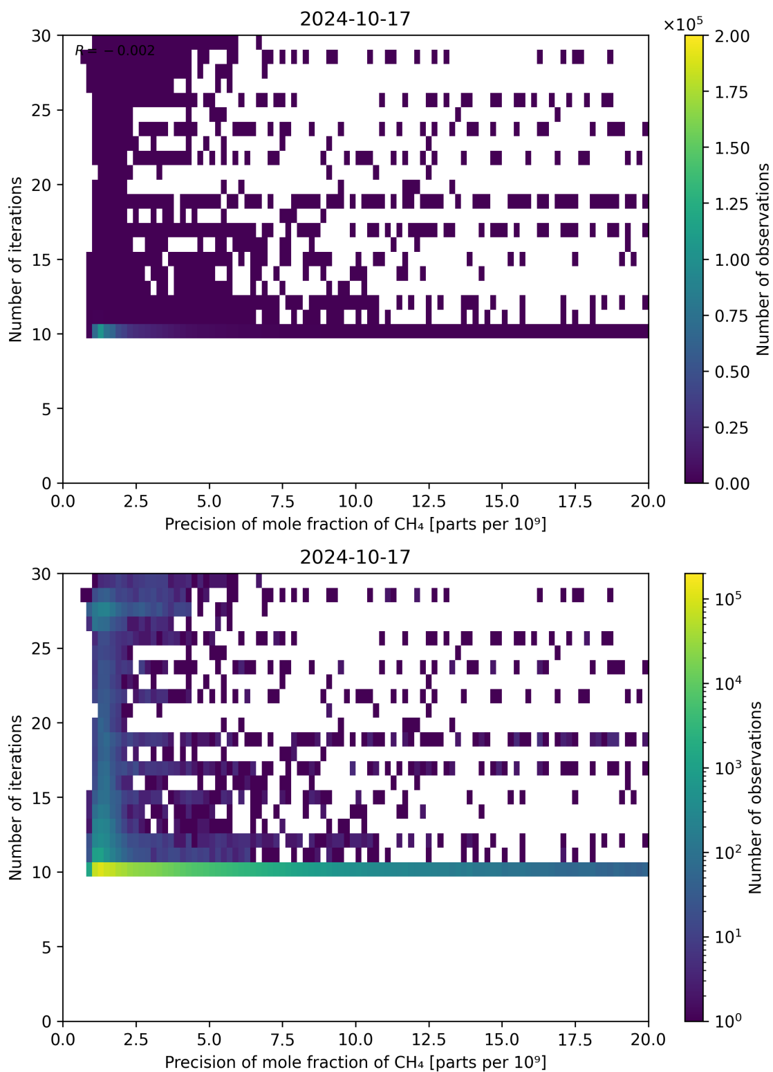
Figure 83: Scatter density plot of “Precision of mole fraction of CH 4 ” against “Number of iterations” for 2024-10-16 to 2024-10-18.
