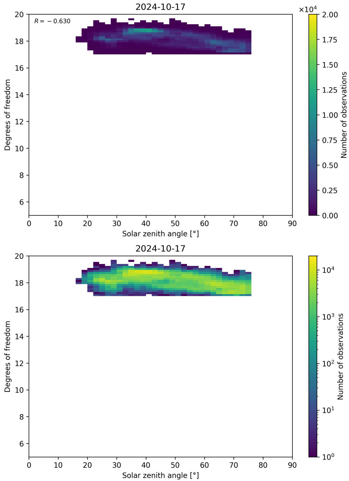
Figure 96: Scatter density plot of “Solar zenith angle” against “Degrees of freedom” for 2024-10-16 to 2024-10-18.
