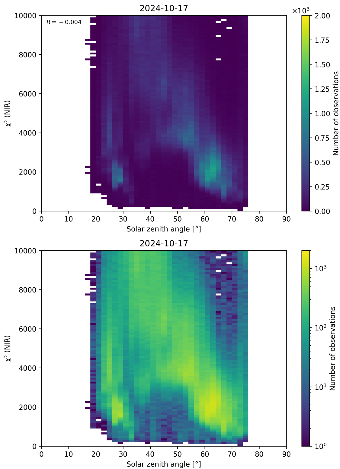
Figure 94: Scatter density plot of “Solar zenith angle” against “ \chi^2 (NIR)” for 2024-10-16 to 2024-10-18.
