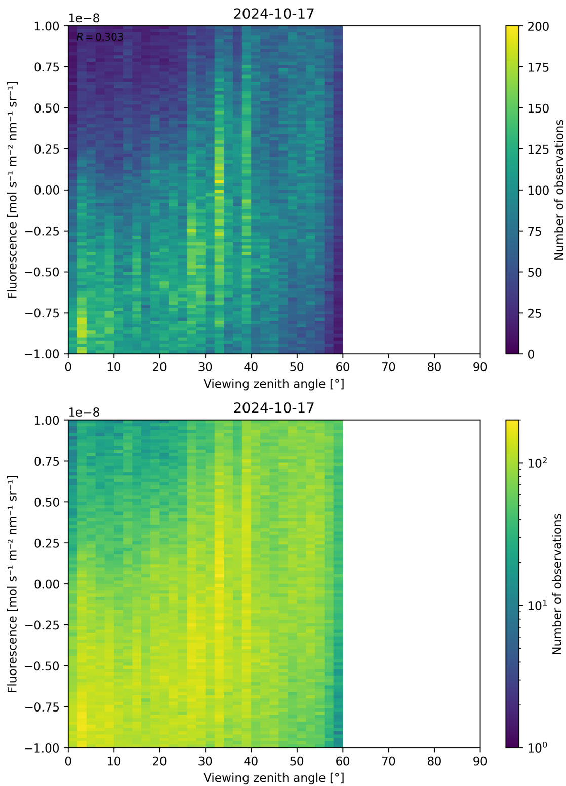
Figure 108: Scatter density plot of “Viewing zenith angle” against “Fluorescence” for 2024-10-16 to 2024-10-18.
