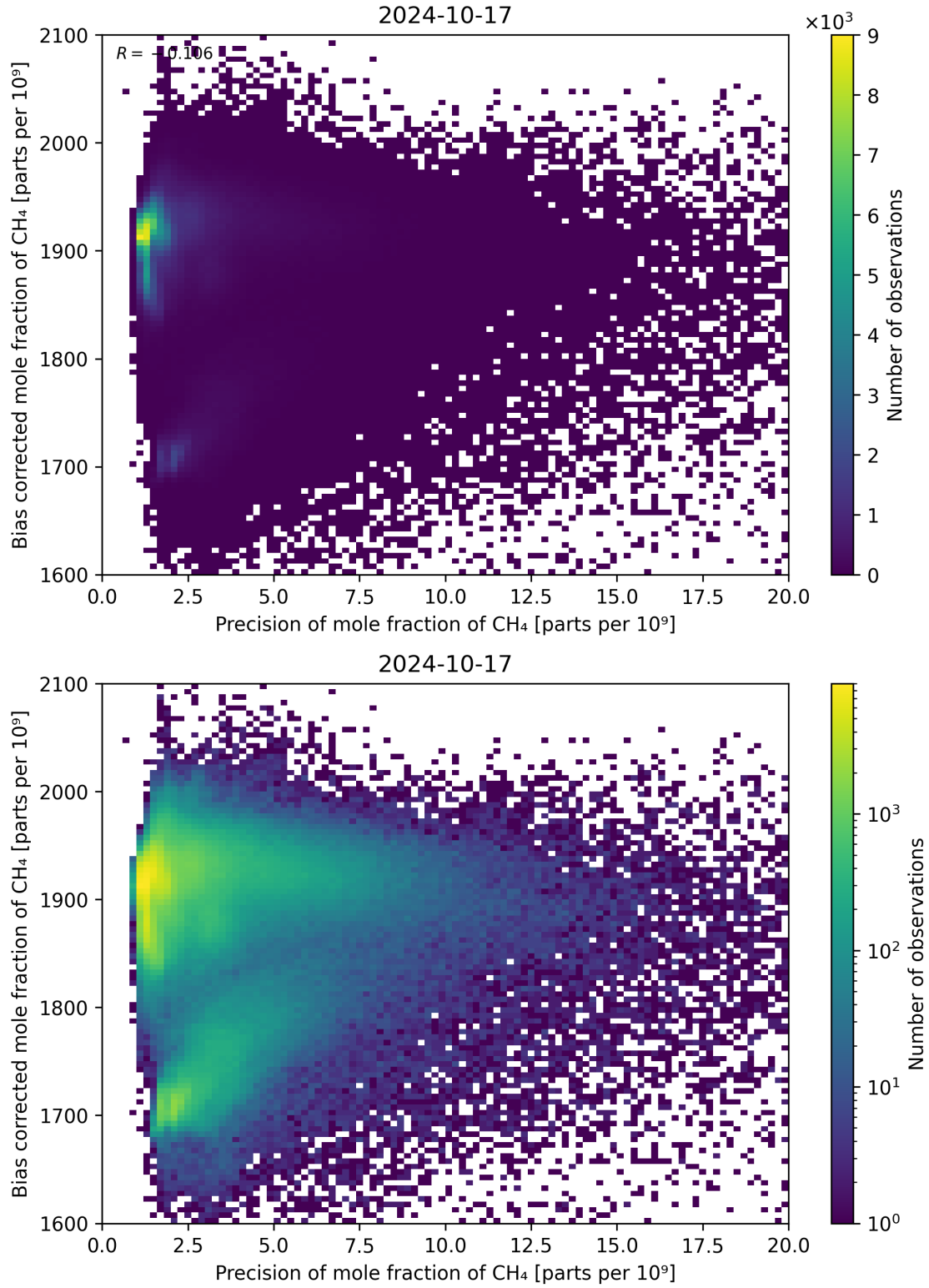
Figure 82: Scatter density plot of “Precision of mole fraction of CH 4 ” against “Bias corrected mole fraction of CH 4 ” for 2024-10-16 to 2024-10-18.
