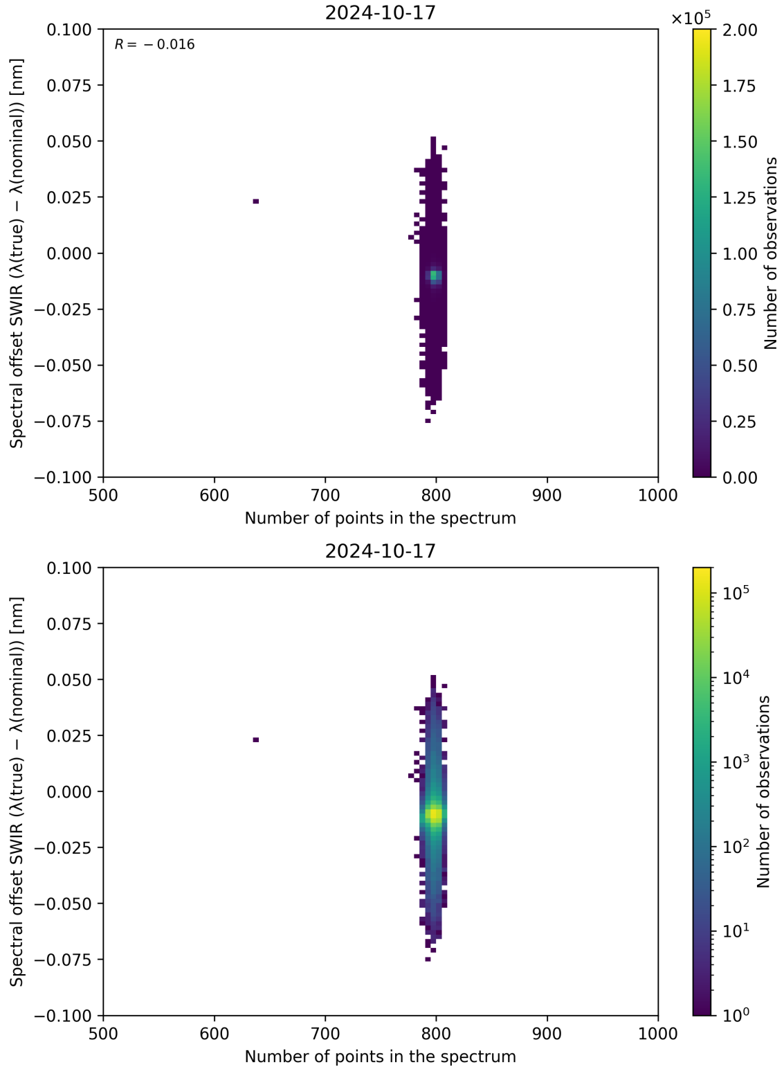
Figure 93: Scatter density plot of “Number of points in the spectrum” against “Spectral offset SWIR ( \lambda_{\text{true}} - \lambda_{\text{nominal}} )” for 2024-10-16 to 2024-10-18.
