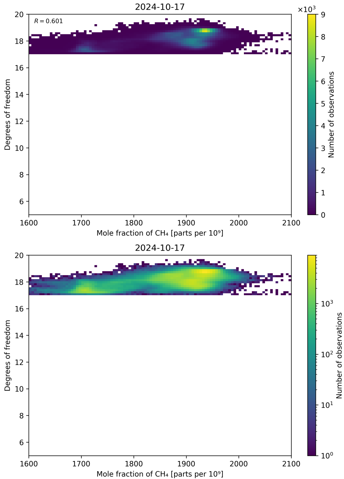
Figure 72: Scatter density plot of “Mole fraction of CH 4 ” against “Degrees of freedom” for 2024-10-16 to 2024-10-18.
