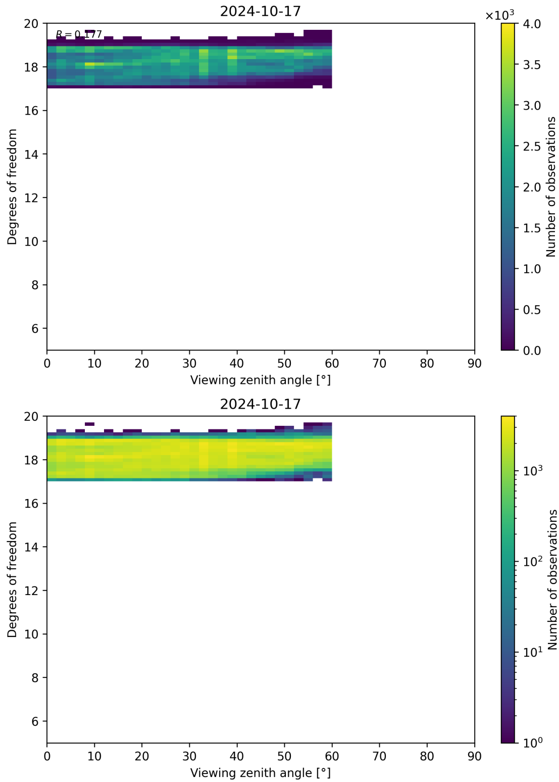
Figure 107: Scatter density plot of “Viewing zenith angle” against “Degrees of freedom” for 2024-10-16 to 2024-10-18.
