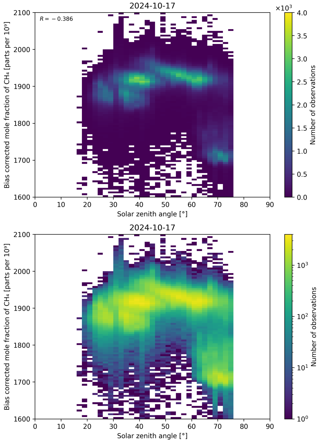
Figure 100: Scatter density plot of “Solar zenith angle” against “Bias corrected mole fraction of \text{CH}_4 ” for 2024-10-16 to 2024-10-18.
