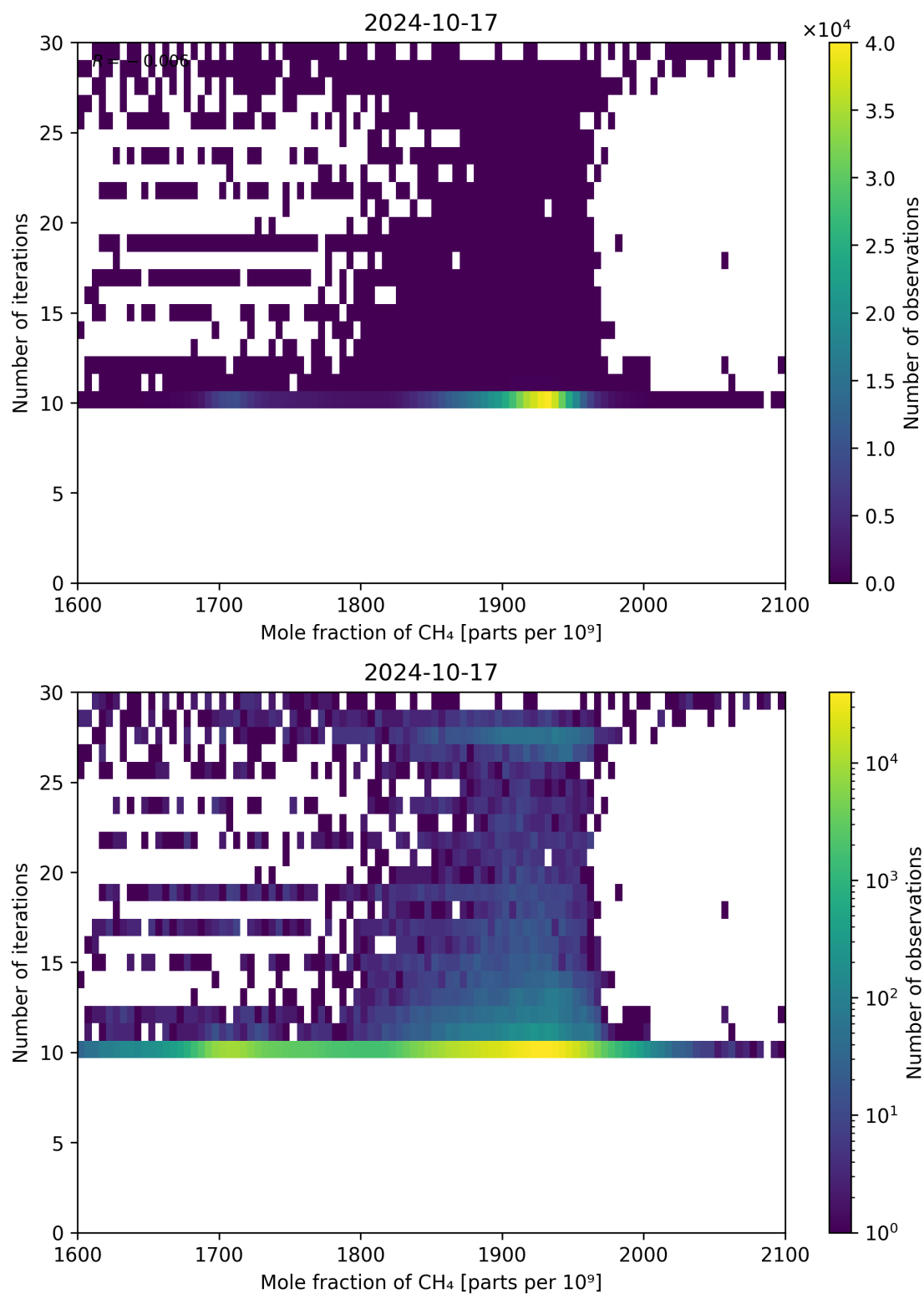
Figure 76: Scatter density plot of “Mole fraction of CH 4 ” against “Number of iterations” for 2024-10-16 to 2024-10-18.
