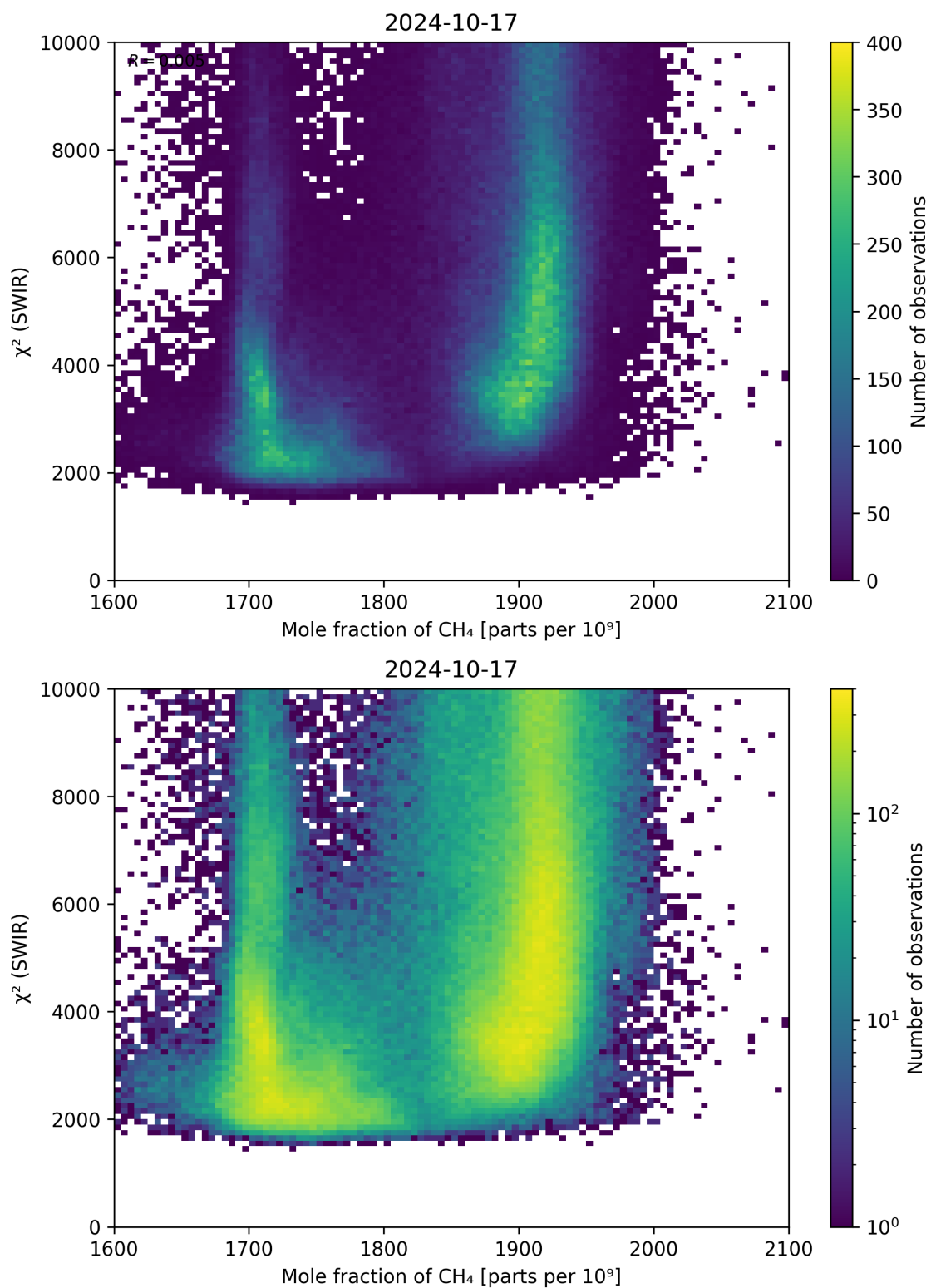
Figure 71: Scatter density plot of “Mole fraction of \text{CH}_4 ” against “ \chi^2 (SWIR)” for 2024-10-16 to 2024-10-18.
