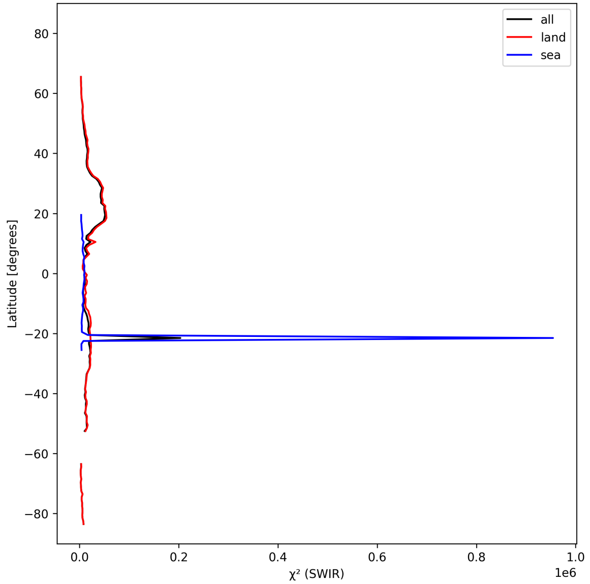
Figure 17: Zonal average of “ \chi^2 (SWIR)” for 2024-10-16 to 2024-10-18.
