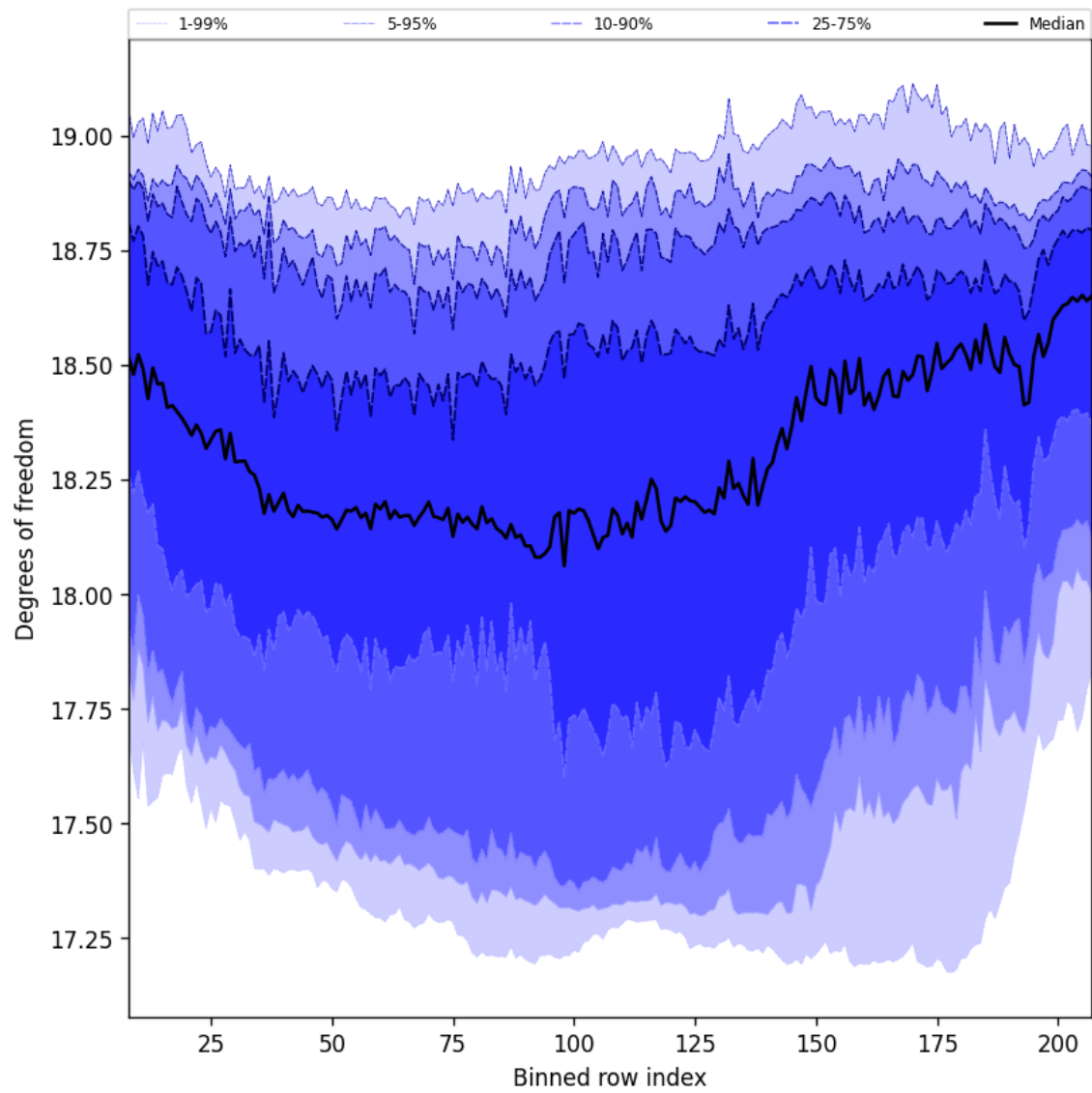
Figure 41: Along track statistics of “Degrees of freedom” for 2024-10-19 to 2024-10-20
