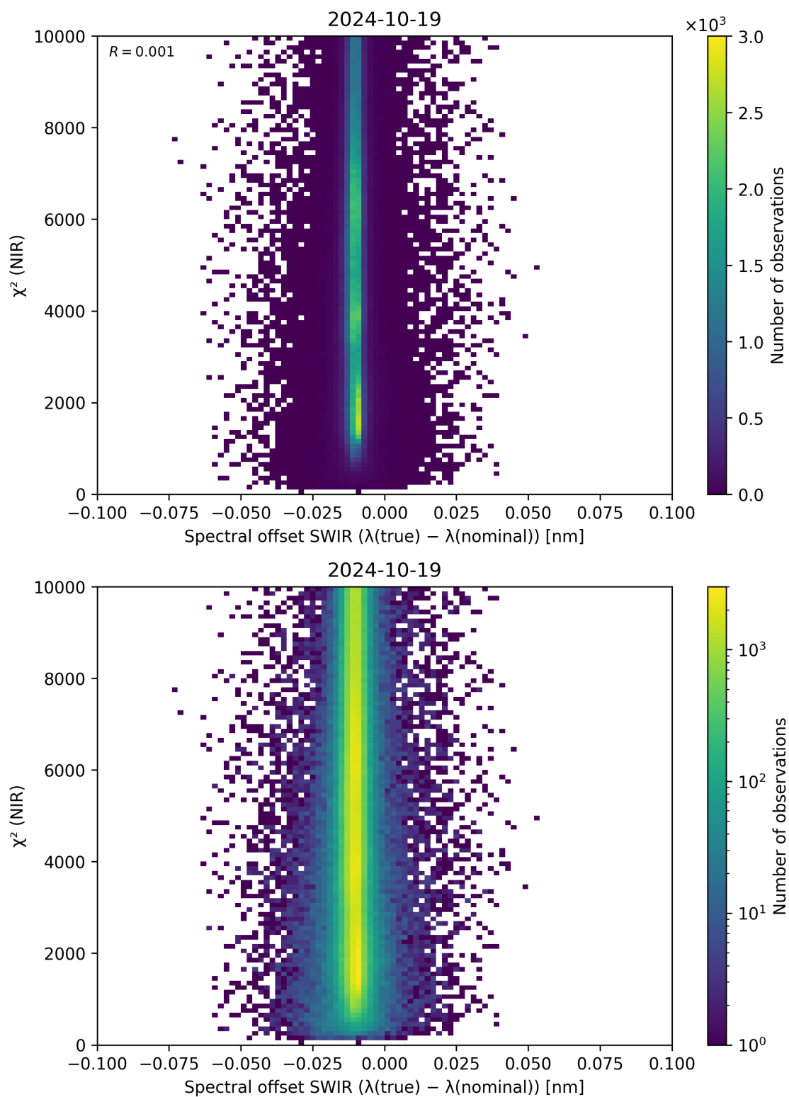
Figure 117: Scatter density plot of “Spectral offset SWIR ( \lambda_{\text{true}} - \lambda_{\text{nominal}} )” against “ \chi^2 (NIR)” for 2024-10-19 to 2024-10-20.
