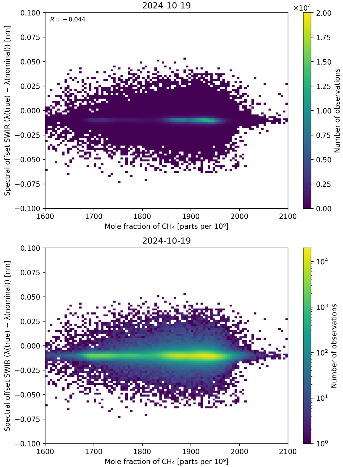
Figure 86: Scatter density plot of “Mole fraction of CH 4 ” against “Spectral offset SWIR ( \lambda_{\text{true}} - \lambda_{\text{nominal}} )” for 2024-10-19 to 2024-10-20.
