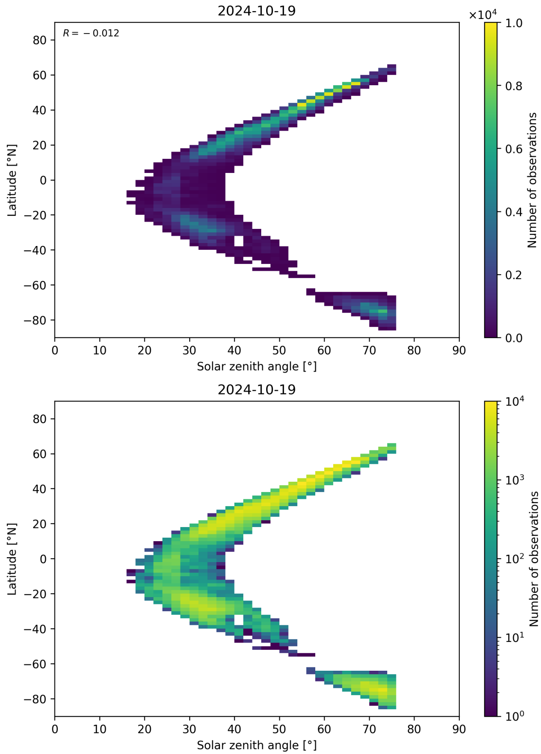
Figure 98: Scatter density plot of “Solar zenith angle” against “Latitude” for 2024-10-19 to 2024-10-20.
