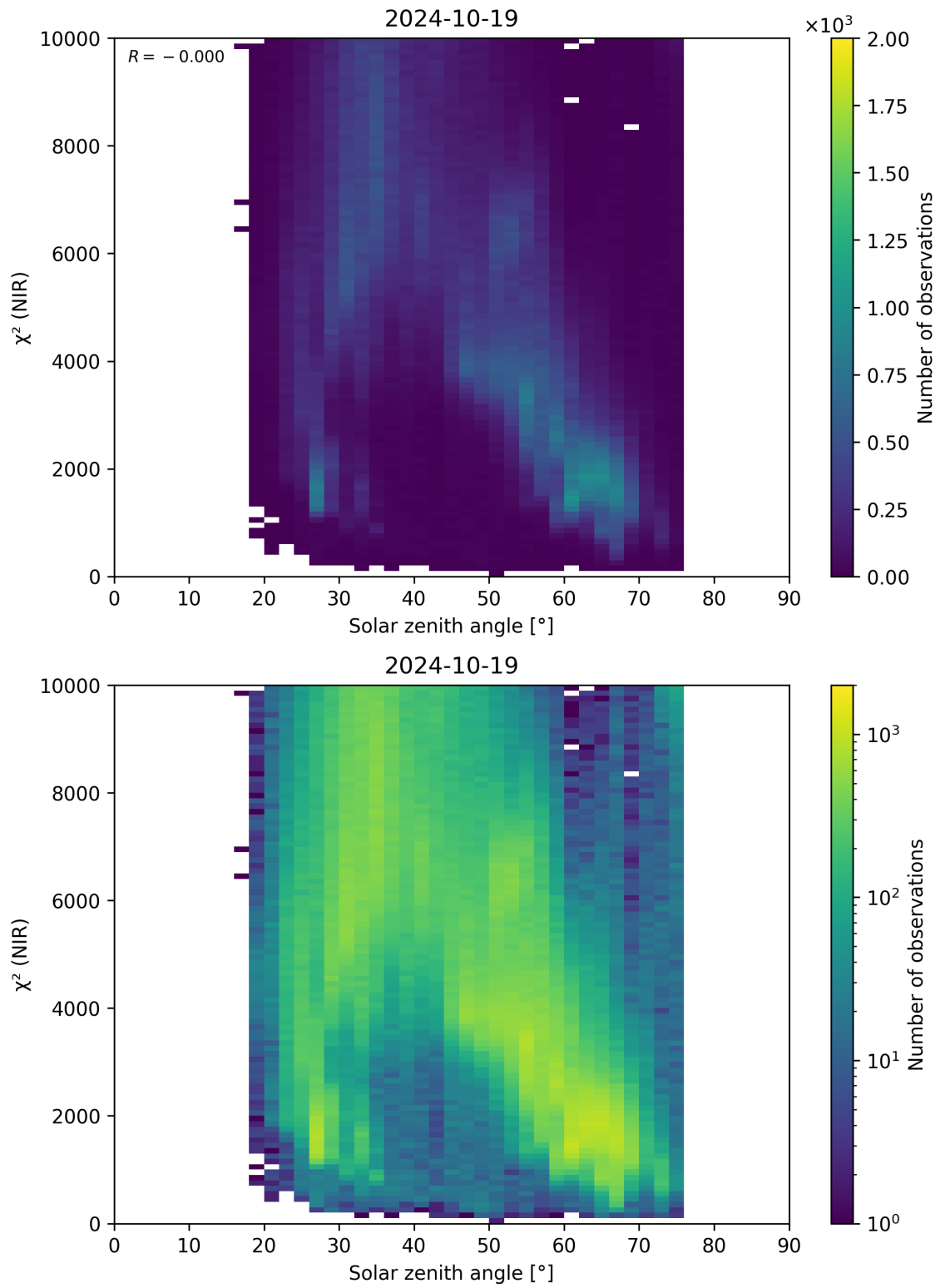
Figure 94: Scatter density plot of “Solar zenith angle” against “ \chi^2 (NIR)” for 2024-10-19 to 2024-10-20.
