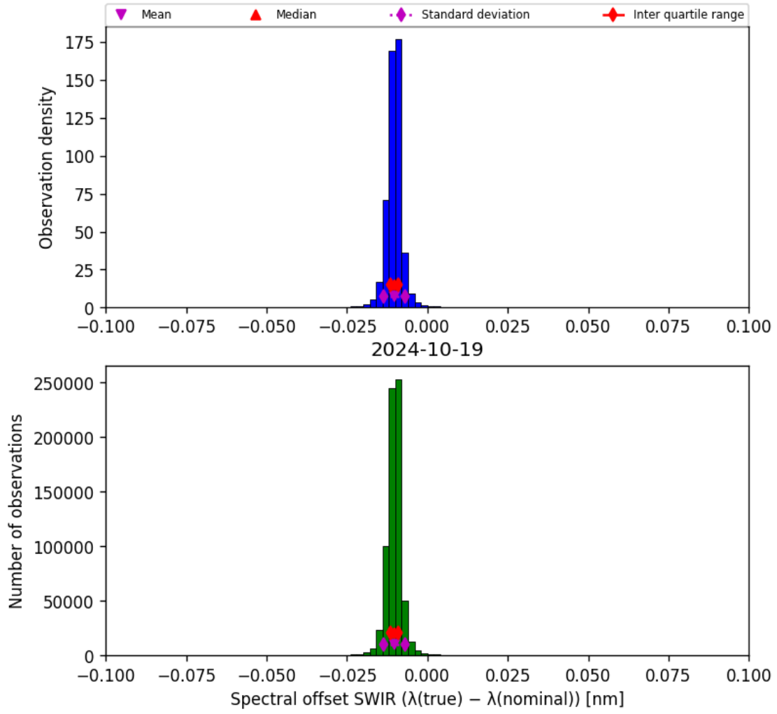
Figure 27: Histogram of “Spectral offset SWIR ( \lambda_{\text{true}} - \lambda_{\text{nominal}} )” for 2024-10-19 to 2024-10-20
