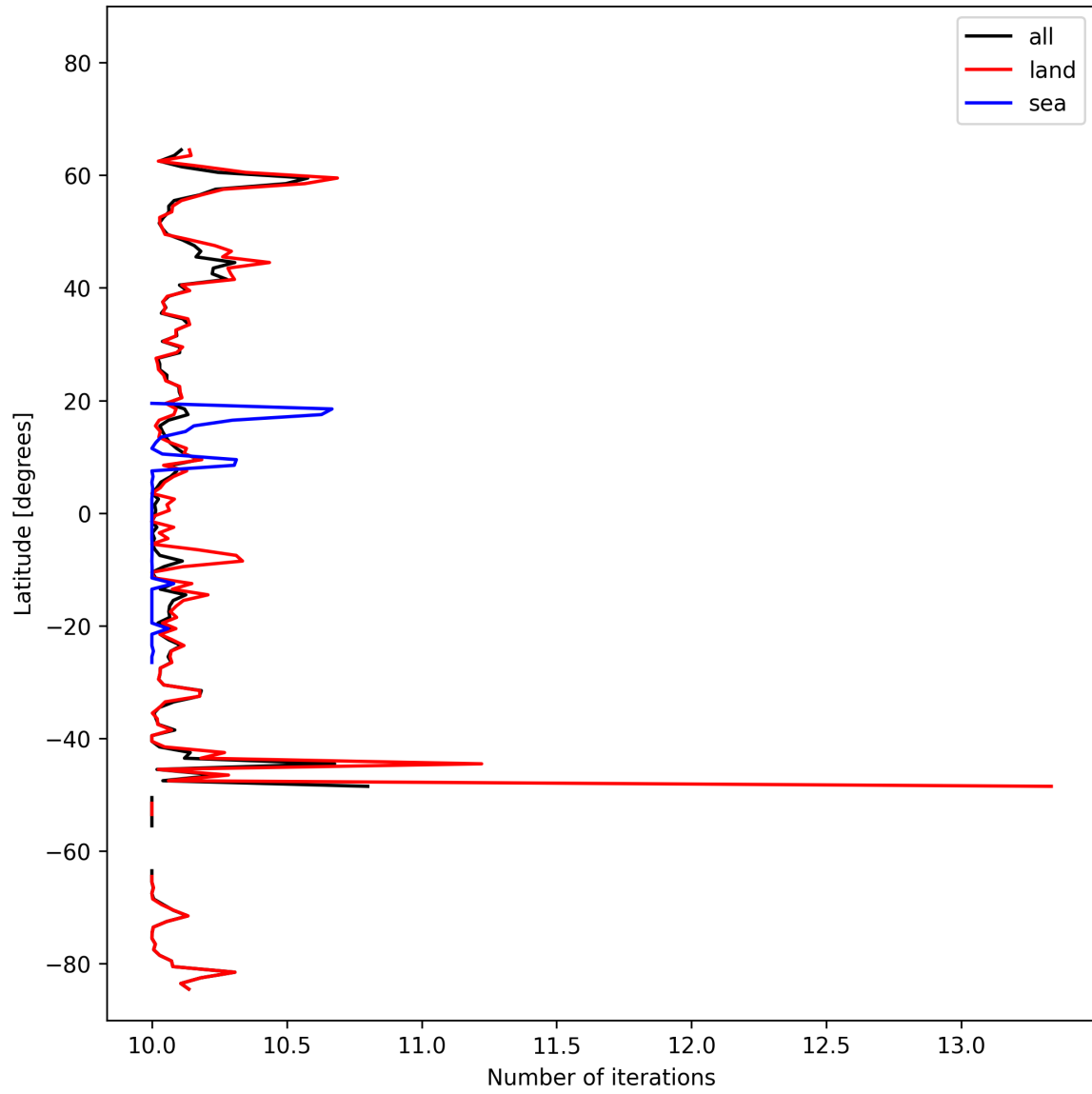
Figure 20: Zonal average of “Number of iterations” for 2024-10-19 to 2024-10-20.
