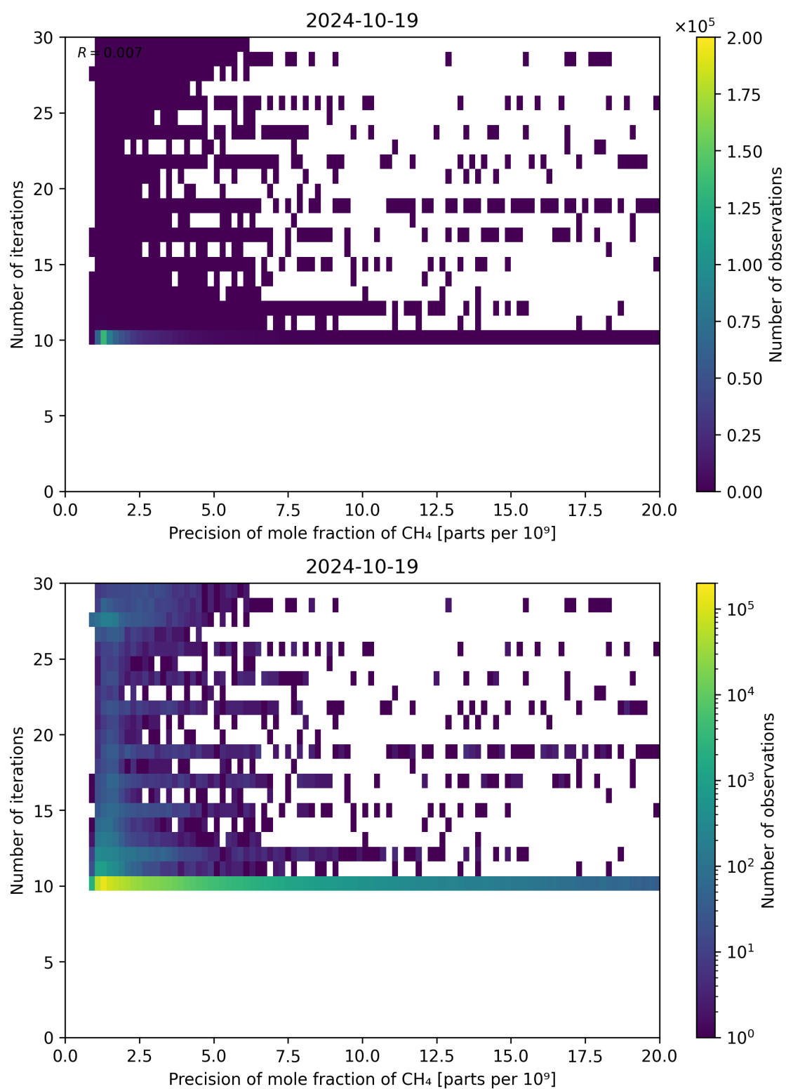
Figure 83: Scatter density plot of “Precision of mole fraction of \text{CH}_4 ” against “Number of iterations” for 2024-10-19 to 2024-10-20.
