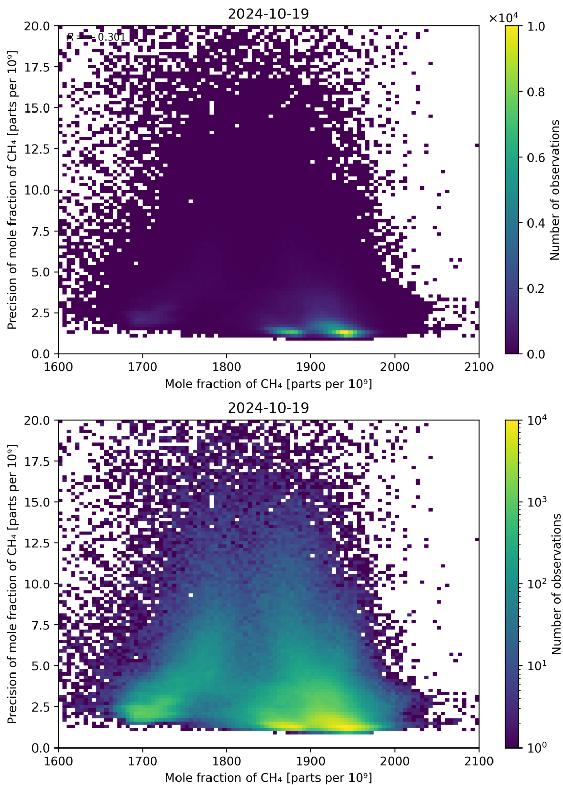
Figure 75: Scatter density plot of “Mole fraction of CH 4 ” against “Precision of mole fraction of CH 4 ” for 2024-10-19 to 2024-10-20.
