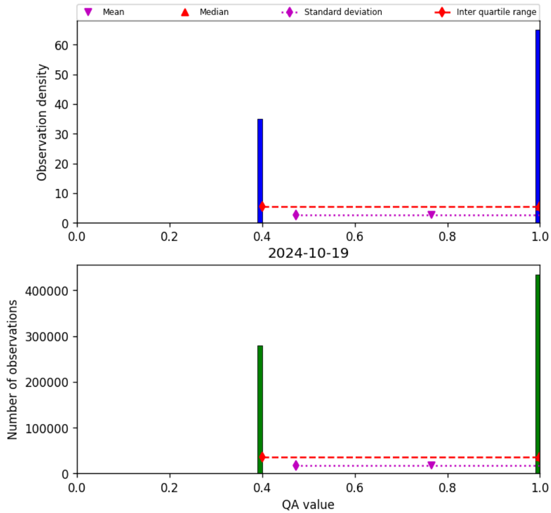
Figure 22: Histogram of “QA value” for 2024-10-19 to 2024-10-20
