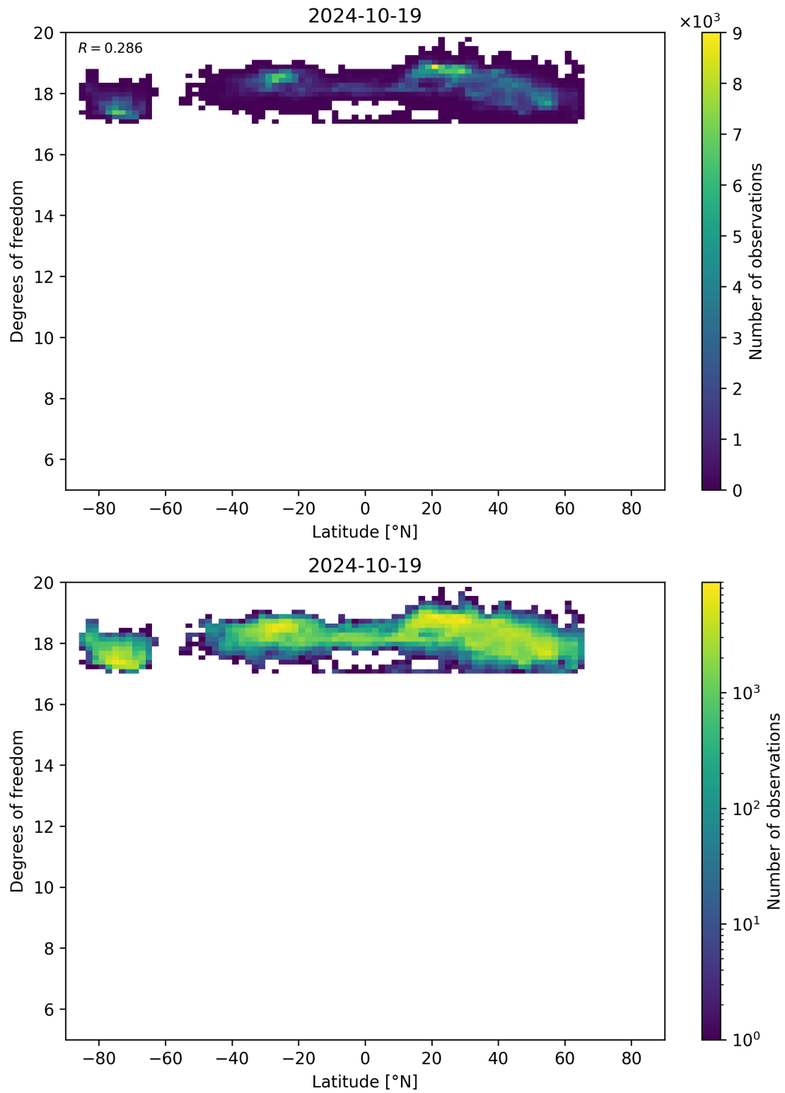
Figure 55: Scatter density plot of “Latitude” against “Degrees of freedom” for 2024-10-19 to 2024-10-20.
