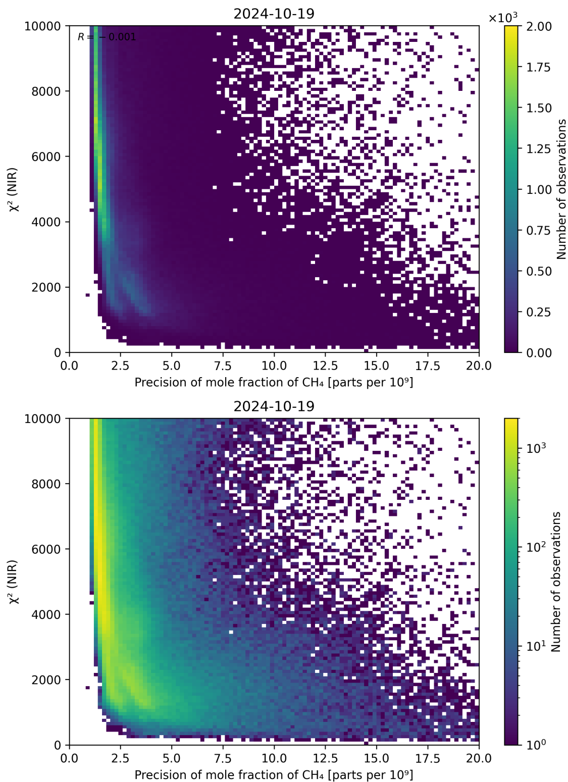
Figure 78: Scatter density plot of “Precision of mole fraction of CH 4 ” against “ \chi^2 (NIR)” for 2024-10-19 to 2024-10-20.
