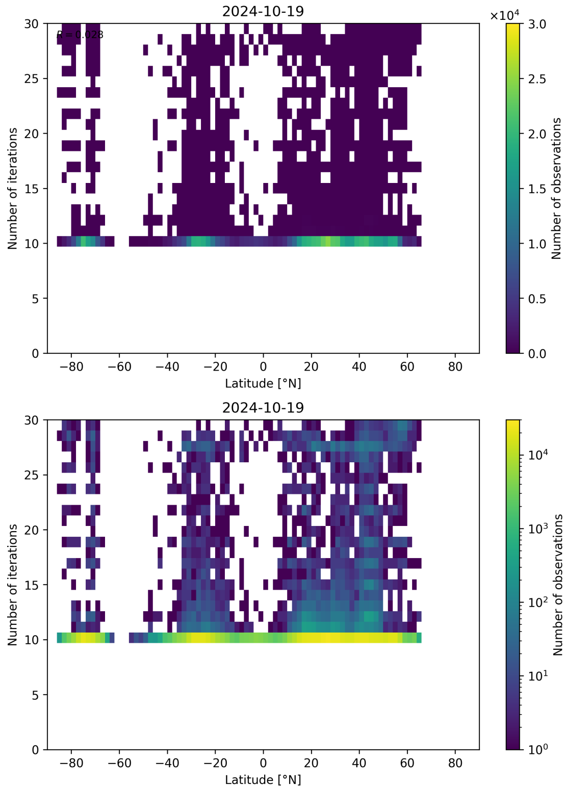
Figure 60: Scatter density plot of “Latitude” against “Number of iterations” for 2024-10-19 to 2024-10-20.
