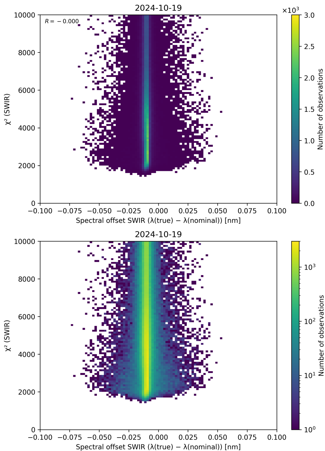
Figure 118: Scatter density plot of “Spectral offset SWIR ( \lambda_{\text{true}} - \lambda_{\text{nominal}} )” against “ \chi^2 (SWIR)” for 2024-10-19 to 2024-10-20.
