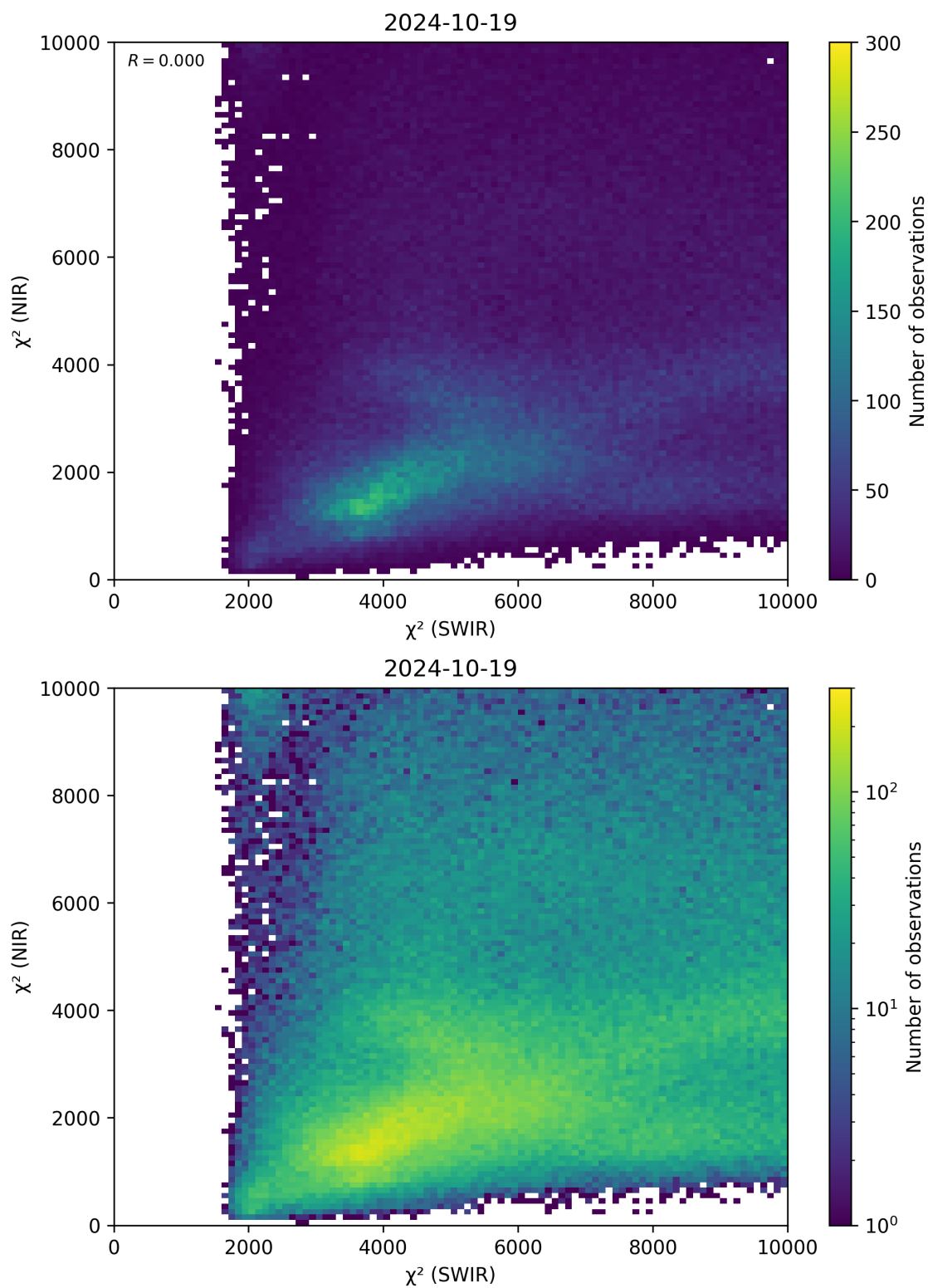
Figure 47: Scatter density plot of “ \chi^2 (SWIR)” against “ \chi^2 (NIR)” for 2024-10-19 to 2024-10-20.
