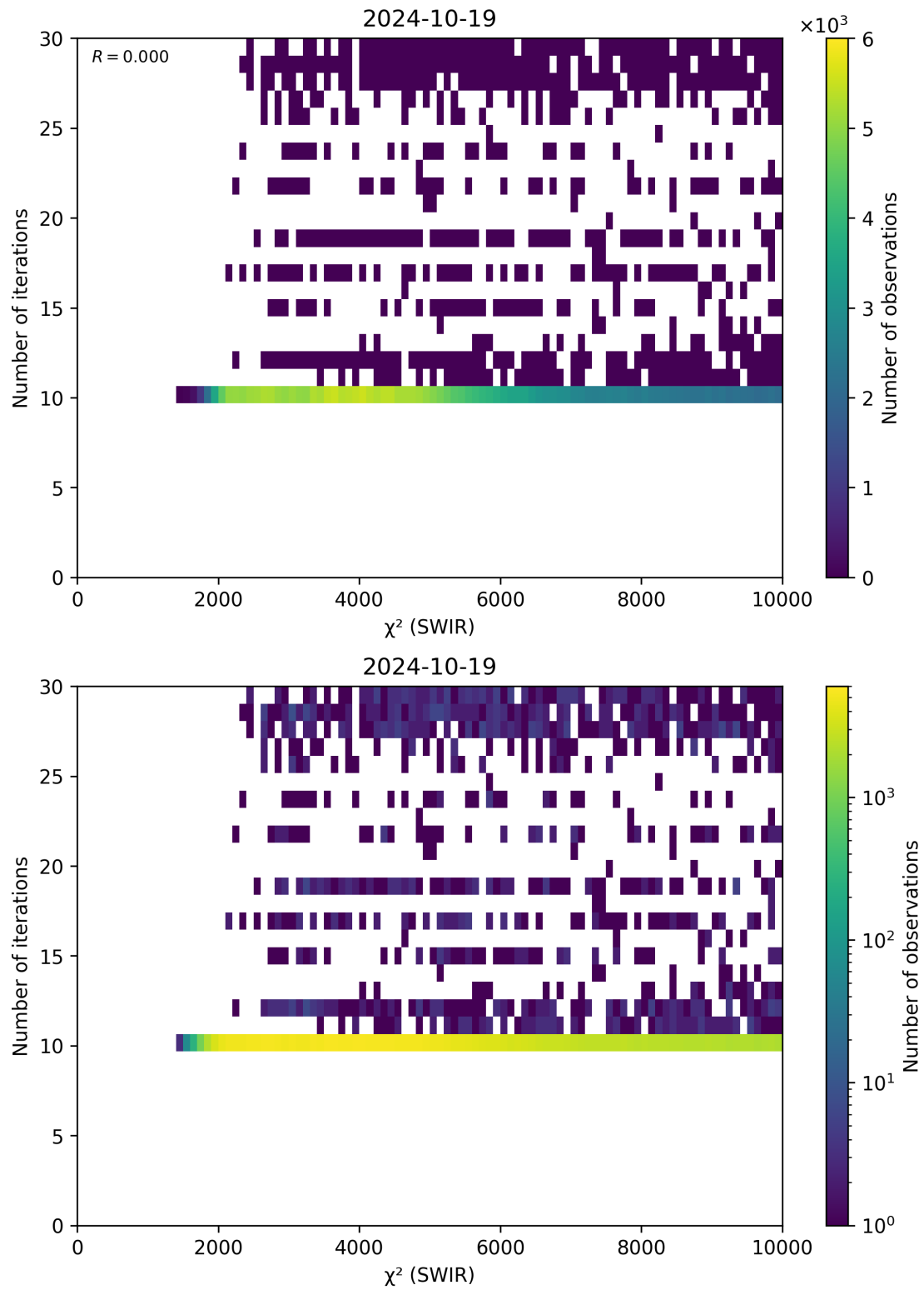
Figure 50: Scatter density plot of “ \chi^2 (SWIR)” against “Number of iterations” for 2024-10-19 to 2024-10-20.
