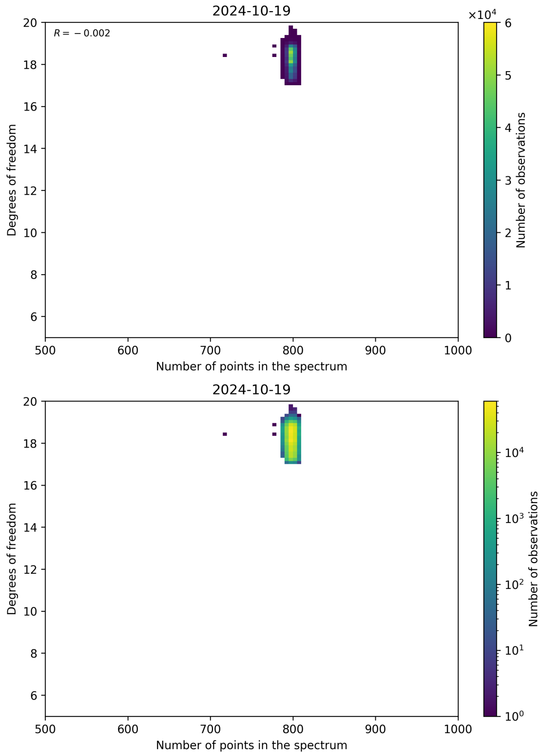
Figure 90: Scatter density plot of “Number of points in the spectrum” against “Degrees of freedom” for 2024-10-19 to 2024-10-20.
