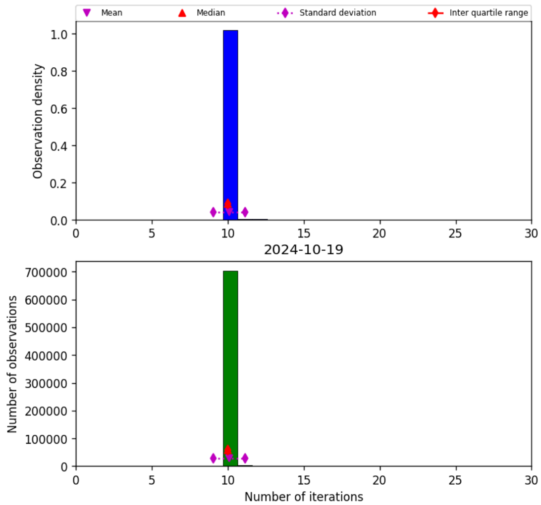
Figure 31: Histogram of “Number of iterations” for 2024-10-19 to 2024-10-20
