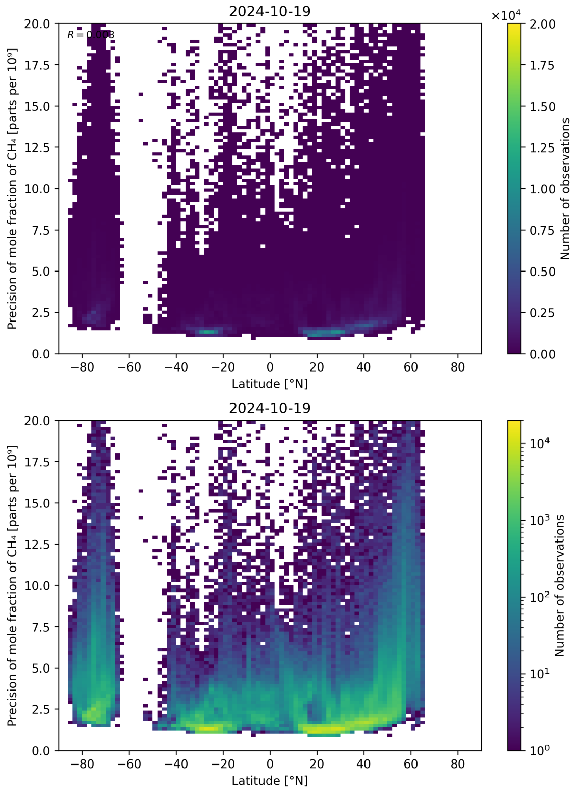
Figure 59: Scatter density plot of “Latitude” against “Precision of mole fraction of CH 4 ” for 2024-10-19 to 2024-10-20.
