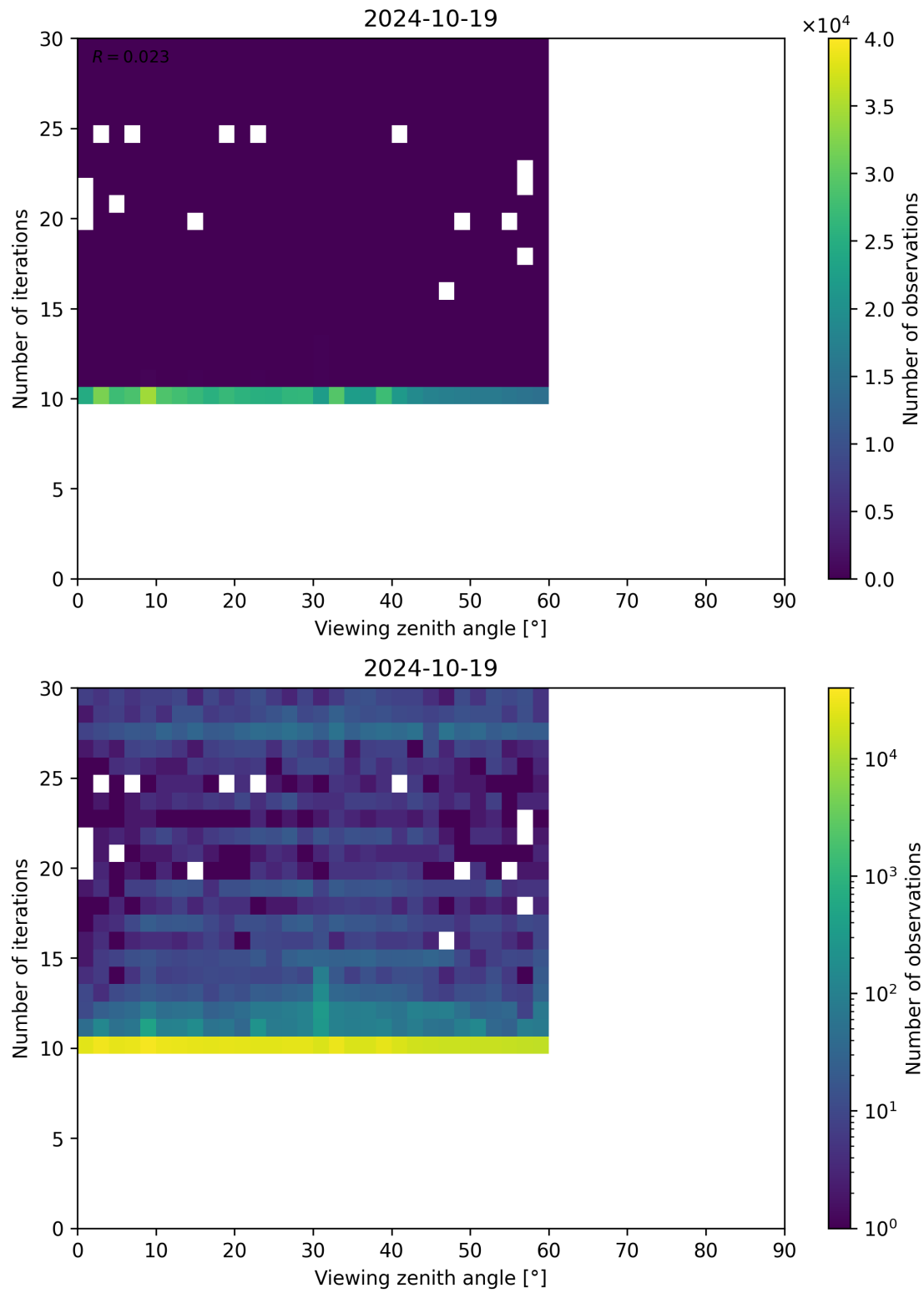
Figure 113: Scatter density plot of “Viewing zenith angle” against “Number of iterations” for 2024-10-19 to 2024-10-20.
