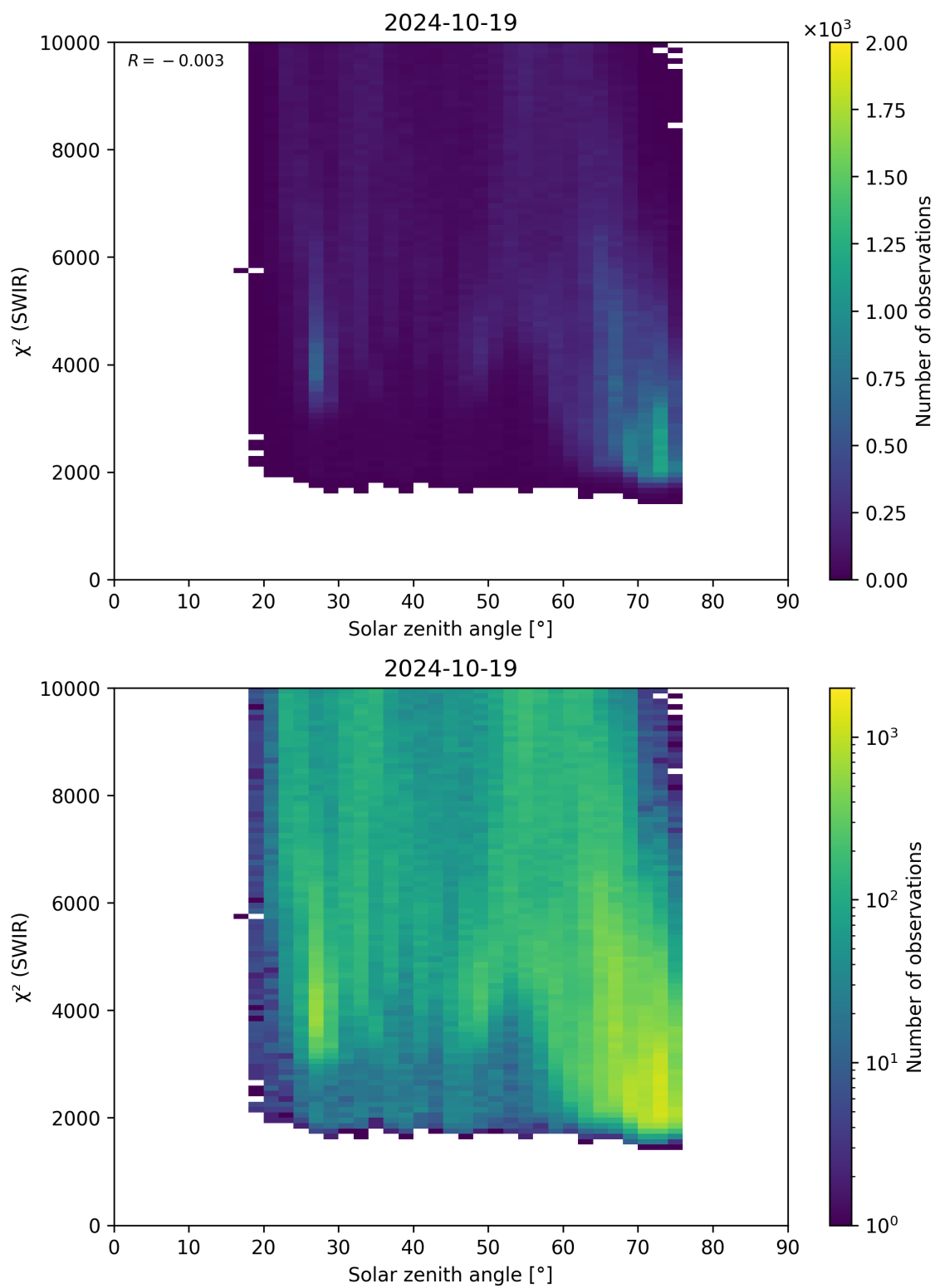
Figure 95: Scatter density plot of “Solar zenith angle” against “ \chi^2 (SWIR)” for 2024-10-19 to 2024-10-20.
