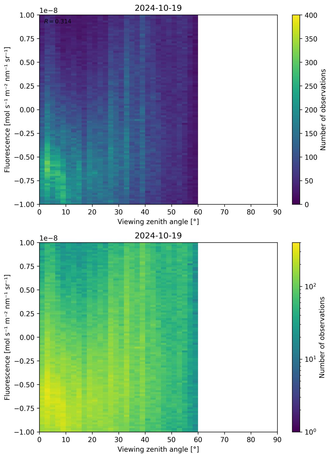
Figure 108: Scatter density plot of “Viewing zenith angle” against “Fluorescence” for 2024-10-19 to 2024-10-20.
