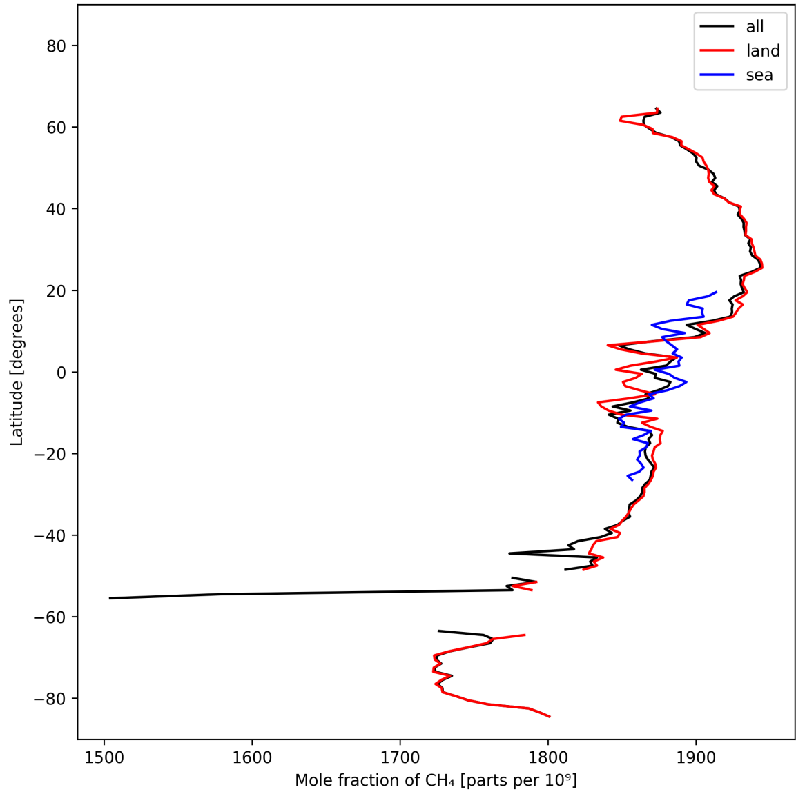
Figure 12: Zonal average of “Mole fraction of \text{CH}_4 ” for 2024-10-19 to 2024-10-20.
