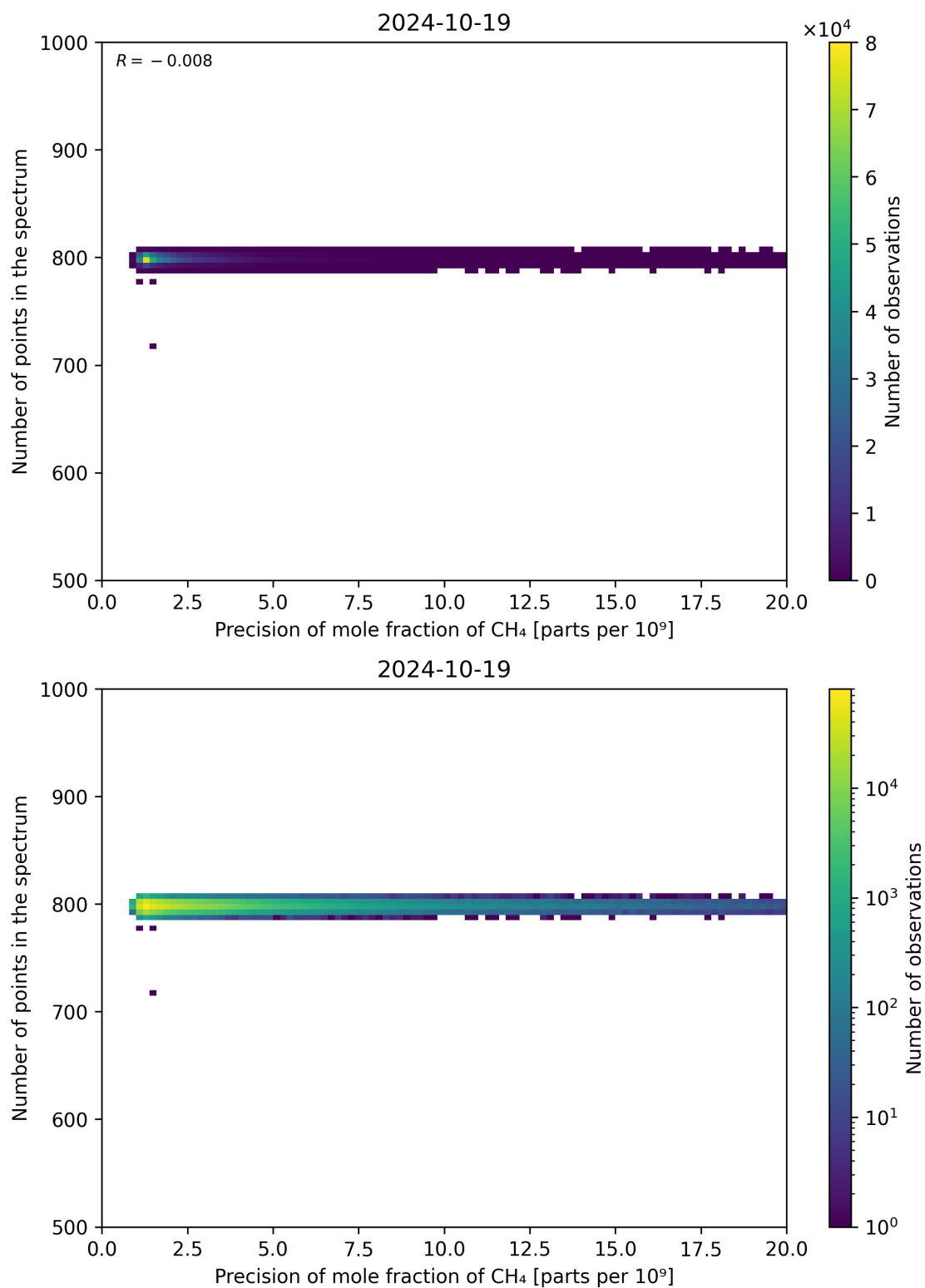
Figure 84: Scatter density plot of “Precision of mole fraction of CH 4 ” against “Number of points in the spectrum” for 2024-10-19 to 2024-10-20.
