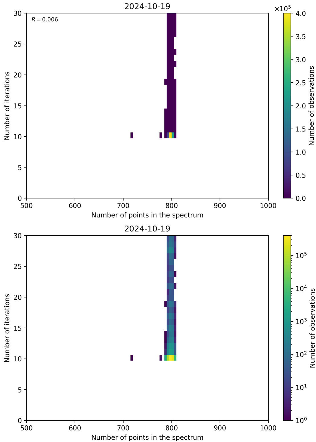
Figure 92: Scatter density plot of “Number of points in the spectrum” against “Number of iterations” for 2024-10-19 to 2024-10-20.
