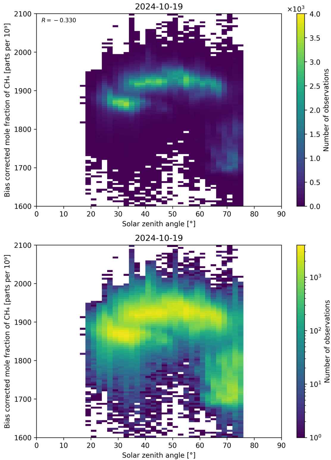
Figure 100: Scatter density plot of “Solar zenith angle” against “Bias corrected mole fraction of CH 4 ” for 2024-10-19 to 2024-10-20.
