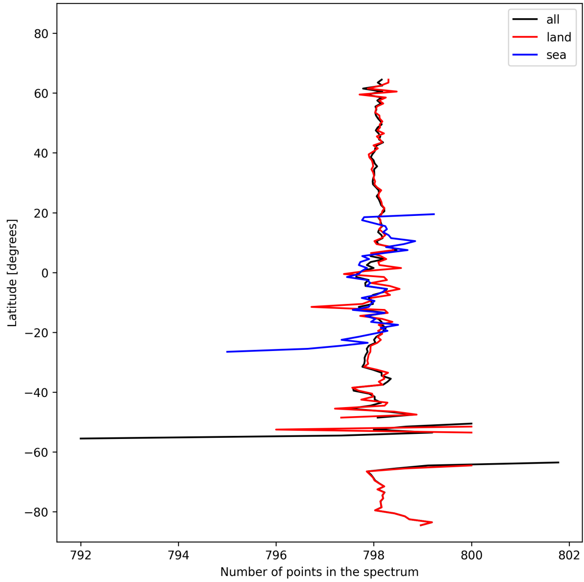
Figure 15: Zonal average of “Number of points in the spectrum” for 2024-10-19 to 2024-10-20.
