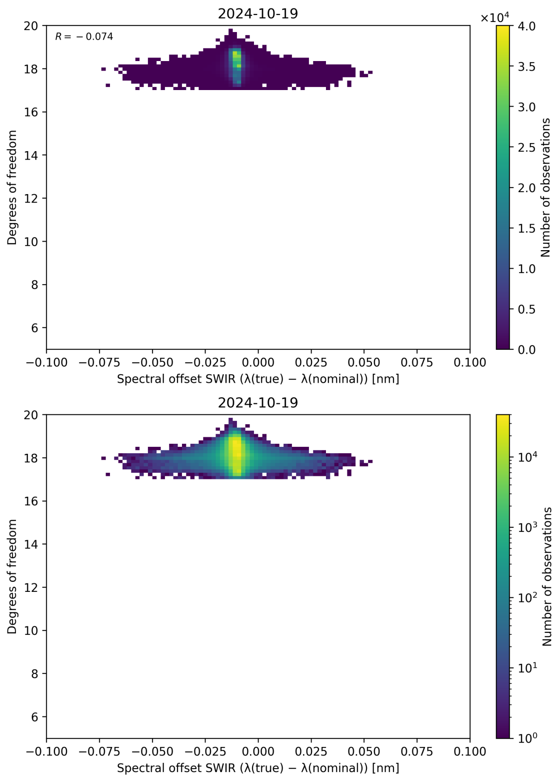
Figure 119: Scatter density plot of “Spectral offset SWIR ( \lambda_{\text{true}} - \lambda_{\text{nominal}} )” against “Degrees of freedom” for 2024-10-19 to 2024-10-20.
