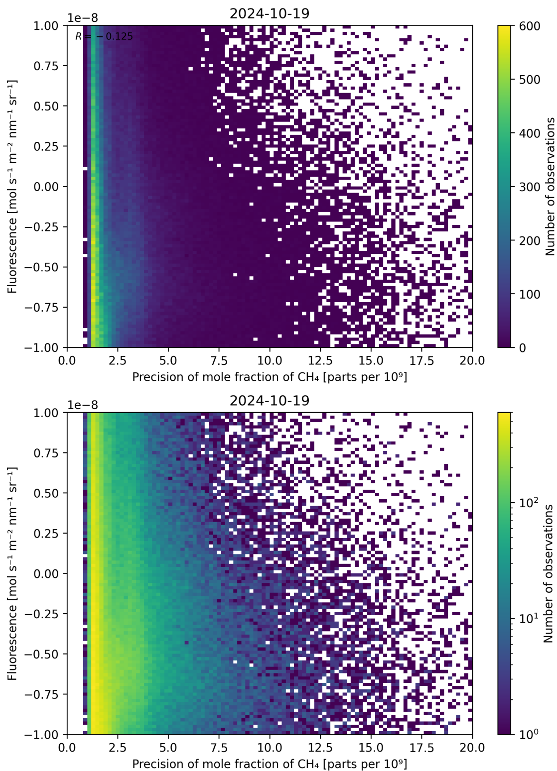
Figure 81: Scatter density plot of “Precision of mole fraction of CH 4 ” against “Fluorescence” for 2024-10-19 to 2024-10-20.
