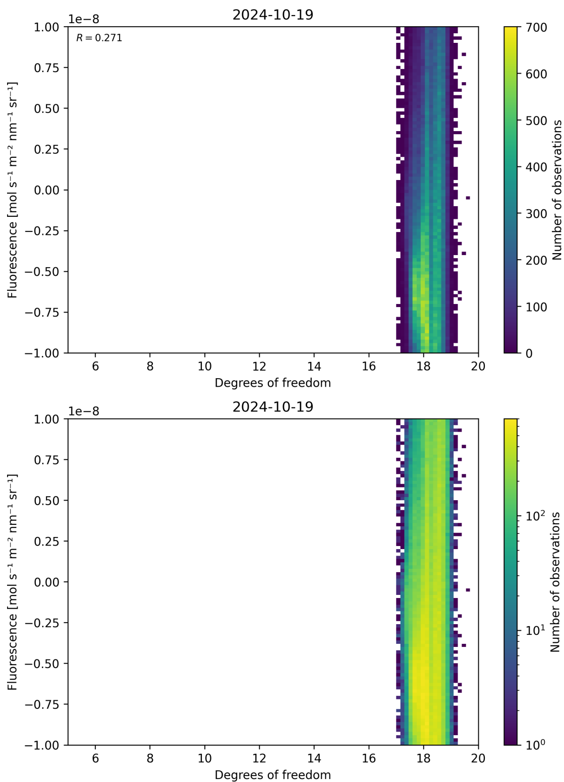
Figure 51: Scatter density plot of “Degrees of freedom” against “Fluorescence” for 2024-10-19 to 2024-10-20.
