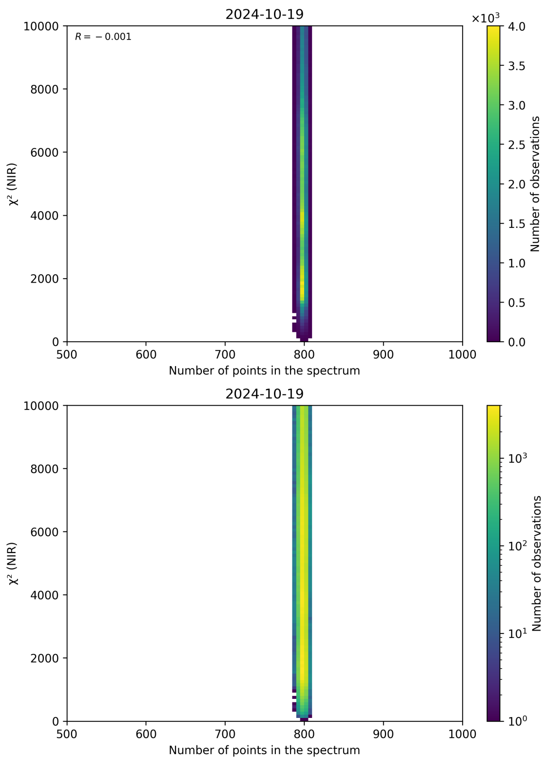
Figure 88: Scatter density plot of “Number of points in the spectrum” against “ \chi^2 (NIR)” for 2024-10-19 to 2024-10-20.
