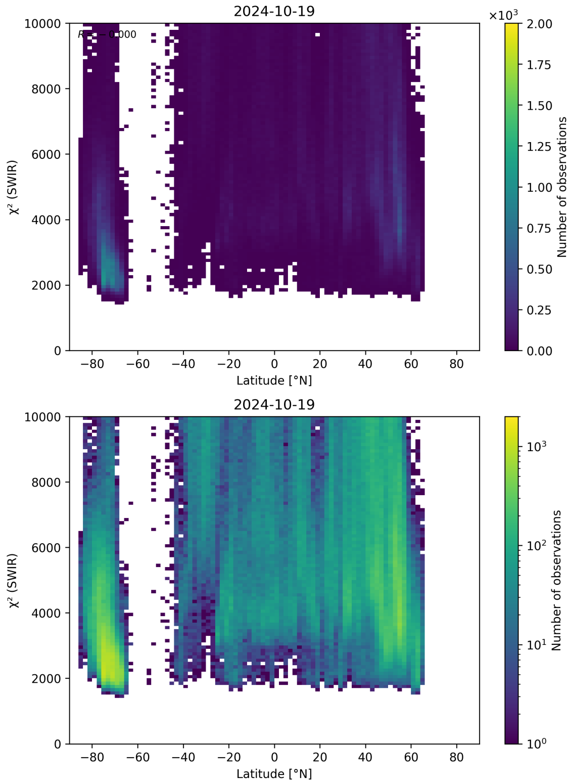
Figure 54: Scatter density plot of “Latitude” against “ \chi^2 (SWIR)” for 2024-10-19 to 2024-10-20.
