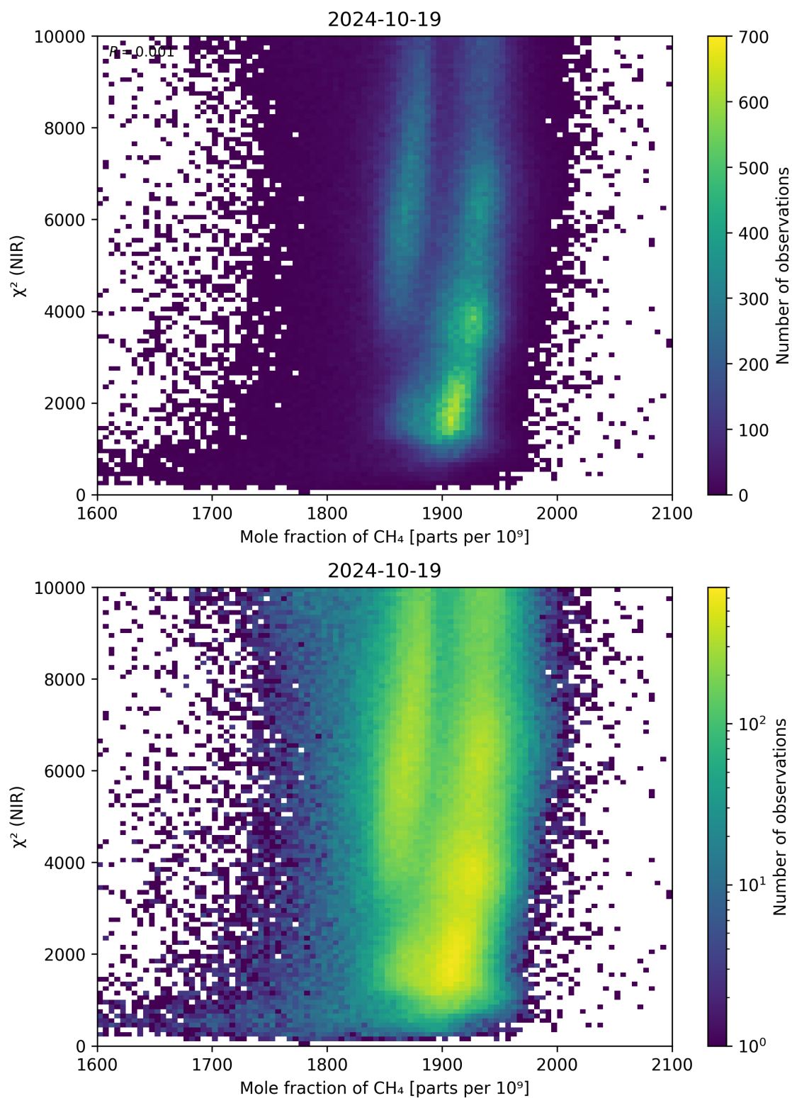
Figure 70: Scatter density plot of “Mole fraction of \text{CH}_4 ” against “ \chi^2 (NIR)” for 2024-10-19 to 2024-10-20.
