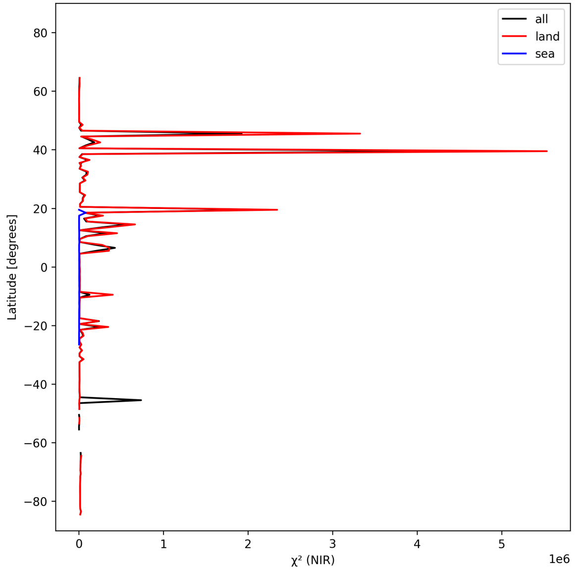
Figure 18: Zonal average of “ \chi^2 (NIR)” for 2024-10-19 to 2024-10-20.
