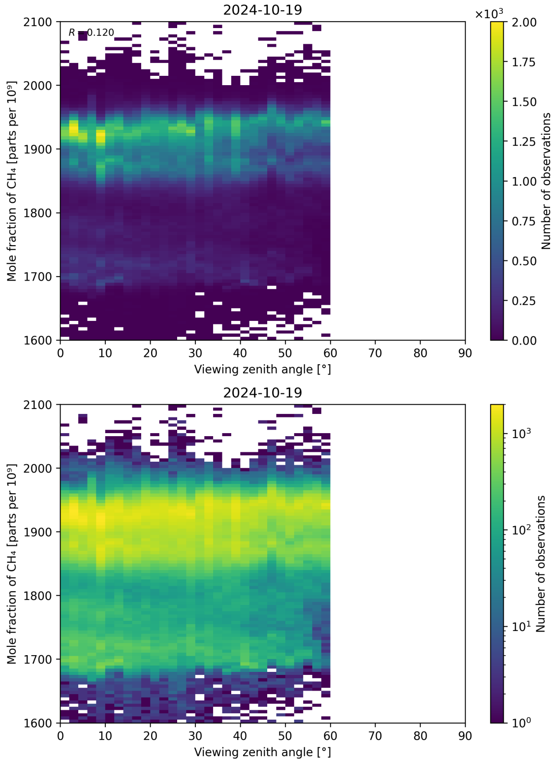
Figure 110: Scatter density plot of “Viewing zenith angle” against “Mole fraction of CH 4 ” for 2024-10-19 to 2024-10-20.
