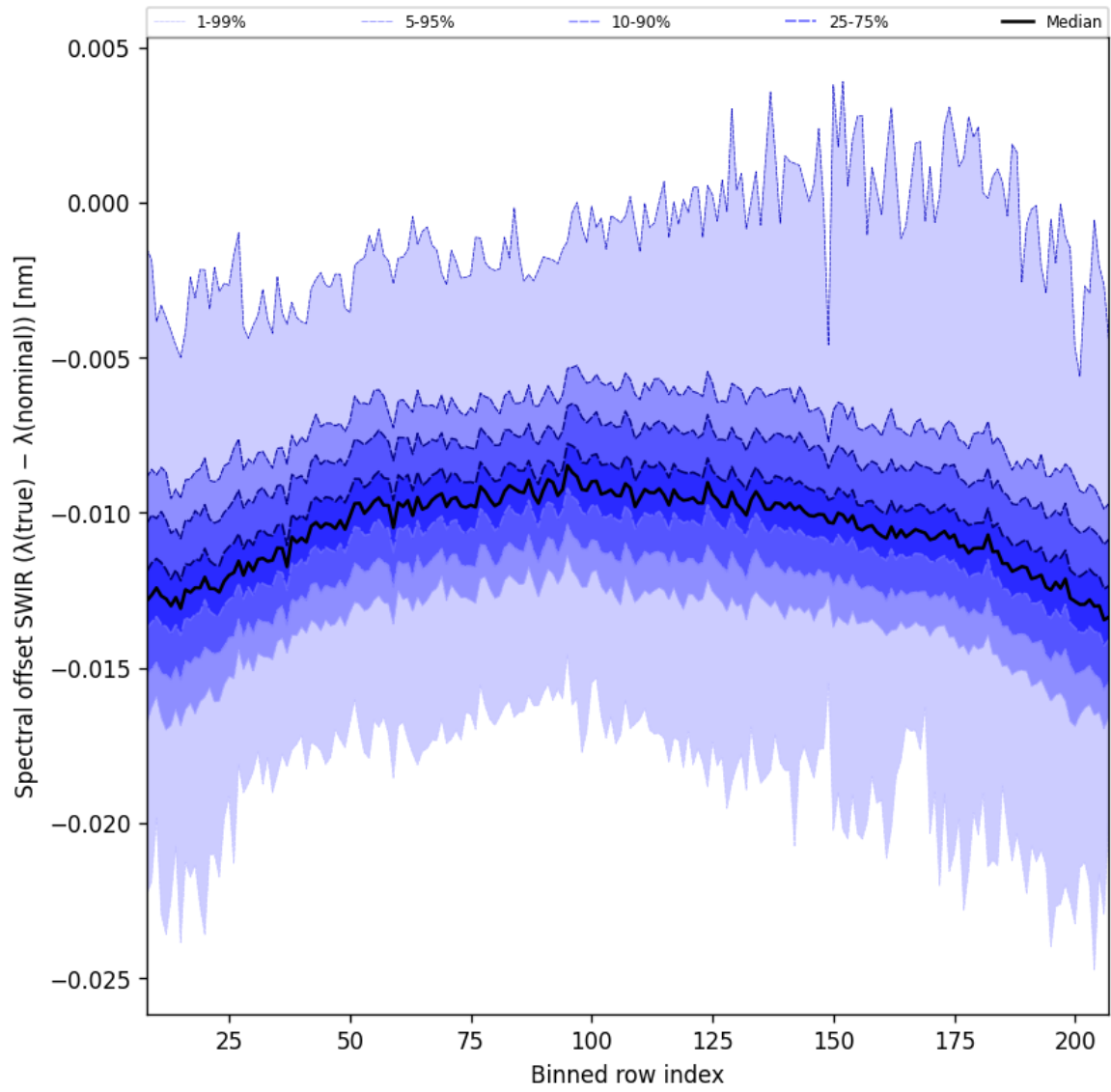
Figure 38: Along track statistics of “Spectral offset SWIR ( \lambda_{\text{true}} - \lambda_{\text{nominal}} )” for 2024-10-19 to 2024-10-20
