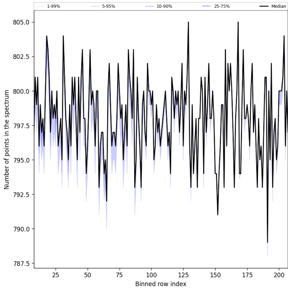
Figure 37: Along track statistics of “Number of points in the spectrum” for 2024-10-19 to 2024-10-20
