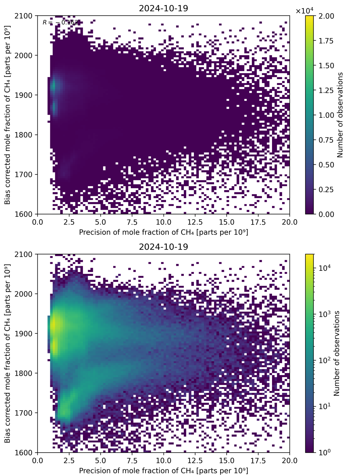
Figure 82: Scatter density plot of “Precision of mole fraction of CH 4 ” against “Bias corrected mole fraction of CH 4 ” for 2024-10-19 to 2024-10-20.
