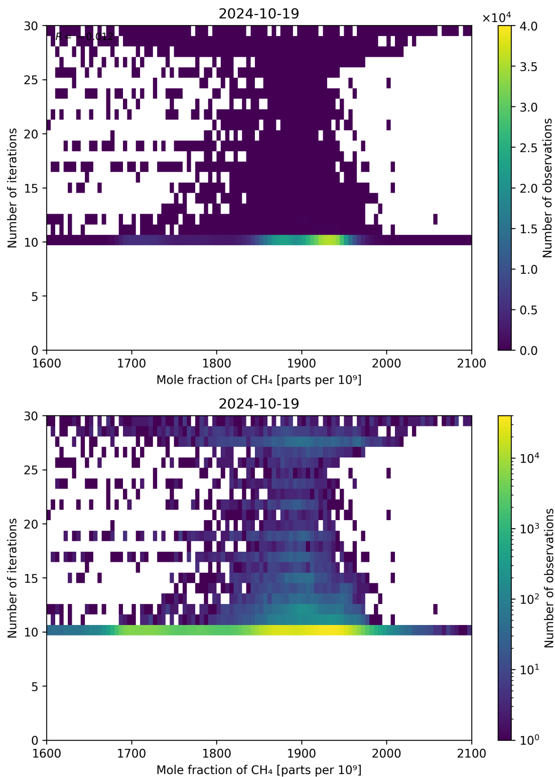
Figure 76: Scatter density plot of “Mole fraction of CH 4 ” against “Number of iterations” for 2024-10-19 to 2024-10-20.
