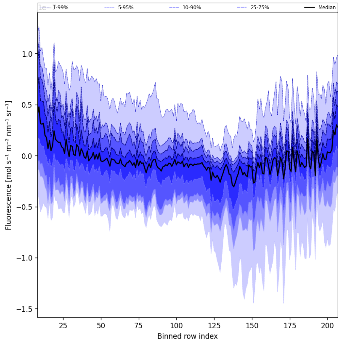
Figure 43: Along track statistics of “Fluorescence” for 2024-10-19 to 2024-10-20
