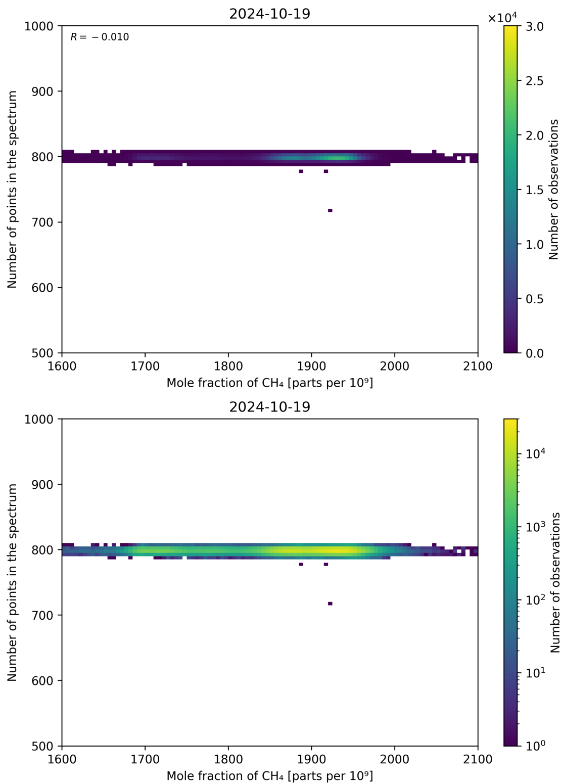
Figure 77: Scatter density plot of “Mole fraction of CH 4 ” against “Number of points in the spectrum” for 2024-10-19 to 2024-10-20.
