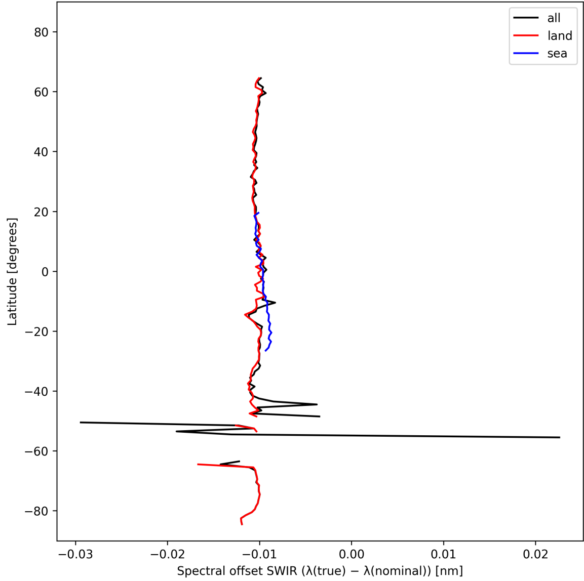
Figure 16: Zonal average of “Spectral offset SWIR ( \lambda_{\text{true}} - \lambda_{\text{nominal}} )” for 2024-10-19 to 2024-10-20.
