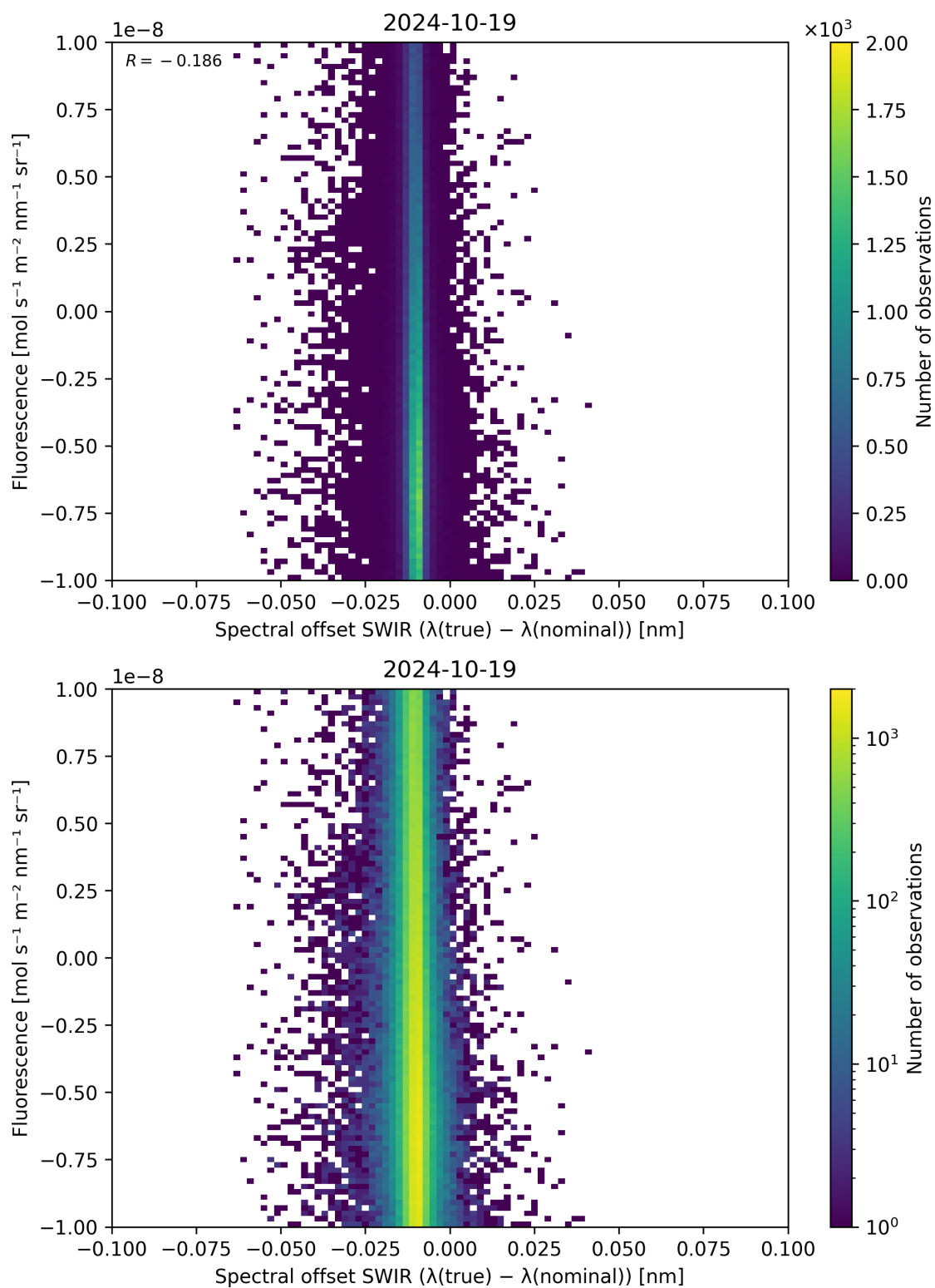
Figure 120: Scatter density plot of “Spectral offset SWIR ( \lambda_{\text{true}} - \lambda_{\text{nominal}} )” against “Fluorescence” for 2024-10-19 to 2024-10-20.
