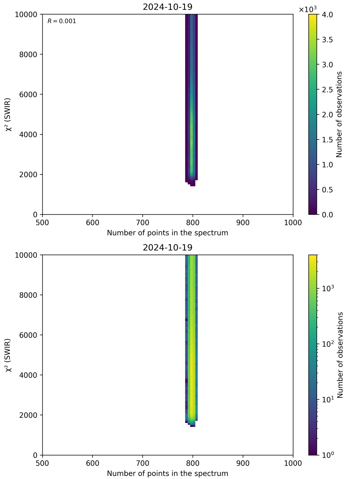
Figure 89: Scatter density plot of “Number of points in the spectrum” against “ \chi^2 (SWIR)” for 2024-10-19 to 2024-10-20.
