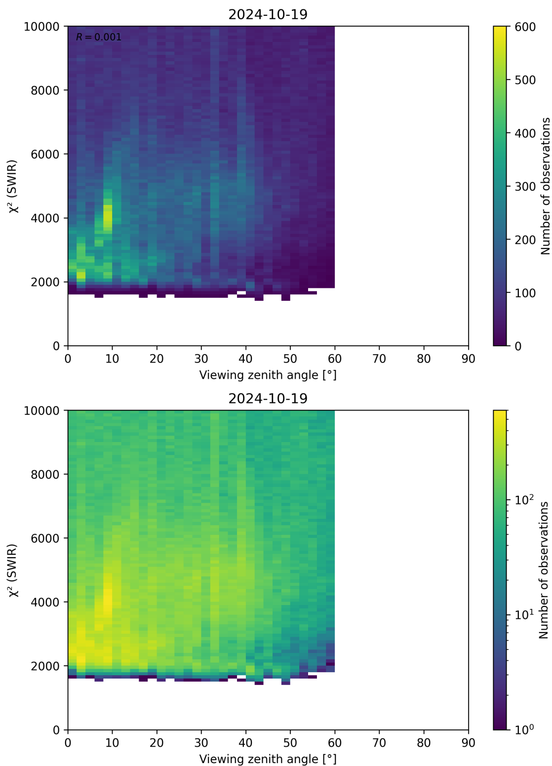
Figure 106: Scatter density plot of “Viewing zenith angle” against “ \chi^2 (SWIR)” for 2024-10-19 to 2024-10-20.
