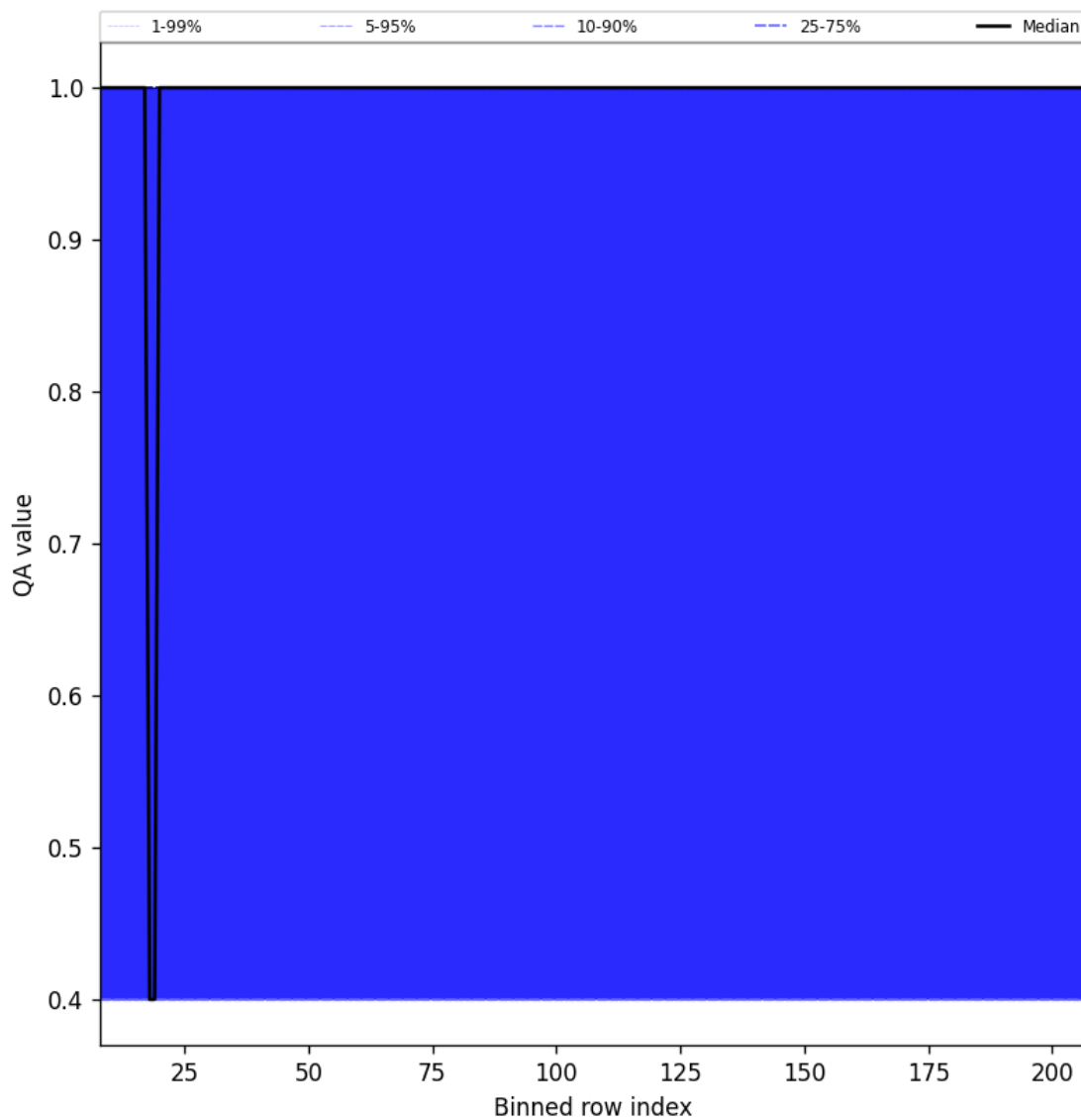
Figure 33: Along track statistics of “QA value” for 2024-10-19 to 2024-10-20
