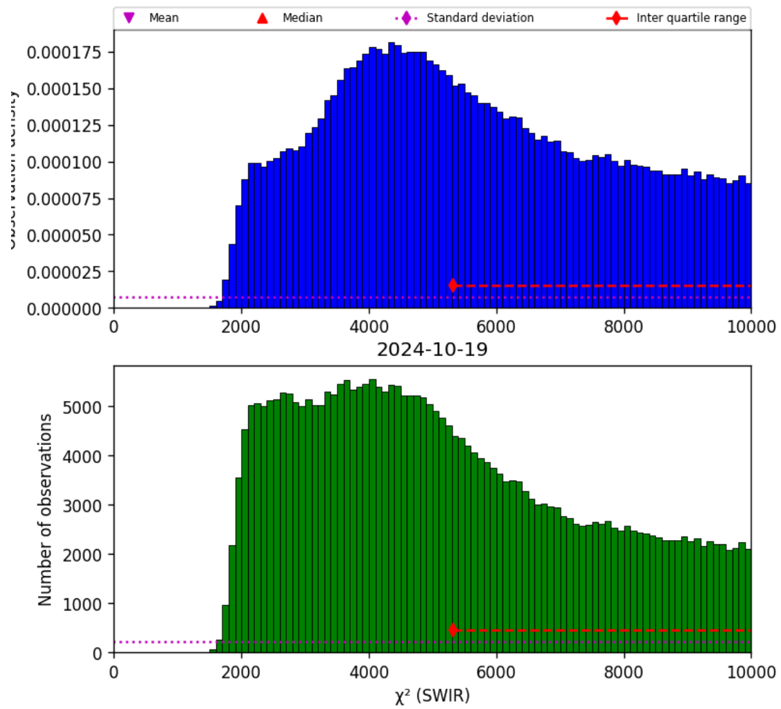
Figure 28: Histogram of “ \chi^2 (SWIR)” for 2024-10-19 to 2024-10-20
