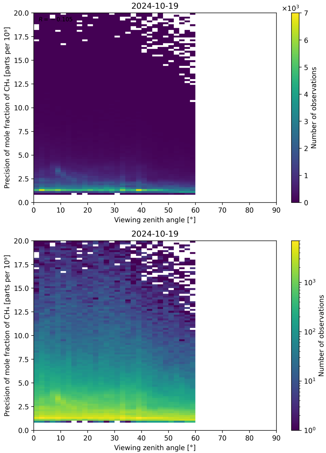
Figure 112: Scatter density plot of “Viewing zenith angle” against “Precision of mole fraction of CH 4 ” for 2024-10-19 to 2024-10-20.
