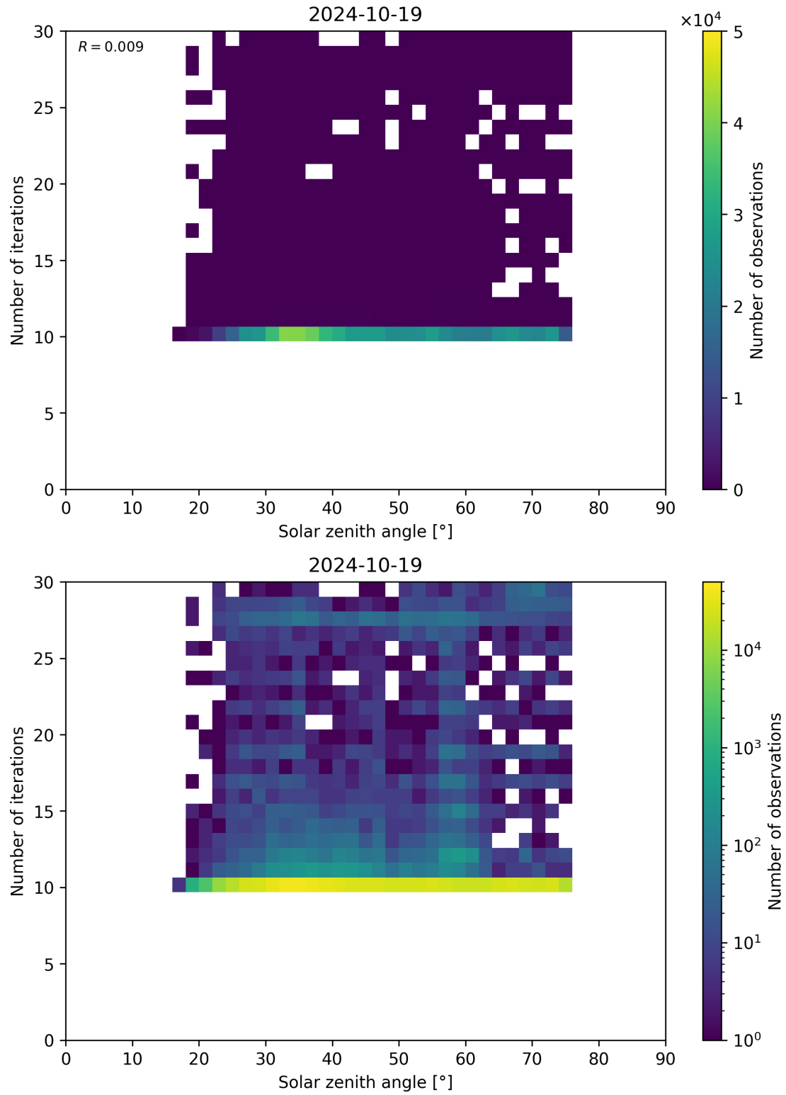
Figure 102: Scatter density plot of “Solar zenith angle” against “Number of iterations” for 2024-10-19 to 2024-10-20.
