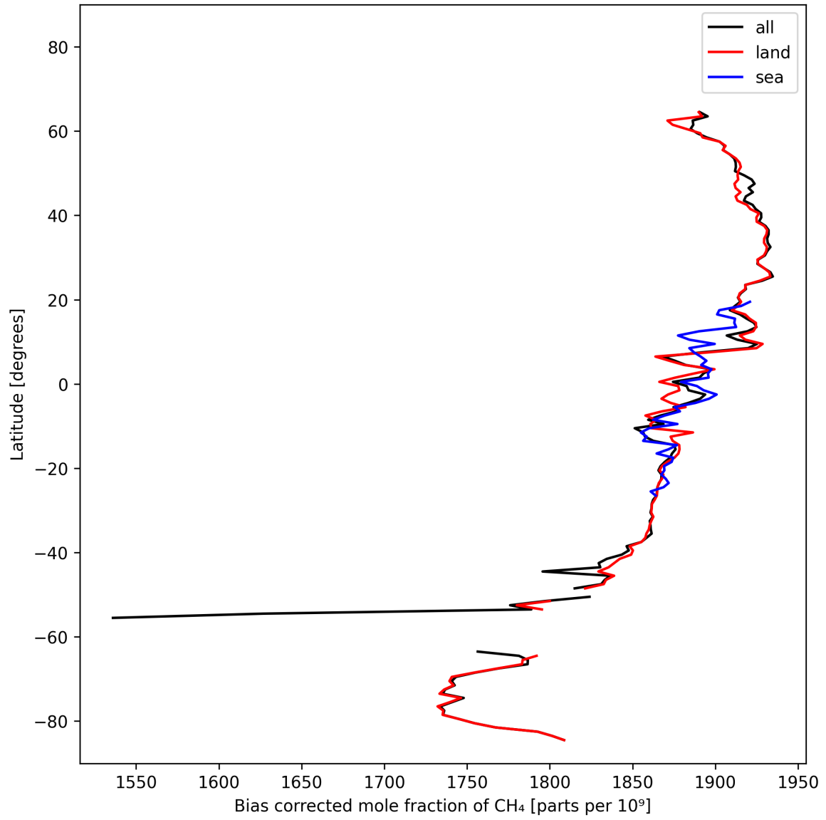
Figure 14: Zonal average of “Bias corrected mole fraction of CH 4 ” for 2024-10-19 to 2024-10-20.
