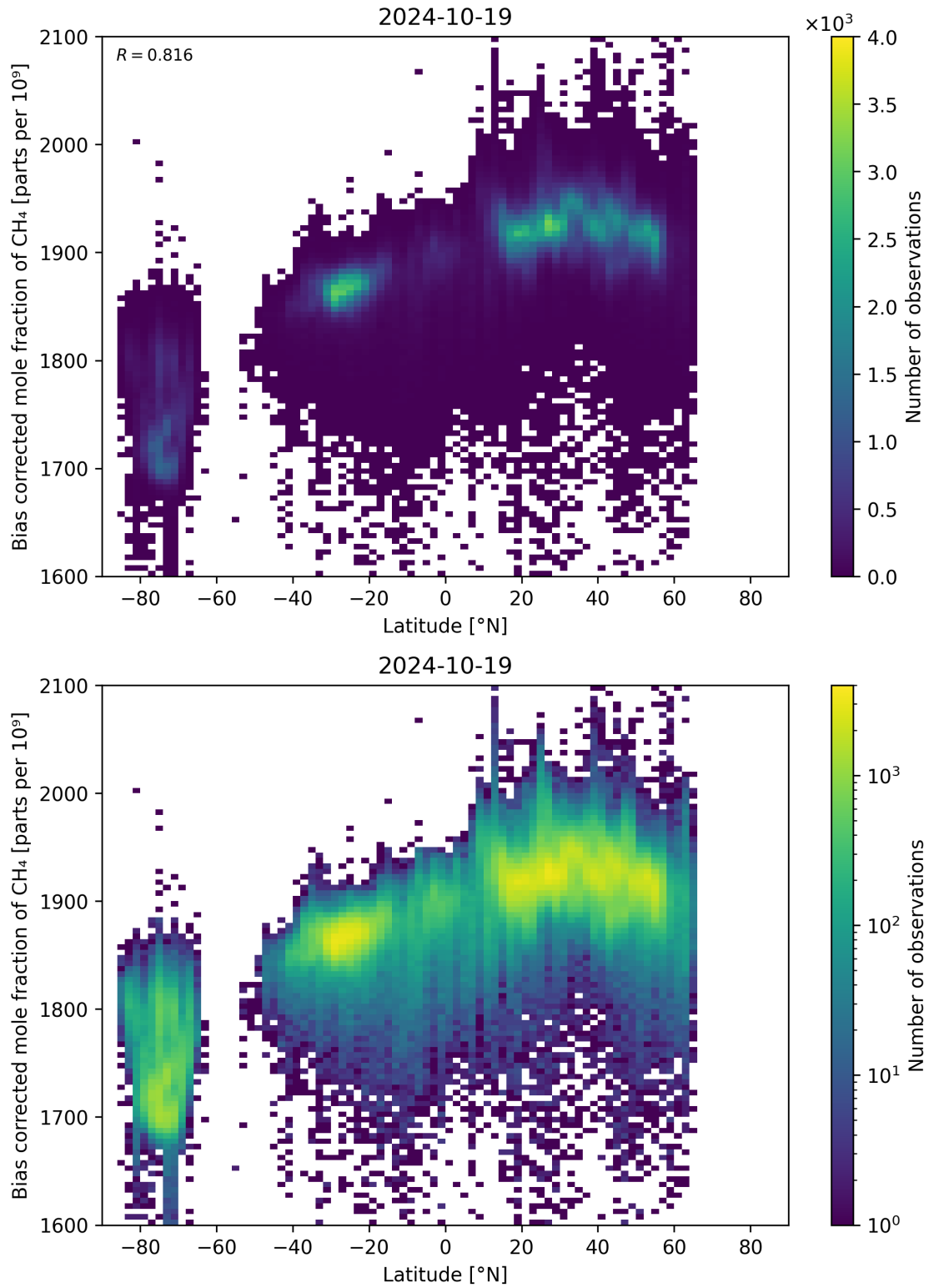
Figure 58: Scatter density plot of “Latitude” against “Bias corrected mole fraction of CH 4 ” for 2024-10-19 to 2024-10-20.
