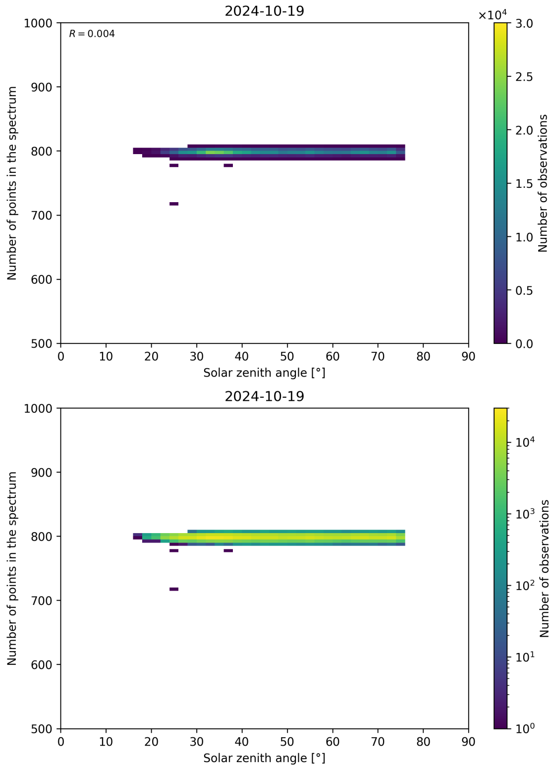
Figure 103: Scatter density plot of “Solar zenith angle” against “Number of points in the spectrum” for 2024-10-19 to 2024-10-20.
