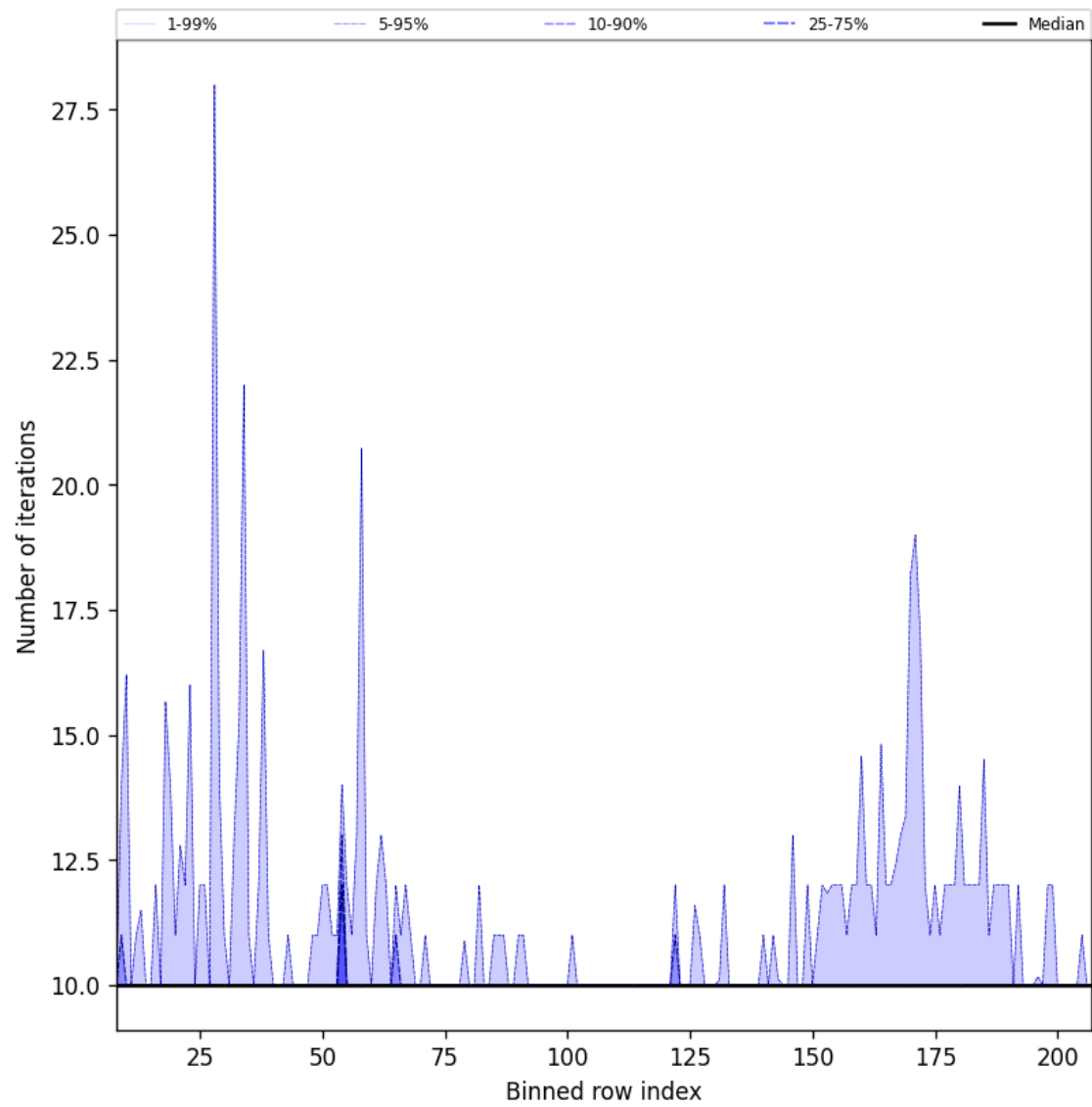
Figure 42: Along track statistics of “Number of iterations” for 2024-10-19 to 2024-10-20
