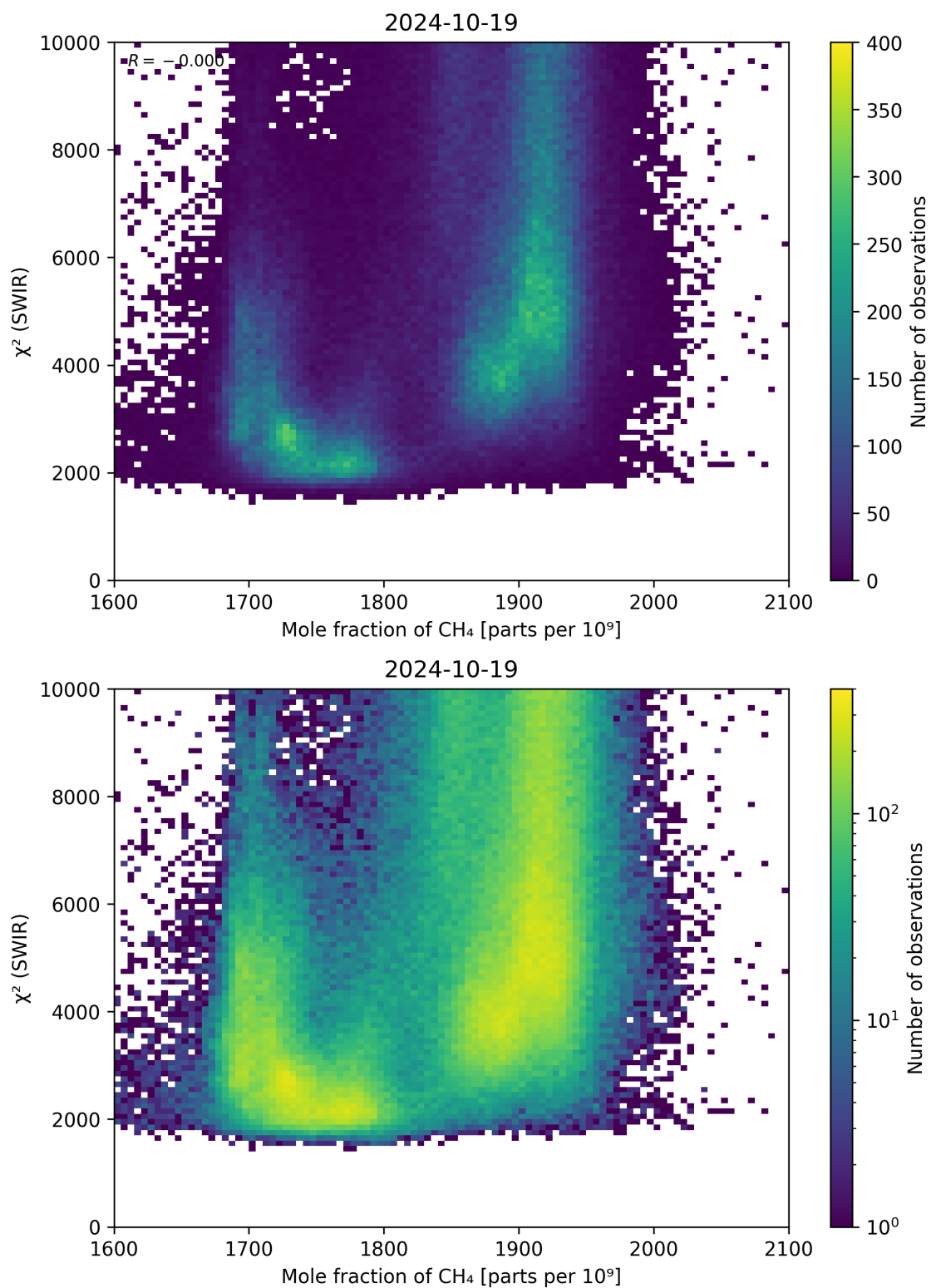
Figure 71: Scatter density plot of “Mole fraction of \text{CH}_4 ” against “ \chi^2 (SWIR)” for 2024-10-19 to 2024-10-20.
