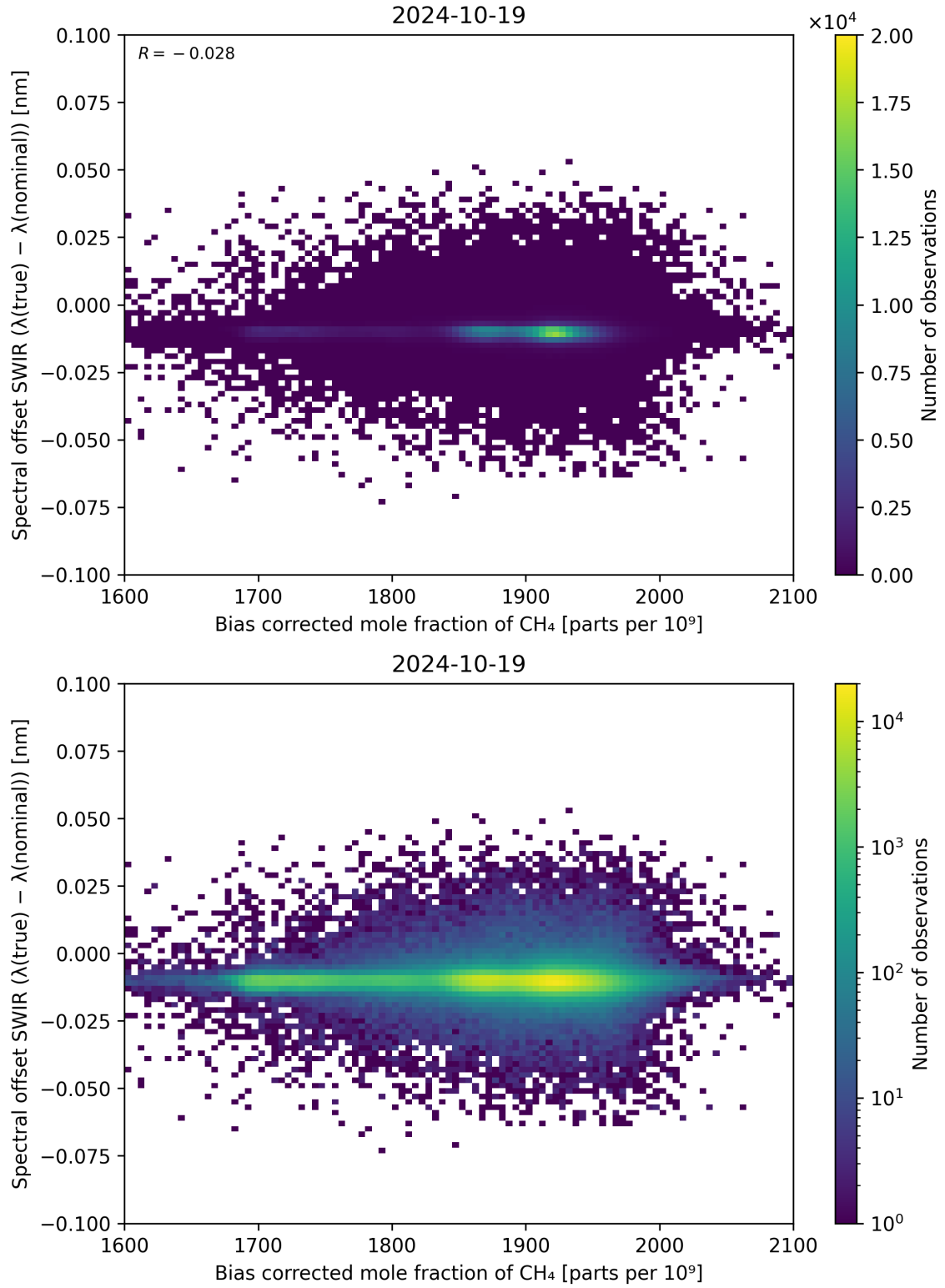
Figure 69: Scatter density plot of “Bias corrected mole fraction of \text{CH}_4 ” against “Spectral offset SWIR ( \lambda_{\text{true}} - \lambda_{\text{nominal}} )” for 2024-10-19 to 2024-10-20.
