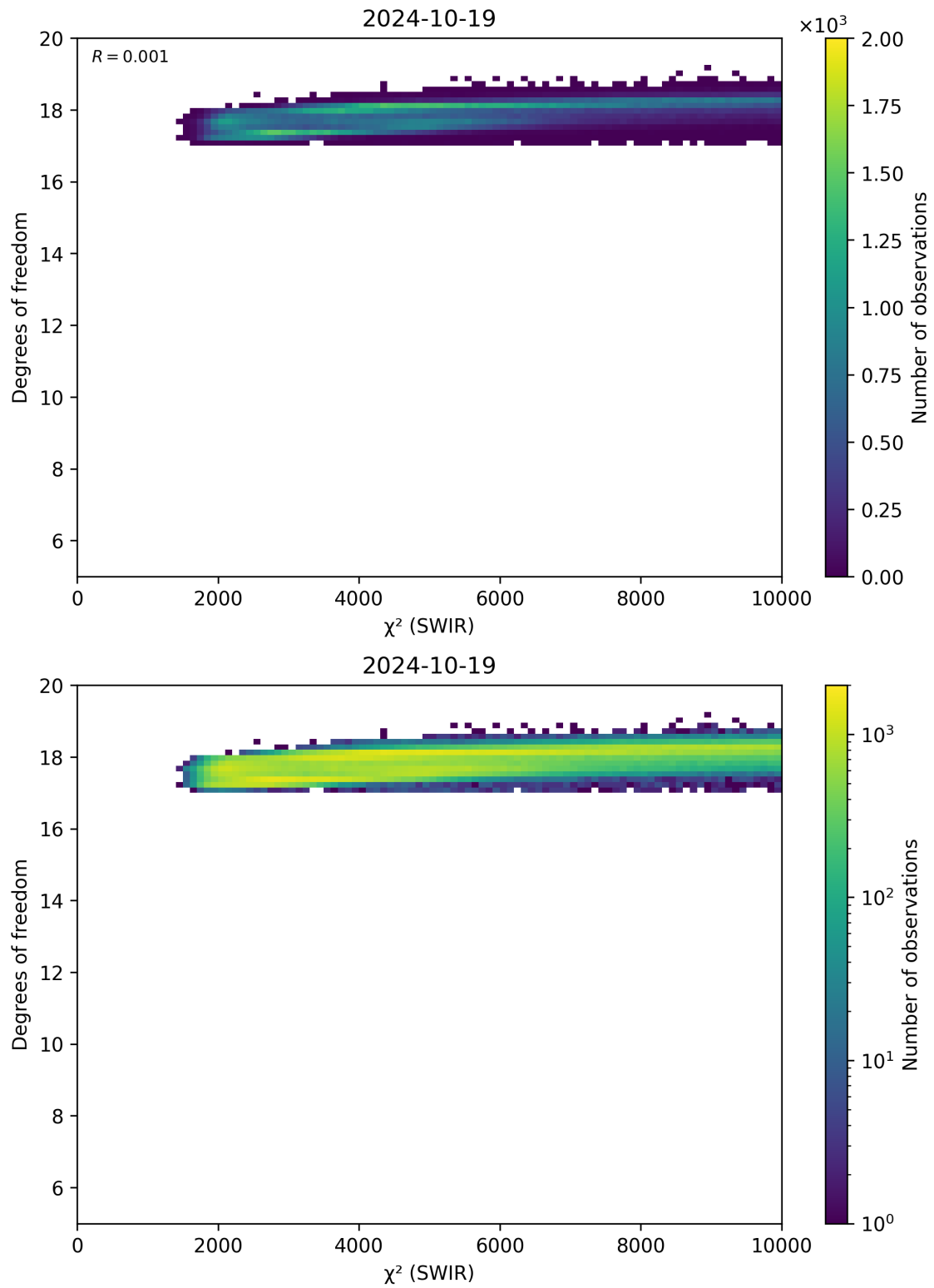
Figure 48: Scatter density plot of “ \chi^2 (SWIR)” against “Degrees of freedom” for 2024-10-19 to 2024-10-20.
