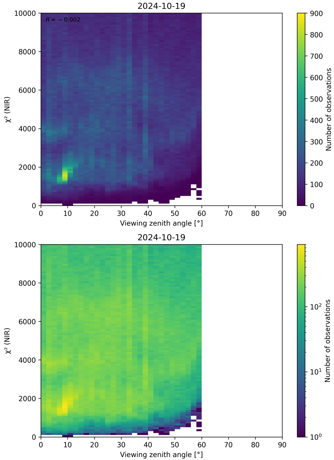
Figure 105: Scatter density plot of “Viewing zenith angle” against “ \chi^2 (NIR)” for 2024-10-19 to 2024-10-20.
