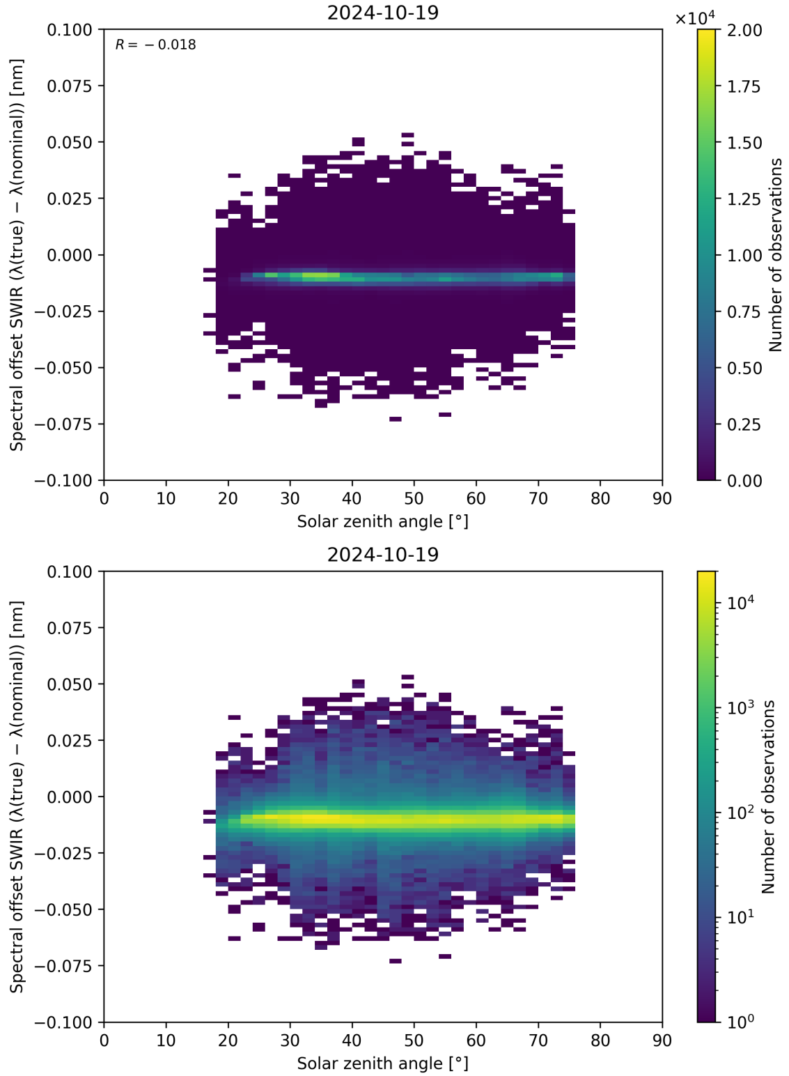
Figure 104: Scatter density plot of “Solar zenith angle” against “Spectral offset SWIR ( \lambda_{\text{true}} - \lambda_{\text{nominal}} )” for 2024-10-19 to 2024-10-20.
