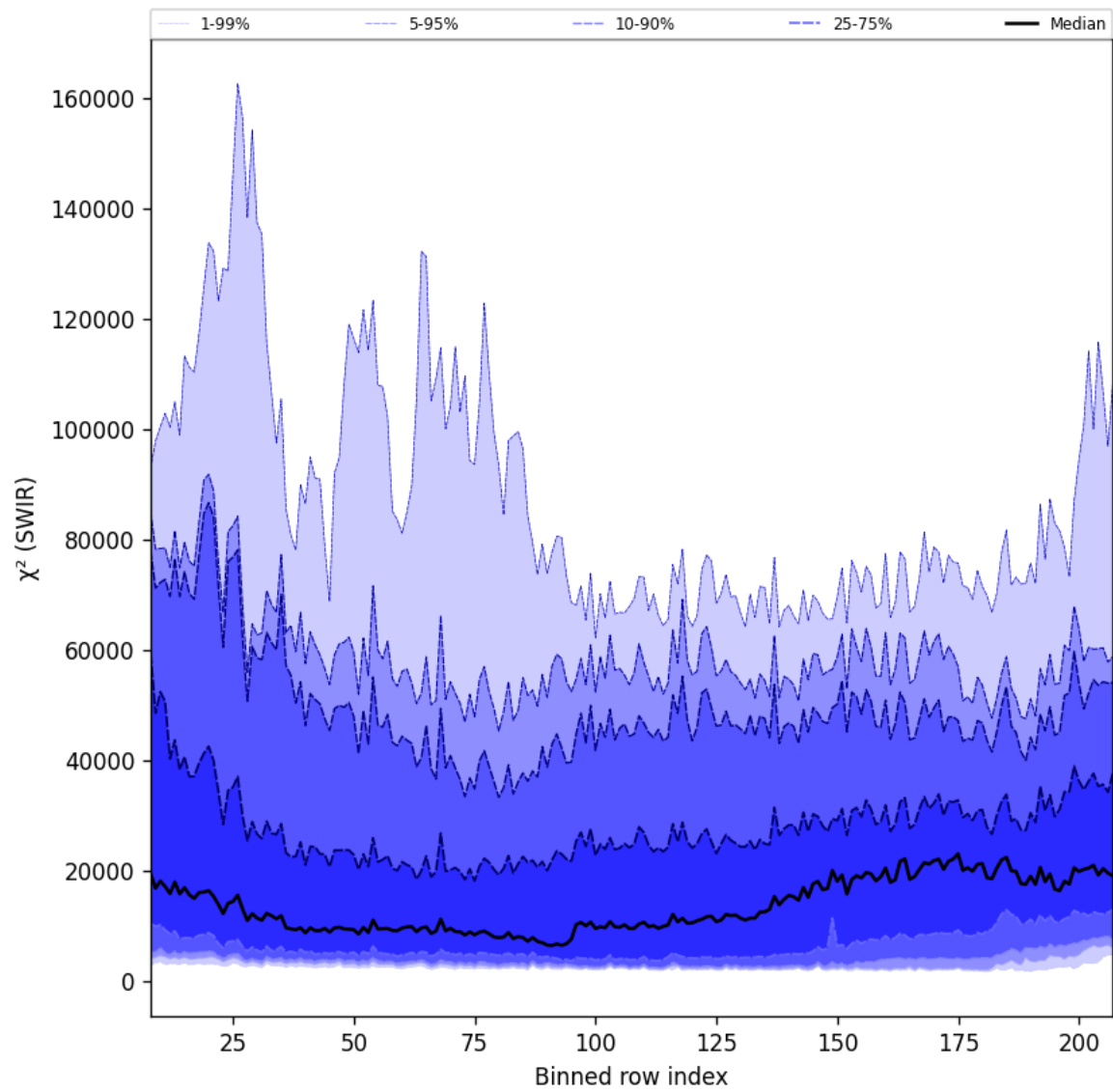
Figure 39: Along track statistics of “ \chi^2 (SWIR)” for 2024-10-19 to 2024-10-20
