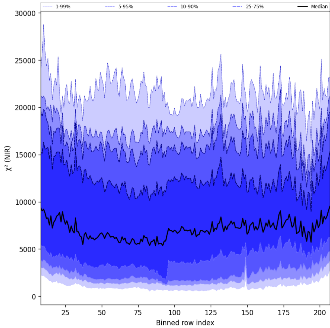
Figure 40: Along track statistics of “ \chi^2 (NIR)” for 2024-10-19 to 2024-10-20
