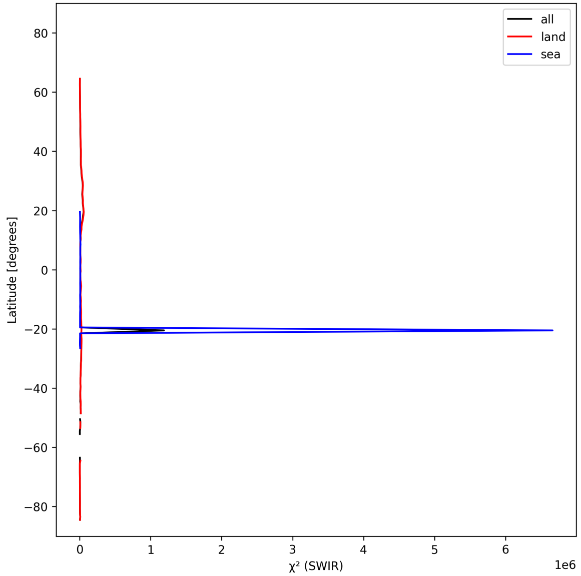
Figure 17: Zonal average of “ \chi^2 (SWIR)” for 2024-10-19 to 2024-10-20.
