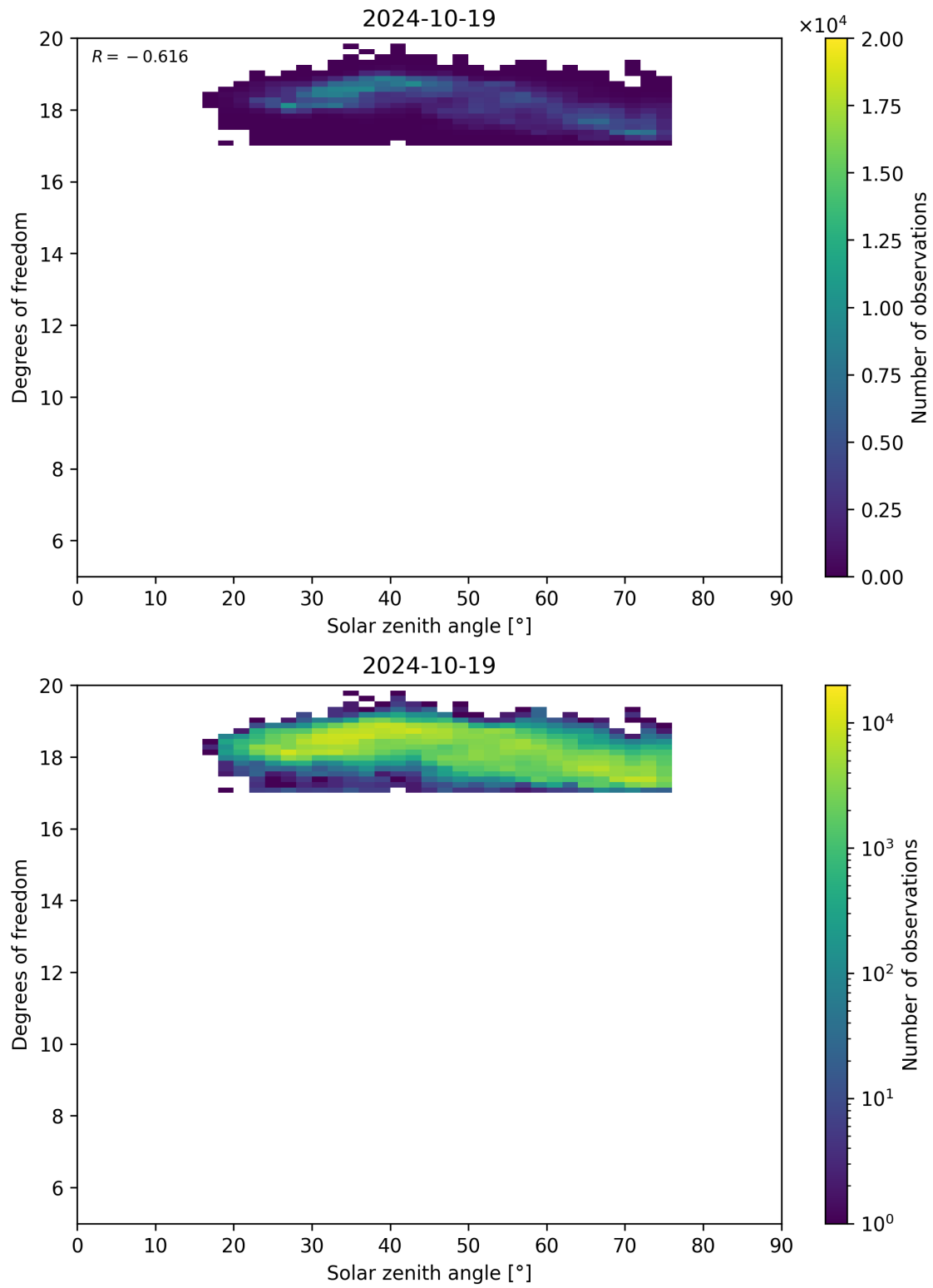
Figure 96: Scatter density plot of “Solar zenith angle” against “Degrees of freedom” for 2024-10-19 to 2024-10-20.
