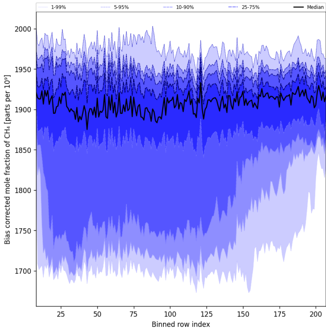
Figure 36: Along track statistics of “Bias corrected mole fraction of CH 4 ” for 2024-10-19 to 2024-10-20
