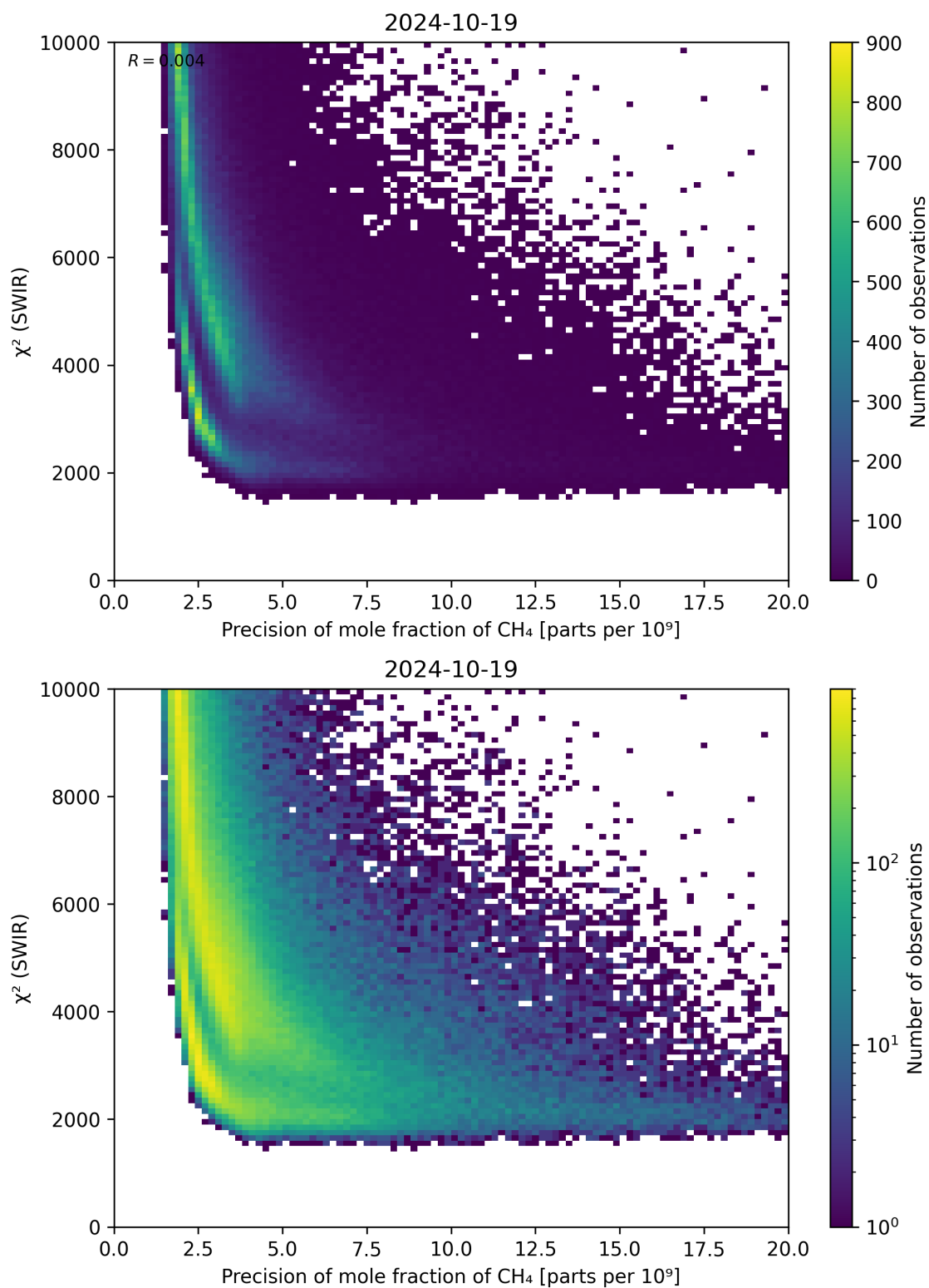
Figure 79: Scatter density plot of “Precision of mole fraction of CH 4 ” against “ \chi^2 (SWIR)” for 2024-10-19 to 2024-10-20.
