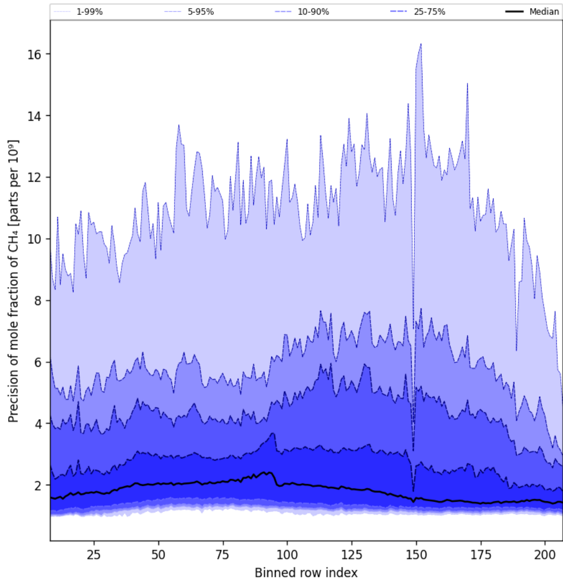
Figure 35: Along track statistics of “Precision of mole fraction of \text{CH}_4 ” for 2024-10-19 to 2024-10-20
