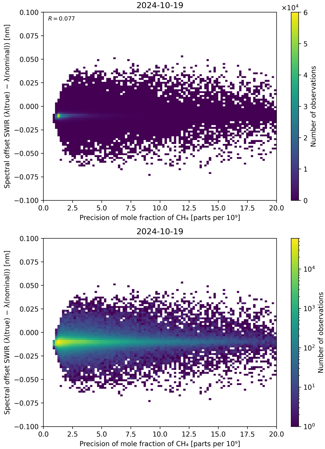
Figure 85: Scatter density plot of “Precision of mole fraction of CH 4 ” against “Spectral offset SWIR ( \lambda_{\text{true}} - \lambda_{\text{nominal}} )” for 2024-10-19 to 2024-10-20.
