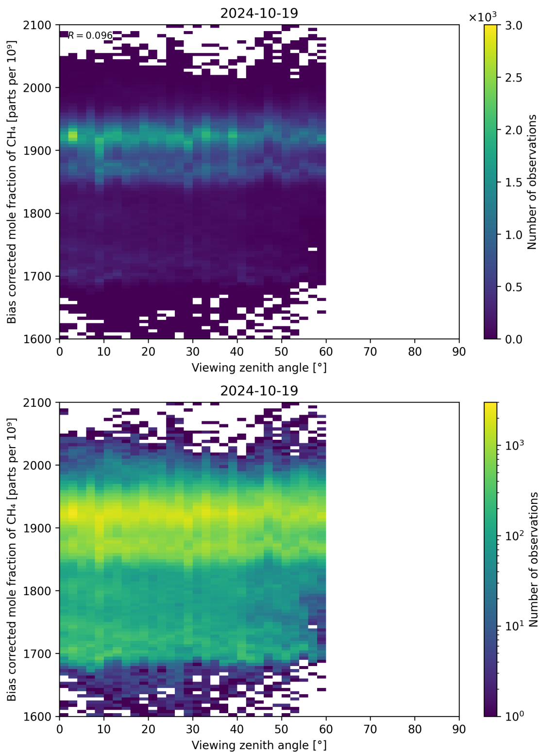
Figure 111: Scatter density plot of “Viewing zenith angle” against “Bias corrected mole fraction of CH 4 ” for 2024-10-19 to 2024-10-20.
