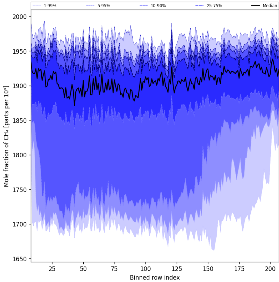
Figure 34: Along track statistics of “Mole fraction of CH 4 ” for 2024-10-19 to 2024-10-20
