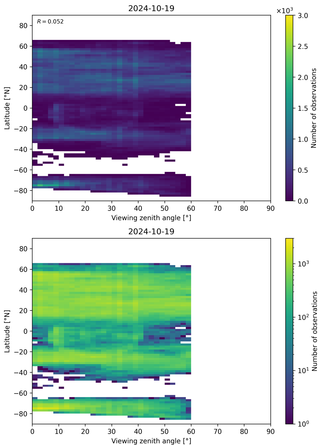
Figure 109: Scatter density plot of “Viewing zenith angle” against “Latitude” for 2024-10-19 to 2024-10-20.
