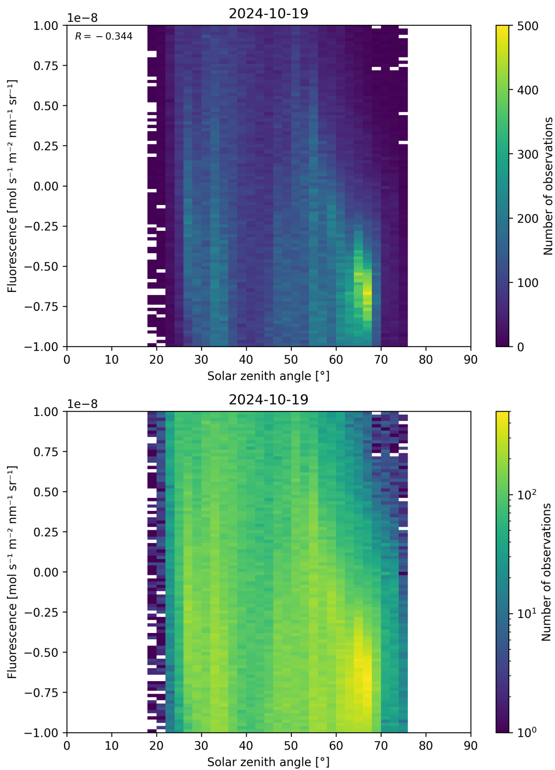
Figure 97: Scatter density plot of “Solar zenith angle” against “Fluorescence” for 2024-10-19 to 2024-10-20.
