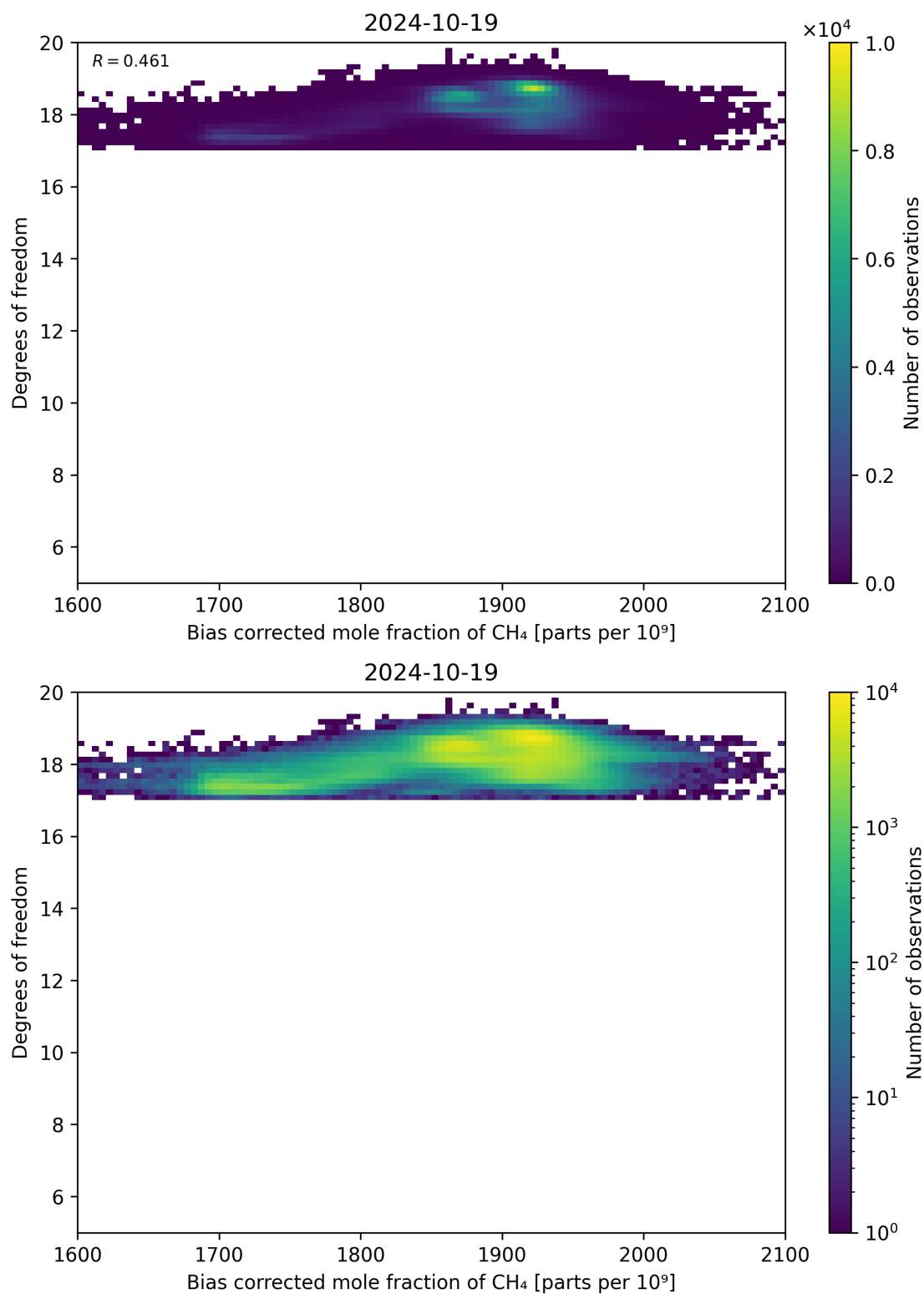
Figure 65: Scatter density plot of “Bias corrected mole fraction of \text{CH}_4 ” against “Degrees of freedom” for 2024-10-19 to 2024-10-20.
