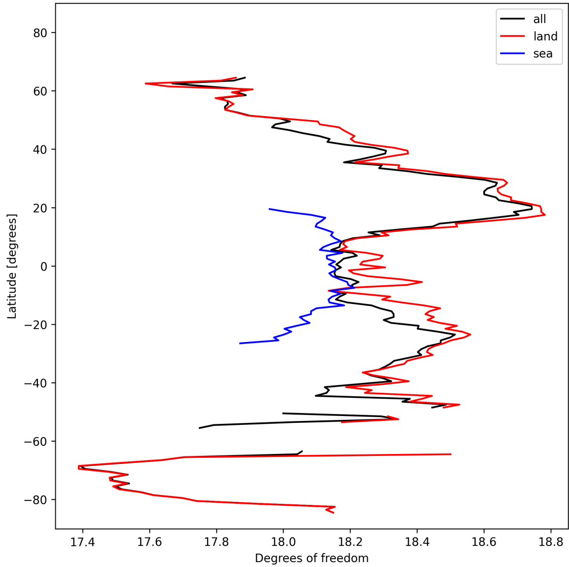
Figure 19: Zonal average of “Degrees of freedom” for 2024-10-19 to 2024-10-20.
