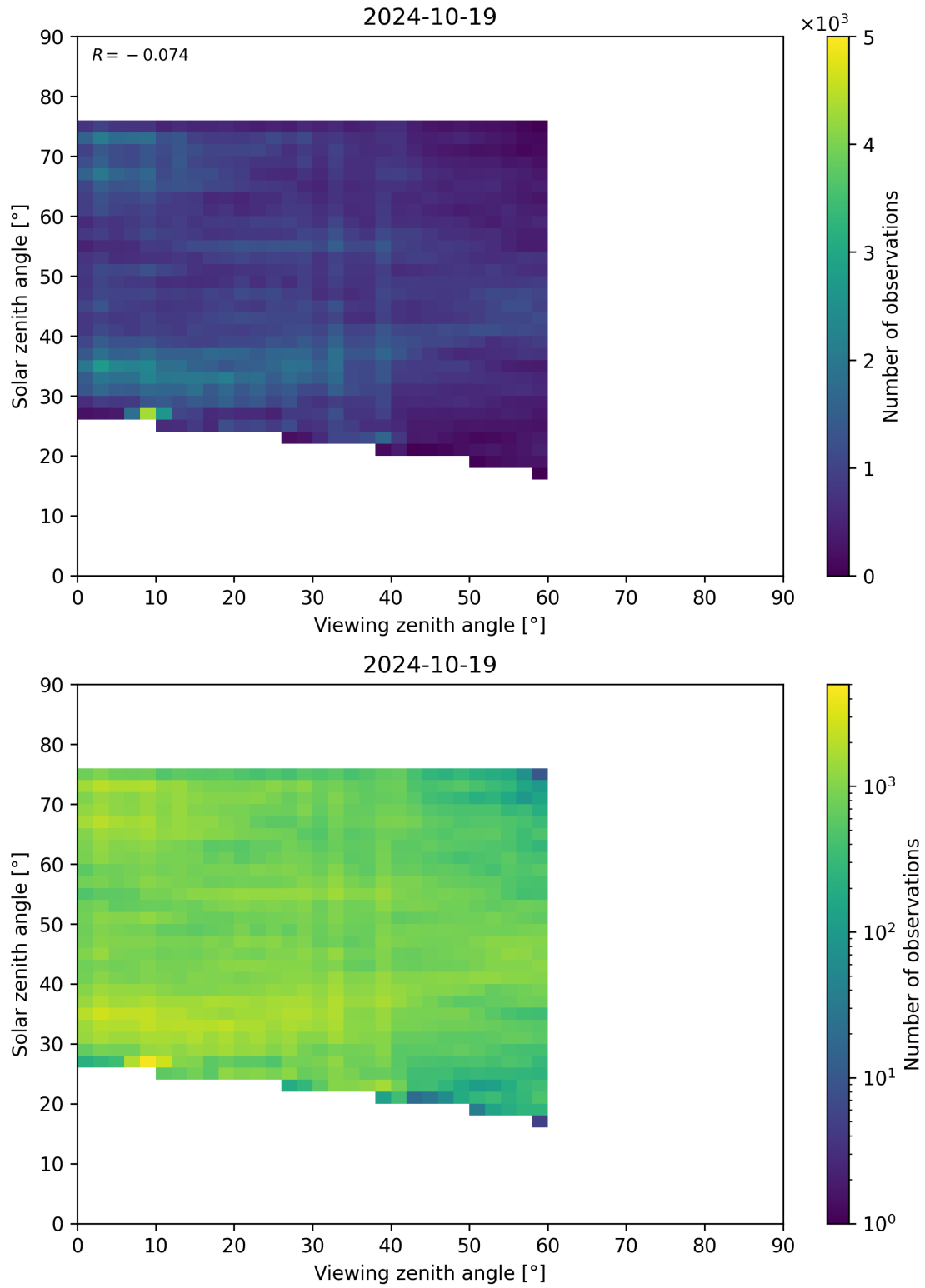
Figure 115: Scatter density plot of “Viewing zenith angle” against “Solar zenith angle” for 2024-10-19 to 2024-10-20.
