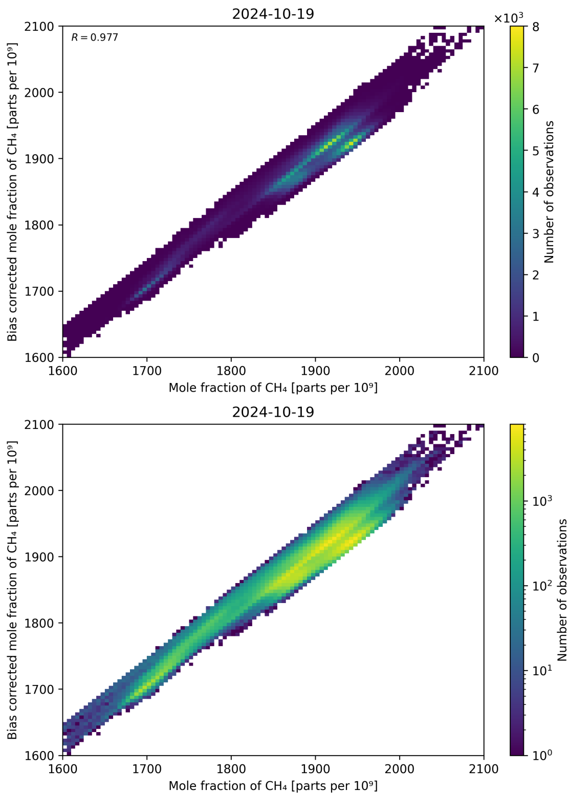
Figure 74: Scatter density plot of “Mole fraction of CH 4 ” against “Bias corrected mole fraction of CH 4 ” for 2024-10-19 to 2024-10-20.
