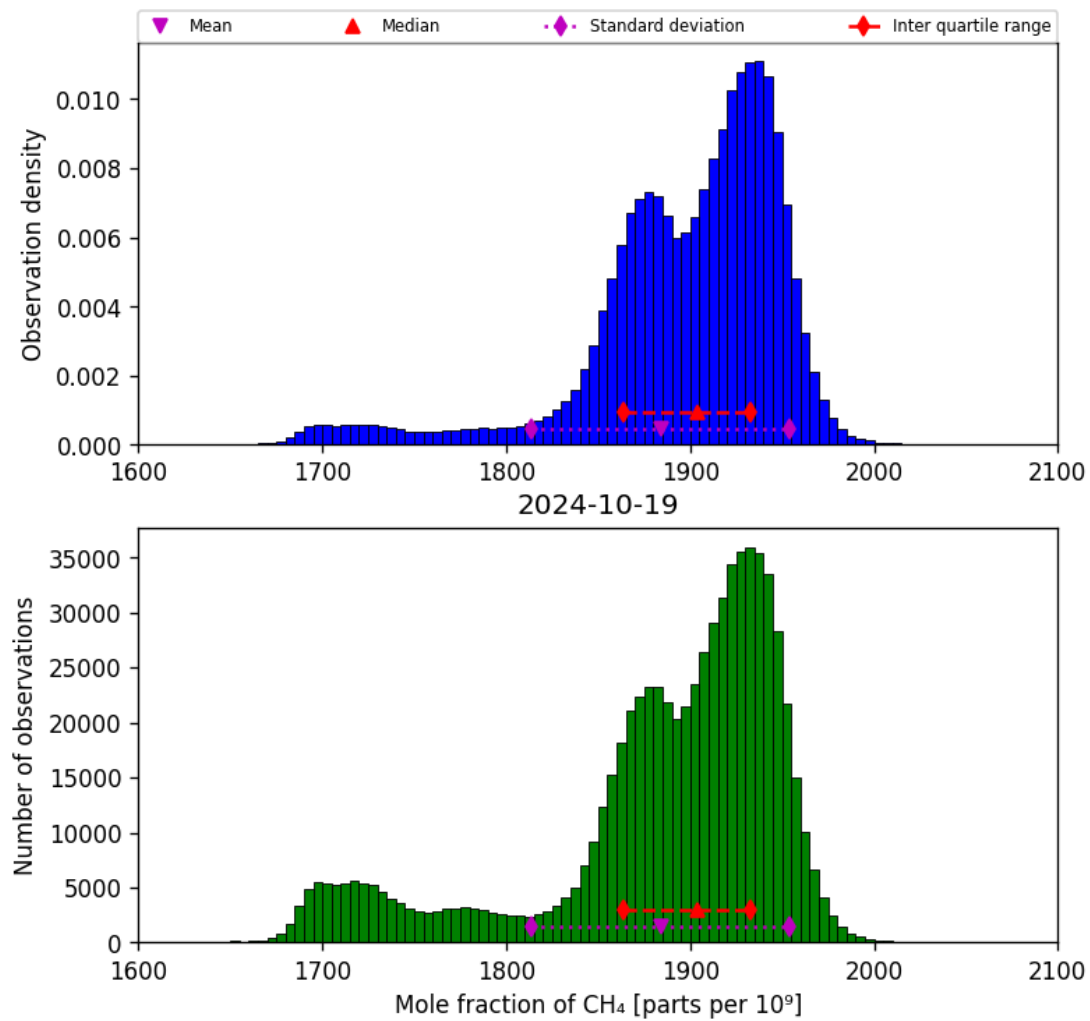
Figure 23: Histogram of “Mole fraction of CH 4 ” for 2024-10-19 to 2024-10-20
