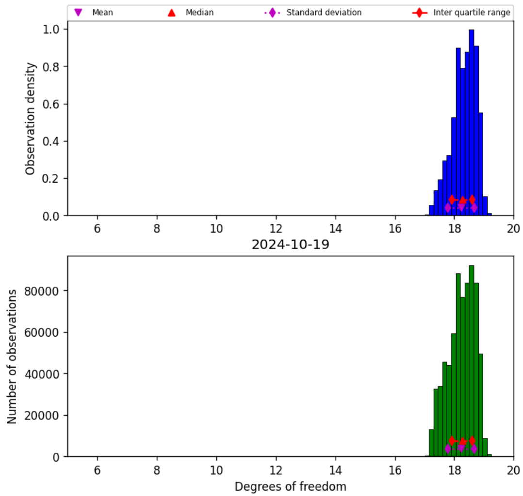
Figure 30: Histogram of “Degrees of freedom” for 2024-10-19 to 2024-10-20
