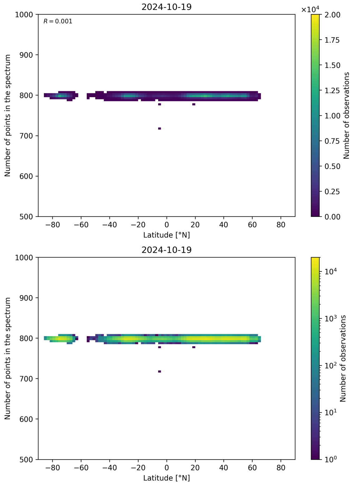
Figure 61: Scatter density plot of “Latitude” against “Number of points in the spectrum” for 2024-10-19 to 2024-10-20.
