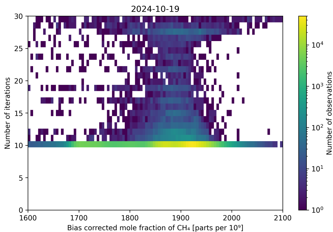
Figure 67: Scatter density plot of “Bias corrected mole fraction of CH 4 ” against “Number of iterations” for 2024-10-19 to 2024-10-20.
