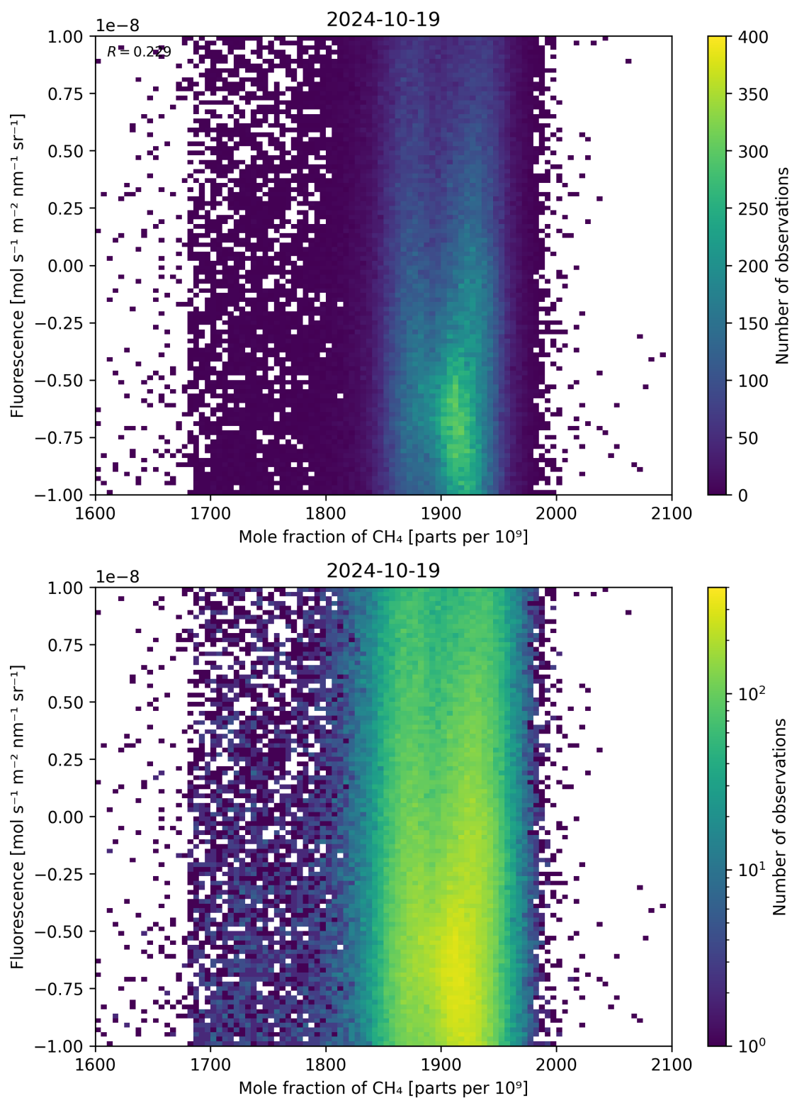
Figure 73: Scatter density plot of “Mole fraction of \text{CH}_4 ” against “Fluorescence” for 2024-10-19 to 2024-10-20.
