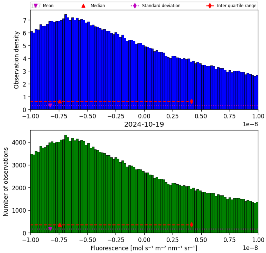
Figure 32: Histogram of “Fluorescence” for 2024-10-19 to 2024-10-20
