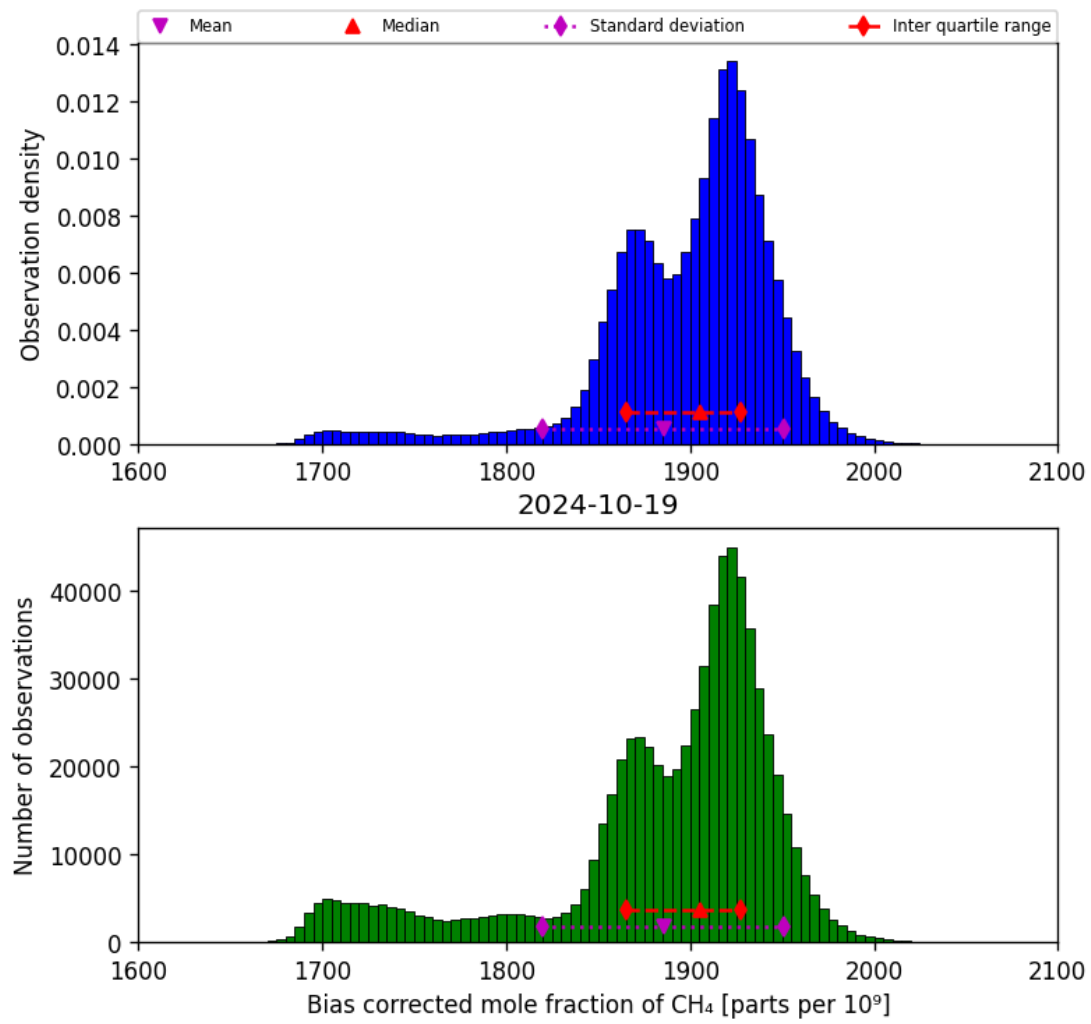
Figure 25: Histogram of “Bias corrected mole fraction of CH 4 ” for 2024-10-19 to 2024-10-20
