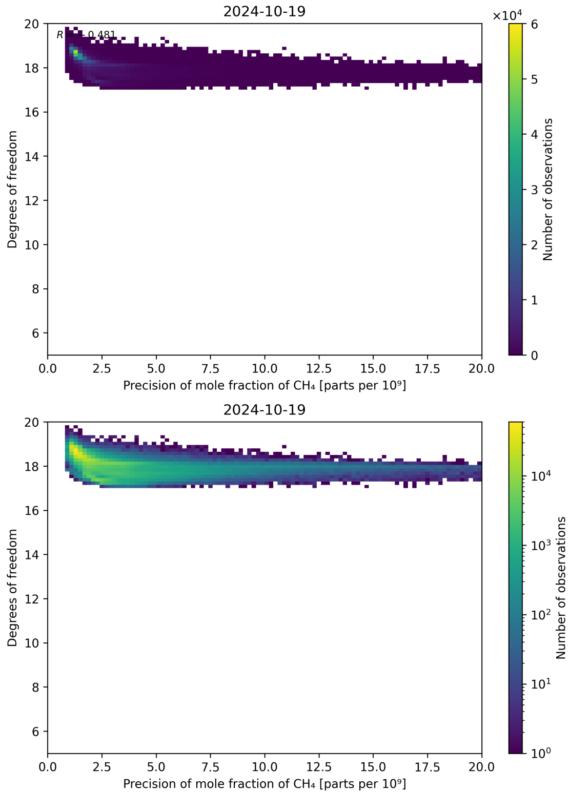
Figure 80: Scatter density plot of “Precision of mole fraction of CH 4 ” against “Degrees of freedom” for 2024-10-19 to 2024-10-20.
