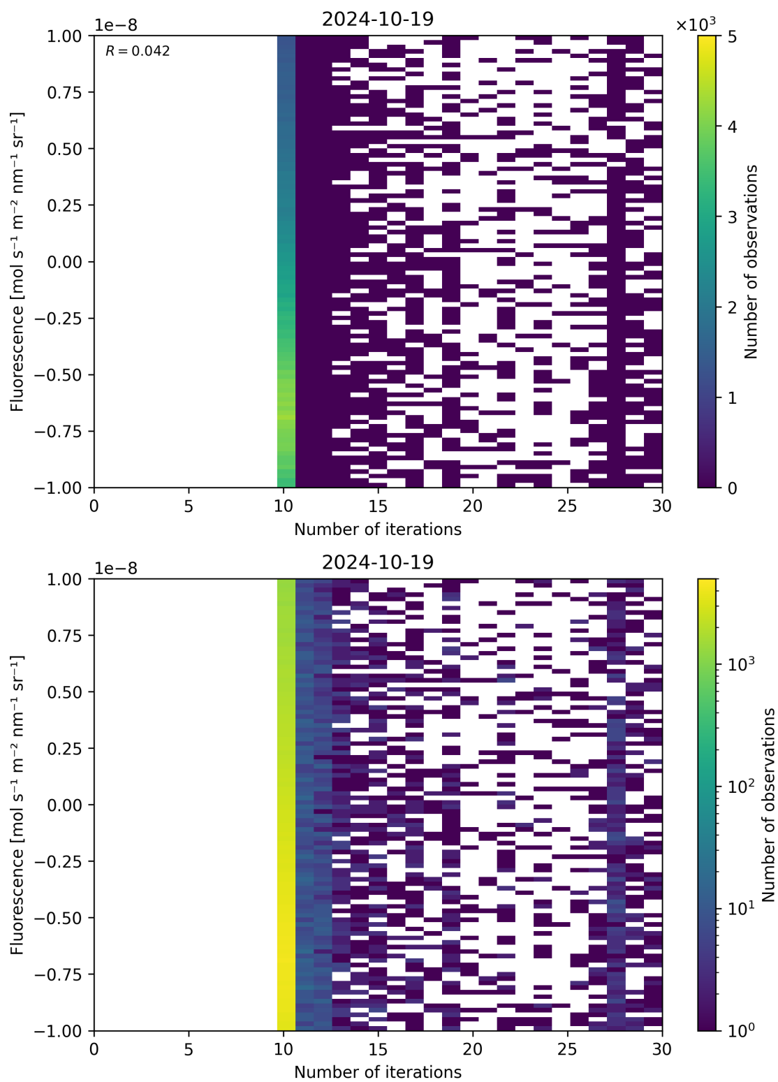
Figure 87: Scatter density plot of “Number of iterations” against “Fluorescence” for 2024-10-19 to 2024-10-20.
