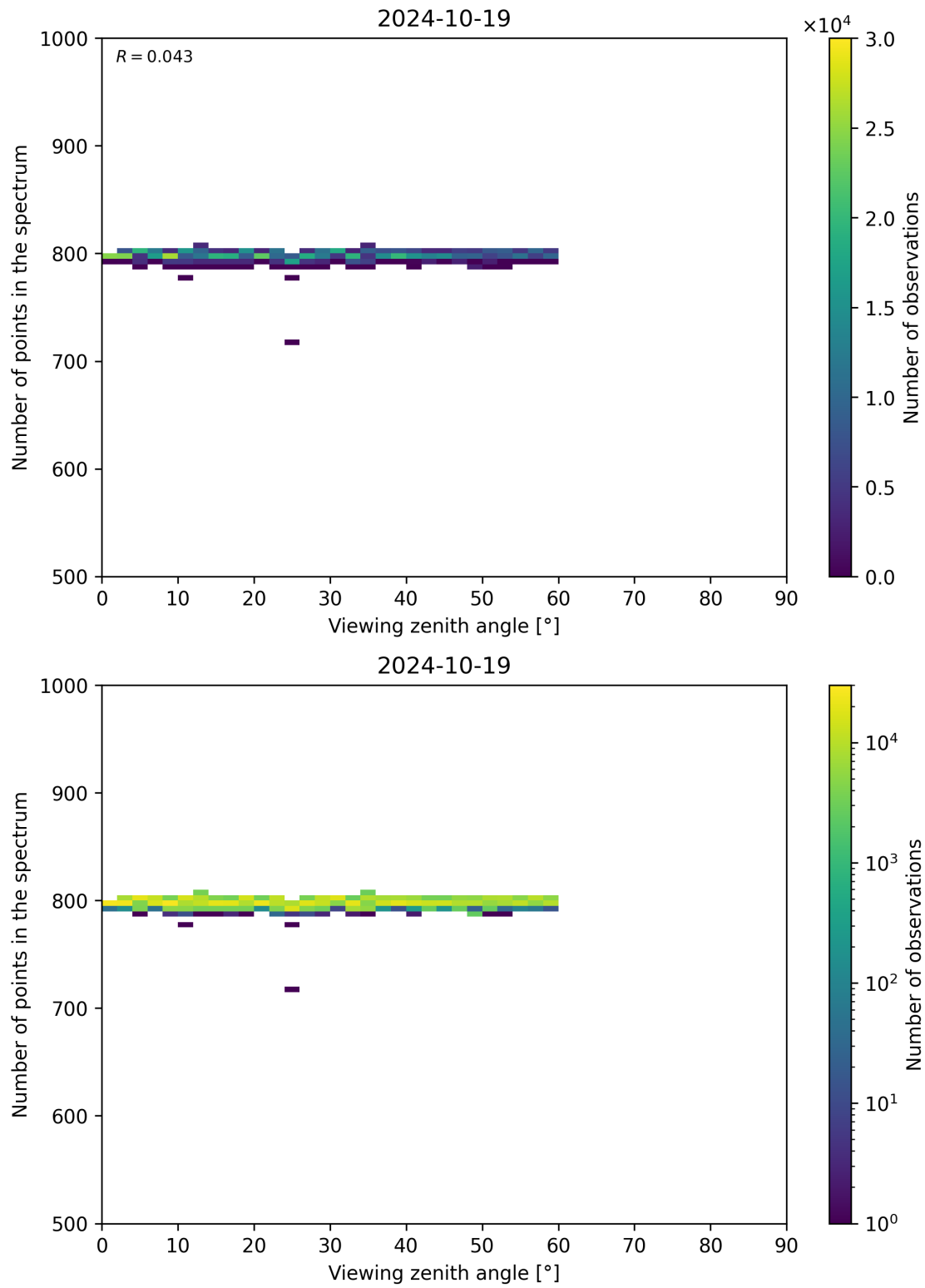
Figure 114: Scatter density plot of “Viewing zenith angle” against “Number of points in the spectrum” for 2024-10-19 to 2024-10-20.
