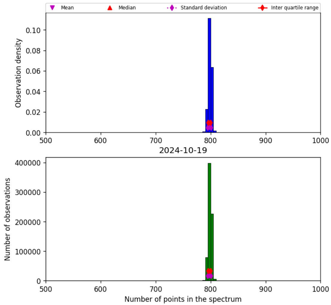
Figure 26: Histogram of “Number of points in the spectrum” for 2024-10-19 to 2024-10-20
