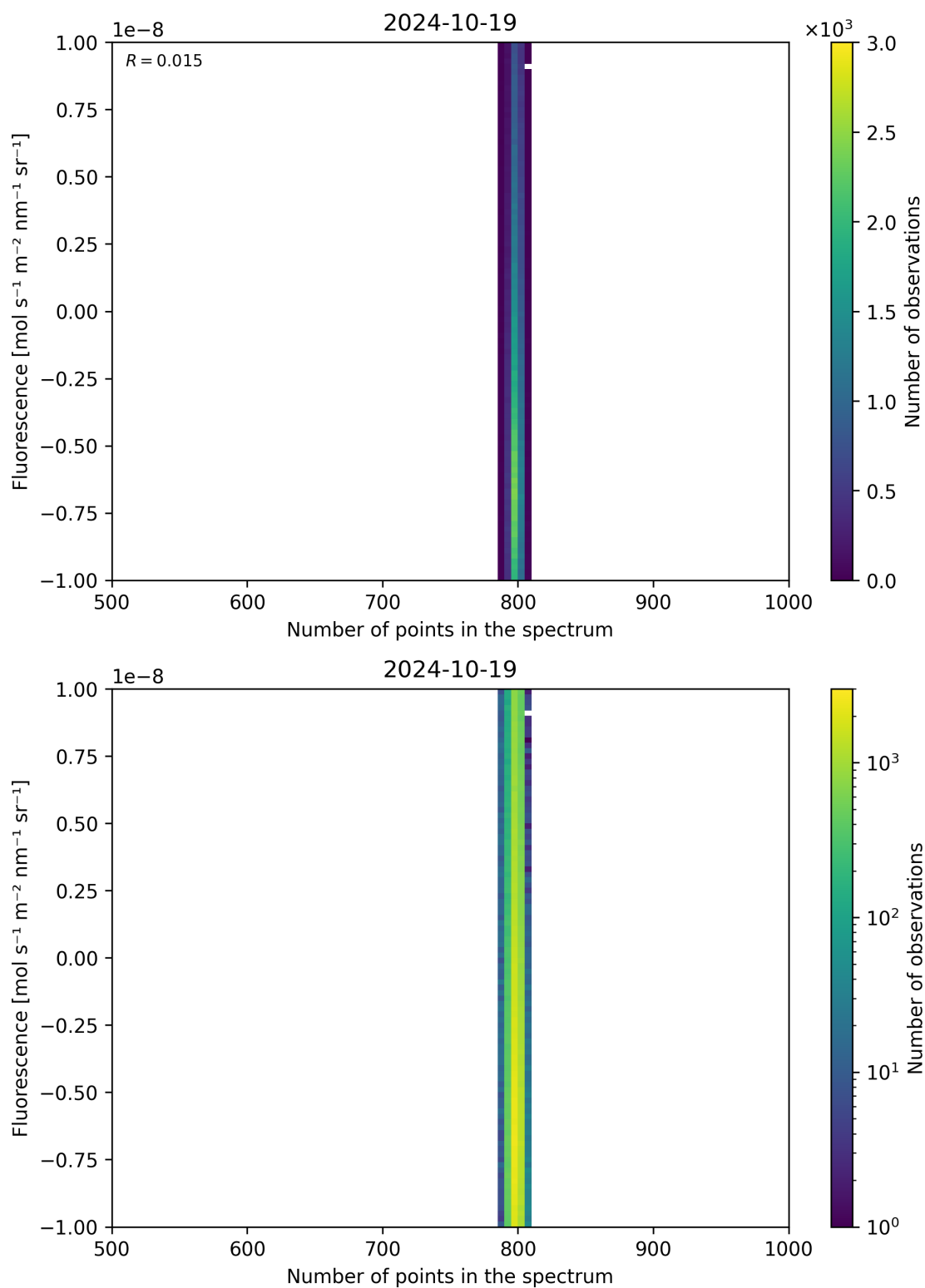
Figure 91: Scatter density plot of “Number of points in the spectrum” against “Fluorescence” for 2024-10-19 to 2024-10-20.
