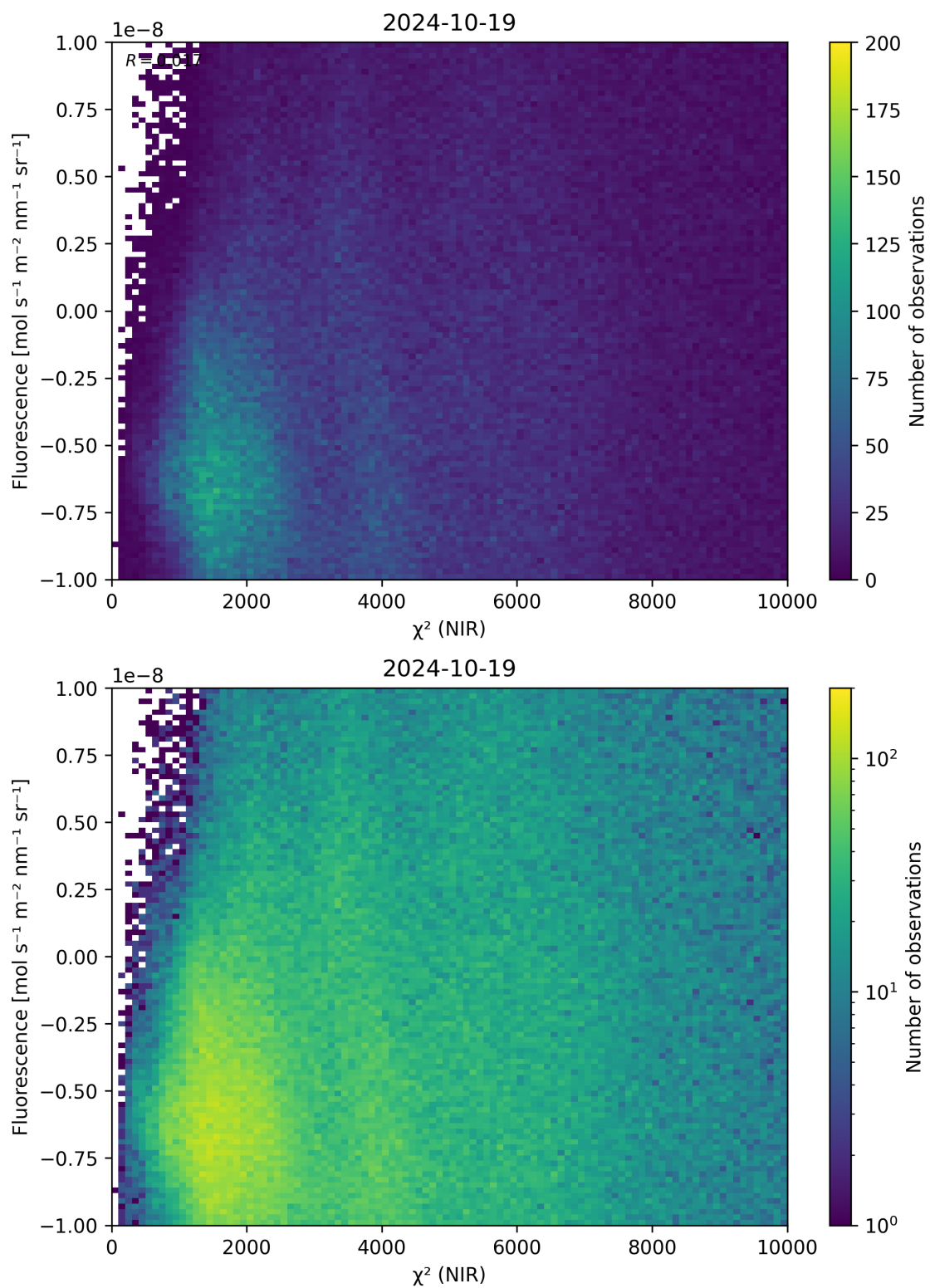
Figure 45: Scatter density plot of “ \chi^2 (NIR)” against “Fluorescence” for 2024-10-19 to 2024-10-20.
