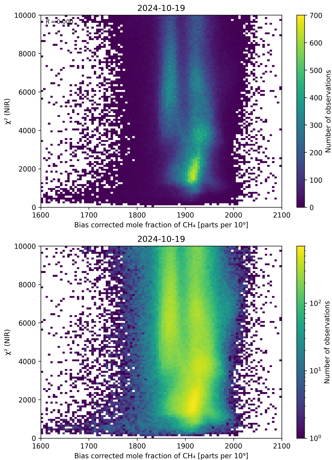
Figure 63: Scatter density plot of “Bias corrected mole fraction of CH 4 ” against “ \chi^2 (NIR)” for 2024-10-19 to 2024-10-20.
