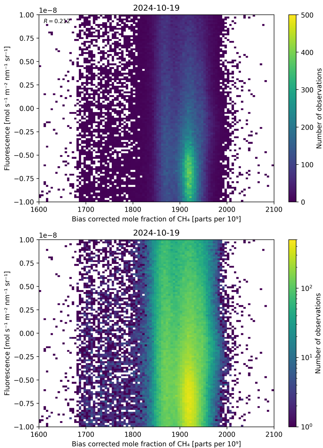
Figure 66: Scatter density plot of “Bias corrected mole fraction of \text{CH}_4 ” against “Fluorescence” for 2024-10-19 to 2024-10-20.
