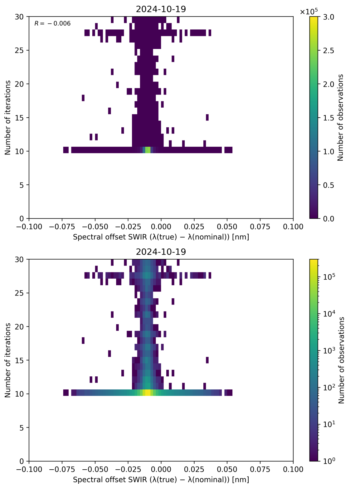
Figure 121: Scatter density plot of “Spectral offset SWIR ( \lambda_{\text{true}} - \lambda_{\text{nominal}} )” against “Number of iterations” for 2024-10-19 to 2024-10-20.
