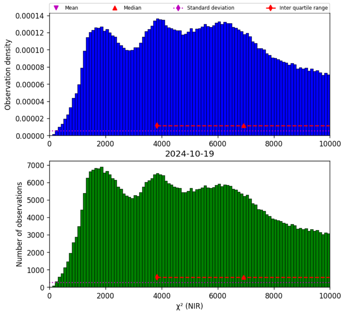
Figure 29: Histogram of “ \chi^2 (NIR)” for 2024-10-19 to 2024-10-20
