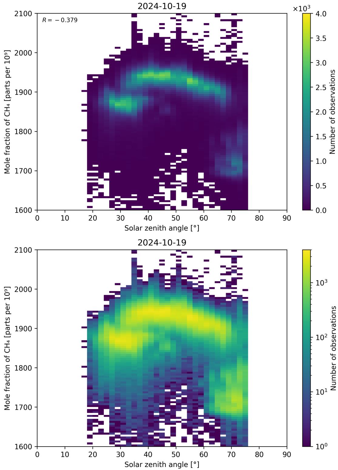
Figure 99: Scatter density plot of “Solar zenith angle” against “Mole fraction of CH 4 ” for 2024-10-19 to 2024-10-20.
