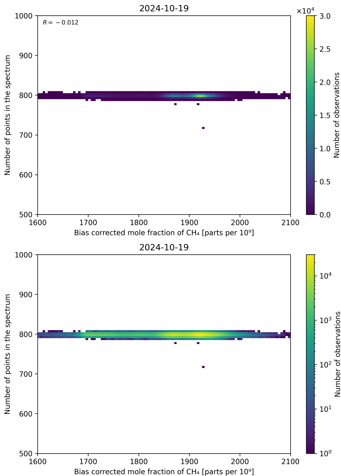
Figure 68: Scatter density plot of “Bias corrected mole fraction of CH 4 ” against “Number of points in the spectrum” for 2024-10-19 to 2024-10-20.
