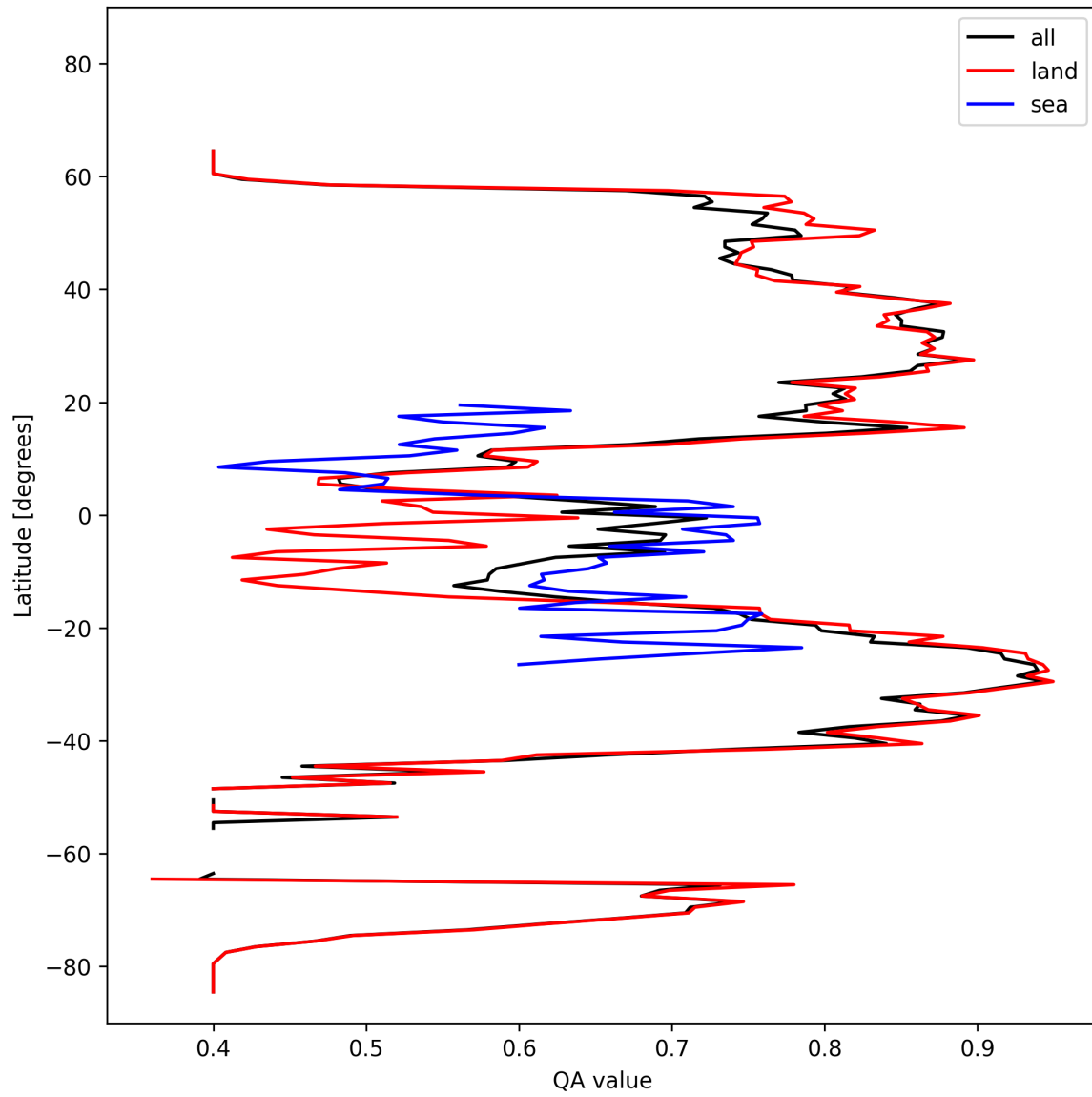
Figure 11: Zonal average of “QA value” for 2024-10-19 to 2024-10-20.
