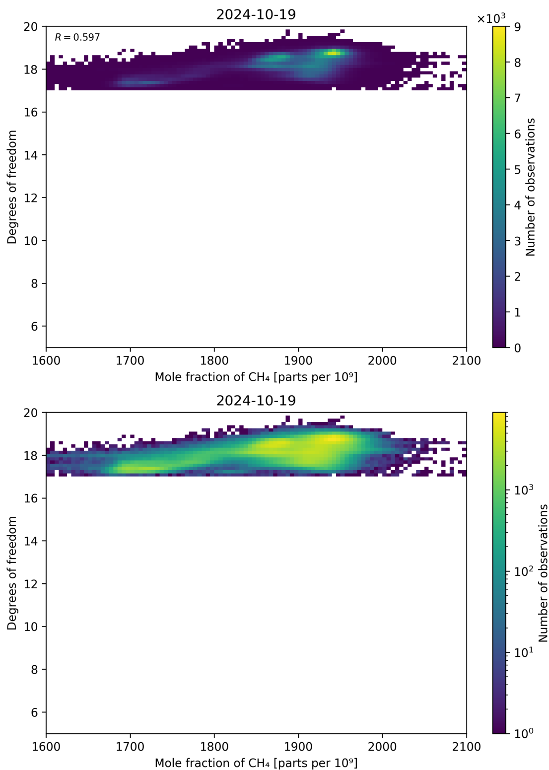
Figure 72: Scatter density plot of “Mole fraction of CH 4 ” against “Degrees of freedom” for 2024-10-19 to 2024-10-20.
