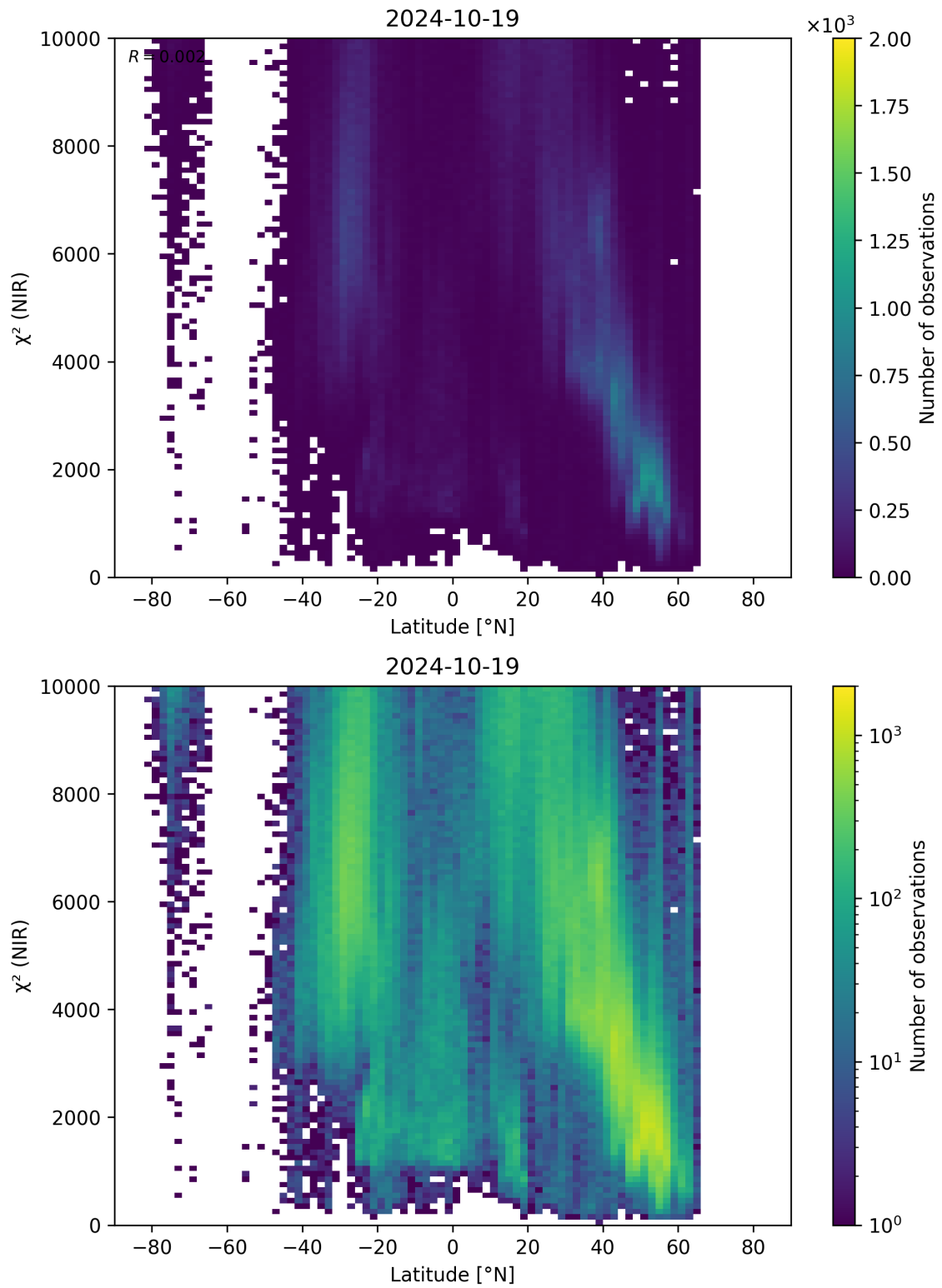
Figure 53: Scatter density plot of “Latitude” against “ \chi^2 (NIR)” for 2024-10-19 to 2024-10-20.
