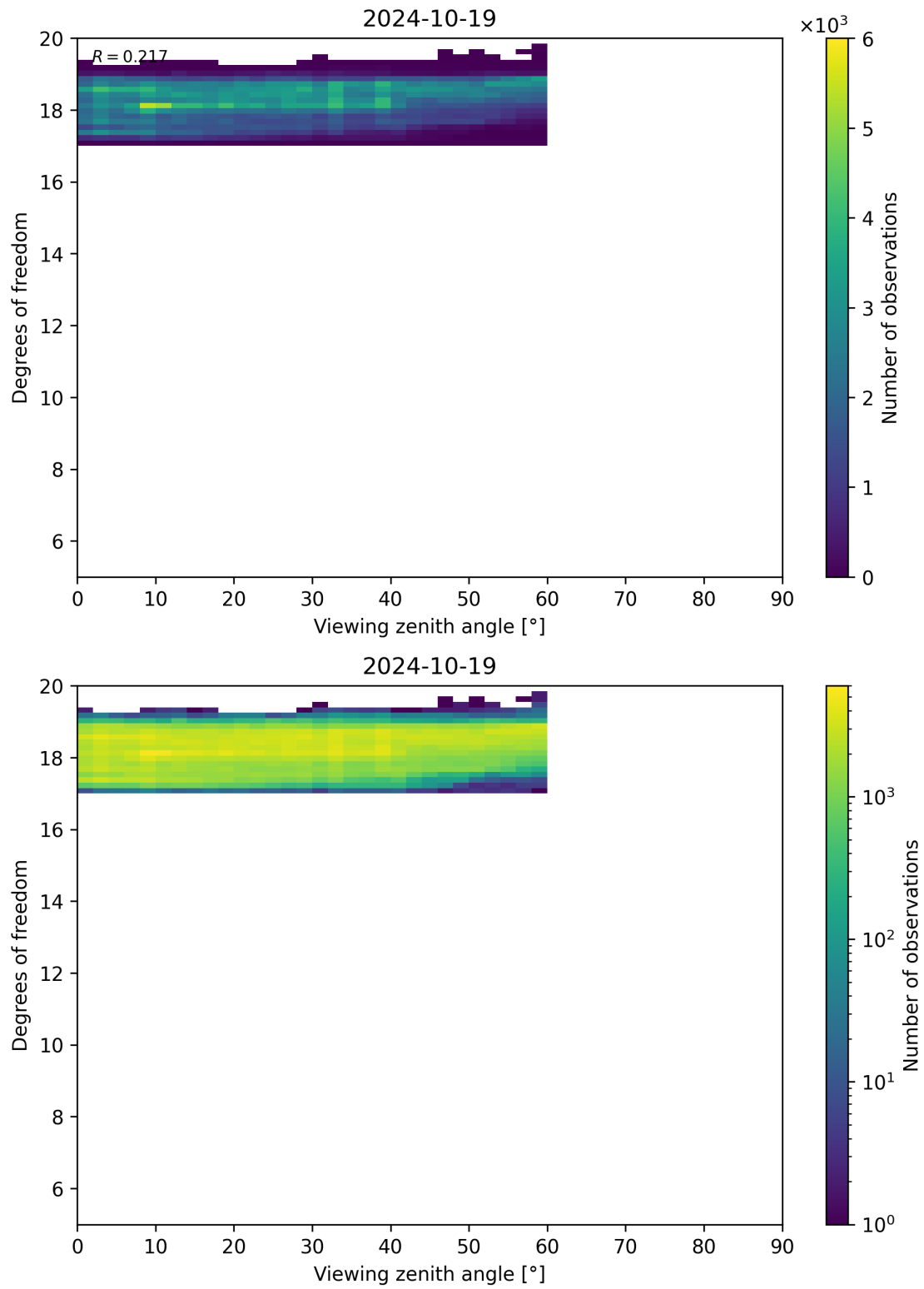
Figure 107: Scatter density plot of “Viewing zenith angle” against “Degrees of freedom” for 2024-10-19 to 2024-10-20.
