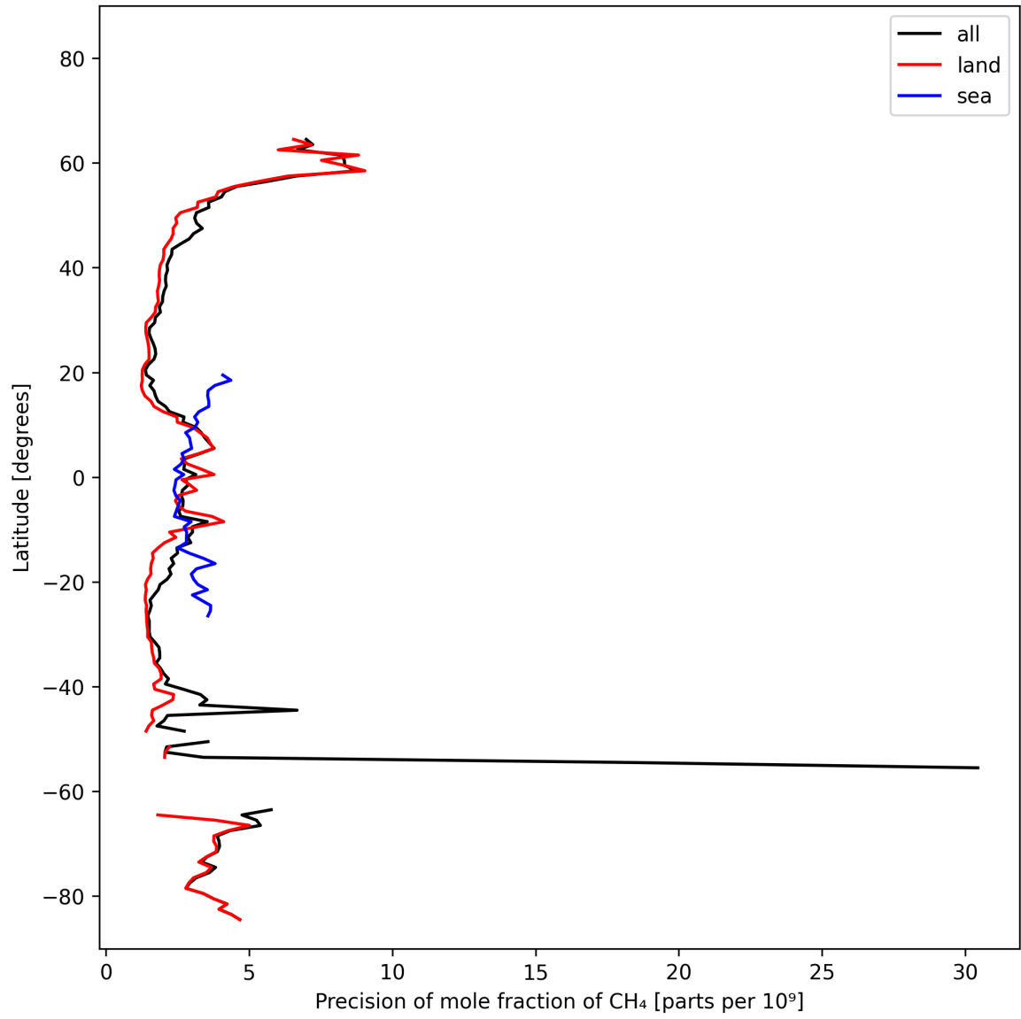
Figure 13: Zonal average of “Precision of mole fraction of CH 4 ” for 2024-10-19 to 2024-10-20.
