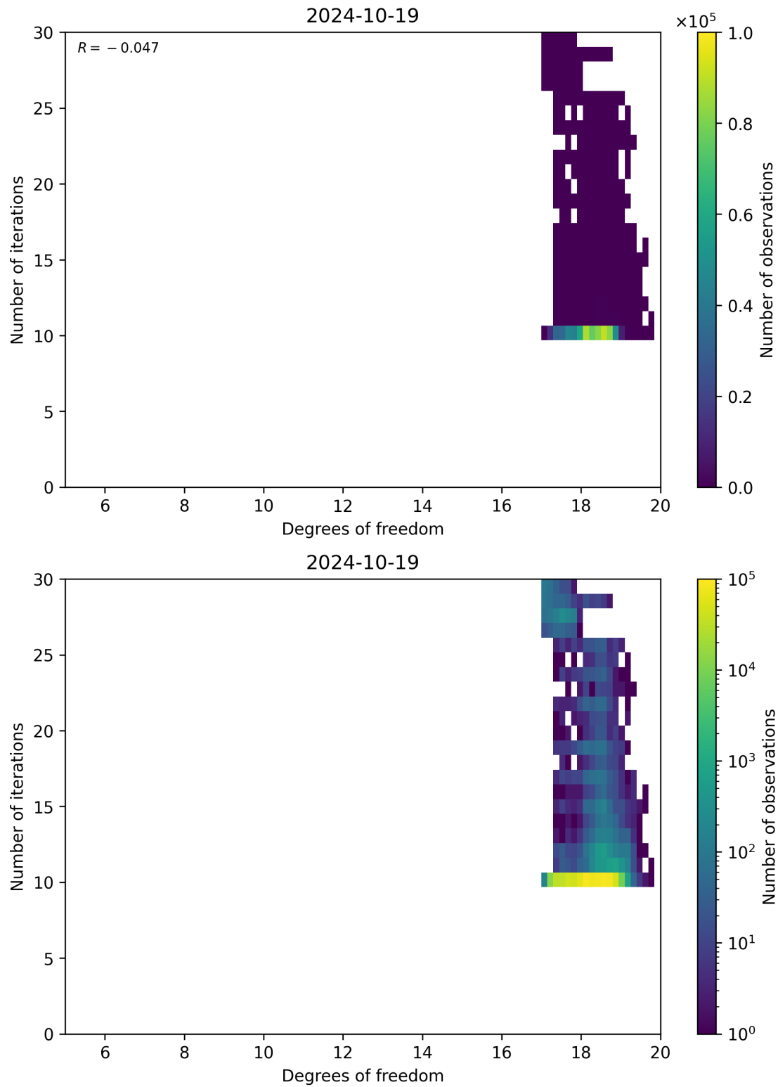
Figure 52: Scatter density plot of “Degrees of freedom” against “Number of iterations” for 2024-10-19 to 2024-10-20.
