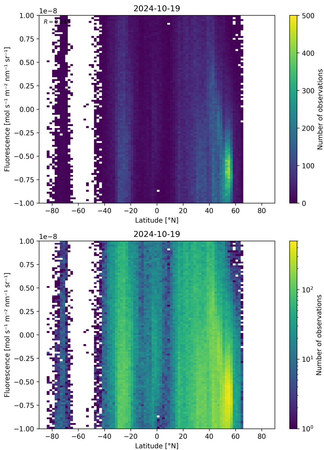
Figure 56: Scatter density plot of “Latitude” against “Fluorescence” for 2024-10-19 to 2024-10-20.
