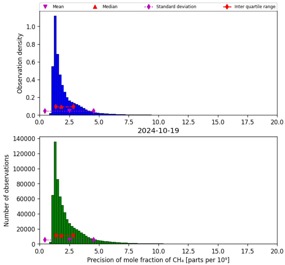
Figure 24: Histogram of “Precision of mole fraction of CH 4 ” for 2024-10-19 to 2024-10-20
