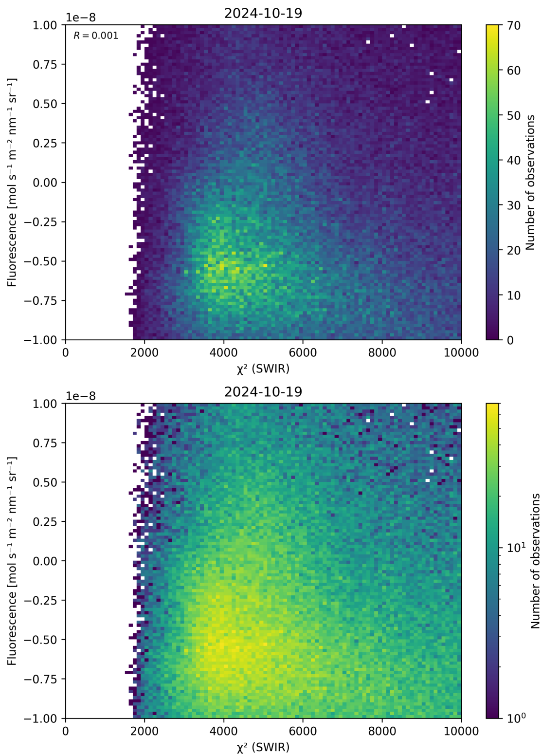
Figure 49: Scatter density plot of “ \chi^2 (SWIR)” against “Fluorescence” for 2024-10-19 to 2024-10-20.
