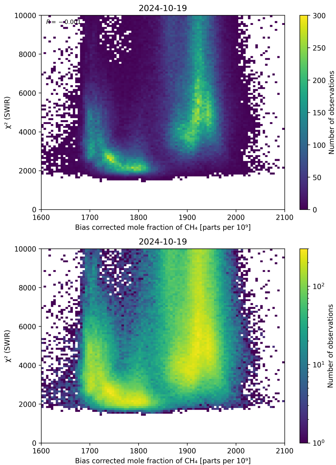
Figure 64: Scatter density plot of “Bias corrected mole fraction of CH 4 ” against “ \chi^2 (SWIR)” for 2024-10-19 to 2024-10-20.
