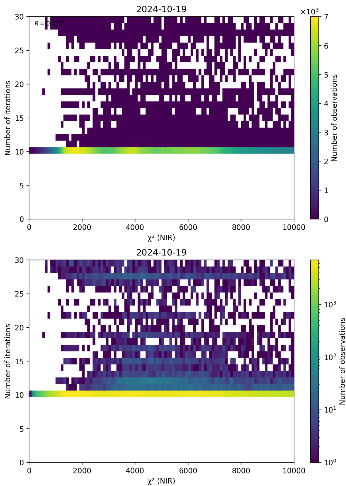
Figure 46: Scatter density plot of “ \chi^2 (NIR)” against “Number of iterations” for 2024-10-19 to 2024-10-20.
