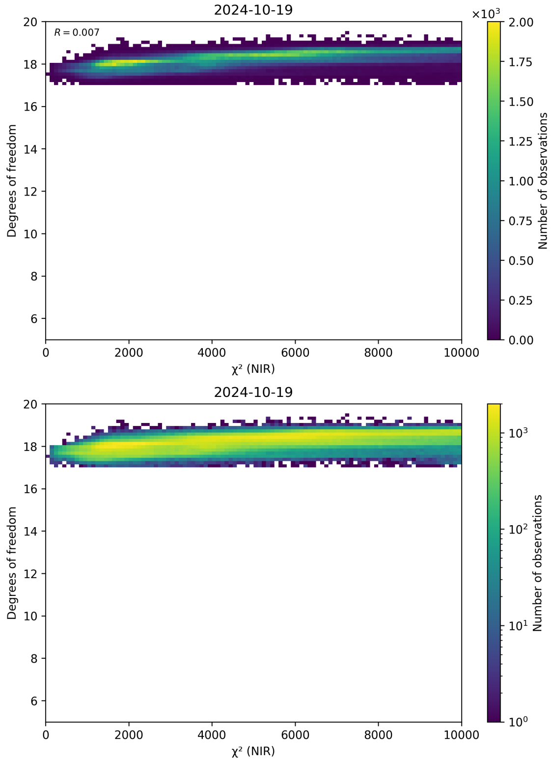
Figure 44: Scatter density plot of “ \chi^2 (NIR)” against “Degrees of freedom” for 2024-10-19 to 2024-10-20.
