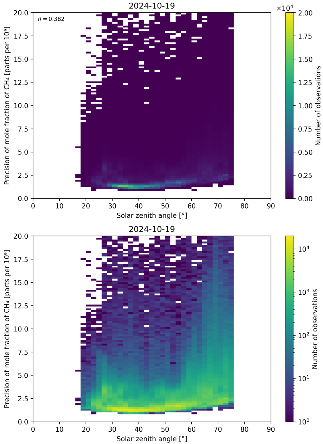
Figure 101: Scatter density plot of “Solar zenith angle” against “Precision of mole fraction of \text{CH}_4 ” for 2024-10-19 to 2024-10-20.
