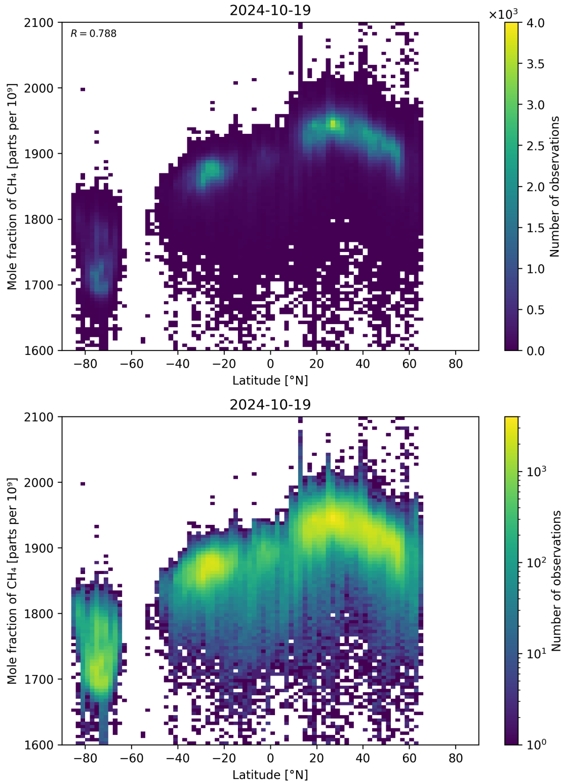
Figure 57: Scatter density plot of “Latitude” against “Mole fraction of CH 4 ” for 2024-10-19 to 2024-10-20.
