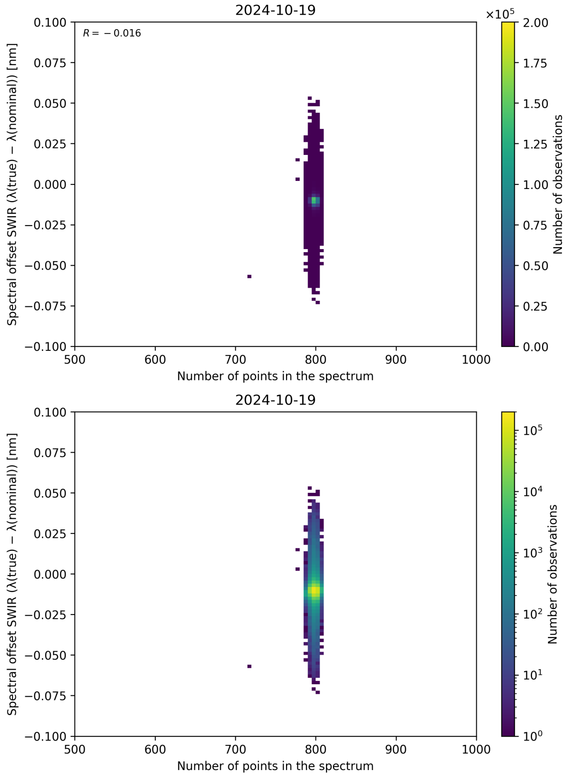
Figure 93: Scatter density plot of “Number of points in the spectrum” against “Spectral offset SWIR ( \lambda_{\text{true}} - \lambda_{\text{nominal}} )” for 2024-10-19 to 2024-10-20.
