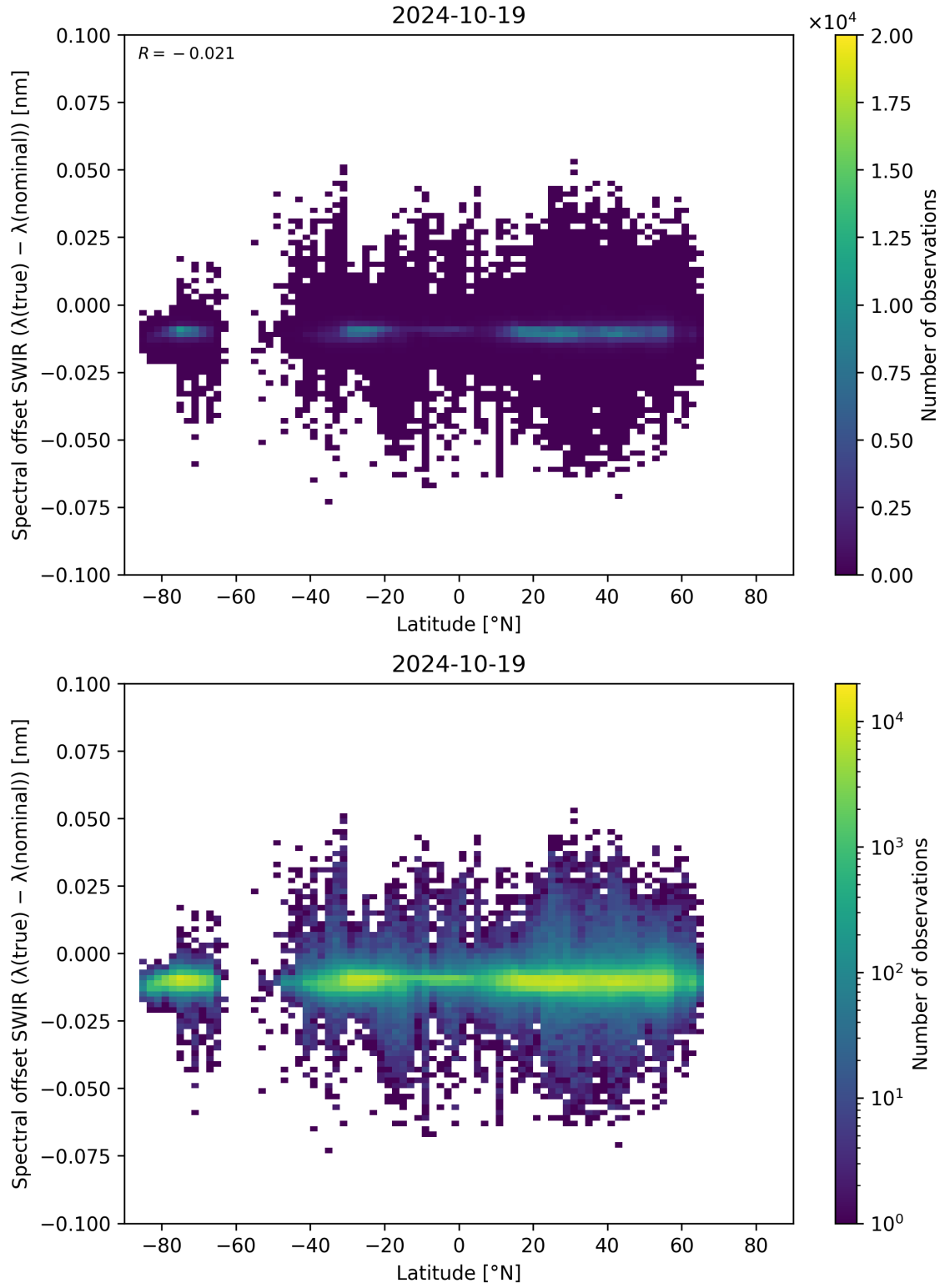
Figure 62: Scatter density plot of “Latitude” against “Spectral offset SWIR ( \lambda_{\text{true}} - \lambda_{\text{nominal}} )” for 2024-10-19 to 2024-10-20.
