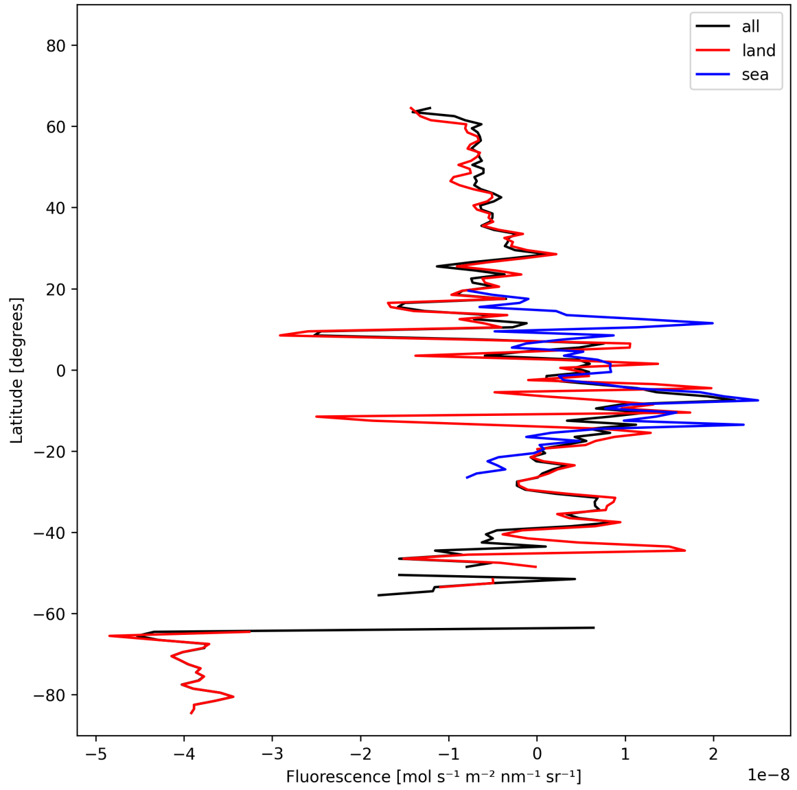
Figure 21: Zonal average of “Fluorescence” for 2024-10-19 to 2024-10-20.
