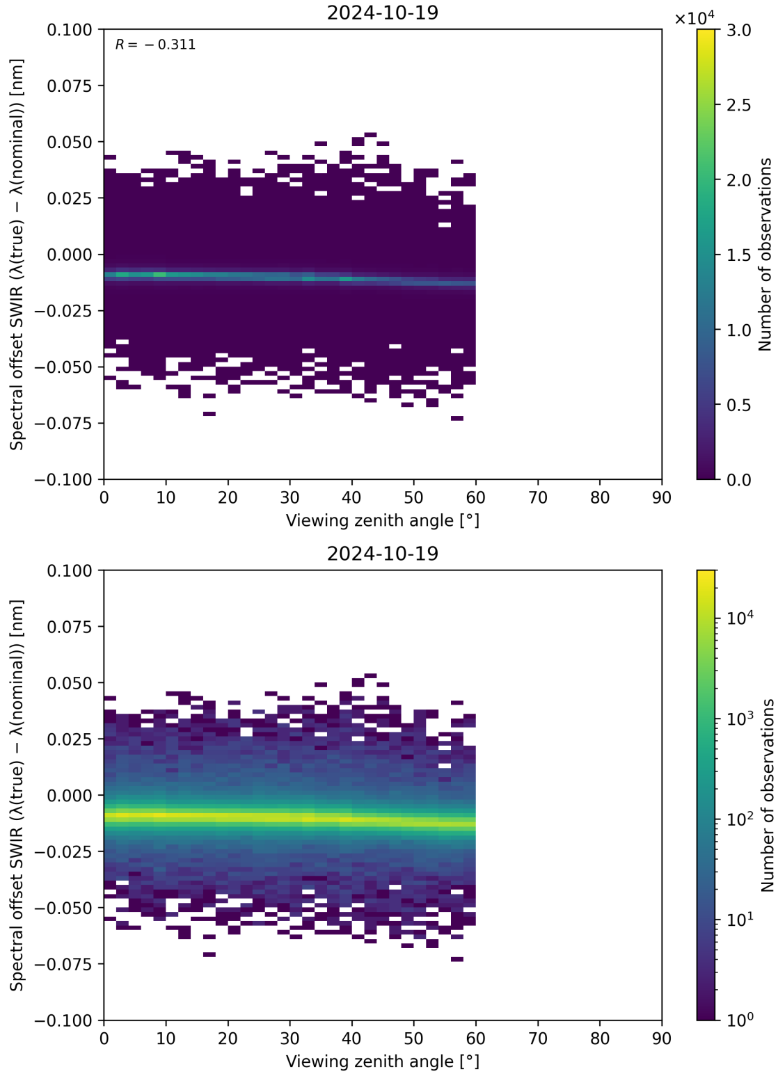
Figure 116: Scatter density plot of “Viewing zenith angle” against “Spectral offset SWIR ( \lambda_{\text{true}} - \lambda_{\text{nominal}} )” for 2024-10-19 to 2024-10-20.
