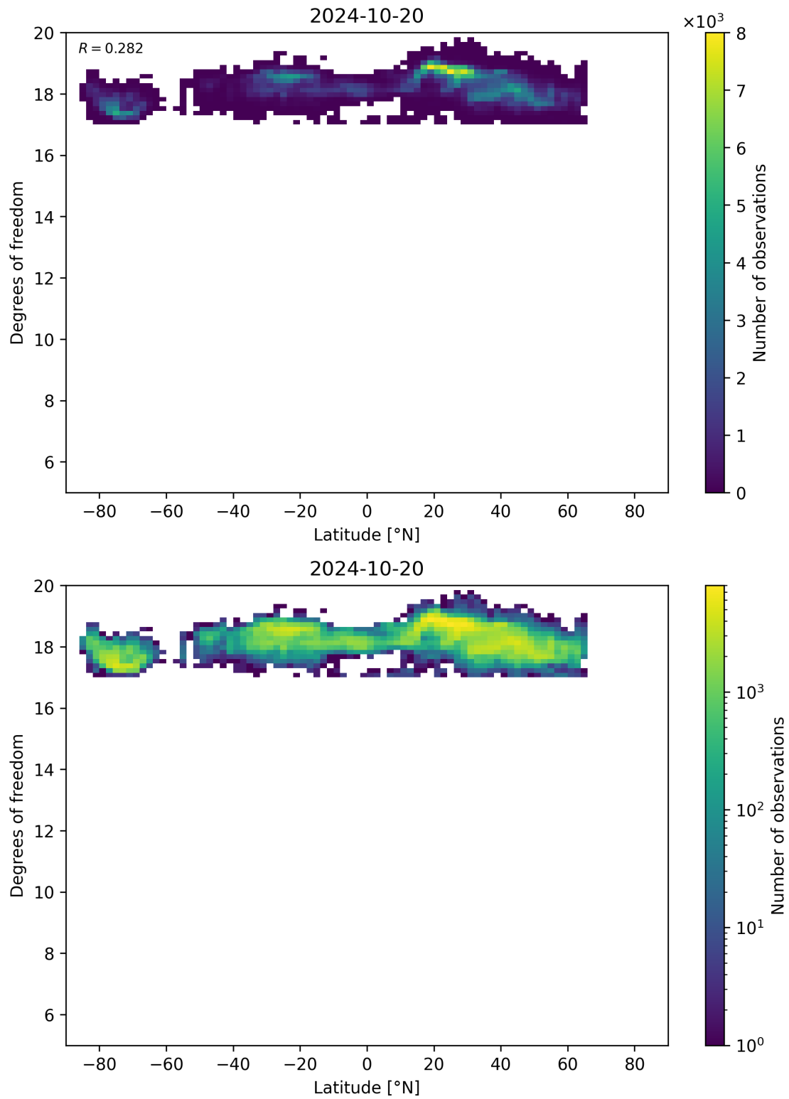
Figure 55: Scatter density plot of “Latitude” against “Degrees of freedom” for 2024-10-19 to 2024-10-21.
