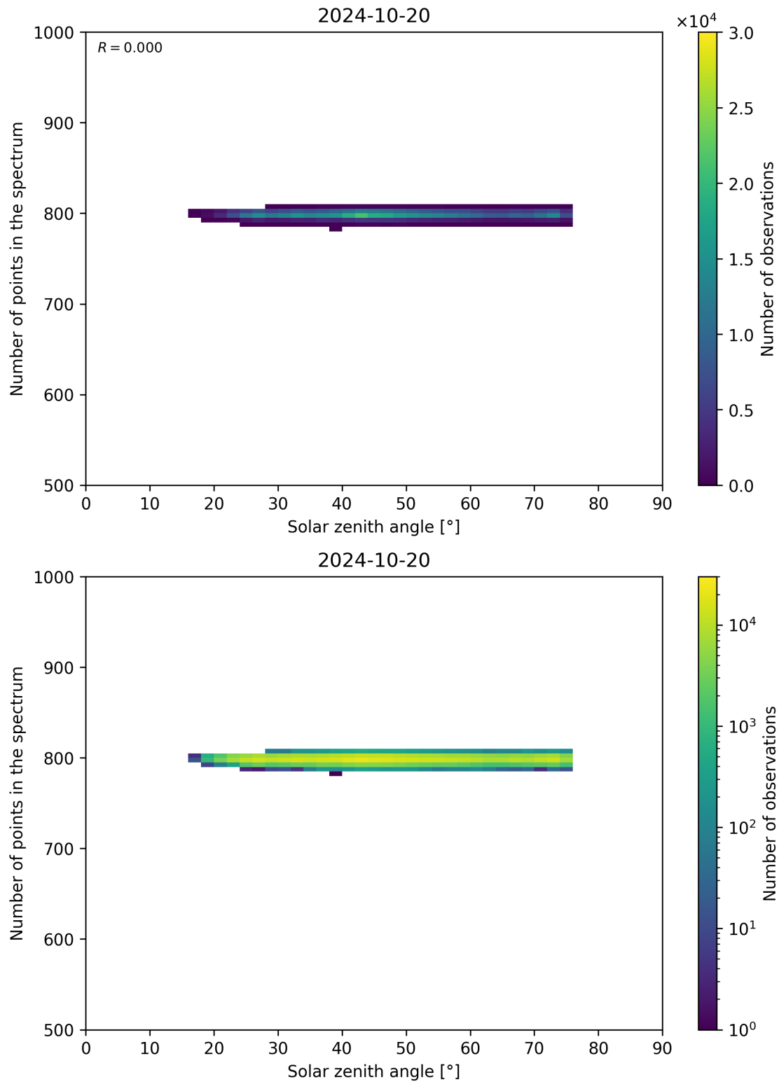
Figure 103: Scatter density plot of “Solar zenith angle” against “Number of points in the spectrum” for 2024-10-19 to 2024-10-21.
