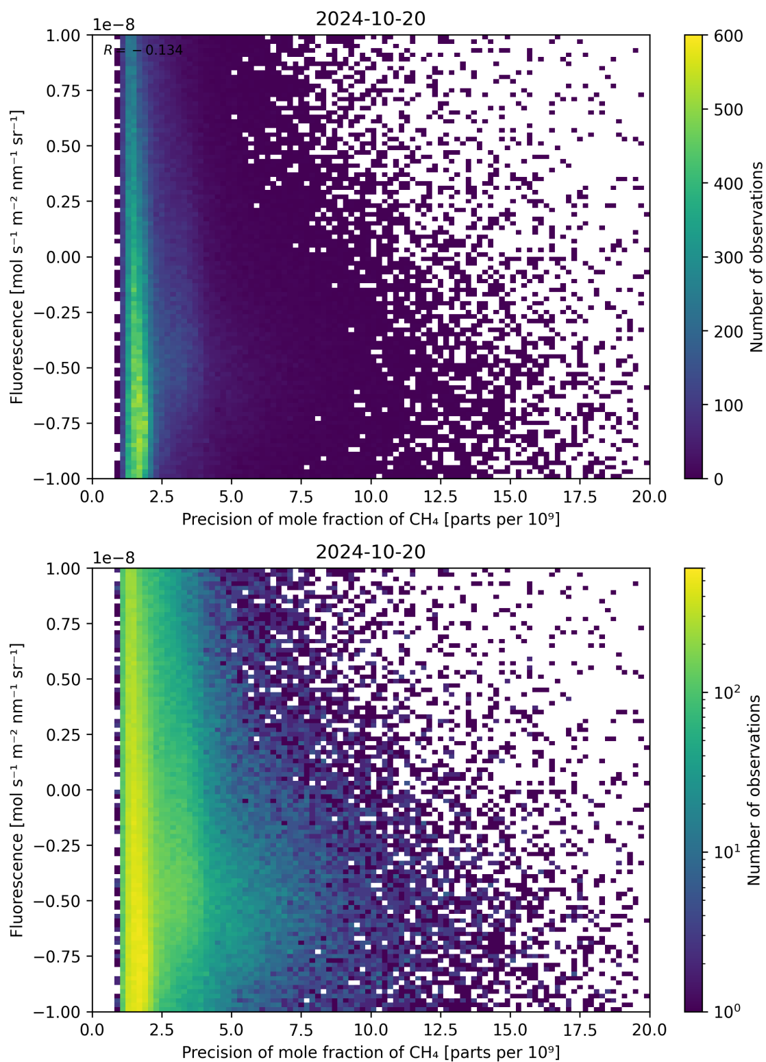
Figure 81: Scatter density plot of “Precision of mole fraction of \text{CH}_4 ” against “Fluorescence” for 2024-10-19 to 2024-10-21.
