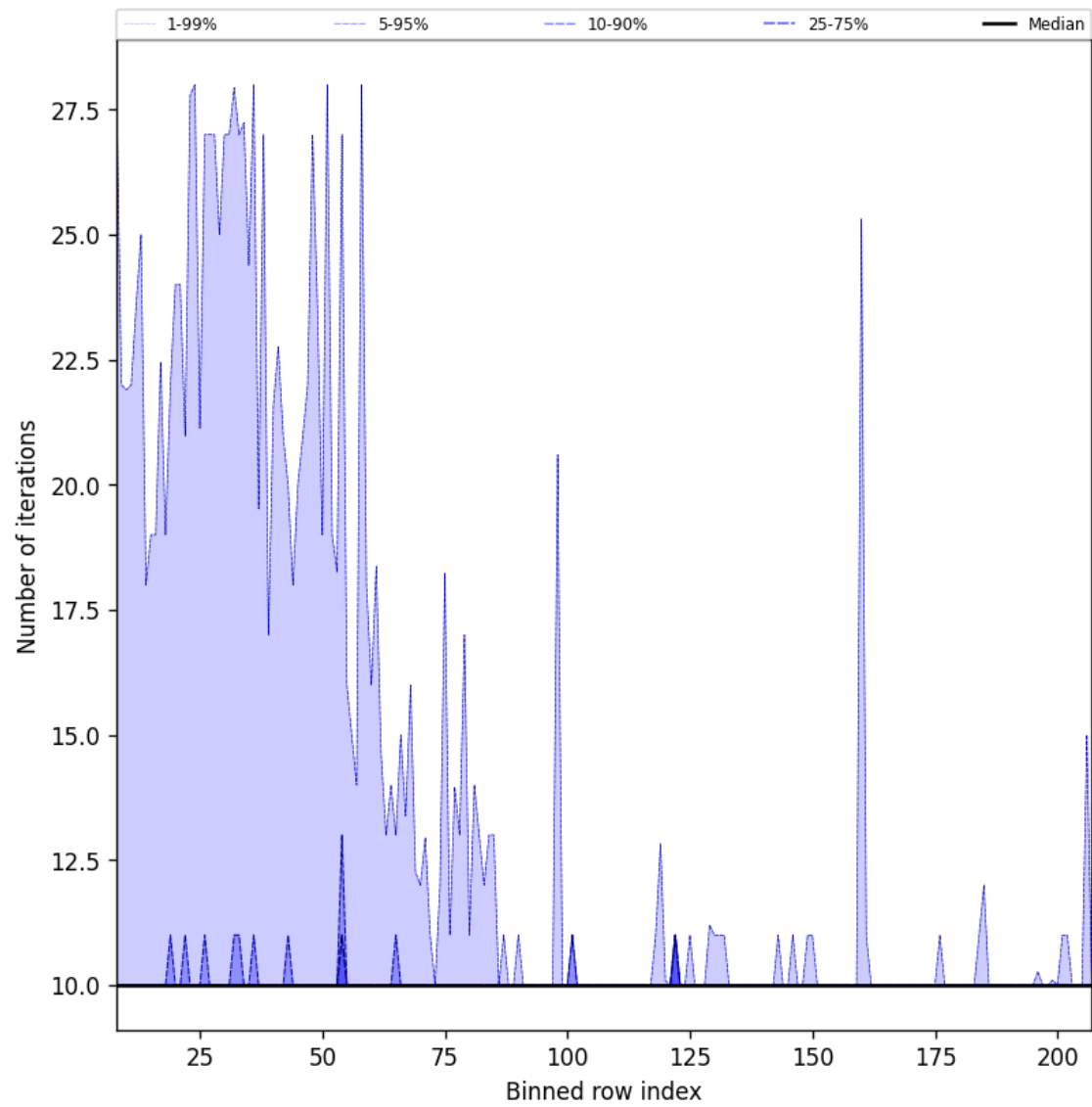
Figure 42: Along track statistics of “Number of iterations” for 2024-10-19 to 2024-10-21
