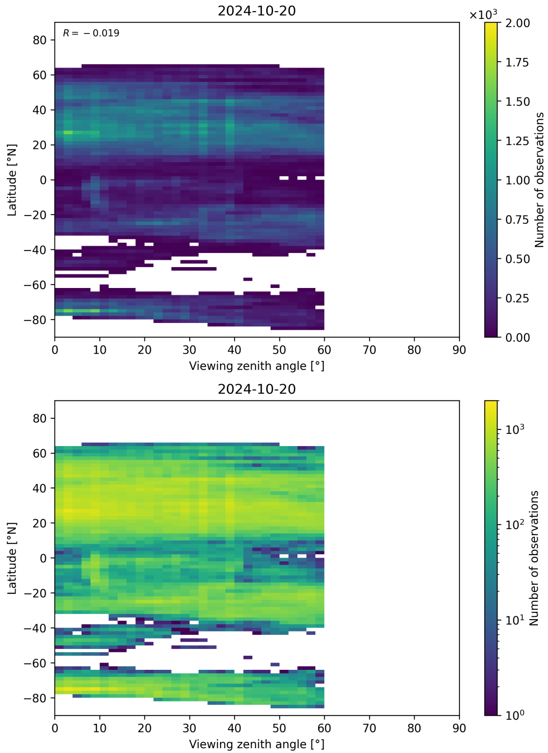
Figure 109: Scatter density plot of “Viewing zenith angle” against “Latitude” for 2024-10-19 to 2024-10-21.
