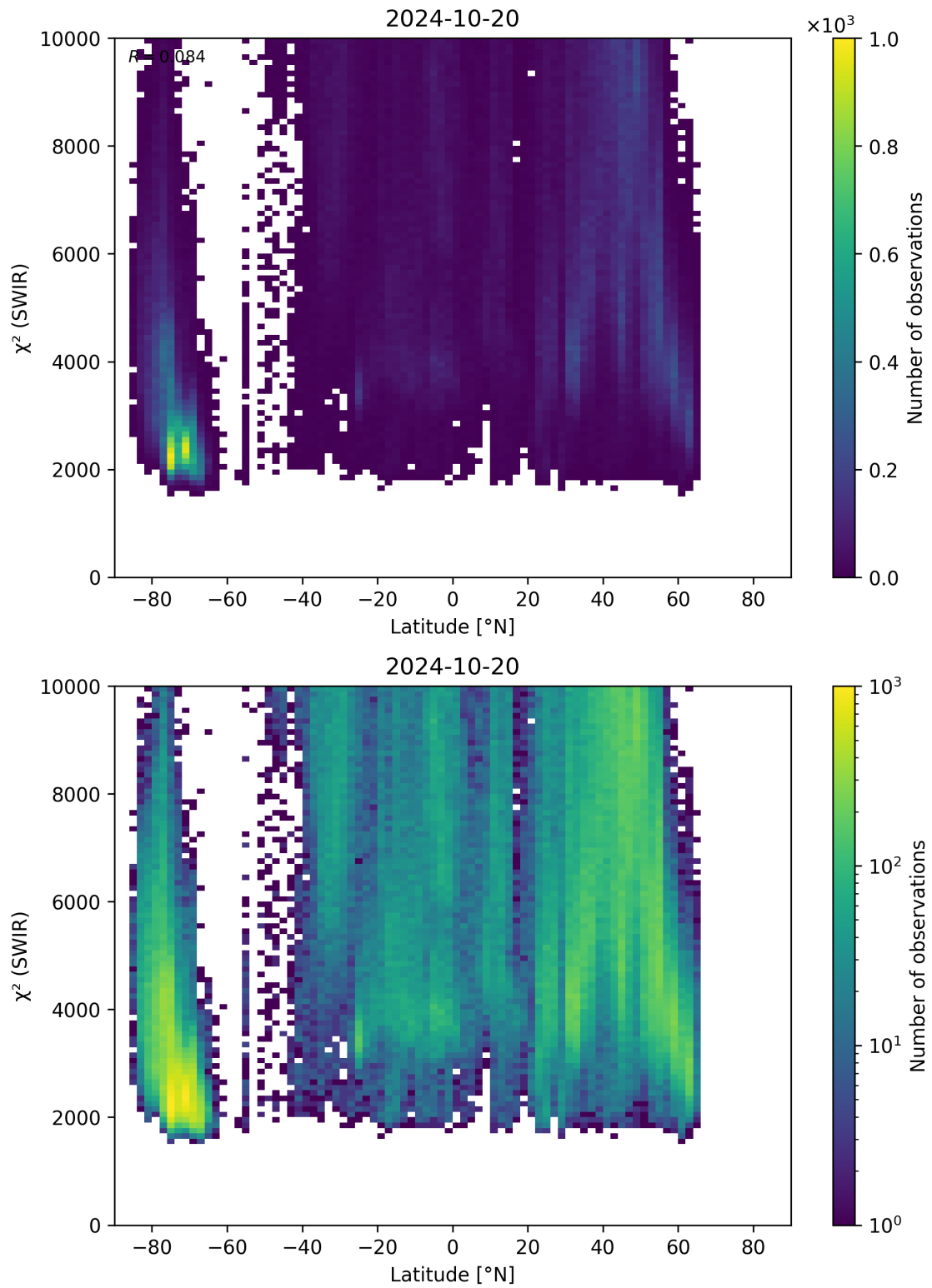
Figure 54: Scatter density plot of “Latitude” against “ \chi^2 (SWIR)” for 2024-10-19 to 2024-10-21.
