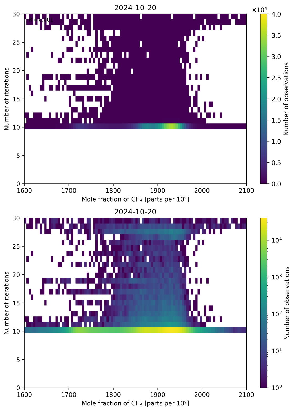
Figure 76: Scatter density plot of “Mole fraction of CH 4 ” against “Number of iterations” for 2024-10-19 to 2024-10-21.
