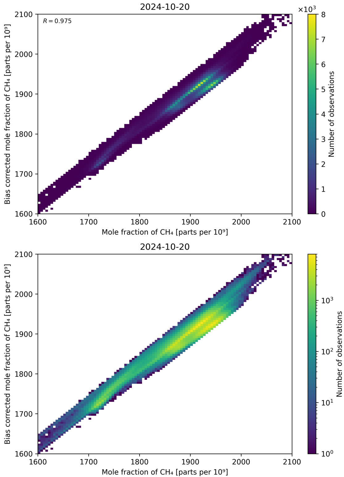
Figure 74: Scatter density plot of “Mole fraction of CH 4 ” against “Bias corrected mole fraction of CH 4 ” for 2024-10-19 to 2024-10-21.
