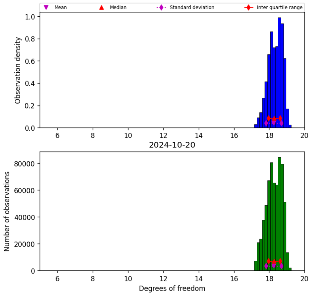
Figure 30: Histogram of “Degrees of freedom” for 2024-10-19 to 2024-10-21
