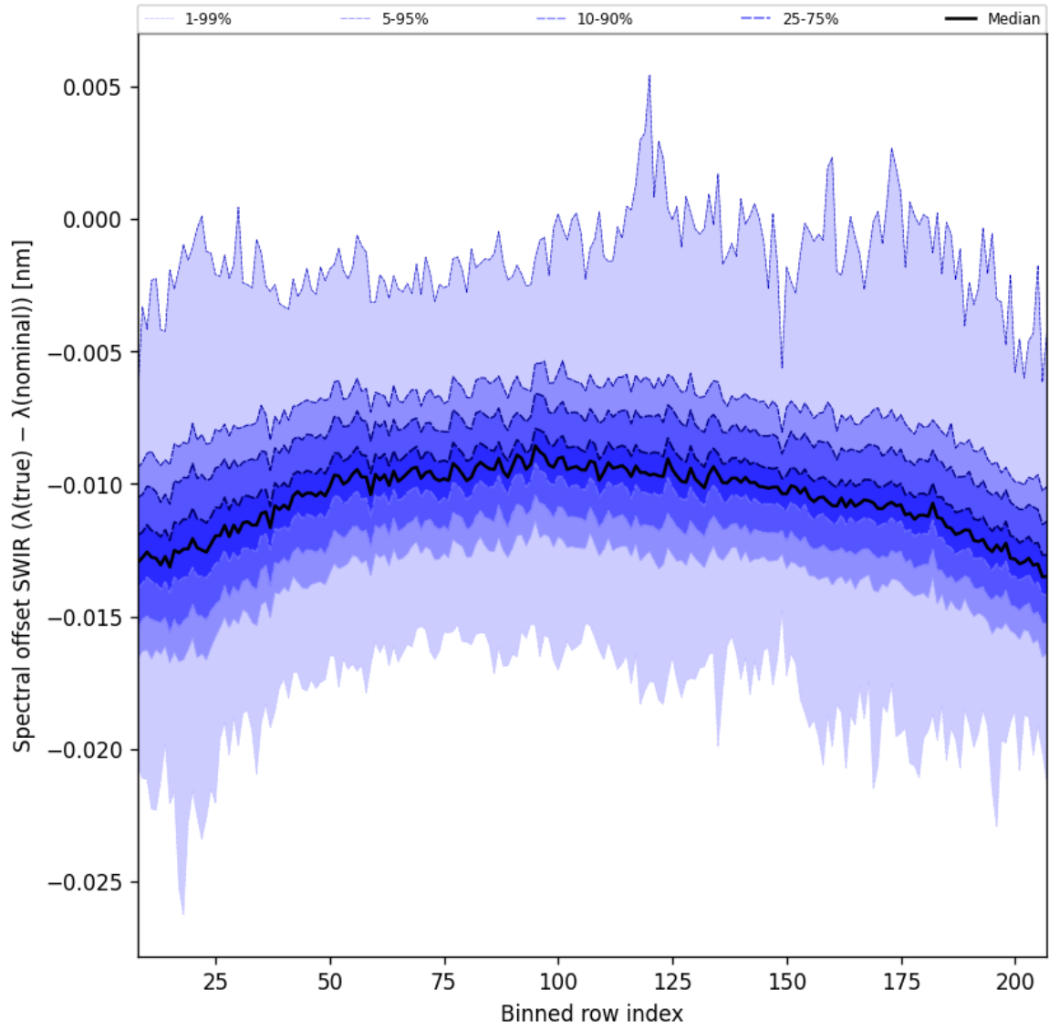
Figure 38: Along track statistics of “Spectral offset SWIR ( \lambda_{\text{true}} - \lambda_{\text{nominal}} )” for 2024-10-19 to 2024-10-21
