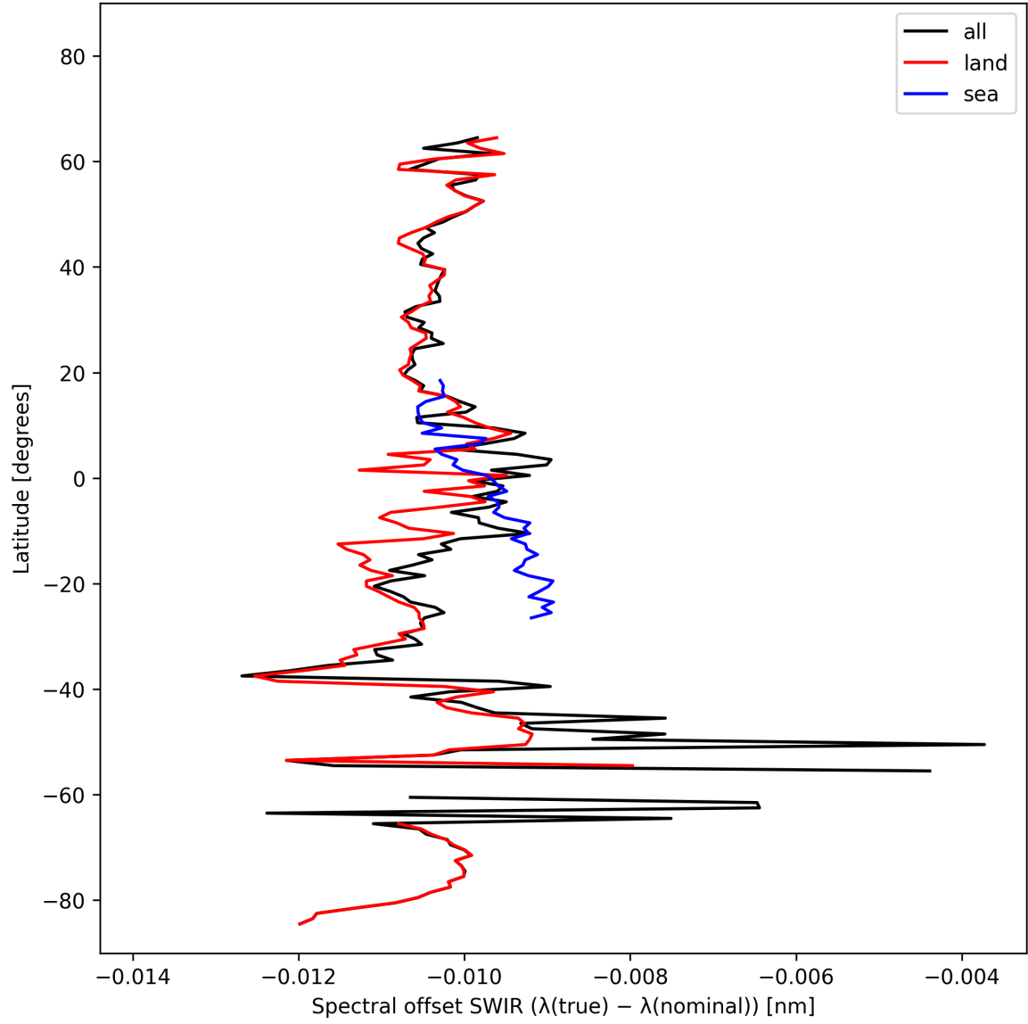
Figure 16: Zonal average of “Spectral offset SWIR ( \lambda_{\text{true}} - \lambda_{\text{nominal}} )” for 2024-10-19 to 2024-10-21.
