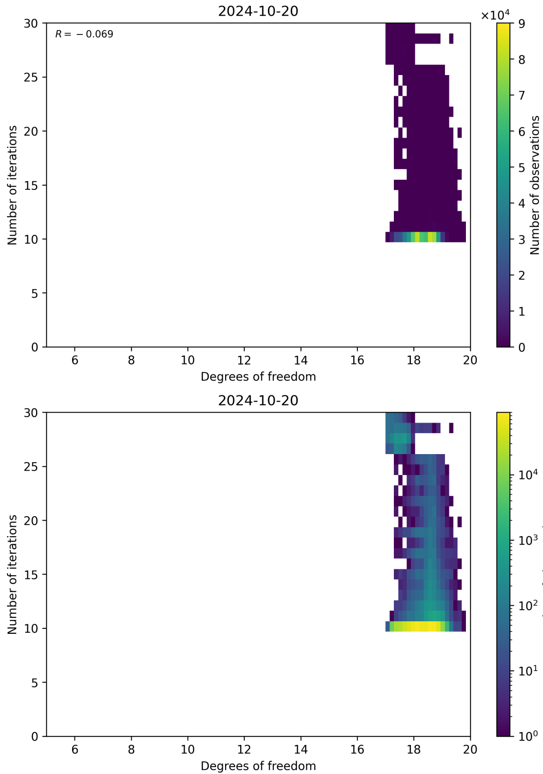
Figure 52: Scatter density plot of “Degrees of freedom” against “Number of iterations” for 2024-10-19 to 2024-10-21.
