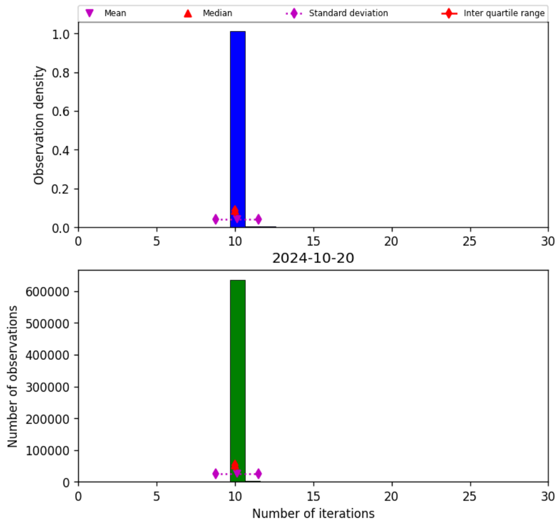
Figure 31: Histogram of “Number of iterations” for 2024-10-19 to 2024-10-21
