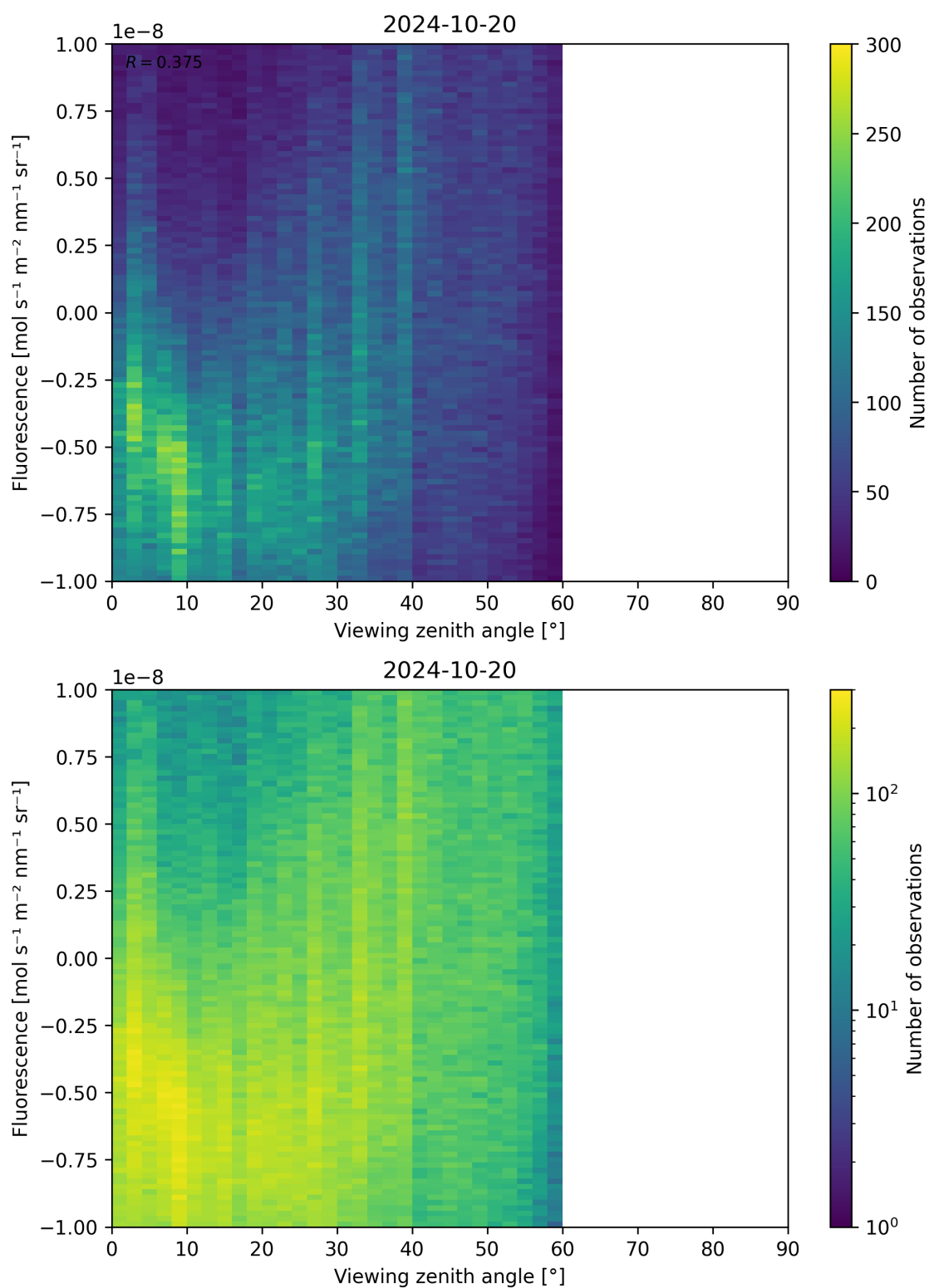
Figure 108: Scatter density plot of “Viewing zenith angle” against “Fluorescence” for 2024-10-19 to 2024-10-21.
