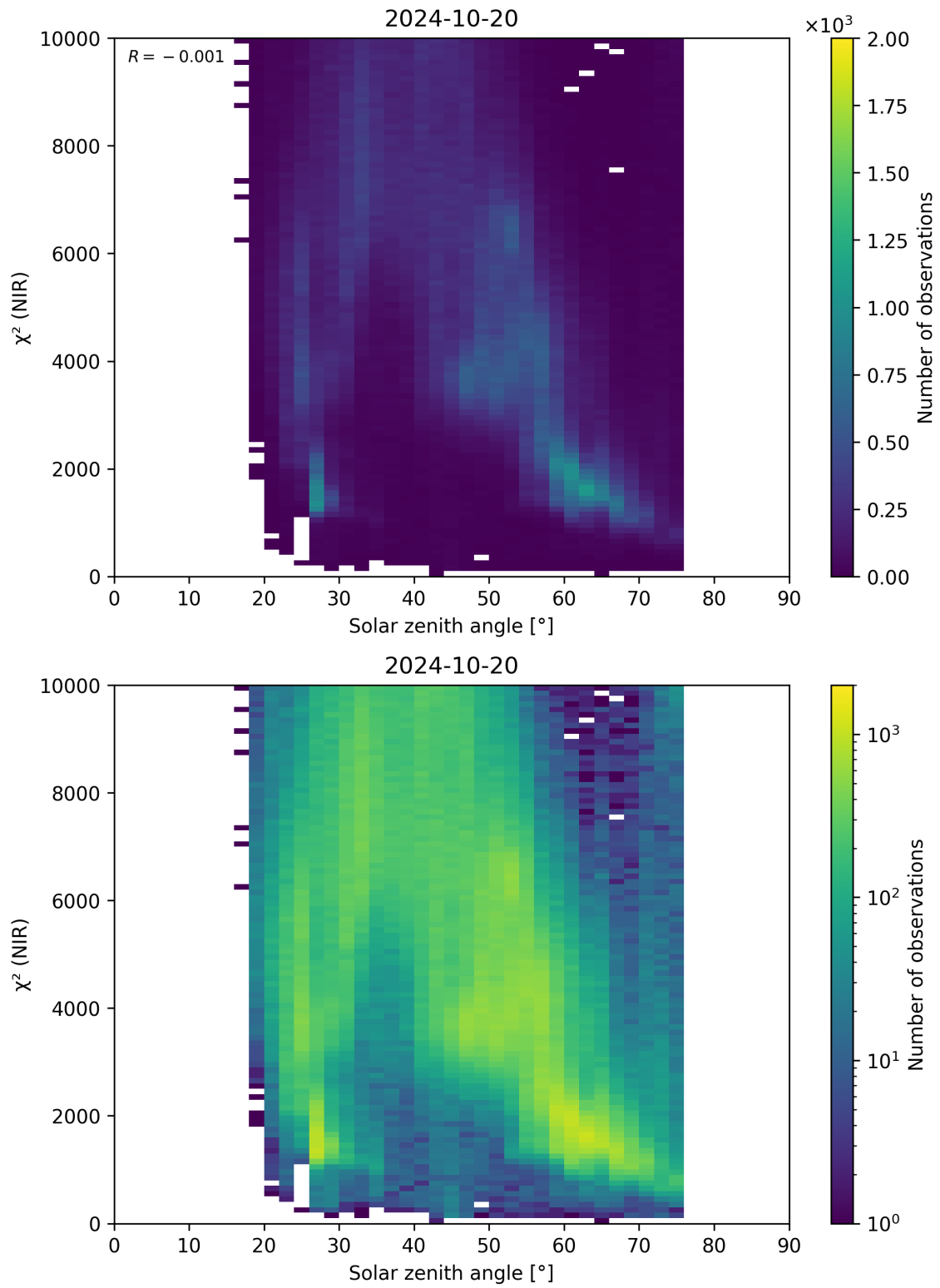
Figure 94: Scatter density plot of “Solar zenith angle” against “ \chi^2 (NIR)” for 2024-10-19 to 2024-10-21.
