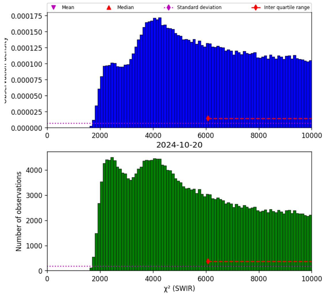
Figure 28: Histogram of “ \chi^2 (SWIR)” for 2024-10-19 to 2024-10-21
