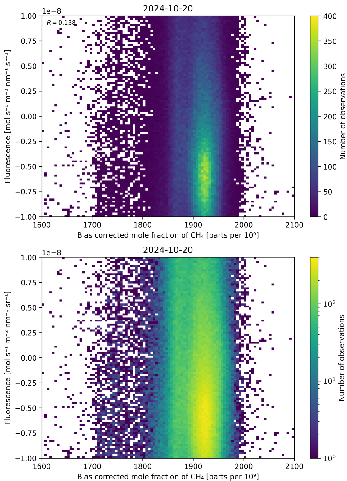
Figure 66: Scatter density plot of “Bias corrected mole fraction of \text{CH}_4 ” against “Fluorescence” for 2024-10-19 to 2024-10-21.
