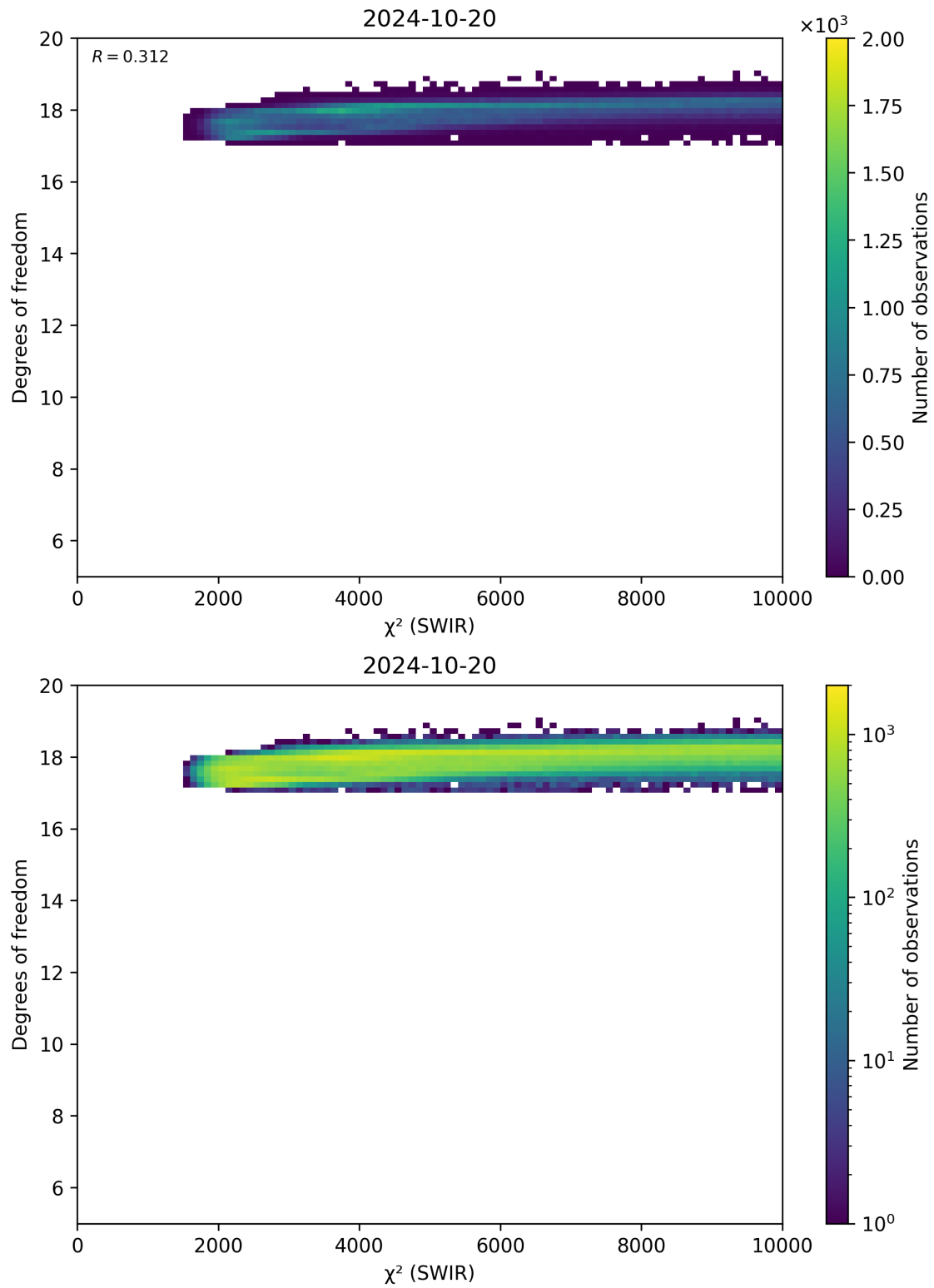
Figure 48: Scatter density plot of “ \chi^2 (SWIR)” against “Degrees of freedom” for 2024-10-19 to 2024-10-21.
