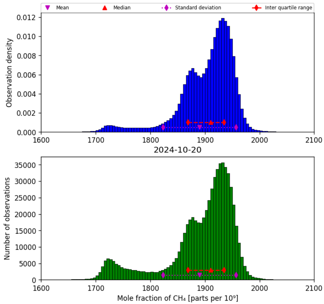
Figure 23: Histogram of “Mole fraction of CH 4 ” for 2024-10-19 to 2024-10-21
