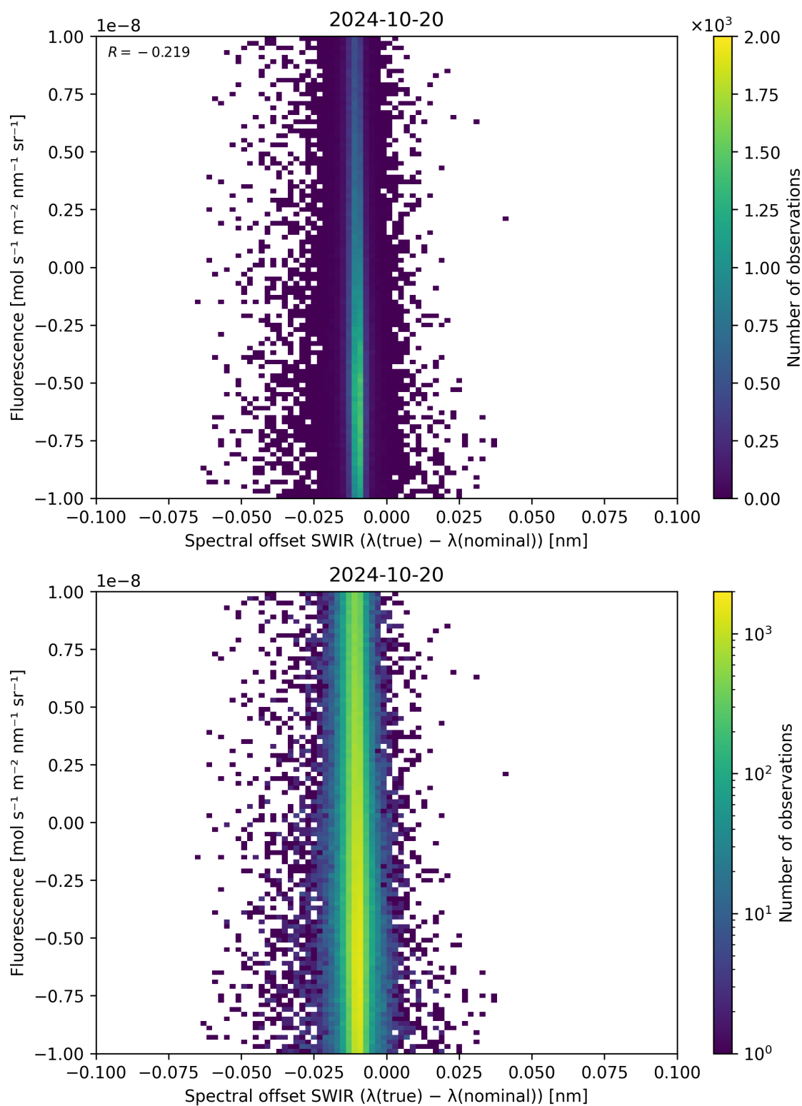
Figure 120: Scatter density plot of “Spectral offset SWIR ( \lambda_{\text{true}} - \lambda_{\text{nominal}} )” against “Fluorescence” for 2024-10-19 to 2024-10-21.
