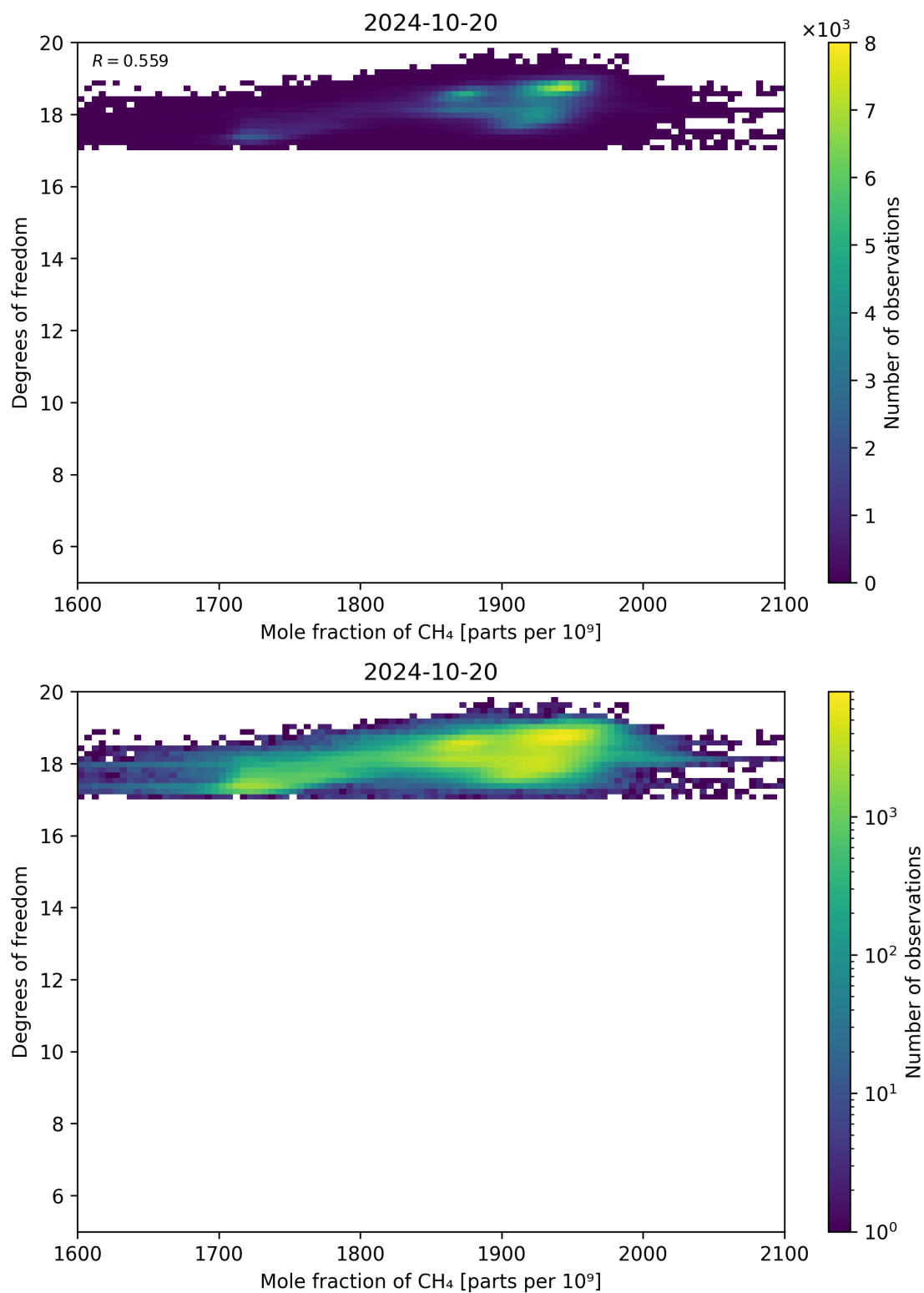
Figure 72: Scatter density plot of “Mole fraction of CH 4 ” against “Degrees of freedom” for 2024-10-19 to 2024-10-21.
