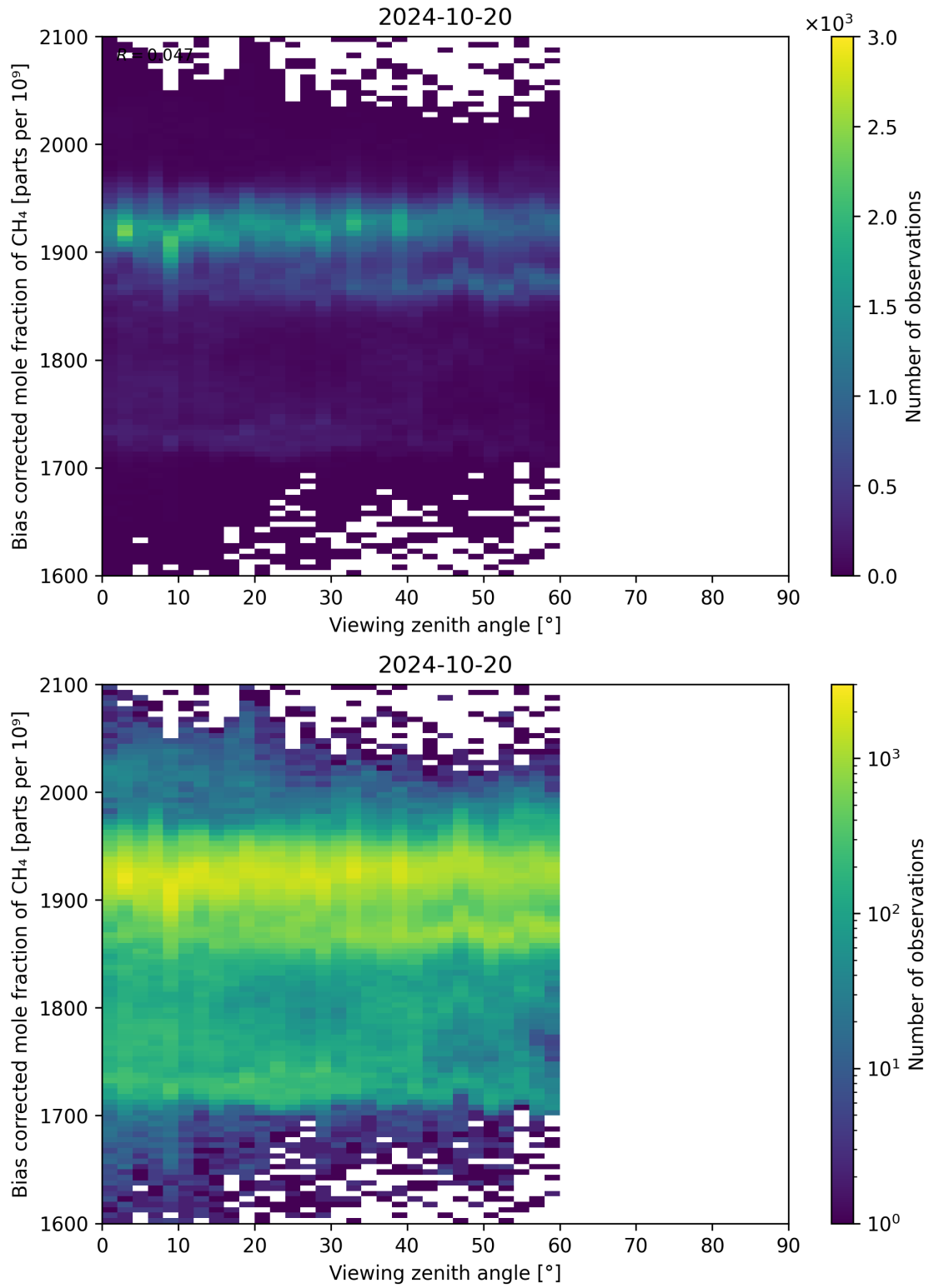
Figure 111: Scatter density plot of “Viewing zenith angle” against “Bias corrected mole fraction of CH 4 ” for 2024-10-19 to 2024-10-21.
