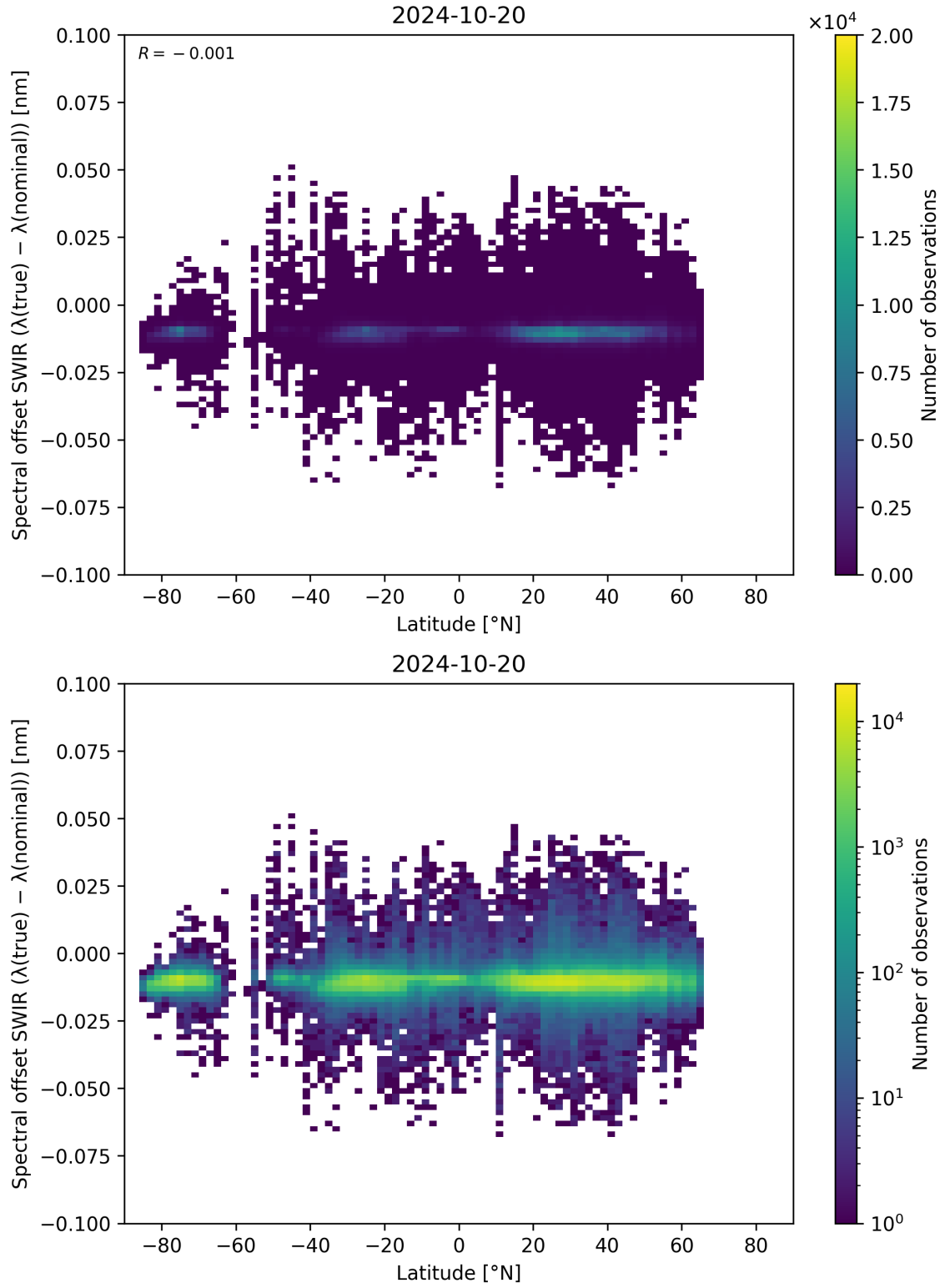
Figure 62: Scatter density plot of “Latitude” against “Spectral offset SWIR ( \lambda_{\text{true}} - \lambda_{\text{nominal}} )” for 2024-10-19 to 2024-10-21.
