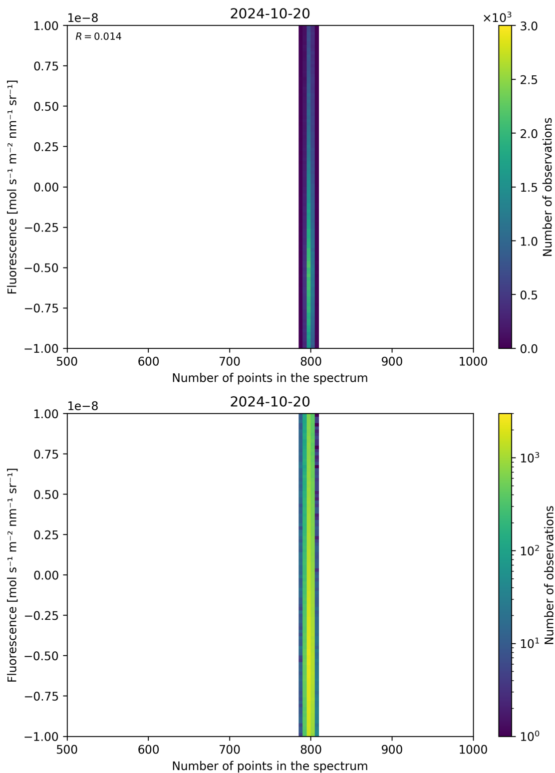
Figure 91: Scatter density plot of “Number of points in the spectrum” against “Fluorescence” for 2024-10-19 to 2024-10-21.
