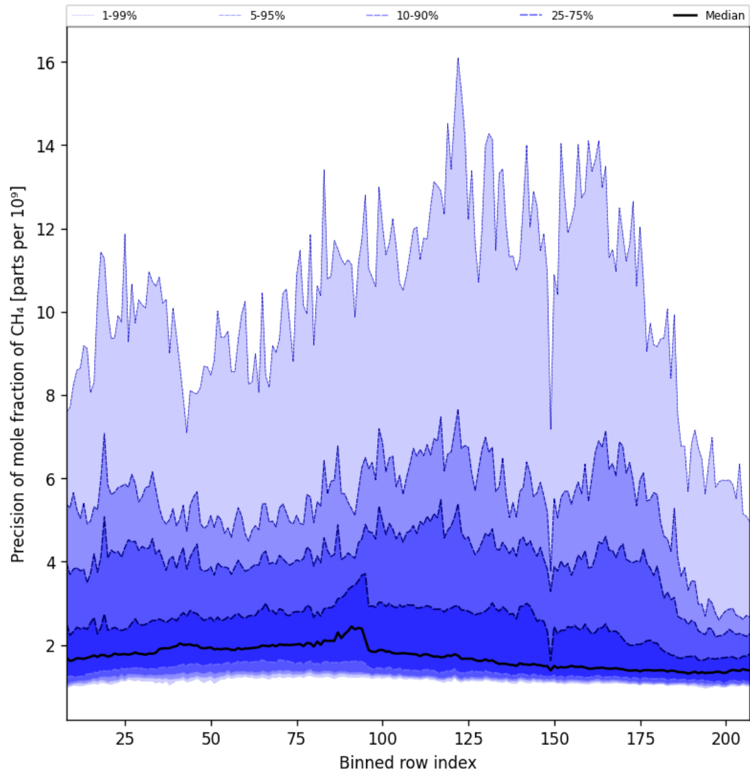
Figure 35: Along track statistics of "Precision of mole fraction of CH 4 " for 2024-10-19 to 2024-10-21
