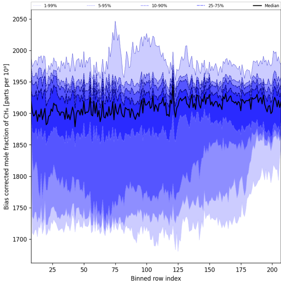
Figure 36: Along track statistics of “Bias corrected mole fraction of CH 4 ” for 2024-10-19 to 2024-10-21
