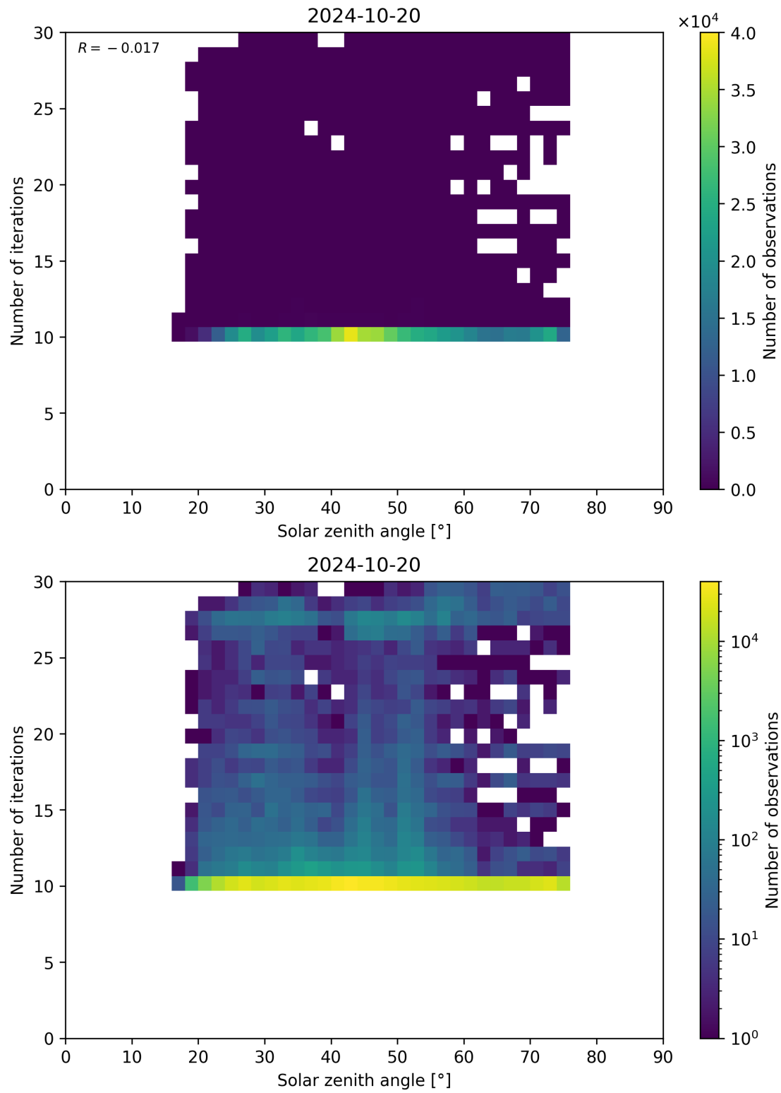
Figure 102: Scatter density plot of “Solar zenith angle” against “Number of iterations” for 2024-10-19 to 2024-10-21.
