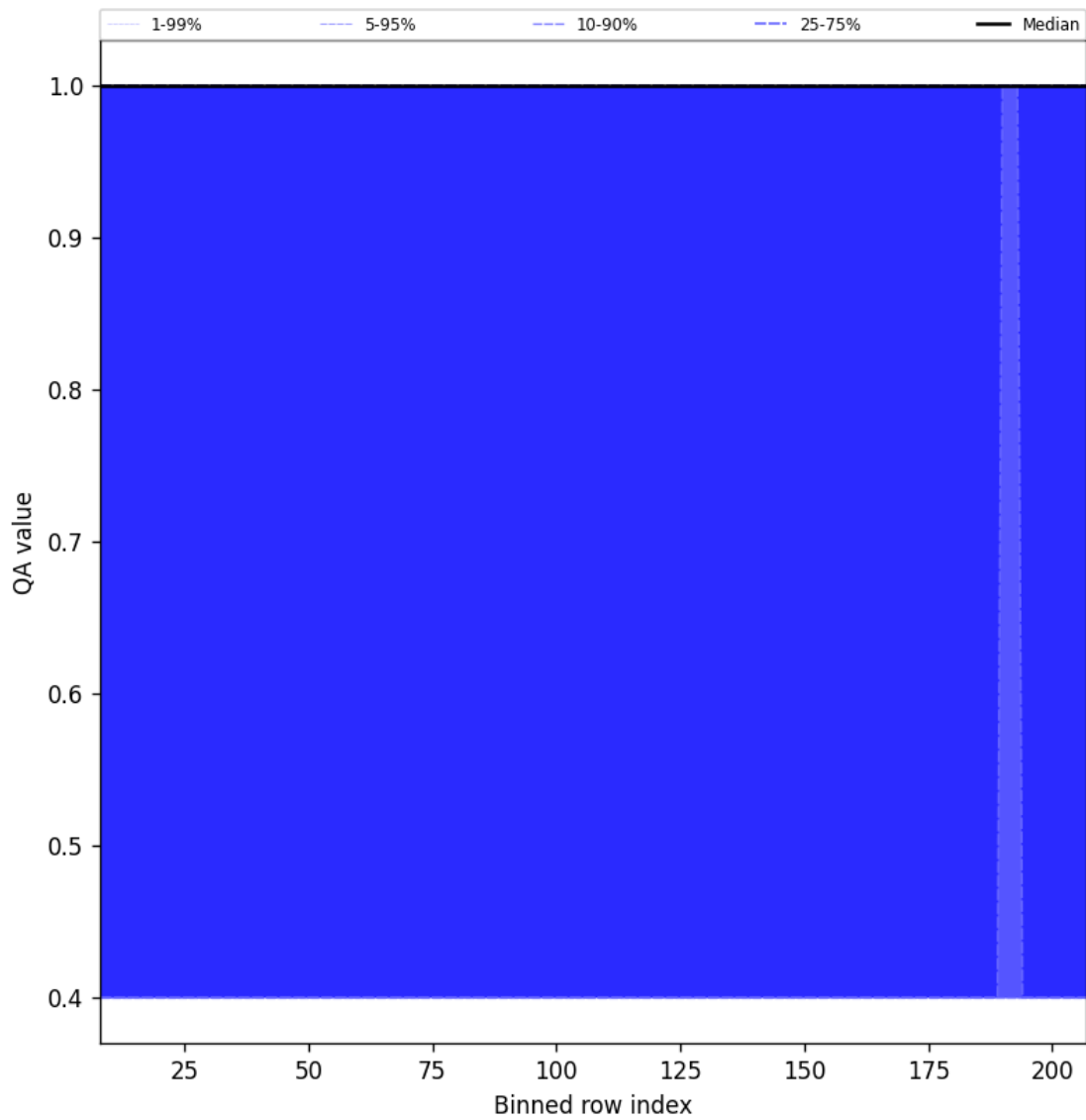
Figure 33: Along track statistics of “QA value” for 2024-10-19 to 2024-10-21
