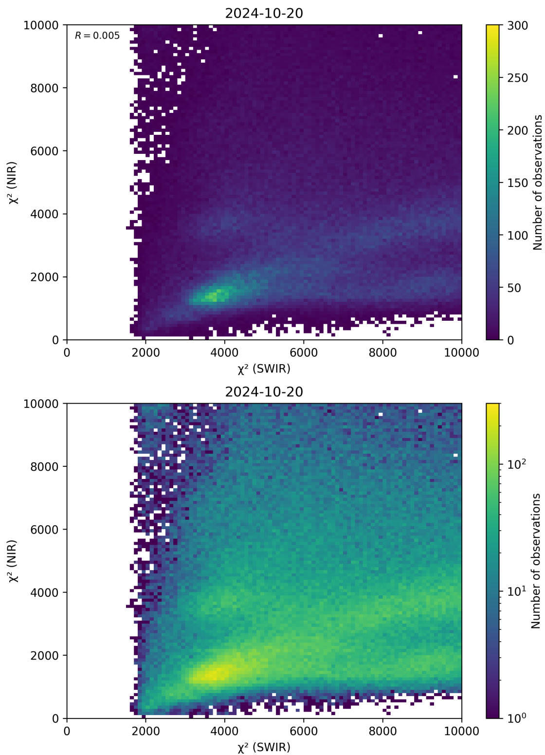
Figure 47: Scatter density plot of “ \chi^2 (SWIR)” against “ \chi^2 (NIR)” for 2024-10-19 to 2024-10-21.
