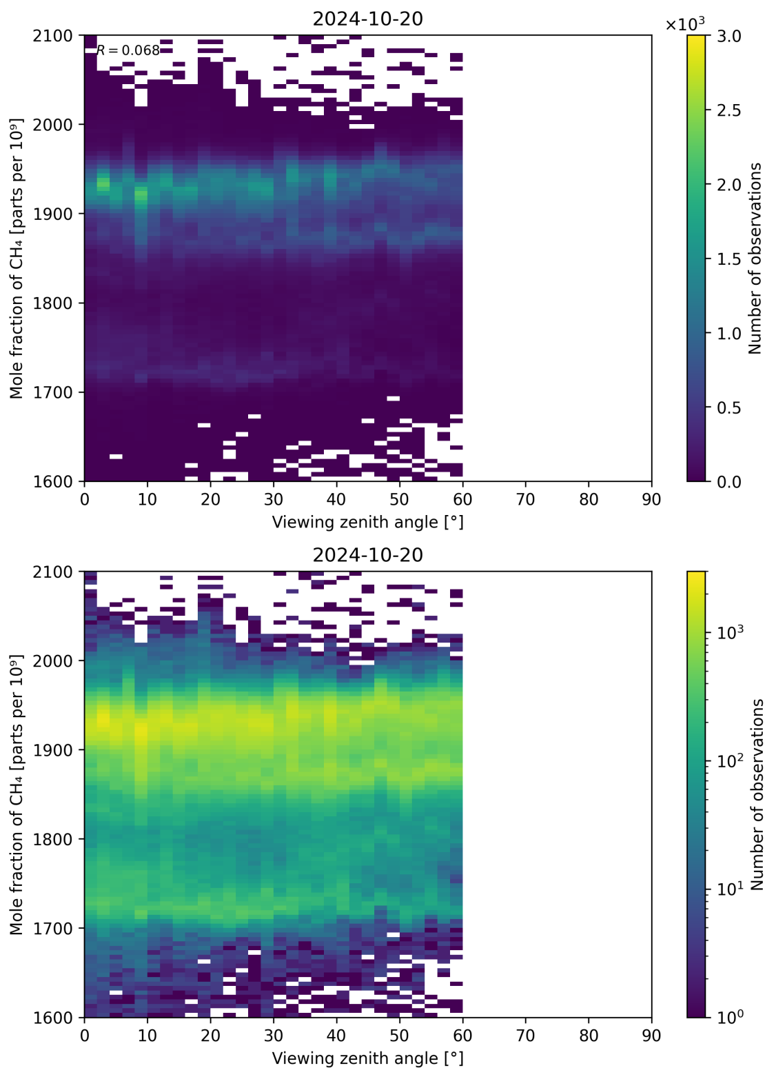
Figure 110: Scatter density plot of “Viewing zenith angle” against “Mole fraction of \text{CH}_4 ” for 2024-10-19 to 2024-10-21.
