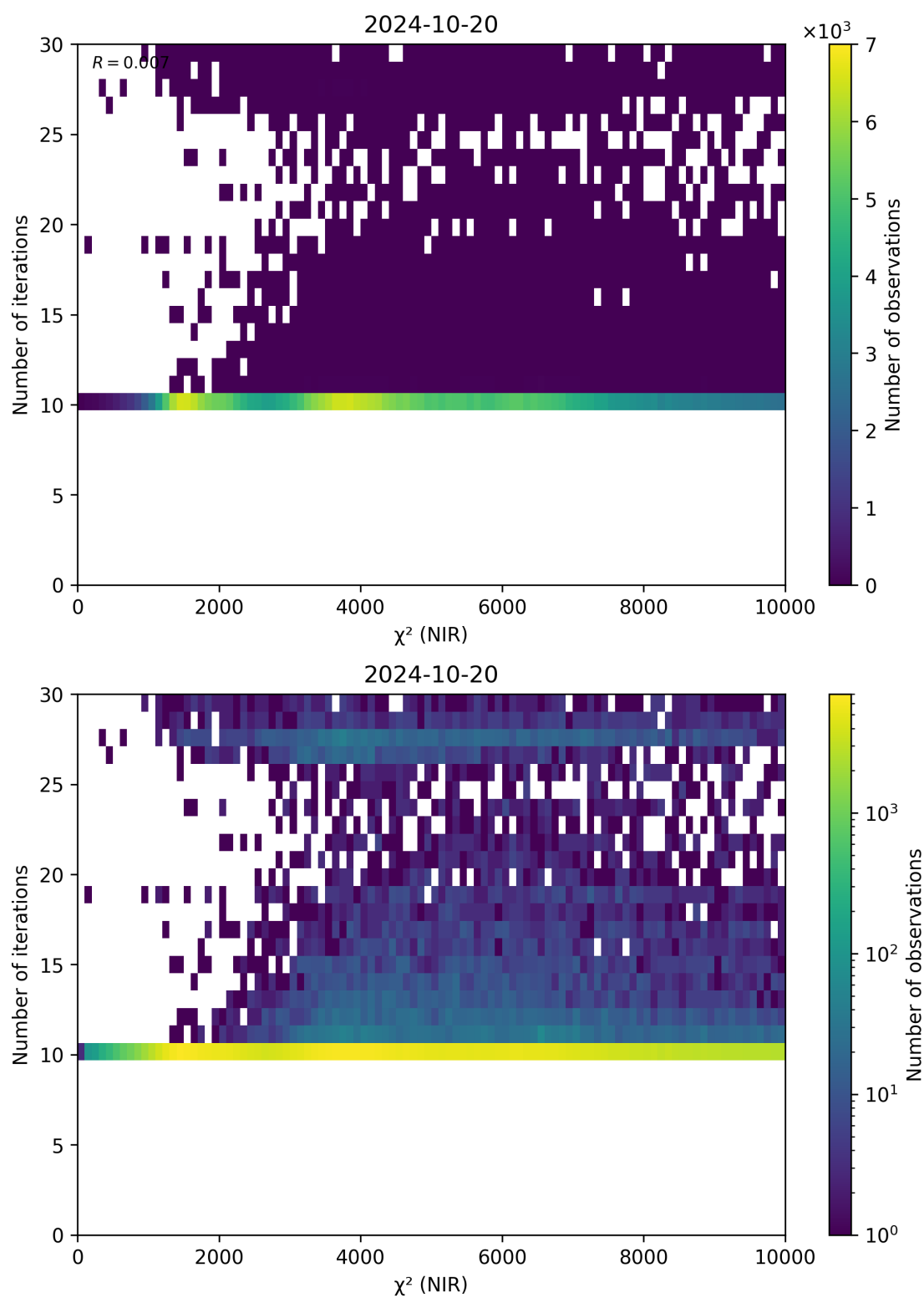
Figure 46: Scatter density plot of “ \chi^2 (NIR)” against “Number of iterations” for 2024-10-19 to 2024-10-21.
