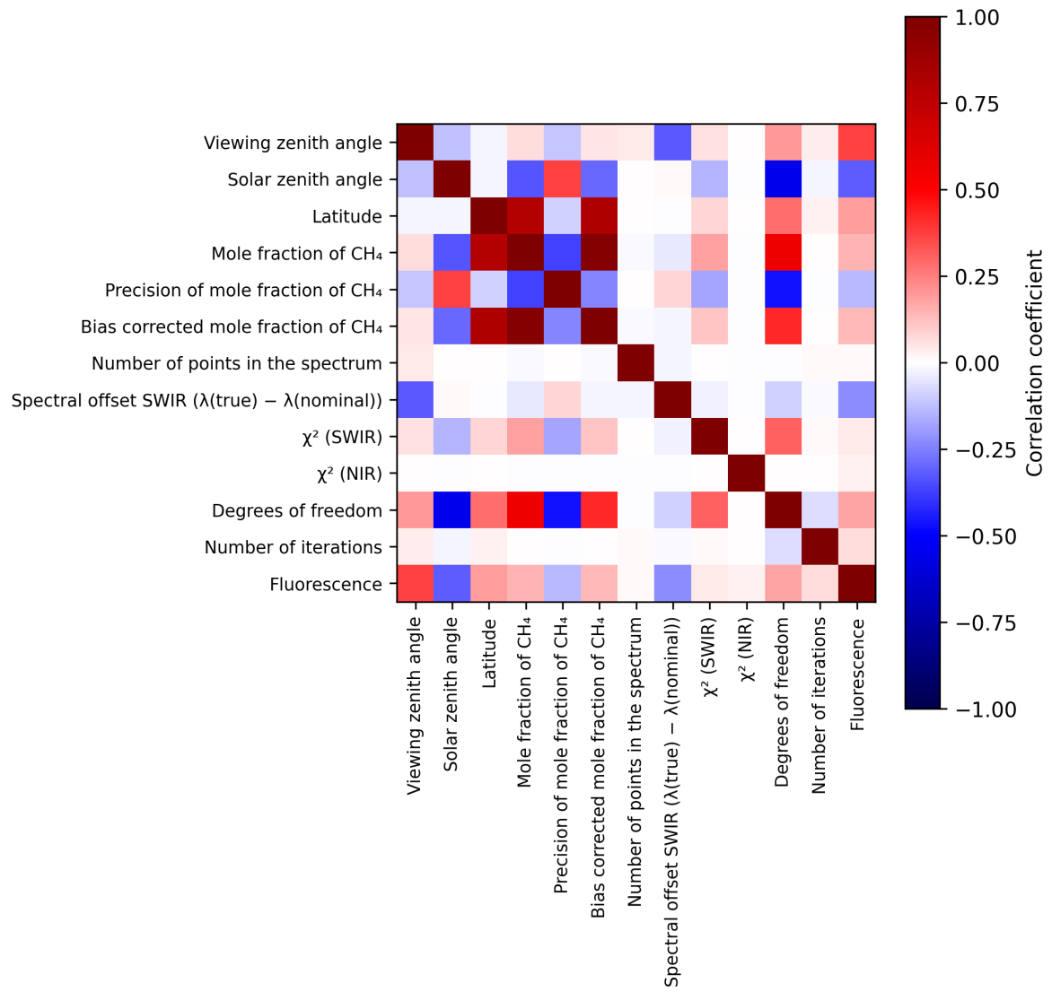
Figure 2: Map of correlation matrix for 2024-10-19 to 2024-10-21.
