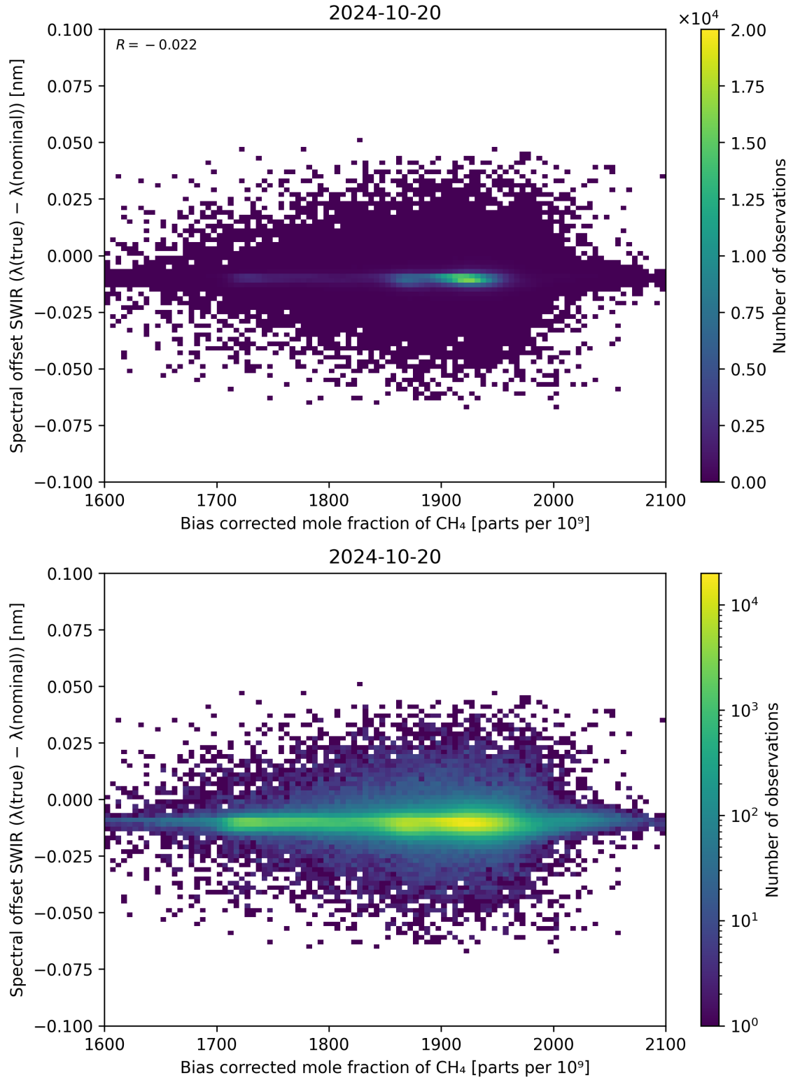
Figure 69: Scatter density plot of “Bias corrected mole fraction of \text{CH}_4 ” against “Spectral offset SWIR ( \lambda_{\text{true}} - \lambda_{\text{nominal}} )” for 2024-10-19 to 2024-10-21.
