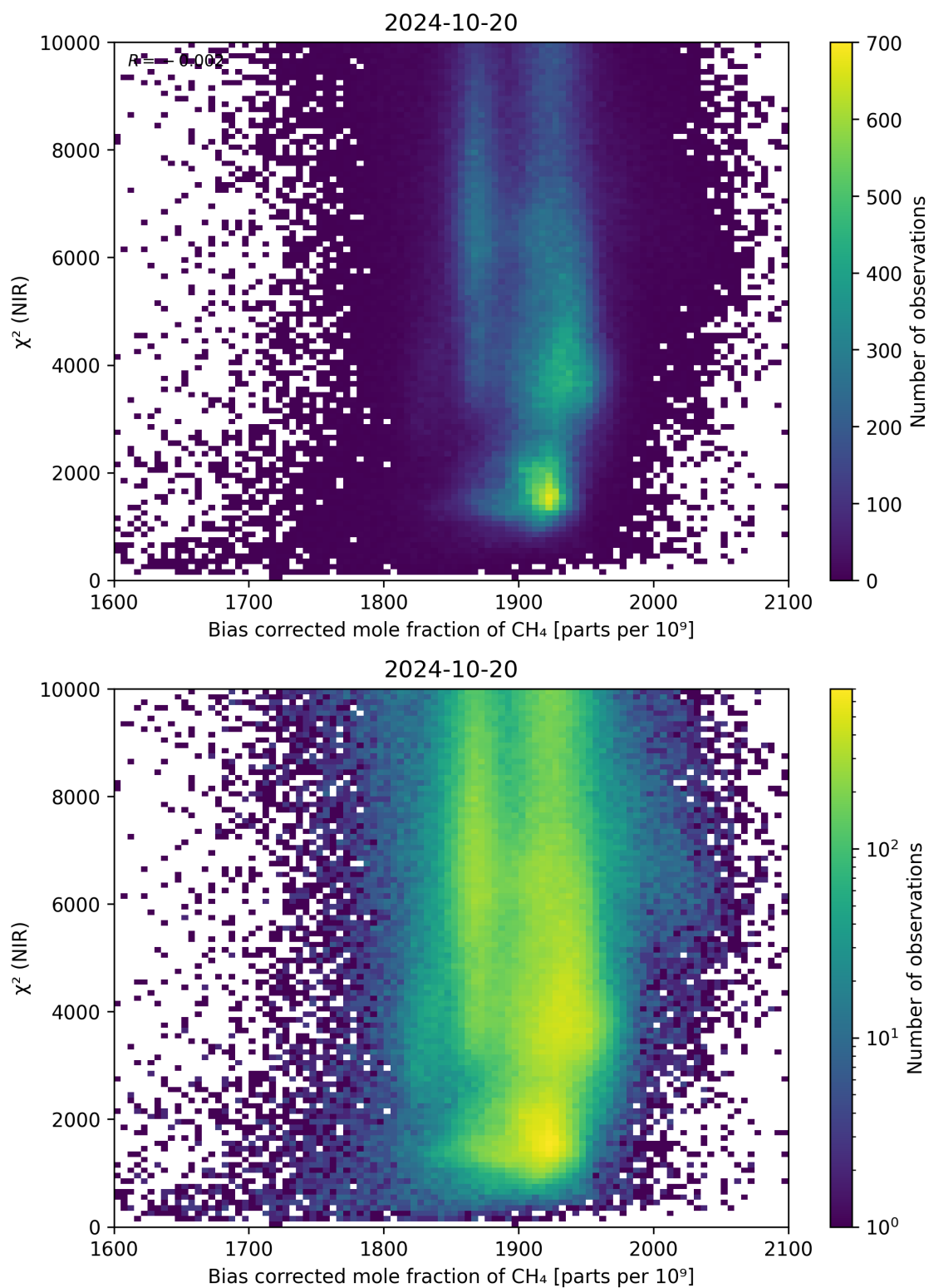
Figure 63: Scatter density plot of “Bias corrected mole fraction of \text{CH}_4 ” against “ \chi^2 (NIR)” for 2024-10-19 to 2024-10-21.
