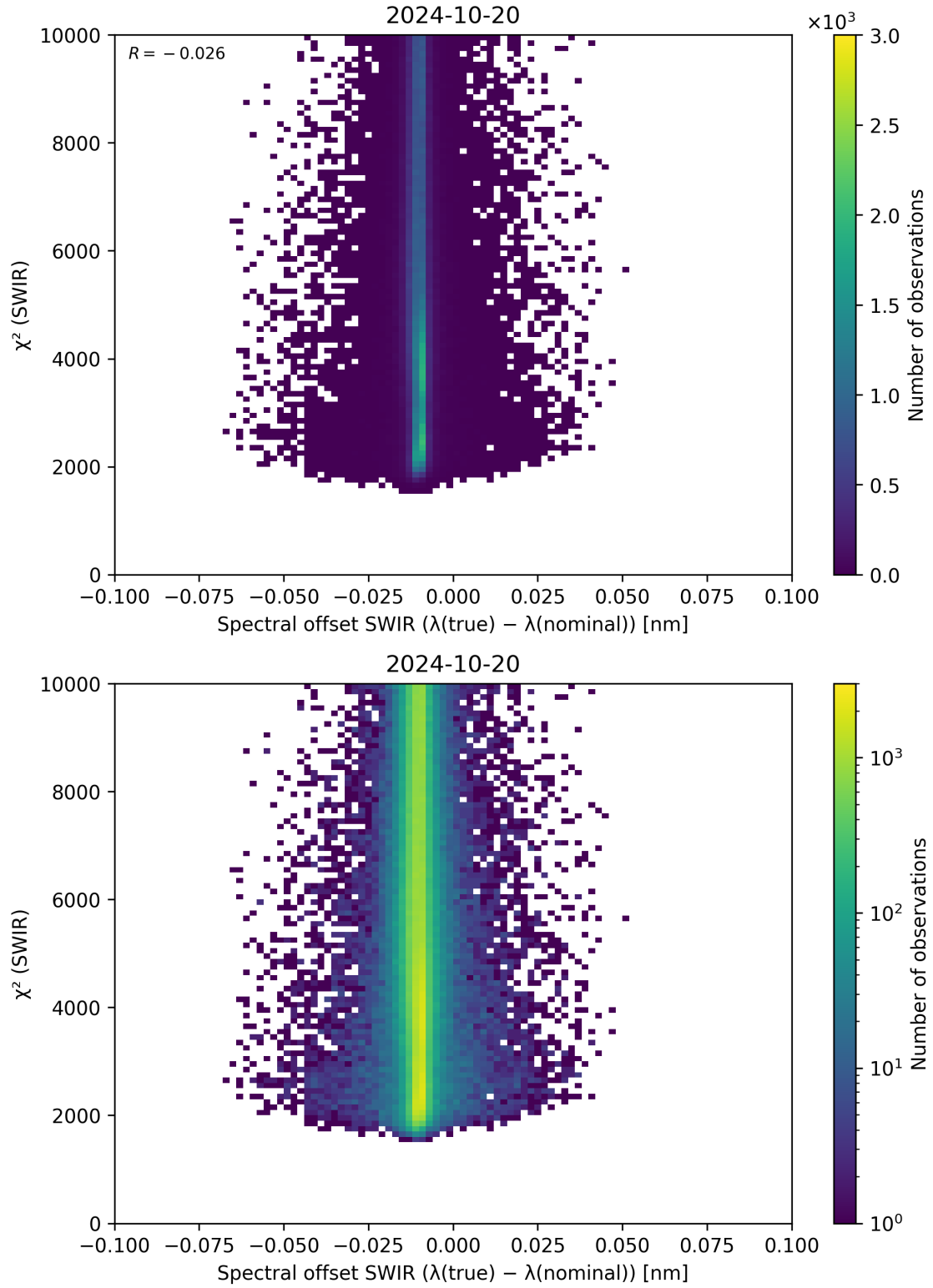
Figure 118: Scatter density plot of “Spectral offset SWIR ( \lambda_{\text{true}} - \lambda_{\text{nominal}} )” against “ \chi^2 (SWIR)” for 2024-10-19 to 2024-10-21.
