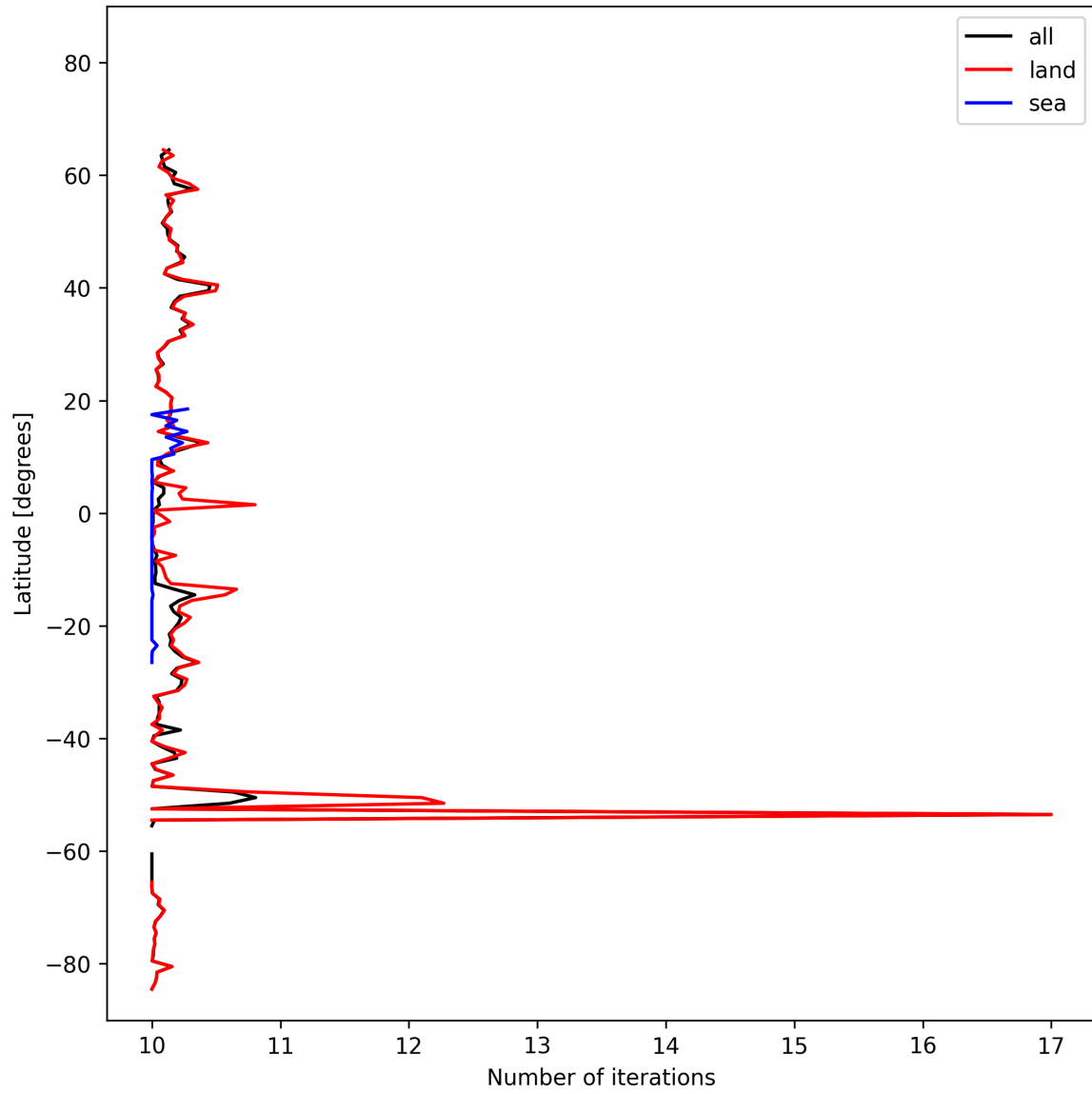
Figure 20: Zonal average of “Number of iterations” for 2024-10-19 to 2024-10-21.
