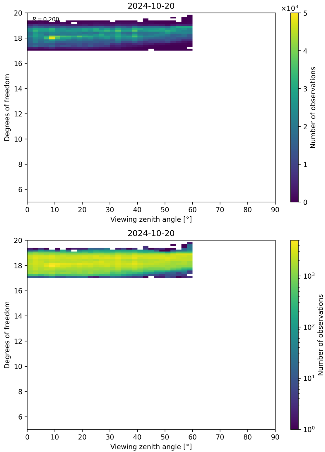
Figure 107: Scatter density plot of “Viewing zenith angle” against “Degrees of freedom” for 2024-10-19 to 2024-10-21.
