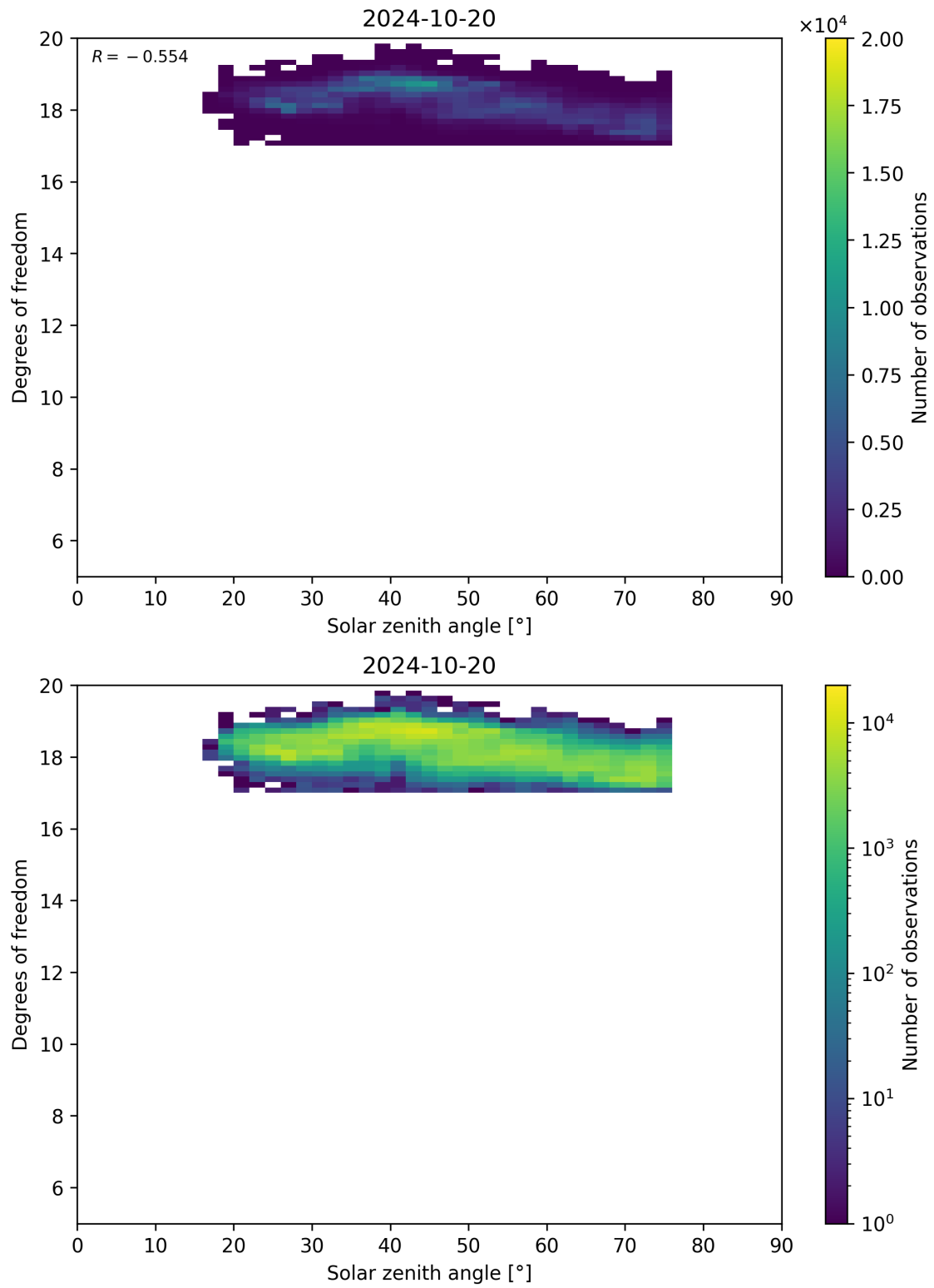
Figure 96: Scatter density plot of “Solar zenith angle” against “Degrees of freedom” for 2024-10-19 to 2024-10-21.
