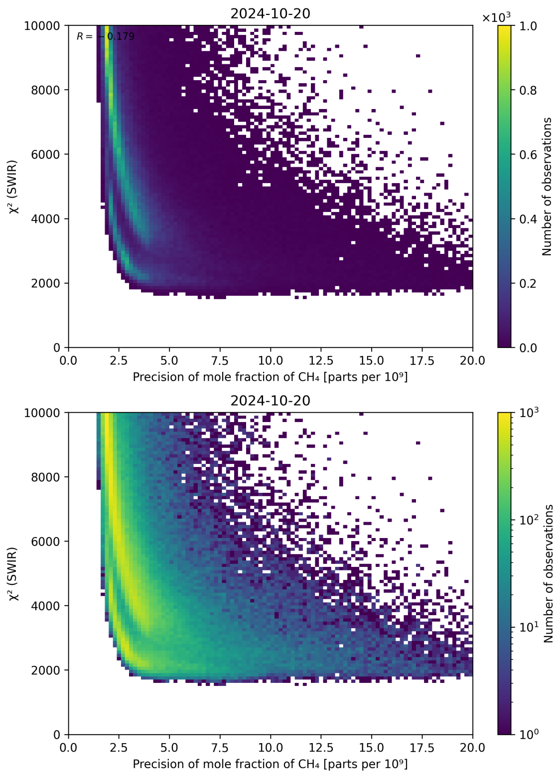
Figure 79: Scatter density plot of “Precision of mole fraction of \text{CH}_4 ” against “ \chi^2 (SWIR)” for 2024-10-19 to 2024-10-21.
