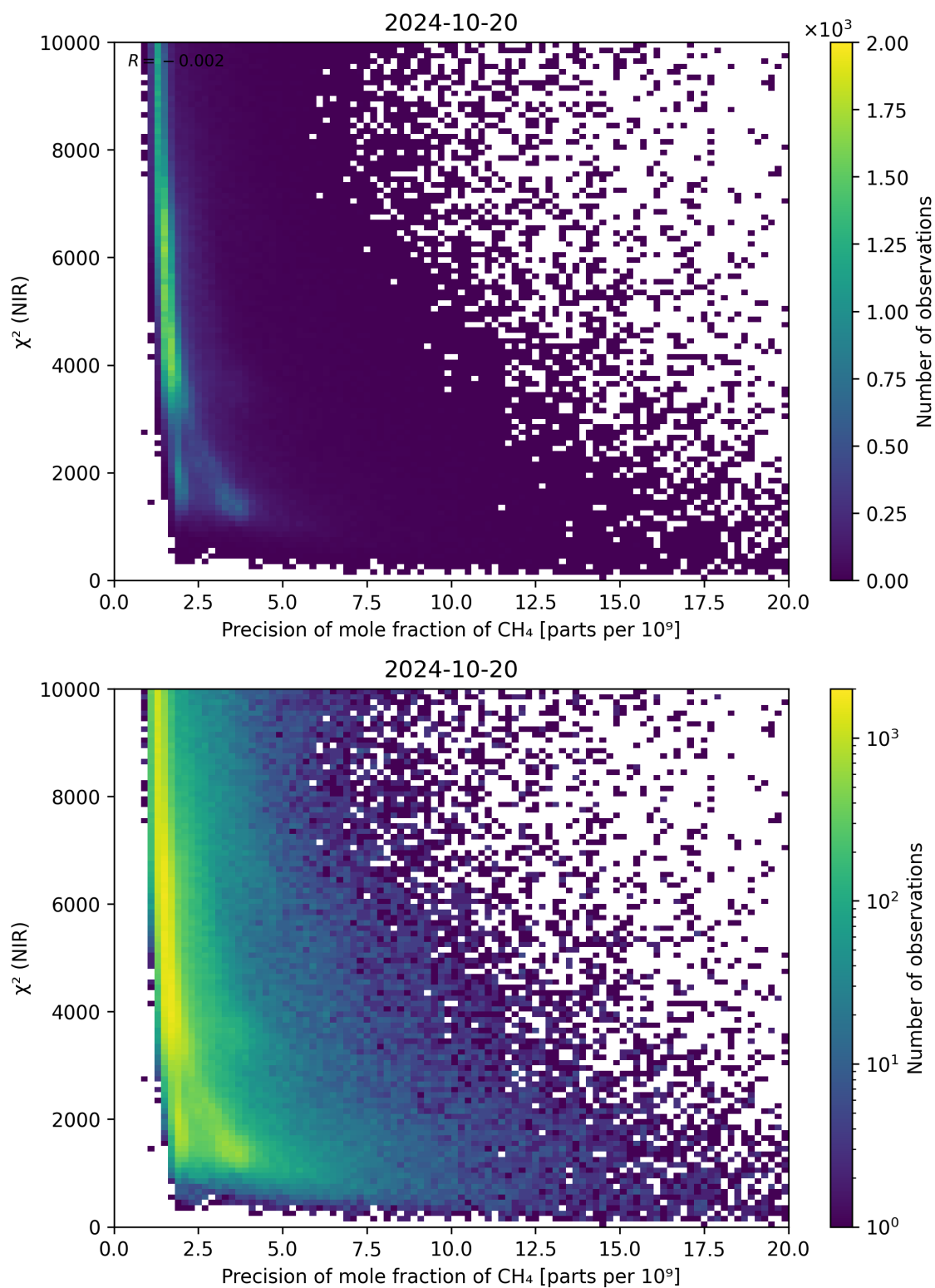
Figure 78: Scatter density plot of “Precision of mole fraction of \text{CH}_4 ” against “ \chi^2 (NIR)” for 2024-10-19 to 2024-10-21.
