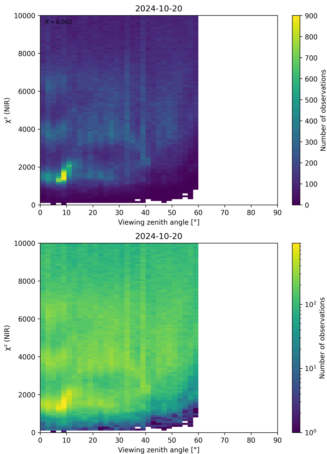
Figure 105: Scatter density plot of “Viewing zenith angle” against “ \chi^2 (NIR)” for 2024-10-19 to 2024-10-21.
