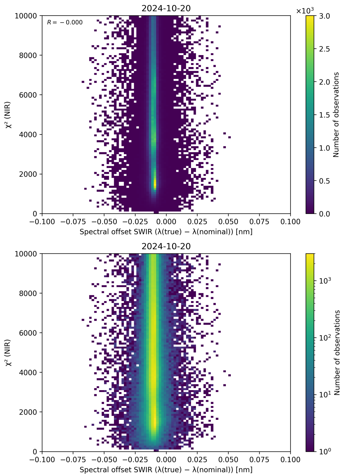
Figure 117: Scatter density plot of “Spectral offset SWIR ( \lambda_{\text{true}} - \lambda_{\text{nominal}} )” against “ \chi^2 (NIR)” for 2024-10-19 to 2024-10-21.
