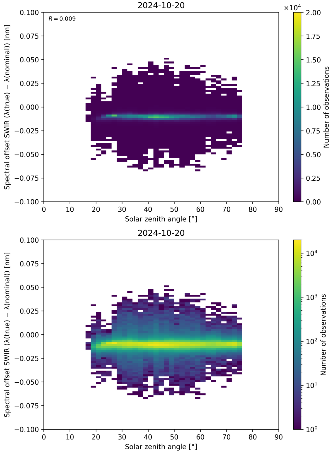
Figure 104: Scatter density plot of “Solar zenith angle” against “Spectral offset SWIR ( \lambda_{\text{true}} - \lambda_{\text{nominal}} )” for 2024-10-19 to 2024-10-21.
