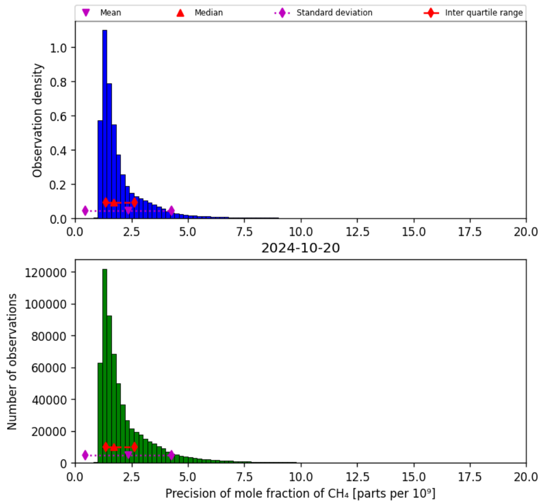
Figure 24: Histogram of “Precision of mole fraction of CH 4 ” for 2024-10-19 to 2024-10-21
