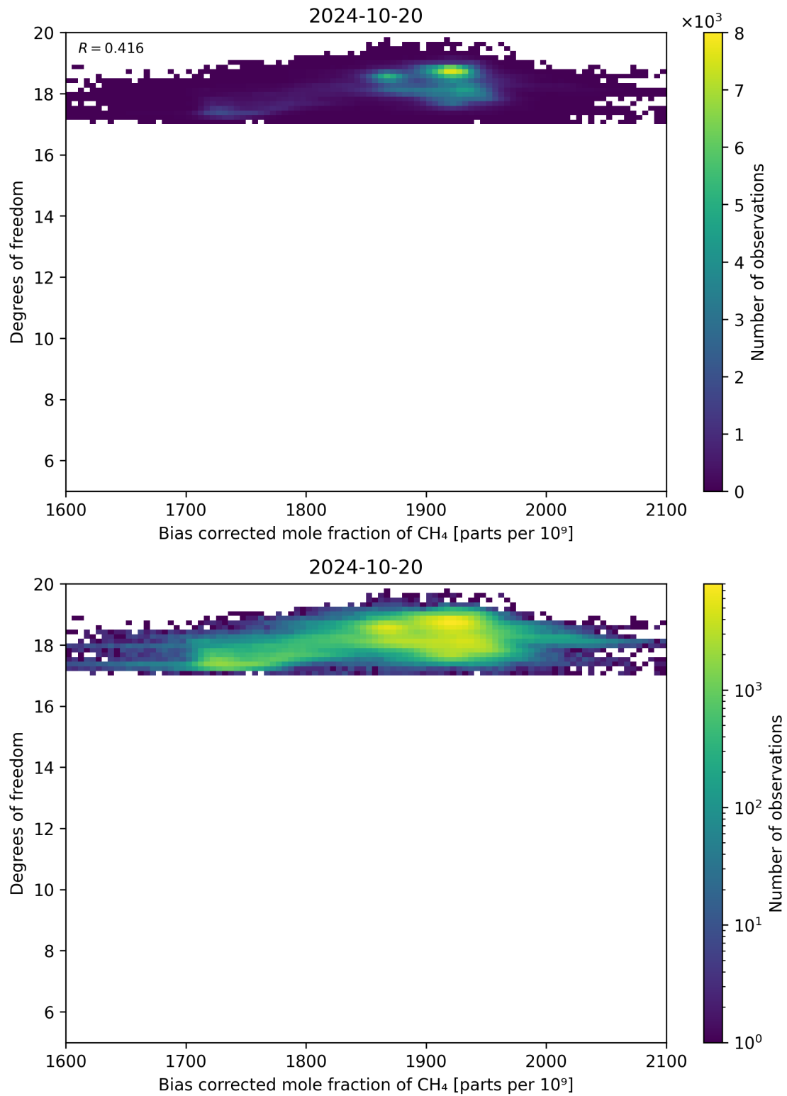
Figure 65: Scatter density plot of “Bias corrected mole fraction of CH 4 ” against “Degrees of freedom” for 2024-10-19 to 2024-10-21.
