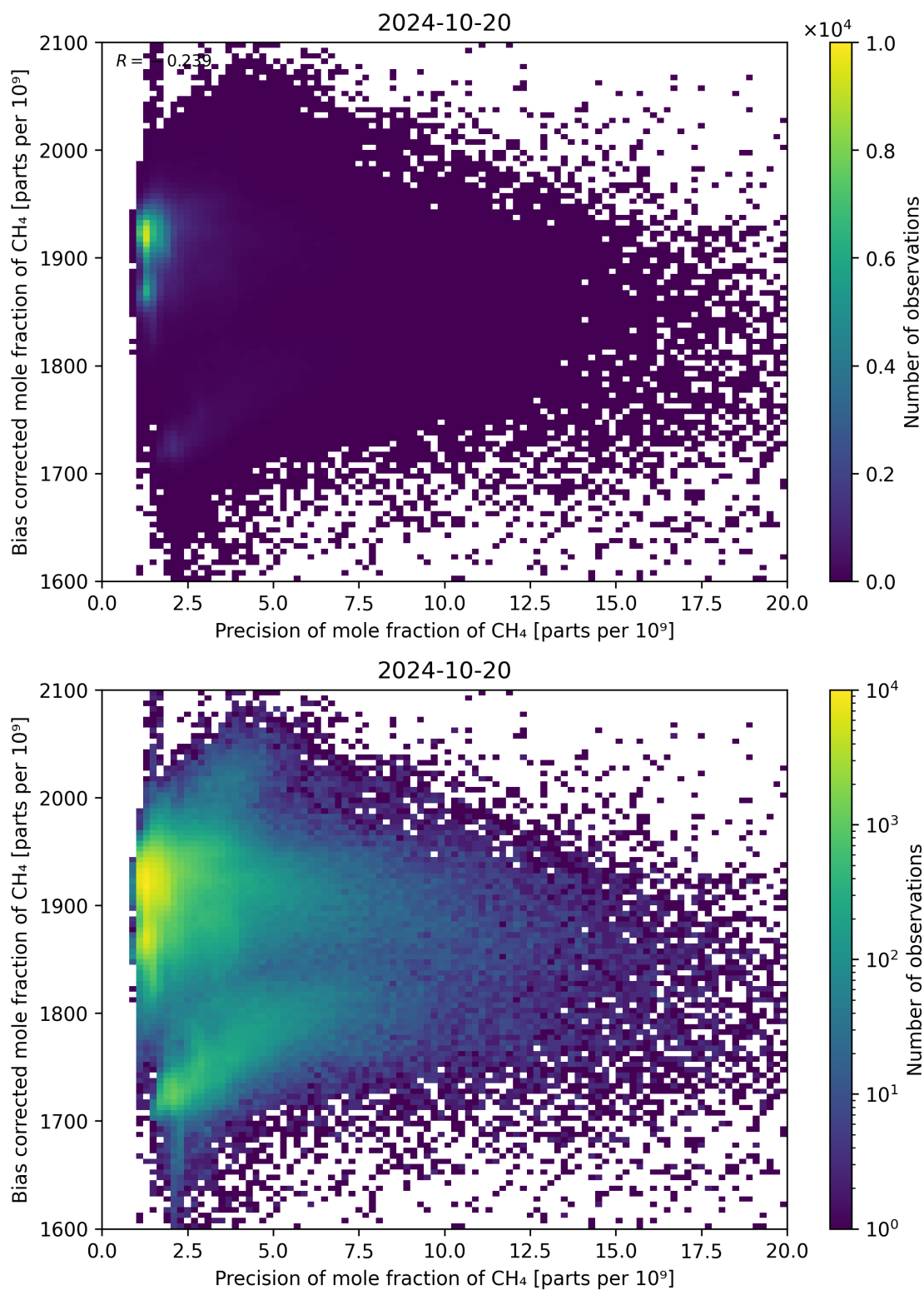
Figure 82: Scatter density plot of “Precision of mole fraction of CH 4 ” against “Bias corrected mole fraction of CH 4 ” for 2024-10-19 to 2024-10-21.
