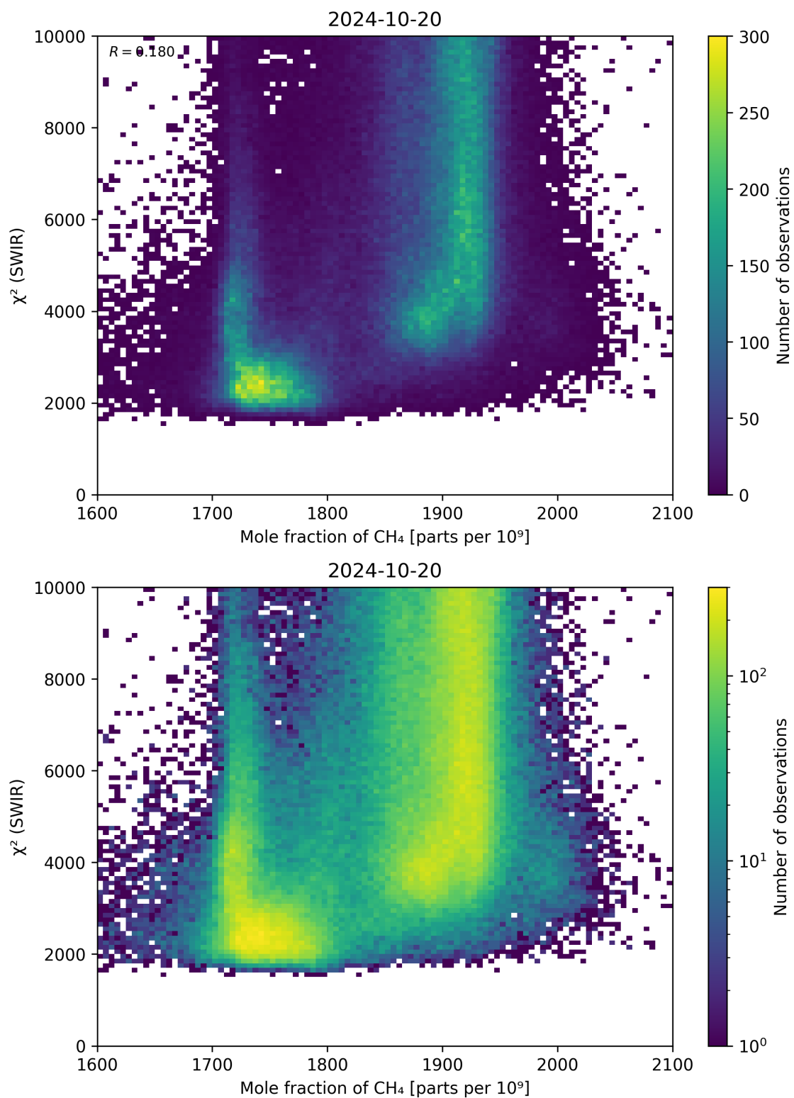
Figure 71: Scatter density plot of “Mole fraction of CH 4 ” against “ \chi^2 (SWIR)” for 2024-10-19 to 2024-10-21.
