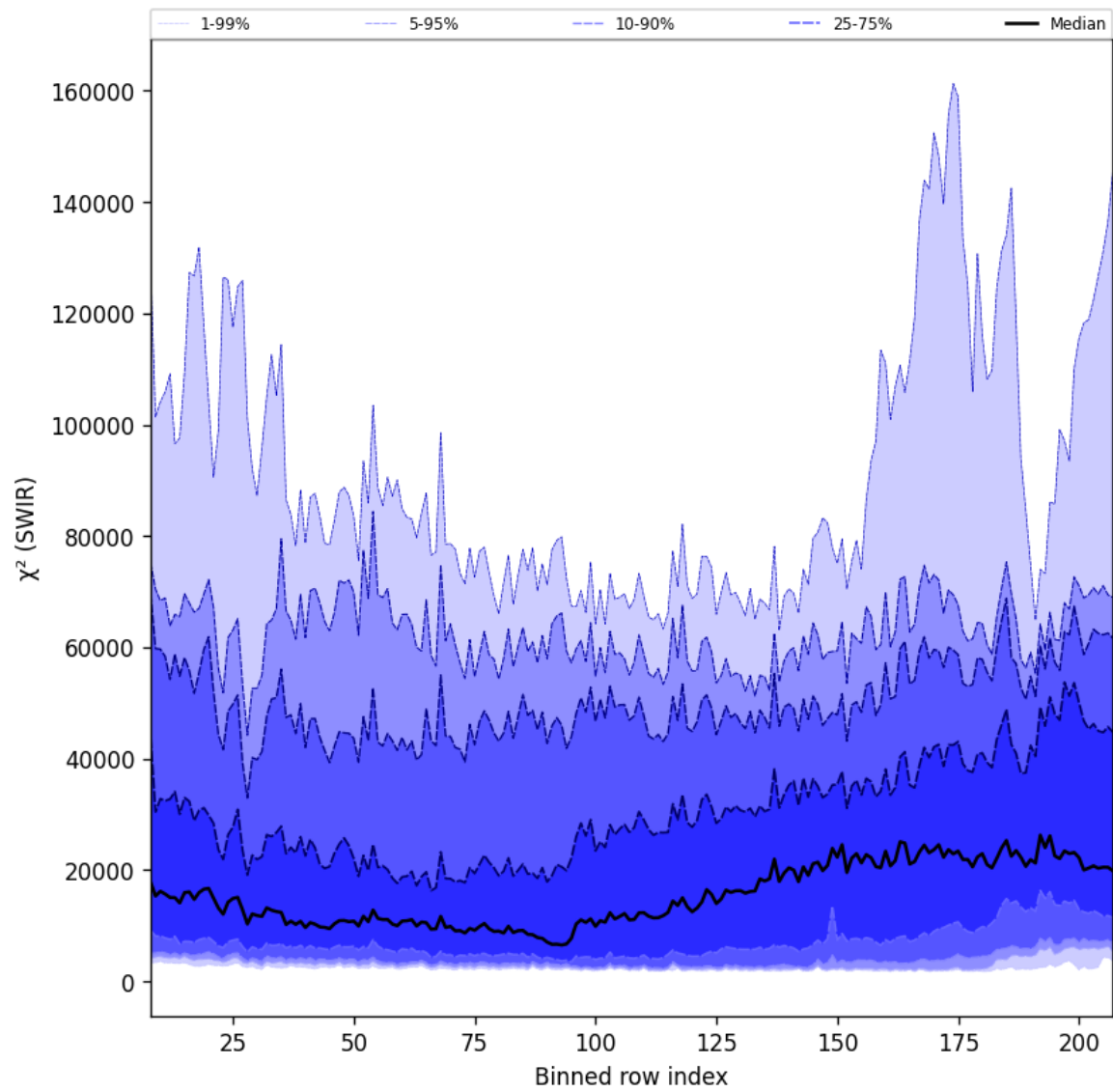
Figure 39: Along track statistics of “ \chi^2 (SWIR)” for 2024-10-19 to 2024-10-21
