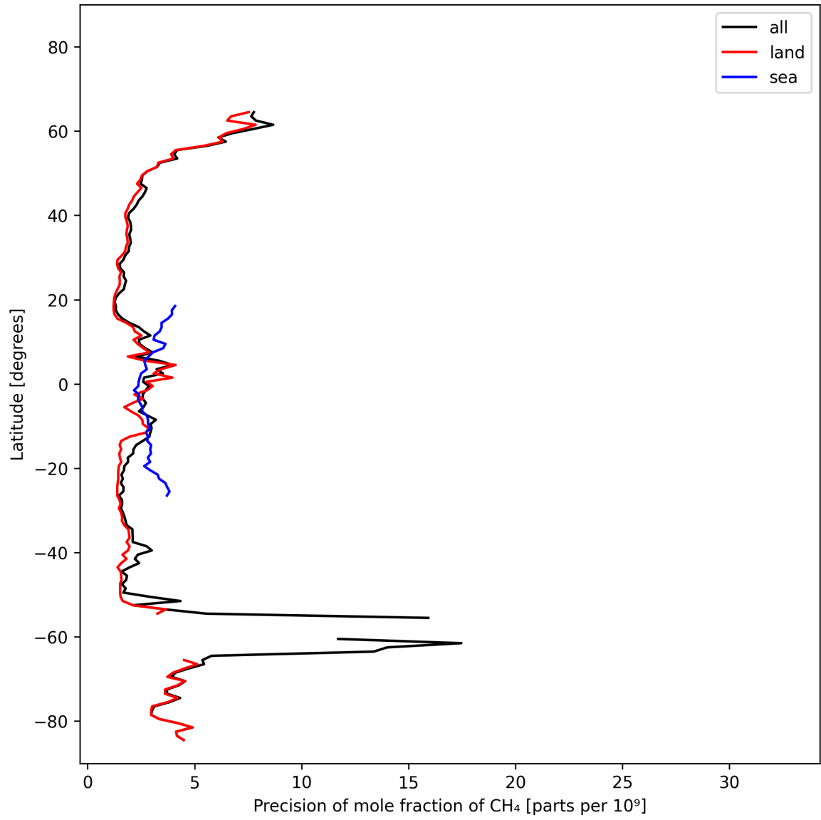
Figure 13: Zonal average of “Precision of mole fraction of CH 4 ” for 2024-10-19 to 2024-10-21.
