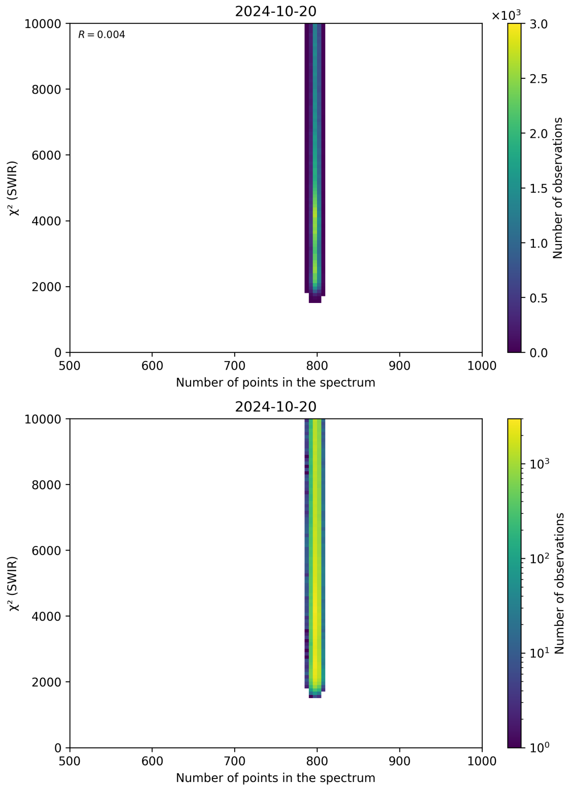
Figure 89: Scatter density plot of “Number of points in the spectrum” against “ \chi^2 (SWIR)” for 2024-10-19 to 2024-10-21.
