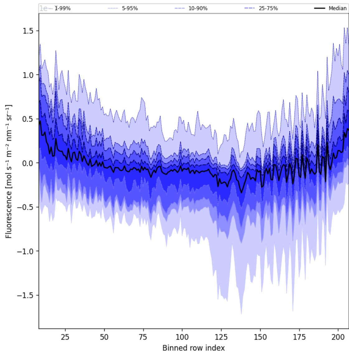
Figure 43: Along track statistics of “Fluorescence” for 2024-10-19 to 2024-10-21
