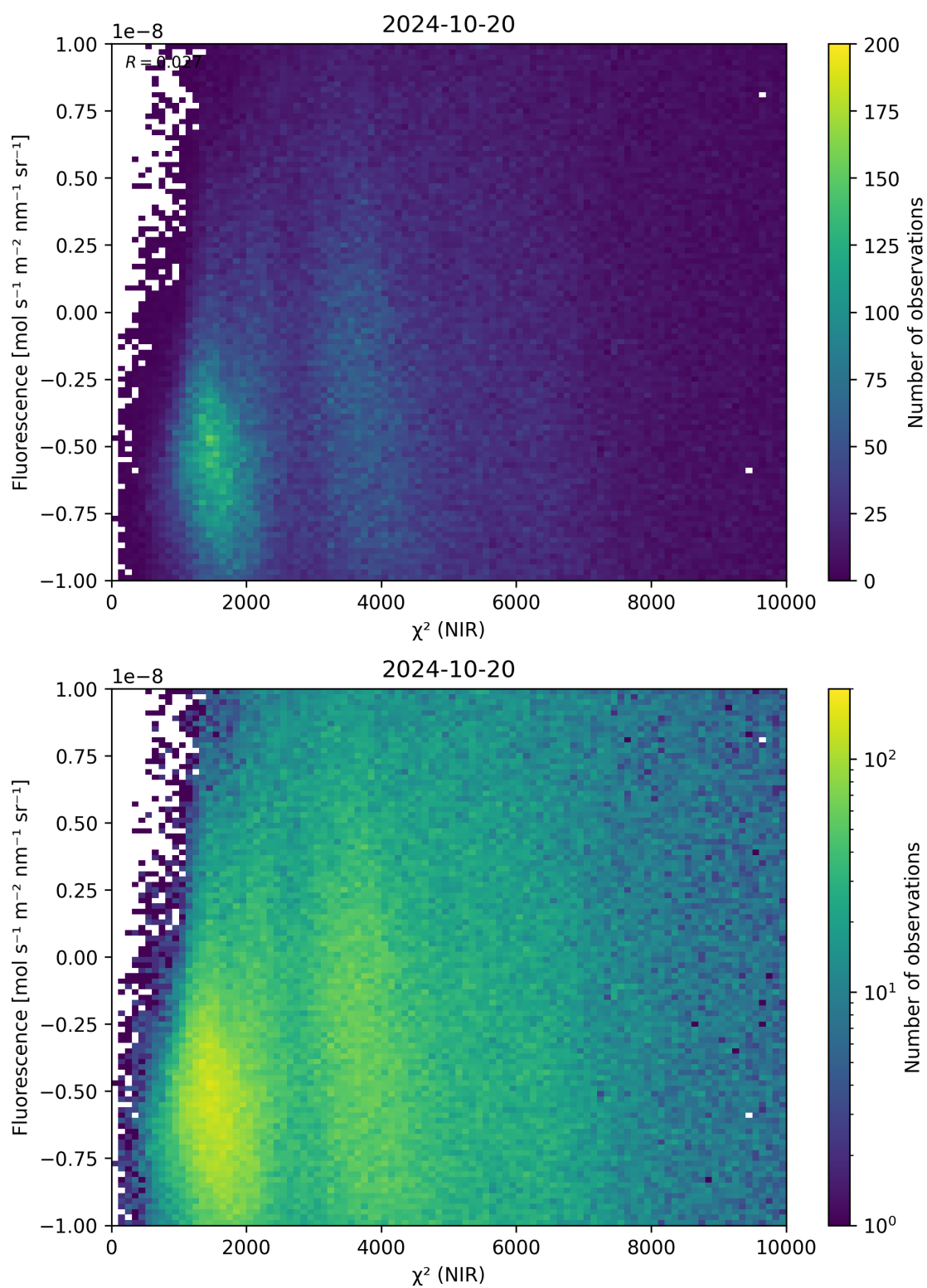
Figure 45: Scatter density plot of “ \chi^2 (NIR)” against “Fluorescence” for 2024-10-19 to 2024-10-21.
