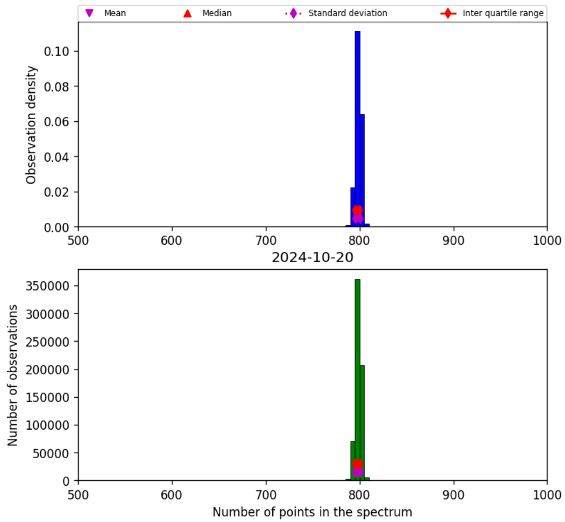
Figure 26: Histogram of “Number of points in the spectrum” for 2024-10-19 to 2024-10-21
