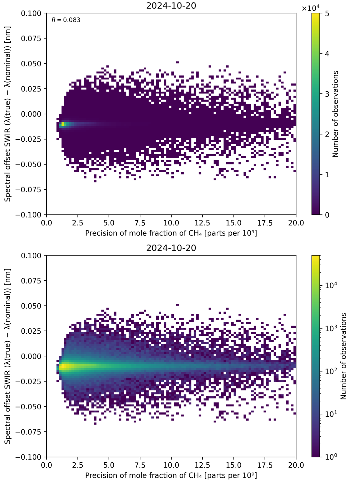
Figure 85: Scatter density plot of “Precision of mole fraction of \text{CH}_4 ” against “Spectral offset SWIR ( \lambda_{\text{true}} - \lambda_{\text{nominal}} )” for 2024-10-19 to 2024-10-21.
