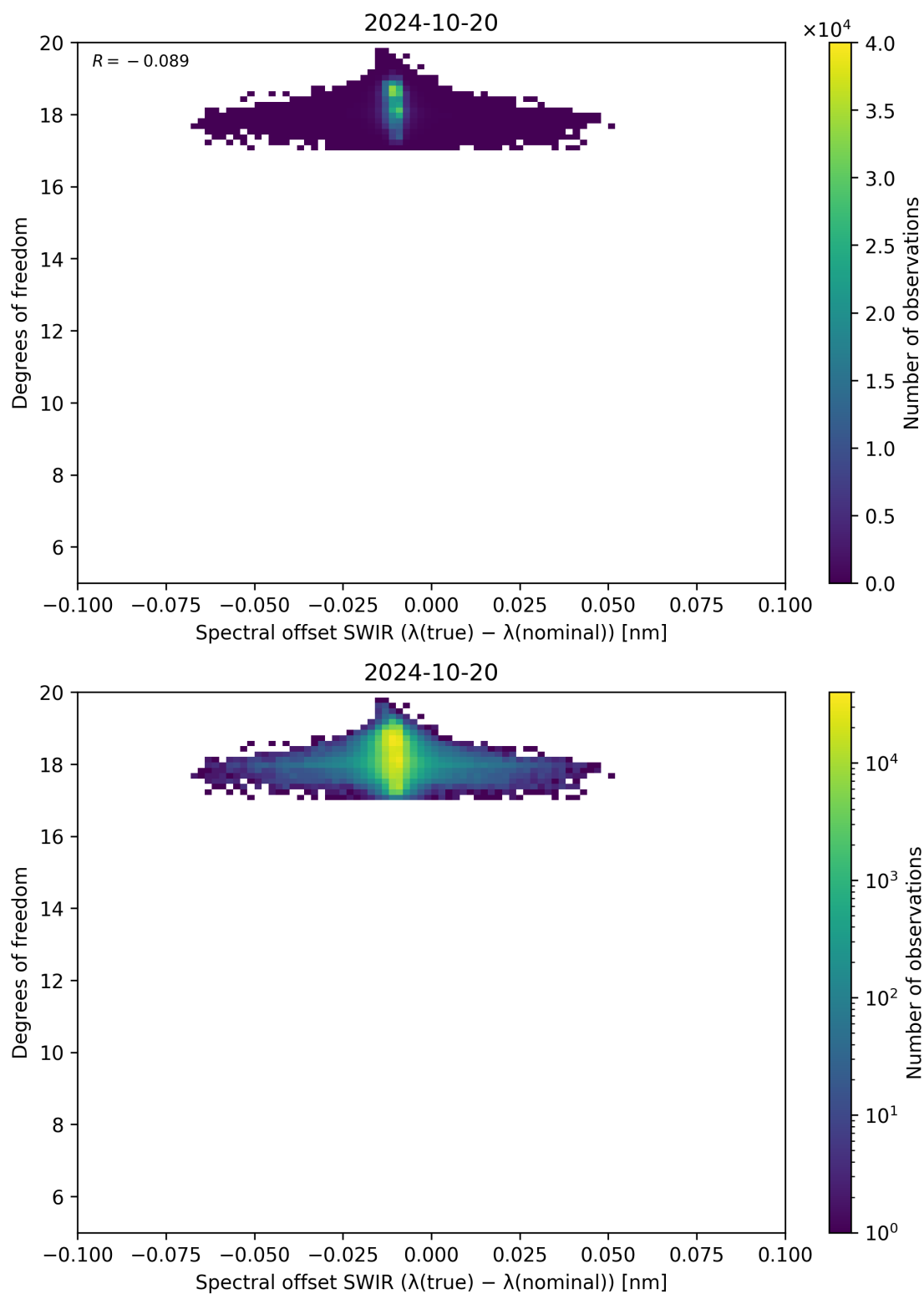
Figure 119: Scatter density plot of “Spectral offset SWIR ( \lambda_{\text{true}} - \lambda_{\text{nominal}} )” against “Degrees of freedom” for 2024-10-19 to 2024-10-21.
