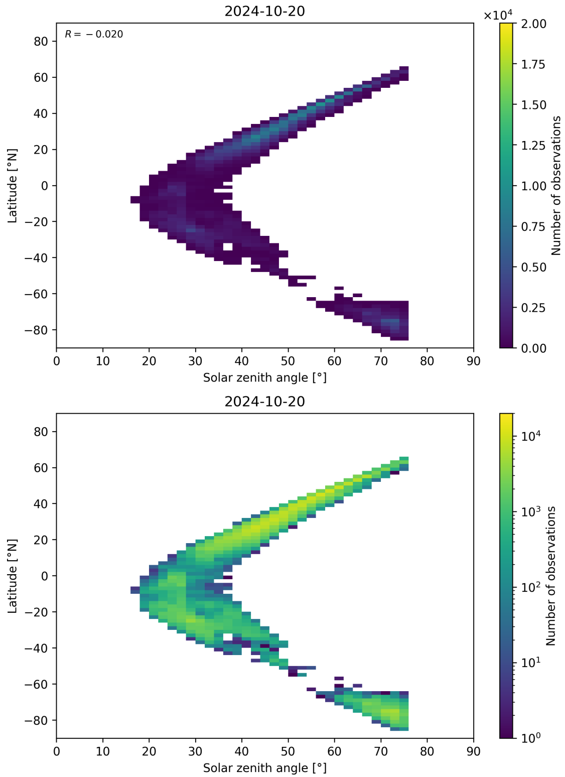
Figure 98: Scatter density plot of “Solar zenith angle” against “Latitude” for 2024-10-19 to 2024-10-21.
