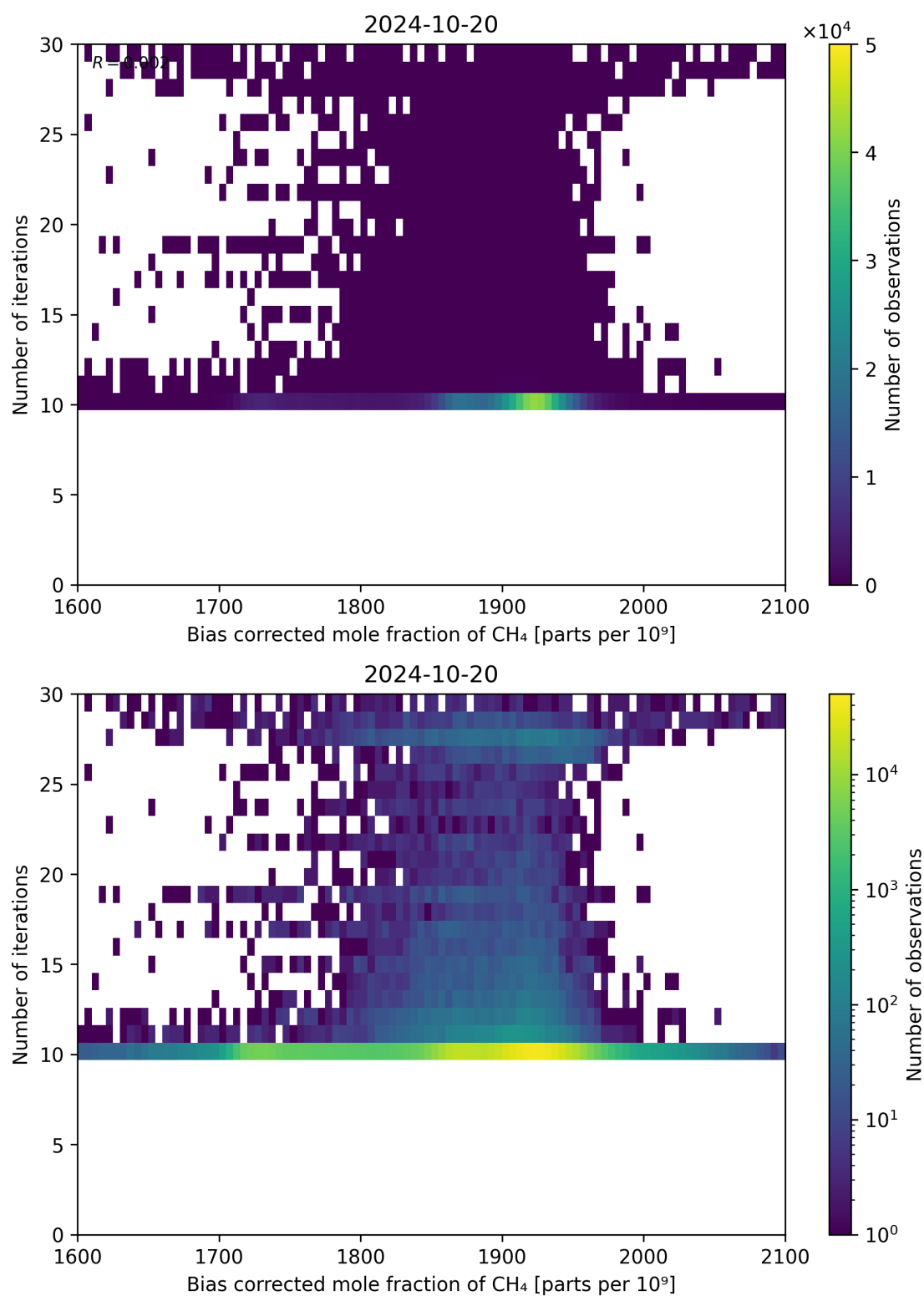
Figure 67: Scatter density plot of “Bias corrected mole fraction of \text{CH}_4 ” against “Number of iterations” for 2024-10-19 to 2024-10-21.
