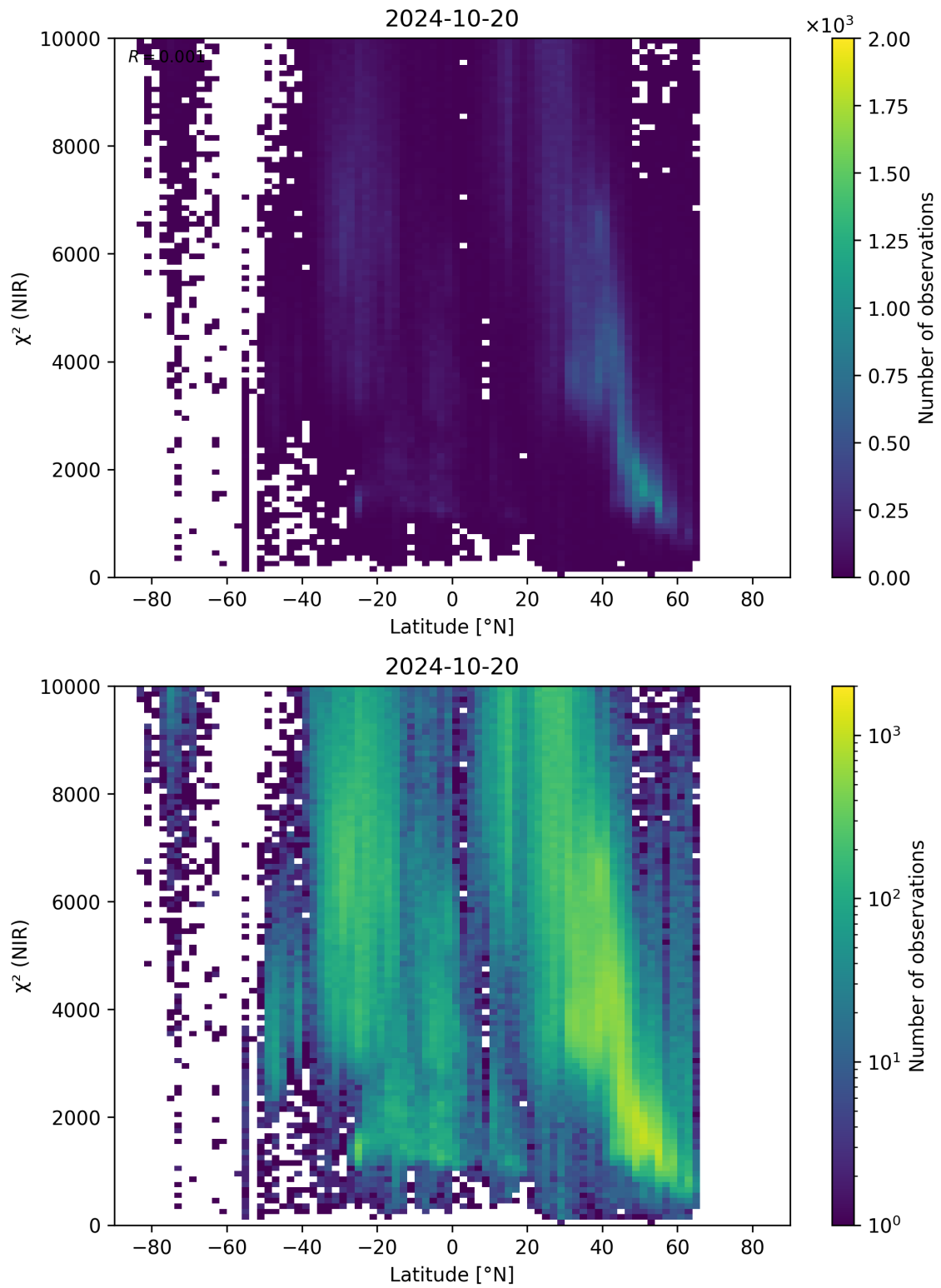
Figure 53: Scatter density plot of “Latitude” against “ \chi^2 (NIR)” for 2024-10-19 to 2024-10-21.
