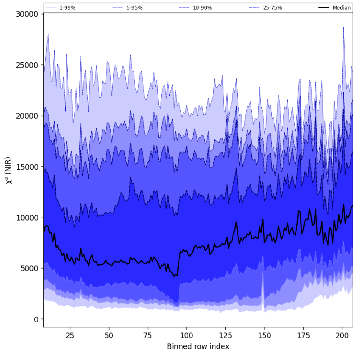
Figure 40: Along track statistics of “ \chi^2 (NIR)” for 2024-10-19 to 2024-10-21
