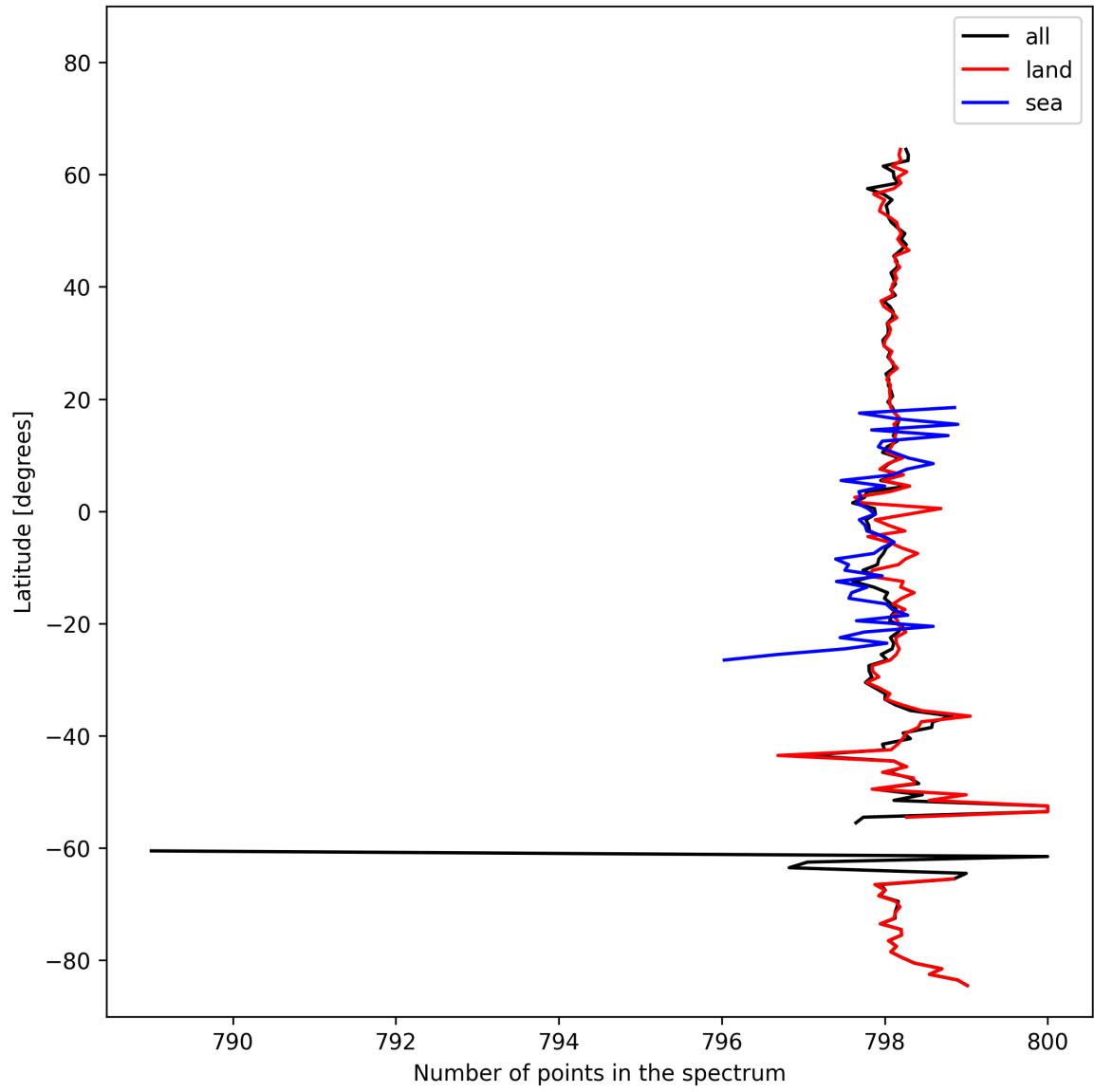
Figure 15: Zonal average of “Number of points in the spectrum” for 2024-10-19 to 2024-10-21.
