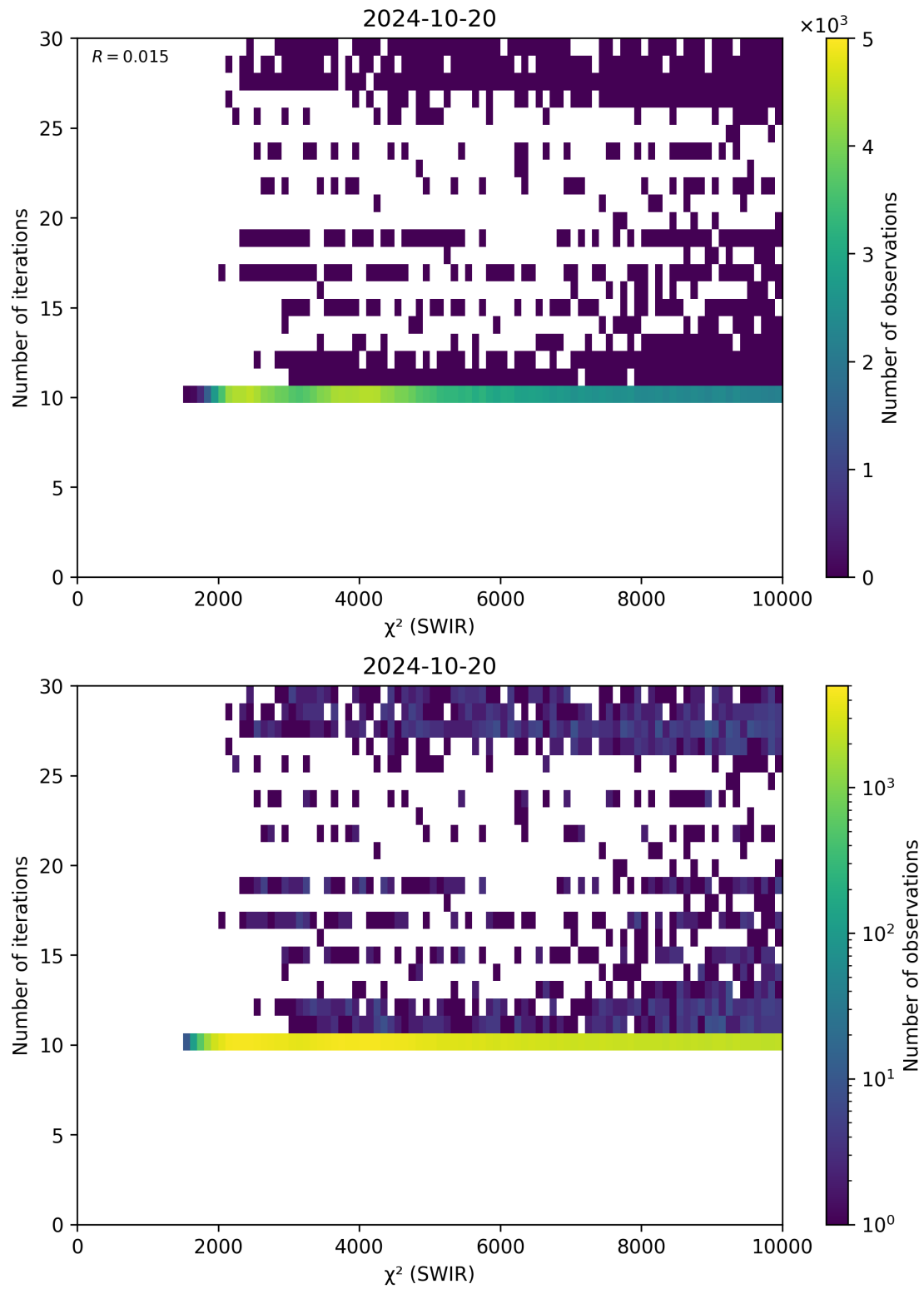
Figure 50: Scatter density plot of “ \chi^2 (SWIR)” against “Number of iterations” for 2024-10-19 to 2024-10-21.
