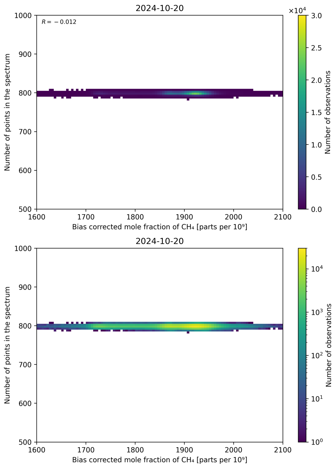
Figure 68: Scatter density plot of “Bias corrected mole fraction of CH 4 ” against “Number of points in the spectrum” for 2024-10-19 to 2024-10-21.
