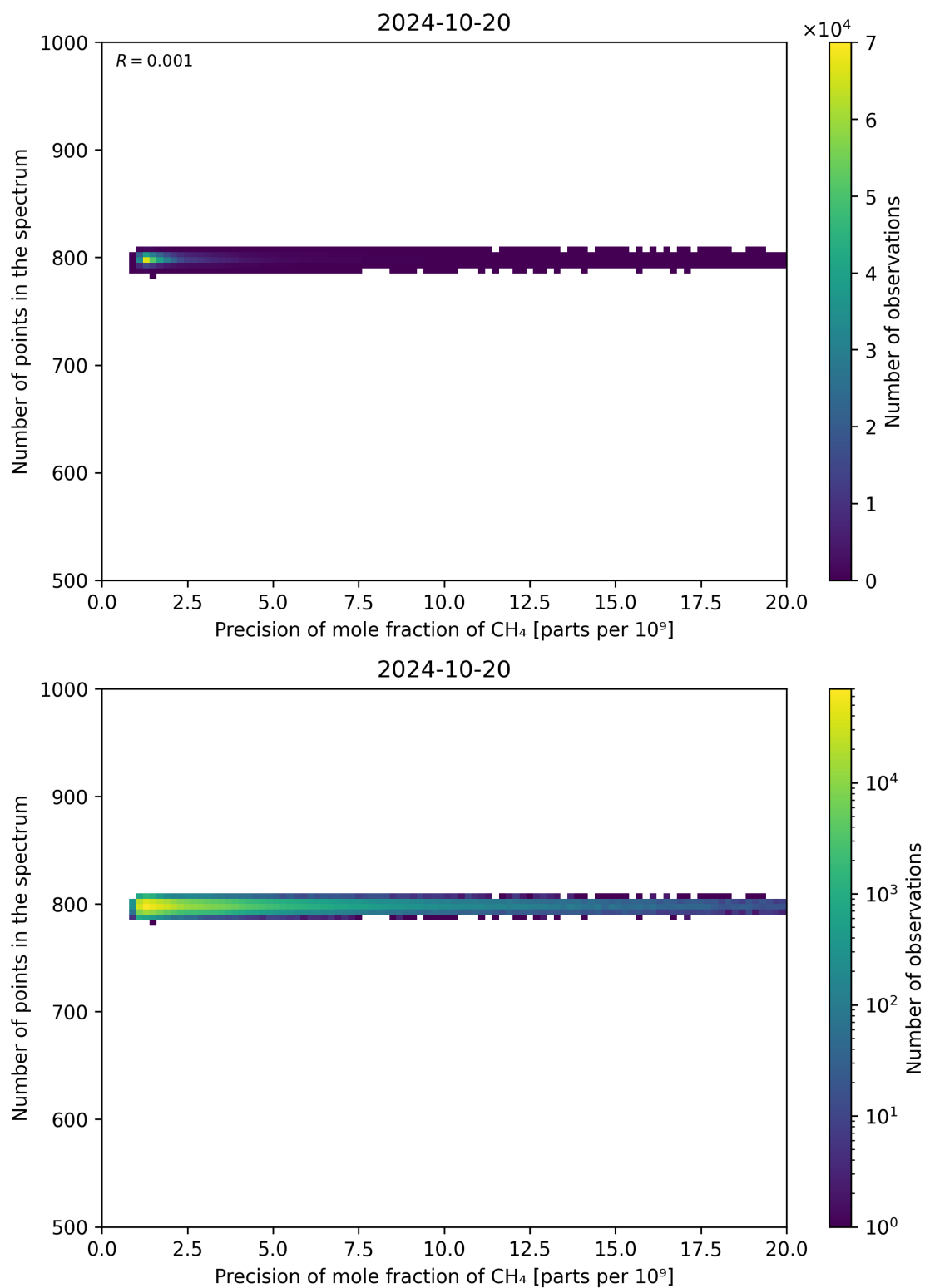
Figure 84: Scatter density plot of “Precision of mole fraction of CH 4 ” against “Number of points in the spectrum” for 2024-10-19 to 2024-10-21.
