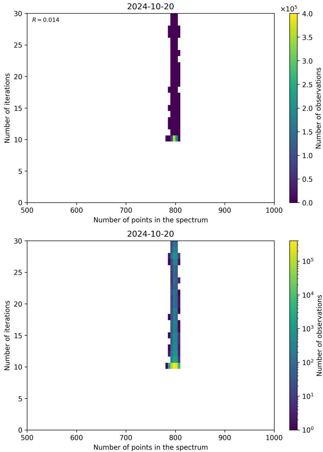
Figure 92: Scatter density plot of “Number of points in the spectrum” against “Number of iterations” for 2024-10-19 to 2024-10-21.
