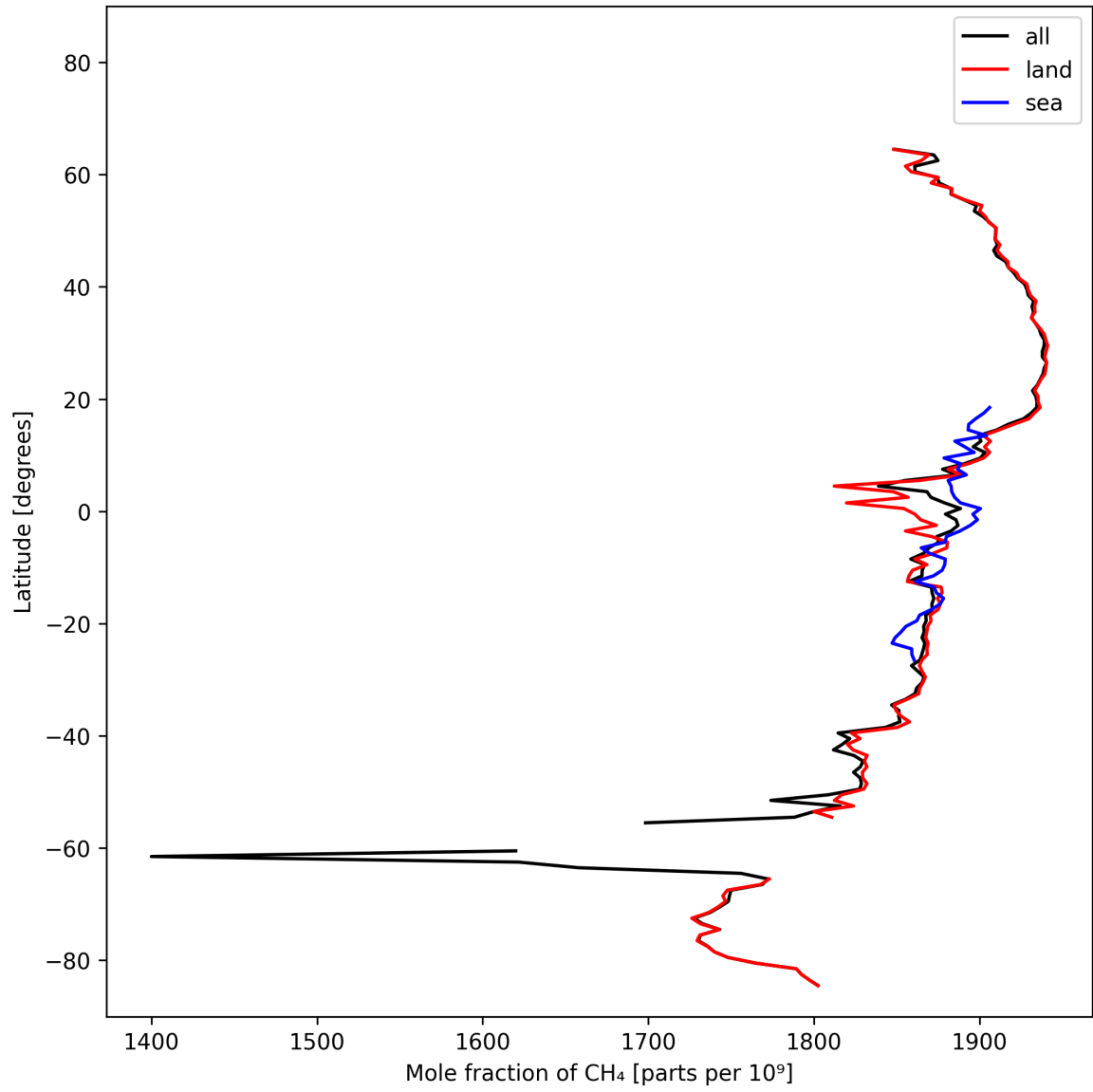
Figure 12: Zonal average of “Mole fraction of CH 4 ” for 2024-10-19 to 2024-10-21.
