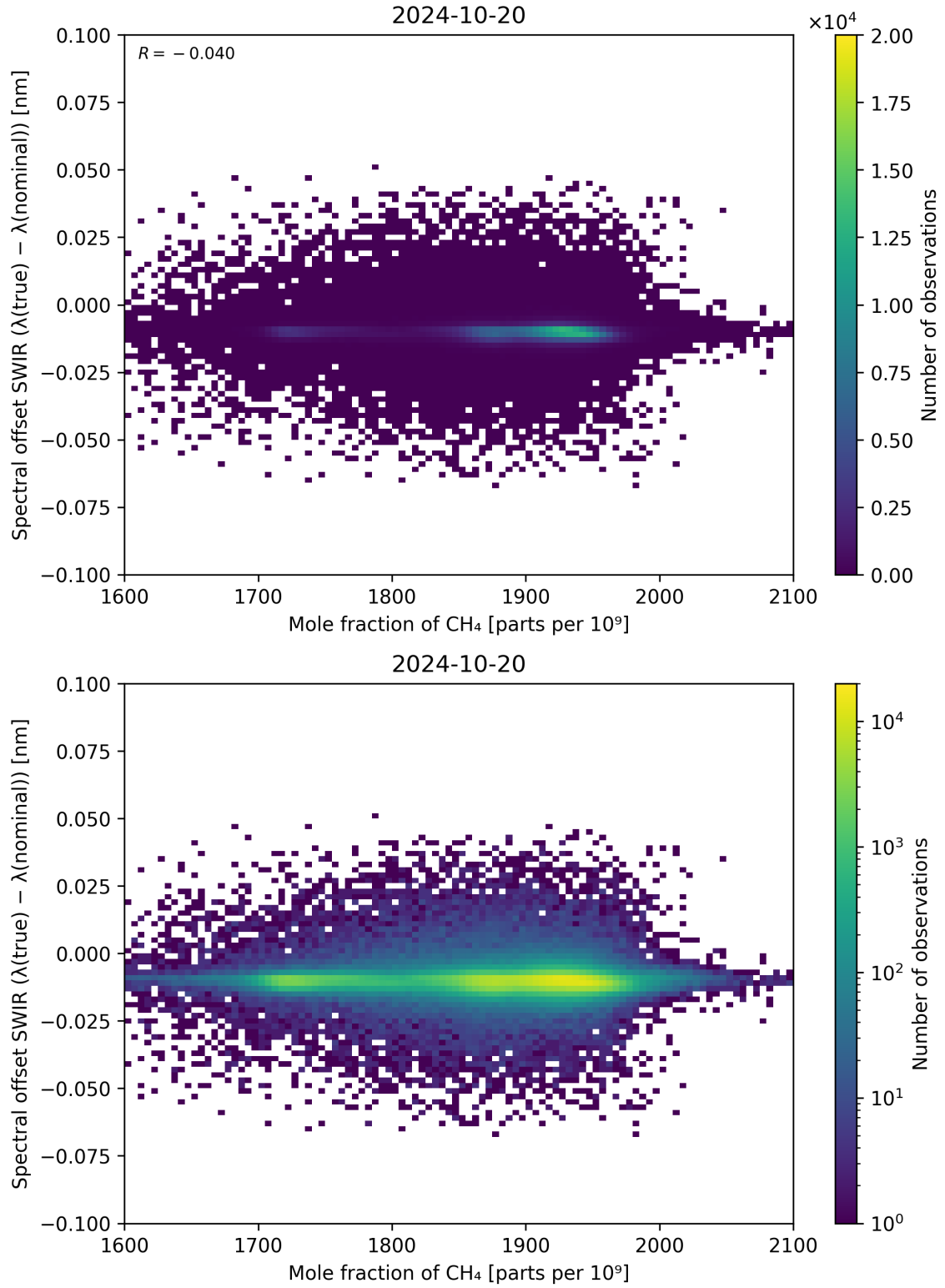
Figure 86: Scatter density plot of “Mole fraction of CH 4 ” against “Spectral offset SWIR ( \lambda_{\text{true}} - \lambda_{\text{nominal}} )” for 2024-10-19 to 2024-10-21.
