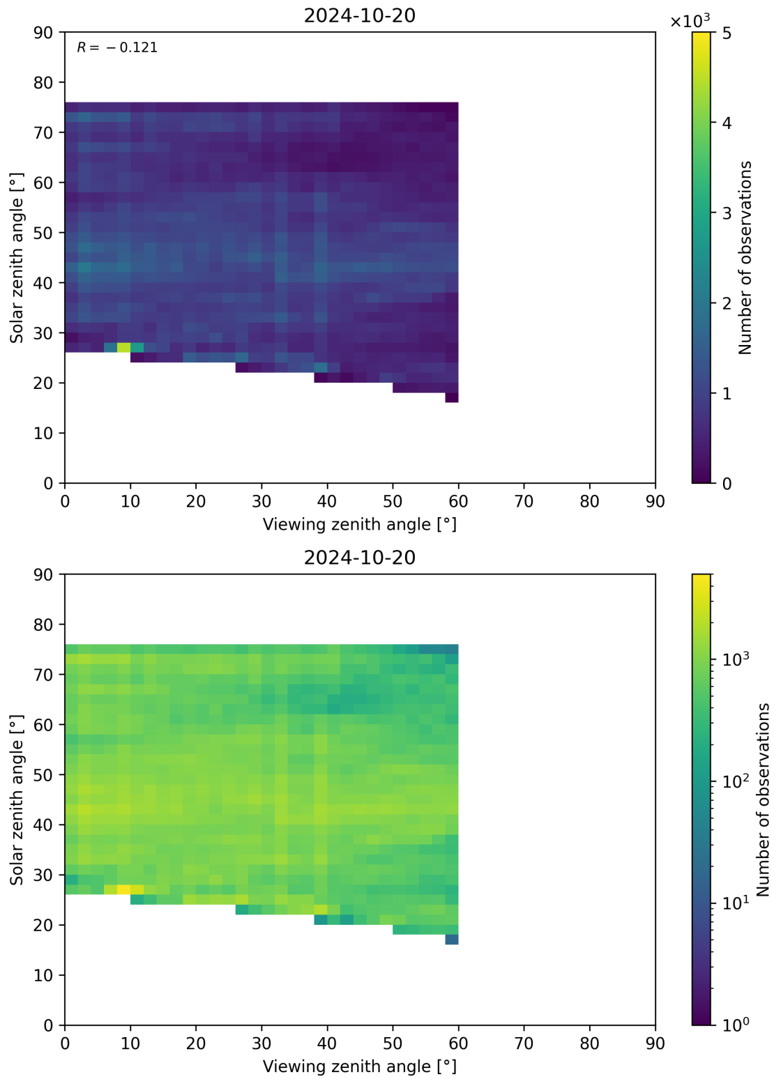
Figure 115: Scatter density plot of “Viewing zenith angle” against “Solar zenith angle” for 2024-10-19 to 2024-10-21.
