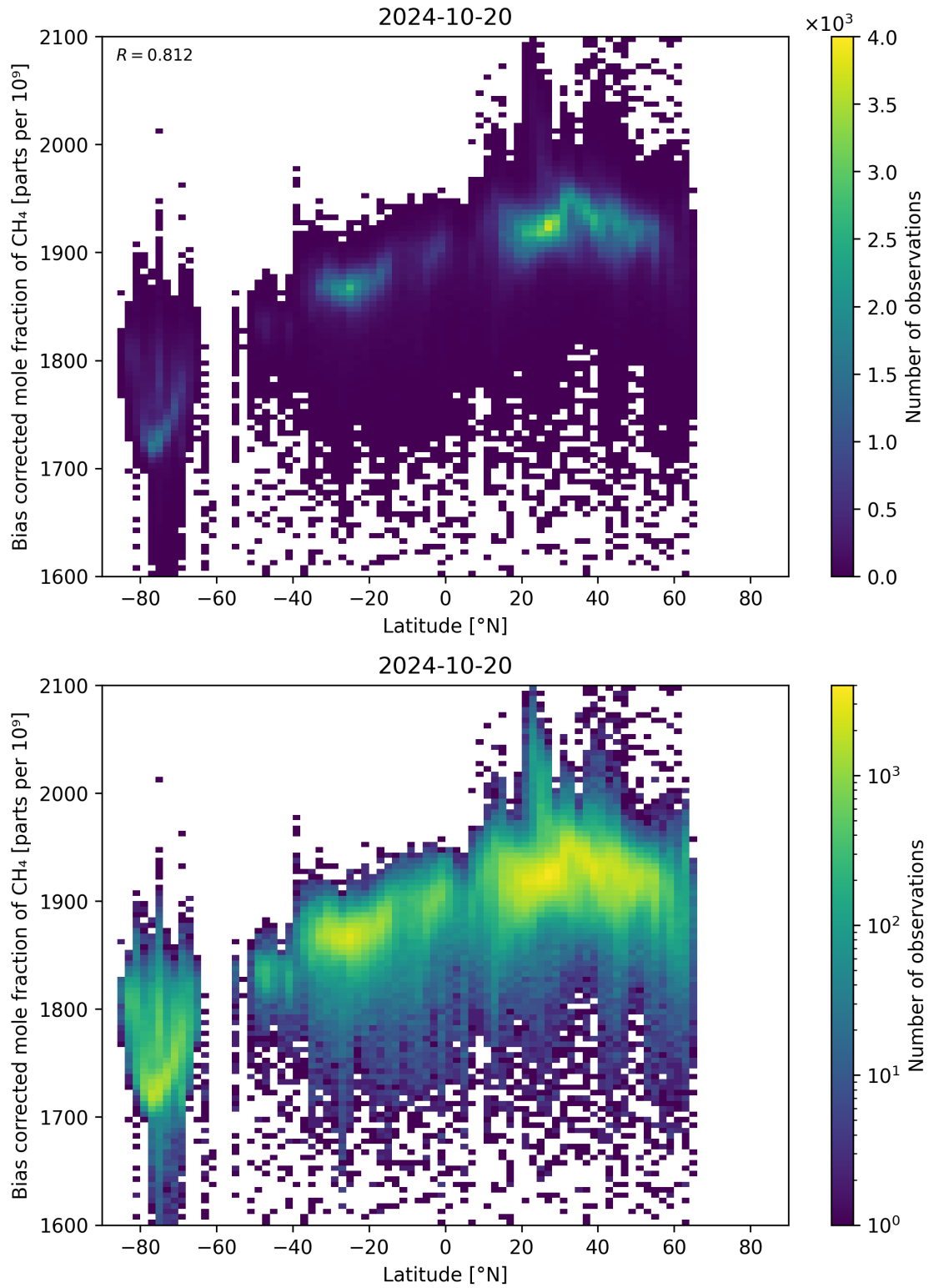
Figure 58: Scatter density plot of “Latitude” against “Bias corrected mole fraction of \text{CH}_4 ” for 2024-10-19 to 2024-10-21.
