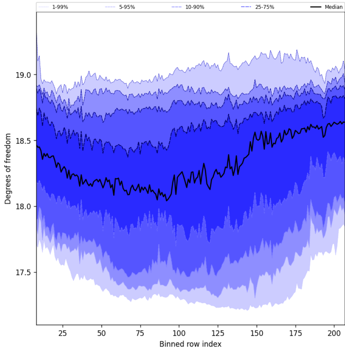
Figure 41: Along track statistics of “Degrees of freedom” for 2024-10-19 to 2024-10-21
