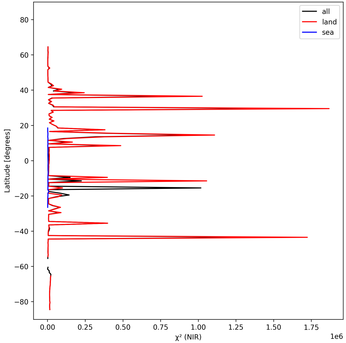
Figure 18: Zonal average of “ \chi^2 (NIR)” for 2024-10-19 to 2024-10-21.
