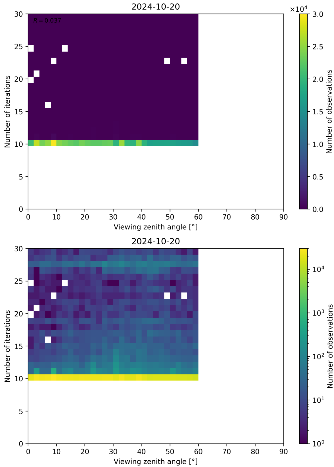
Figure 113: Scatter density plot of “Viewing zenith angle” against “Number of iterations” for 2024-10-19 to 2024-10-21.
