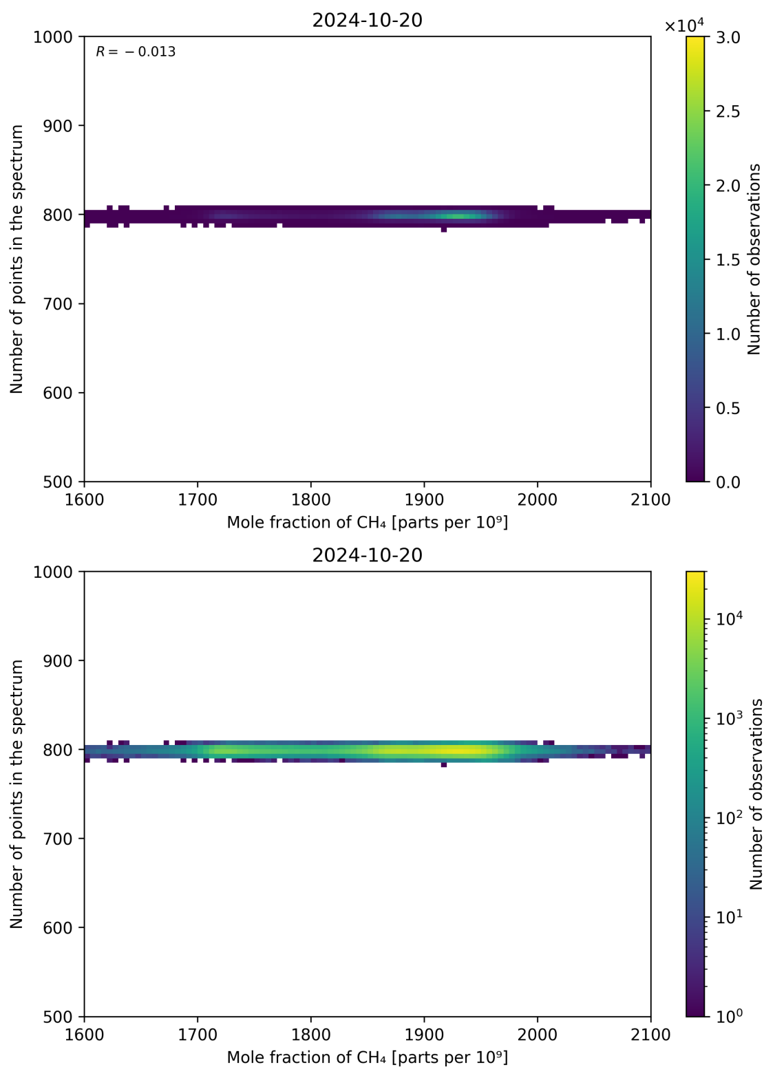
Figure 77: Scatter density plot of “Mole fraction of CH 4 ” against “Number of points in the spectrum” for 2024-10-19 to 2024-10-21.
