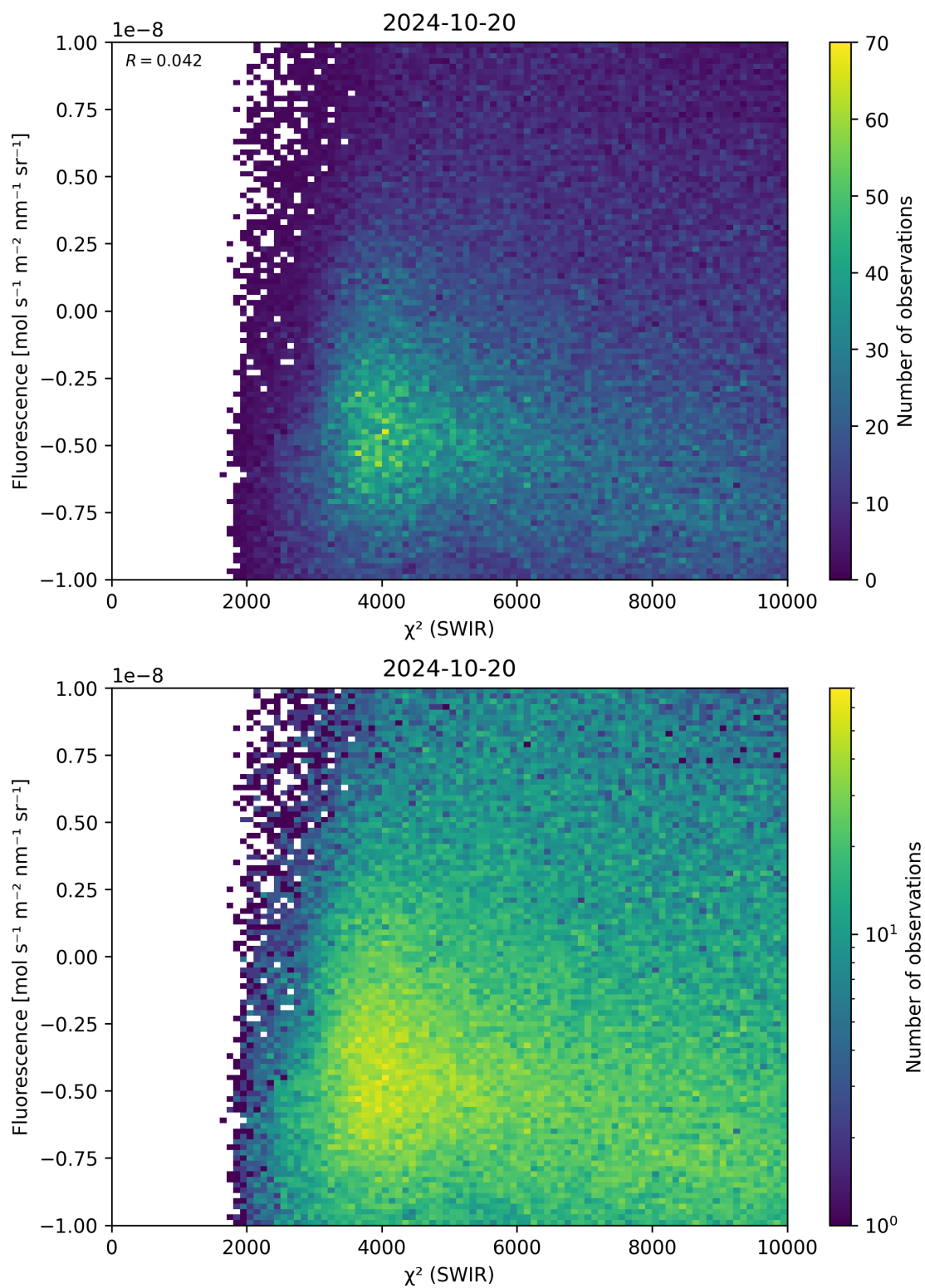
Figure 49: Scatter density plot of “ \chi^2 (SWIR)” against “Fluorescence” for 2024-10-19 to 2024-10-21.
