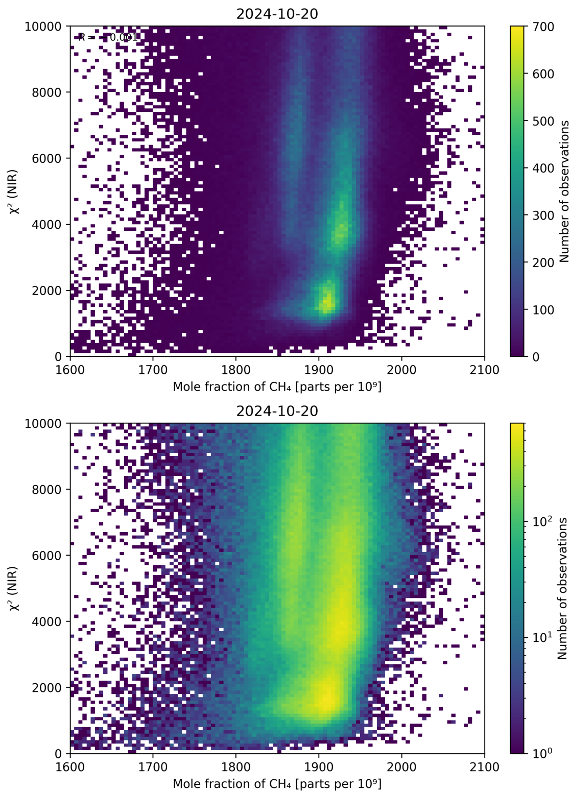
Figure 70: Scatter density plot of “Mole fraction of \text{CH}_4 ” against “ \chi^2 (NIR)” for 2024-10-19 to 2024-10-21.
