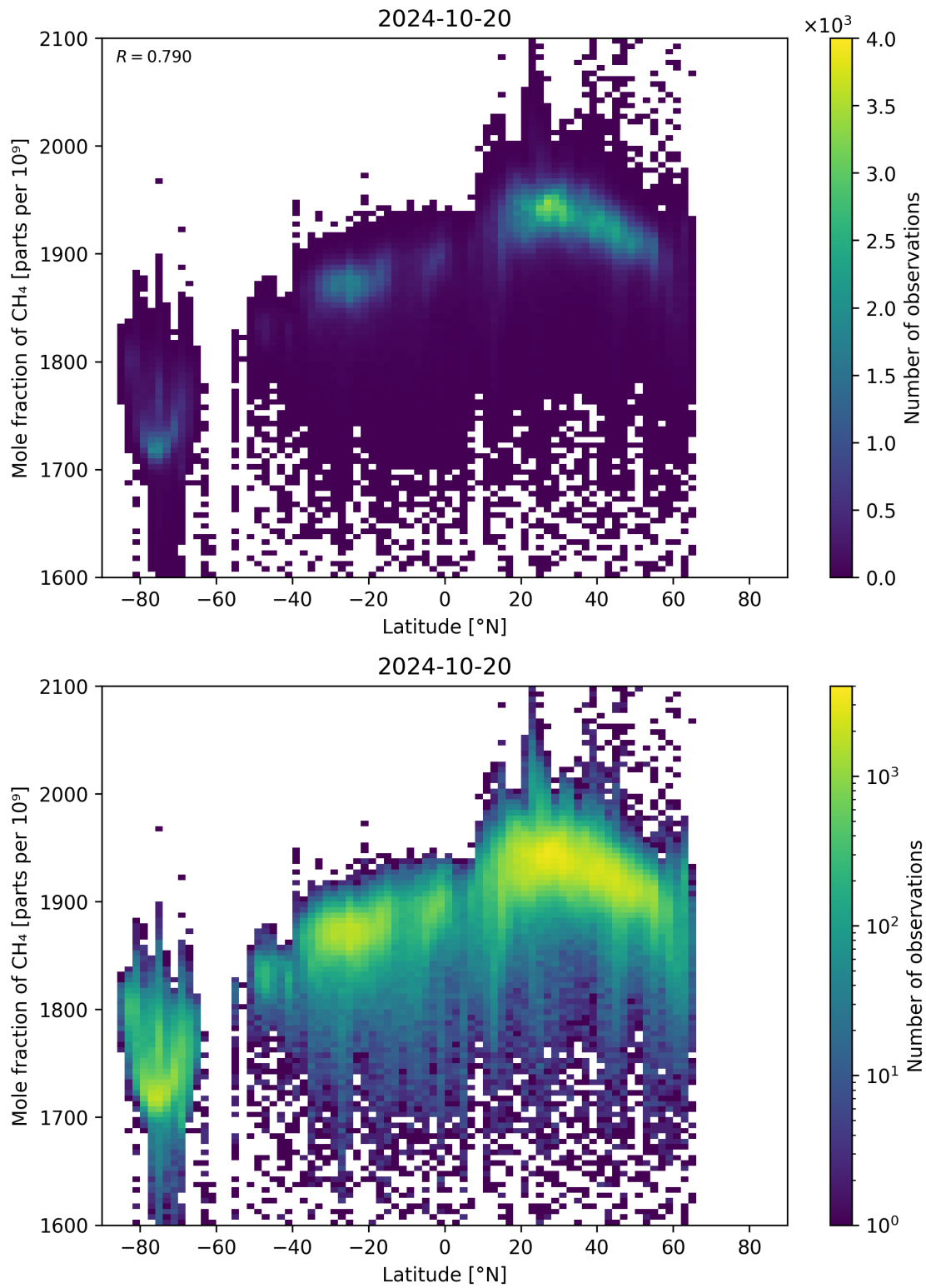
Figure 57: Scatter density plot of “Latitude” against “Mole fraction of CH 4 ” for 2024-10-19 to 2024-10-21.
