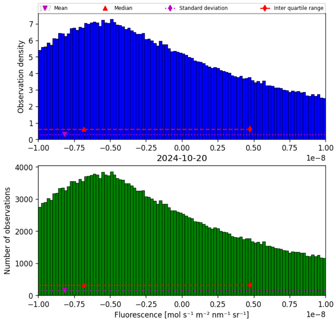
Figure 32: Histogram of “Fluorescence” for 2024-10-19 to 2024-10-21
