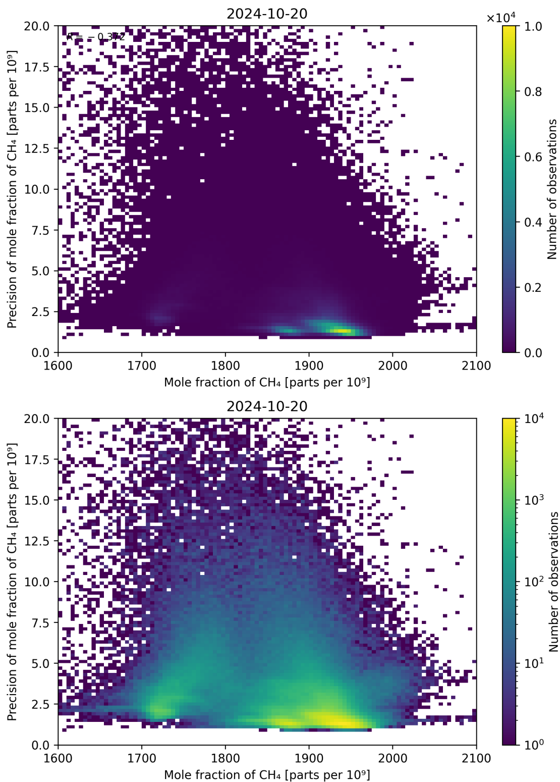
Figure 75: Scatter density plot of “Mole fraction of CH 4 ” against “Precision of mole fraction of CH 4 ” for 2024-10-19 to 2024-10-21.
