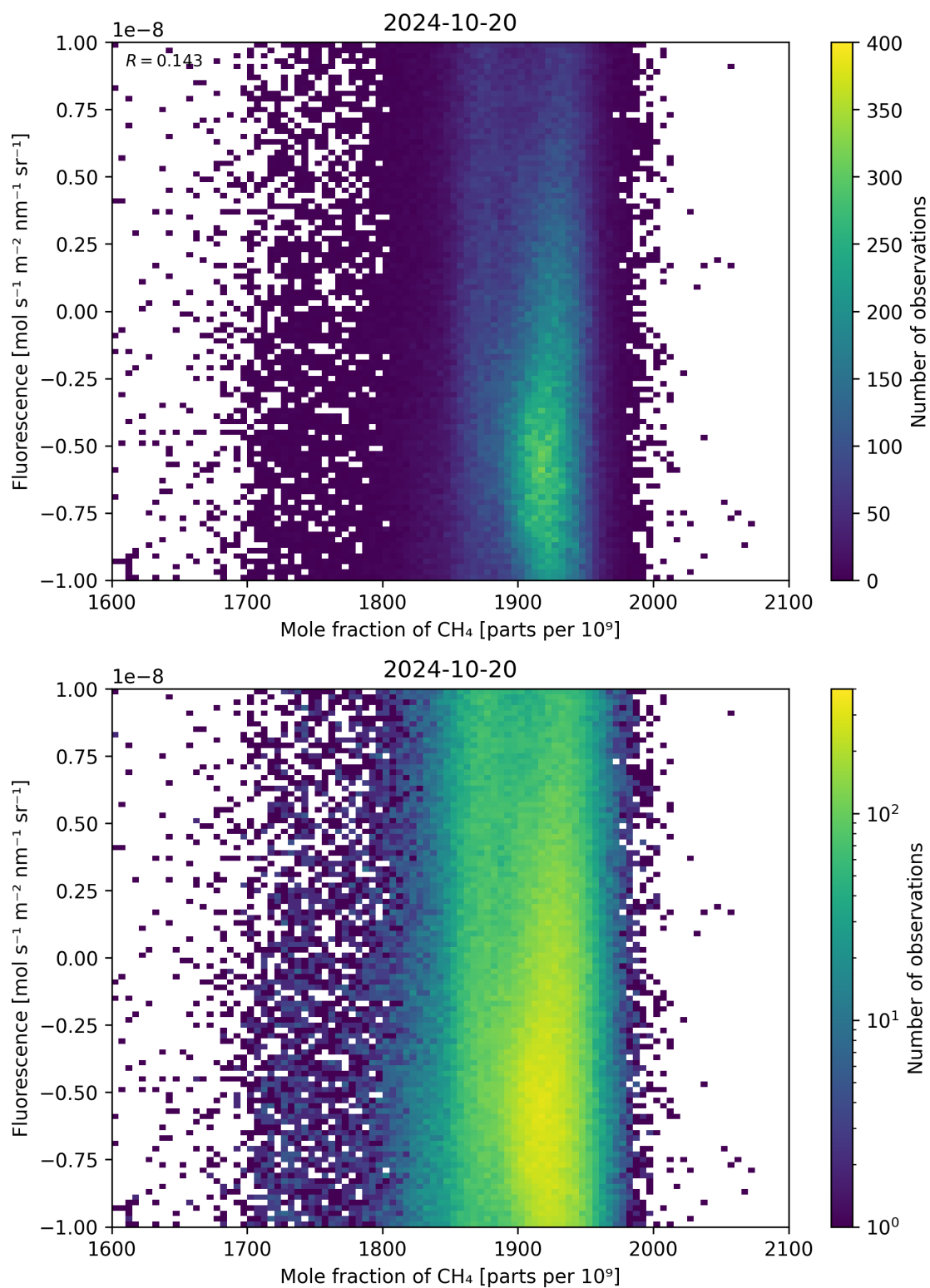
Figure 73: Scatter density plot of “Mole fraction of \text{CH}_4 ” against “Fluorescence” for 2024-10-19 to 2024-10-21.
