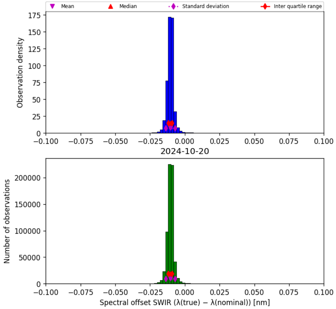
Figure 27: Histogram of “Spectral offset SWIR ( \lambda_{\text{true}} - \lambda_{\text{nominal}} )” for 2024-10-19 to 2024-10-21
