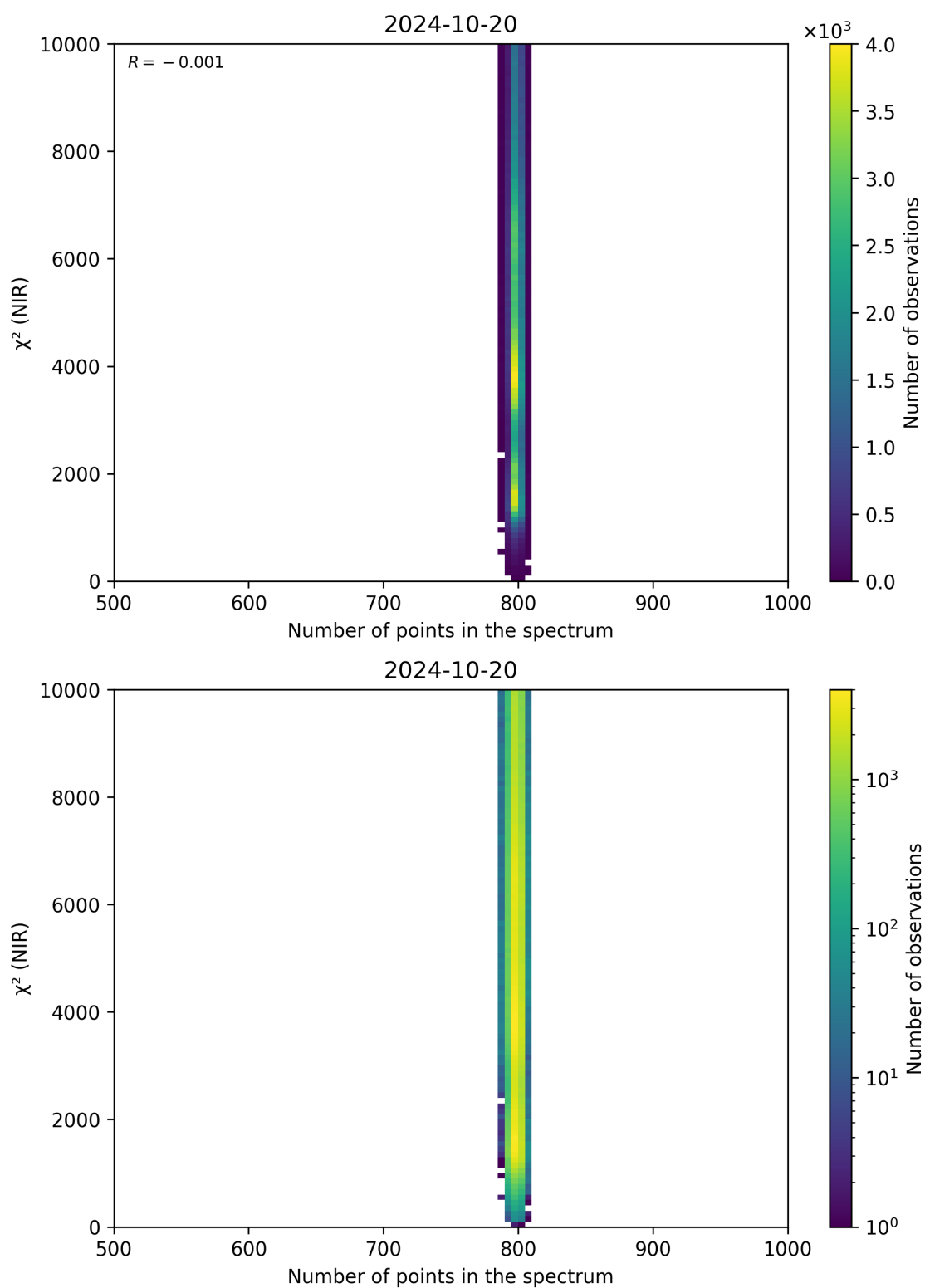
Figure 88: Scatter density plot of “Number of points in the spectrum” against “ \chi^2 (NIR)” for 2024-10-19 to 2024-10-21.
