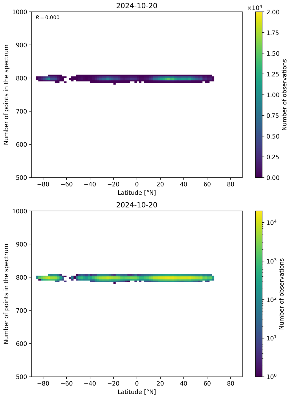
Figure 61: Scatter density plot of “Latitude” against “Number of points in the spectrum” for 2024-10-19 to 2024-10-21.
