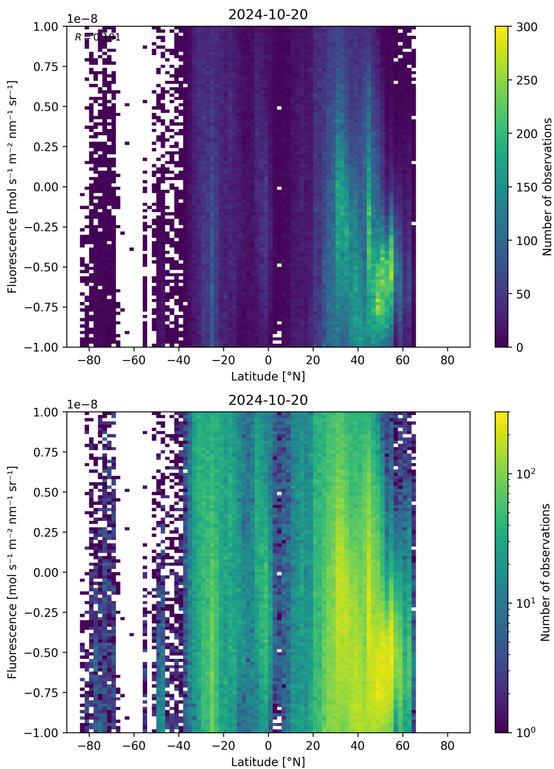
Figure 56: Scatter density plot of “Latitude” against “Fluorescence” for 2024-10-19 to 2024-10-21.
