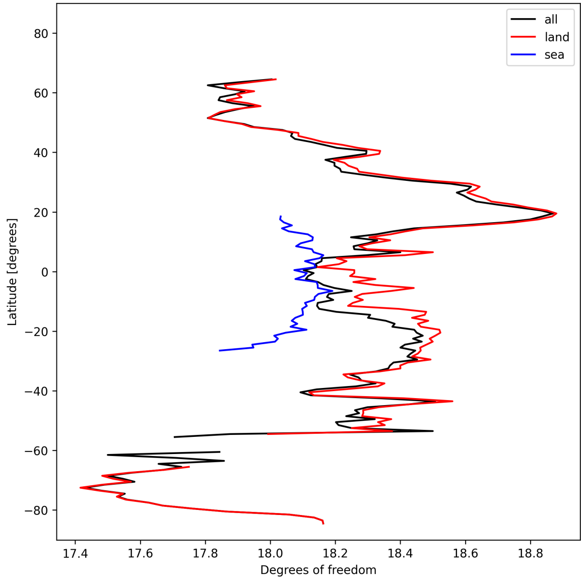
Figure 19: Zonal average of “Degrees of freedom” for 2024-10-19 to 2024-10-21.
