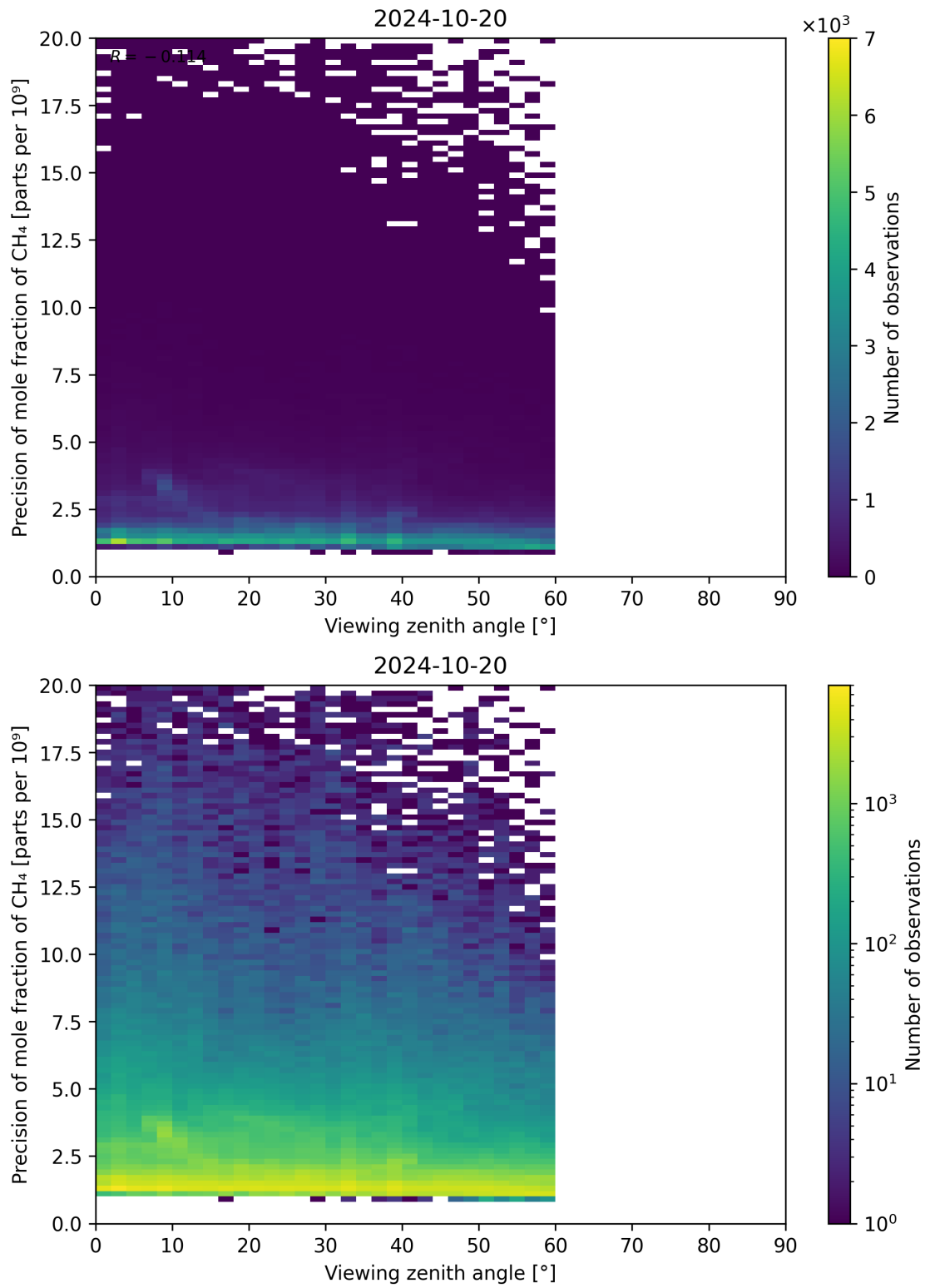
Figure 112: Scatter density plot of “Viewing zenith angle” against “Precision of mole fraction of CH 4 ” for 2024-10-19 to 2024-10-21.
