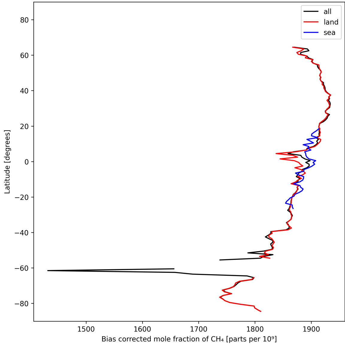
Figure 14: Zonal average of “Bias corrected mole fraction of \text{CH}_4 ” for 2024-10-19 to 2024-10-21.
