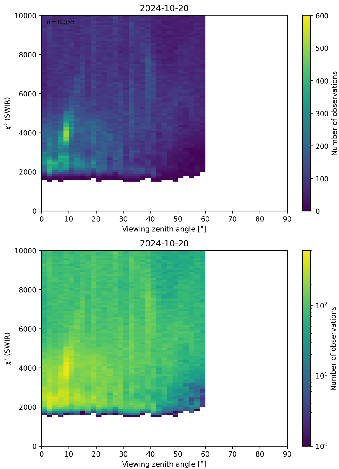
Figure 106: Scatter density plot of “Viewing zenith angle” against “ \chi^2 (SWIR)” for 2024-10-19 to 2024-10-21.
