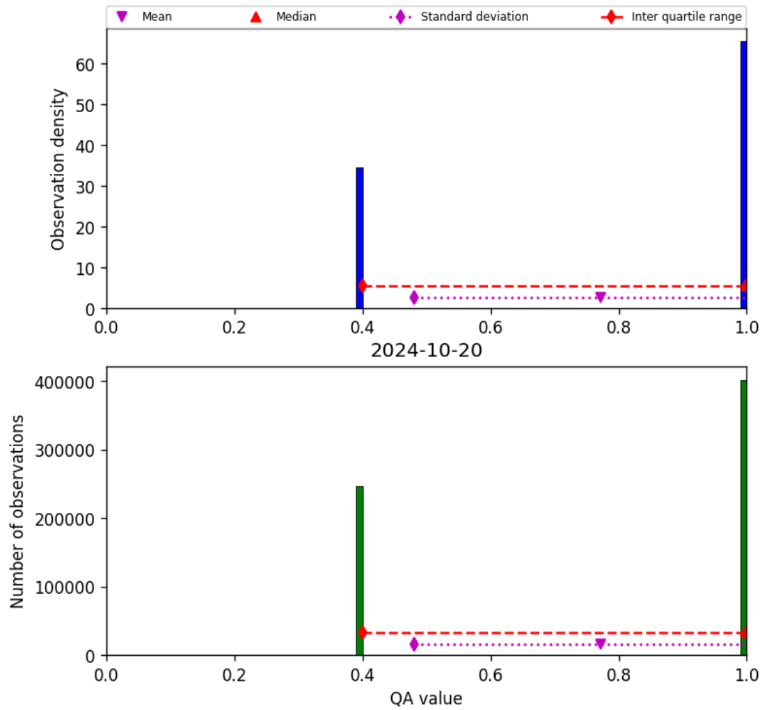
Figure 22: Histogram of “QA value” for 2024-10-19 to 2024-10-21
