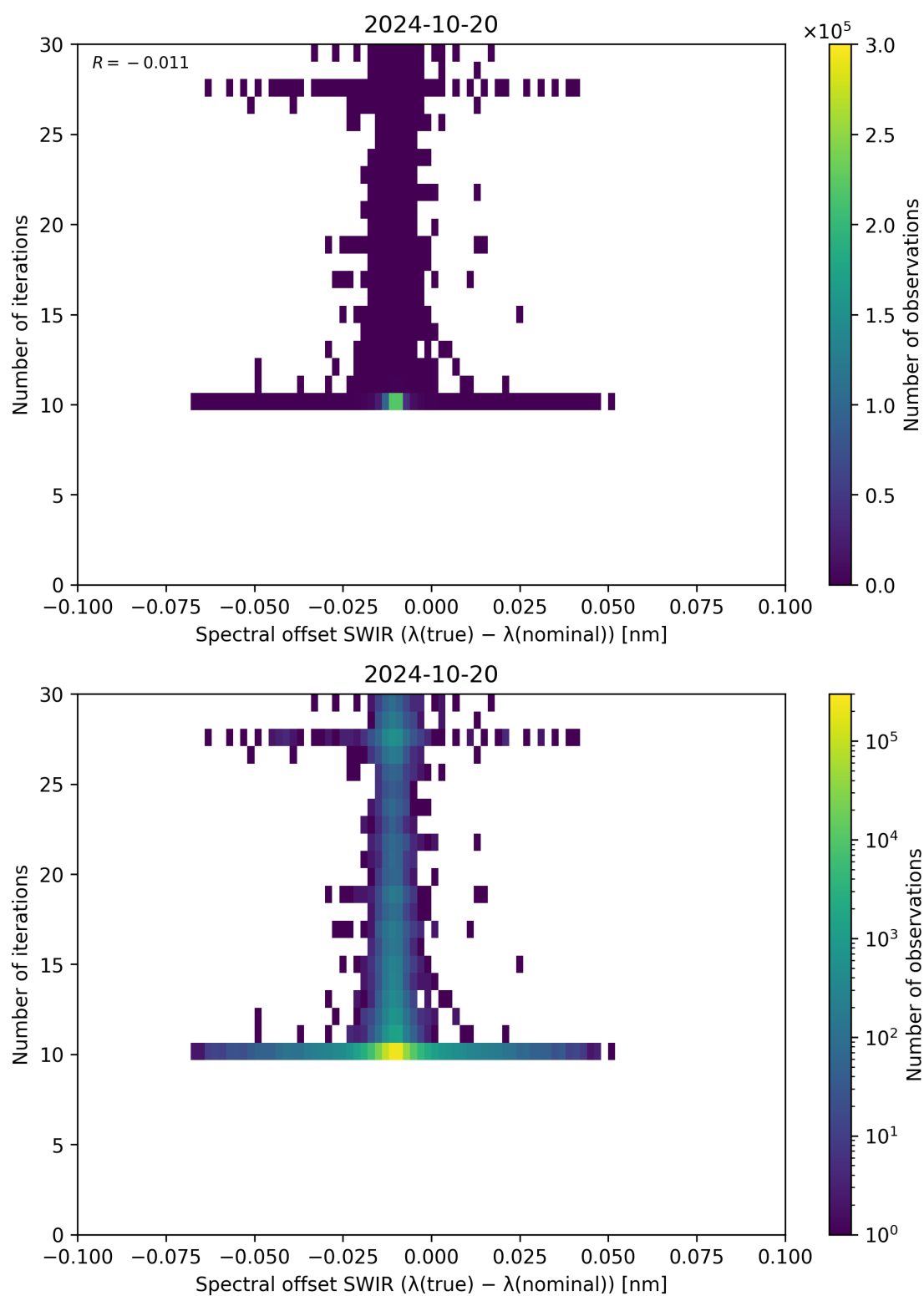
Figure 121: Scatter density plot of “Spectral offset SWIR ( \lambda_{\text{true}} - \lambda_{\text{nominal}} )” against “Number of iterations” for 2024-10-19 to 2024-10-21.
