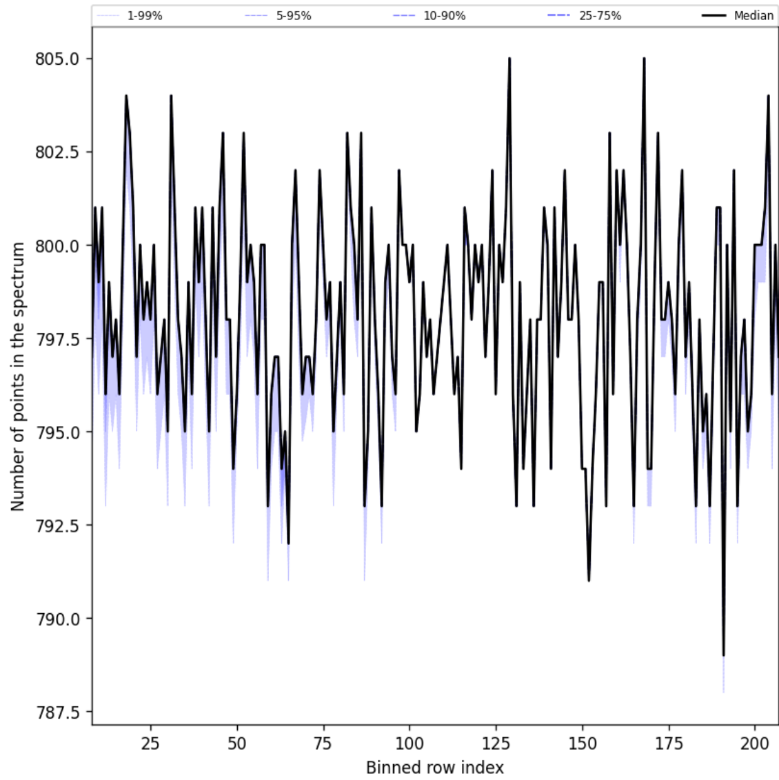
Figure 37: Along track statistics of “Number of points in the spectrum” for 2024-10-19 to 2024-10-21
