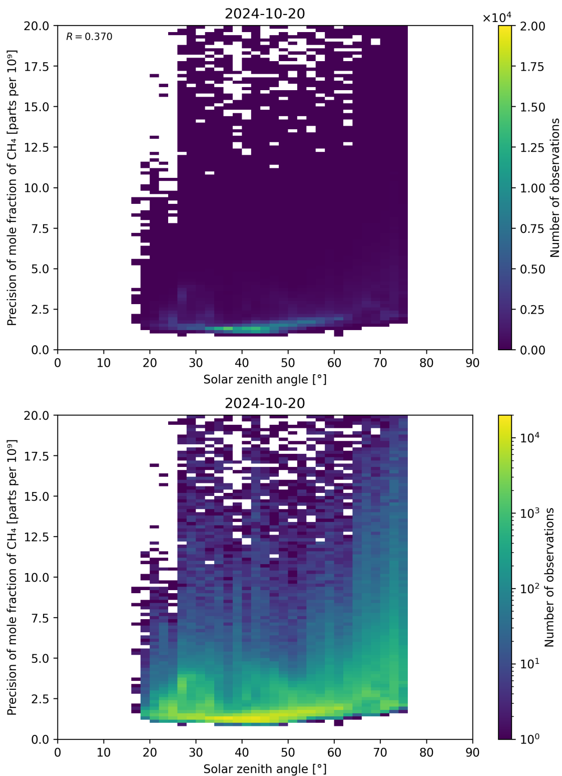
Figure 101: Scatter density plot of “Solar zenith angle” against “Precision of mole fraction of \text{CH}_4 ” for 2024-10-19 to 2024-10-21.
