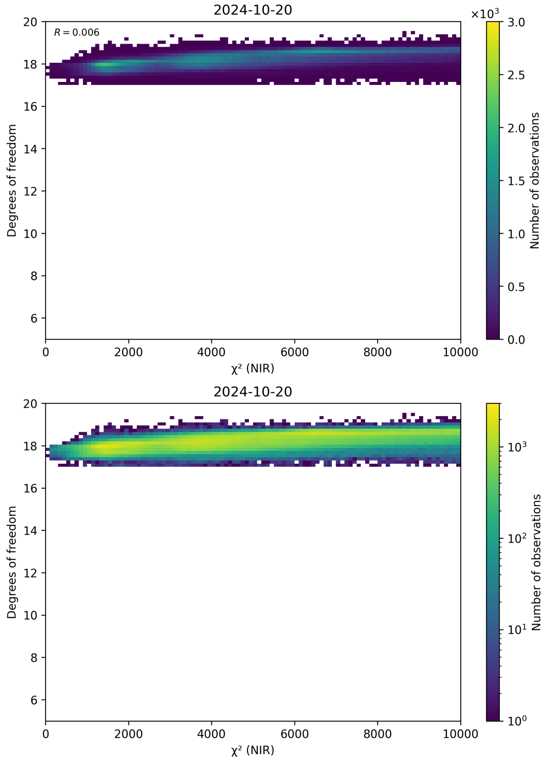
Figure 44: Scatter density plot of “ \chi^2 (NIR)” against “Degrees of freedom” for 2024-10-19 to 2024-10-21.
