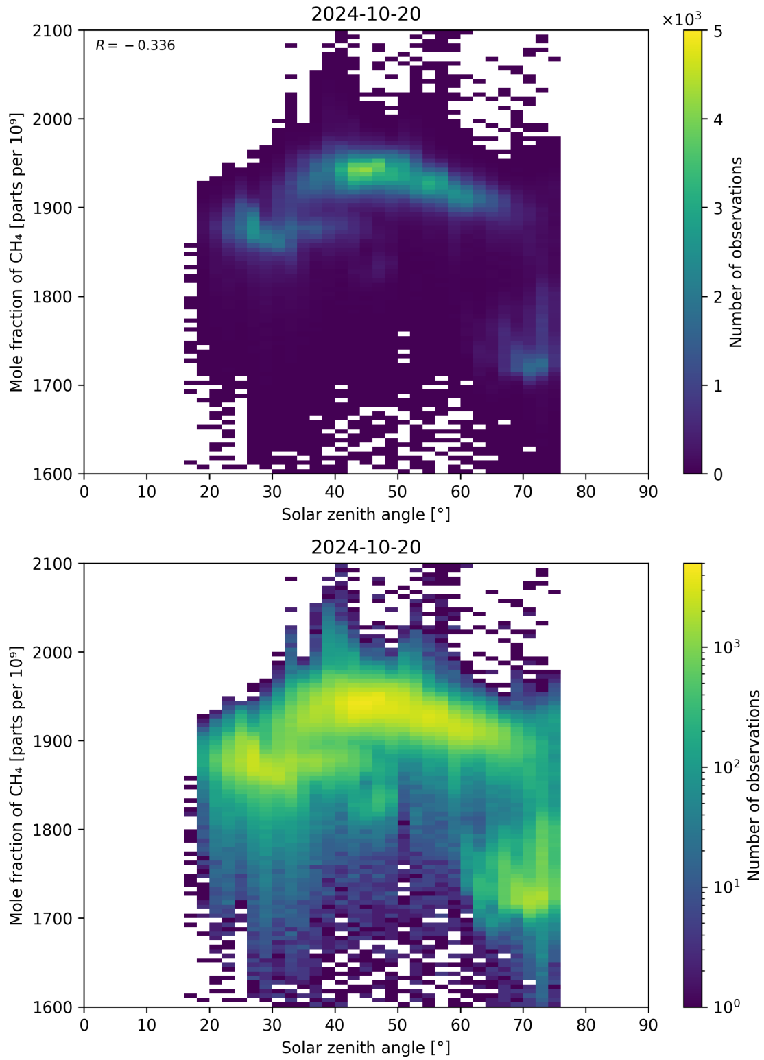
Figure 99: Scatter density plot of “Solar zenith angle” against “Mole fraction of \text{CH}_4 ” for 2024-10-19 to 2024-10-21.
