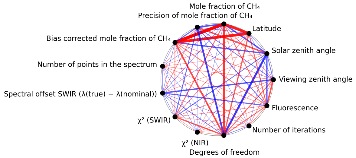
Figure 1: Map of correlation graph for 2024-10-19 to 2024-10-21.
