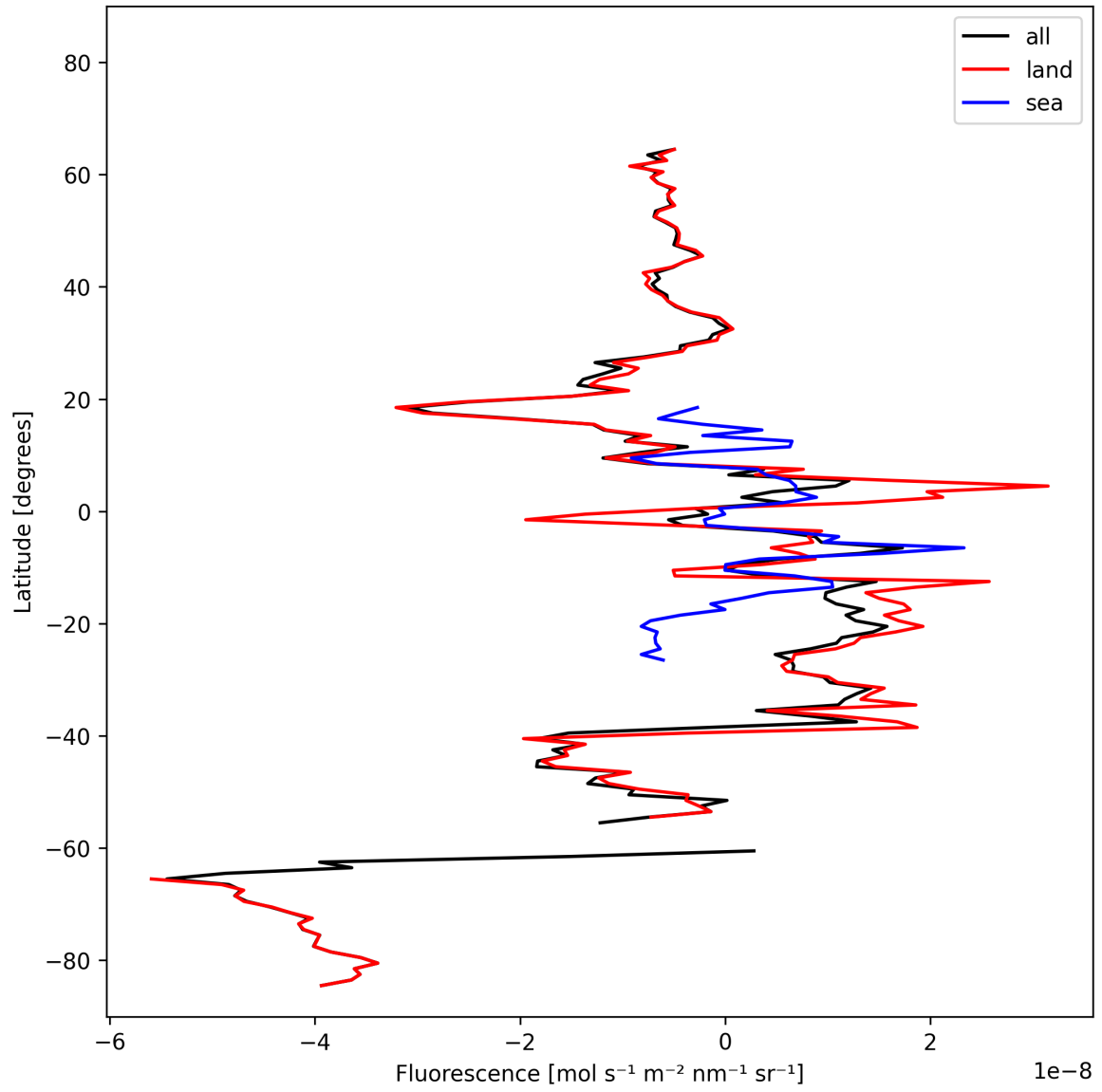
Figure 21: Zonal average of “Fluorescence” for 2024-10-19 to 2024-10-21.
