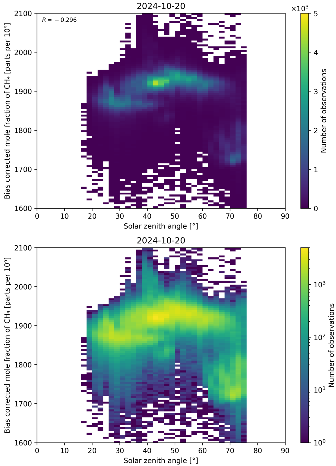
Figure 100: Scatter density plot of “Solar zenith angle” against “Bias corrected mole fraction of \text{CH}_4 ” for 2024-10-19 to 2024-10-21.
