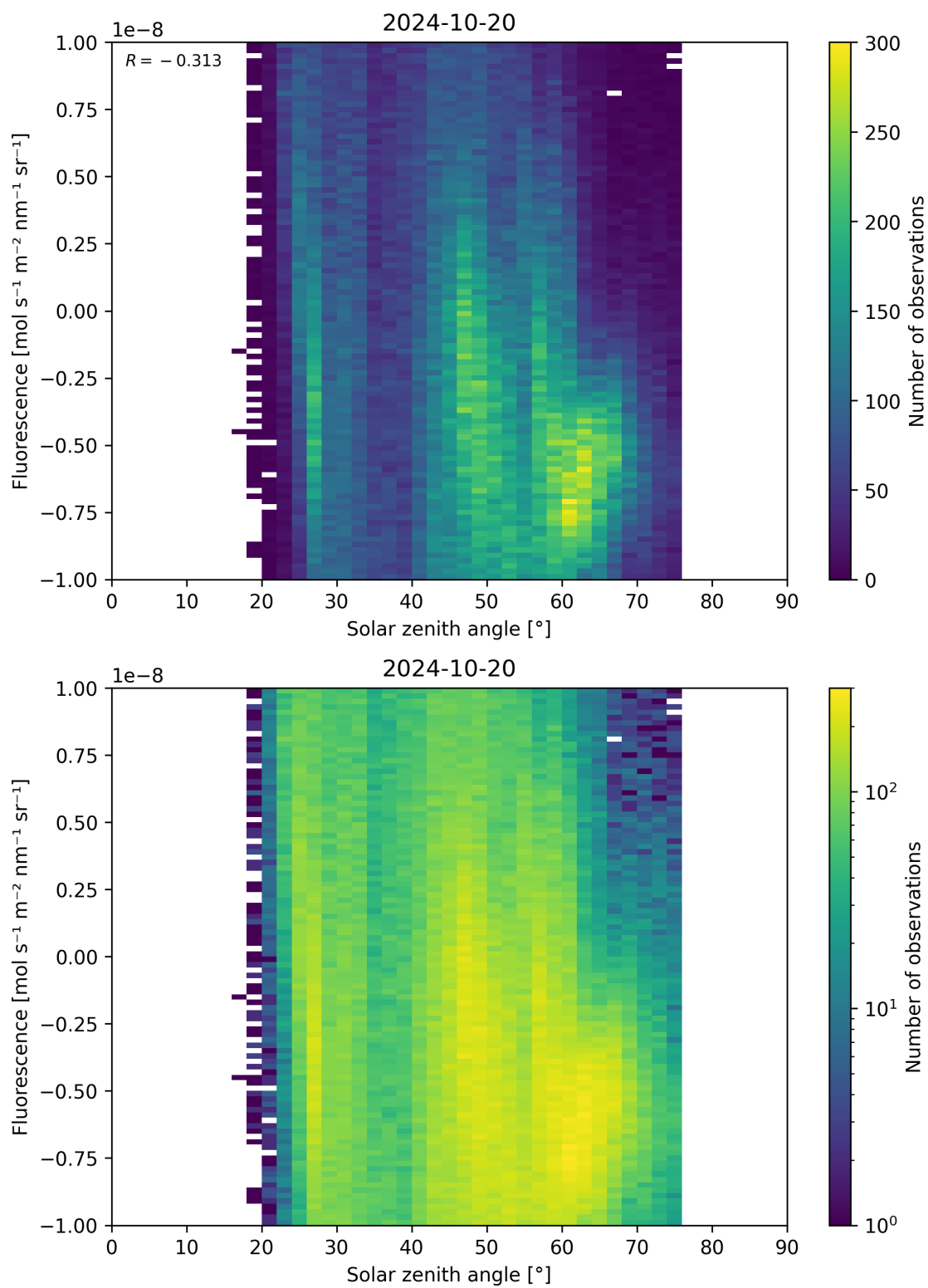
Figure 97: Scatter density plot of “Solar zenith angle” against “Fluorescence” for 2024-10-19 to 2024-10-21.
