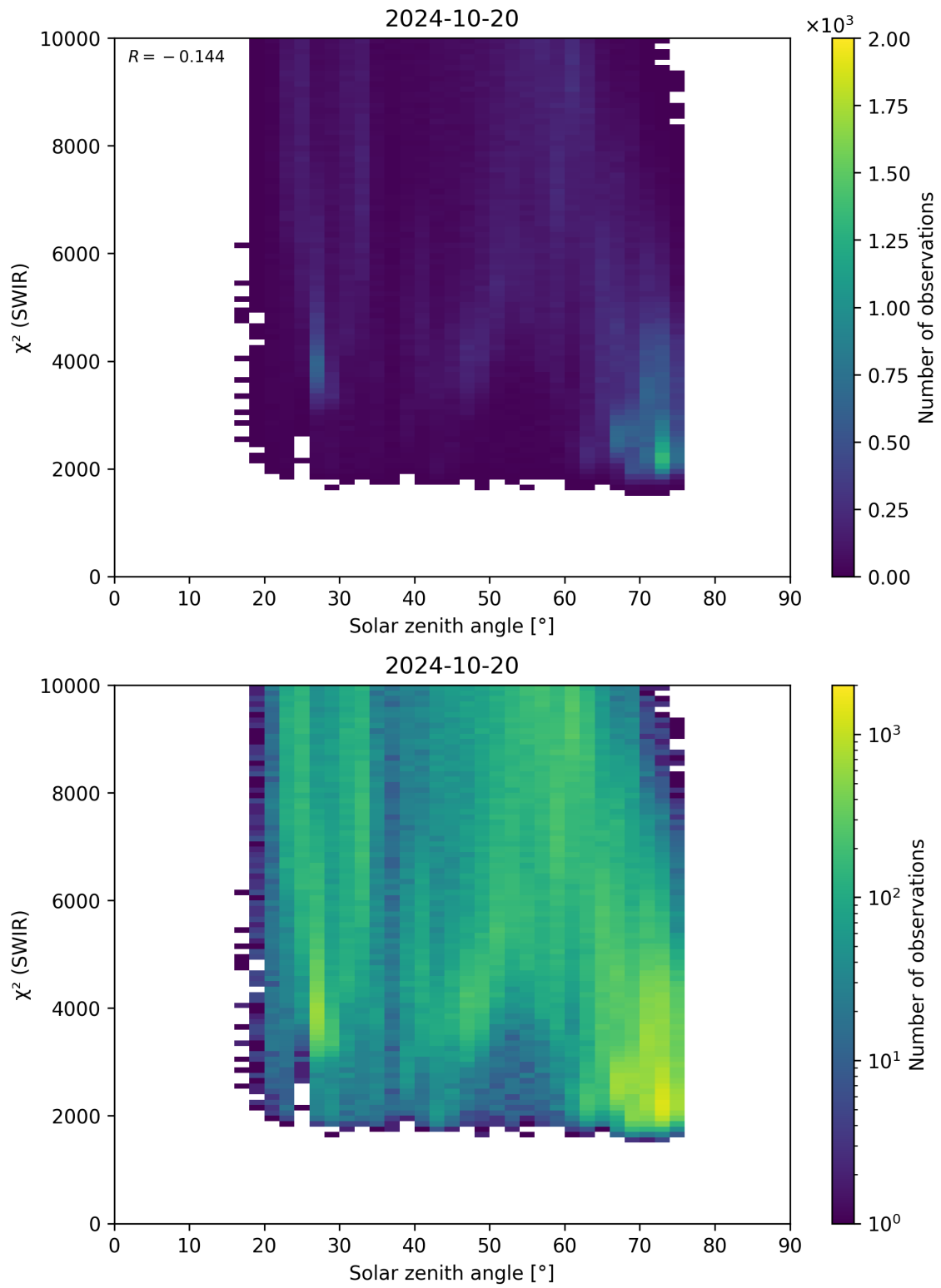
Figure 95: Scatter density plot of “Solar zenith angle” against “ \chi^2 (SWIR)” for 2024-10-19 to 2024-10-21.
