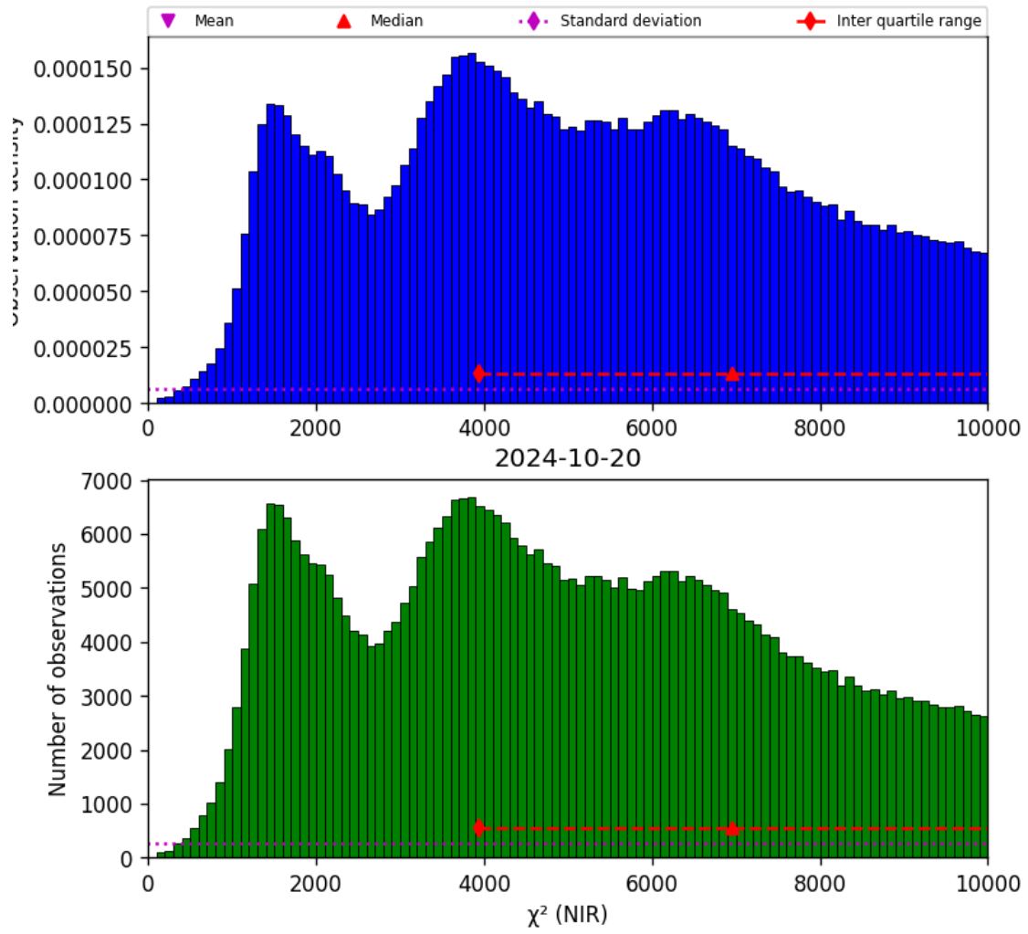
Figure 29: Histogram of “ \chi^2 (NIR)” for 2024-10-19 to 2024-10-21
