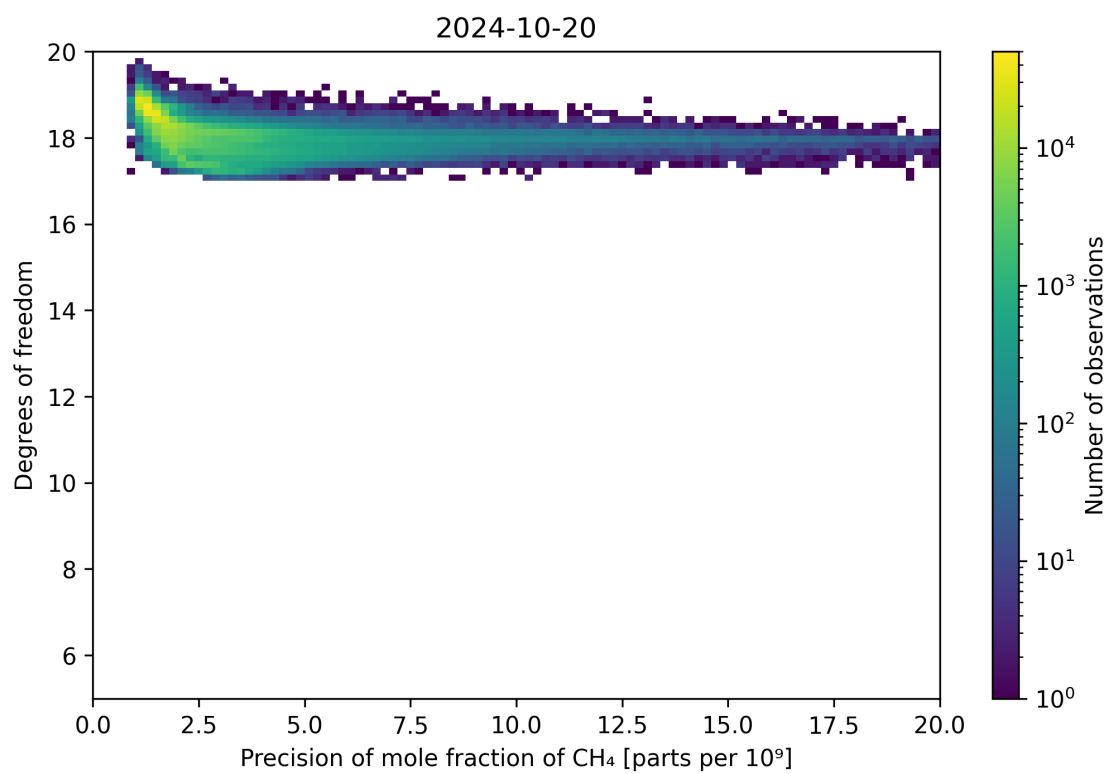
Figure 80: Scatter density plot of “Precision of mole fraction of CH 4 ” against “Degrees of freedom” for 2024-10-19 to 2024-10-21.
