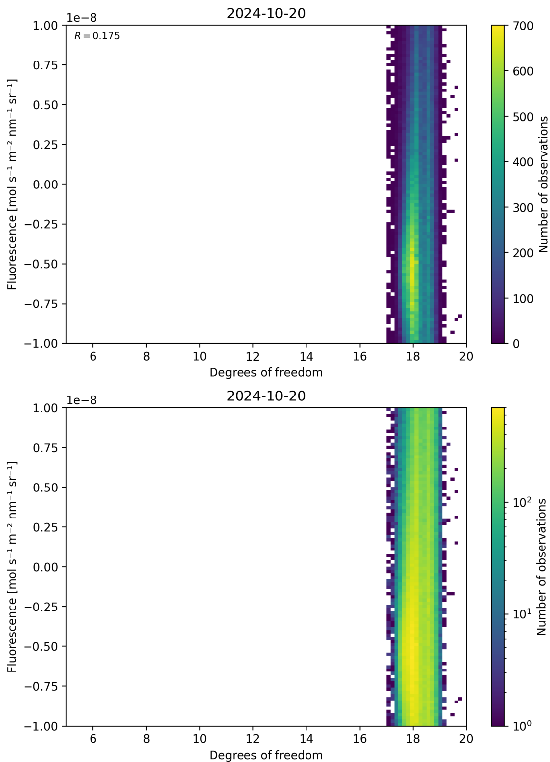
Figure 51: Scatter density plot of “Degrees of freedom” against “Fluorescence” for 2024-10-19 to 2024-10-21.
