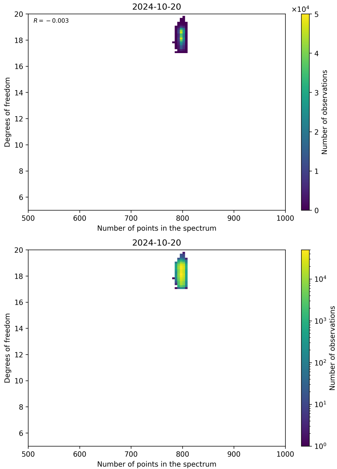
Figure 90: Scatter density plot of “Number of points in the spectrum” against “Degrees of freedom” for 2024-10-19 to 2024-10-21.
