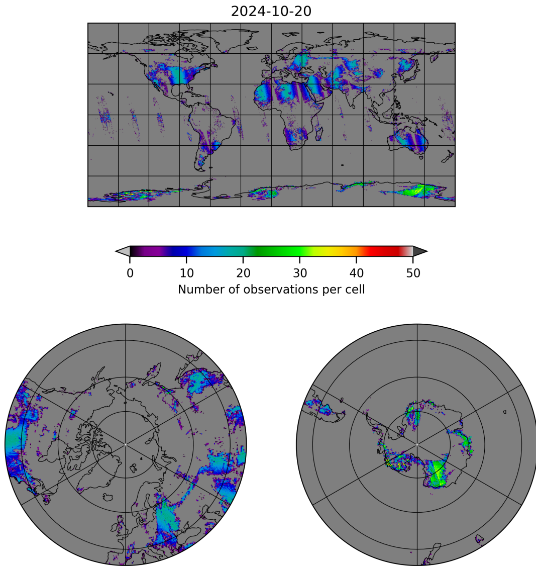
Figure 10: Map of the number of observations for 2024-10-19 to 2024-10-21
