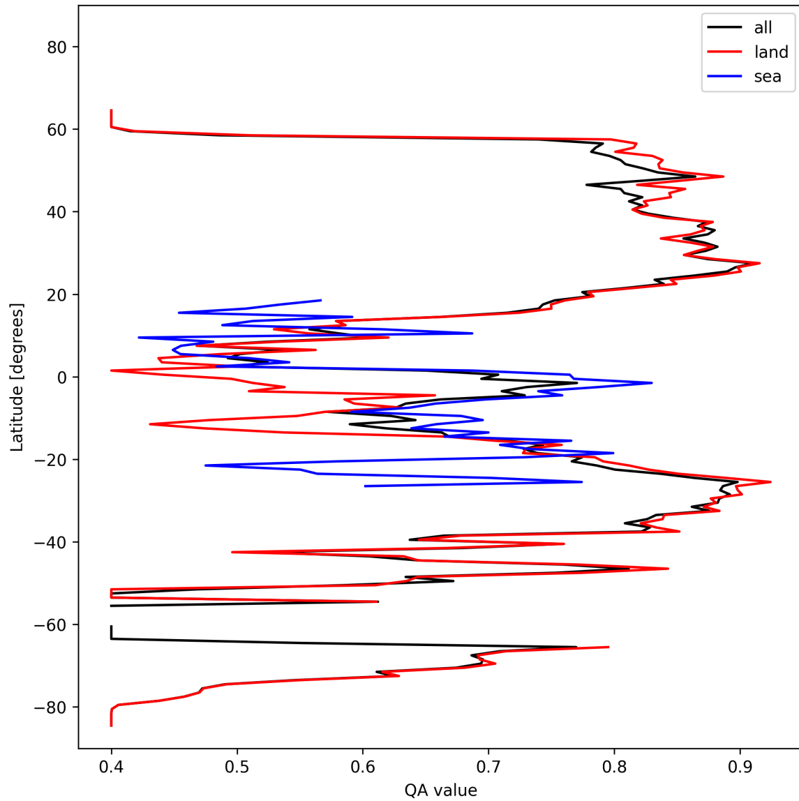
Figure 11: Zonal average of “QA value” for 2024-10-19 to 2024-10-21.
