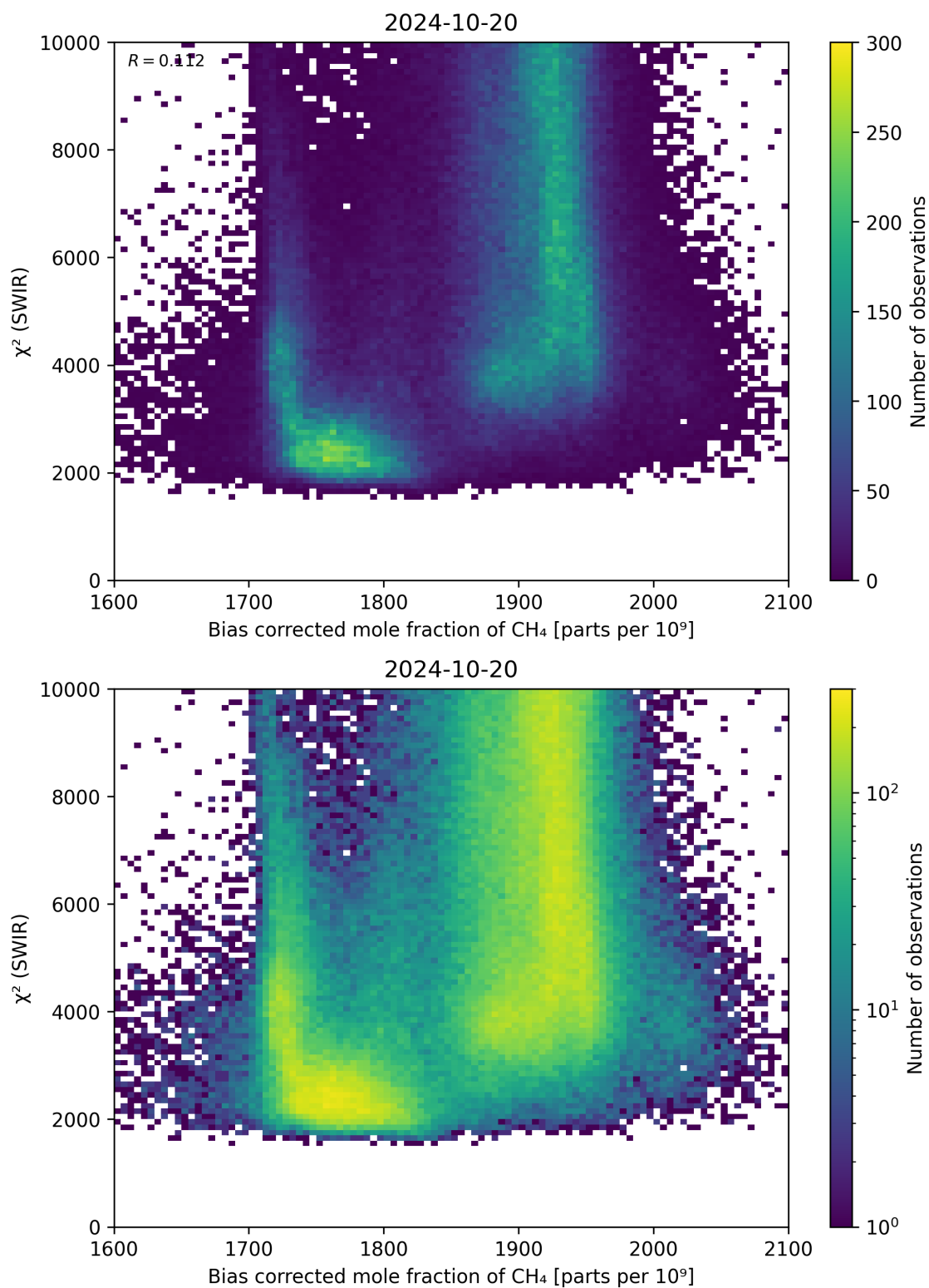
Figure 64: Scatter density plot of “Bias corrected mole fraction of CH 4 ” against “ \chi^2 (SWIR)” for 2024-10-19 to 2024-10-21.
