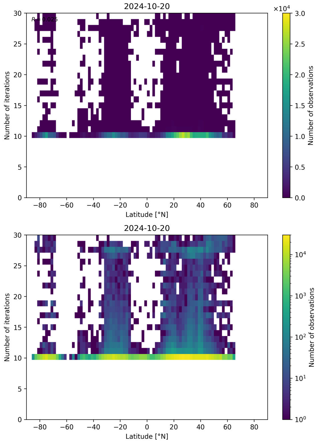
Figure 60: Scatter density plot of “Latitude” against “Number of iterations” for 2024-10-19 to 2024-10-21.
