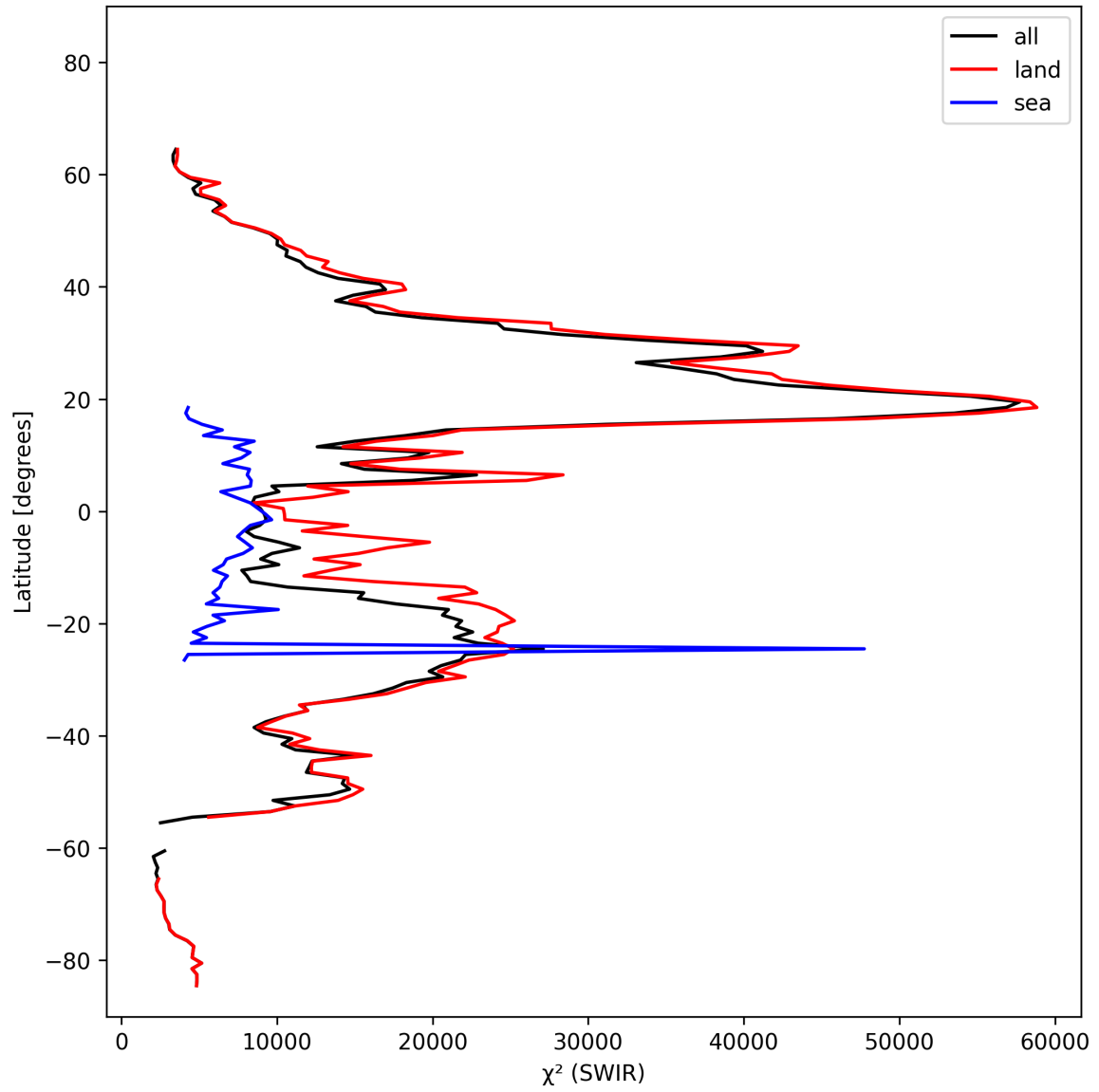
Figure 17: Zonal average of “ \chi^2 (SWIR)” for 2024-10-19 to 2024-10-21.
