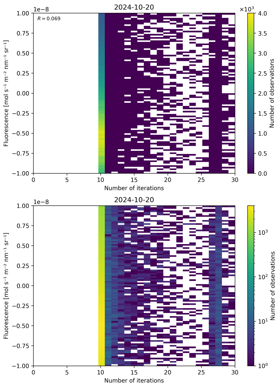
Figure 87: Scatter density plot of “Number of iterations” against “Fluorescence” for 2024-10-19 to 2024-10-21.
