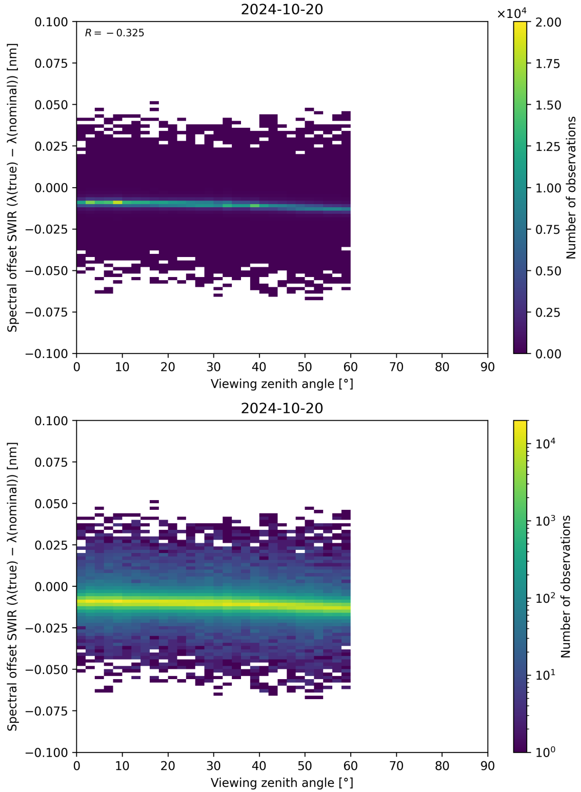
Figure 116: Scatter density plot of “Viewing zenith angle” against “Spectral offset SWIR ( \lambda_{\text{true}} - \lambda_{\text{nominal}} )” for 2024-10-19 to 2024-10-21.
