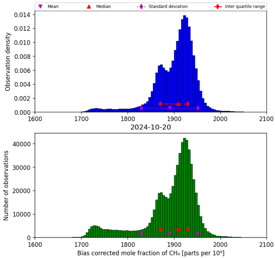
Figure 25: Histogram of “Bias corrected mole fraction of CH 4 ” for 2024-10-19 to 2024-10-21
