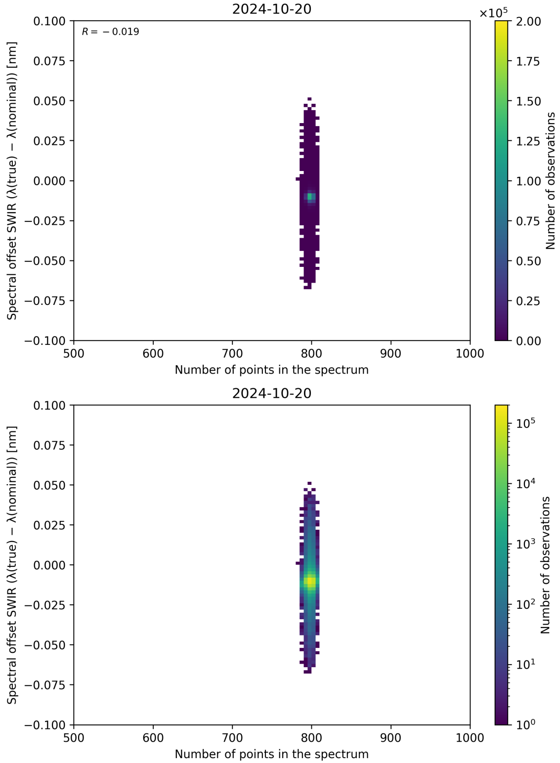
Figure 93: Scatter density plot of “Number of points in the spectrum” against “Spectral offset SWIR ( \lambda_{\text{true}} - \lambda_{\text{nominal}} )” for 2024-10-19 to 2024-10-21.
