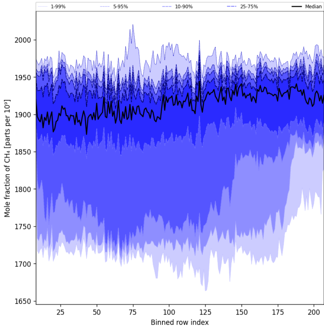
Figure 34: Along track statistics of “Mole fraction of CH 4 ” for 2024-10-19 to 2024-10-21
