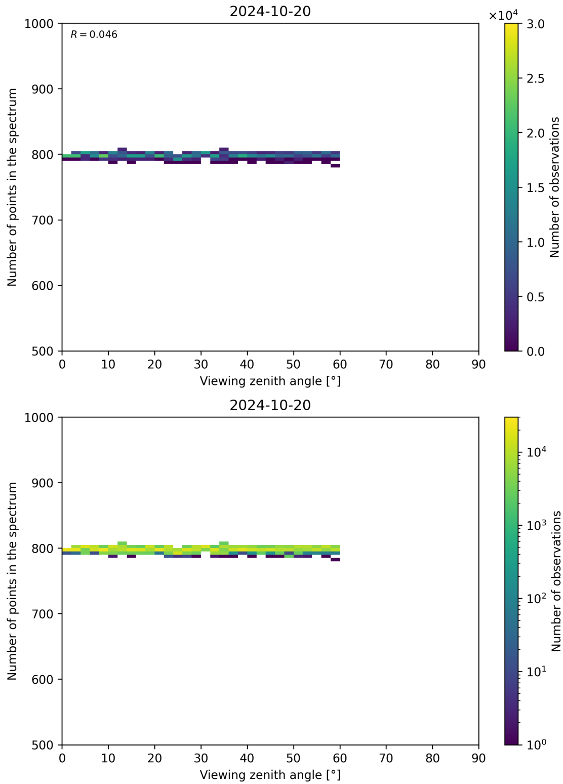
Figure 114: Scatter density plot of “Viewing zenith angle” against “Number of points in the spectrum” for 2024-10-19 to 2024-10-21.
