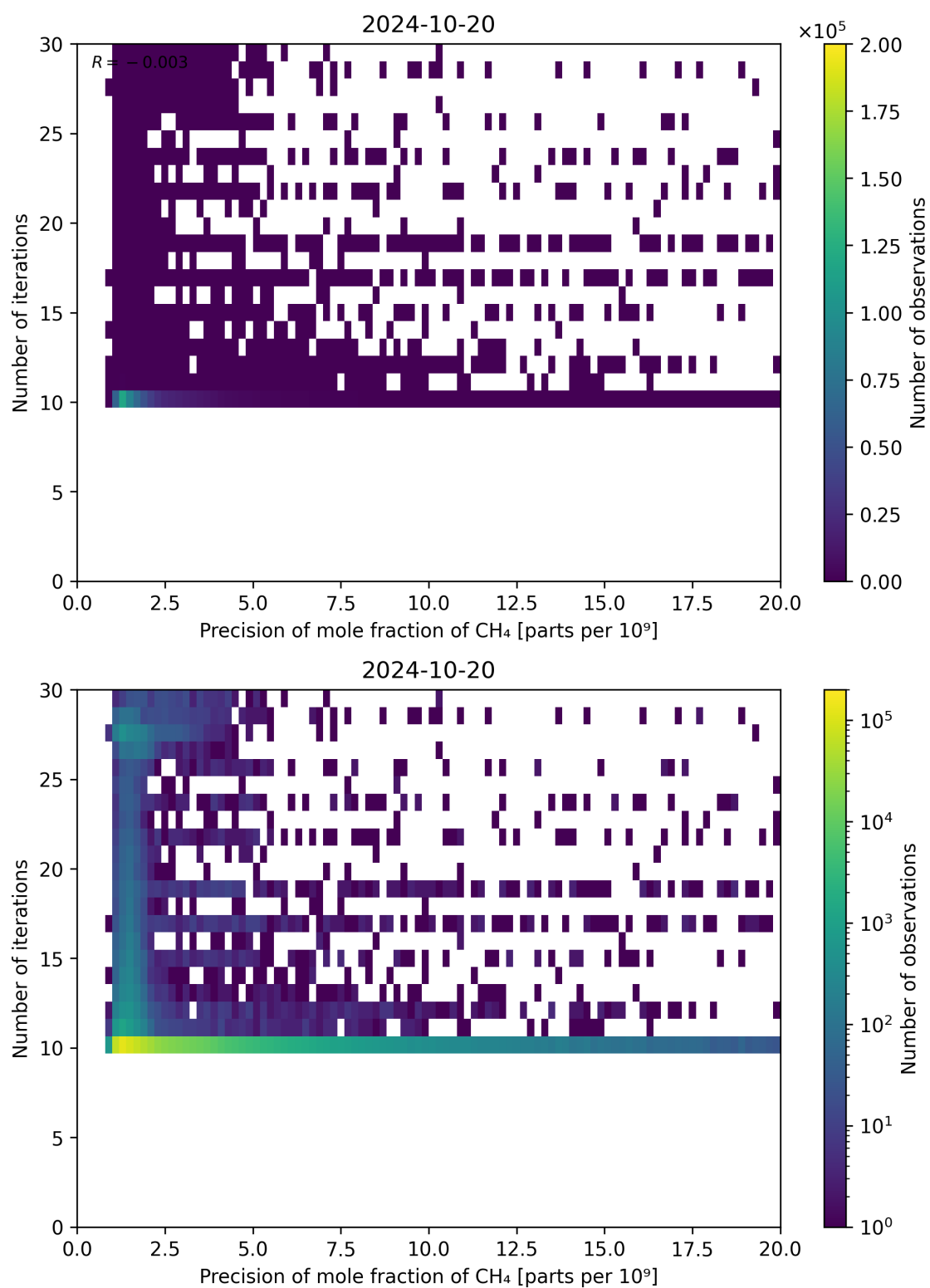
Figure 83: Scatter density plot of “Precision of mole fraction of CH 4 ” against “Number of iterations” for 2024-10-19 to 2024-10-21.
