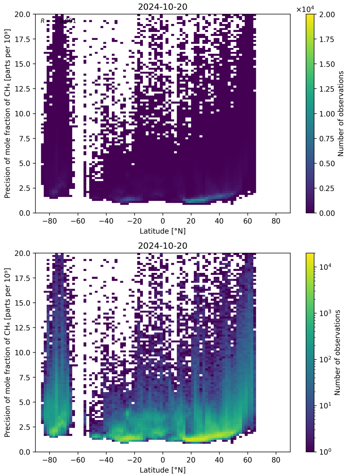
Figure 59: Scatter density plot of “Latitude” against “Precision of mole fraction of CH 4 ” for 2024-10-19 to 2024-10-21.
