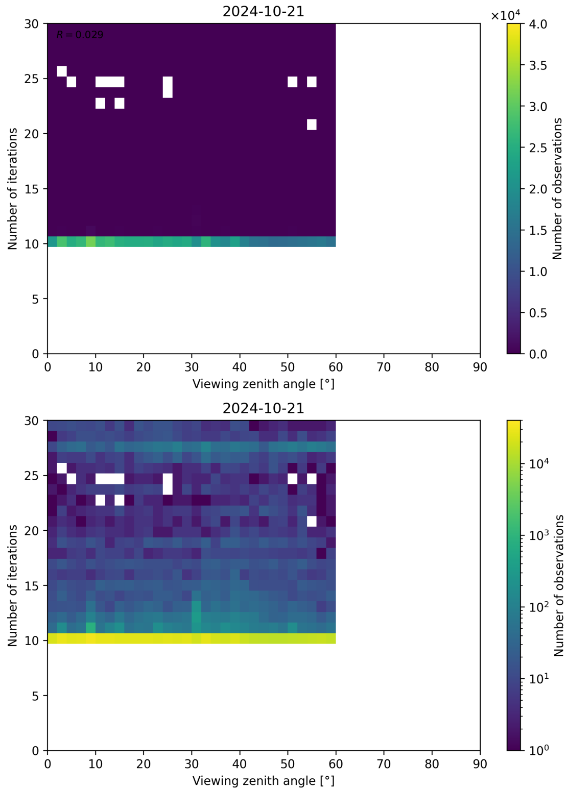
Figure 113: Scatter density plot of “Viewing zenith angle” against “Number of iterations” for 2024-10-20 to 2024-10-22.
