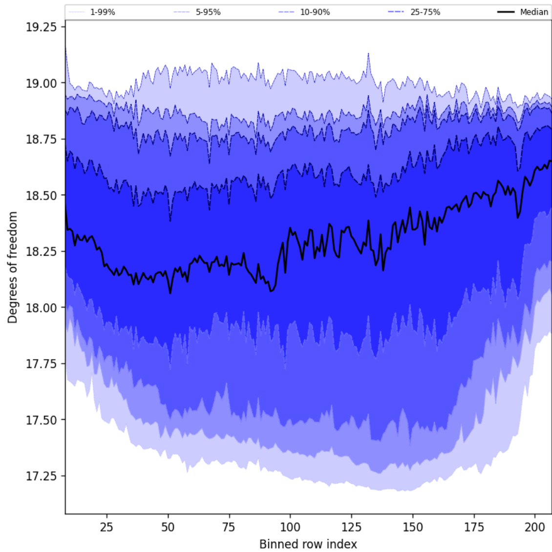
Figure 41: Along track statistics of “Degrees of freedom” for 2024-10-20 to 2024-10-22
