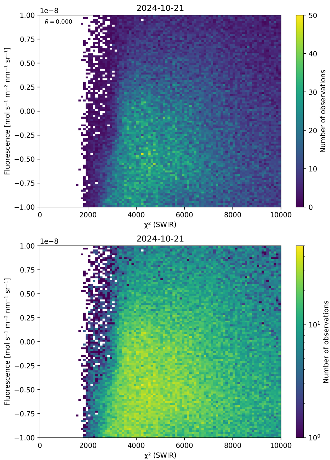
Figure 49: Scatter density plot of “ \chi^2 (SWIR)” against “Fluorescence” for 2024-10-20 to 2024-10-22.
