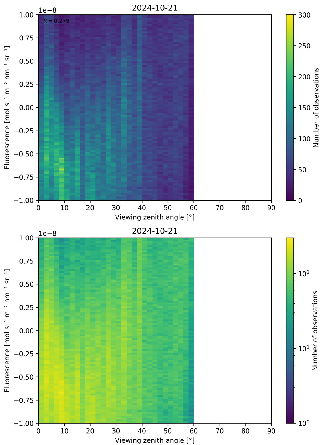
Figure 108: Scatter density plot of “Viewing zenith angle” against “Fluorescence” for 2024-10-20 to 2024-10-22.
