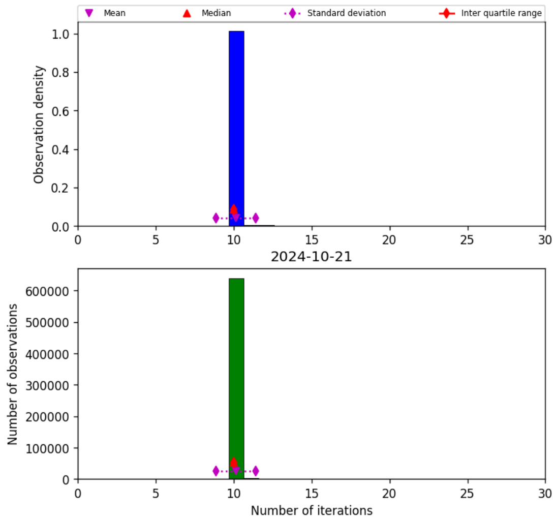
Figure 31: Histogram of “Number of iterations” for 2024-10-20 to 2024-10-22
