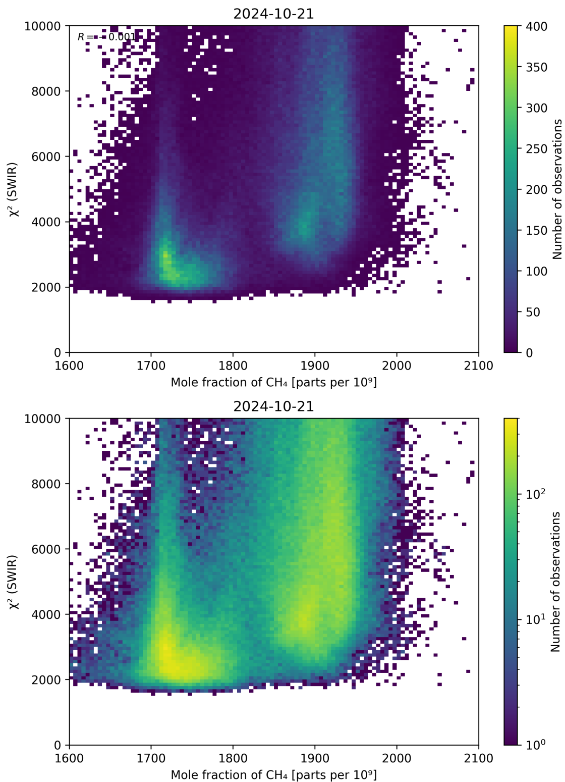
Figure 71: Scatter density plot of “Mole fraction of \text{CH}_4 ” against “ \chi^2 (SWIR)” for 2024-10-20 to 2024-10-22.
