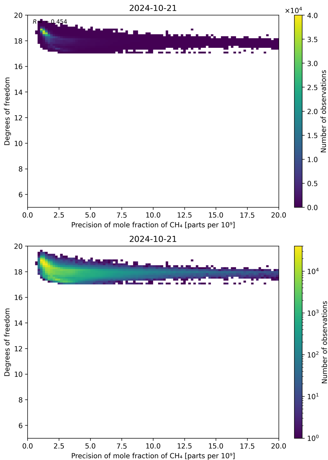
Figure 80: Scatter density plot of “Precision of mole fraction of CH 4 ” against “Degrees of freedom” for 2024-10-20 to 2024-10-22.
