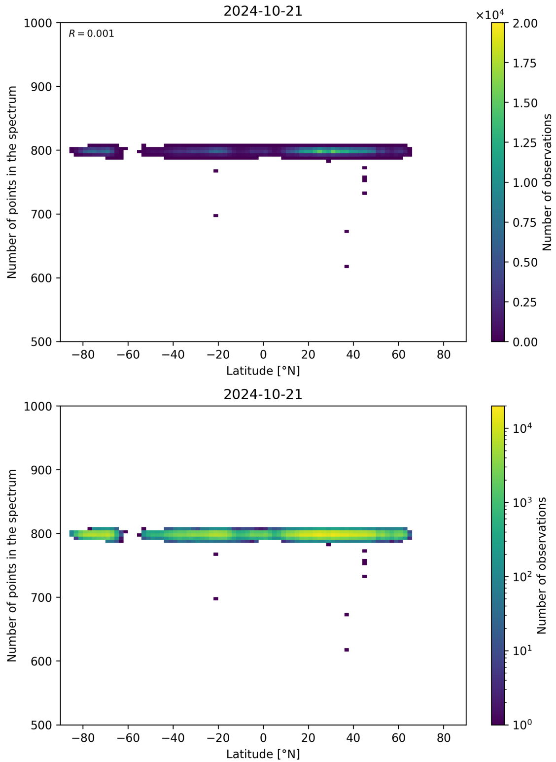
Figure 61: Scatter density plot of “Latitude” against “Number of points in the spectrum” for 2024-10-20 to 2024-10-22.
