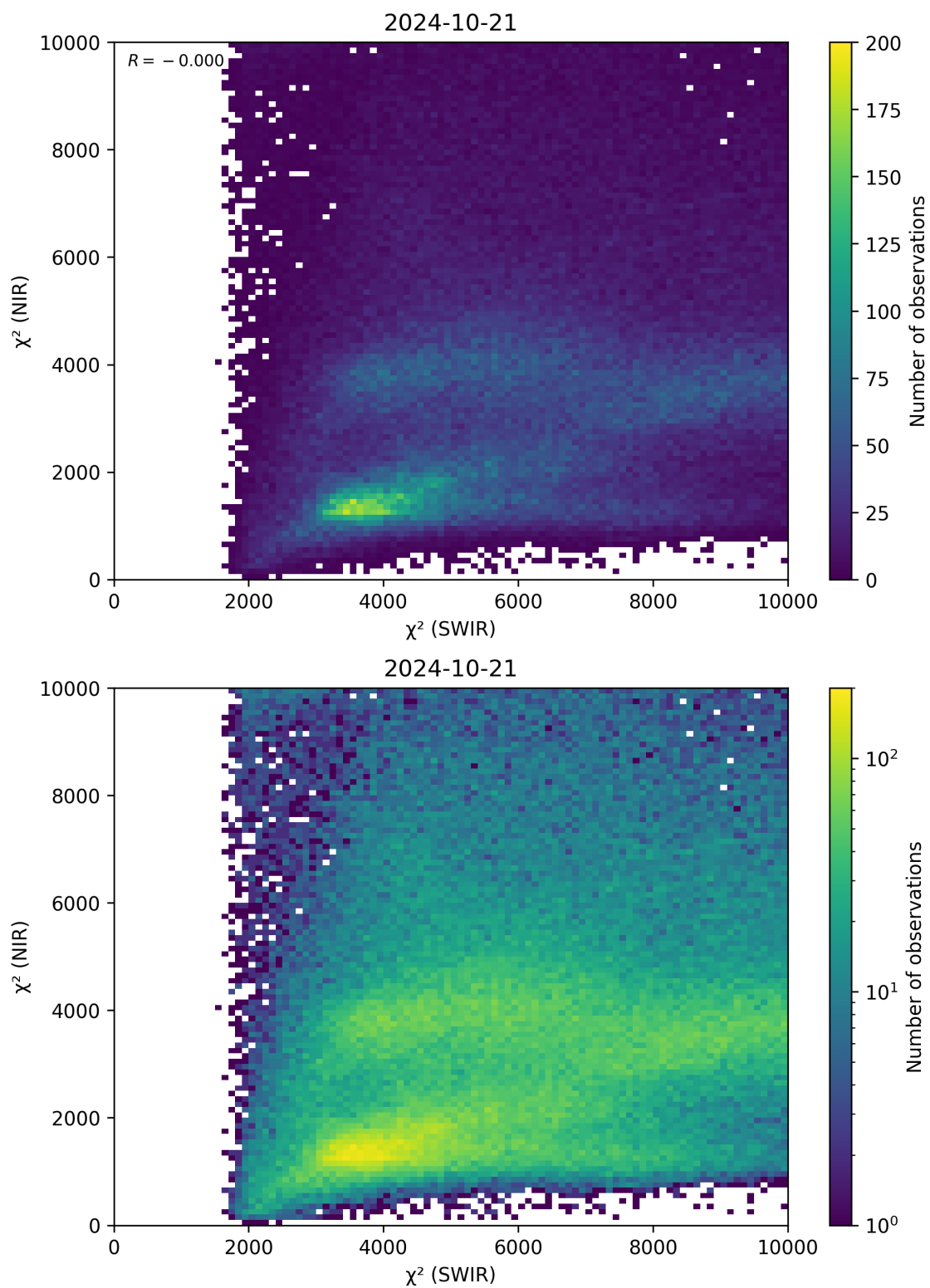
Figure 47: Scatter density plot of “ \chi^2 (SWIR)” against “ \chi^2 (NIR)” for 2024-10-20 to 2024-10-22.
