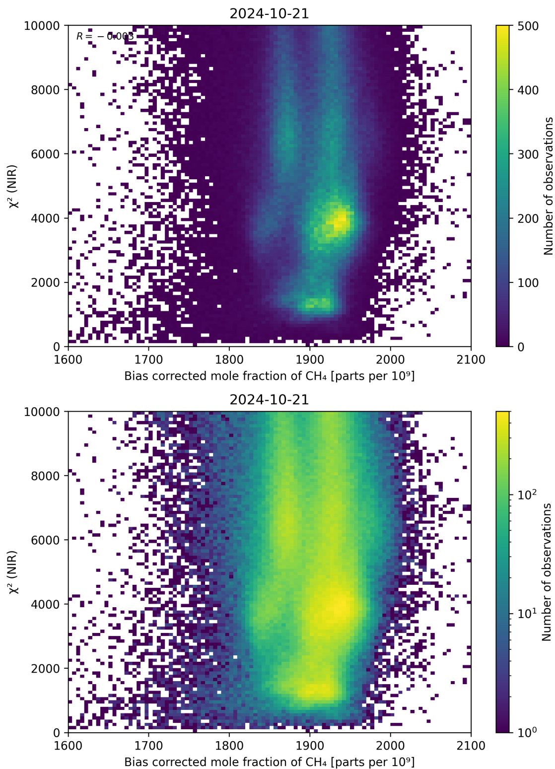
Figure 63: Scatter density plot of “Bias corrected mole fraction of CH 4 ” against “ \chi^2 (NIR)” for 2024-10-20 to 2024-10-22.
