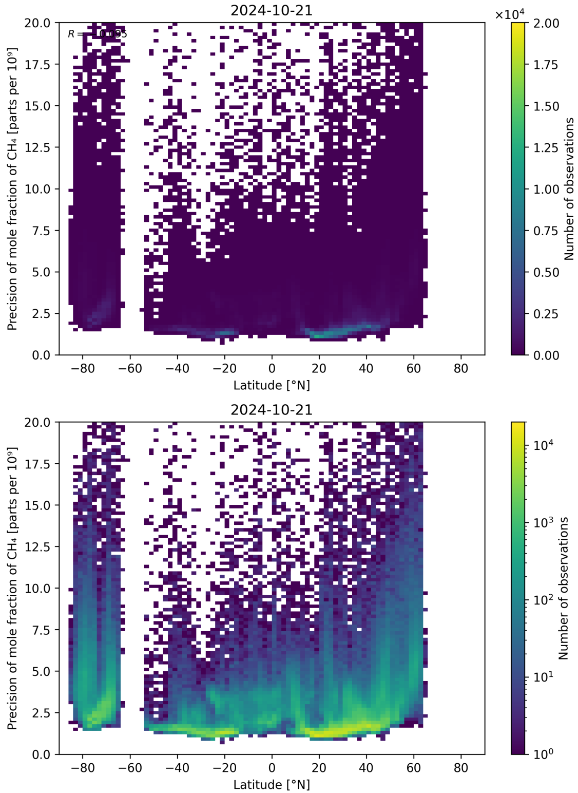
Figure 59: Scatter density plot of “Latitude” against “Precision of mole fraction of CH 4 ” for 2024-10-20 to 2024-10-22.
