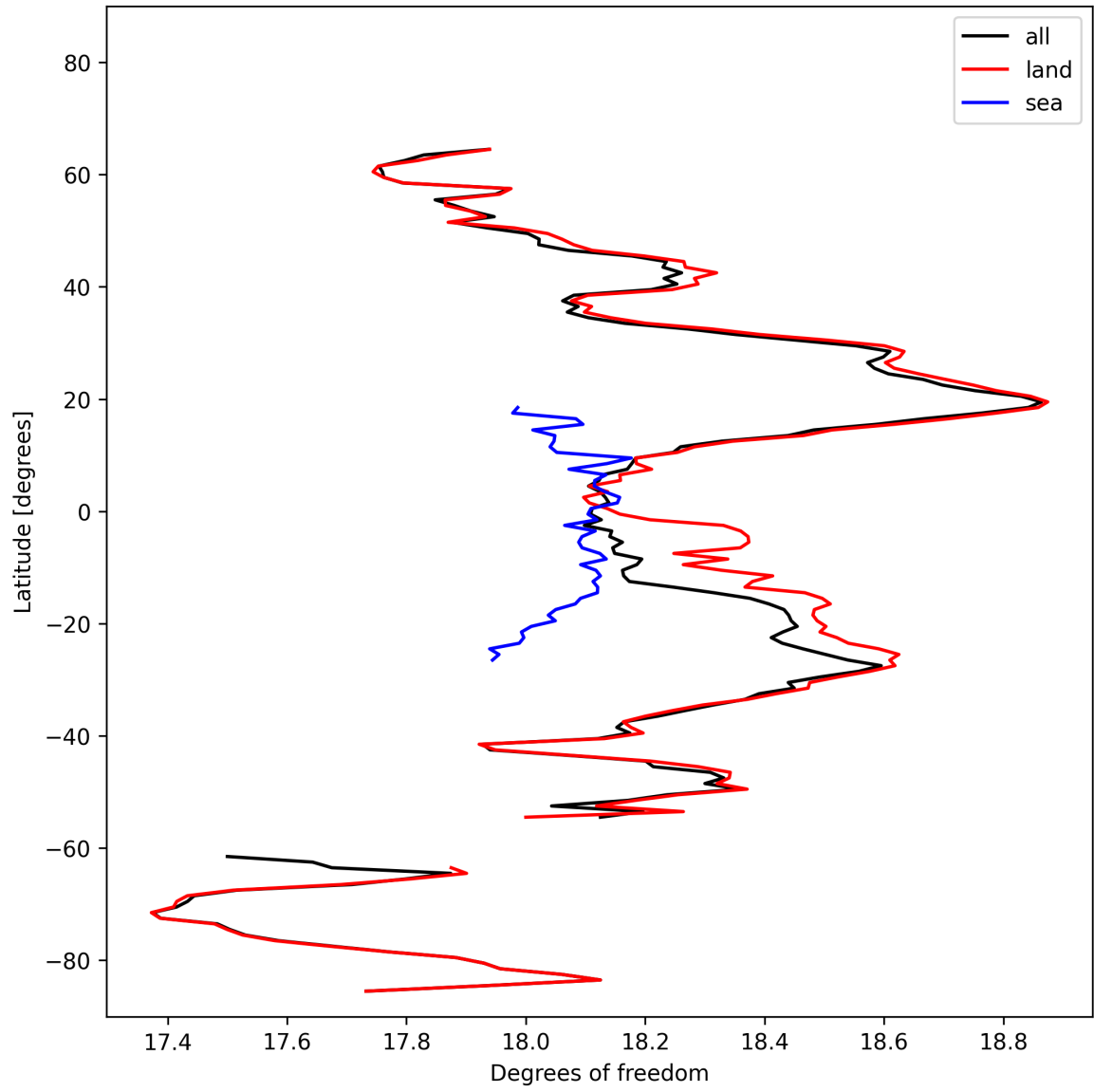
Figure 19: Zonal average of “Degrees of freedom” for 2024-10-20 to 2024-10-22.
