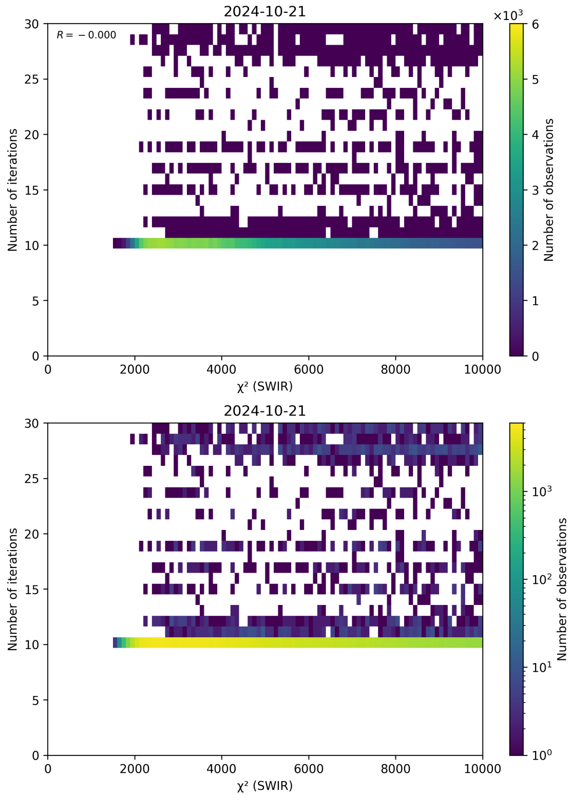
Figure 50: Scatter density plot of “ \chi^2 (SWIR)” against “Number of iterations” for 2024-10-20 to 2024-10-22.
