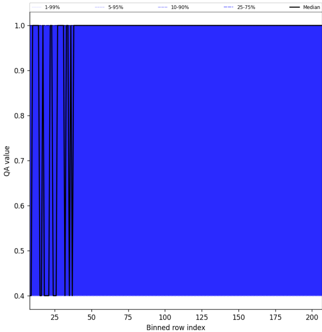
Figure 33: Along track statistics of “QA value” for 2024-10-20 to 2024-10-22
