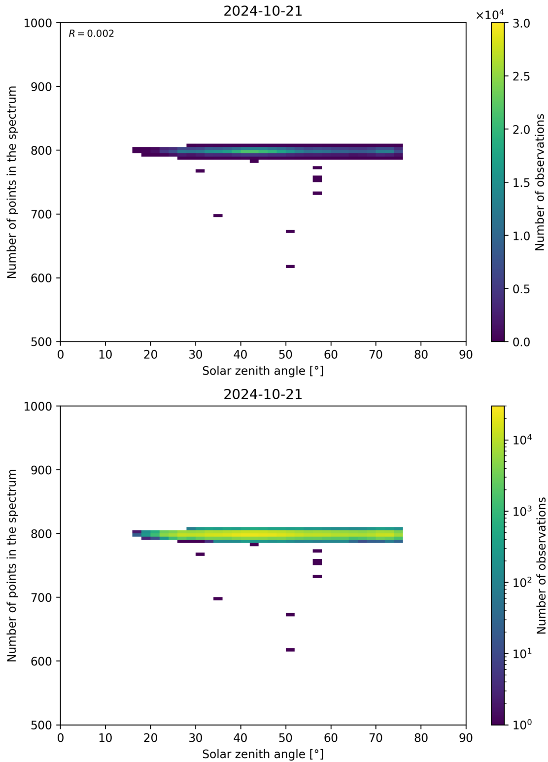
Figure 103: Scatter density plot of “Solar zenith angle” against “Number of points in the spectrum” for 2024-10-20 to 2024-10-22.
