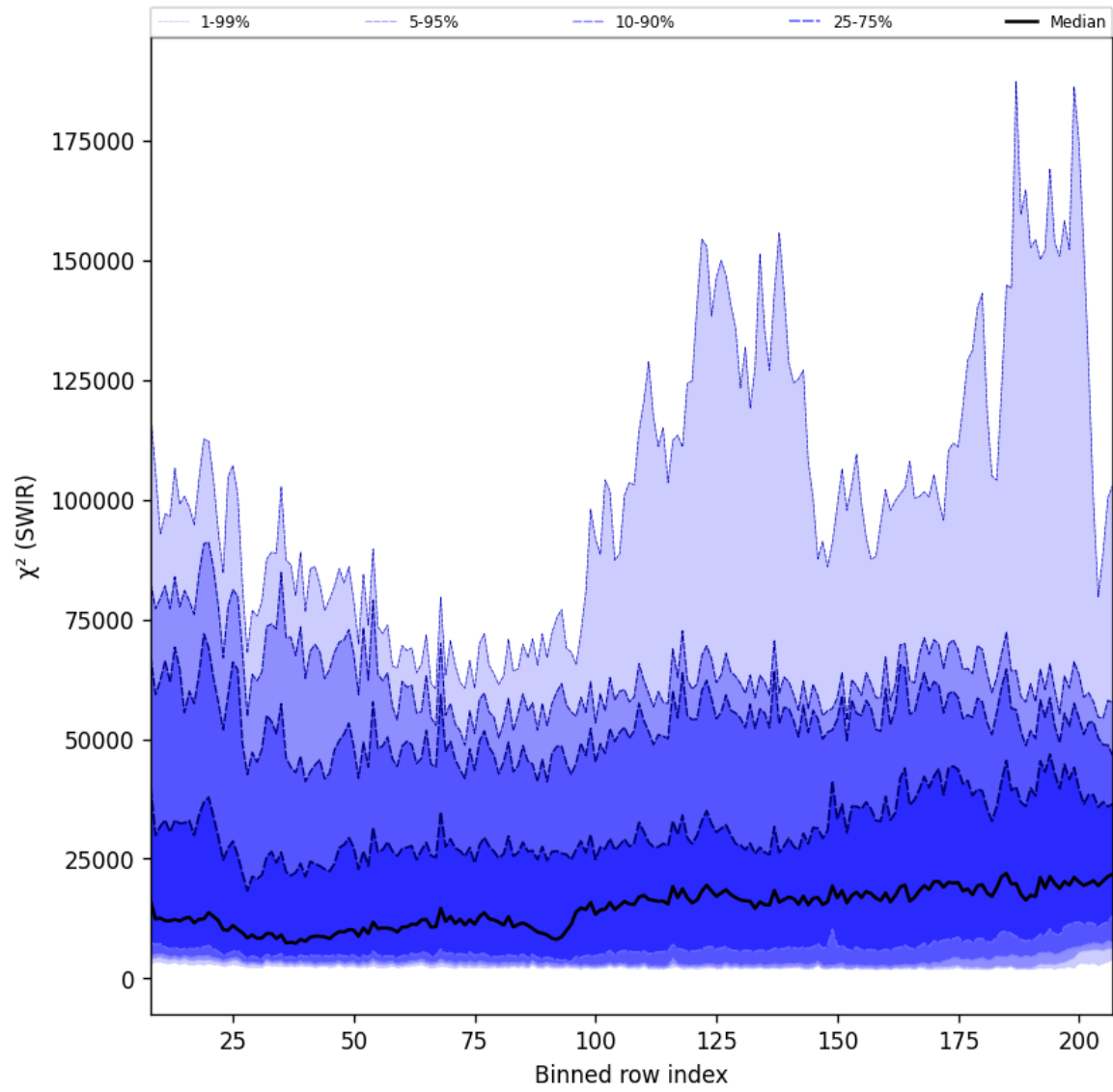
Figure 39: Along track statistics of “ \chi^2 (SWIR)” for 2024-10-20 to 2024-10-22
