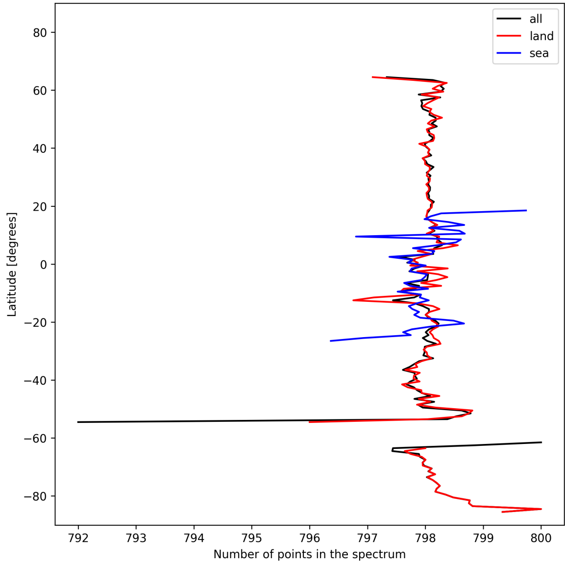
Figure 15: Zonal average of “Number of points in the spectrum” for 2024-10-20 to 2024-10-22.
