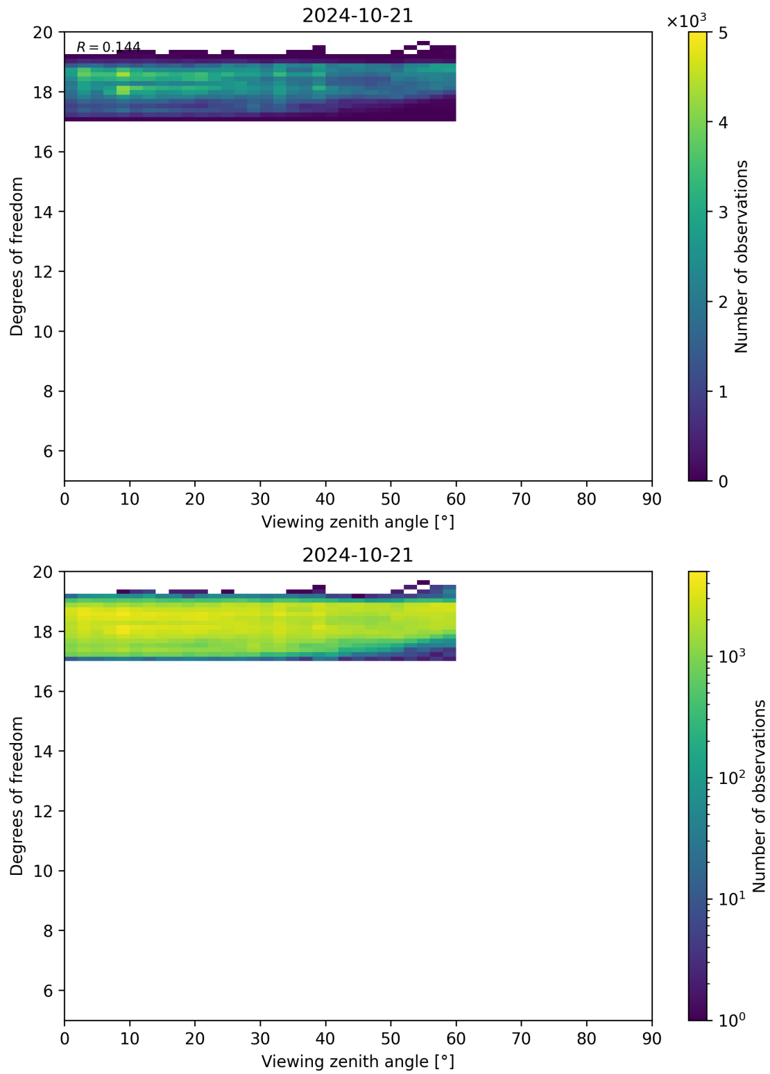
Figure 107: Scatter density plot of “Viewing zenith angle” against “Degrees of freedom” for 2024-10-20 to 2024-10-22.
