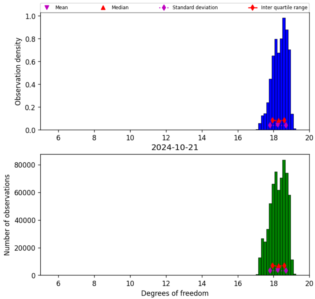
Figure 30: Histogram of “Degrees of freedom” for 2024-10-20 to 2024-10-22
