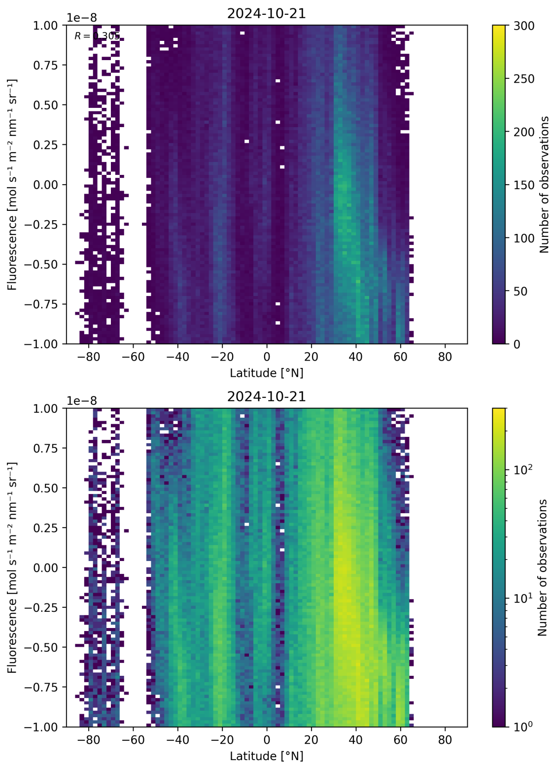
Figure 56: Scatter density plot of “Latitude” against “Fluorescence” for 2024-10-20 to 2024-10-22.
