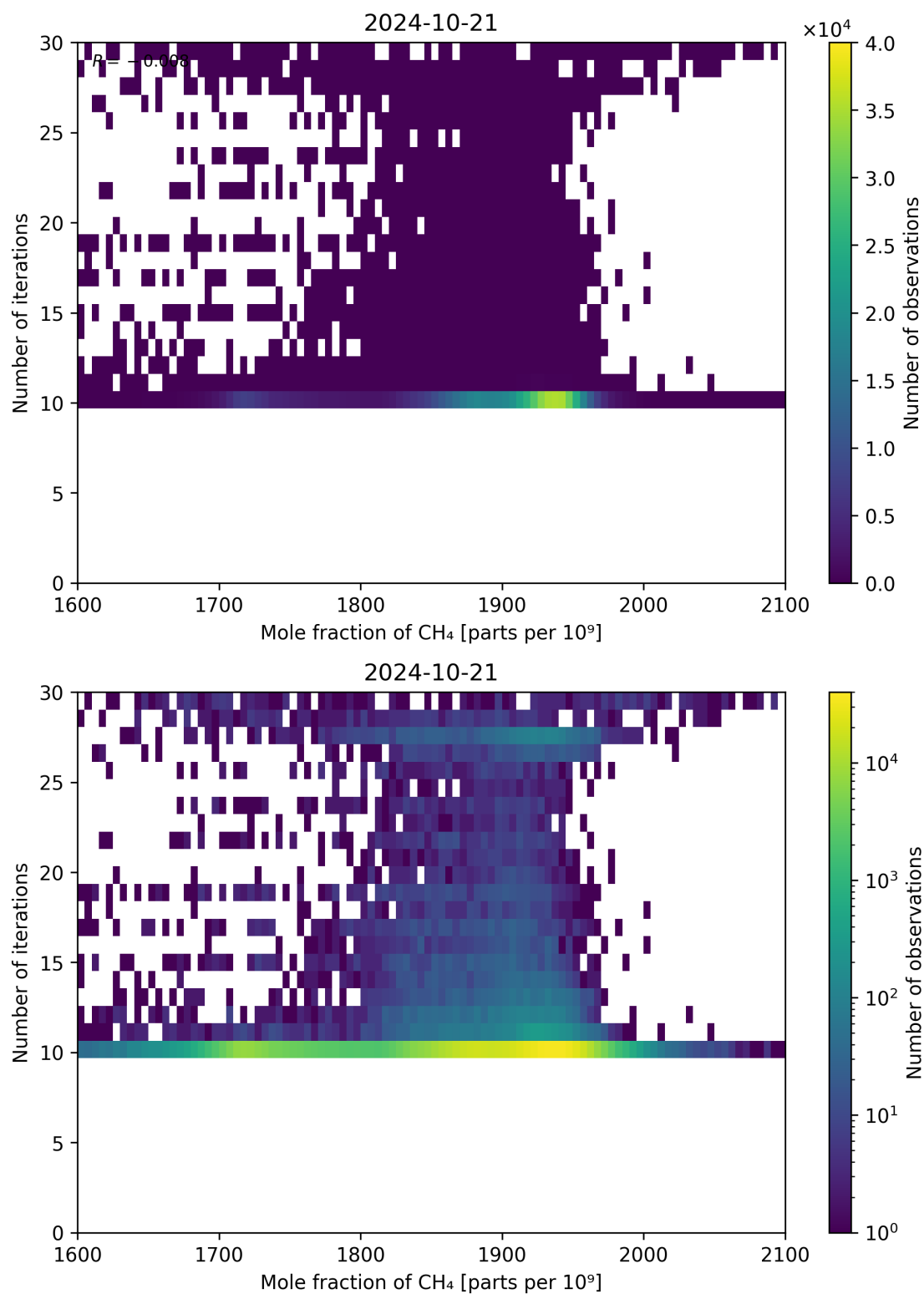
Figure 76: Scatter density plot of “Mole fraction of CH 4 ” against “Number of iterations” for 2024-10-20 to 2024-10-22.
