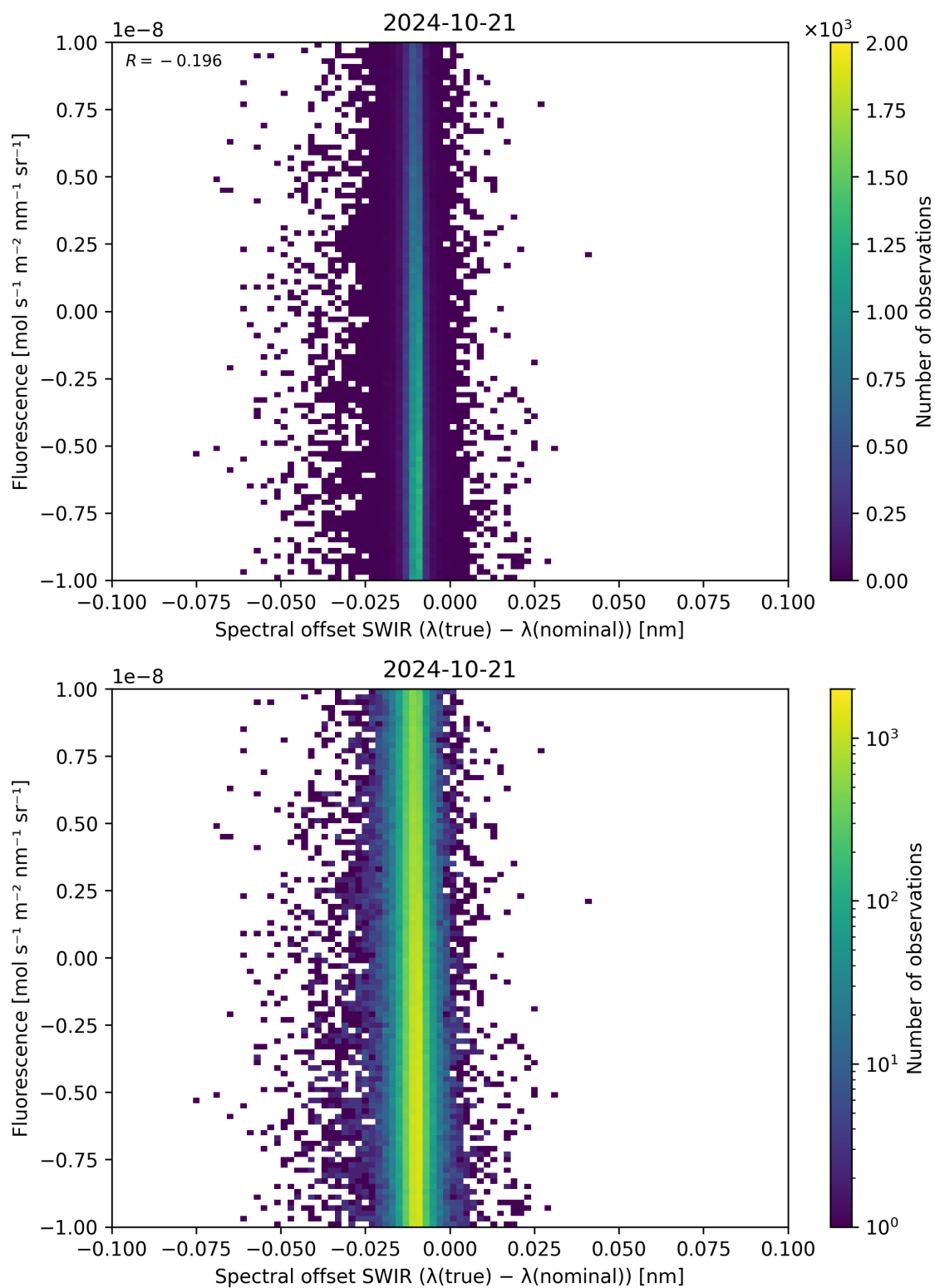
Figure 120: Scatter density plot of “Spectral offset SWIR ( \lambda_{\text{true}} - \lambda_{\text{nominal}} )” against “Fluorescence” for 2024-10-20 to 2024-10-22.
