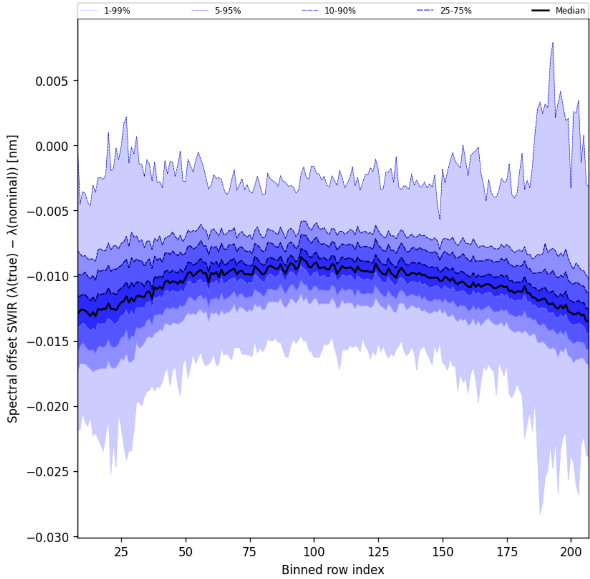
Figure 38: Along track statistics of “Spectral offset SWIR ( \lambda_{\text{true}} - \lambda_{\text{nominal}} )” for 2024-10-20 to 2024-10-22
