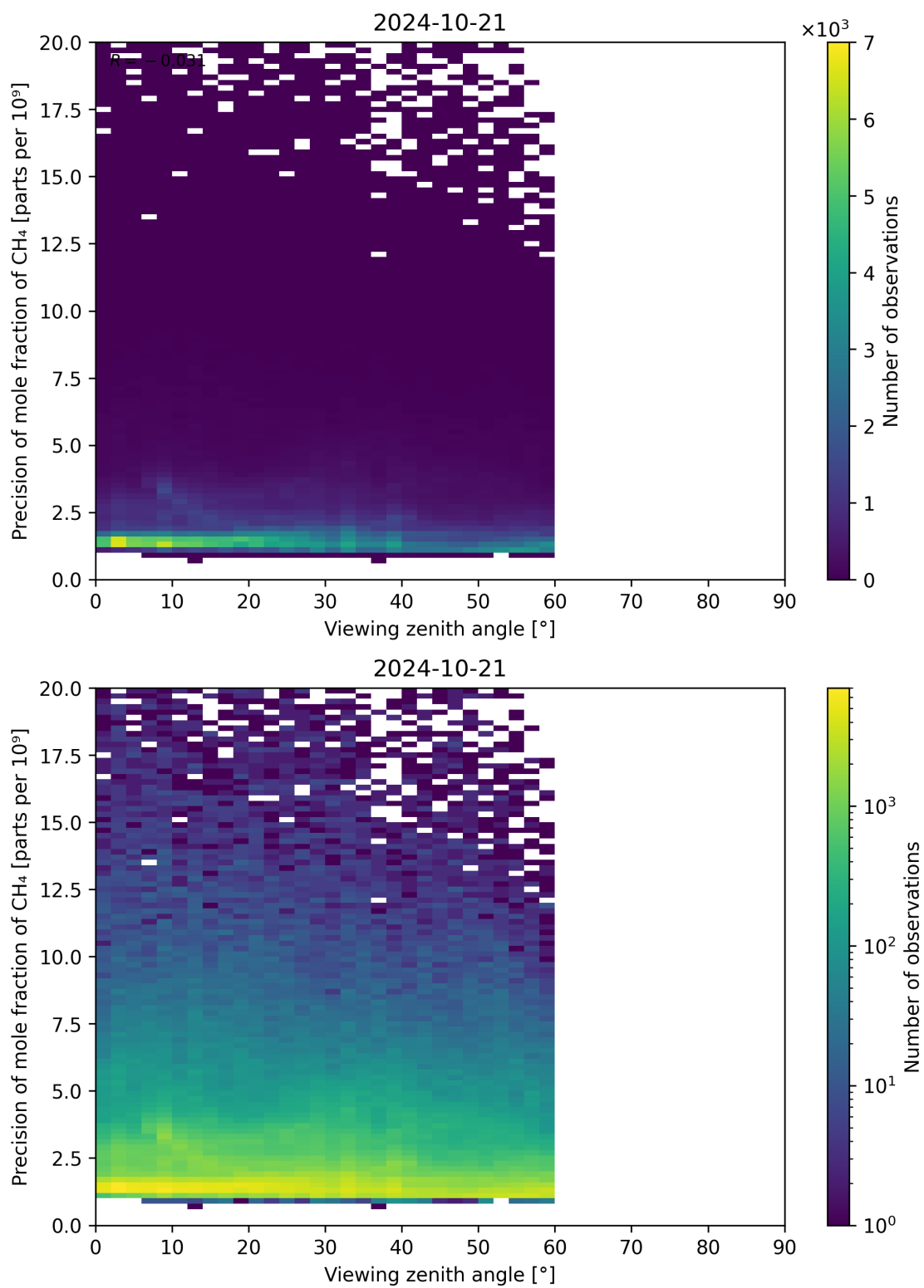
Figure 112: Scatter density plot of “Viewing zenith angle” against “Precision of mole fraction of CH 4 ” for 2024-10-20 to 2024-10-22.
