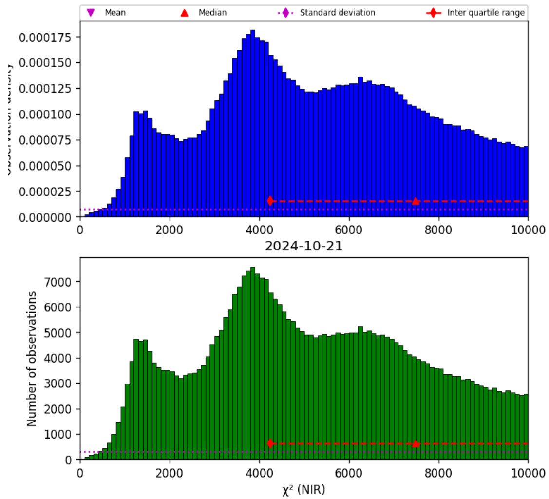
Figure 29: Histogram of “ \chi^2 (NIR)” for 2024-10-20 to 2024-10-22
