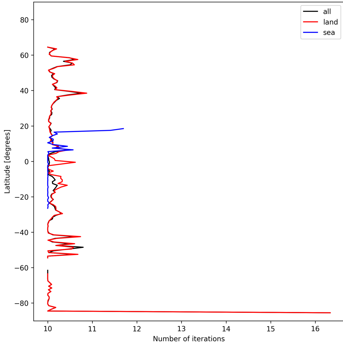
Figure 20: Zonal average of “Number of iterations” for 2024-10-20 to 2024-10-22.
