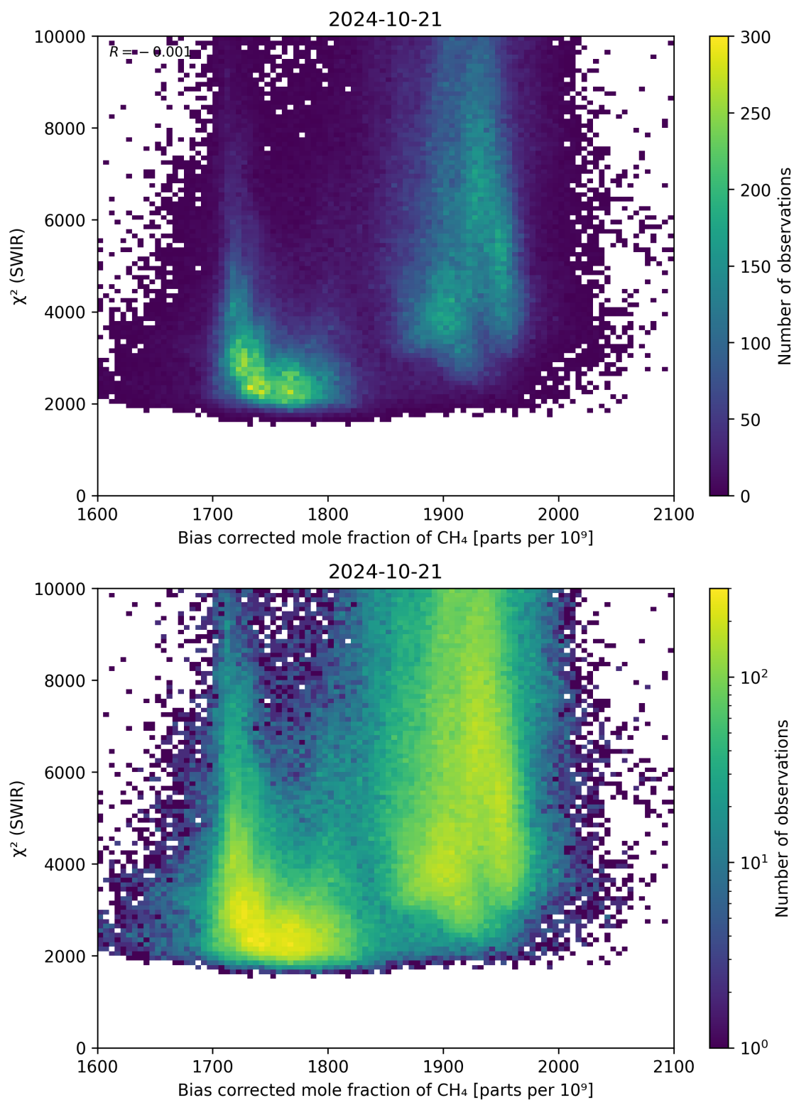
Figure 64: Scatter density plot of “Bias corrected mole fraction of \text{CH}_4 ” against “ \chi^2 (SWIR)” for 2024-10-20 to 2024-10-22.
