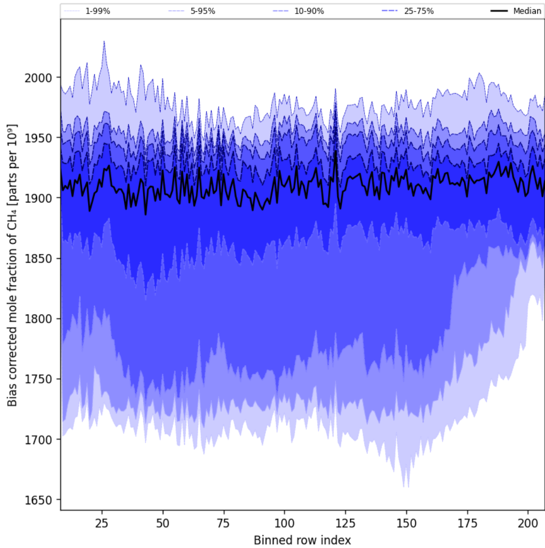
Figure 36: Along track statistics of “Bias corrected mole fraction of CH 4 ” for 2024-10-20 to 2024-10-22
