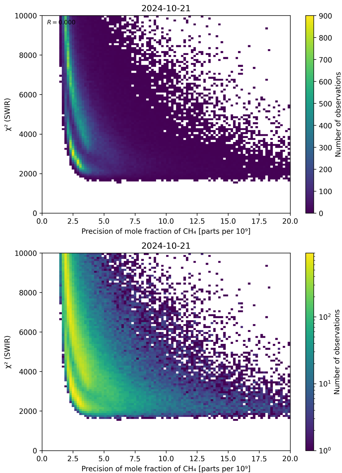
Figure 79: Scatter density plot of “Precision of mole fraction of \text{CH}_4 ” against “ \chi^2 (SWIR)” for 2024-10-20 to 2024-10-22.
