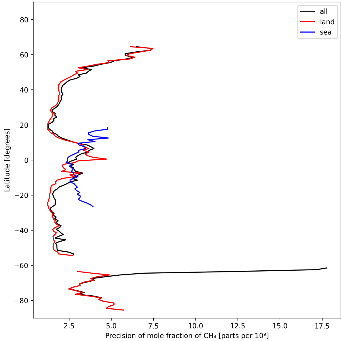
Figure 13: Zonal average of “Precision of mole fraction of CH 4 ” for 2024-10-20 to 2024-10-22.
