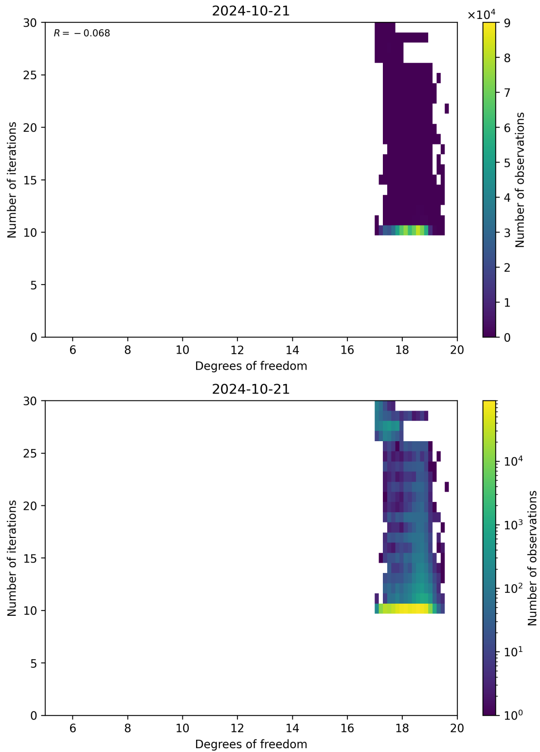
Figure 52: Scatter density plot of “Degrees of freedom” against “Number of iterations” for 2024-10-20 to 2024-10-22.
