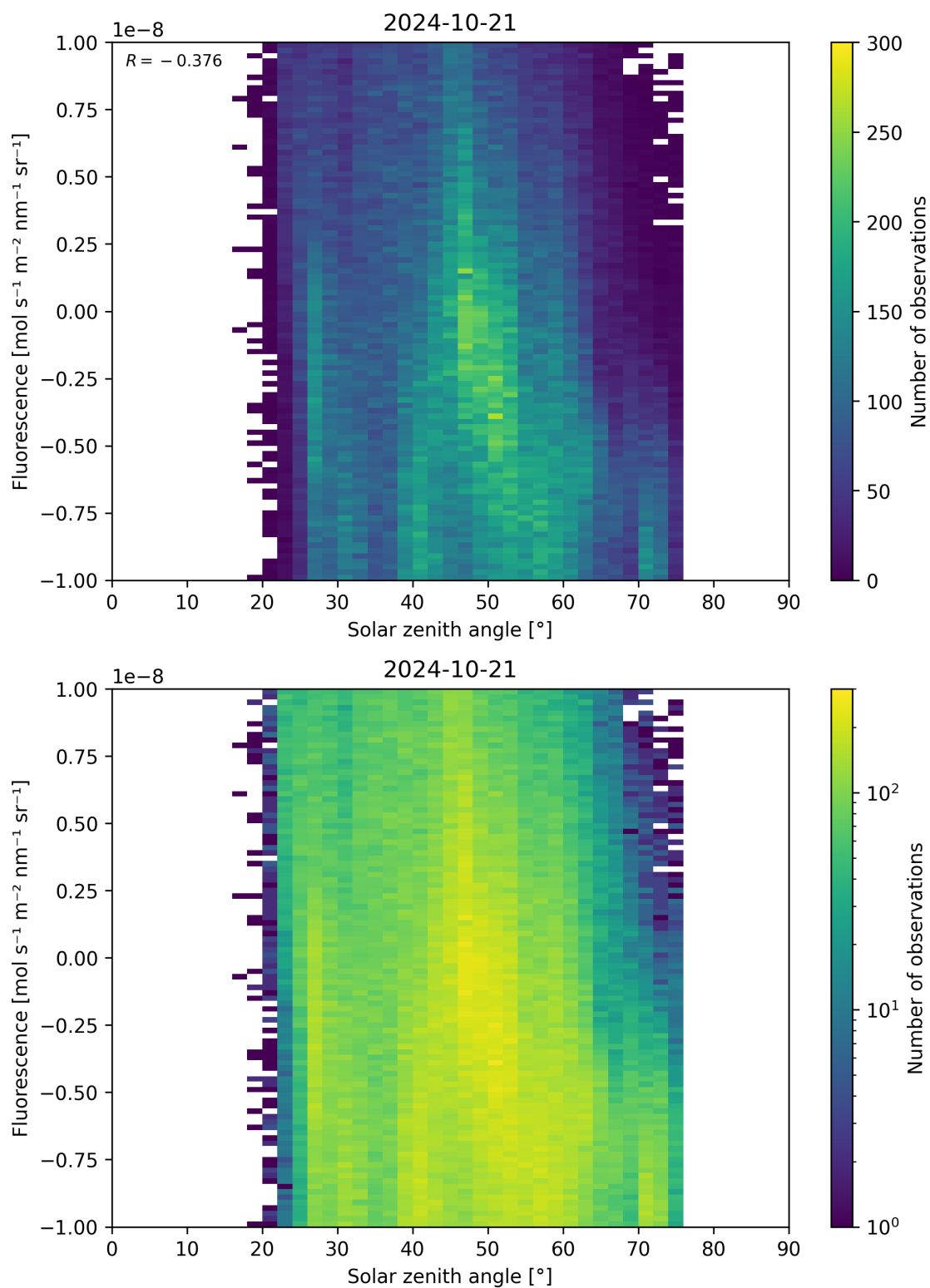
Figure 97: Scatter density plot of “Solar zenith angle” against “Fluorescence” for 2024-10-20 to 2024-10-22.
