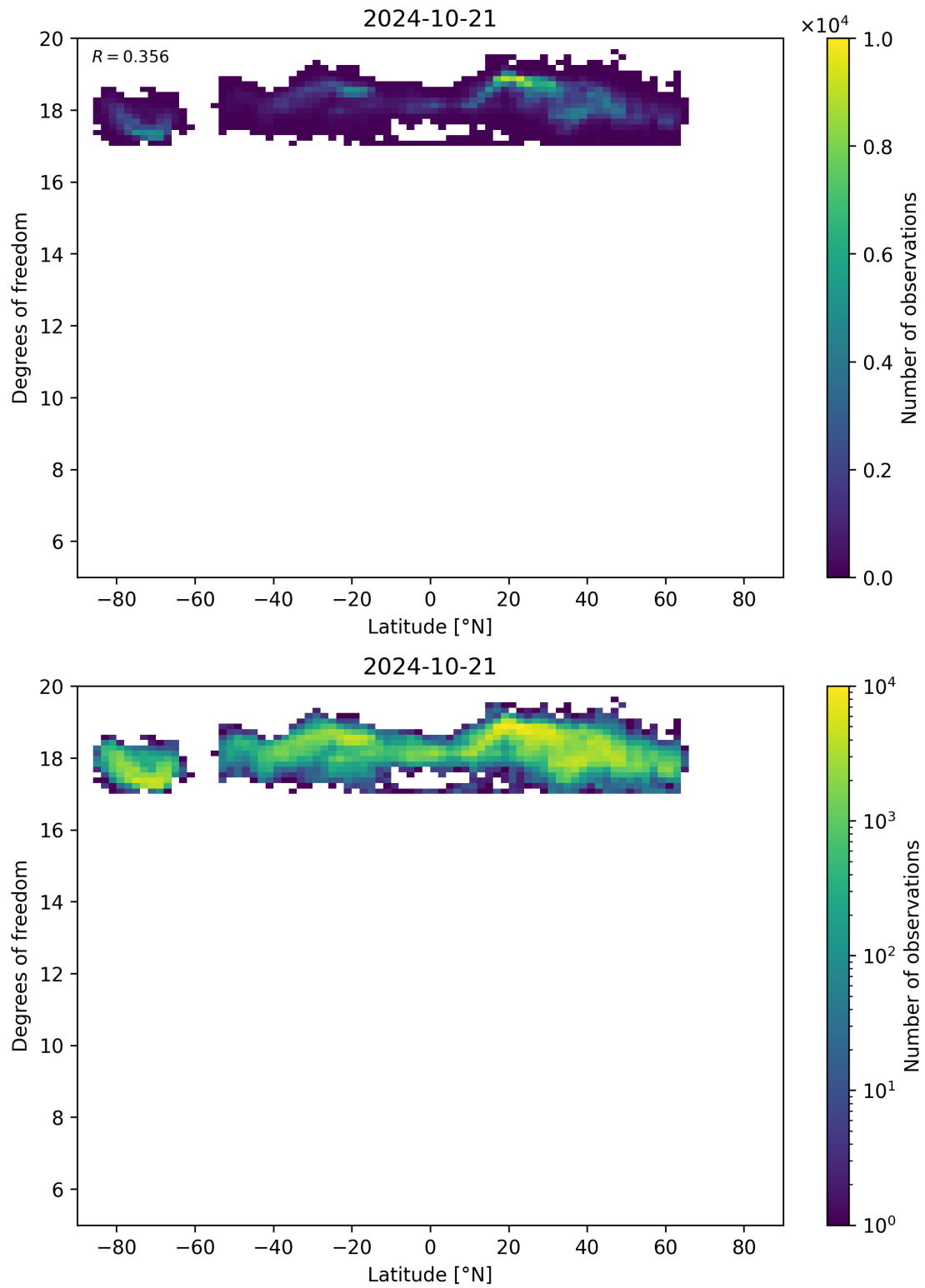
Figure 55: Scatter density plot of “Latitude” against “Degrees of freedom” for 2024-10-20 to 2024-10-22.
