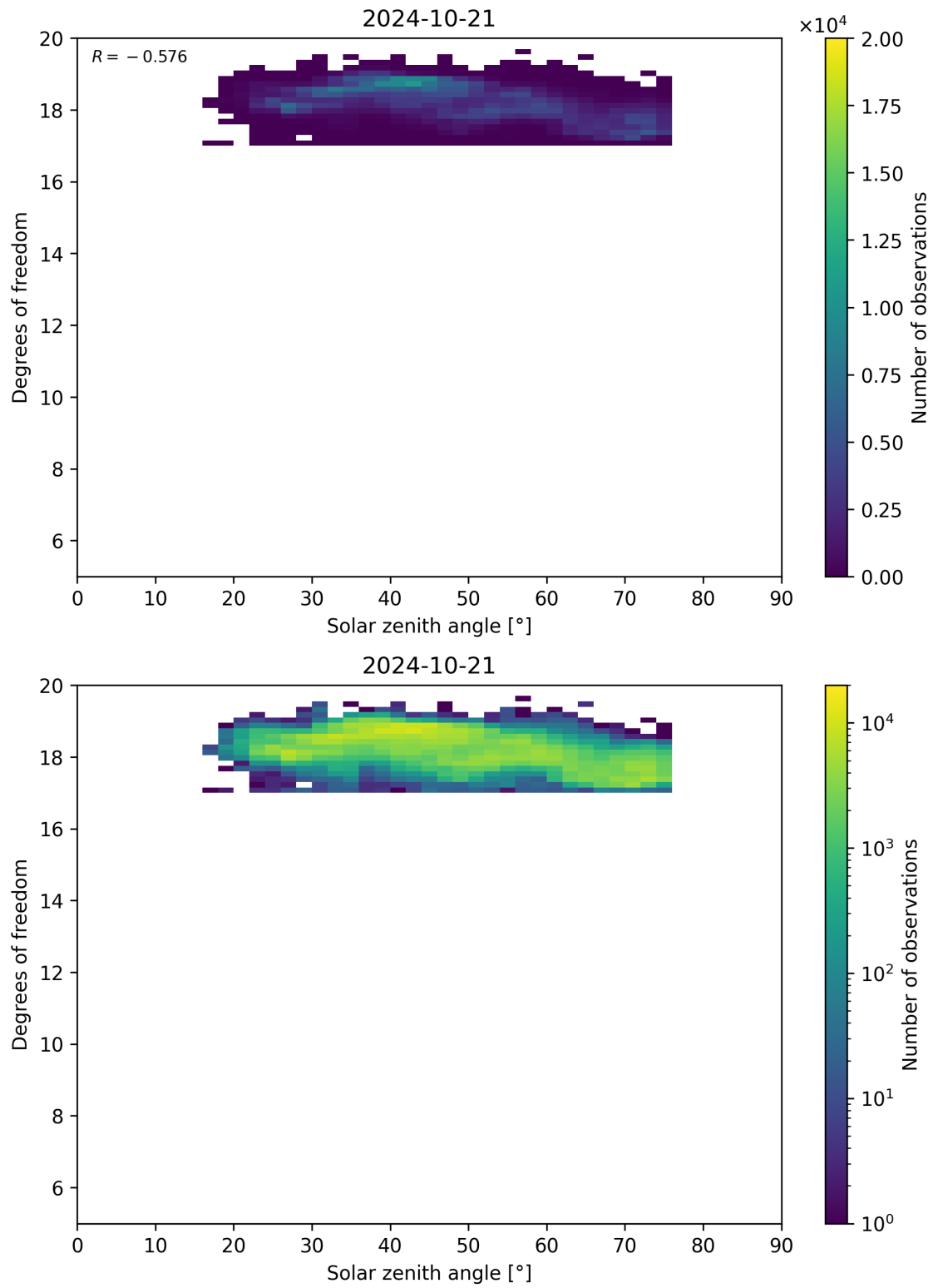
Figure 96: Scatter density plot of “Solar zenith angle” against “Degrees of freedom” for 2024-10-20 to 2024-10-22.
