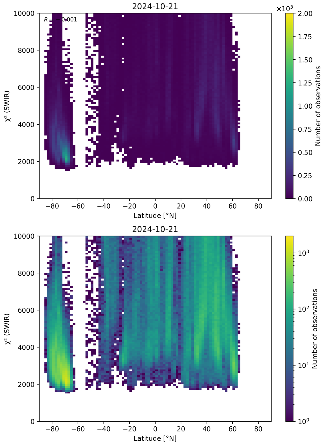
Figure 54: Scatter density plot of “Latitude” against “ \chi^2 (SWIR)” for 2024-10-20 to 2024-10-22.
