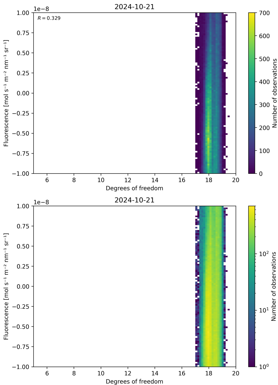
Figure 51: Scatter density plot of “Degrees of freedom” against “Fluorescence” for 2024-10-20 to 2024-10-22.
