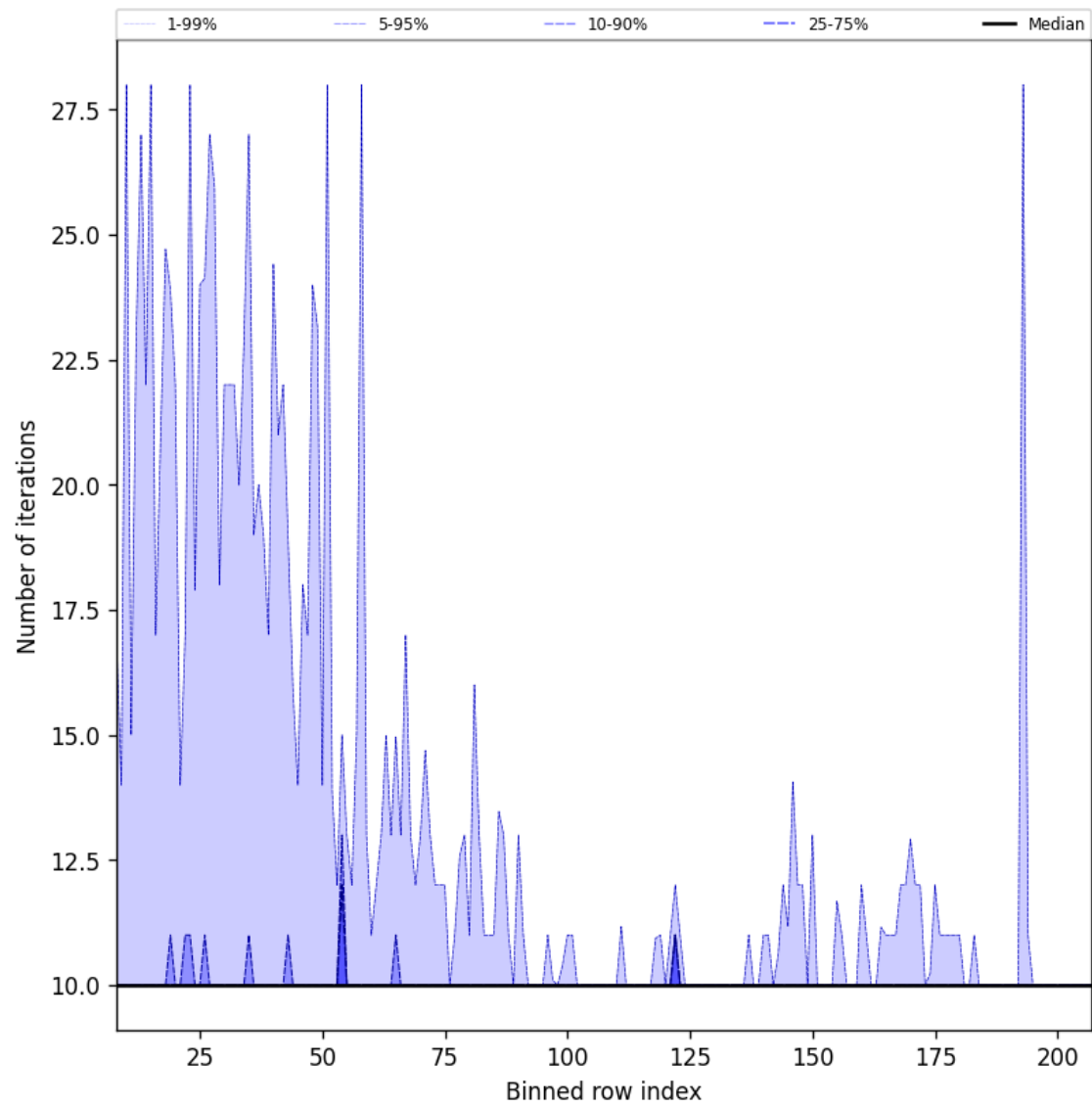
Figure 42: Along track statistics of “Number of iterations” for 2024-10-20 to 2024-10-22
