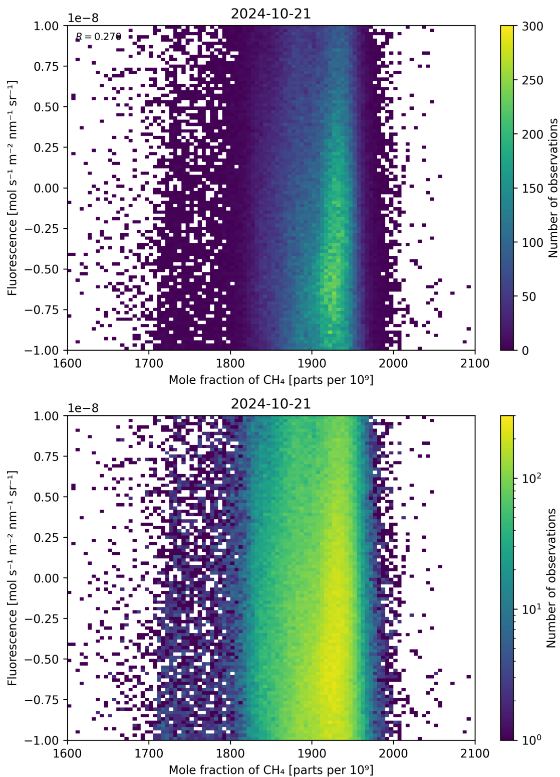
Figure 73: Scatter density plot of “Mole fraction of \text{CH}_4 ” against “Fluorescence” for 2024-10-20 to 2024-10-22.
