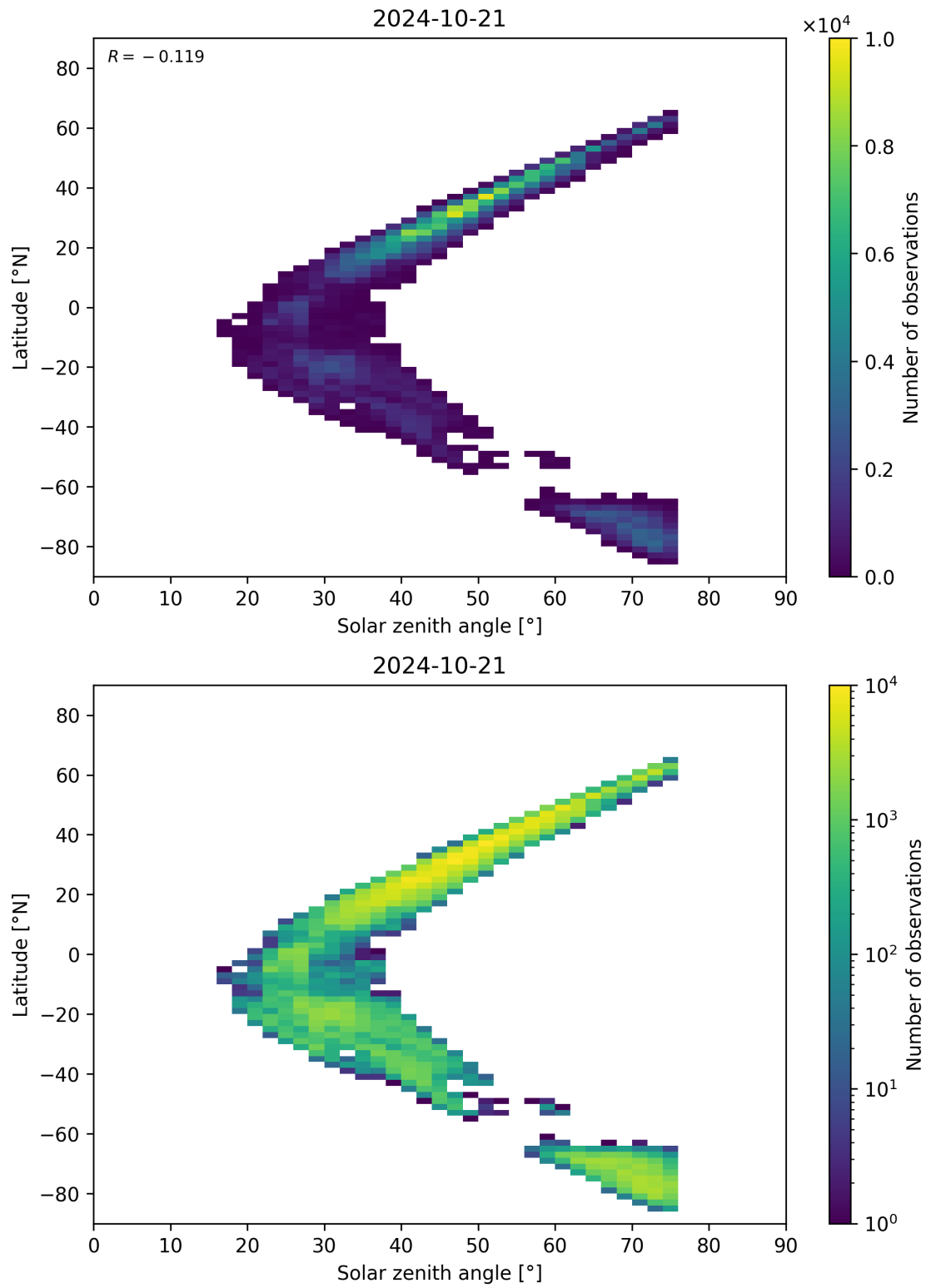
Figure 98: Scatter density plot of “Solar zenith angle” against “Latitude” for 2024-10-20 to 2024-10-22.
