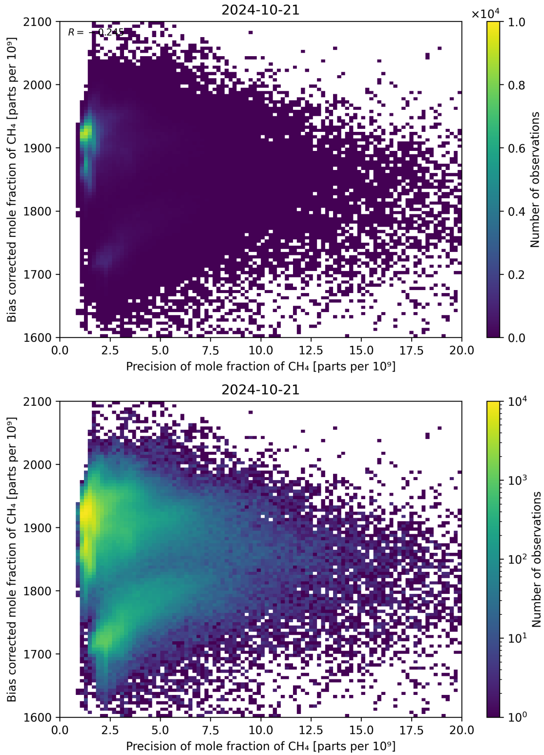
Figure 82: Scatter density plot of “Precision of mole fraction of CH 4 ” against “Bias corrected mole fraction of CH 4 ” for 2024-10-20 to 2024-10-22.
