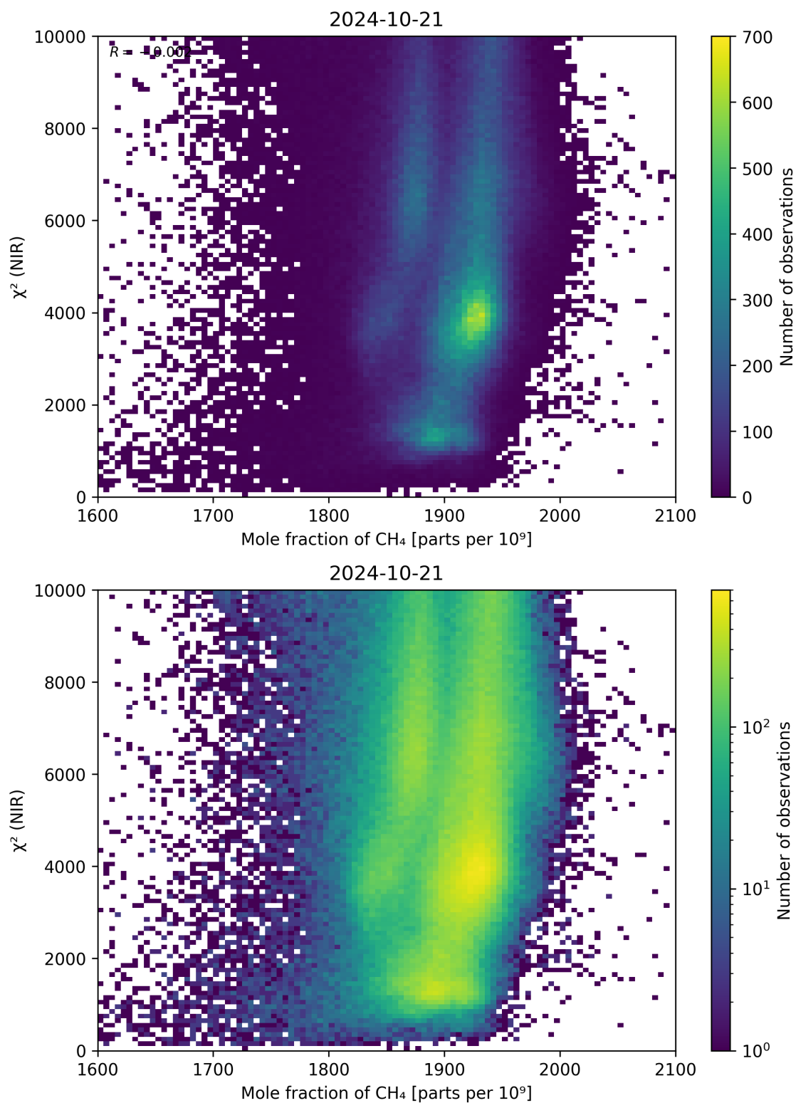
Figure 70: Scatter density plot of “Mole fraction of CH 4 ” against “ \chi^2 (NIR)” for 2024-10-20 to 2024-10-22.
