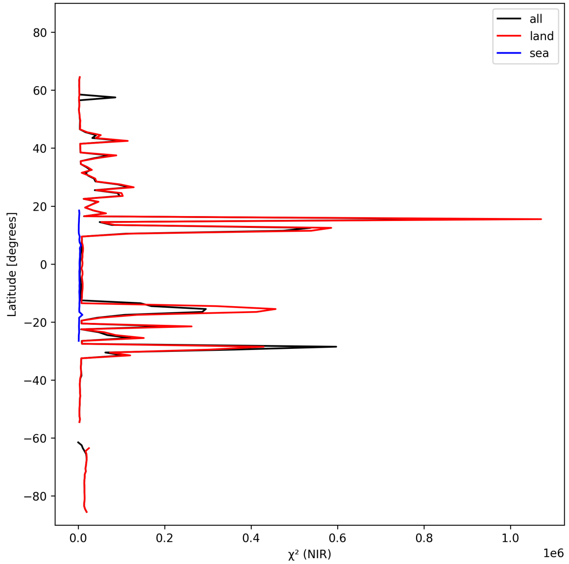
Figure 18: Zonal average of “ \chi^2 (NIR)” for 2024-10-20 to 2024-10-22.
