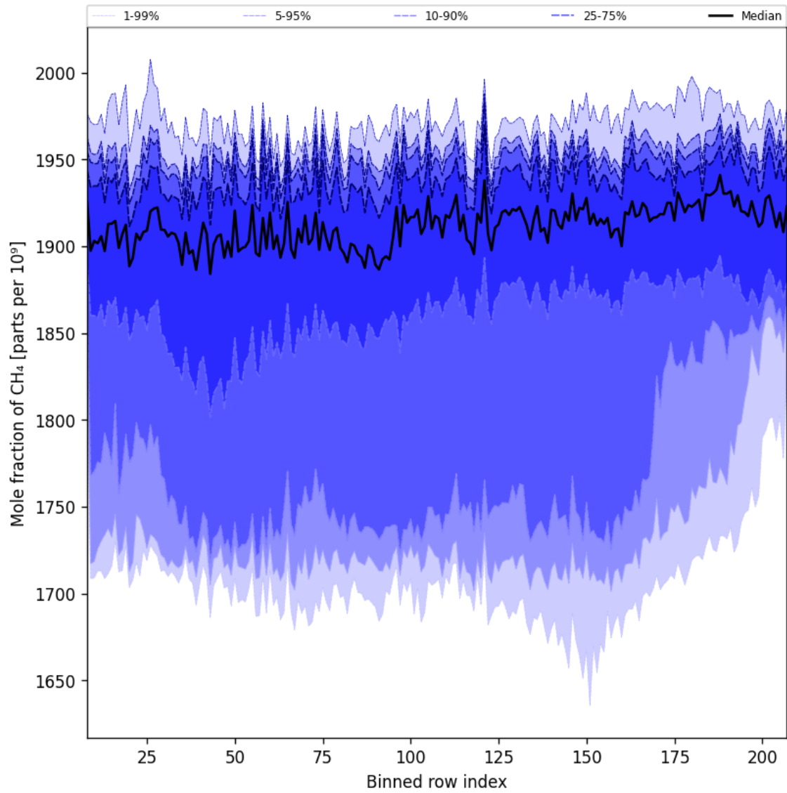
Figure 34: Along track statistics of “Mole fraction of CH 4 ” for 2024-10-20 to 2024-10-22
