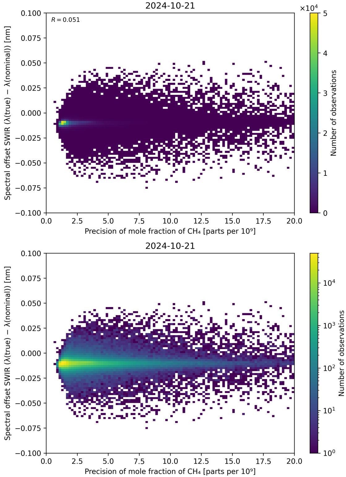
Figure 85: Scatter density plot of “Precision of mole fraction of \text{CH}_4 ” against “Spectral offset SWIR ( \lambda_{\text{true}} - \lambda_{\text{nominal}} )” for 2024-10-20 to 2024-10-22.
