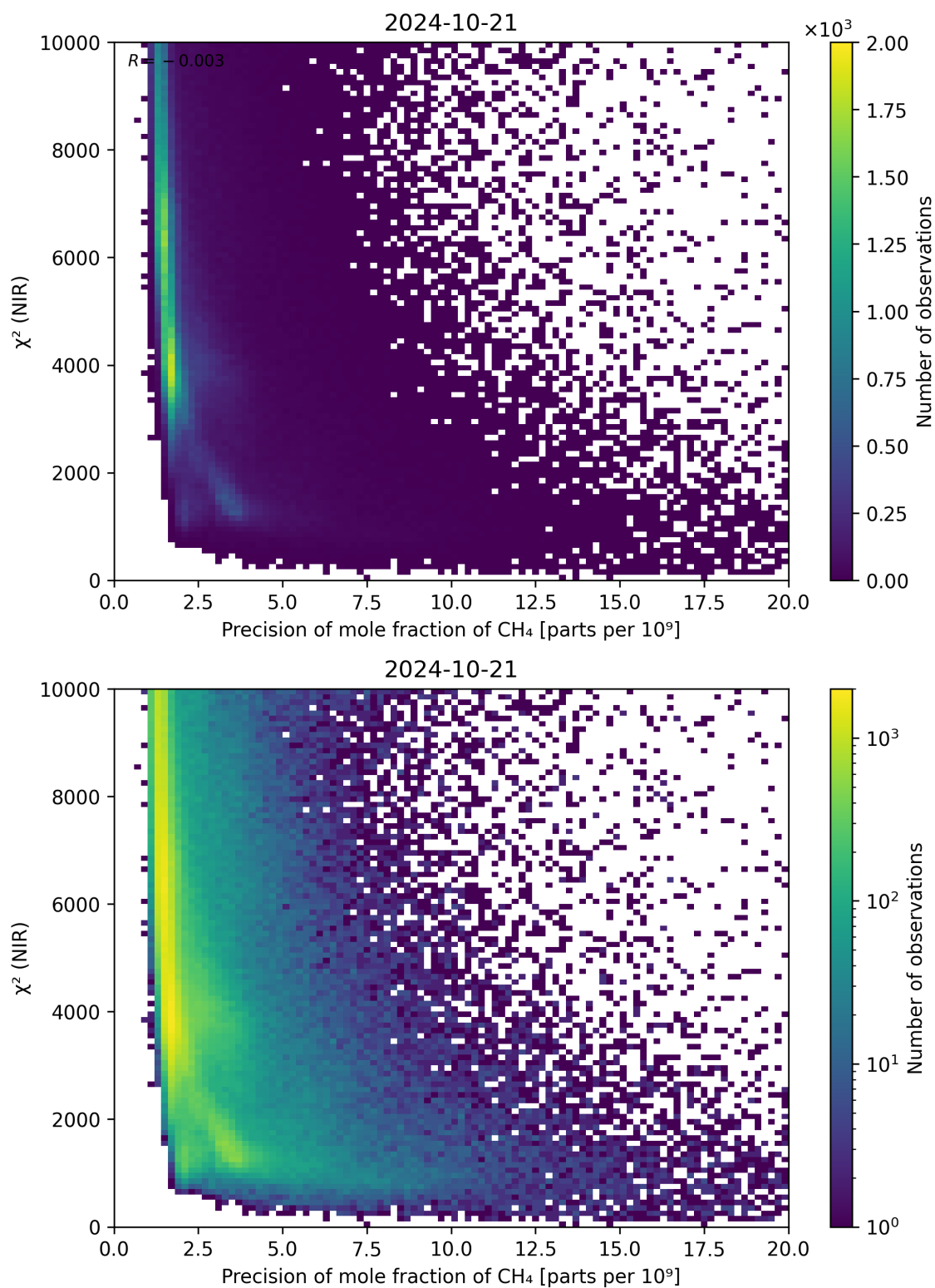
Figure 78: Scatter density plot of “Precision of mole fraction of \text{CH}_4 ” against “ \chi^2 (NIR)” for 2024-10-20 to 2024-10-22.
