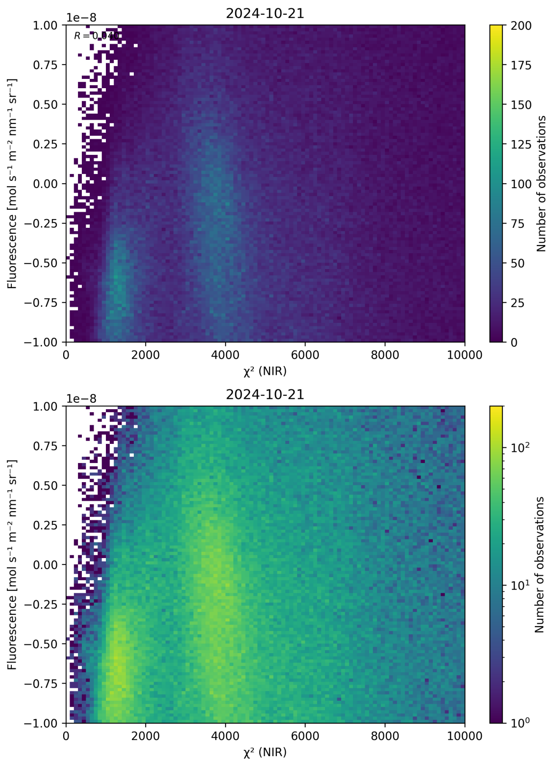
Figure 45: Scatter density plot of “ \chi^2 (NIR)” against “Fluorescence” for 2024-10-20 to 2024-10-22.
