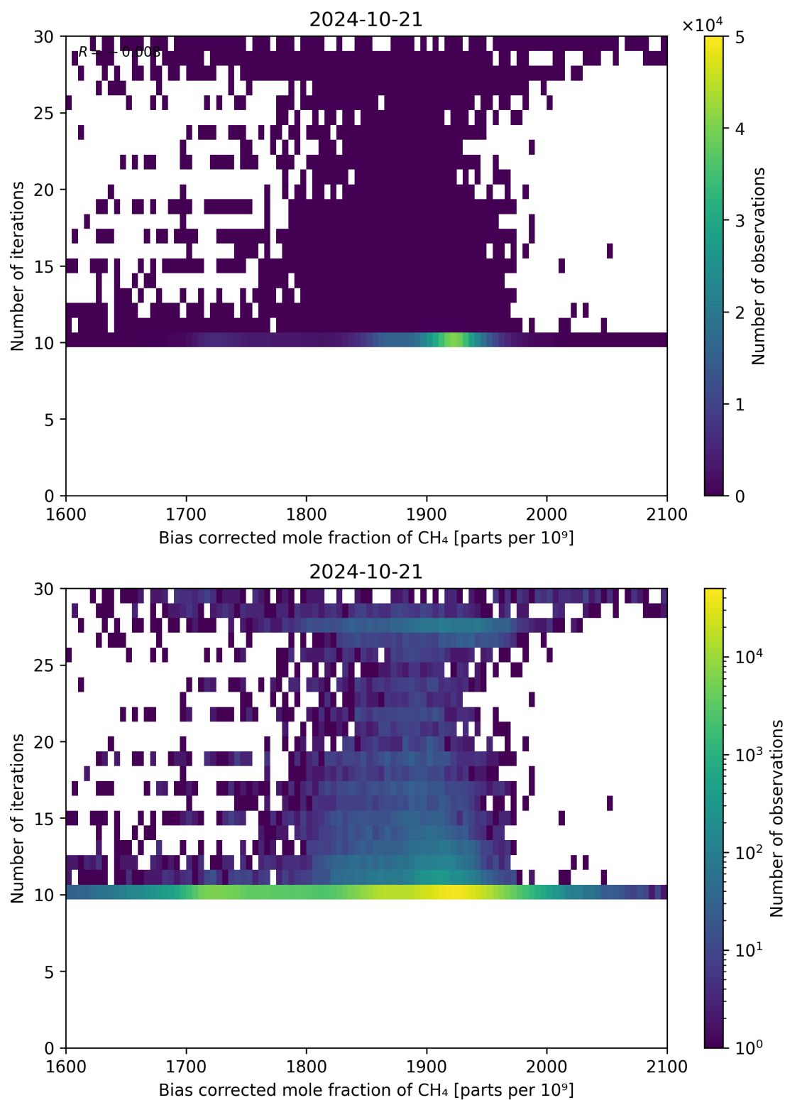
Figure 67: Scatter density plot of “Bias corrected mole fraction of \text{CH}_4 ” against “Number of iterations” for 2024-10-20 to 2024-10-22.
