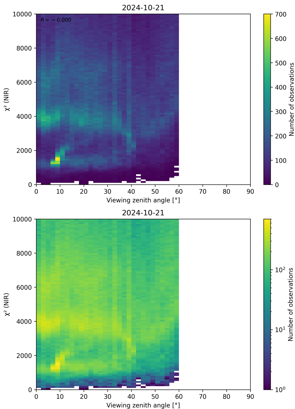
Figure 105: Scatter density plot of “Viewing zenith angle” against “ \chi^2 (NIR)” for 2024-10-20 to 2024-10-22.
