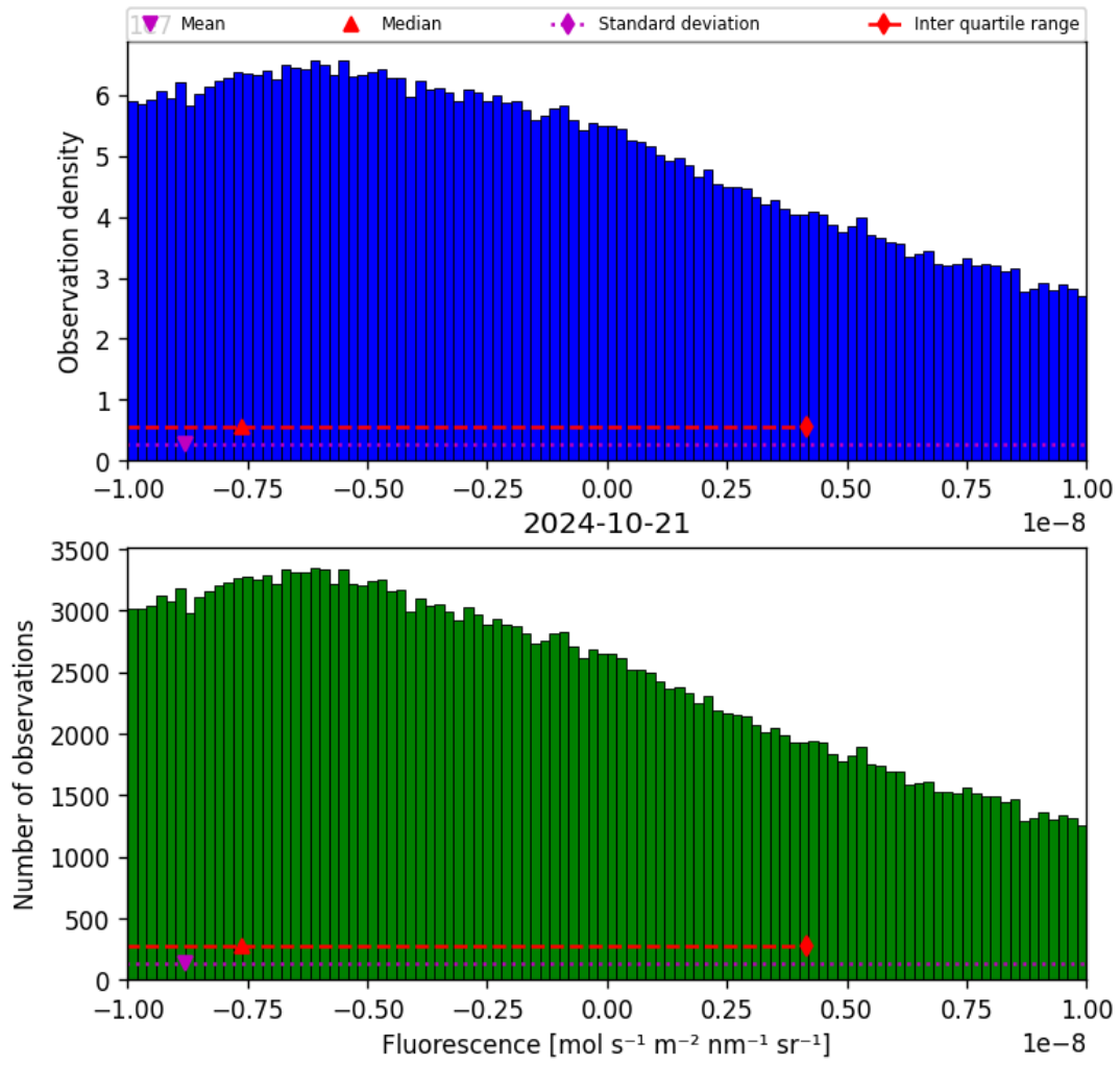
Figure 32: Histogram of “Fluorescence” for 2024-10-20 to 2024-10-22
