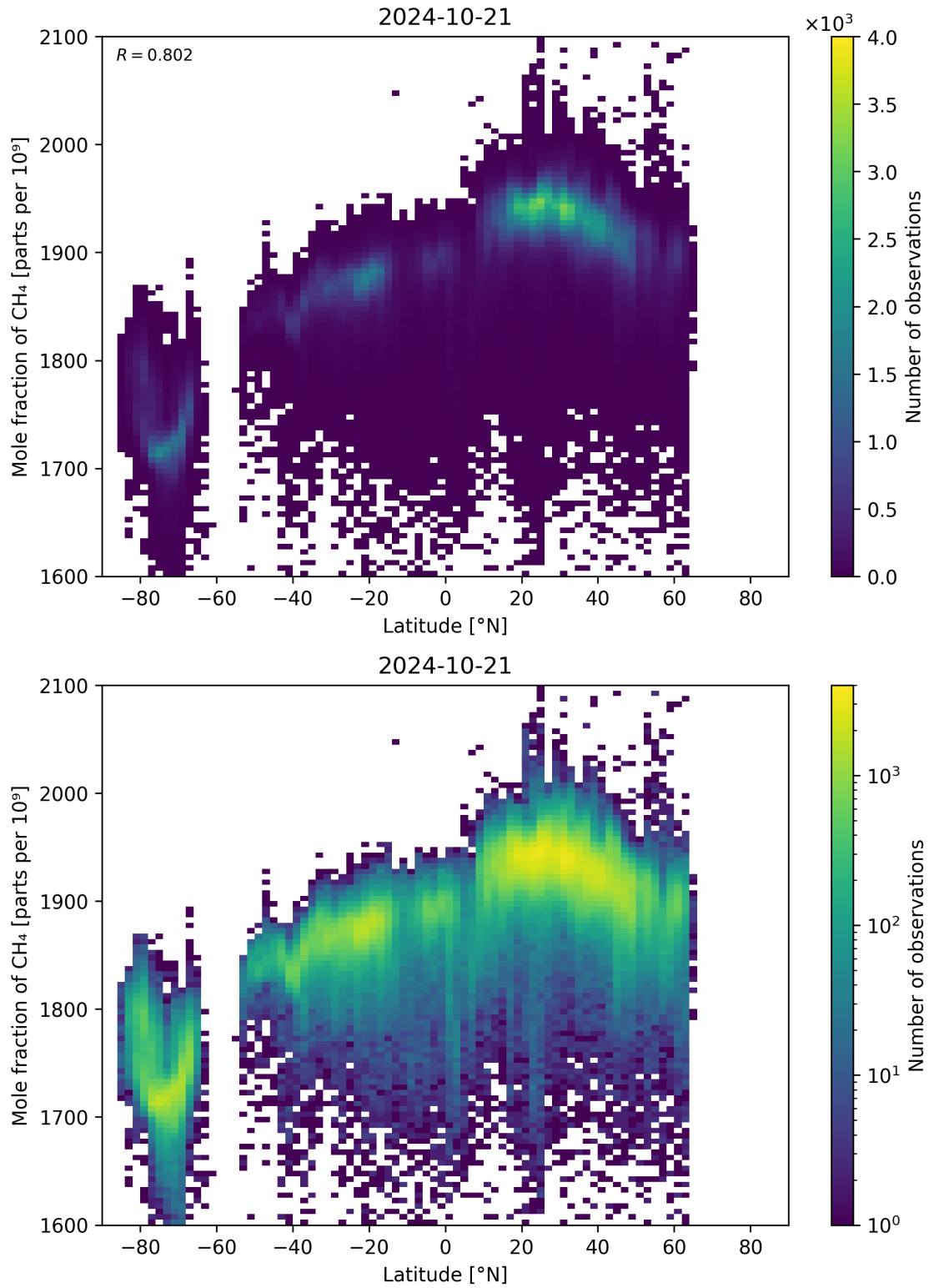
Figure 57: Scatter density plot of “Latitude” against “Mole fraction of CH 4 ” for 2024-10-20 to 2024-10-22.
