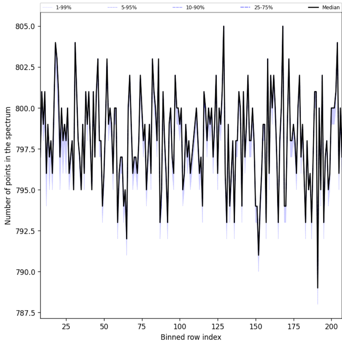
Figure 37: Along track statistics of “Number of points in the spectrum” for 2024-10-20 to 2024-10-22
