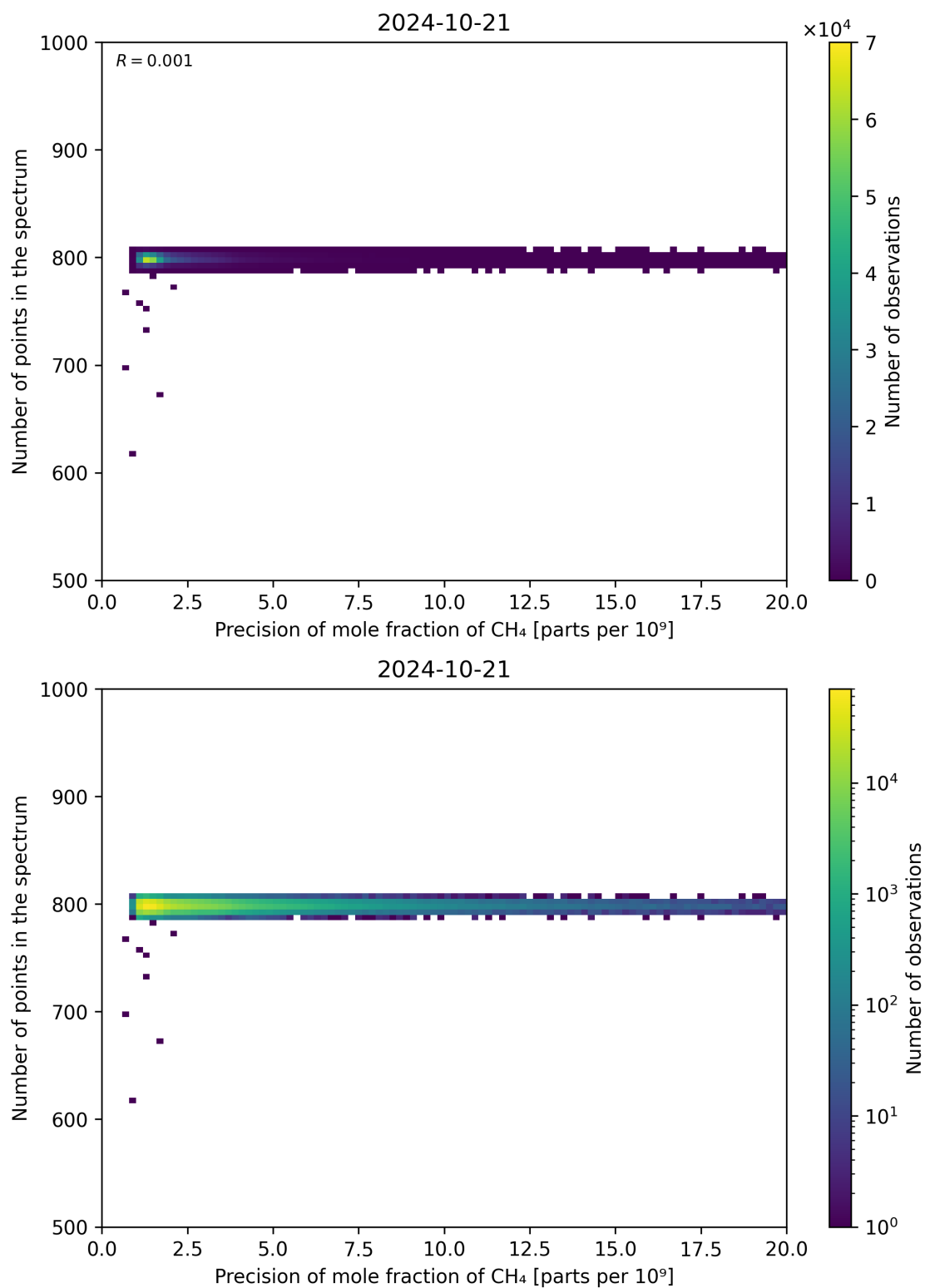
Figure 84: Scatter density plot of “Precision of mole fraction of CH 4 ” against “Number of points in the spectrum” for 2024-10-20 to 2024-10-22.
