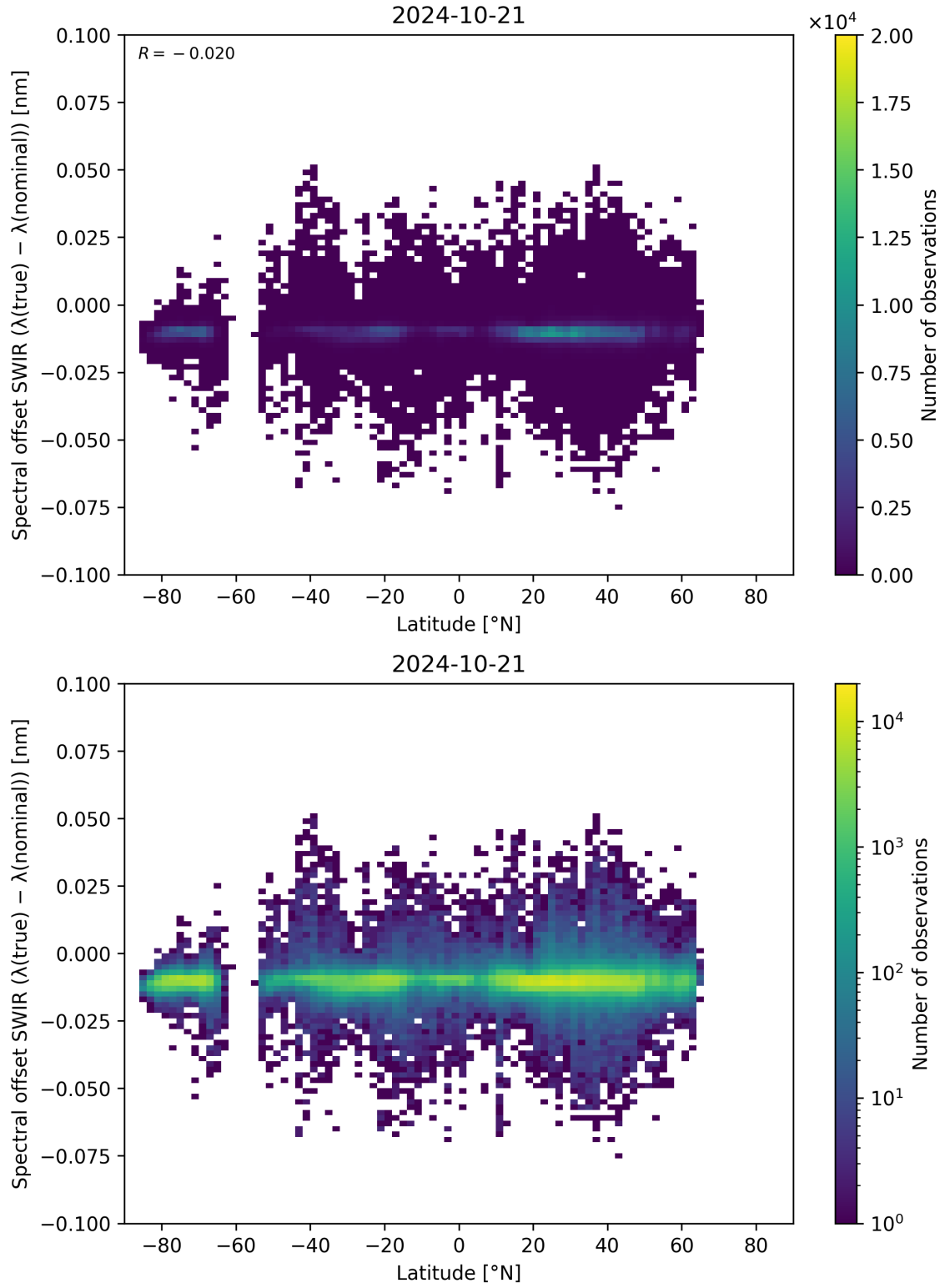
Figure 62: Scatter density plot of “Latitude” against “Spectral offset SWIR ( \lambda_{\text{true}} - \lambda_{\text{nominal}} )” for 2024-10-20 to 2024-10-22.
