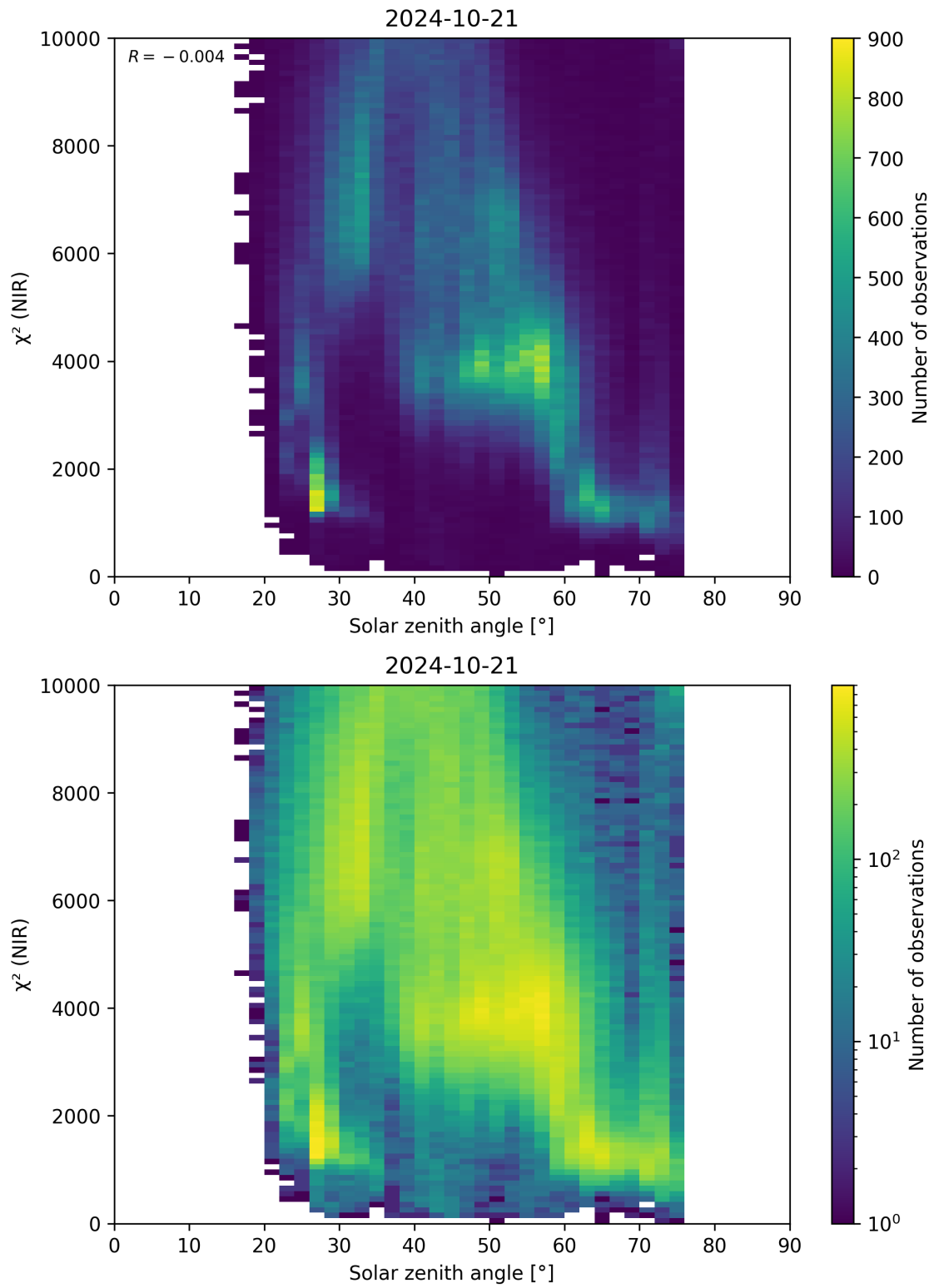
Figure 94: Scatter density plot of “Solar zenith angle” against “ \chi^2 (NIR)” for 2024-10-20 to 2024-10-22.
