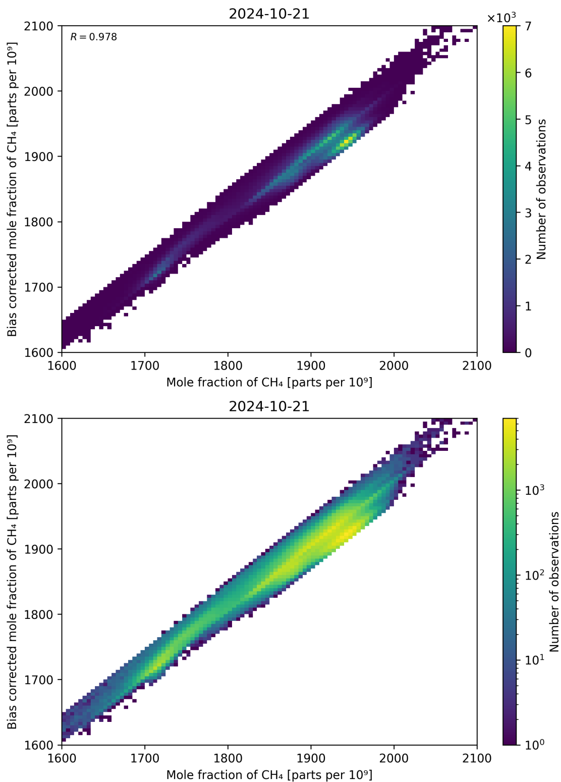
Figure 74: Scatter density plot of “Mole fraction of CH 4 ” against “Bias corrected mole fraction of CH 4 ” for 2024-10-20 to 2024-10-22.
