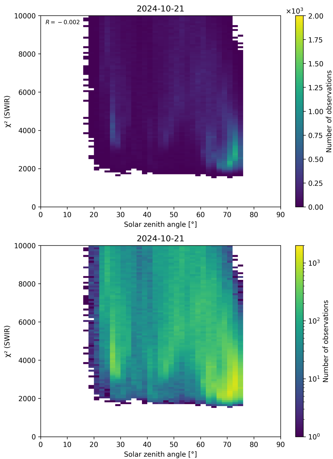
Figure 95: Scatter density plot of “Solar zenith angle” against “ \chi^2 (SWIR)” for 2024-10-20 to 2024-10-22.
