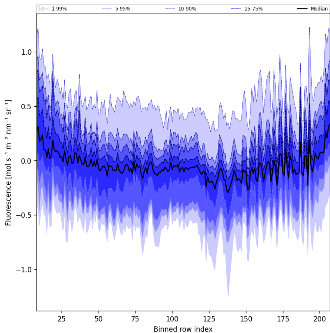
Figure 43: Along track statistics of “Fluorescence” for 2024-10-20 to 2024-10-22
