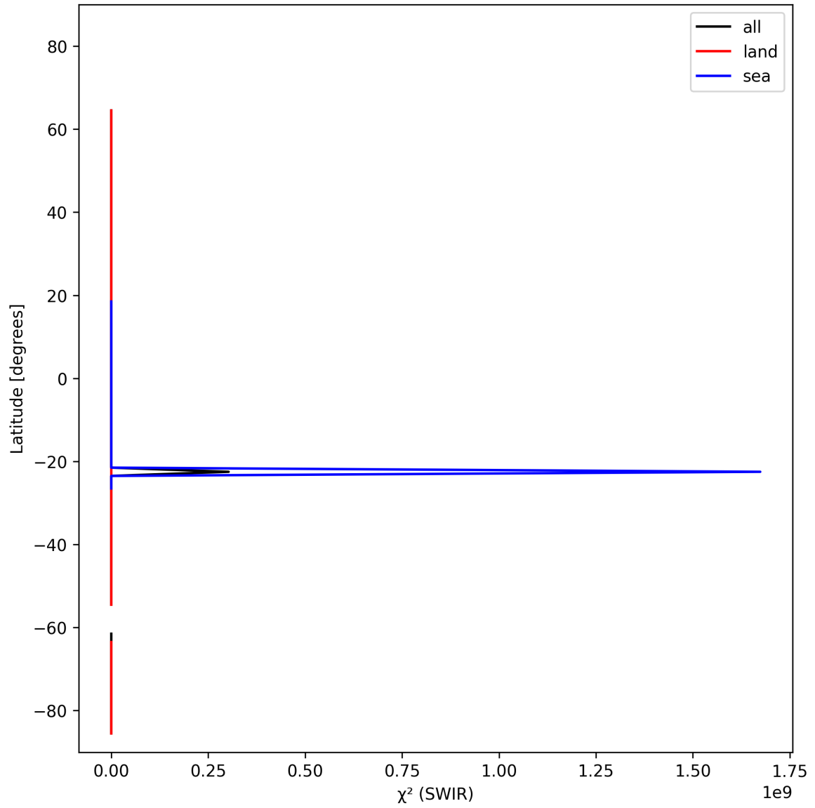
Figure 17: Zonal average of “ \chi^2 (SWIR)” for 2024-10-20 to 2024-10-22.
