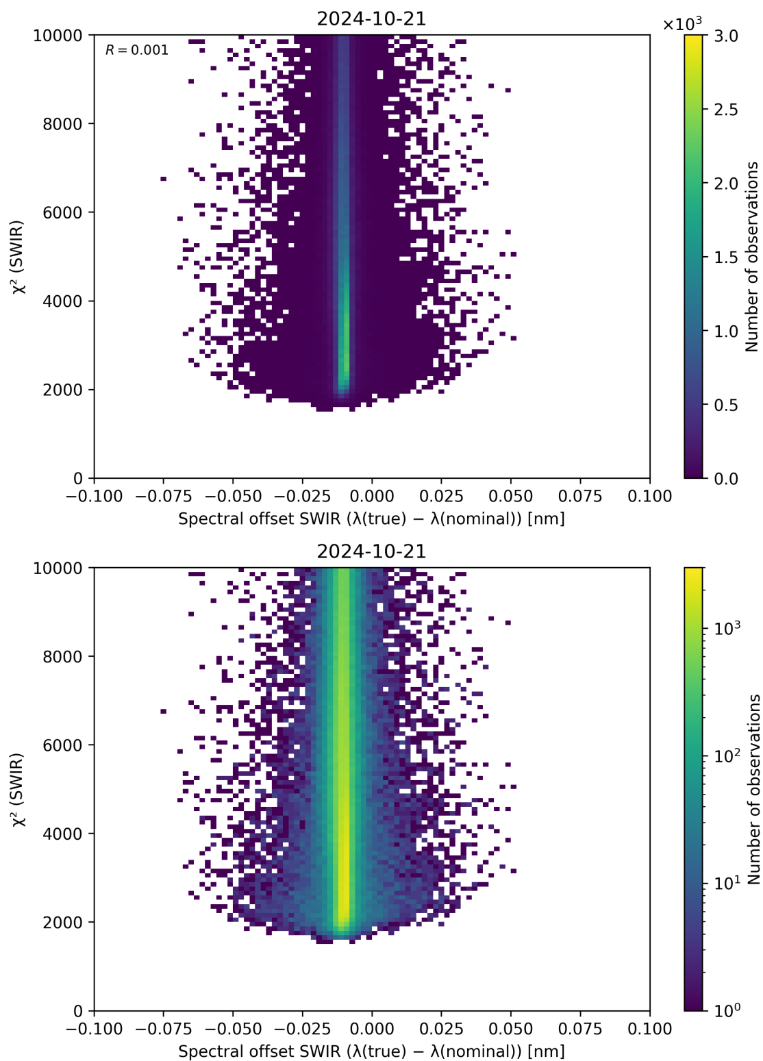
Figure 118: Scatter density plot of “Spectral offset SWIR ( \lambda_{\text{true}} - \lambda_{\text{nominal}} )” against “ \chi^2 (SWIR)” for 2024-10-20 to 2024-10-22.
