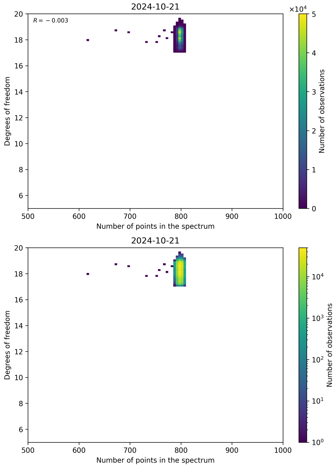
Figure 90: Scatter density plot of “Number of points in the spectrum” against “Degrees of freedom” for 2024-10-20 to 2024-10-22.
