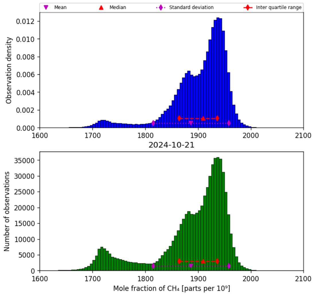
Figure 23: Histogram of “Mole fraction of CH 4 ” for 2024-10-20 to 2024-10-22
