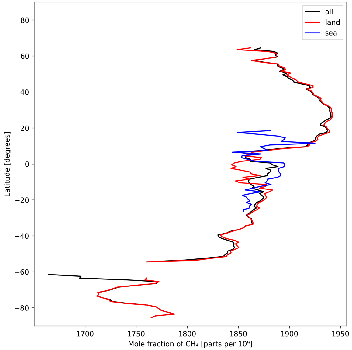
Figure 12: Zonal average of “Mole fraction of CH 4 ” for 2024-10-20 to 2024-10-22.
