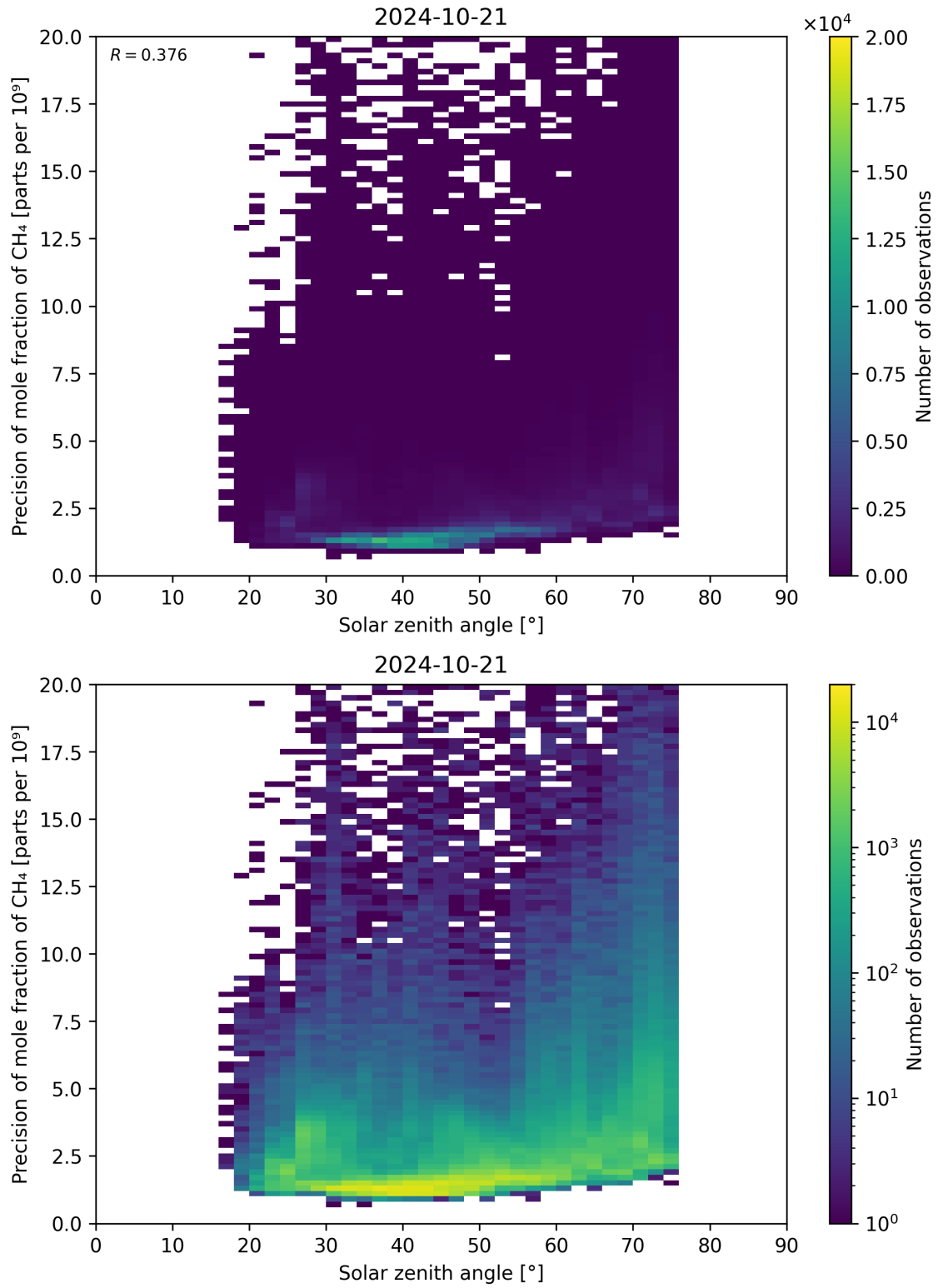
Figure 101: Scatter density plot of “Solar zenith angle” against “Precision of mole fraction of CH 4 ” for 2024-10-20 to 2024-10-22.
