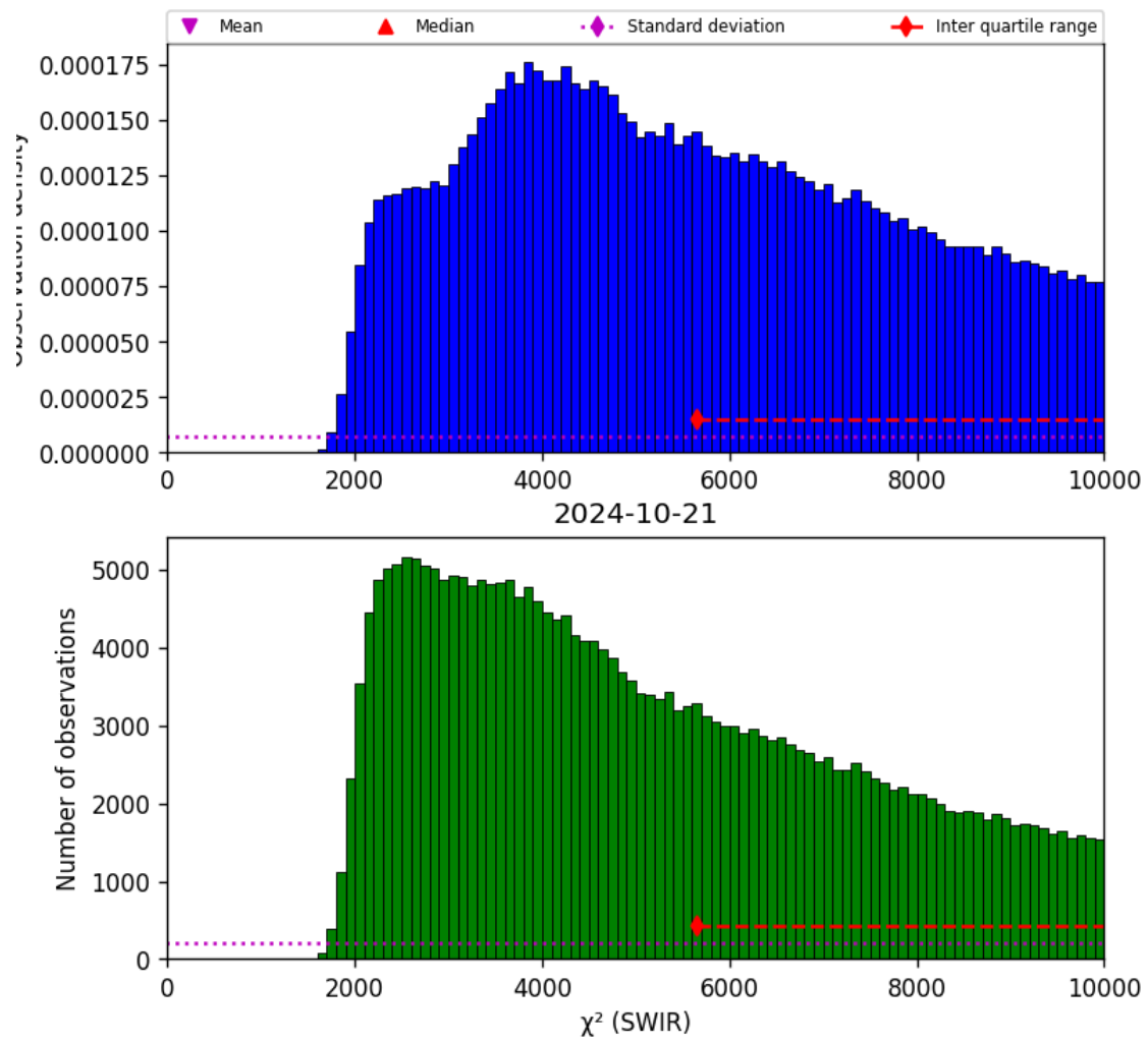
Figure 28: Histogram of “ \chi^2 (SWIR)” for 2024-10-20 to 2024-10-22
