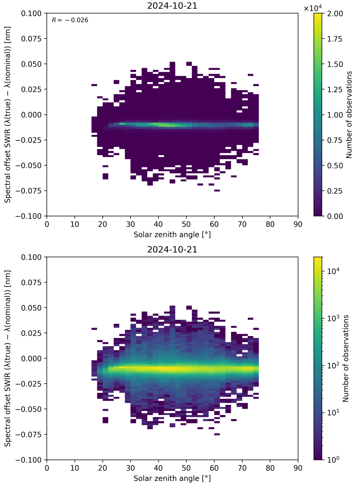
Figure 104: Scatter density plot of “Solar zenith angle” against “Spectral offset SWIR ( \lambda_{\text{true}} - \lambda_{\text{nominal}} )” for 2024-10-20 to 2024-10-22.
