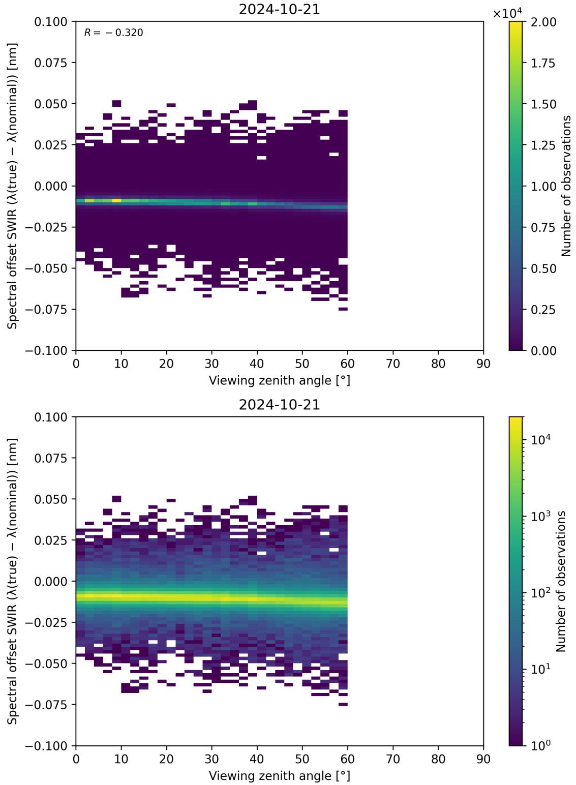
Figure 116: Scatter density plot of “Viewing zenith angle” against “Spectral offset SWIR ( \lambda_{\text{true}} - \lambda_{\text{nominal}} )” for 2024-10-20 to 2024-10-22.
