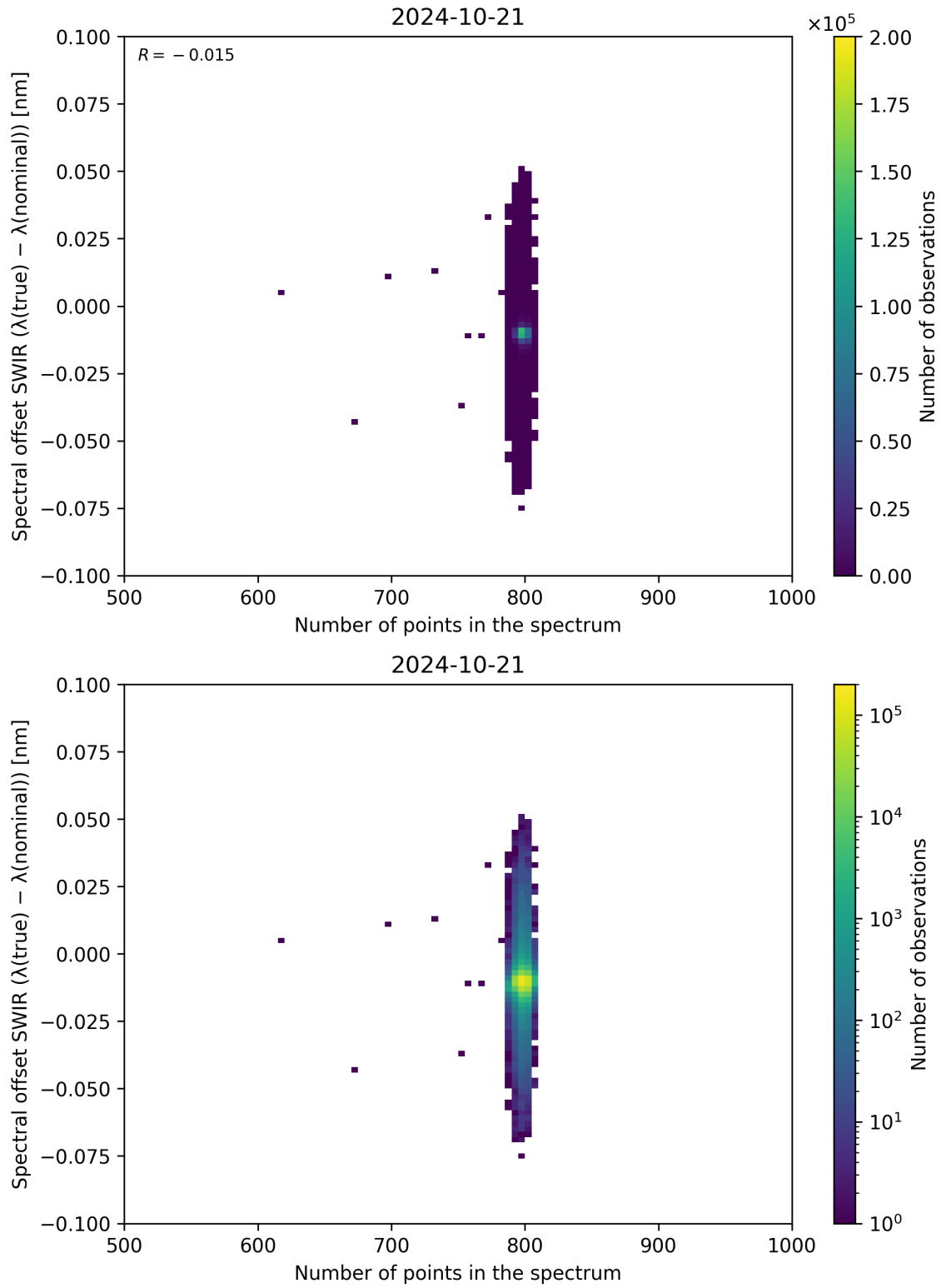
Figure 93: Scatter density plot of “Number of points in the spectrum” against “Spectral offset SWIR ( \lambda_{\text{true}} - \lambda_{\text{nominal}} )” for 2024-10-20 to 2024-10-22.
