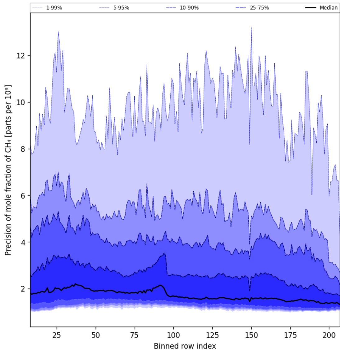
Figure 35: Along track statistics of “Precision of mole fraction of CH 4 ” for 2024-10-20 to 2024-10-22
