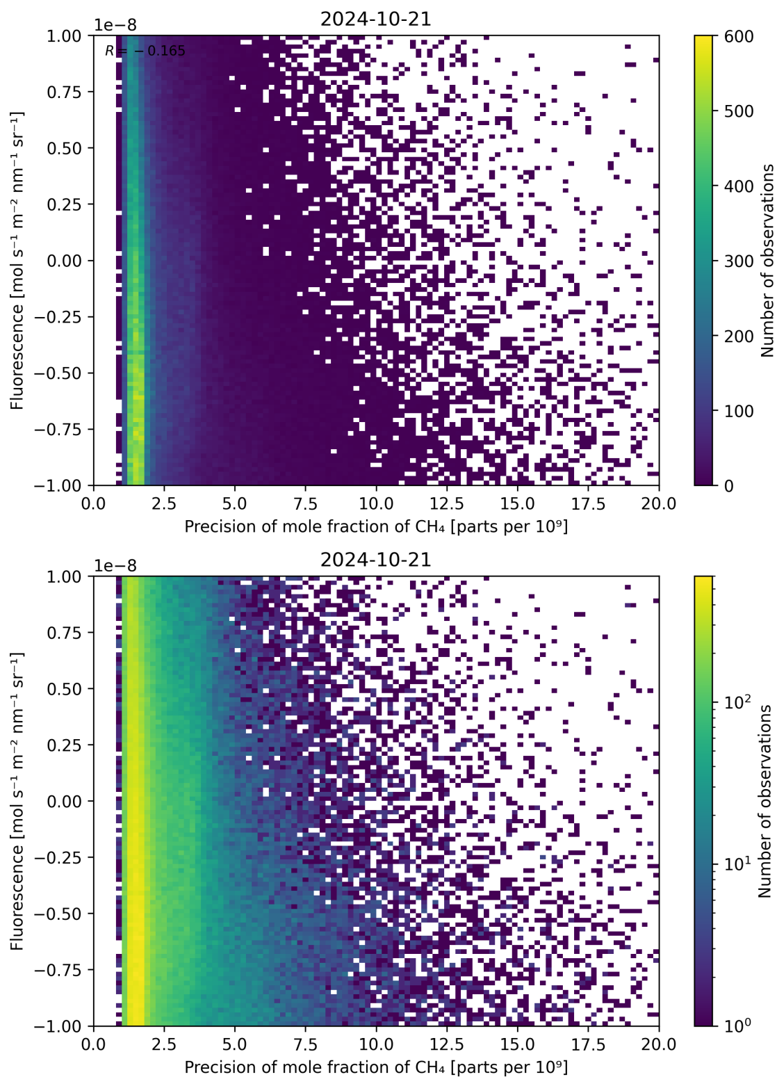
Figure 81: Scatter density plot of “Precision of mole fraction of \text{CH}_4 ” against “Fluorescence” for 2024-10-20 to 2024-10-22.
