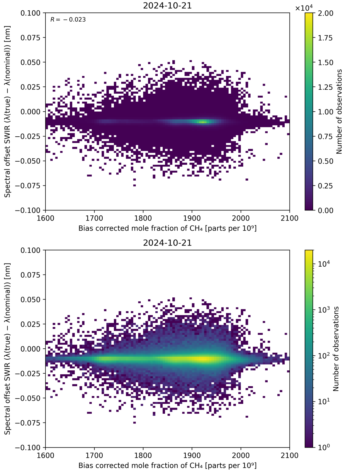
Figure 69: Scatter density plot of “Bias corrected mole fraction of \text{CH}_4 ” against “Spectral offset SWIR ( \lambda_{\text{true}} - \lambda_{\text{nominal}} )” for 2024-10-20 to 2024-10-22.
