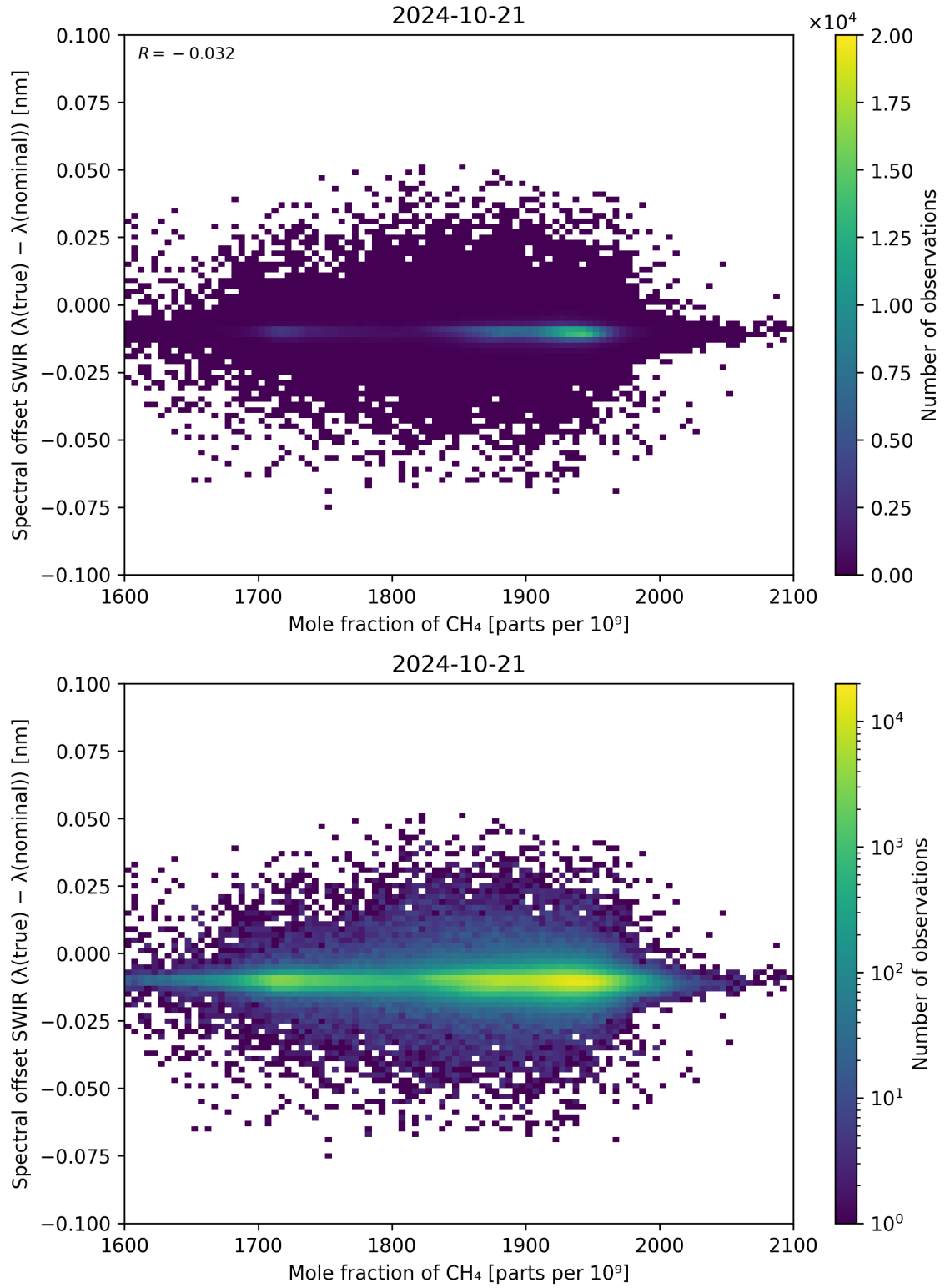
Figure 86: Scatter density plot of “Mole fraction of \text{CH}_4 ” against “Spectral offset SWIR ( \lambda_{\text{true}} - \lambda_{\text{nominal}} )” for 2024-10-20 to 2024-10-22.
