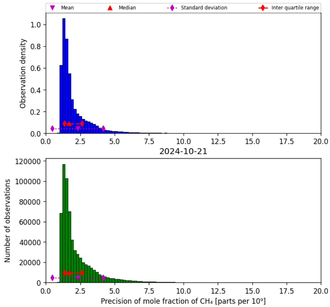
Figure 24: Histogram of “Precision of mole fraction of CH 4 ” for 2024-10-20 to 2024-10-22
