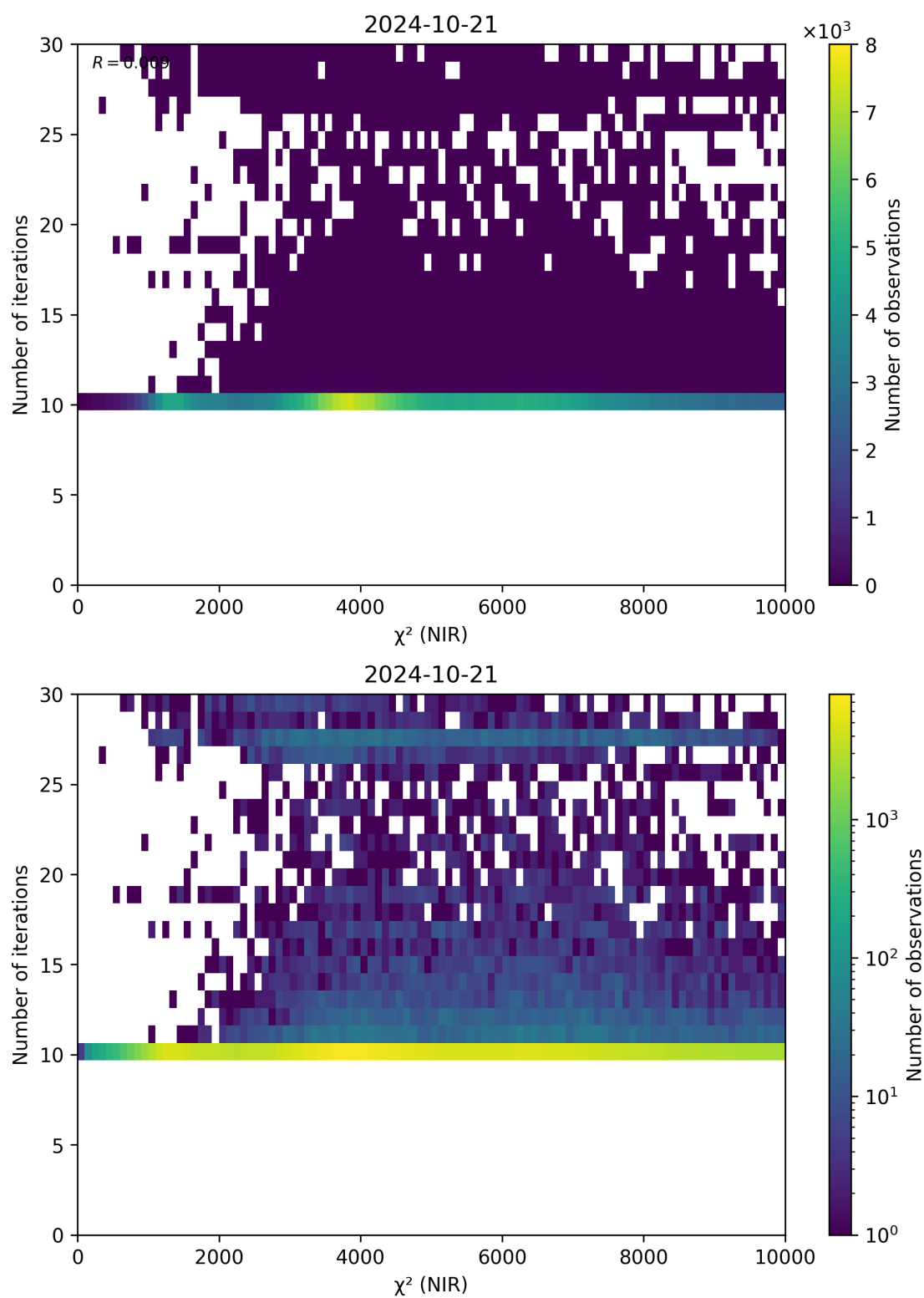
Figure 46: Scatter density plot of “ \chi^2 (NIR)” against “Number of iterations” for 2024-10-20 to 2024-10-22.
