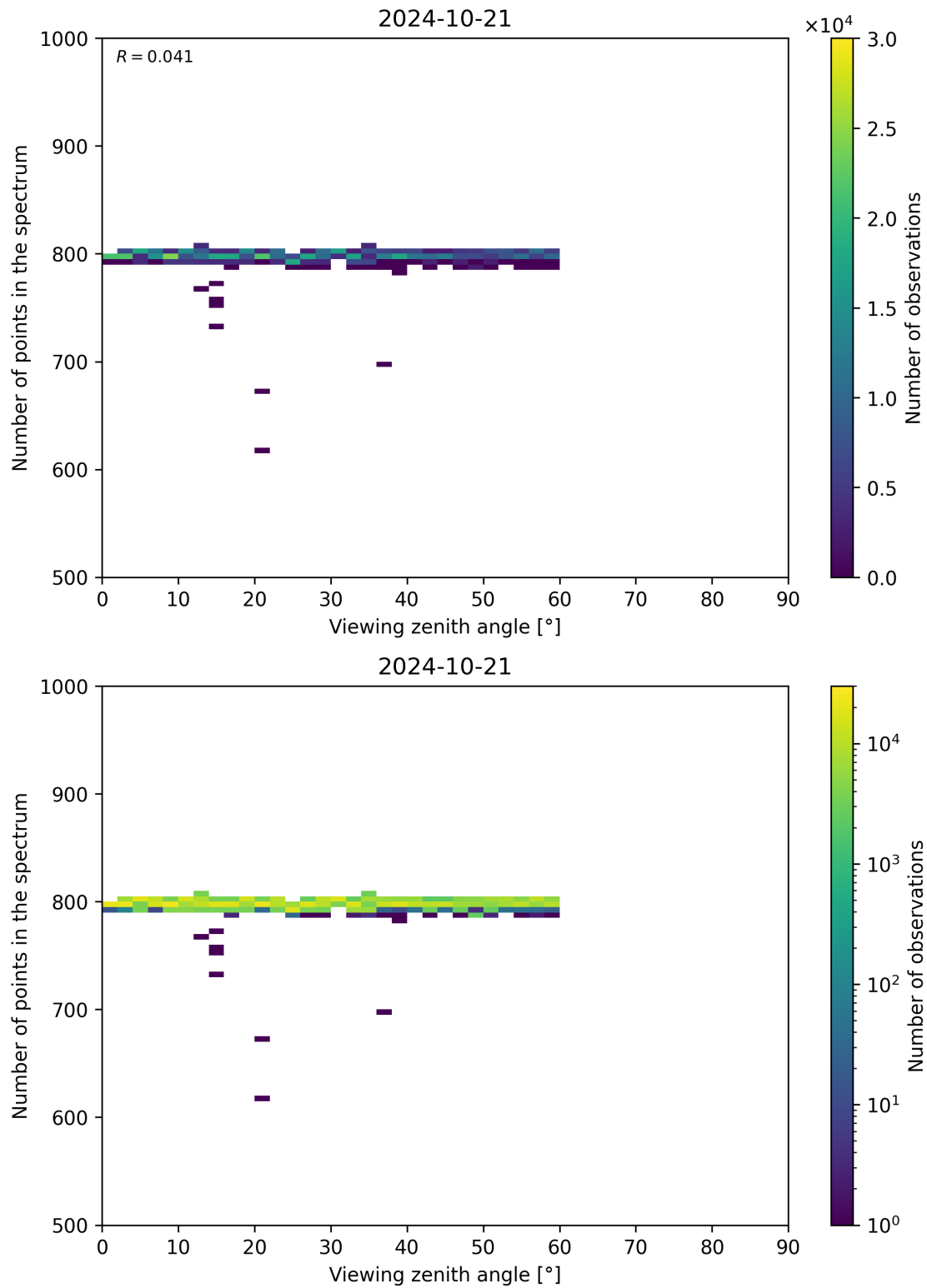
Figure 114: Scatter density plot of “Viewing zenith angle” against “Number of points in the spectrum” for 2024-10-20 to 2024-10-22.
