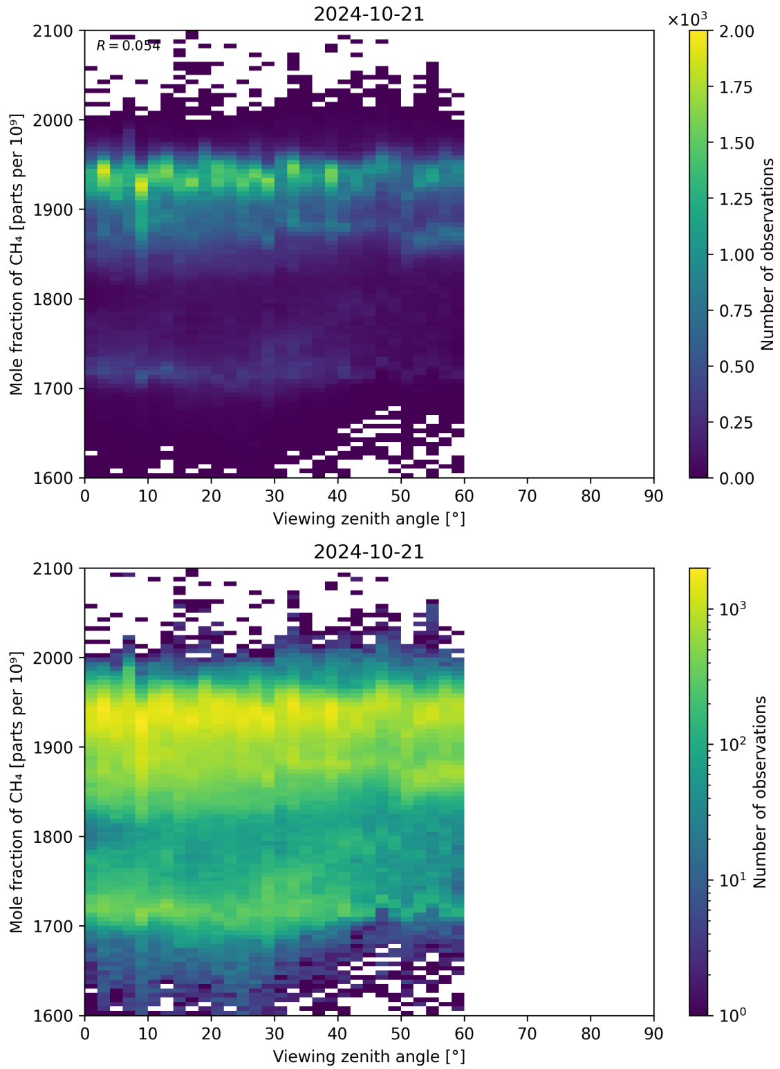
Figure 110: Scatter density plot of “Viewing zenith angle” against “Mole fraction of CH 4 ” for 2024-10-20 to 2024-10-22.
