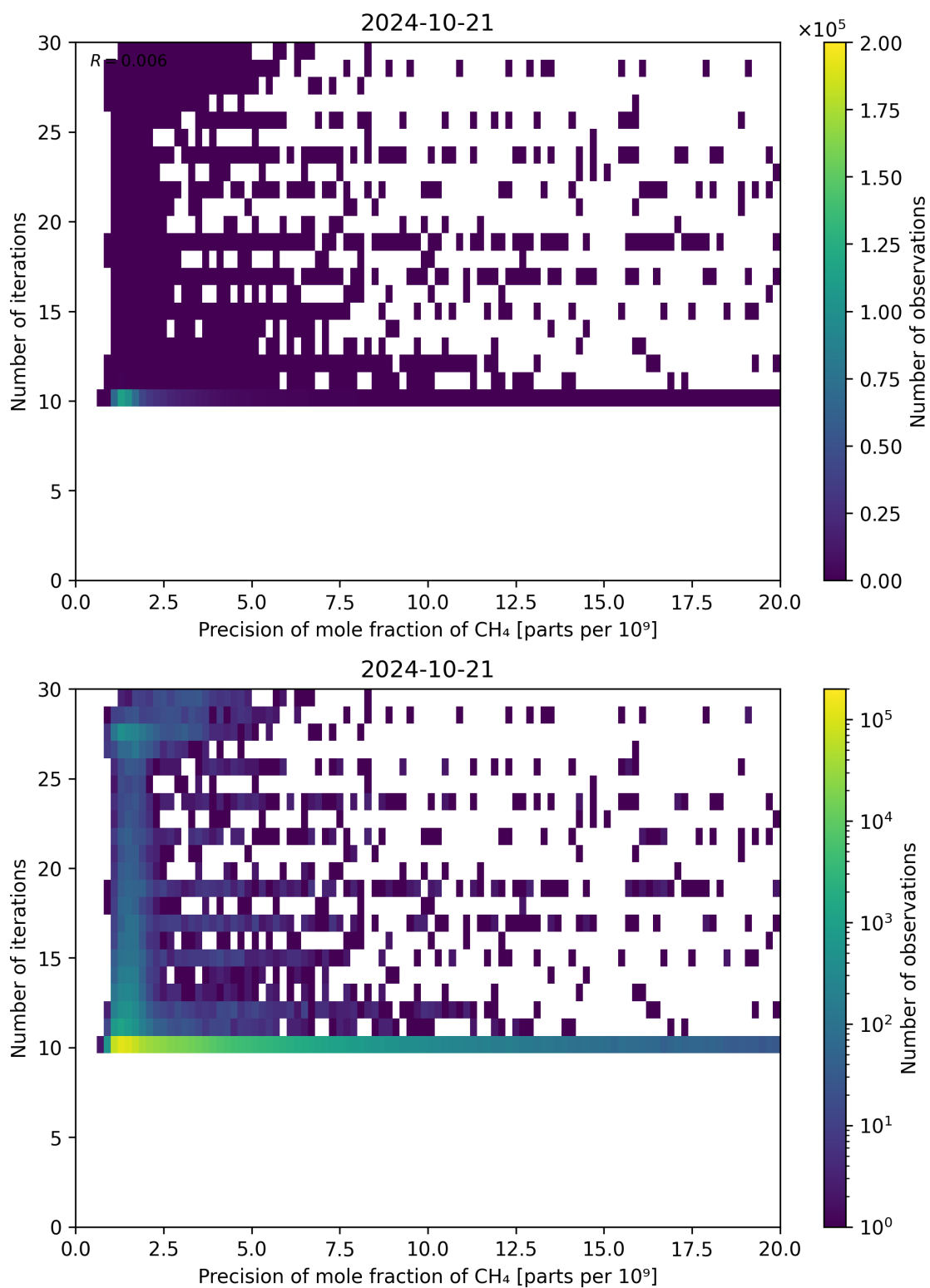
Figure 83: Scatter density plot of “Precision of mole fraction of CH 4 ” against “Number of iterations” for 2024-10-20 to 2024-10-22.
