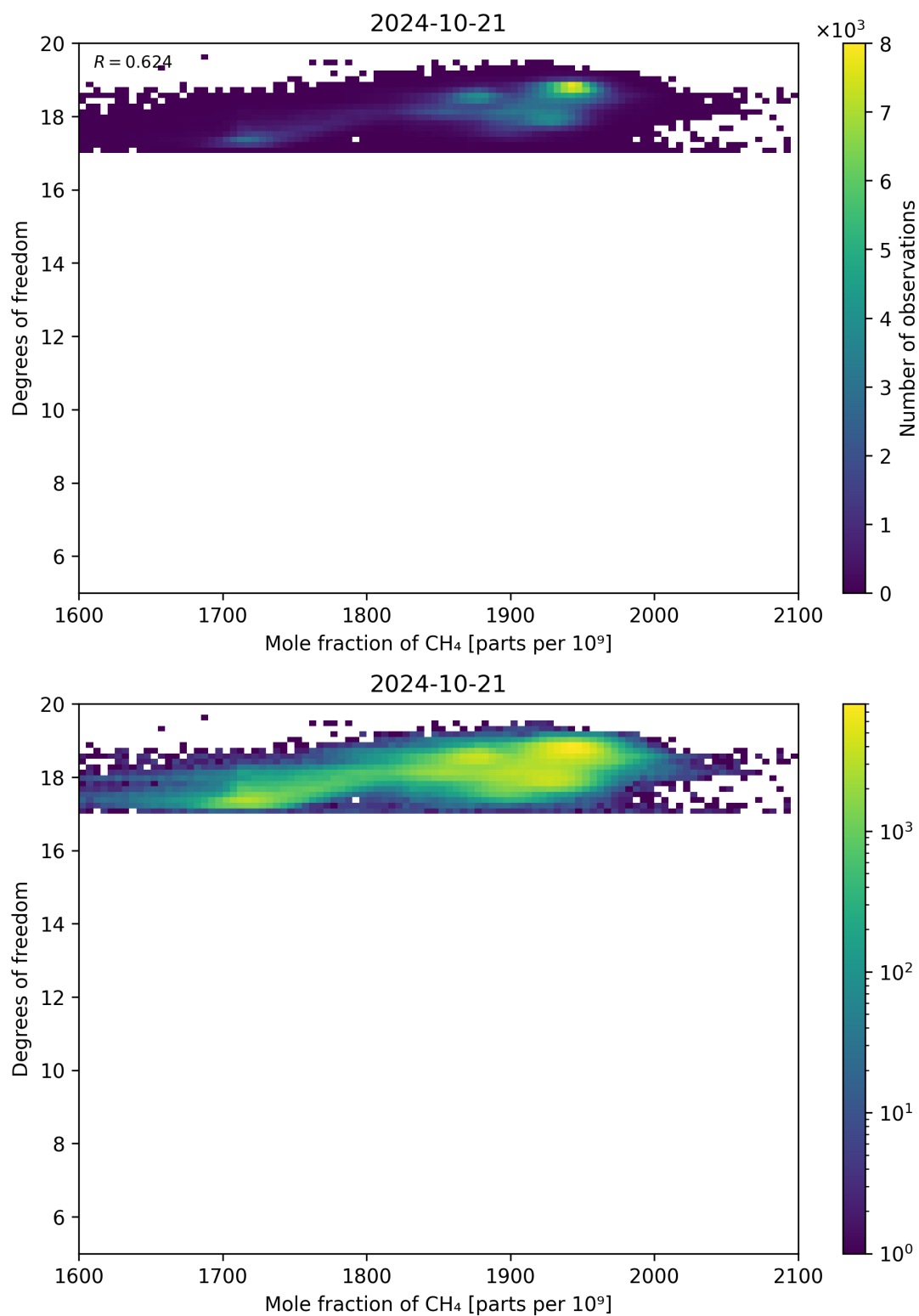
Figure 72: Scatter density plot of “Mole fraction of CH 4 ” against “Degrees of freedom” for 2024-10-20 to 2024-10-22.
