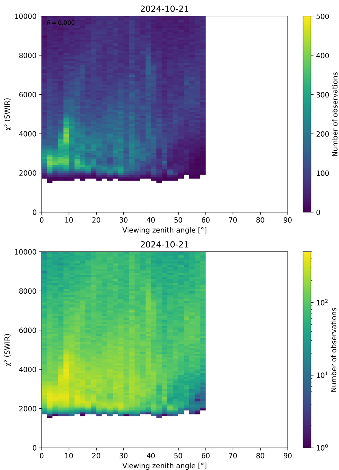
Figure 106: Scatter density plot of “Viewing zenith angle” against “ \chi^2 (SWIR)” for 2024-10-20 to 2024-10-22.
