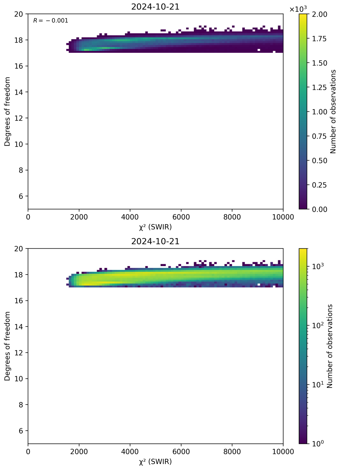
Figure 48: Scatter density plot of “ \chi^2 (SWIR)” against “Degrees of freedom” for 2024-10-20 to 2024-10-22.
