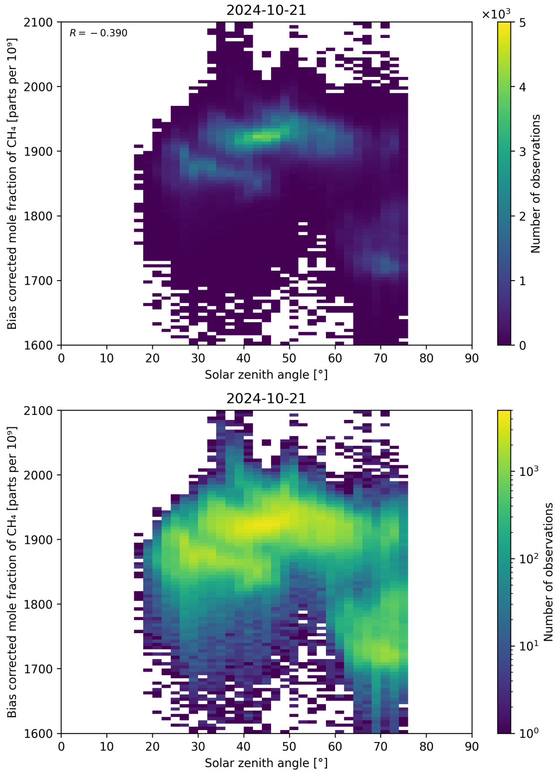
Figure 100: Scatter density plot of “Solar zenith angle” against “Bias corrected mole fraction of \text{CH}_4 ” for 2024-10-20 to 2024-10-22.
