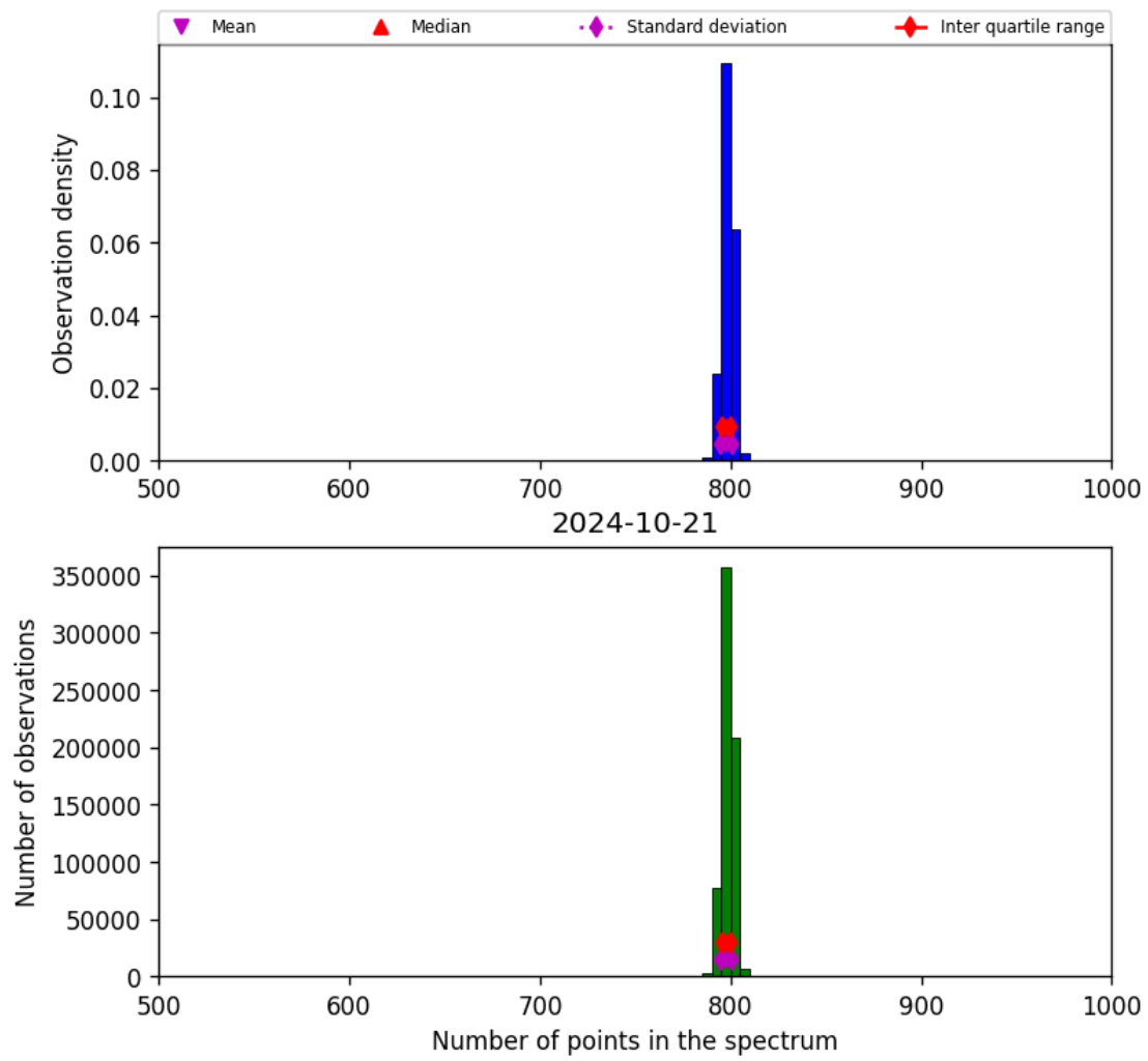
Figure 26: Histogram of “Number of points in the spectrum” for 2024-10-20 to 2024-10-22
