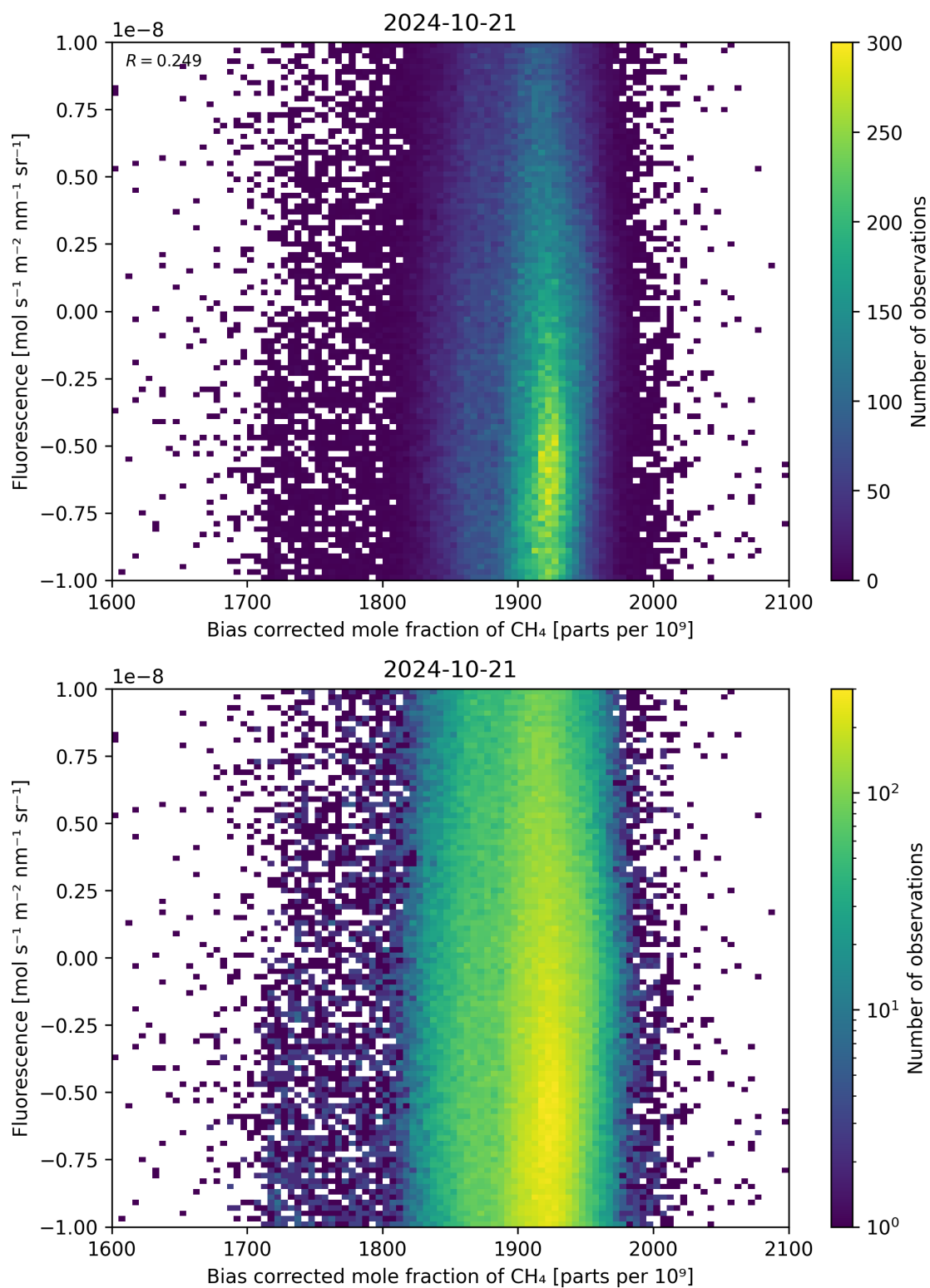
Figure 66: Scatter density plot of “Bias corrected mole fraction of \text{CH}_4 ” against “Fluorescence” for 2024-10-20 to 2024-10-22.
