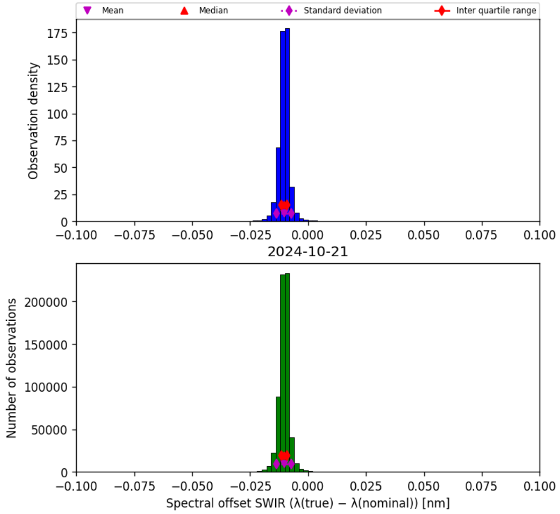
Figure 27: Histogram of “Spectral offset SWIR ( \lambda_{\text{true}} - \lambda_{\text{nominal}} )” for 2024-10-20 to 2024-10-22
