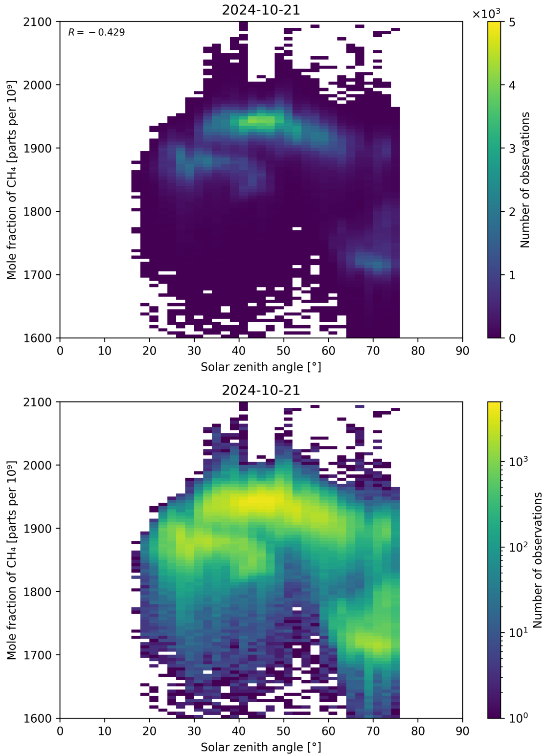
Figure 99: Scatter density plot of “Solar zenith angle” against “Mole fraction of CH 4 ” for 2024-10-20 to 2024-10-22.
