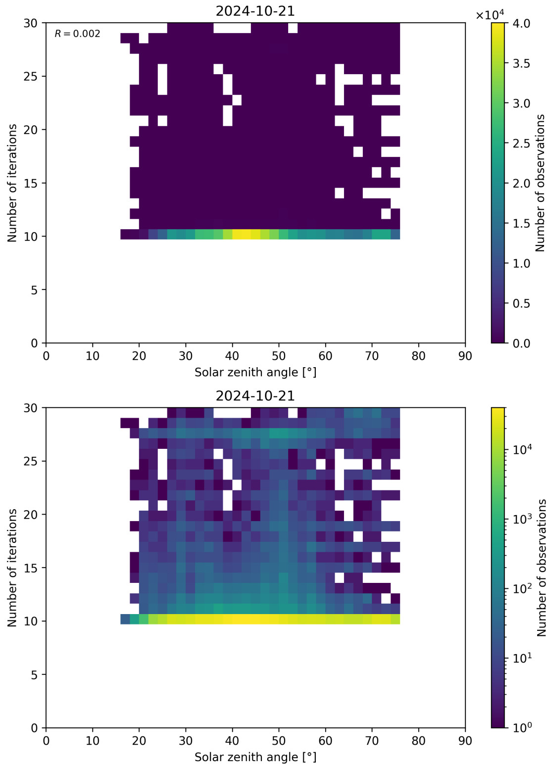
Figure 102: Scatter density plot of “Solar zenith angle” against “Number of iterations” for 2024-10-20 to 2024-10-22.
