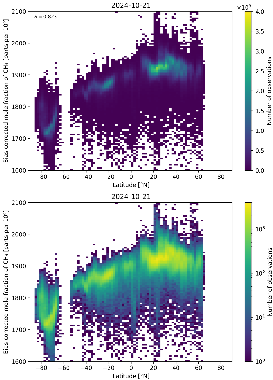
Figure 58: Scatter density plot of “Latitude” against “Bias corrected mole fraction of \text{CH}_4 ” for 2024-10-20 to 2024-10-22.
