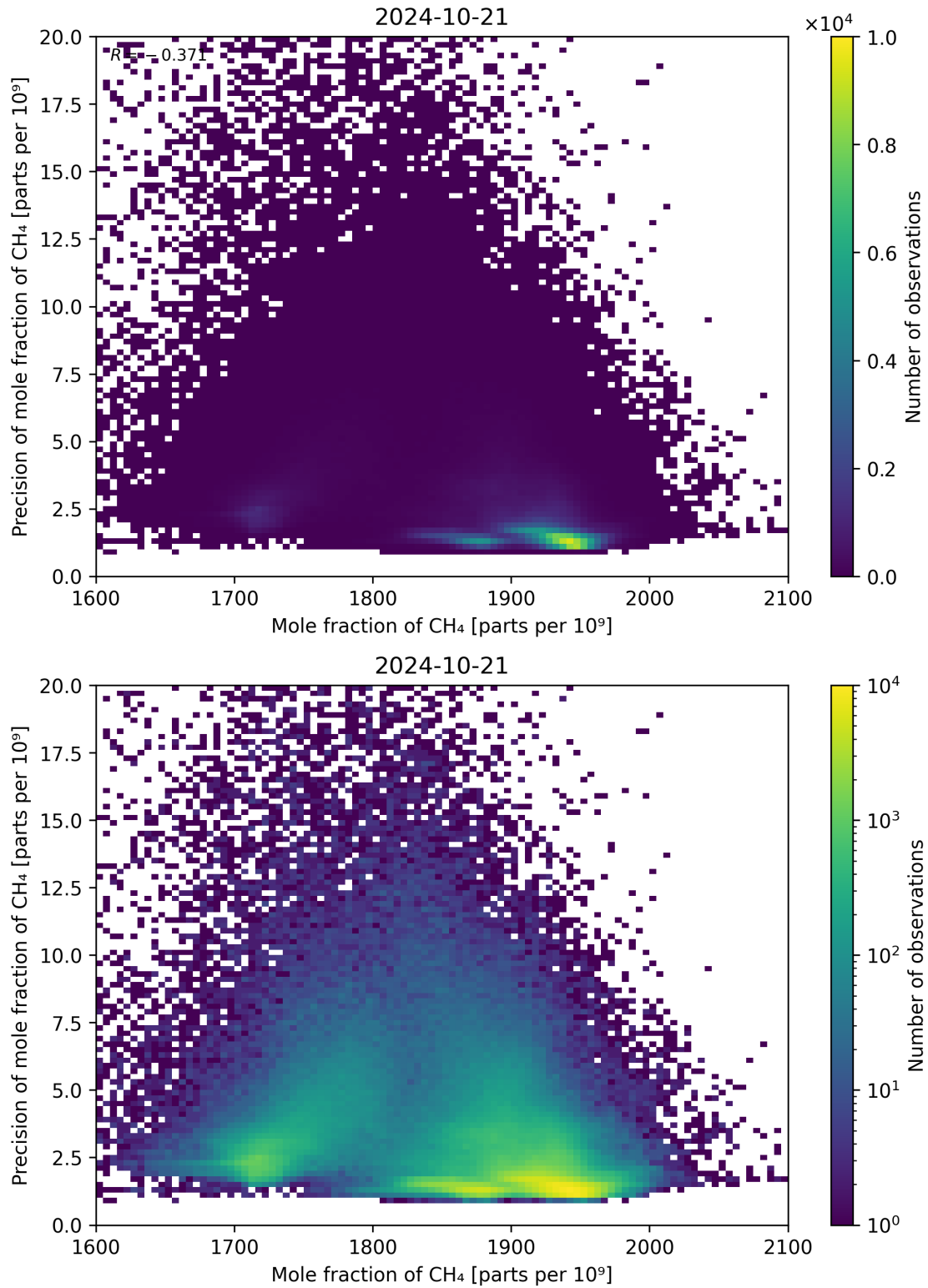
Figure 75: Scatter density plot of “Mole fraction of CH 4 ” against “Precision of mole fraction of CH 4 ” for 2024-10-20 to 2024-10-22.
