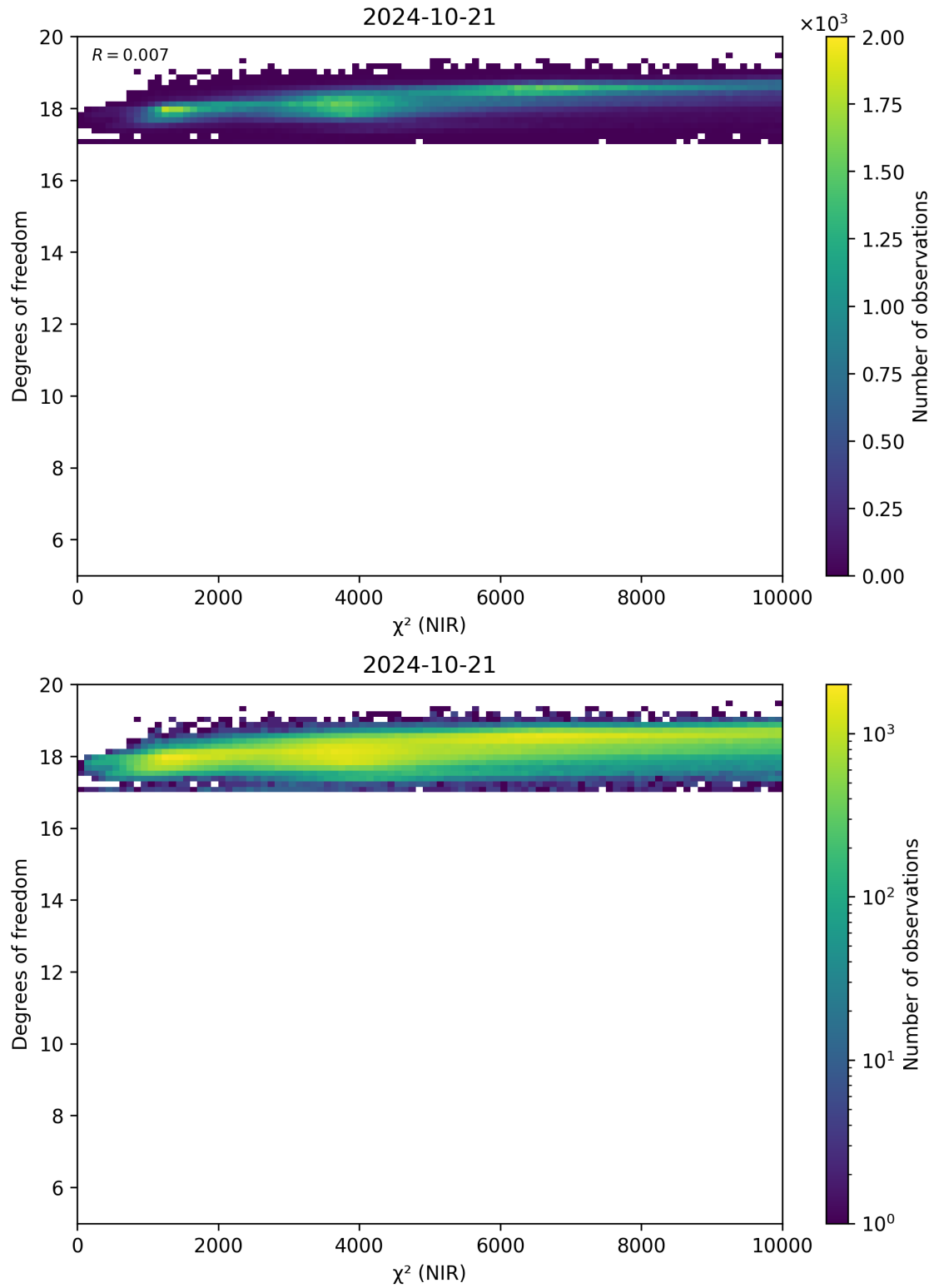
Figure 44: Scatter density plot of “ \chi^2 (NIR)” against “Degrees of freedom” for 2024-10-20 to 2024-10-22.
