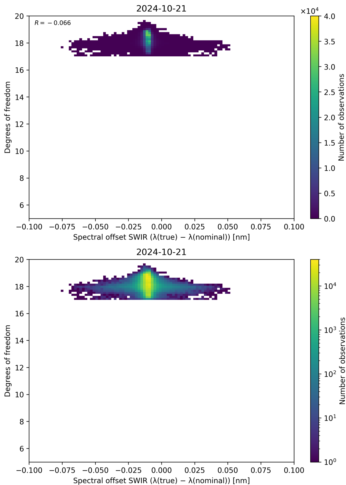
Figure 119: Scatter density plot of “Spectral offset SWIR ( \lambda_{\text{true}} - \lambda_{\text{nominal}} )” against “Degrees of freedom” for 2024-10-20 to 2024-10-22.
