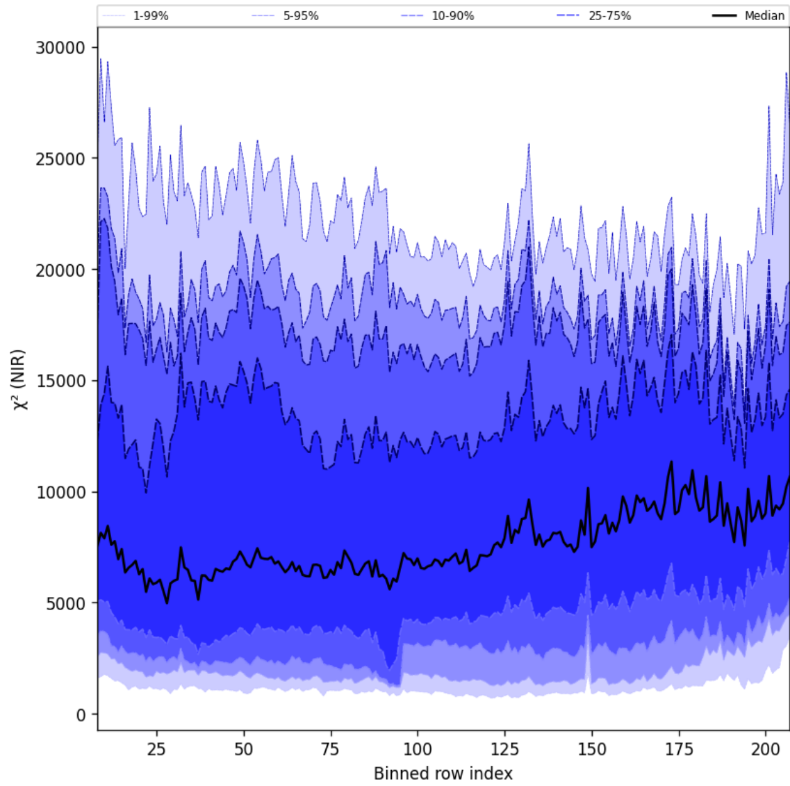
Figure 40: Along track statistics of “ \chi^2 (NIR)” for 2024-10-20 to 2024-10-22
