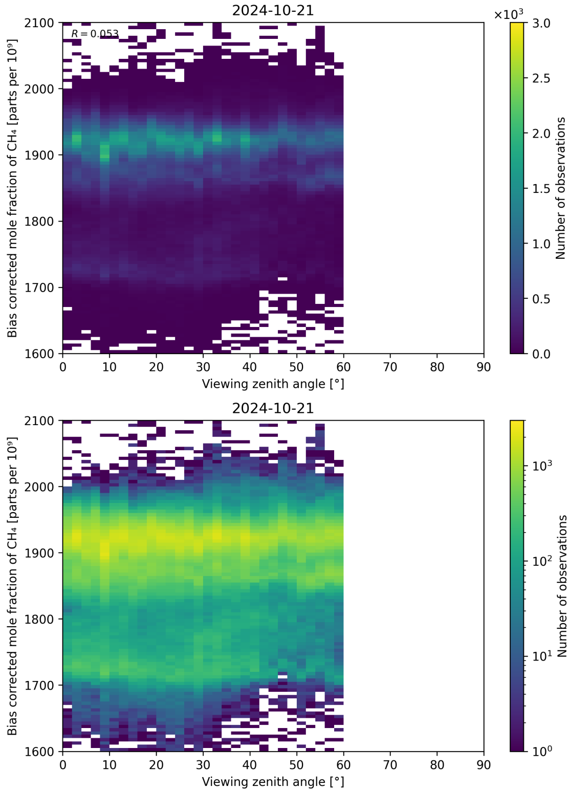
Figure 111: Scatter density plot of “Viewing zenith angle” against “Bias corrected mole fraction of CH 4 ” for 2024-10-20 to 2024-10-22.
