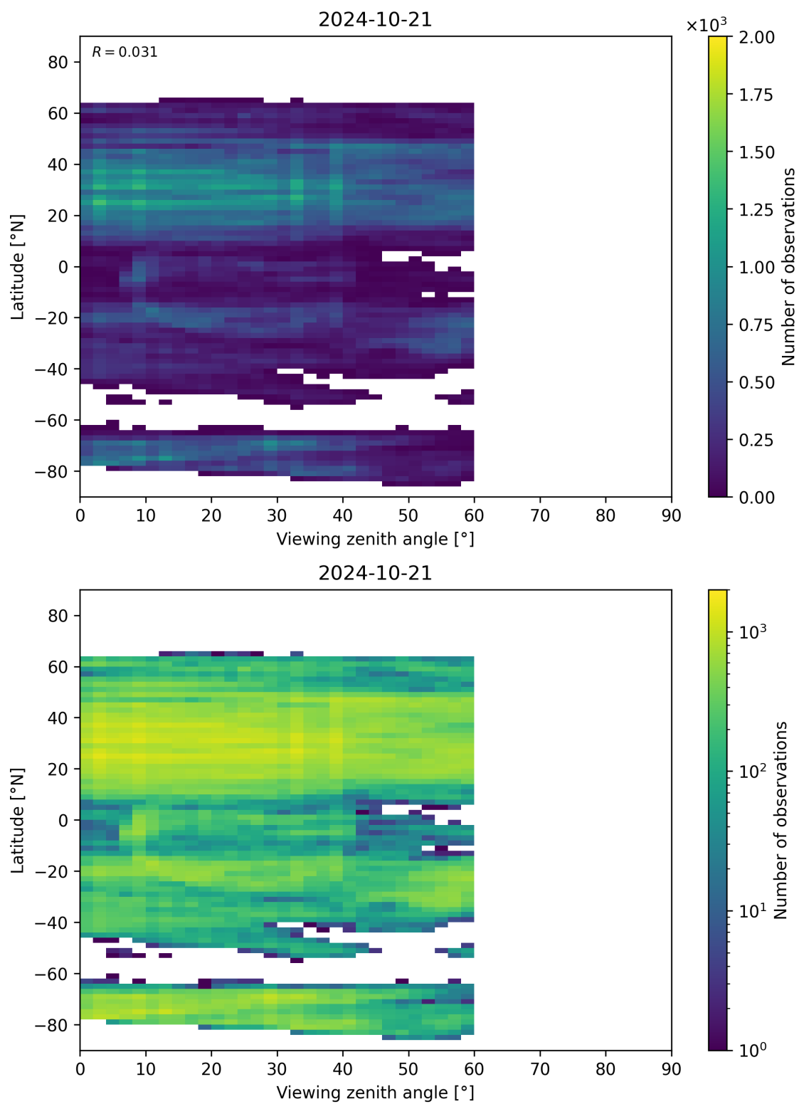
Figure 109: Scatter density plot of “Viewing zenith angle” against “Latitude” for 2024-10-20 to 2024-10-22.
