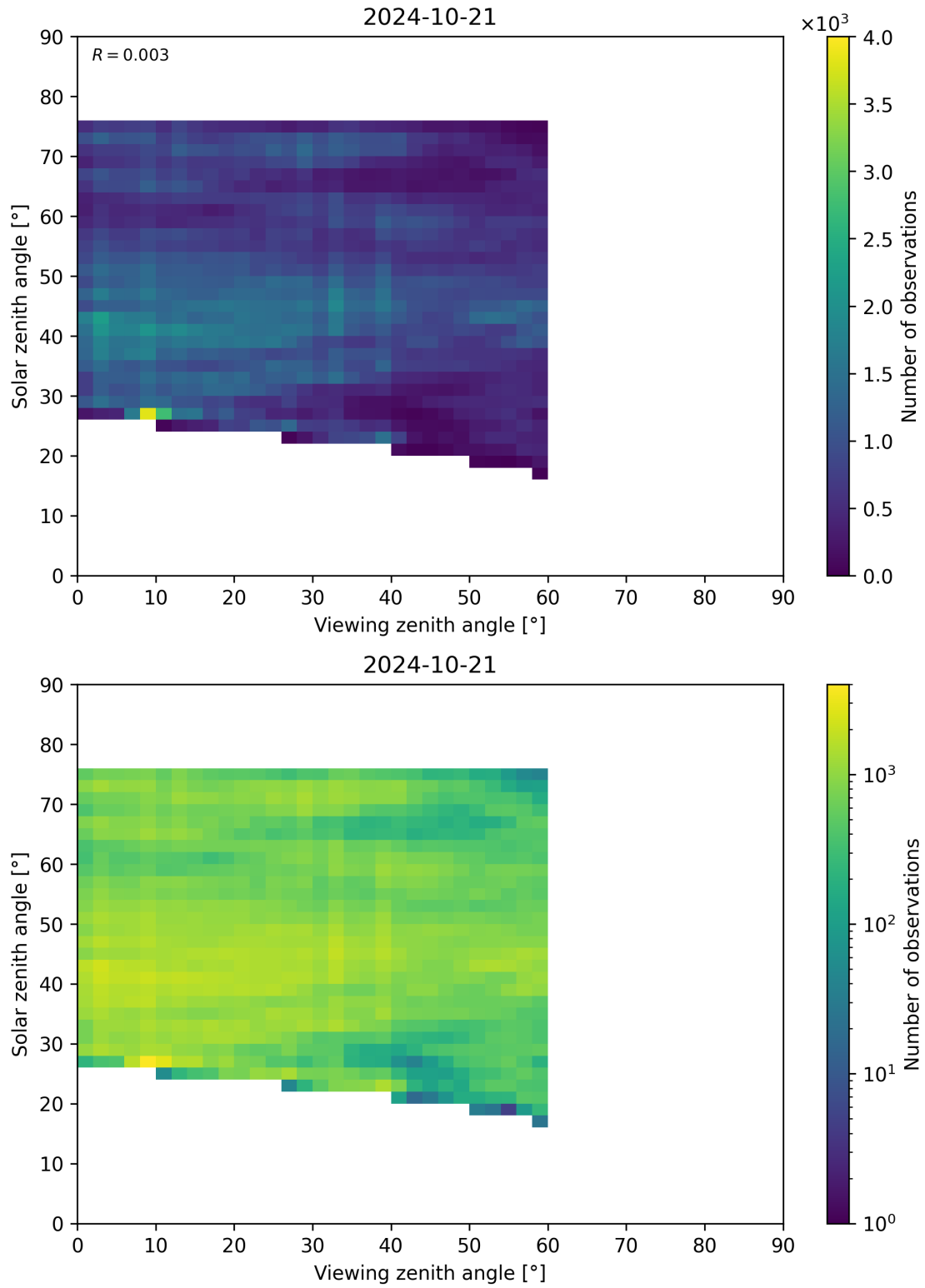
Figure 115: Scatter density plot of “Viewing zenith angle” against “Solar zenith angle” for 2024-10-20 to 2024-10-22.
