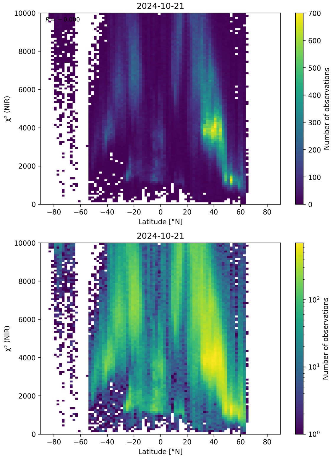
Figure 53: Scatter density plot of “Latitude” against “ \chi^2 (NIR)” for 2024-10-20 to 2024-10-22.
