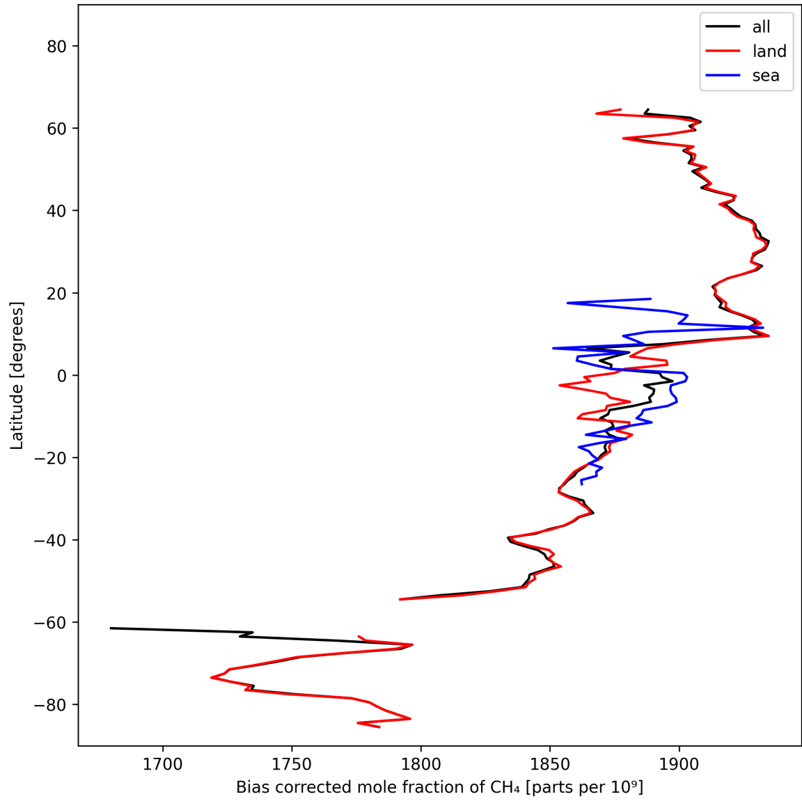
Figure 14: Zonal average of “Bias corrected mole fraction of CH 4 ” for 2024-10-20 to 2024-10-22.
