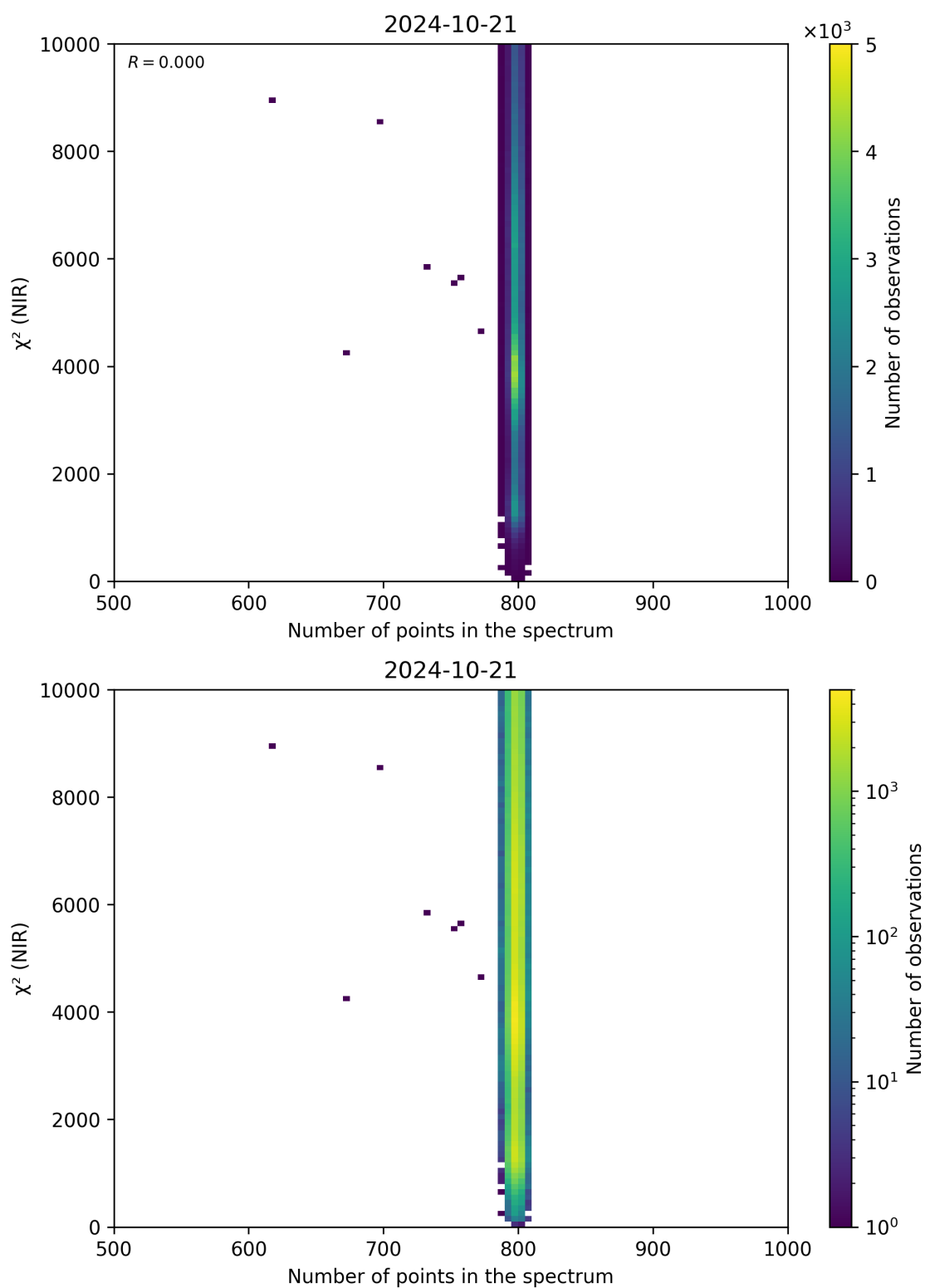
Figure 88: Scatter density plot of “Number of points in the spectrum” against “ \chi^2 (NIR)” for 2024-10-20 to 2024-10-22.
