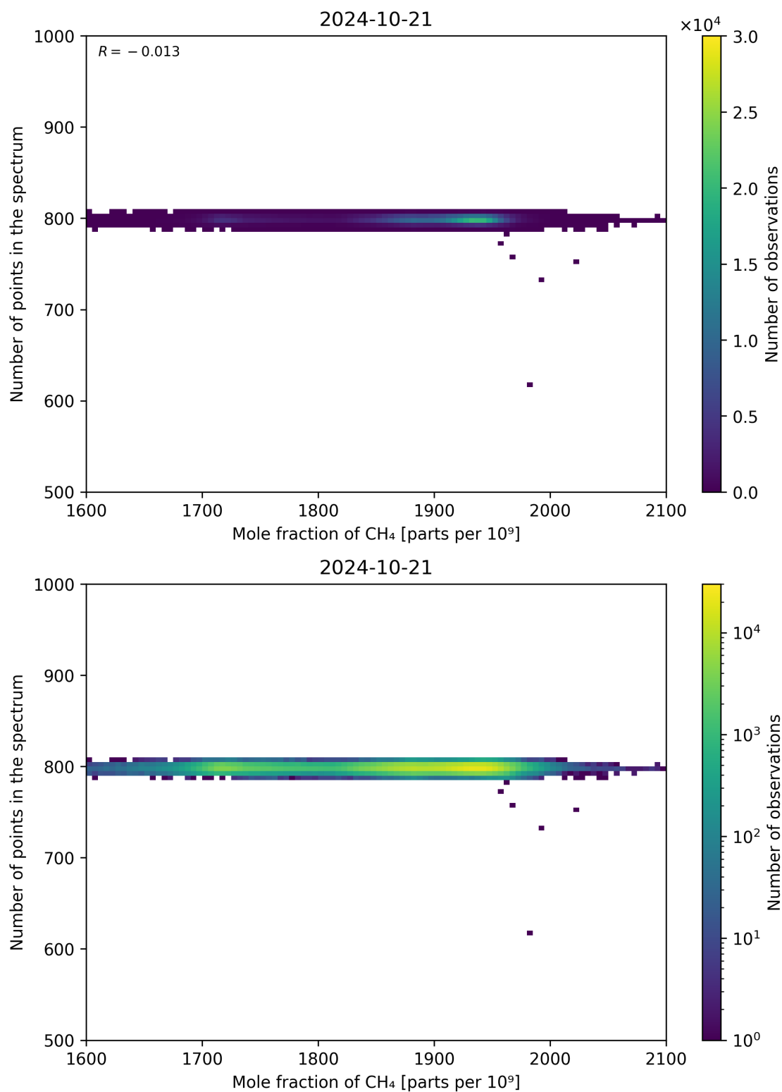
Figure 77: Scatter density plot of “Mole fraction of CH 4 ” against “Number of points in the spectrum” for 2024-10-20 to 2024-10-22.
