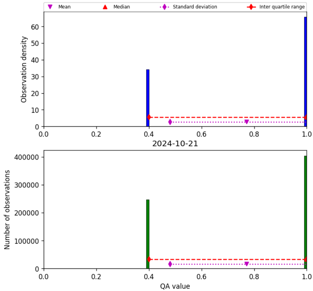
Figure 22: Histogram of “QA value” for 2024-10-20 to 2024-10-22
