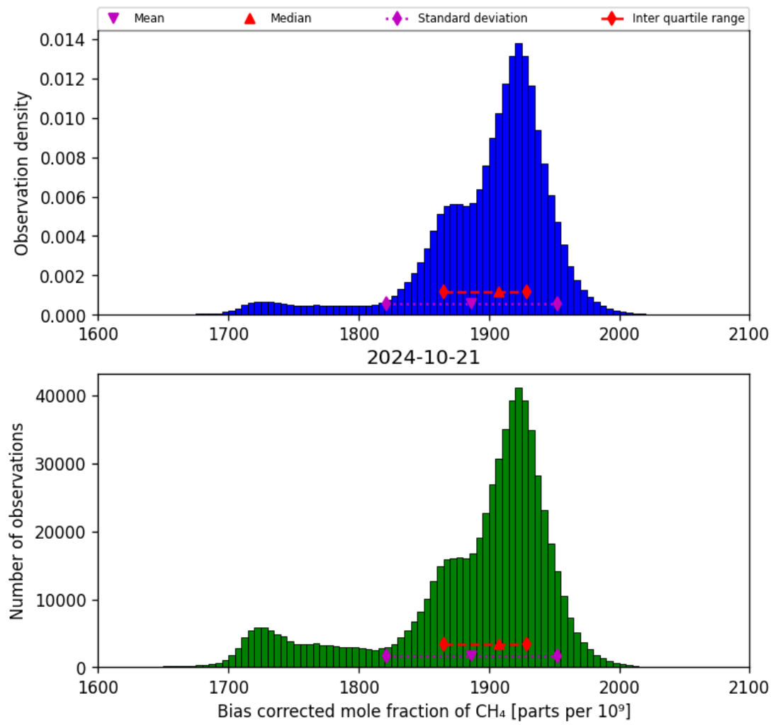
Figure 25: Histogram of “Bias corrected mole fraction of CH 4 ” for 2024-10-20 to 2024-10-22
