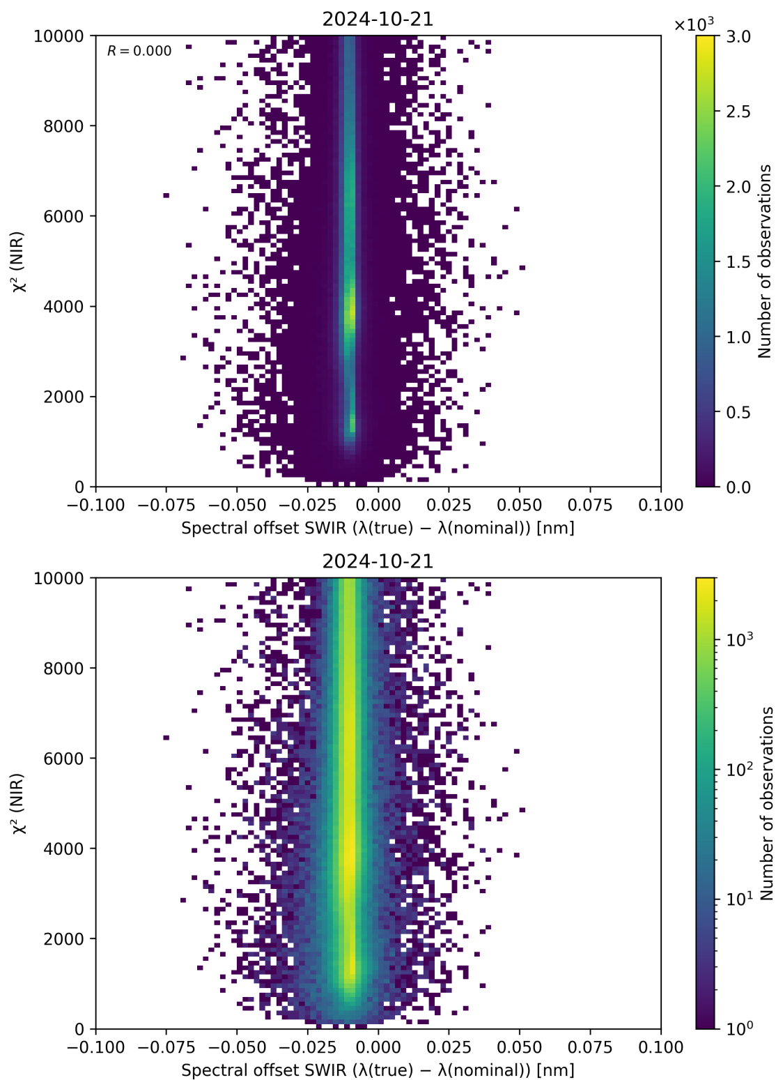
Figure 117: Scatter density plot of “Spectral offset SWIR ( \lambda_{\text{true}} - \lambda_{\text{nominal}} )” against “ \chi^2 (NIR)” for 2024-10-20 to 2024-10-22.
