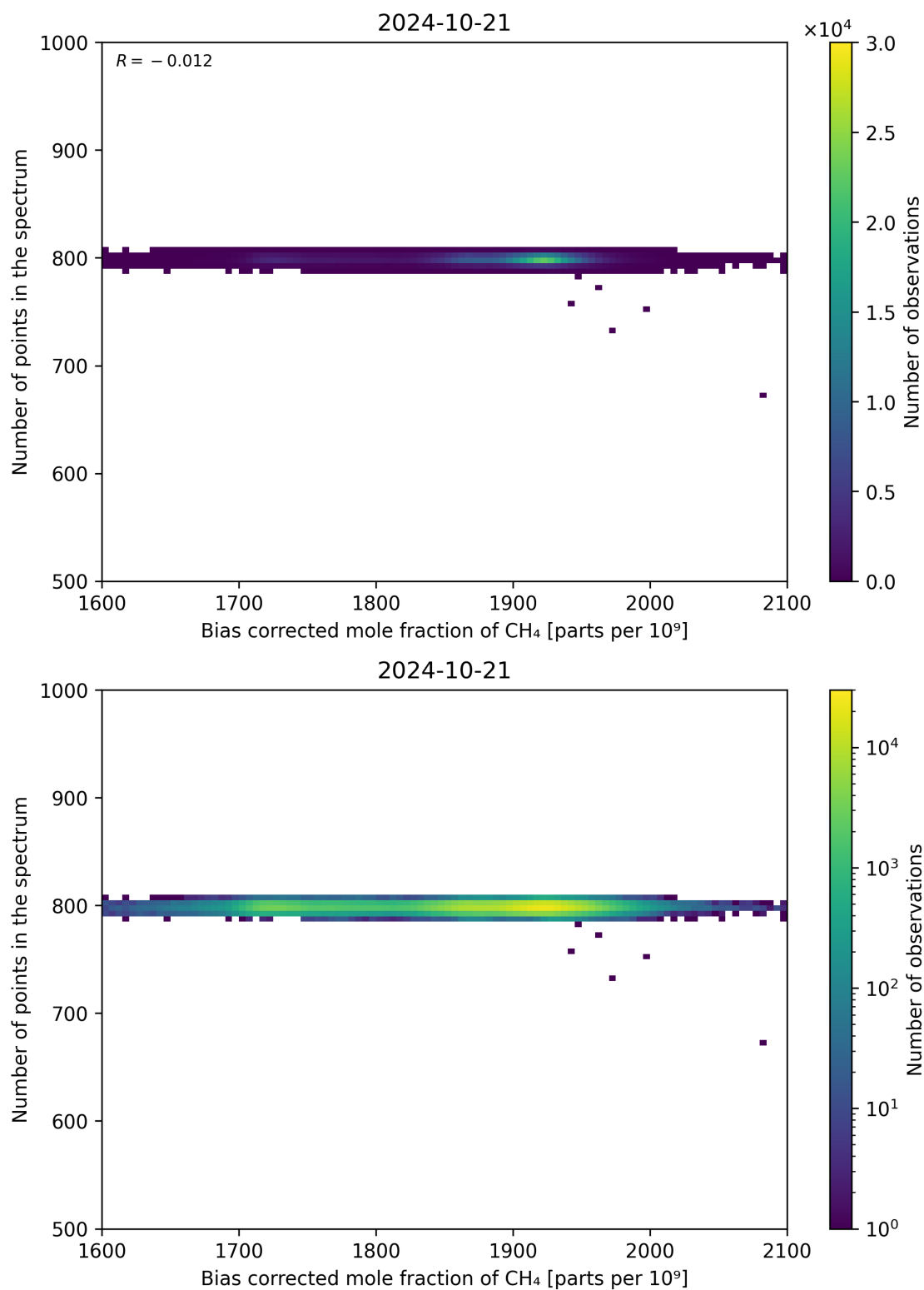
Figure 68: Scatter density plot of “Bias corrected mole fraction of CH 4 ” against “Number of points in the spectrum” for 2024-10-20 to 2024-10-22.
