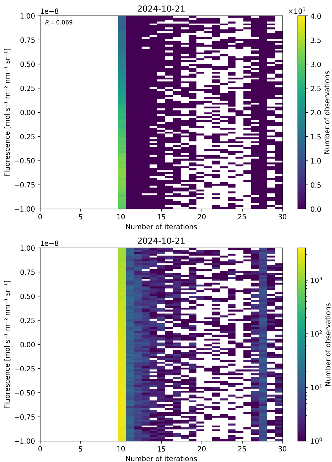
Figure 87: Scatter density plot of “Number of iterations” against “Fluorescence” for 2024-10-20 to 2024-10-22.
