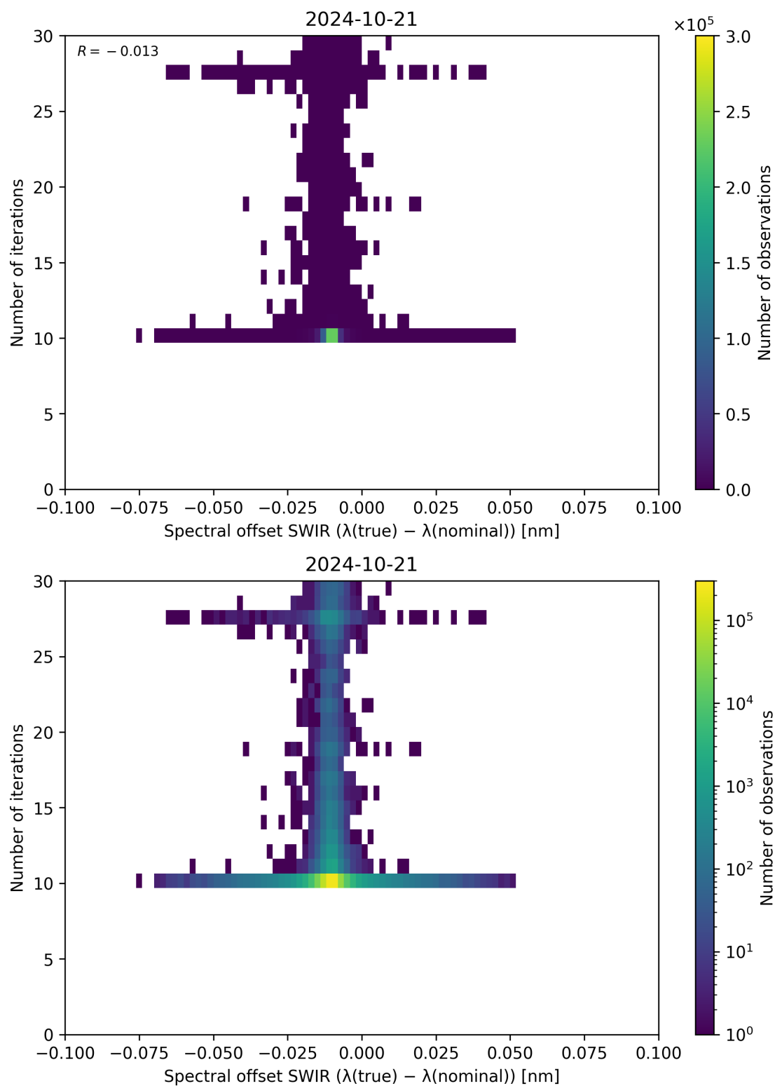
Figure 121: Scatter density plot of “Spectral offset SWIR ( \lambda_{\text{true}} - \lambda_{\text{nominal}} )” against “Number of iterations” for 2024-10-20 to 2024-10-22.
