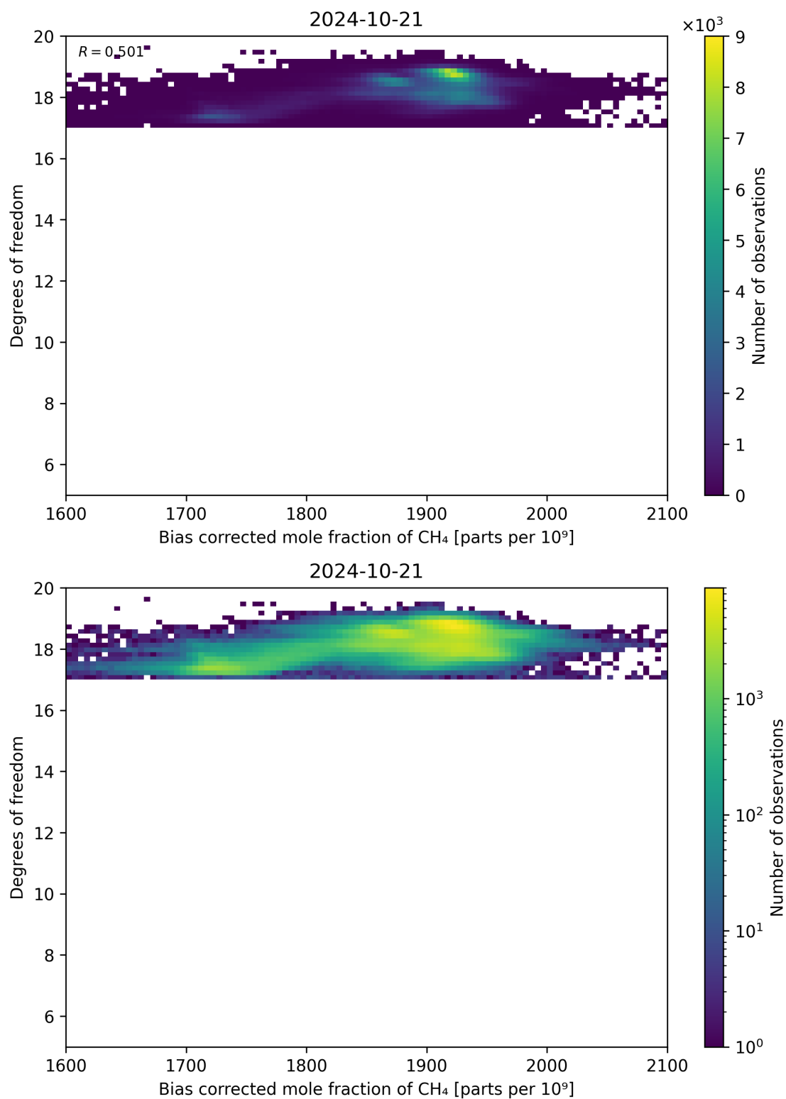
Figure 65: Scatter density plot of “Bias corrected mole fraction of CH 4 ” against “Degrees of freedom” for 2024-10-20 to 2024-10-22.
