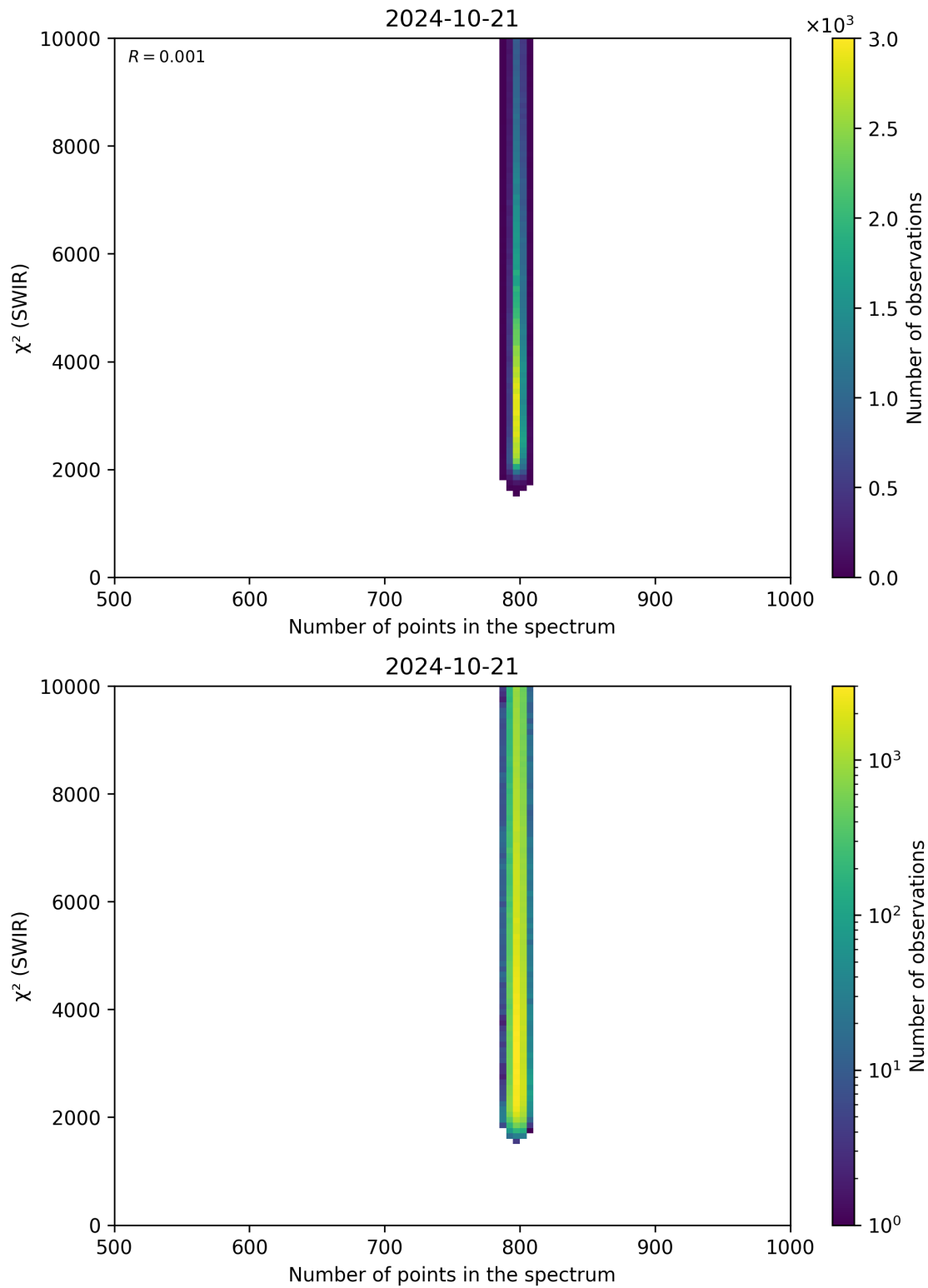
Figure 89: Scatter density plot of “Number of points in the spectrum” against “ \chi^2 (SWIR)” for 2024-10-20 to 2024-10-22.
