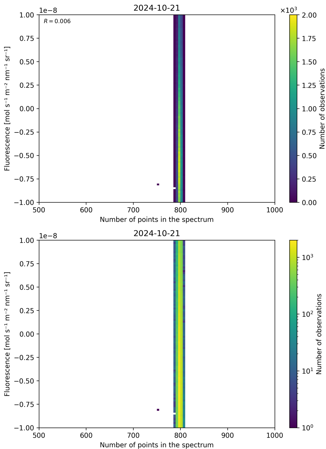
Figure 91: Scatter density plot of “Number of points in the spectrum” against “Fluorescence” for 2024-10-20 to 2024-10-22.
