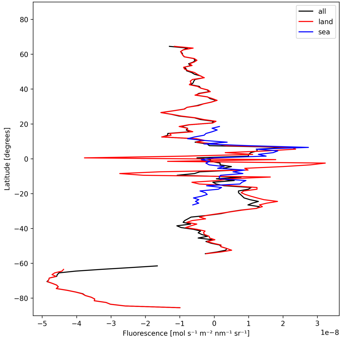
Figure 21: Zonal average of “Fluorescence” for 2024-10-20 to 2024-10-22.
