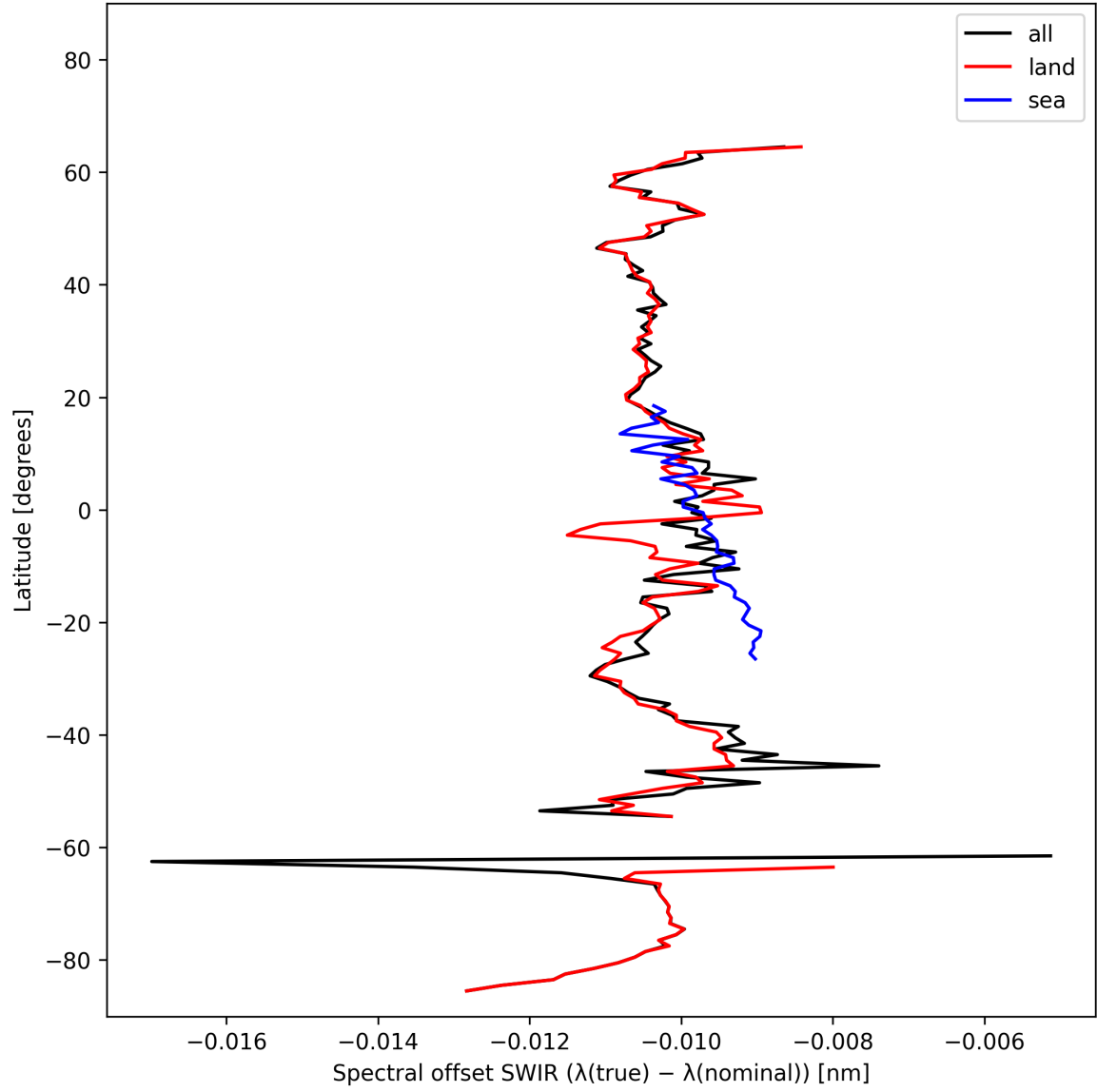
Figure 16: Zonal average of “Spectral offset SWIR ( \lambda_{\text{true}} - \lambda_{\text{nominal}} )” for 2024-10-20 to 2024-10-22.
