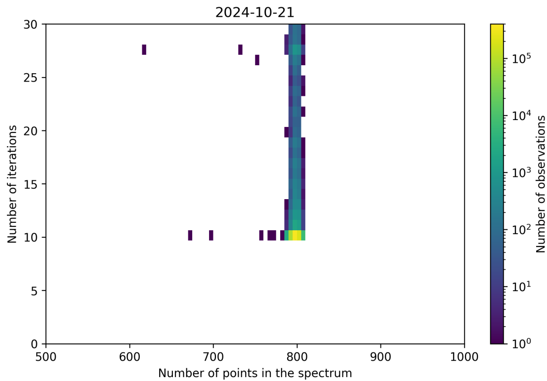
Figure 92: Scatter density plot of “Number of points in the spectrum” against “Number of iterations” for 2024-10-20 to 2024-10-22.
