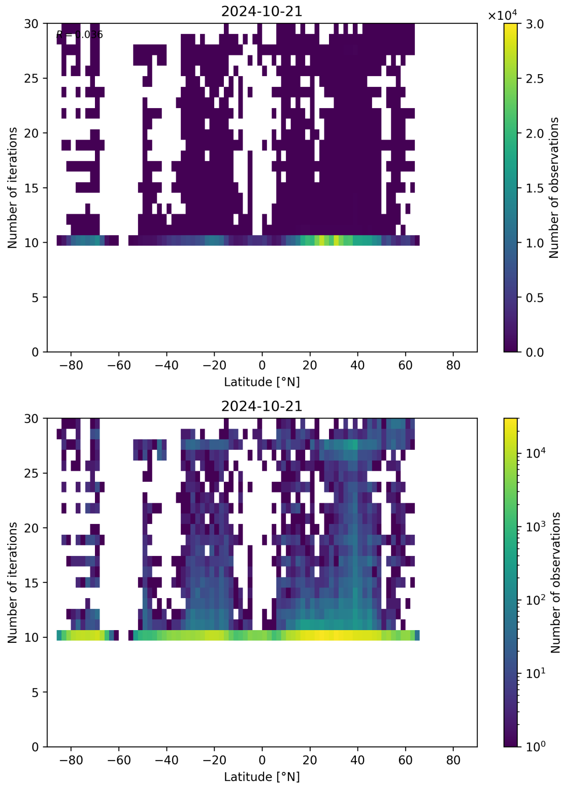
Figure 60: Scatter density plot of “Latitude” against “Number of iterations” for 2024-10-20 to 2024-10-22.
