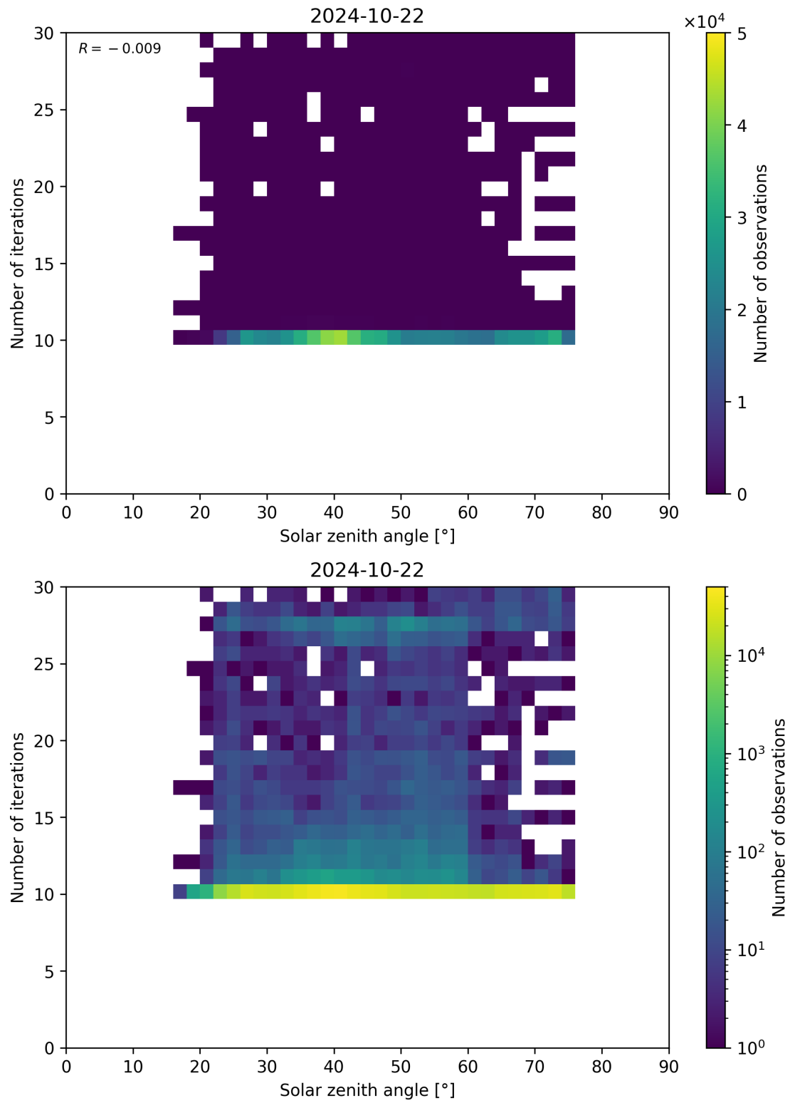
Figure 102: Scatter density plot of “Solar zenith angle” against “Number of iterations” for 2024-10-21 to 2024-10-23.
