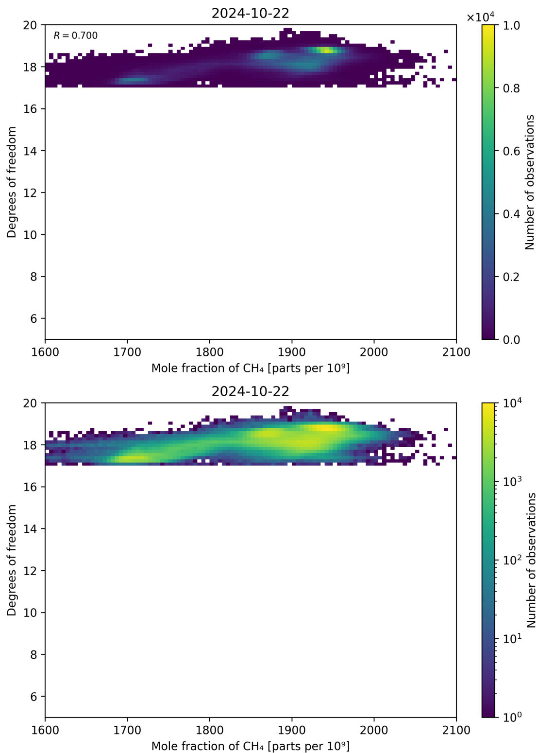
Figure 72: Scatter density plot of “Mole fraction of CH 4 ” against “Degrees of freedom” for 2024-10-21 to 2024-10-23.
