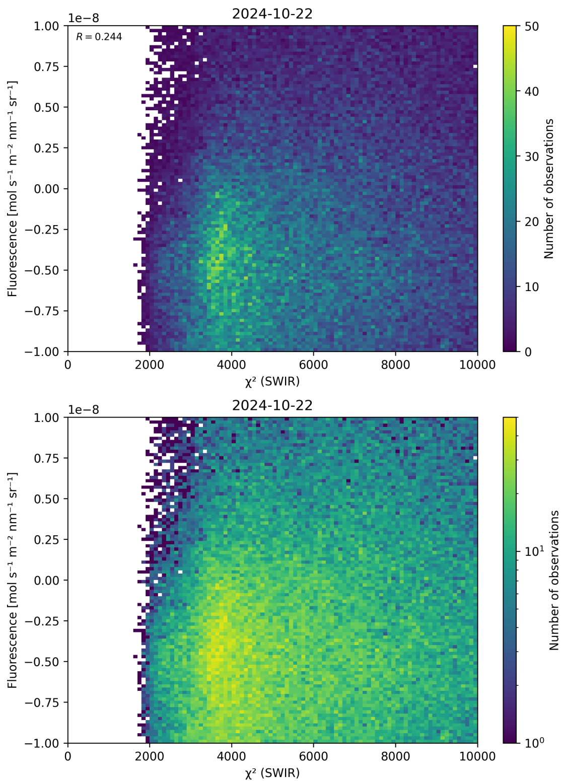
Figure 49: Scatter density plot of “ \chi^2 (SWIR)” against “Fluorescence” for 2024-10-21 to 2024-10-23.
