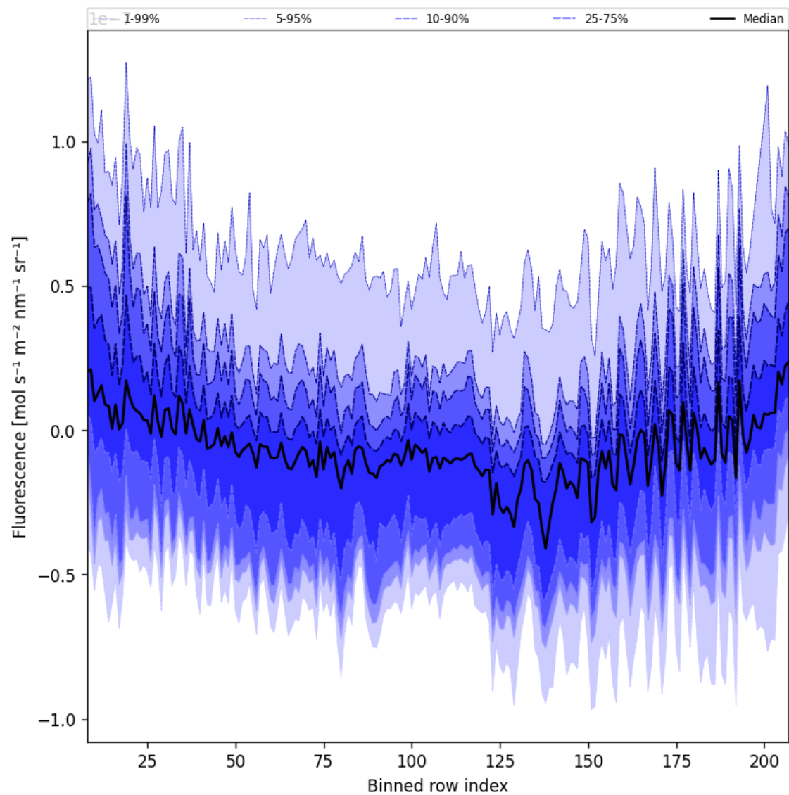
Figure 43: Along track statistics of “Fluorescence” for 2024-10-21 to 2024-10-23
