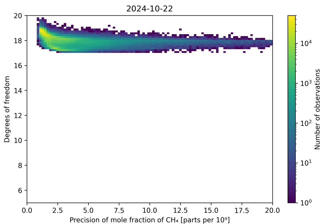
Figure 80: Scatter density plot of “Precision of mole fraction of CH 4 ” against “Degrees of freedom” for 2024-10-21 to 2024-10-23.
