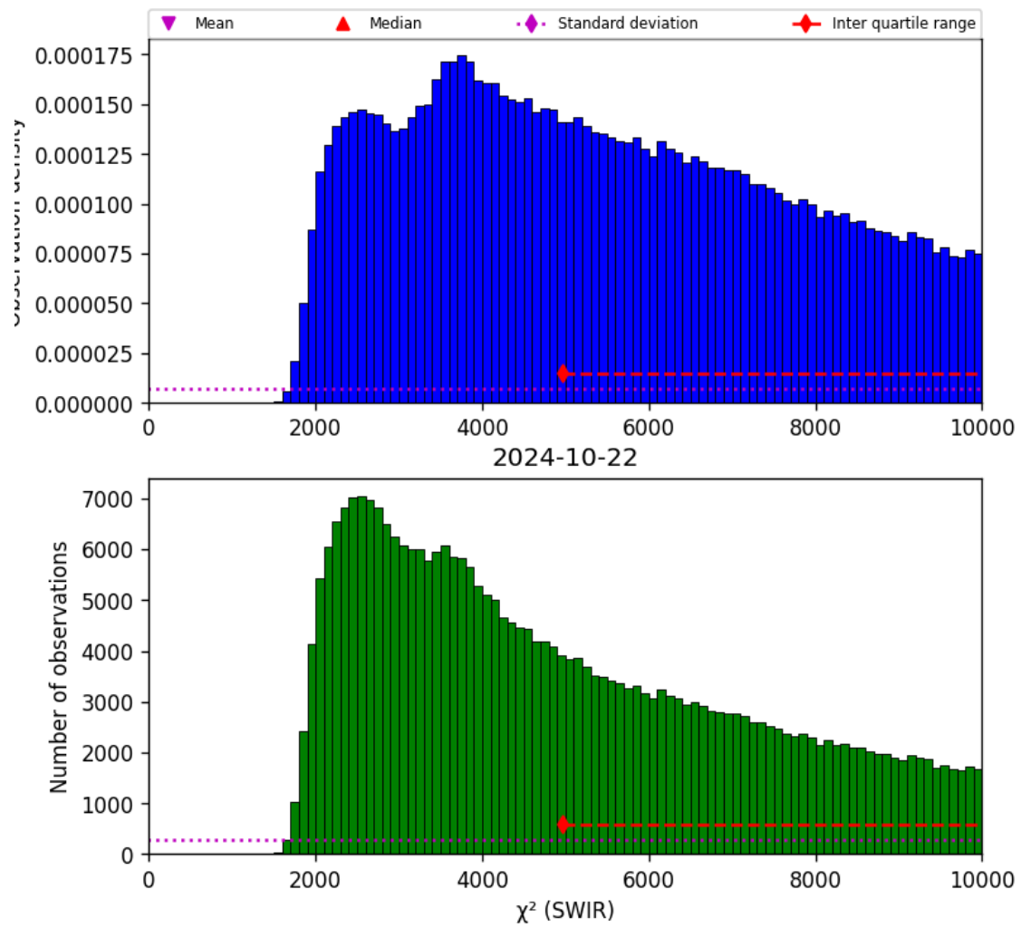
Figure 28: Histogram of “ \chi^2 (SWIR)” for 2024-10-21 to 2024-10-23
