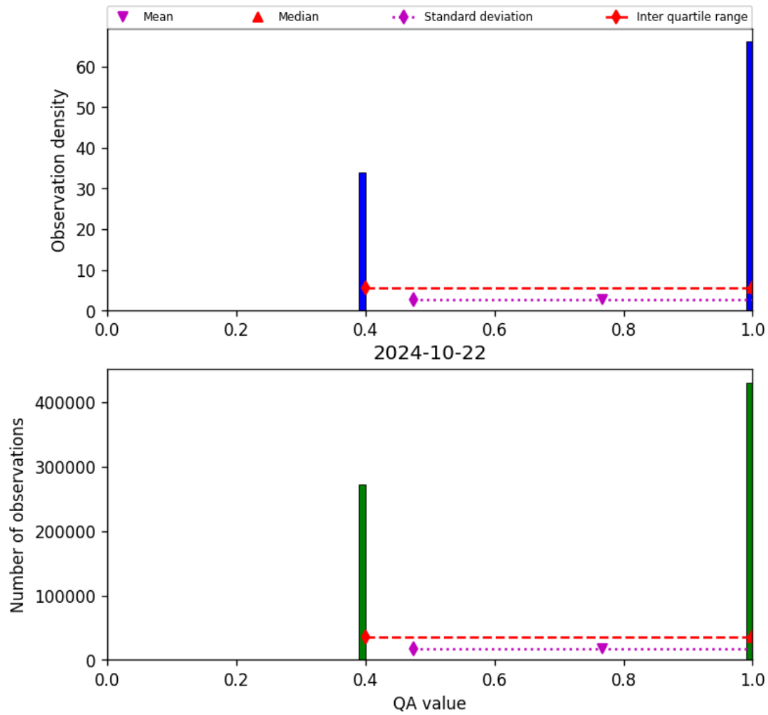
Figure 22: Histogram of “QA value” for 2024-10-21 to 2024-10-23
