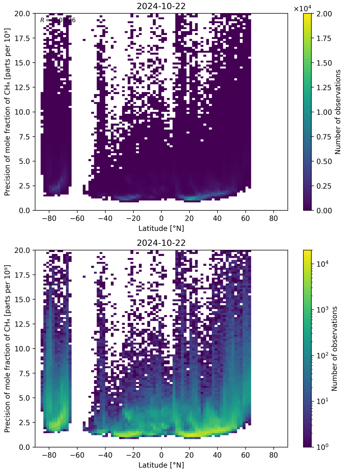
Figure 59: Scatter density plot of “Latitude” against “Precision of mole fraction of CH 4 ” for 2024-10-21 to 2024-10-23.
