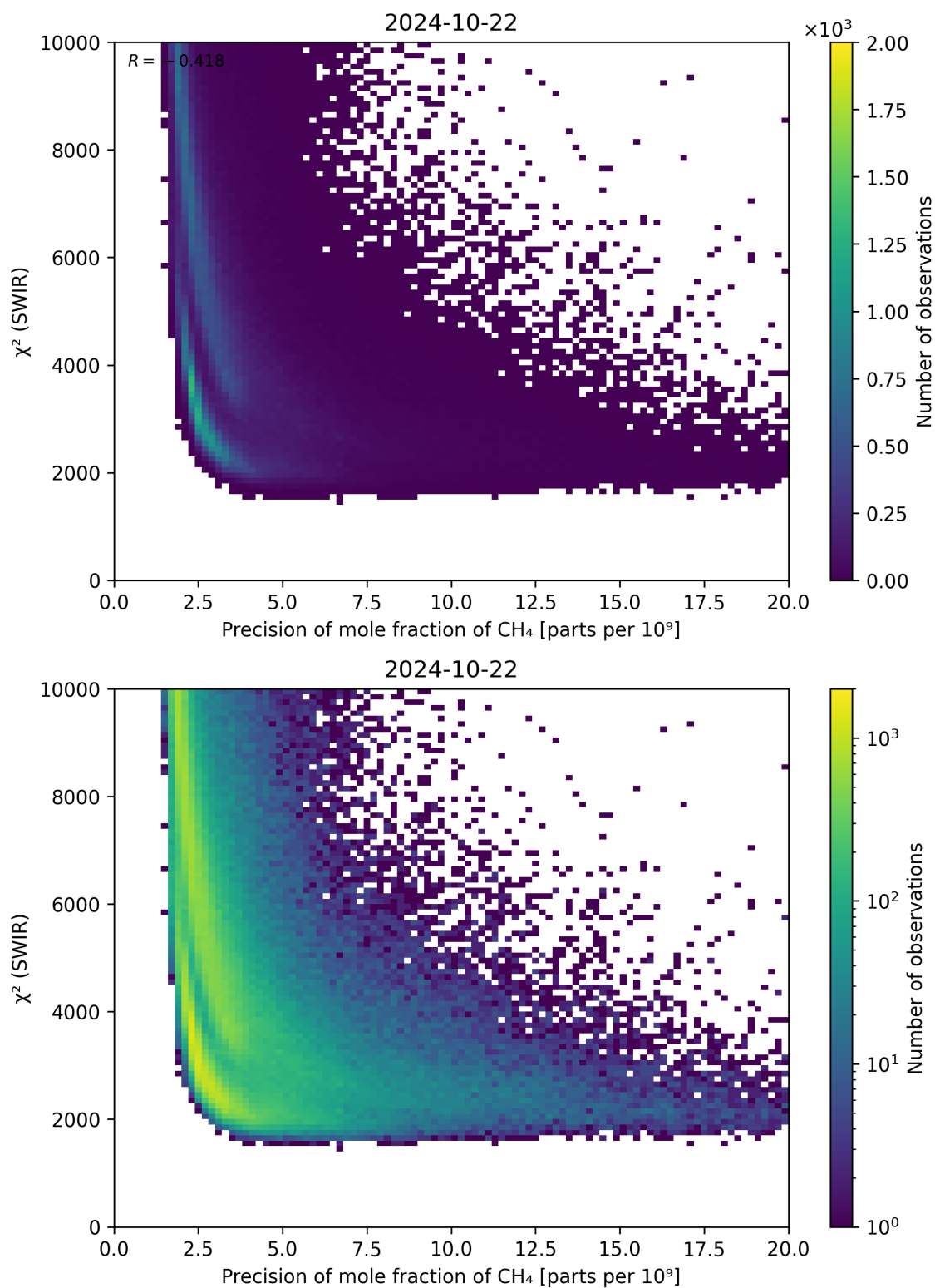
Figure 79: Scatter density plot of “Precision of mole fraction of \text{CH}_4 ” against “ \chi^2 (SWIR)” for 2024-10-21 to 2024-10-23.
