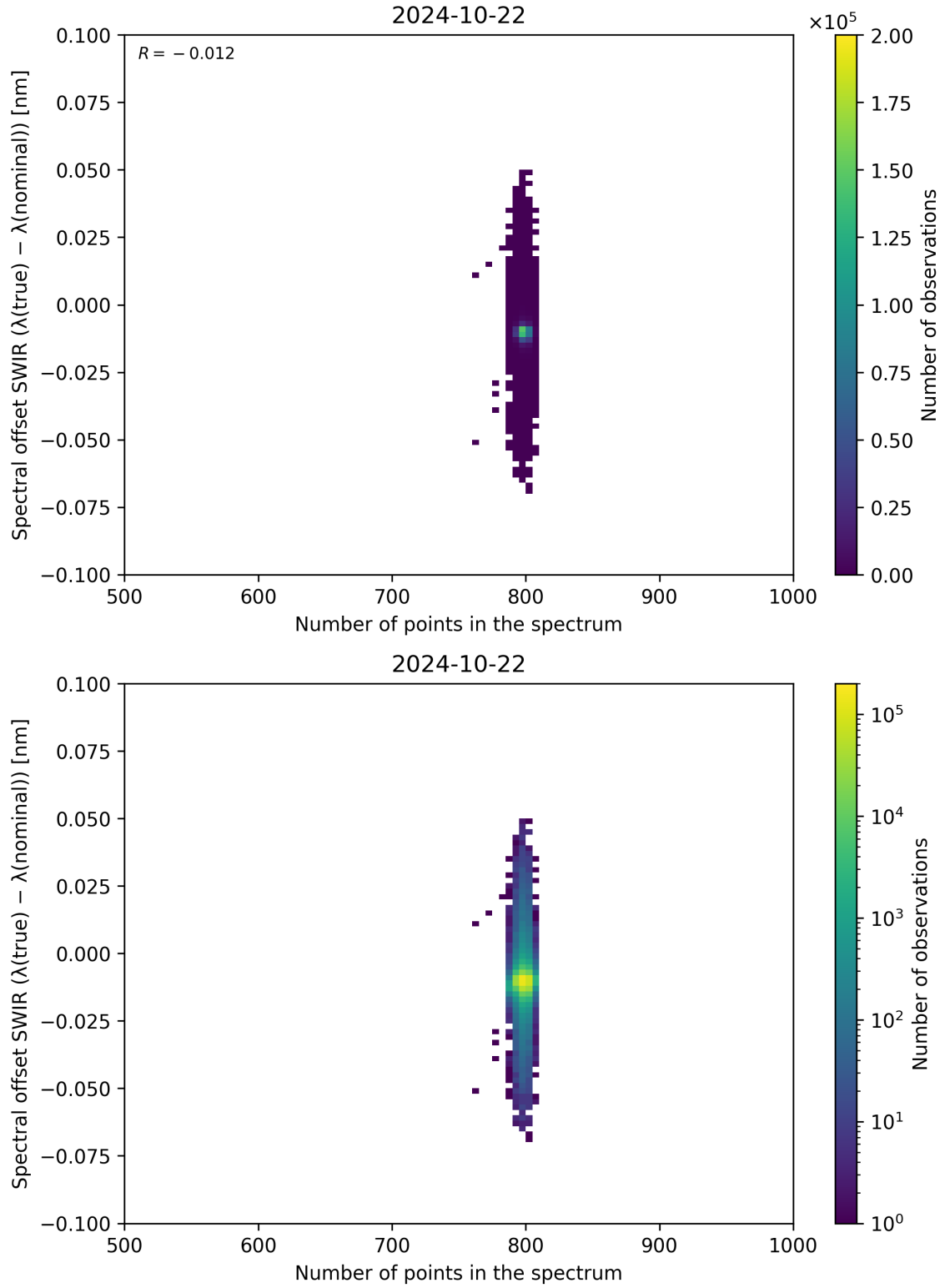
Figure 93: Scatter density plot of “Number of points in the spectrum” against “Spectral offset SWIR ( \lambda_{\text{true}} - \lambda_{\text{nominal}} )” for 2024-10-21 to 2024-10-23.
