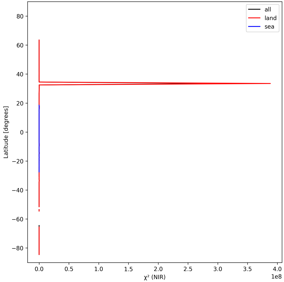
Figure 18: Zonal average of “ \chi^2 (NIR)” for 2024-10-21 to 2024-10-23.
