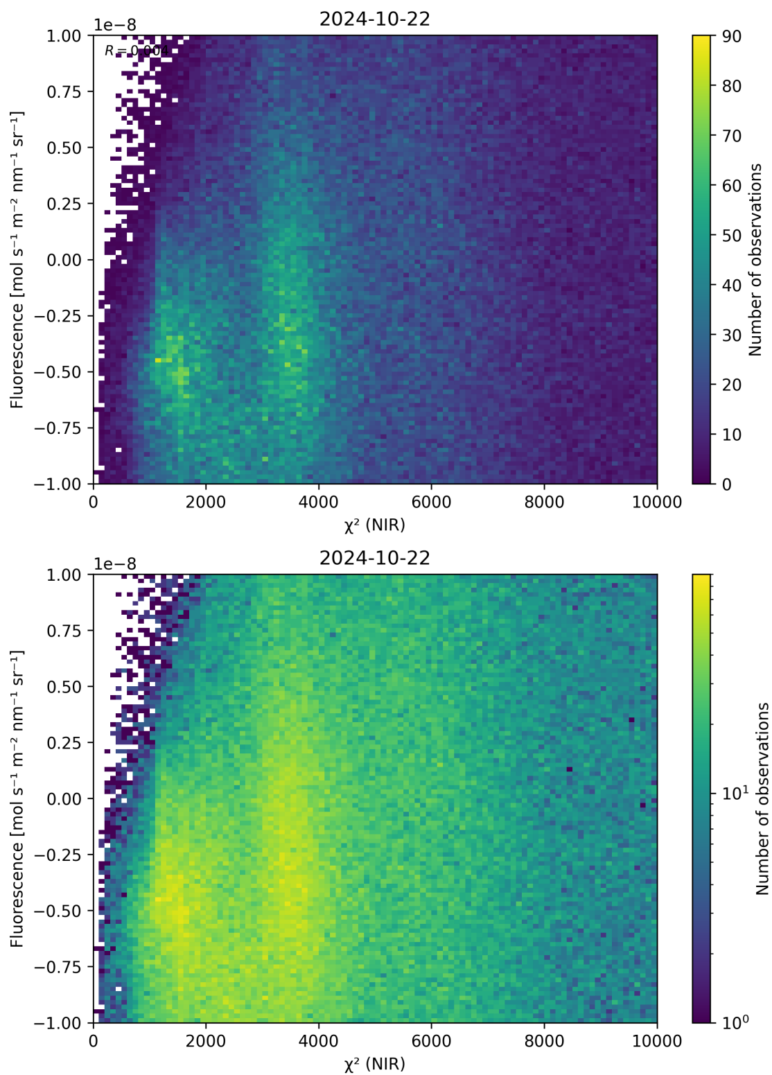
Figure 45: Scatter density plot of “ \chi^2 (NIR)” against “Fluorescence” for 2024-10-21 to 2024-10-23.
