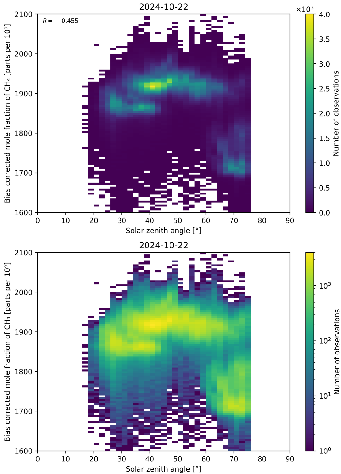
Figure 100: Scatter density plot of “Solar zenith angle” against “Bias corrected mole fraction of CH 4 ” for 2024-10-21 to 2024-10-23.
