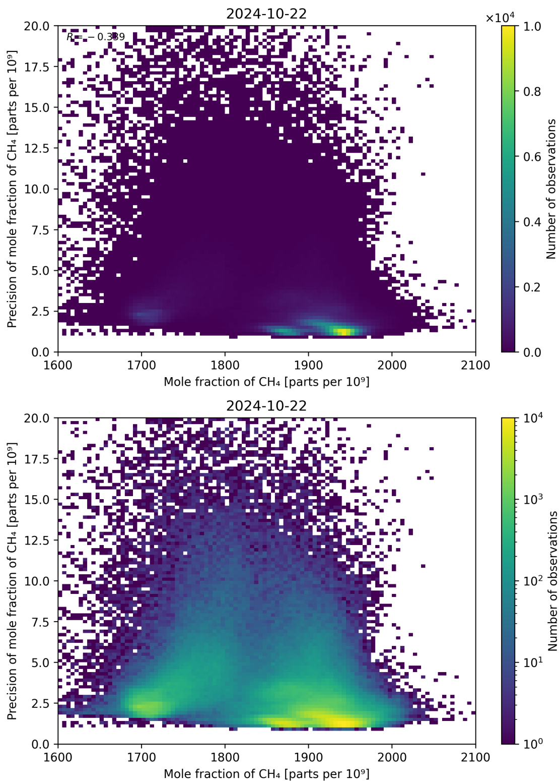
Figure 75: Scatter density plot of “Mole fraction of CH 4 ” against “Precision of mole fraction of CH 4 ” for 2024-10-21 to 2024-10-23.
