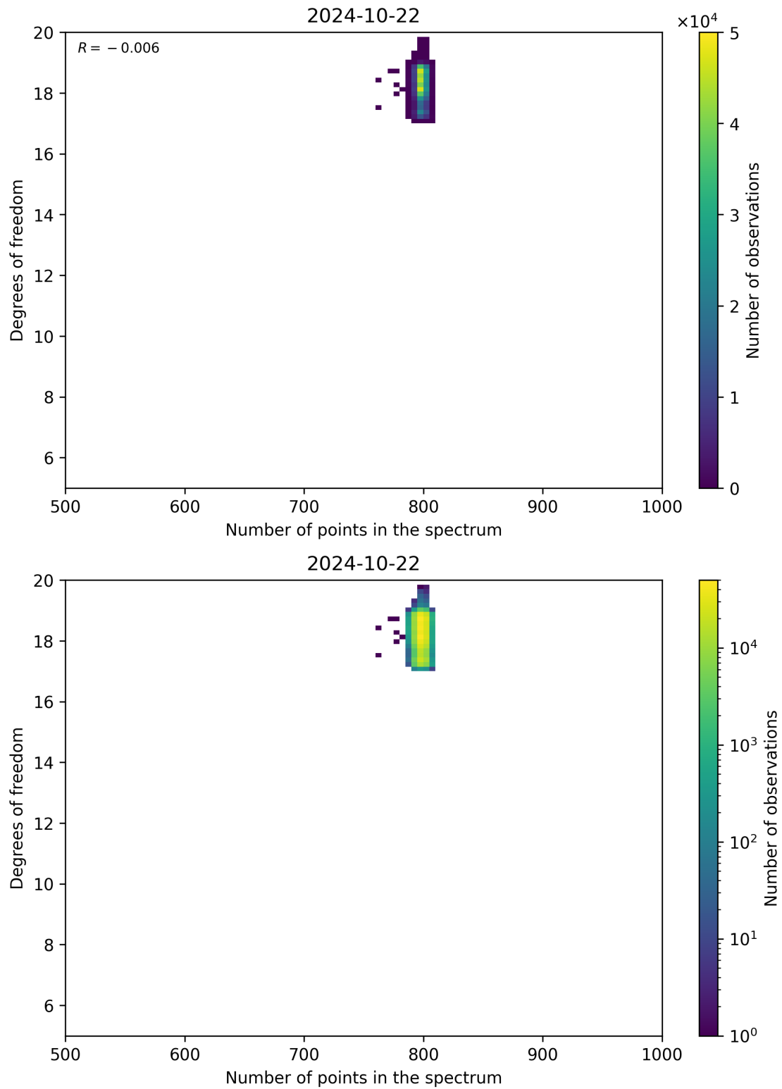
Figure 90: Scatter density plot of “Number of points in the spectrum” against “Degrees of freedom” for 2024-10-21 to 2024-10-23.
