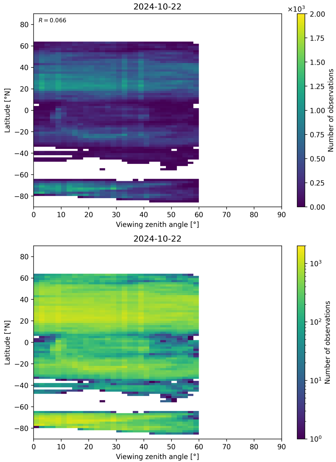
Figure 109: Scatter density plot of “Viewing zenith angle” against “Latitude” for 2024-10-21 to 2024-10-23.
