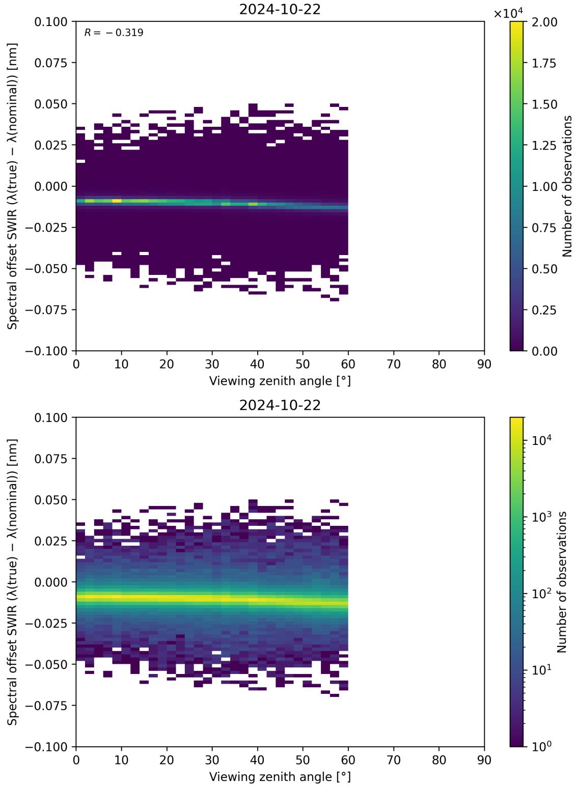
Figure 116: Scatter density plot of “Viewing zenith angle” against “Spectral offset SWIR ( \lambda_{\text{true}} - \lambda_{\text{nominal}} )” for 2024-10-21 to 2024-10-23.
