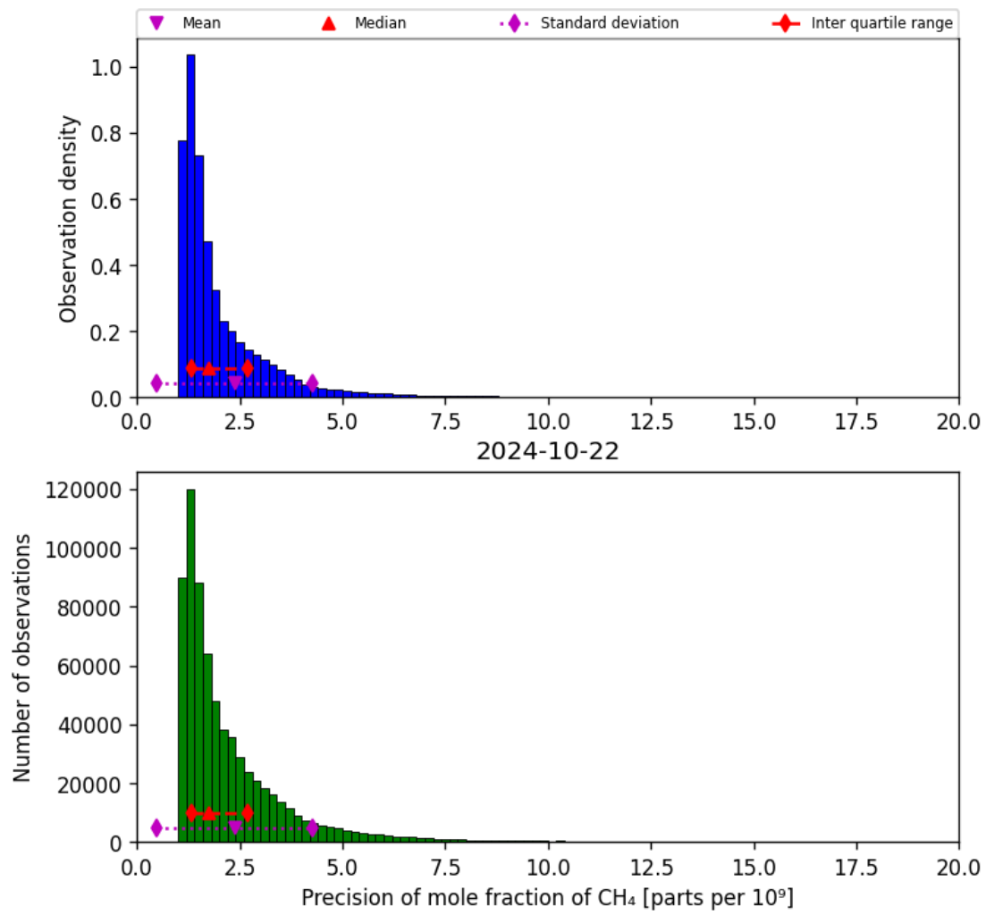
Figure 24: Histogram of “Precision of mole fraction of CH 4 ” for 2024-10-21 to 2024-10-23
