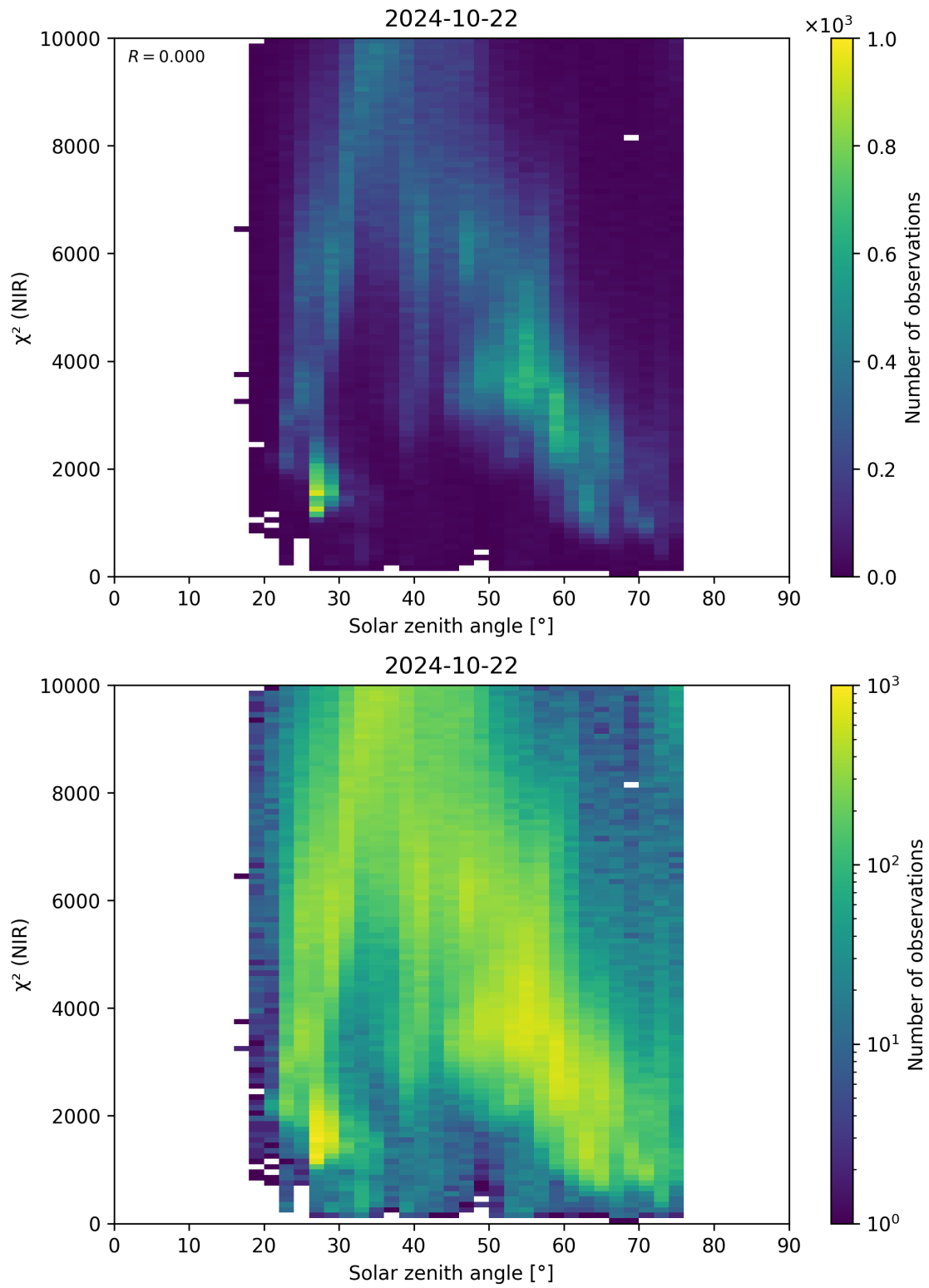
Figure 94: Scatter density plot of “Solar zenith angle” against “ \chi^2 (NIR)” for 2024-10-21 to 2024-10-23.
