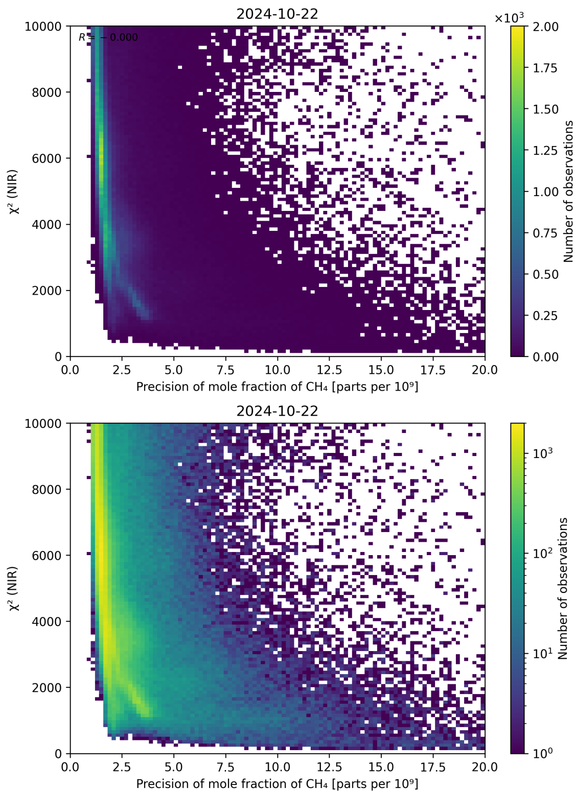
Figure 78: Scatter density plot of “Precision of mole fraction of \text{CH}_4 ” against “ \chi^2 (NIR)” for 2024-10-21 to 2024-10-23.
