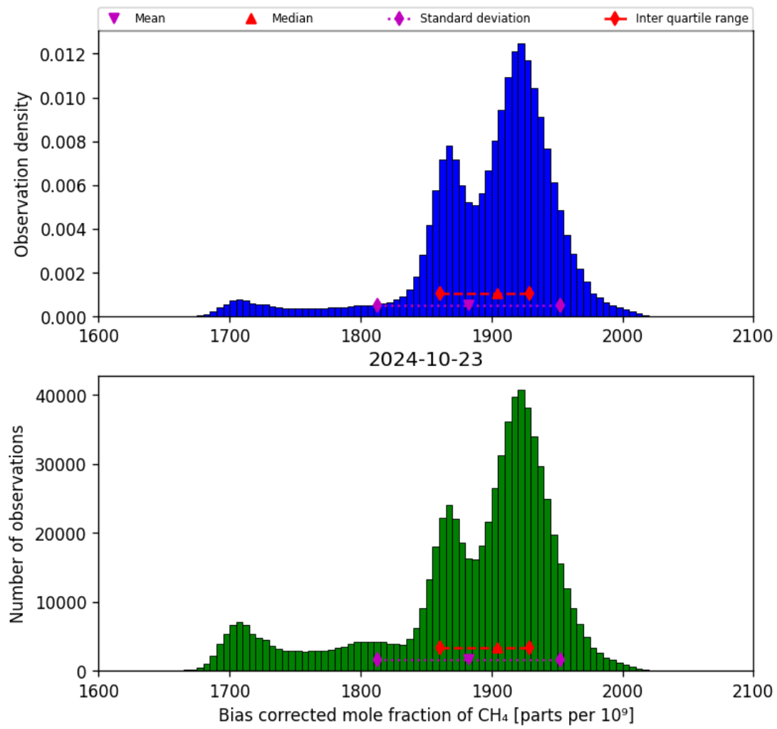
Figure 25: Histogram of “Bias corrected mole fraction of CH 4 ” for 2024-10-22 to 2024-10-24
