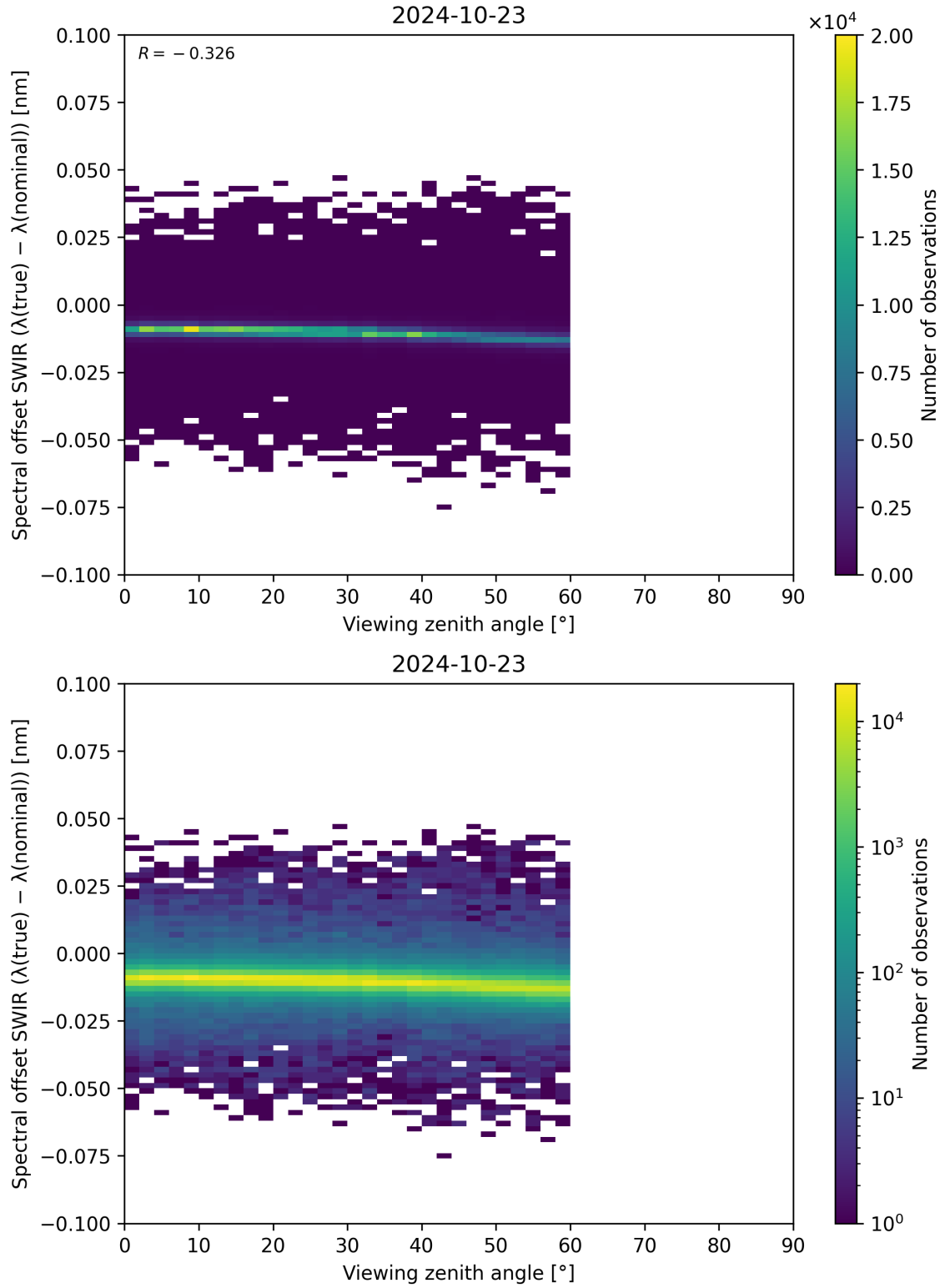
Figure 116: Scatter density plot of “Viewing zenith angle” against “Spectral offset SWIR ( \lambda_{\text{true}} - \lambda_{\text{nominal}} )” for 2024-10-22 to 2024-10-24.
