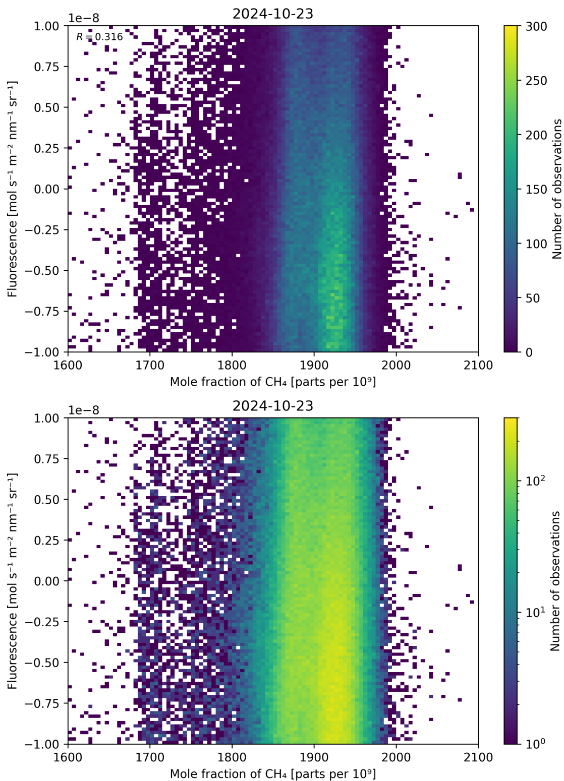
Figure 73: Scatter density plot of “Mole fraction of \text{CH}_4 ” against “Fluorescence” for 2024-10-22 to 2024-10-24.
