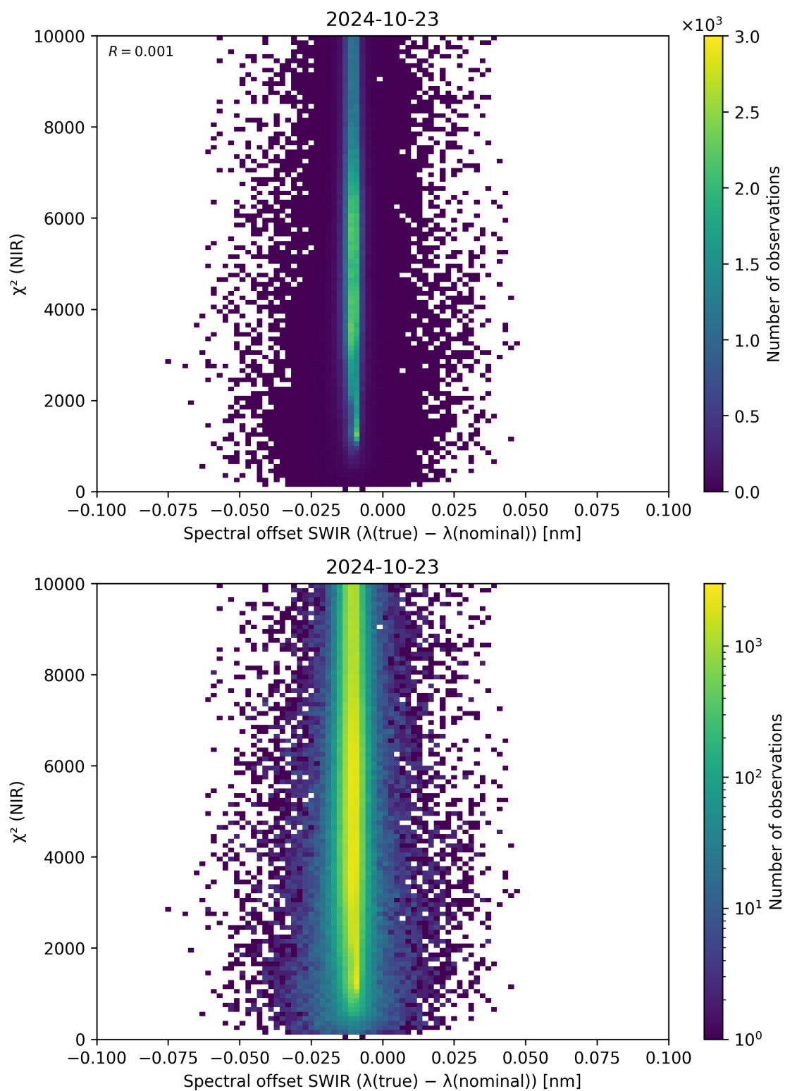
Figure 117: Scatter density plot of “Spectral offset SWIR ( \lambda_{\text{true}} - \lambda_{\text{nominal}} )” against “ \chi^2 (NIR)” for 2024-10-22 to 2024-10-24.
