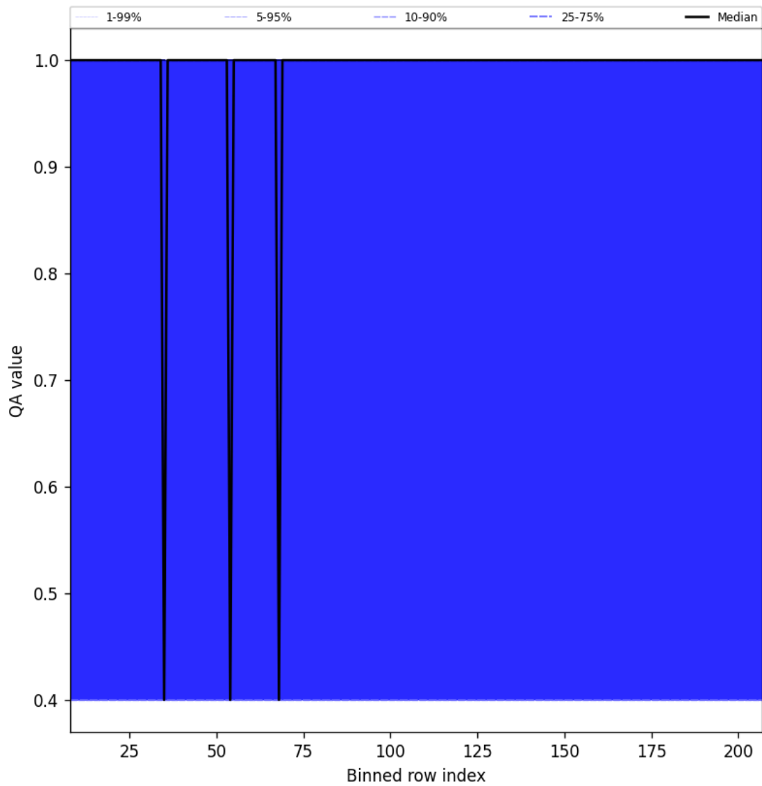
Figure 33: Along track statistics of “QA value” for 2024-10-22 to 2024-10-24
