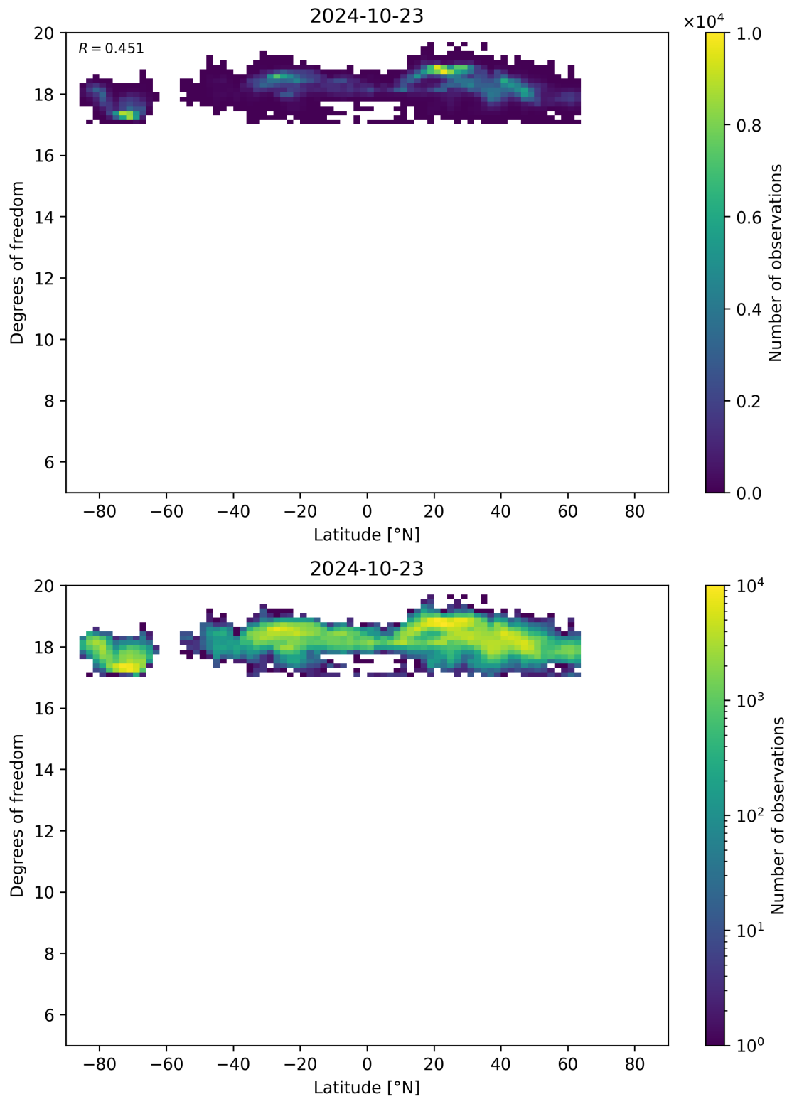
Figure 55: Scatter density plot of “Latitude” against “Degrees of freedom” for 2024-10-22 to 2024-10-24.
