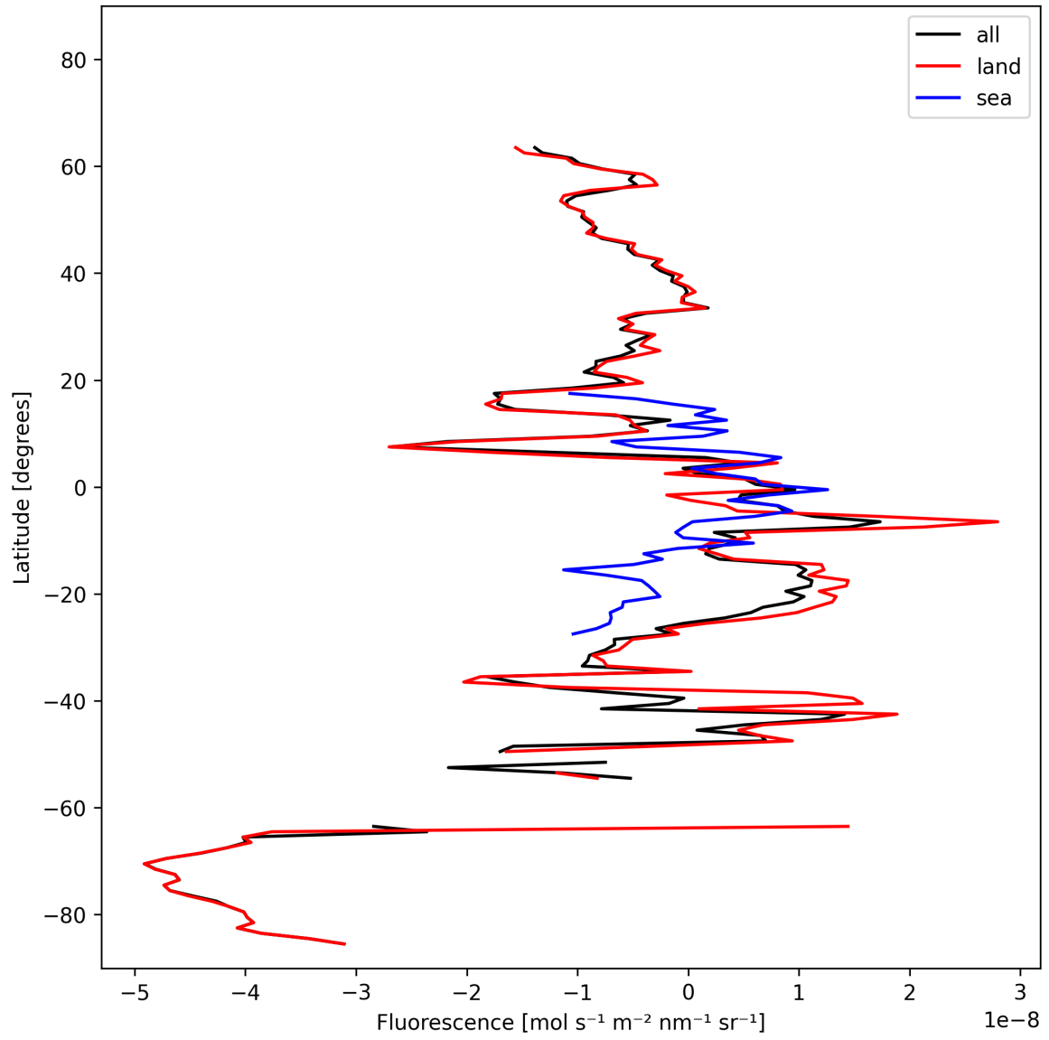
Figure 21: Zonal average of “Fluorescence” for 2024-10-22 to 2024-10-24.
