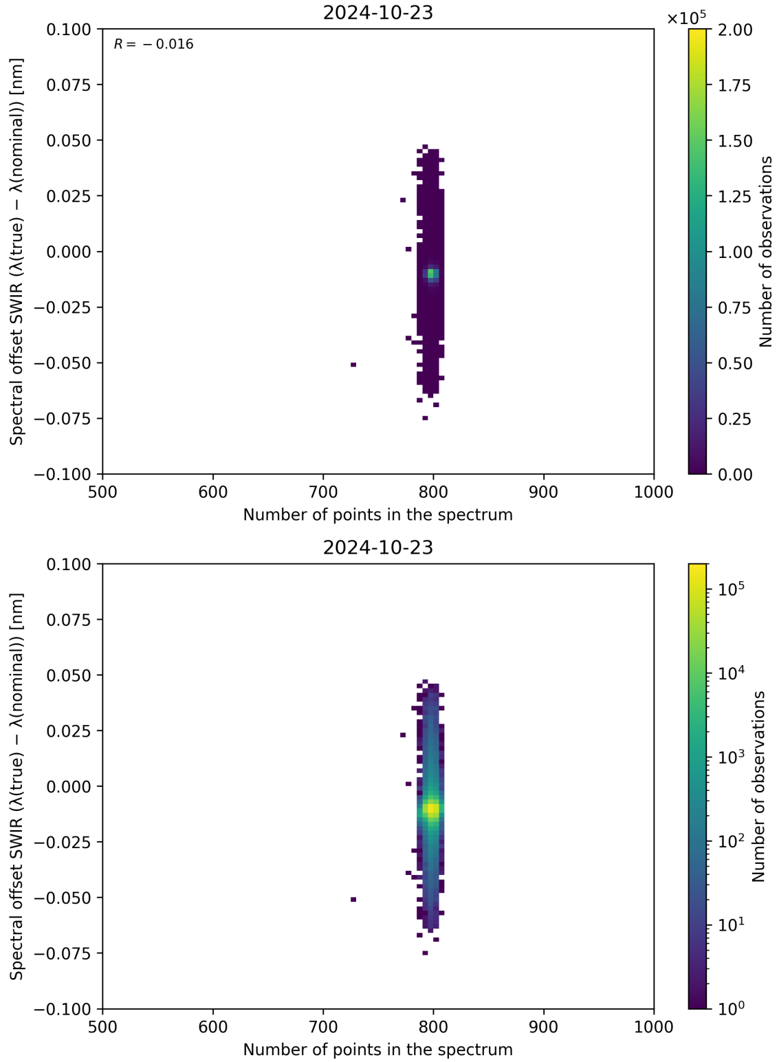
Figure 93: Scatter density plot of “Number of points in the spectrum” against “Spectral offset SWIR ( \lambda_{\text{true}} - \lambda_{\text{nominal}} )” for 2024-10-22 to 2024-10-24.
