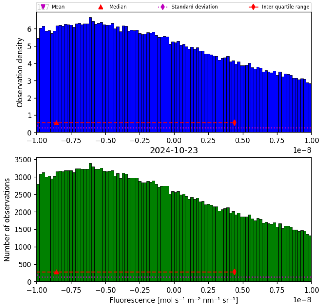
Figure 32: Histogram of “Fluorescence” for 2024-10-22 to 2024-10-24
