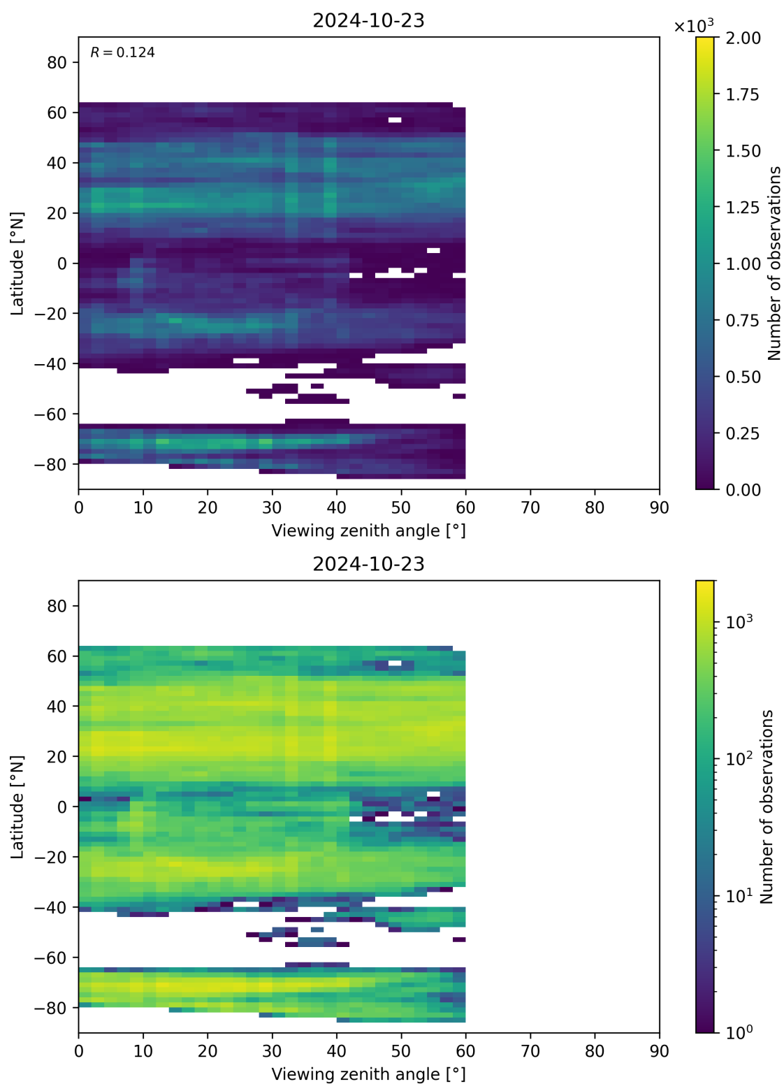
Figure 109: Scatter density plot of “Viewing zenith angle” against “Latitude” for 2024-10-22 to 2024-10-24.
