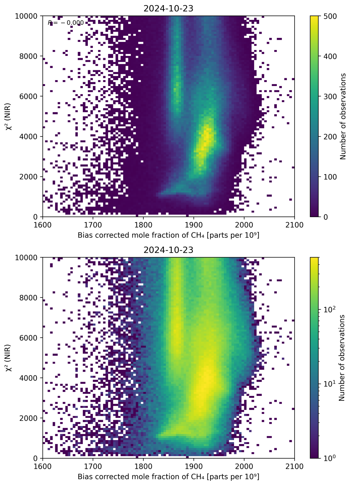
Figure 63: Scatter density plot of “Bias corrected mole fraction of \text{CH}_4 ” against “ \chi^2 (NIR)” for 2024-10-22 to 2024-10-24.
