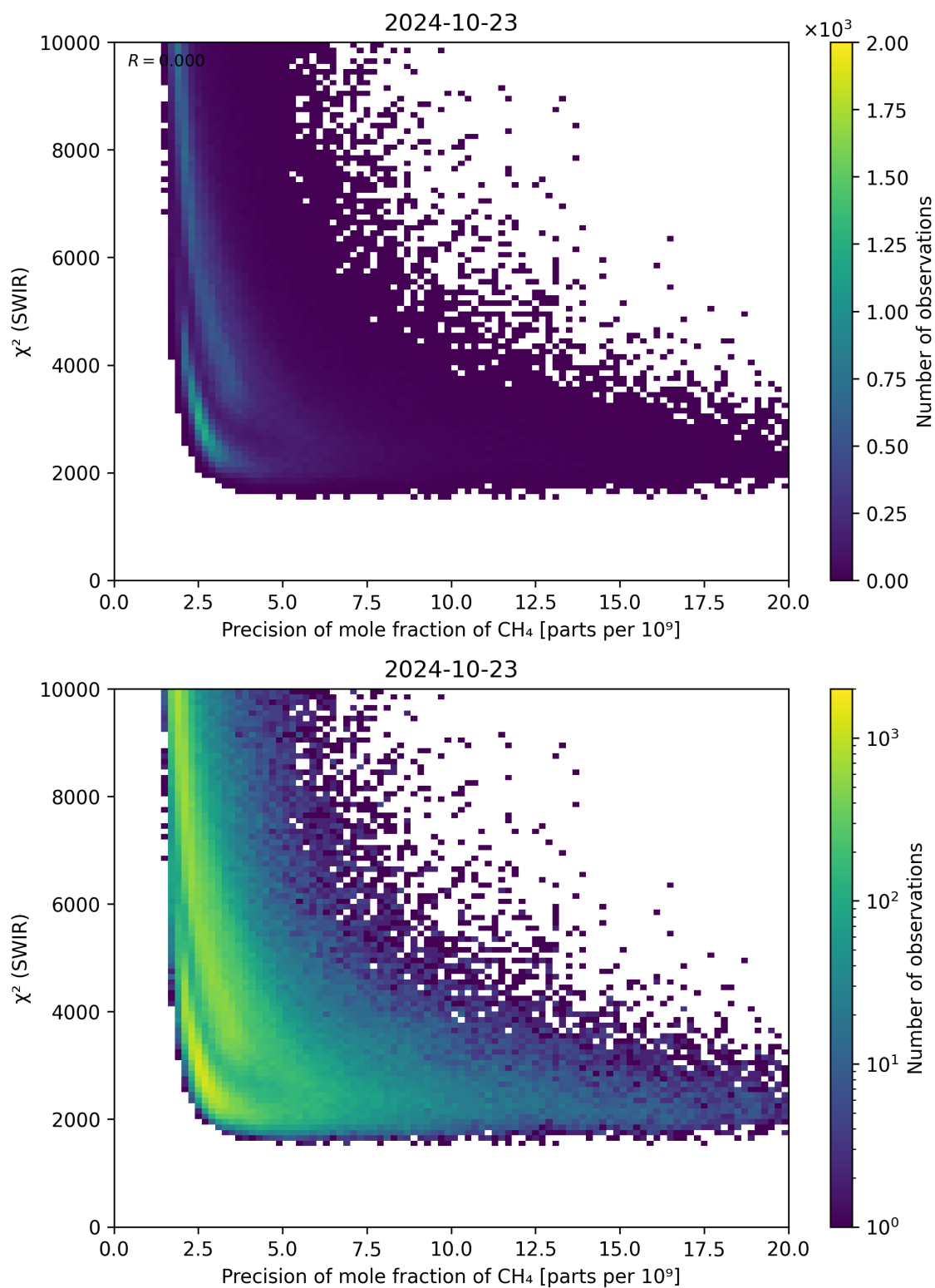
Figure 79: Scatter density plot of “Precision of mole fraction of \text{CH}_4 ” against “ \chi^2 (SWIR)” for 2024-10-22 to 2024-10-24.
