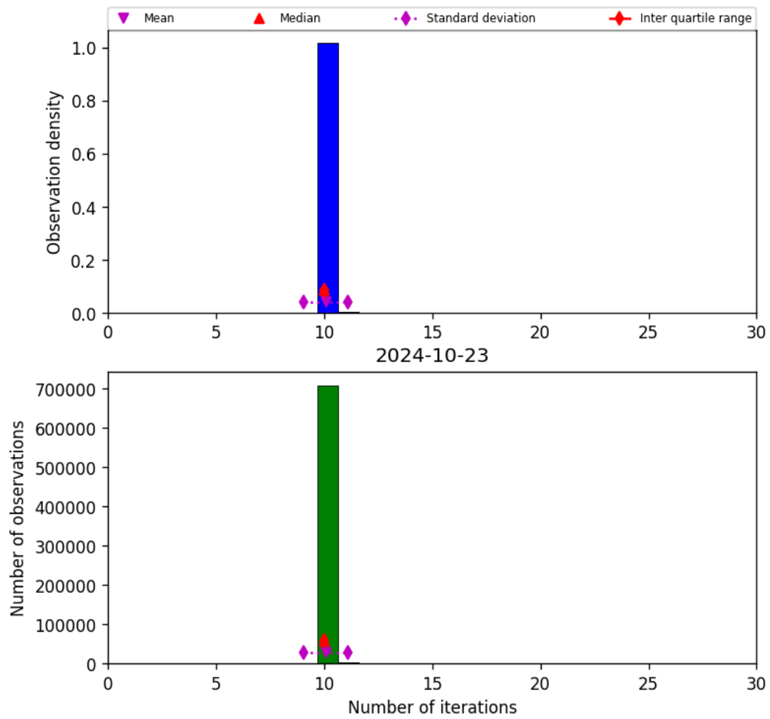
Figure 31: Histogram of “Number of iterations” for 2024-10-22 to 2024-10-24
