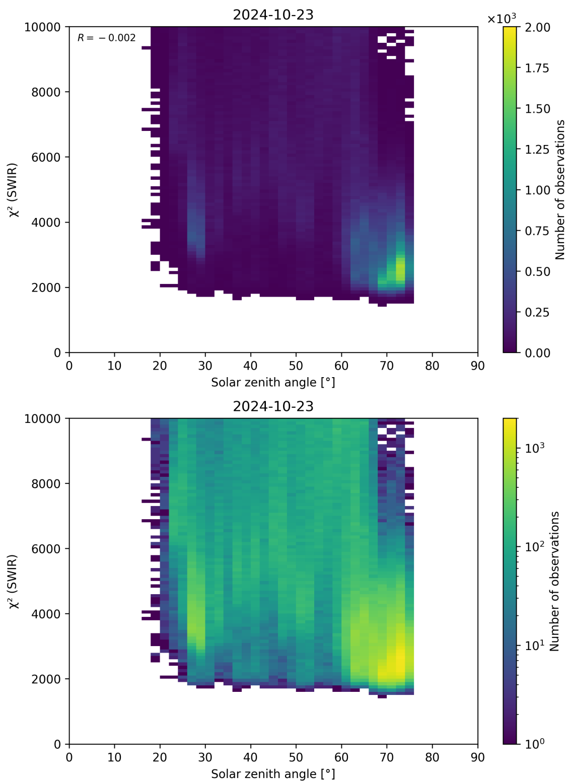
Figure 95: Scatter density plot of “Solar zenith angle” against “ \chi^2 (SWIR)” for 2024-10-22 to 2024-10-24.
