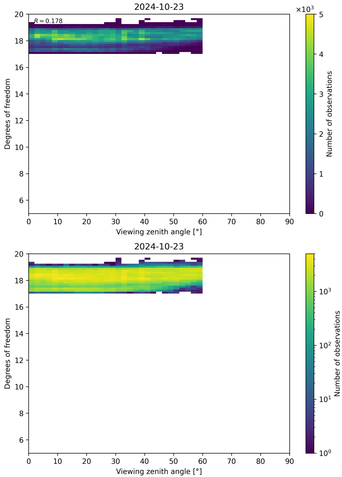
Figure 107: Scatter density plot of “Viewing zenith angle” against “Degrees of freedom” for 2024-10-22 to 2024-10-24.
