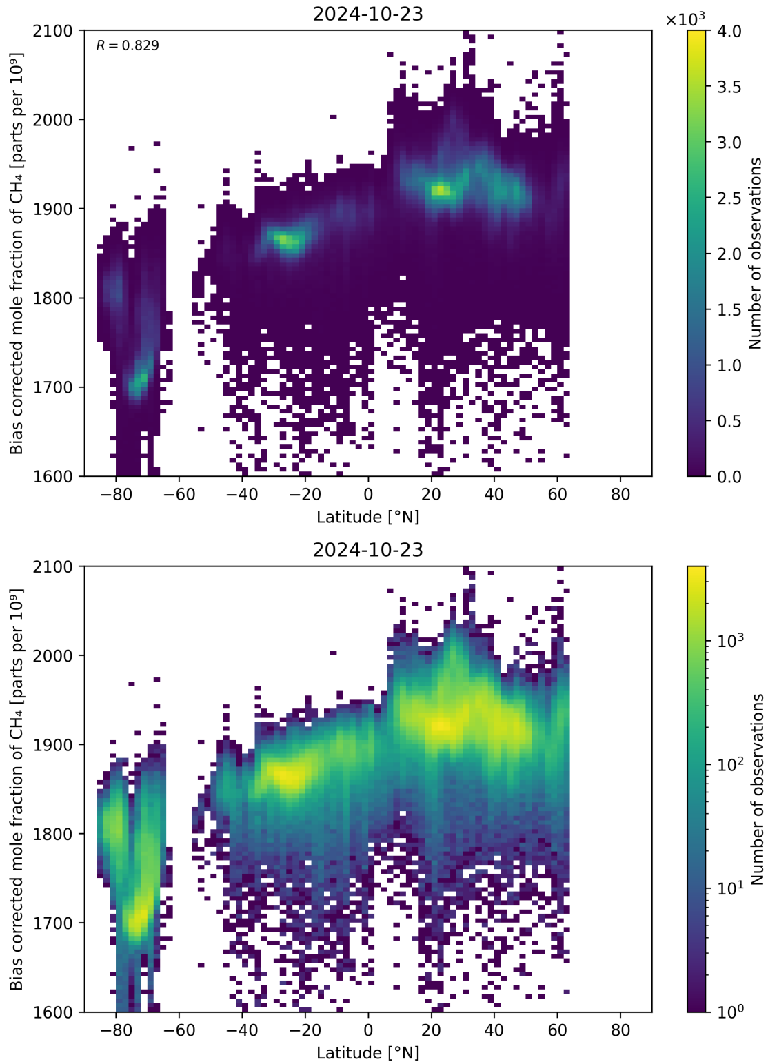
Figure 58: Scatter density plot of “Latitude” against “Bias corrected mole fraction of CH 4 ” for 2024-10-22 to 2024-10-24.
