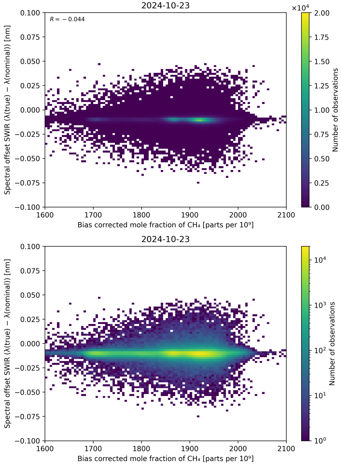
Figure 69: Scatter density plot of “Bias corrected mole fraction of \text{CH}_4 ” against “Spectral offset SWIR ( \lambda_{\text{true}} - \lambda_{\text{nominal}} )” for 2024-10-22 to 2024-10-24.
