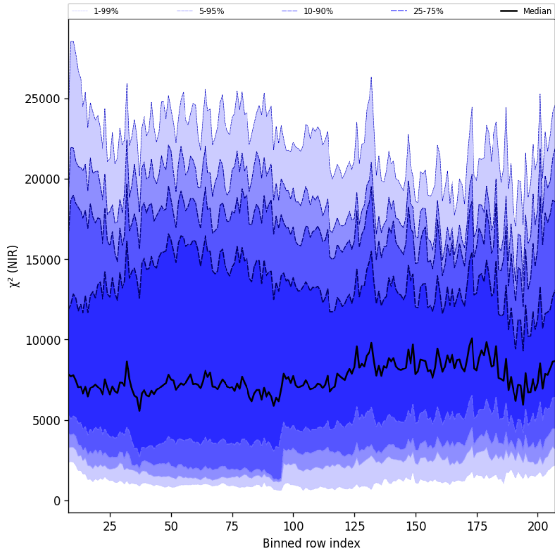
Figure 40: Along track statistics of “ \chi^2 (NIR)” for 2024-10-22 to 2024-10-24
