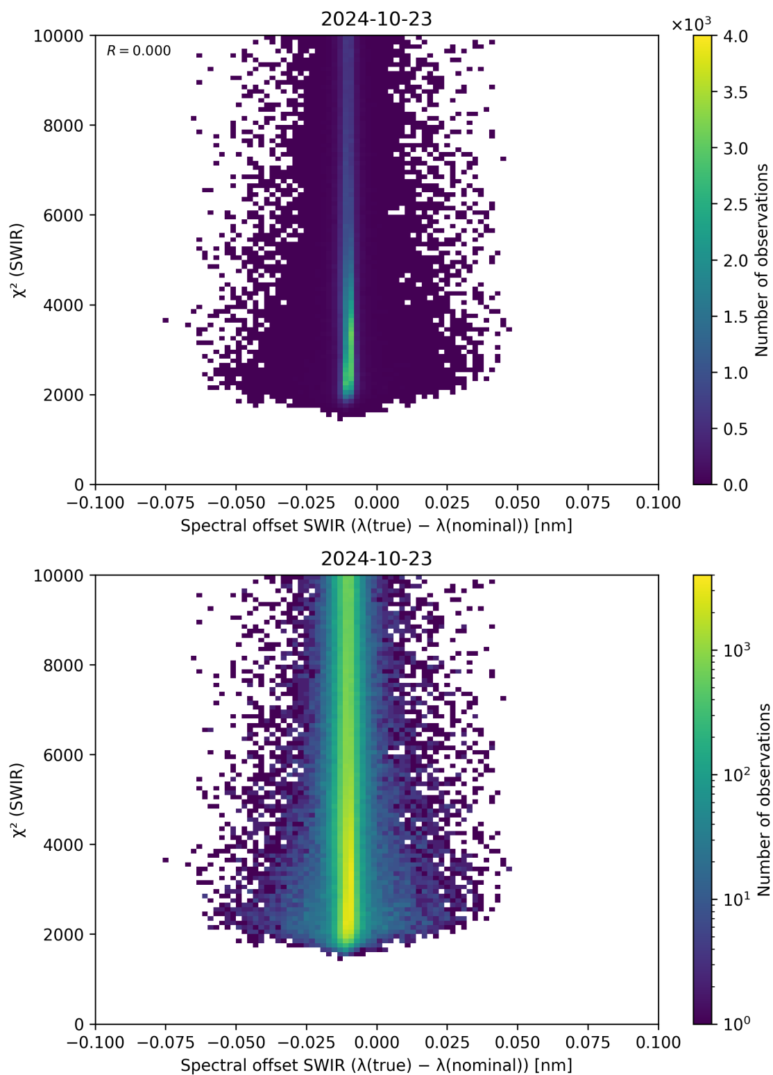
Figure 118: Scatter density plot of “Spectral offset SWIR ( \lambda_{\text{true}} - \lambda_{\text{nominal}} )” against “ \chi^2 (SWIR)” for 2024-10-22 to 2024-10-24.
