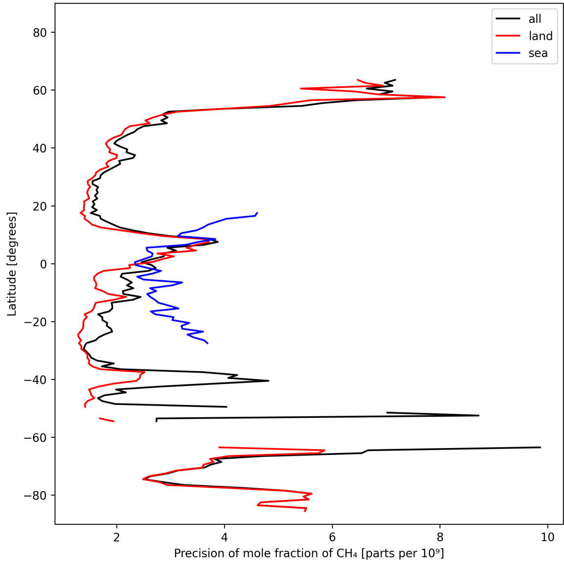
Figure 13: Zonal average of “Precision of mole fraction of CH 4 ” for 2024-10-22 to 2024-10-24.
