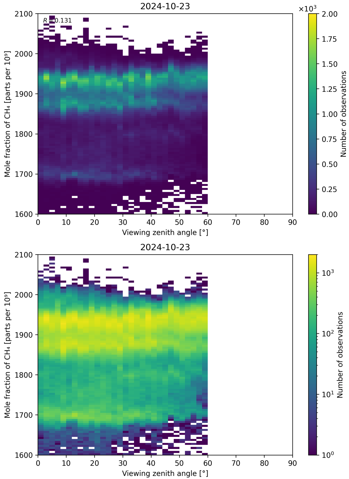
Figure 110: Scatter density plot of “Viewing zenith angle” against “Mole fraction of CH 4 ” for 2024-10-22 to 2024-10-24.
