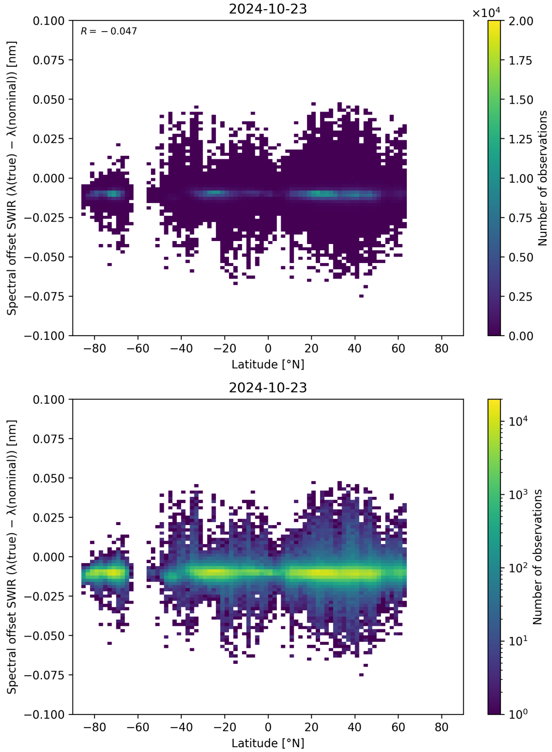
Figure 62: Scatter density plot of “Latitude” against “Spectral offset SWIR ( \lambda_{\text{true}} - \lambda_{\text{nominal}} )” for 2024-10-22 to 2024-10-24.
