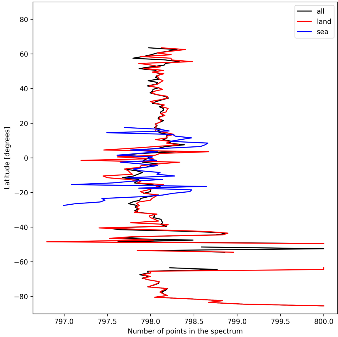
Figure 15: Zonal average of “Number of points in the spectrum” for 2024-10-22 to 2024-10-24.
