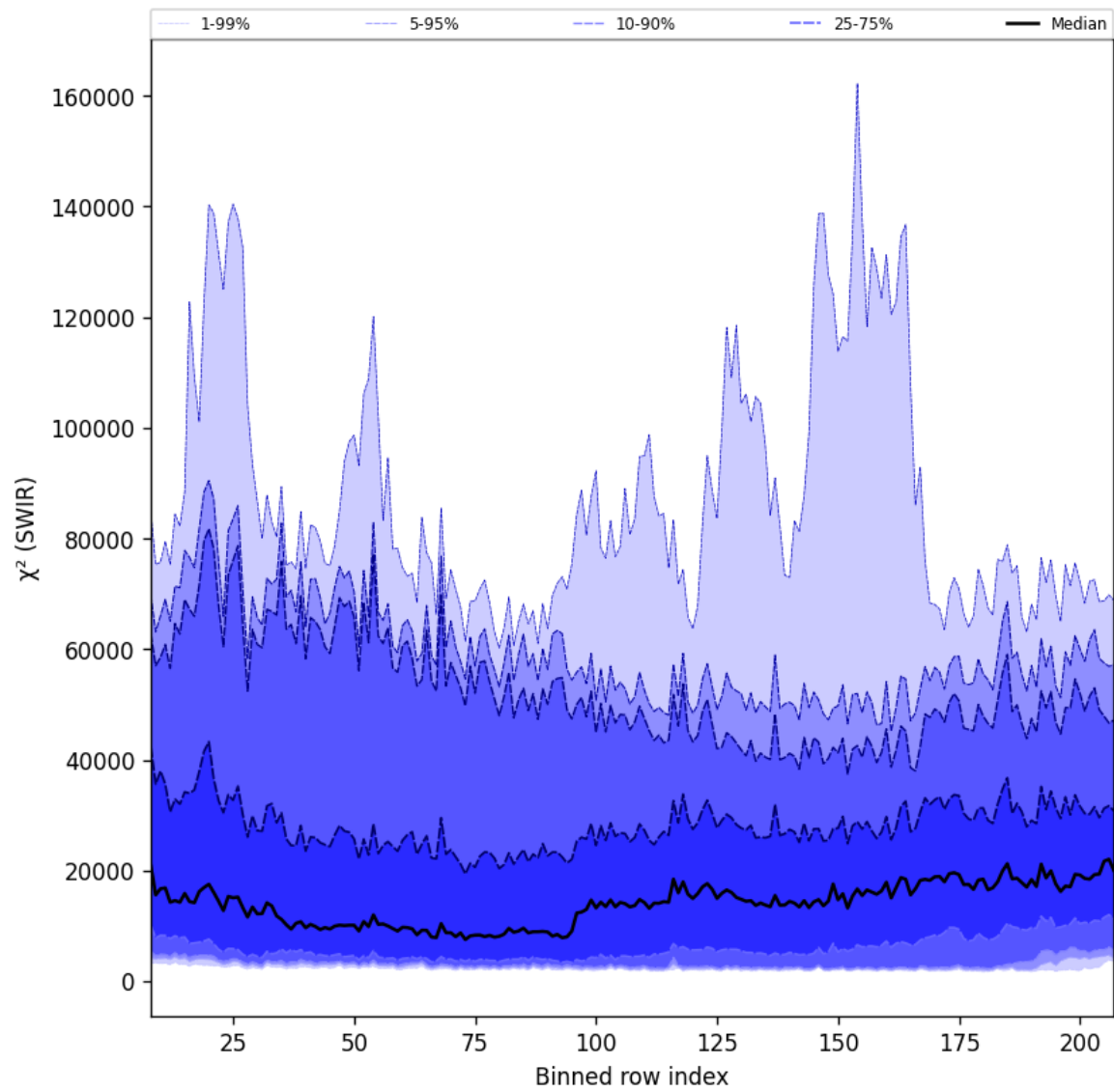
Figure 39: Along track statistics of “ \chi^2 (SWIR)” for 2024-10-22 to 2024-10-24
