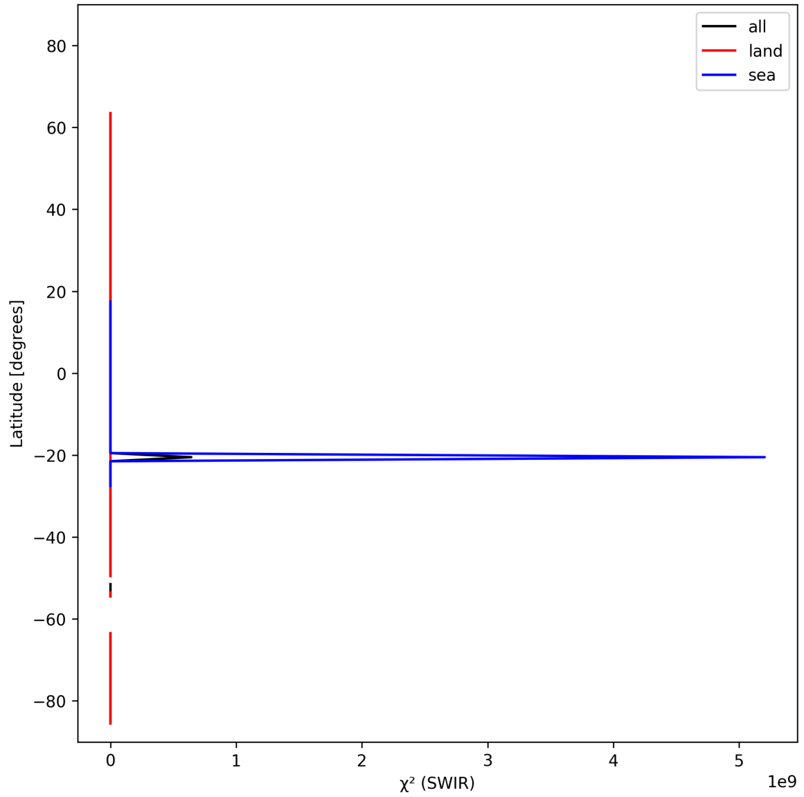
Figure 17: Zonal average of “ \chi^2 (SWIR)” for 2024-10-22 to 2024-10-24.
