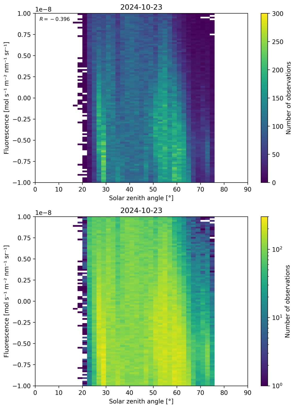
Figure 97: Scatter density plot of “Solar zenith angle” against “Fluorescence” for 2024-10-22 to 2024-10-24.
