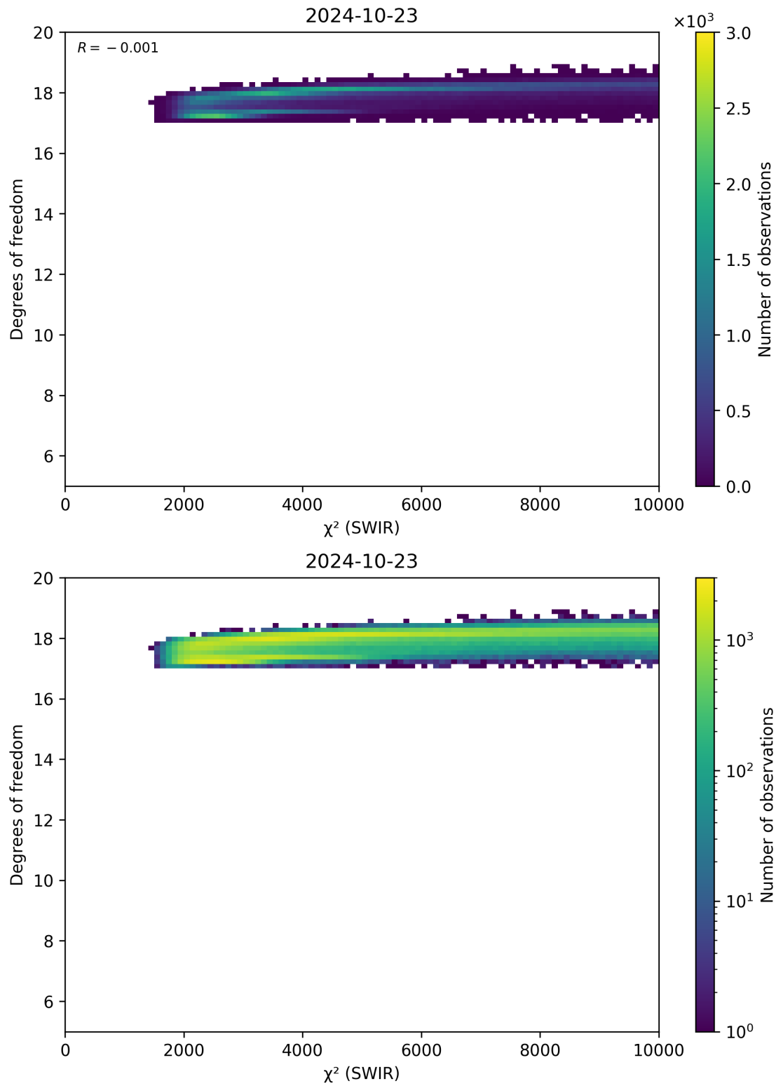
Figure 48: Scatter density plot of “ \chi^2 (SWIR)” against “Degrees of freedom” for 2024-10-22 to 2024-10-24.
