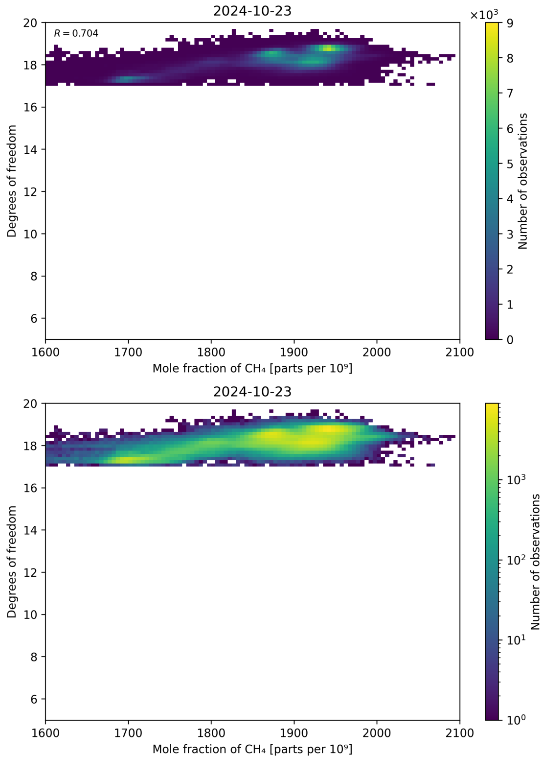
Figure 72: Scatter density plot of “Mole fraction of CH 4 ” against “Degrees of freedom” for 2024-10-22 to 2024-10-24.
