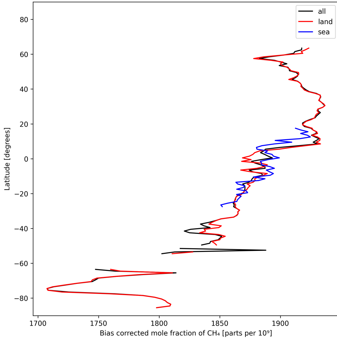
Figure 14: Zonal average of “Bias corrected mole fraction of CH 4 ” for 2024-10-22 to 2024-10-24.
