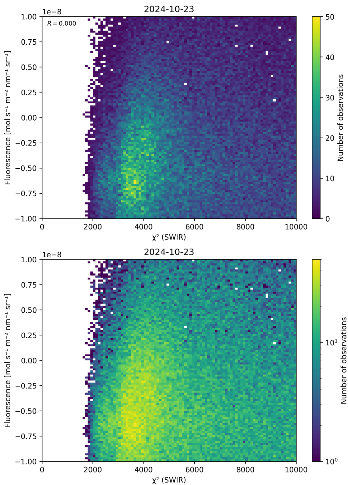
Figure 49: Scatter density plot of “ \chi^2 (SWIR)” against “Fluorescence” for 2024-10-22 to 2024-10-24.
