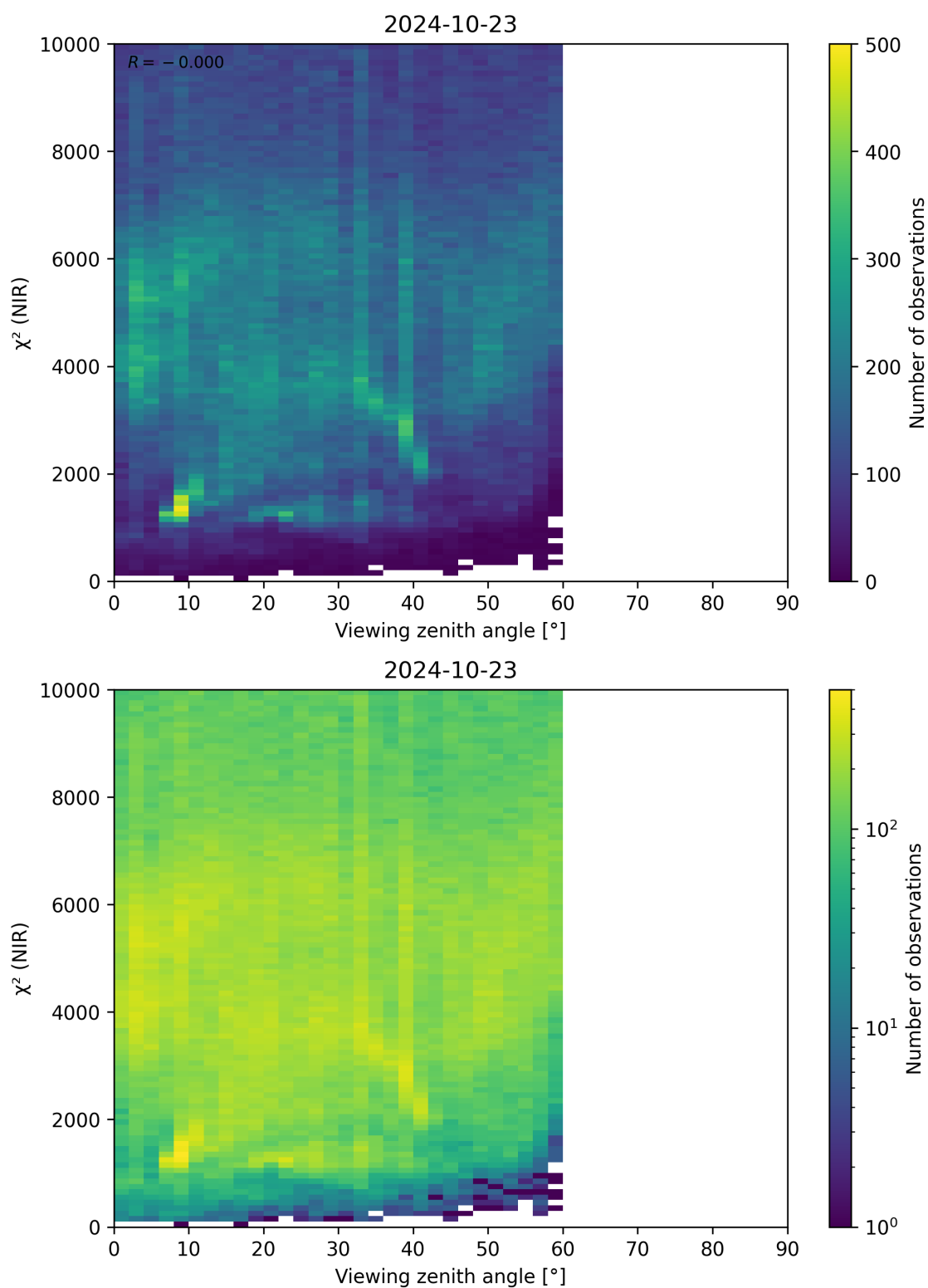
Figure 105: Scatter density plot of “Viewing zenith angle” against “ \chi^2 (NIR)” for 2024-10-22 to 2024-10-24.
