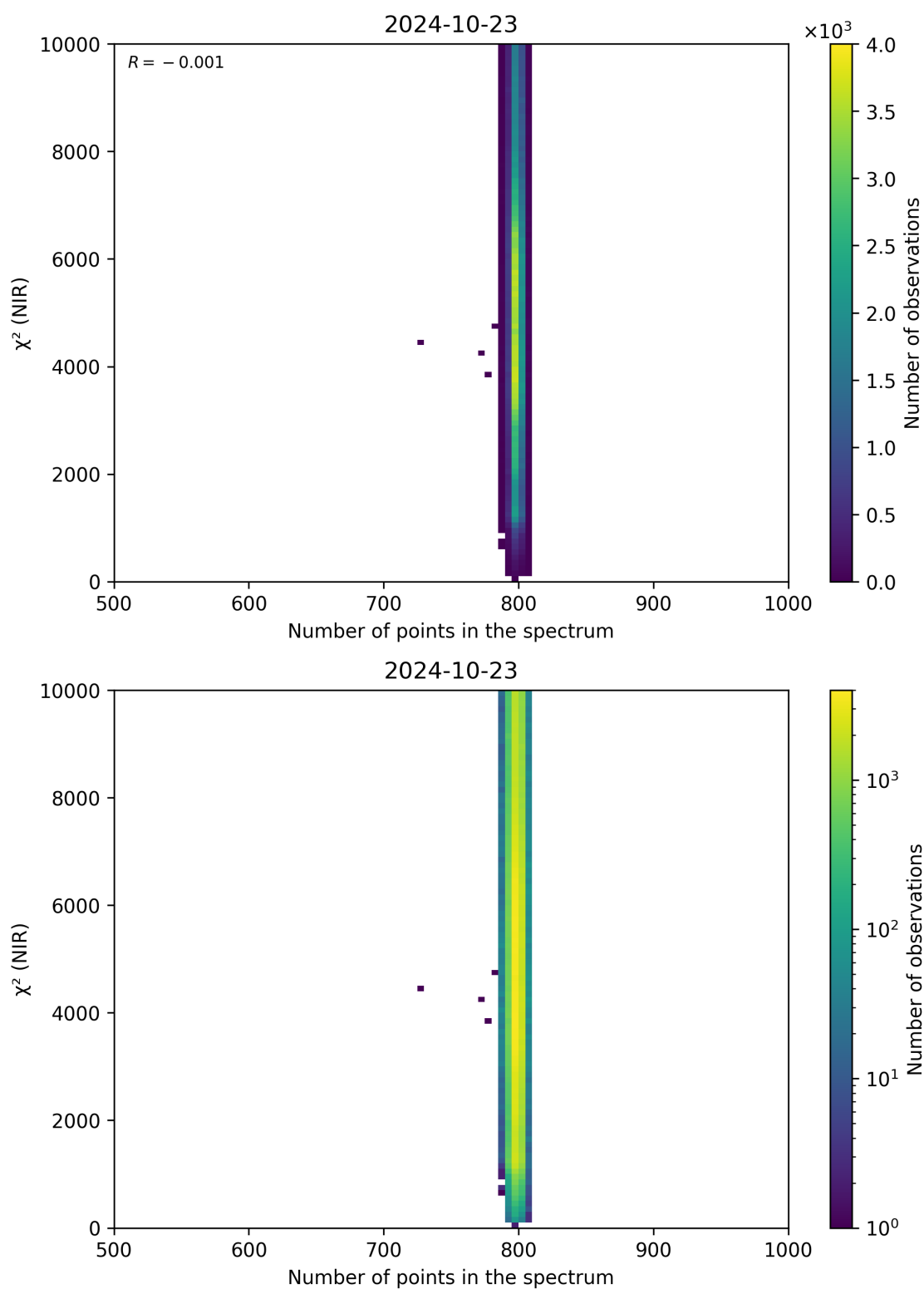
Figure 88: Scatter density plot of “Number of points in the spectrum” against “ \chi^2 (NIR)” for 2024-10-22 to 2024-10-24.
