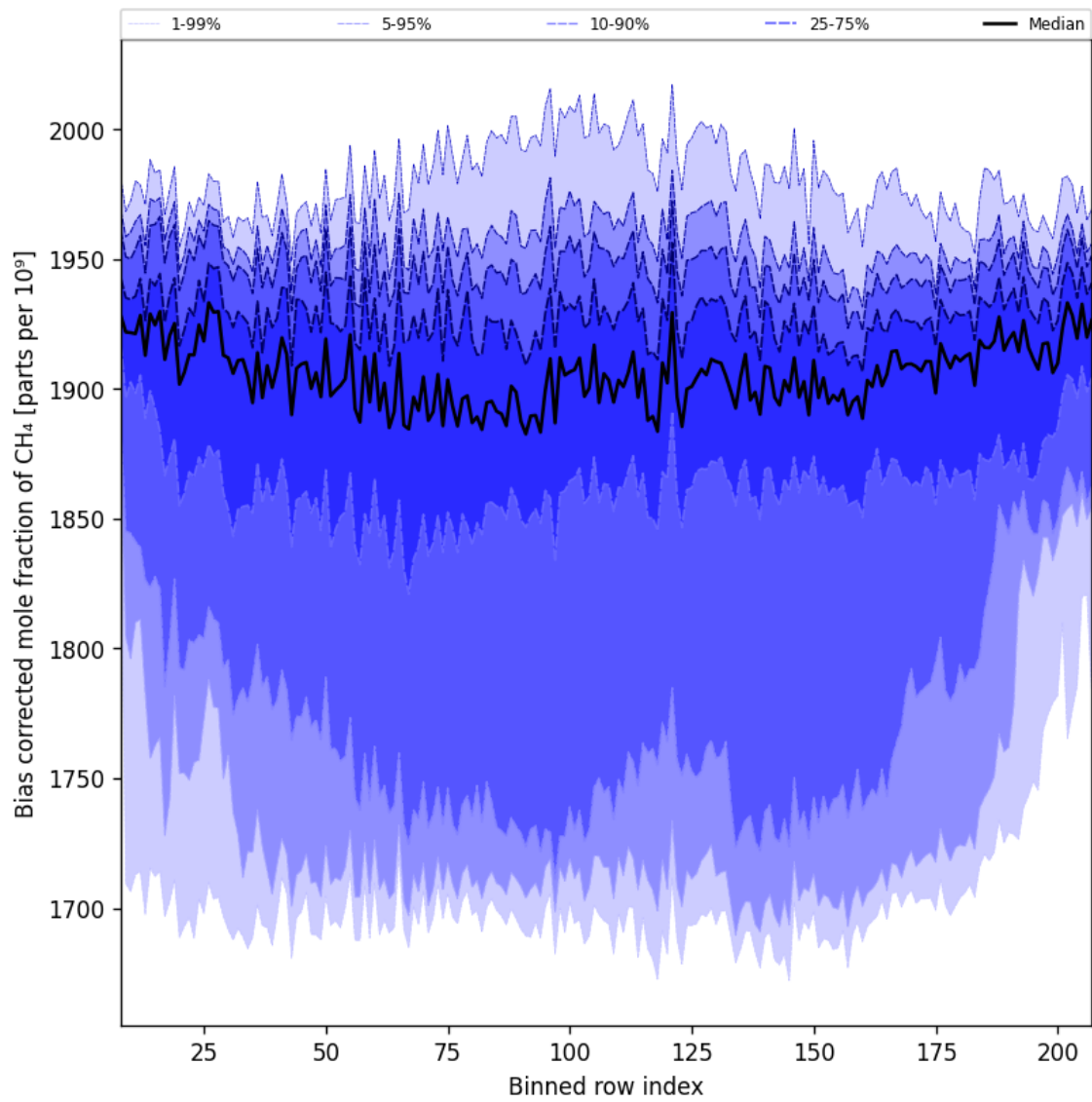
Figure 36: Along track statistics of “Bias corrected mole fraction of CH 4 ” for 2024-10-22 to 2024-10-24
