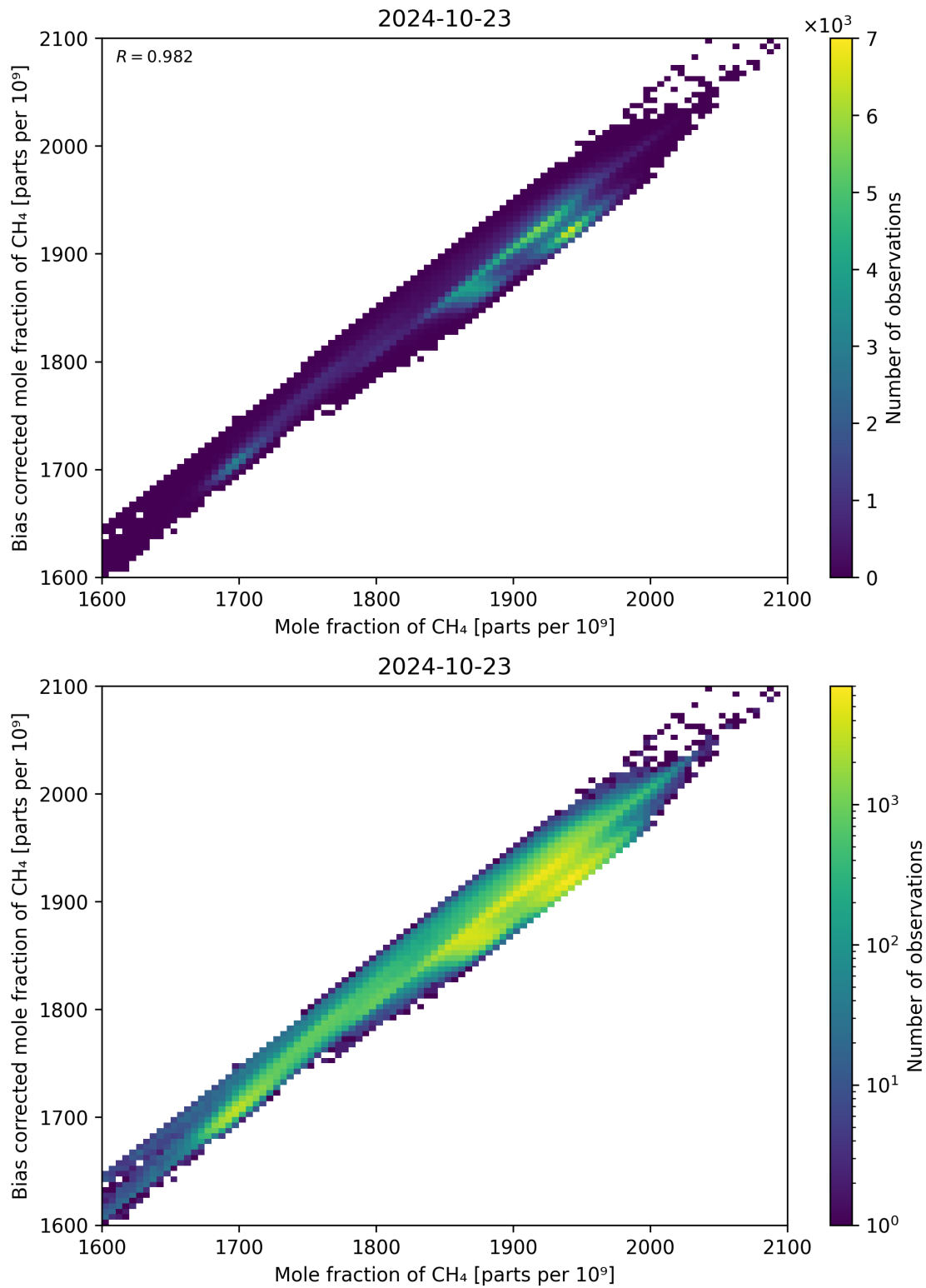
Figure 74: Scatter density plot of “Mole fraction of CH 4 ” against “Bias corrected mole fraction of CH 4 ” for 2024-10-22 to 2024-10-24.
