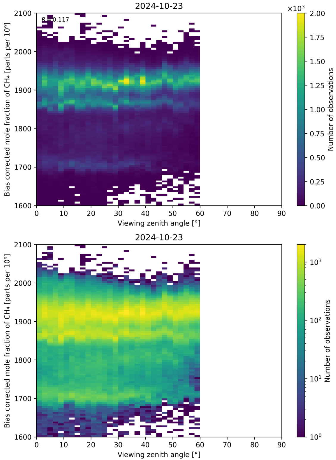
Figure 111: Scatter density plot of “Viewing zenith angle” against “Bias corrected mole fraction of CH 4 ” for 2024-10-22 to 2024-10-24.
