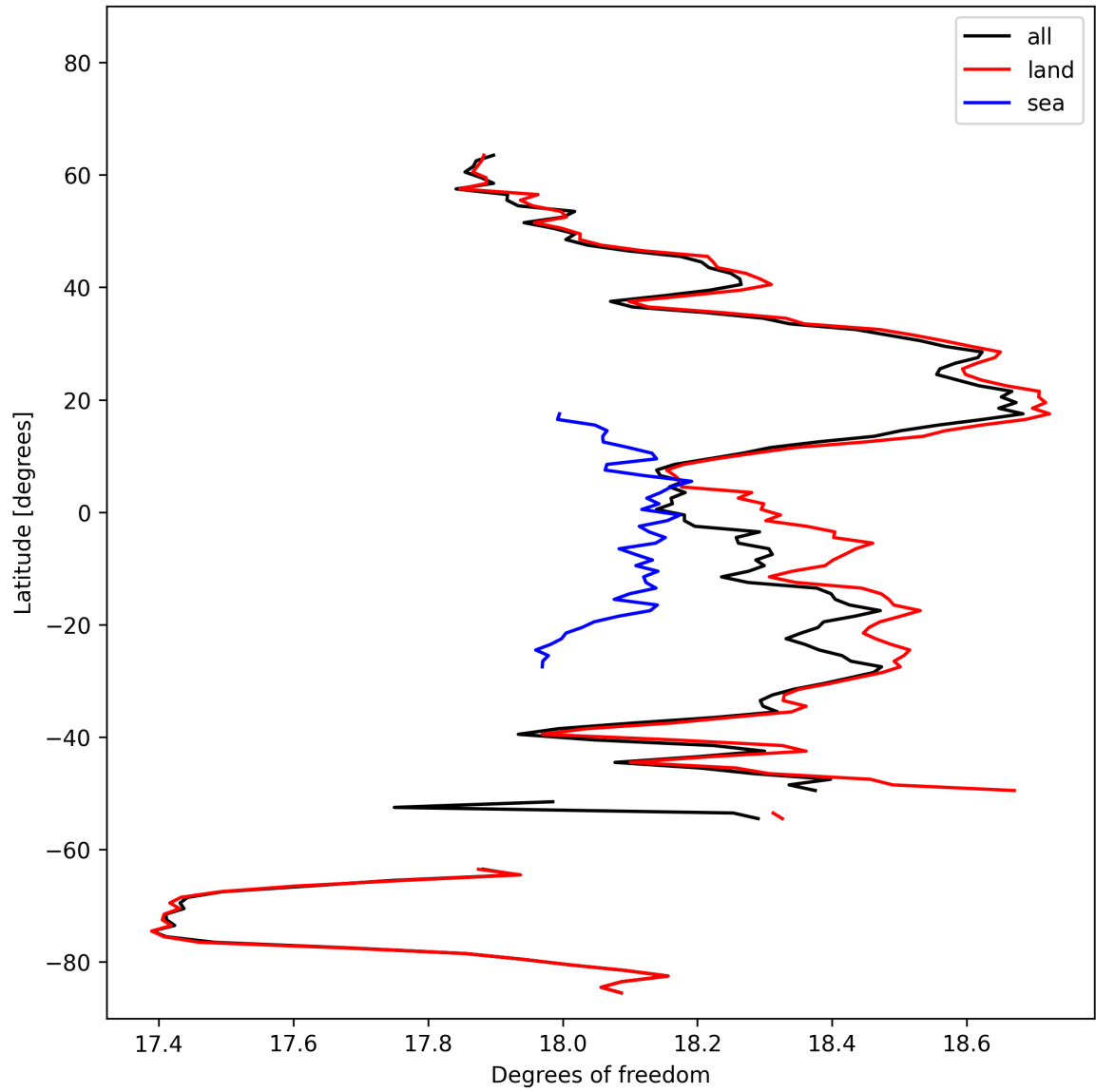
Figure 19: Zonal average of “Degrees of freedom” for 2024-10-22 to 2024-10-24.
