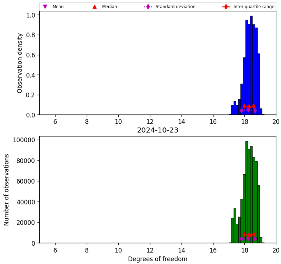
Figure 30: Histogram of “Degrees of freedom” for 2024-10-22 to 2024-10-24
