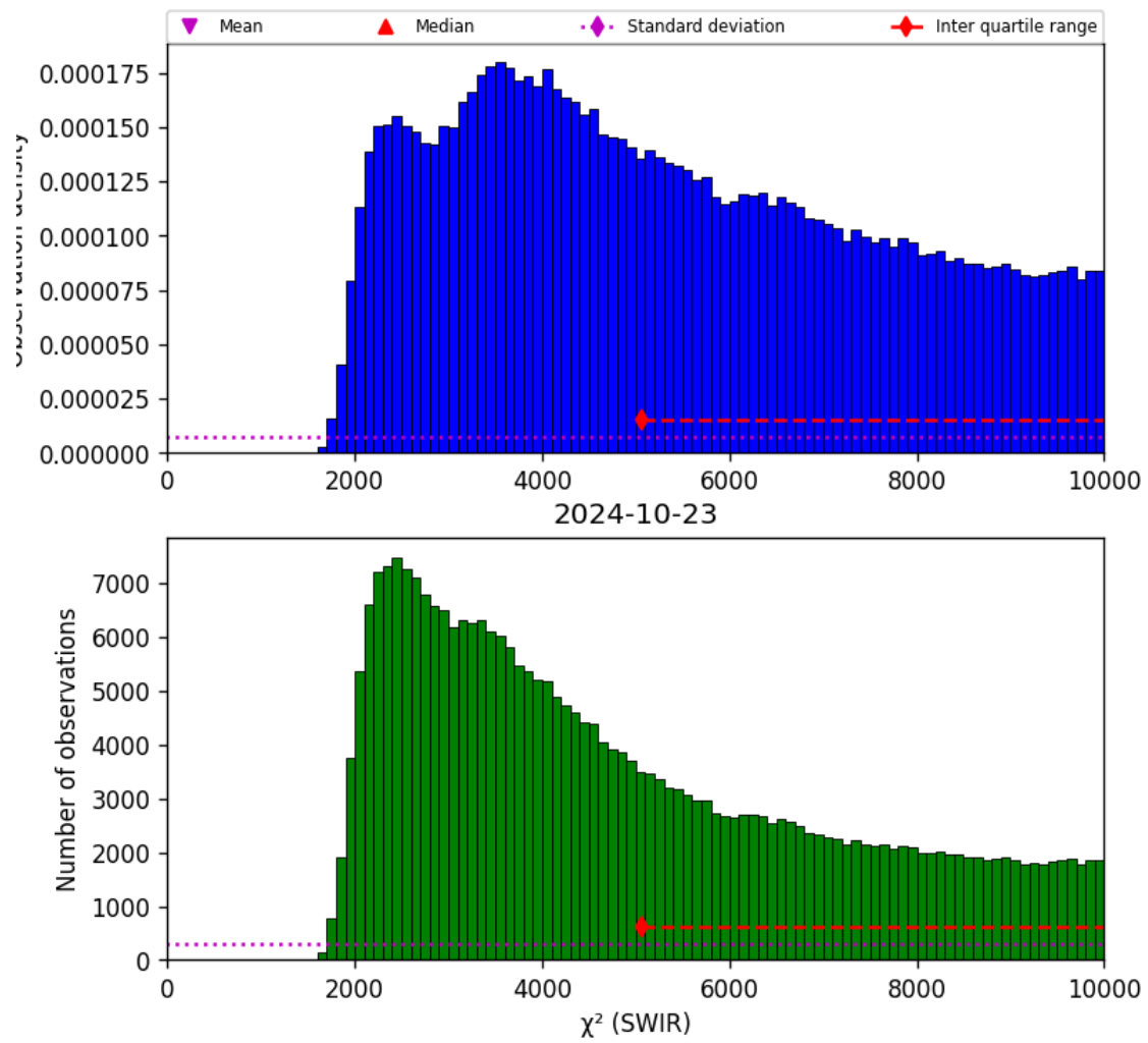
Figure 28: Histogram of “ \chi^2 (SWIR)” for 2024-10-22 to 2024-10-24
