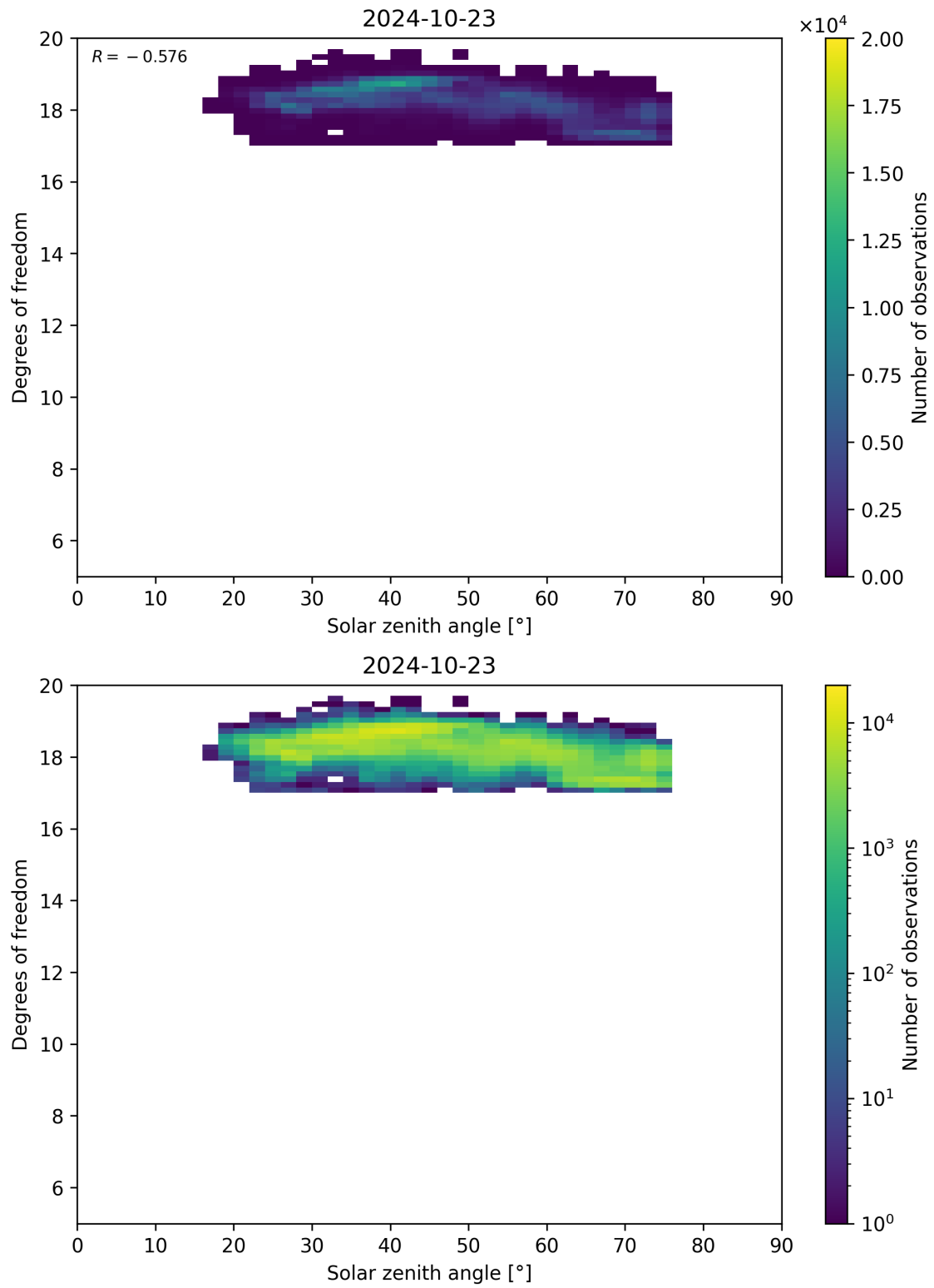
Figure 96: Scatter density plot of “Solar zenith angle” against “Degrees of freedom” for 2024-10-22 to 2024-10-24.
