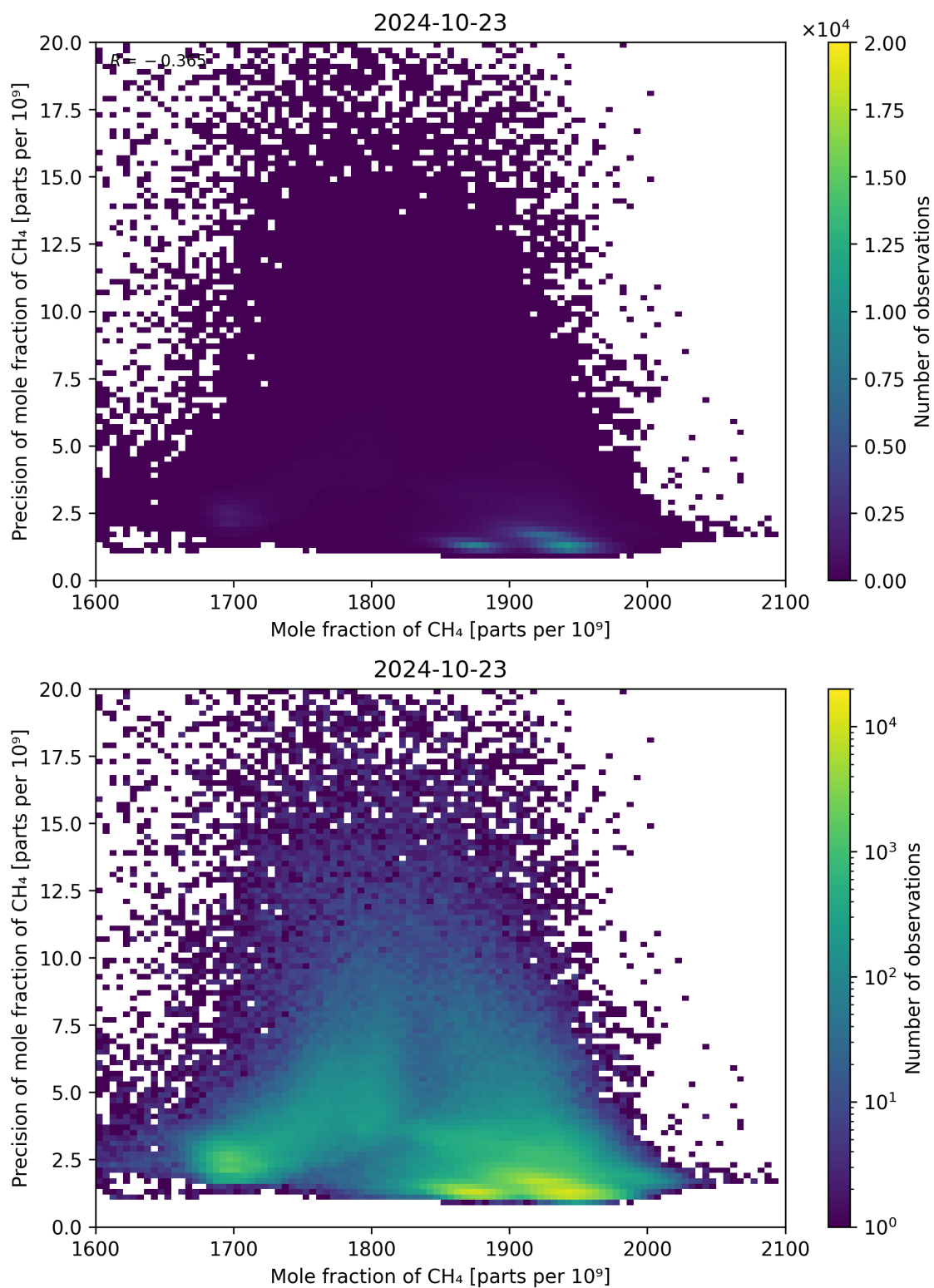
Figure 75: Scatter density plot of “Mole fraction of CH 4 ” against “Precision of mole fraction of CH 4 ” for 2024-10-22 to 2024-10-24.
