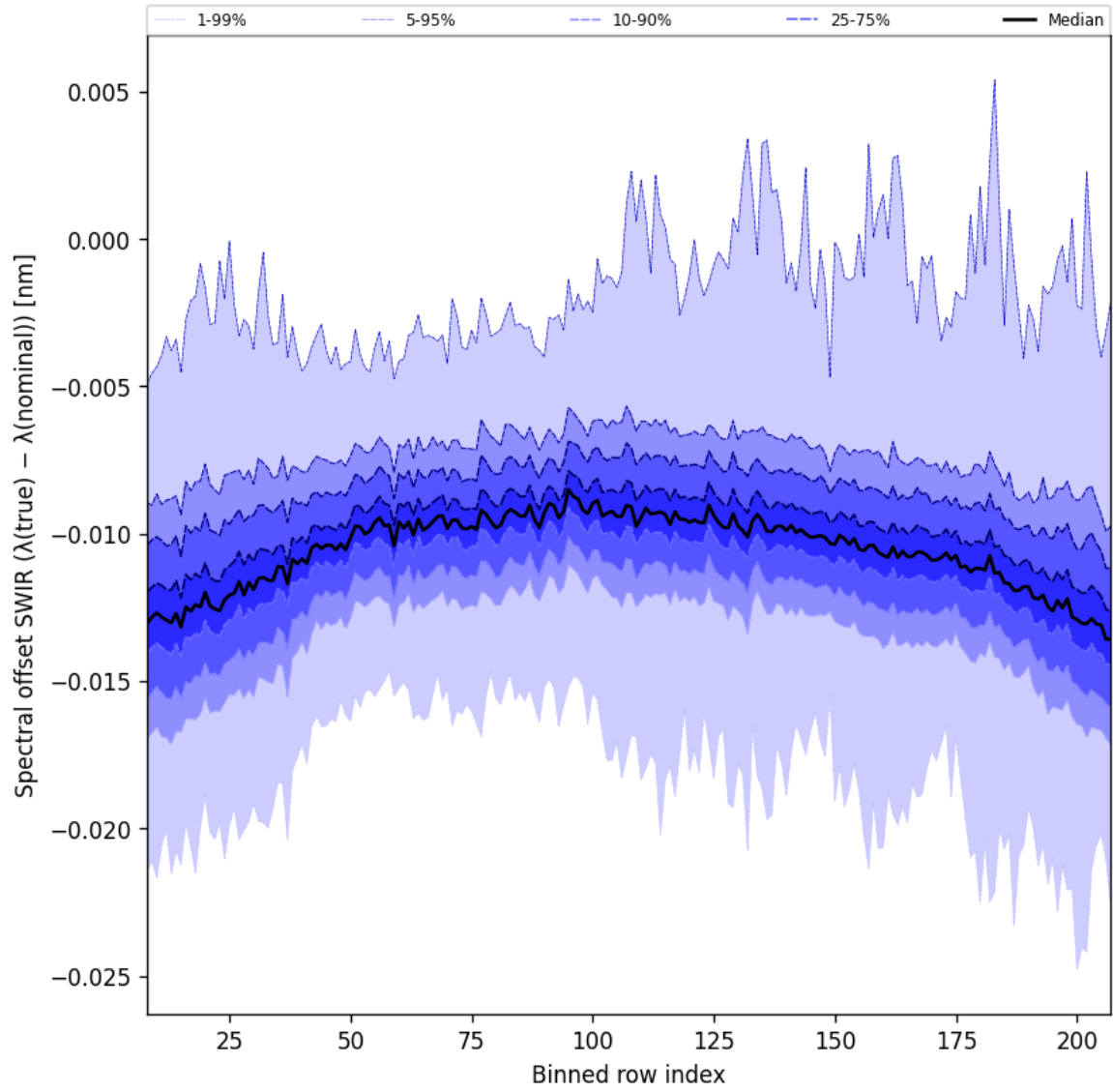
Figure 38: Along track statistics of “Spectral offset SWIR ( \lambda_{\text{true}} - \lambda_{\text{nominal}} )” for 2024-10-22 to 2024-10-24
