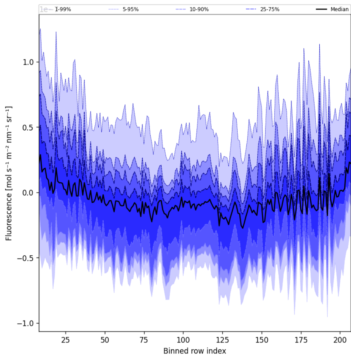
Figure 43: Along track statistics of “Fluorescence” for 2024-10-22 to 2024-10-24
