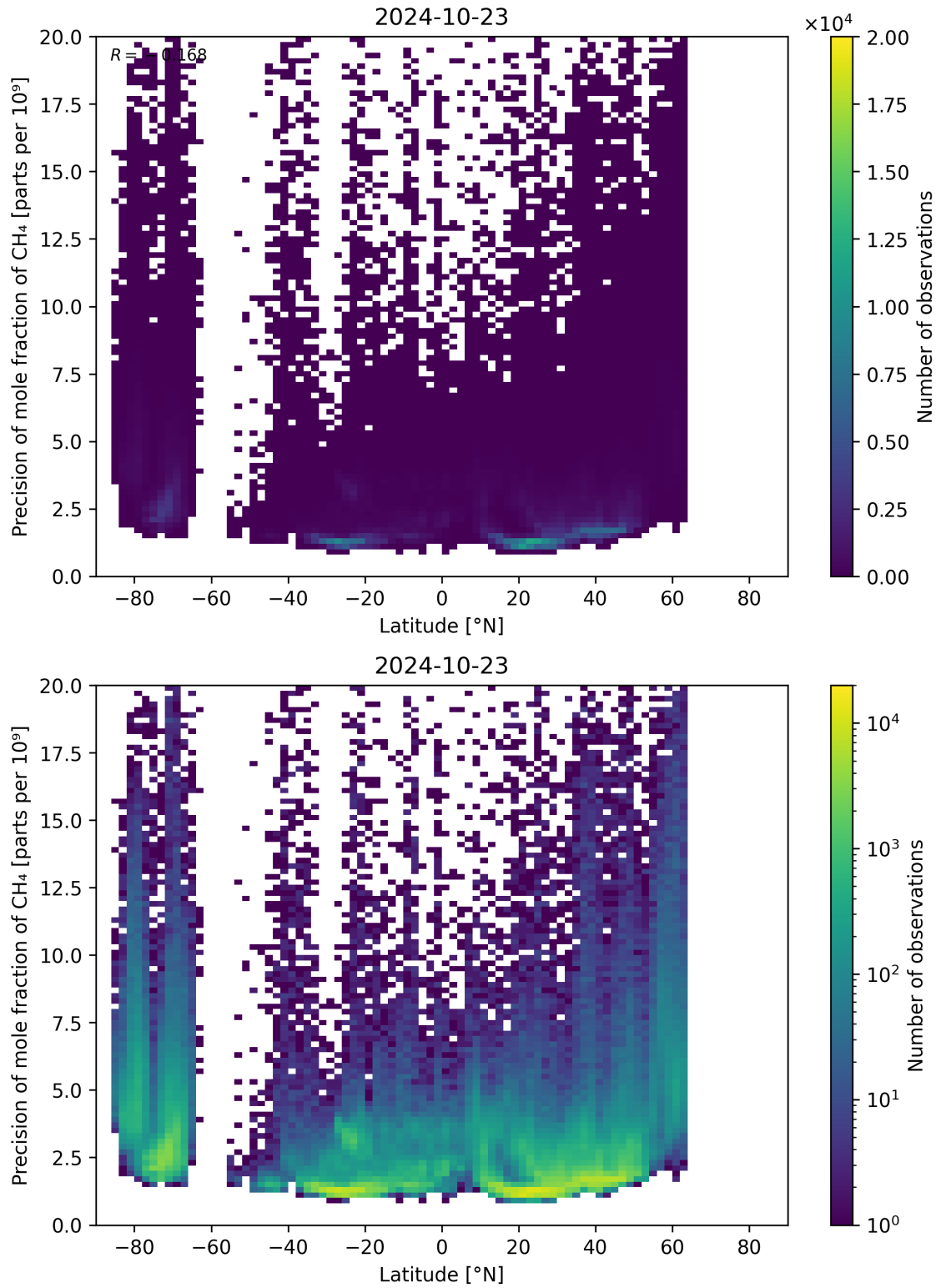
Figure 59: Scatter density plot of “Latitude” against “Precision of mole fraction of CH 4 ” for 2024-10-22 to 2024-10-24.
