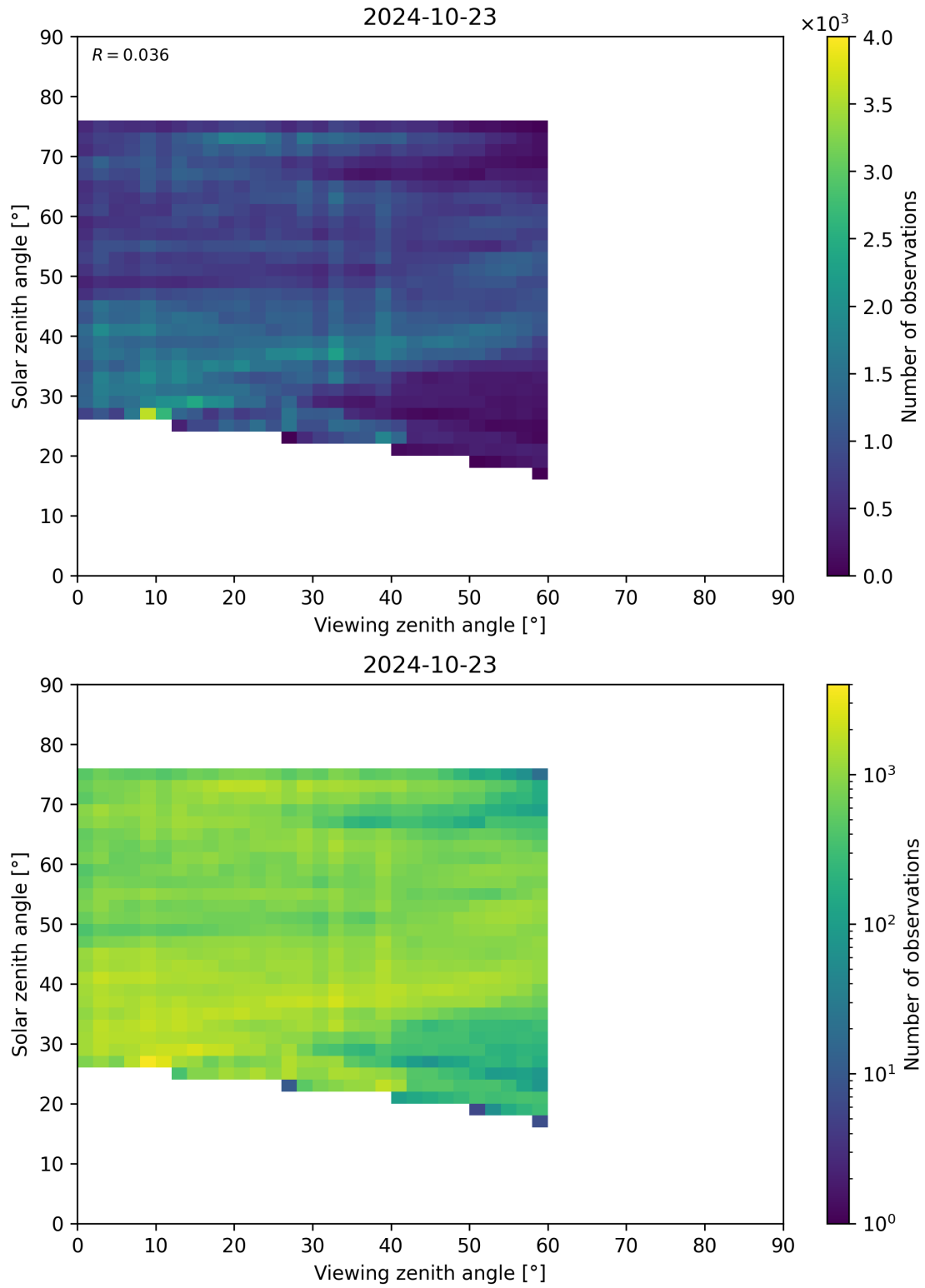
Figure 115: Scatter density plot of “Viewing zenith angle” against “Solar zenith angle” for 2024-10-22 to 2024-10-24.
