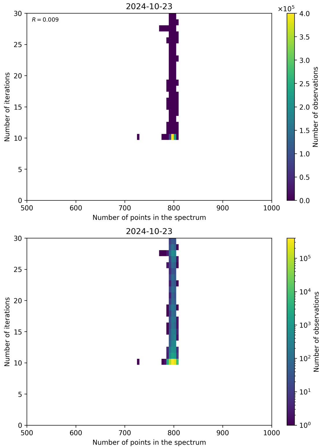
Figure 92: Scatter density plot of “Number of points in the spectrum” against “Number of iterations” for 2024-10-22 to 2024-10-24.
