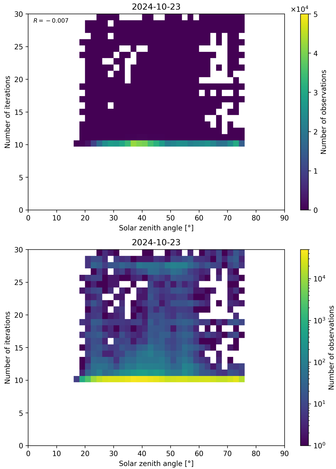
Figure 102: Scatter density plot of “Solar zenith angle” against “Number of iterations” for 2024-10-22 to 2024-10-24.
