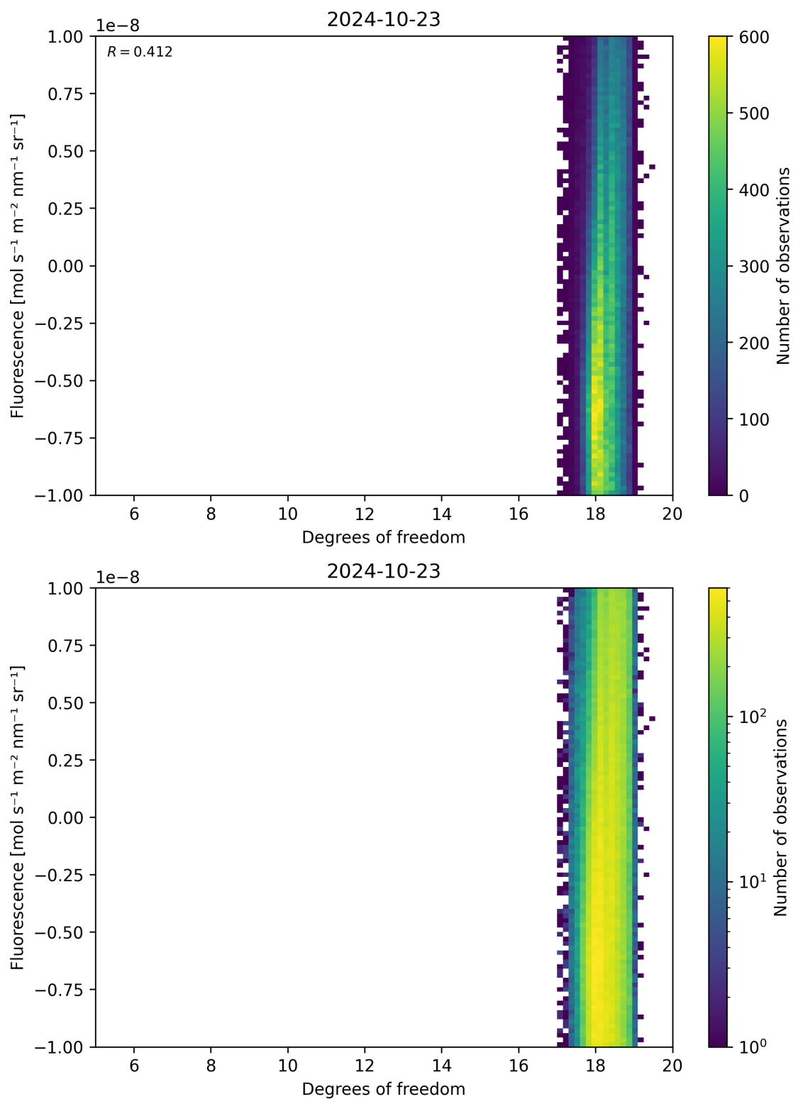
Figure 51: Scatter density plot of “Degrees of freedom” against “Fluorescence” for 2024-10-22 to 2024-10-24.
