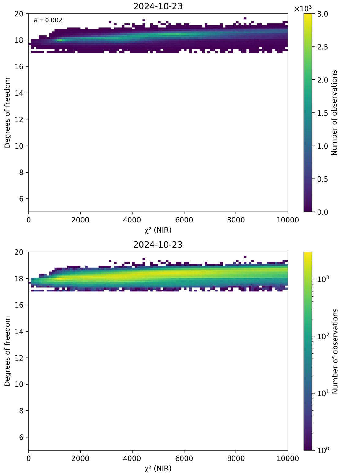
Figure 44: Scatter density plot of “ \chi^2 (NIR)” against “Degrees of freedom” for 2024-10-22 to 2024-10-24.
