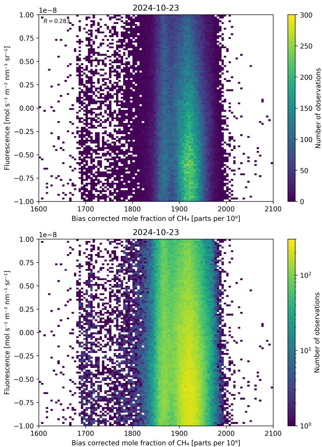
Figure 66: Scatter density plot of “Bias corrected mole fraction of \text{CH}_4 ” against “Fluorescence” for 2024-10-22 to 2024-10-24.
