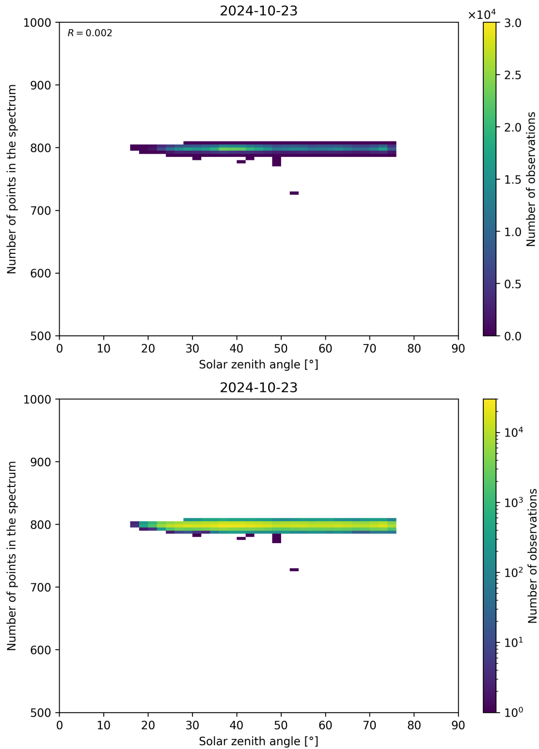
Figure 103: Scatter density plot of “Solar zenith angle” against “Number of points in the spectrum” for 2024-10-22 to 2024-10-24.
