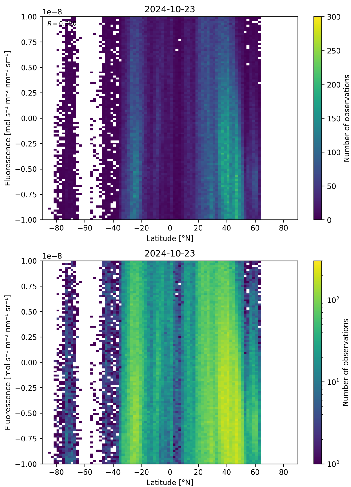
Figure 56: Scatter density plot of “Latitude” against “Fluorescence” for 2024-10-22 to 2024-10-24.
