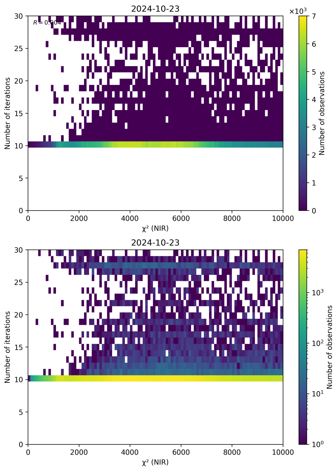
Figure 46: Scatter density plot of “ \chi^2 (NIR)” against “Number of iterations” for 2024-10-22 to 2024-10-24.
