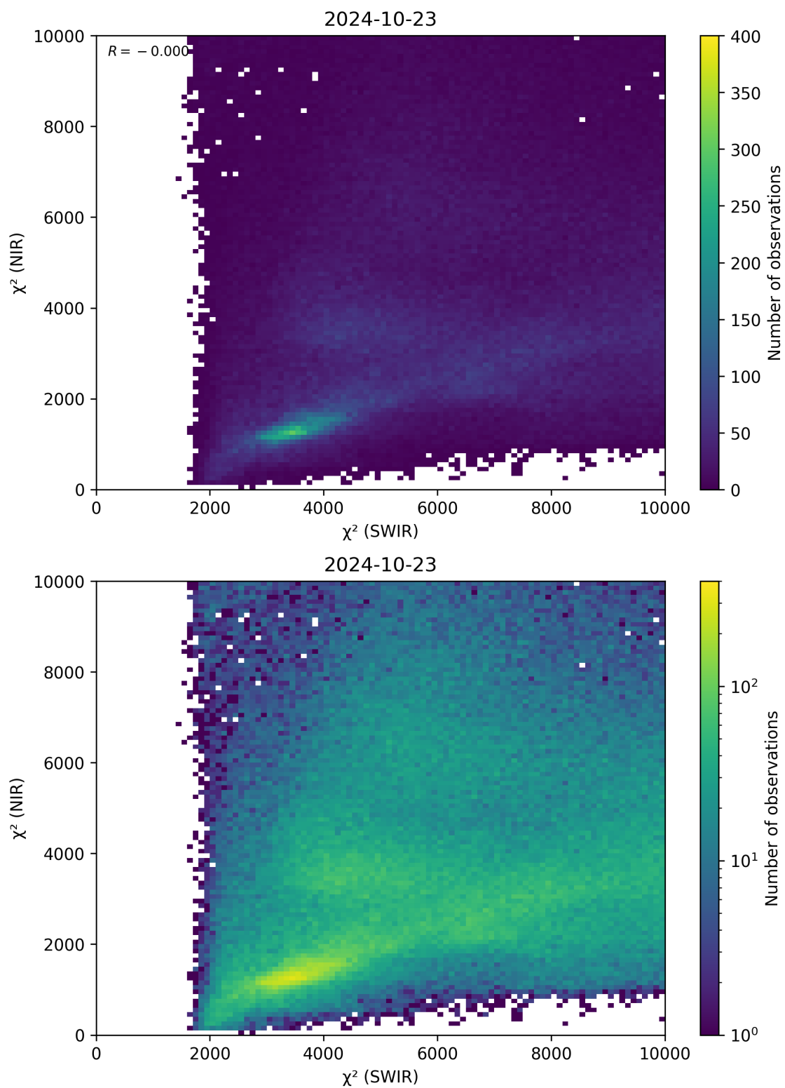
Figure 47: Scatter density plot of “ \chi^2 (SWIR)” against “ \chi^2 (NIR)” for 2024-10-22 to 2024-10-24.
