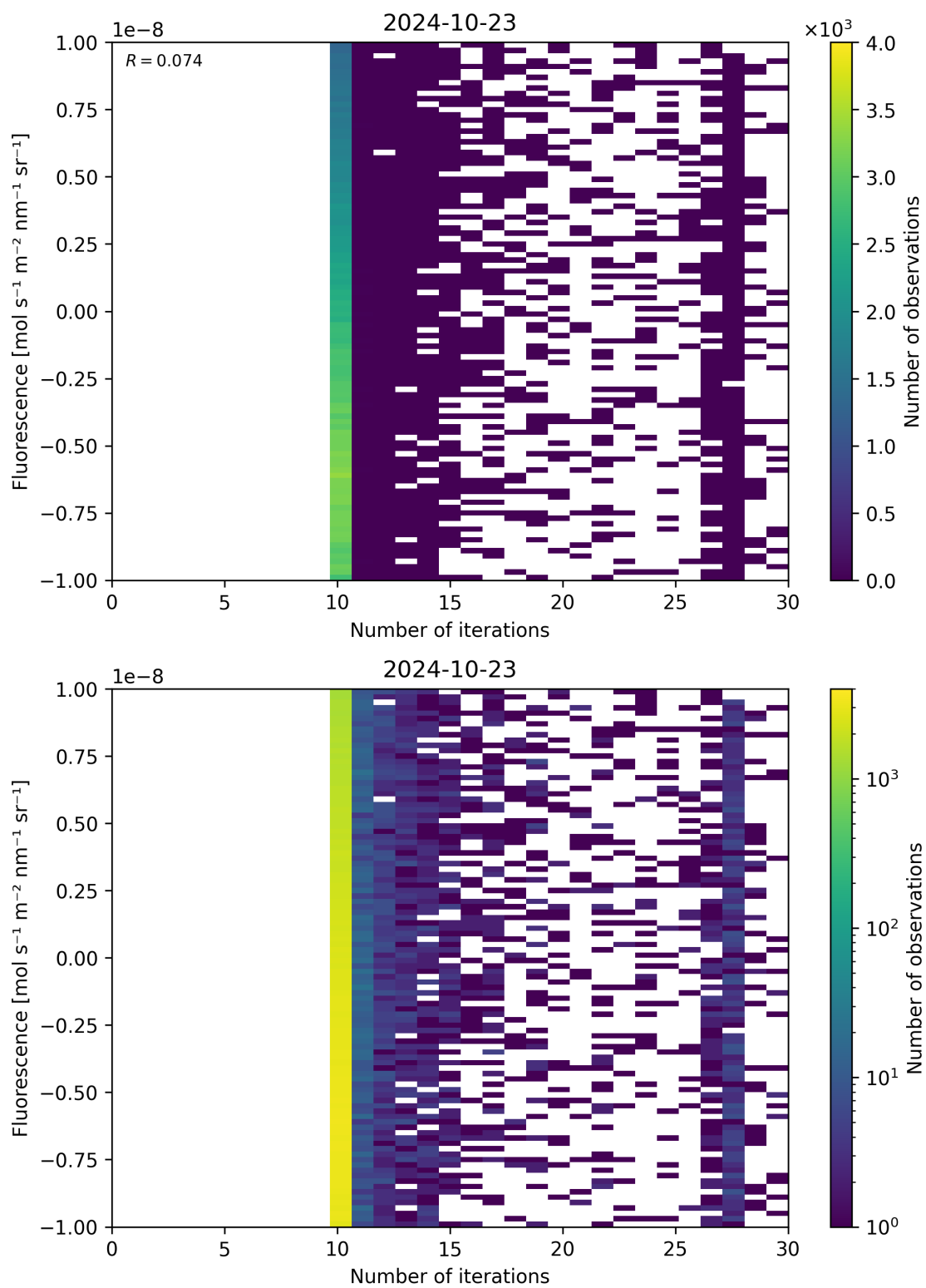
Figure 87: Scatter density plot of “Number of iterations” against “Fluorescence” for 2024-10-22 to 2024-10-24.
