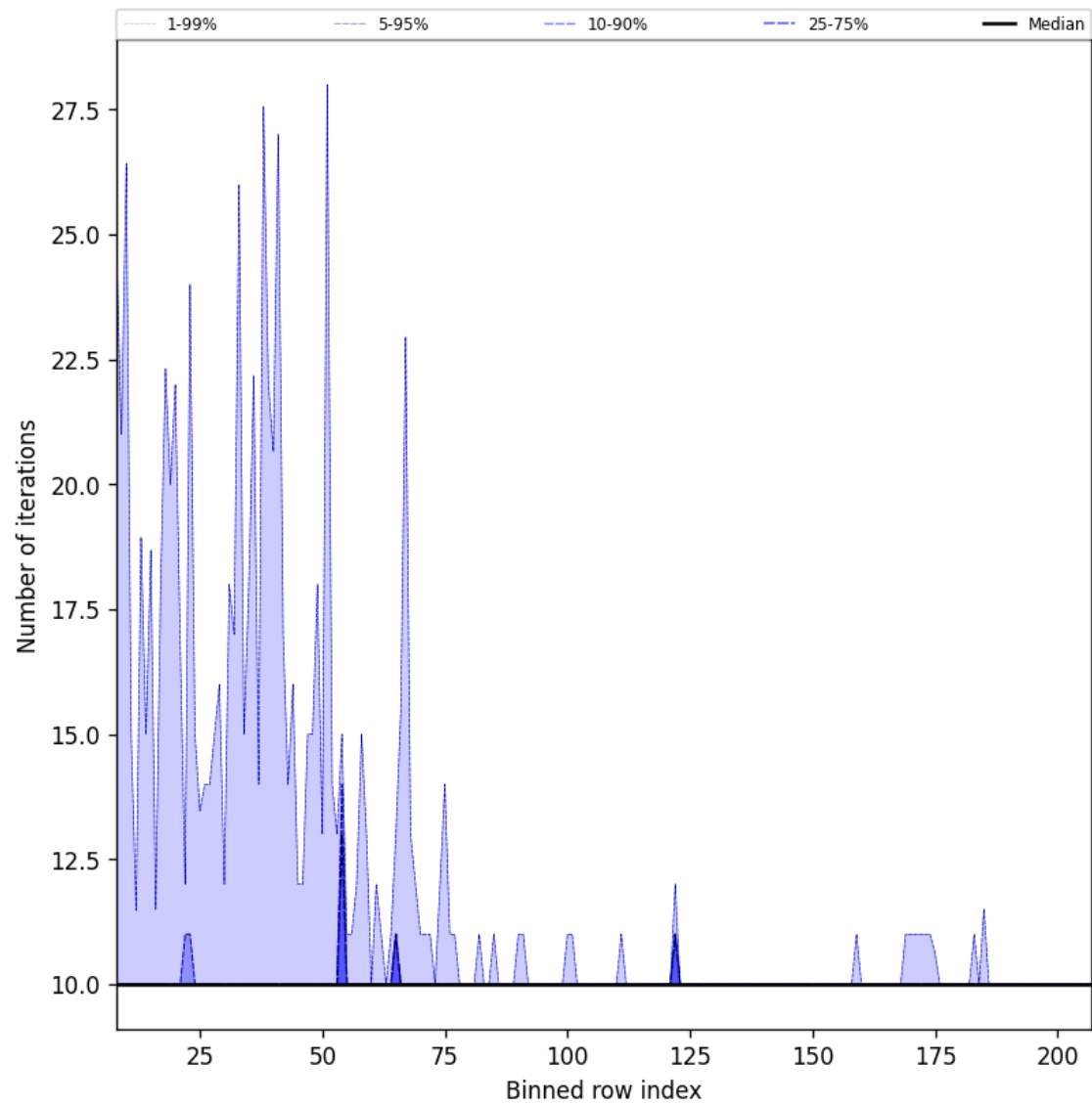
Figure 42: Along track statistics of “Number of iterations” for 2024-10-22 to 2024-10-24
