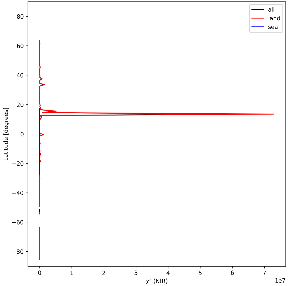
Figure 18: Zonal average of “ \chi^2 (NIR)” for 2024-10-22 to 2024-10-24.
