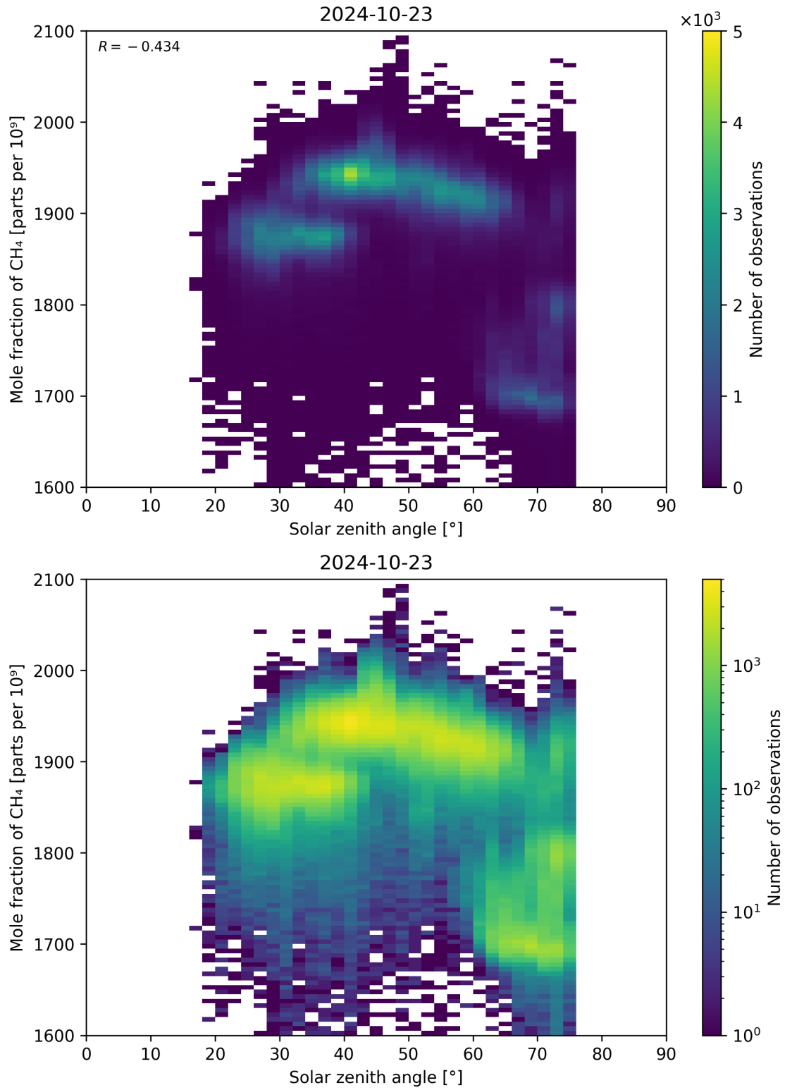
Figure 99: Scatter density plot of “Solar zenith angle” against “Mole fraction of \text{CH}_4 ” for 2024-10-22 to 2024-10-24.
