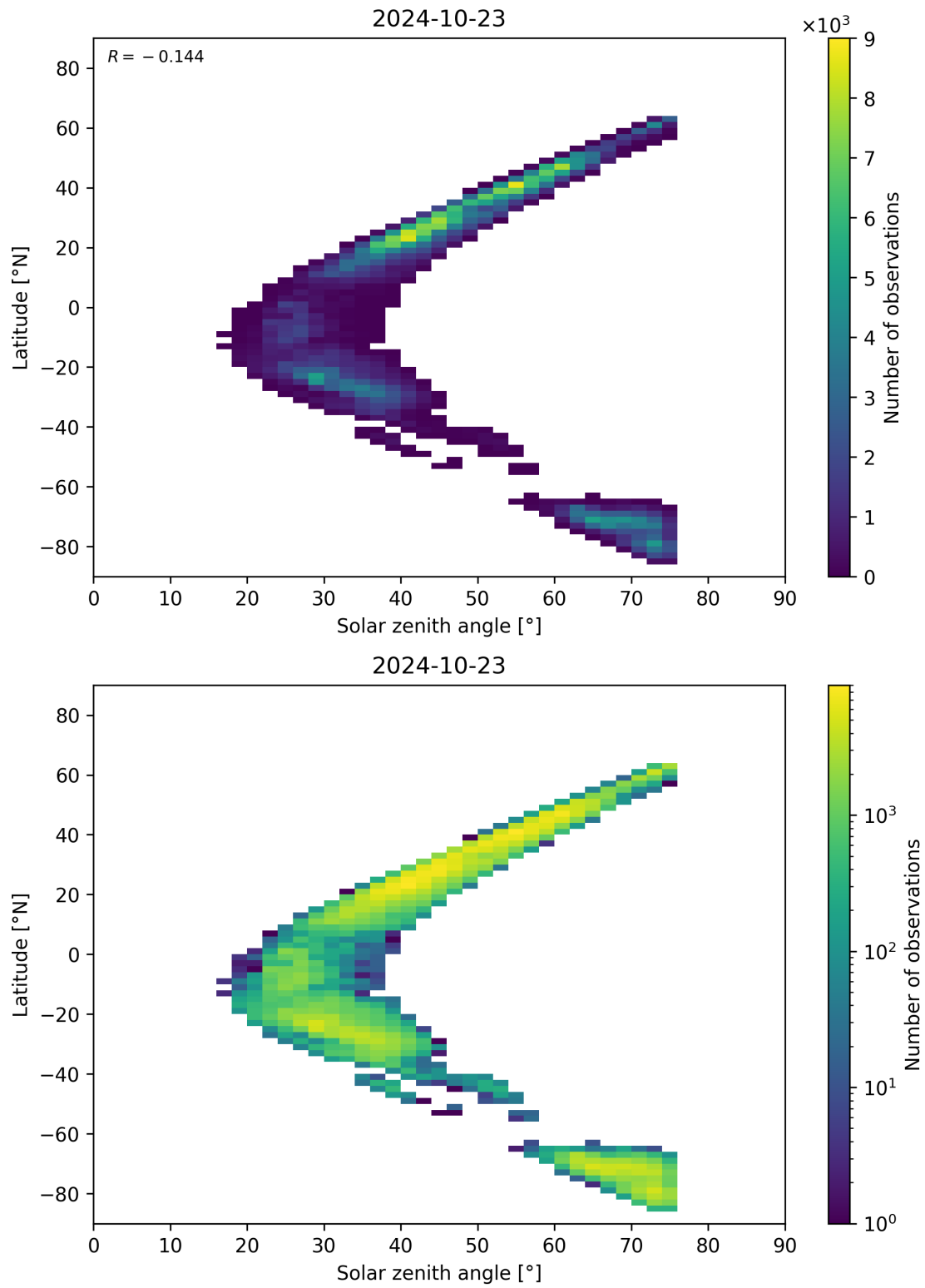
Figure 98: Scatter density plot of “Solar zenith angle” against “Latitude” for 2024-10-22 to 2024-10-24.
