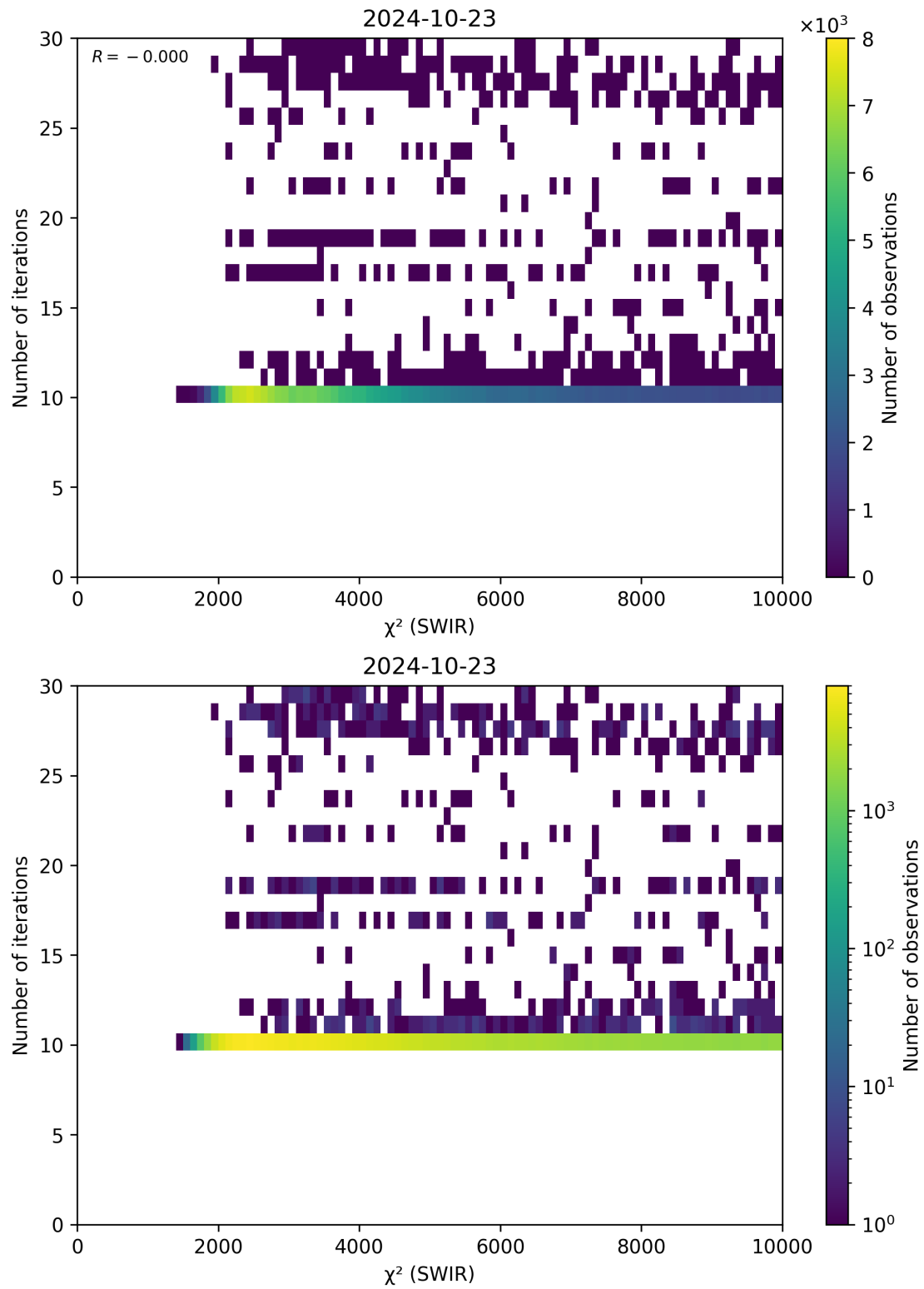
Figure 50: Scatter density plot of “ \chi^2 (SWIR)” against “Number of iterations” for 2024-10-22 to 2024-10-24.
