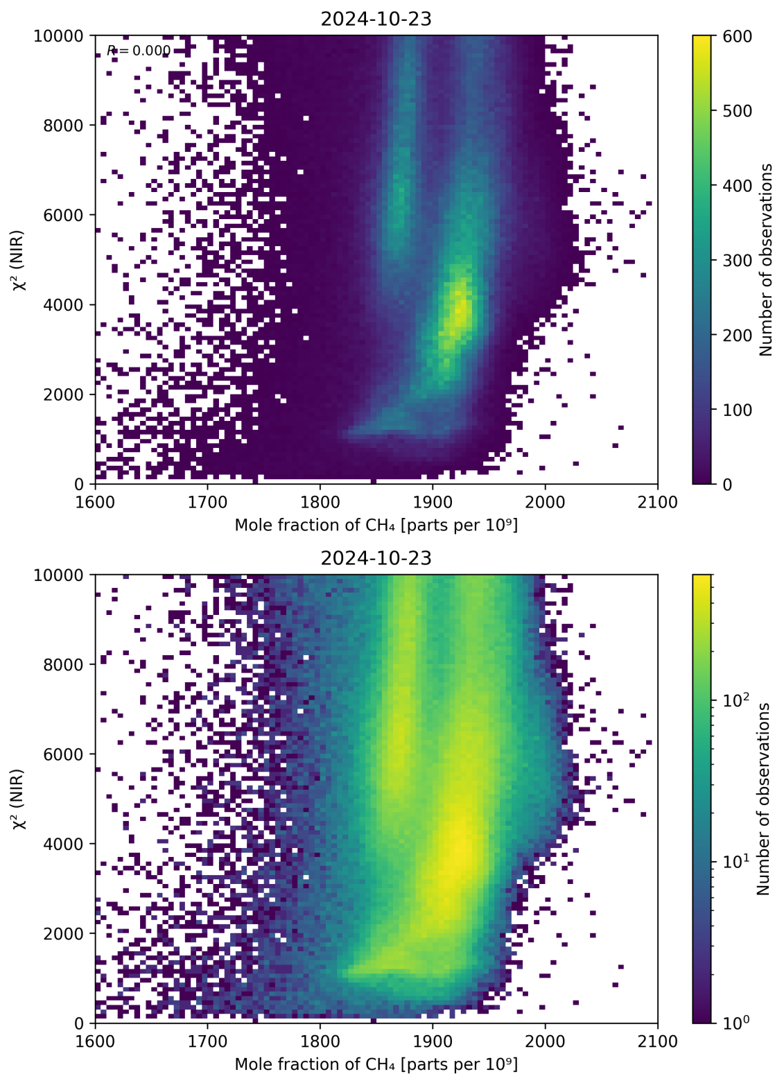
Figure 70: Scatter density plot of “Mole fraction of \text{CH}_4 ” against “ \chi^2 (NIR)” for 2024-10-22 to 2024-10-24.
