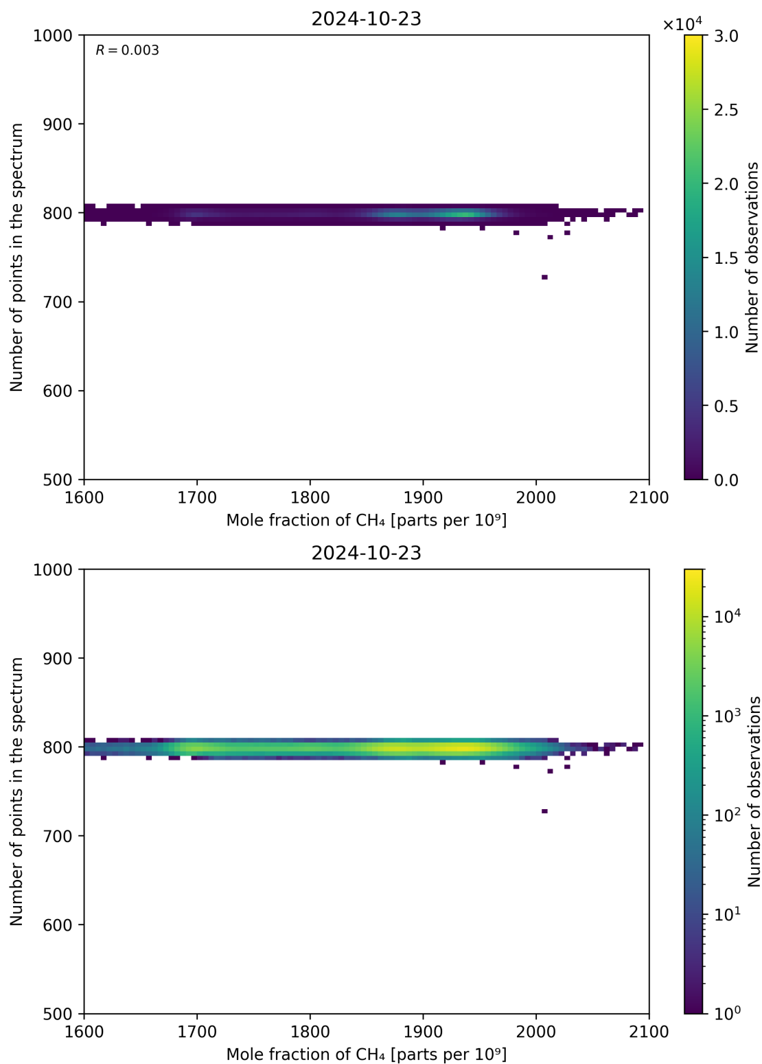
Figure 77: Scatter density plot of “Mole fraction of CH 4 ” against “Number of points in the spectrum” for 2024-10-22 to 2024-10-24.
