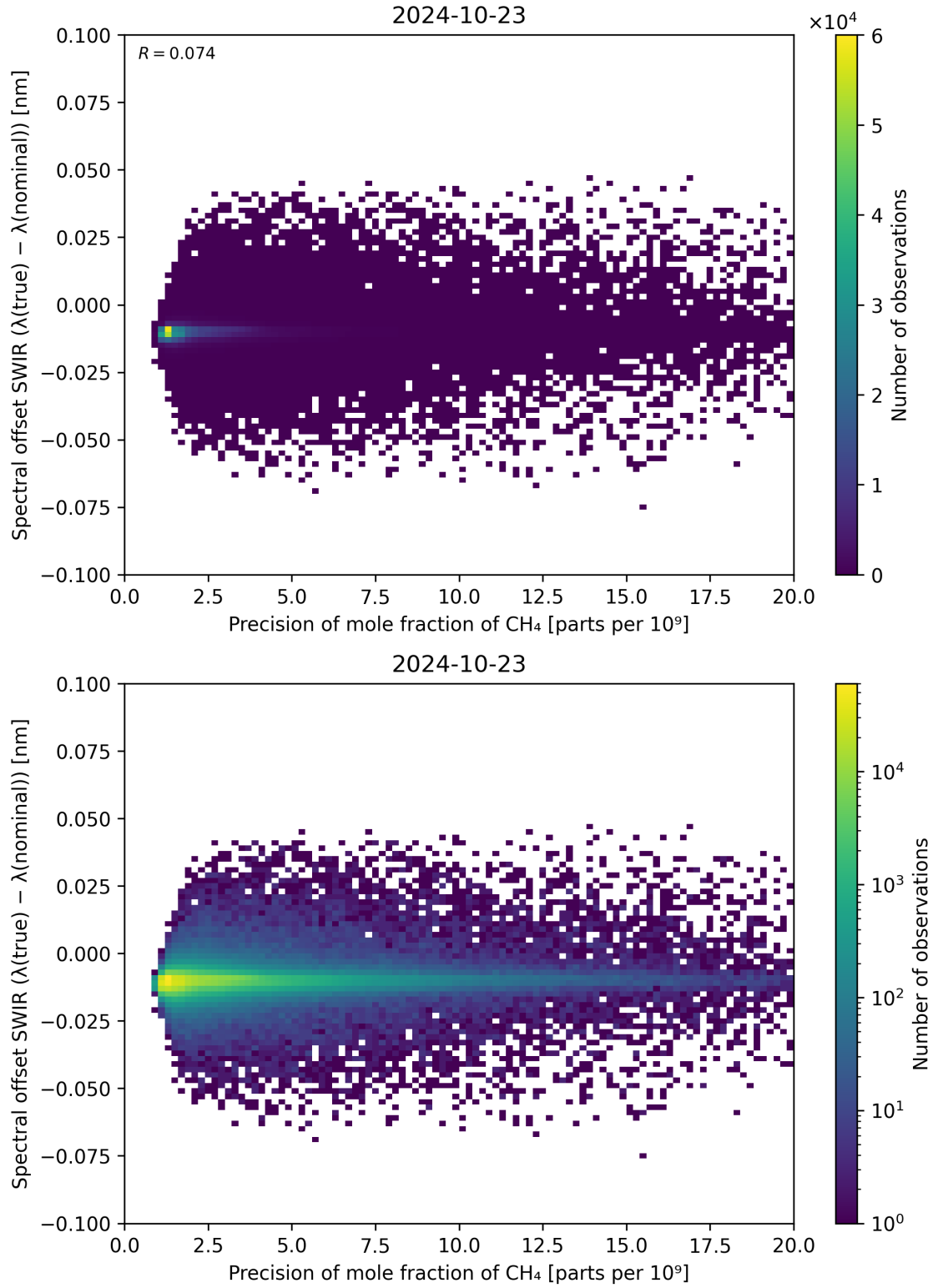
Figure 85: Scatter density plot of “Precision of mole fraction of CH 4 ” against “Spectral offset SWIR ( \lambda_{\text{true}} - \lambda_{\text{nominal}} )” for 2024-10-22 to 2024-10-24.
