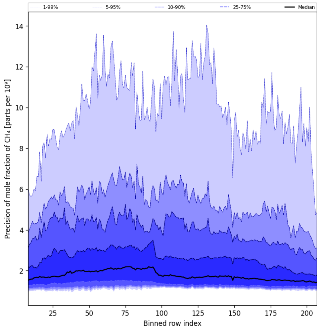
Figure 35: Along track statistics of “Precision of mole fraction of CH 4 ” for 2024-10-22 to 2024-10-24
