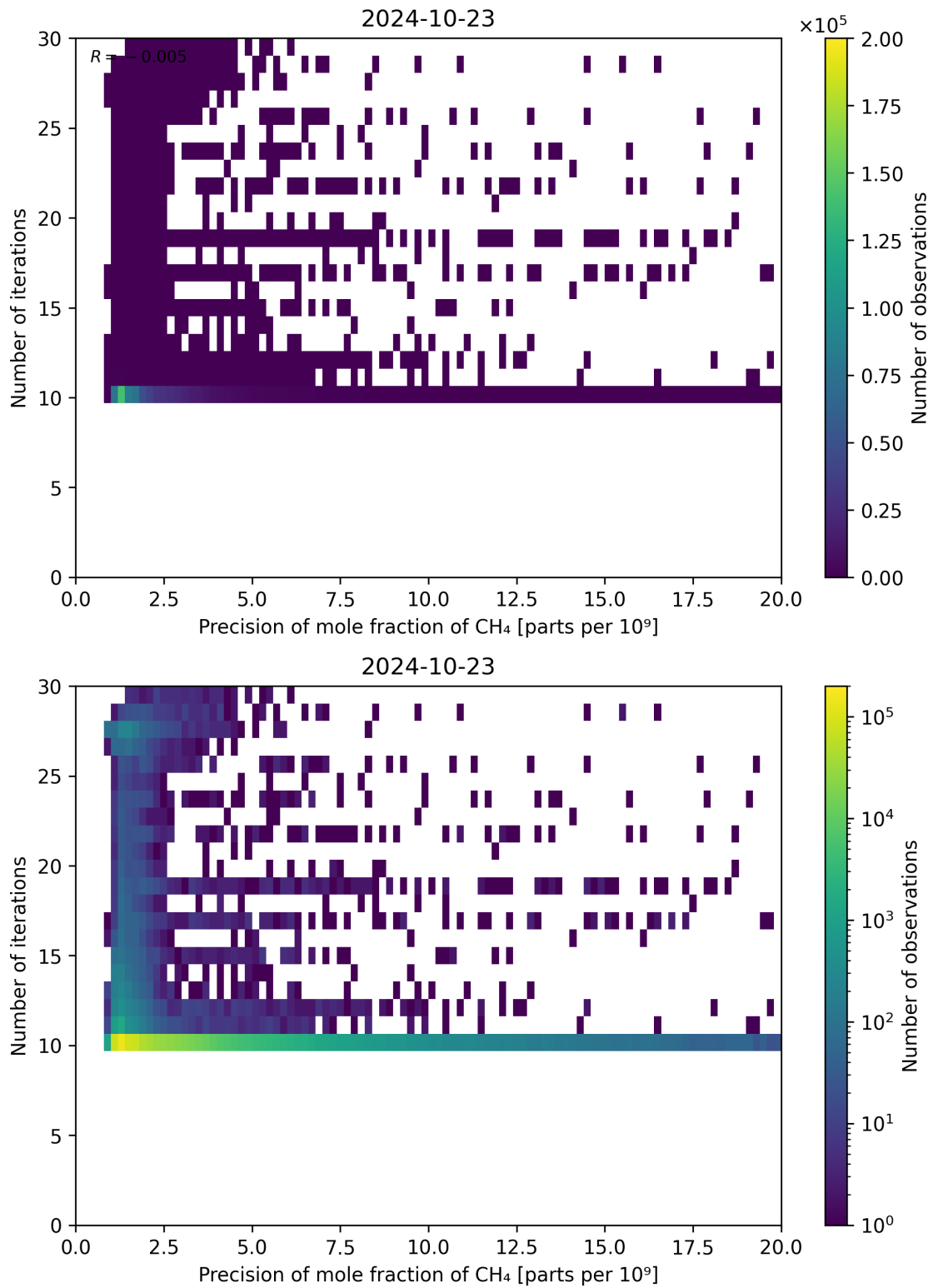
Figure 83: Scatter density plot of “Precision of mole fraction of CH 4 ” against “Number of iterations” for 2024-10-22 to 2024-10-24.
