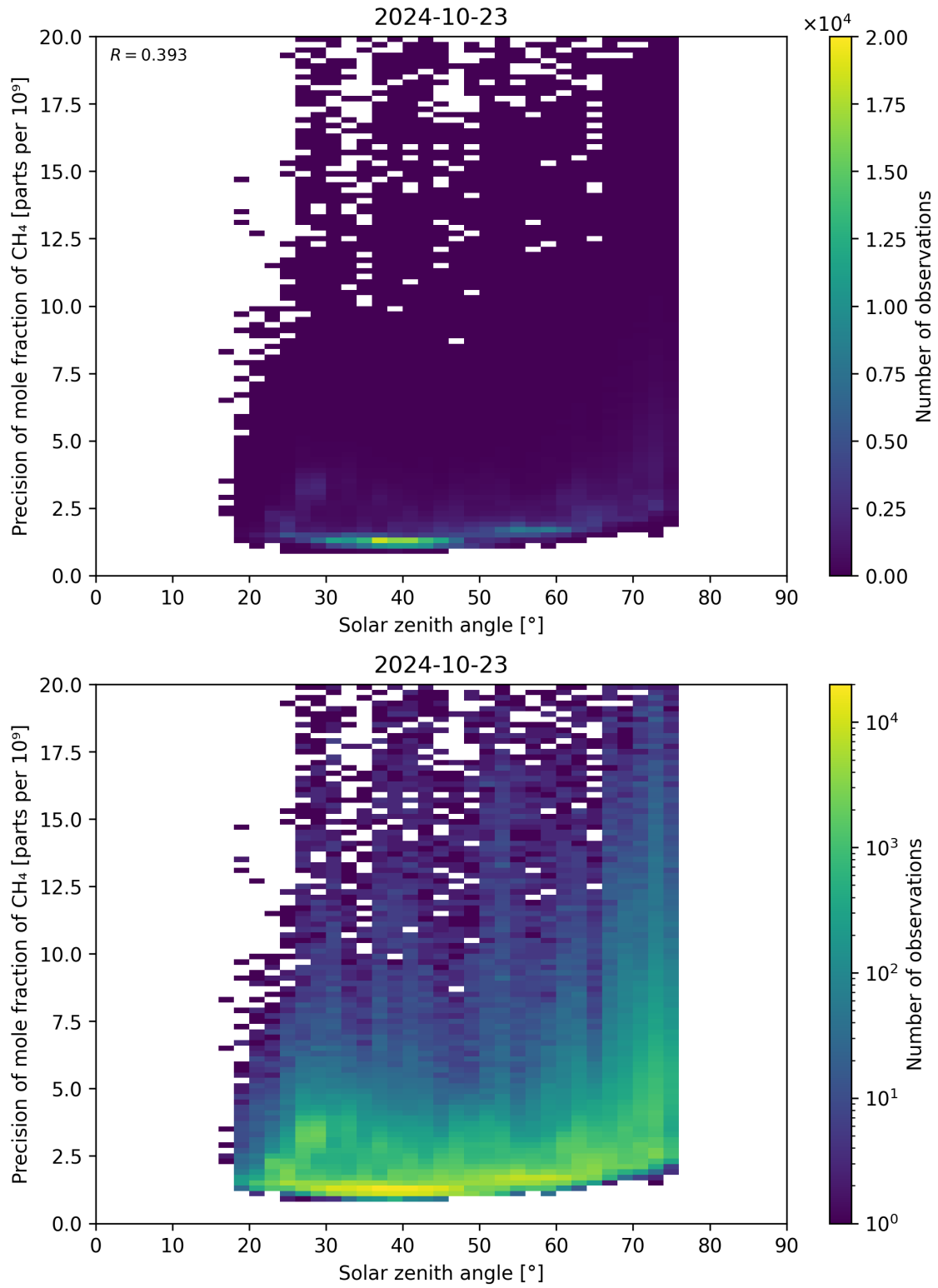
Figure 101: Scatter density plot of “Solar zenith angle” against “Precision of mole fraction of CH 4 ” for 2024-10-22 to 2024-10-24.
