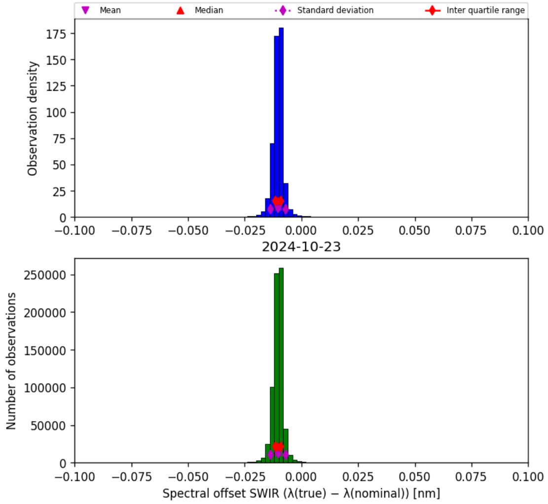
Figure 27: Histogram of “Spectral offset SWIR ( \lambda_{\text{true}} - \lambda_{\text{nominal}} )” for 2024-10-22 to 2024-10-24
