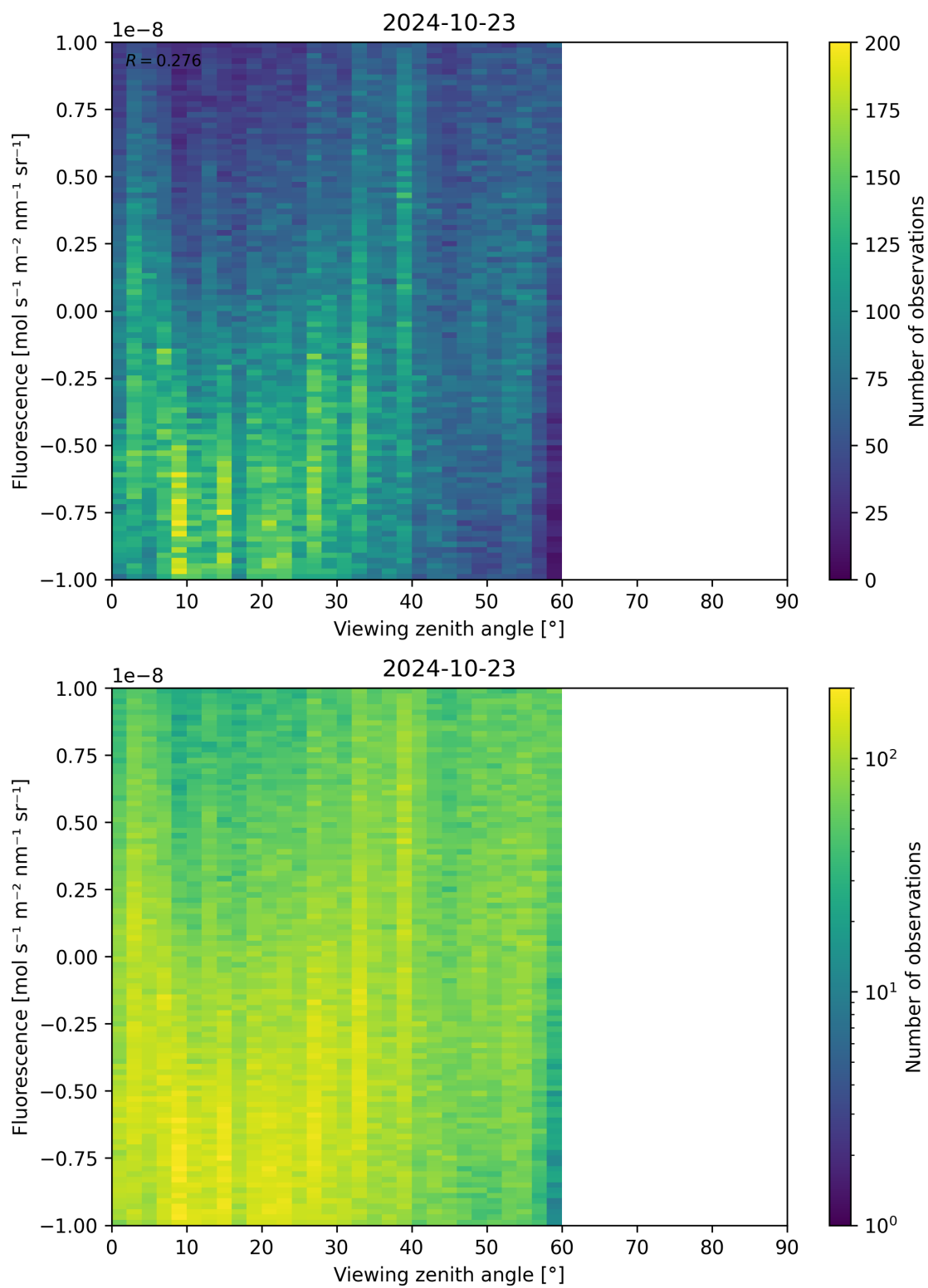
Figure 108: Scatter density plot of “Viewing zenith angle” against “Fluorescence” for 2024-10-22 to 2024-10-24.
