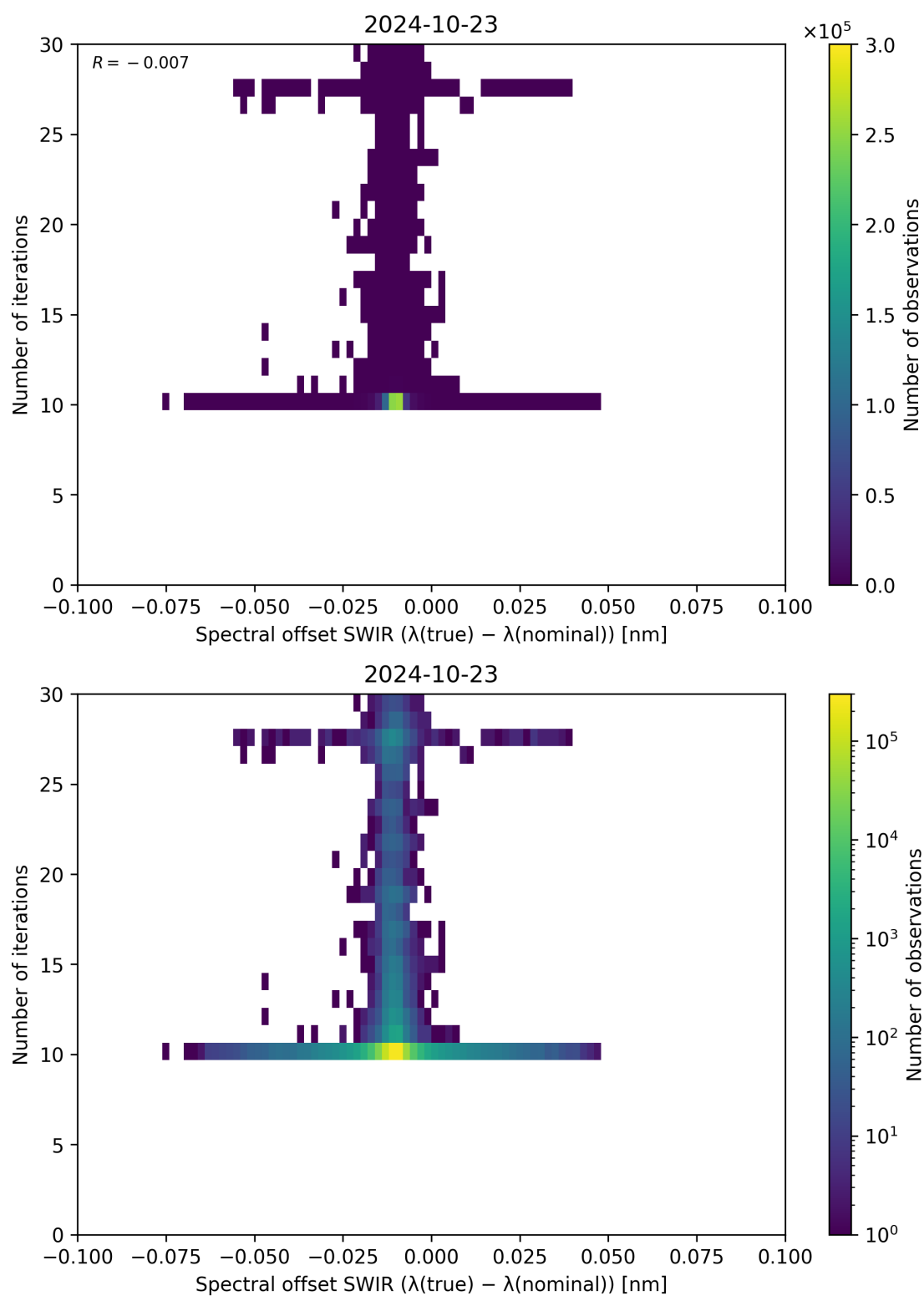
Figure 121: Scatter density plot of “Spectral offset SWIR ( \lambda_{\text{true}} - \lambda_{\text{nominal}} )” against “Number of iterations” for 2024-10-22 to 2024-10-24.
