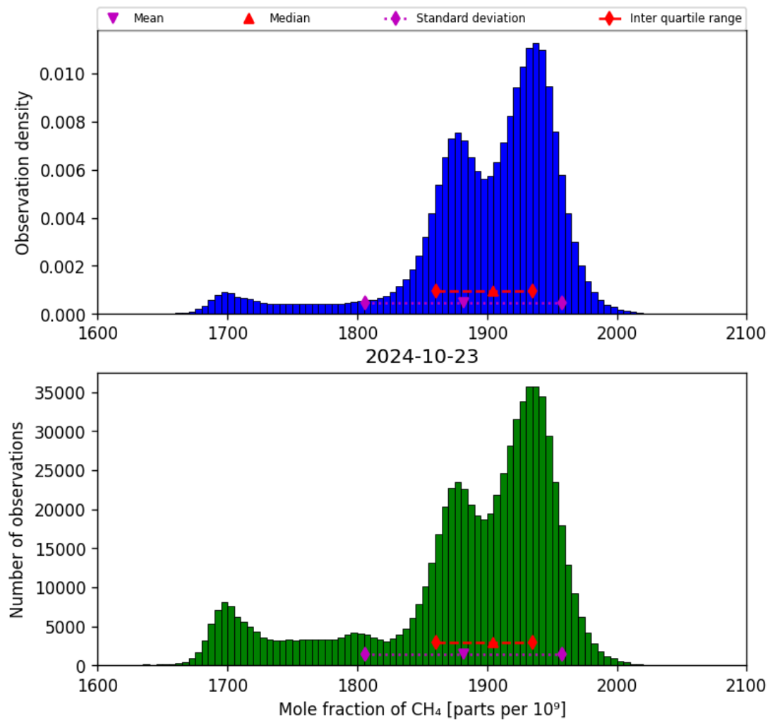
Figure 23: Histogram of “Mole fraction of CH 4 ” for 2024-10-22 to 2024-10-24
