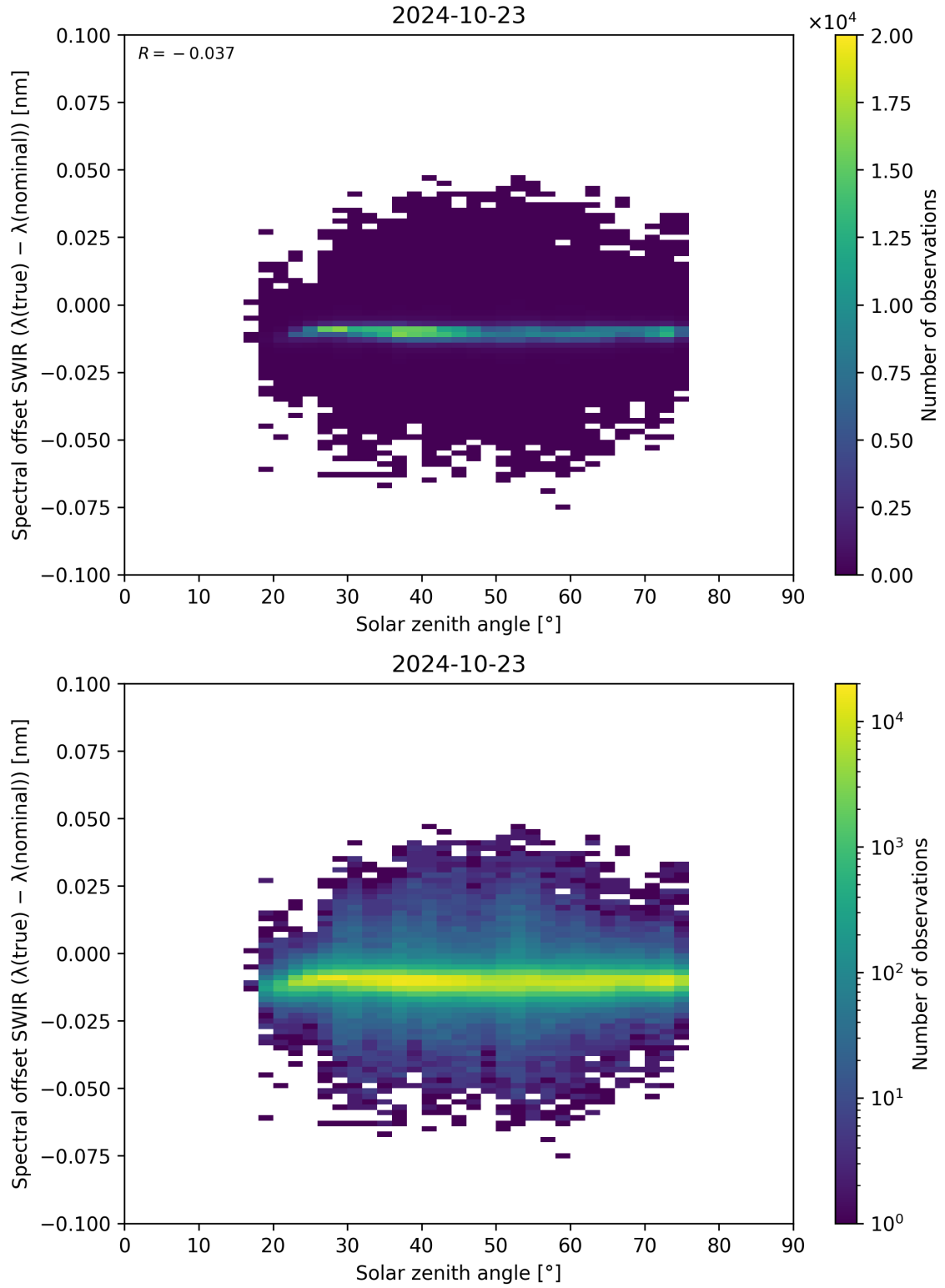
Figure 104: Scatter density plot of “Solar zenith angle” against “Spectral offset SWIR ( \lambda_{\text{true}} - \lambda_{\text{nominal}} )” for 2024-10-22 to 2024-10-24.
