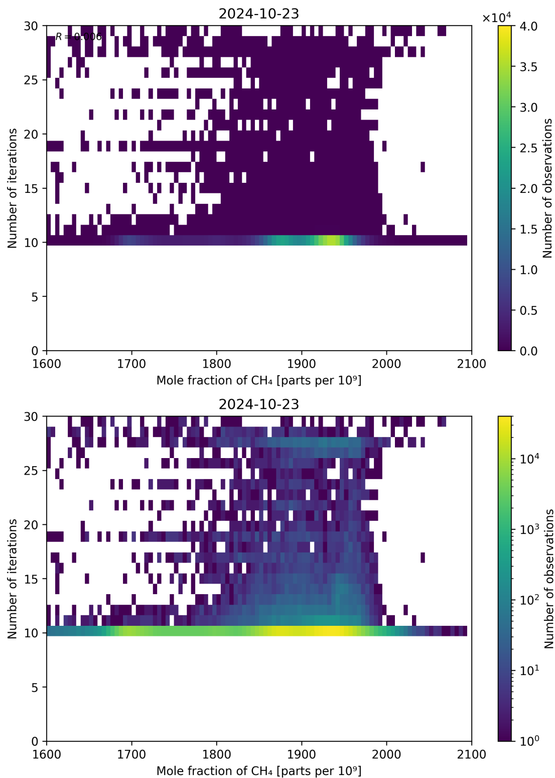
Figure 76: Scatter density plot of “Mole fraction of CH 4 ” against “Number of iterations” for 2024-10-22 to 2024-10-24.
