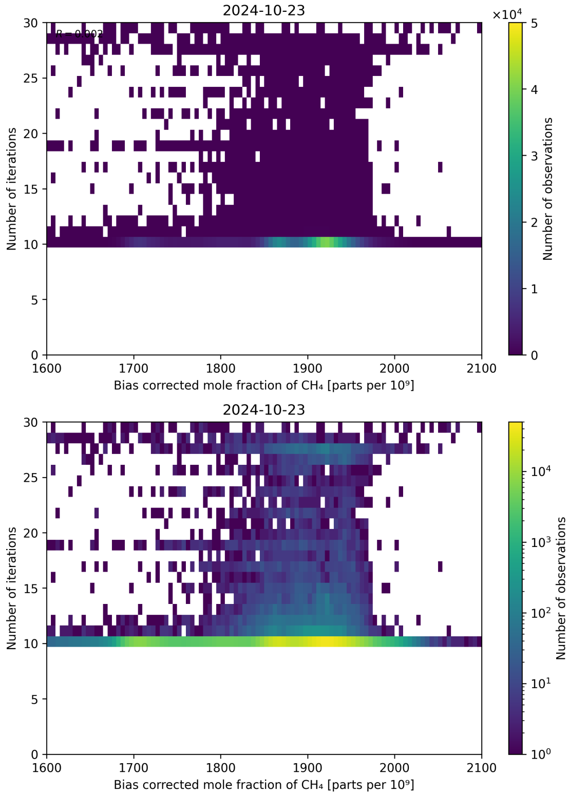
Figure 67: Scatter density plot of “Bias corrected mole fraction of \text{CH}_4 ” against “Number of iterations” for 2024-10-22 to 2024-10-24.
