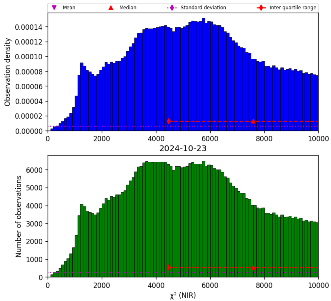
Figure 29: Histogram of “ \chi^2 (NIR)” for 2024-10-22 to 2024-10-24
