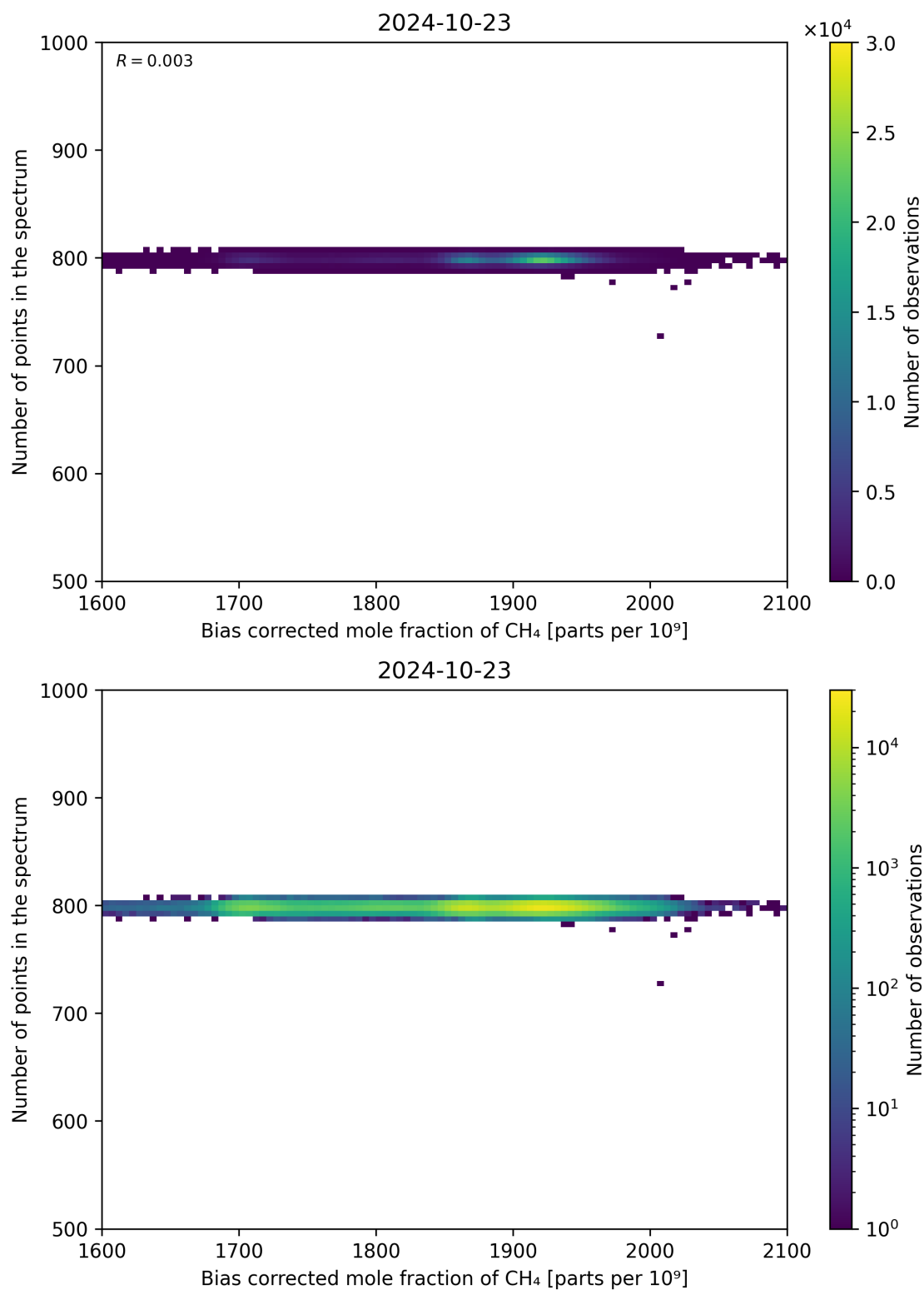
Figure 68: Scatter density plot of “Bias corrected mole fraction of CH 4 ” against “Number of points in the spectrum” for 2024-10-22 to 2024-10-24.
