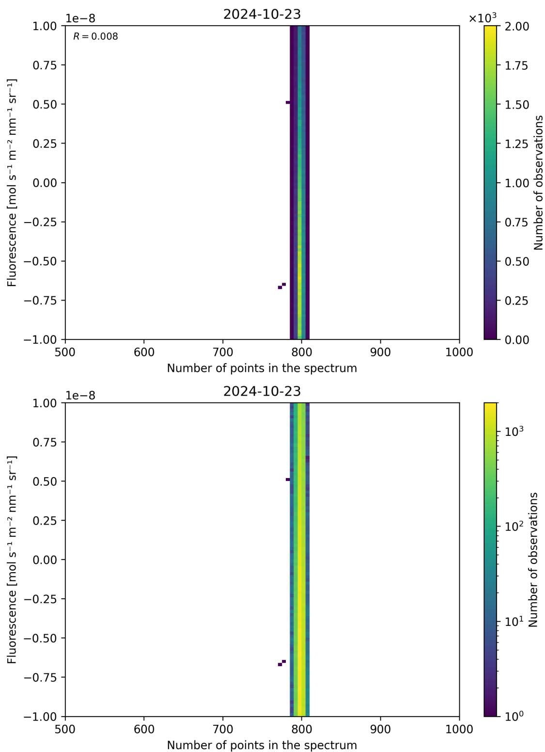
Figure 91: Scatter density plot of “Number of points in the spectrum” against “Fluorescence” for 2024-10-22 to 2024-10-24.
