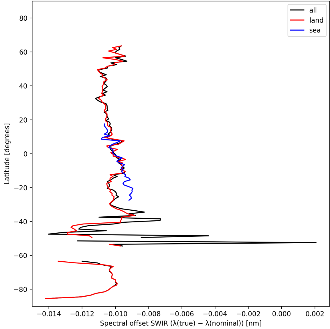
Figure 16: Zonal average of “Spectral offset SWIR ( \lambda_{\text{true}} - \lambda_{\text{nominal}} )” for 2024-10-22 to 2024-10-24.
