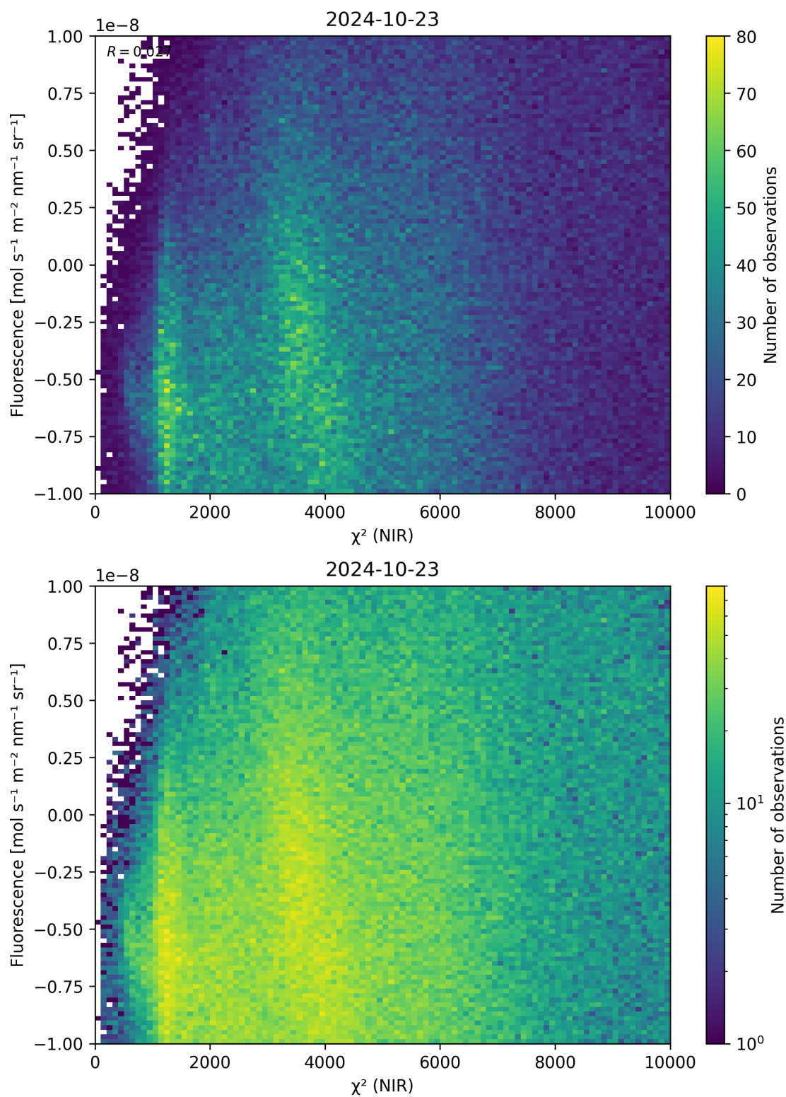
Figure 45: Scatter density plot of “ \chi^2 (NIR)” against “Fluorescence” for 2024-10-22 to 2024-10-24.
