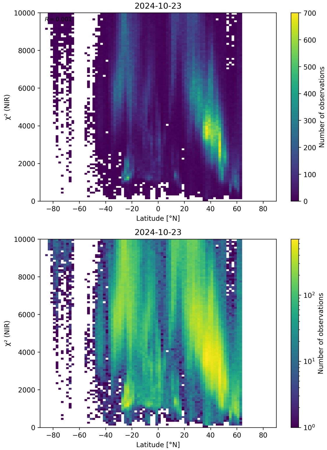
Figure 53: Scatter density plot of “Latitude” against “ \chi^2 (NIR)” for 2024-10-22 to 2024-10-24.
