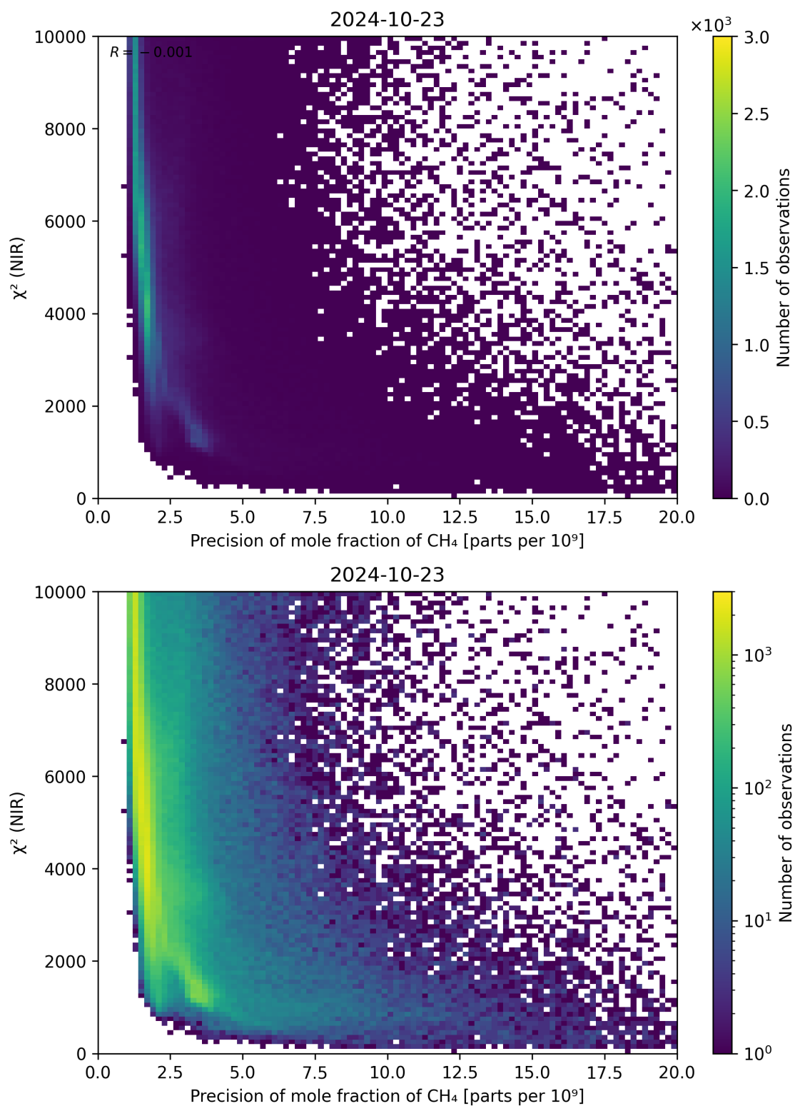
Figure 78: Scatter density plot of “Precision of mole fraction of \text{CH}_4 ” against “ \chi^2 (NIR)” for 2024-10-22 to 2024-10-24.
