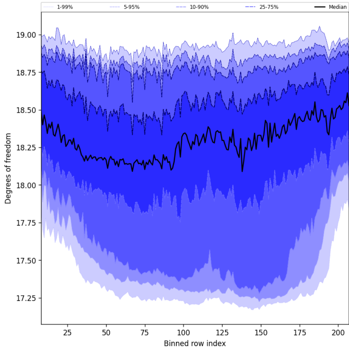
Figure 41: Along track statistics of “Degrees of freedom” for 2024-10-22 to 2024-10-24
