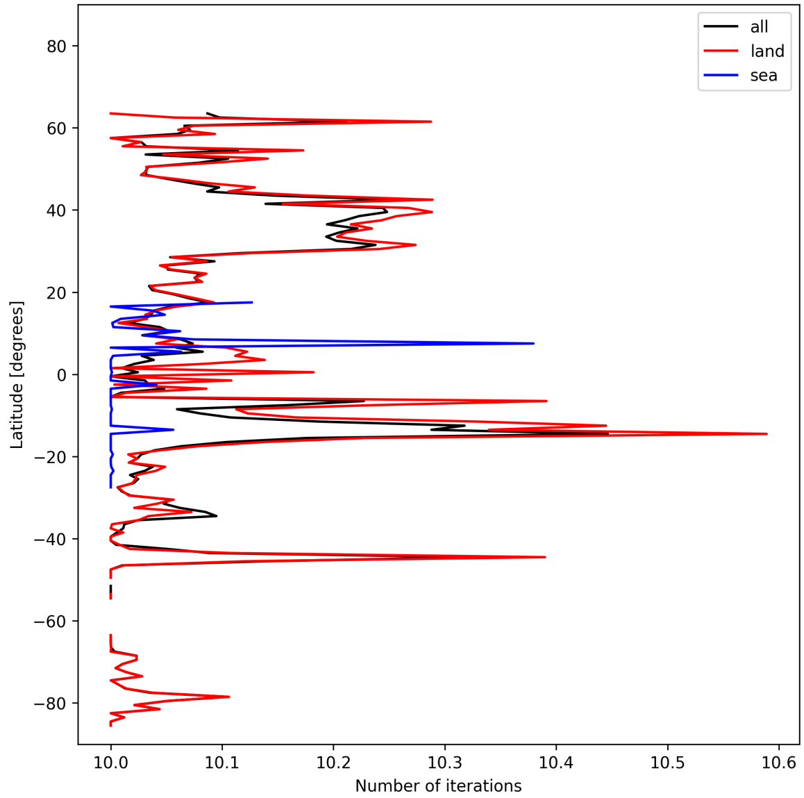
Figure 20: Zonal average of “Number of iterations” for 2024-10-22 to 2024-10-24.
