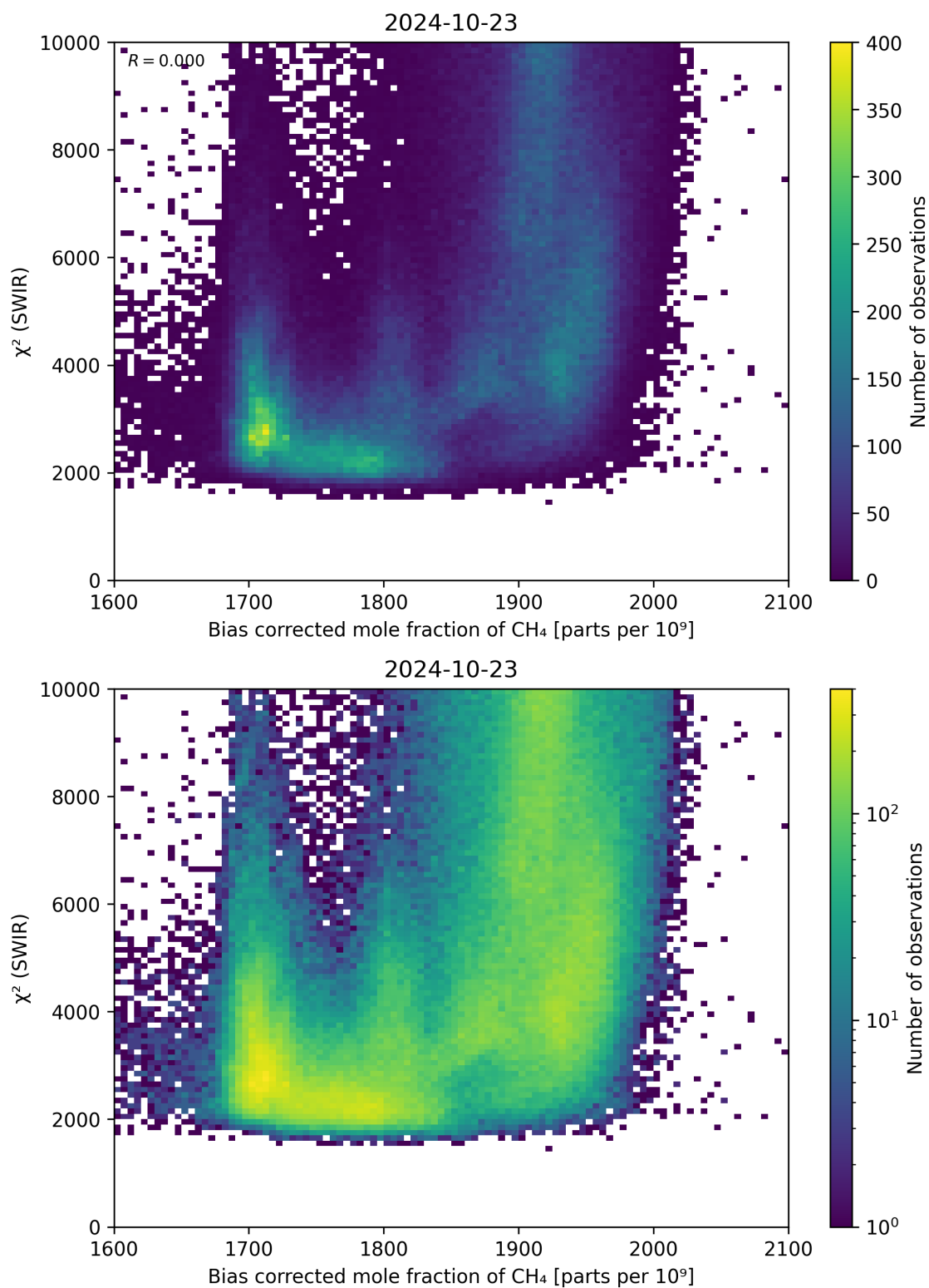
Figure 64: Scatter density plot of “Bias corrected mole fraction of \text{CH}_4 ” against “ \chi^2 (SWIR)” for 2024-10-22 to 2024-10-24.
