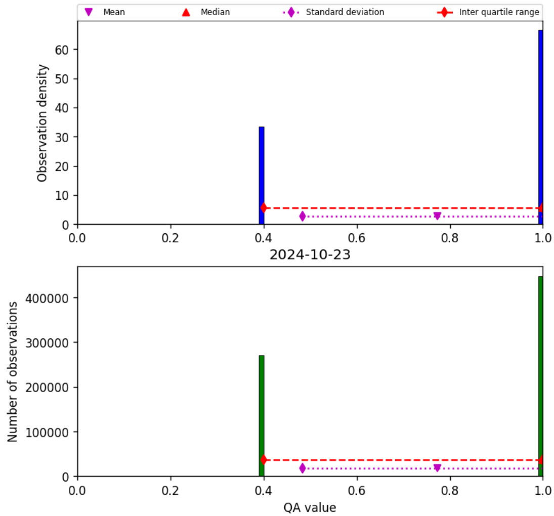
Figure 22: Histogram of “QA value” for 2024-10-22 to 2024-10-24
