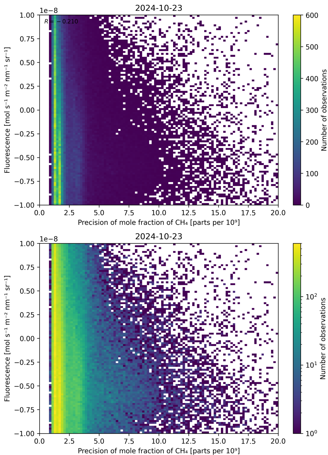
Figure 81: Scatter density plot of “Precision of mole fraction of \text{CH}_4 ” against “Fluorescence” for 2024-10-22 to 2024-10-24.
