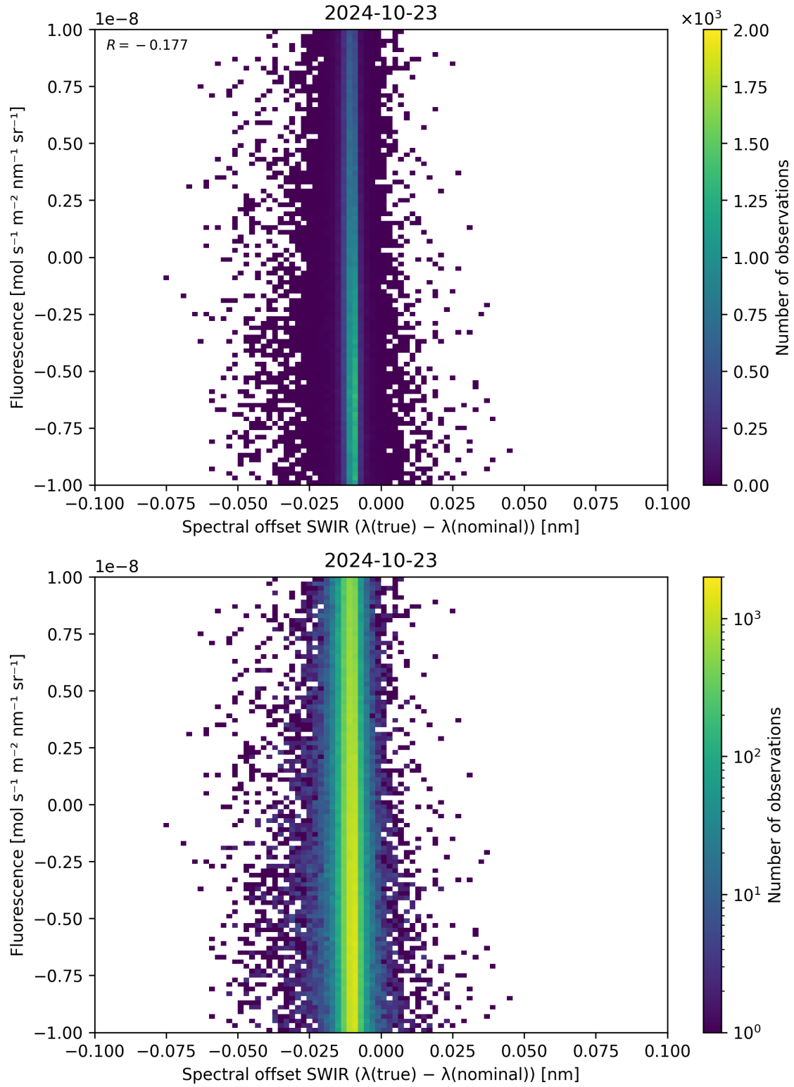
Figure 120: Scatter density plot of “Spectral offset SWIR ( \lambda_{\text{true}} - \lambda_{\text{nominal}} )” against “Fluorescence” for 2024-10-22 to 2024-10-24.
