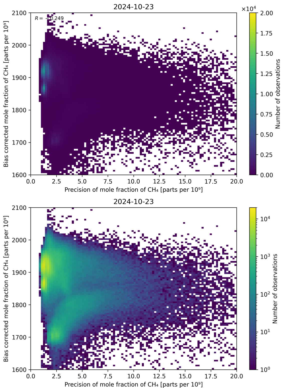
Figure 82: Scatter density plot of “Precision of mole fraction of CH 4 ” against “Bias corrected mole fraction of CH 4 ” for 2024-10-22 to 2024-10-24.
