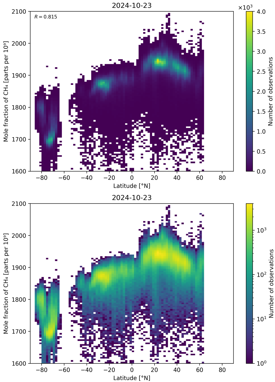
Figure 57: Scatter density plot of “Latitude” against “Mole fraction of CH 4 ” for 2024-10-22 to 2024-10-24.
