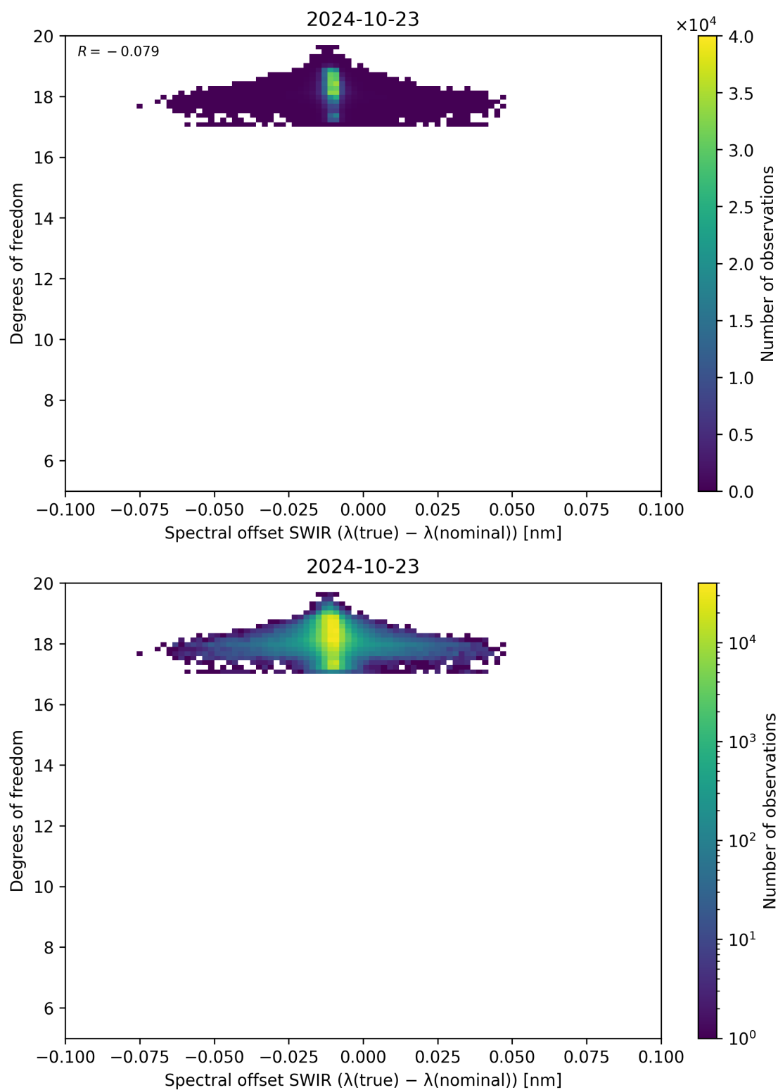
Figure 119: Scatter density plot of “Spectral offset SWIR ( \lambda_{\text{true}} - \lambda_{\text{nominal}} )” against “Degrees of freedom” for 2024-10-22 to 2024-10-24.
