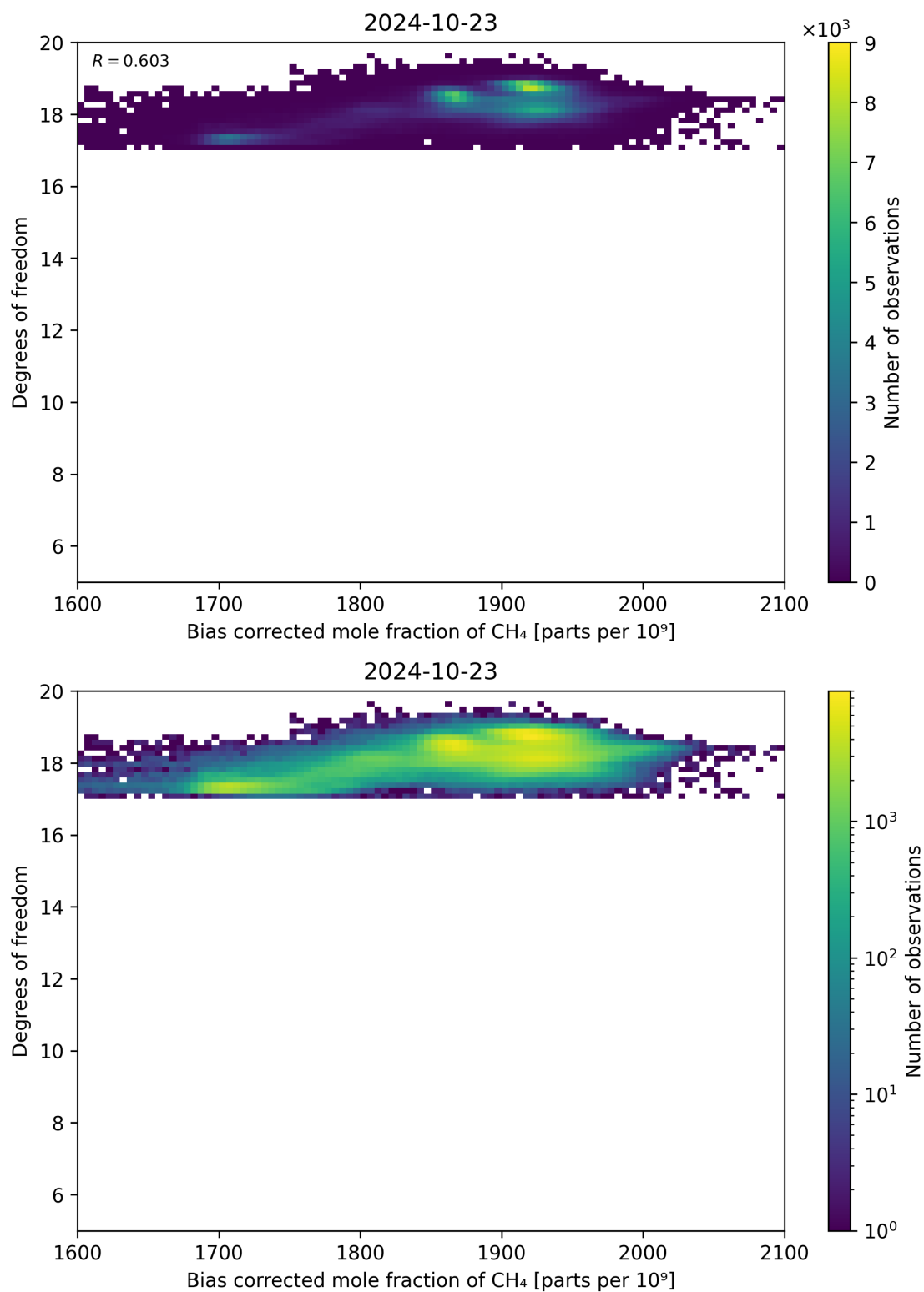
Figure 65: Scatter density plot of “Bias corrected mole fraction of CH 4 ” against “Degrees of freedom” for 2024-10-22 to 2024-10-24.
