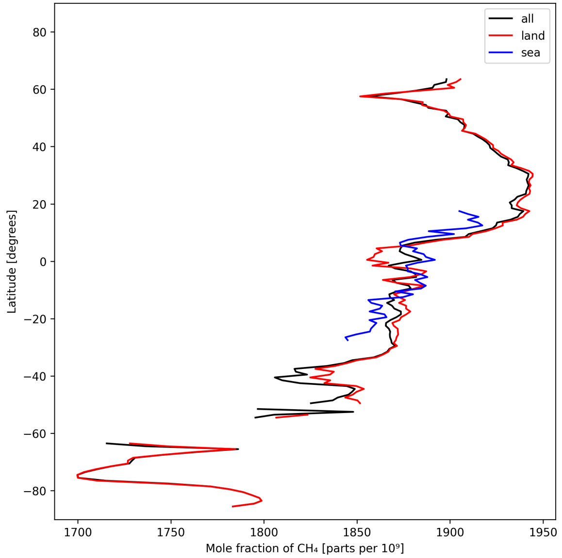
Figure 12: Zonal average of “Mole fraction of CH 4 ” for 2024-10-22 to 2024-10-24.
