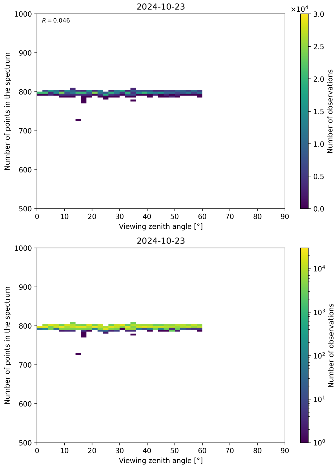
Figure 114: Scatter density plot of “Viewing zenith angle” against “Number of points in the spectrum” for 2024-10-22 to 2024-10-24.
