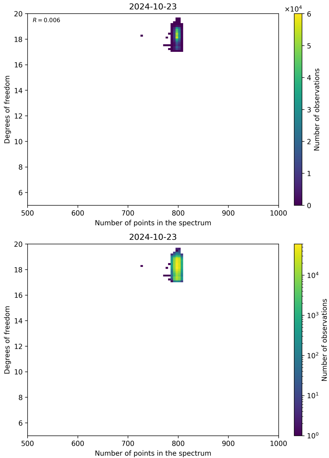
Figure 90: Scatter density plot of “Number of points in the spectrum” against “Degrees of freedom” for 2024-10-22 to 2024-10-24.
