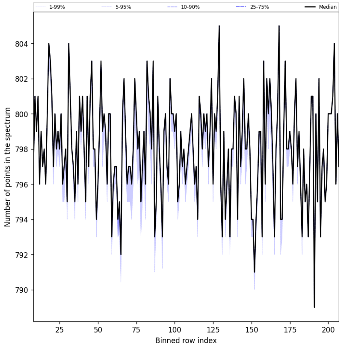
Figure 37: Along track statistics of “Number of points in the spectrum” for 2024-10-22 to 2024-10-24
