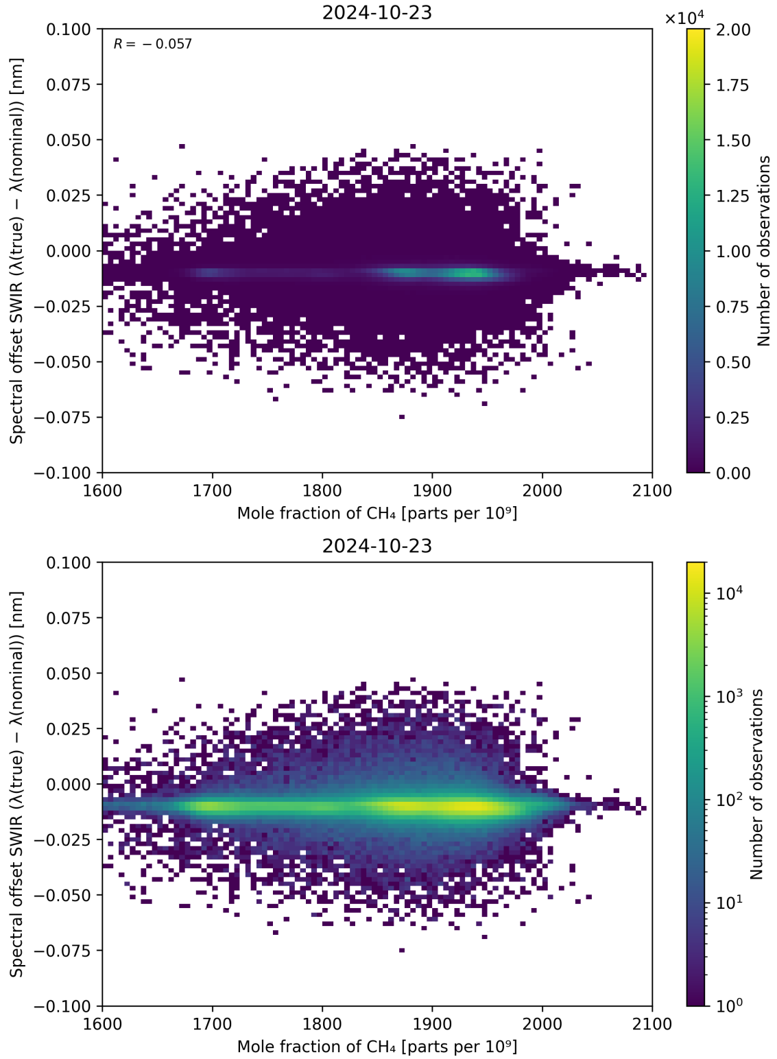
Figure 86: Scatter density plot of “Mole fraction of CH 4 ” against “Spectral offset SWIR ( \lambda_{\text{true}} - \lambda_{\text{nominal}} )” for 2024-10-22 to 2024-10-24.
