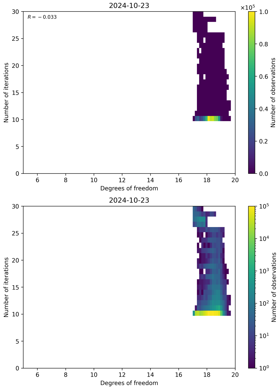
Figure 52: Scatter density plot of “Degrees of freedom” against “Number of iterations” for 2024-10-22 to 2024-10-24.
