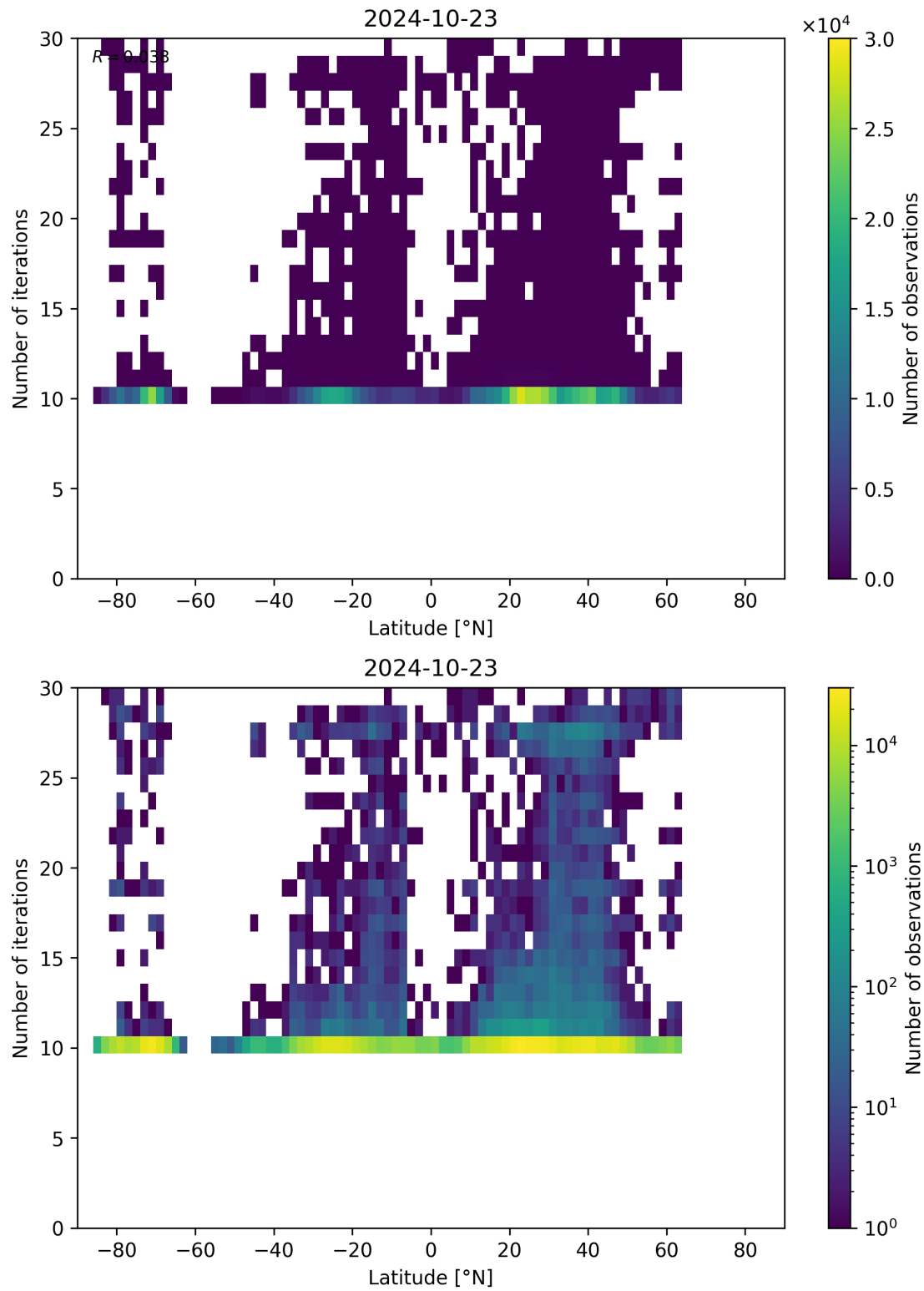
Figure 60: Scatter density plot of “Latitude” against “Number of iterations” for 2024-10-22 to 2024-10-24.
