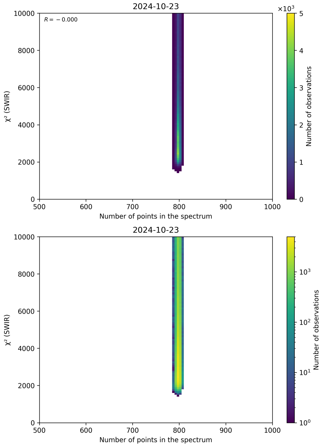
Figure 89: Scatter density plot of “Number of points in the spectrum” against “ \chi^2 (SWIR)” for 2024-10-22 to 2024-10-24.
