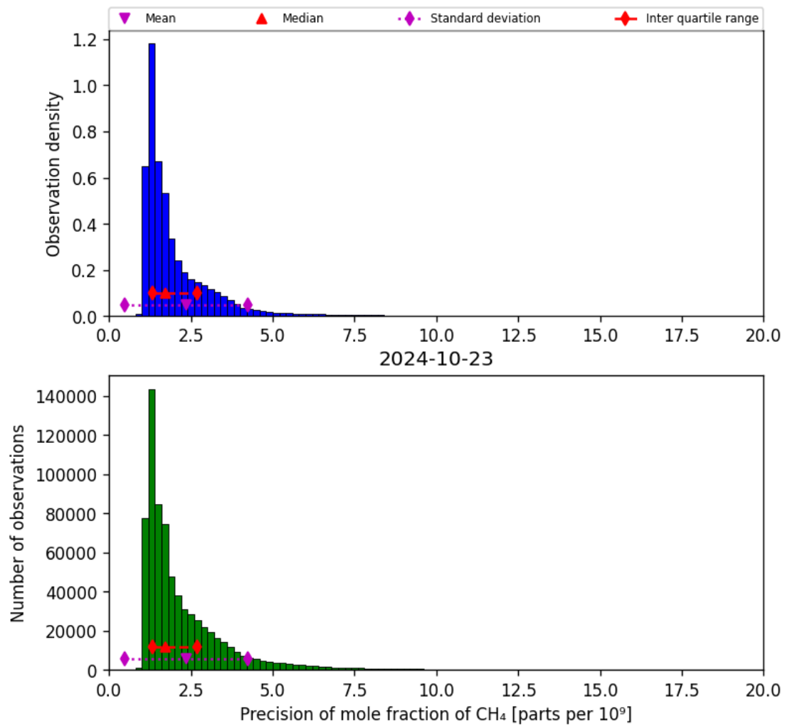
Figure 24: Histogram of “Precision of mole fraction of CH 4 ” for 2024-10-22 to 2024-10-24
