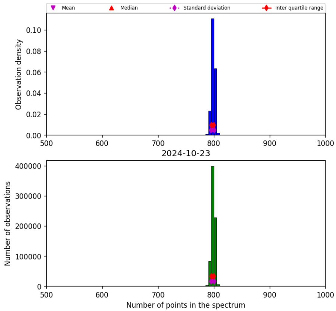
Figure 26: Histogram of “Number of points in the spectrum” for 2024-10-22 to 2024-10-24
