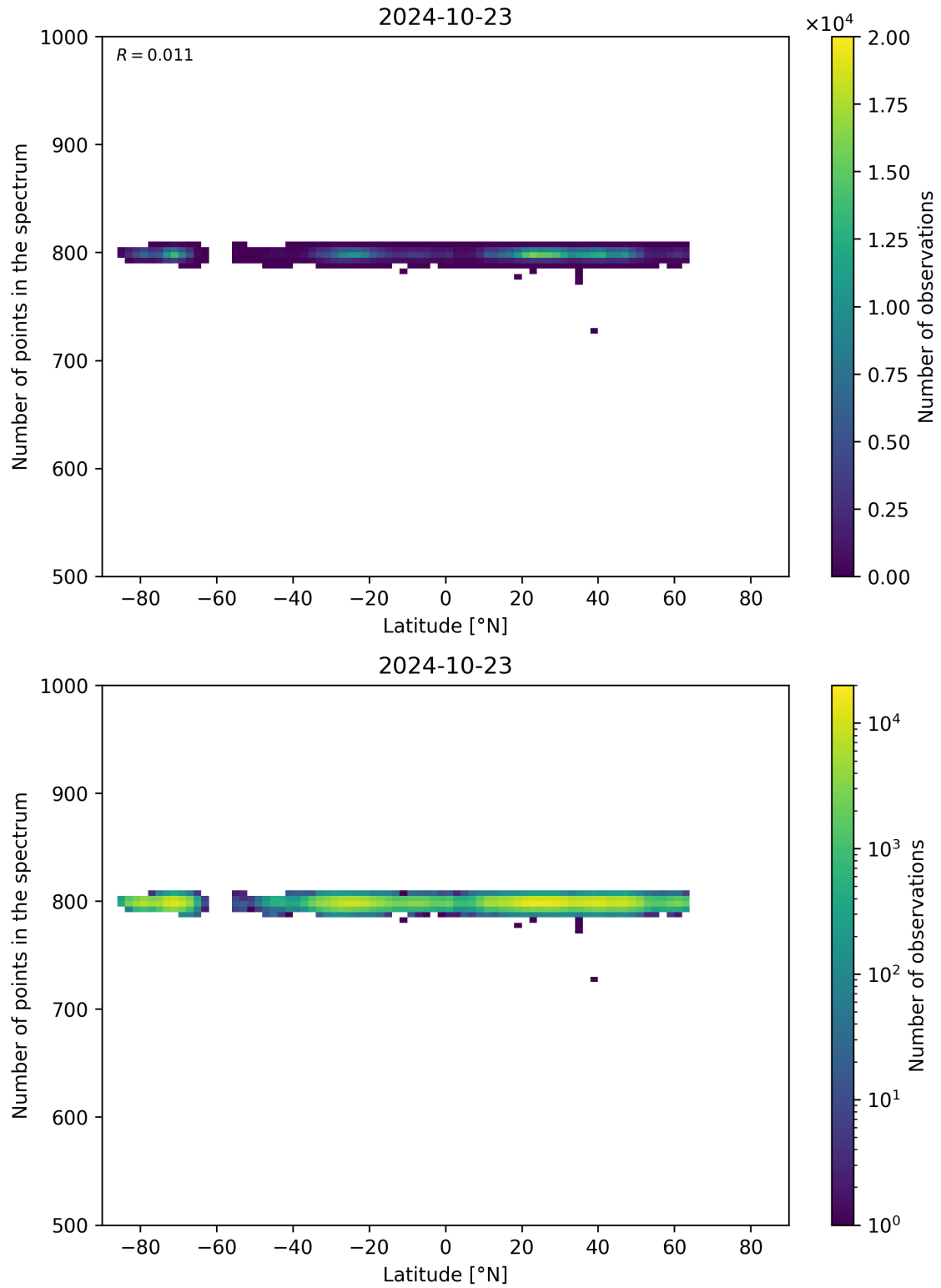
Figure 61: Scatter density plot of “Latitude” against “Number of points in the spectrum” for 2024-10-22 to 2024-10-24.
