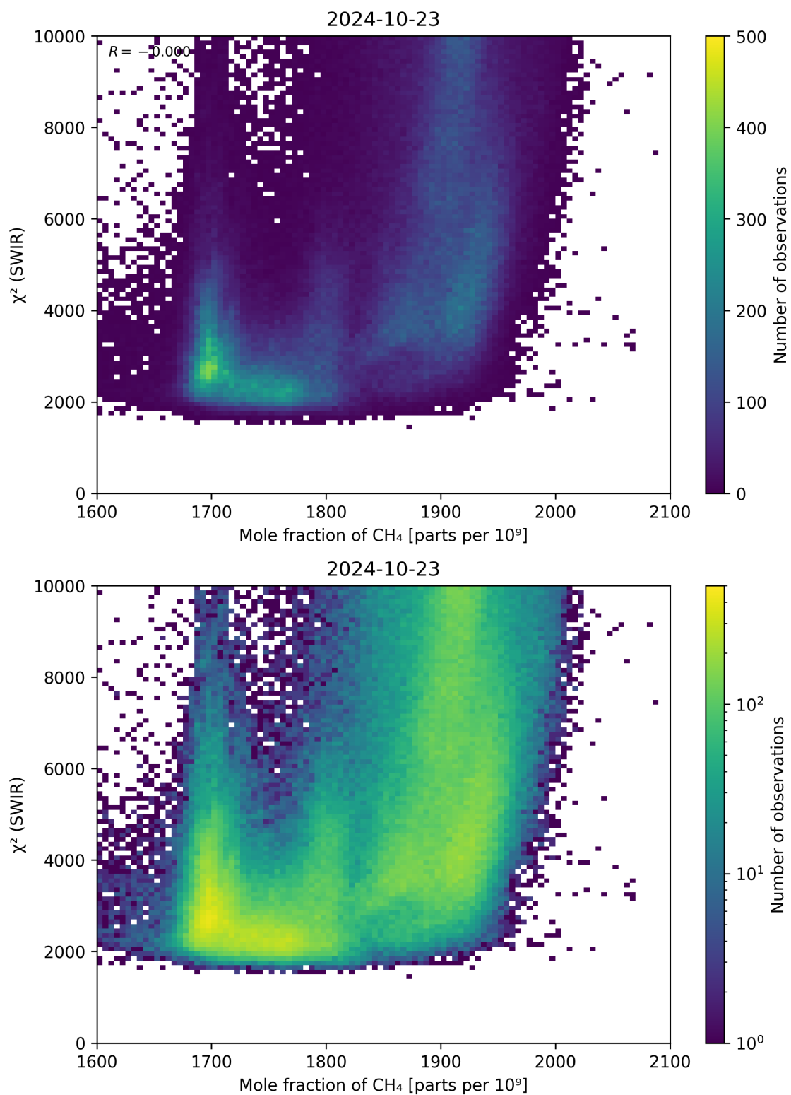
Figure 71: Scatter density plot of “Mole fraction of CH 4 ” against “ \chi^2 (SWIR)” for 2024-10-22 to 2024-10-24.
