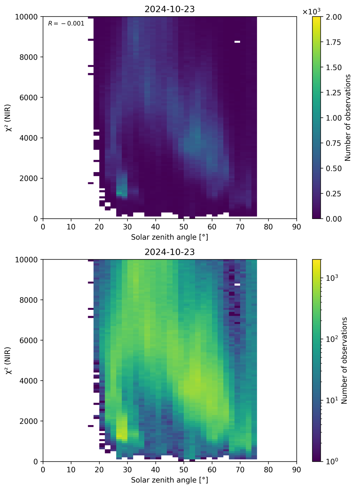
Figure 94: Scatter density plot of “Solar zenith angle” against “ \chi^2 (NIR)” for 2024-10-22 to 2024-10-24.
