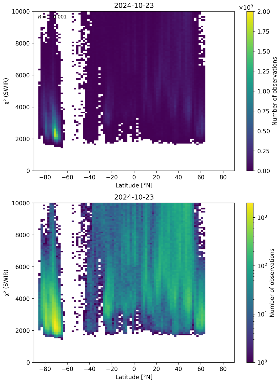
Figure 54: Scatter density plot of “Latitude” against “ \chi^2 (SWIR)” for 2024-10-22 to 2024-10-24.
