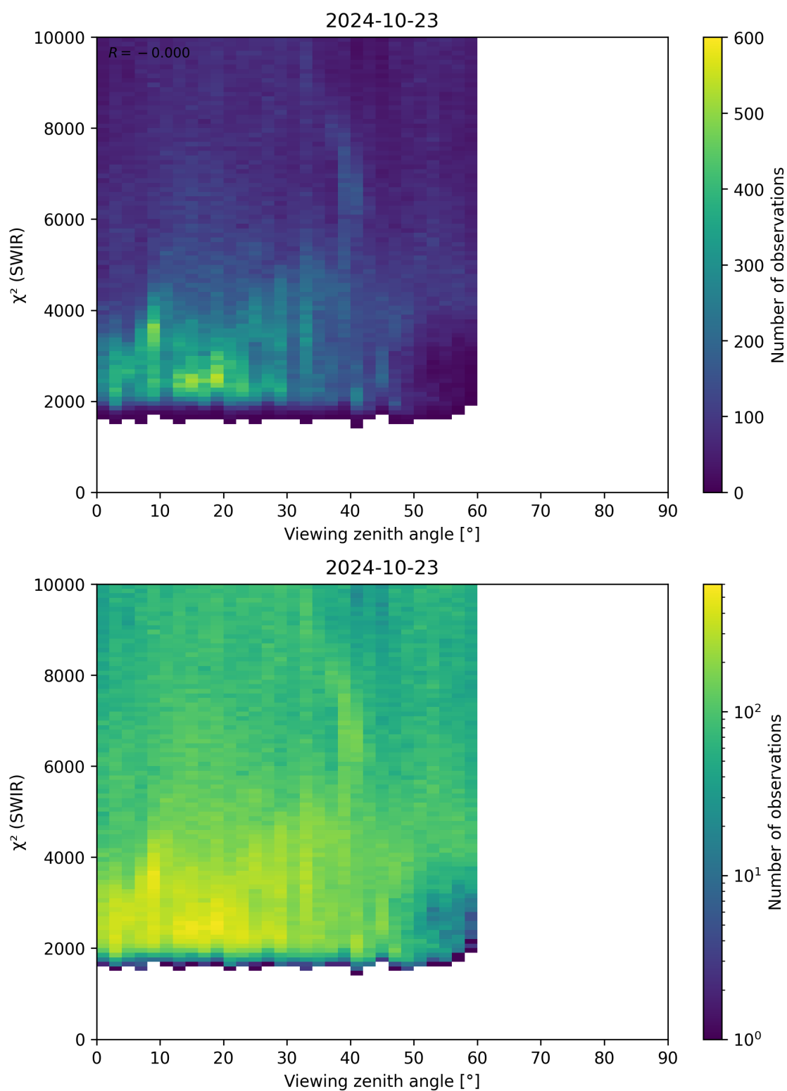
Figure 106: Scatter density plot of “Viewing zenith angle” against “ \chi^2 (SWIR)” for 2024-10-22 to 2024-10-24.
