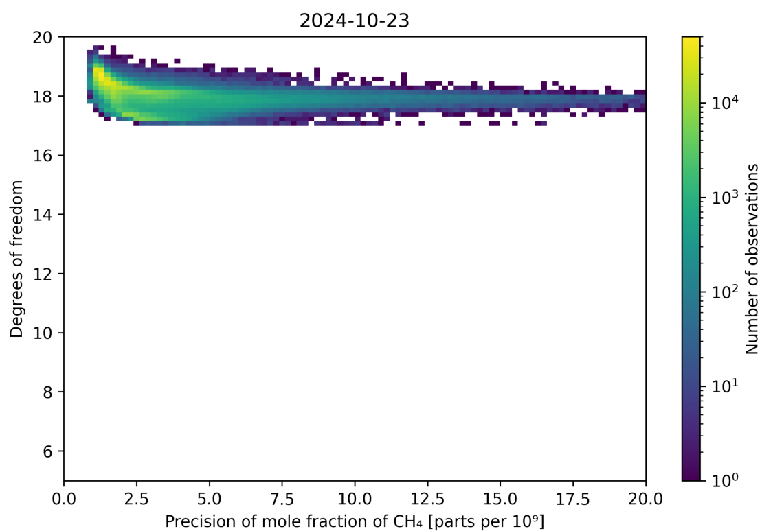
Figure 80: Scatter density plot of “Precision of mole fraction of CH 4 ” against “Degrees of freedom” for 2024-10-22 to 2024-10-24.
