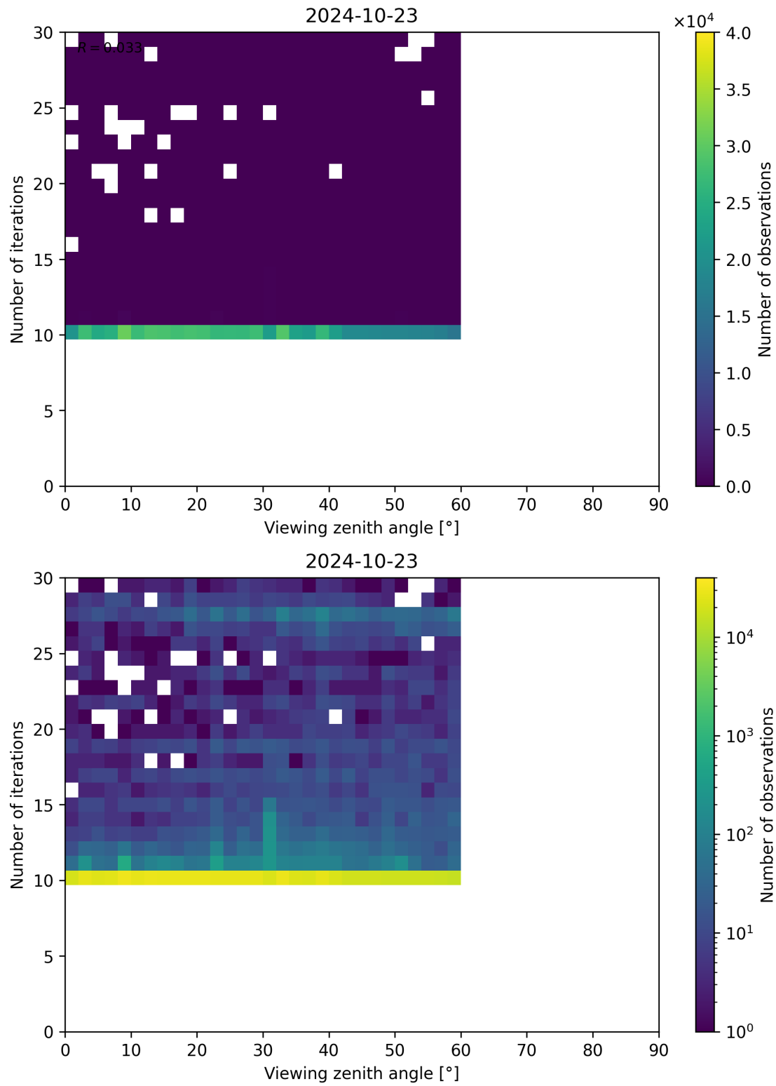
Figure 113: Scatter density plot of “Viewing zenith angle” against “Number of iterations” for 2024-10-22 to 2024-10-24.
