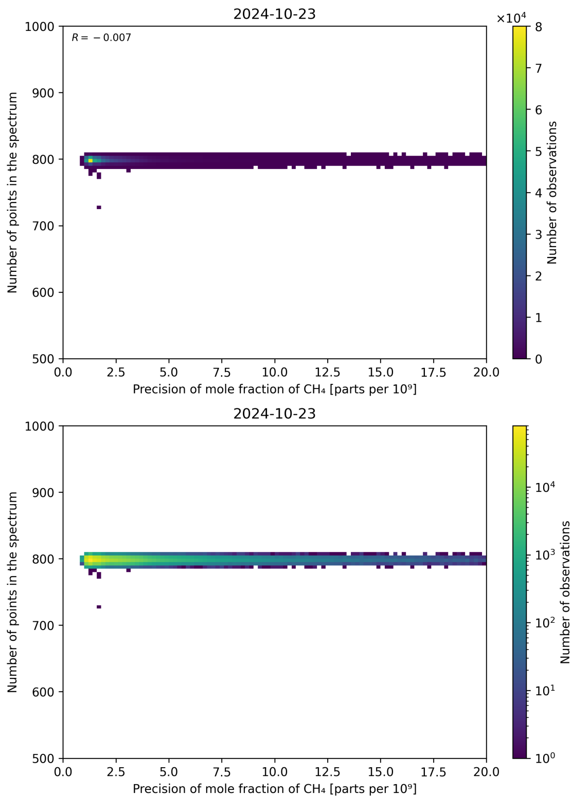
Figure 84: Scatter density plot of “Precision of mole fraction of CH 4 ” against “Number of points in the spectrum” for 2024-10-22 to 2024-10-24.
