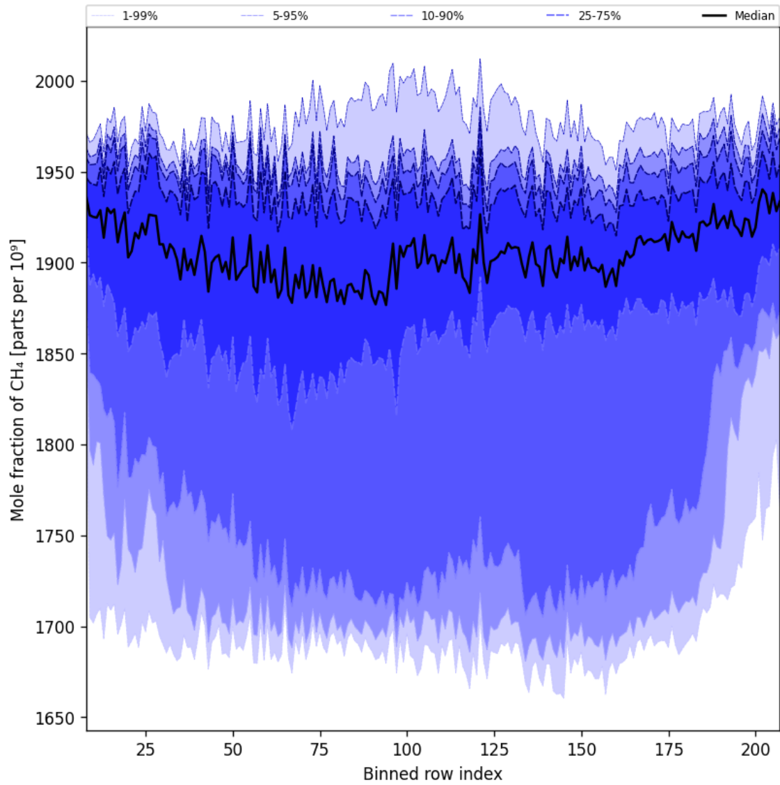
Figure 34: Along track statistics of “Mole fraction of CH 4 ” for 2024-10-22 to 2024-10-24
