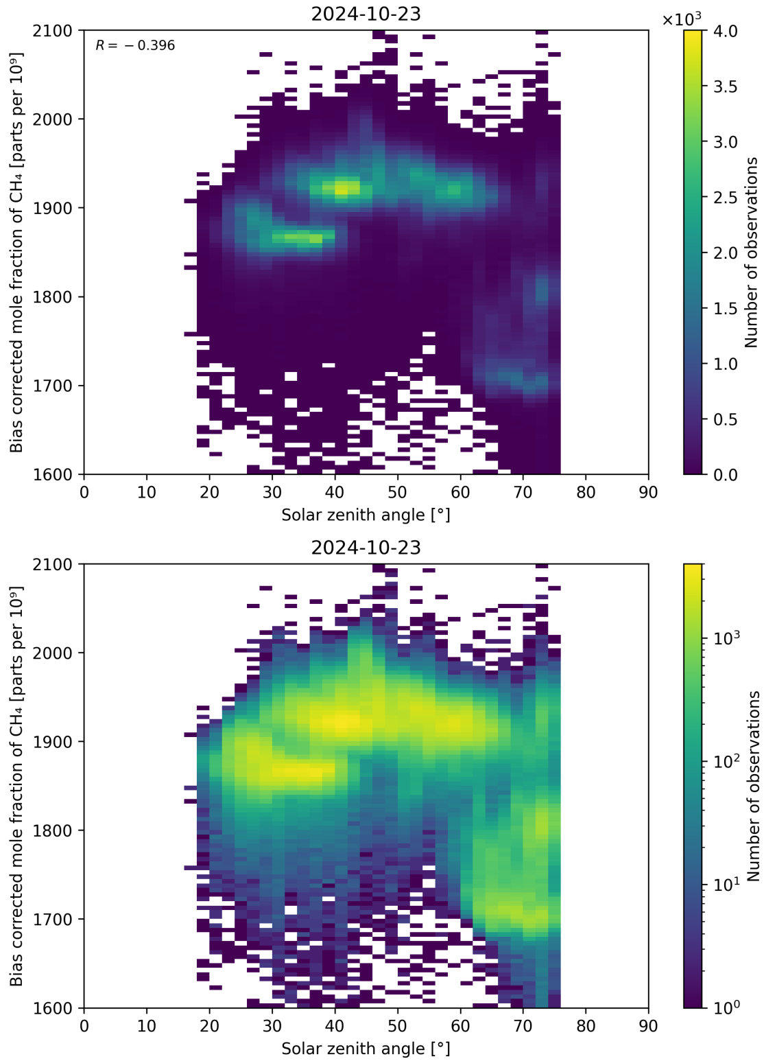
Figure 100: Scatter density plot of “Solar zenith angle” against “Bias corrected mole fraction of CH 4 ” for 2024-10-22 to 2024-10-24.
