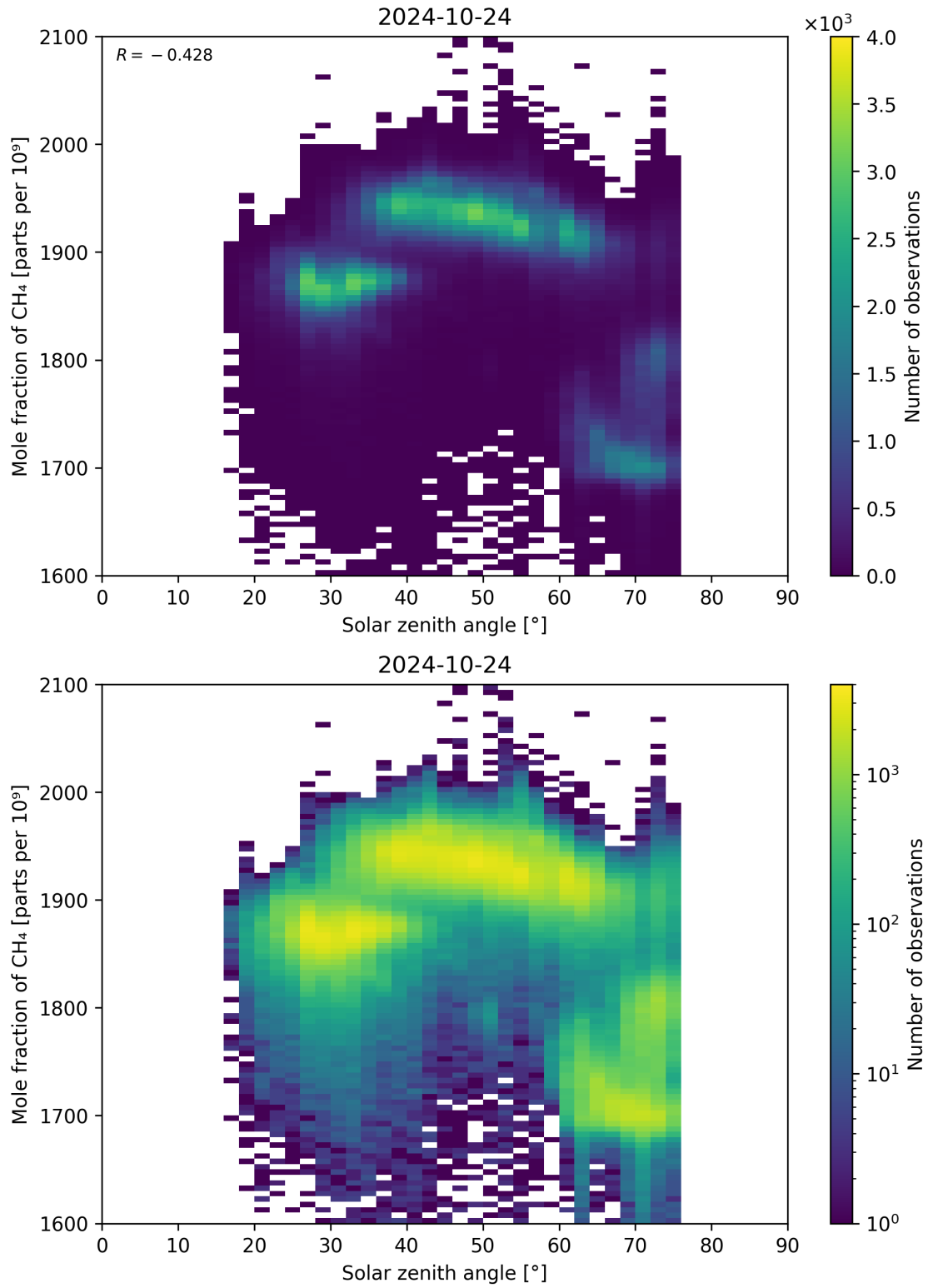
Figure 99: Scatter density plot of “Solar zenith angle” against “Mole fraction of CH 4 ” for 2024-10-24 to 2024-10-25.
