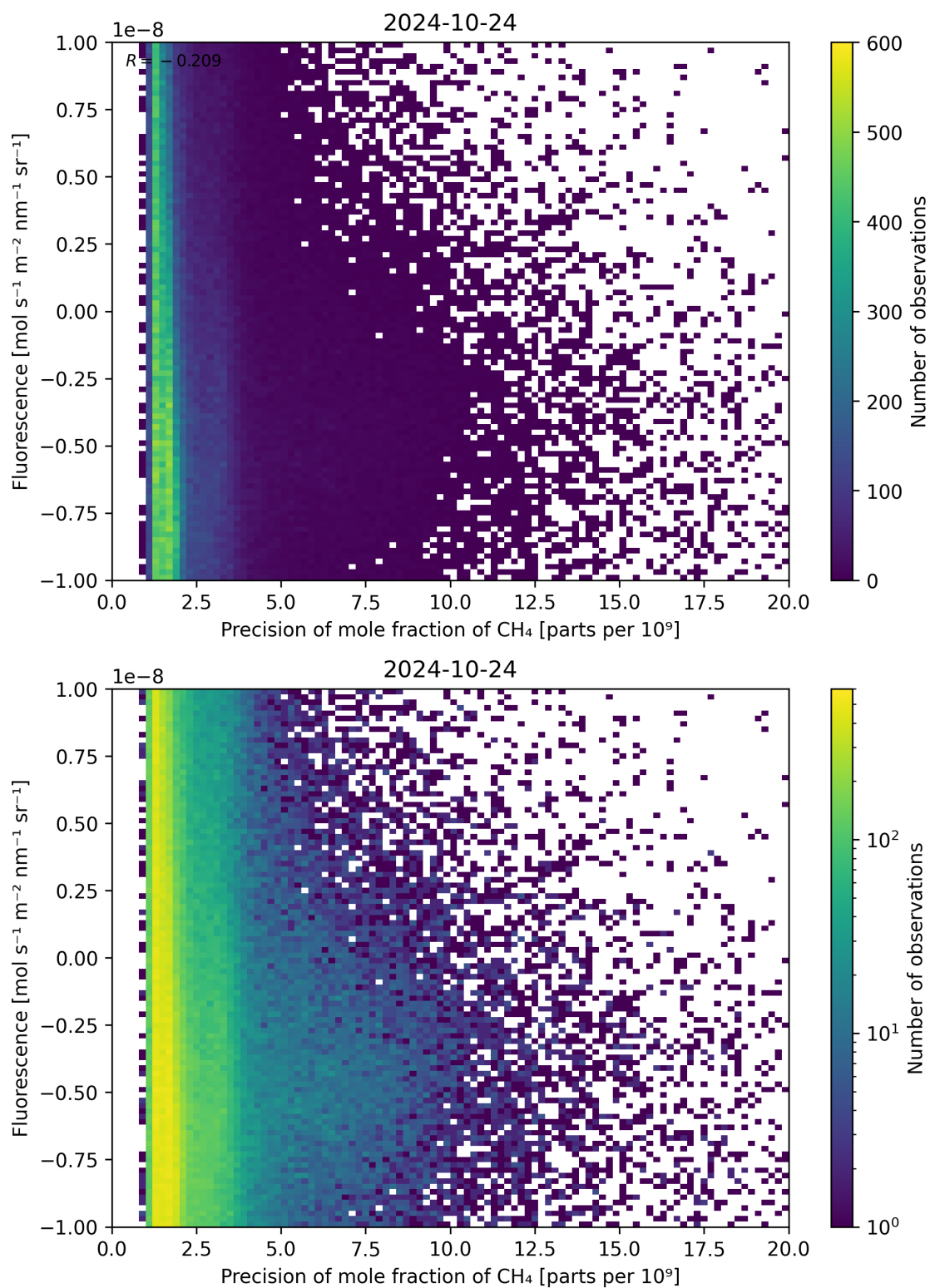
Figure 81: Scatter density plot of “Precision of mole fraction of \text{CH}_4 ” against “Fluorescence” for 2024-10-24 to 2024-10-25.
