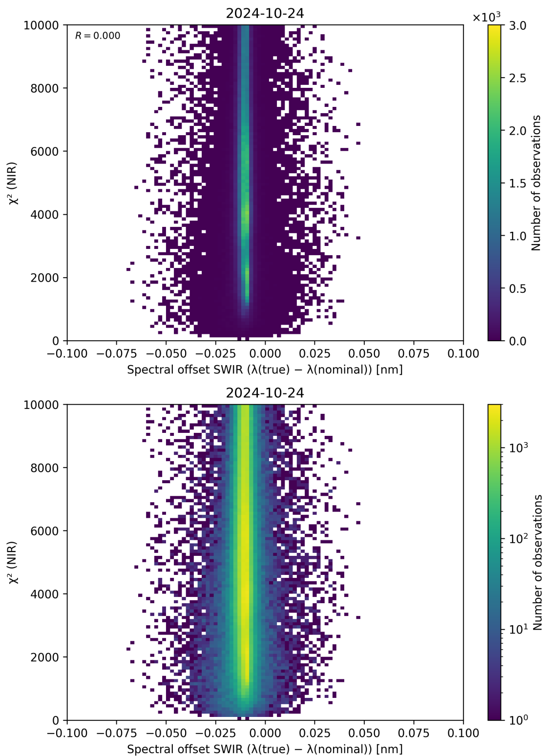
Figure 117: Scatter density plot of “Spectral offset SWIR ( \lambda_{\text{true}} - \lambda_{\text{nominal}} )” against “ \chi^2 (NIR)” for 2024-10-24 to 2024-10-25.
