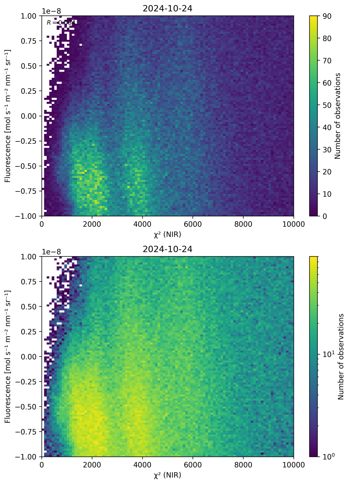
Figure 45: Scatter density plot of “ \chi^2 (NIR)” against “Fluorescence” for 2024-10-24 to 2024-10-25.
