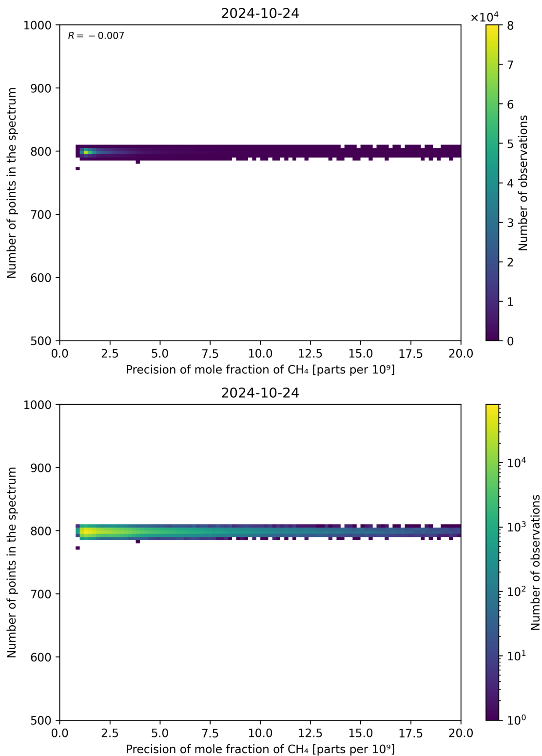
Figure 84: Scatter density plot of “Precision of mole fraction of CH 4 ” against “Number of points in the spectrum” for 2024-10-24 to 2024-10-25.
