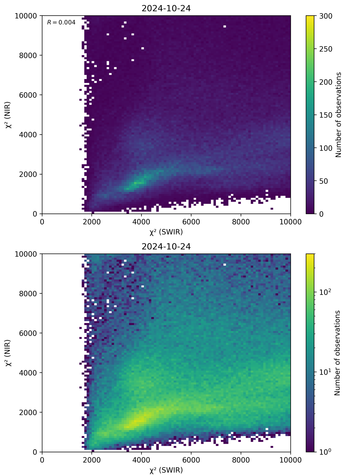
Figure 47: Scatter density plot of “ \chi^2 (SWIR)” against “ \chi^2 (NIR)” for 2024-10-24 to 2024-10-25.
