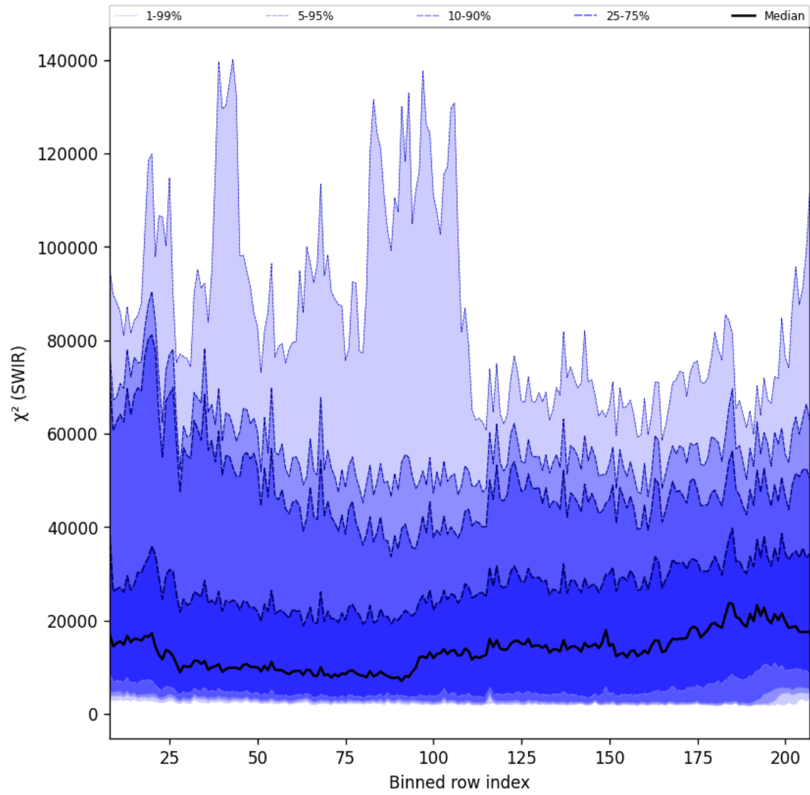
Figure 39: Along track statistics of “ \chi^2 (SWIR)” for 2024-10-24 to 2024-10-25
