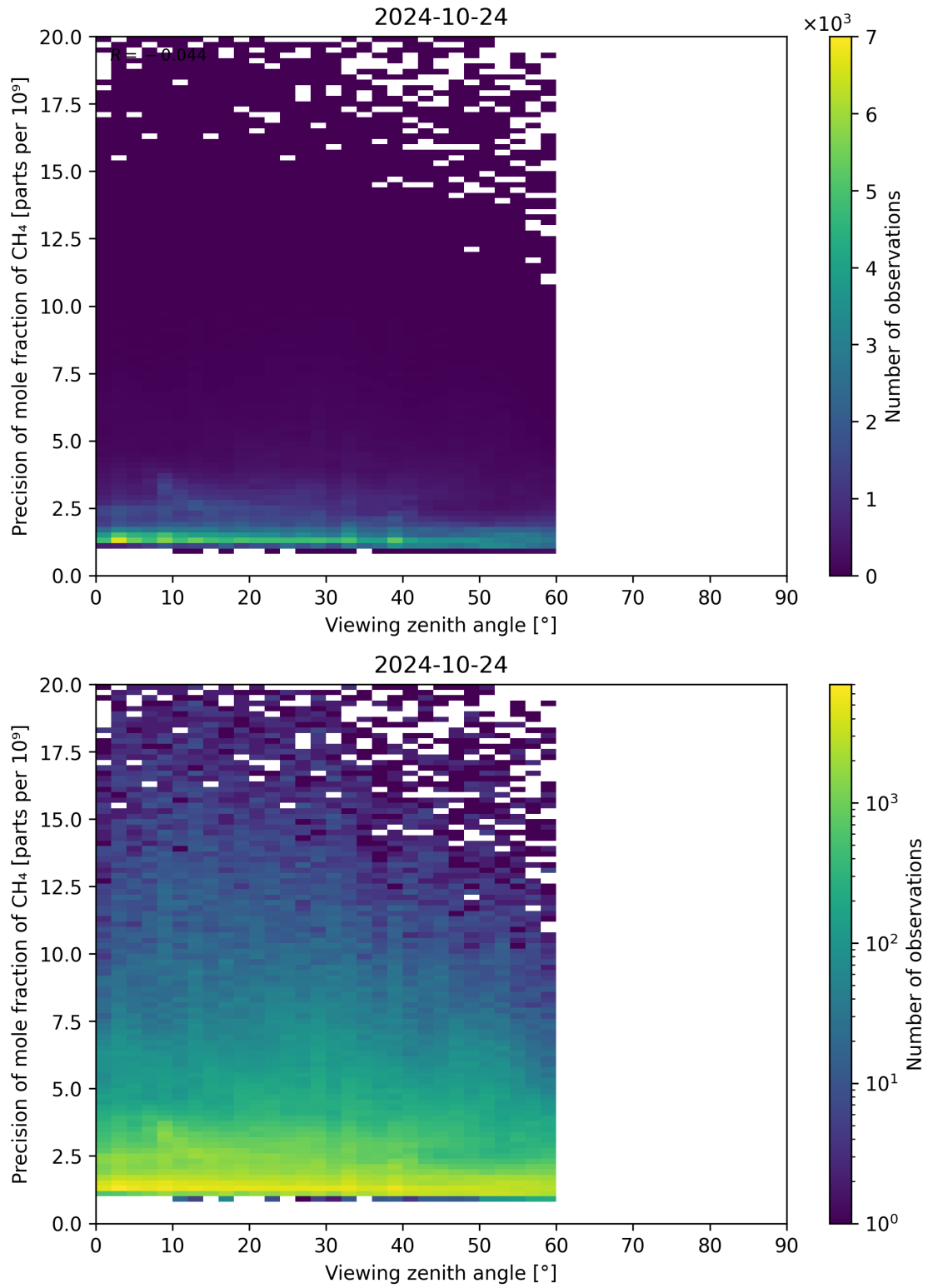
Figure 112: Scatter density plot of “Viewing zenith angle” against “Precision of mole fraction of CH 4 ” for 2024-10-24 to 2024-10-25.
