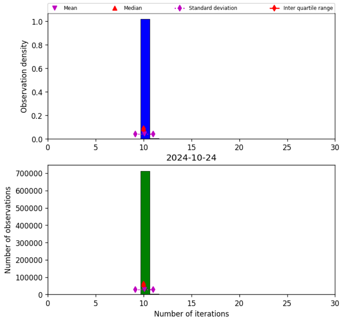
Figure 31: Histogram of “Number of iterations” for 2024-10-24 to 2024-10-25
