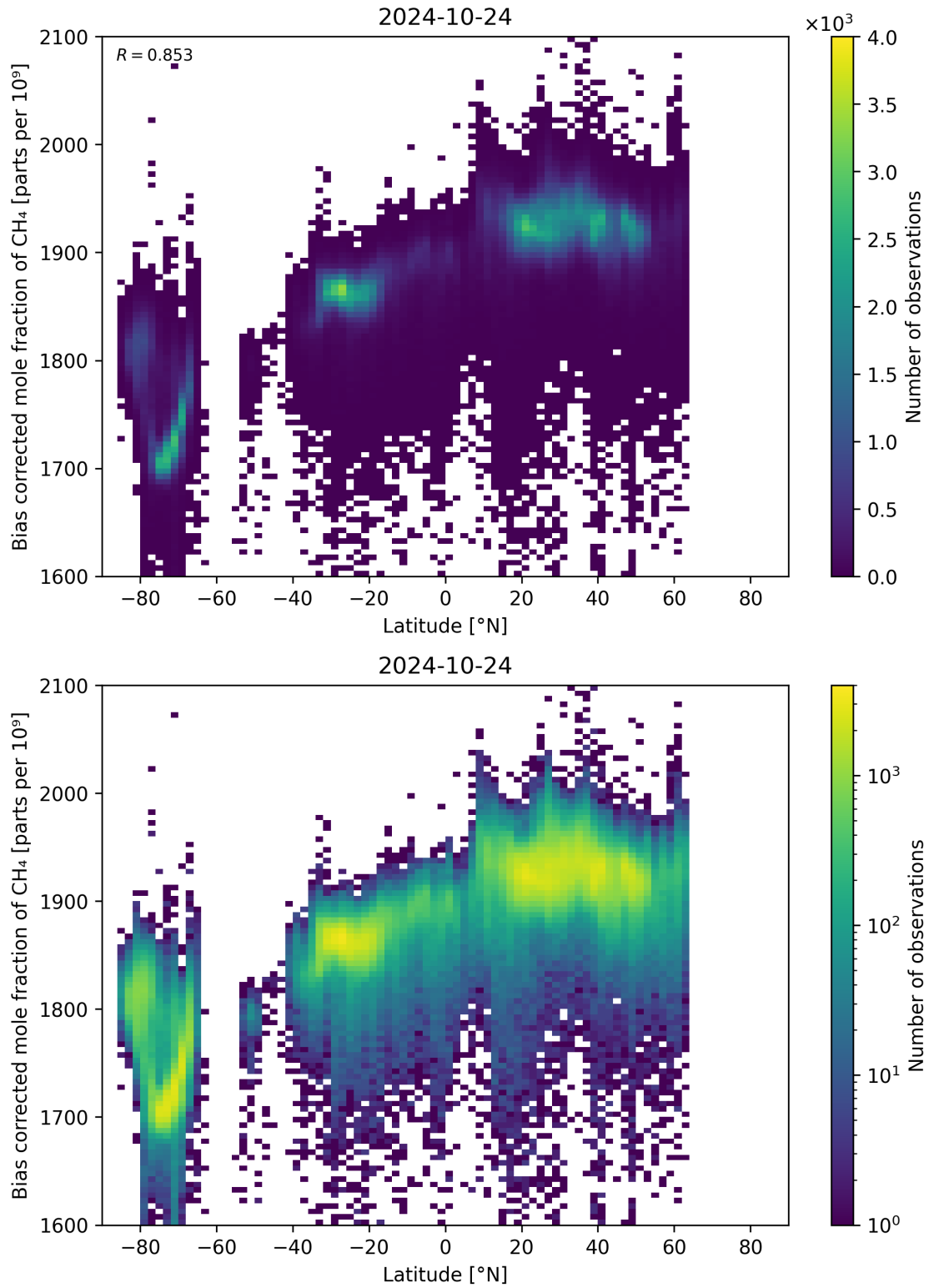
Figure 58: Scatter density plot of “Latitude” against “Bias corrected mole fraction of CH 4 ” for 2024-10-24 to 2024-10-25.
