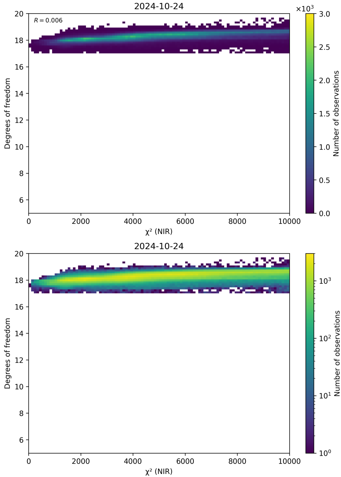
Figure 44: Scatter density plot of “ \chi^2 (NIR)” against “Degrees of freedom” for 2024-10-24 to 2024-10-25.
