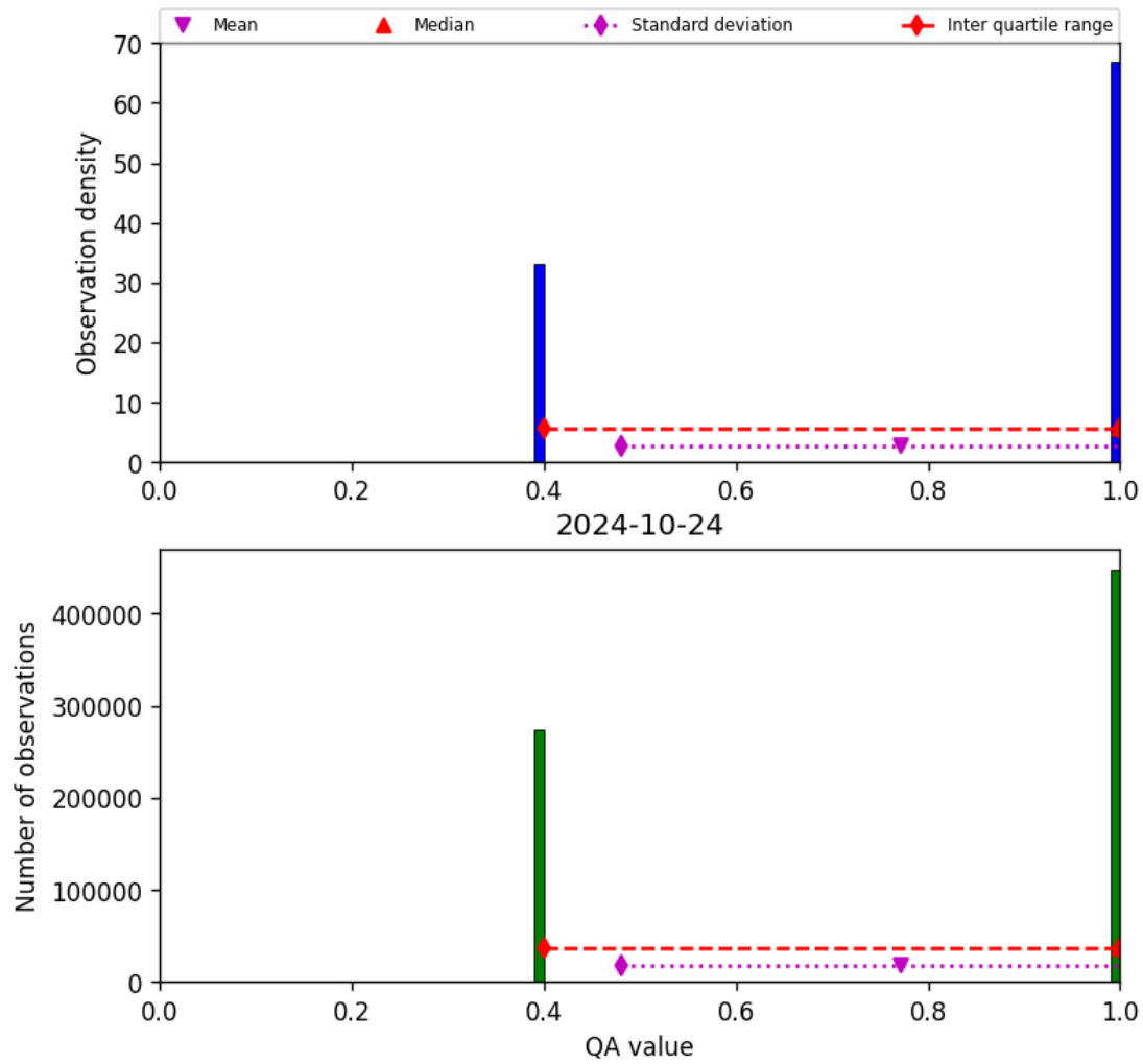
Figure 22: Histogram of “QA value” for 2024-10-24 to 2024-10-25
