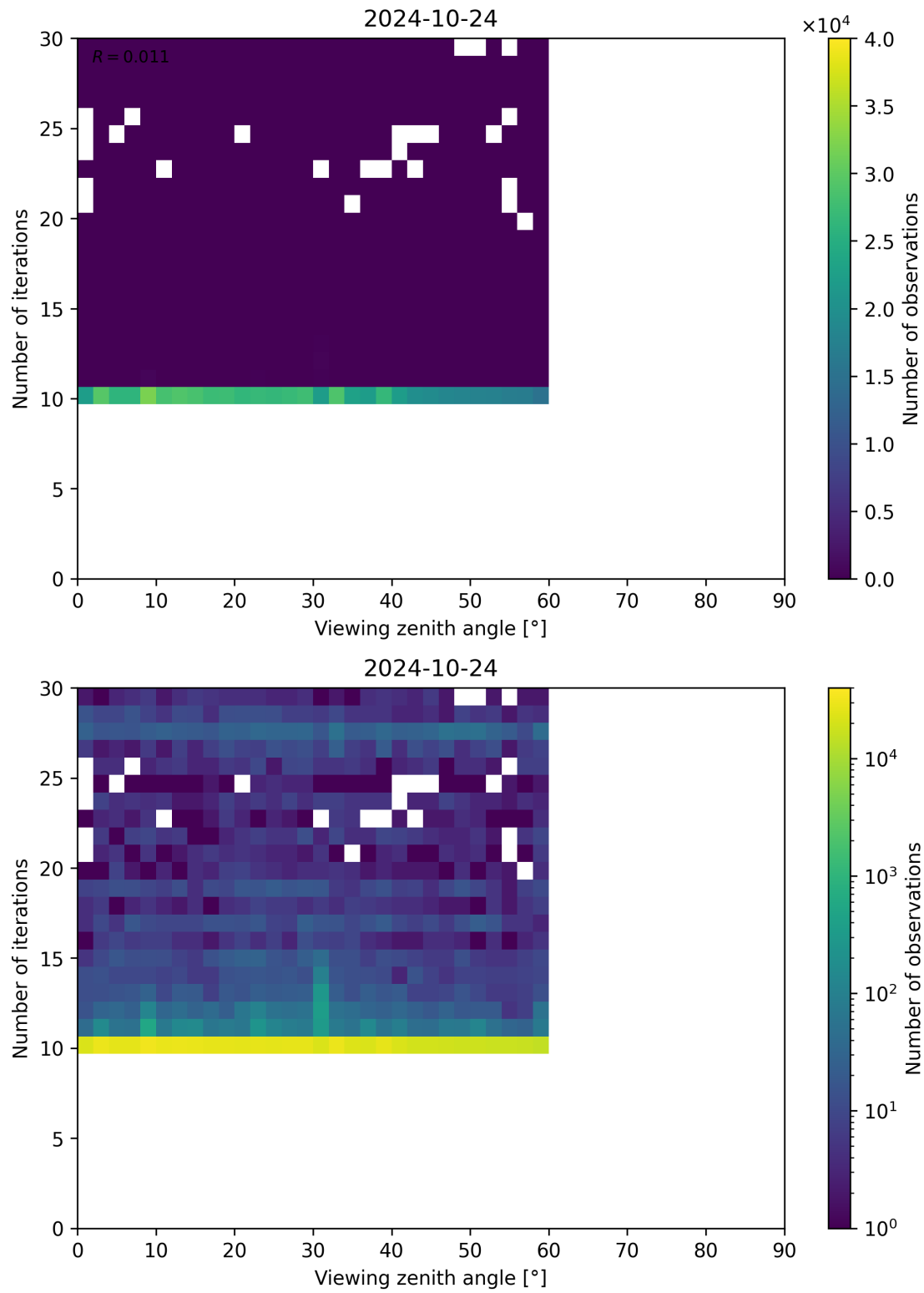
Figure 113: Scatter density plot of “Viewing zenith angle” against “Number of iterations” for 2024-10-24 to 2024-10-25.
