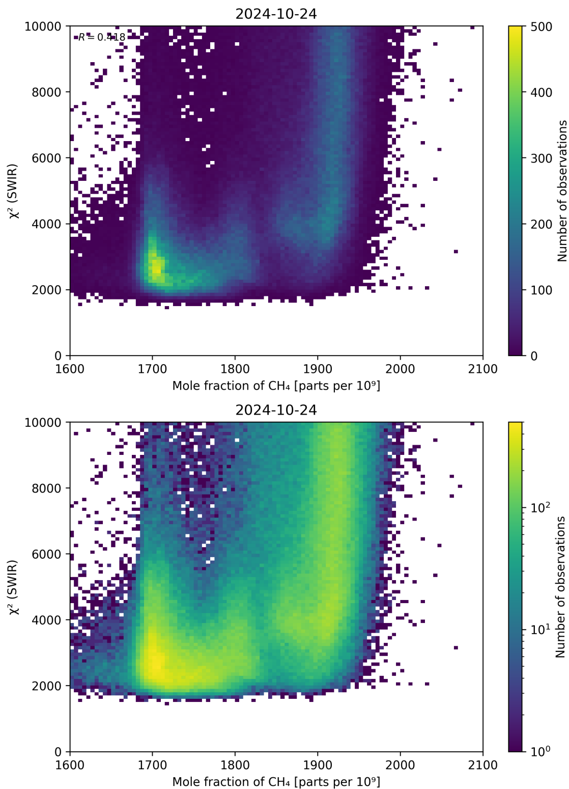
Figure 71: Scatter density plot of “Mole fraction of \text{CH}_4 ” against “ \chi^2 (SWIR)” for 2024-10-24 to 2024-10-25.
