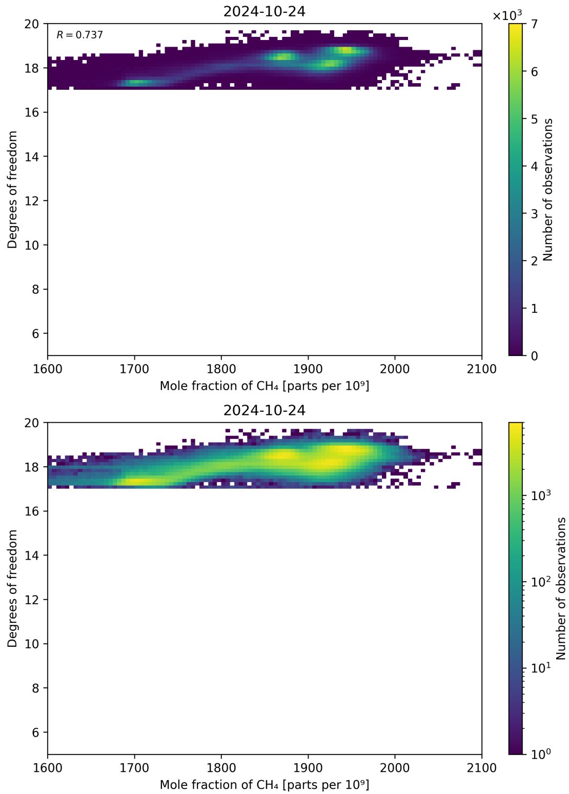
Figure 72: Scatter density plot of “Mole fraction of CH 4 ” against “Degrees of freedom” for 2024-10-24 to 2024-10-25.
