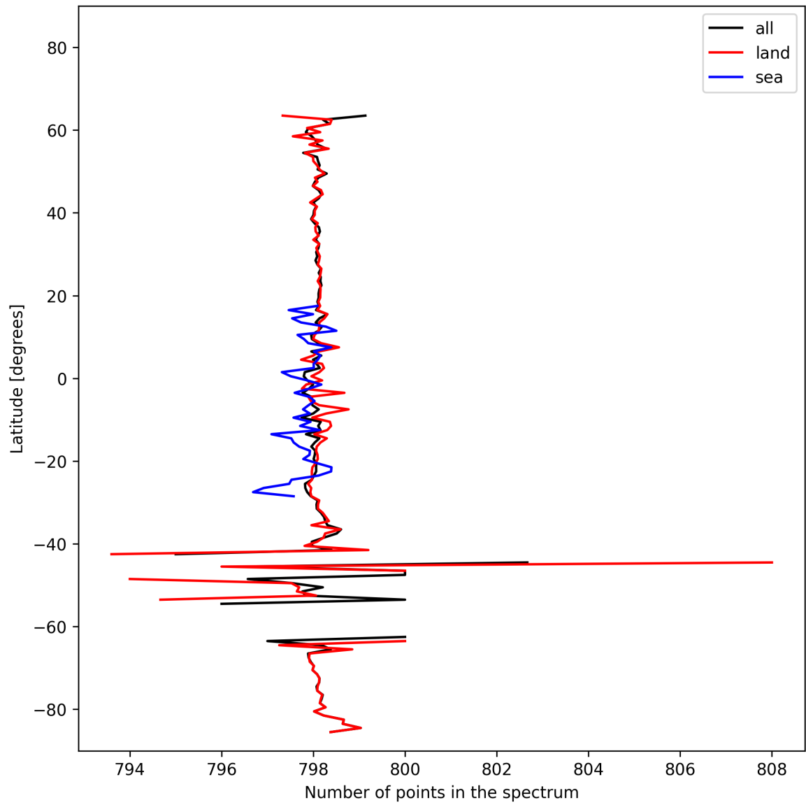
Figure 15: Zonal average of “Number of points in the spectrum” for 2024-10-24 to 2024-10-25.
