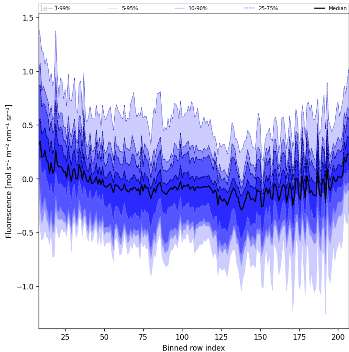
Figure 43: Along track statistics of “Fluorescence” for 2024-10-24 to 2024-10-25
