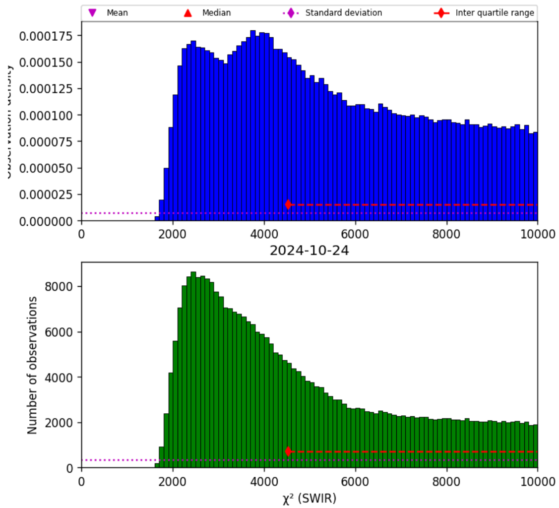
Figure 28: Histogram of “ \chi^2 (SWIR)” for 2024-10-24 to 2024-10-25
