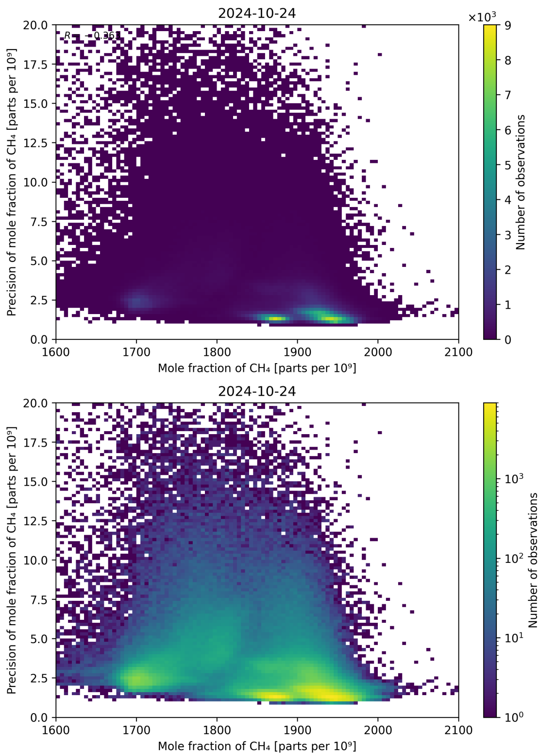
Figure 75: Scatter density plot of “Mole fraction of CH 4 ” against “Precision of mole fraction of CH 4 ” for 2024-10-24 to 2024-10-25.
