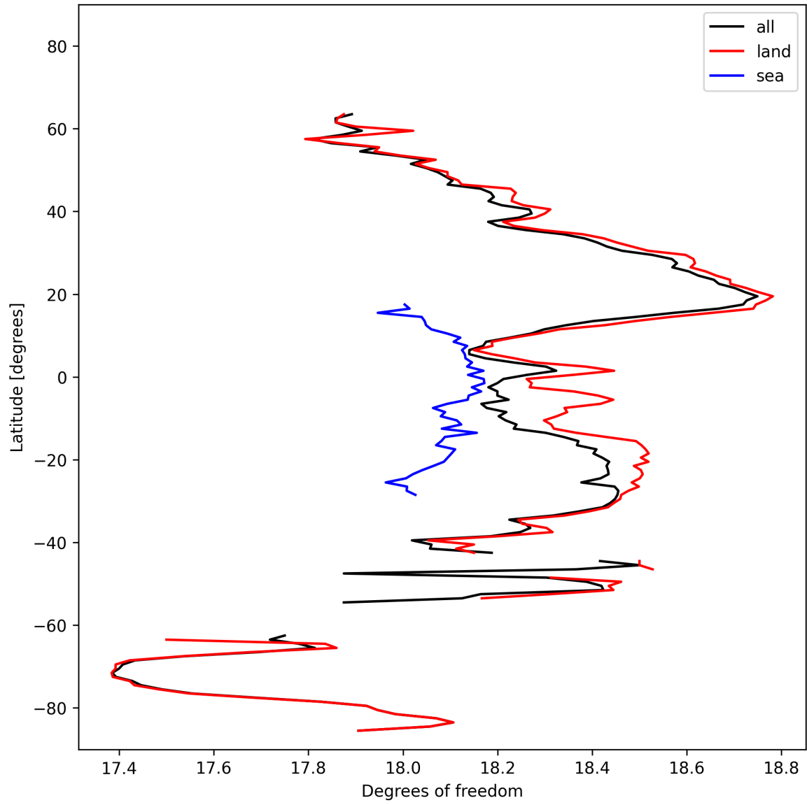
Figure 19: Zonal average of “Degrees of freedom” for 2024-10-24 to 2024-10-25.
