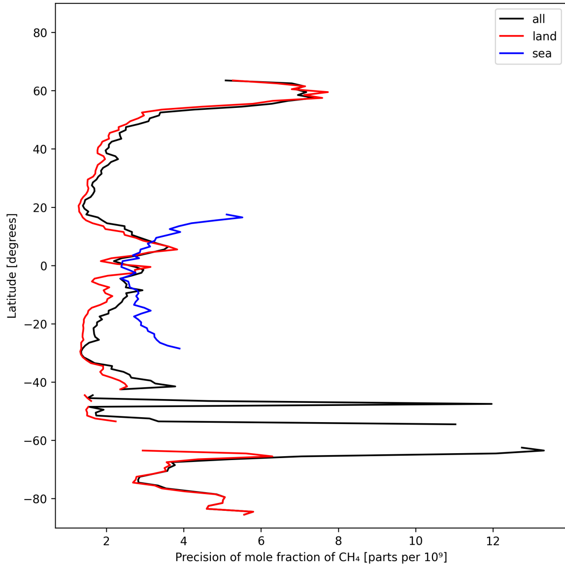
Figure 13: Zonal average of “Precision of mole fraction of CH 4 ” for 2024-10-24 to 2024-10-25.
