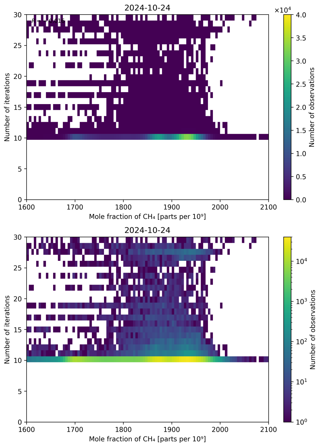
Figure 76: Scatter density plot of “Mole fraction of CH 4 ” against “Number of iterations” for 2024-10-24 to 2024-10-25.
