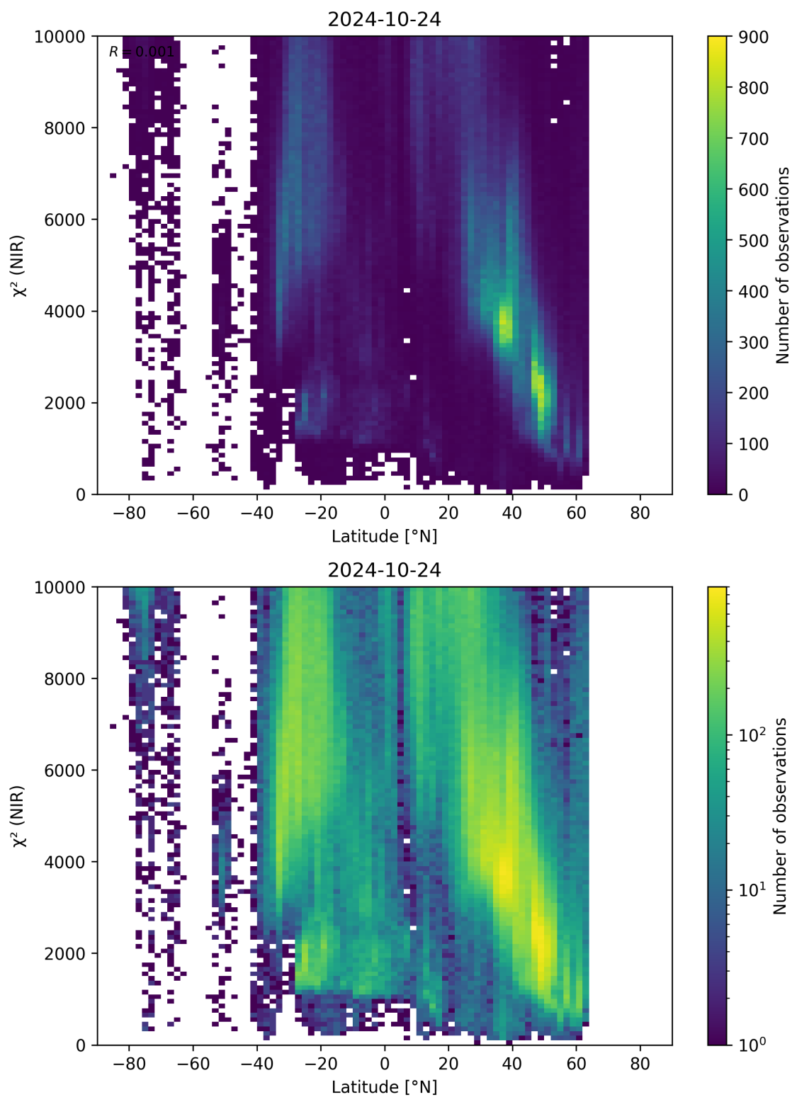
Figure 53: Scatter density plot of “Latitude” against “ \chi^2 (NIR)” for 2024-10-24 to 2024-10-25.
