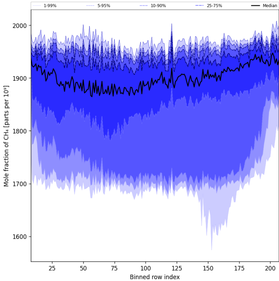
Figure 34: Along track statistics of “Mole fraction of CH 4 ” for 2024-10-24 to 2024-10-25
