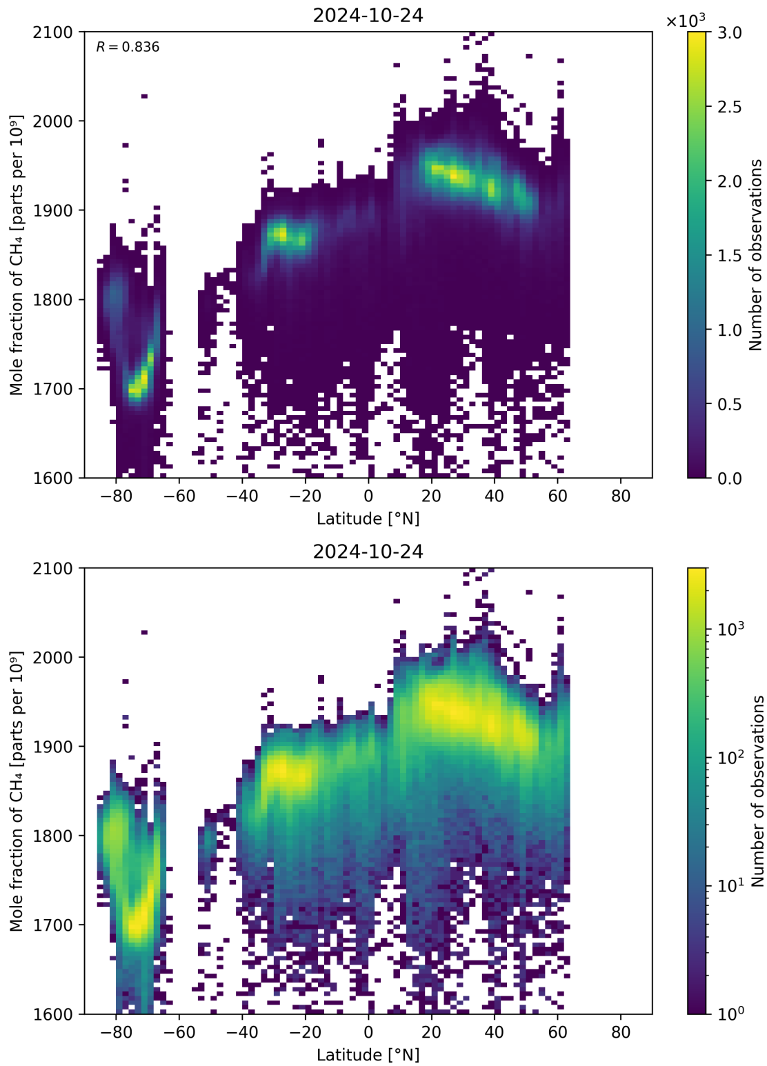
Figure 57: Scatter density plot of “Latitude” against “Mole fraction of CH 4 ” for 2024-10-24 to 2024-10-25.
