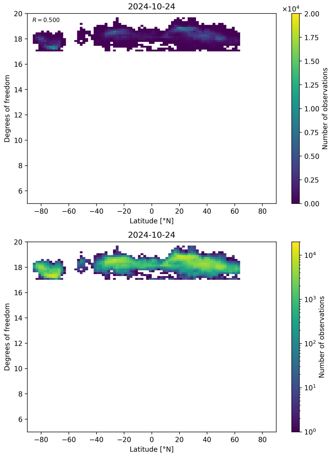
Figure 55: Scatter density plot of “Latitude” against “Degrees of freedom” for 2024-10-24 to 2024-10-25.
