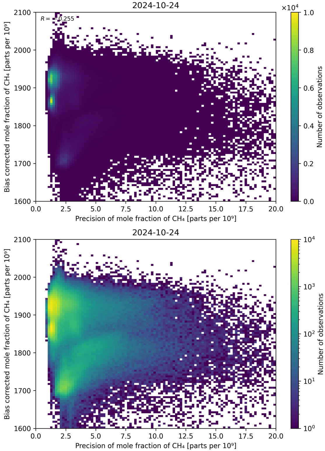
Figure 82: Scatter density plot of “Precision of mole fraction of \text{CH}_4 ” against “Bias corrected mole fraction of \text{CH}_4 ” for 2024-10-24 to 2024-10-25.
