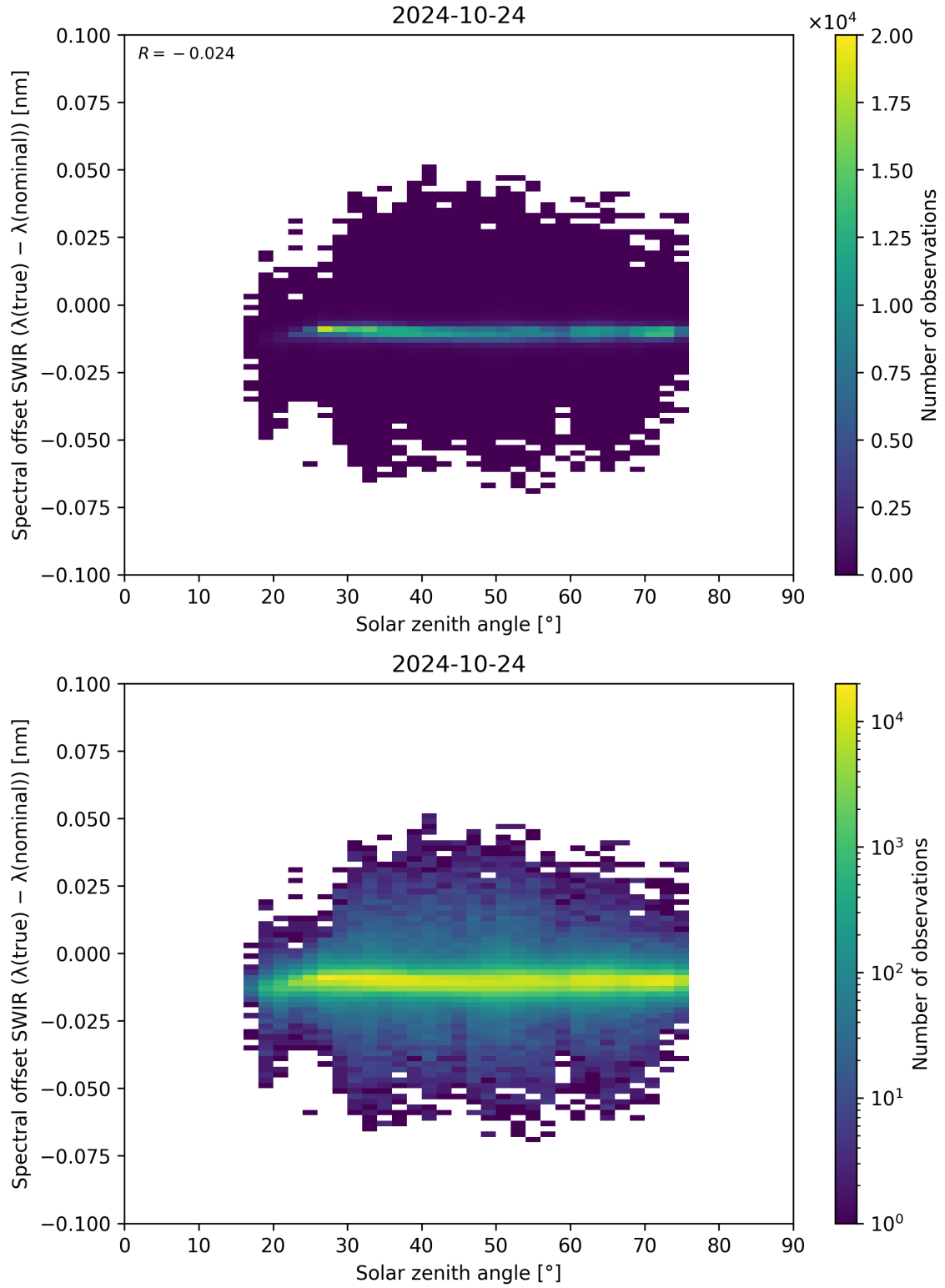
Figure 104: Scatter density plot of “Solar zenith angle” against “Spectral offset SWIR ( \lambda_{\text{true}} - \lambda_{\text{nominal}} )” for 2024-10-24 to 2024-10-25.
