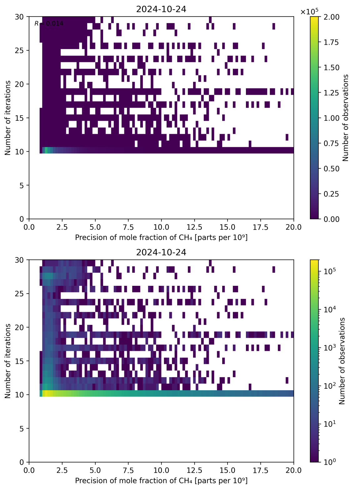
Figure 83: Scatter density plot of “Precision of mole fraction of CH 4 ” against “Number of iterations” for 2024-10-24 to 2024-10-25.
