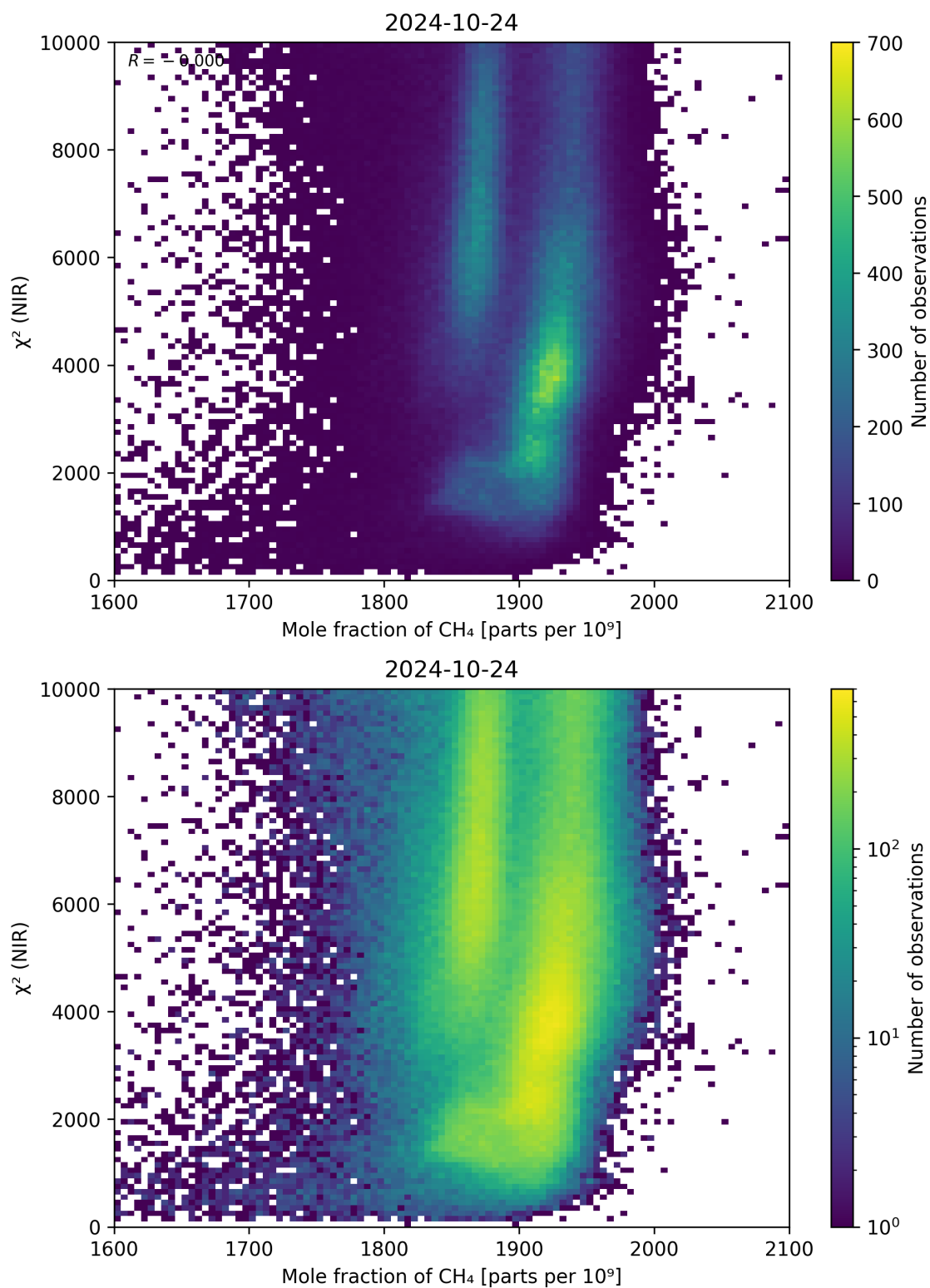
Figure 70: Scatter density plot of “Mole fraction of \text{CH}_4 ” against “ \chi^2 (NIR)” for 2024-10-24 to 2024-10-25.
