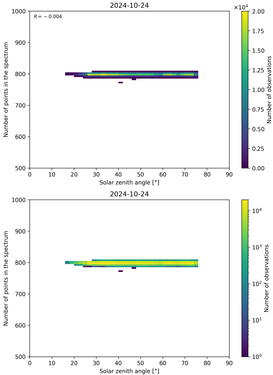
Figure 103: Scatter density plot of “Solar zenith angle” against “Number of points in the spectrum” for 2024-10-24 to 2024-10-25.
