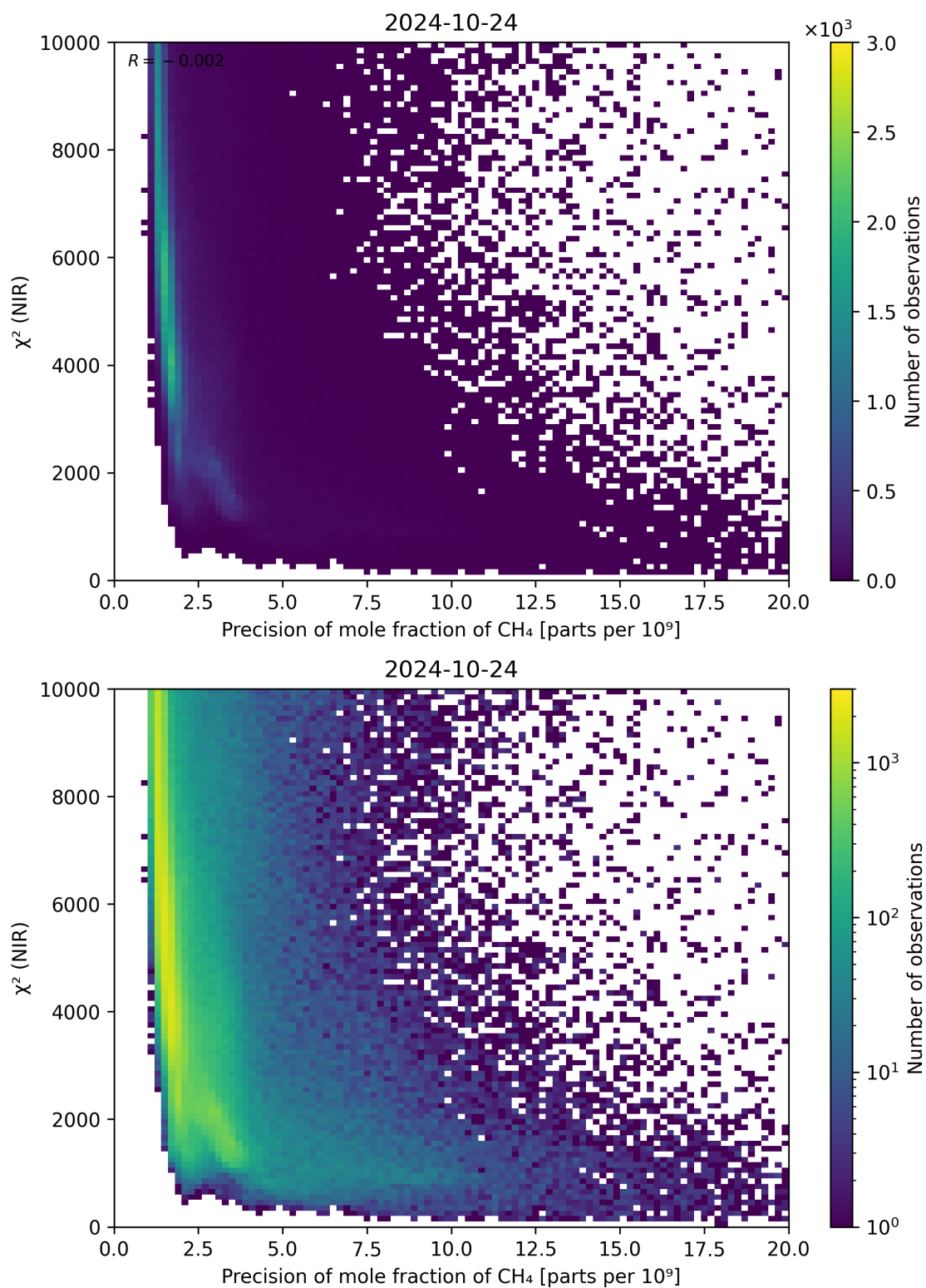
Figure 78: Scatter density plot of “Precision of mole fraction of \text{CH}_4 ” against “ \chi^2 (NIR)” for 2024-10-24 to 2024-10-25.
