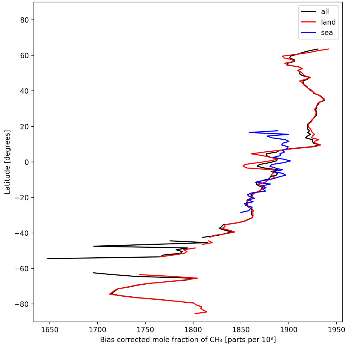
Figure 14: Zonal average of “Bias corrected mole fraction of CH 4 ” for 2024-10-24 to 2024-10-25.
