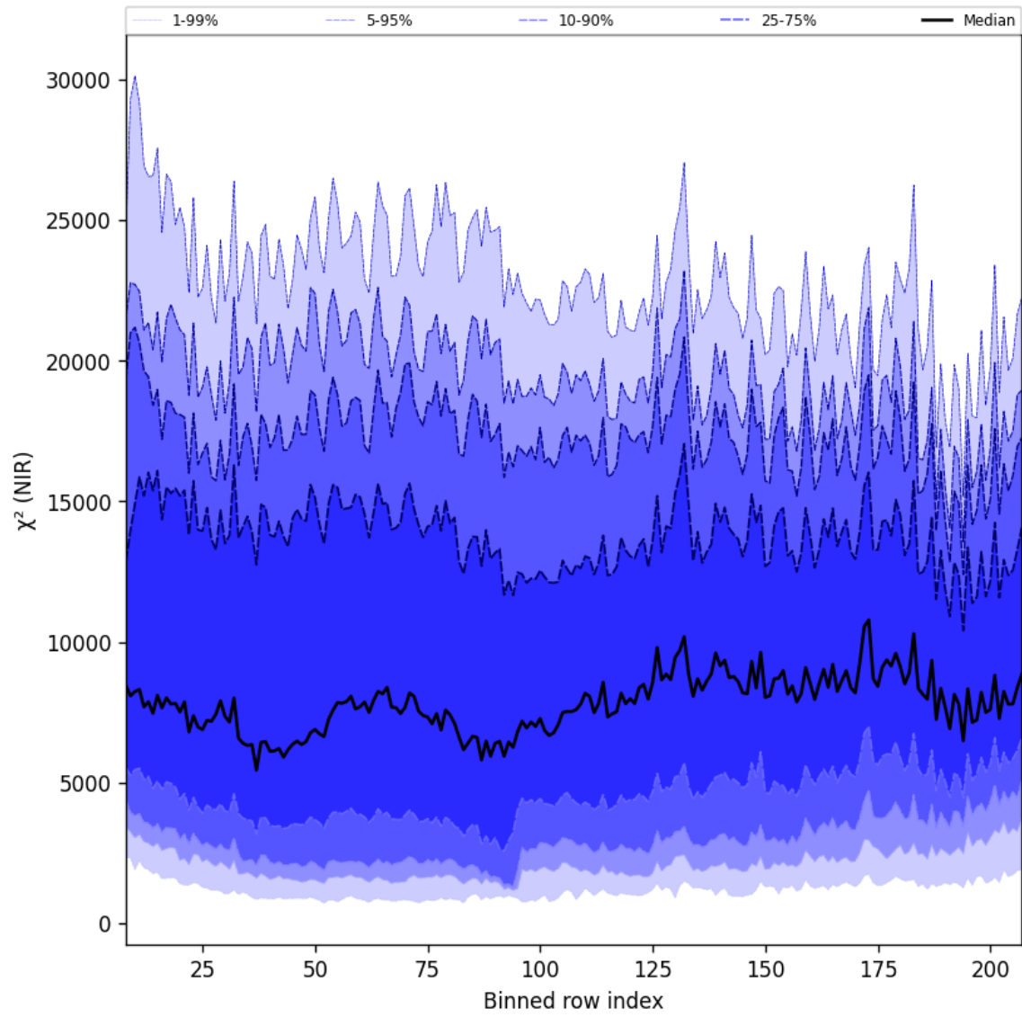
Figure 40: Along track statistics of " \chi^2 (NIR)" for 2024-10-24 to 2024-10-25
