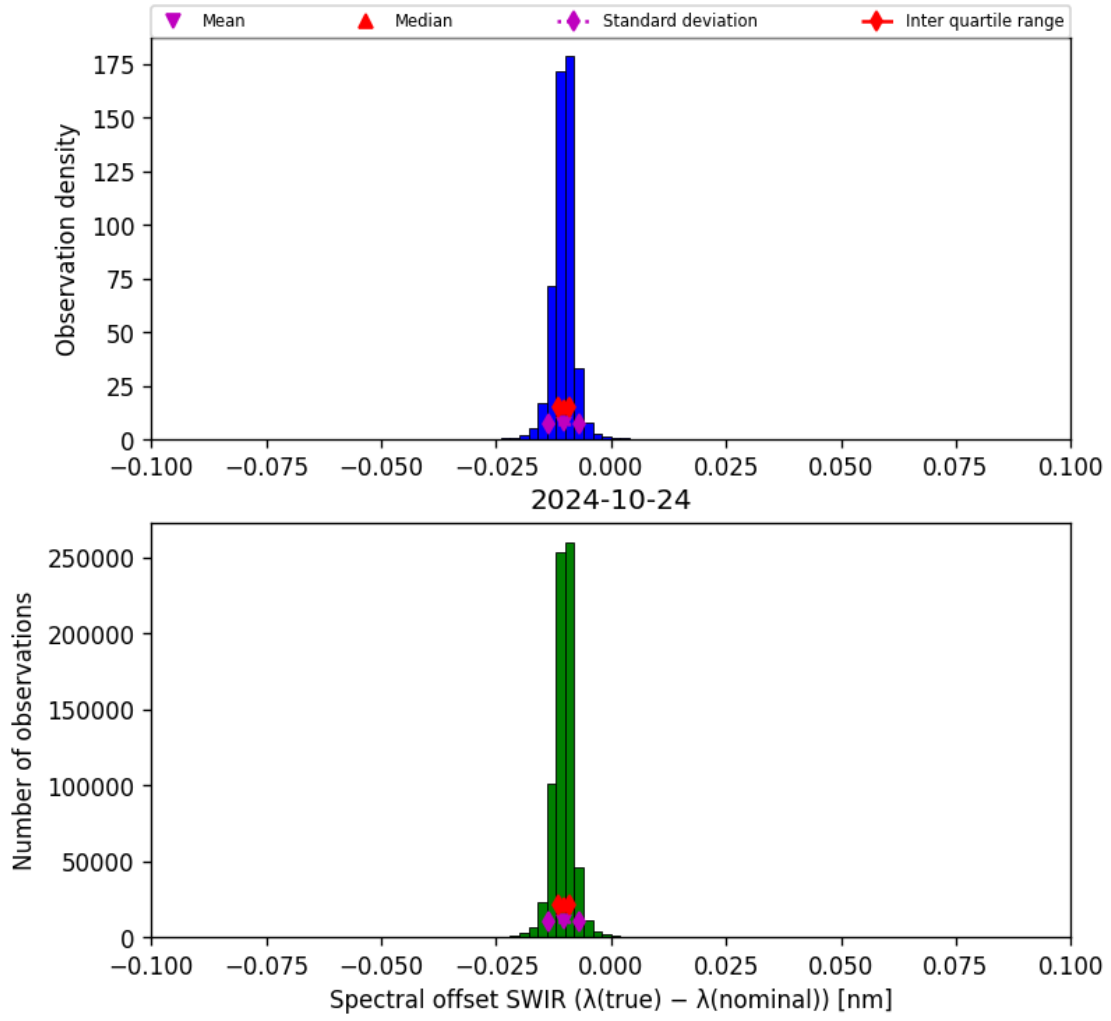
Figure 27: Histogram of “Spectral offset SWIR ( \lambda_{\text{true}} - \lambda_{\text{nominal}} )” for 2024-10-24 to 2024-10-25
