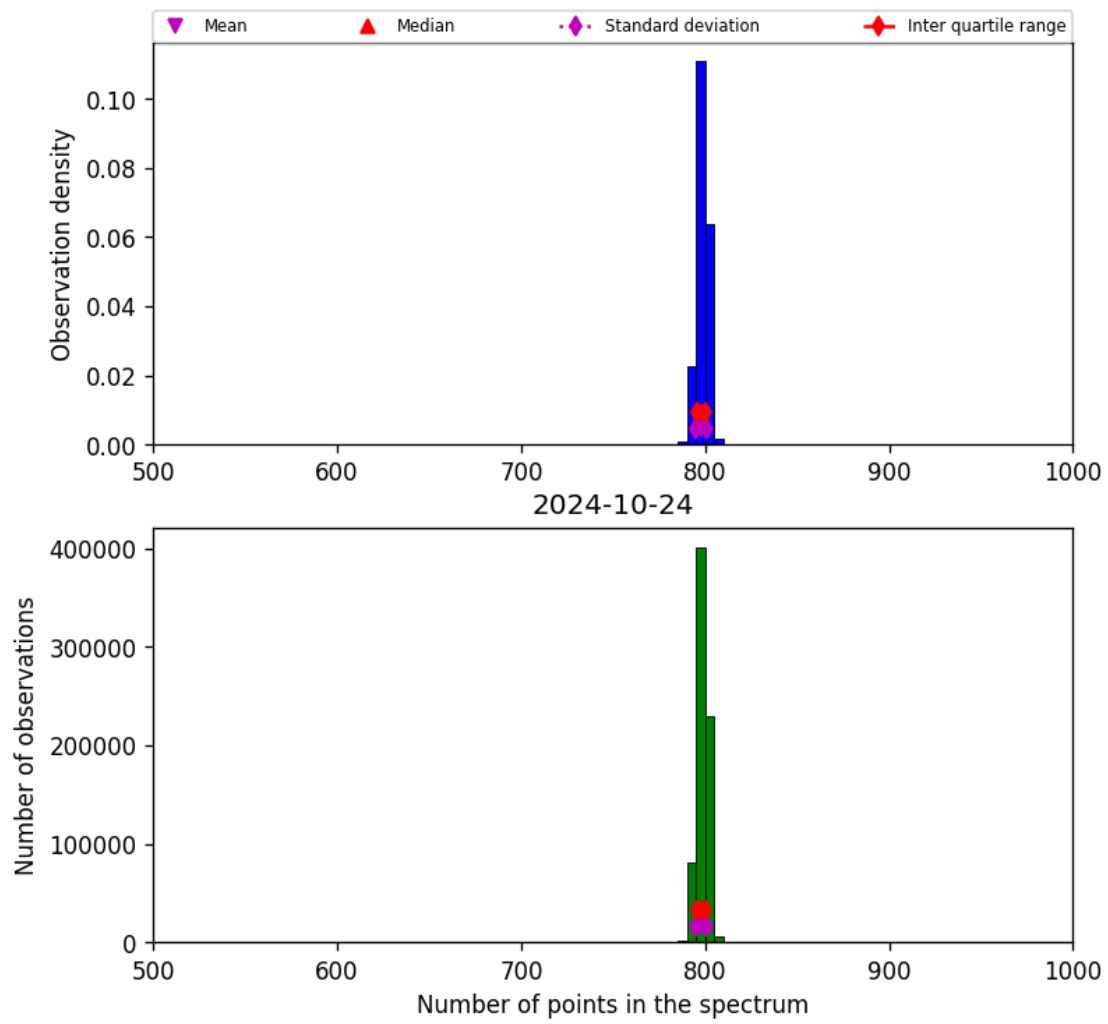
Figure 26: Histogram of “Number of points in the spectrum” for 2024-10-24 to 2024-10-25
