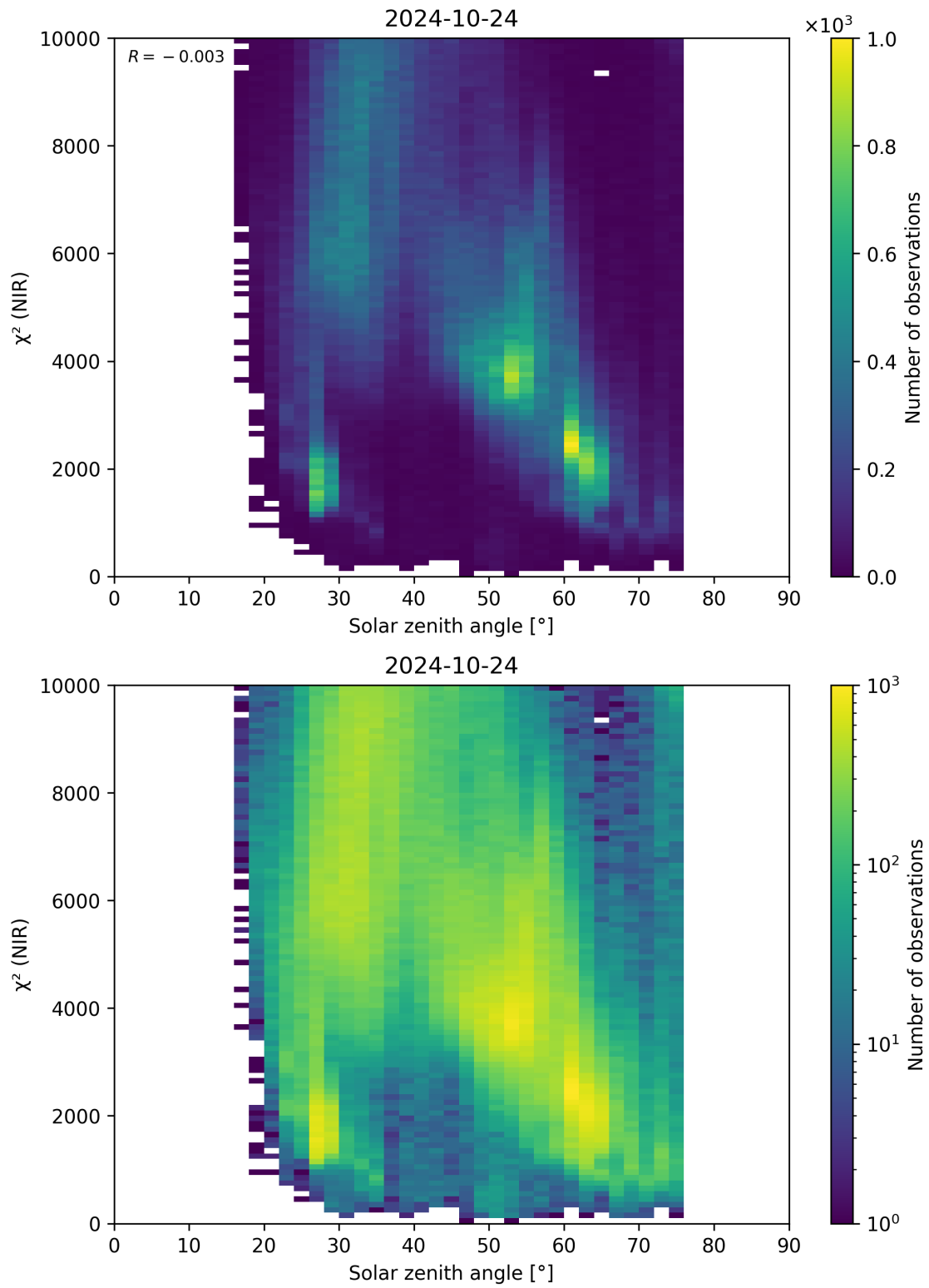
Figure 94: Scatter density plot of “Solar zenith angle” against “ \chi^2 (NIR)” for 2024-10-24 to 2024-10-25.
