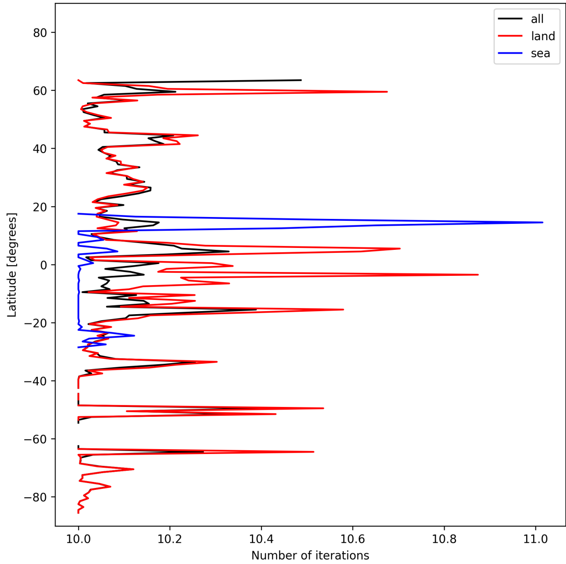
Figure 20: Zonal average of “Number of iterations” for 2024-10-24 to 2024-10-25.
