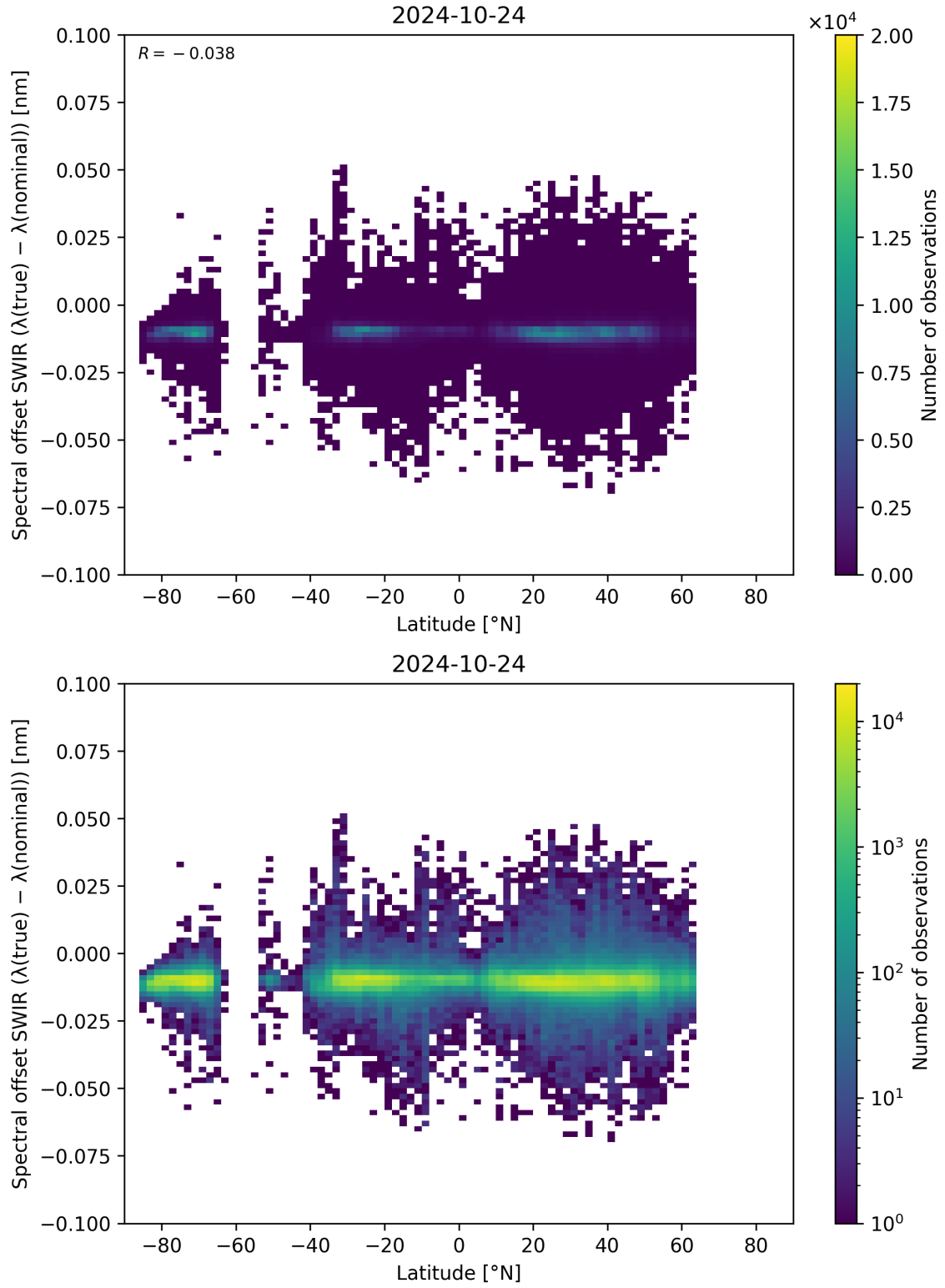
Figure 62: Scatter density plot of “Latitude” against “Spectral offset SWIR ( \lambda_{\text{true}} - \lambda_{\text{nominal}} )” for 2024-10-24 to 2024-10-25.
