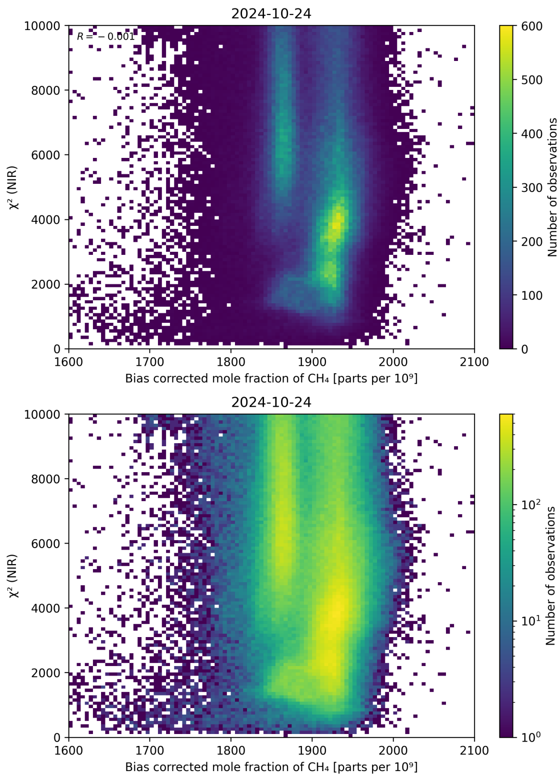
Figure 63: Scatter density plot of “Bias corrected mole fraction of CH 4 ” against “ \chi^2 (NIR)” for 2024-10-24 to 2024-10-25.
