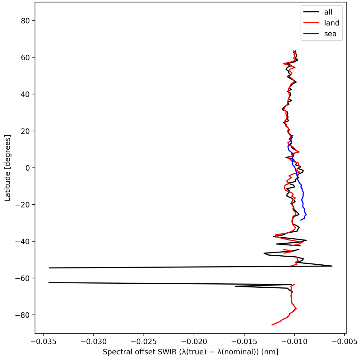
Figure 16: Zonal average of “Spectral offset SWIR ( \lambda_{\text{true}} - \lambda_{\text{nominal}} )” for 2024-10-24 to 2024-10-25.
