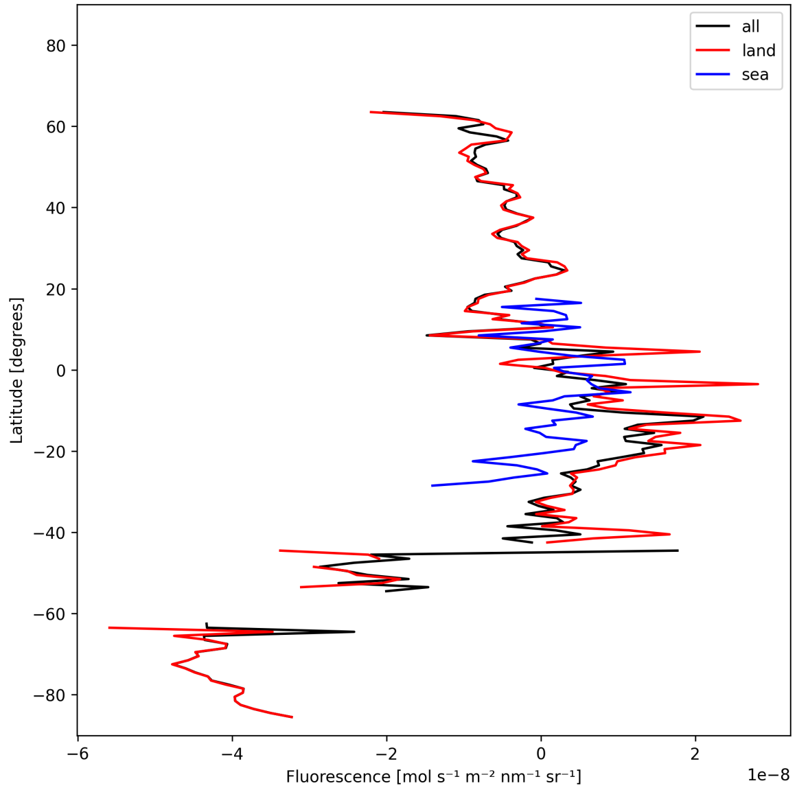
Figure 21: Zonal average of “Fluorescence” for 2024-10-24 to 2024-10-25.
