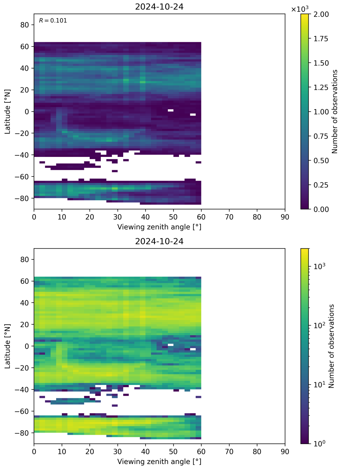
Figure 109: Scatter density plot of “Viewing zenith angle” against “Latitude” for 2024-10-24 to 2024-10-25.
