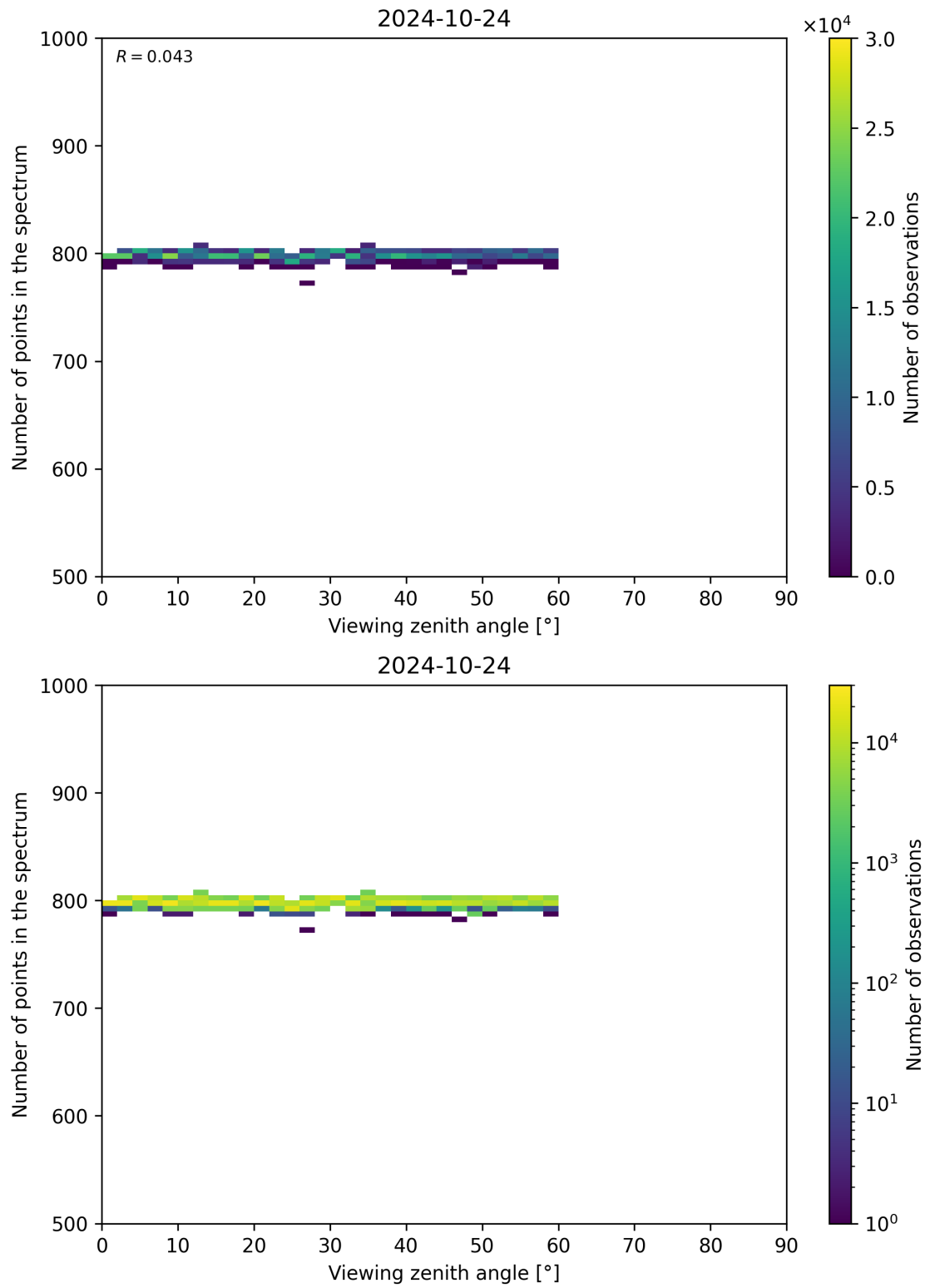
Figure 114: Scatter density plot of “Viewing zenith angle” against “Number of points in the spectrum” for 2024-10-24 to 2024-10-25.
