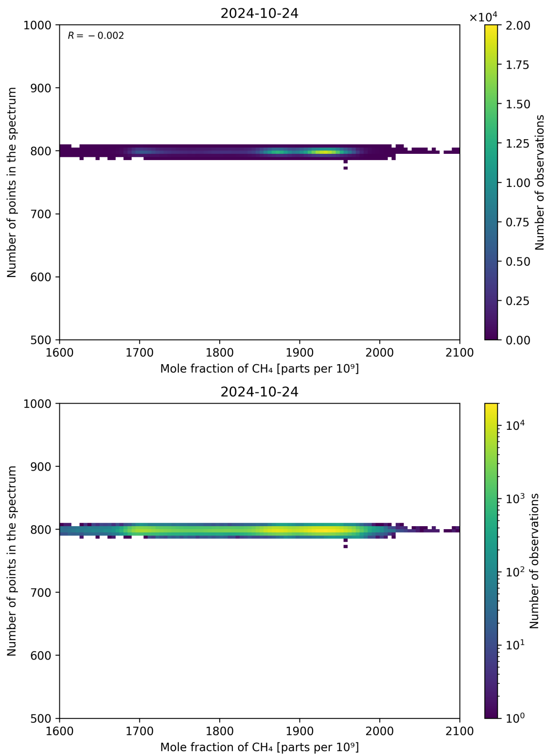
Figure 77: Scatter density plot of “Mole fraction of CH 4 ” against “Number of points in the spectrum” for 2024-10-24 to 2024-10-25.
