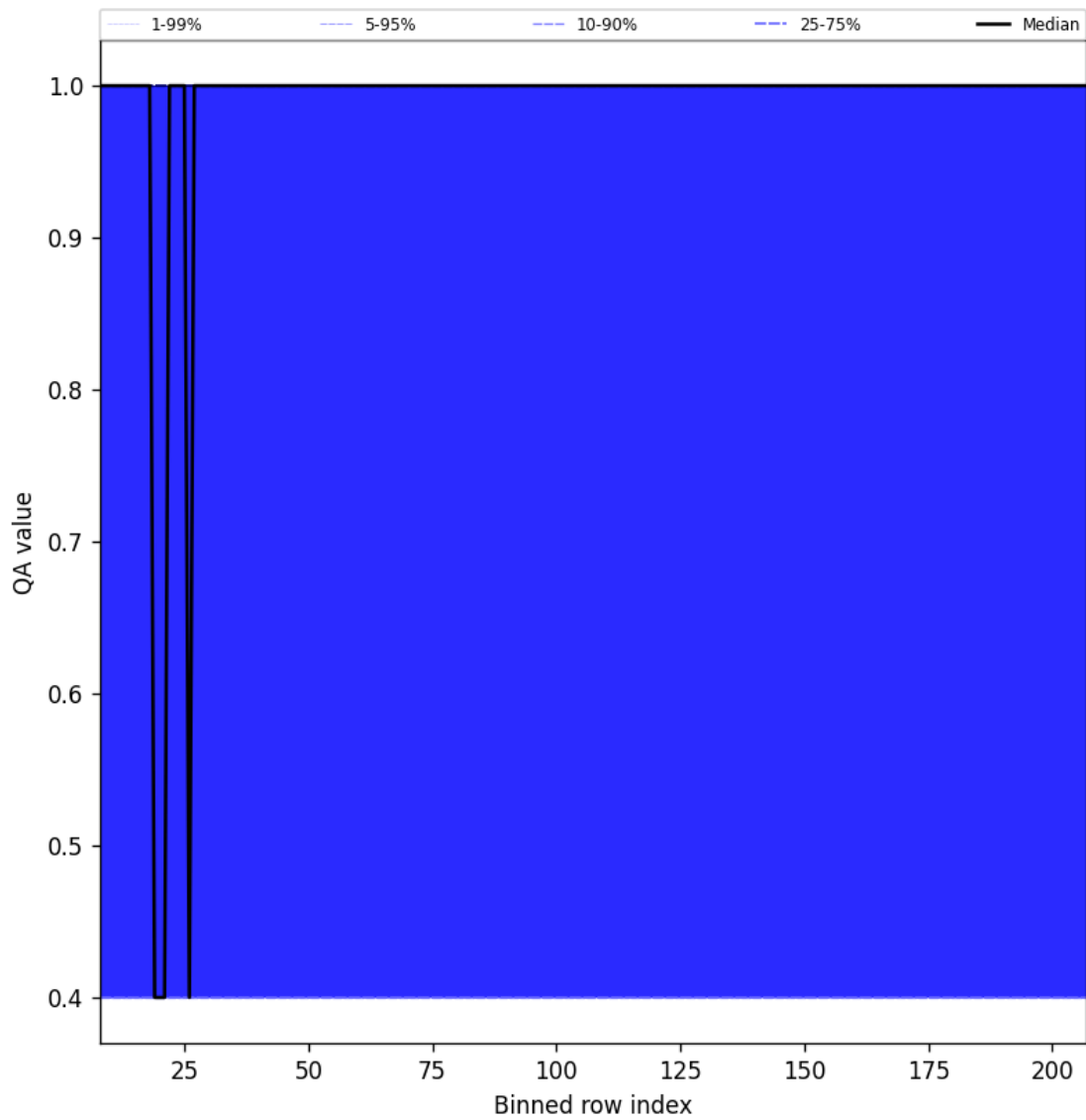
Figure 33: Along track statistics of “QA value” for 2024-10-24 to 2024-10-25
