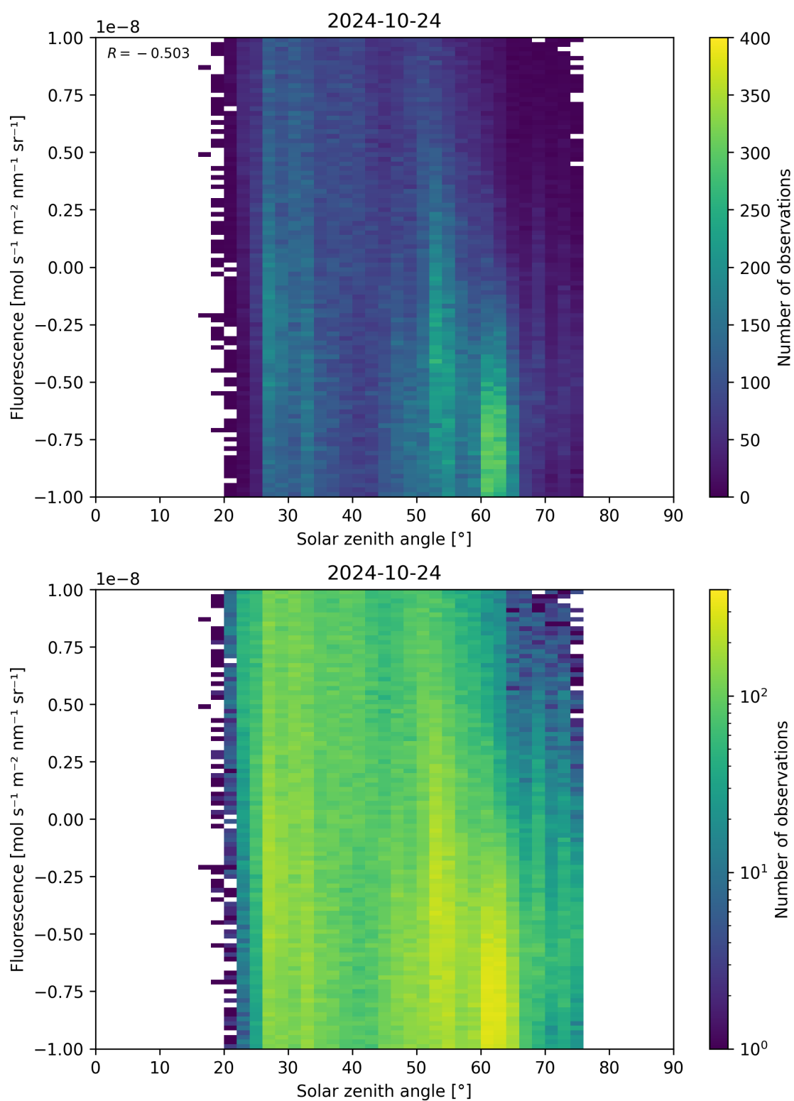
Figure 97: Scatter density plot of “Solar zenith angle” against “Fluorescence” for 2024-10-24 to 2024-10-25.
