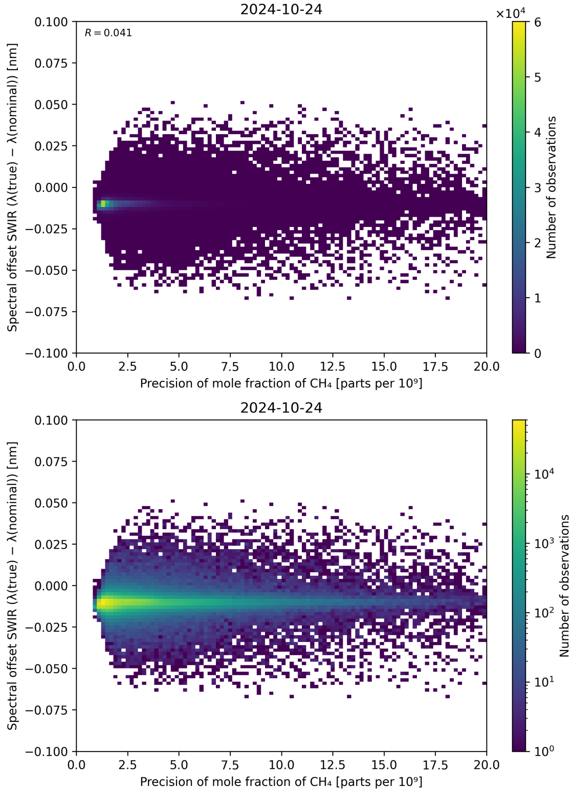
Figure 85: Scatter density plot of “Precision of mole fraction of CH 4 ” against “Spectral offset SWIR ( \lambda_{\text{true}} - \lambda_{\text{nominal}} )” for 2024-10-24 to 2024-10-25.
