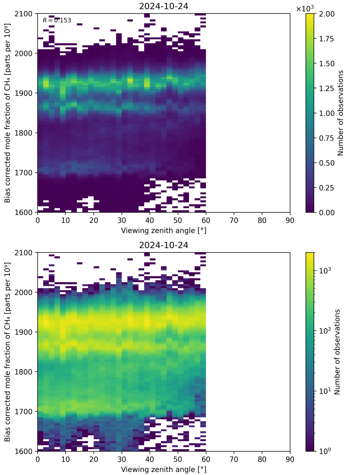
Figure 111: Scatter density plot of “Viewing zenith angle” against “Bias corrected mole fraction of CH 4 ” for 2024-10-24 to 2024-10-25.
