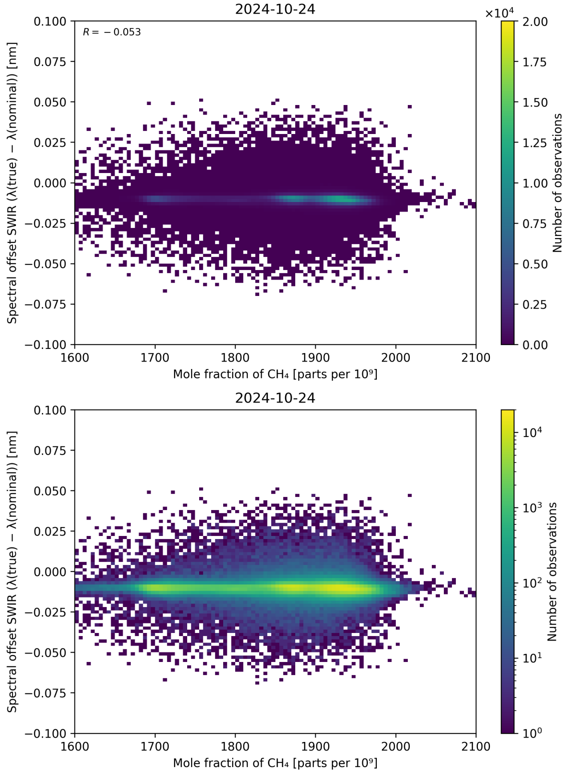
Figure 86: Scatter density plot of “Mole fraction of CH 4 ” against “Spectral offset SWIR ( \lambda_{\text{true}} - \lambda_{\text{nominal}} )” for 2024-10-24 to 2024-10-25.
