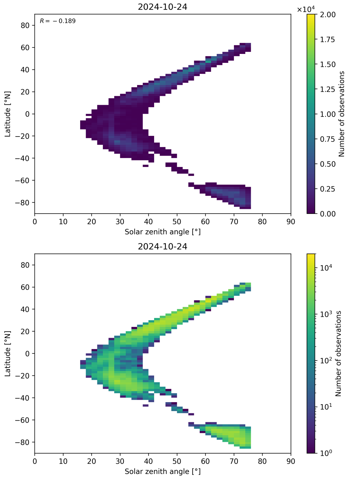
Figure 98: Scatter density plot of “Solar zenith angle” against “Latitude” for 2024-10-24 to 2024-10-25.
