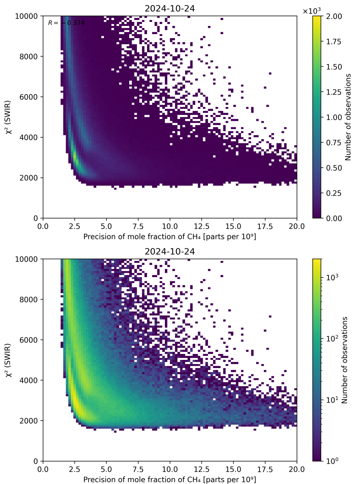
Figure 79: Scatter density plot of “Precision of mole fraction of \text{CH}_4 ” against “ \chi^2 (SWIR)” for 2024-10-24 to 2024-10-25.
