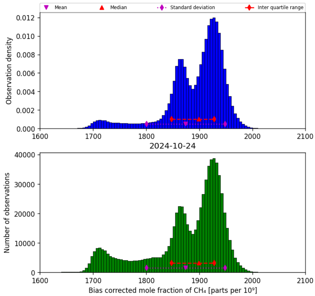
Figure 25: Histogram of “Bias corrected mole fraction of CH 4 ” for 2024-10-24 to 2024-10-25
