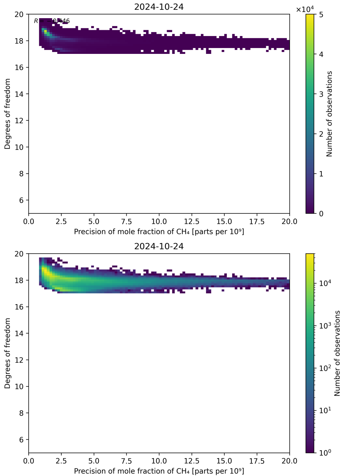
Figure 80: Scatter density plot of “Precision of mole fraction of CH 4 ” against “Degrees of freedom” for 2024-10-24 to 2024-10-25.
