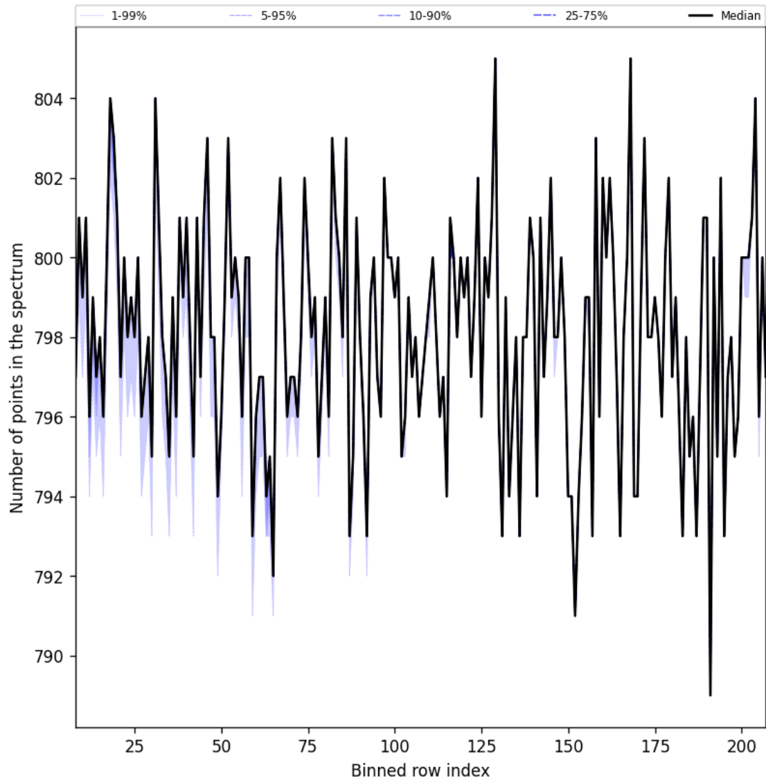
Figure 37: Along track statistics of “Number of points in the spectrum” for 2024-10-24 to 2024-10-25
