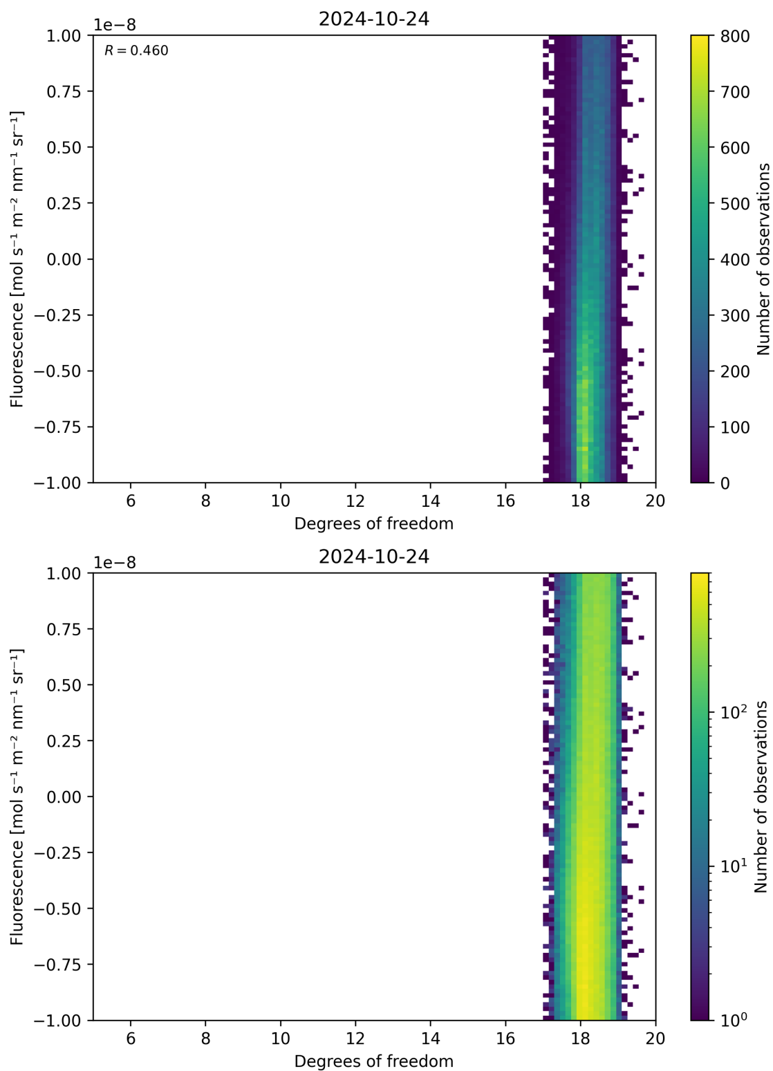
Figure 51: Scatter density plot of “Degrees of freedom” against “Fluorescence” for 2024-10-24 to 2024-10-25.
