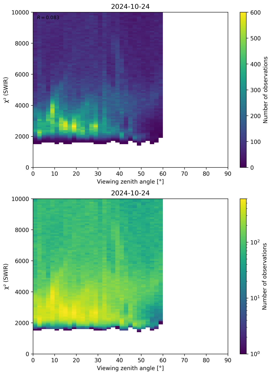
Figure 106: Scatter density plot of “Viewing zenith angle” against “ \chi^2 (SWIR)” for 2024-10-24 to 2024-10-25.
