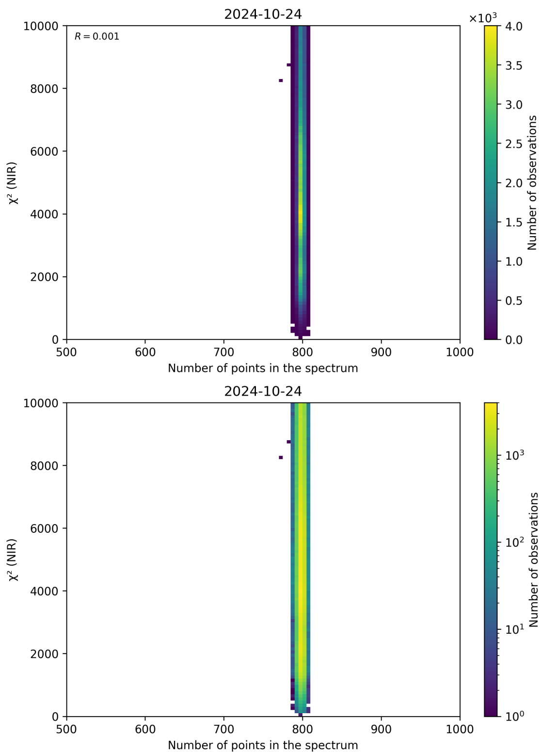
Figure 88: Scatter density plot of “Number of points in the spectrum” against “ \chi^2 (NIR)” for 2024-10-24 to 2024-10-25.
