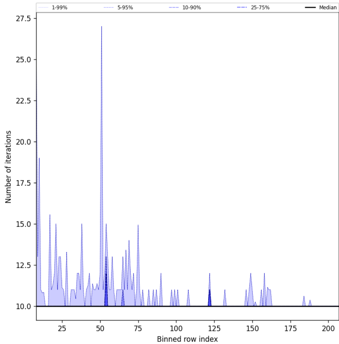
Figure 42: Along track statistics of “Number of iterations” for 2024-10-24 to 2024-10-25
