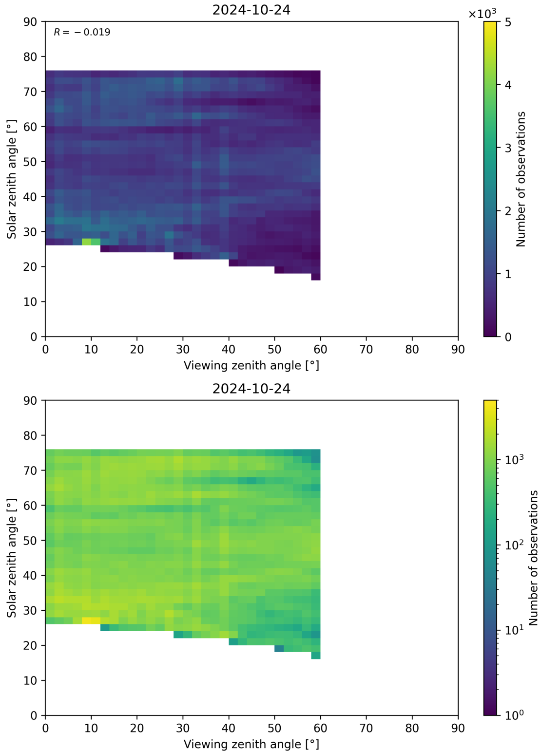
Figure 115: Scatter density plot of “Viewing zenith angle” against “Solar zenith angle” for 2024-10-24 to 2024-10-25.
