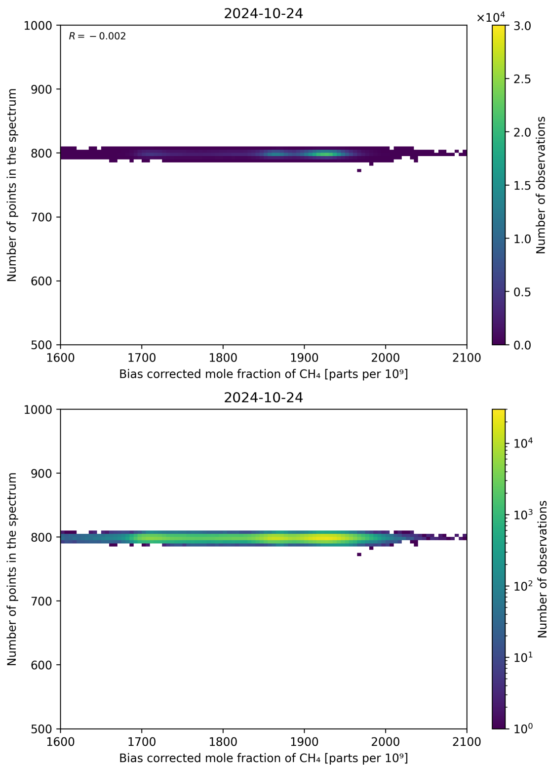
Figure 68: Scatter density plot of “Bias corrected mole fraction of CH 4 ” against “Number of points in the spectrum” for 2024-10-24 to 2024-10-25.
