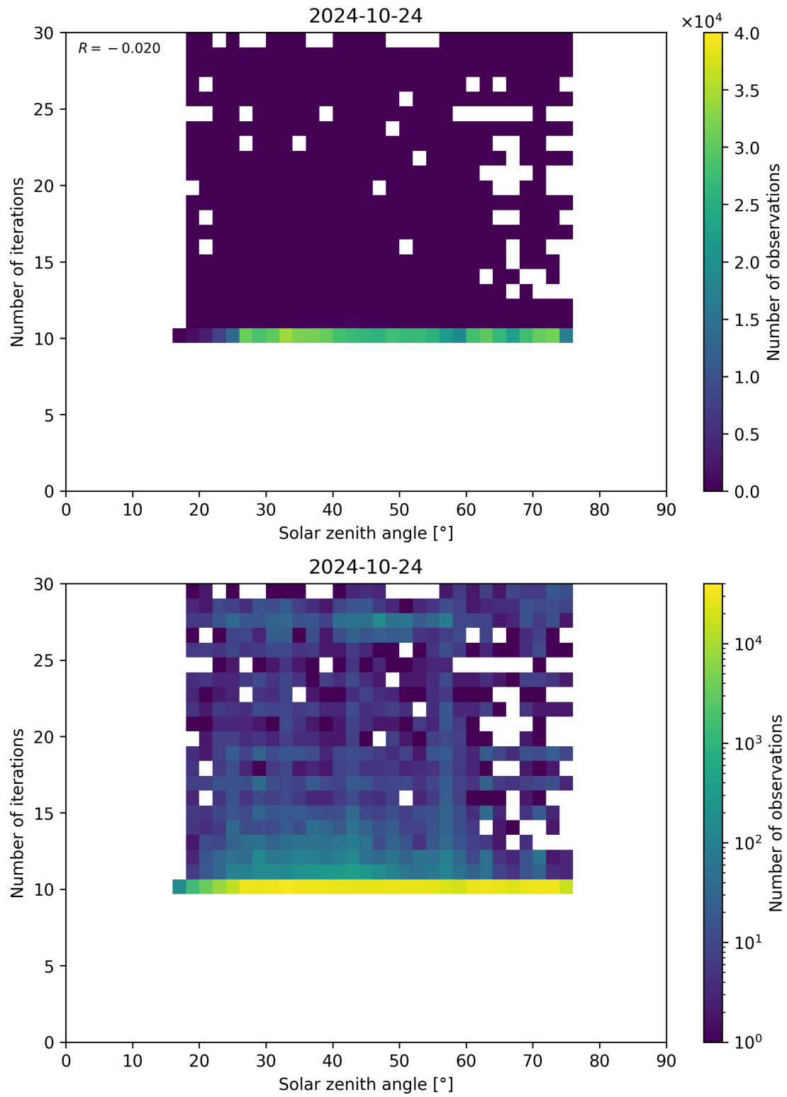
Figure 102: Scatter density plot of “Solar zenith angle” against “Number of iterations” for 2024-10-24 to 2024-10-25.
