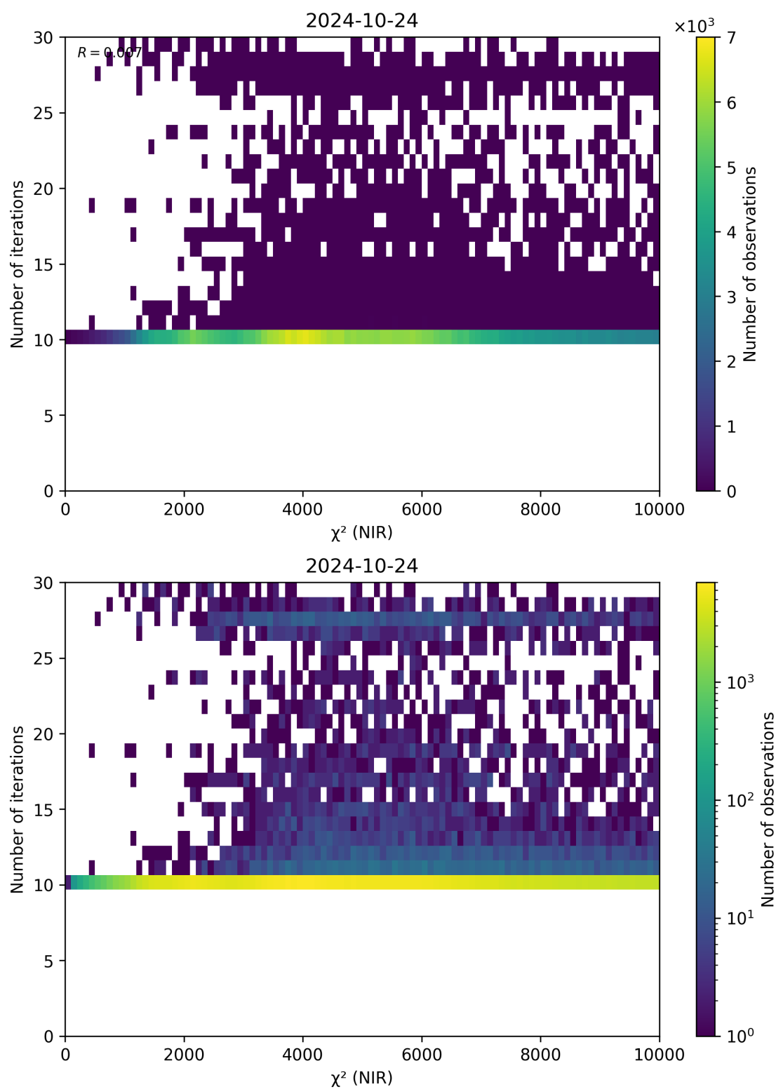
Figure 46: Scatter density plot of “ \chi^2 (NIR)” against “Number of iterations” for 2024-10-24 to 2024-10-25.
