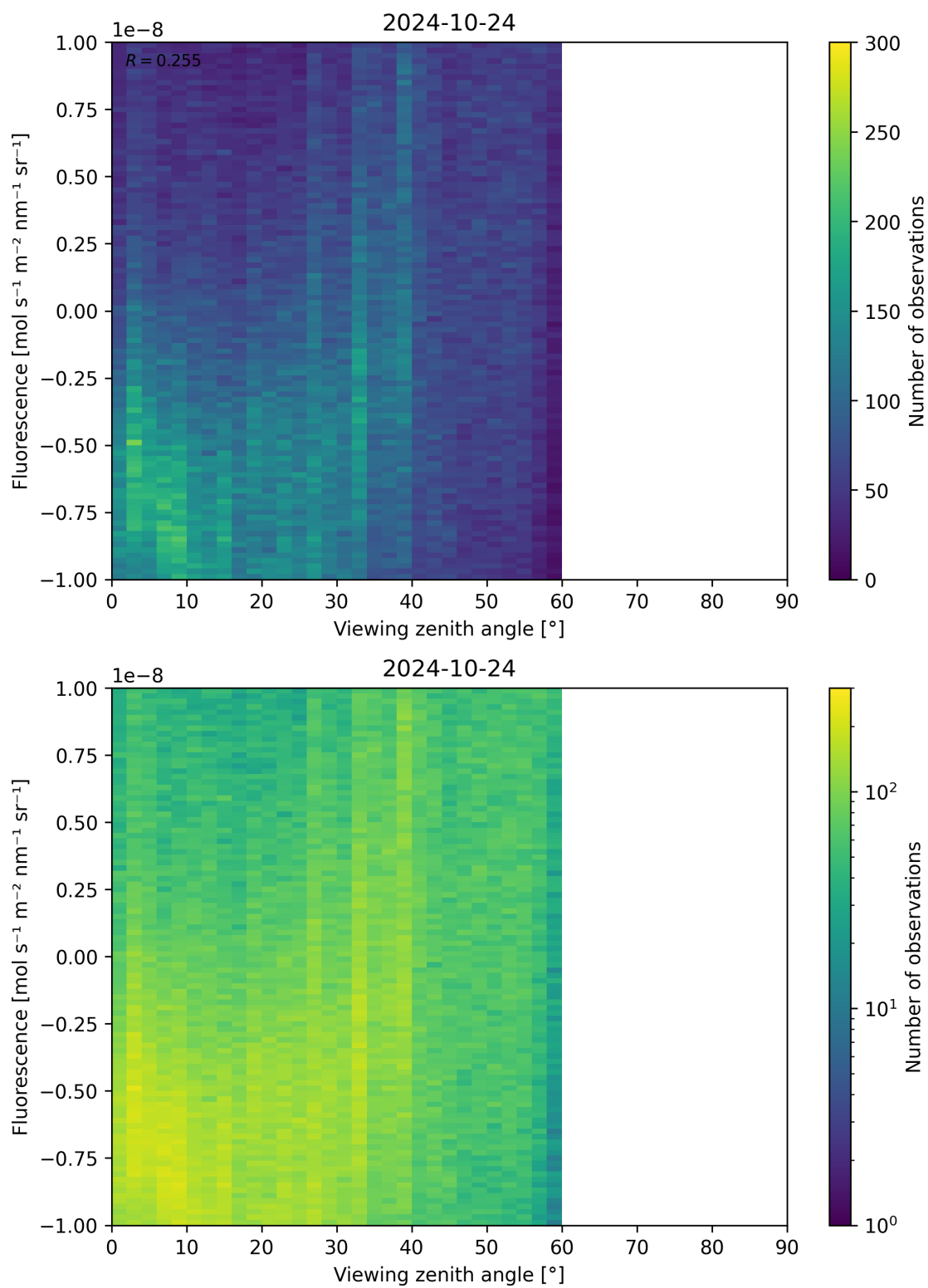
Figure 108: Scatter density plot of “Viewing zenith angle” against “Fluorescence” for 2024-10-24 to 2024-10-25.
