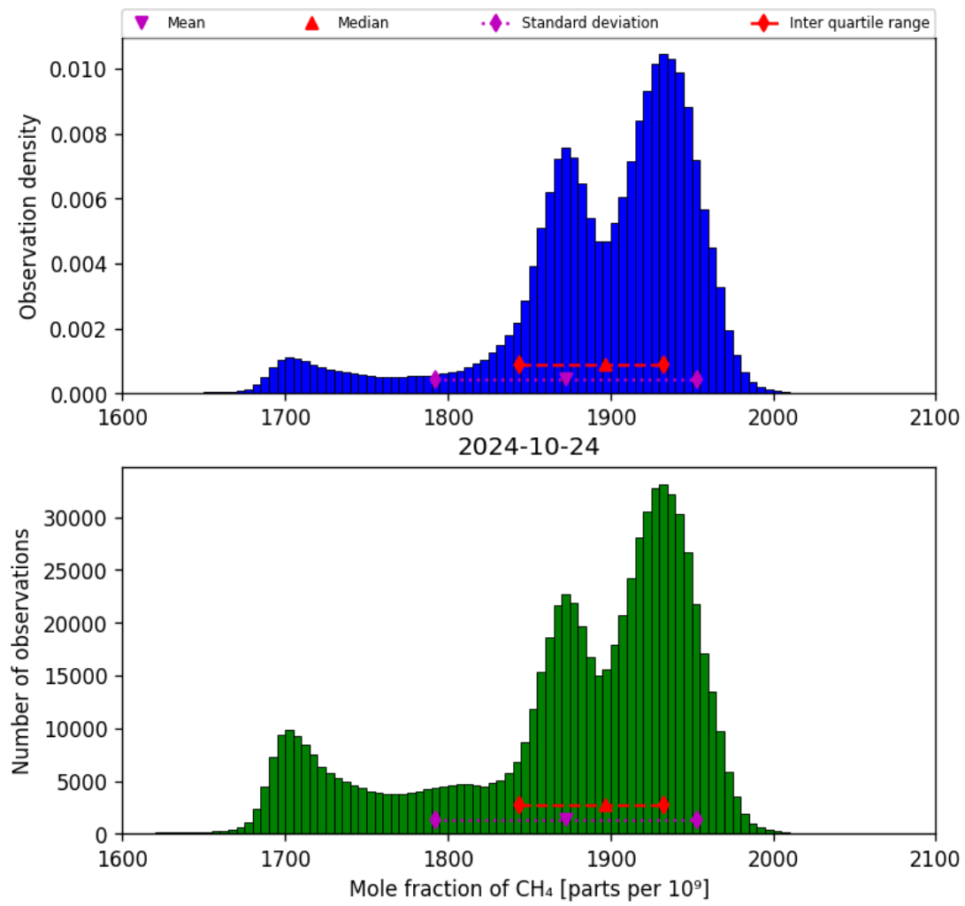
Figure 23: Histogram of “Mole fraction of CH 4 ” for 2024-10-24 to 2024-10-25
