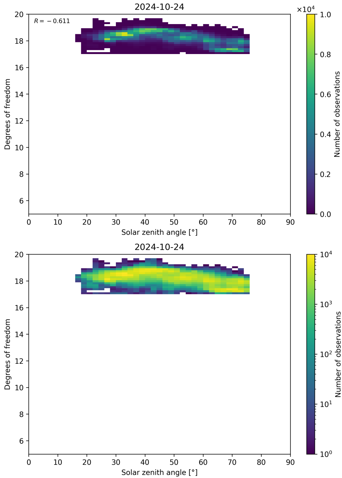
Figure 96: Scatter density plot of “Solar zenith angle” against “Degrees of freedom” for 2024-10-24 to 2024-10-25.
