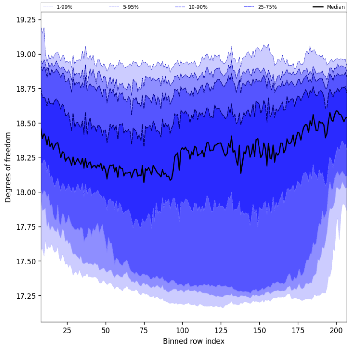
Figure 41: Along track statistics of “Degrees of freedom” for 2024-10-24 to 2024-10-25
