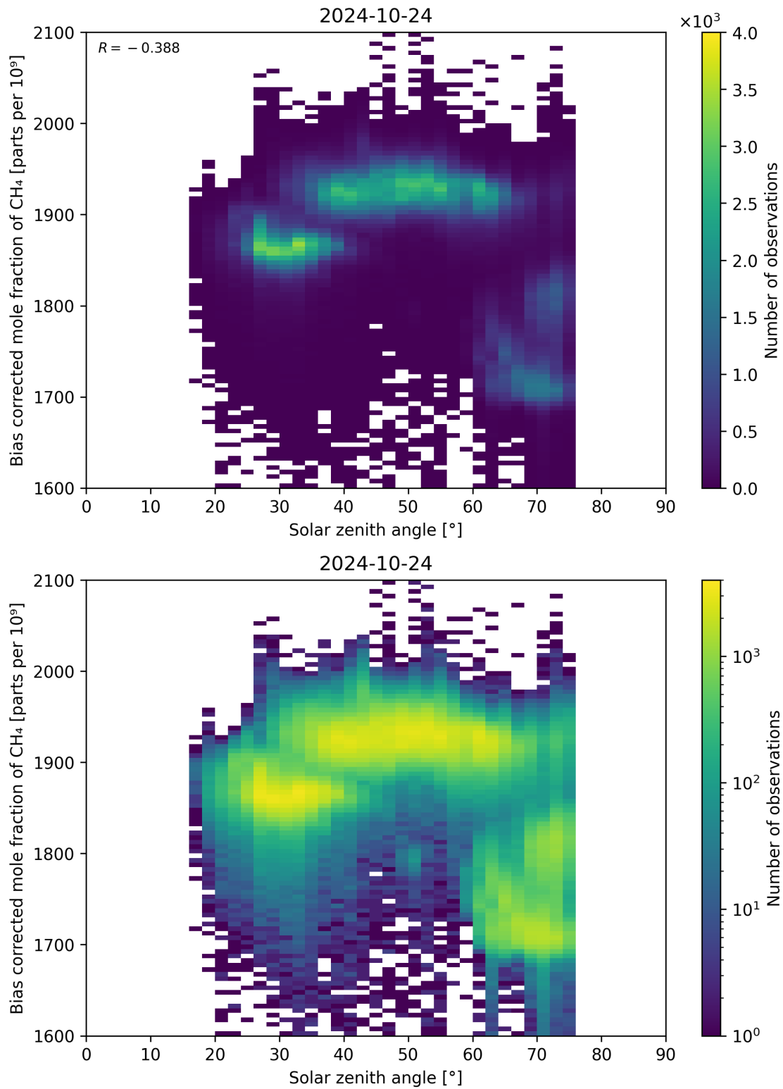
Figure 100: Scatter density plot of “Solar zenith angle” against “Bias corrected mole fraction of CH 4 ” for 2024-10-24 to 2024-10-25.
