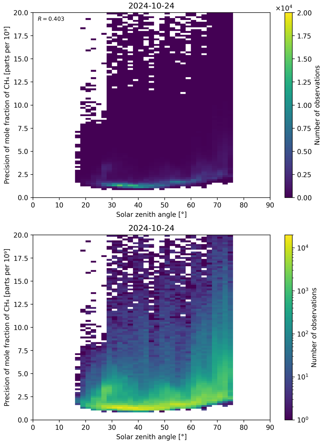
Figure 101: Scatter density plot of “Solar zenith angle” against “Precision of mole fraction of \text{CH}_4 ” for 2024-10-24 to 2024-10-25.
