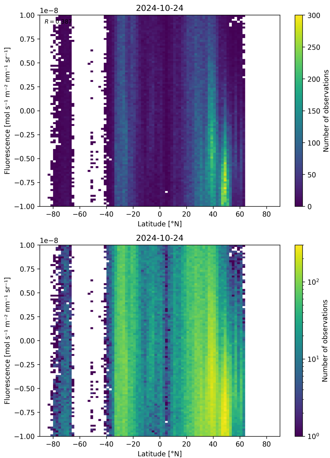
Figure 56: Scatter density plot of “Latitude” against “Fluorescence” for 2024-10-24 to 2024-10-25.
