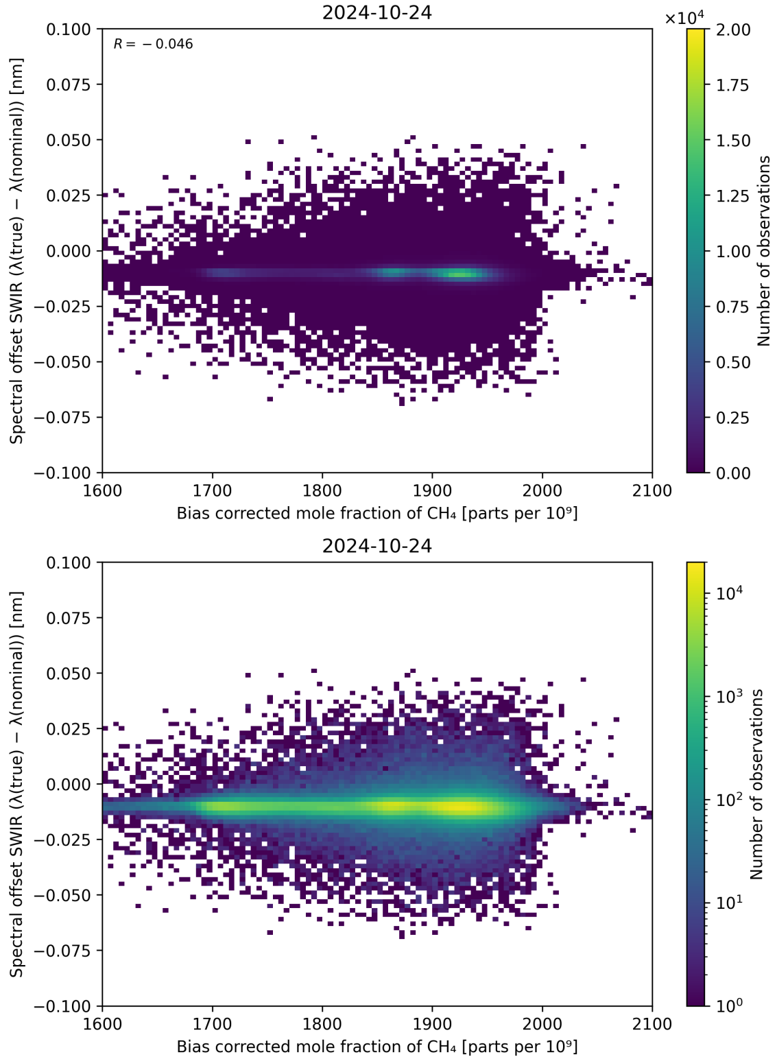
Figure 69: Scatter density plot of “Bias corrected mole fraction of CH 4 ” against “Spectral offset SWIR ( \lambda_{\text{true}} - \lambda_{\text{nominal}} )” for 2024-10-24 to 2024-10-25.
