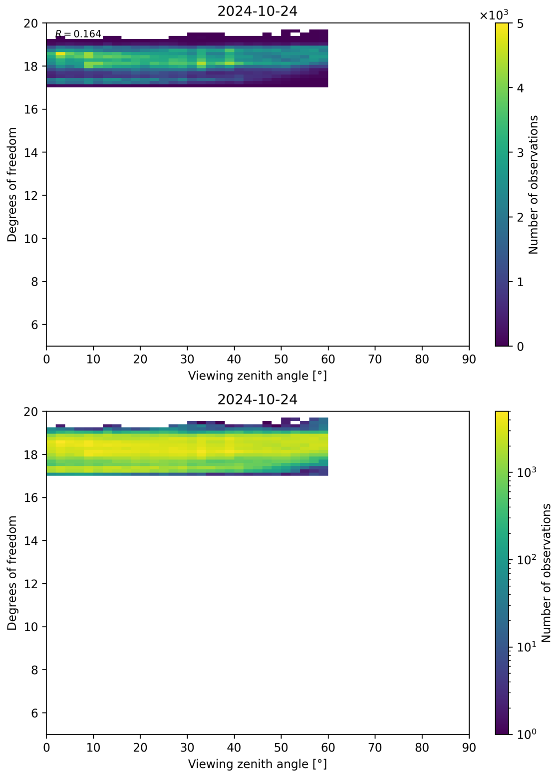
Figure 107: Scatter density plot of “Viewing zenith angle” against “Degrees of freedom” for 2024-10-24 to 2024-10-25.
