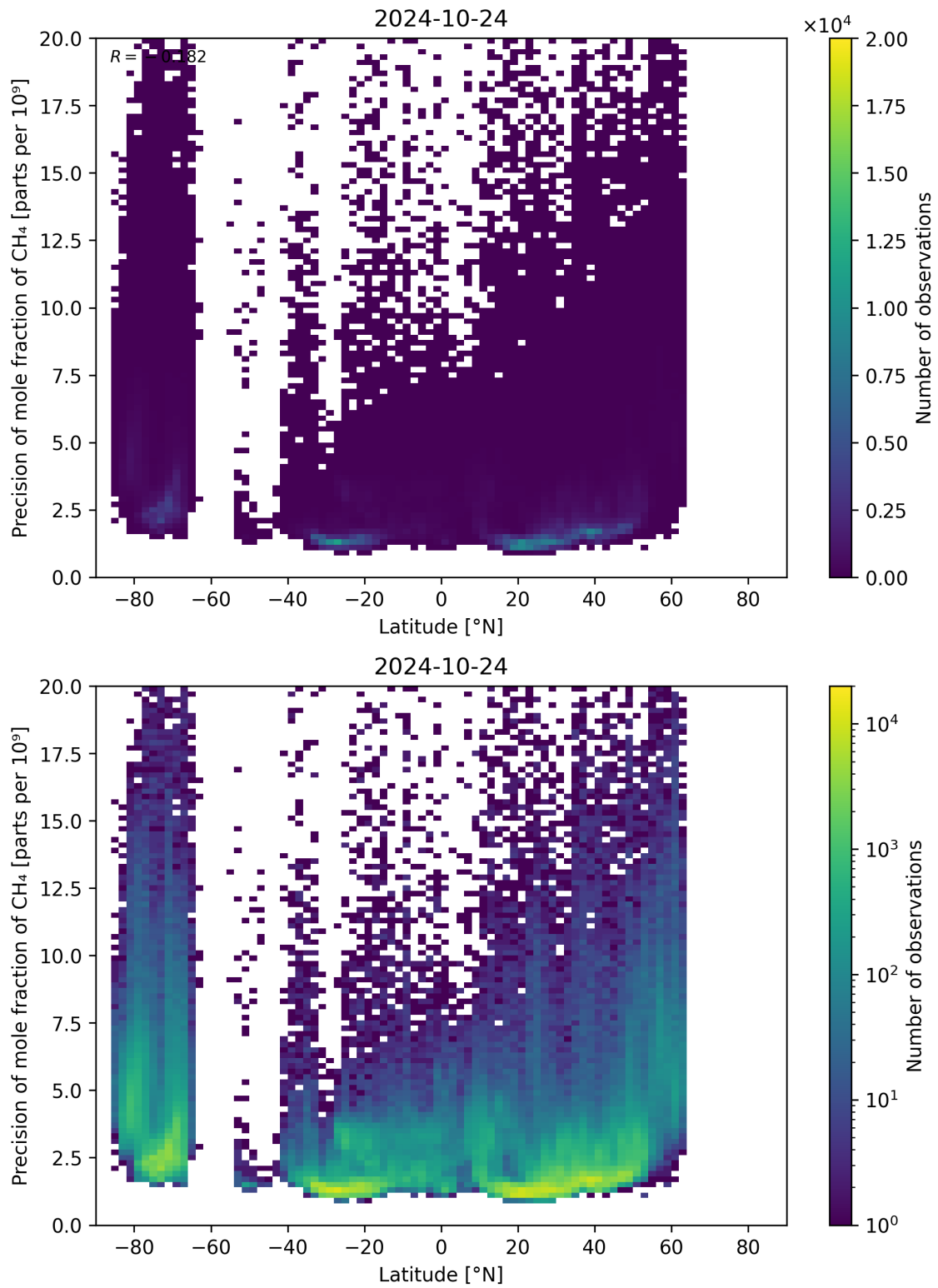
Figure 59: Scatter density plot of “Latitude” against “Precision of mole fraction of CH 4 ” for 2024-10-24 to 2024-10-25.
