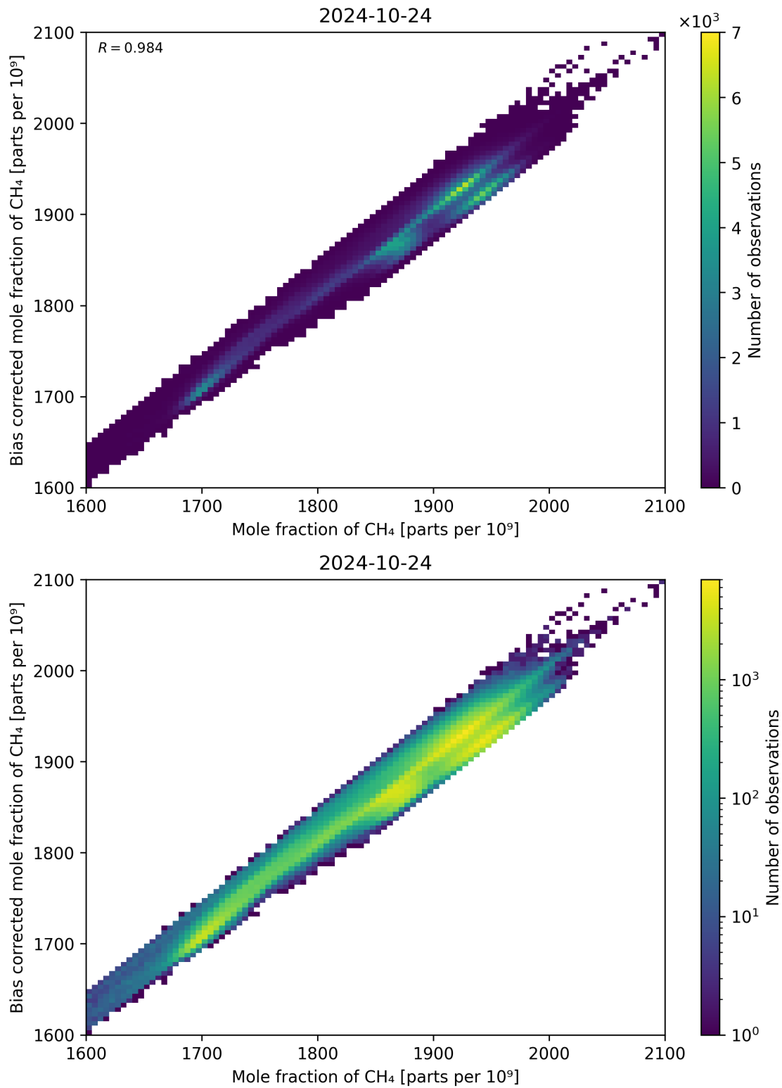
Figure 74: Scatter density plot of “Mole fraction of CH 4 ” against “Bias corrected mole fraction of CH 4 ” for 2024-10-24 to 2024-10-25.
