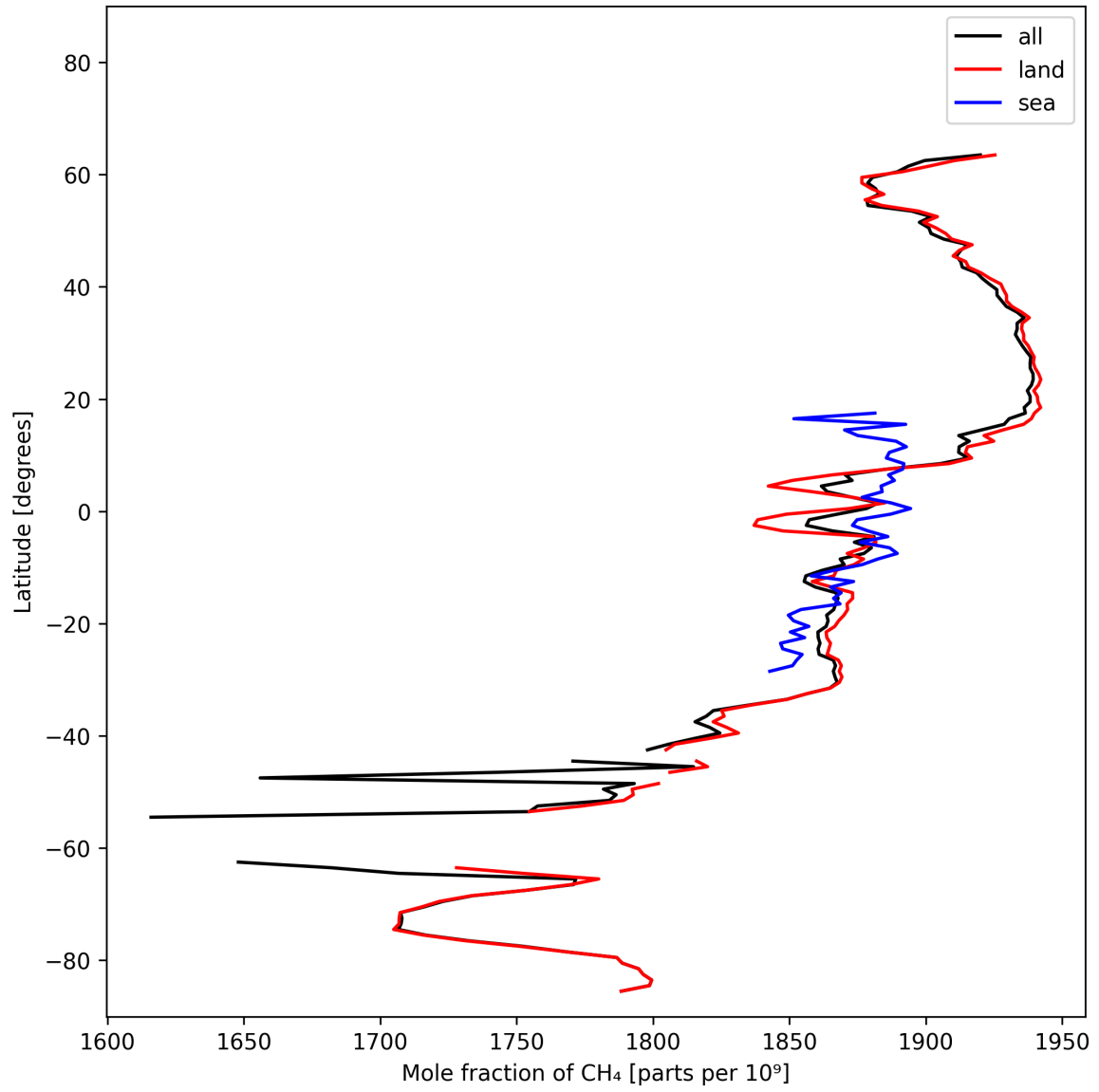
Figure 12: Zonal average of “Mole fraction of \text{CH}_4 ” for 2024-10-24 to 2024-10-25.
