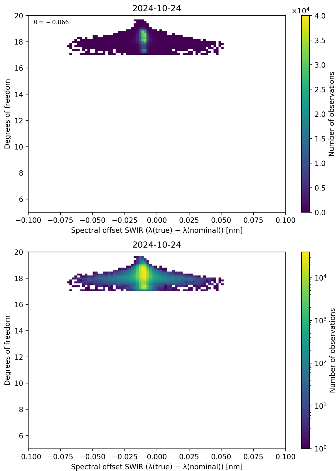
Figure 119: Scatter density plot of “Spectral offset SWIR ( \lambda_{\text{true}} - \lambda_{\text{nominal}} )” against “Degrees of freedom” for 2024-10-24 to 2024-10-25.
