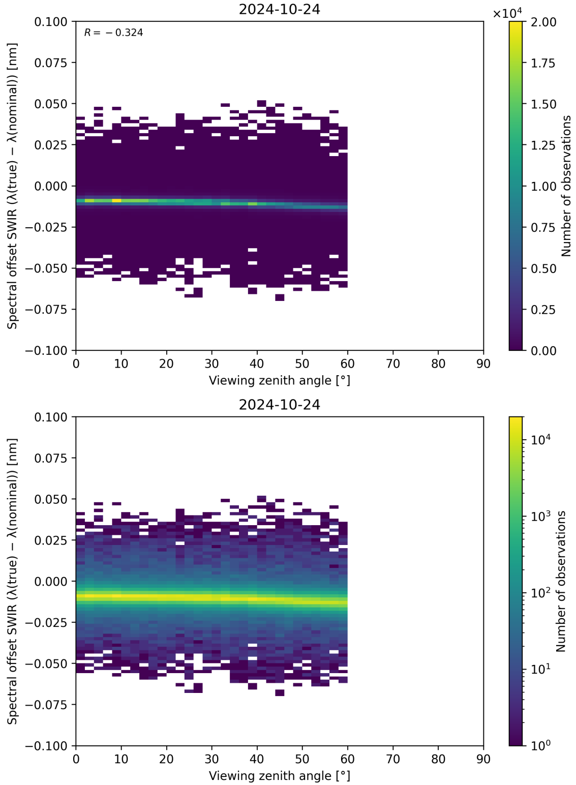
Figure 116: Scatter density plot of “Viewing zenith angle” against “Spectral offset SWIR ( \lambda_{\text{true}} - \lambda_{\text{nominal}} )” for 2024-10-24 to 2024-10-25.
