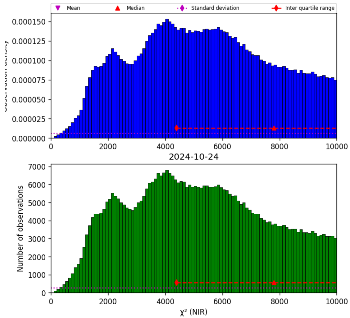
Figure 29: Histogram of “ \chi^2 (NIR)” for 2024-10-24 to 2024-10-25
