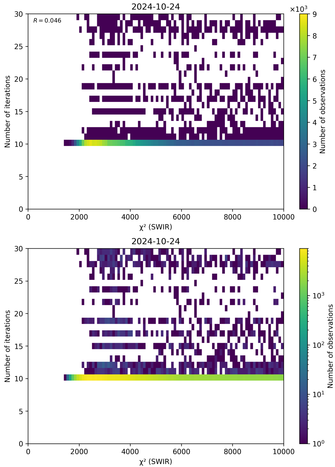
Figure 50: Scatter density plot of “ \chi^2 (SWIR)” against “Number of iterations” for 2024-10-24 to 2024-10-25.
