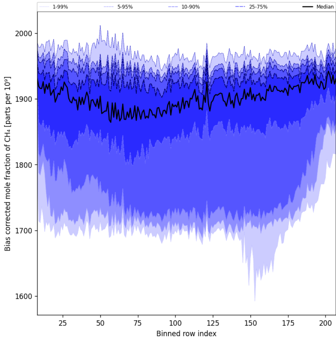
Figure 36: Along track statistics of “Bias corrected mole fraction of CH 4 ” for 2024-10-24 to 2024-10-25
