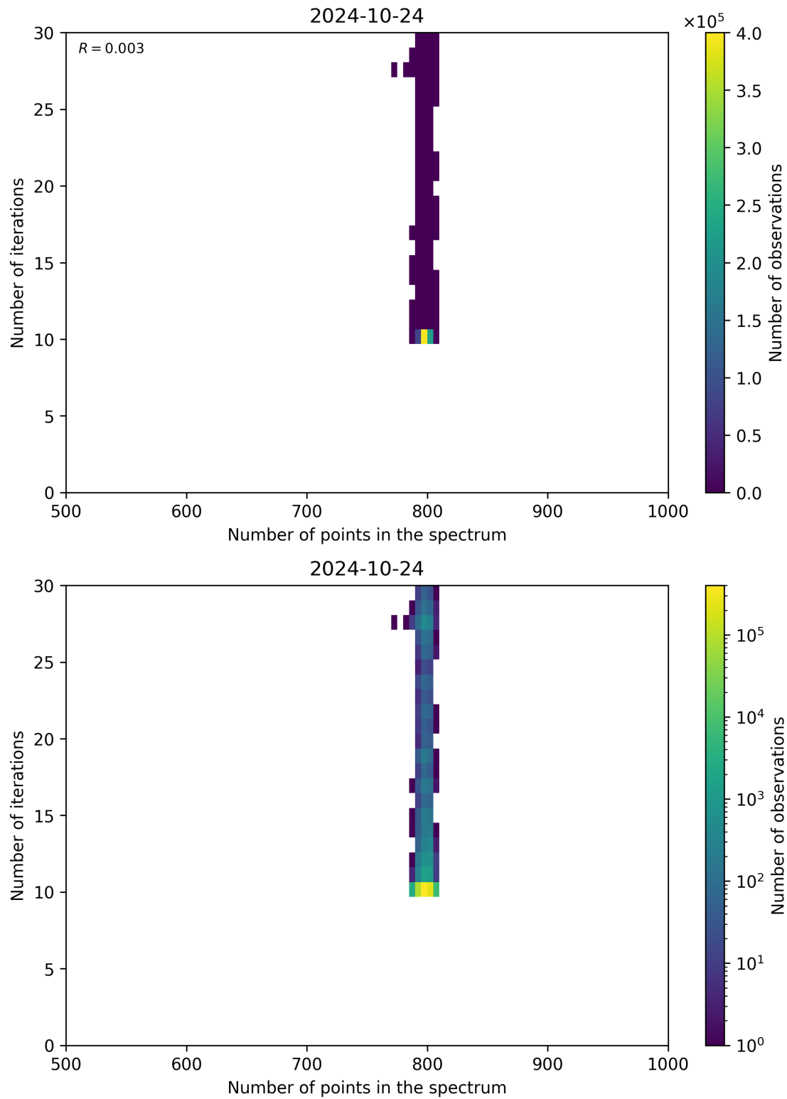
Figure 92: Scatter density plot of “Number of points in the spectrum” against “Number of iterations” for 2024-10-24 to 2024-10-25.
