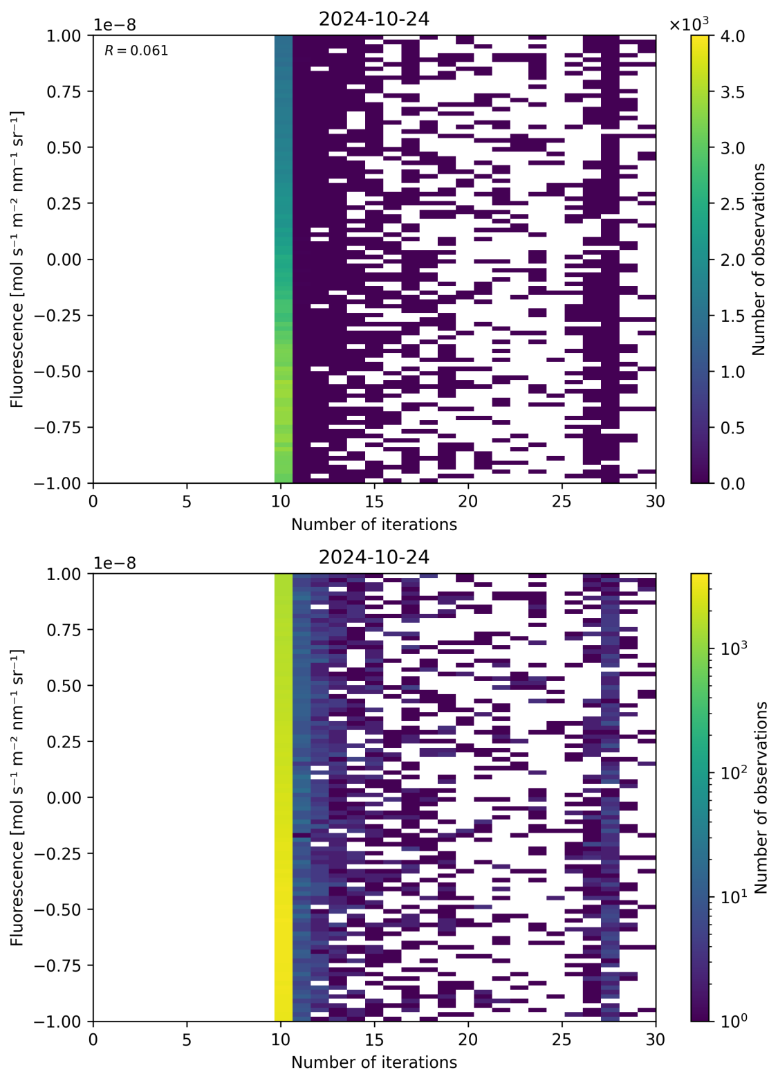
Figure 87: Scatter density plot of “Number of iterations” against “Fluorescence” for 2024-10-24 to 2024-10-25.
