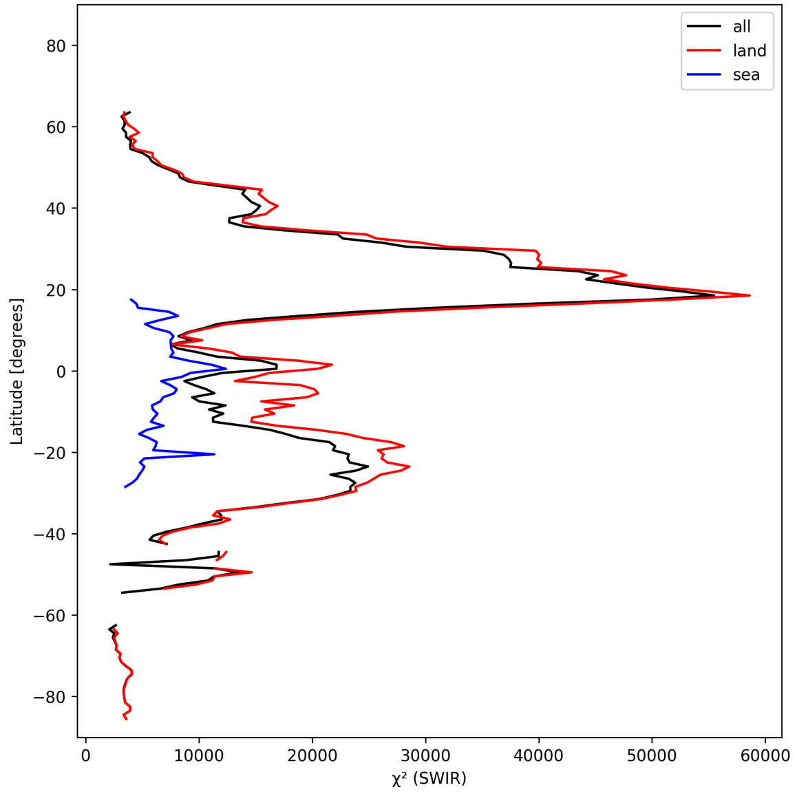
Figure 17: Zonal average of “ \chi^2 (SWIR)” for 2024-10-24 to 2024-10-25.
