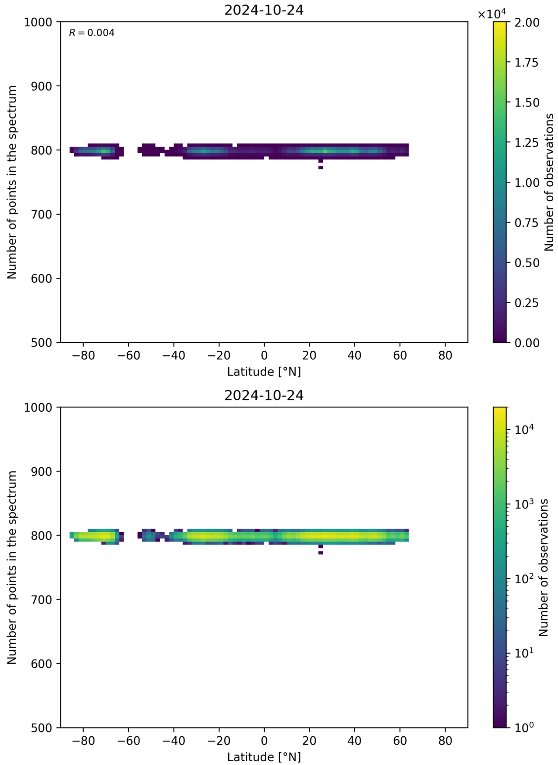
Figure 61: Scatter density plot of “Latitude” against “Number of points in the spectrum” for 2024-10-24 to 2024-10-25.
