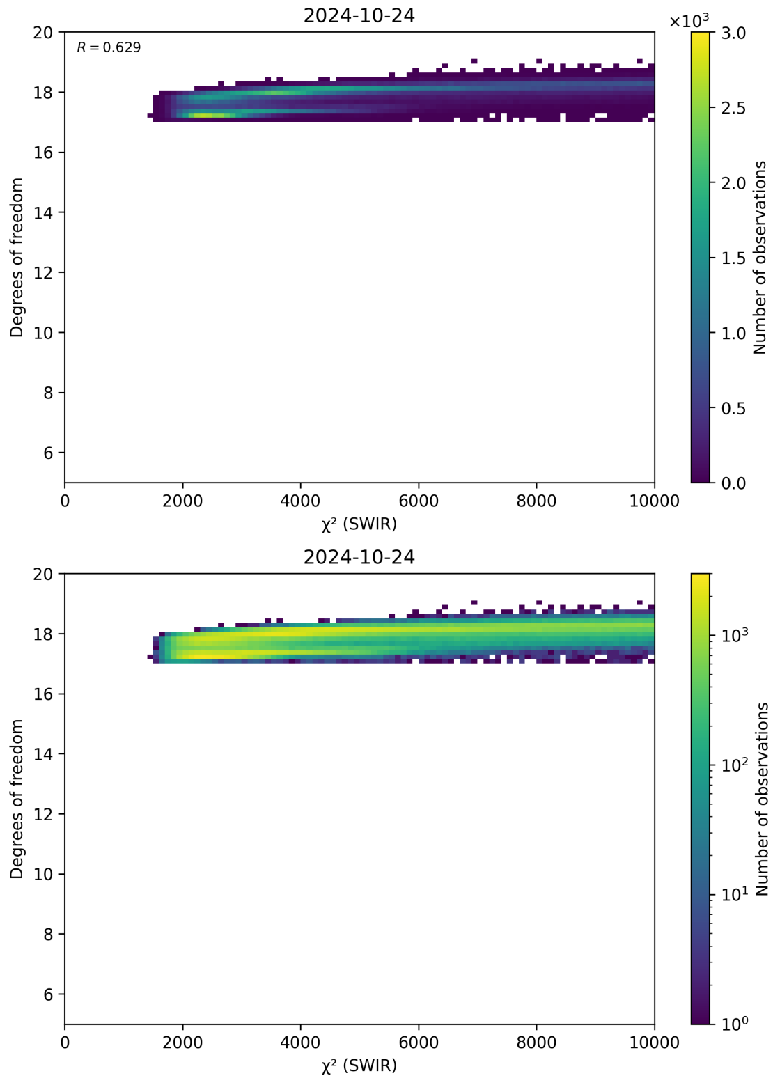
Figure 48: Scatter density plot of " \chi^2 (SWIR)" against "Degrees of freedom" for 2024-10-24 to 2024-10-25.
