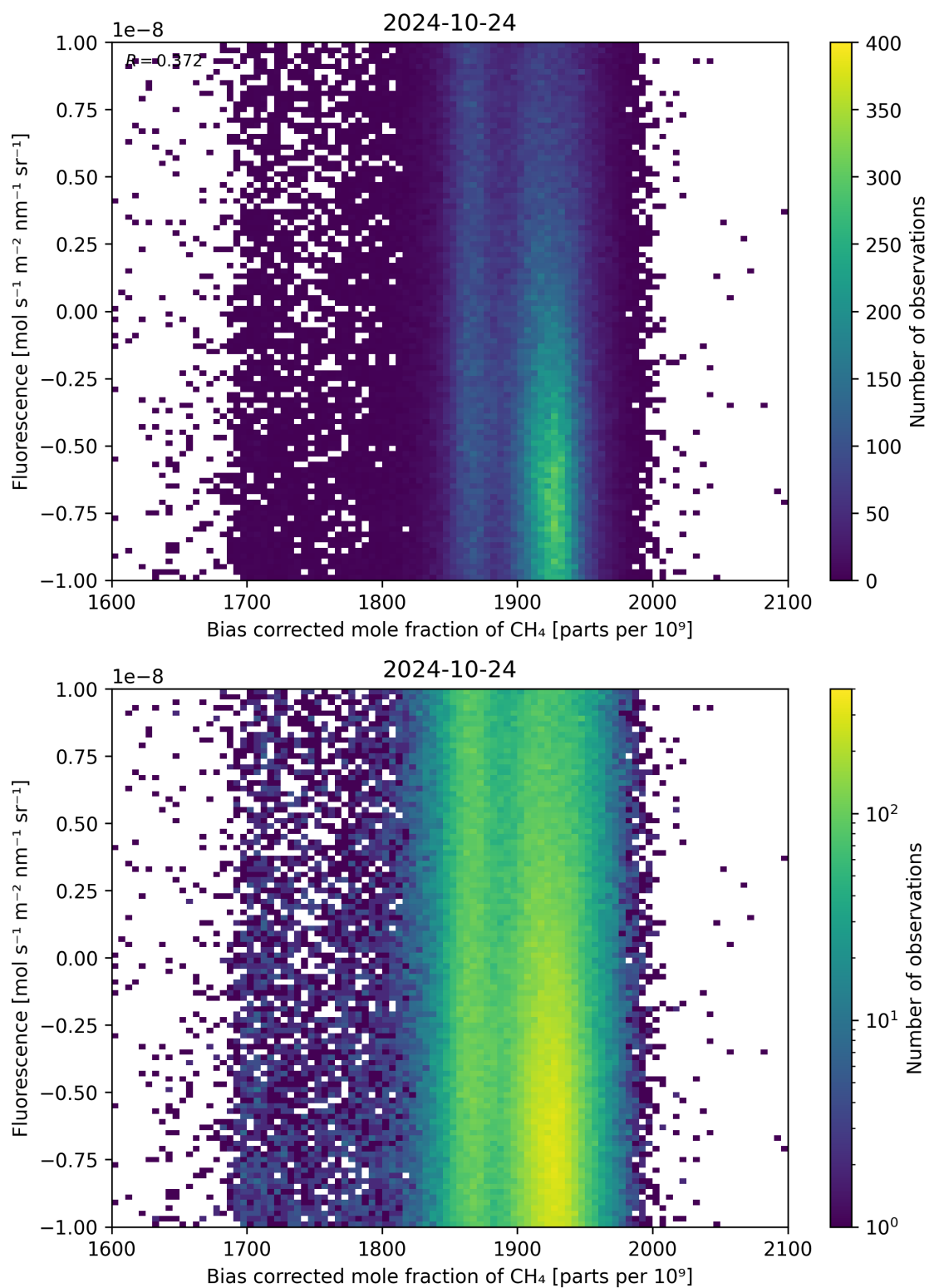
Figure 66: Scatter density plot of “Bias corrected mole fraction of \text{CH}_4 ” against “Fluorescence” for 2024-10-24 to 2024-10-25.
