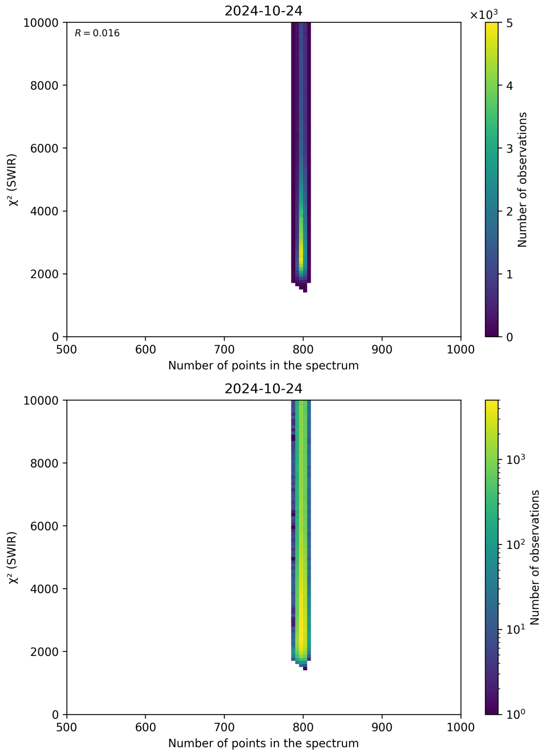
Figure 89: Scatter density plot of “Number of points in the spectrum” against “ \chi^2 (SWIR)” for 2024-10-24 to 2024-10-25.
