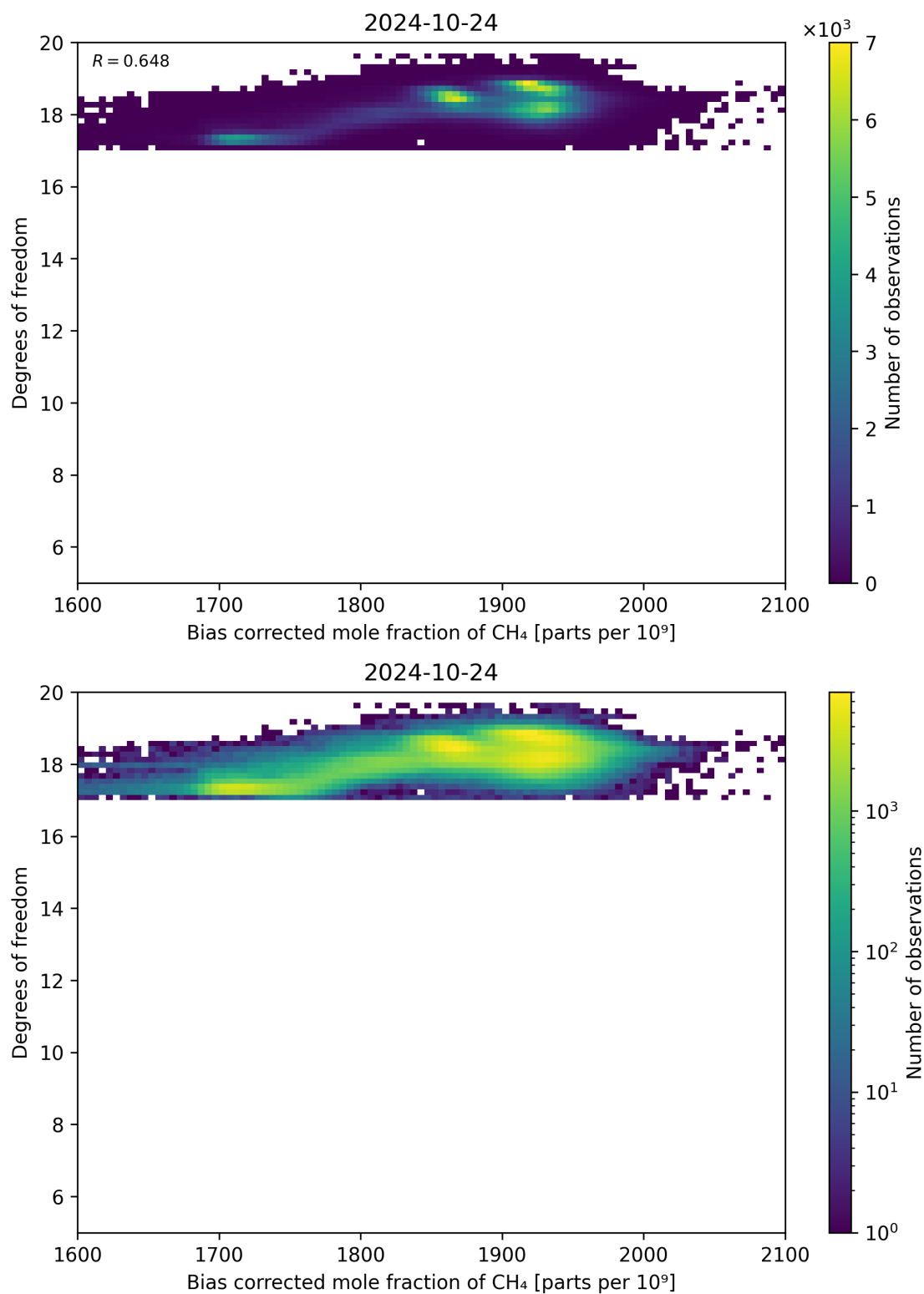
Figure 65: Scatter density plot of “Bias corrected mole fraction of CH 4 ” against “Degrees of freedom” for 2024-10-24 to 2024-10-25.
