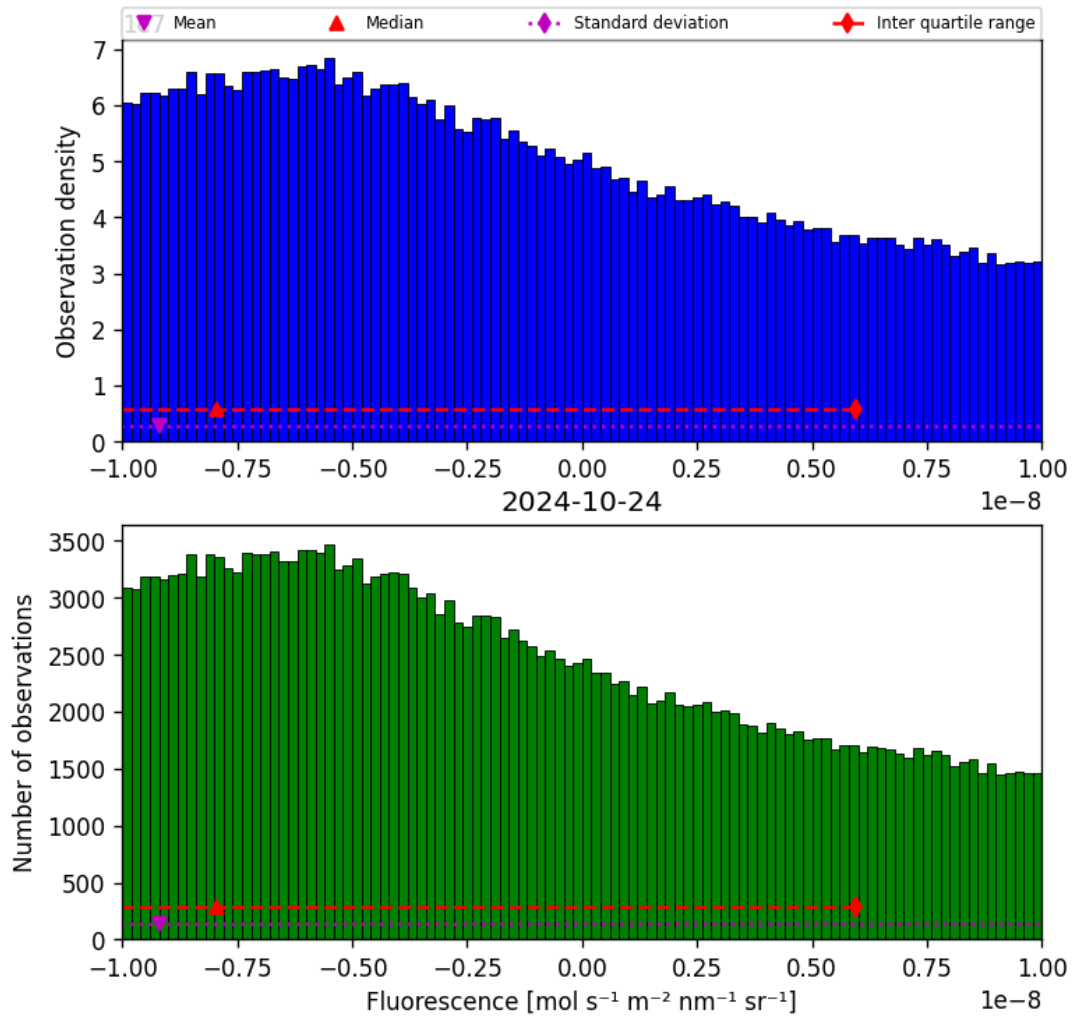
Figure 32: Histogram of “Fluorescence” for 2024-10-24 to 2024-10-25
