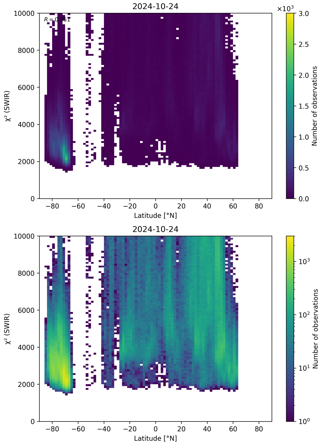
Figure 54: Scatter density plot of “Latitude” against “ \chi^2 (SWIR)” for 2024-10-24 to 2024-10-25.
