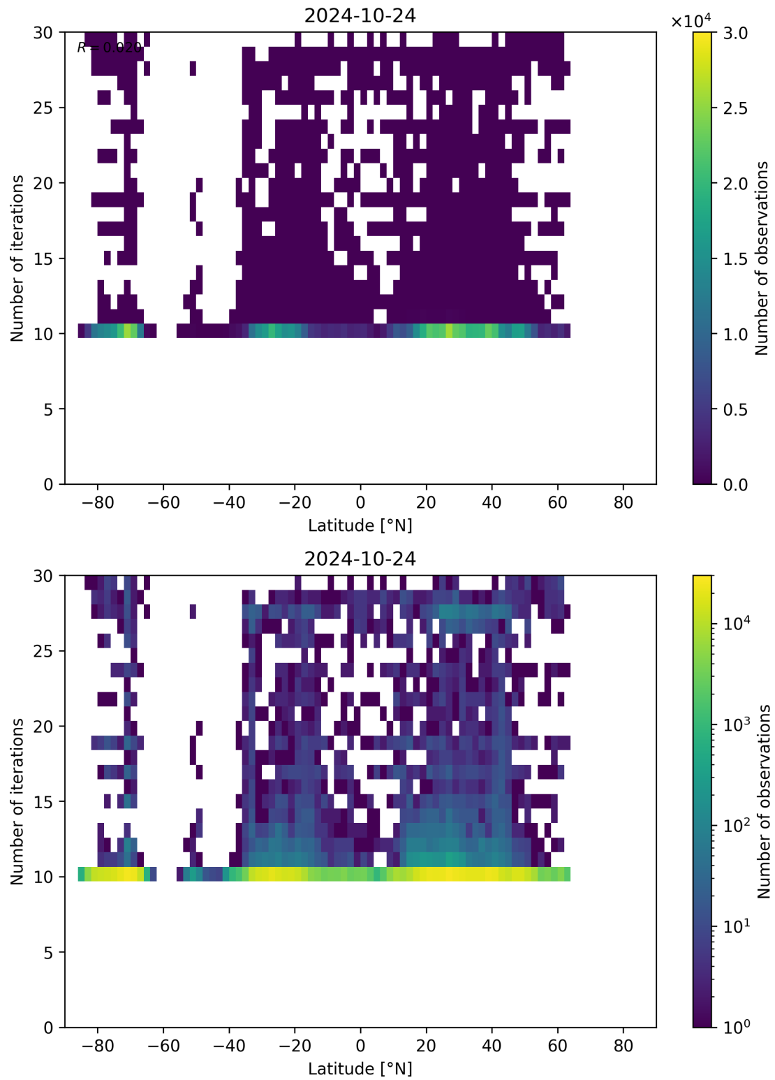
Figure 60: Scatter density plot of “Latitude” against “Number of iterations” for 2024-10-24 to 2024-10-25.
