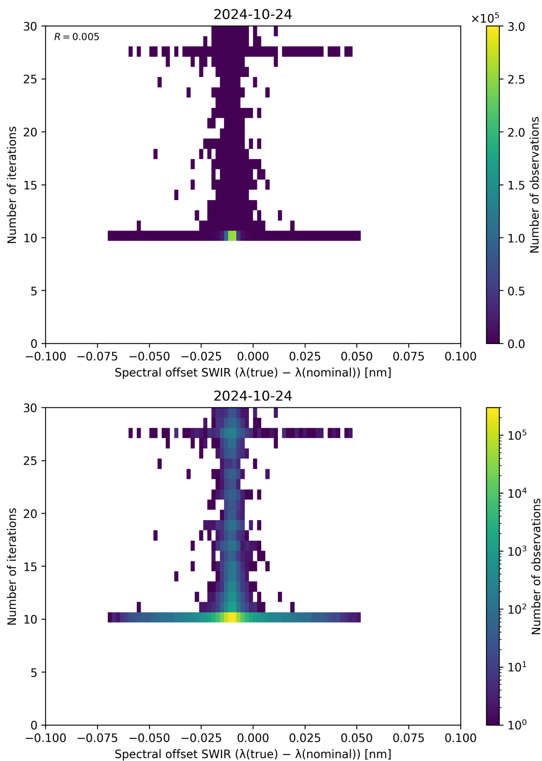
Figure 121: Scatter density plot of “Spectral offset SWIR ( \lambda_{\text{true}} - \lambda_{\text{nominal}} )” against “Number of iterations” for 2024-10-24 to 2024-10-25.
