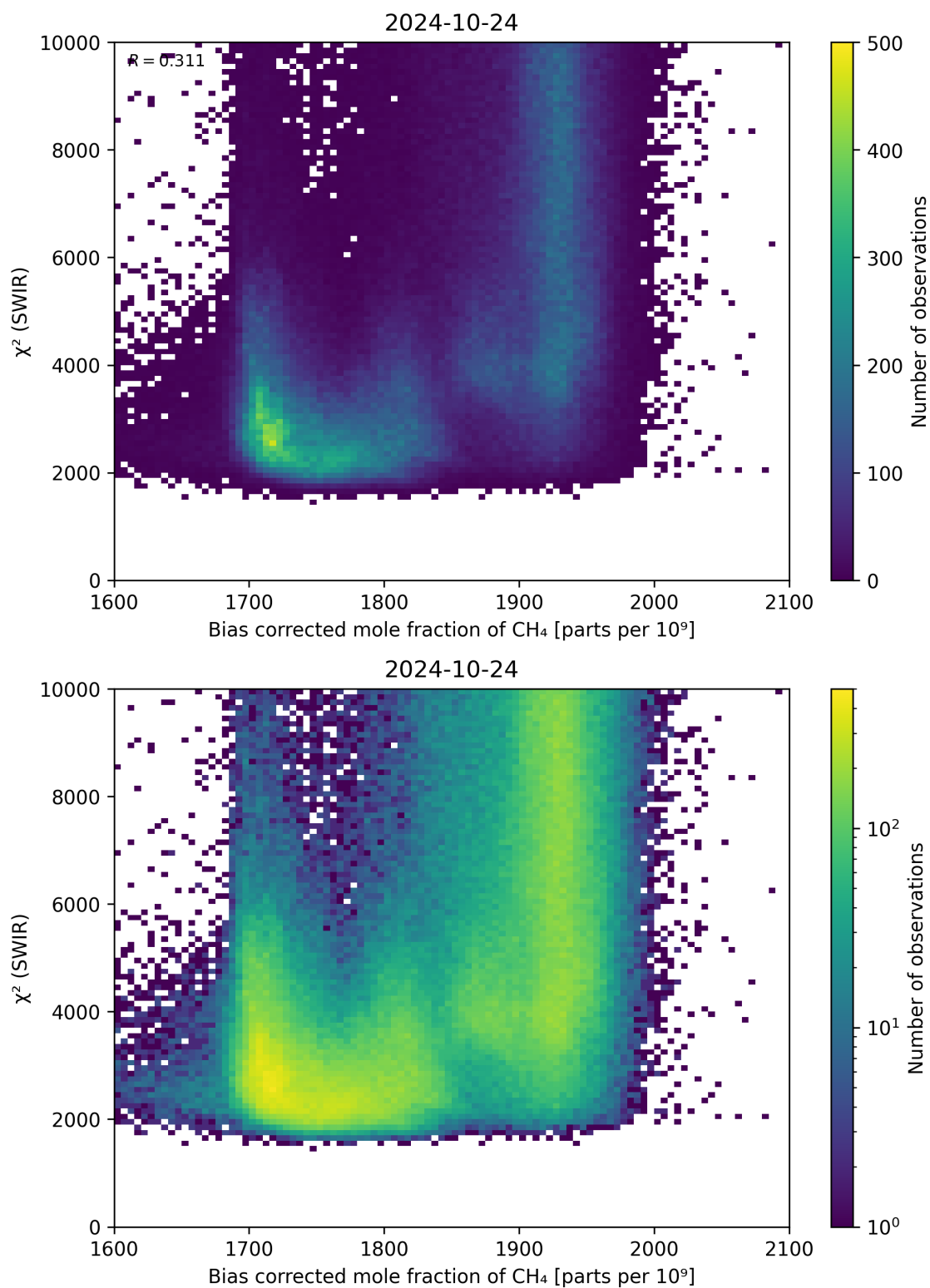
Figure 64: Scatter density plot of “Bias corrected mole fraction of CH 4 ” against “ \chi^2 (SWIR)” for 2024-10-24 to 2024-10-25.
