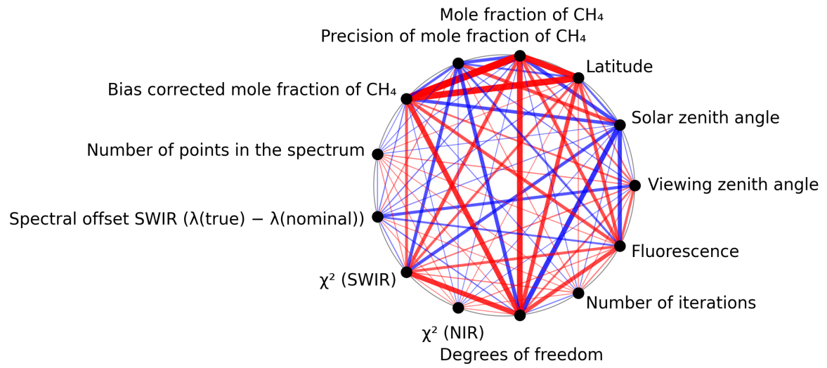
Figure 1: Map of correlation graph for 2024-10-24 to 2024-10-25.
