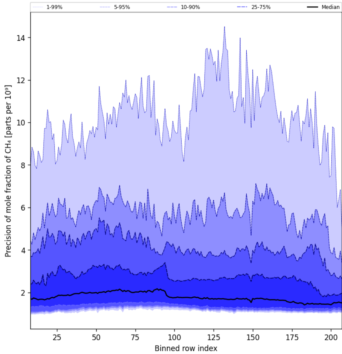
Figure 35: Along track statistics of “Precision of mole fraction of CH 4 ” for 2024-10-24 to 2024-10-25
