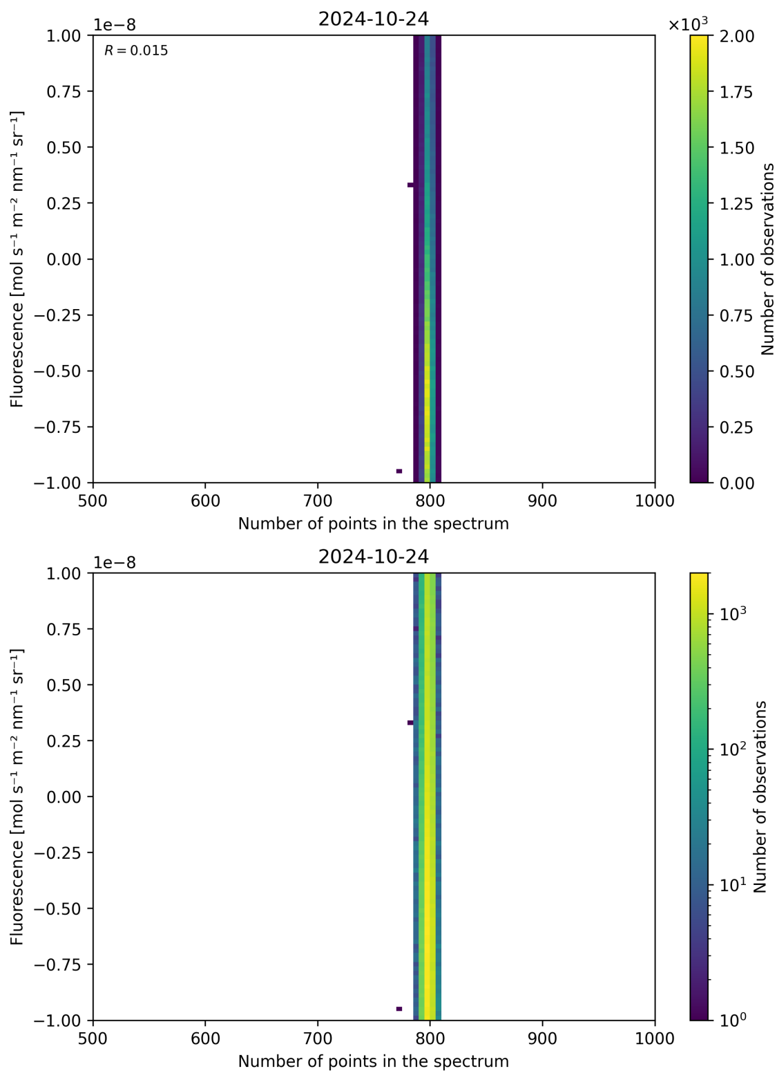
Figure 91: Scatter density plot of “Number of points in the spectrum” against “Fluorescence” for 2024-10-24 to 2024-10-25.
