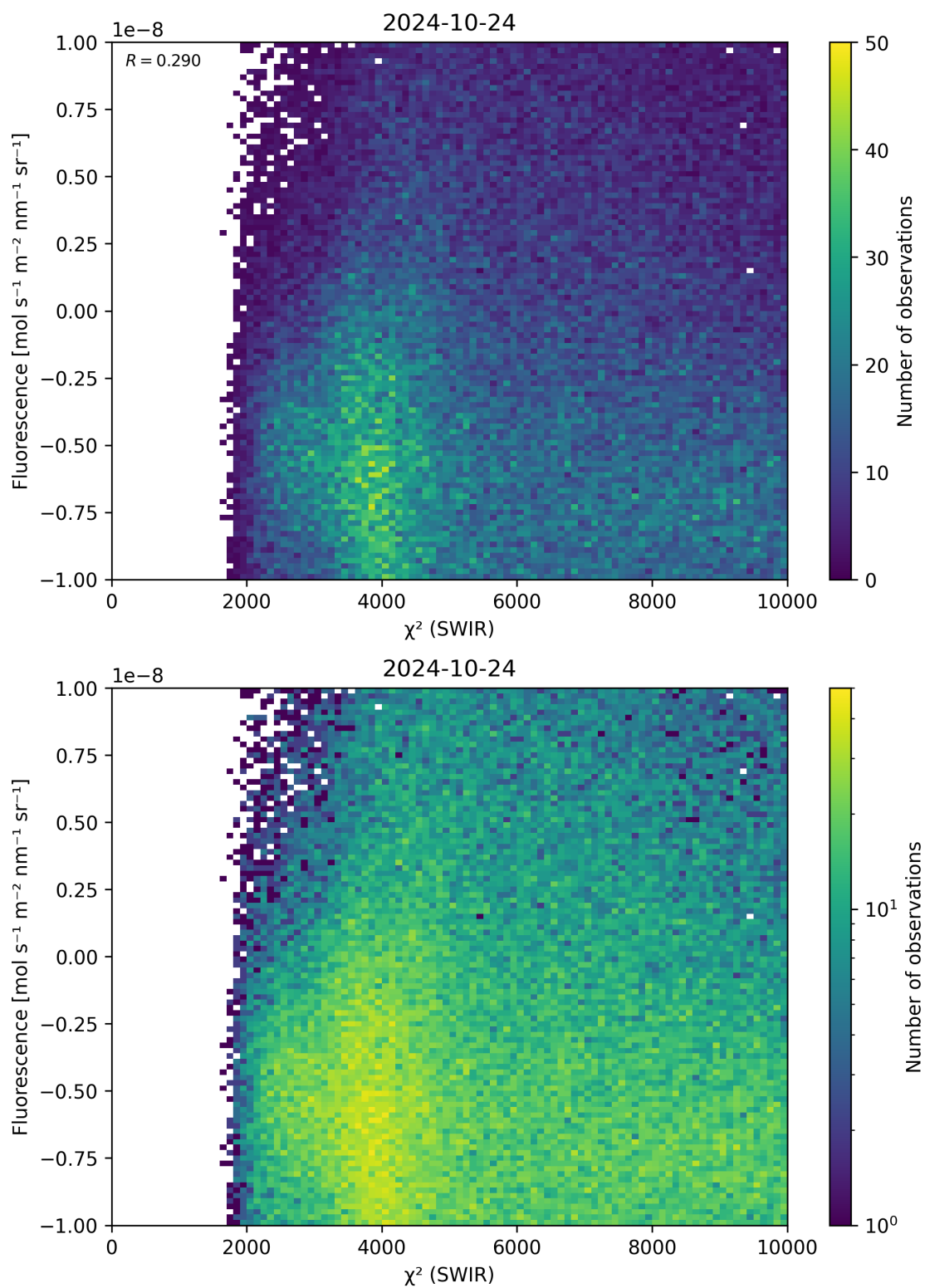
Figure 49: Scatter density plot of “ \chi^2 (SWIR)” against “Fluorescence” for 2024-10-24 to 2024-10-25.
