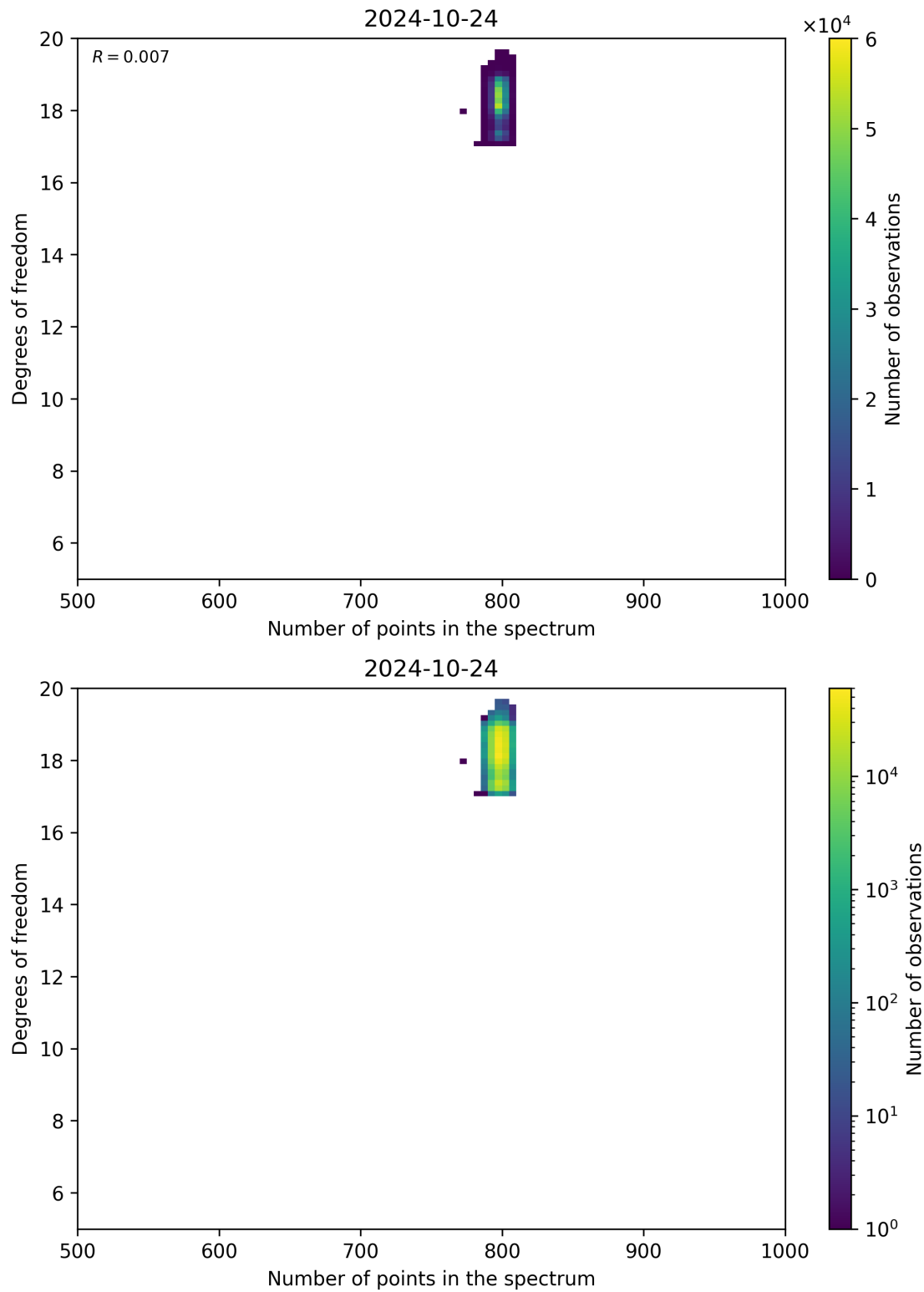
Figure 90: Scatter density plot of “Number of points in the spectrum” against “Degrees of freedom” for 2024-10-24 to 2024-10-25.
