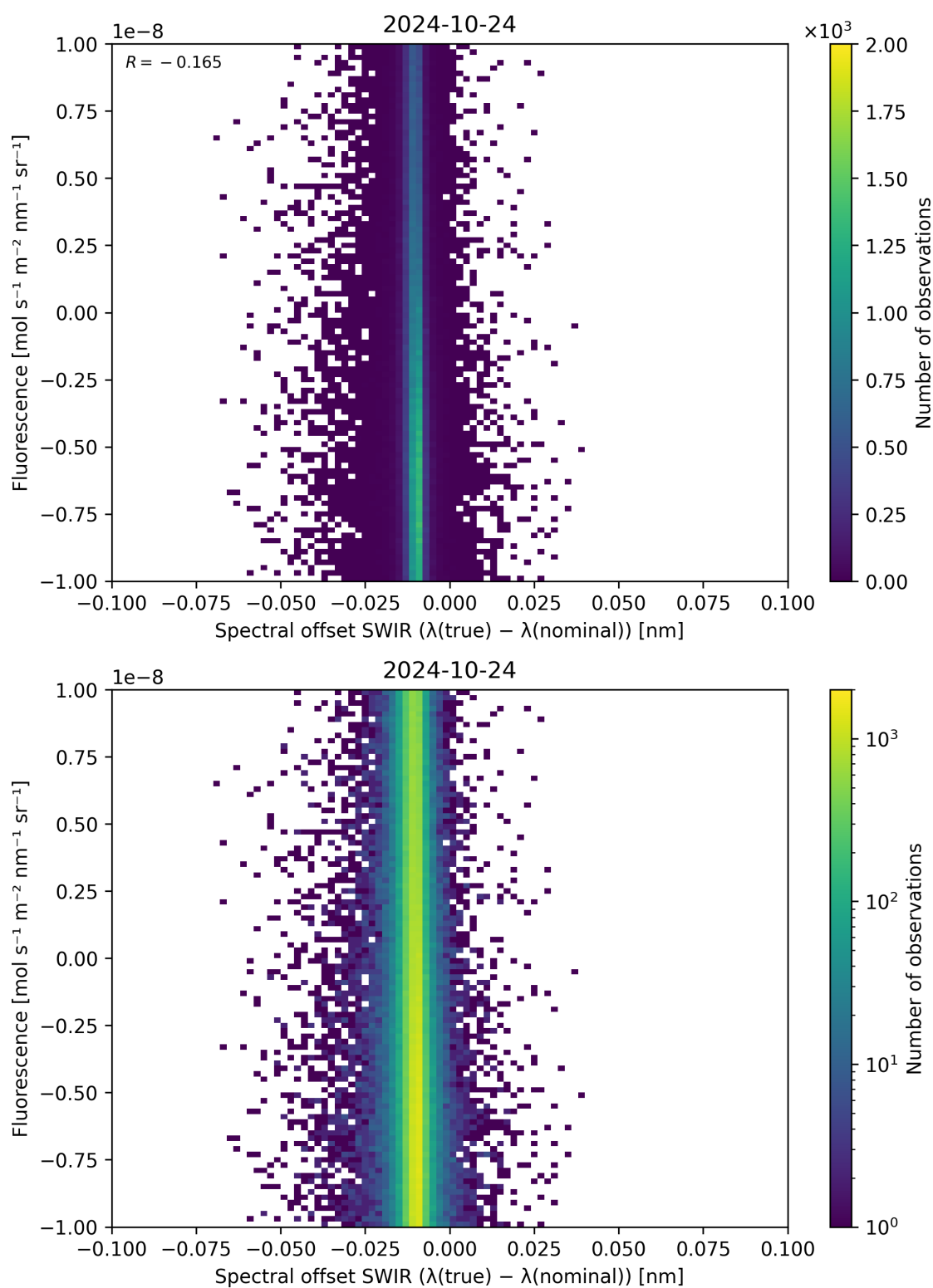
Figure 120: Scatter density plot of “Spectral offset SWIR ( \lambda_{\text{true}} - \lambda_{\text{nominal}} )” against “Fluorescence” for 2024-10-24 to 2024-10-25.
