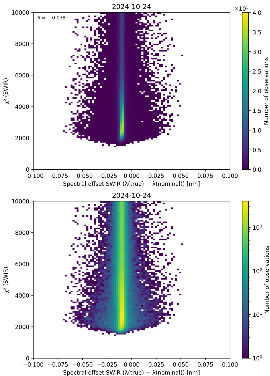
Figure 118: Scatter density plot of “Spectral offset SWIR ( \lambda_{\text{true}} - \lambda_{\text{nominal}} )” against “ \chi^2 (SWIR)” for 2024-10-24 to 2024-10-25.
