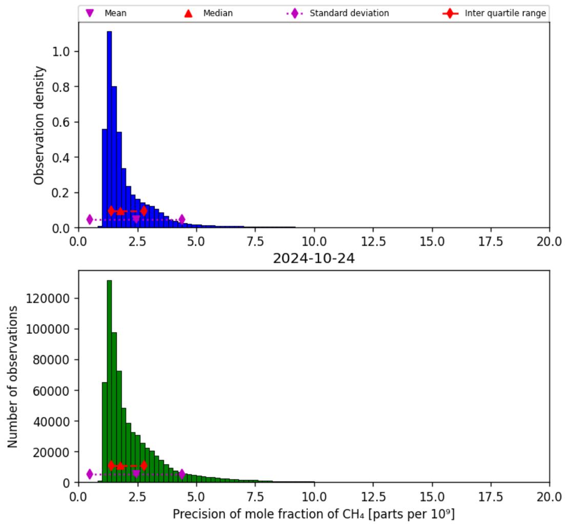
Figure 24: Histogram of “Precision of mole fraction of CH 4 ” for 2024-10-24 to 2024-10-25
