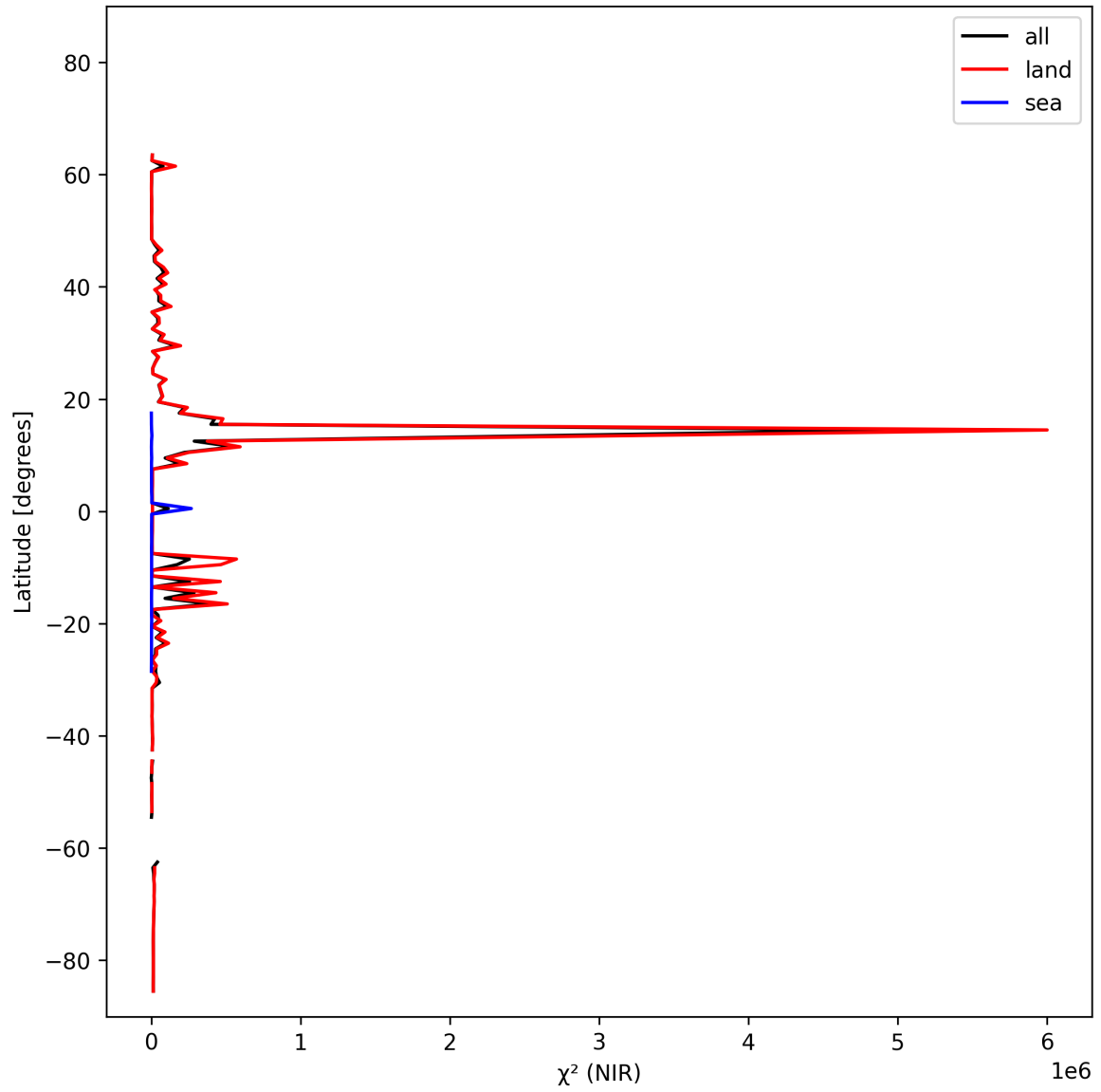
Figure 18: Zonal average of “ \chi^2 (NIR)” for 2024-10-24 to 2024-10-25.
