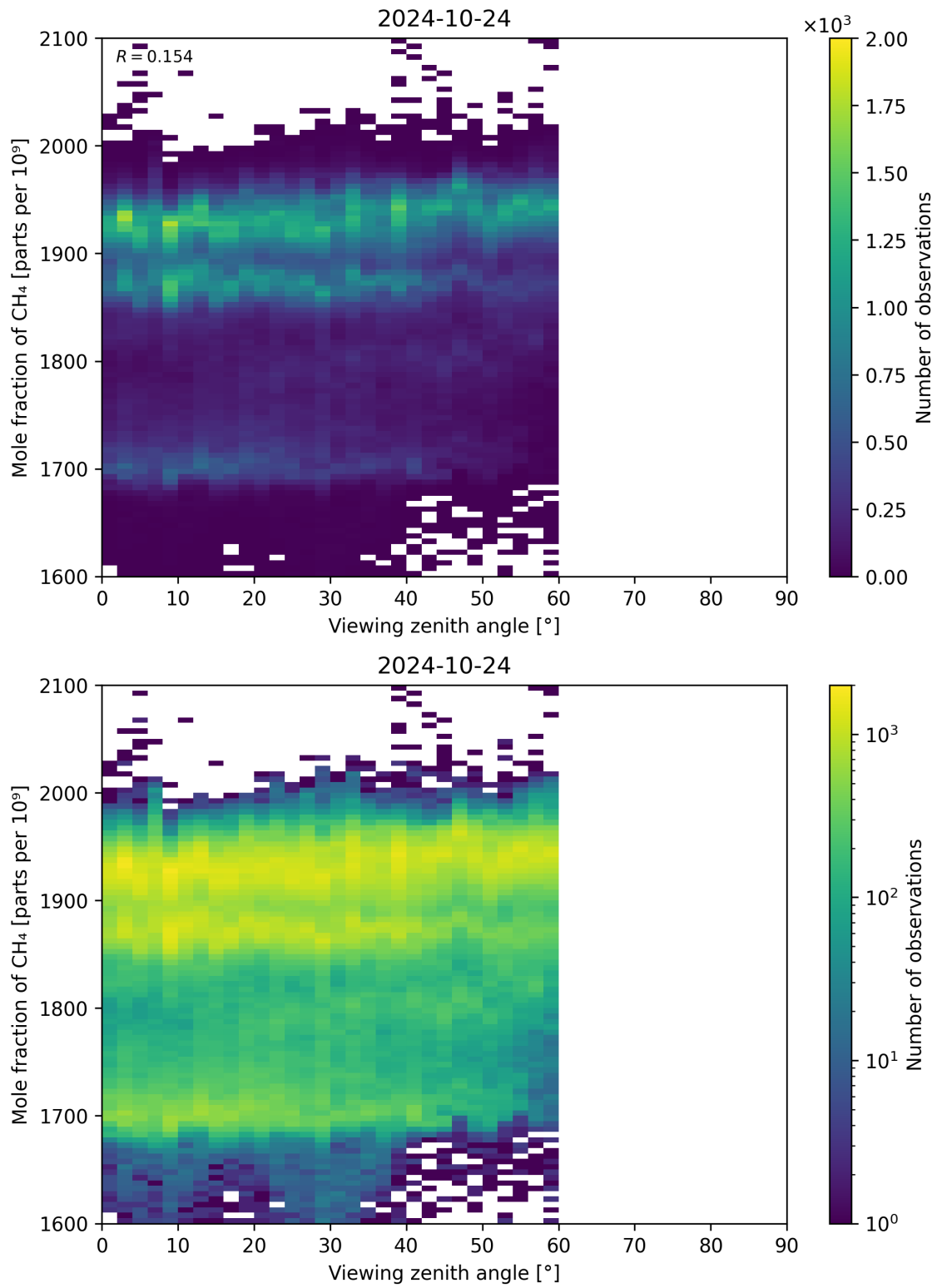
Figure 110: Scatter density plot of “Viewing zenith angle” against “Mole fraction of CH 4 ” for 2024-10-24 to 2024-10-25.
