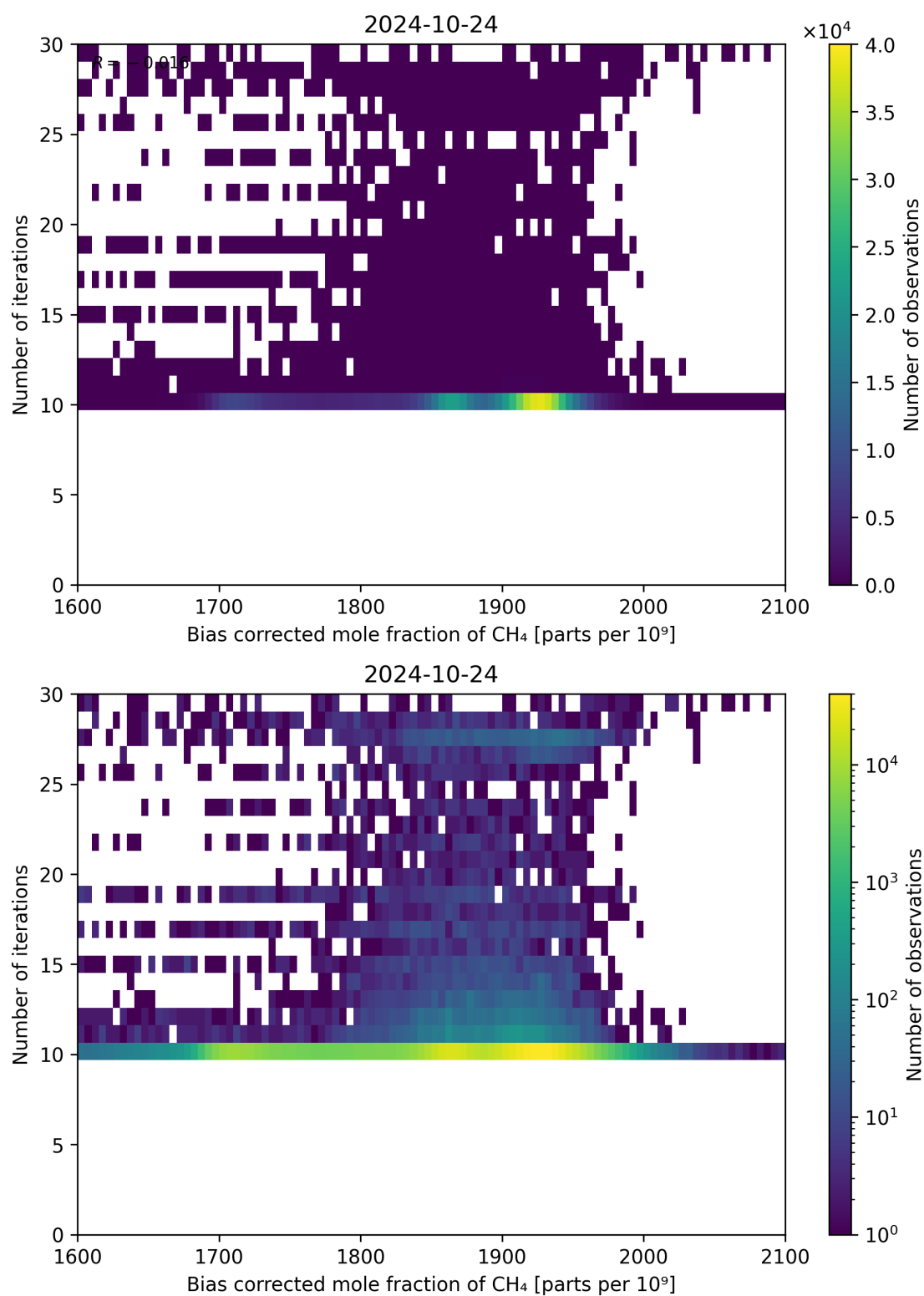
Figure 67: Scatter density plot of “Bias corrected mole fraction of \text{CH}_4 ” against “Number of iterations” for 2024-10-24 to 2024-10-25.
