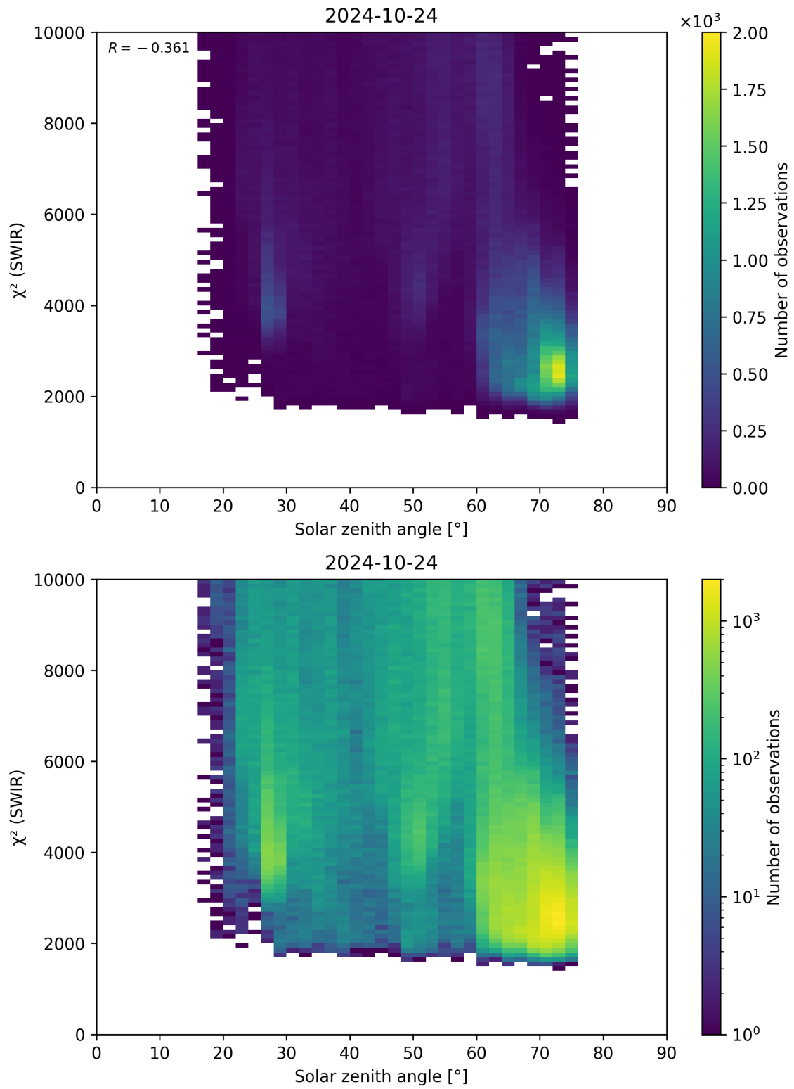
Figure 95: Scatter density plot of “Solar zenith angle” against “ \chi^2 (SWIR)” for 2024-10-24 to 2024-10-25.
