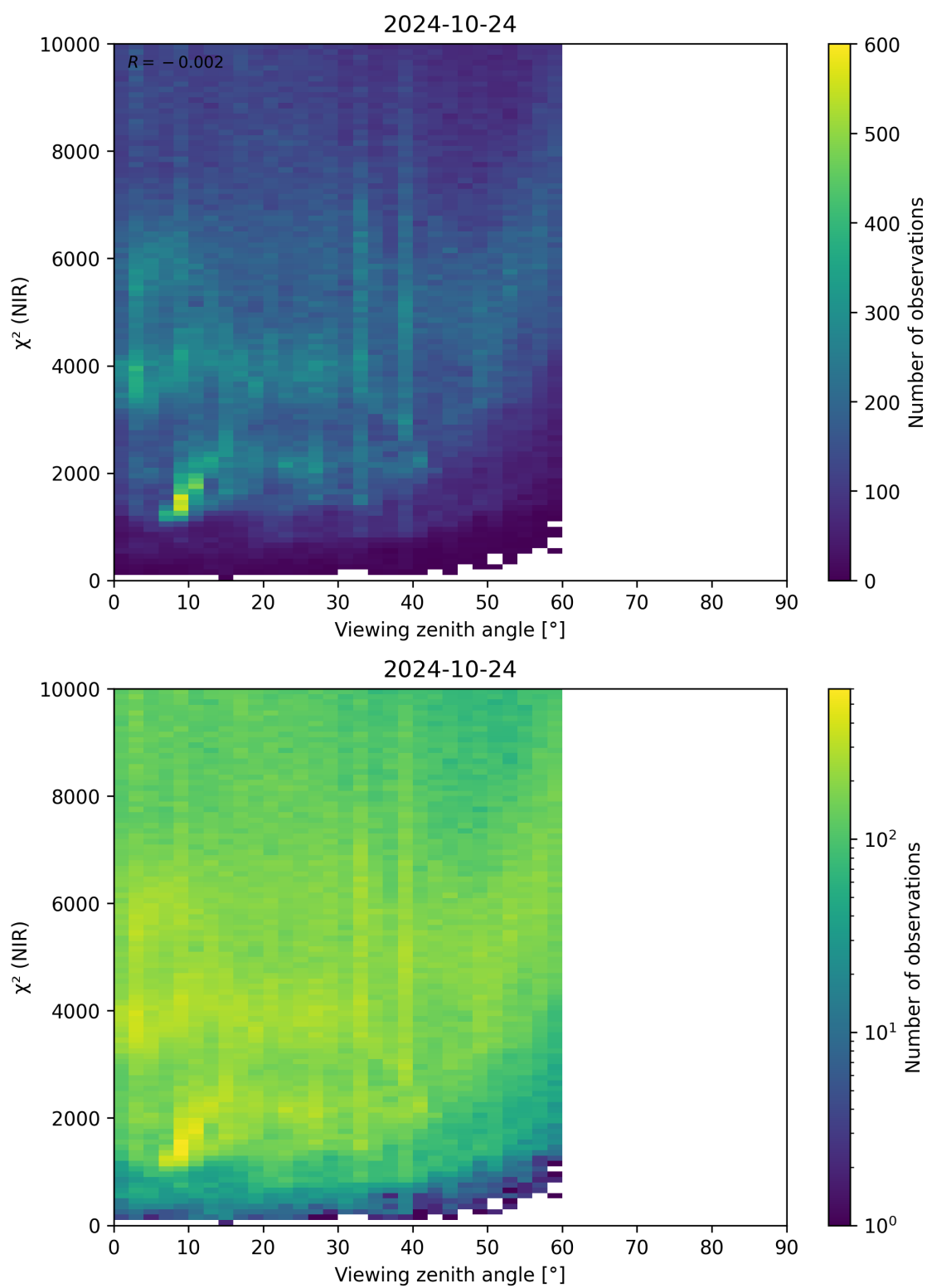
Figure 105: Scatter density plot of “Viewing zenith angle” against “ \chi^2 (NIR)” for 2024-10-24 to 2024-10-25.
