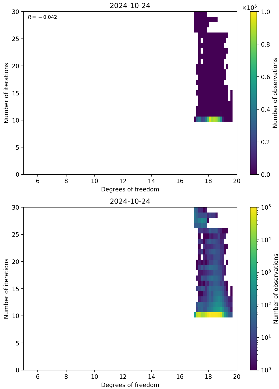
Figure 52: Scatter density plot of “Degrees of freedom” against “Number of iterations” for 2024-10-24 to 2024-10-25.
