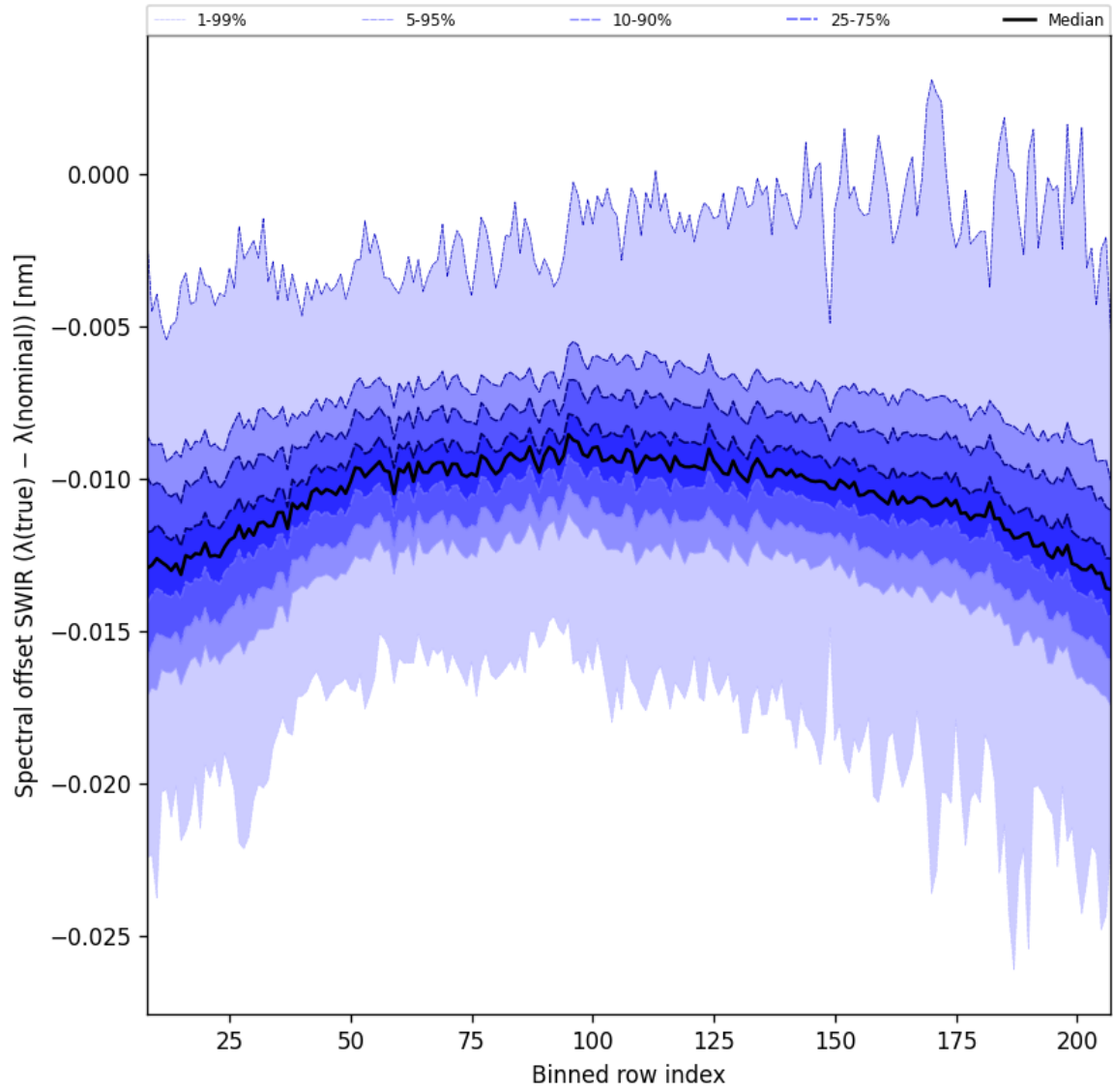
Figure 38: Along track statistics of “Spectral offset SWIR ( \lambda_{\text{true}} - \lambda_{\text{nominal}} )” for 2024-10-24 to 2024-10-25
