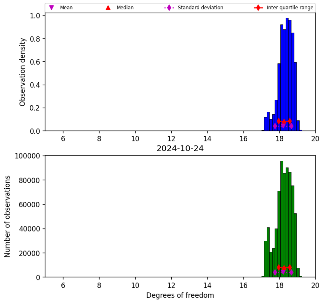
Figure 30: Histogram of “Degrees of freedom” for 2024-10-24 to 2024-10-25
