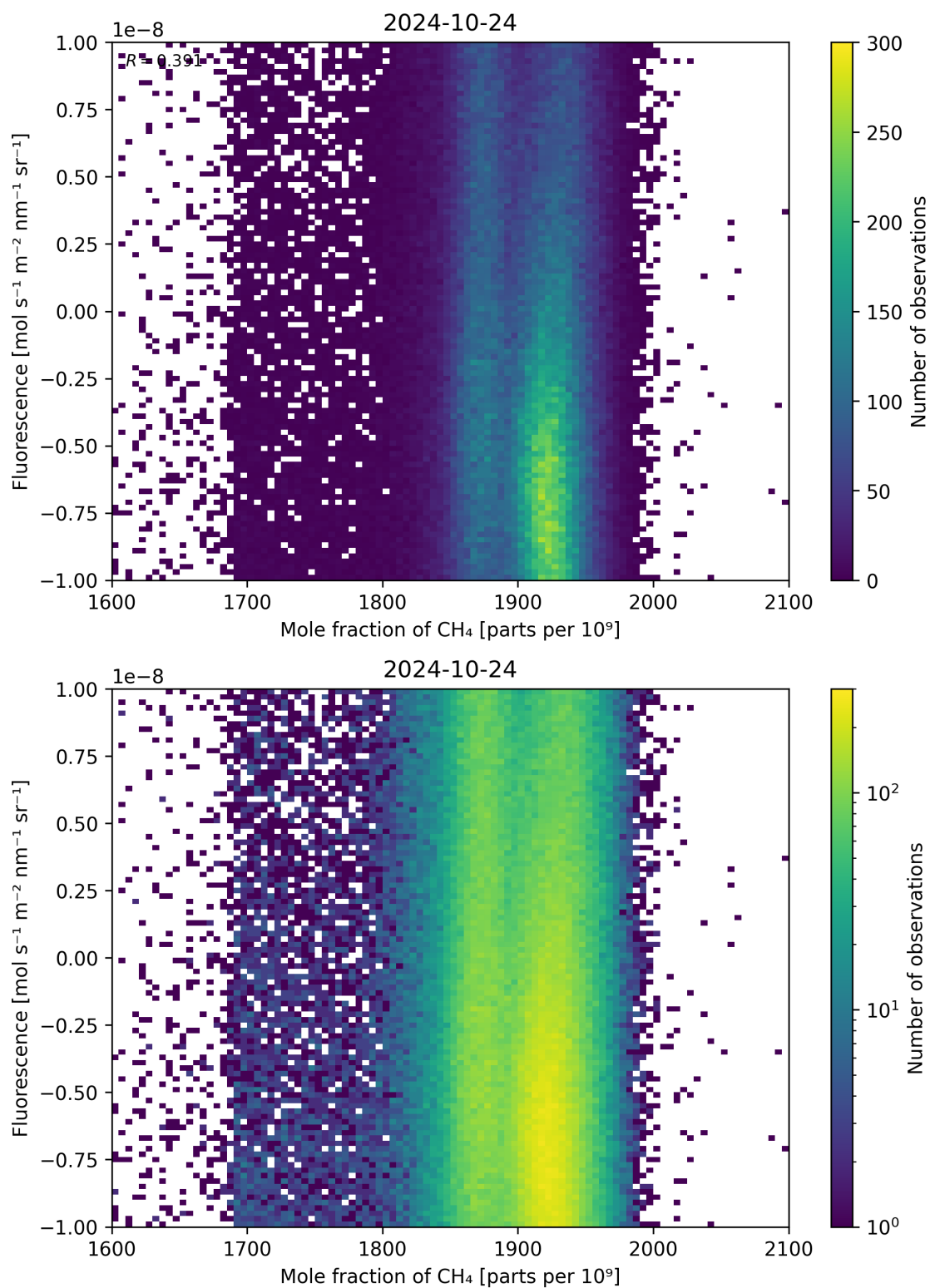
Figure 73: Scatter density plot of “Mole fraction of \text{CH}_4 ” against “Fluorescence” for 2024-10-24 to 2024-10-25.
