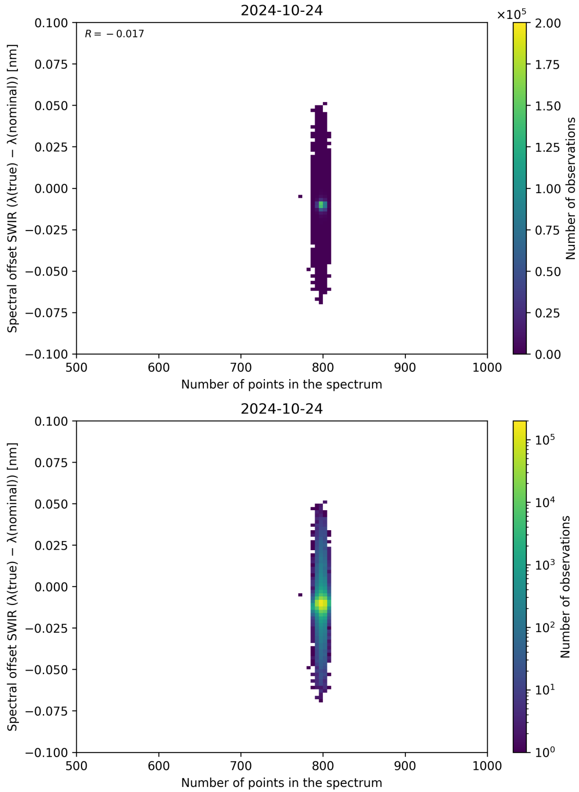
Figure 93: Scatter density plot of “Number of points in the spectrum” against “Spectral offset SWIR ( \lambda_{\text{true}} - \lambda_{\text{nominal}} )” for 2024-10-24 to 2024-10-25.
