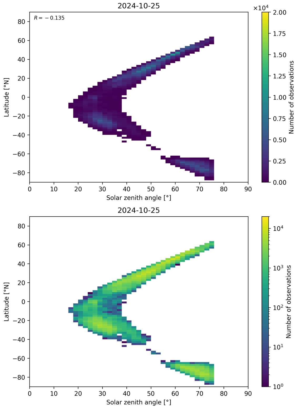
Figure 98: Scatter density plot of “Solar zenith angle” against “Latitude” for 2024-10-24 to 2024-10-26.
