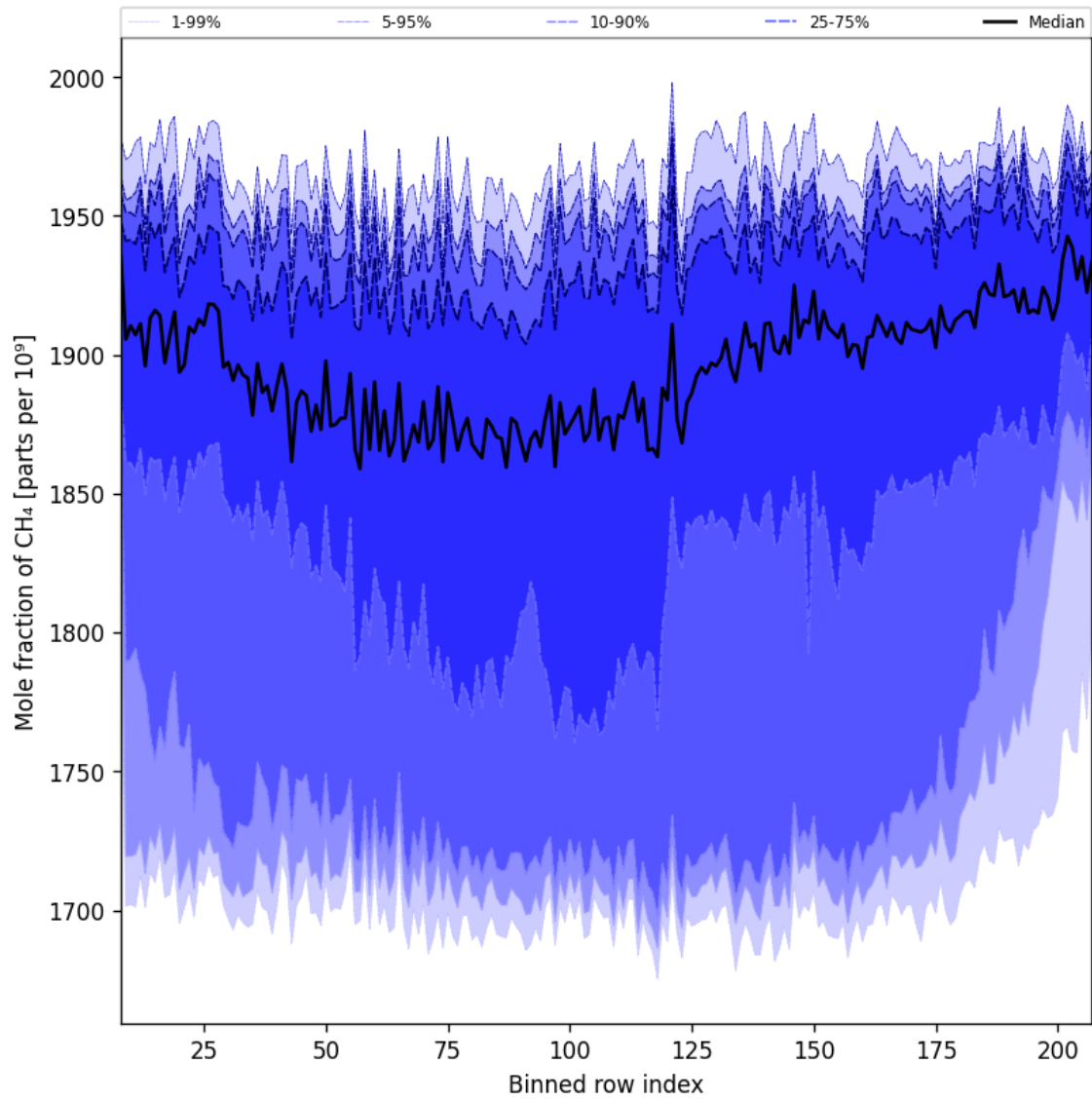
Figure 34: Along track statistics of “Mole fraction of CH 4 ” for 2024-10-24 to 2024-10-26
