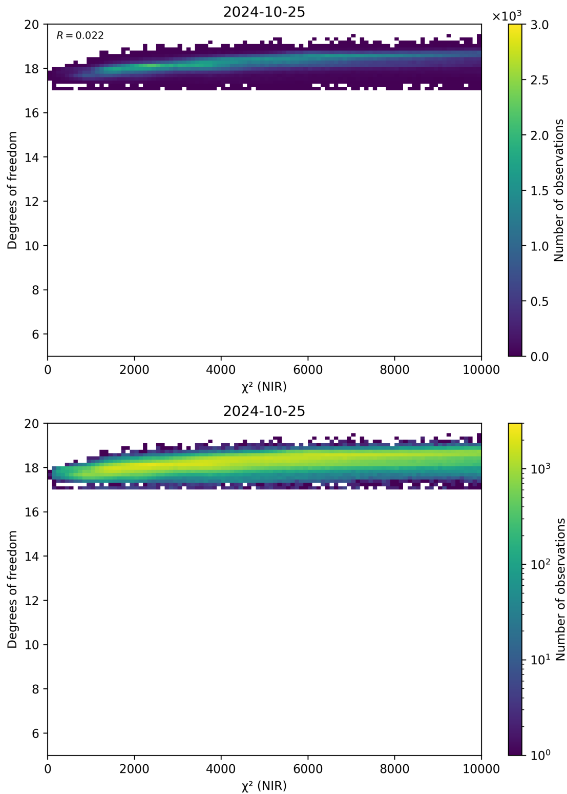
Figure 44: Scatter density plot of “ \chi^2 (NIR)” against “Degrees of freedom” for 2024-10-24 to 2024-10-26.
