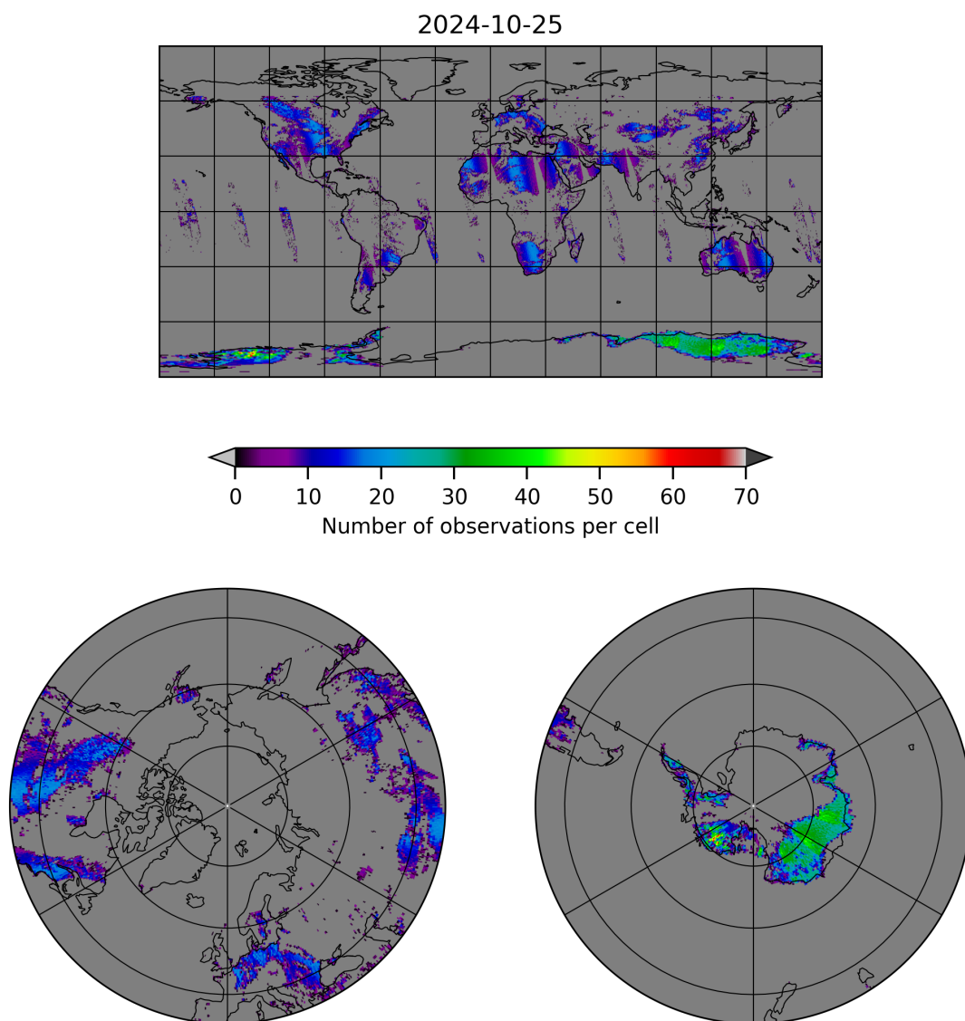
Figure 10: Map of the number of observations for 2024-10-24 to 2024-10-26
