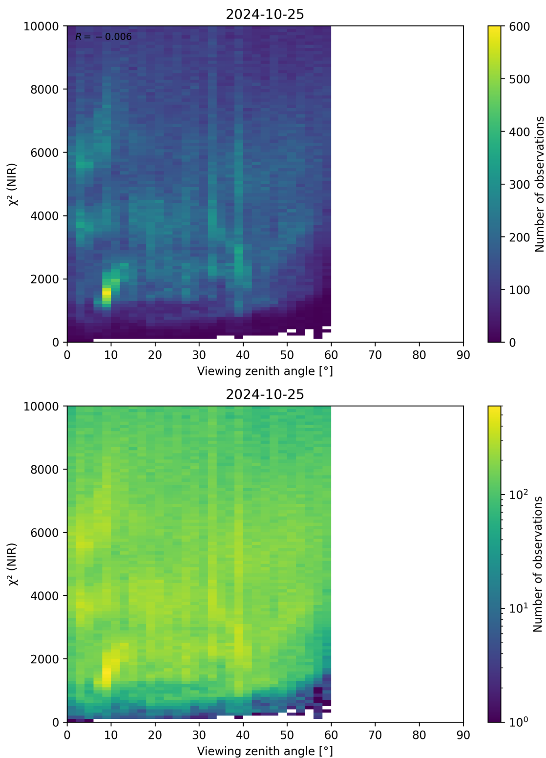
Figure 105: Scatter density plot of “Viewing zenith angle” against “ \chi^2 (NIR)” for 2024-10-24 to 2024-10-26.
