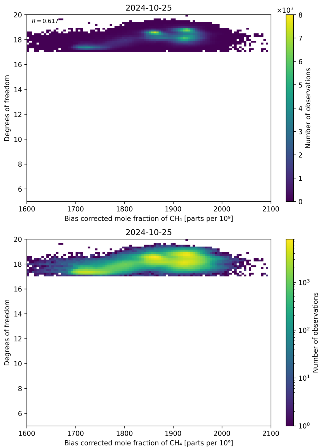
Figure 65: Scatter density plot of “Bias corrected mole fraction of CH 4 ” against “Degrees of freedom” for 2024-10-24 to 2024-10-26.
