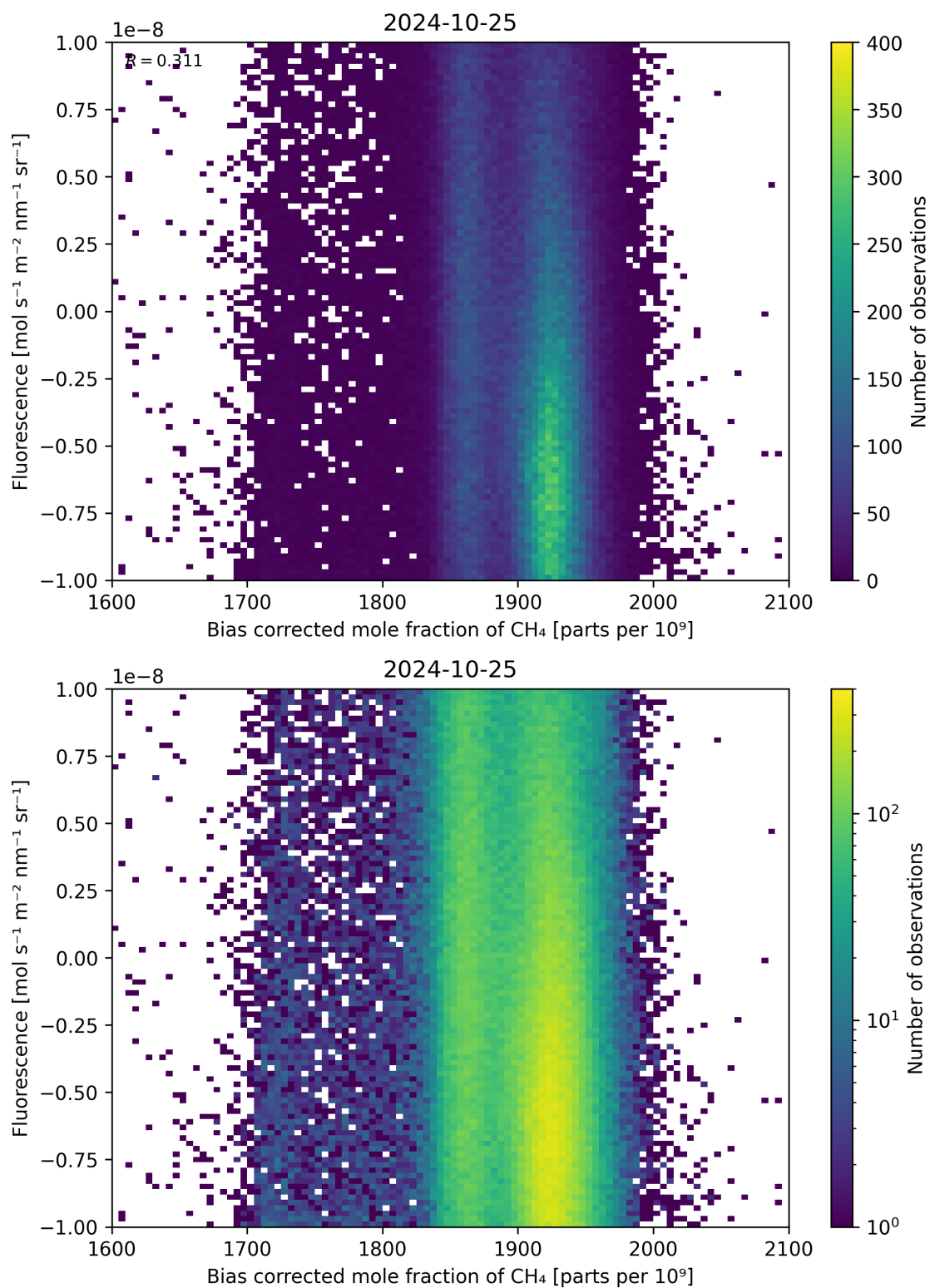
Figure 66: Scatter density plot of “Bias corrected mole fraction of \text{CH}_4 ” against “Fluorescence” for 2024-10-24 to 2024-10-26.
