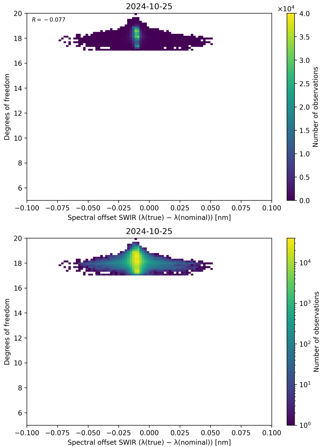
Figure 119: Scatter density plot of “Spectral offset SWIR ( \lambda_{\text{true}} - \lambda_{\text{nominal}} )” against “Degrees of freedom” for 2024-10-24 to 2024-10-26.
