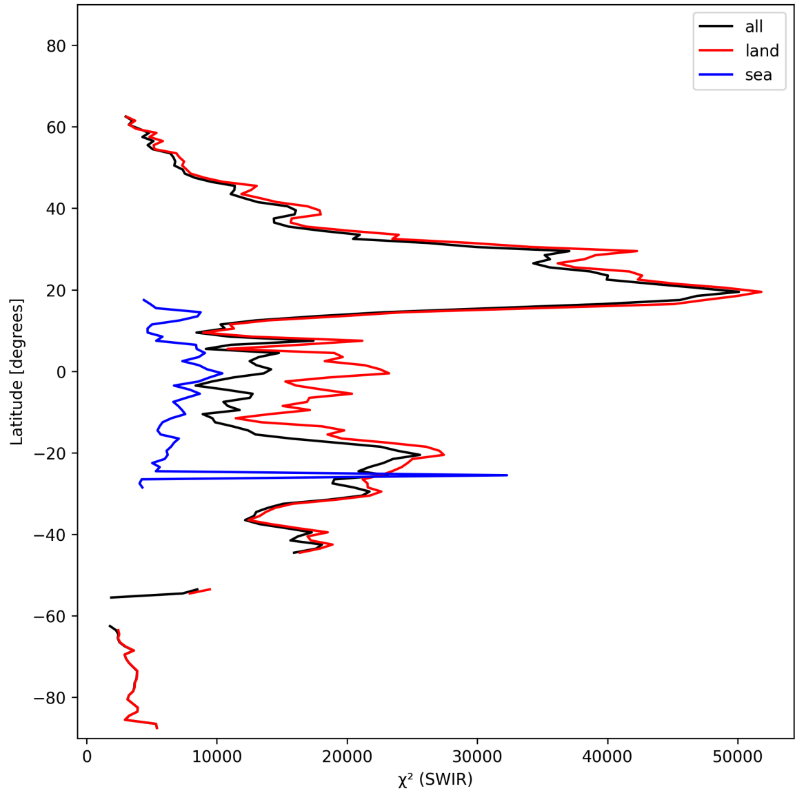
Figure 17: Zonal average of “ \chi^2 (SWIR)” for 2024-10-24 to 2024-10-26.
