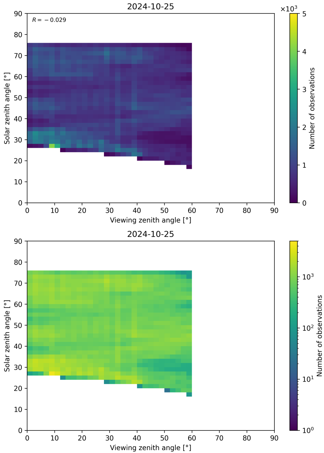
Figure 115: Scatter density plot of “Viewing zenith angle” against “Solar zenith angle” for 2024-10-24 to 2024-10-26.
