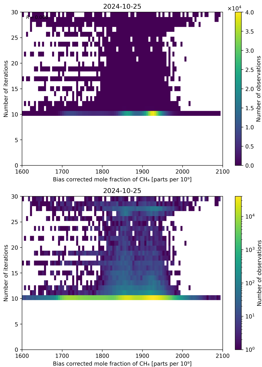
Figure 67: Scatter density plot of “Bias corrected mole fraction of \text{CH}_4 ” against “Number of iterations” for 2024-10-24 to 2024-10-26.
