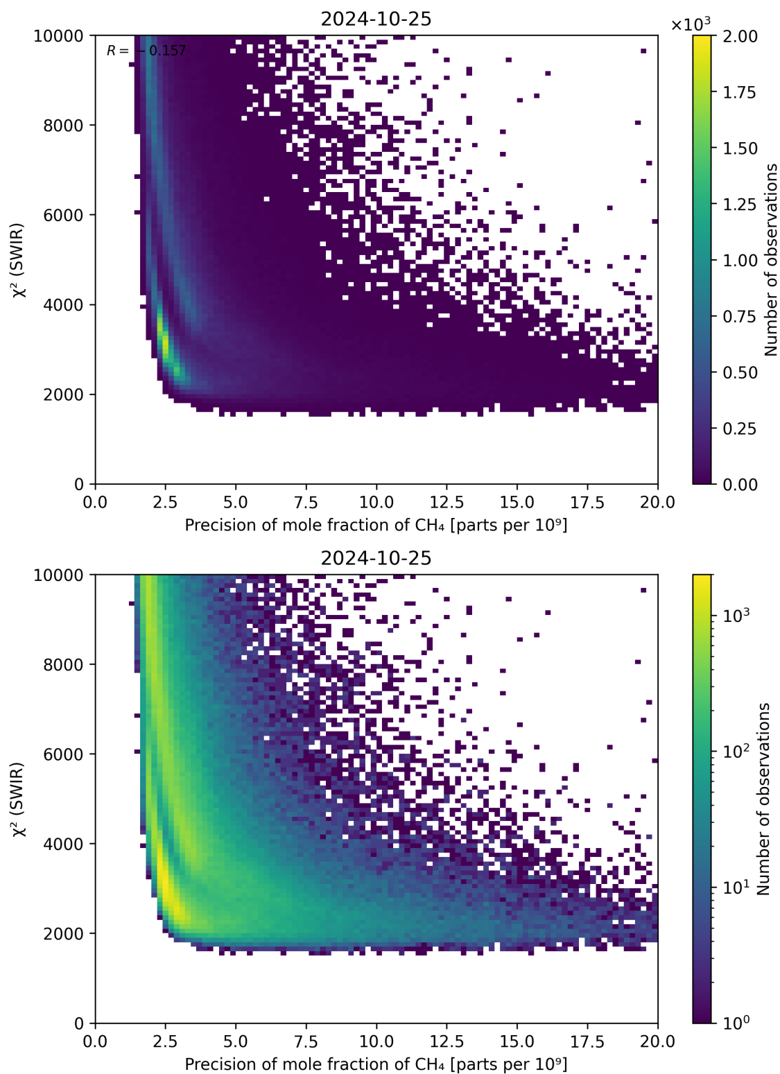
Figure 79: Scatter density plot of “Precision of mole fraction of \text{CH}_4 ” against “ \chi^2 (SWIR)” for 2024-10-24 to 2024-10-26.
