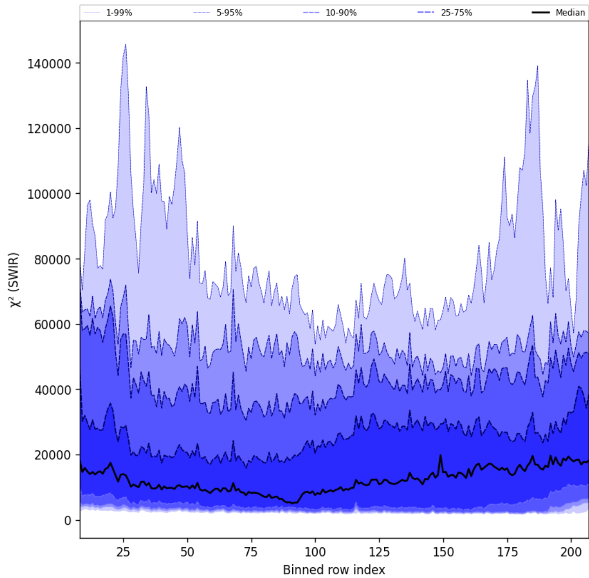
Figure 39: Along track statistics of " \chi^2 (SWIR)" for 2024-10-24 to 2024-10-26
