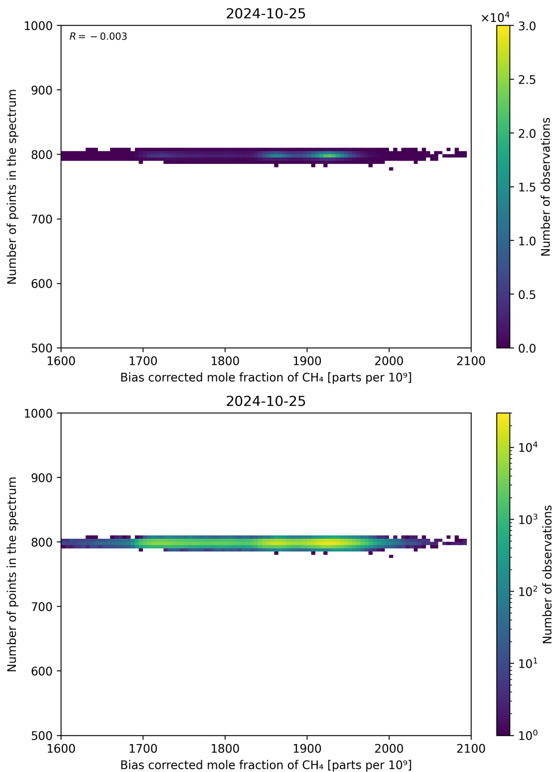
Figure 68: Scatter density plot of “Bias corrected mole fraction of CH 4 ” against “Number of points in the spectrum” for 2024-10-24 to 2024-10-26.
