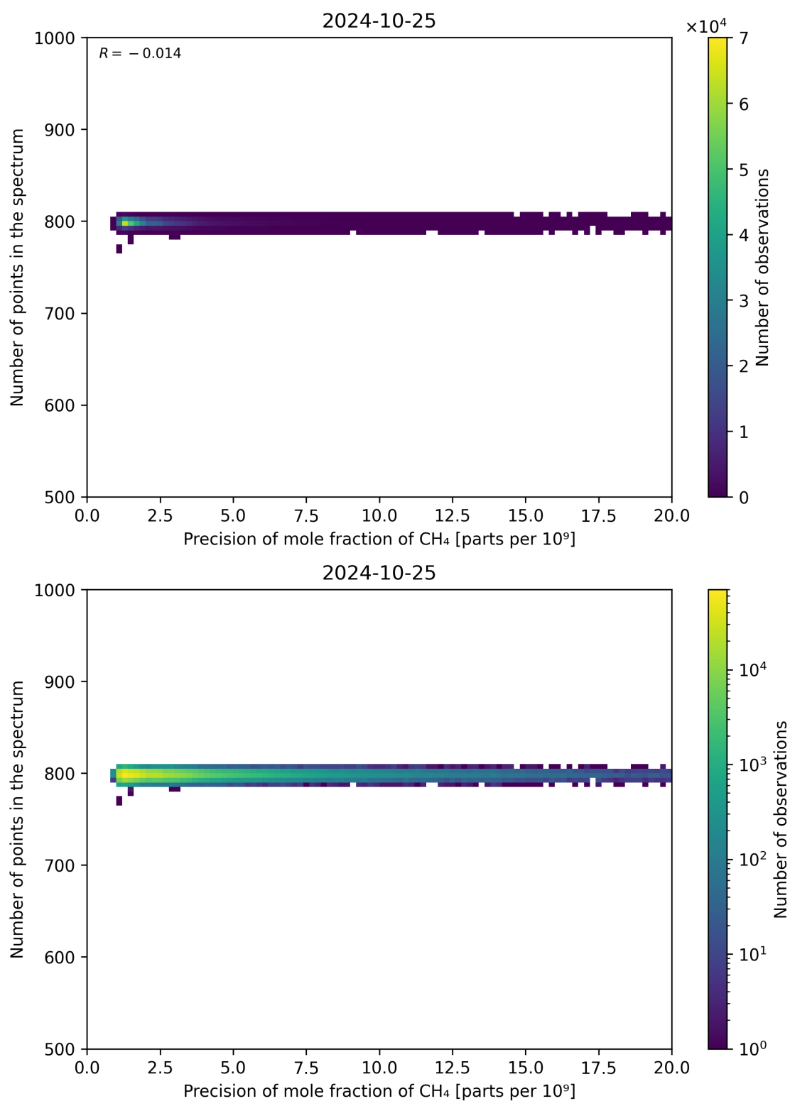
Figure 84: Scatter density plot of “Precision of mole fraction of CH 4 ” against “Number of points in the spectrum” for 2024-10-24 to 2024-10-26.
