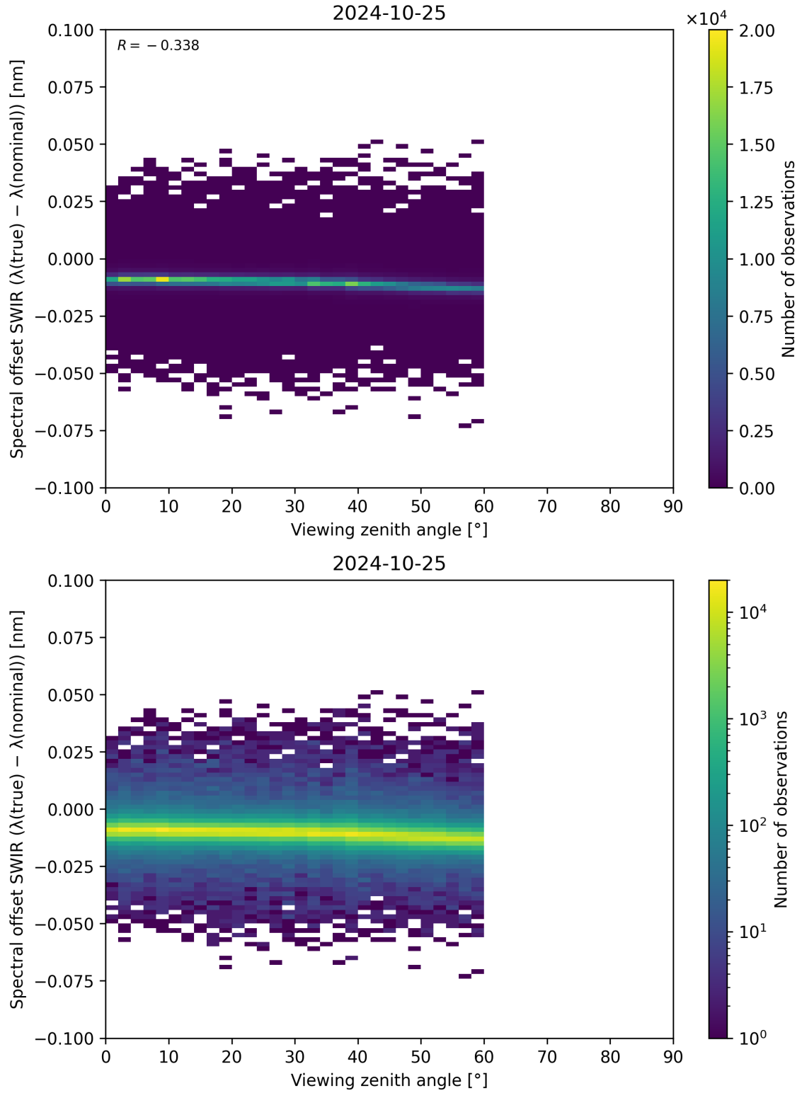
Figure 116: Scatter density plot of “Viewing zenith angle” against “Spectral offset SWIR ( \lambda_{\text{true}} - \lambda_{\text{nominal}} )” for 2024-10-24 to 2024-10-26.
