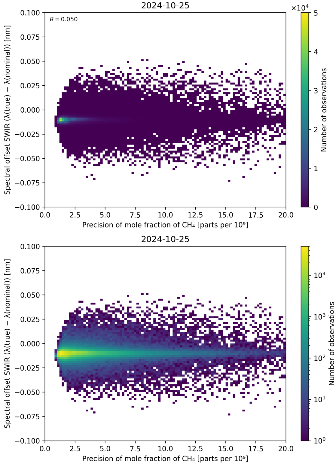
Figure 85: Scatter density plot of “Precision of mole fraction of CH 4 ” against “Spectral offset SWIR ( \lambda_{\text{true}} - \lambda_{\text{nominal}} )” for 2024-10-24 to 2024-10-26.
