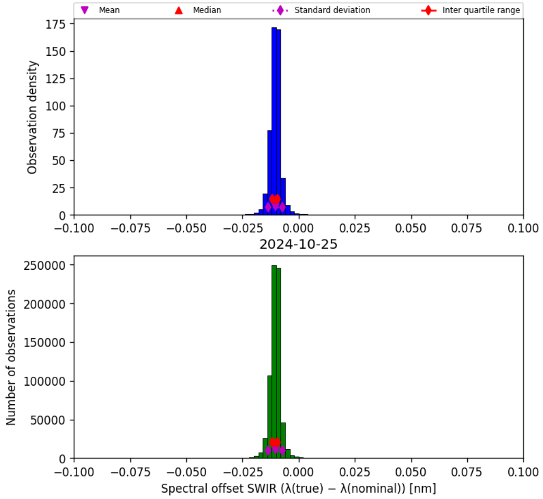
Figure 27: Histogram of “Spectral offset SWIR ( \lambda_{\text{true}} - \lambda_{\text{nominal}} )” for 2024-10-24 to 2024-10-26
