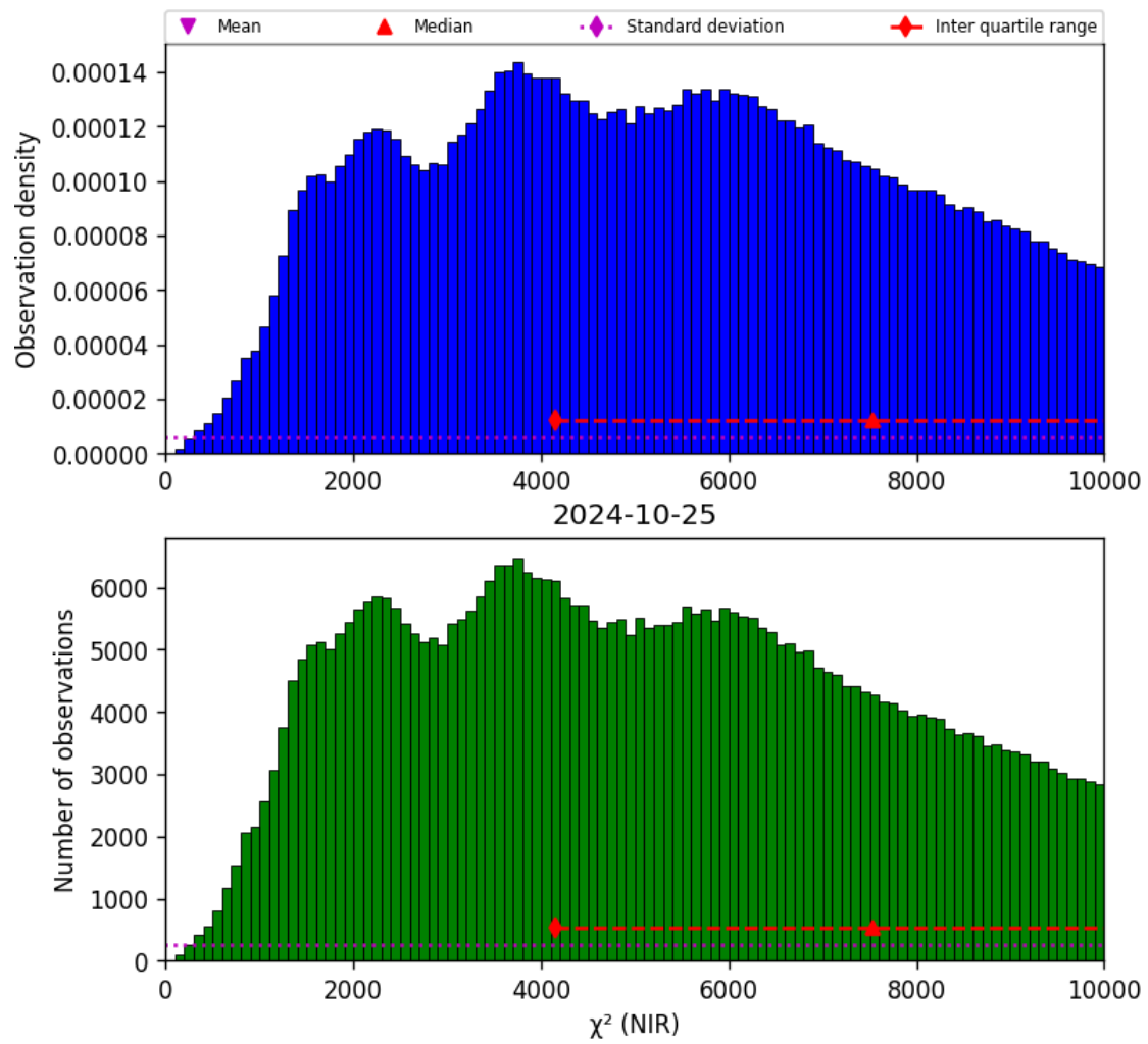
Figure 29: Histogram of “ \chi^2 (NIR)” for 2024-10-24 to 2024-10-26
