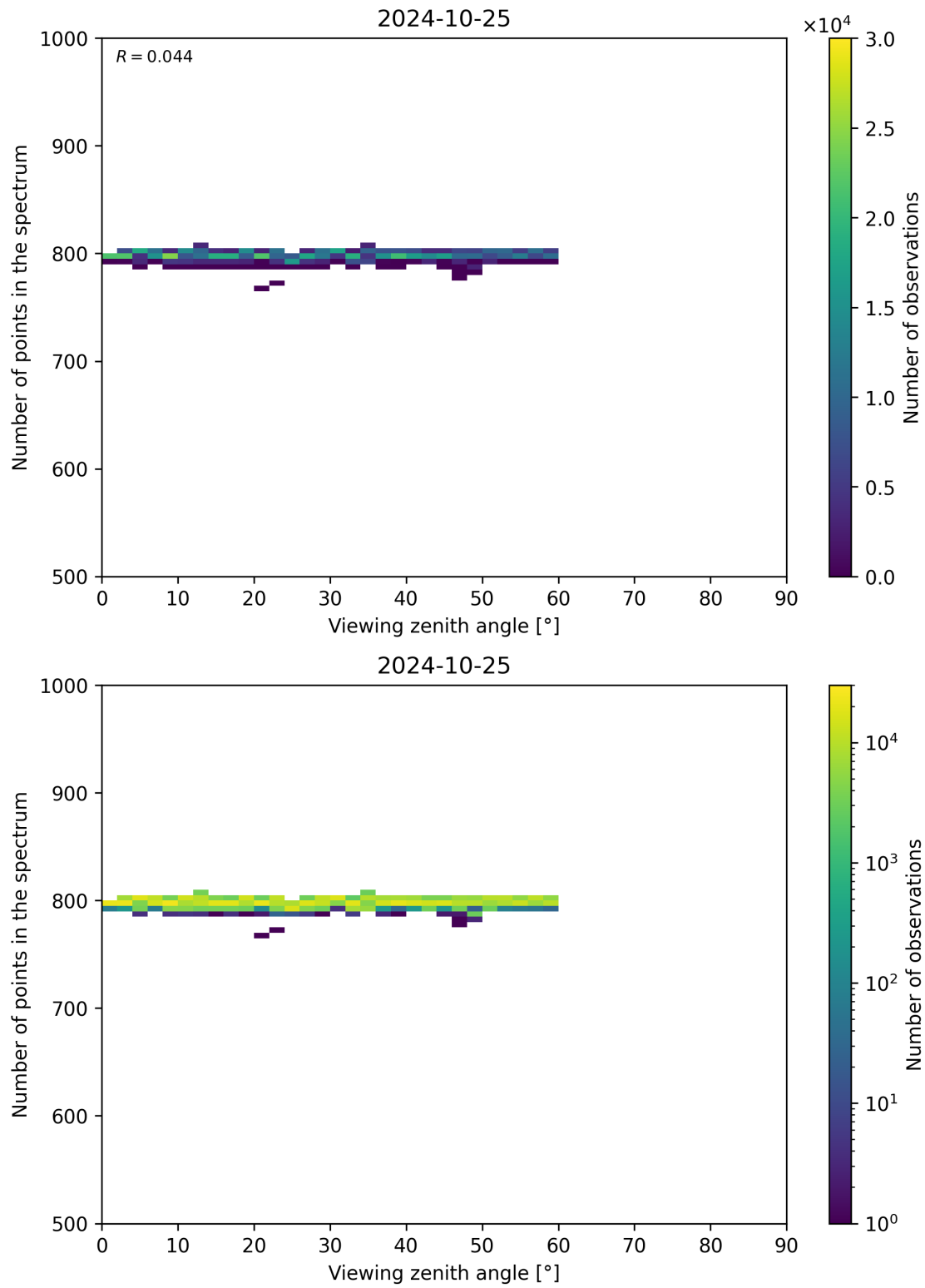
Figure 114: Scatter density plot of “Viewing zenith angle” against “Number of points in the spectrum” for 2024-10-24 to 2024-10-26.
