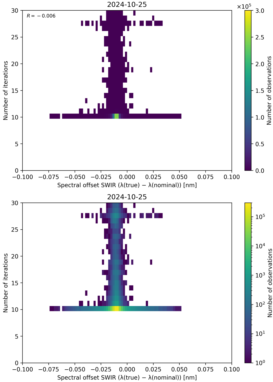
Figure 121: Scatter density plot of “Spectral offset SWIR ( \lambda_{\text{true}} - \lambda_{\text{nominal}} )” against “Number of iterations” for 2024-10-24 to 2024-10-26.
