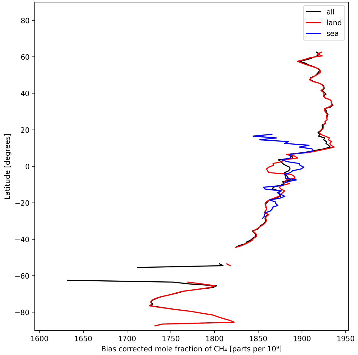
Figure 14: Zonal average of “Bias corrected mole fraction of CH 4 ” for 2024-10-24 to 2024-10-26.
