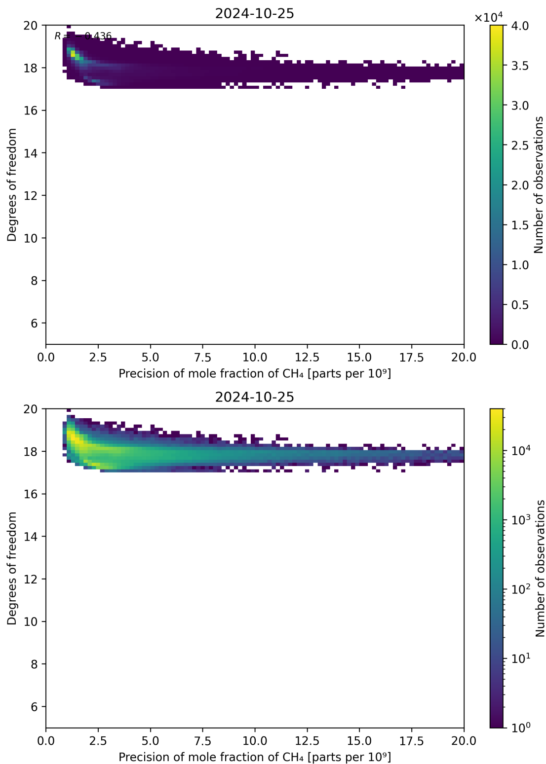
Figure 80: Scatter density plot of “Precision of mole fraction of CH 4 ” against “Degrees of freedom” for 2024-10-24 to 2024-10-26.
