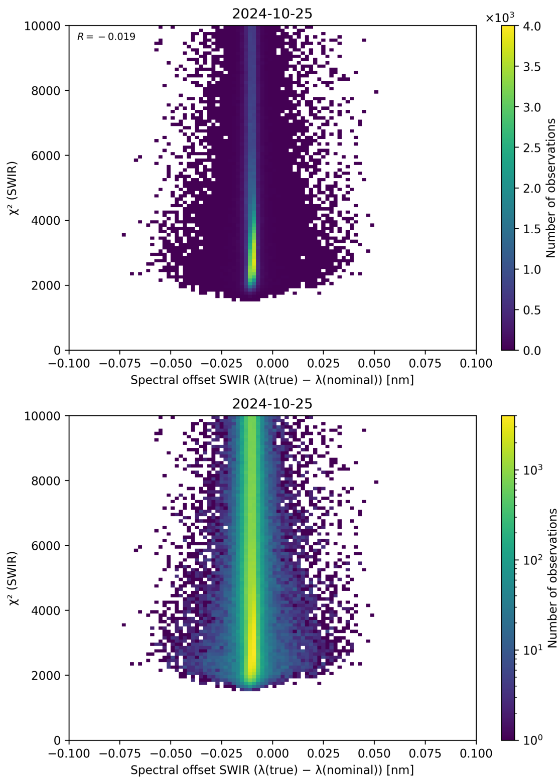
Figure 118: Scatter density plot of “Spectral offset SWIR ( \lambda_{\text{true}} - \lambda_{\text{nominal}} )” against “ \chi^2 (SWIR)” for 2024-10-24 to 2024-10-26.
