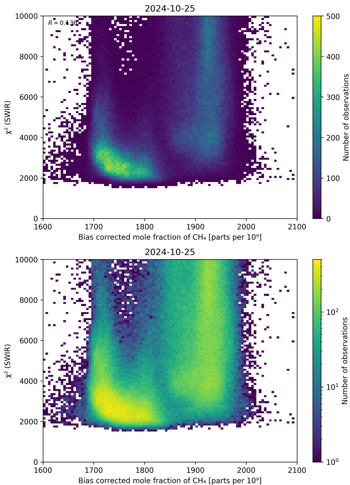
Figure 64: Scatter density plot of “Bias corrected mole fraction of \text{CH}_4 ” against “ \chi^2 (SWIR)” for 2024-10-24 to 2024-10-26.
