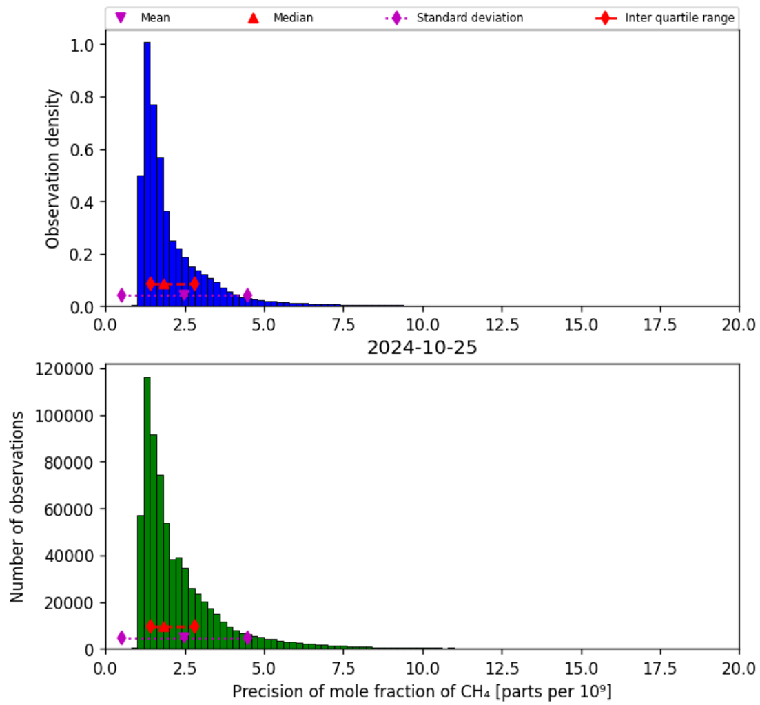
Figure 24: Histogram of “Precision of mole fraction of CH 4 ” for 2024-10-24 to 2024-10-26
