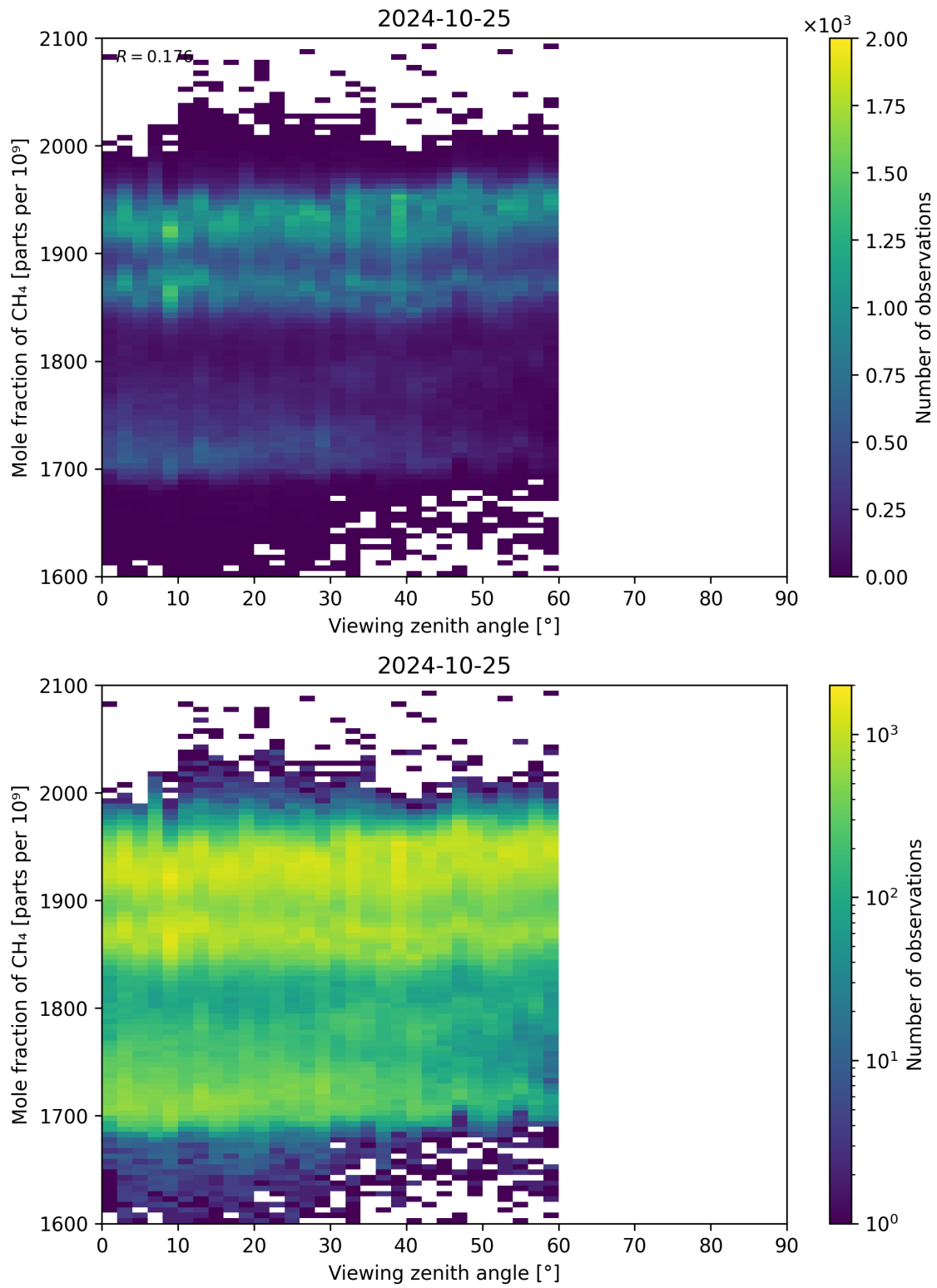
Figure 110: Scatter density plot of “Viewing zenith angle” against “Mole fraction of CH 4 ” for 2024-10-24 to 2024-10-26.
