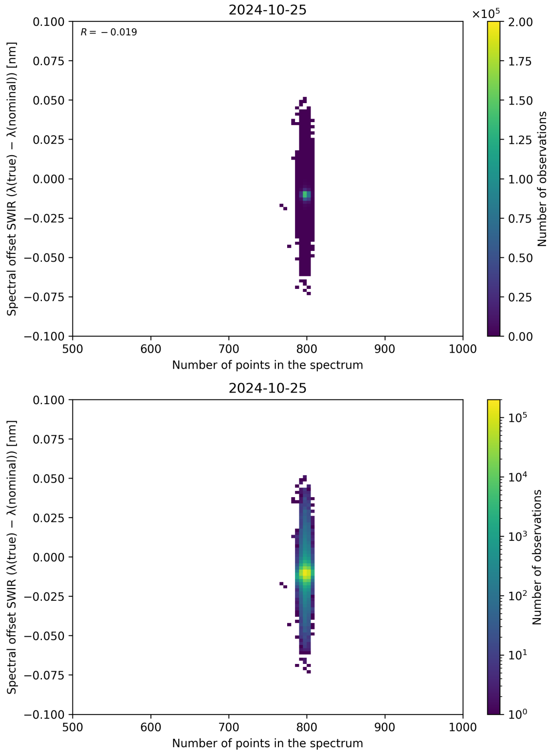
Figure 93: Scatter density plot of “Number of points in the spectrum” against “Spectral offset SWIR ( \lambda_{\text{true}} - \lambda_{\text{nominal}} )” for 2024-10-24 to 2024-10-26.
