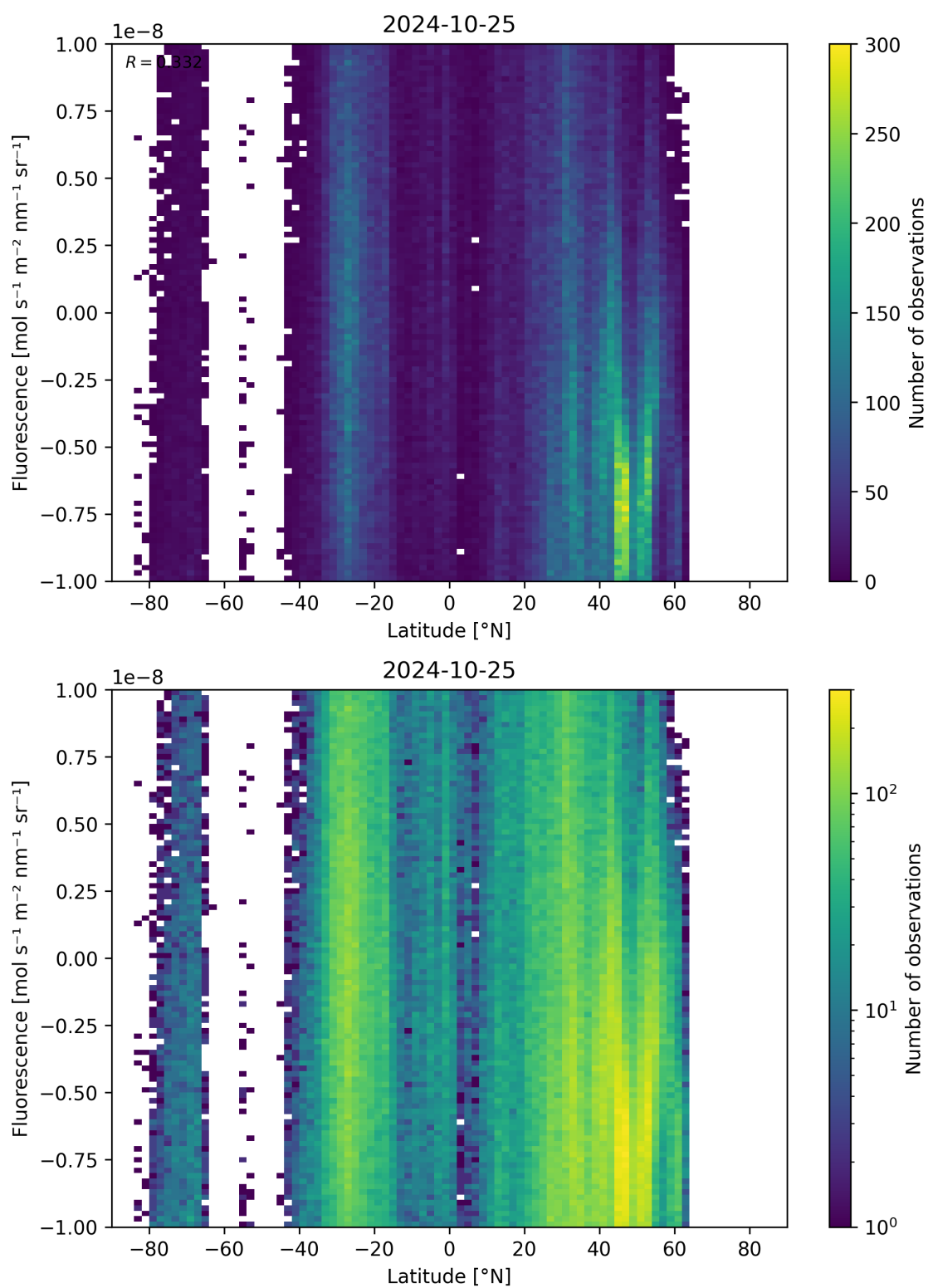
Figure 56: Scatter density plot of “Latitude” against “Fluorescence” for 2024-10-24 to 2024-10-26.
