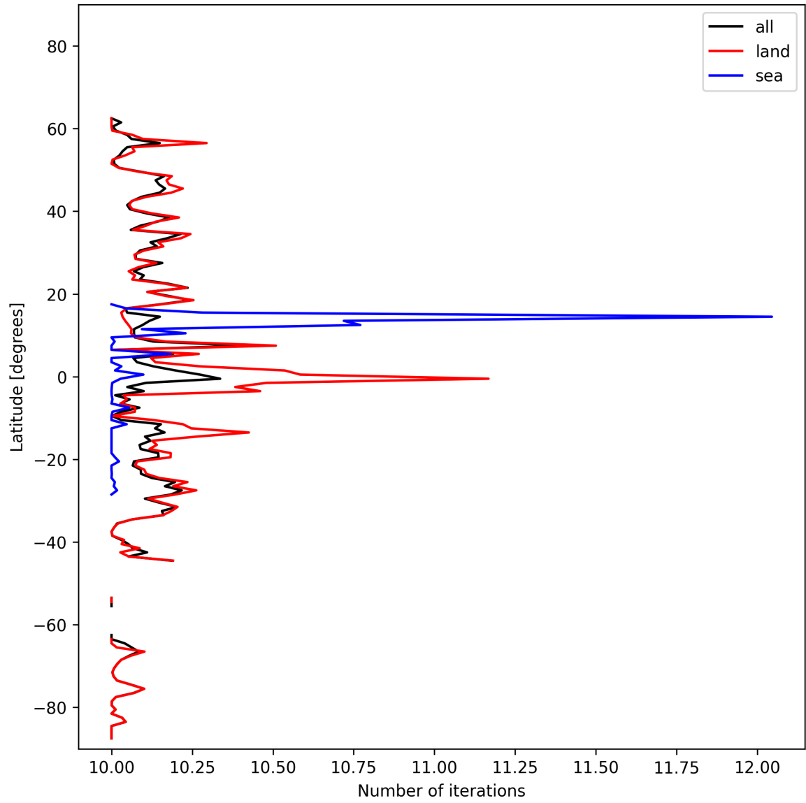
Figure 20: Zonal average of “Number of iterations” for 2024-10-24 to 2024-10-26.
