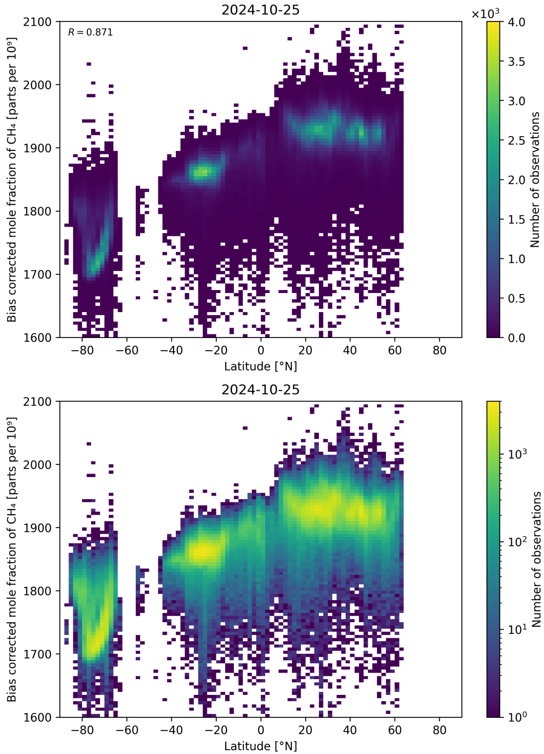
Figure 58: Scatter density plot of “Latitude” against “Bias corrected mole fraction of \text{CH}_4 ” for 2024-10-24 to 2024-10-26.
