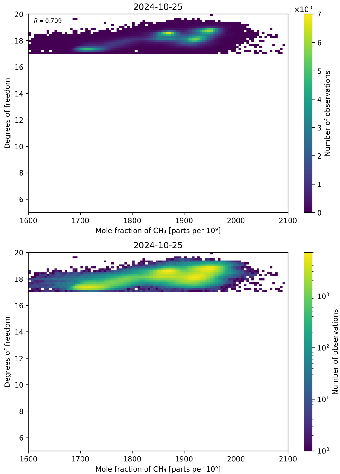
Figure 72: Scatter density plot of “Mole fraction of CH 4 ” against “Degrees of freedom” for 2024-10-24 to 2024-10-26.
