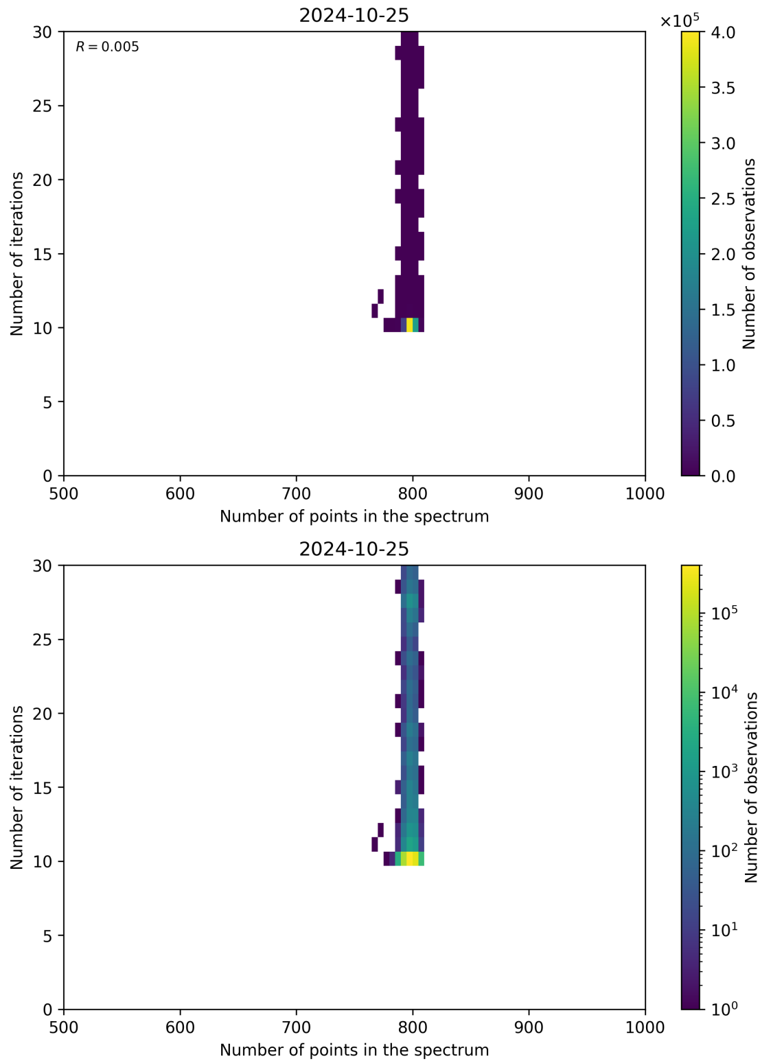
Figure 92: Scatter density plot of “Number of points in the spectrum” against “Number of iterations” for 2024-10-24 to 2024-10-26.
