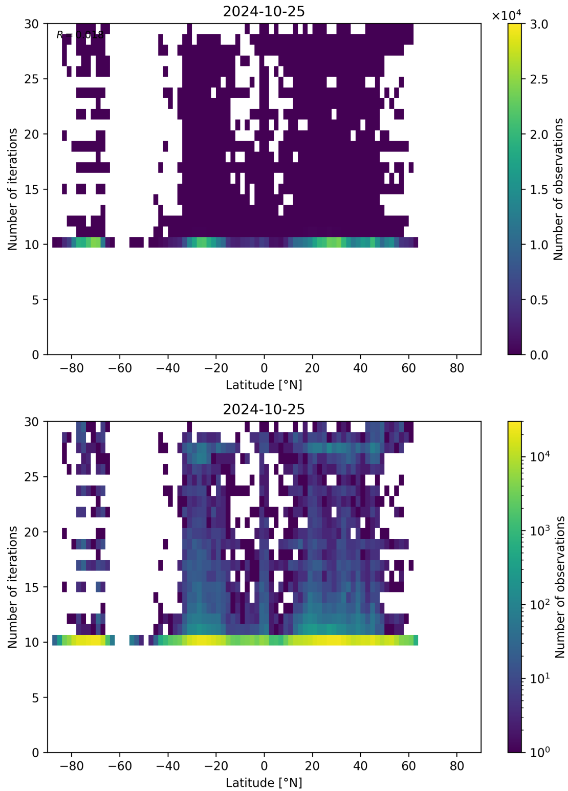
Figure 60: Scatter density plot of “Latitude” against “Number of iterations” for 2024-10-24 to 2024-10-26.
