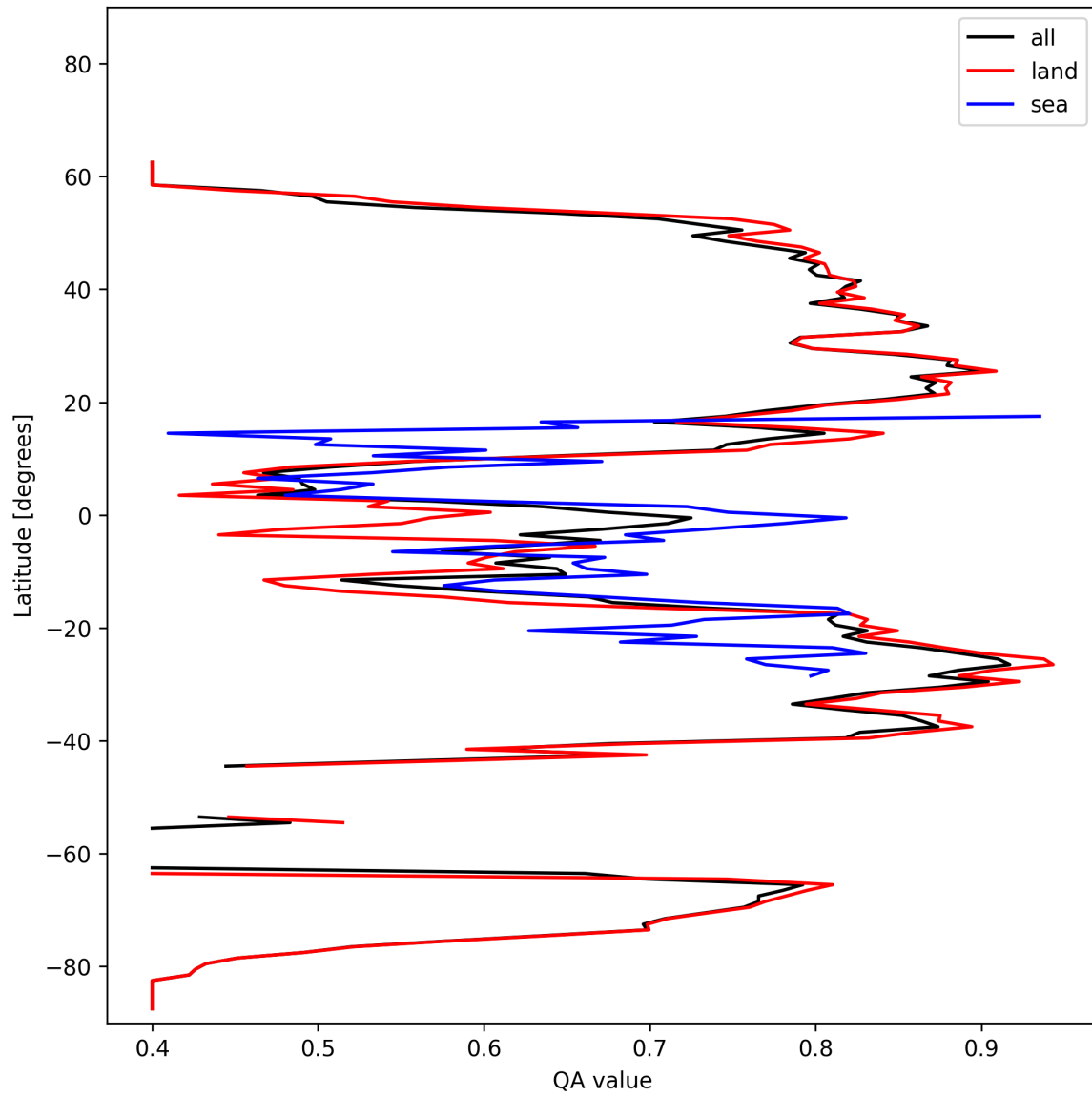
Figure 11: Zonal average of “QA value” for 2024-10-24 to 2024-10-26.
