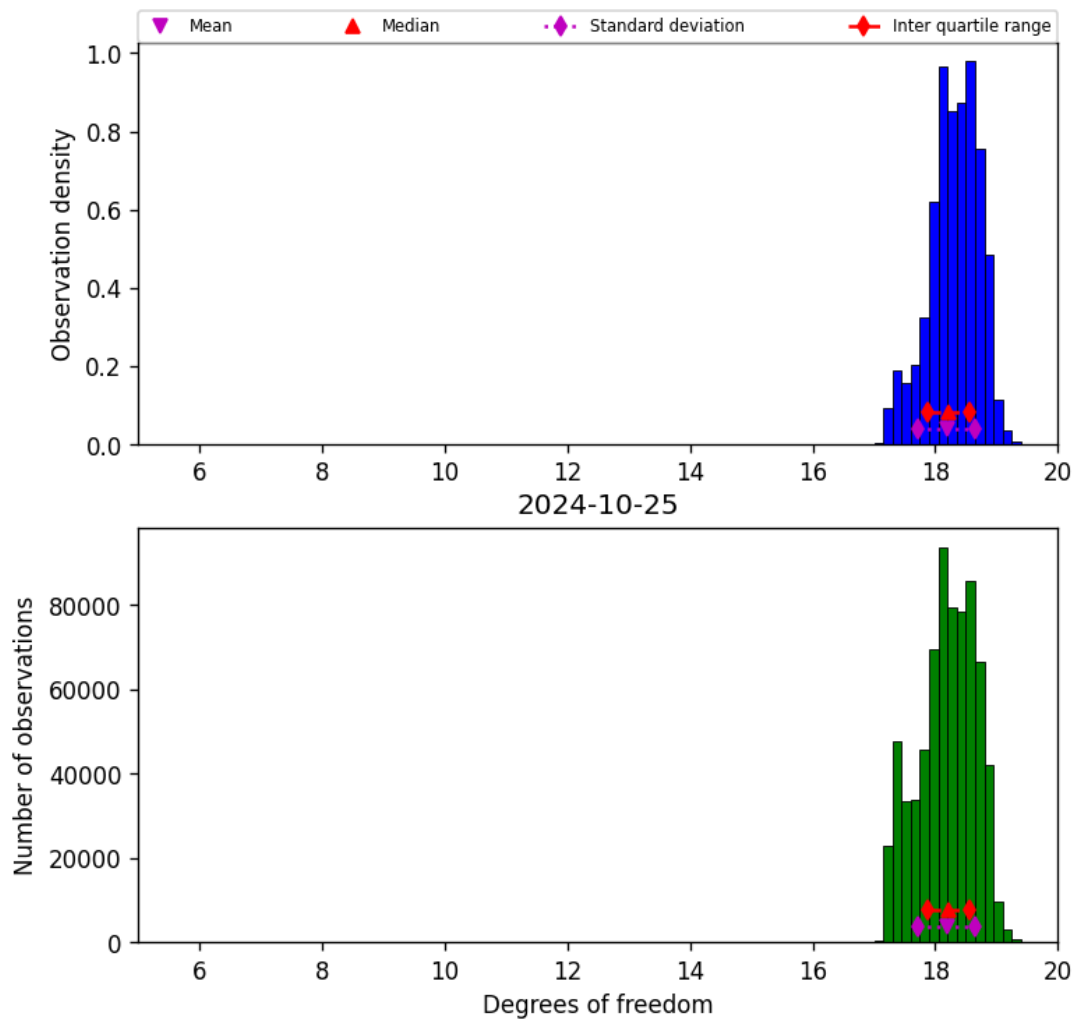
Figure 30: Histogram of “Degrees of freedom” for 2024-10-24 to 2024-10-26
