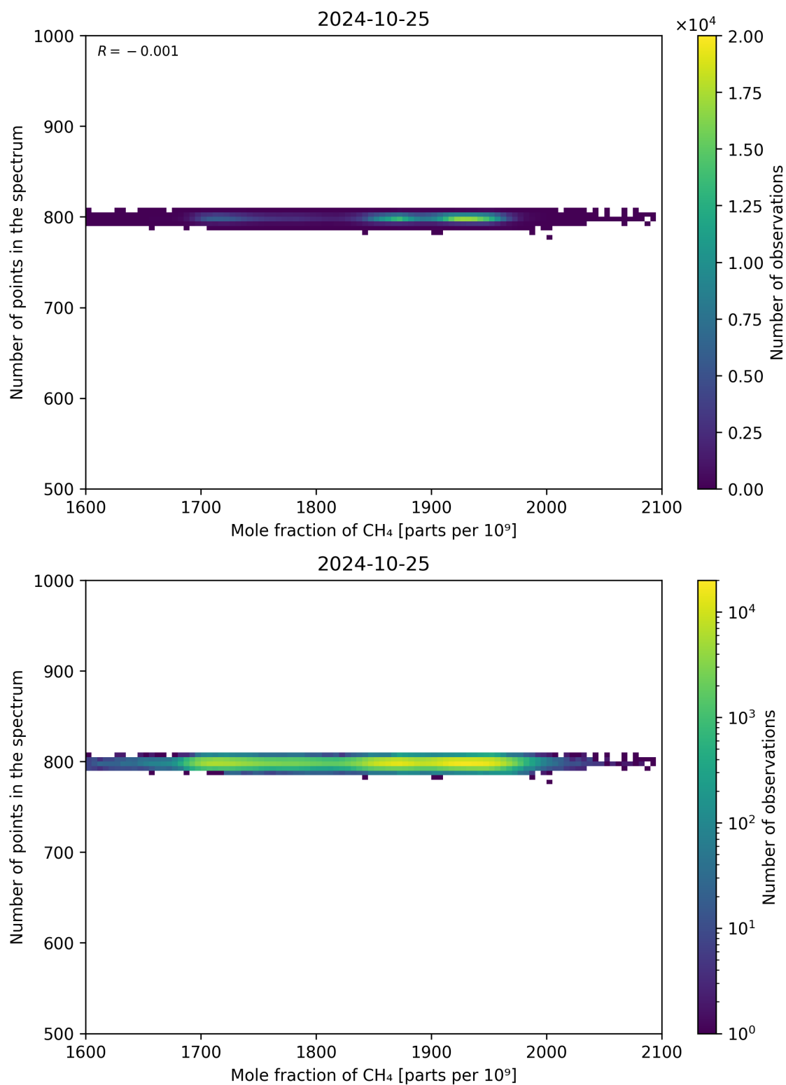
Figure 77: Scatter density plot of “Mole fraction of CH 4 ” against “Number of points in the spectrum” for 2024-10-24 to 2024-10-26.
