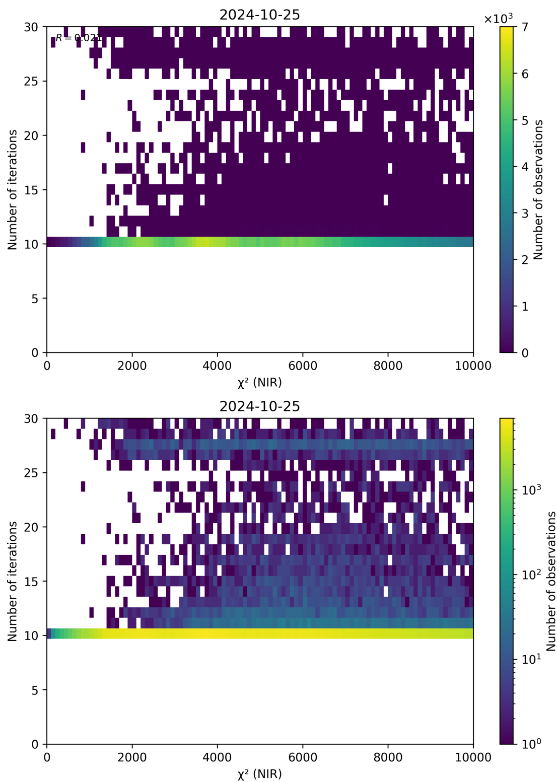
Figure 46: Scatter density plot of “ \chi^2 (NIR)” against “Number of iterations” for 2024-10-24 to 2024-10-26.
