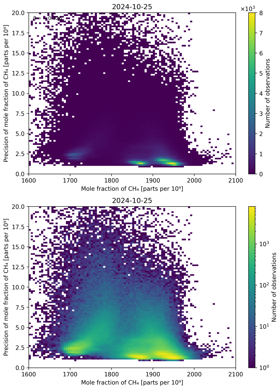
Figure 75: Scatter density plot of “Mole fraction of CH 4 ” against “Precision of mole fraction of CH 4 ” for 2024-10-24 to 2024-10-26.
