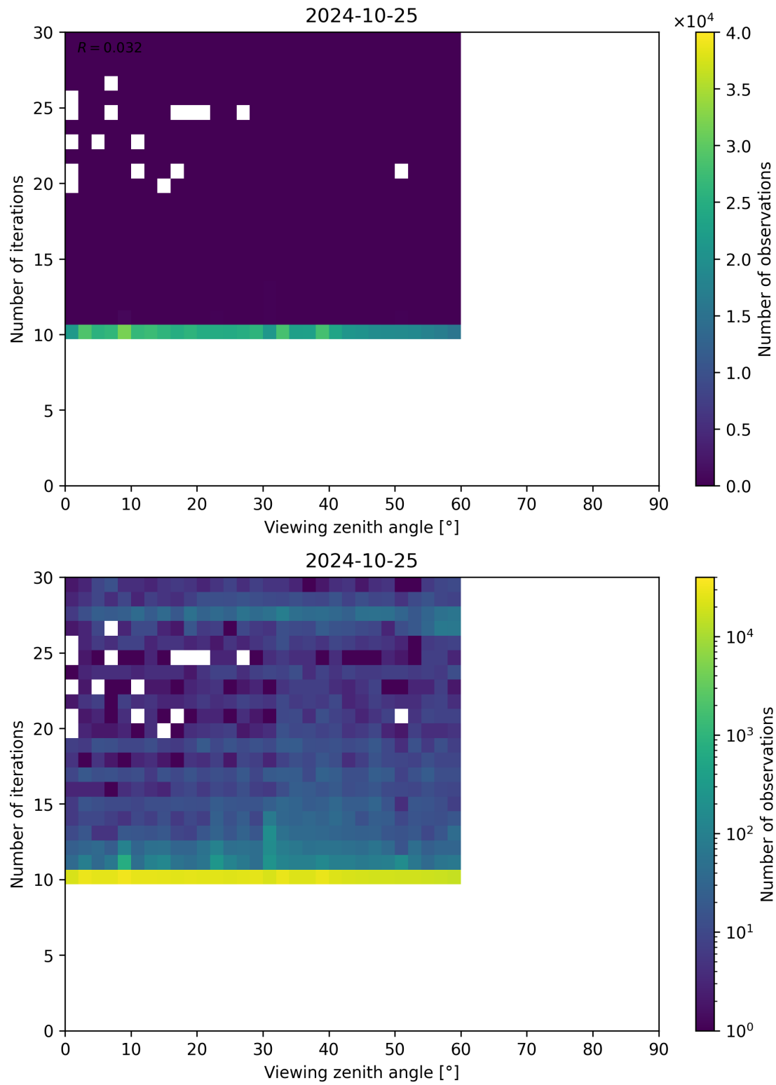
Figure 113: Scatter density plot of “Viewing zenith angle” against “Number of iterations” for 2024-10-24 to 2024-10-26.
