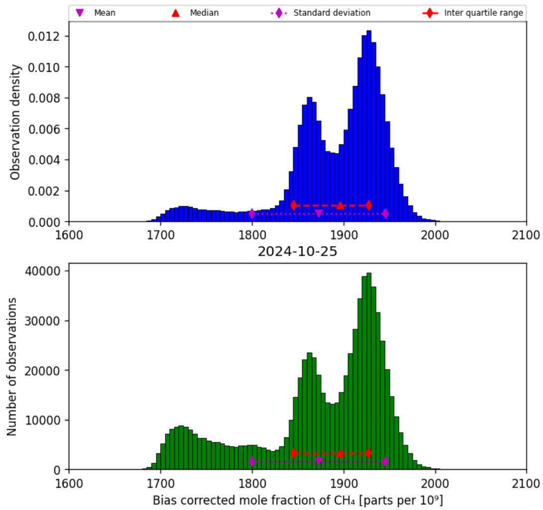
Figure 25: Histogram of “Bias corrected mole fraction of CH 4 ” for 2024-10-24 to 2024-10-26
