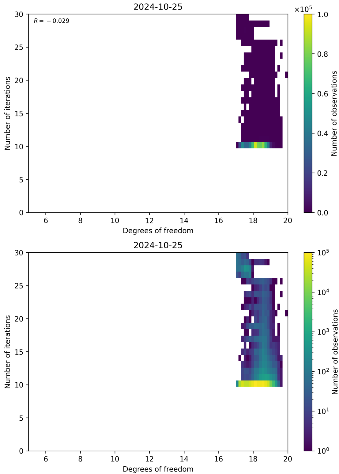
Figure 52: Scatter density plot of “Degrees of freedom” against “Number of iterations” for 2024-10-24 to 2024-10-26.
