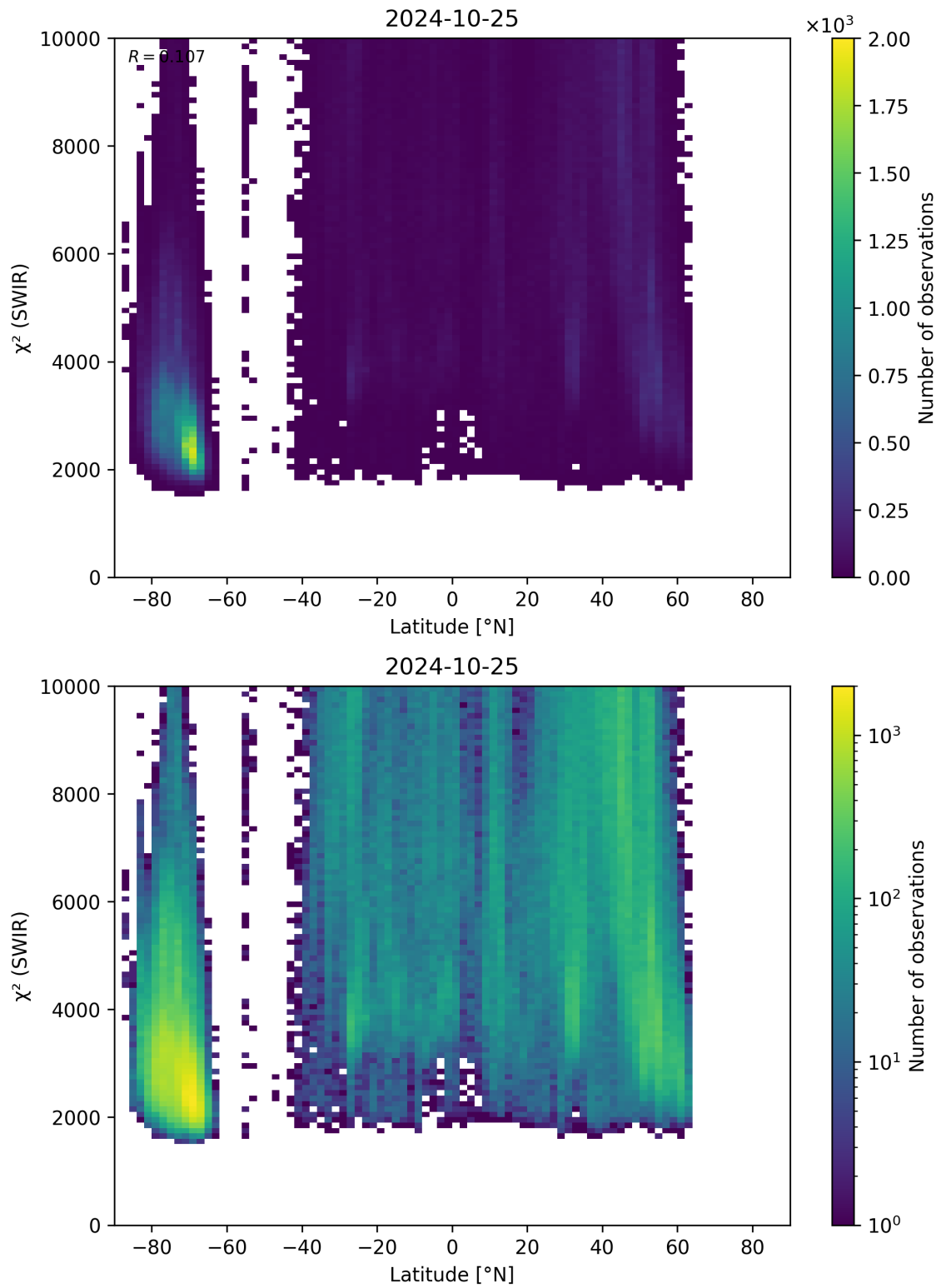
Figure 54: Scatter density plot of “Latitude” against “ \chi^2 (SWIR)” for 2024-10-24 to 2024-10-26.
