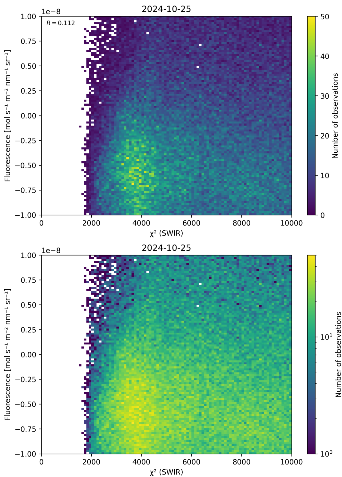
Figure 49: Scatter density plot of “ \chi^2 (SWIR)” against “Fluorescence” for 2024-10-24 to 2024-10-26.
