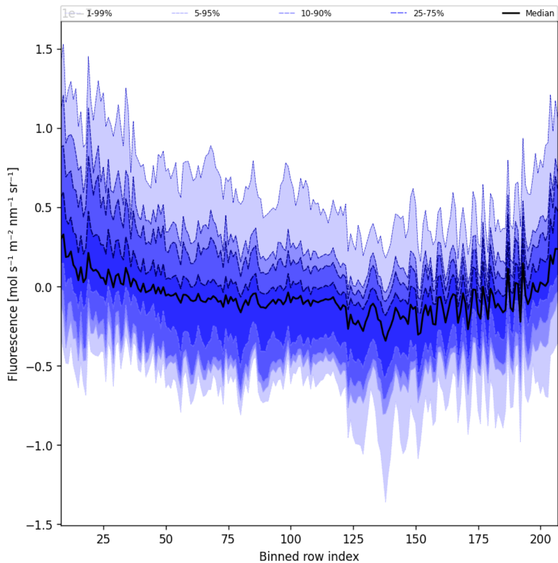
Figure 43: Along track statistics of “Fluorescence” for 2024-10-24 to 2024-10-26
