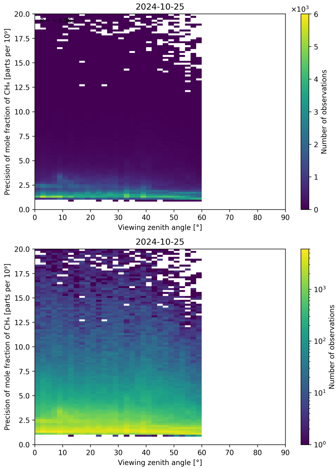
Figure 112: Scatter density plot of “Viewing zenith angle” against “Precision of mole fraction of CH 4 ” for 2024-10-24 to 2024-10-26.
