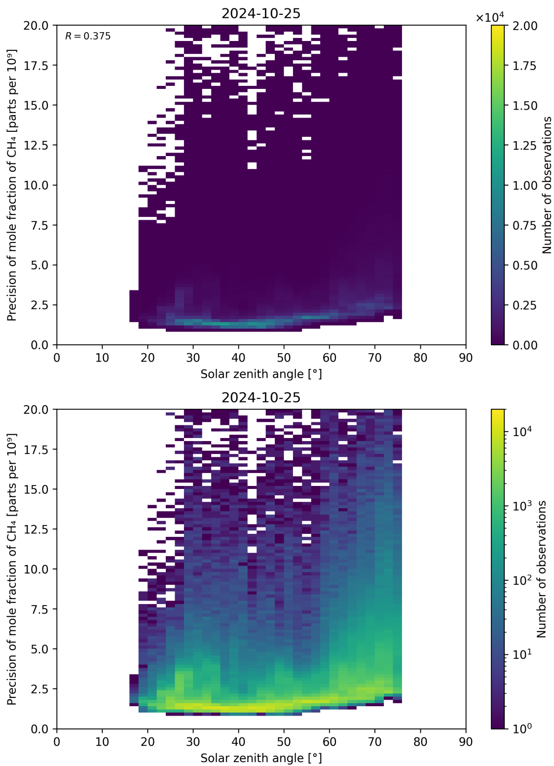
Figure 101: Scatter density plot of “Solar zenith angle” against “Precision of mole fraction of CH 4 ” for 2024-10-24 to 2024-10-26.
