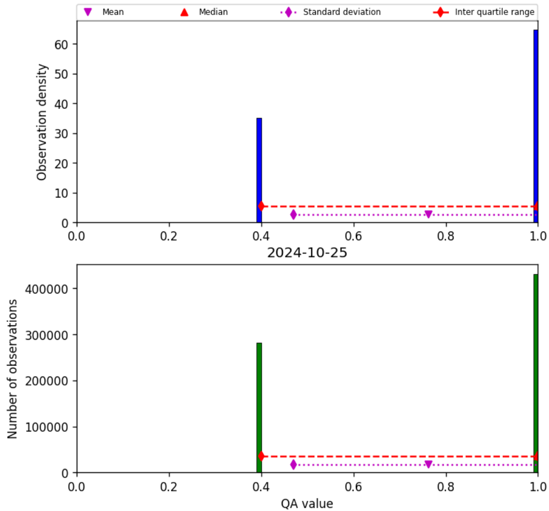
Figure 22: Histogram of “QA value” for 2024-10-24 to 2024-10-26
