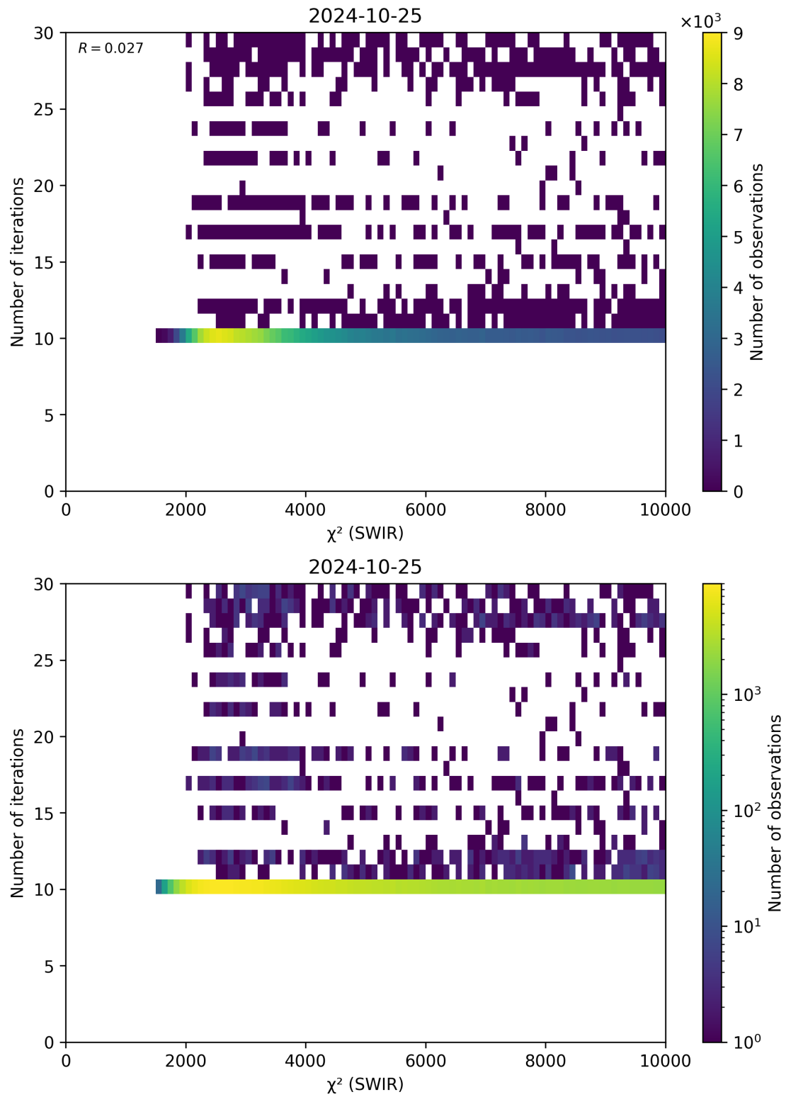
Figure 50: Scatter density plot of “ \chi^2 (SWIR)” against “Number of iterations” for 2024-10-24 to 2024-10-26.
