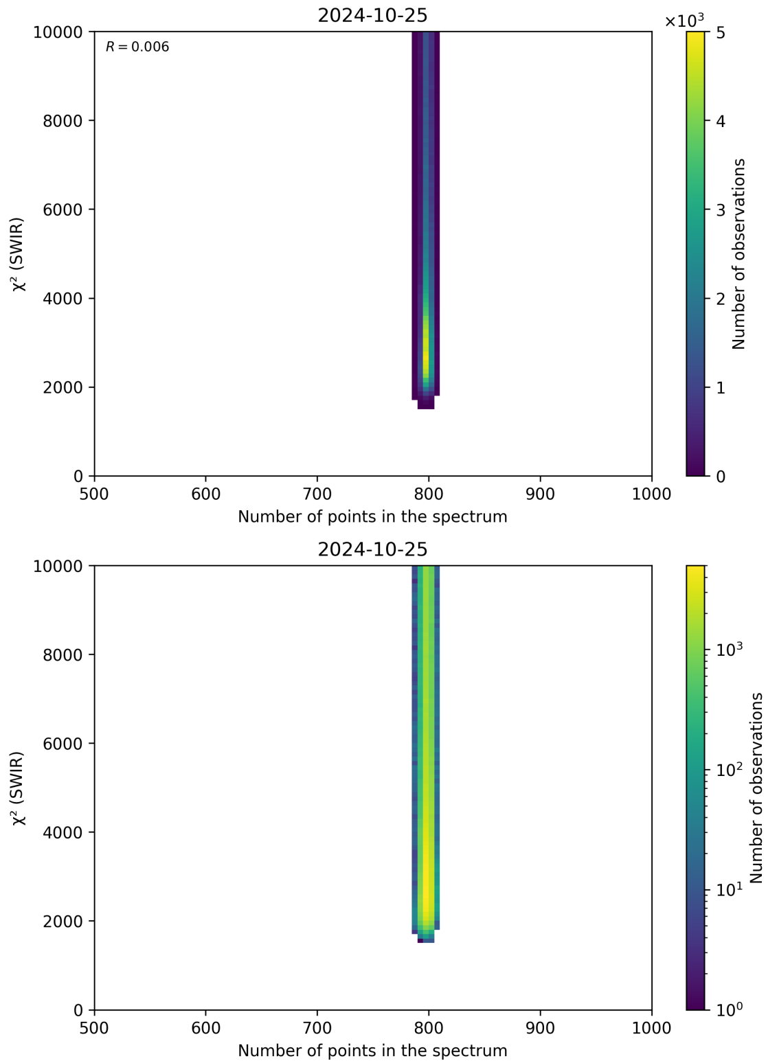
Figure 89: Scatter density plot of “Number of points in the spectrum” against “ \chi^2 (SWIR)” for 2024-10-24 to 2024-10-26.
