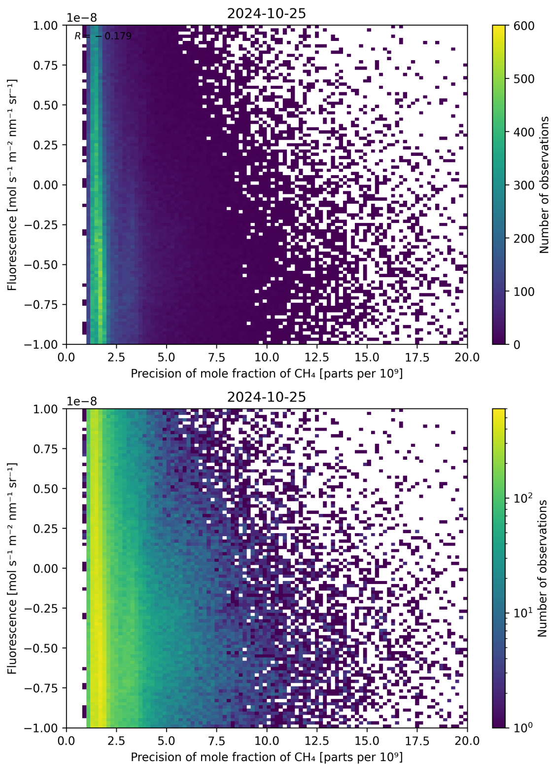
Figure 81: Scatter density plot of “Precision of mole fraction of \text{CH}_4 ” against “Fluorescence” for 2024-10-24 to 2024-10-26.
