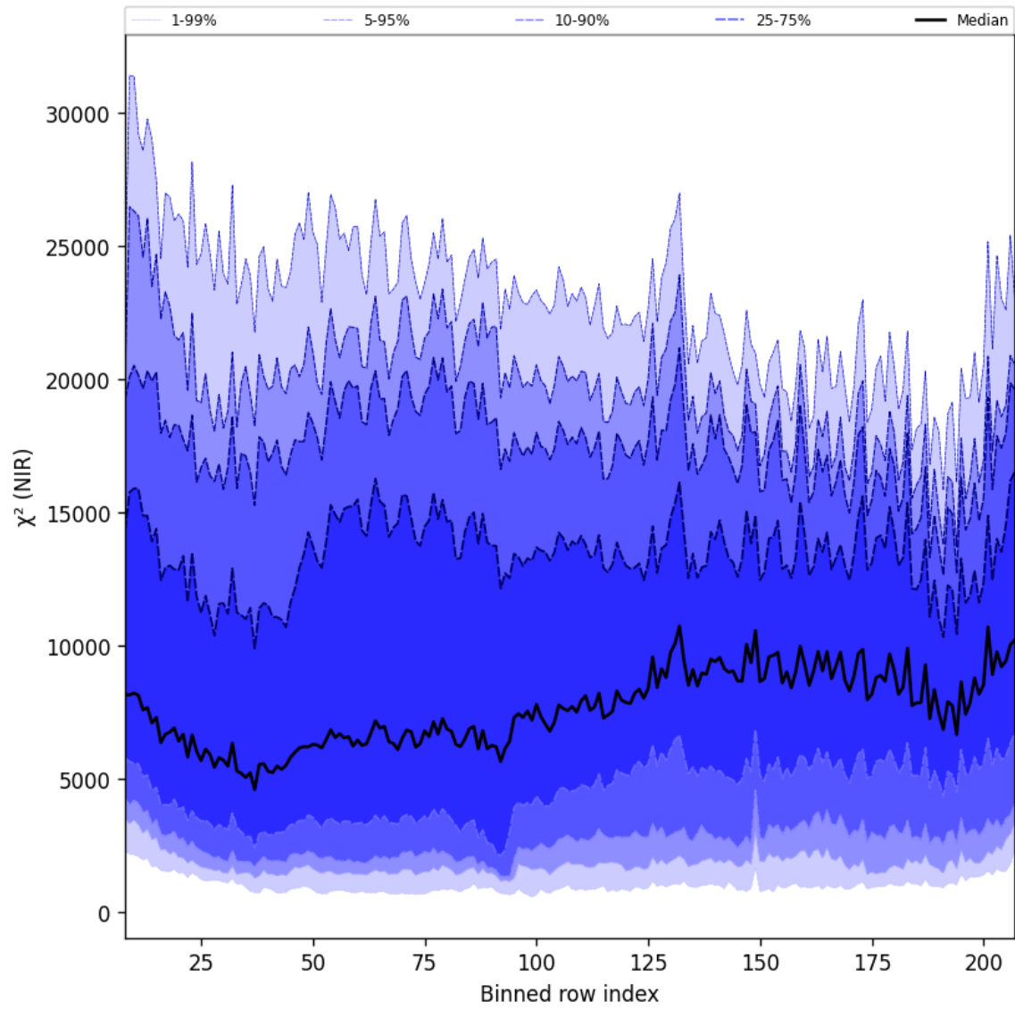
Figure 40: Along track statistics of “ \chi^2 (NIR)” for 2024-10-24 to 2024-10-26
