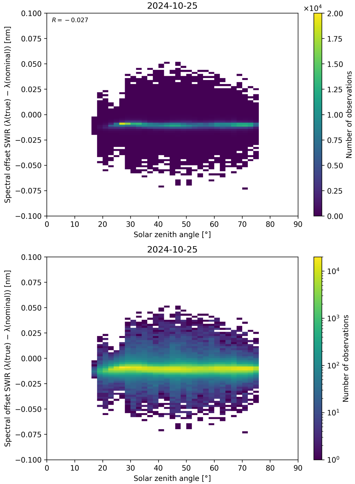
Figure 104: Scatter density plot of “Solar zenith angle” against “Spectral offset SWIR ( \lambda_{\text{true}} - \lambda_{\text{nominal}} )” for 2024-10-24 to 2024-10-26.
