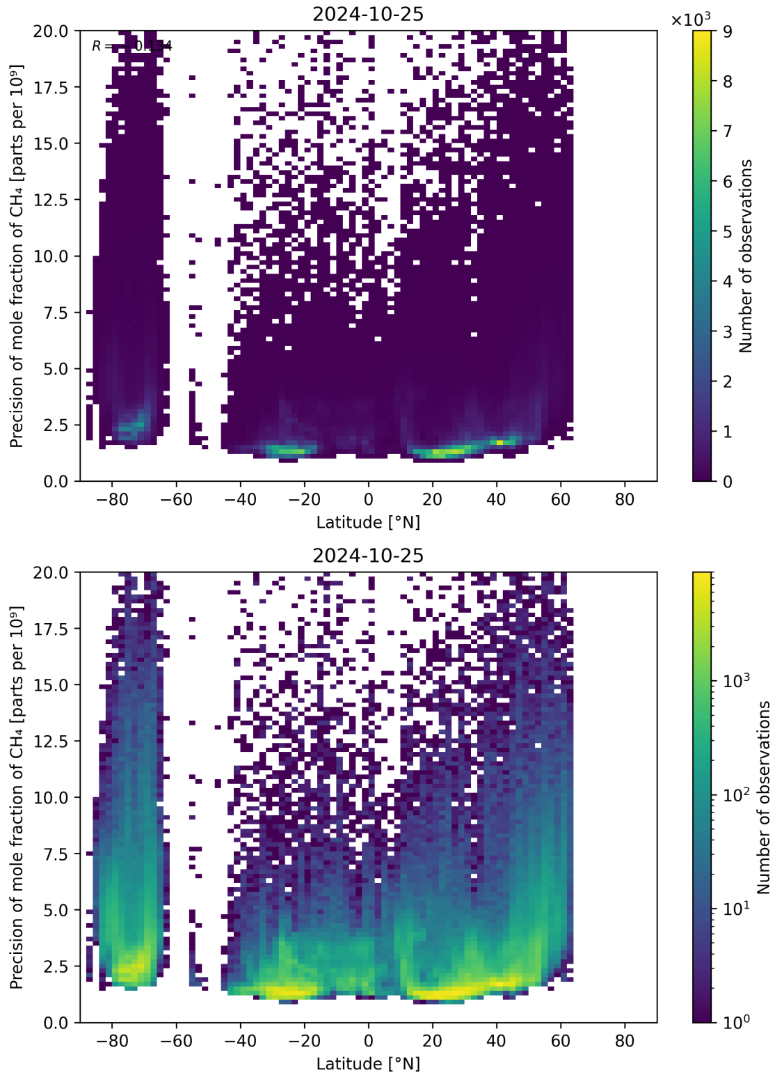
Figure 59: Scatter density plot of “Latitude” against “Precision of mole fraction of CH 4 ” for 2024-10-24 to 2024-10-26.
