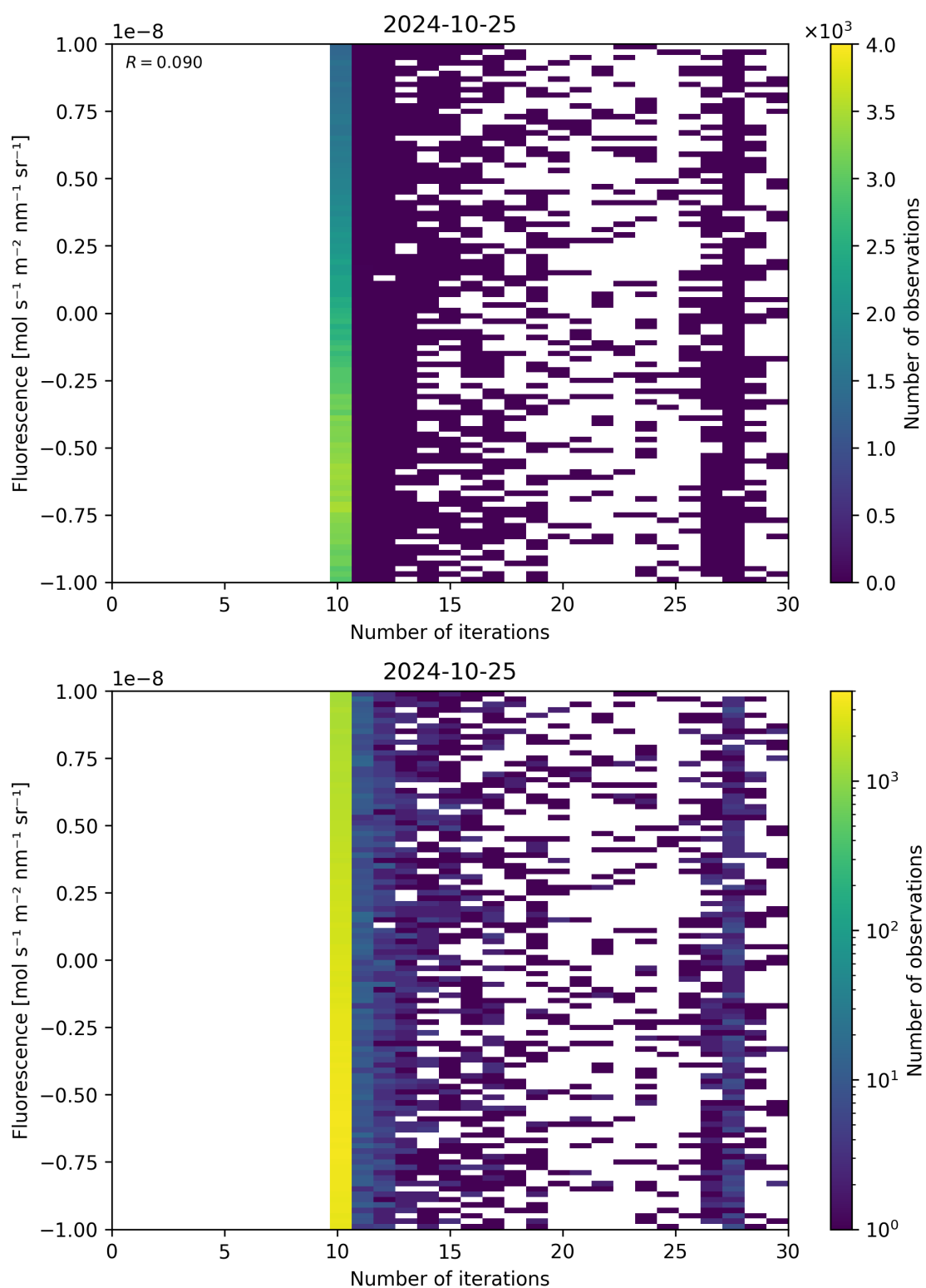
Figure 87: Scatter density plot of “Number of iterations” against “Fluorescence” for 2024-10-24 to 2024-10-26.
