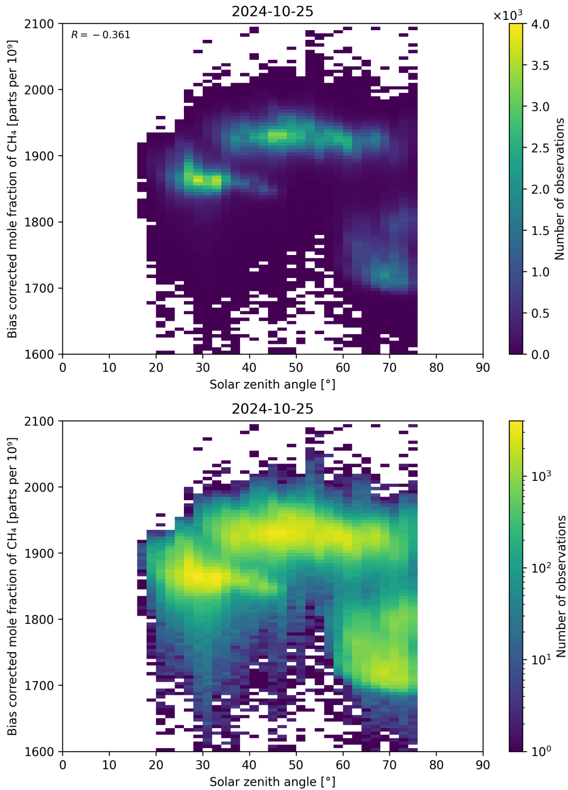
Figure 100: Scatter density plot of “Solar zenith angle” against “Bias corrected mole fraction of CH 4 ” for 2024-10-24 to 2024-10-26.
