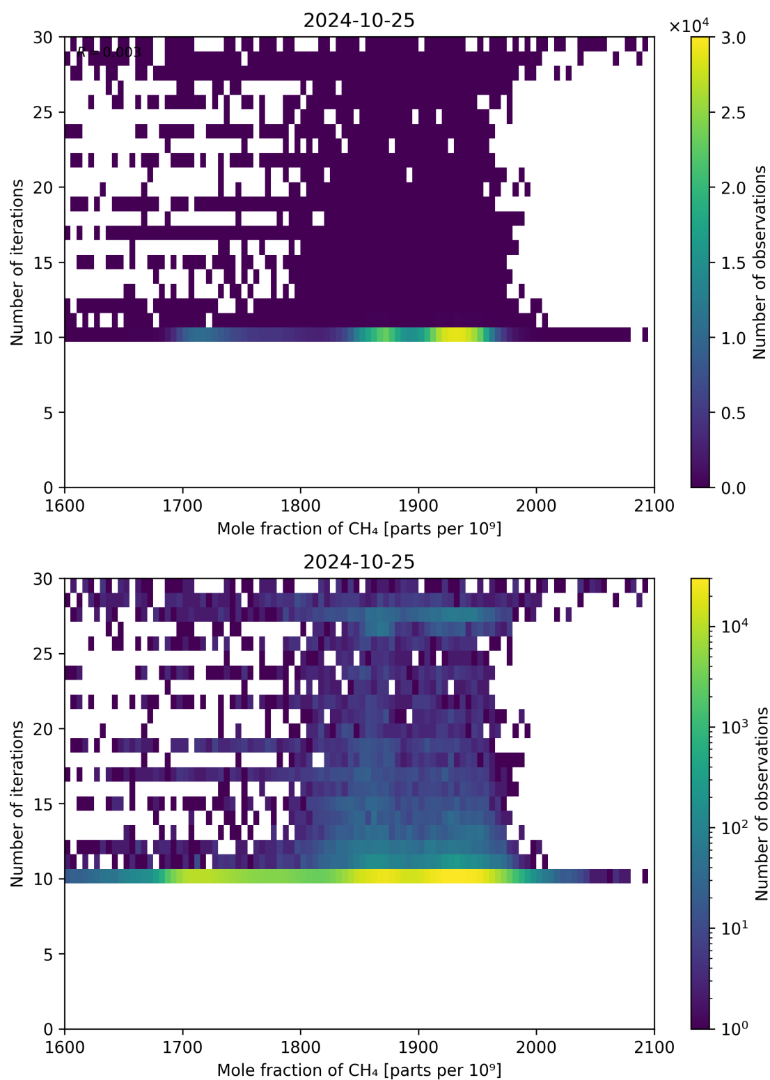
Figure 76: Scatter density plot of “Mole fraction of CH 4 ” against “Number of iterations” for 2024-10-24 to 2024-10-26.
