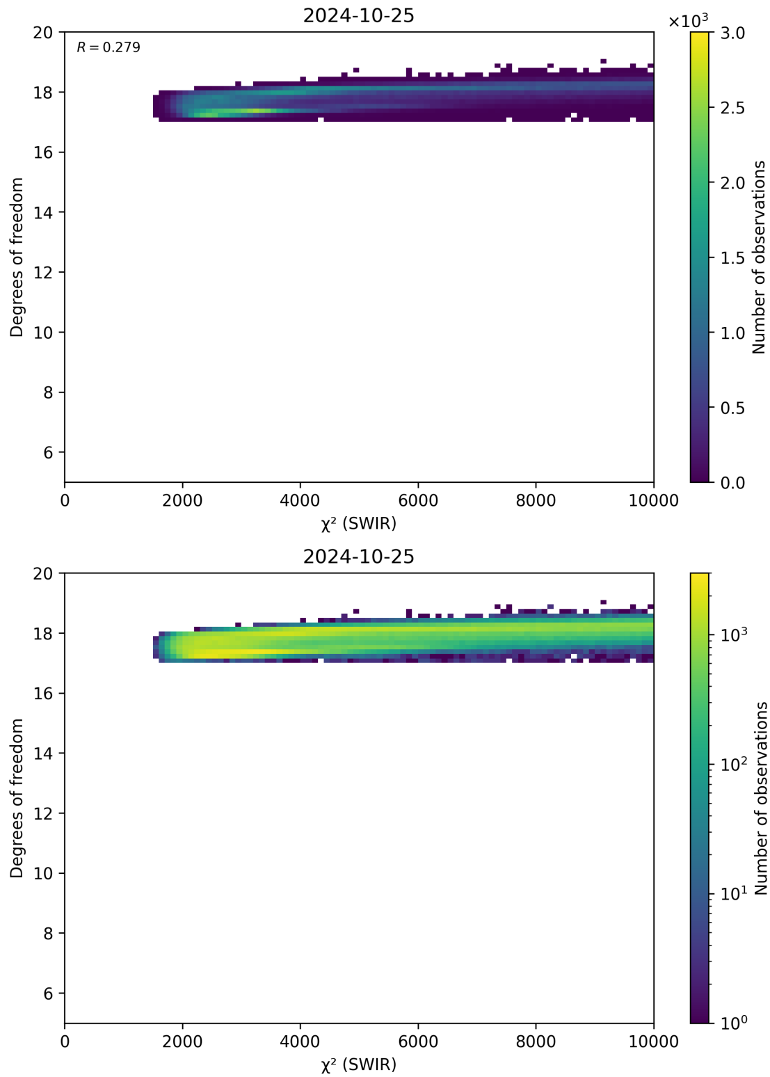
Figure 48: Scatter density plot of “ \chi^2 (SWIR)” against “Degrees of freedom” for 2024-10-24 to 2024-10-26.
