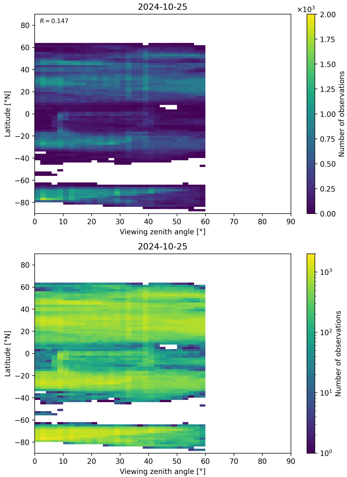
Figure 109: Scatter density plot of “Viewing zenith angle” against “Latitude” for 2024-10-24 to 2024-10-26.
