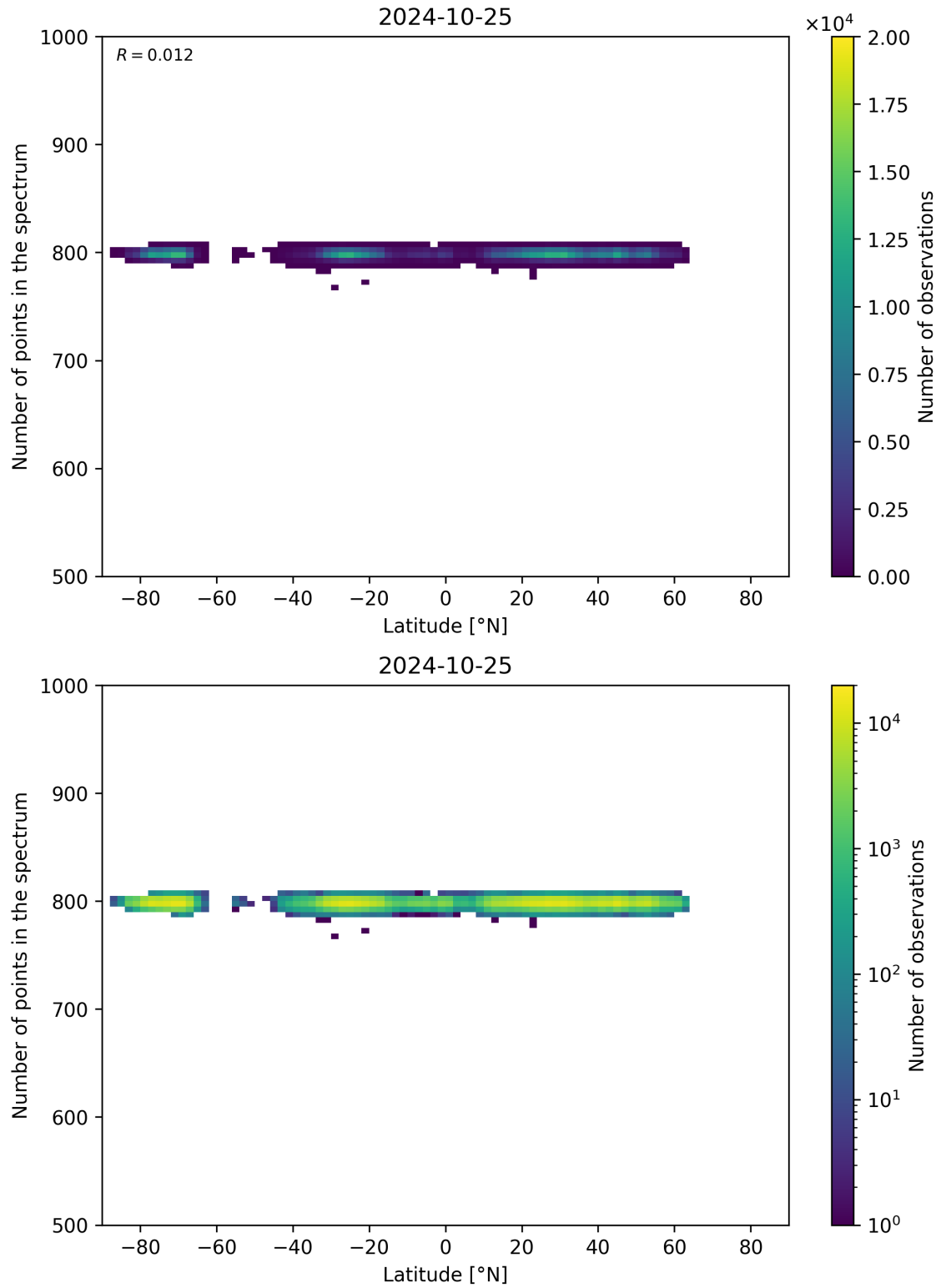
Figure 61: Scatter density plot of “Latitude” against “Number of points in the spectrum” for 2024-10-24 to 2024-10-26.
