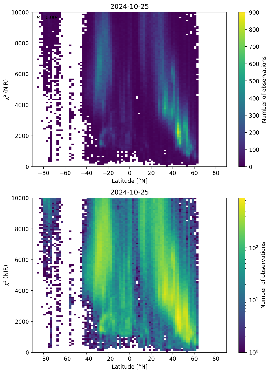
Figure 53: Scatter density plot of “Latitude” against “ \chi^2 (NIR)” for 2024-10-24 to 2024-10-26.
