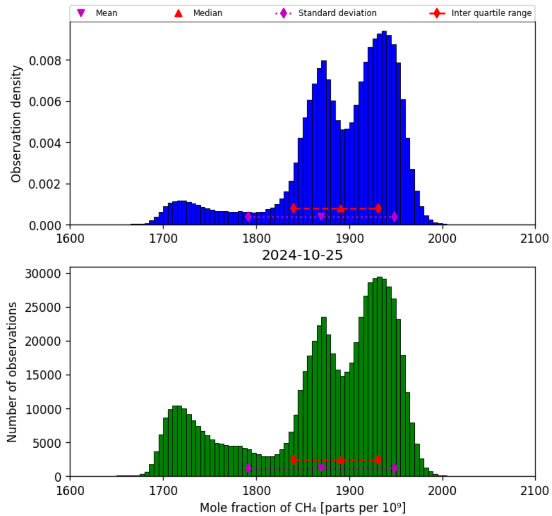
Figure 23: Histogram of “Mole fraction of CH 4 ” for 2024-10-24 to 2024-10-26
