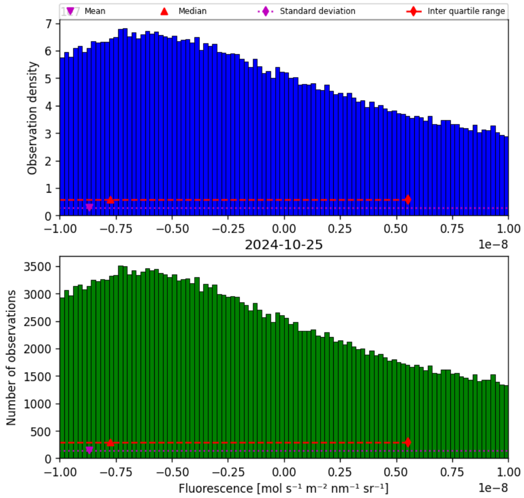
Figure 32: Histogram of “Fluorescence” for 2024-10-24 to 2024-10-26
