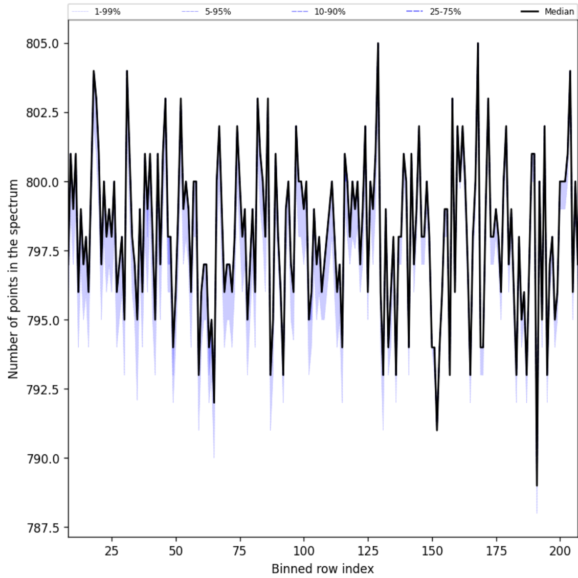
Figure 37: Along track statistics of “Number of points in the spectrum” for 2024-10-24 to 2024-10-26
