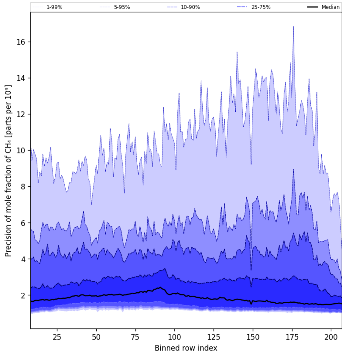
Figure 35: Along track statistics of “Precision of mole fraction of CH 4 ” for 2024-10-24 to 2024-10-26
