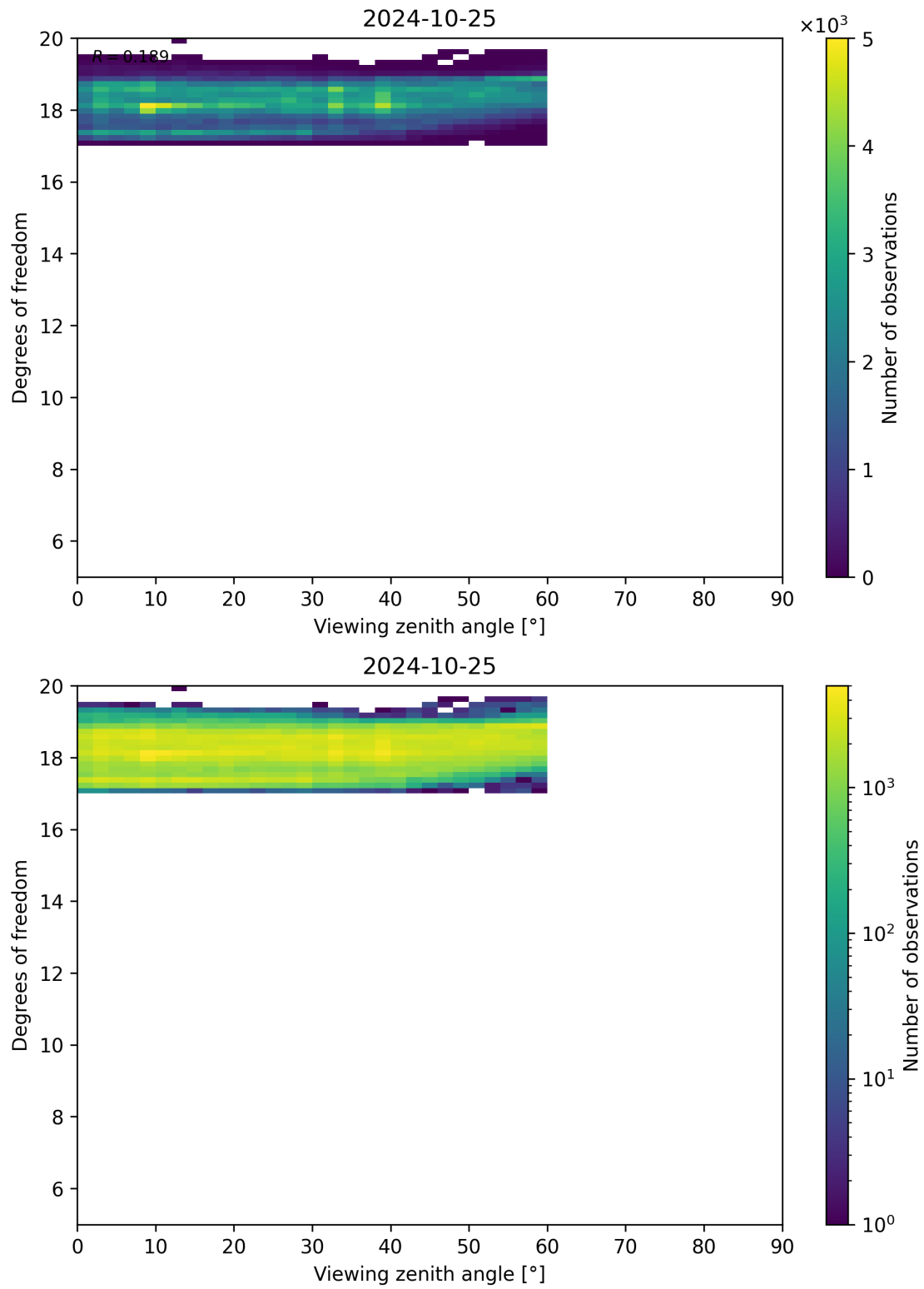
Figure 107: Scatter density plot of “Viewing zenith angle” against “Degrees of freedom” for 2024-10-24 to 2024-10-26.
