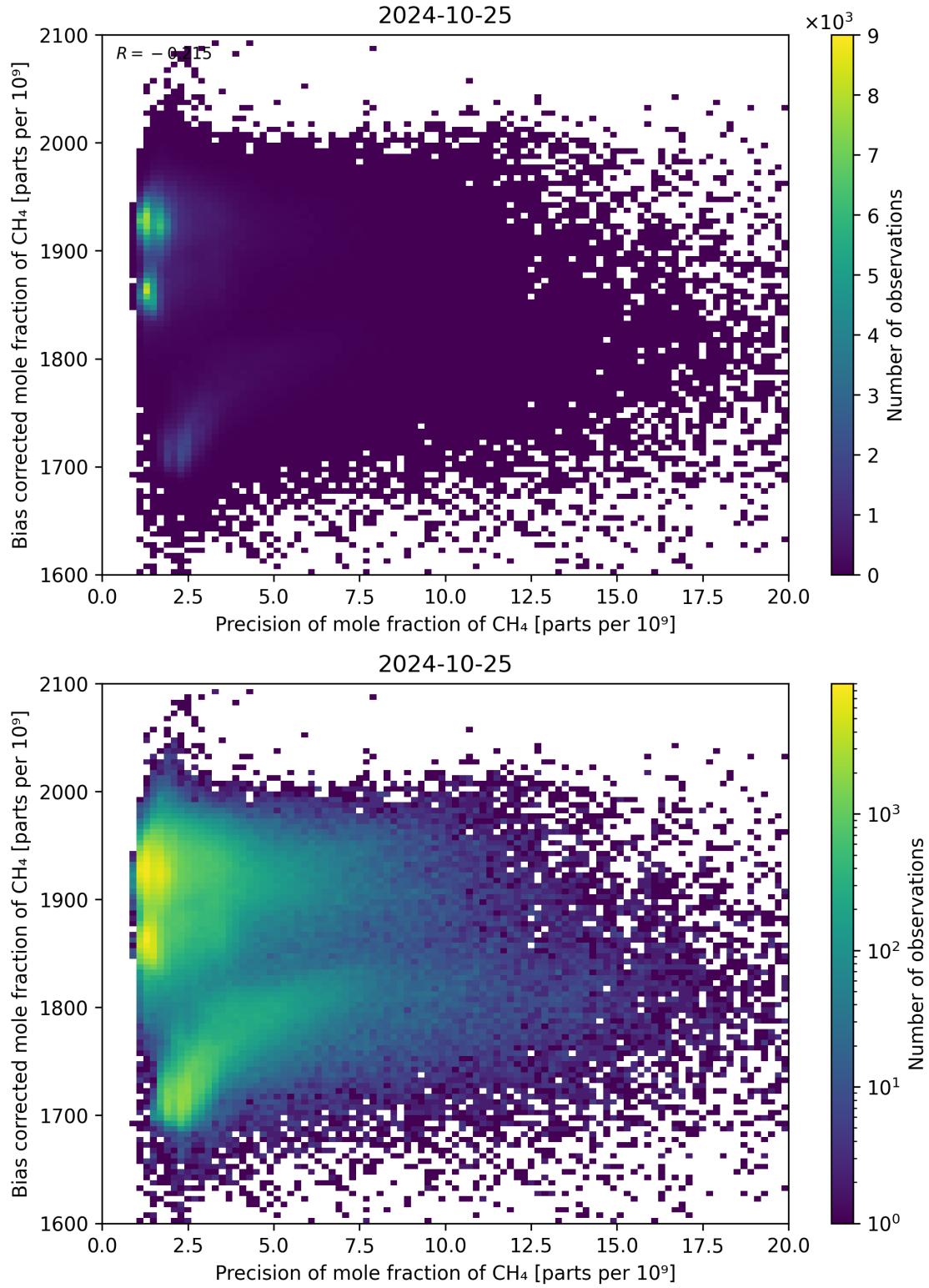
Figure 82: Scatter density plot of “Precision of mole fraction of CH 4 ” against “Bias corrected mole fraction of CH 4 ” for 2024-10-24 to 2024-10-26.
