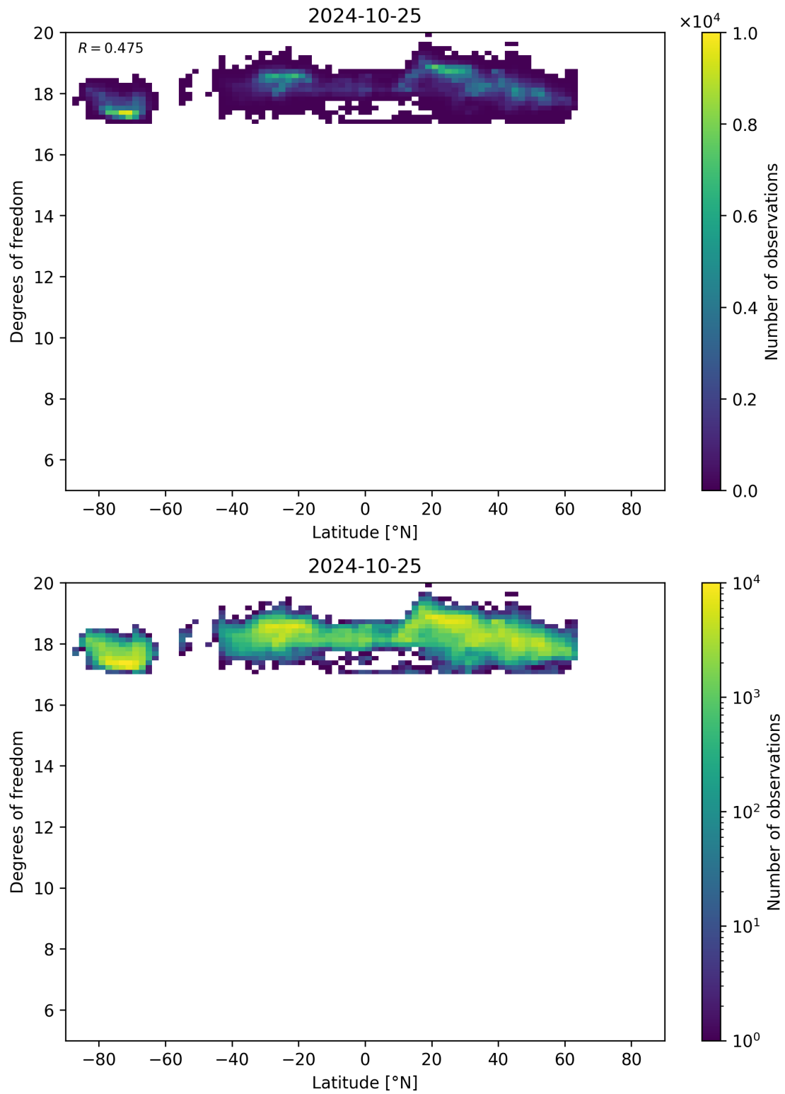
Figure 55: Scatter density plot of “Latitude” against “Degrees of freedom” for 2024-10-24 to 2024-10-26.
