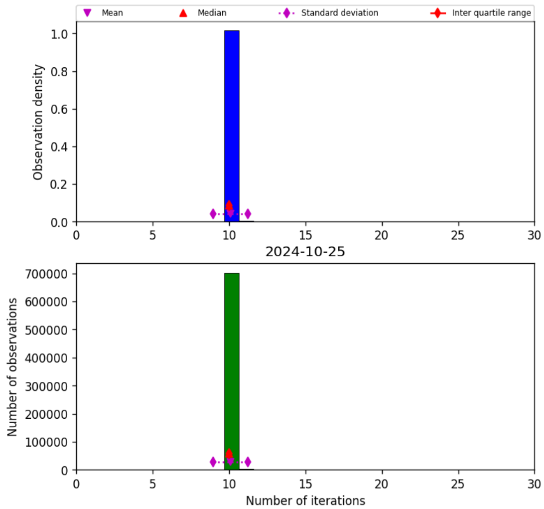
Figure 31: Histogram of “Number of iterations” for 2024-10-24 to 2024-10-26
