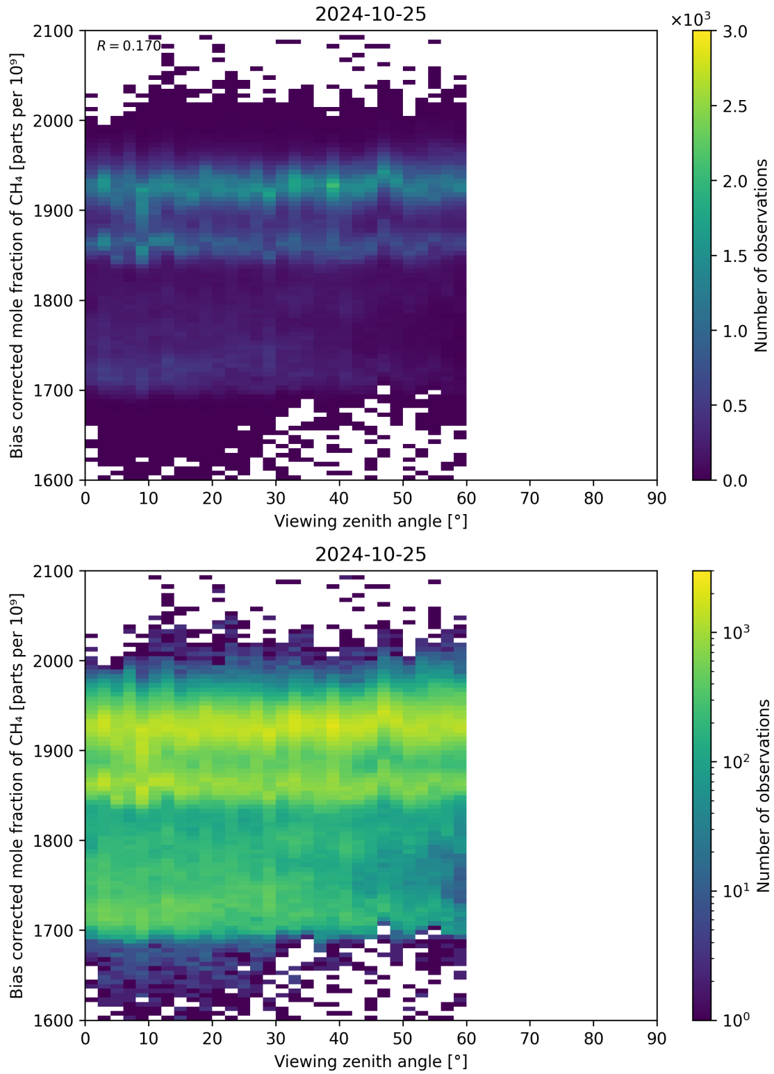
Figure 111: Scatter density plot of “Viewing zenith angle” against “Bias corrected mole fraction of CH 4 ” for 2024-10-24 to 2024-10-26.
