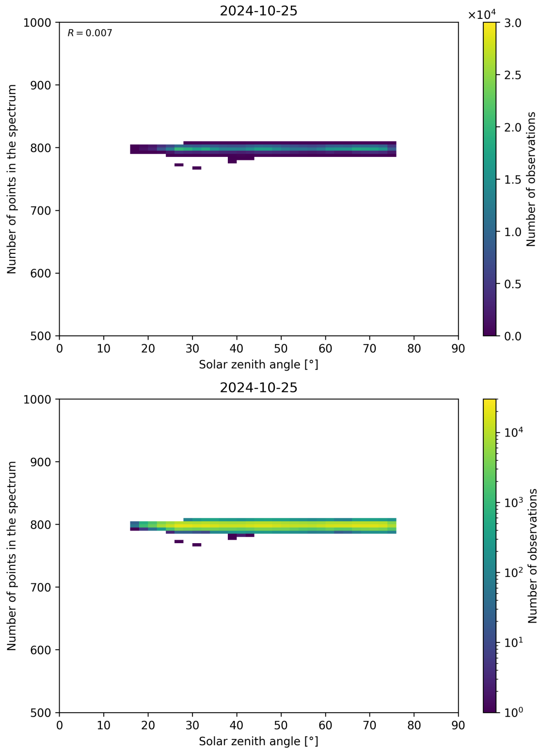
Figure 103: Scatter density plot of “Solar zenith angle” against “Number of points in the spectrum” for 2024-10-24 to 2024-10-26.
