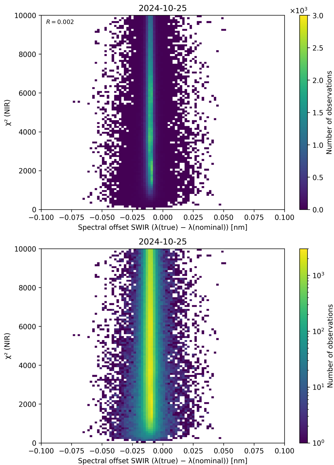
Figure 117: Scatter density plot of “Spectral offset SWIR ( \lambda_{\text{true}} - \lambda_{\text{nominal}} )” against “ \chi^2 (NIR)” for 2024-10-24 to 2024-10-26.
