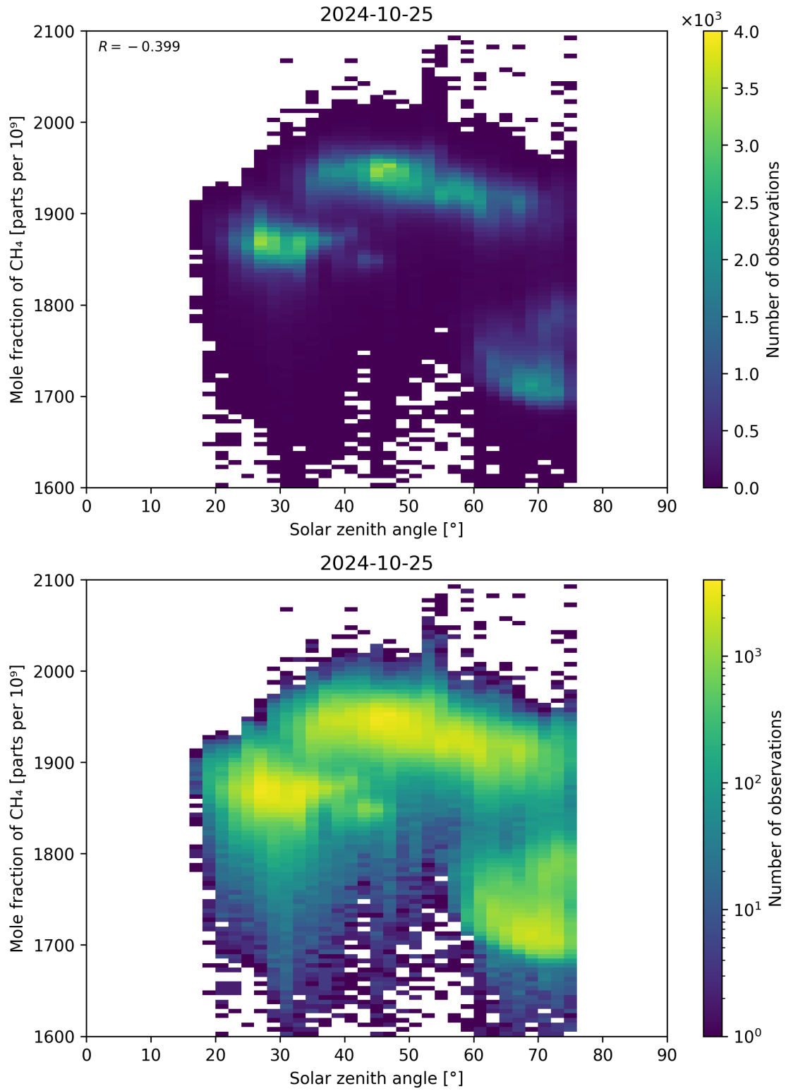
Figure 99: Scatter density plot of “Solar zenith angle” against “Mole fraction of \text{CH}_4 ” for 2024-10-24 to 2024-10-26.
