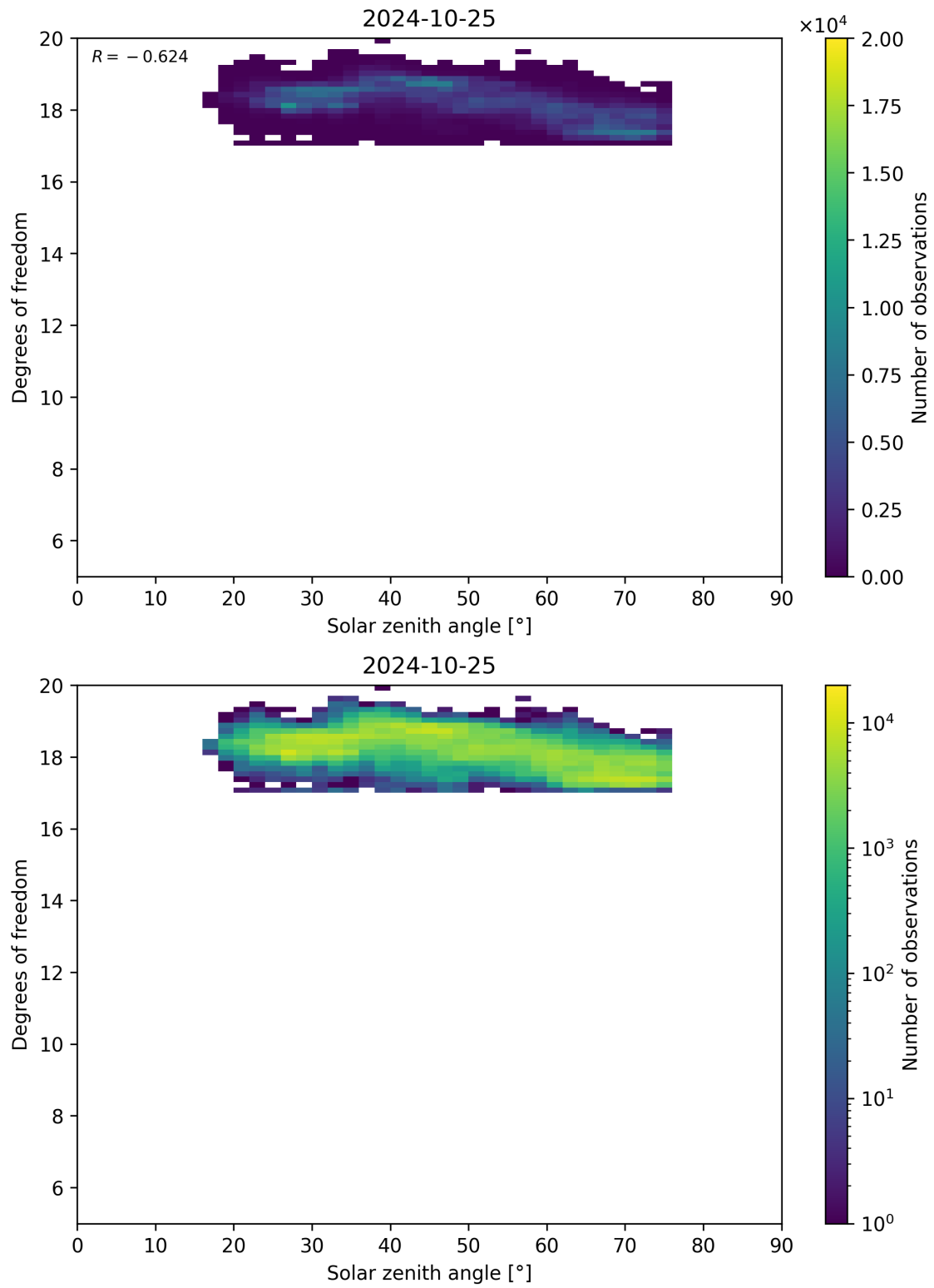
Figure 96: Scatter density plot of “Solar zenith angle” against “Degrees of freedom” for 2024-10-24 to 2024-10-26.
