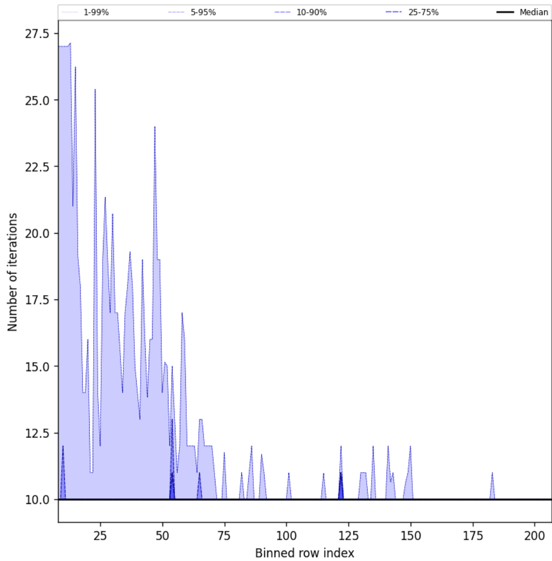
Figure 42: Along track statistics of “Number of iterations” for 2024-10-24 to 2024-10-26
