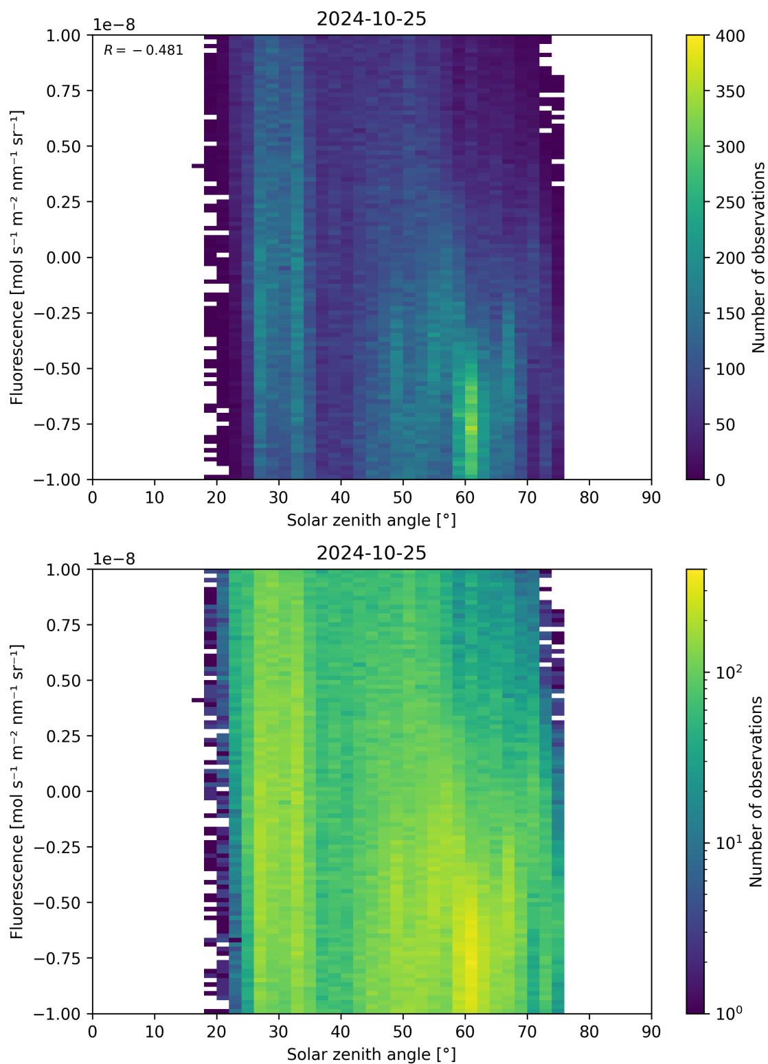
Figure 97: Scatter density plot of “Solar zenith angle” against “Fluorescence” for 2024-10-24 to 2024-10-26.
