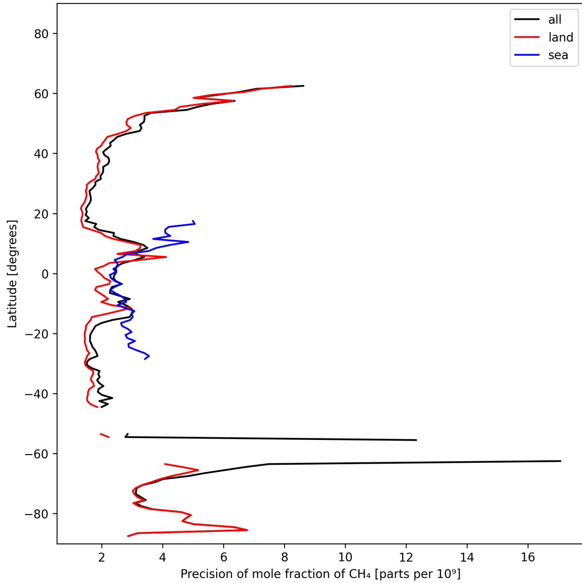
Figure 13: Zonal average of “Precision of mole fraction of CH 4 ” for 2024-10-24 to 2024-10-26.
