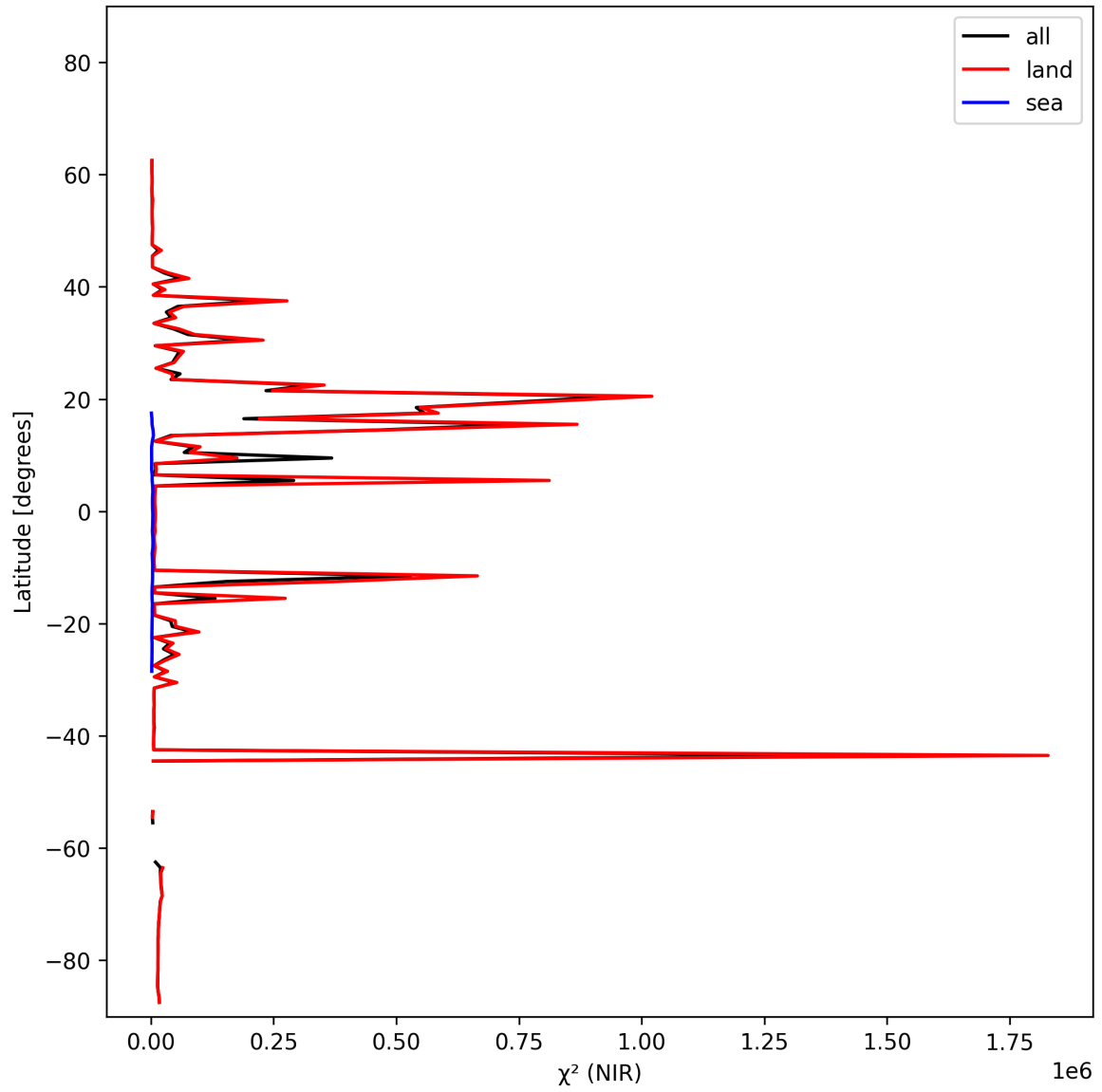
Figure 18: Zonal average of “ \chi^2 (NIR)” for 2024-10-24 to 2024-10-26.
