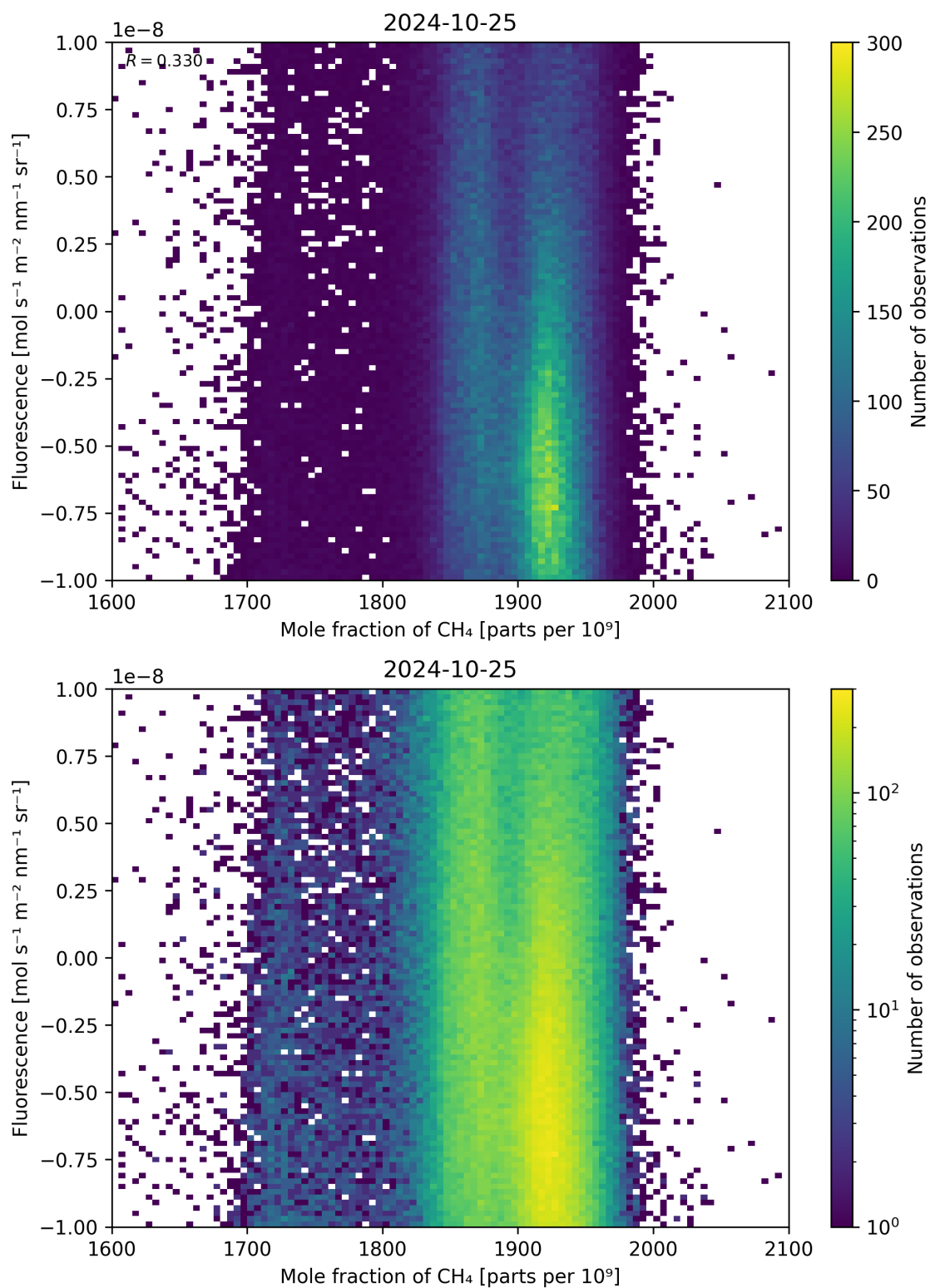
Figure 73: Scatter density plot of “Mole fraction of \text{CH}_4 ” against “Fluorescence” for 2024-10-24 to 2024-10-26.
