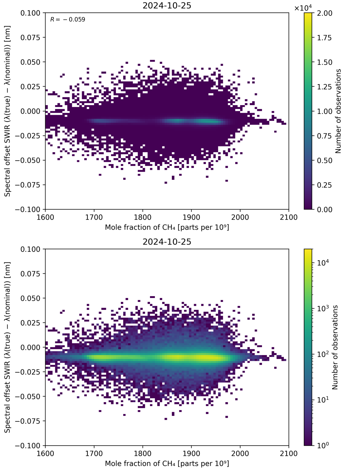
Figure 86: Scatter density plot of “Mole fraction of \text{CH}_4 ” against “Spectral offset SWIR ( \lambda_{\text{true}} - \lambda_{\text{nominal}} )” for 2024-10-24 to 2024-10-26.
