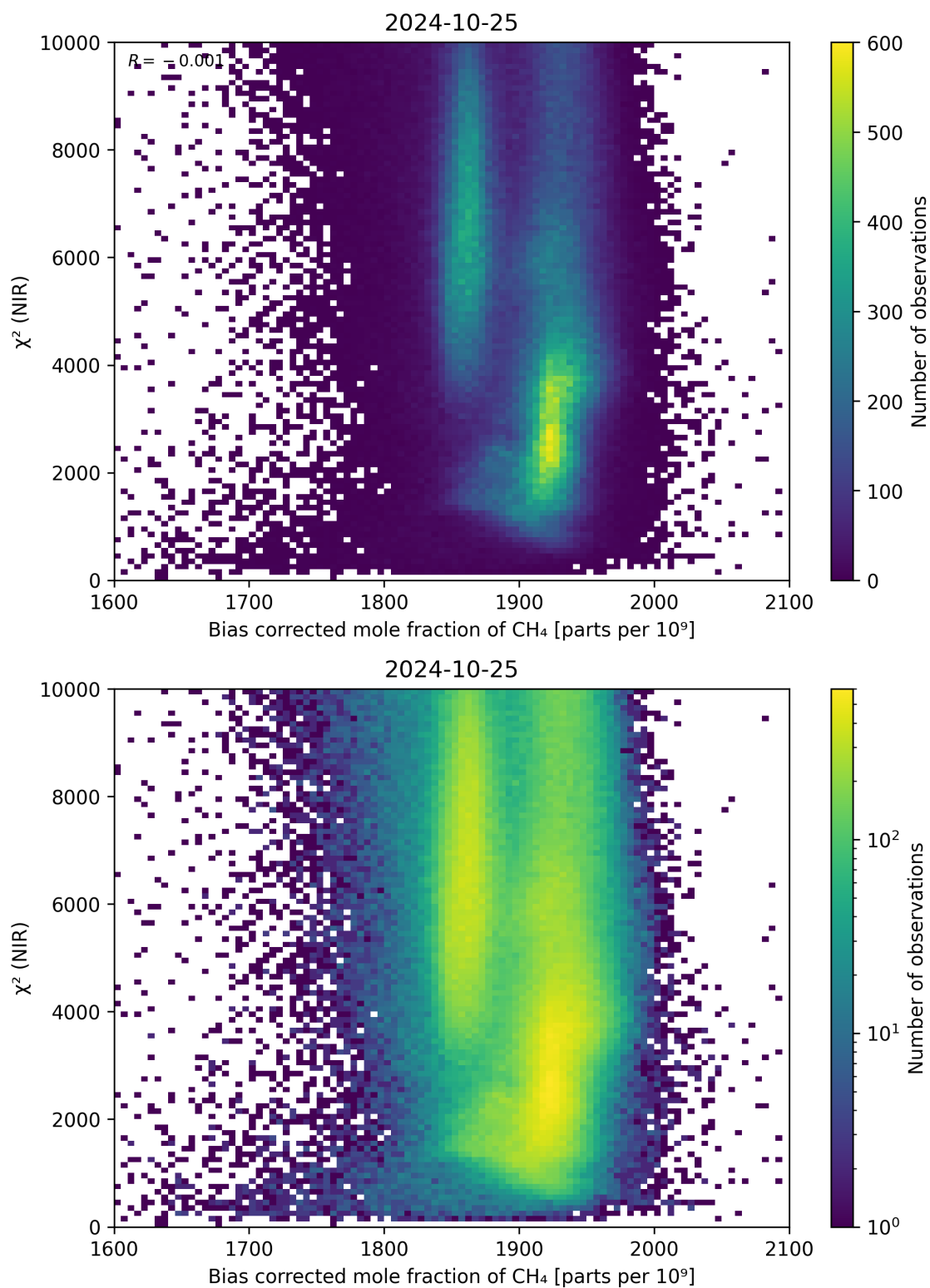
Figure 63: Scatter density plot of “Bias corrected mole fraction of CH 4 ” against “ \chi^2 (NIR)” for 2024-10-24 to 2024-10-26.
