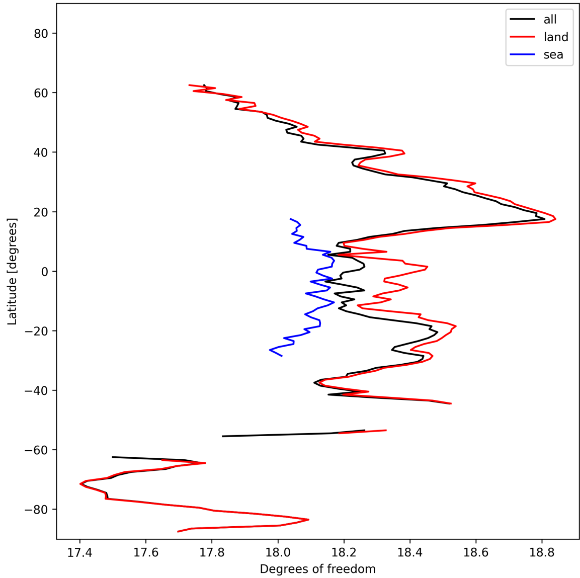
Figure 19: Zonal average of “Degrees of freedom” for 2024-10-24 to 2024-10-26.
