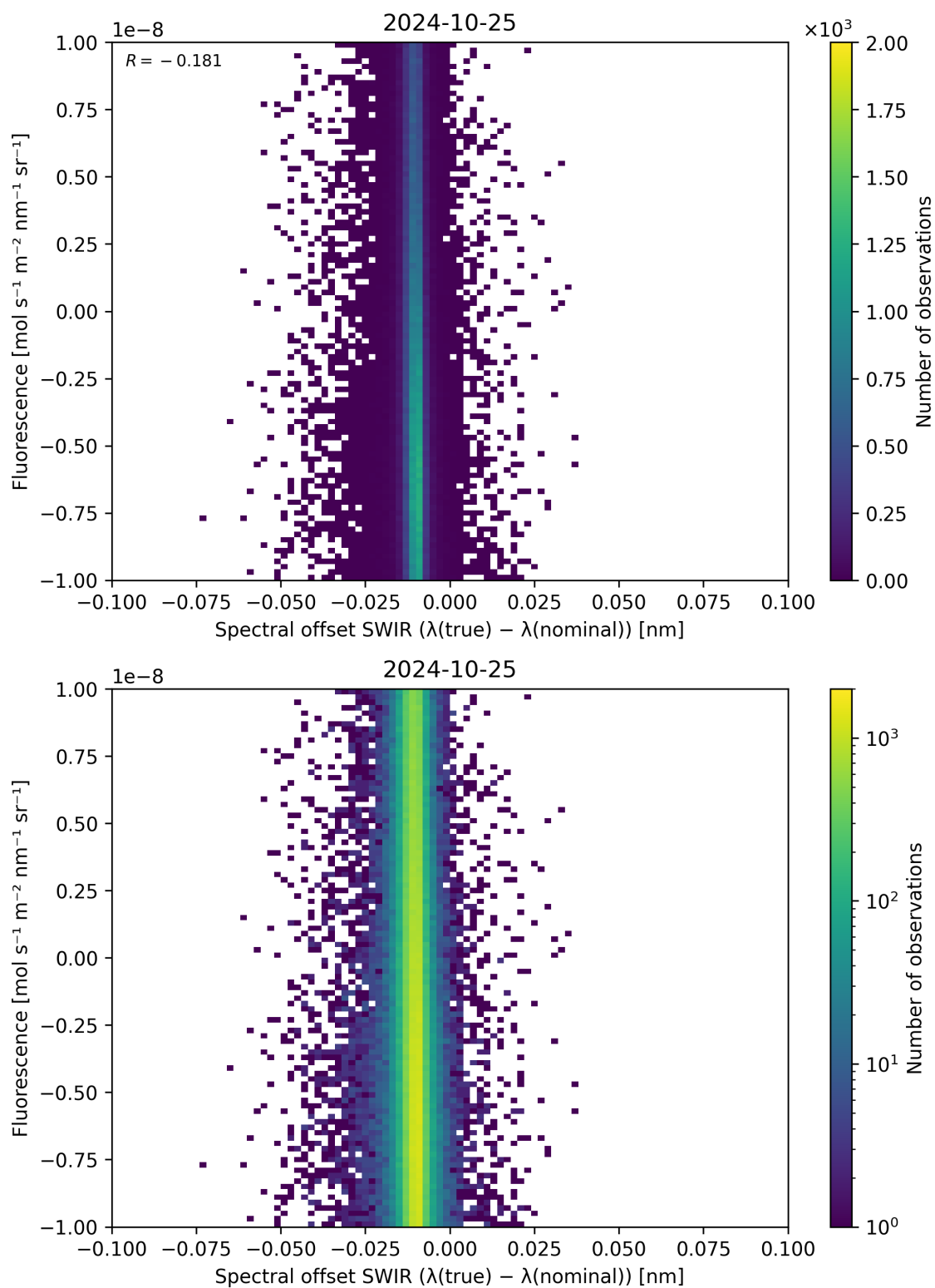
Figure 120: Scatter density plot of “Spectral offset SWIR ( \lambda_{\text{true}} - \lambda_{\text{nominal}} )” against “Fluorescence” for 2024-10-24 to 2024-10-26.
