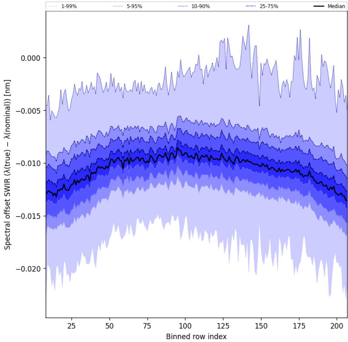
Figure 38: Along track statistics of “Spectral offset SWIR ( \lambda_{\text{true}} - \lambda_{\text{nominal}} )” for 2024-10-24 to 2024-10-26
