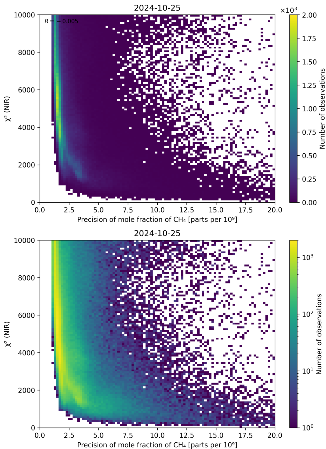
Figure 78: Scatter density plot of “Precision of mole fraction of CH 4 ” against “ \chi^2 (NIR)” for 2024-10-24 to 2024-10-26.
