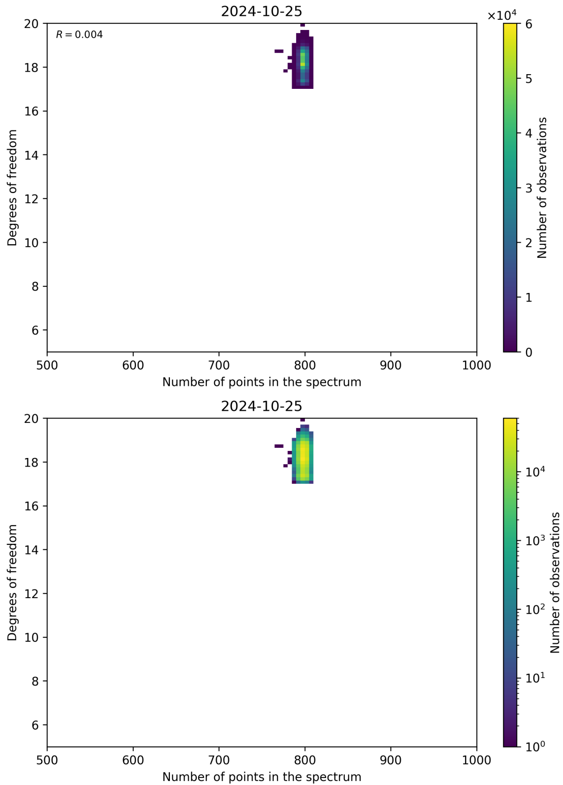
Figure 90: Scatter density plot of “Number of points in the spectrum” against “Degrees of freedom” for 2024-10-24 to 2024-10-26.
