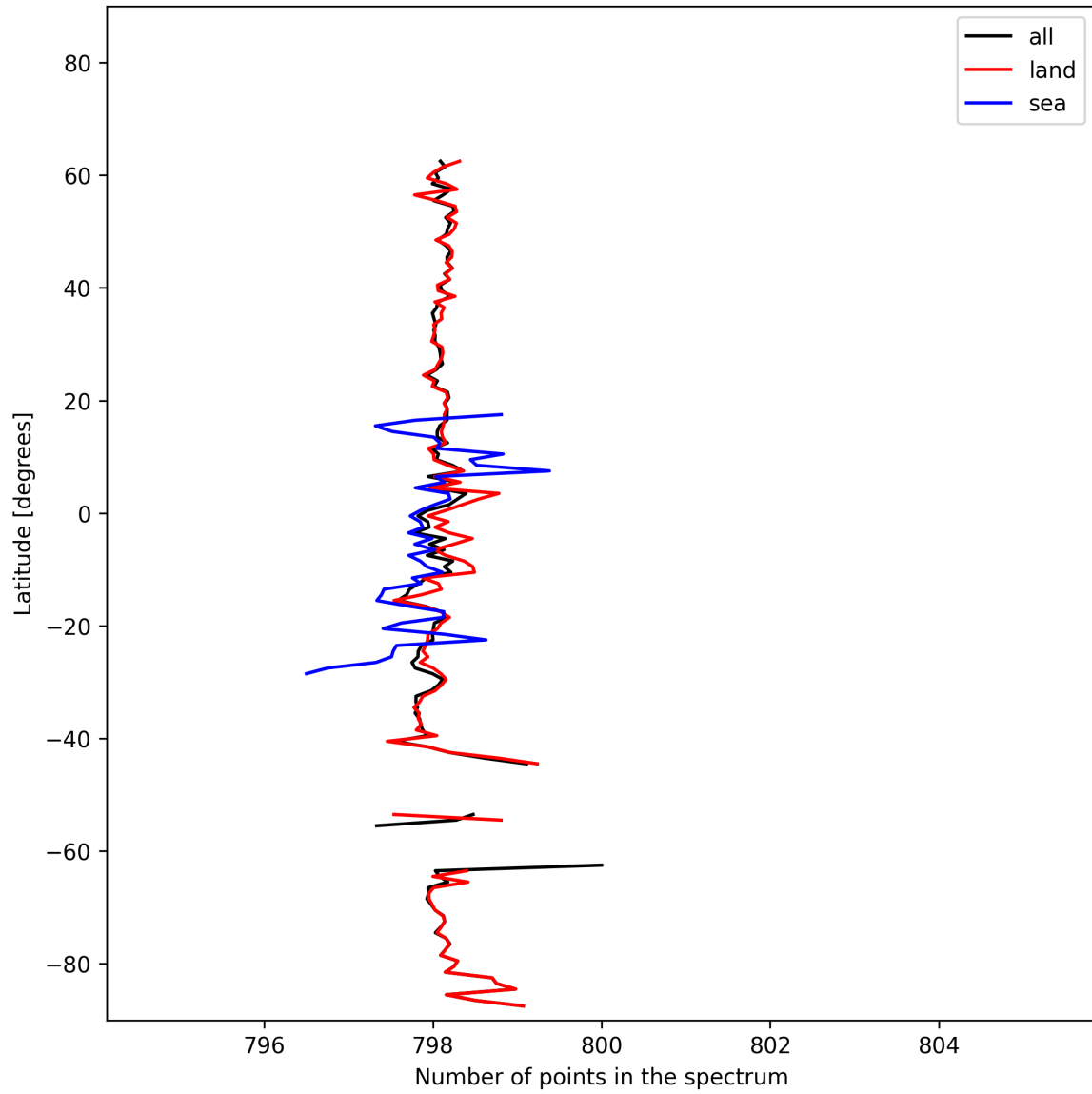
Figure 15: Zonal average of “Number of points in the spectrum” for 2024-10-24 to 2024-10-26.
