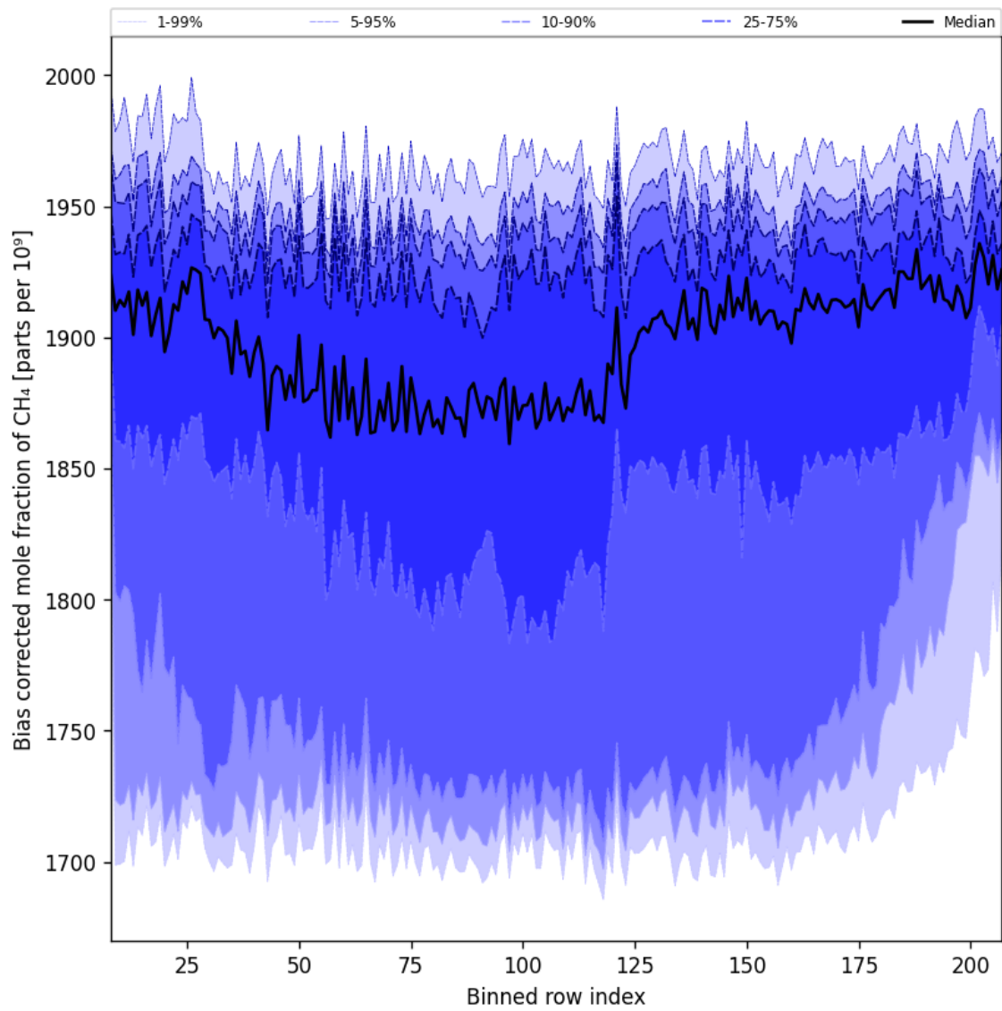
Figure 36: Along track statistics of “Bias corrected mole fraction of CH 4 ” for 2024-10-24 to 2024-10-26
