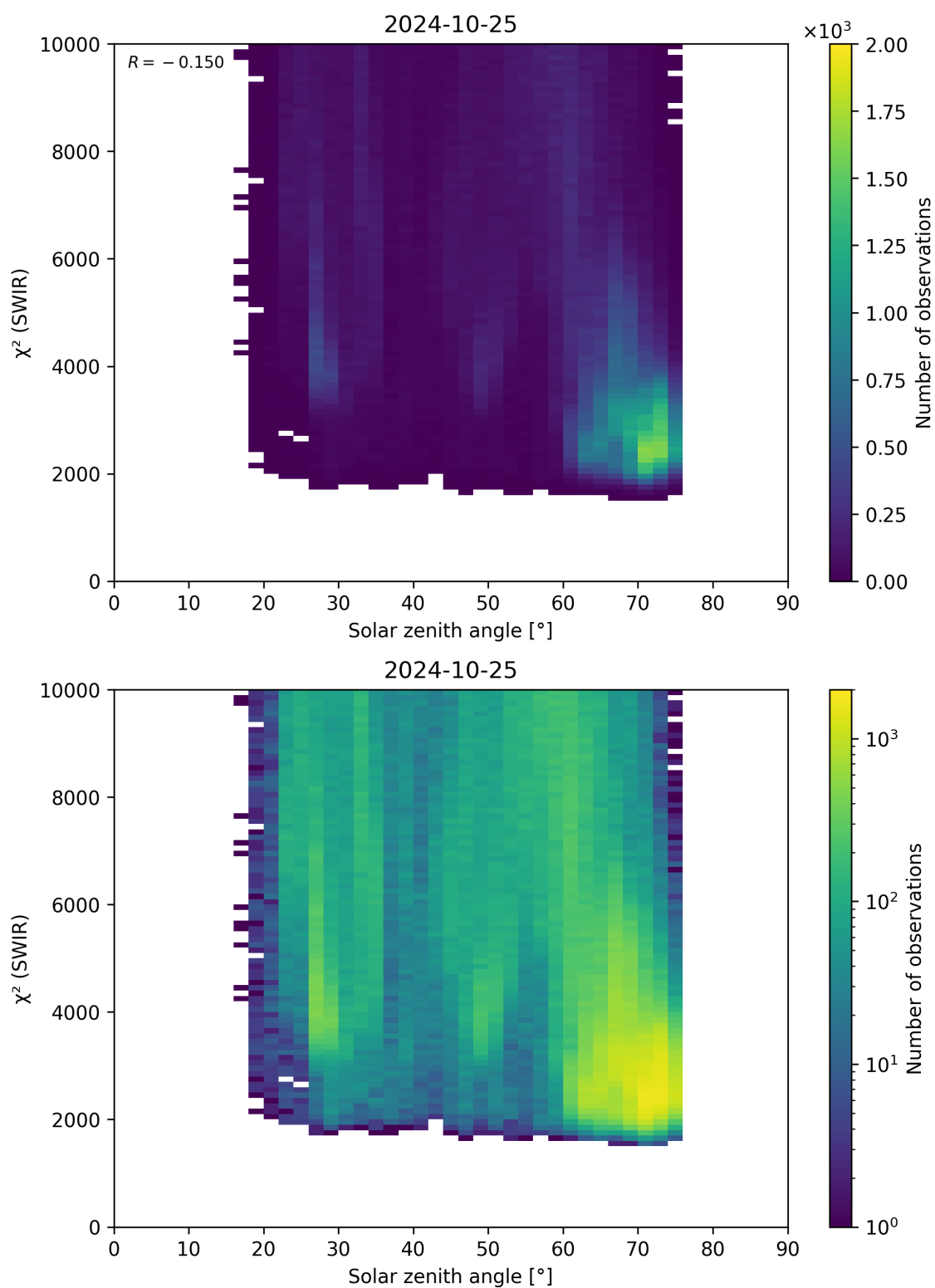
Figure 95: Scatter density plot of “Solar zenith angle” against “ \chi^2 (SWIR)” for 2024-10-24 to 2024-10-26.
