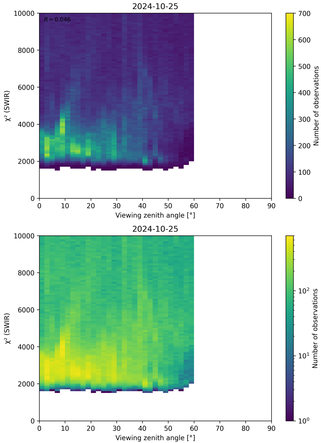
Figure 106: Scatter density plot of “Viewing zenith angle” against “ \chi^2 (SWIR)” for 2024-10-24 to 2024-10-26.
