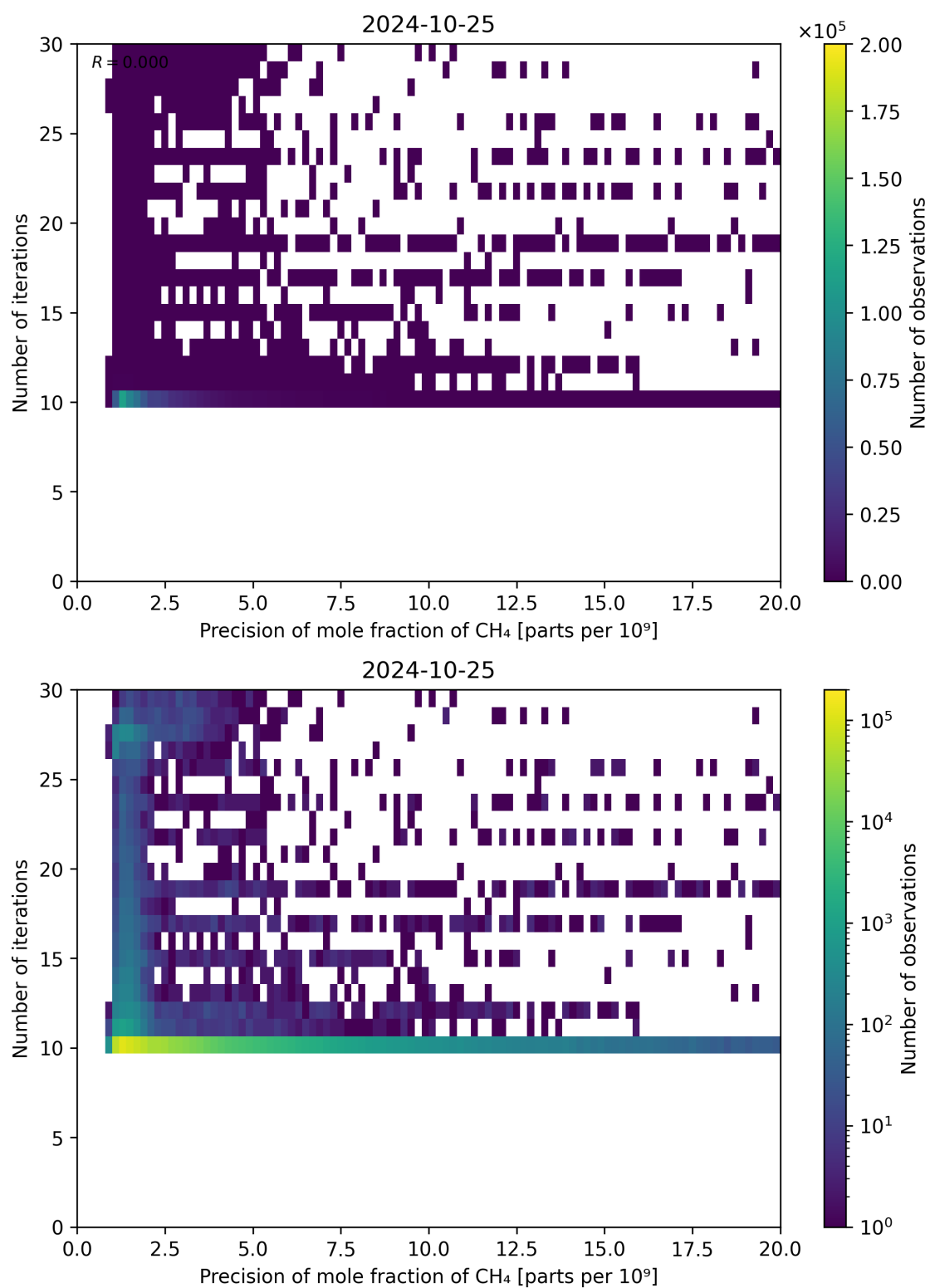
Figure 83: Scatter density plot of “Precision of mole fraction of CH 4 ” against “Number of iterations” for 2024-10-24 to 2024-10-26.
