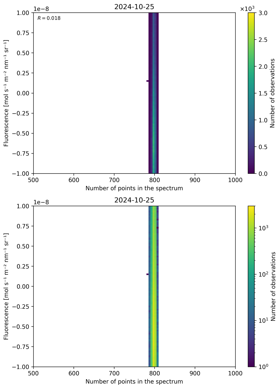
Figure 91: Scatter density plot of “Number of points in the spectrum” against “Fluorescence” for 2024-10-24 to 2024-10-26.
