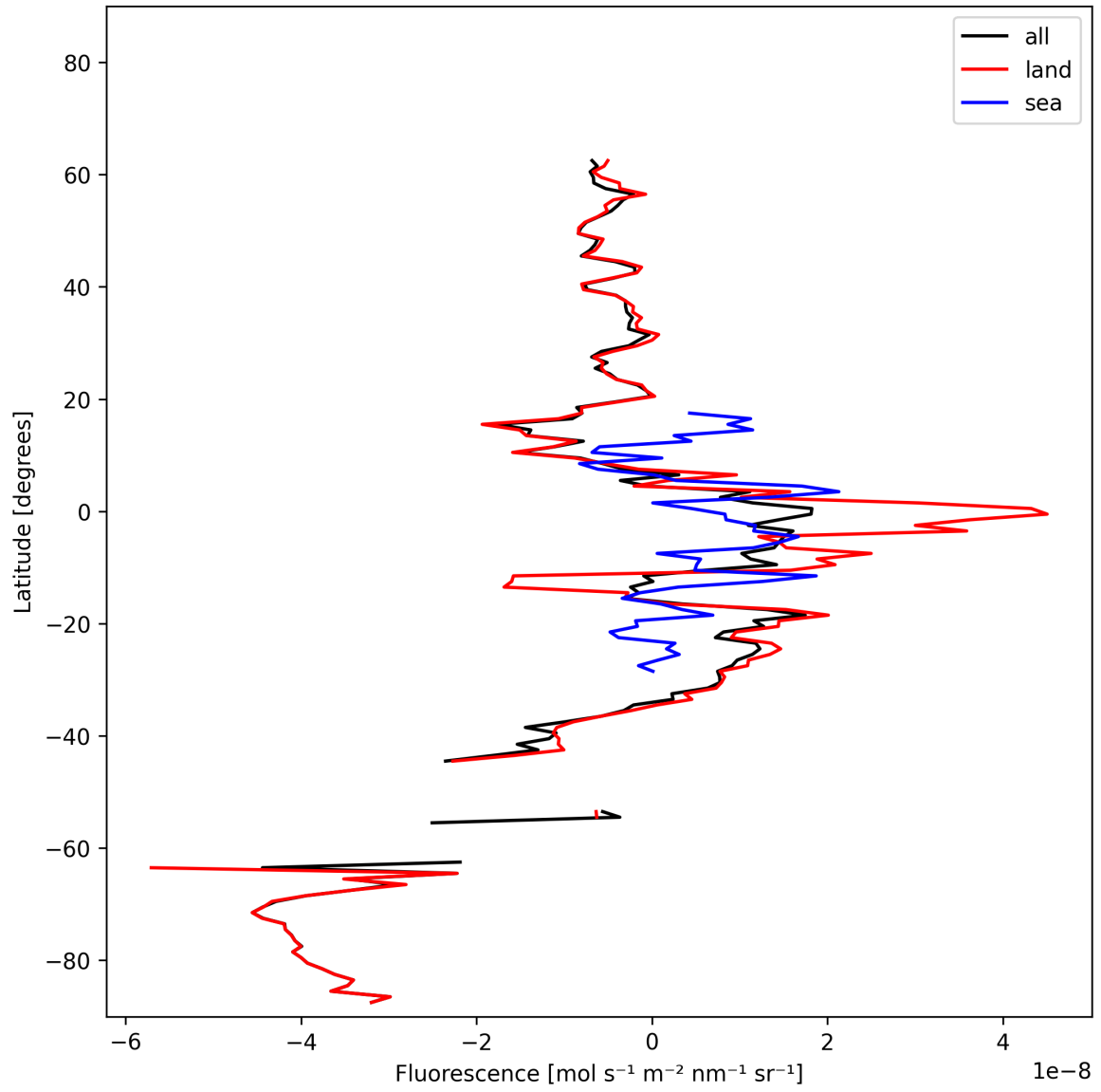
Figure 21: Zonal average of “Fluorescence” for 2024-10-24 to 2024-10-26.
