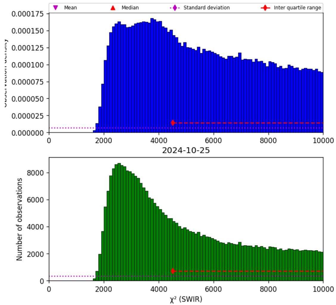
Figure 28: Histogram of “ \chi^2 (SWIR)” for 2024-10-24 to 2024-10-26
