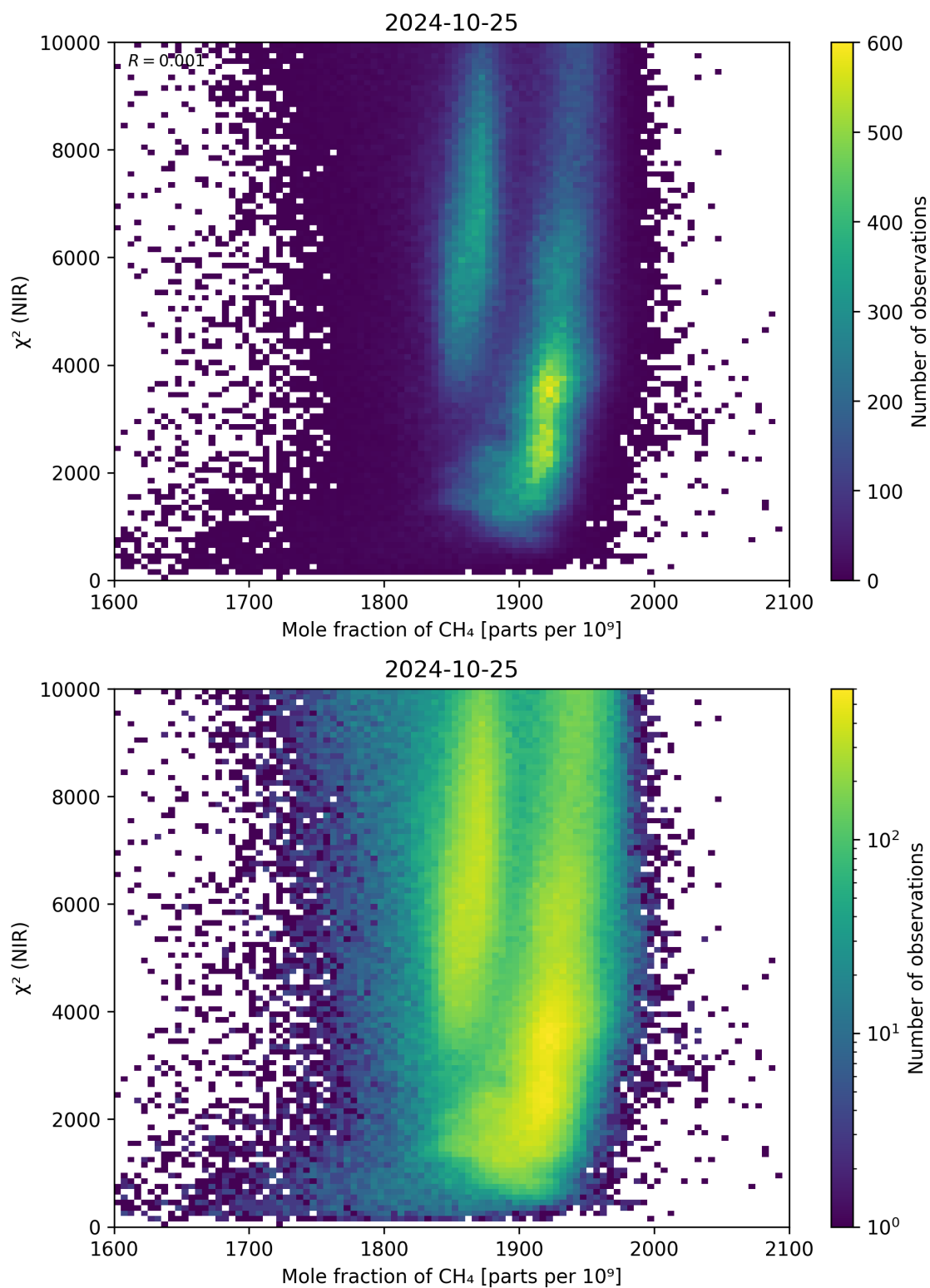
Figure 70: Scatter density plot of “Mole fraction of \text{CH}_4 ” against “ \chi^2 (NIR)” for 2024-10-24 to 2024-10-26.
