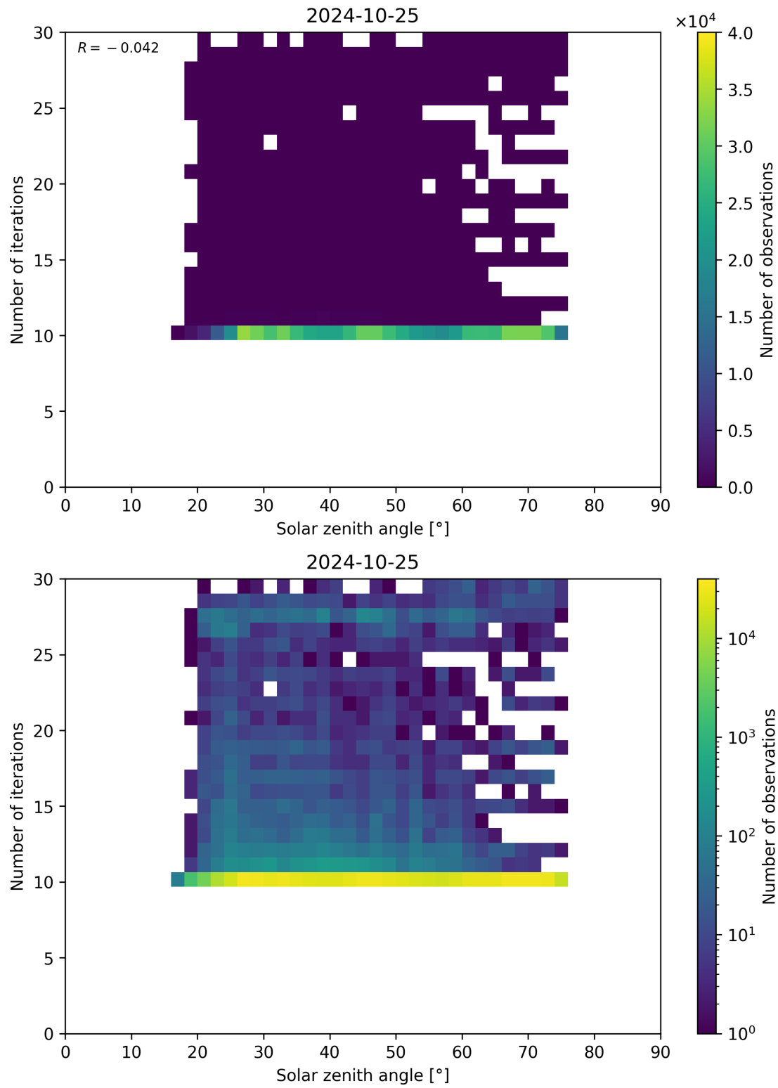
Figure 102: Scatter density plot of “Solar zenith angle” against “Number of iterations” for 2024-10-24 to 2024-10-26.
