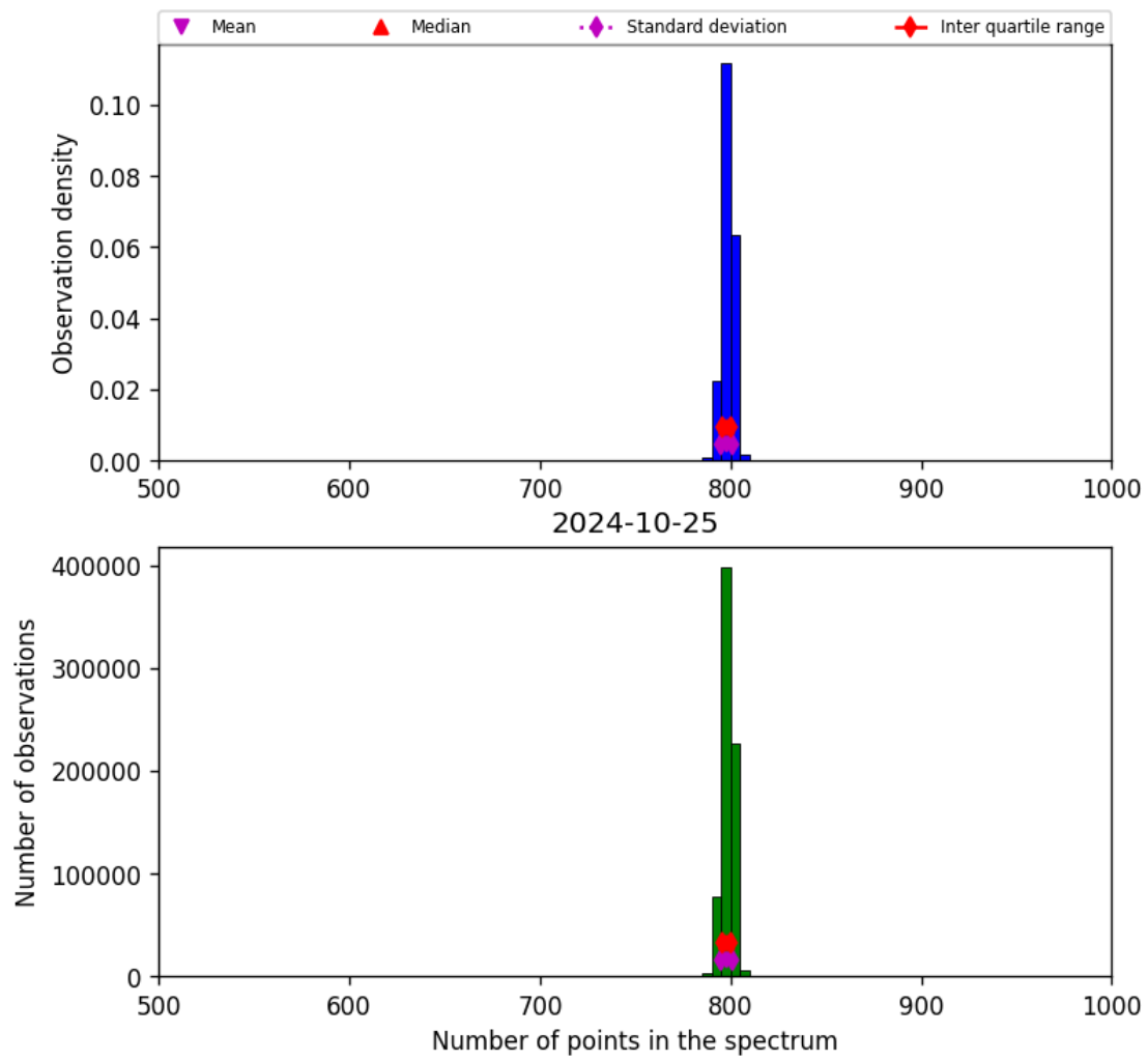
Figure 26: Histogram of “Number of points in the spectrum” for 2024-10-24 to 2024-10-26
