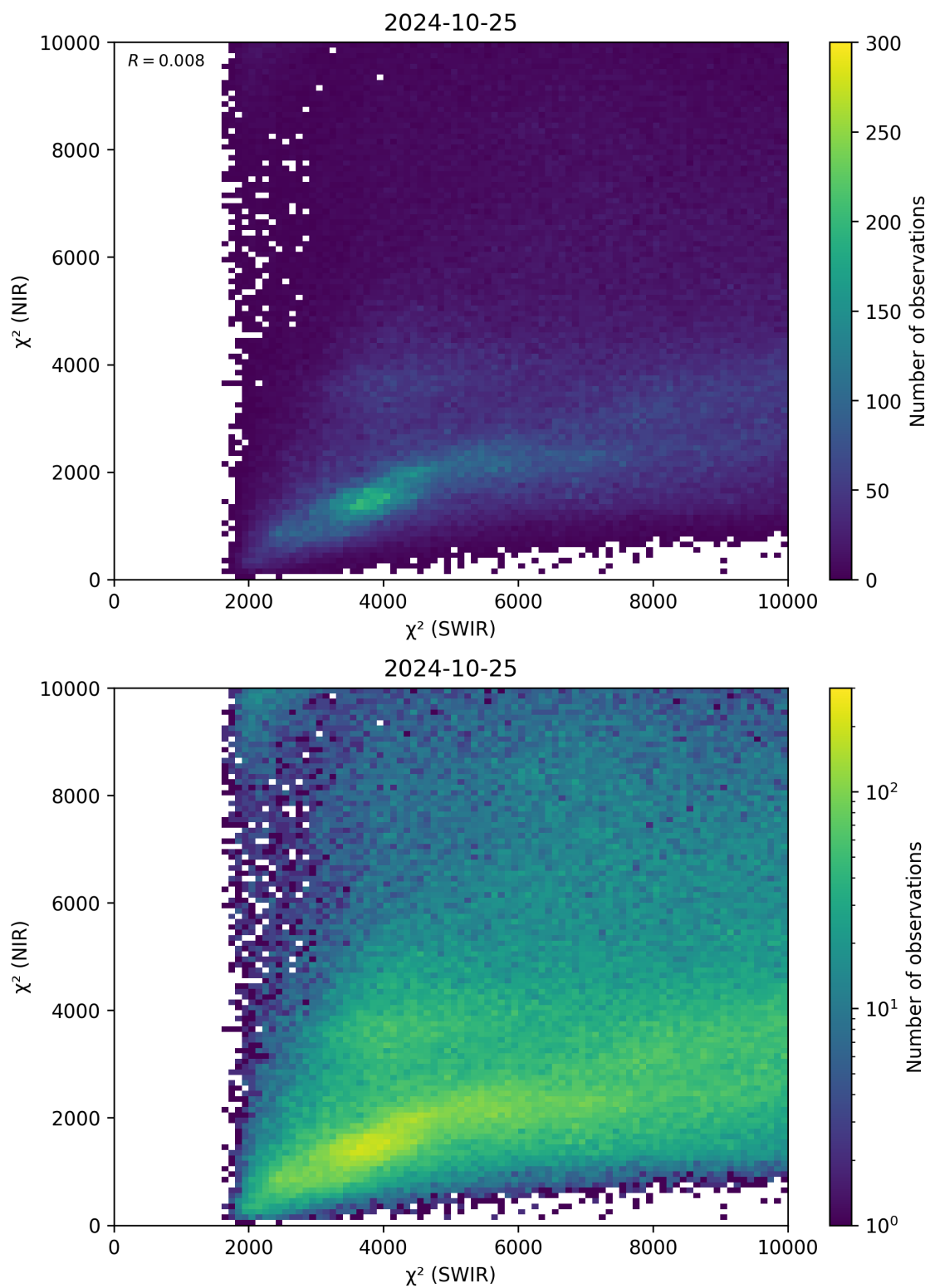
Figure 47: Scatter density plot of “ \chi^2 (SWIR)” against “ \chi^2 (NIR)” for 2024-10-24 to 2024-10-26.
