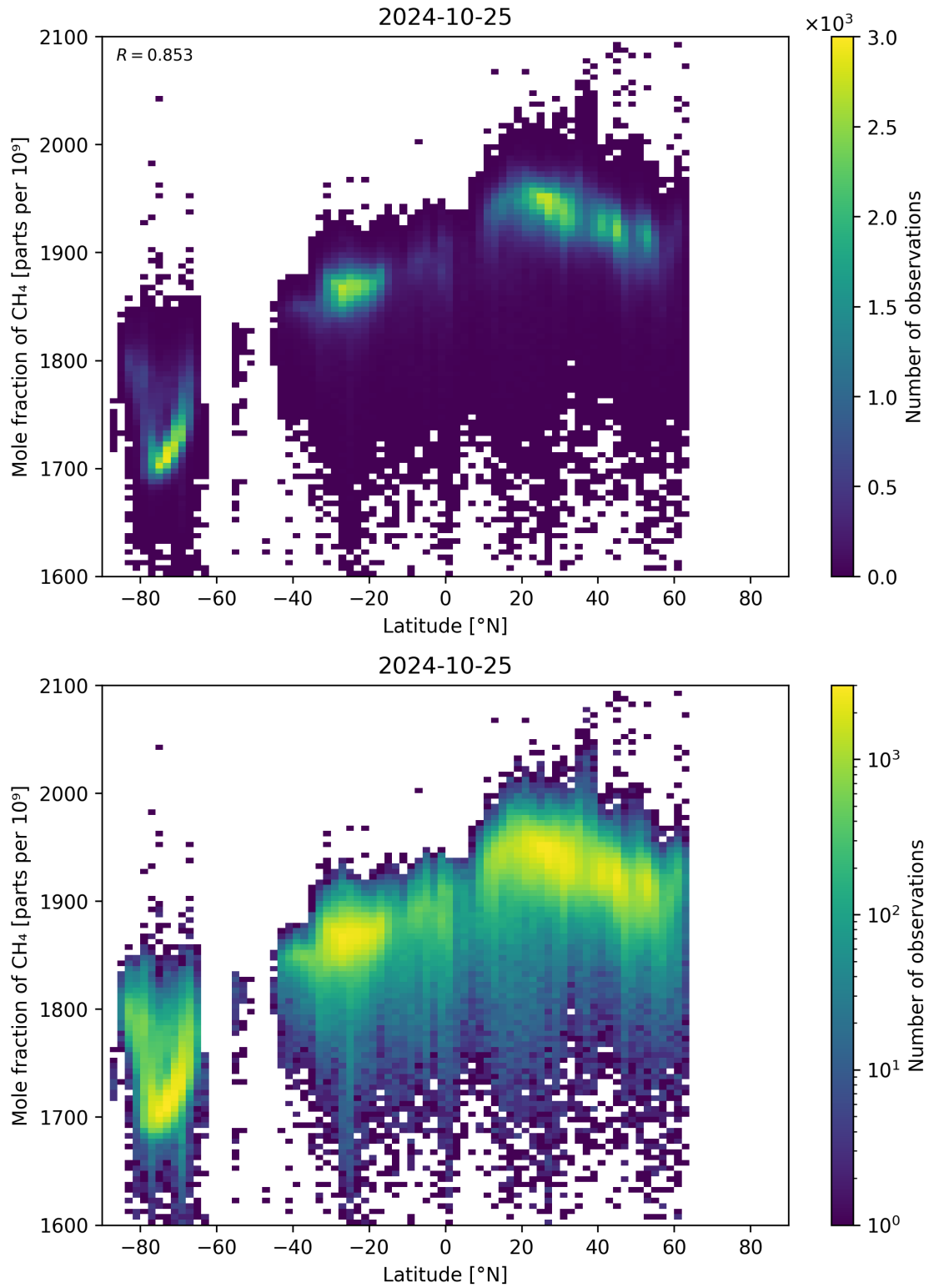
Figure 57: Scatter density plot of “Latitude” against “Mole fraction of CH 4 ” for 2024-10-24 to 2024-10-26.
