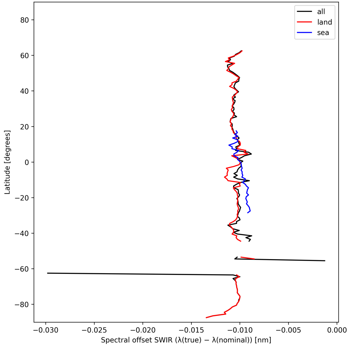
Figure 16: Zonal average of “Spectral offset SWIR ( \lambda_{\text{true}} - \lambda_{\text{nominal}} )” for 2024-10-24 to 2024-10-26.
