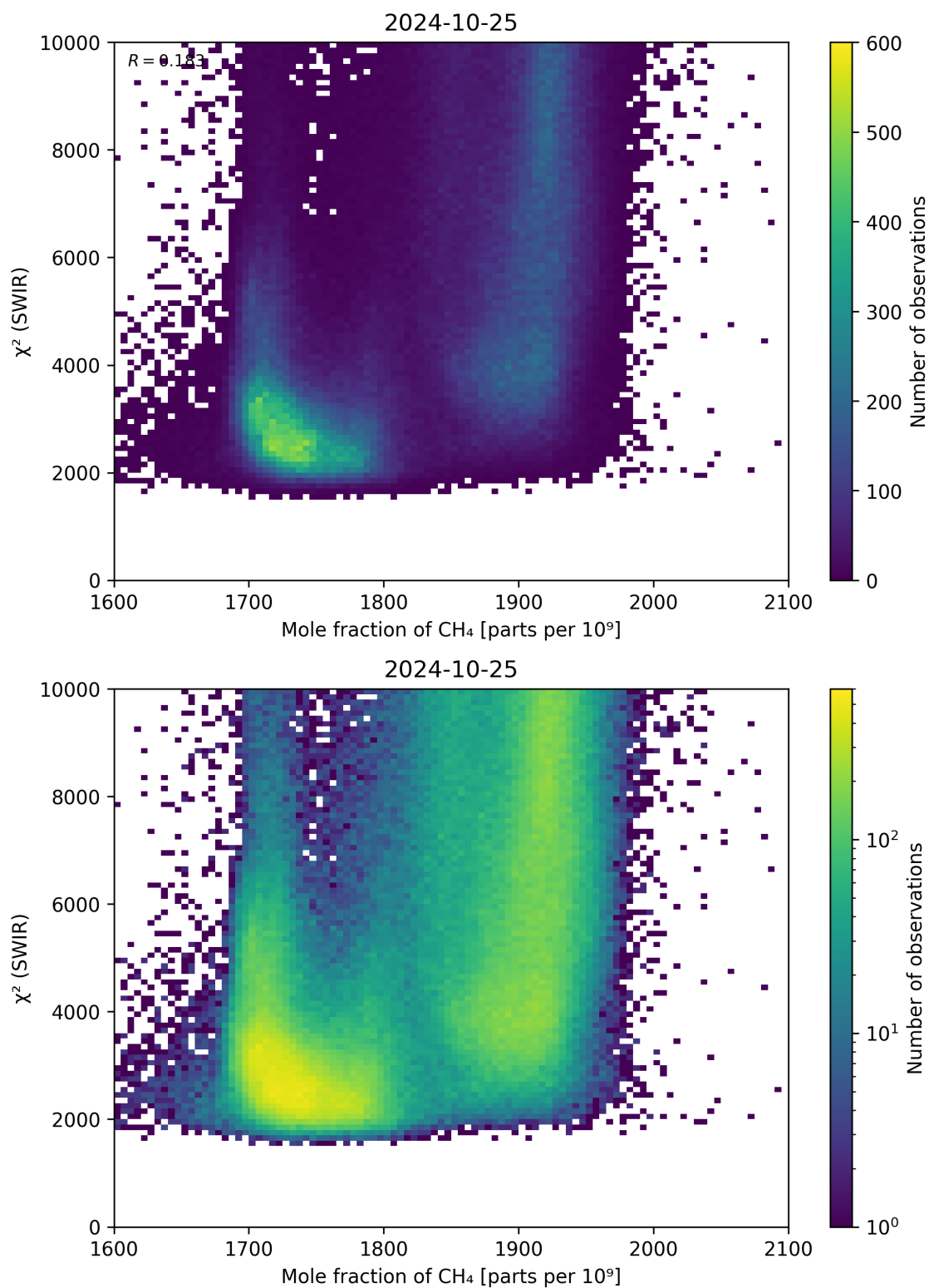
Figure 71: Scatter density plot of “Mole fraction of \text{CH}_4 ” against “ \chi^2 (SWIR)” for 2024-10-24 to 2024-10-26.
