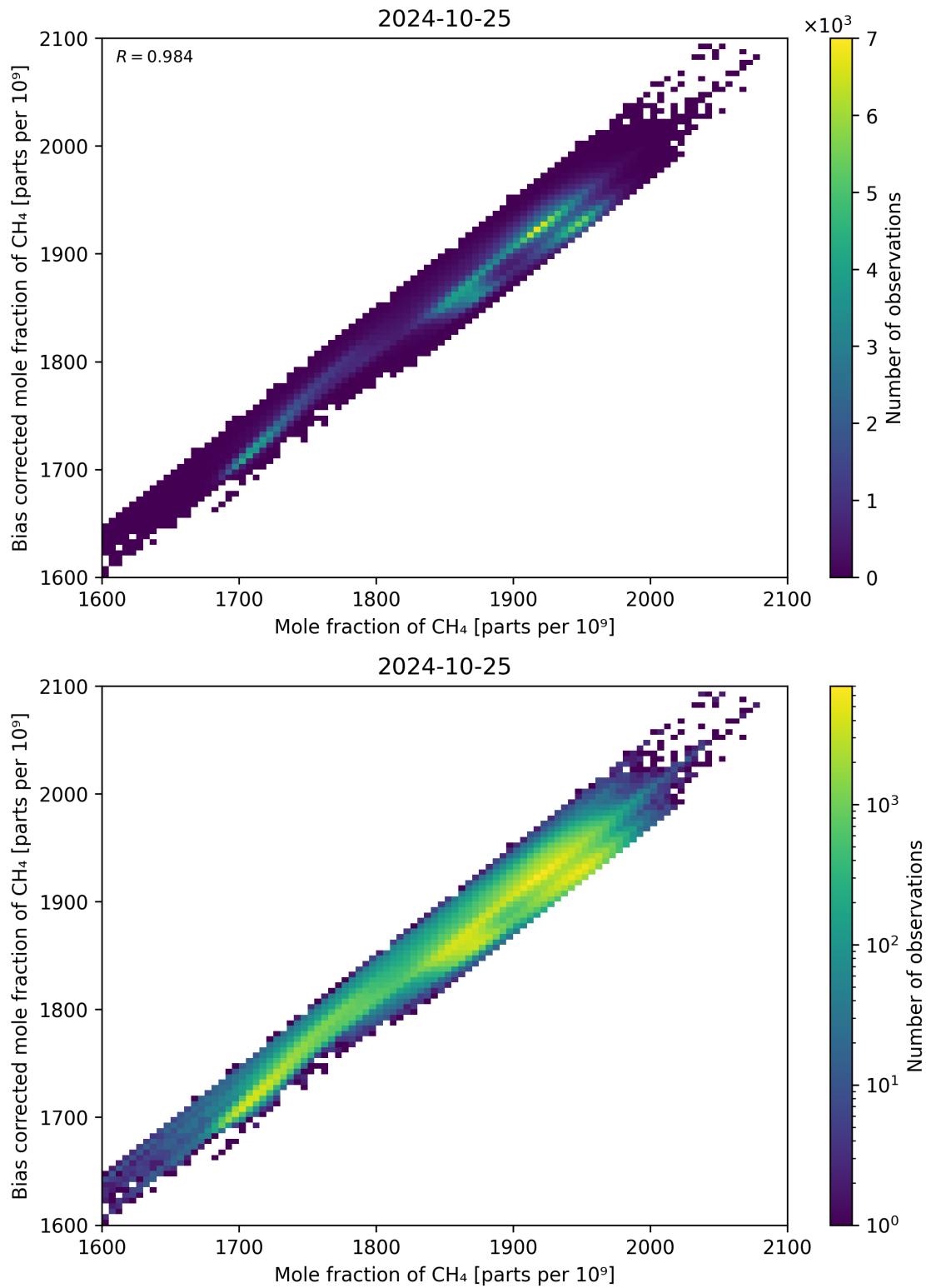
Figure 74: Scatter density plot of “Mole fraction of CH 4 ” against “Bias corrected mole fraction of CH 4 ” for 2024-10-24 to 2024-10-26.
