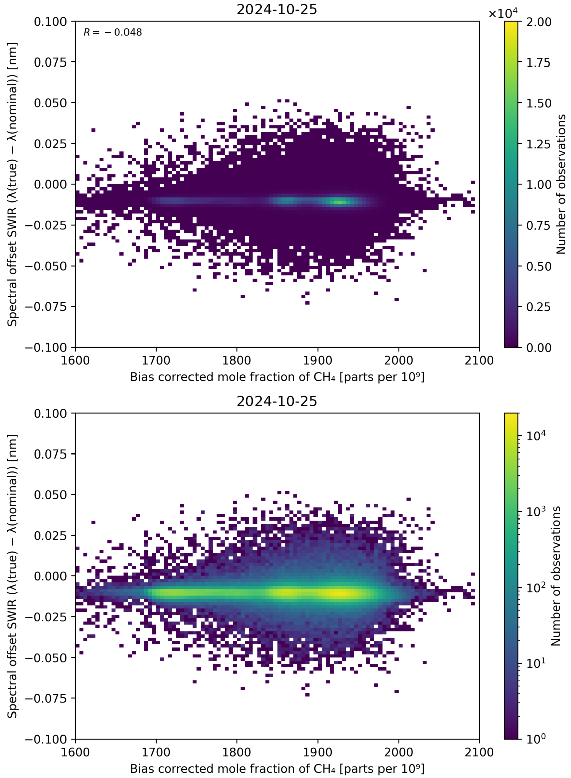
Figure 69: Scatter density plot of “Bias corrected mole fraction of \text{CH}_4 ” against “Spectral offset SWIR ( \lambda_{\text{true}} - \lambda_{\text{nominal}} )” for 2024-10-24 to 2024-10-26.
