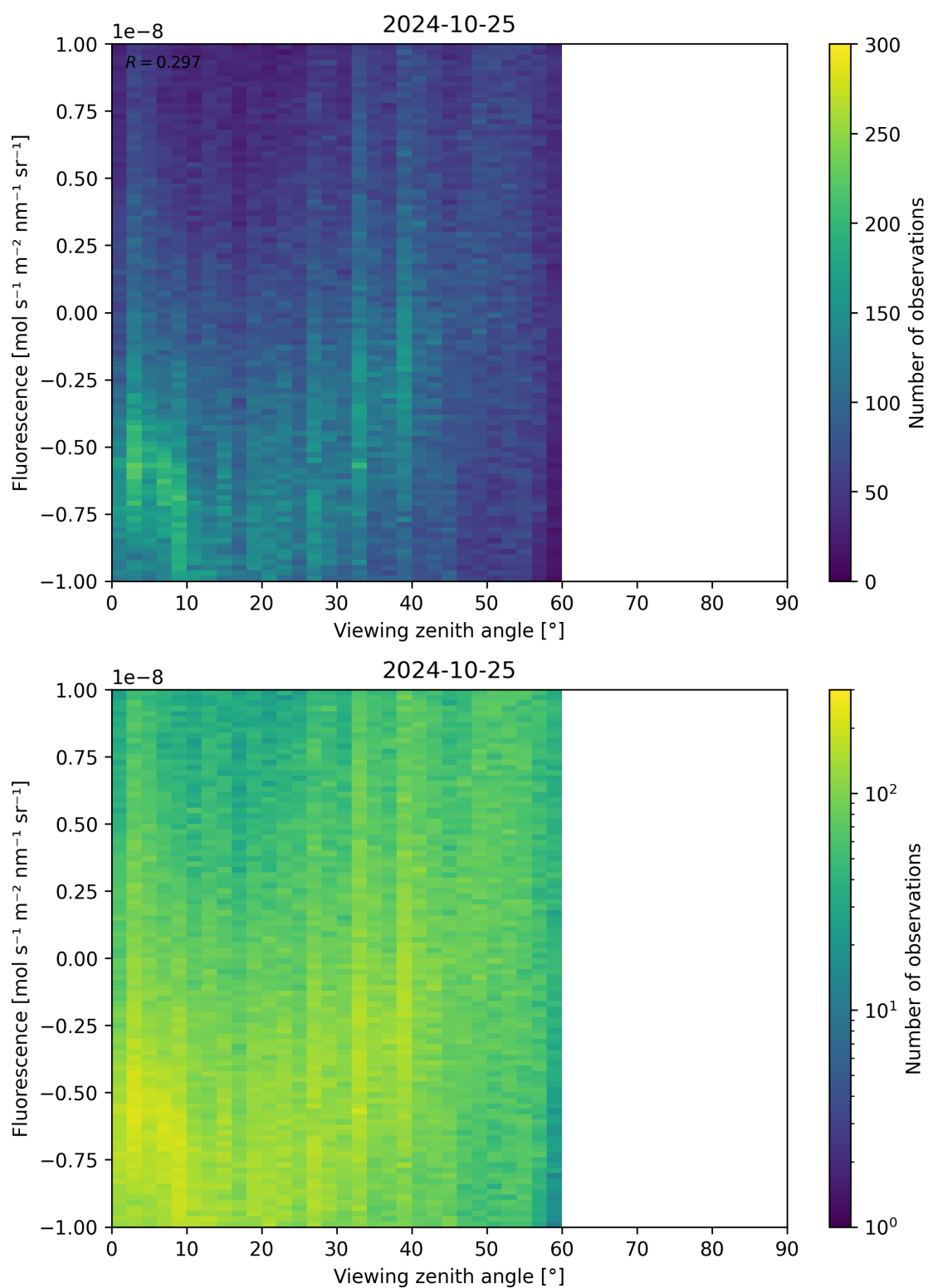
Figure 108: Scatter density plot of “Viewing zenith angle” against “Fluorescence” for 2024-10-24 to 2024-10-26.
