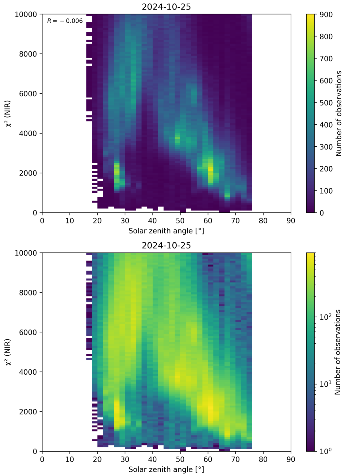
Figure 94: Scatter density plot of “Solar zenith angle” against “ \chi^2 (NIR)” for 2024-10-24 to 2024-10-26.
