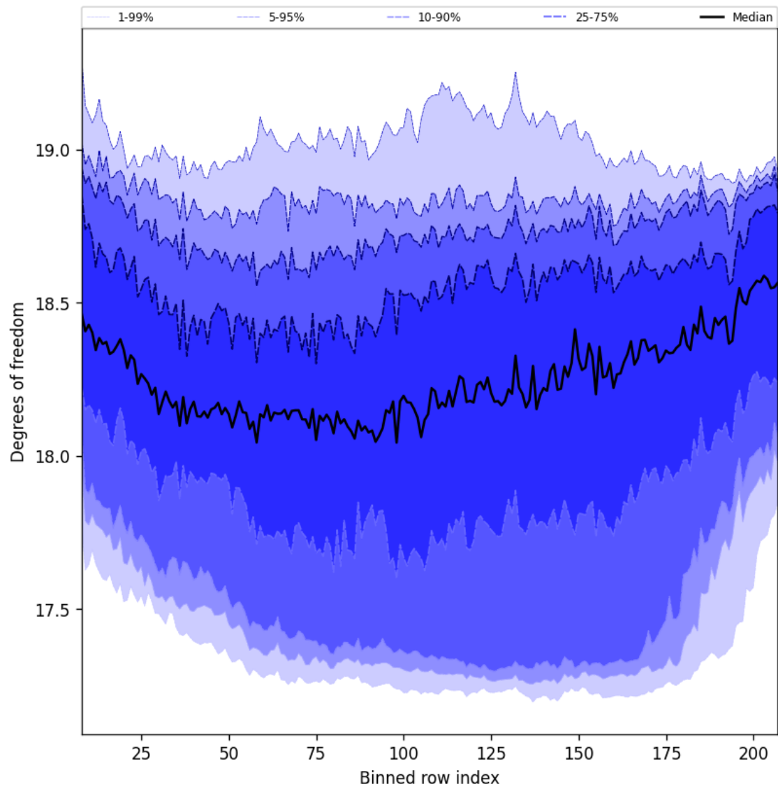
Figure 41: Along track statistics of “Degrees of freedom” for 2024-10-24 to 2024-10-26
