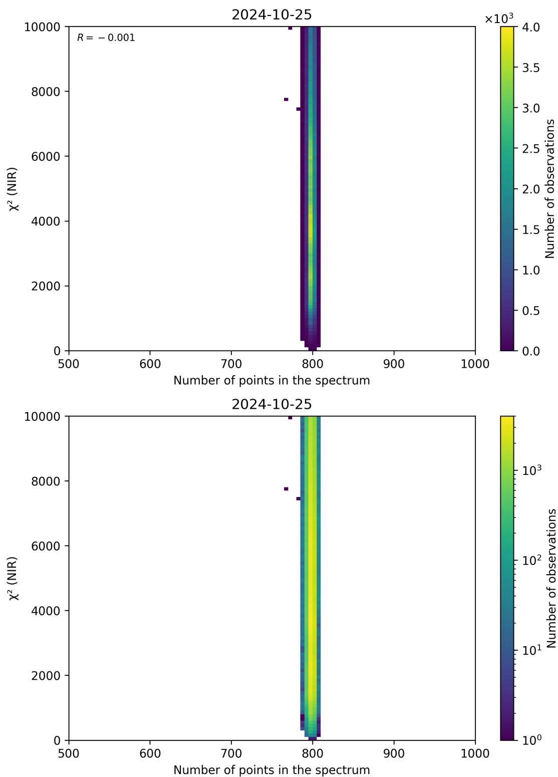
Figure 88: Scatter density plot of “Number of points in the spectrum” against “ \chi^2 (NIR)” for 2024-10-24 to 2024-10-26.
