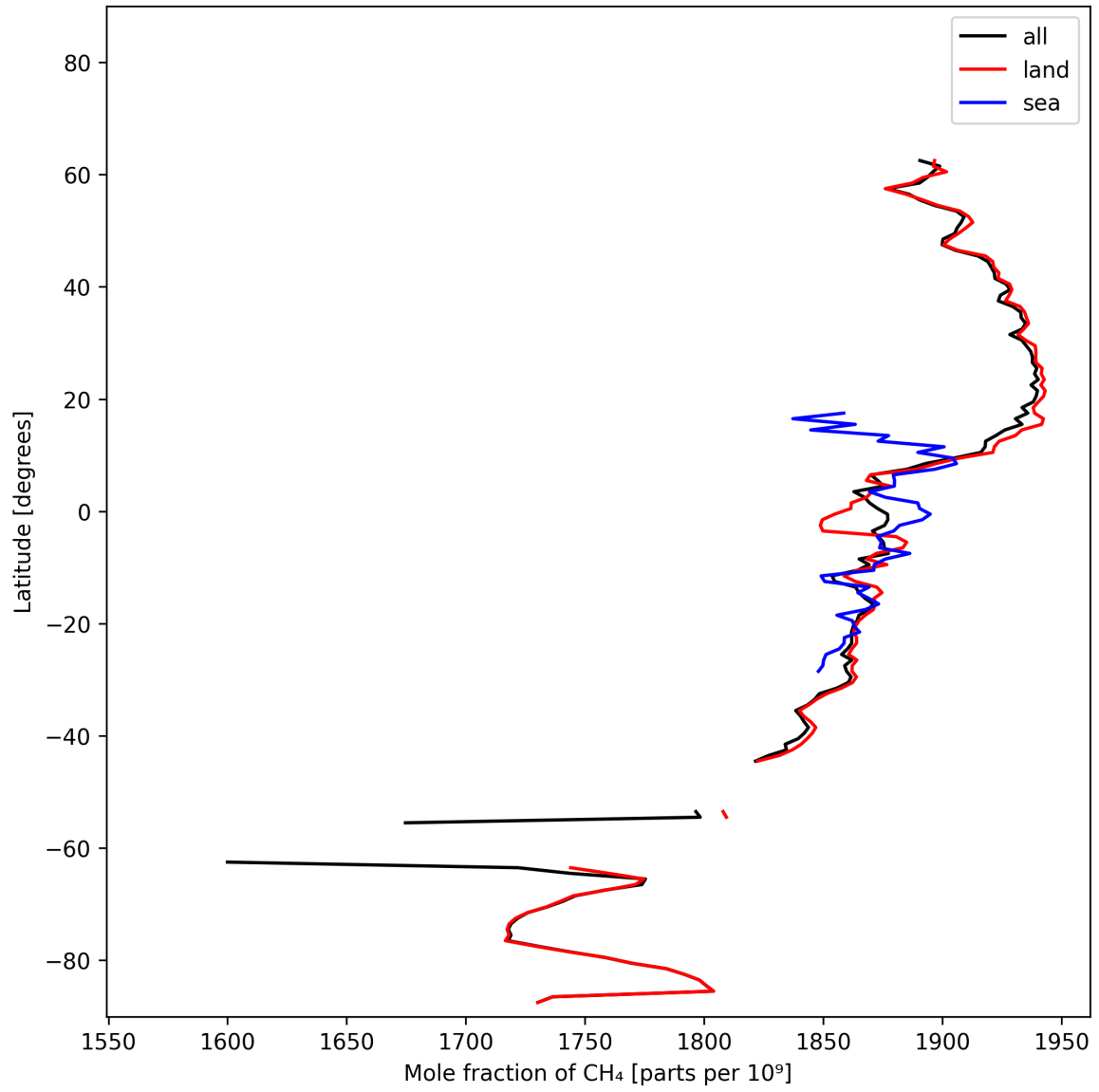
Figure 12: Zonal average of “Mole fraction of \text{CH}_4 ” for 2024-10-24 to 2024-10-26.
