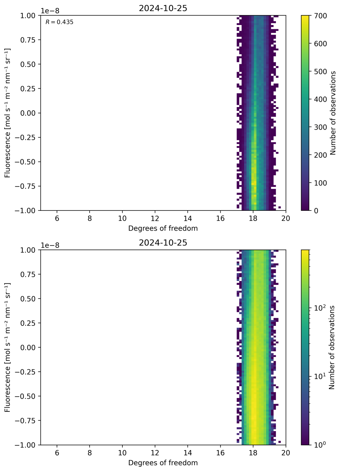
Figure 51: Scatter density plot of “Degrees of freedom” against “Fluorescence” for 2024-10-24 to 2024-10-26.
