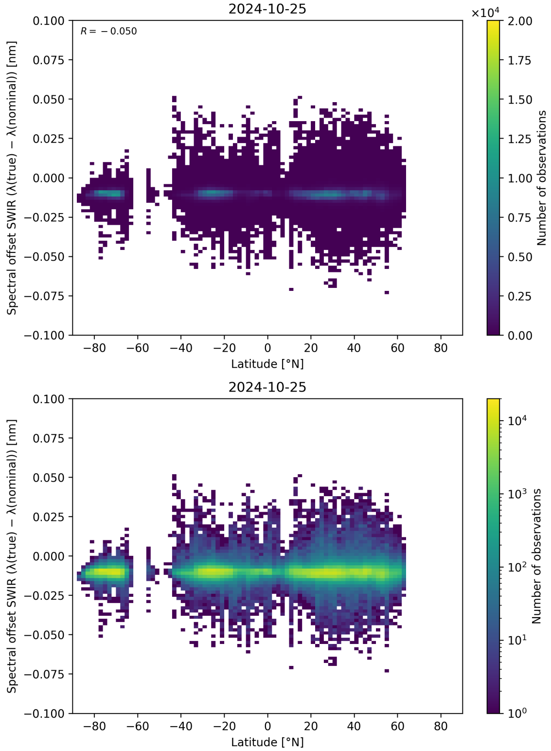
Figure 62: Scatter density plot of “Latitude” against “Spectral offset SWIR ( \lambda_{\text{true}} - \lambda_{\text{nominal}} )” for 2024-10-24 to 2024-10-26.
