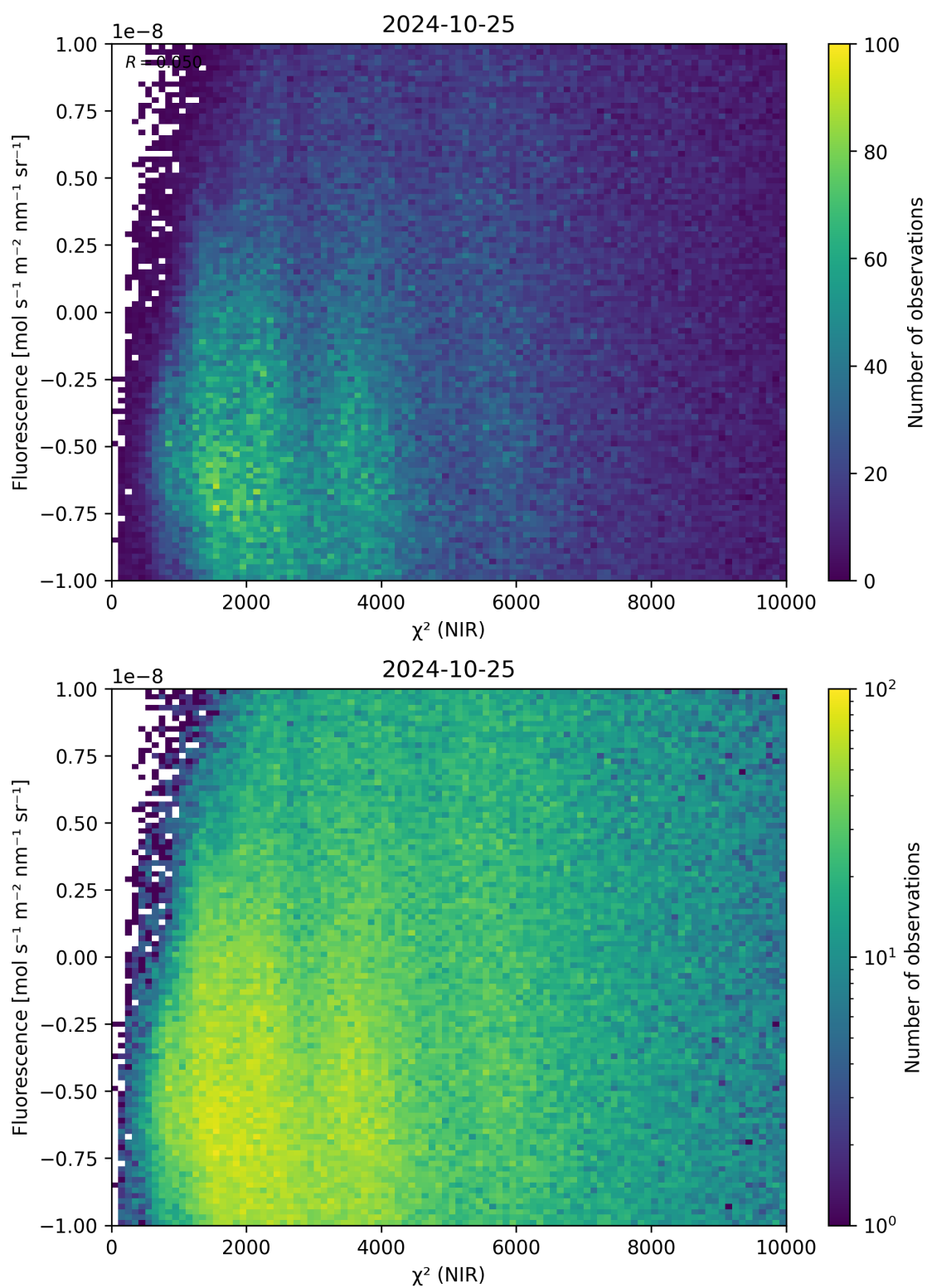
Figure 45: Scatter density plot of “ \chi^2 (NIR)” against “Fluorescence” for 2024-10-24 to 2024-10-26.
