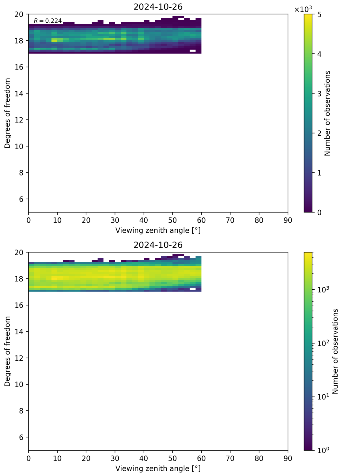
Figure 107: Scatter density plot of “Viewing zenith angle” against “Degrees of freedom” for 2024-10-25 to 2024-10-27.
