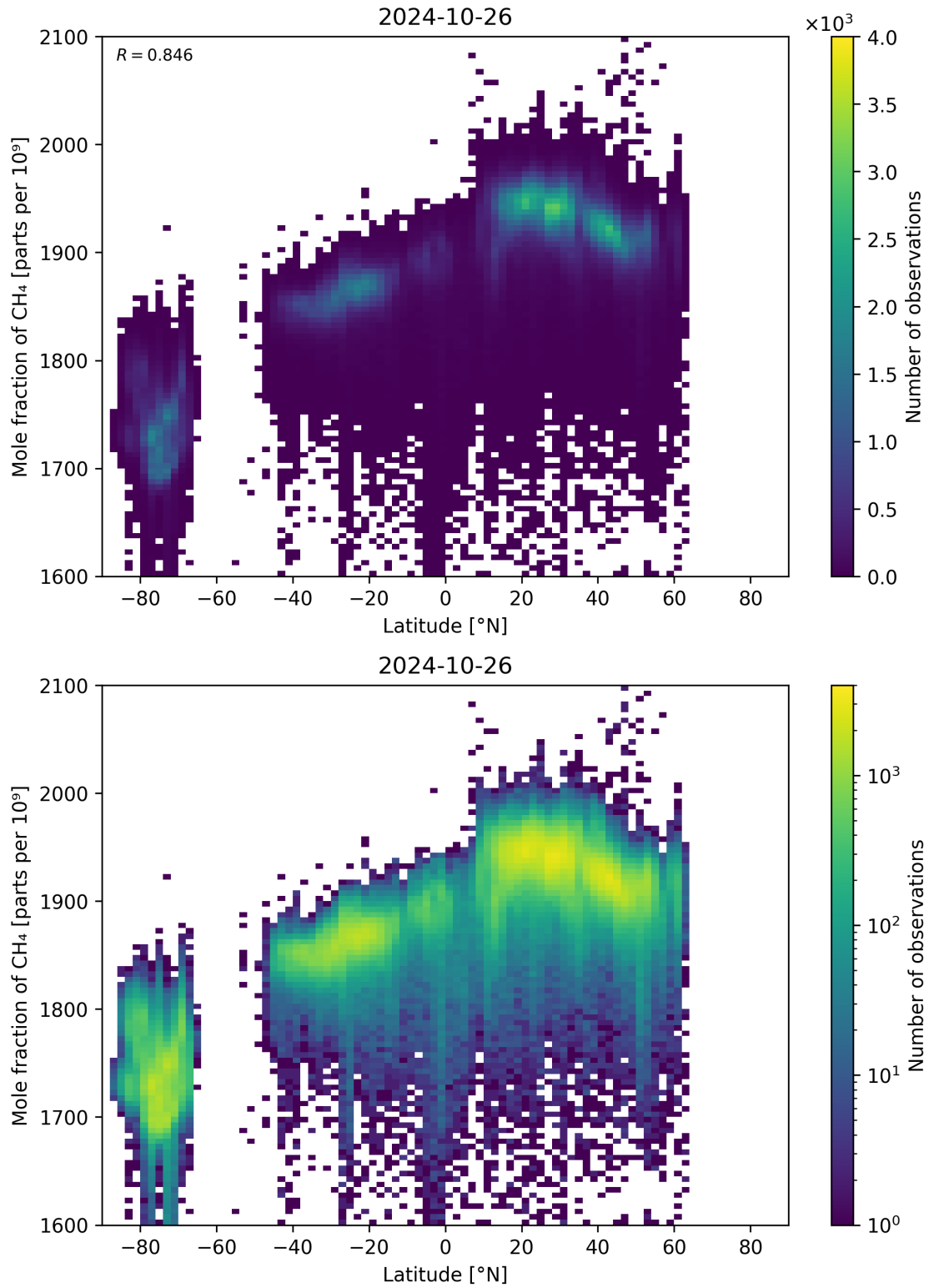
Figure 57: Scatter density plot of “Latitude” against “Mole fraction of \text{CH}_4 ” for 2024-10-25 to 2024-10-27.
