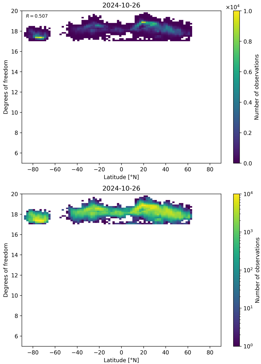
Figure 55: Scatter density plot of “Latitude” against “Degrees of freedom” for 2024-10-25 to 2024-10-27.
