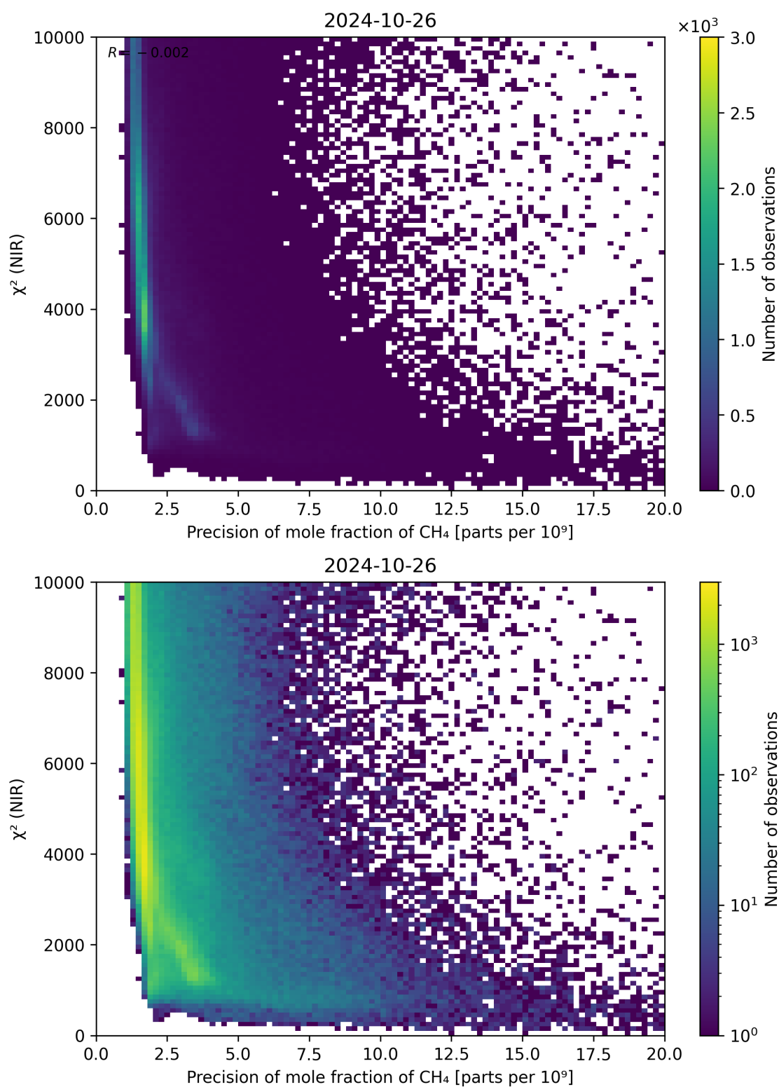
Figure 78: Scatter density plot of “Precision of mole fraction of \text{CH}_4 ” against “ \chi^2 (NIR)” for 2024-10-25 to 2024-10-27.
