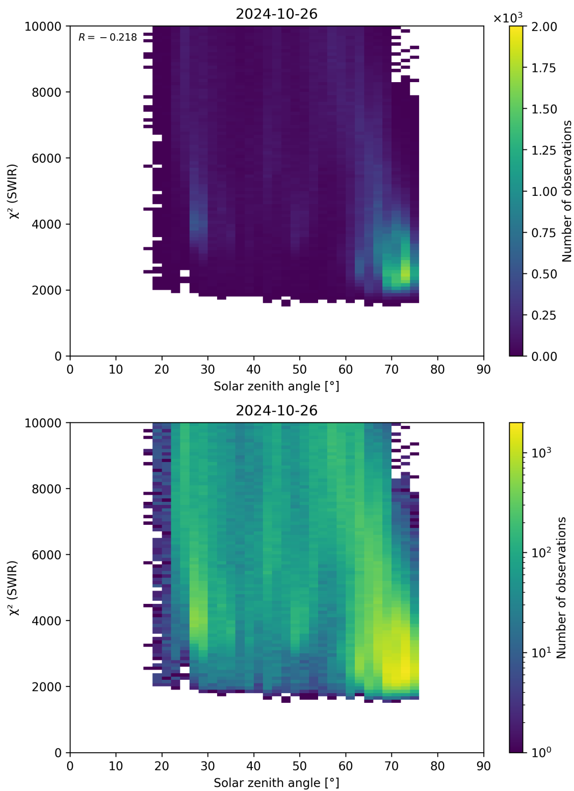
Figure 95: Scatter density plot of “Solar zenith angle” against “ \chi^2 (SWIR)” for 2024-10-25 to 2024-10-27.
