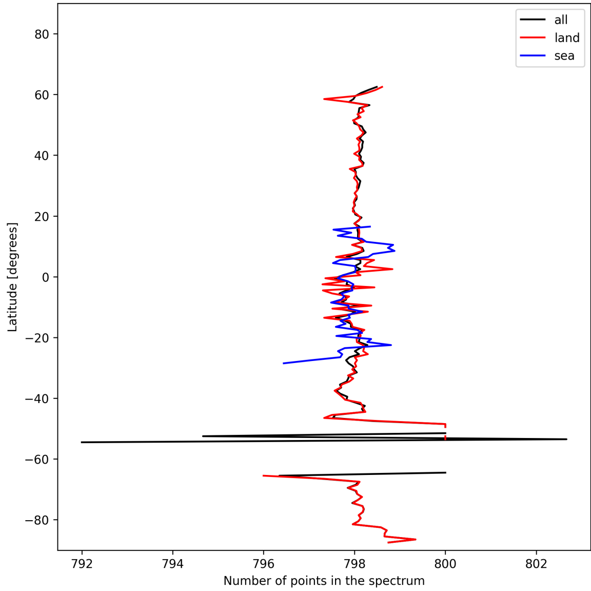
Figure 15: Zonal average of “Number of points in the spectrum” for 2024-10-25 to 2024-10-27.
