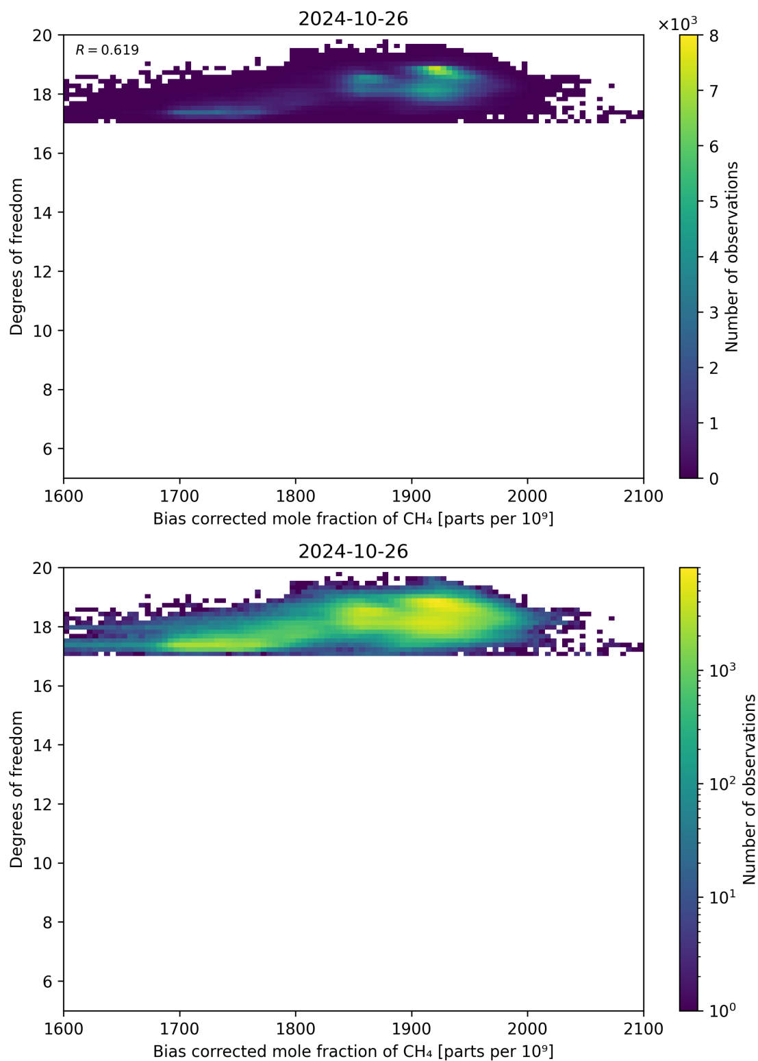
Figure 65: Scatter density plot of “Bias corrected mole fraction of CH 4 ” against “Degrees of freedom” for 2024-10-25 to 2024-10-27.
