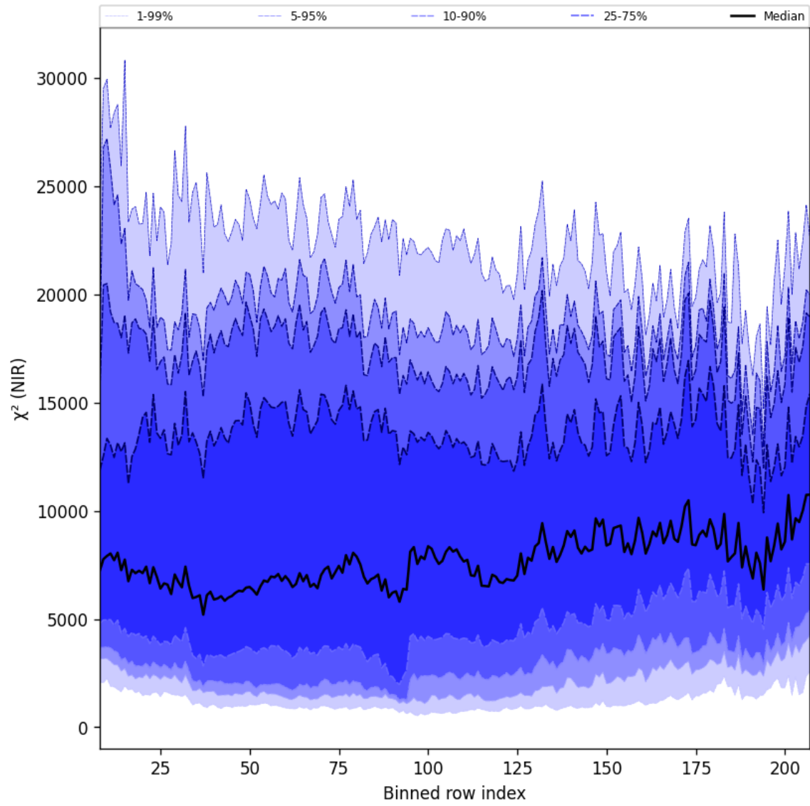
Figure 40: Along track statistics of “ \chi^2 (NIR)” for 2024-10-25 to 2024-10-27
