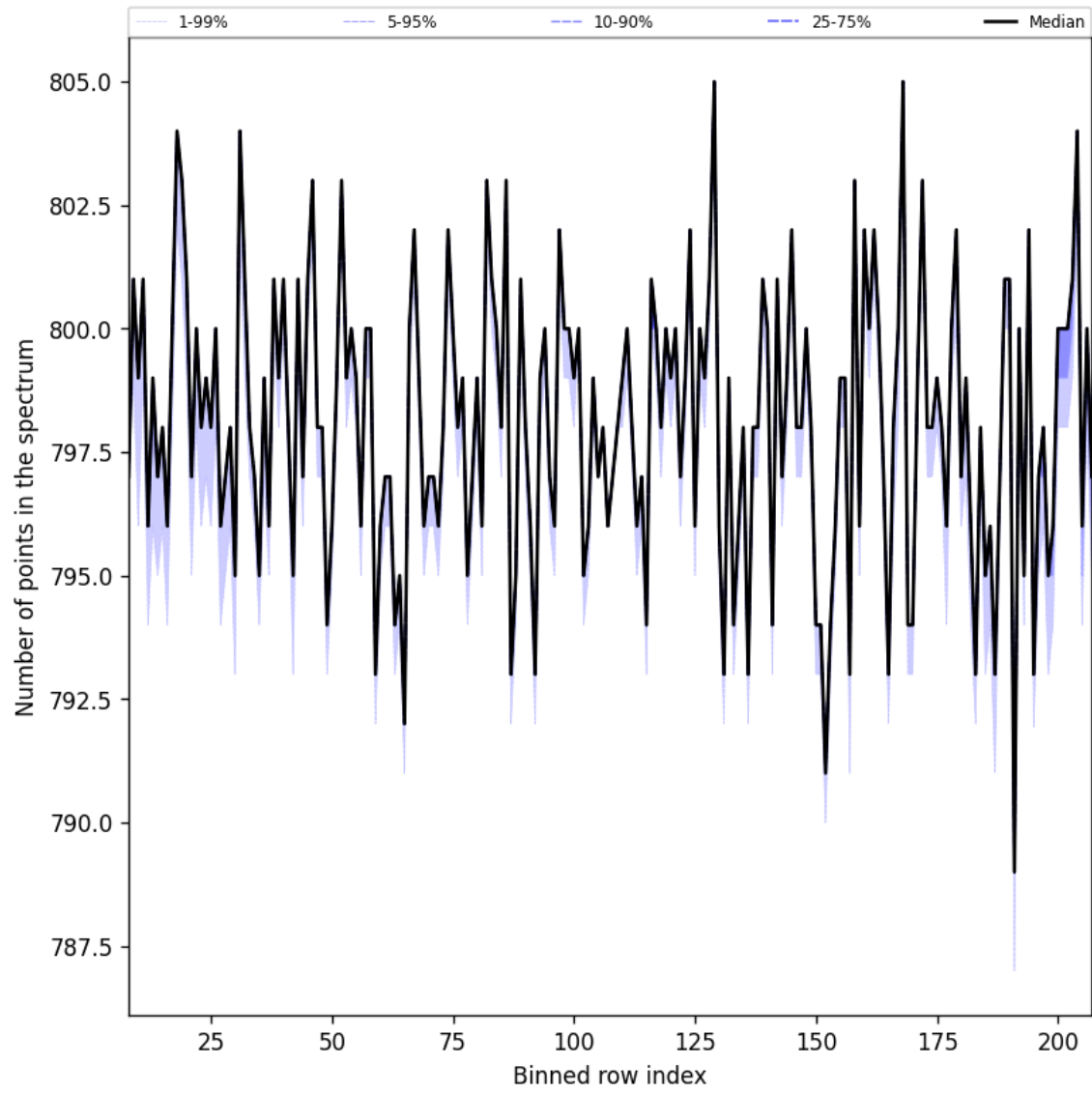
Figure 37: Along track statistics of “Number of points in the spectrum” for 2024-10-25 to 2024-10-27
