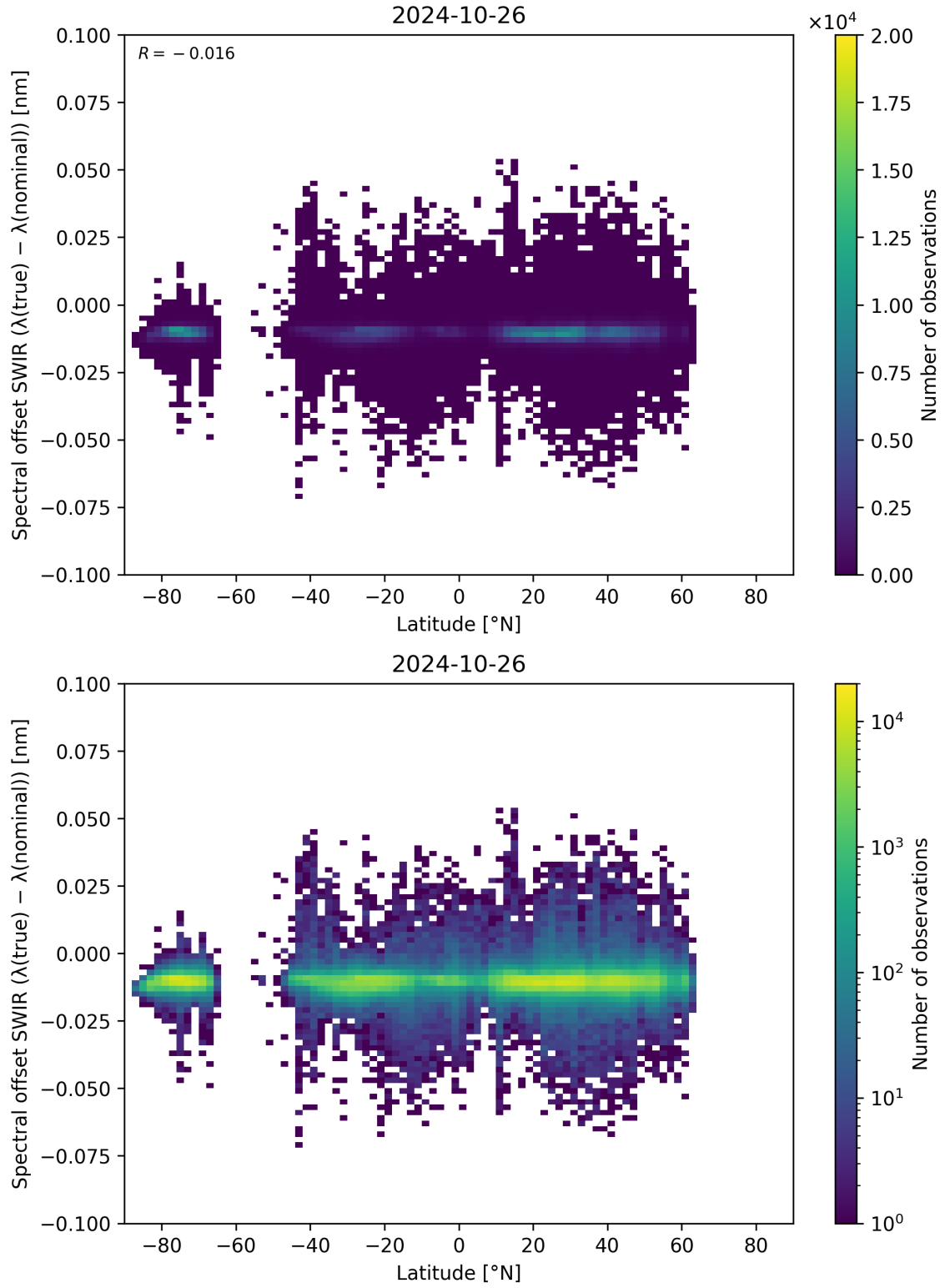
Figure 62: Scatter density plot of “Latitude” against “Spectral offset SWIR ( \lambda_{\text{true}} - \lambda_{\text{nominal}} )” for 2024-10-25 to 2024-10-27.
