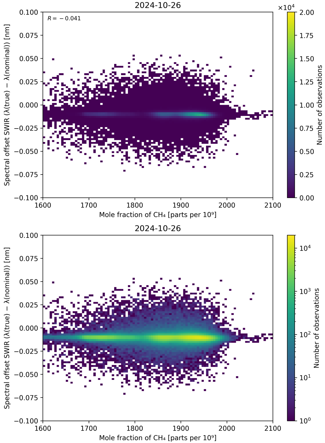
Figure 86: Scatter density plot of “Mole fraction of CH 4 ” against “Spectral offset SWIR ( \lambda_{\text{true}} - \lambda_{\text{nominal}} )” for 2024-10-25 to 2024-10-27.
