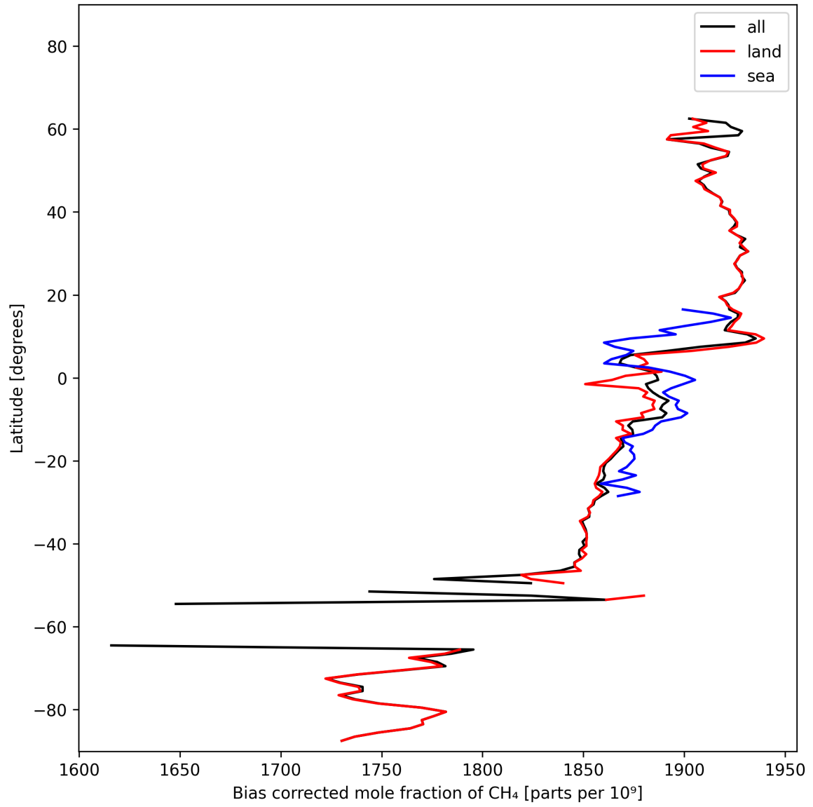
Figure 14: Zonal average of “Bias corrected mole fraction of CH 4 ” for 2024-10-25 to 2024-10-27.
