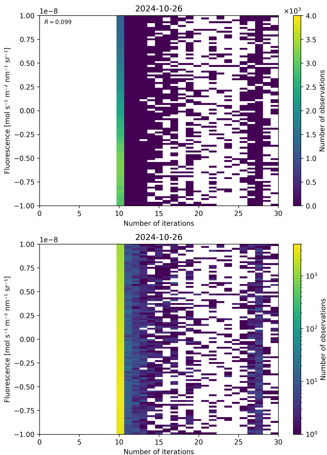
Figure 87: Scatter density plot of “Number of iterations” against “Fluorescence” for 2024-10-25 to 2024-10-27.
