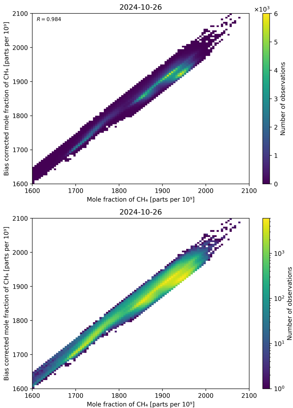
Figure 74: Scatter density plot of “Mole fraction of CH 4 ” against “Bias corrected mole fraction of CH 4 ” for 2024-10-25 to 2024-10-27.
