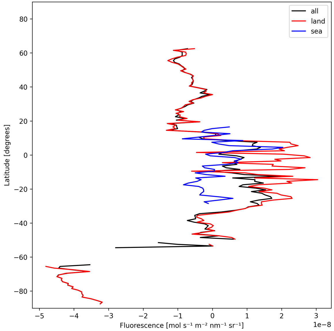
Figure 21: Zonal average of “Fluorescence” for 2024-10-25 to 2024-10-27.
