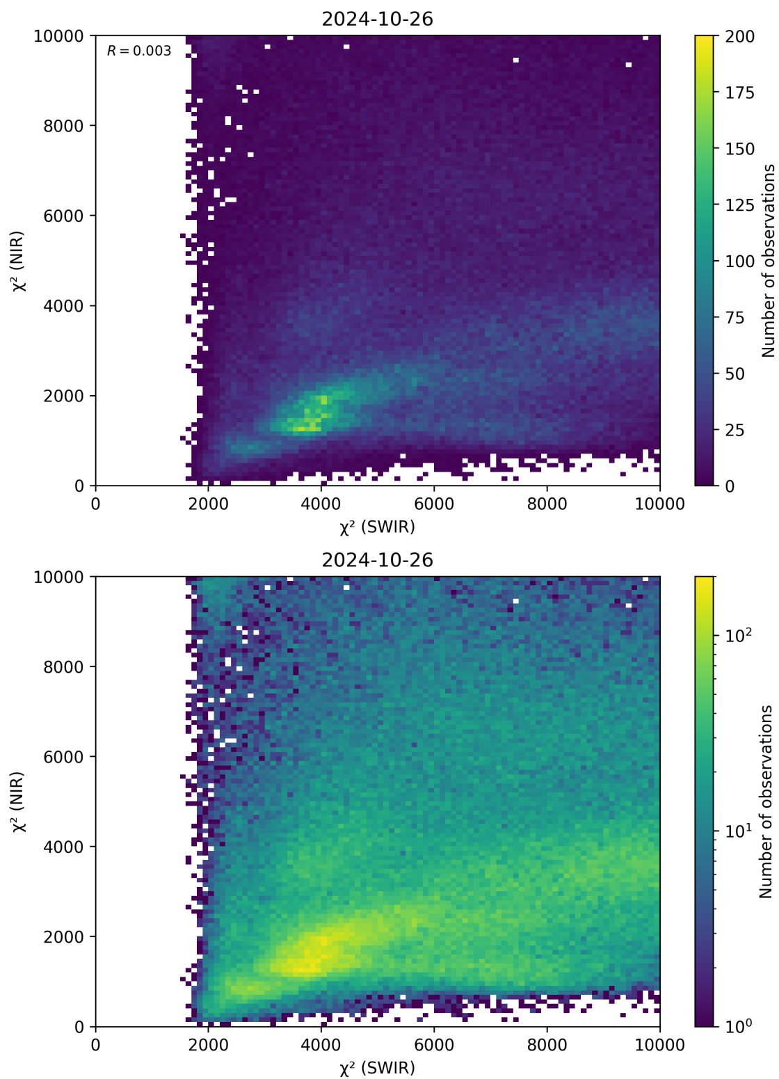
Figure 47: Scatter density plot of “ \chi^2 (SWIR)” against “ \chi^2 (NIR)” for 2024-10-25 to 2024-10-27.
