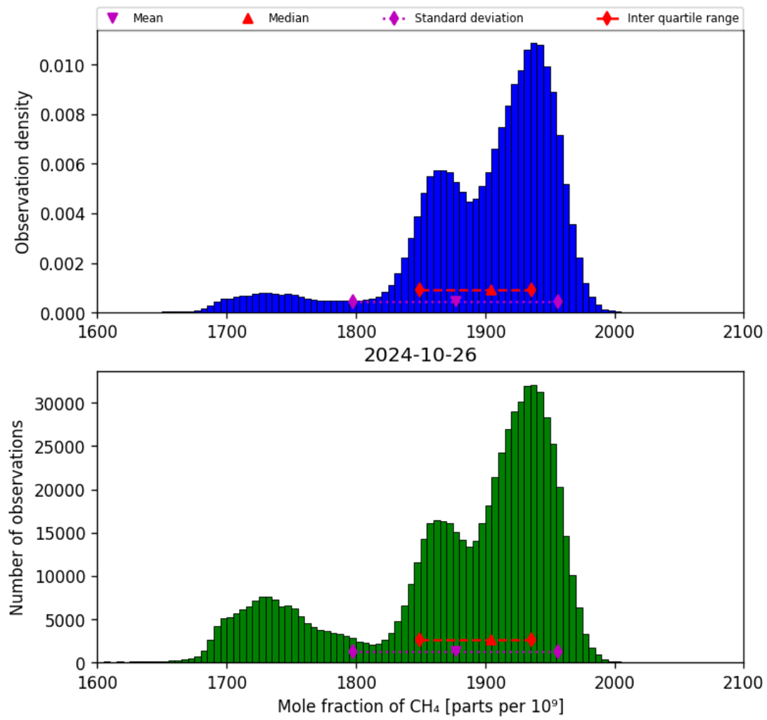
Figure 23: Histogram of “Mole fraction of CH 4 ” for 2024-10-25 to 2024-10-27
