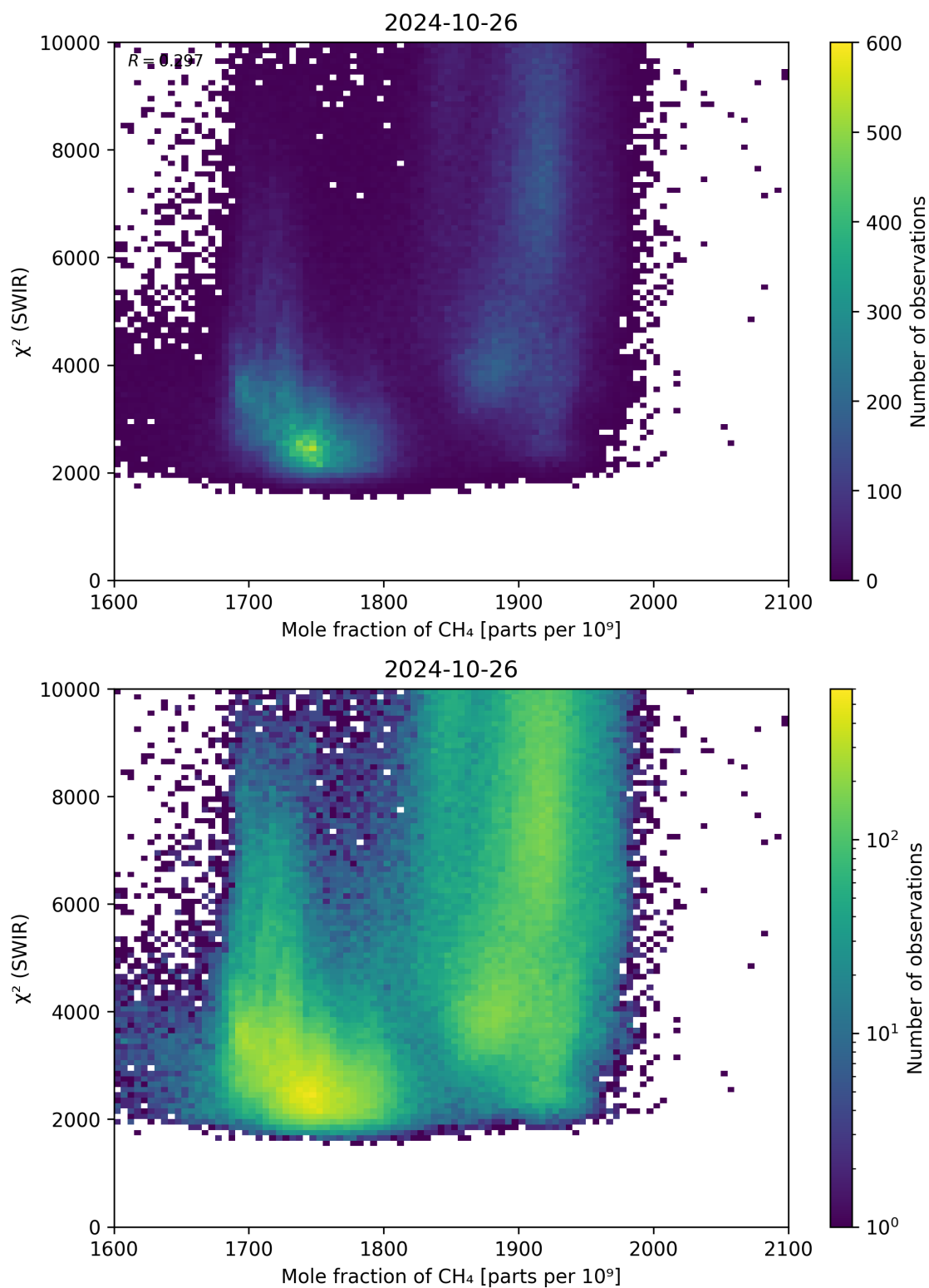
Figure 71: Scatter density plot of “Mole fraction of CH 4 ” against “ \chi^2 (SWIR)” for 2024-10-25 to 2024-10-27.
