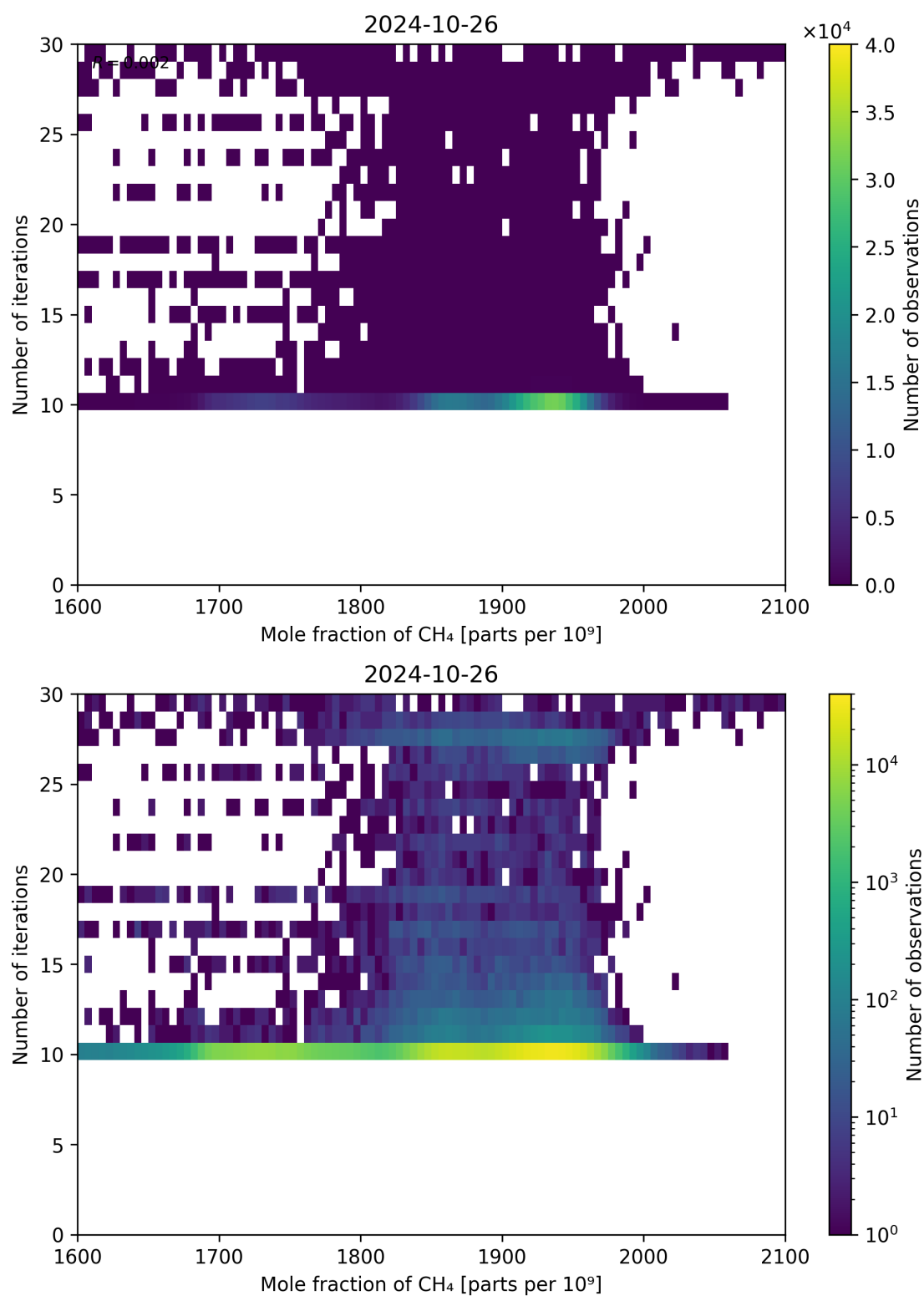
Figure 76: Scatter density plot of “Mole fraction of CH 4 ” against “Number of iterations” for 2024-10-25 to 2024-10-27.
