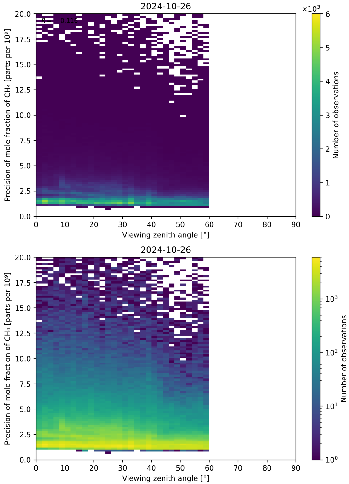
Figure 112: Scatter density plot of “Viewing zenith angle” against “Precision of mole fraction of CH 4 ” for 2024-10-25 to 2024-10-27.
