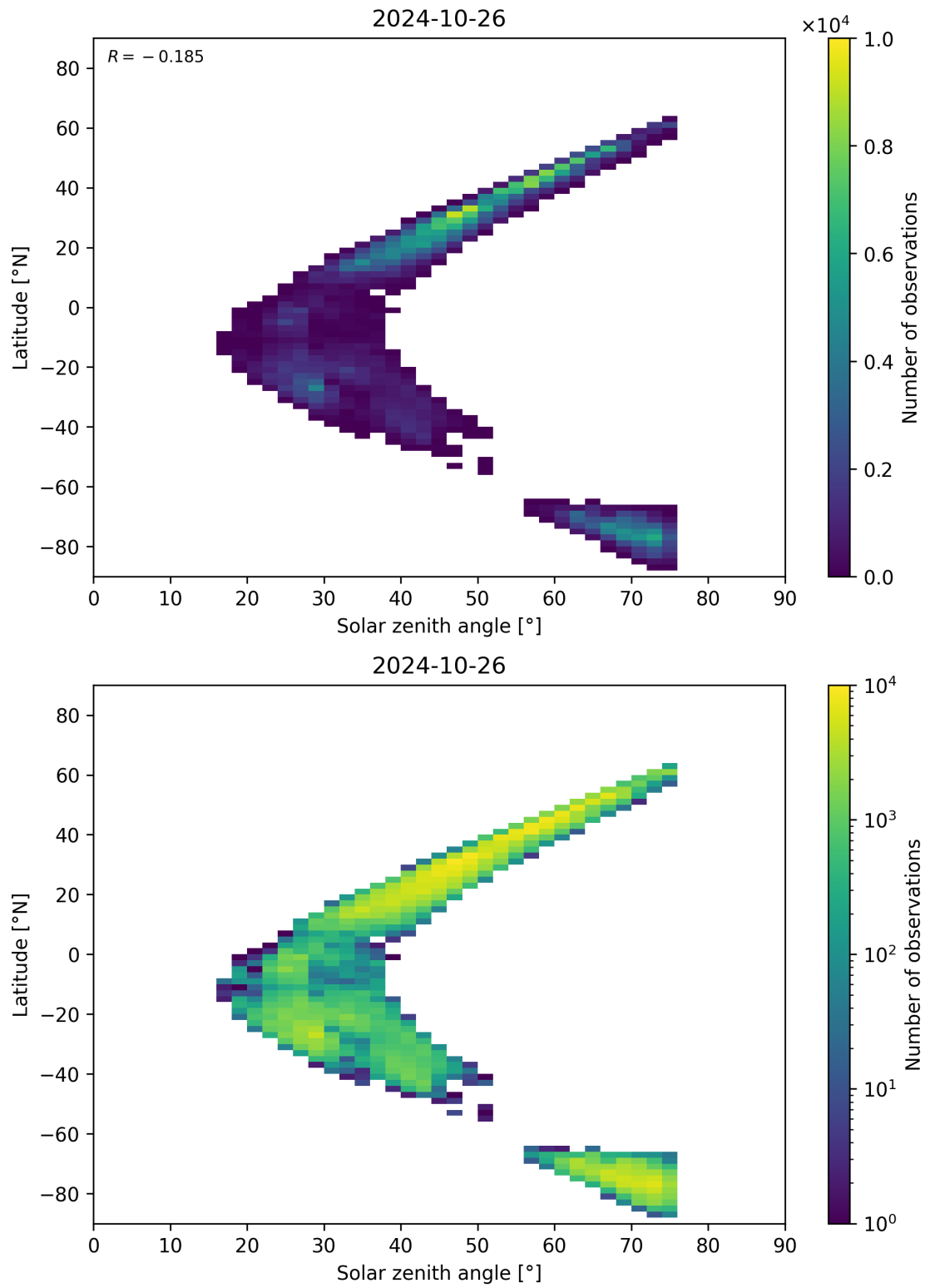
Figure 98: Scatter density plot of “Solar zenith angle” against “Latitude” for 2024-10-25 to 2024-10-27.
