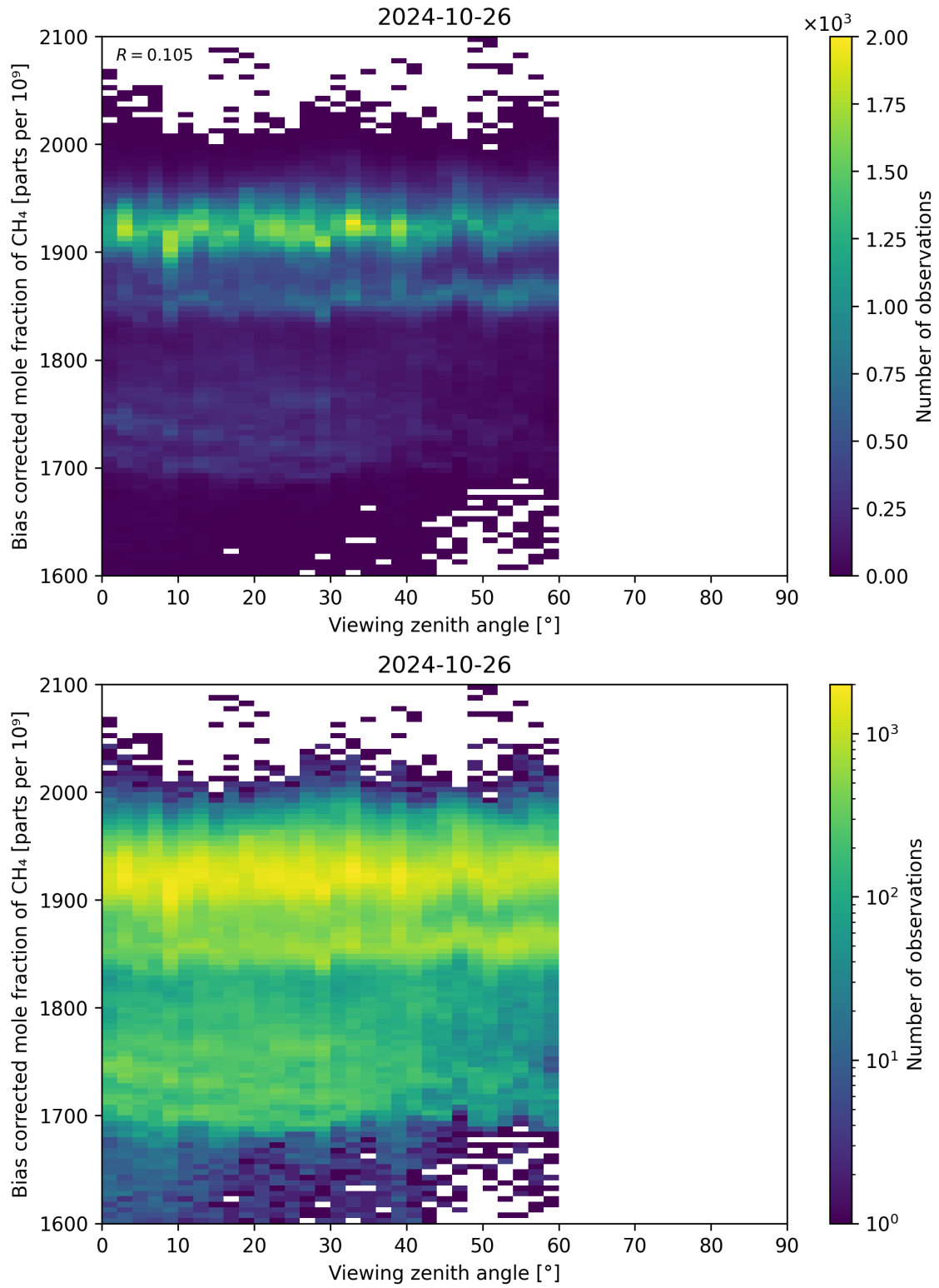
Figure 111: Scatter density plot of “Viewing zenith angle” against “Bias corrected mole fraction of CH 4 ” for 2024-10-25 to 2024-10-27.
