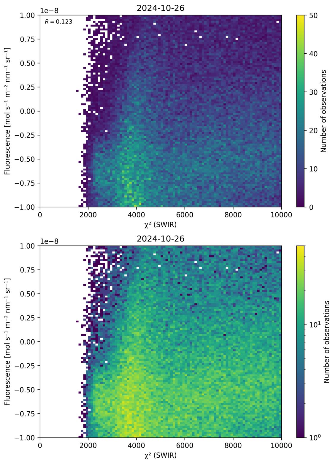
Figure 49: Scatter density plot of “ \chi^2 (SWIR)” against “Fluorescence” for 2024-10-25 to 2024-10-27.
