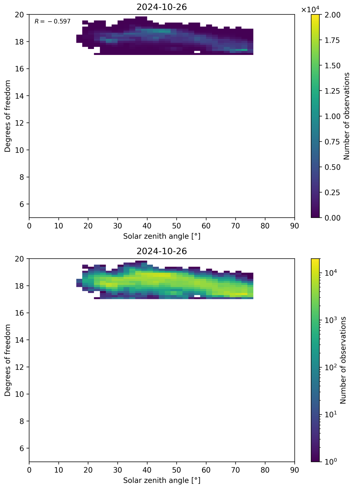
Figure 96: Scatter density plot of “Solar zenith angle” against “Degrees of freedom” for 2024-10-25 to 2024-10-27.
