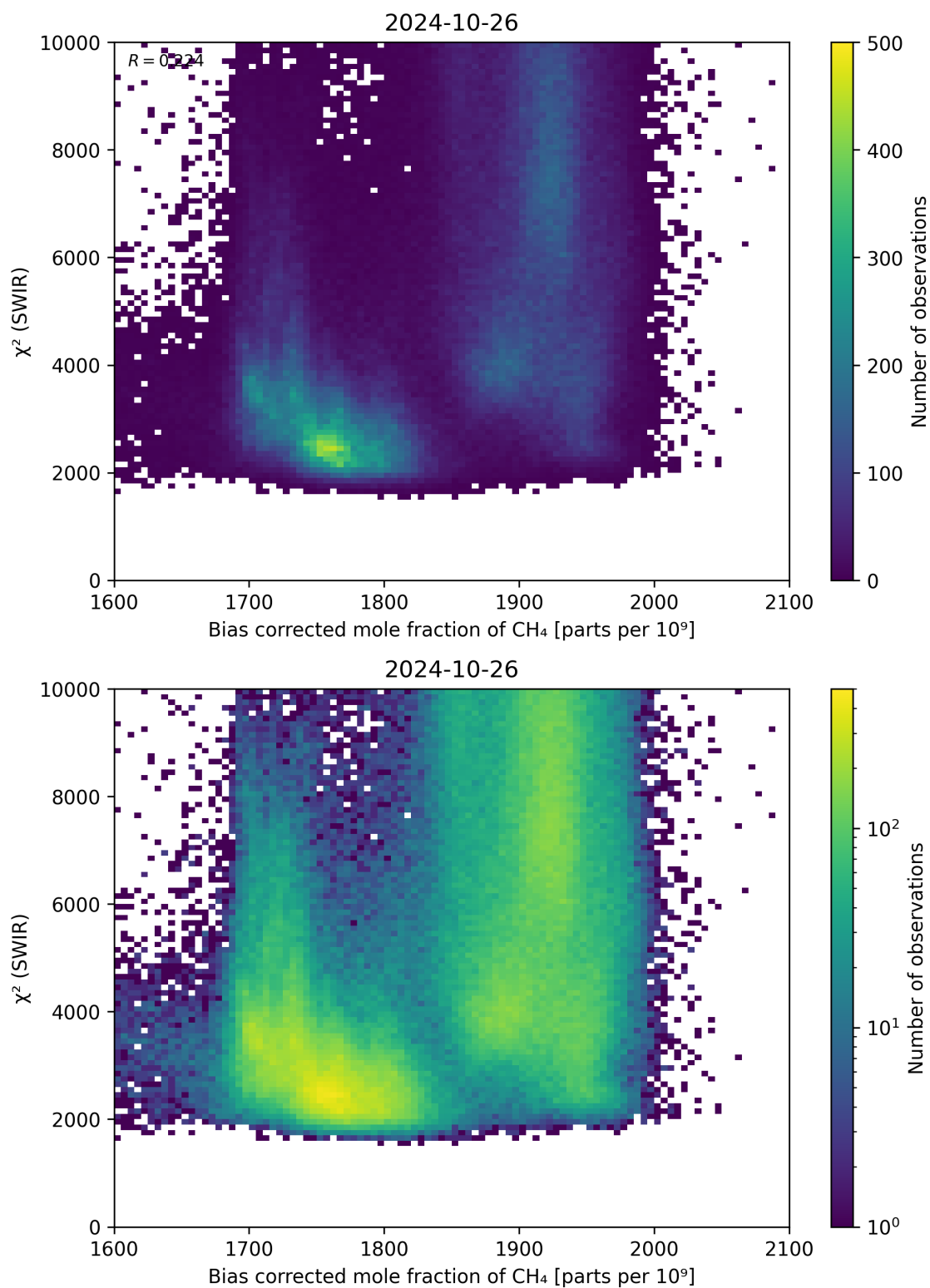
Figure 64: Scatter density plot of “Bias corrected mole fraction of CH 4 ” against “ \chi^2 (SWIR)” for 2024-10-25 to 2024-10-27.
