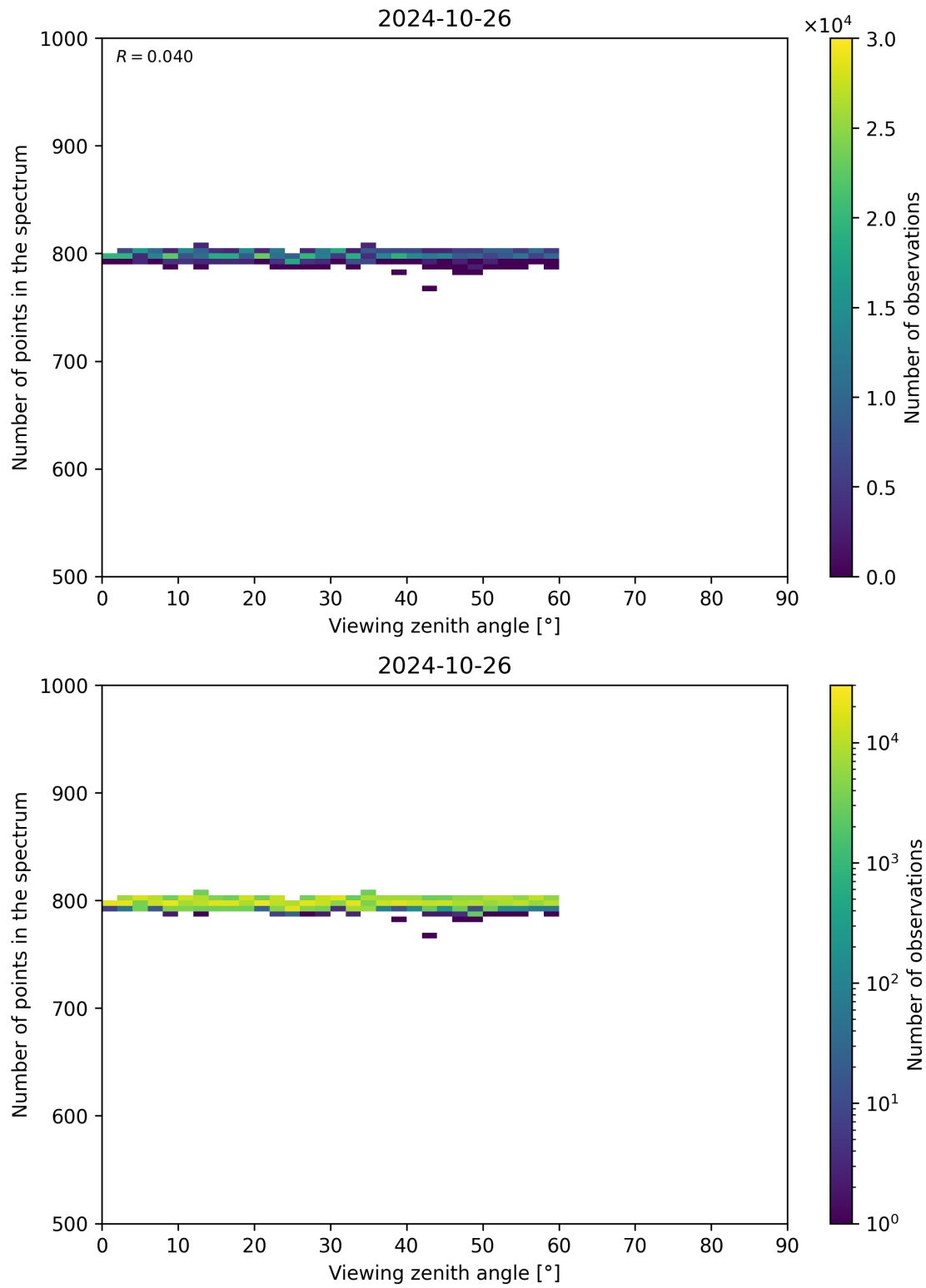
Figure 114: Scatter density plot of “Viewing zenith angle” against “Number of points in the spectrum” for 2024-10-25 to 2024-10-27.
