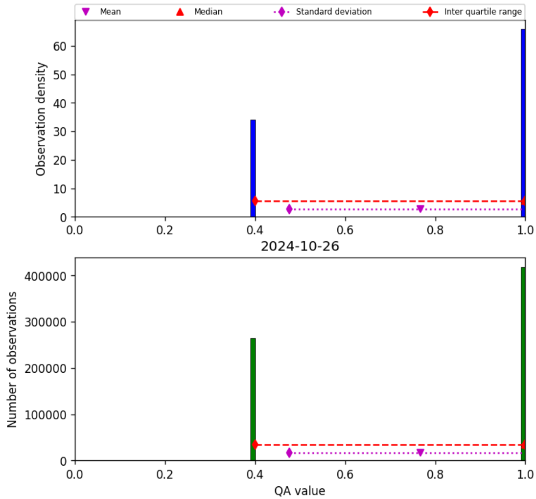
Figure 22: Histogram of “QA value” for 2024-10-25 to 2024-10-27
