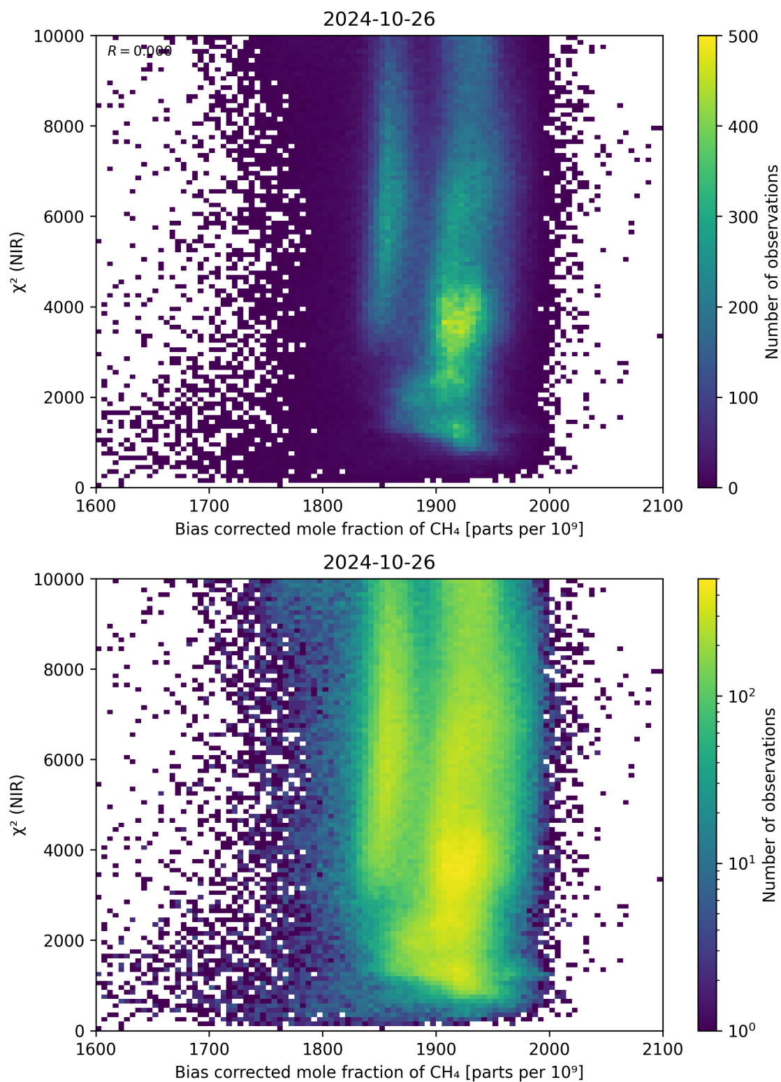
Figure 63: Scatter density plot of “Bias corrected mole fraction of CH 4 ” against “ \chi^2 (NIR)” for 2024-10-25 to 2024-10-27.
