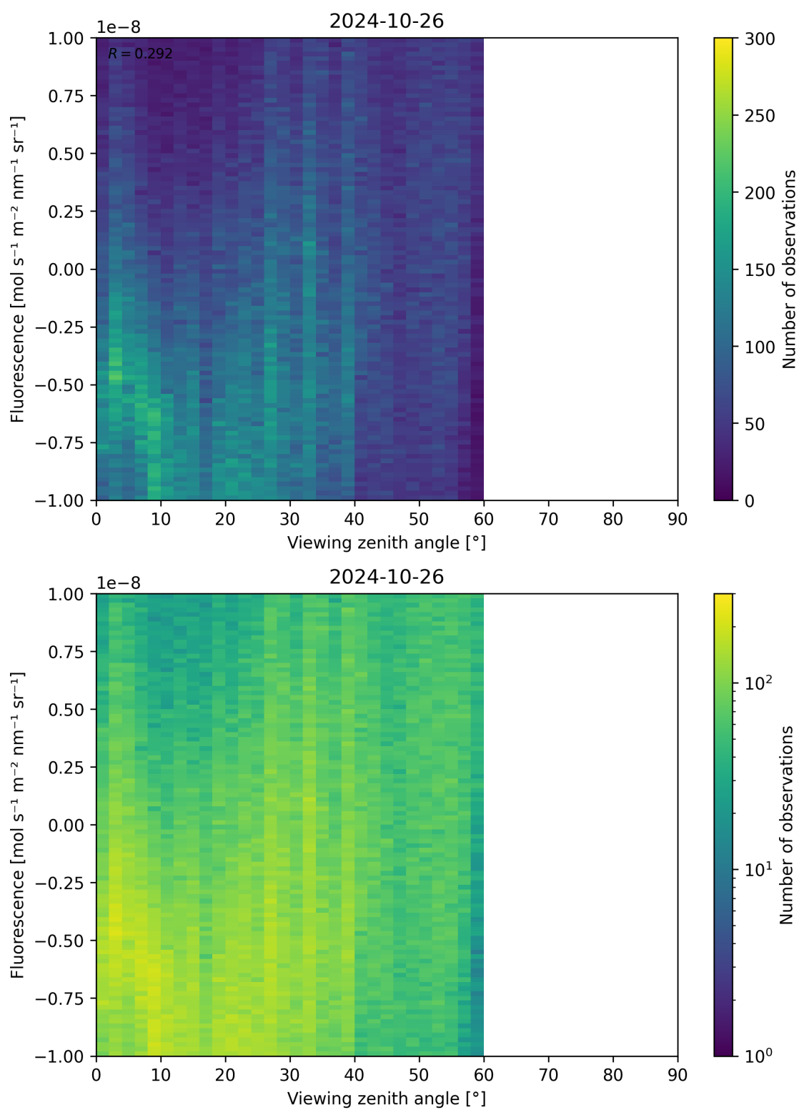
Figure 108: Scatter density plot of “Viewing zenith angle” against “Fluorescence” for 2024-10-25 to 2024-10-27.
