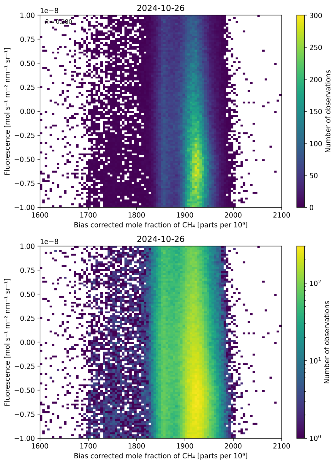
Figure 66: Scatter density plot of “Bias corrected mole fraction of \text{CH}_4 ” against “Fluorescence” for 2024-10-25 to 2024-10-27.
