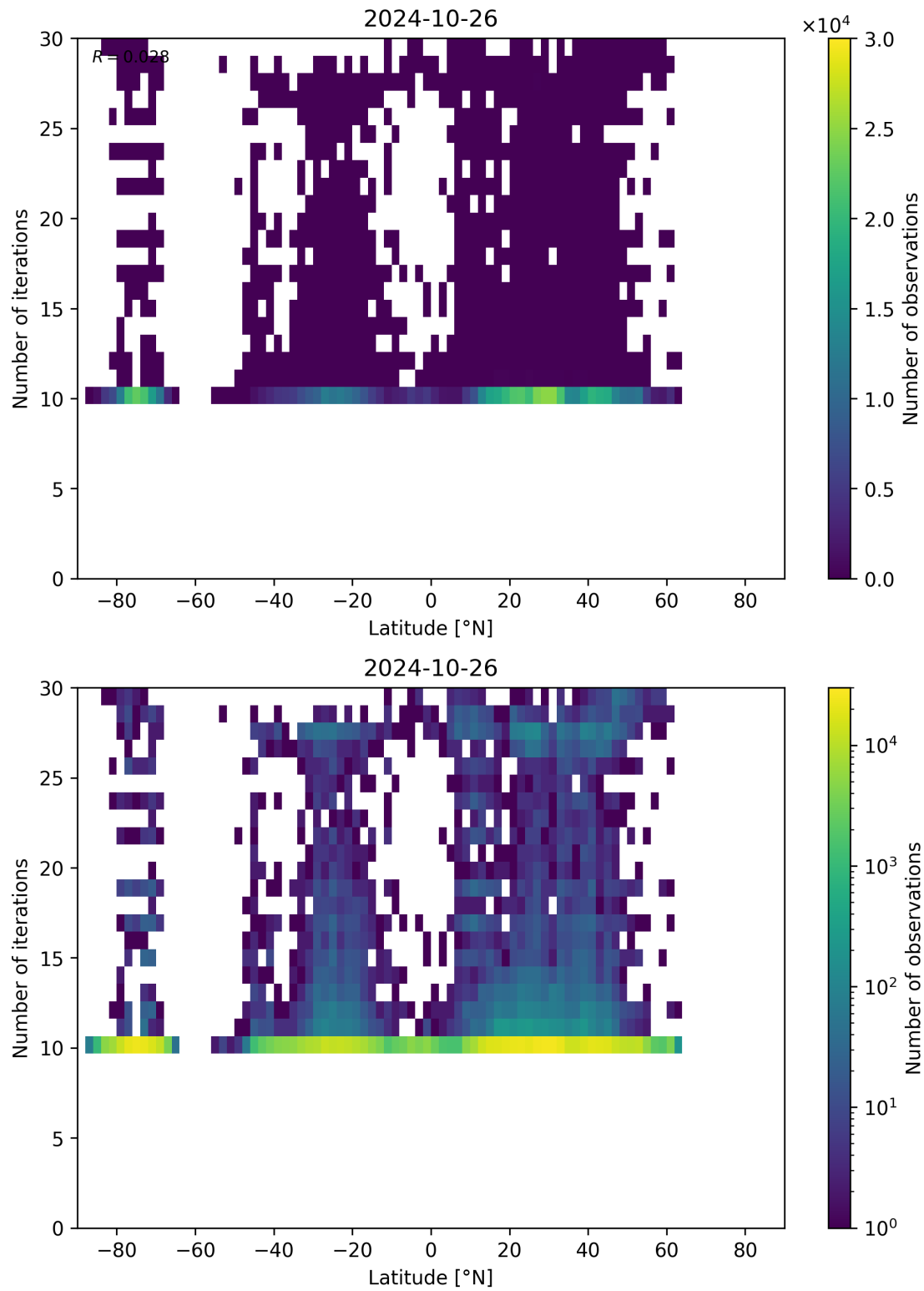
Figure 60: Scatter density plot of “Latitude” against “Number of iterations” for 2024-10-25 to 2024-10-27.
