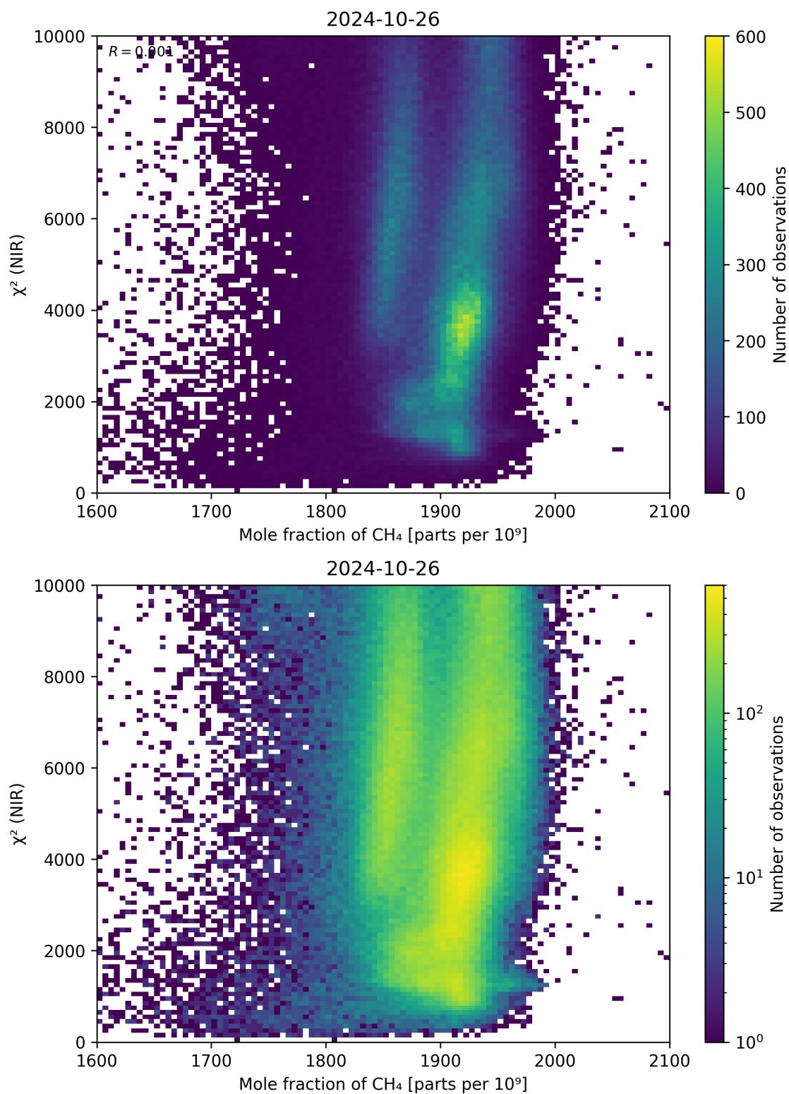
Figure 70: Scatter density plot of “Mole fraction of \text{CH}_4 ” against “ \chi^2 (NIR)” for 2024-10-25 to 2024-10-27.
