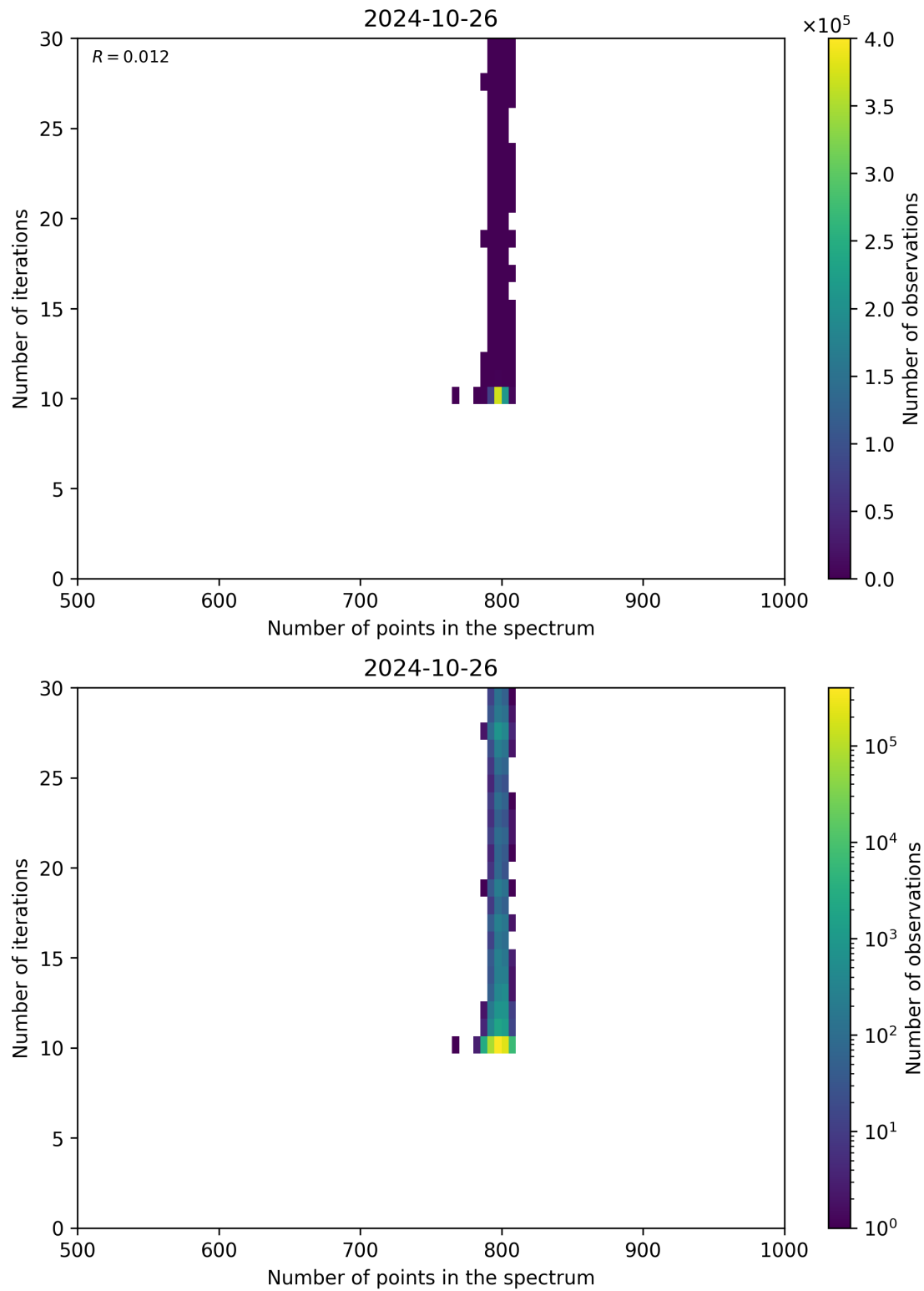
Figure 92: Scatter density plot of “Number of points in the spectrum” against “Number of iterations” for 2024-10-25 to 2024-10-27.
