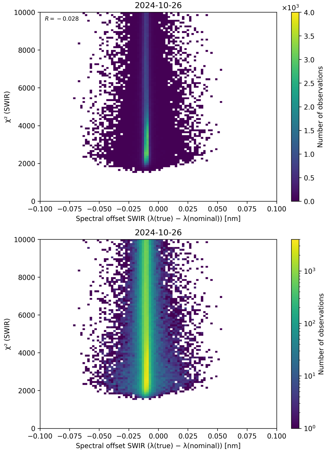
Figure 118: Scatter density plot of “Spectral offset SWIR ( \lambda_{\text{true}} - \lambda_{\text{nominal}} )” against “ \chi^2 (SWIR)” for 2024-10-25 to 2024-10-27.
