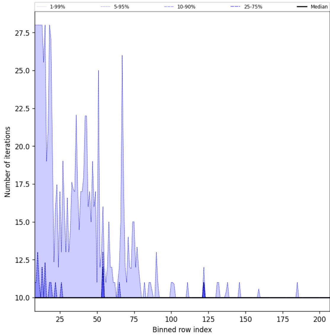
Figure 42: Along track statistics of “Number of iterations” for 2024-10-25 to 2024-10-27
