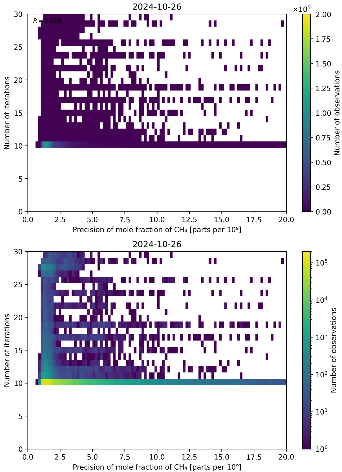
Figure 83: Scatter density plot of “Precision of mole fraction of \text{CH}_4 ” against “Number of iterations” for 2024-10-25 to 2024-10-27.
