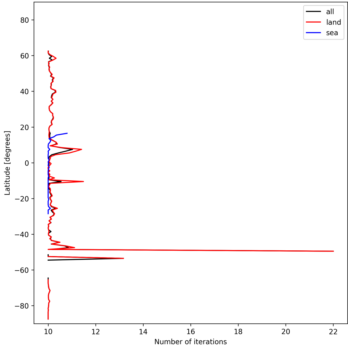
Figure 20: Zonal average of “Number of iterations” for 2024-10-25 to 2024-10-27.
