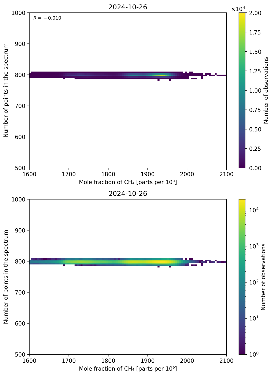
Figure 77: Scatter density plot of “Mole fraction of CH 4 ” against “Number of points in the spectrum” for 2024-10-25 to 2024-10-27.
