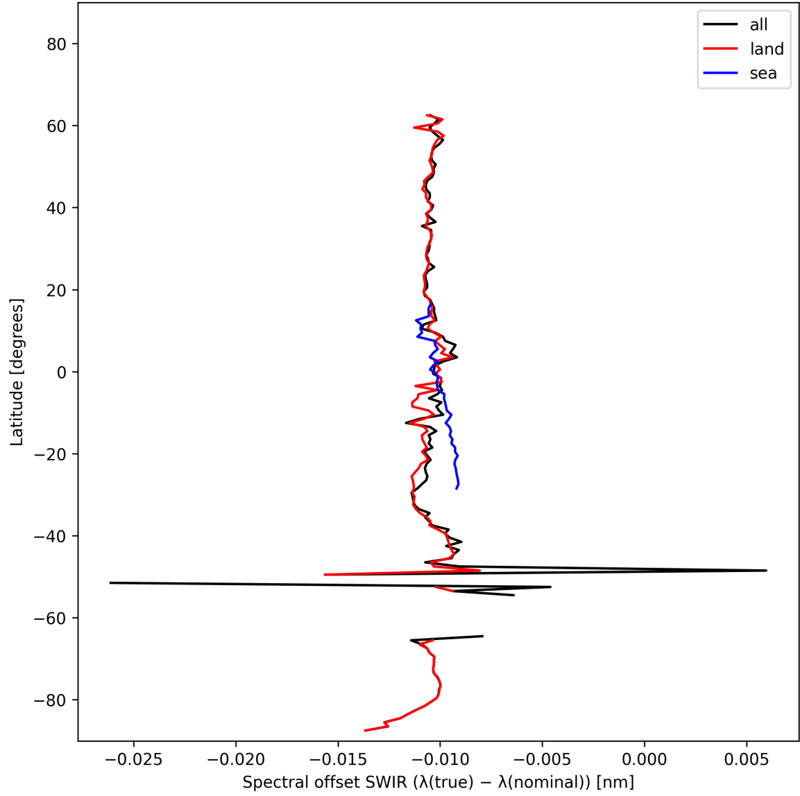
Figure 16: Zonal average of “Spectral offset SWIR ( \lambda_{\text{true}} - \lambda_{\text{nominal}} )” for 2024-10-25 to 2024-10-27.
