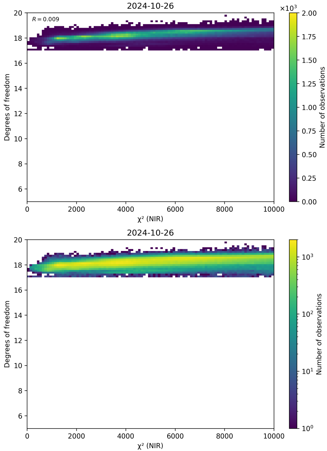
Figure 44: Scatter density plot of “ \chi^2 (NIR)” against “Degrees of freedom” for 2024-10-25 to 2024-10-27.
