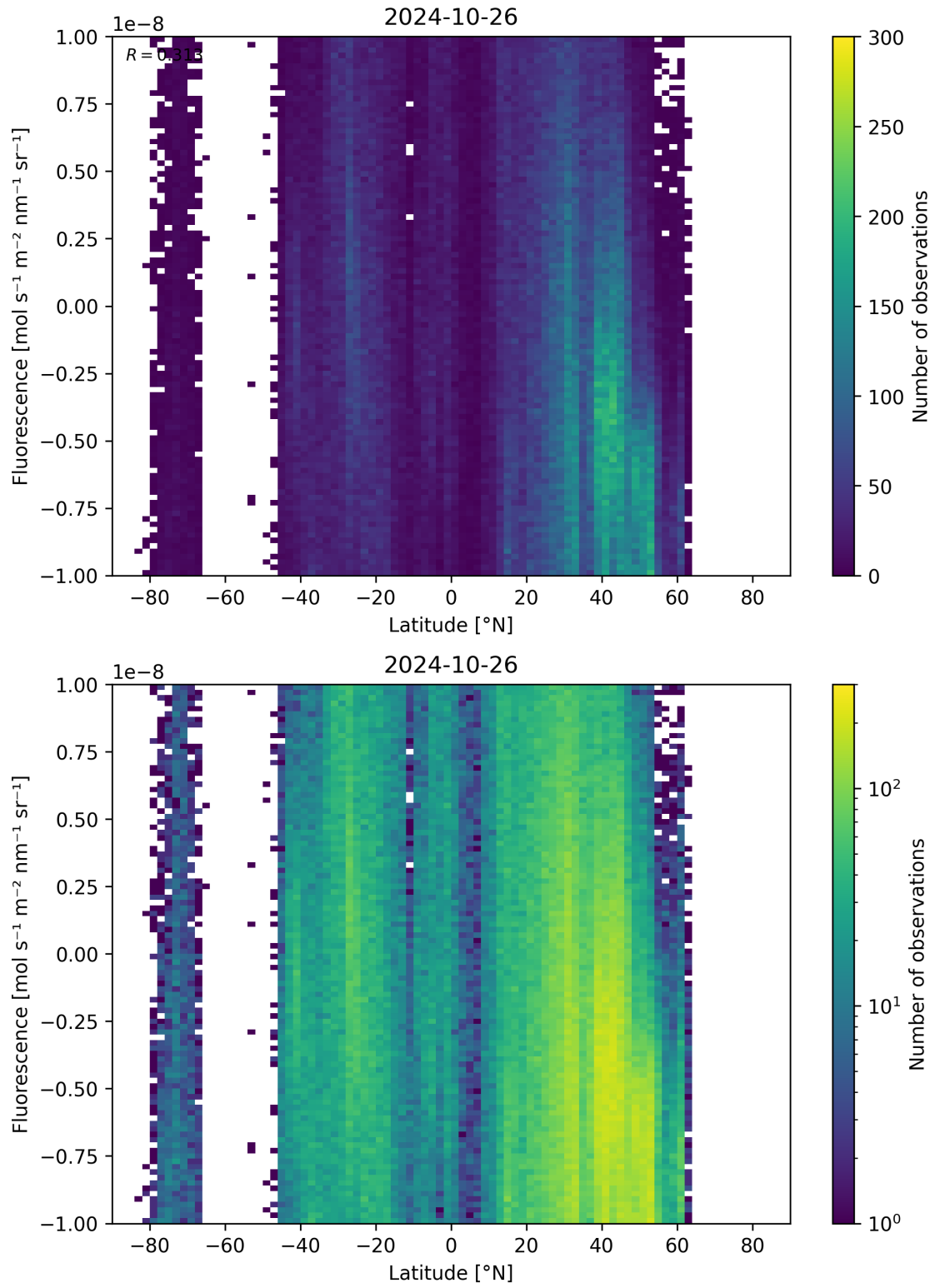
Figure 56: Scatter density plot of “Latitude” against “Fluorescence” for 2024-10-25 to 2024-10-27.
