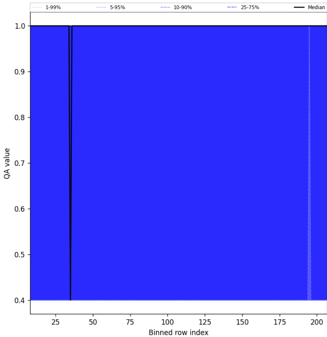
Figure 33: Along track statistics of “QA value” for 2024-10-25 to 2024-10-27
