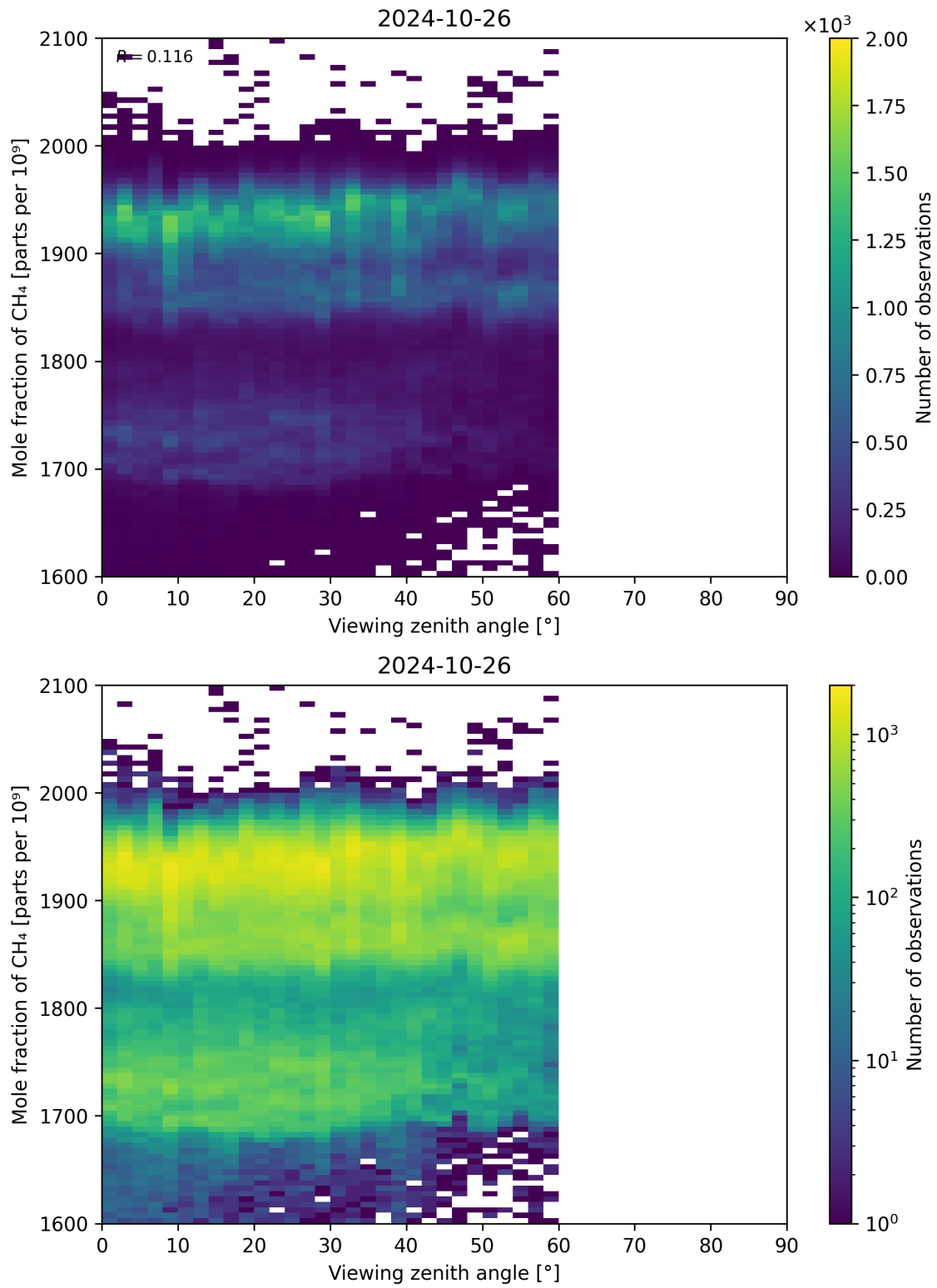
Figure 110: Scatter density plot of “Viewing zenith angle” against “Mole fraction of CH 4 ” for 2024-10-25 to 2024-10-27.
