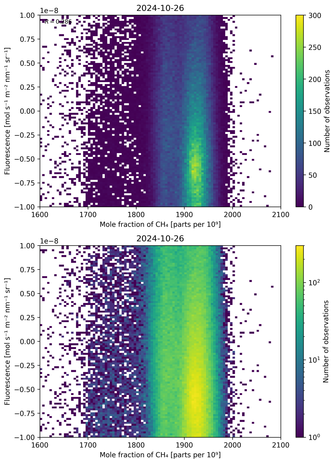
Figure 73: Scatter density plot of “Mole fraction of CH 4 ” against “Fluorescence” for 2024-10-25 to 2024-10-27.
