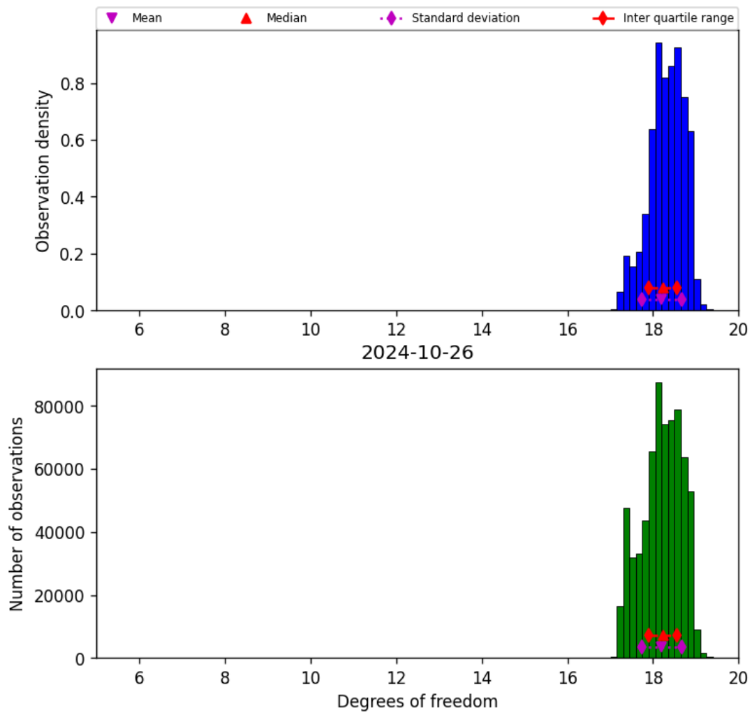
Figure 30: Histogram of “Degrees of freedom” for 2024-10-25 to 2024-10-27
