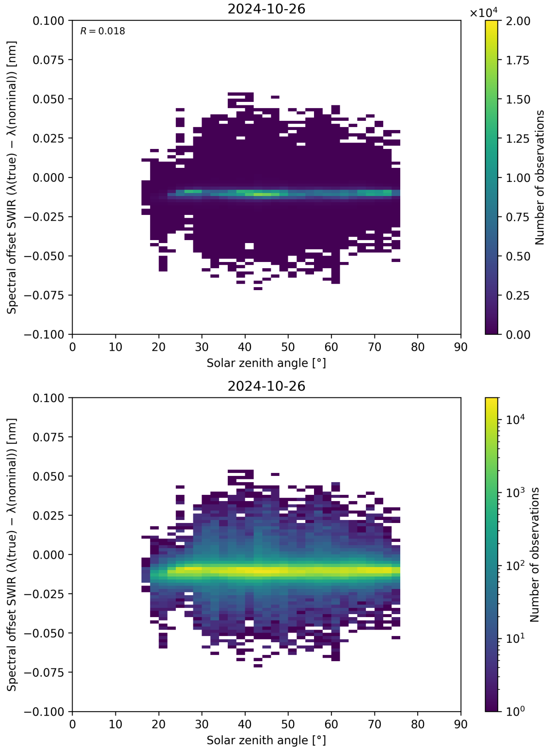
Figure 104: Scatter density plot of “Solar zenith angle” against “Spectral offset SWIR ( \lambda_{\text{true}} - \lambda_{\text{nominal}} )” for 2024-10-25 to 2024-10-27.
