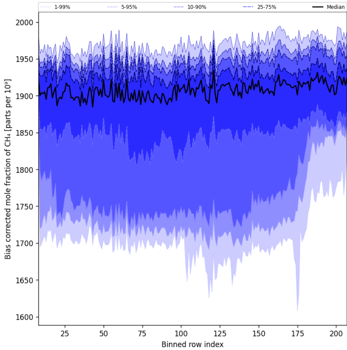
Figure 36: Along track statistics of “Bias corrected mole fraction of CH 4 ” for 2024-10-25 to 2024-10-27
