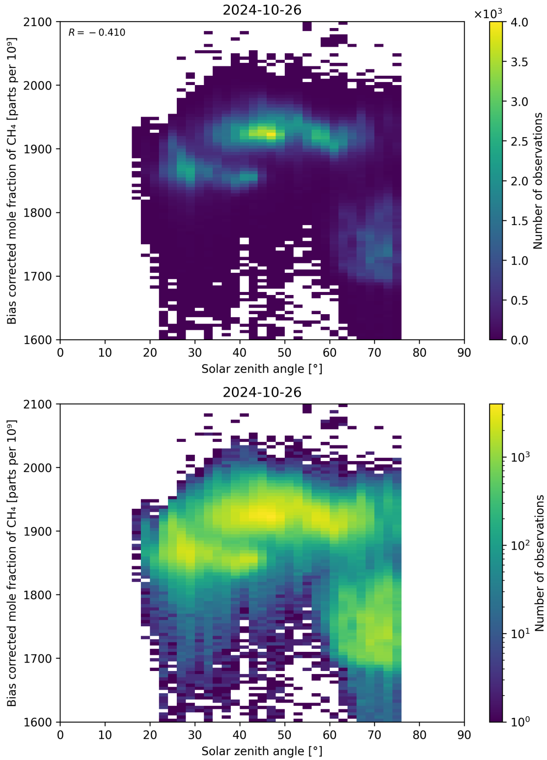
Figure 100: Scatter density plot of “Solar zenith angle” against “Bias corrected mole fraction of CH 4 ” for 2024-10-25 to 2024-10-27.
