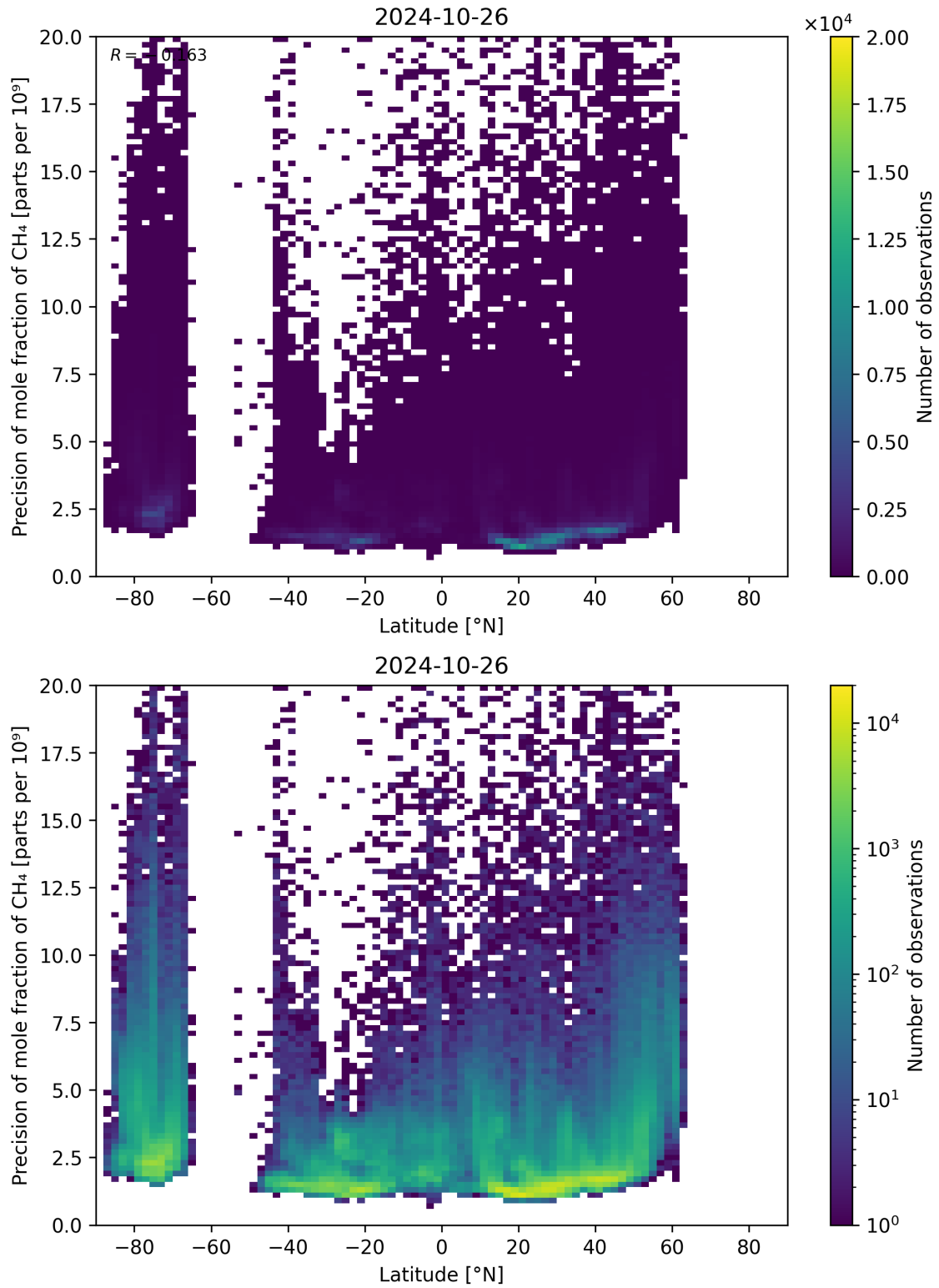
Figure 59: Scatter density plot of “Latitude” against “Precision of mole fraction of CH 4 ” for 2024-10-25 to 2024-10-27.
