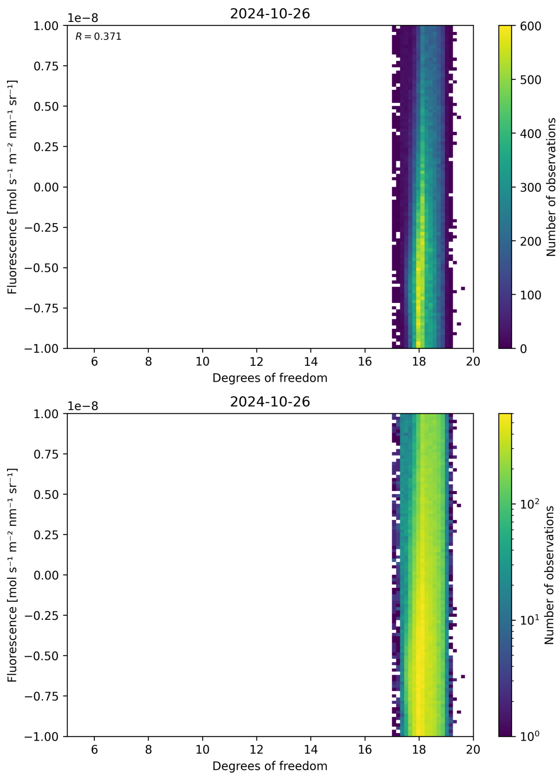
Figure 51: Scatter density plot of “Degrees of freedom” against “Fluorescence” for 2024-10-25 to 2024-10-27.
