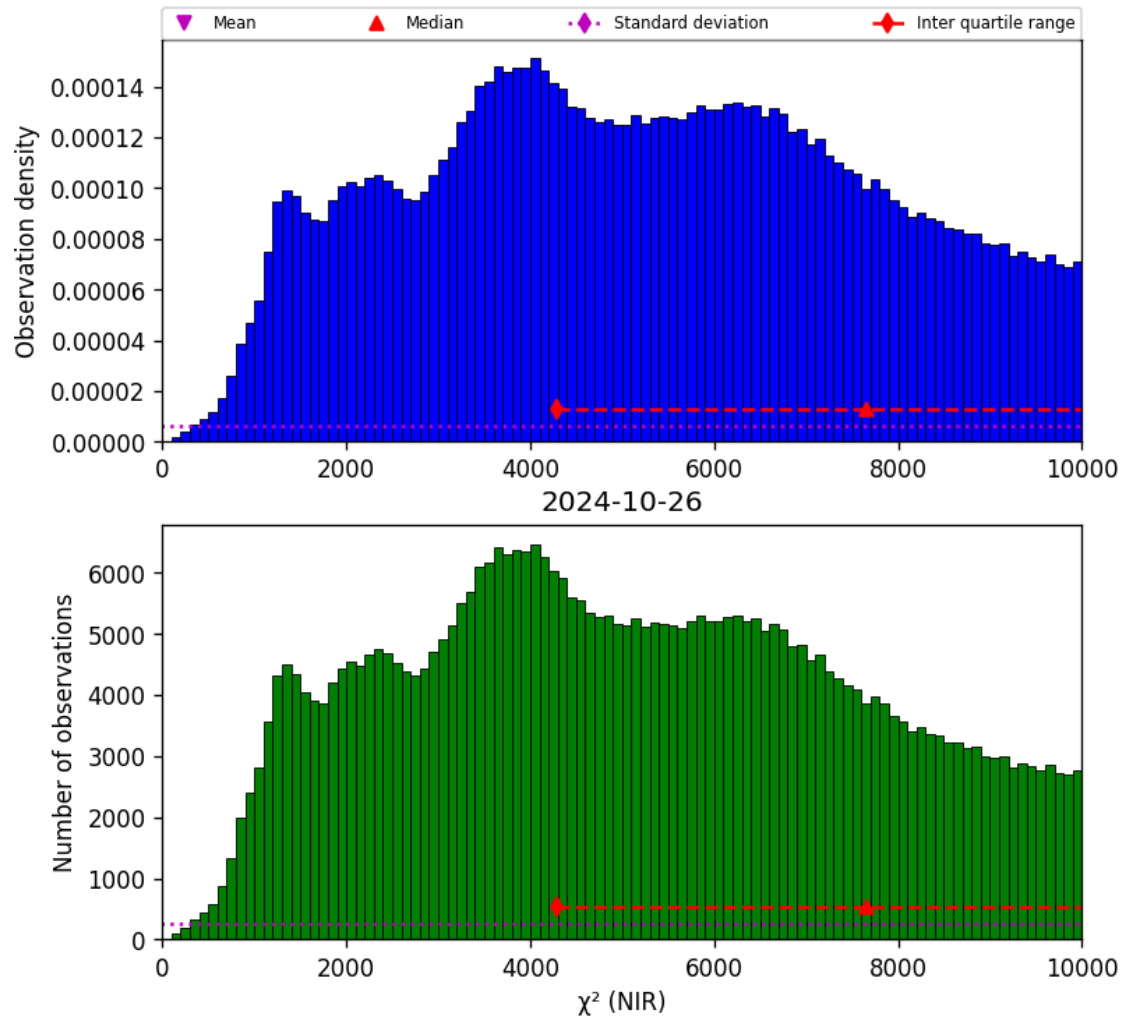
Figure 29: Histogram of “ \chi^2 (NIR)” for 2024-10-25 to 2024-10-27
