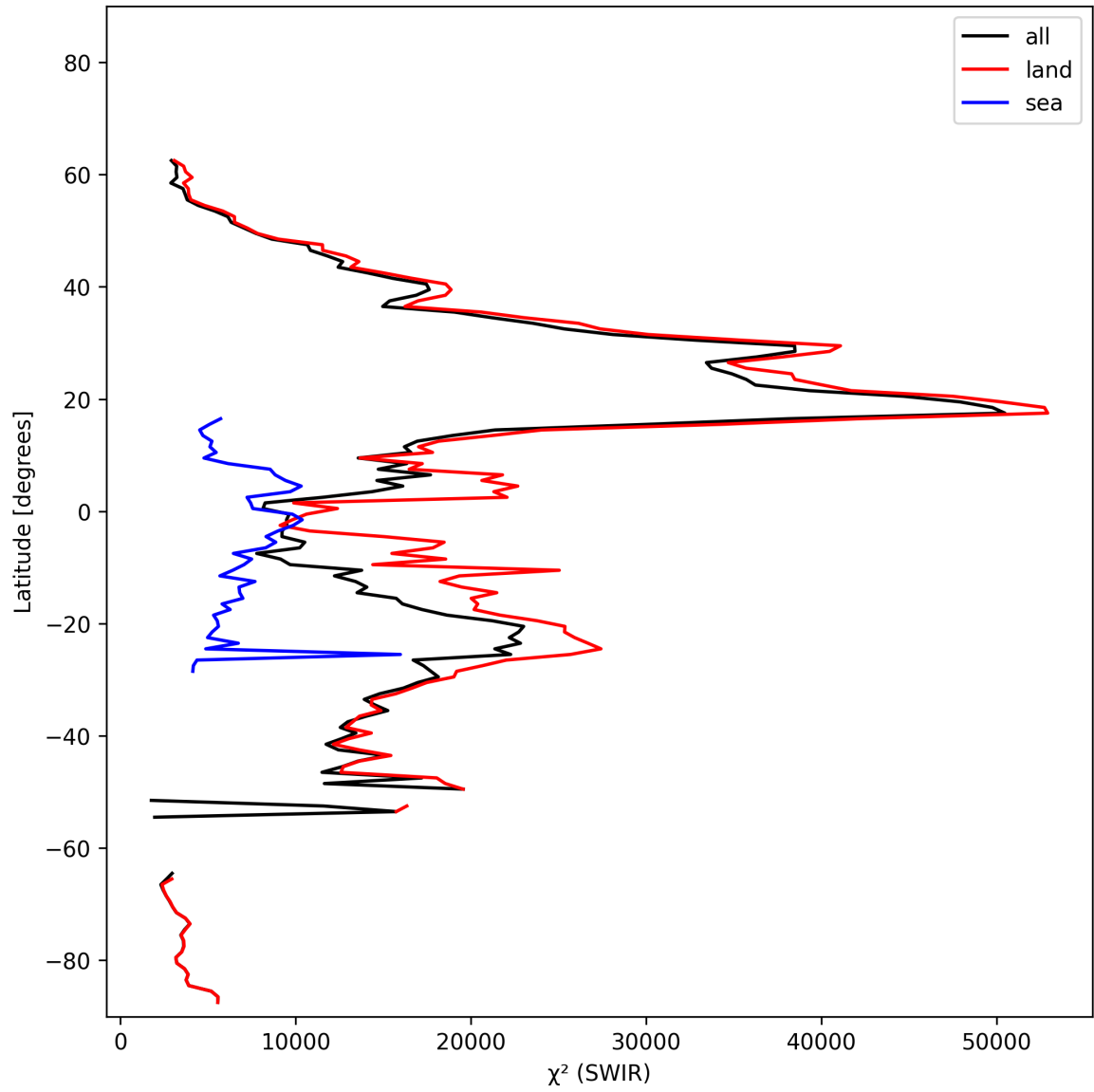
Figure 17: Zonal average of “ \chi^2 (SWIR)” for 2024-10-25 to 2024-10-27.
