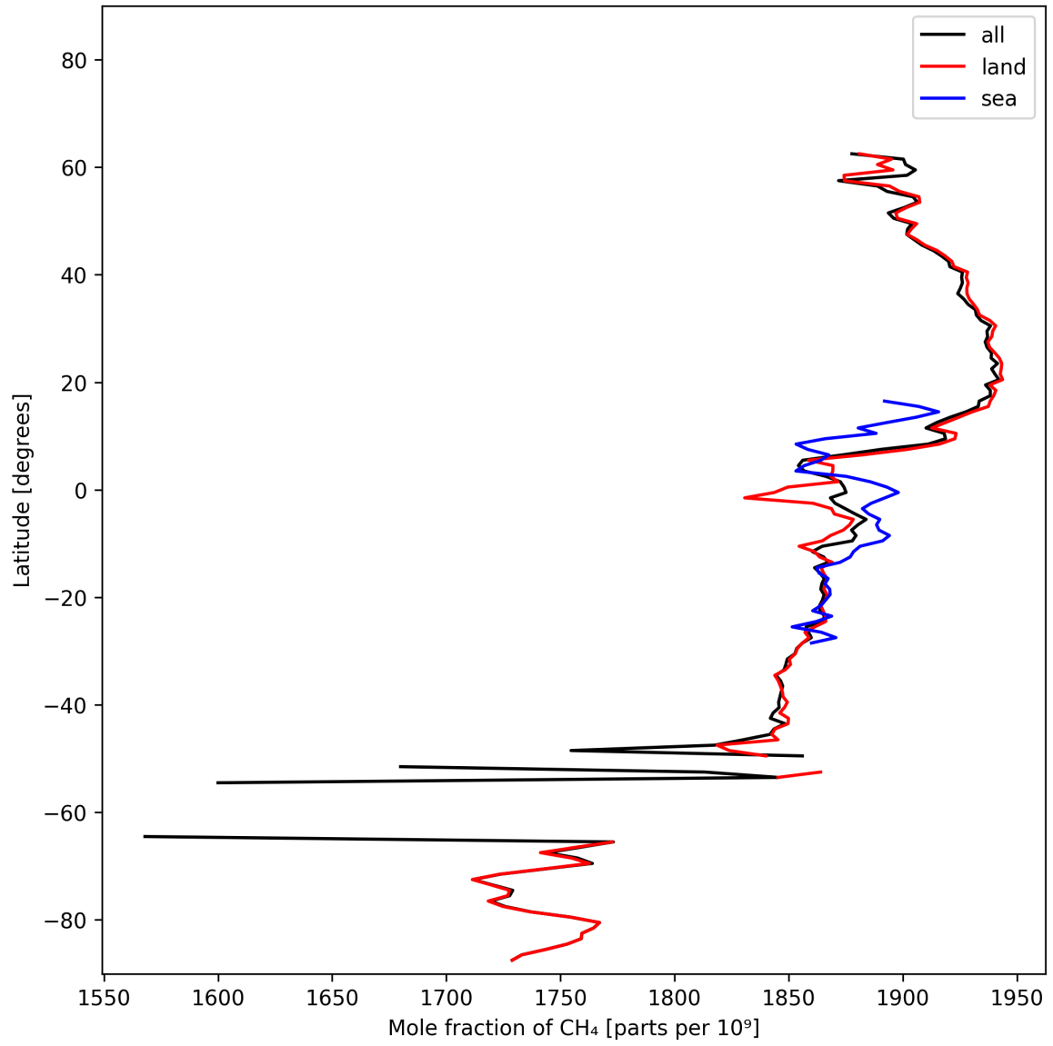
Figure 12: Zonal average of “Mole fraction of CH 4 ” for 2024-10-25 to 2024-10-27.
