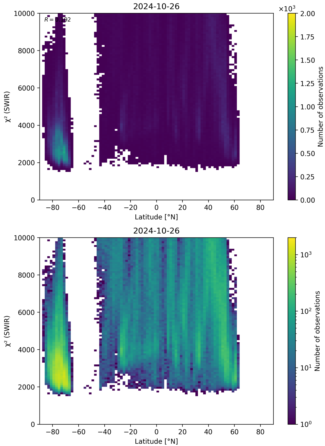
Figure 54: Scatter density plot of “Latitude” against “ \chi^2 (SWIR)” for 2024-10-25 to 2024-10-27.
