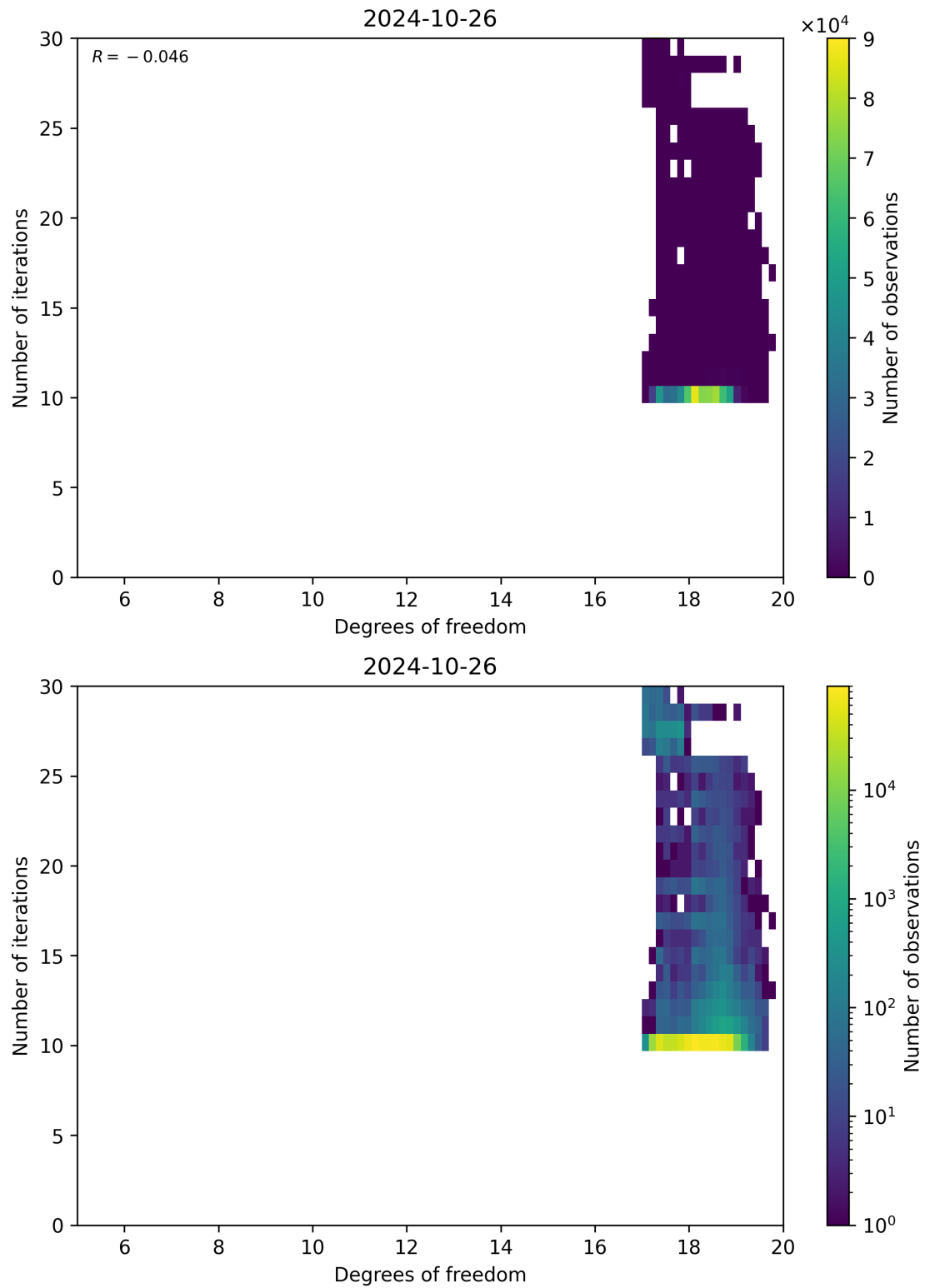
Figure 52: Scatter density plot of “Degrees of freedom” against “Number of iterations” for 2024-10-25 to 2024-10-27.
