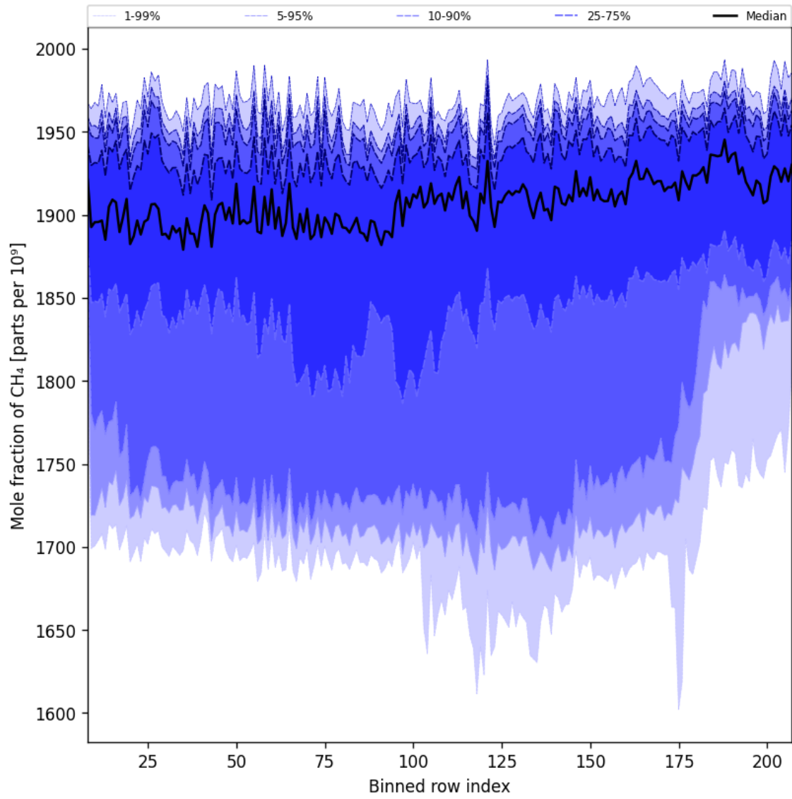
Figure 34: Along track statistics of “Mole fraction of CH 4 ” for 2024-10-25 to 2024-10-27
