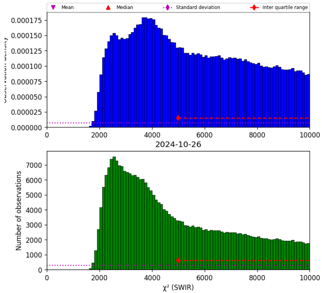
Figure 28: Histogram of “ \chi^2 (SWIR)” for 2024-10-25 to 2024-10-27
