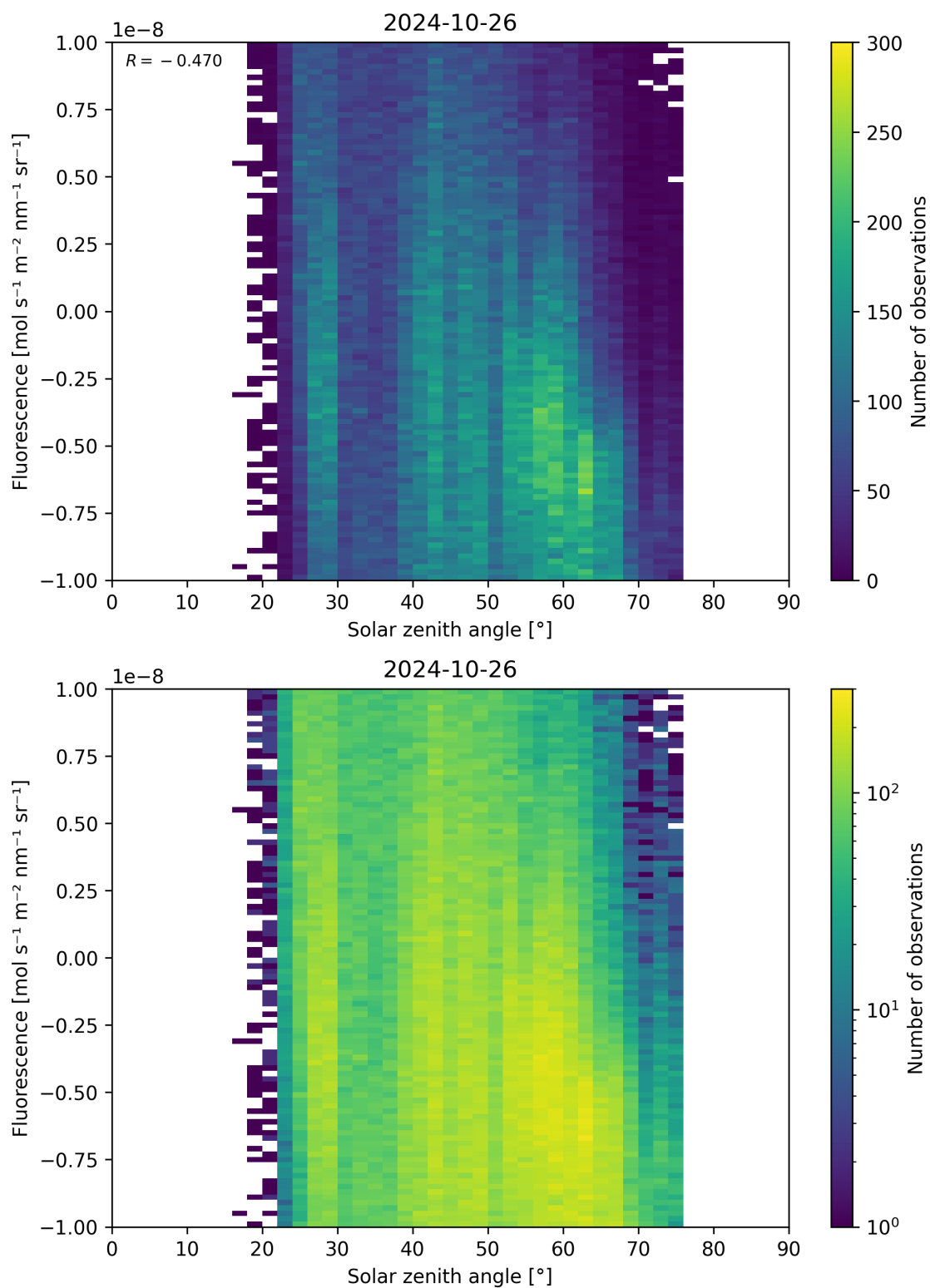
Figure 97: Scatter density plot of “Solar zenith angle” against “Fluorescence” for 2024-10-25 to 2024-10-27.
