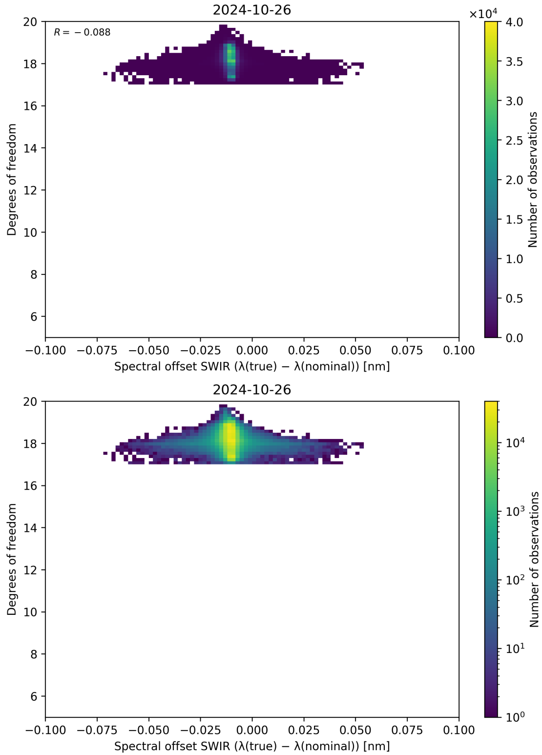
Figure 119: Scatter density plot of “Spectral offset SWIR ( \lambda_{\text{true}} - \lambda_{\text{nominal}} )” against “Degrees of freedom” for 2024-10-25 to 2024-10-27.
