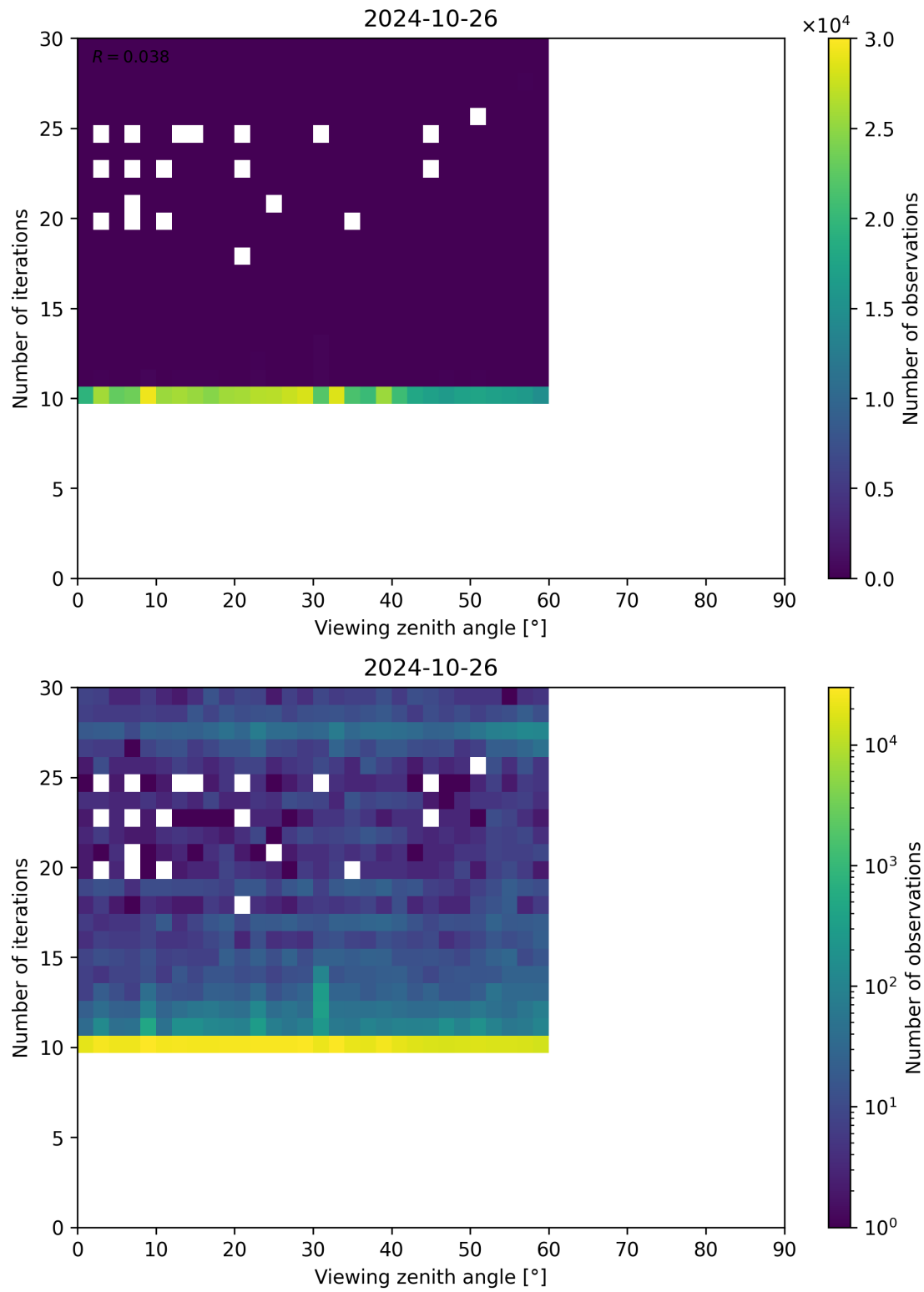
Figure 113: Scatter density plot of “Viewing zenith angle” against “Number of iterations” for 2024-10-25 to 2024-10-27.
