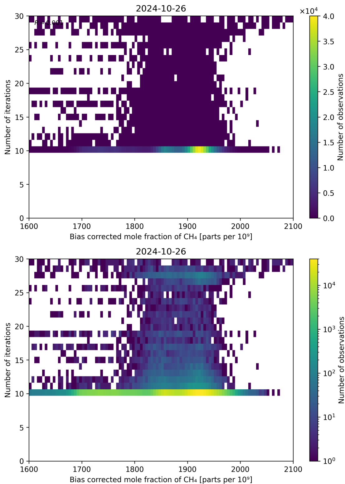
Figure 67: Scatter density plot of “Bias corrected mole fraction of CH 4 ” against “Number of iterations” for 2024-10-25 to 2024-10-27.
