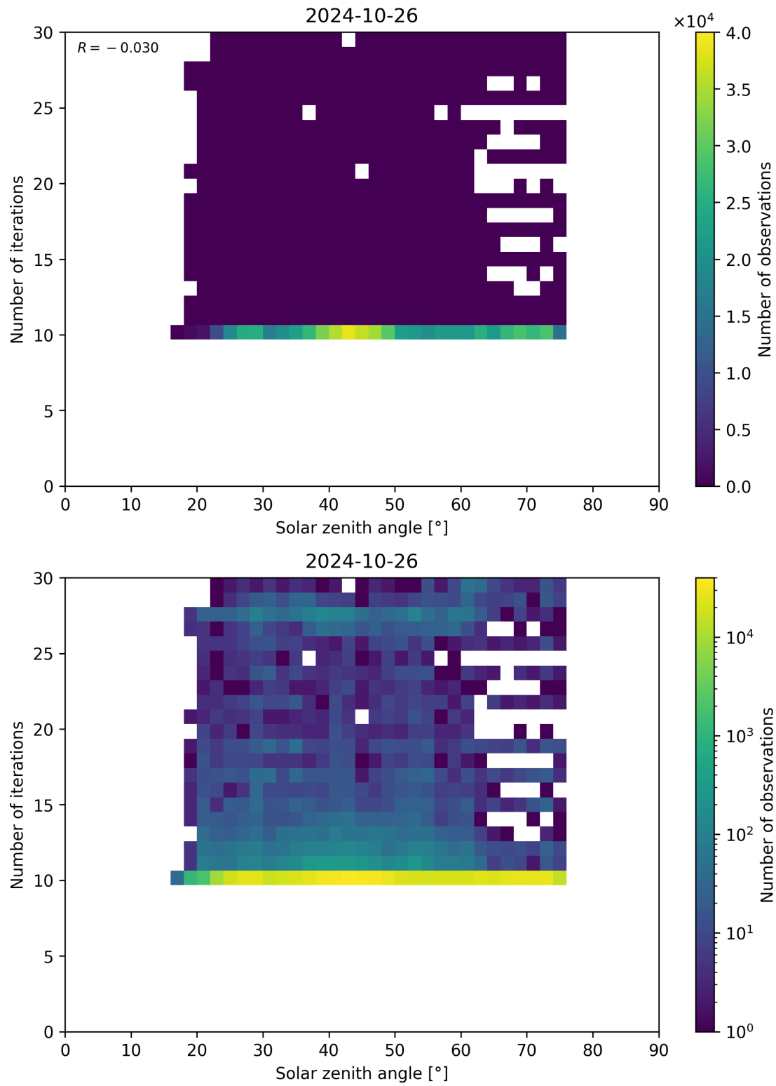
Figure 102: Scatter density plot of “Solar zenith angle” against “Number of iterations” for 2024-10-25 to 2024-10-27.
