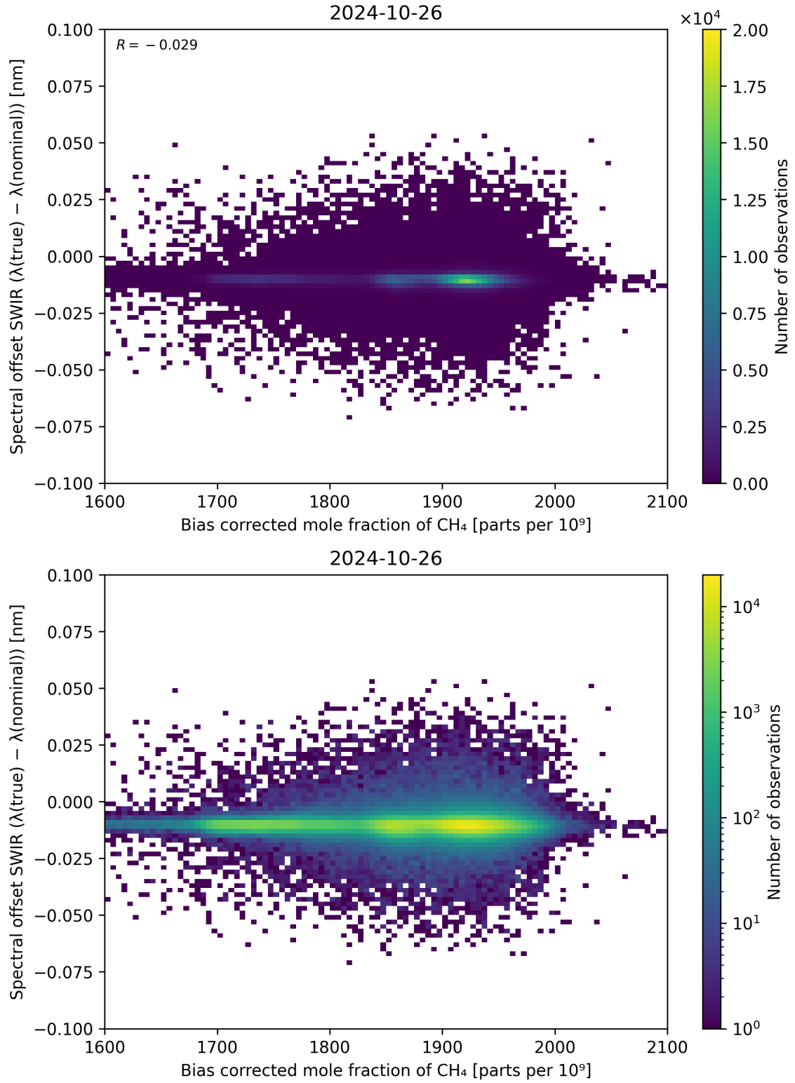
Figure 69: Scatter density plot of “Bias corrected mole fraction of \text{CH}_4 ” against “Spectral offset SWIR ( \lambda_{\text{true}} - \lambda_{\text{nominal}} )” for 2024-10-25 to 2024-10-27.
