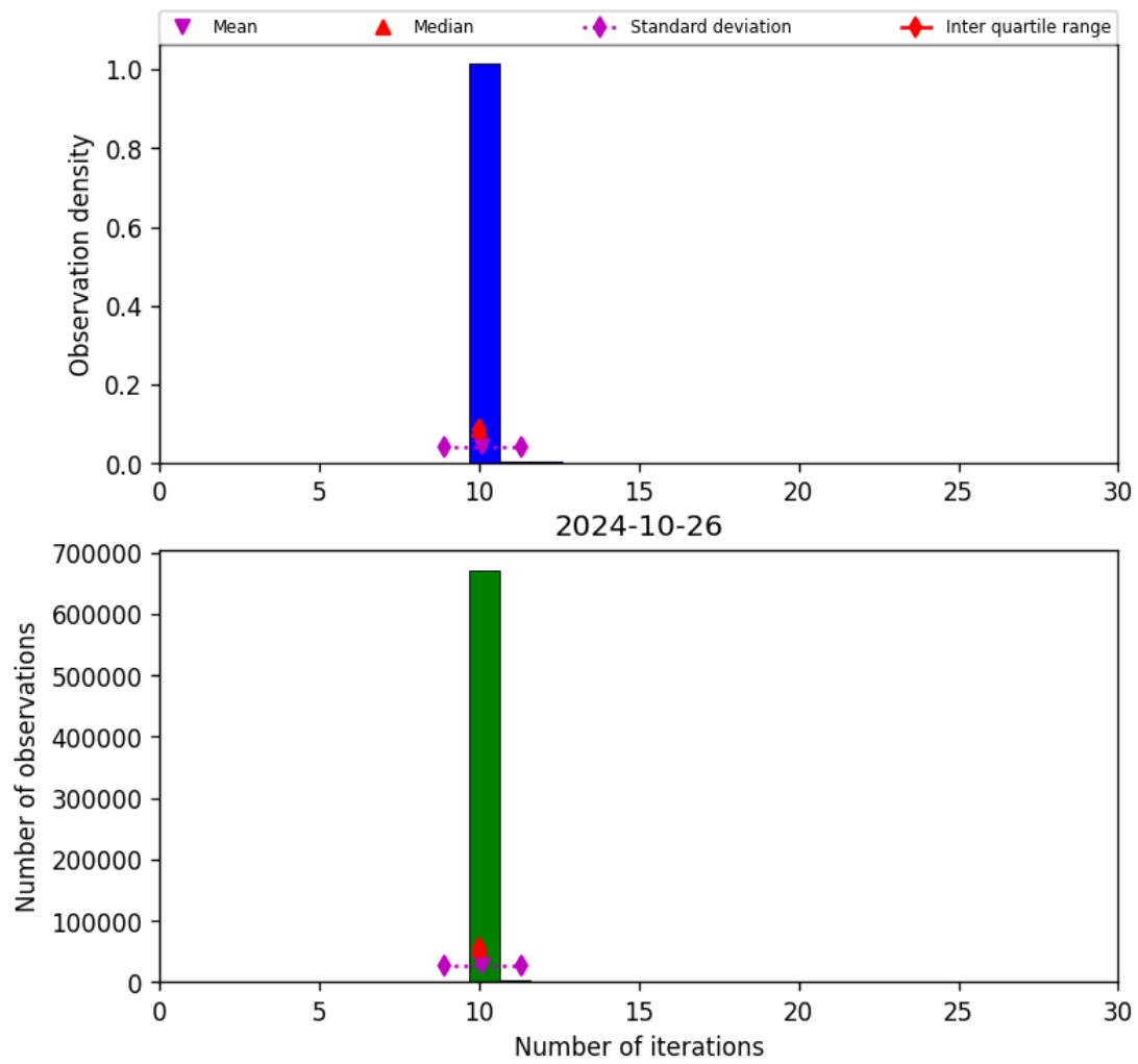
Figure 31: Histogram of “Number of iterations” for 2024-10-25 to 2024-10-27
