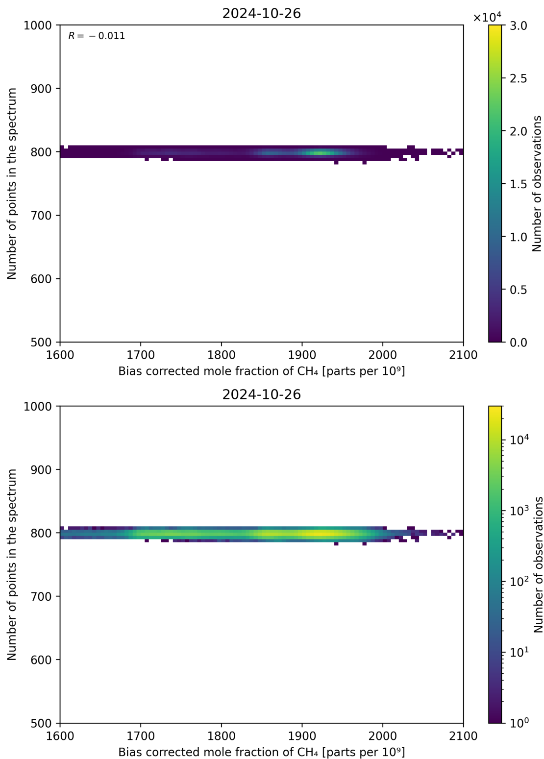
Figure 68: Scatter density plot of “Bias corrected mole fraction of CH 4 ” against “Number of points in the spectrum” for 2024-10-25 to 2024-10-27.
