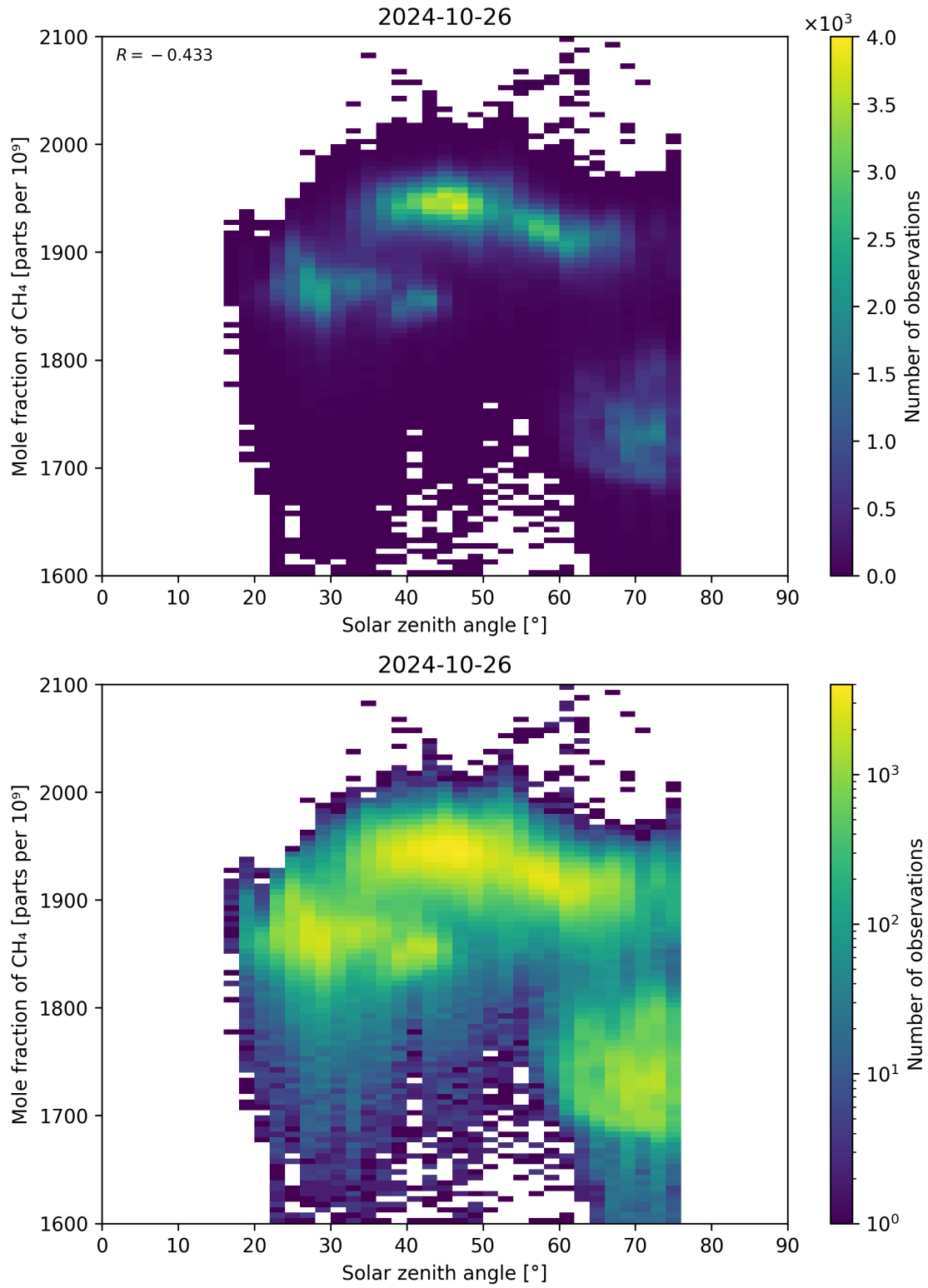
Figure 99: Scatter density plot of “Solar zenith angle” against “Mole fraction of CH 4 ” for 2024-10-25 to 2024-10-27.
