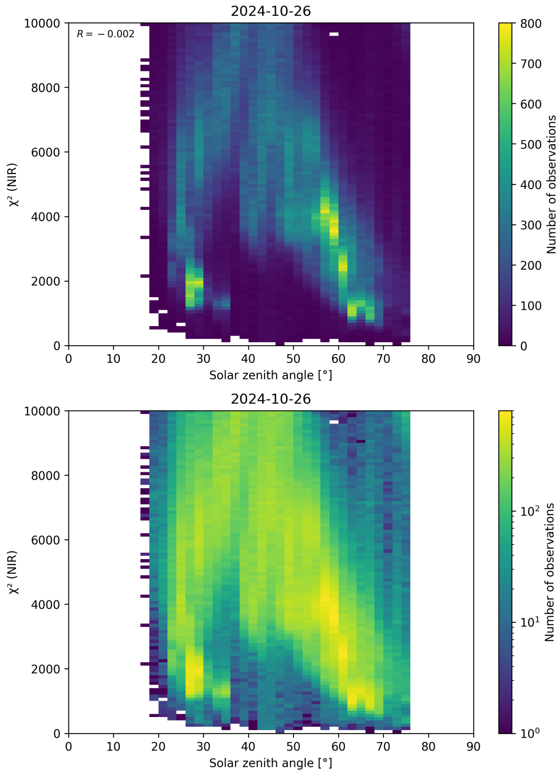
Figure 94: Scatter density plot of “Solar zenith angle” against “ \chi^2 (NIR)” for 2024-10-25 to 2024-10-27.
