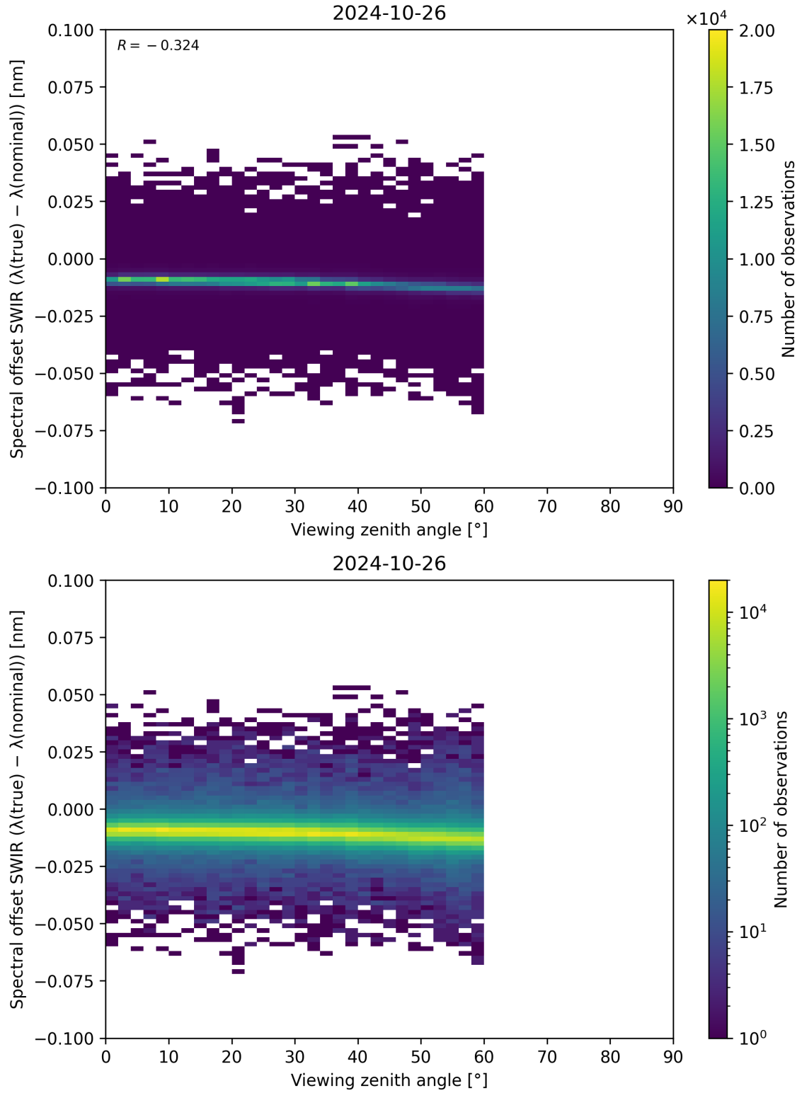
Figure 116: Scatter density plot of “Viewing zenith angle” against “Spectral offset SWIR ( \lambda_{\text{true}} - \lambda_{\text{nominal}} )” for 2024-10-25 to 2024-10-27.
