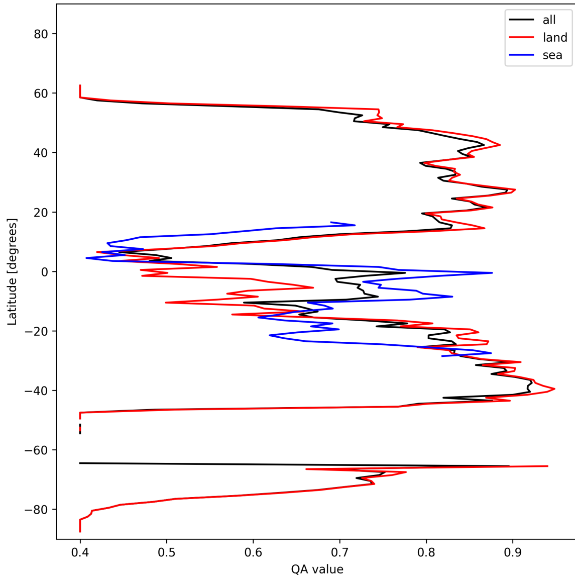
Figure 11: Zonal average of “QA value” for 2024-10-25 to 2024-10-27.
