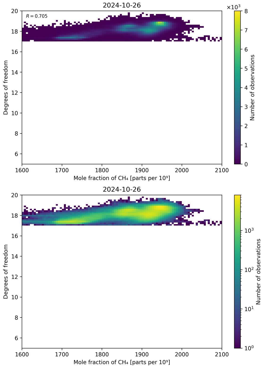
Figure 72: Scatter density plot of “Mole fraction of CH 4 ” against “Degrees of freedom” for 2024-10-25 to 2024-10-27.
