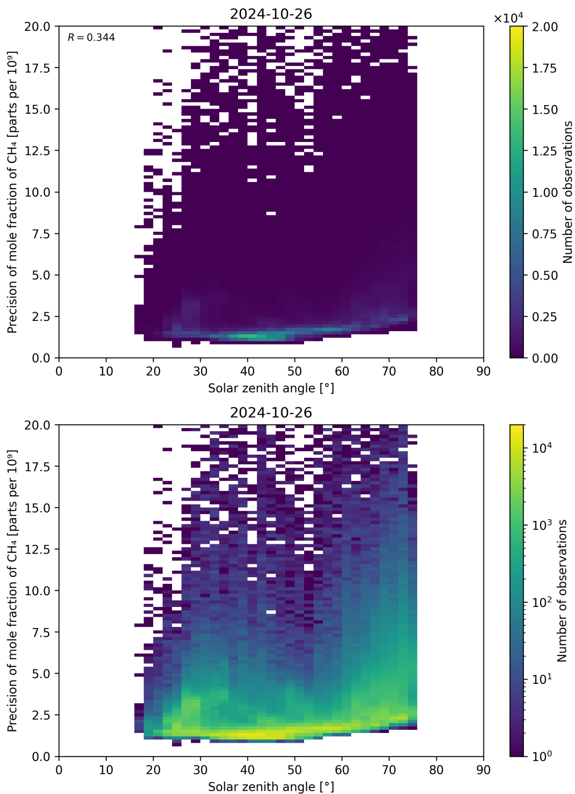
Figure 101: Scatter density plot of “Solar zenith angle” against “Precision of mole fraction of CH 4 ” for 2024-10-25 to 2024-10-27.
