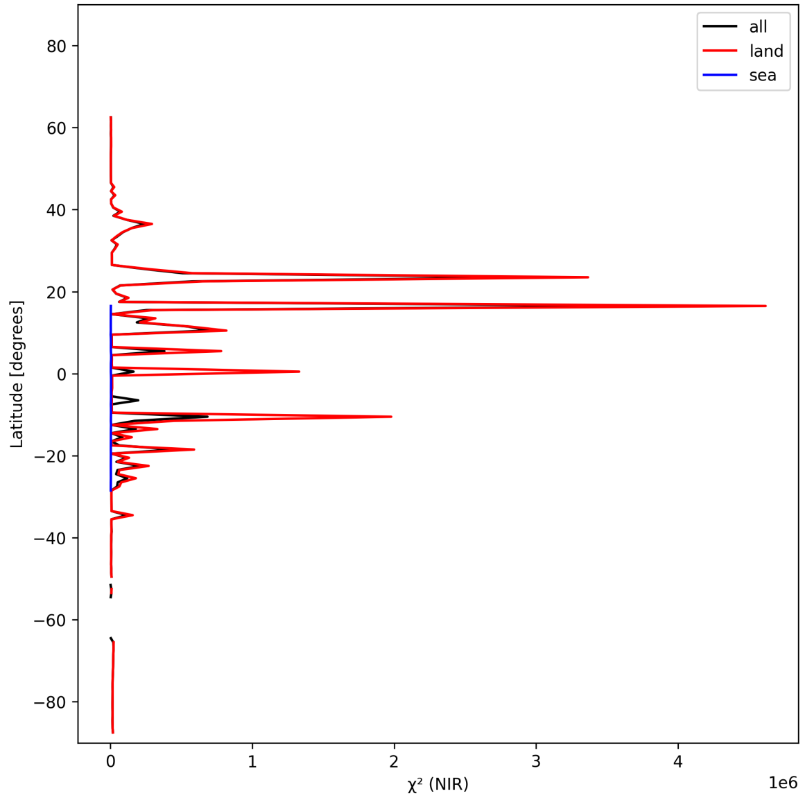
Figure 18: Zonal average of “ \chi^2 (NIR)” for 2024-10-25 to 2024-10-27.
