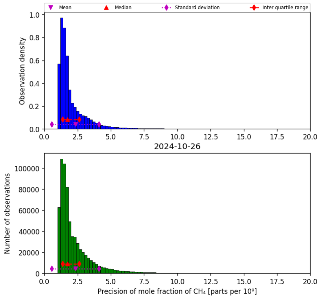
Figure 24: Histogram of “Precision of mole fraction of CH 4 ” for 2024-10-25 to 2024-10-27
