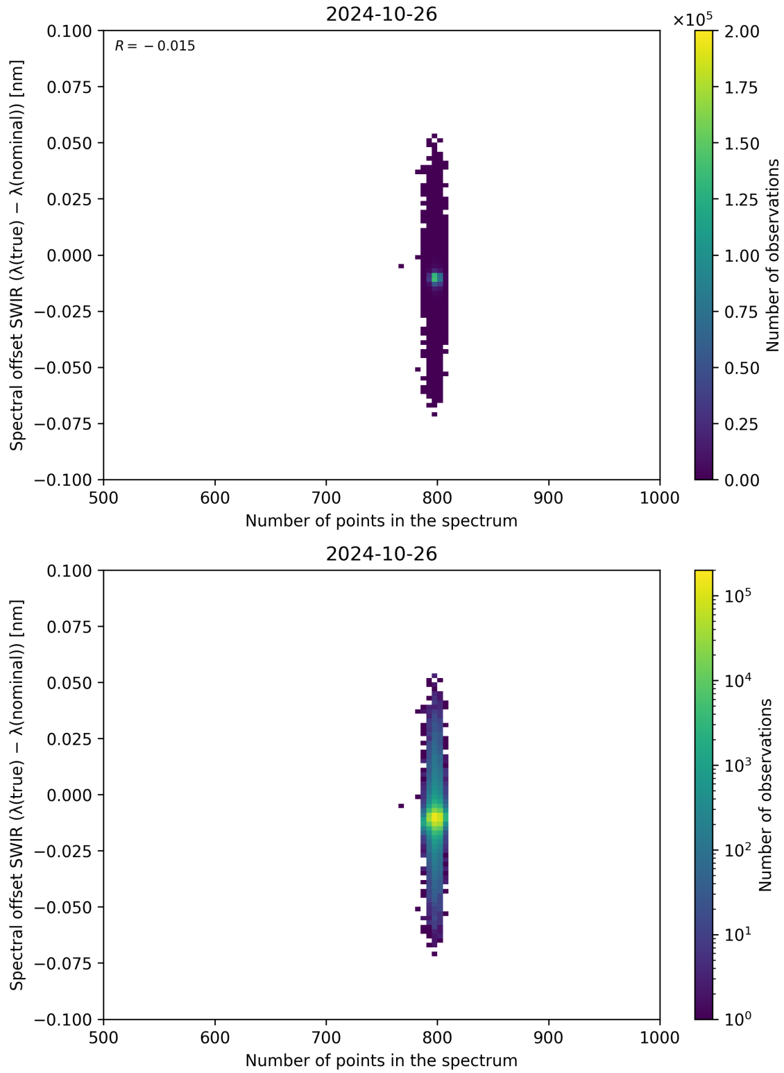
Figure 93: Scatter density plot of “Number of points in the spectrum” against “Spectral offset SWIR ( \lambda_{\text{true}} - \lambda_{\text{nominal}} )” for 2024-10-25 to 2024-10-27.
