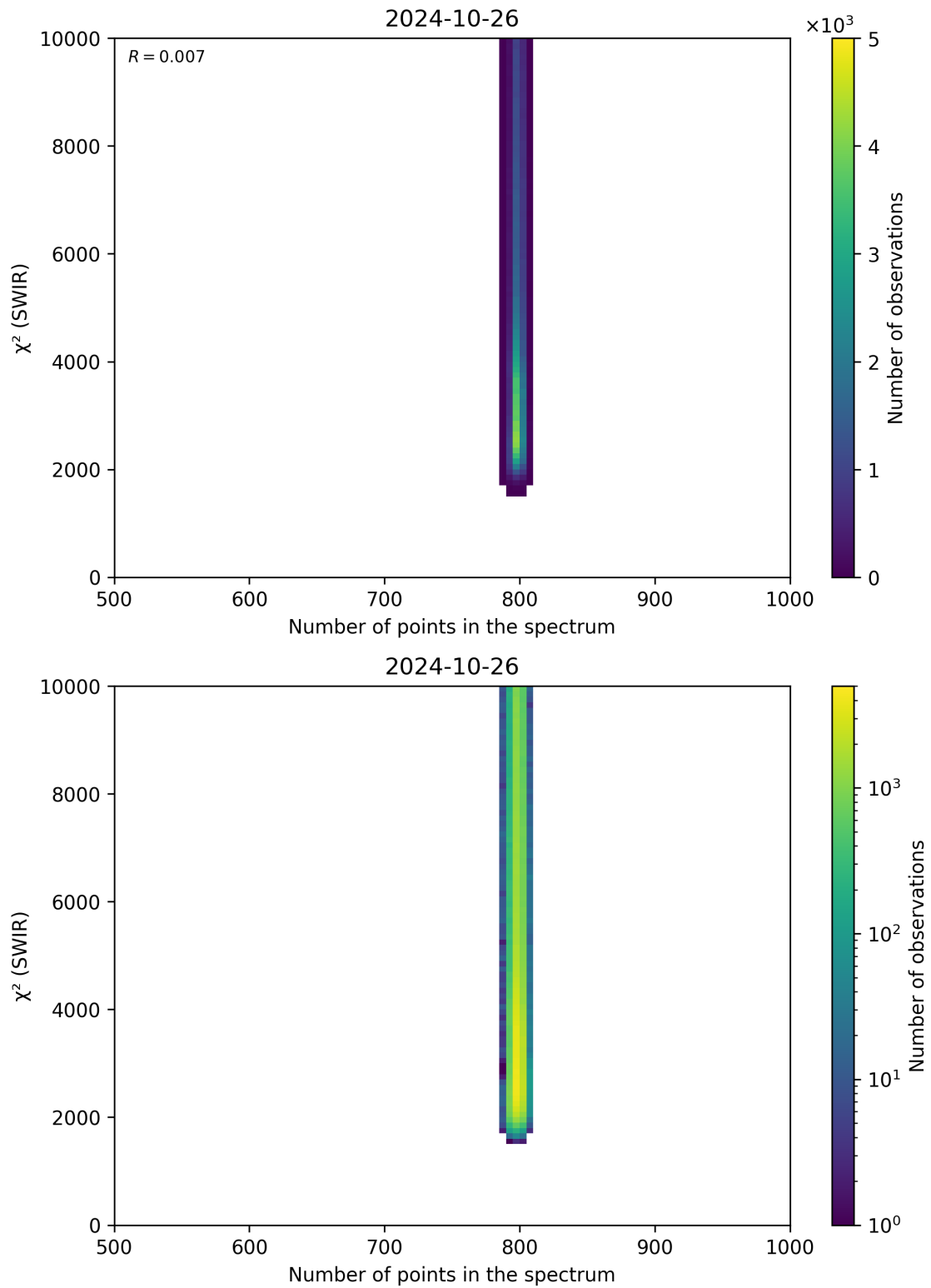
Figure 89: Scatter density plot of “Number of points in the spectrum” against “ \chi^2 (SWIR)” for 2024-10-25 to 2024-10-27.
