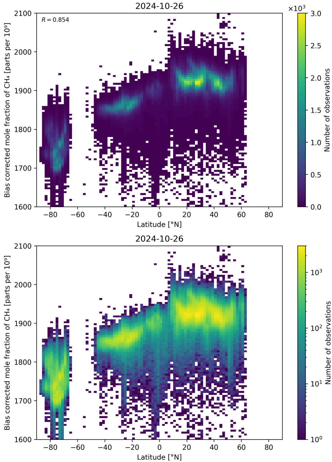
Figure 58: Scatter density plot of “Latitude” against “Bias corrected mole fraction of CH 4 ” for 2024-10-25 to 2024-10-27.
