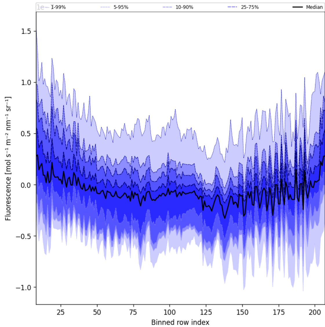
Figure 43: Along track statistics of “Fluorescence” for 2024-10-25 to 2024-10-27
