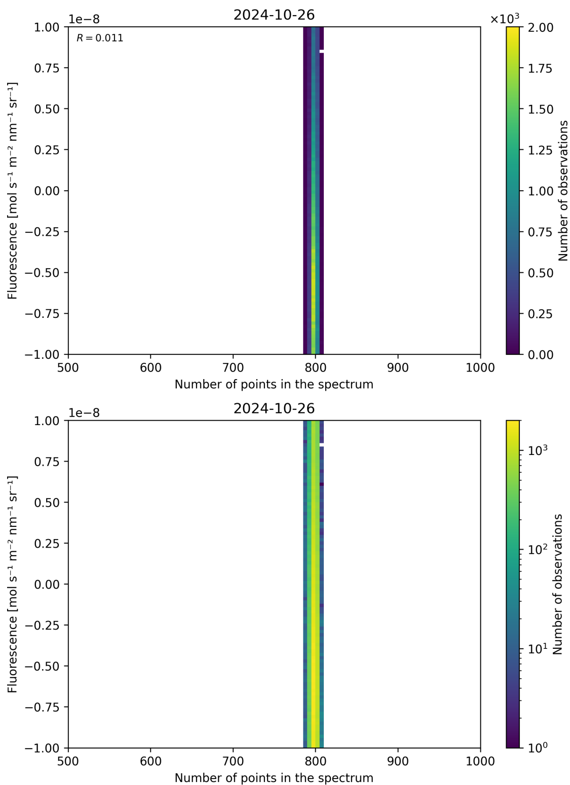
Figure 91: Scatter density plot of “Number of points in the spectrum” against “Fluorescence” for 2024-10-25 to 2024-10-27.
