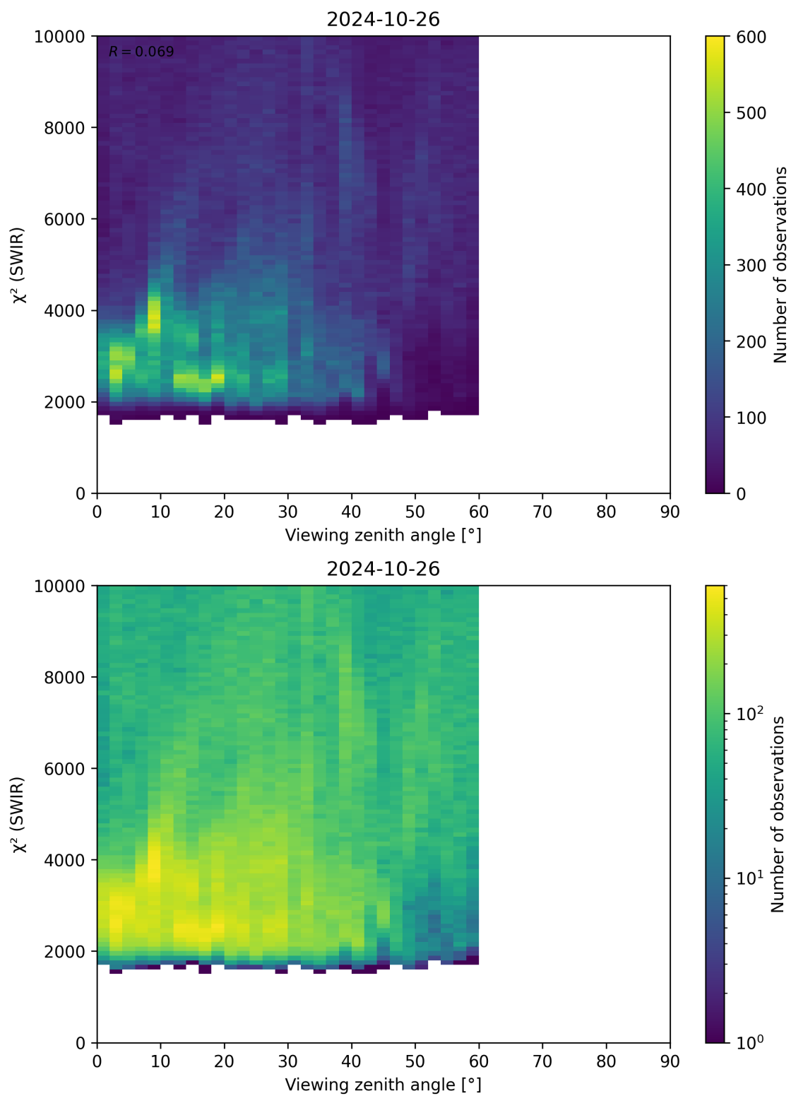
Figure 106: Scatter density plot of “Viewing zenith angle” against “ \chi^2 (SWIR)” for 2024-10-25 to 2024-10-27.
