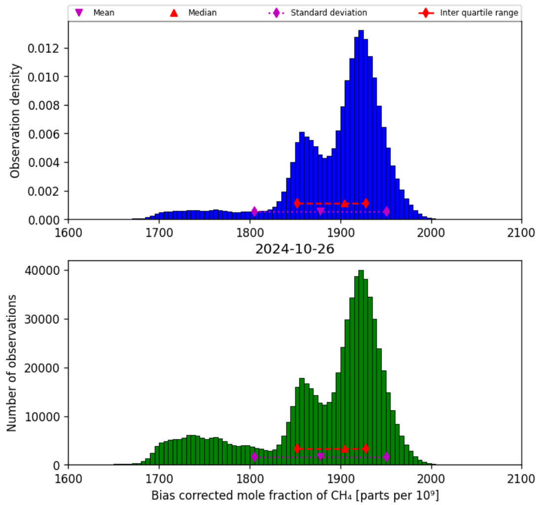
Figure 25: Histogram of “Bias corrected mole fraction of CH 4 ” for 2024-10-25 to 2024-10-27
