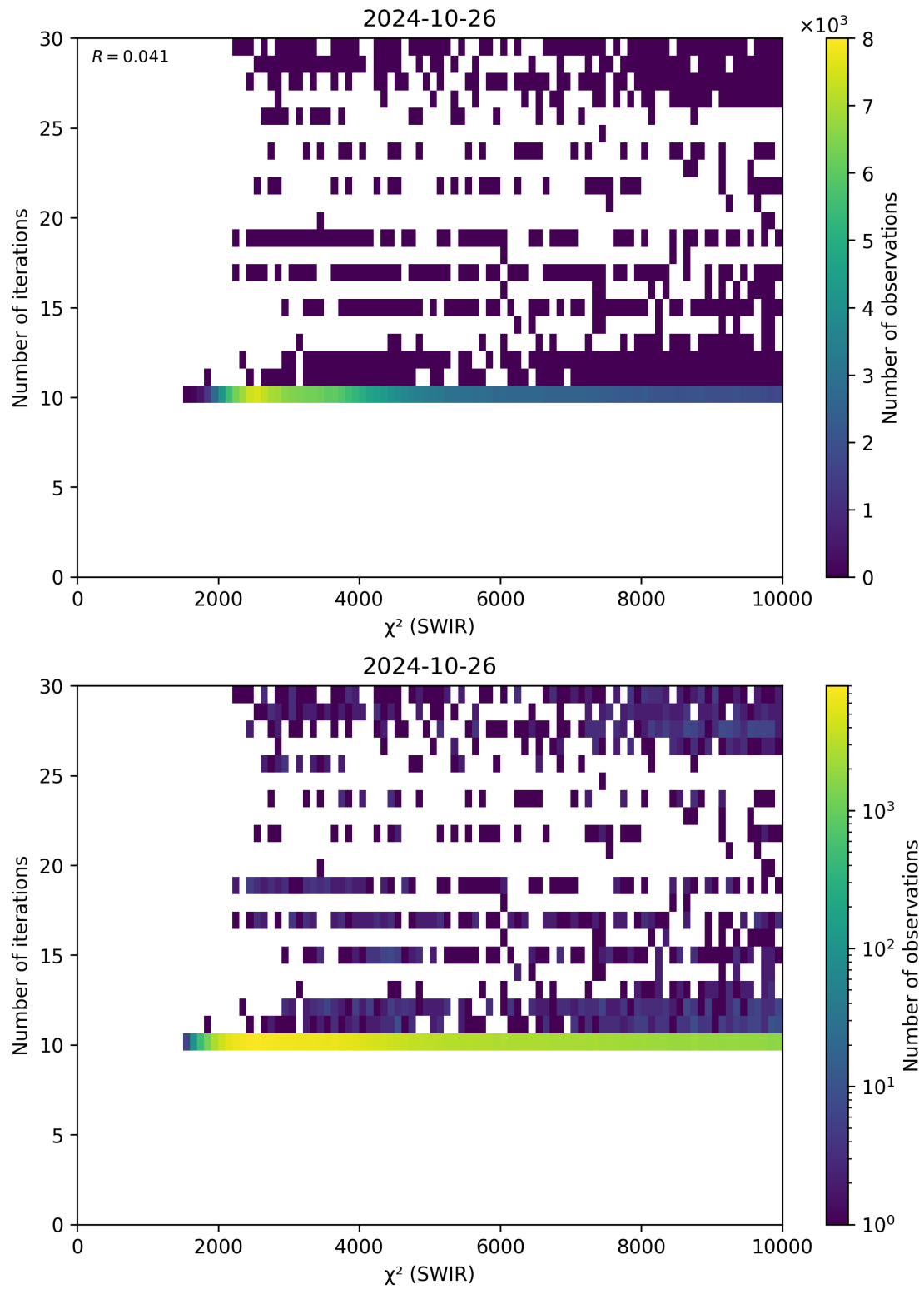
Figure 50: Scatter density plot of “ \chi^2 (SWIR)” against “Number of iterations” for 2024-10-25 to 2024-10-27.
