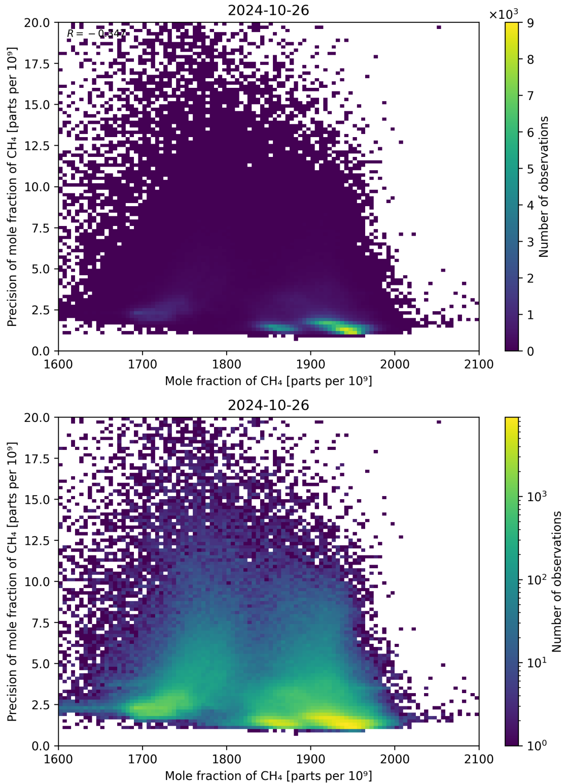
Figure 75: Scatter density plot of “Mole fraction of CH 4 ” against “Precision of mole fraction of CH 4 ” for 2024-10-25 to 2024-10-27.
