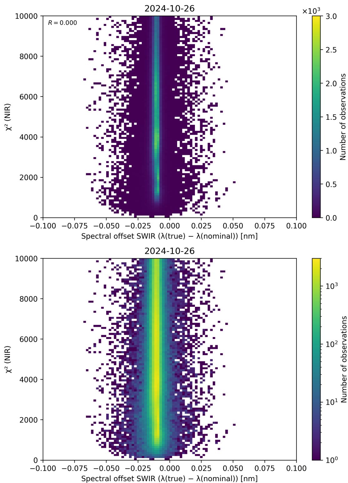
Figure 117: Scatter density plot of “Spectral offset SWIR ( \lambda_{\text{true}} - \lambda_{\text{nominal}} )” against “ \chi^2 (NIR)” for 2024-10-25 to 2024-10-27.
