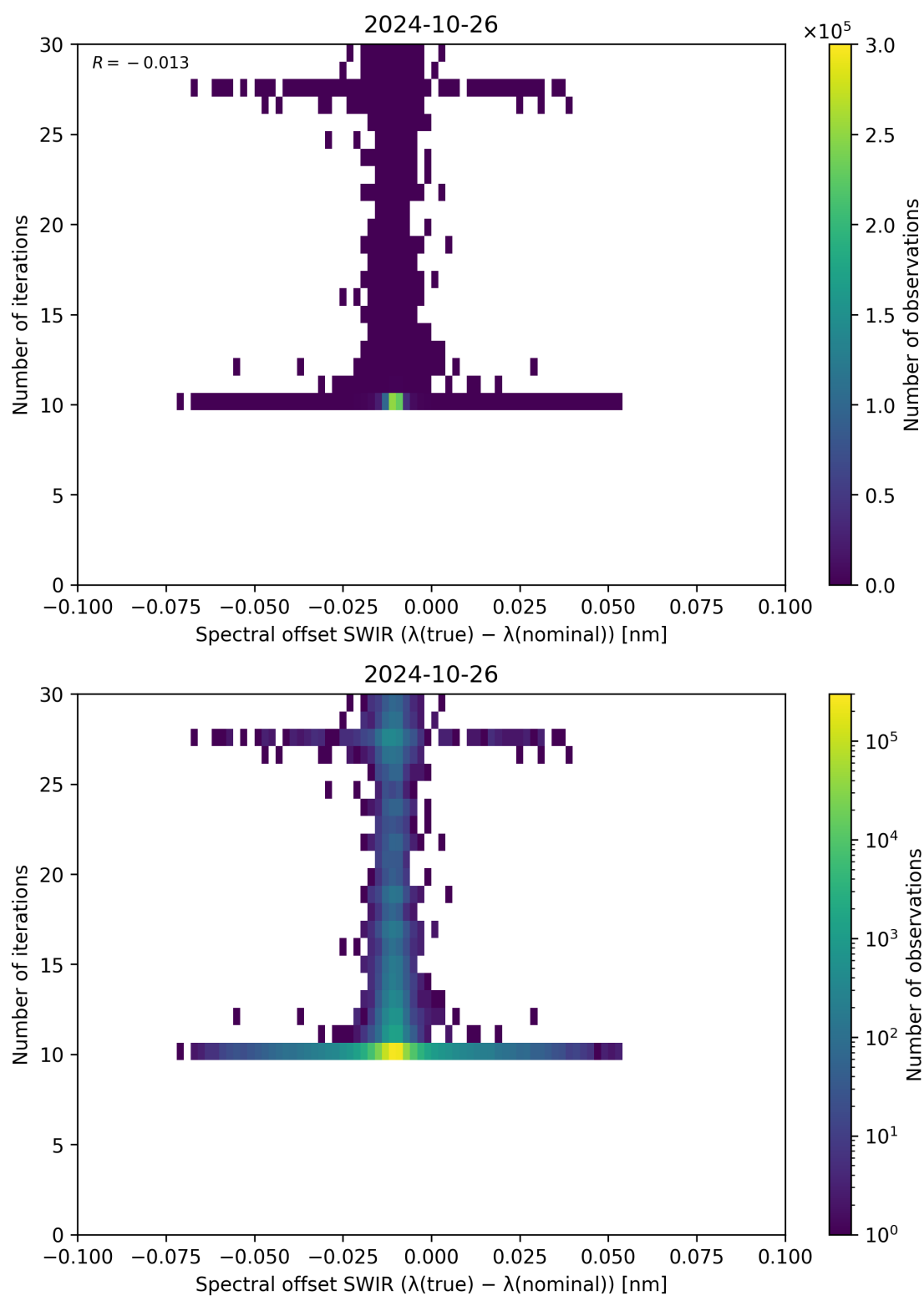
Figure 121: Scatter density plot of “Spectral offset SWIR ( \lambda_{\text{true}} - \lambda_{\text{nominal}} )” against “Number of iterations” for 2024-10-25 to 2024-10-27.
