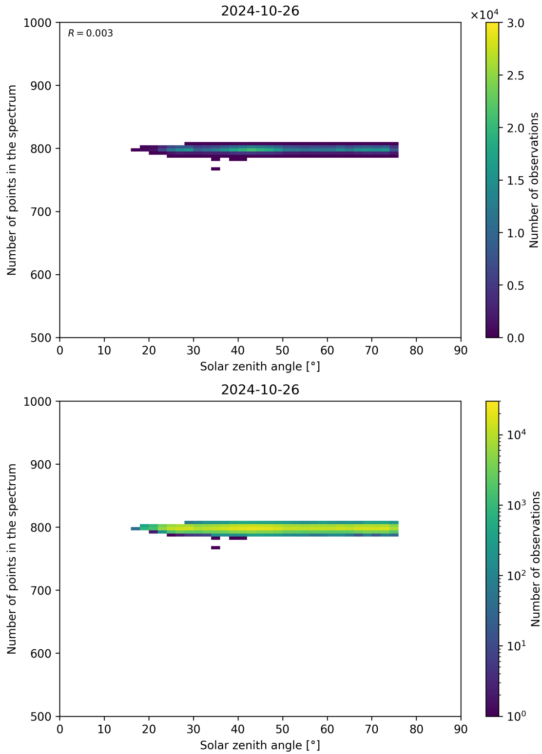
Figure 103: Scatter density plot of “Solar zenith angle” against “Number of points in the spectrum” for 2024-10-25 to 2024-10-27.
