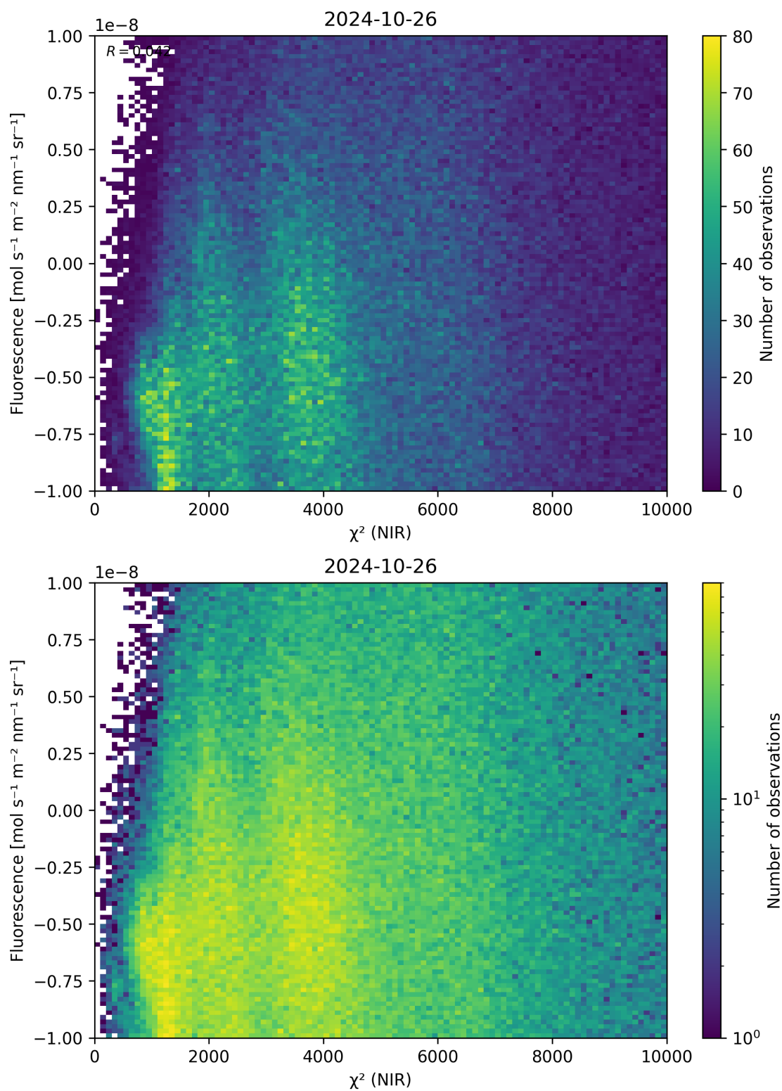
Figure 45: Scatter density plot of “ \chi^2 (NIR)” against “Fluorescence” for 2024-10-25 to 2024-10-27.
