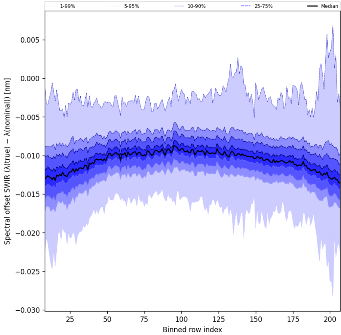
Figure 38: Along track statistics of “Spectral offset SWIR ( \lambda_{\text{true}} - \lambda_{\text{nominal}} )” for 2024-10-25 to 2024-10-27
