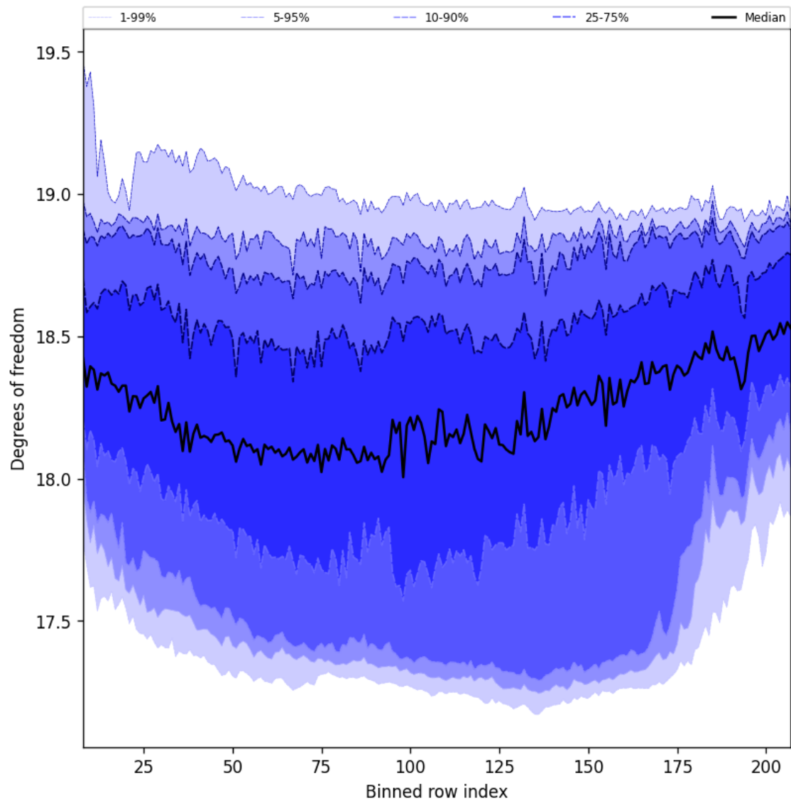
Figure 41: Along track statistics of “Degrees of freedom” for 2024-10-25 to 2024-10-27
