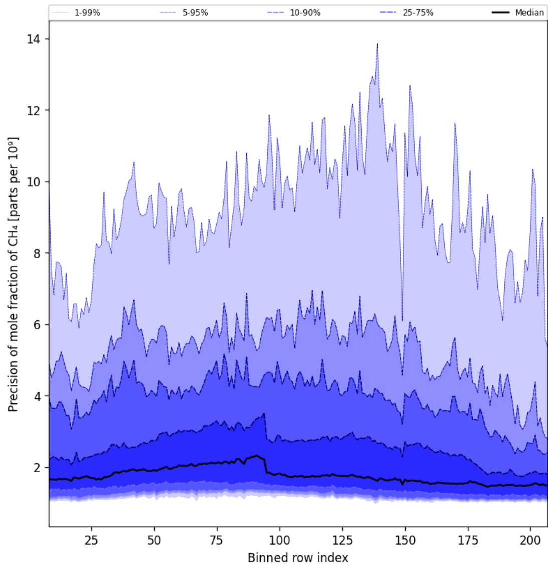
Figure 35: Along track statistics of “Precision of mole fraction of CH 4 ” for 2024-10-25 to 2024-10-27
