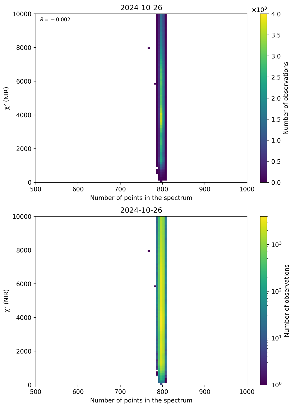
Figure 88: Scatter density plot of “Number of points in the spectrum” against “ \chi^2 (NIR)” for 2024-10-25 to 2024-10-27.
