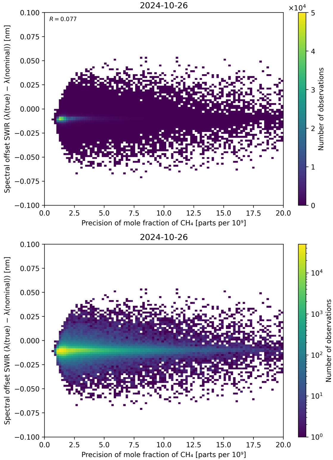
Figure 85: Scatter density plot of “Precision of mole fraction of \text{CH}_4 ” against “Spectral offset SWIR ( \lambda_{\text{true}} - \lambda_{\text{nominal}} )” for 2024-10-25 to 2024-10-27.
