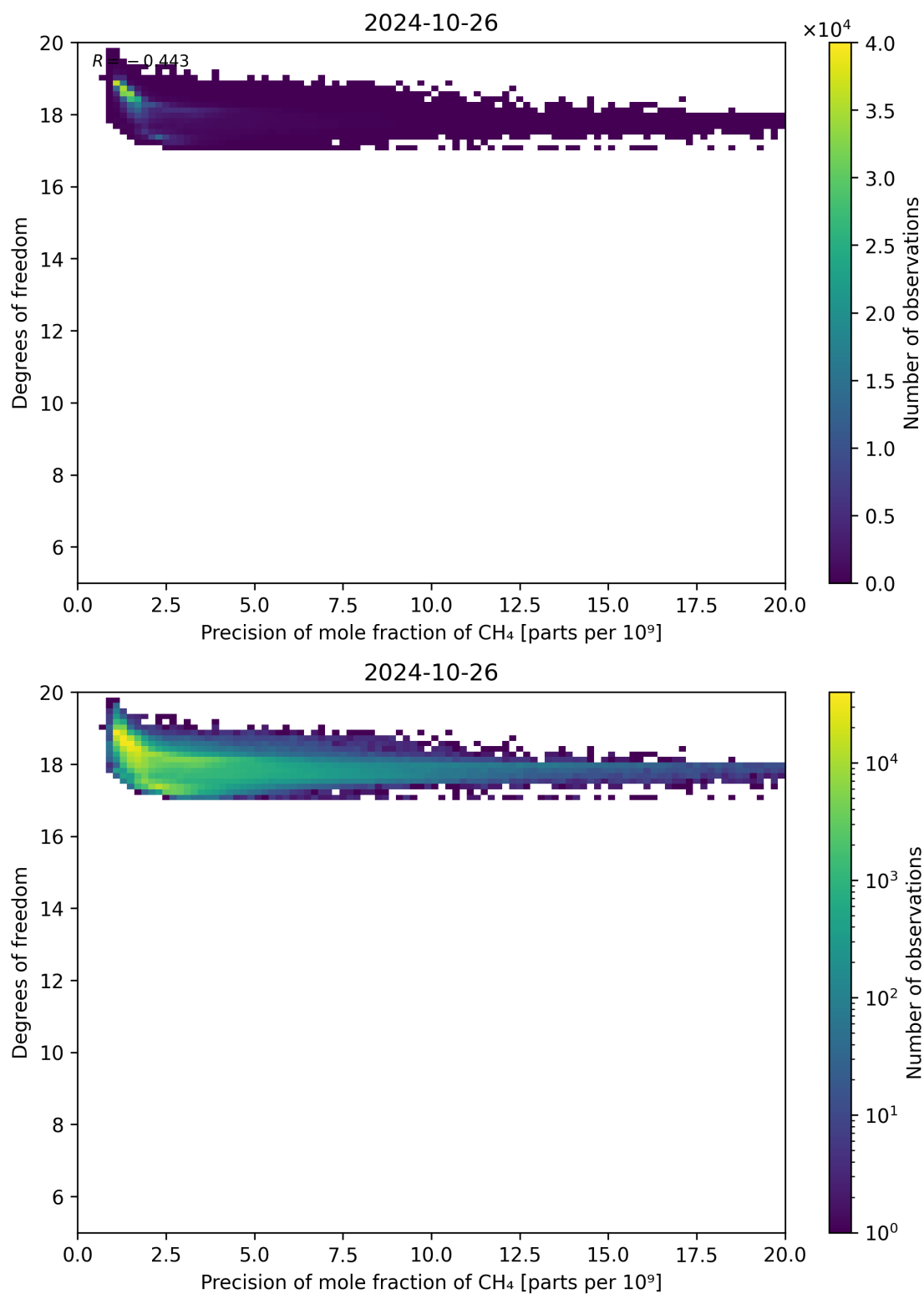
Figure 80: Scatter density plot of “Precision of mole fraction of CH 4 ” against “Degrees of freedom” for 2024-10-25 to 2024-10-27.
