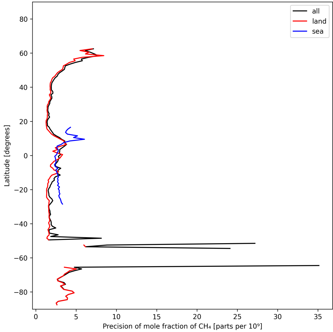
Figure 13: Zonal average of “Precision of mole fraction of CH 4 ” for 2024-10-25 to 2024-10-27.
