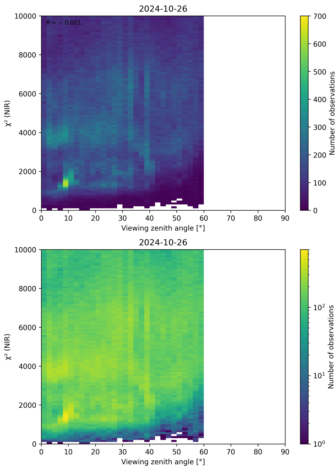
Figure 105: Scatter density plot of “Viewing zenith angle” against “ \chi^2 (NIR)” for 2024-10-25 to 2024-10-27.
