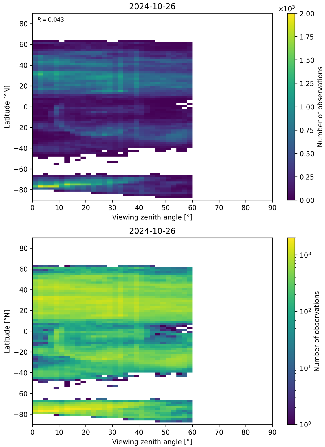
Figure 109: Scatter density plot of “Viewing zenith angle” against “Latitude” for 2024-10-25 to 2024-10-27.
