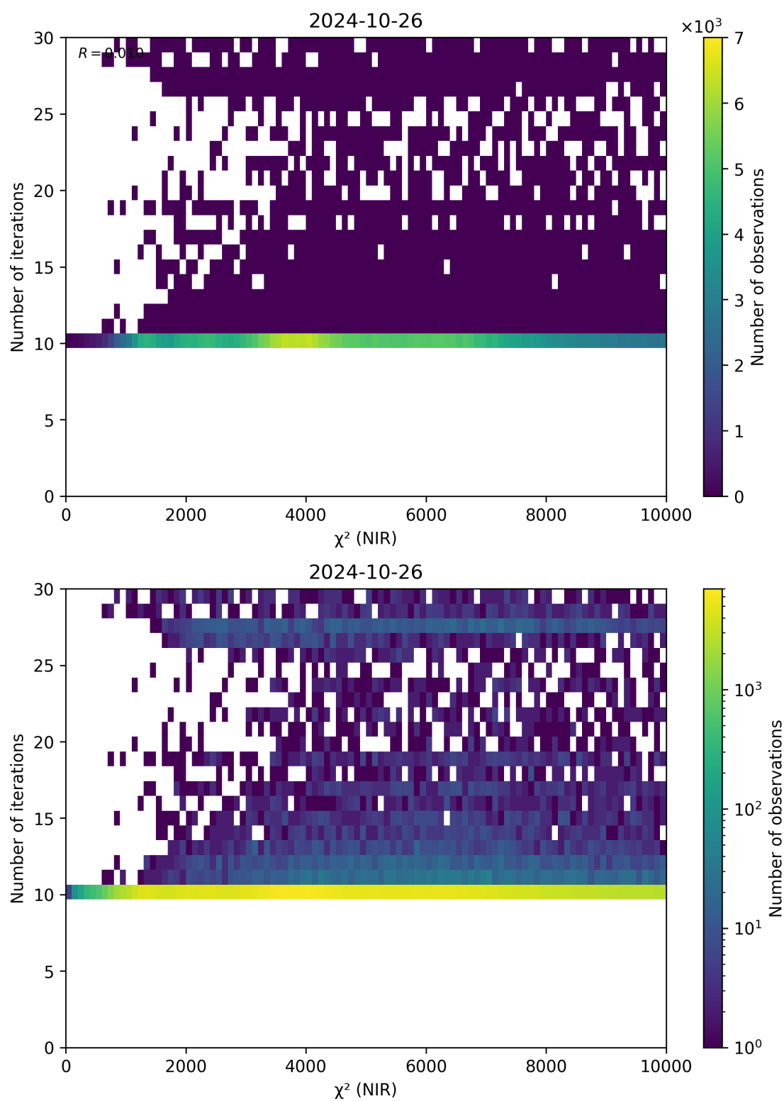
Figure 46: Scatter density plot of “ \chi^2 (NIR)” against “Number of iterations” for 2024-10-25 to 2024-10-27.
