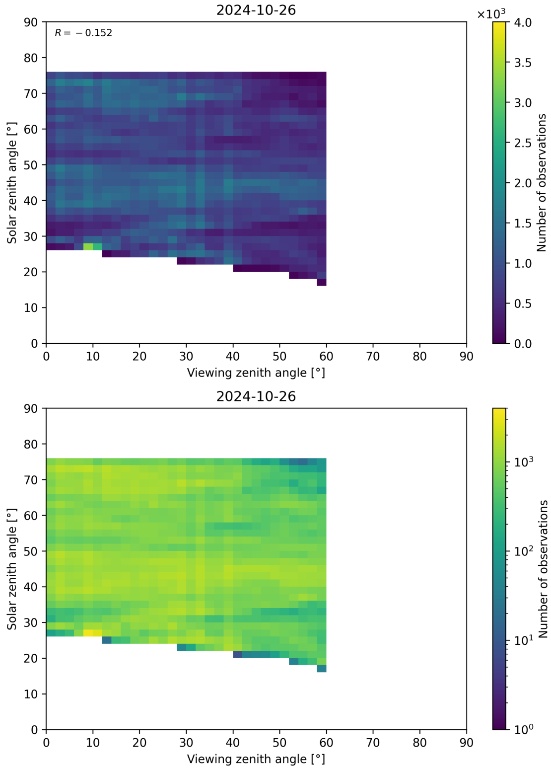
Figure 115: Scatter density plot of “Viewing zenith angle” against “Solar zenith angle” for 2024-10-25 to 2024-10-27.
