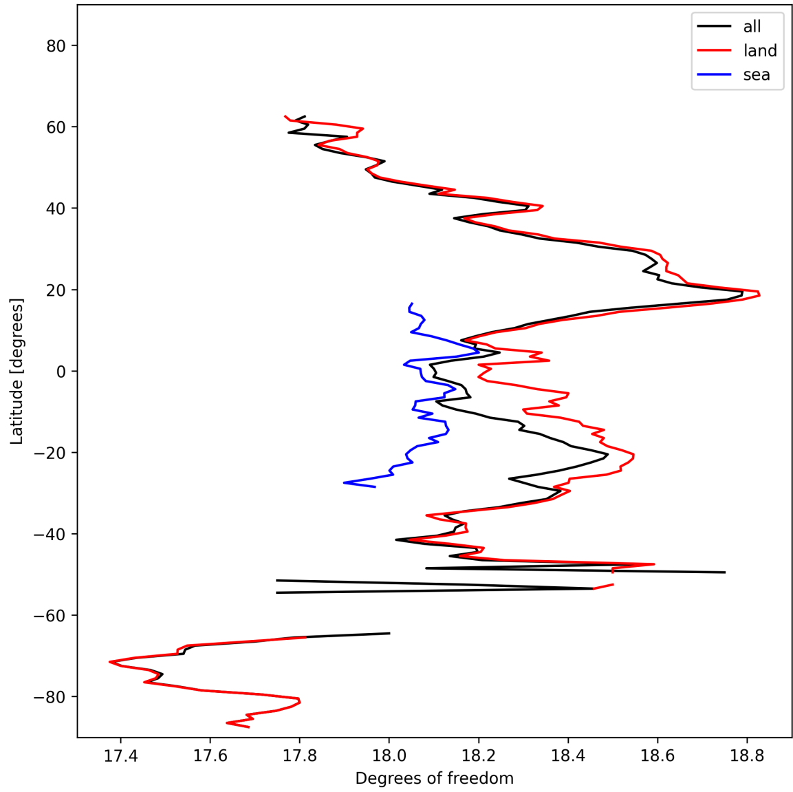
Figure 19: Zonal average of “Degrees of freedom” for 2024-10-25 to 2024-10-27.
