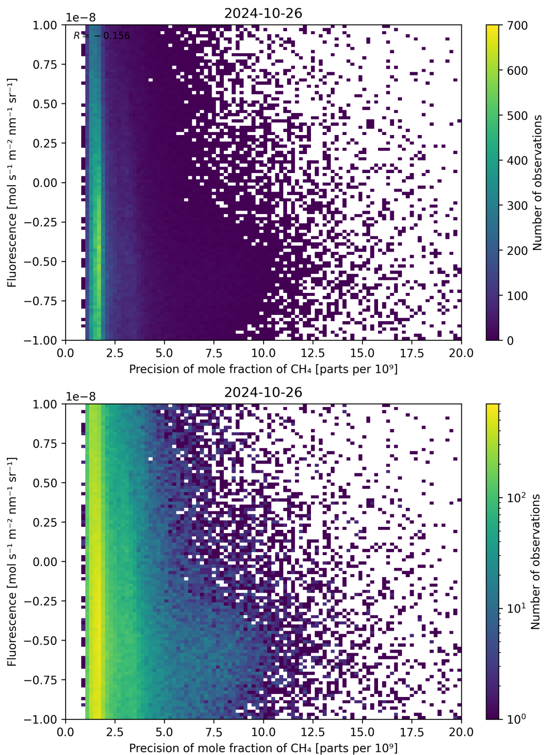
Figure 81: Scatter density plot of “Precision of mole fraction of \text{CH}_4 ” against “Fluorescence” for 2024-10-25 to 2024-10-27.
