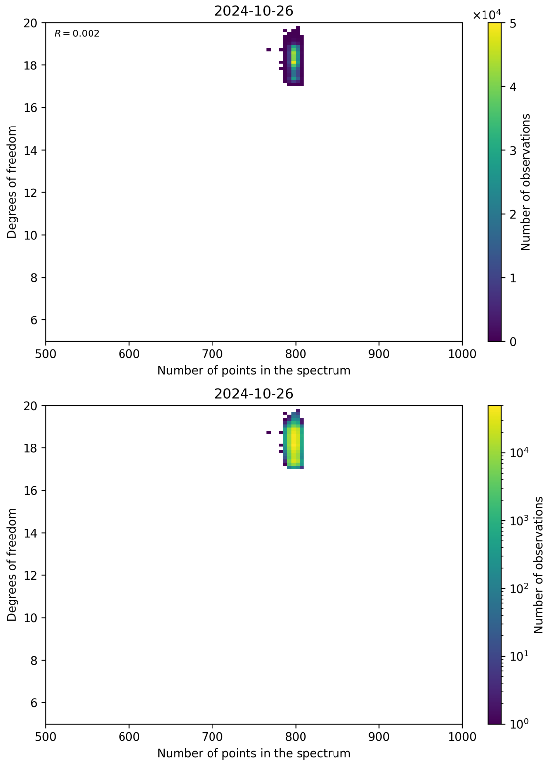
Figure 90: Scatter density plot of “Number of points in the spectrum” against “Degrees of freedom” for 2024-10-25 to 2024-10-27.
