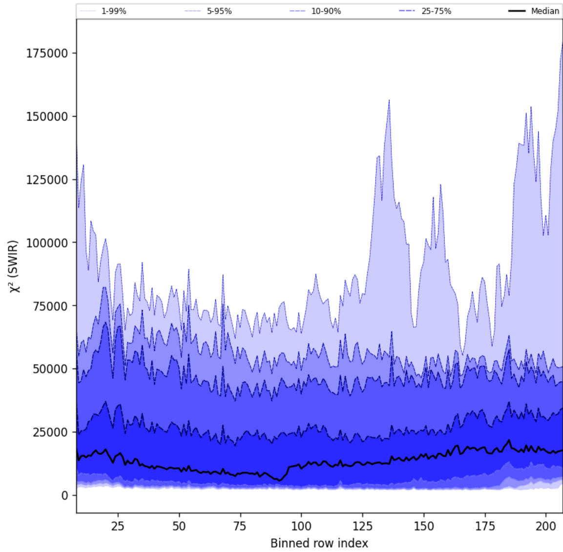
Figure 39: Along track statistics of “ \chi^2 (SWIR)” for 2024-10-25 to 2024-10-27
