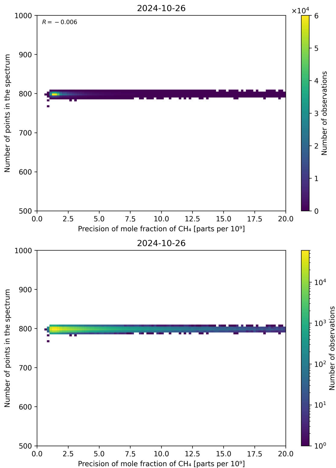
Figure 84: Scatter density plot of “Precision of mole fraction of CH 4 ” against “Number of points in the spectrum” for 2024-10-25 to 2024-10-27.
