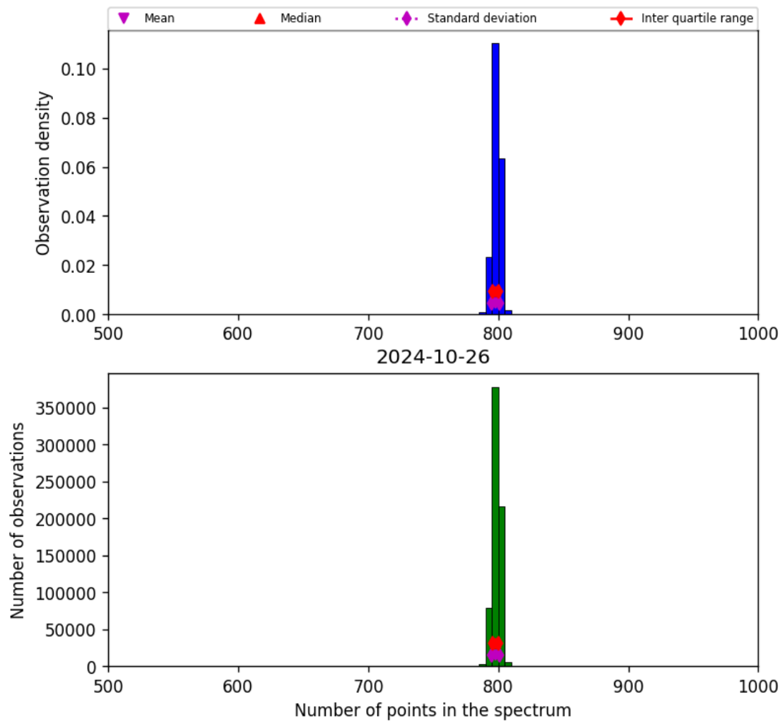
Figure 26: Histogram of “Number of points in the spectrum” for 2024-10-25 to 2024-10-27
