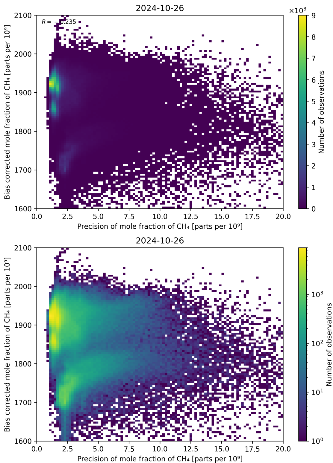
Figure 82: Scatter density plot of “Precision of mole fraction of CH 4 ” against “Bias corrected mole fraction of CH 4 ” for 2024-10-25 to 2024-10-27.
