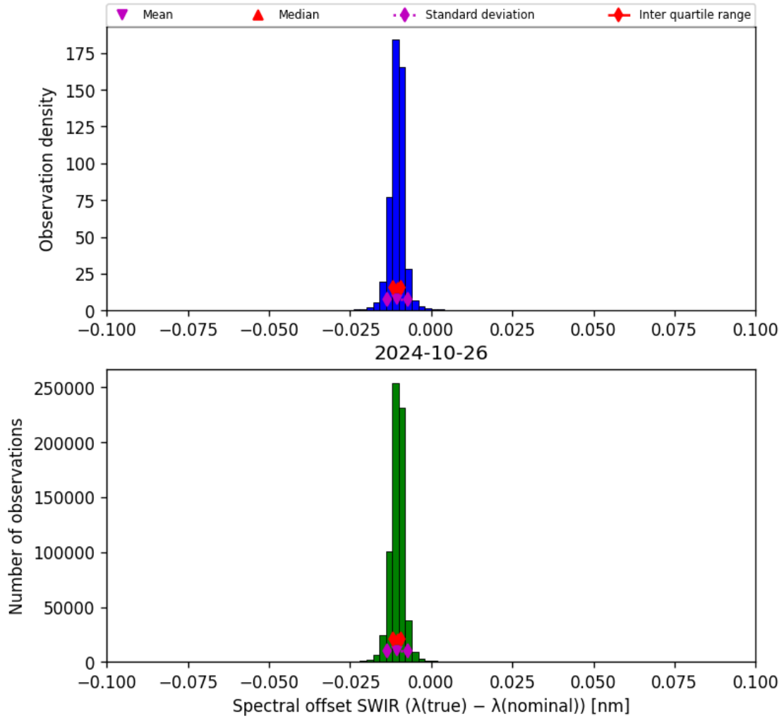
Figure 27: Histogram of “Spectral offset SWIR ( \lambda_{\text{true}} - \lambda_{\text{nominal}} )” for 2024-10-25 to 2024-10-27
