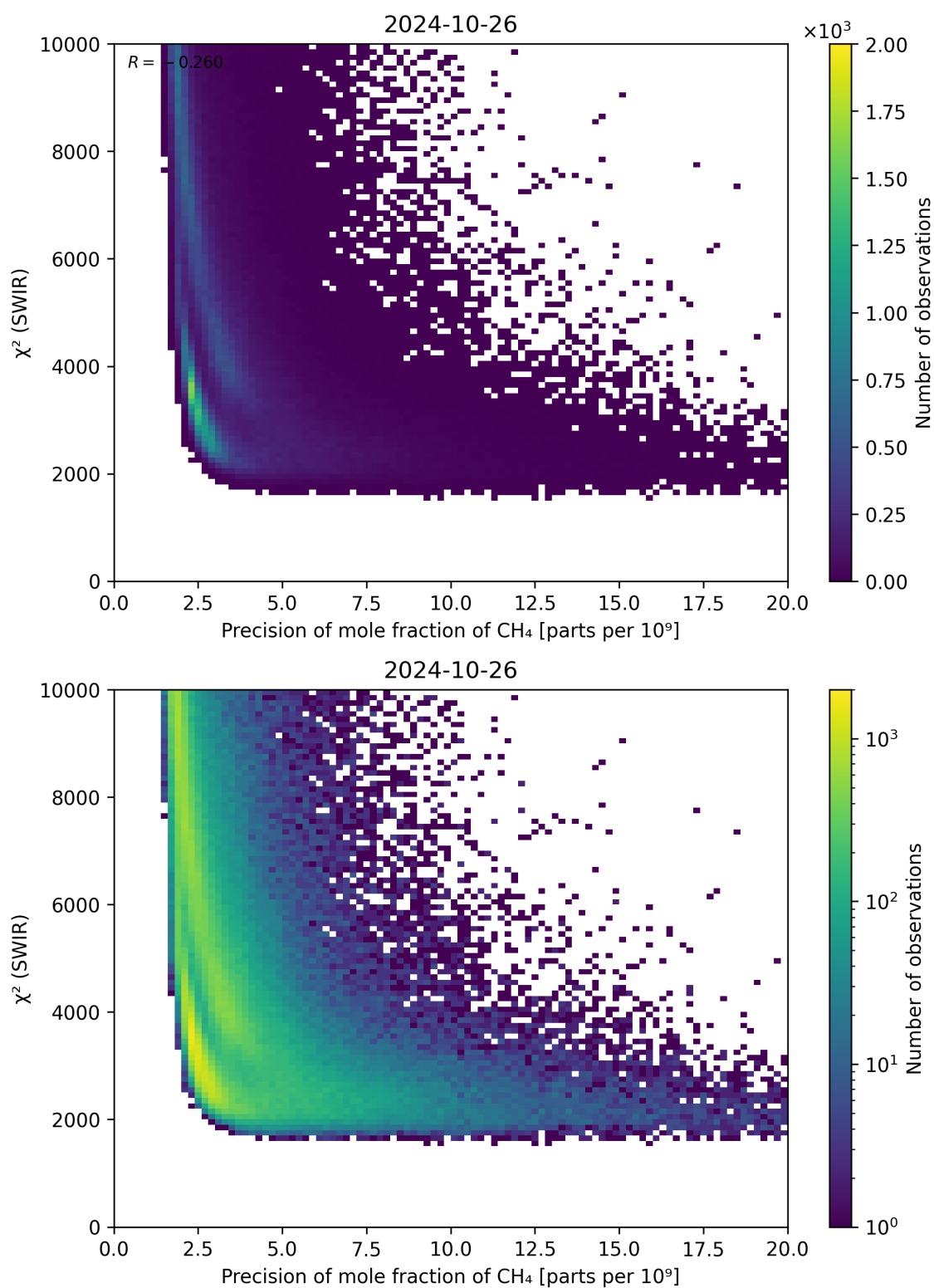
Figure 79: Scatter density plot of “Precision of mole fraction of \text{CH}_4 ” against “ \chi^2 (SWIR)” for 2024-10-25 to 2024-10-27.
