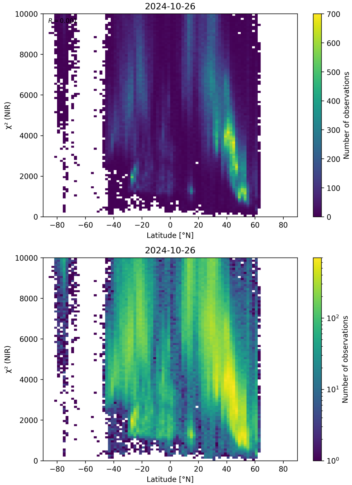
Figure 53: Scatter density plot of “Latitude” against “ \chi^2 (NIR)” for 2024-10-25 to 2024-10-27.
