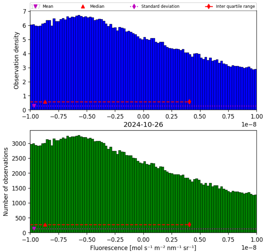
Figure 32: Histogram of “Fluorescence” for 2024-10-25 to 2024-10-27
