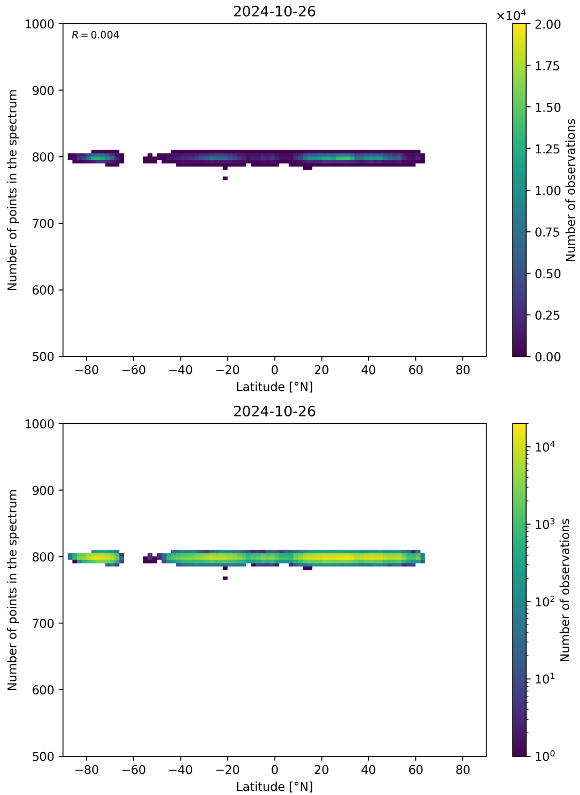
Figure 61: Scatter density plot of “Latitude” against “Number of points in the spectrum” for 2024-10-25 to 2024-10-27.
