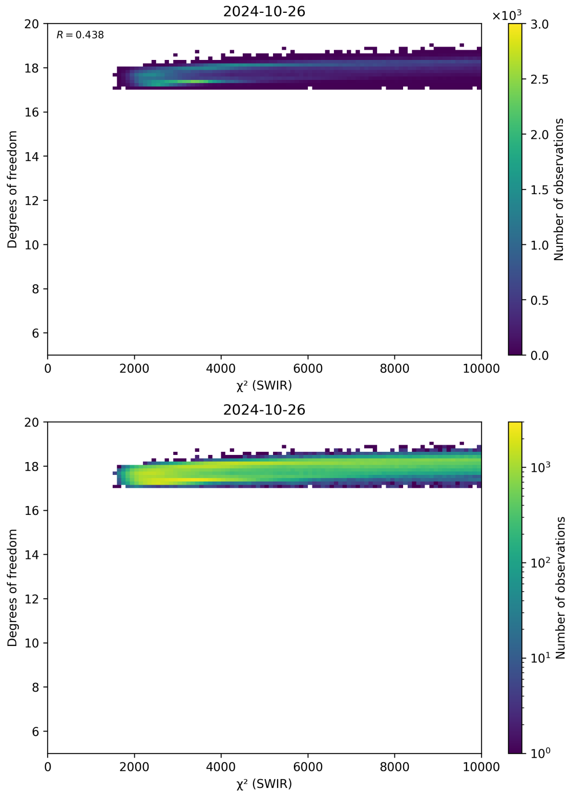
Figure 48: Scatter density plot of “ \chi^2 (SWIR)” against “Degrees of freedom” for 2024-10-25 to 2024-10-27.
