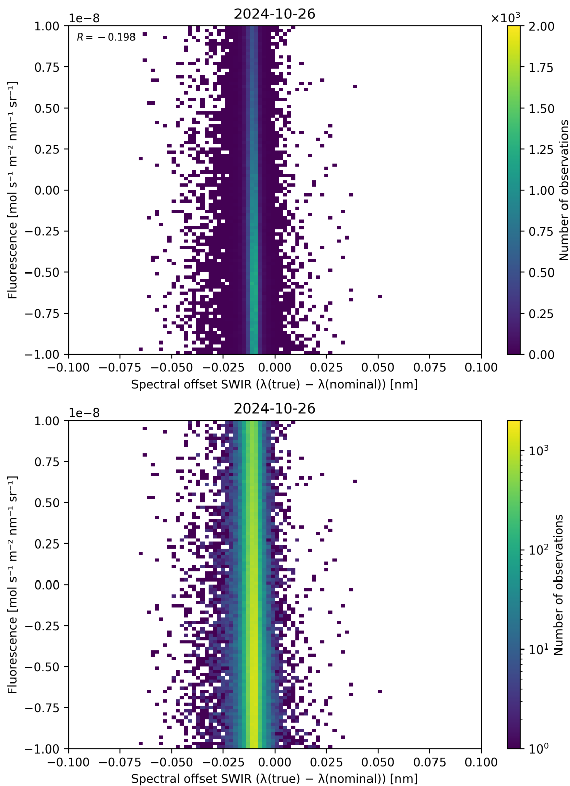
Figure 120: Scatter density plot of “Spectral offset SWIR ( \lambda_{\text{true}} - \lambda_{\text{nominal}} )” against “Fluorescence” for 2024-10-25 to 2024-10-27.
