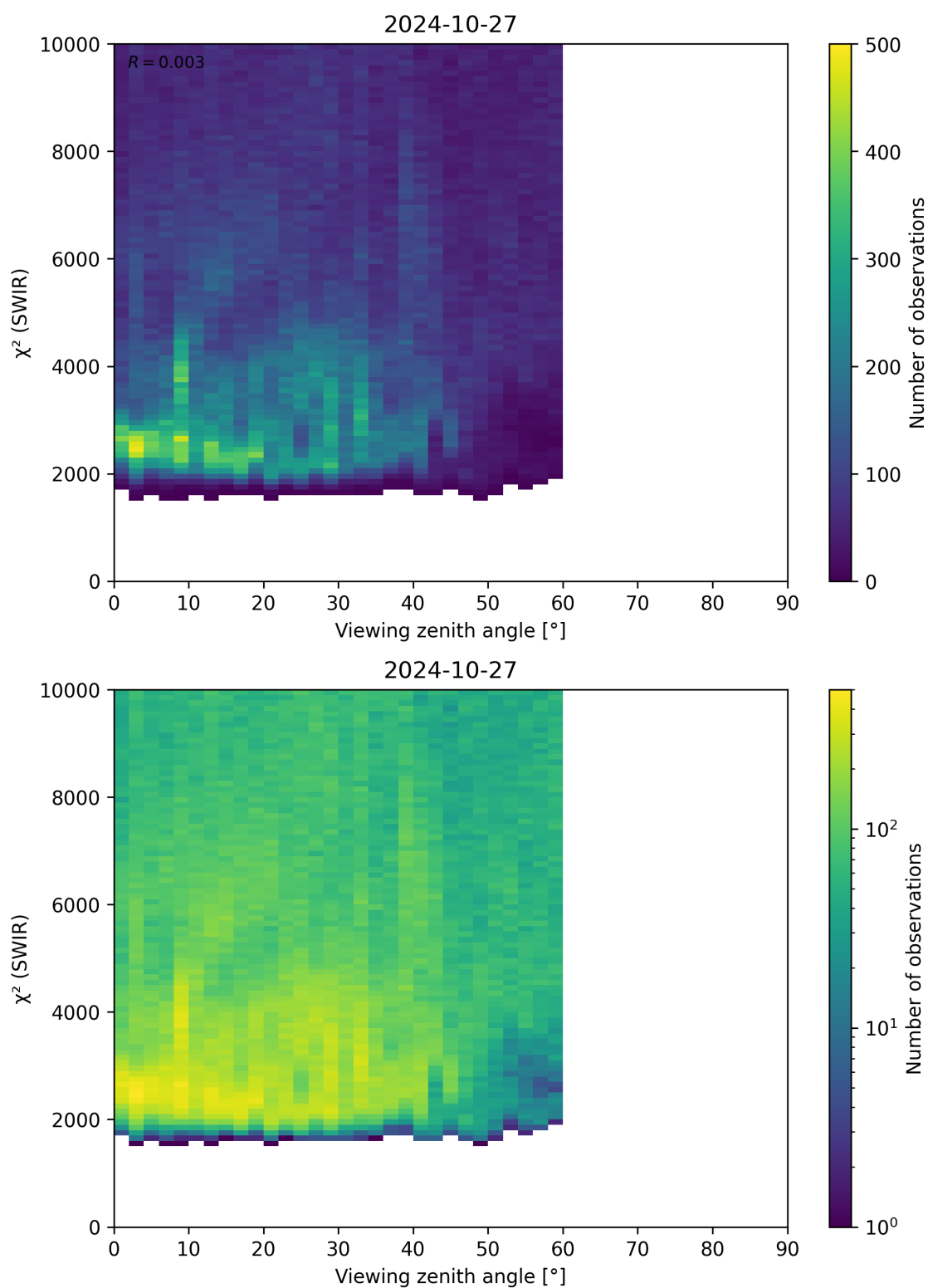
Figure 106: Scatter density plot of “Viewing zenith angle” against “ \chi^2 (SWIR)” for 2024-10-26 to 2024-10-28.
