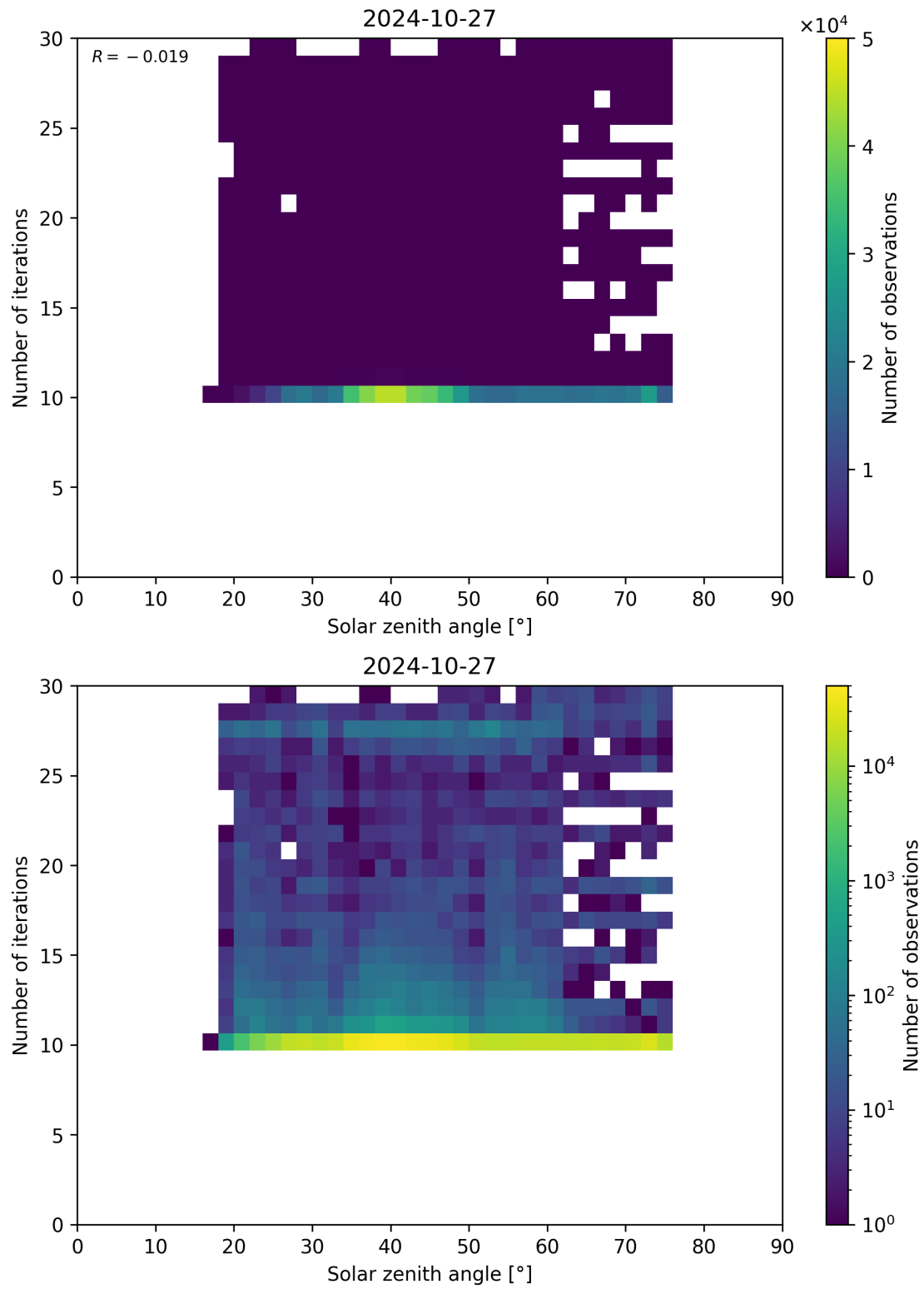
Figure 102: Scatter density plot of “Solar zenith angle” against “Number of iterations” for 2024-10-26 to 2024-10-28.
