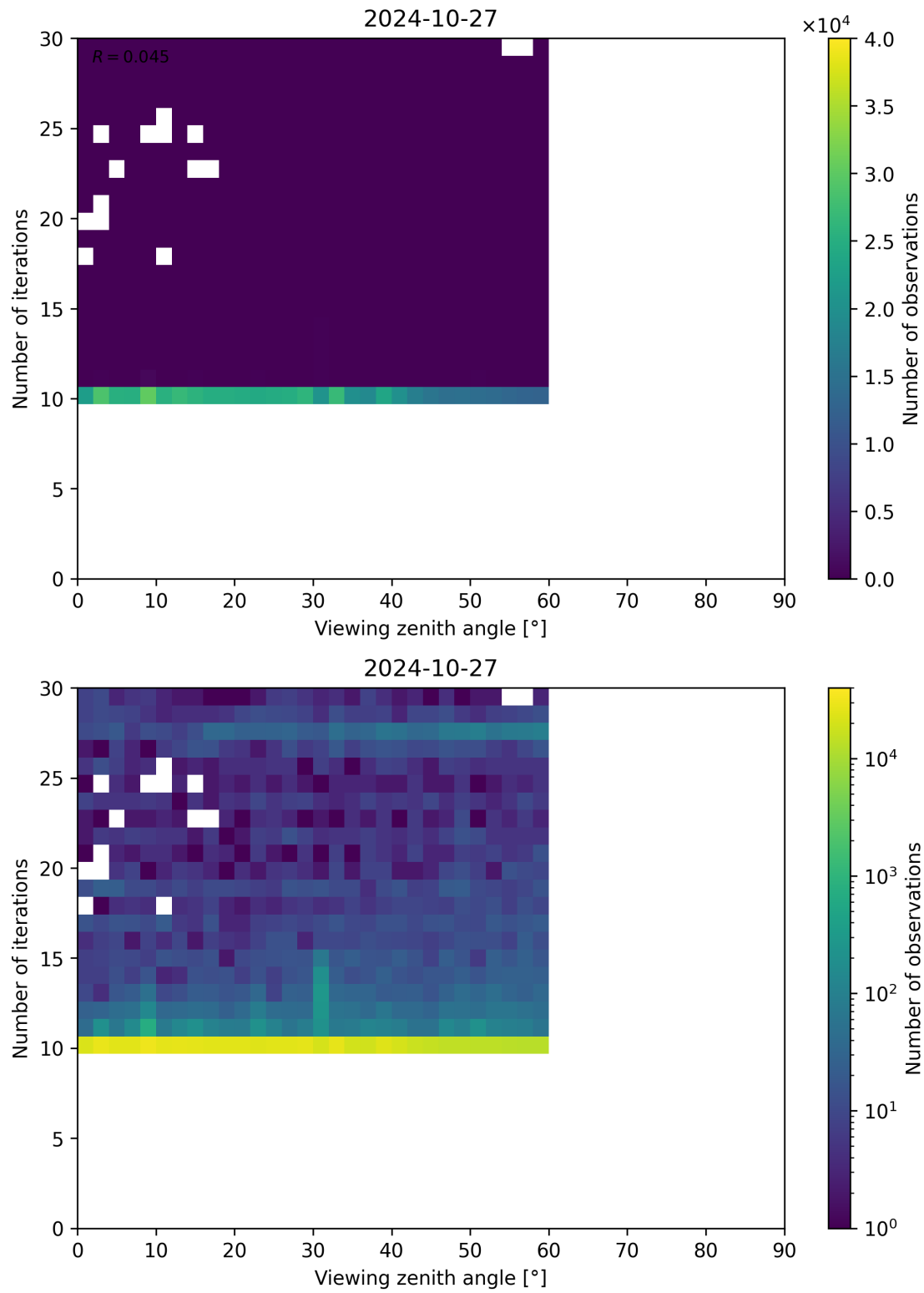
Figure 113: Scatter density plot of “Viewing zenith angle” against “Number of iterations” for 2024-10-26 to 2024-10-28.
