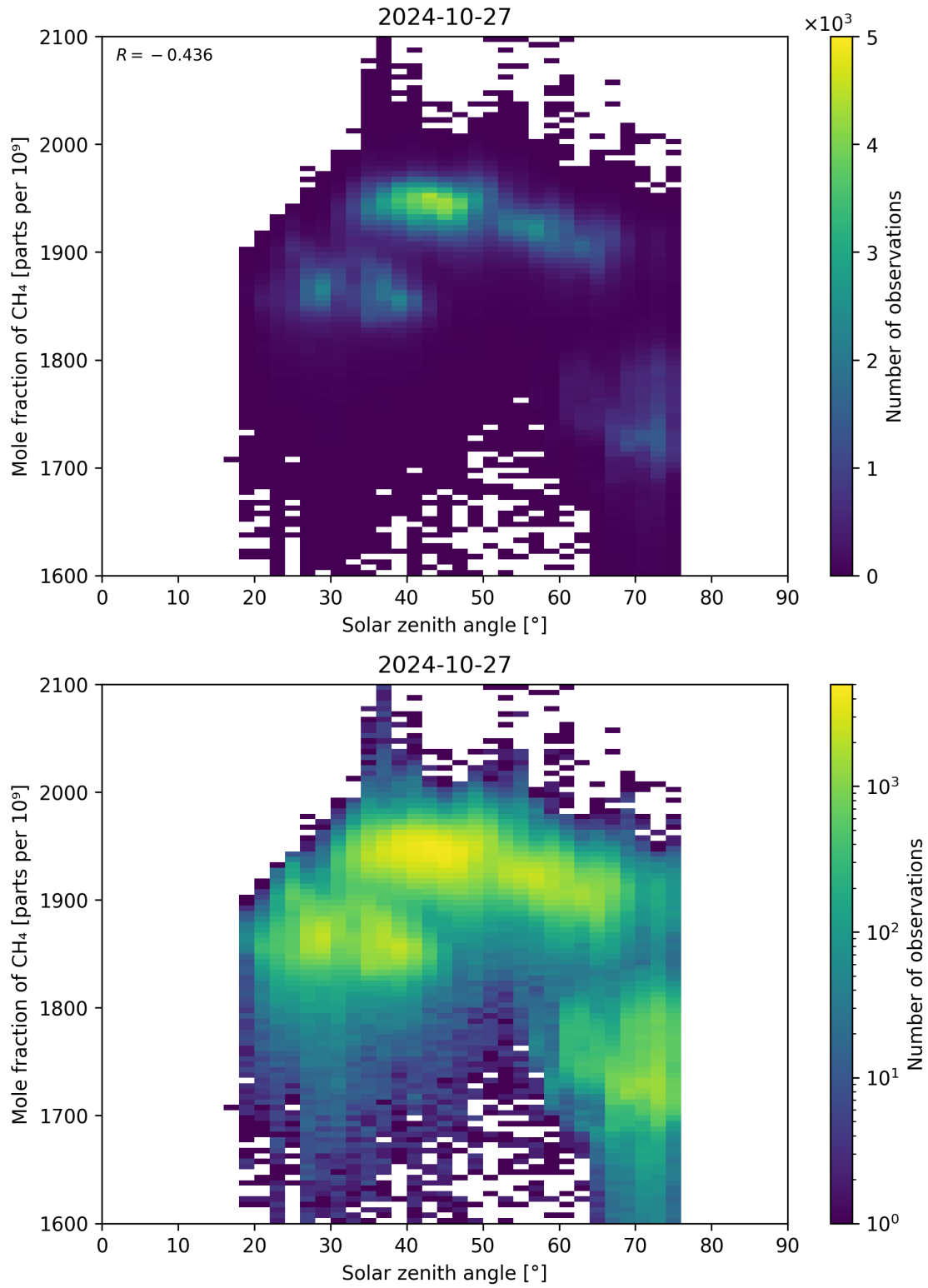
Figure 99: Scatter density plot of “Solar zenith angle” against “Mole fraction of \text{CH}_4 ” for 2024-10-26 to 2024-10-28.
