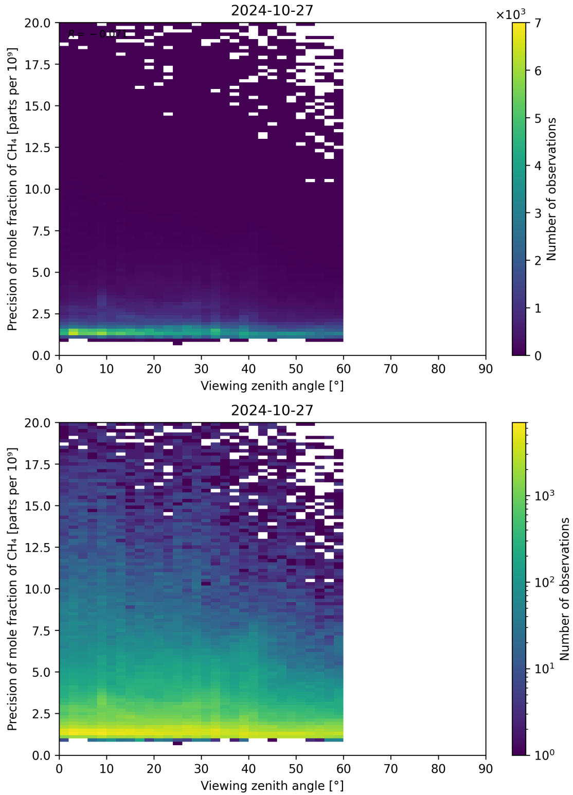
Figure 112: Scatter density plot of “Viewing zenith angle” against “Precision of mole fraction of CH 4 ” for 2024-10-26 to 2024-10-28.
