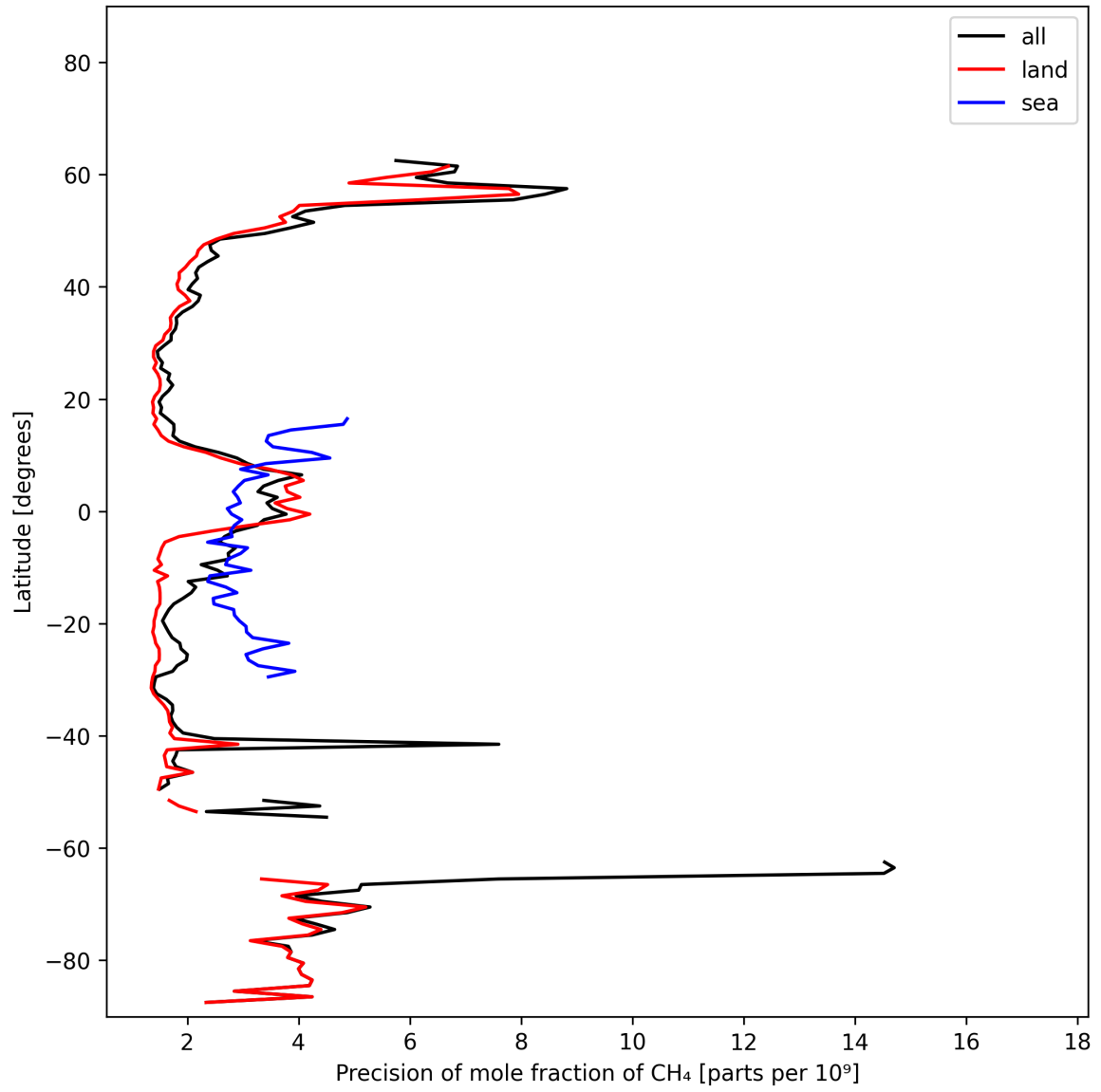
Figure 13: Zonal average of “Precision of mole fraction of CH 4 ” for 2024-10-26 to 2024-10-28.
