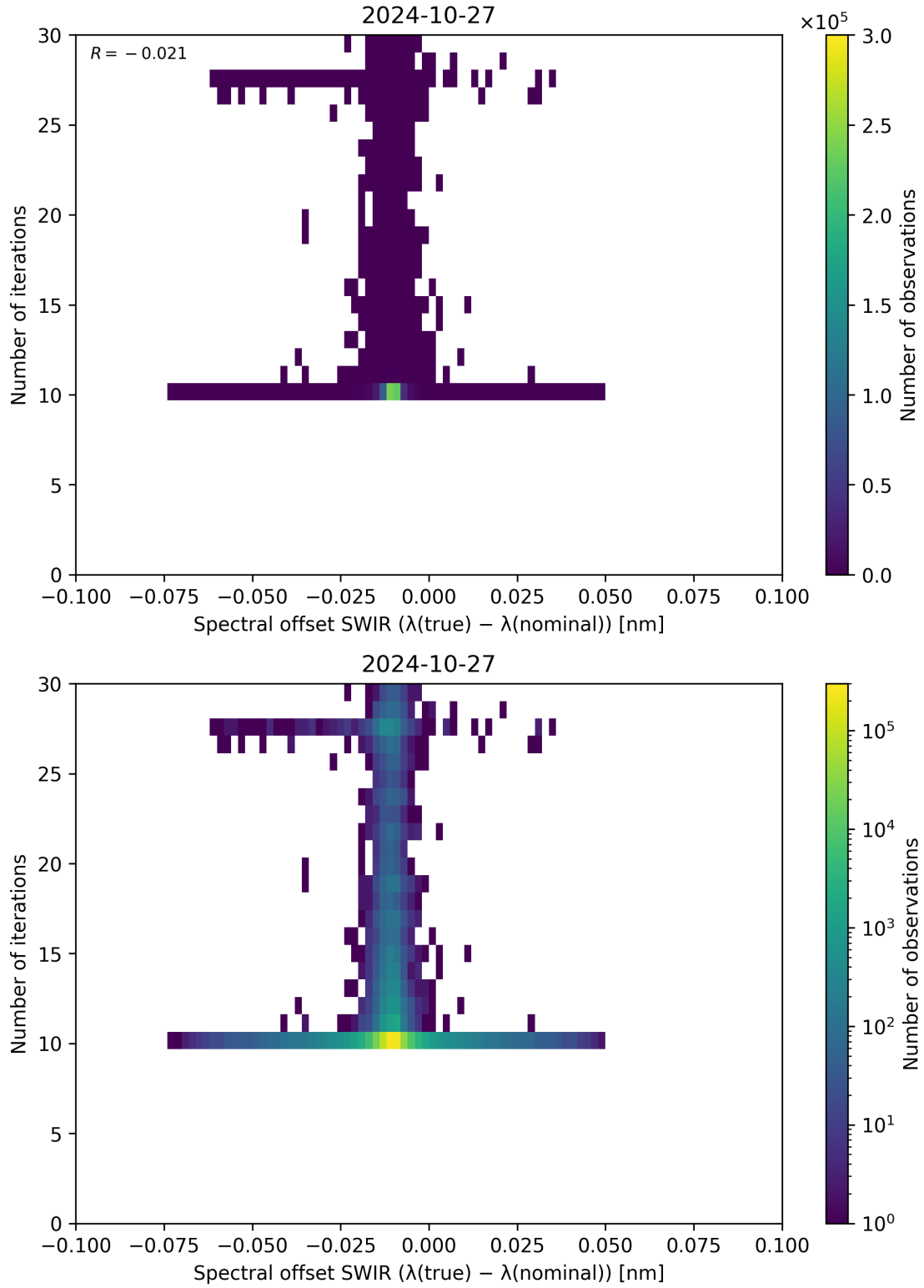
Figure 121: Scatter density plot of “Spectral offset SWIR ( \lambda_{\text{true}} - \lambda_{\text{nominal}} )” against “Number of iterations” for 2024-10-26 to 2024-10-28.
