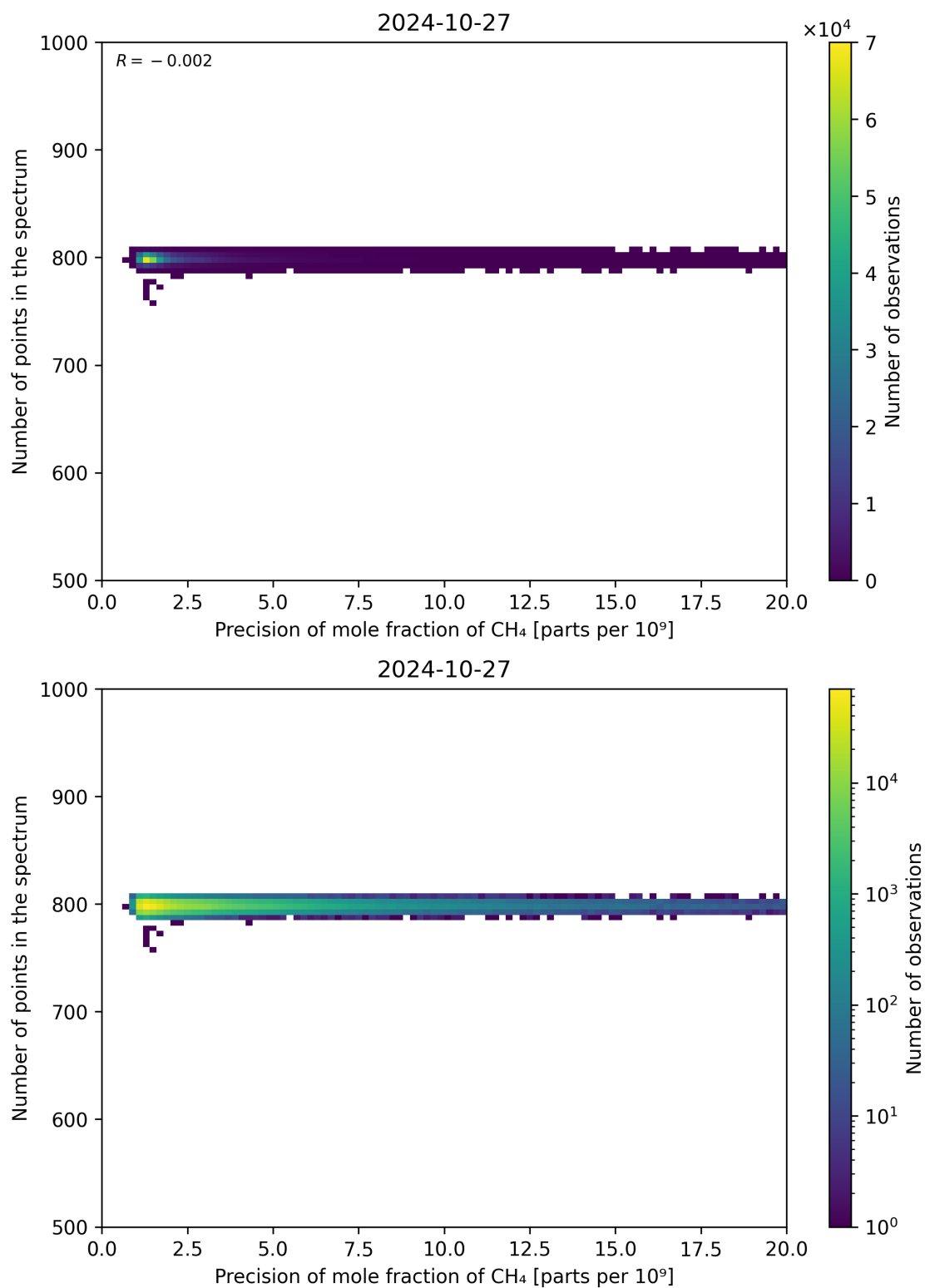
Figure 84: Scatter density plot of “Precision of mole fraction of CH 4 ” against “Number of points in the spectrum” for 2024-10-26 to 2024-10-28.
