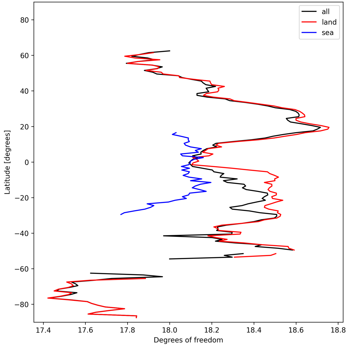
Figure 19: Zonal average of “Degrees of freedom” for 2024-10-26 to 2024-10-28.
