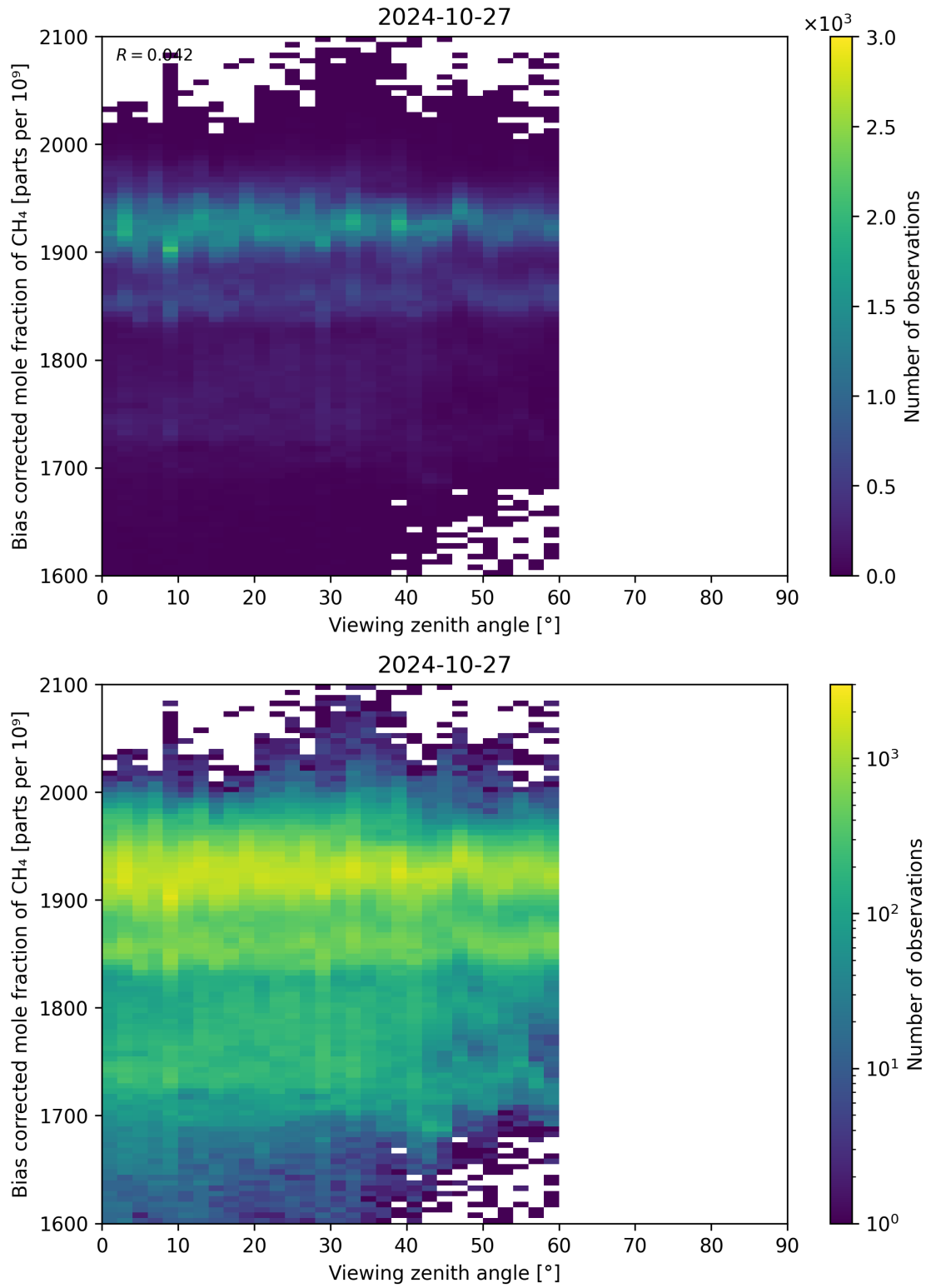
Figure 111: Scatter density plot of “Viewing zenith angle” against “Bias corrected mole fraction of CH 4 ” for 2024-10-26 to 2024-10-28.
