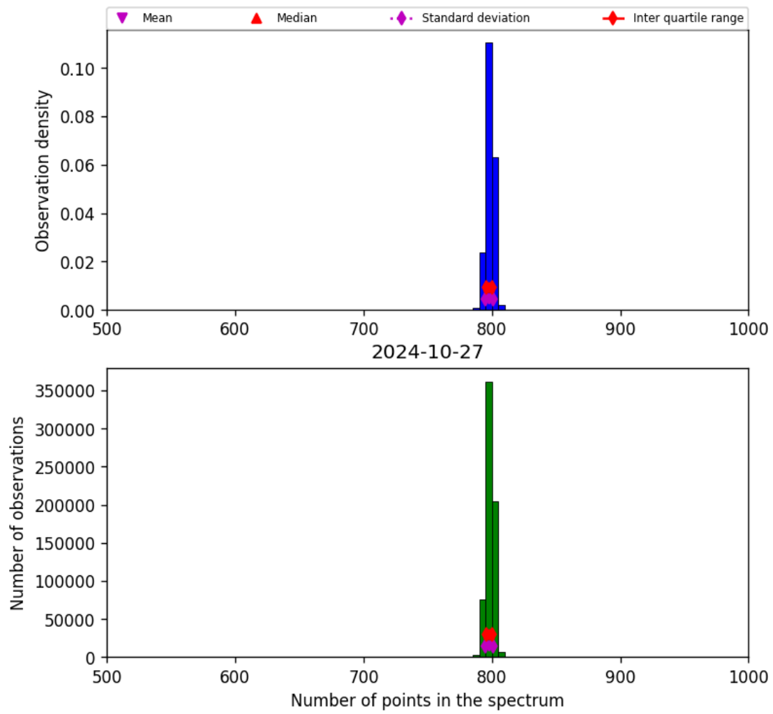
Figure 26: Histogram of “Number of points in the spectrum” for 2024-10-26 to 2024-10-28
