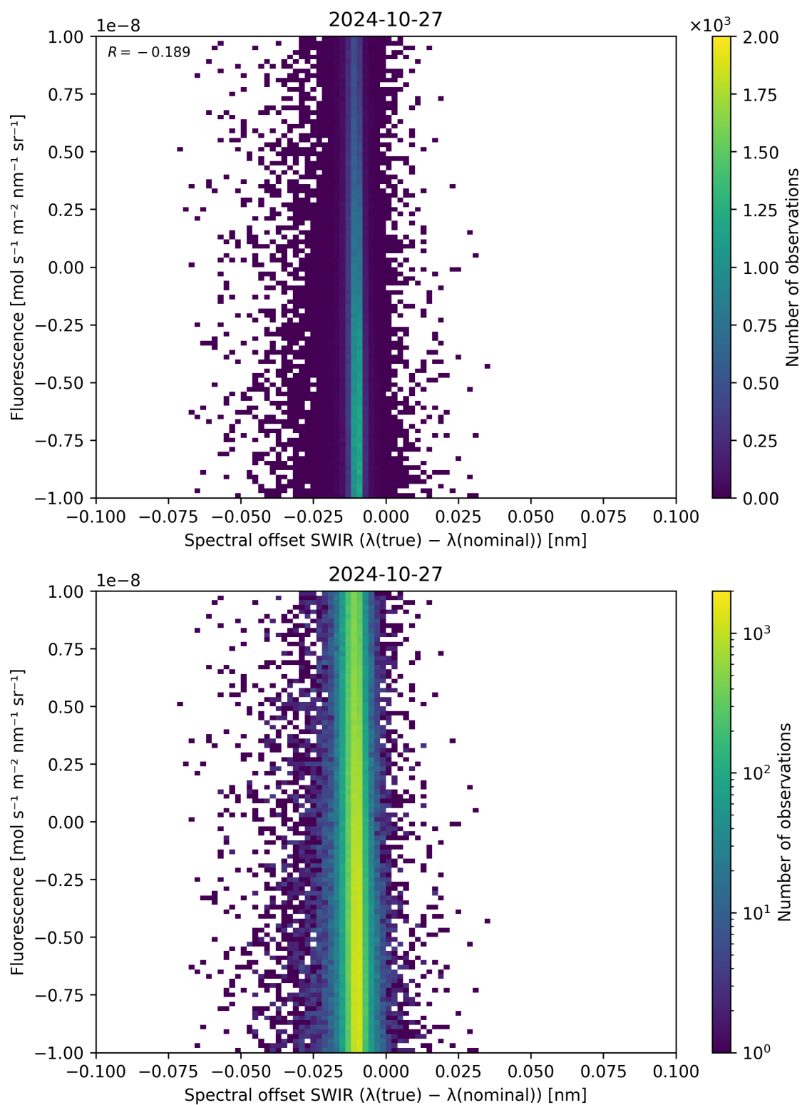
Figure 120: Scatter density plot of “Spectral offset SWIR ( \lambda_{\text{true}} - \lambda_{\text{nominal}} )” against “Fluorescence” for 2024-10-26 to 2024-10-28.
