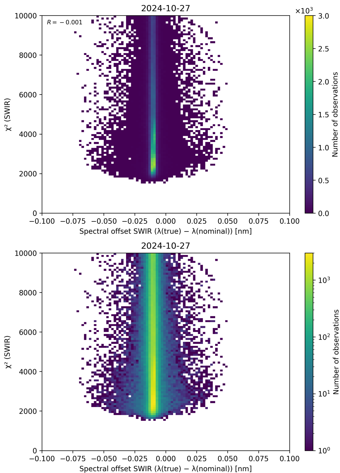
Figure 118: Scatter density plot of “Spectral offset SWIR ( \lambda_{\text{true}} - \lambda_{\text{nominal}} )” against “ \chi^2 (SWIR)” for 2024-10-26 to 2024-10-28.
