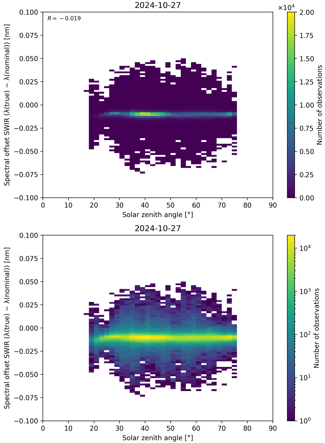
Figure 104: Scatter density plot of “Solar zenith angle” against “Spectral offset SWIR ( \lambda_{\text{true}} - \lambda_{\text{nominal}} )” for 2024-10-26 to 2024-10-28.
