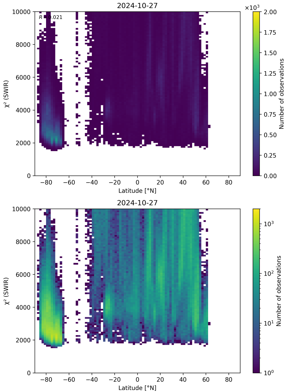
Figure 54: Scatter density plot of “Latitude” against “ \chi^2 (SWIR)” for 2024-10-26 to 2024-10-28.
