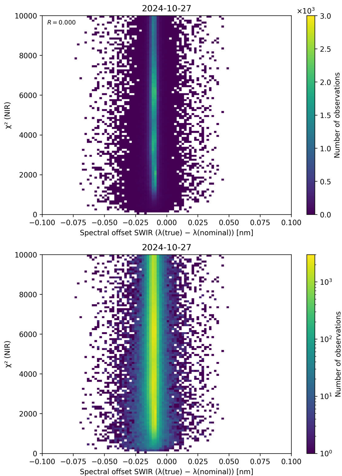
Figure 117: Scatter density plot of “Spectral offset SWIR ( \lambda_{\text{true}} - \lambda_{\text{nominal}} )” against “ \chi^2 (NIR)” for 2024-10-26 to 2024-10-28.
