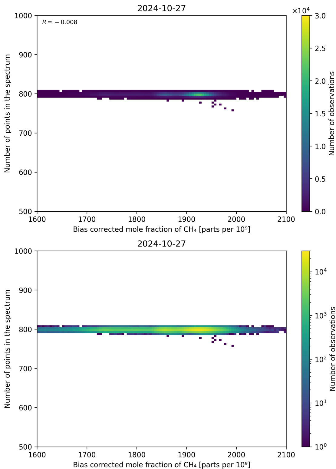
Figure 68: Scatter density plot of “Bias corrected mole fraction of CH 4 ” against “Number of points in the spectrum” for 2024-10-26 to 2024-10-28.
