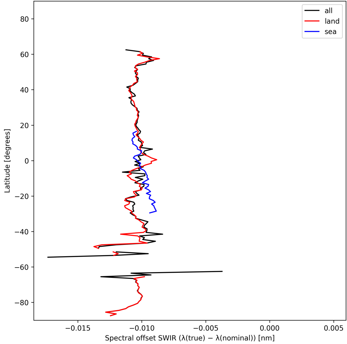
Figure 16: Zonal average of “Spectral offset SWIR ( \lambda_{\text{true}} - \lambda_{\text{nominal}} )” for 2024-10-26 to 2024-10-28.
