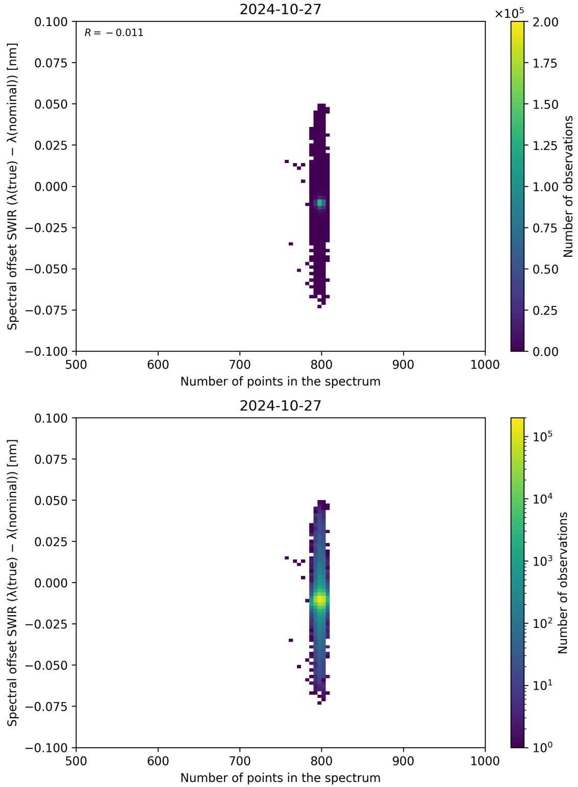
Figure 93: Scatter density plot of “Number of points in the spectrum” against “Spectral offset SWIR ( \lambda_{\text{true}} - \lambda_{\text{nominal}} )” for 2024-10-26 to 2024-10-28.
