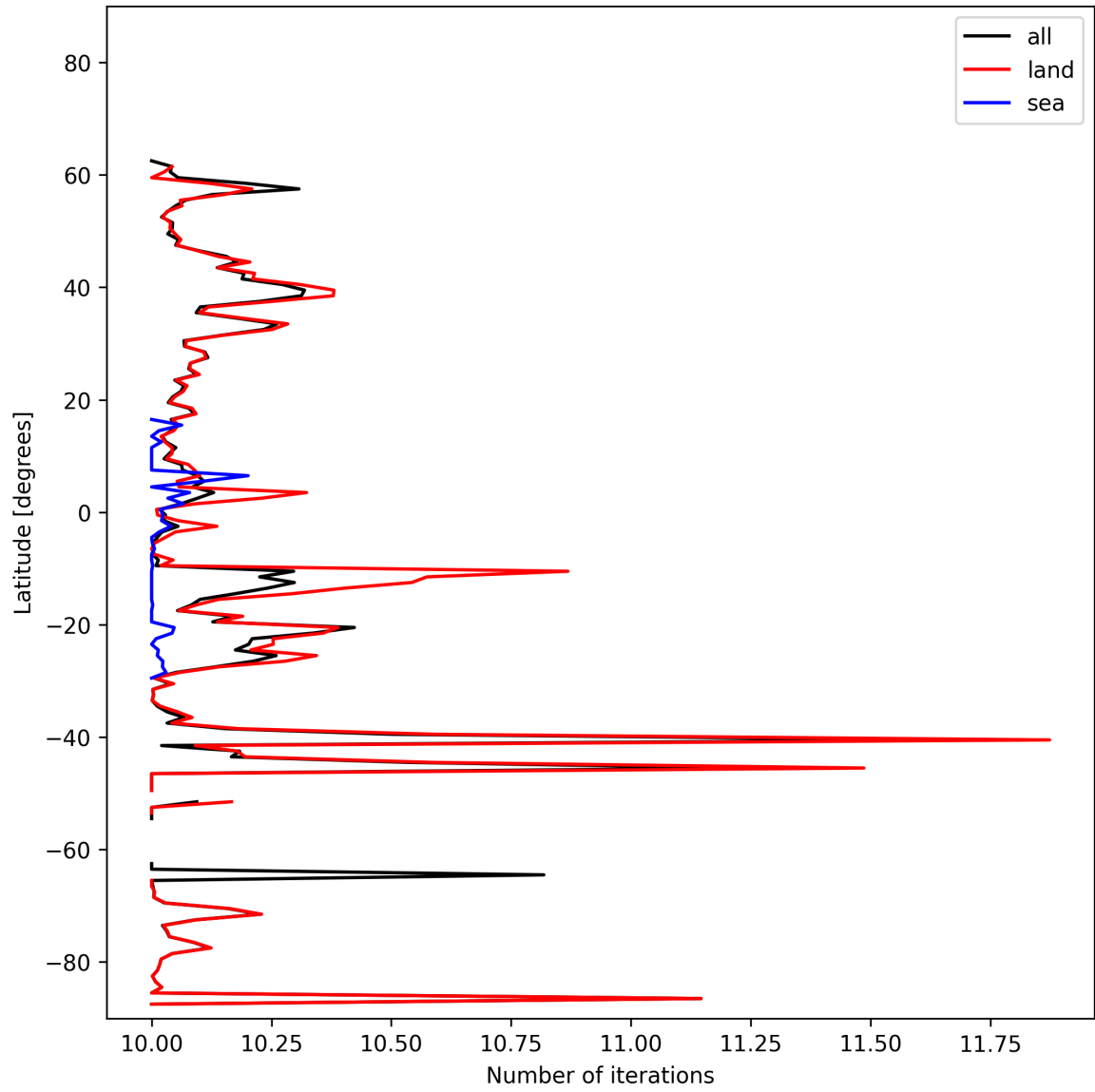
Figure 20: Zonal average of “Number of iterations” for 2024-10-26 to 2024-10-28.
