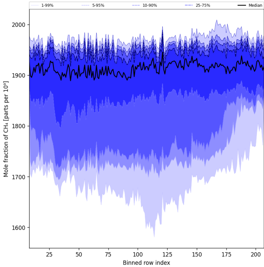
Figure 34: Along track statistics of “Mole fraction of CH 4 ” for 2024-10-26 to 2024-10-28
