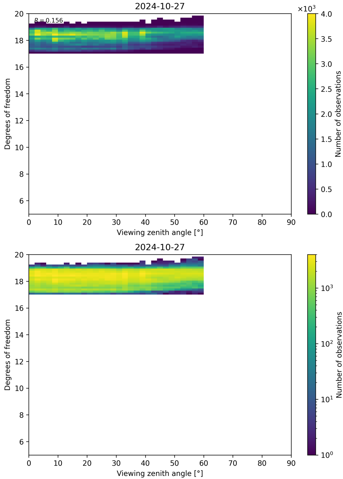
Figure 107: Scatter density plot of “Viewing zenith angle” against “Degrees of freedom” for 2024-10-26 to 2024-10-28.
