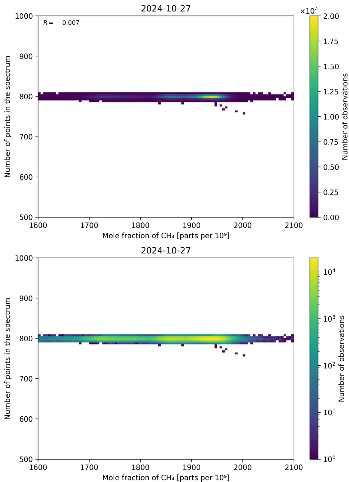
Figure 77: Scatter density plot of “Mole fraction of CH 4 ” against “Number of points in the spectrum” for 2024-10-26 to 2024-10-28.
