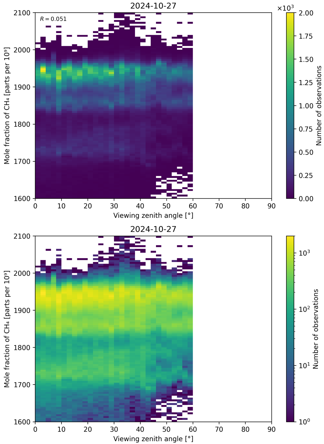
Figure 110: Scatter density plot of “Viewing zenith angle” against “Mole fraction of \text{CH}_4 ” for 2024-10-26 to 2024-10-28.
