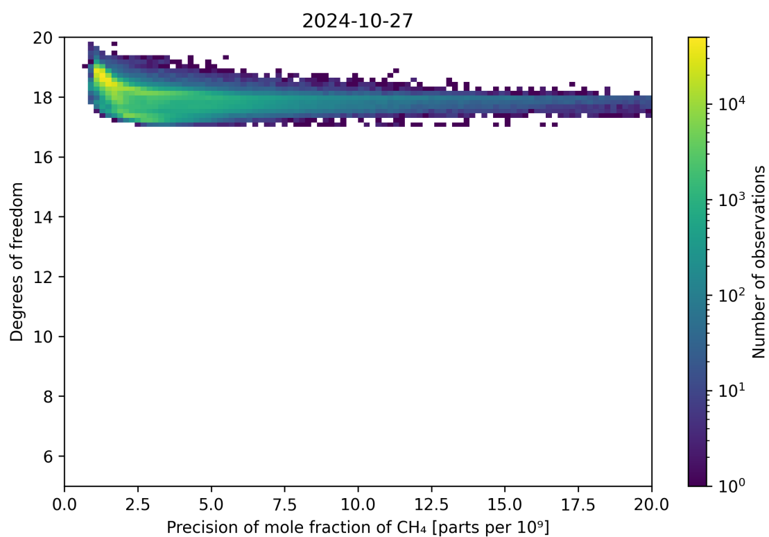
Figure 80: Scatter density plot of “Precision of mole fraction of CH 4 ” against “Degrees of freedom” for 2024-10-26 to 2024-10-28.
