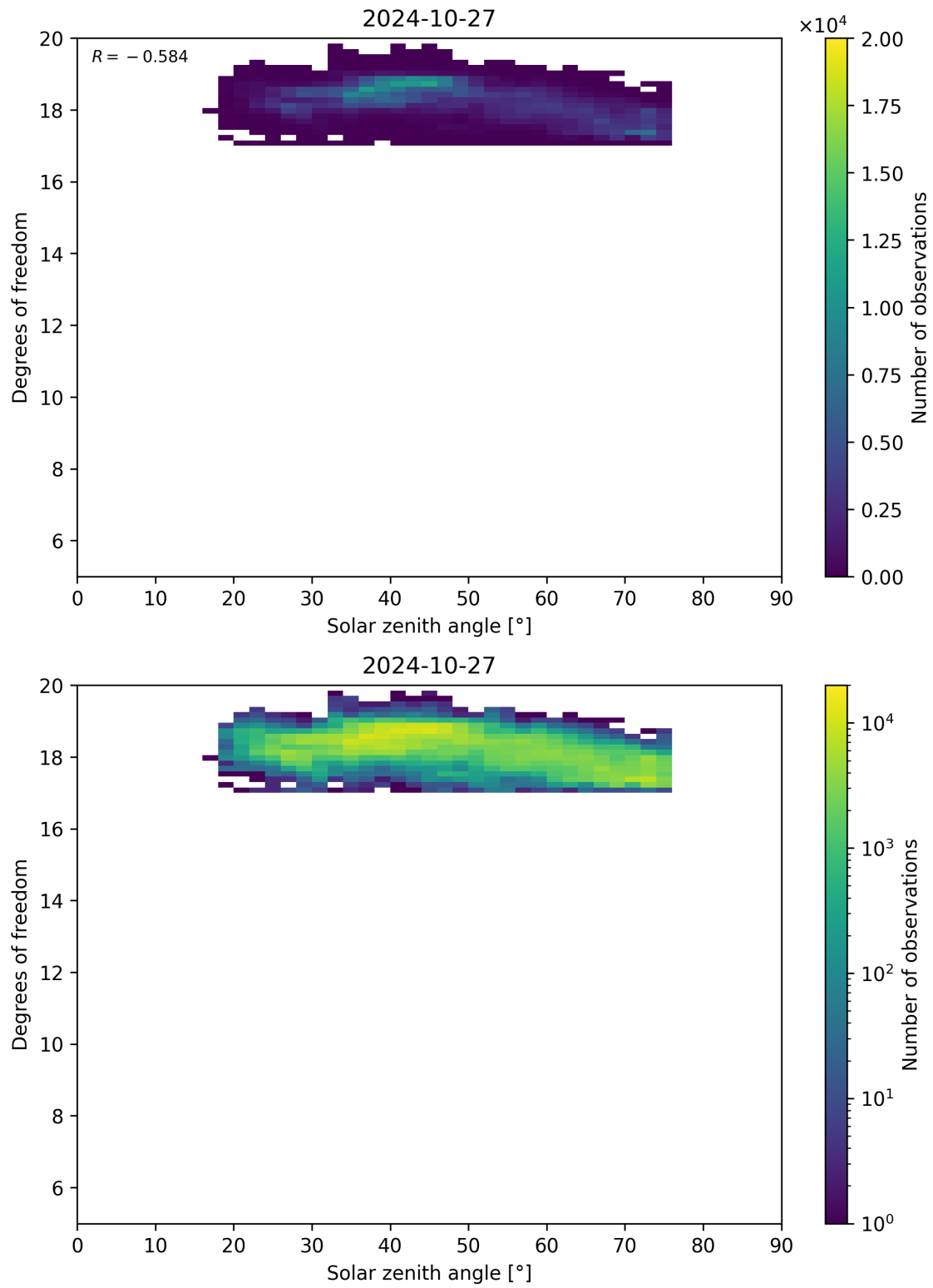
Figure 96: Scatter density plot of “Solar zenith angle” against “Degrees of freedom” for 2024-10-26 to 2024-10-28.
