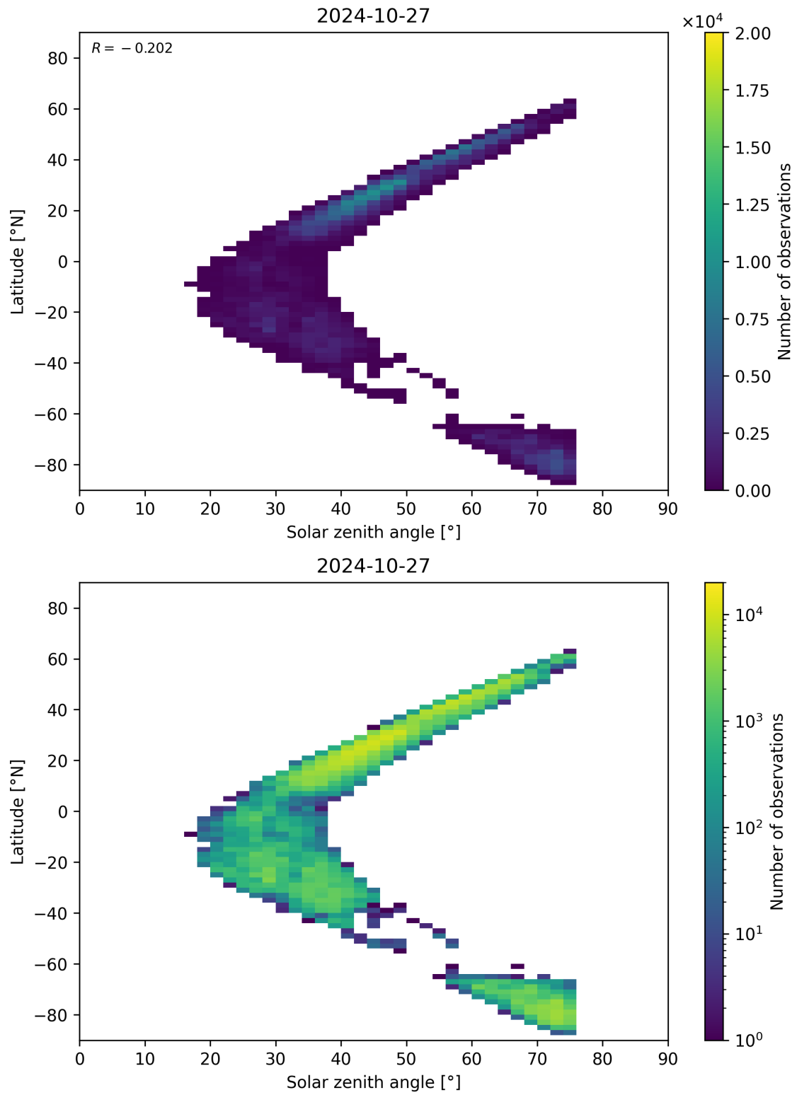
Figure 98: Scatter density plot of “Solar zenith angle” against “Latitude” for 2024-10-26 to 2024-10-28.
