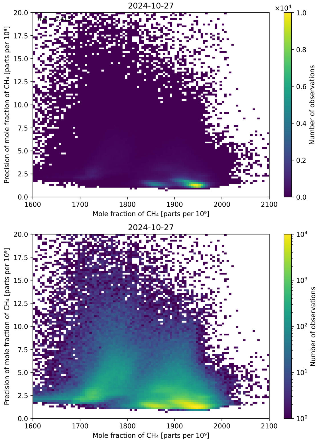
Figure 75: Scatter density plot of “Mole fraction of CH 4 ” against “Precision of mole fraction of CH 4 ” for 2024-10-26 to 2024-10-28.
