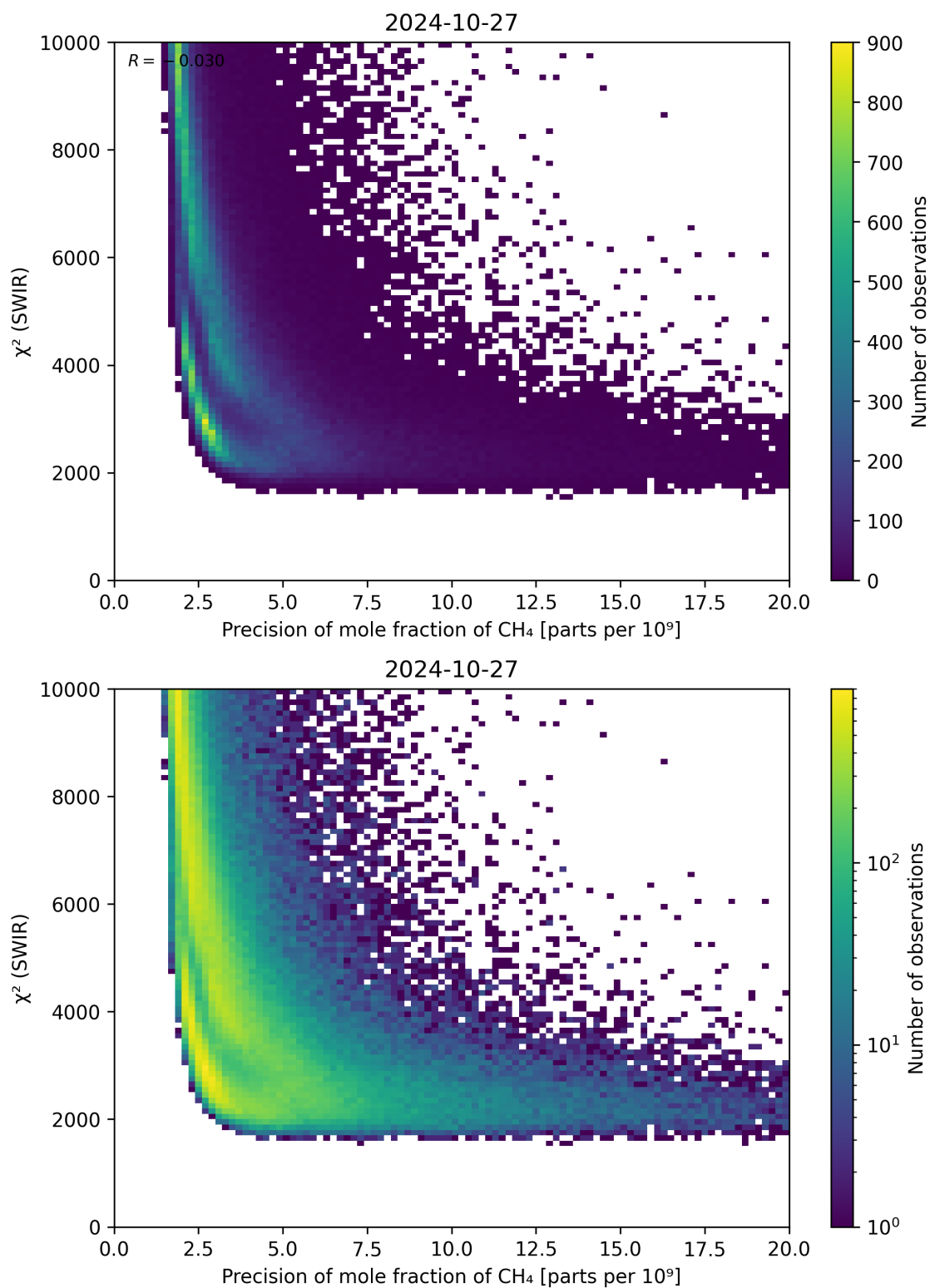
Figure 79: Scatter density plot of “Precision of mole fraction of CH 4 ” against “ \chi^2 (SWIR)” for 2024-10-26 to 2024-10-28.
