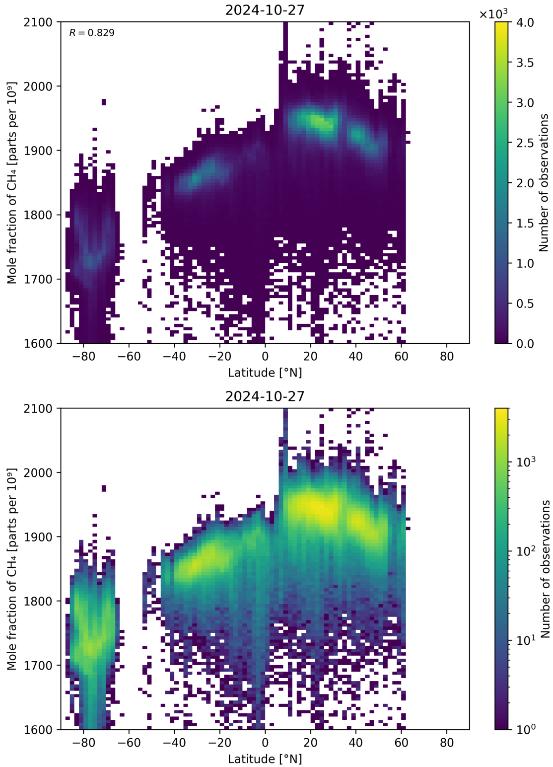
Figure 57: Scatter density plot of “Latitude” against “Mole fraction of CH 4 ” for 2024-10-26 to 2024-10-28.
