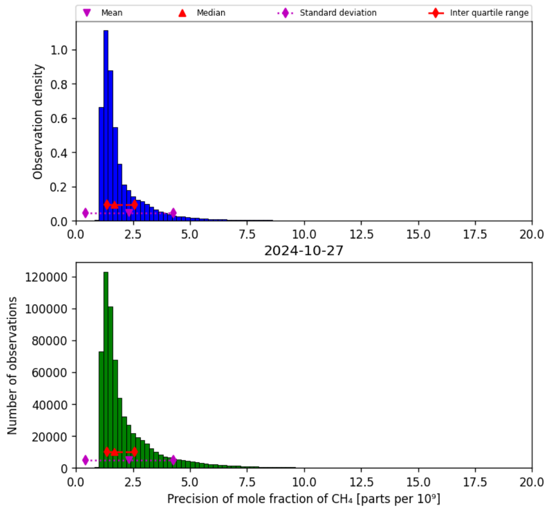
Figure 24: Histogram of “Precision of mole fraction of CH 4 ” for 2024-10-26 to 2024-10-28
