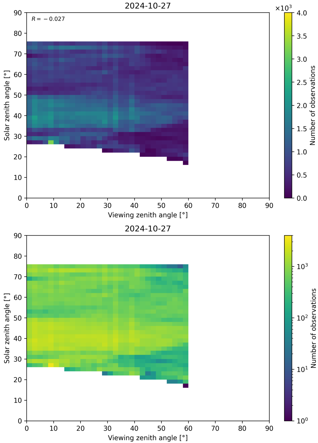
Figure 115: Scatter density plot of “Viewing zenith angle” against “Solar zenith angle” for 2024-10-26 to 2024-10-28.
