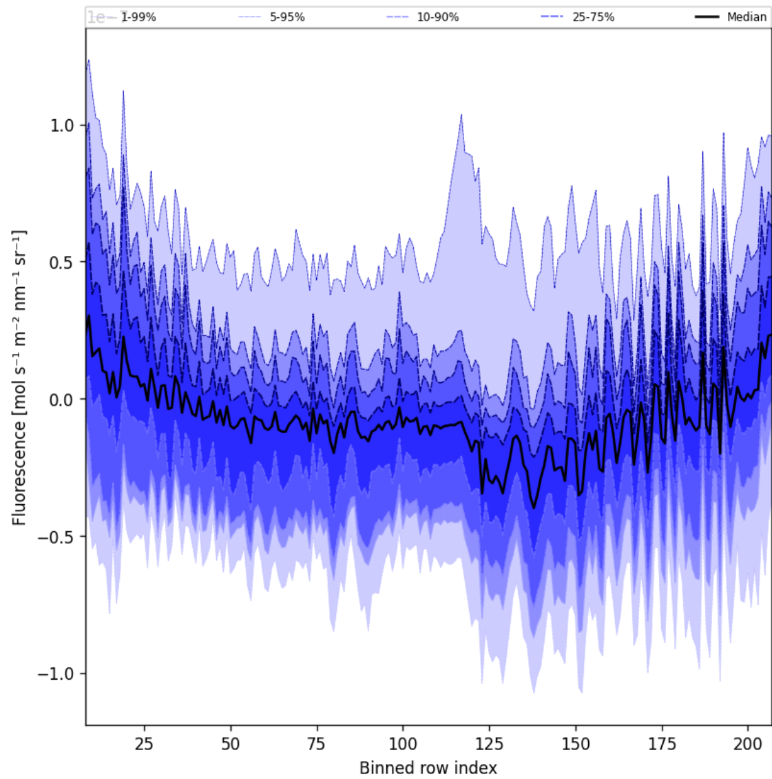
Figure 43: Along track statistics of “Fluorescence” for 2024-10-26 to 2024-10-28
