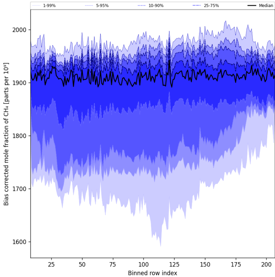
Figure 36: Along track statistics of “Bias corrected mole fraction of CH 4 ” for 2024-10-26 to 2024-10-28
