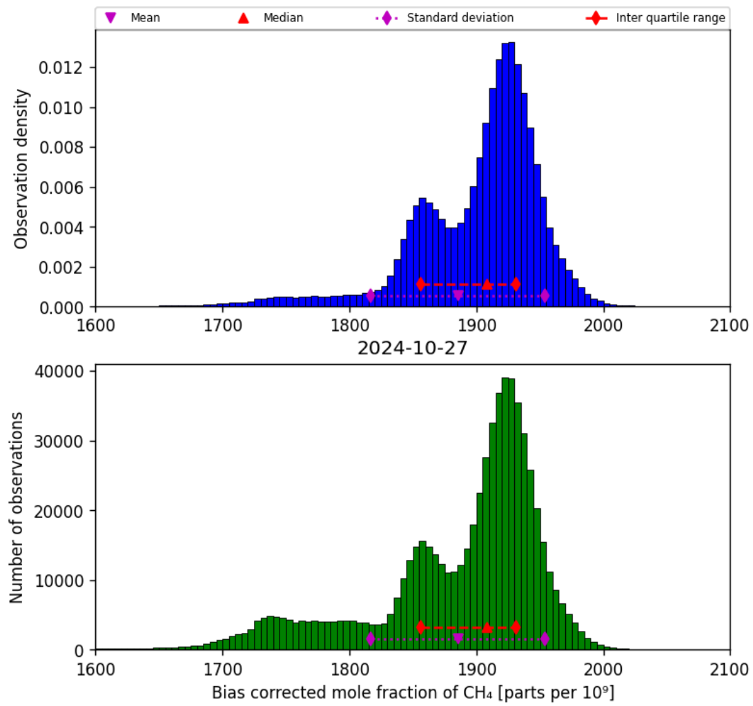
Figure 25: Histogram of “Bias corrected mole fraction of CH 4 ” for 2024-10-26 to 2024-10-28
