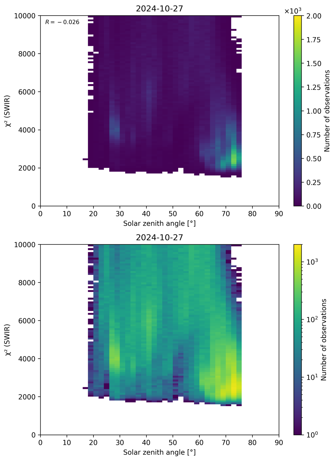
Figure 95: Scatter density plot of “Solar zenith angle” against “ \chi^2 (SWIR)” for 2024-10-26 to 2024-10-28.
