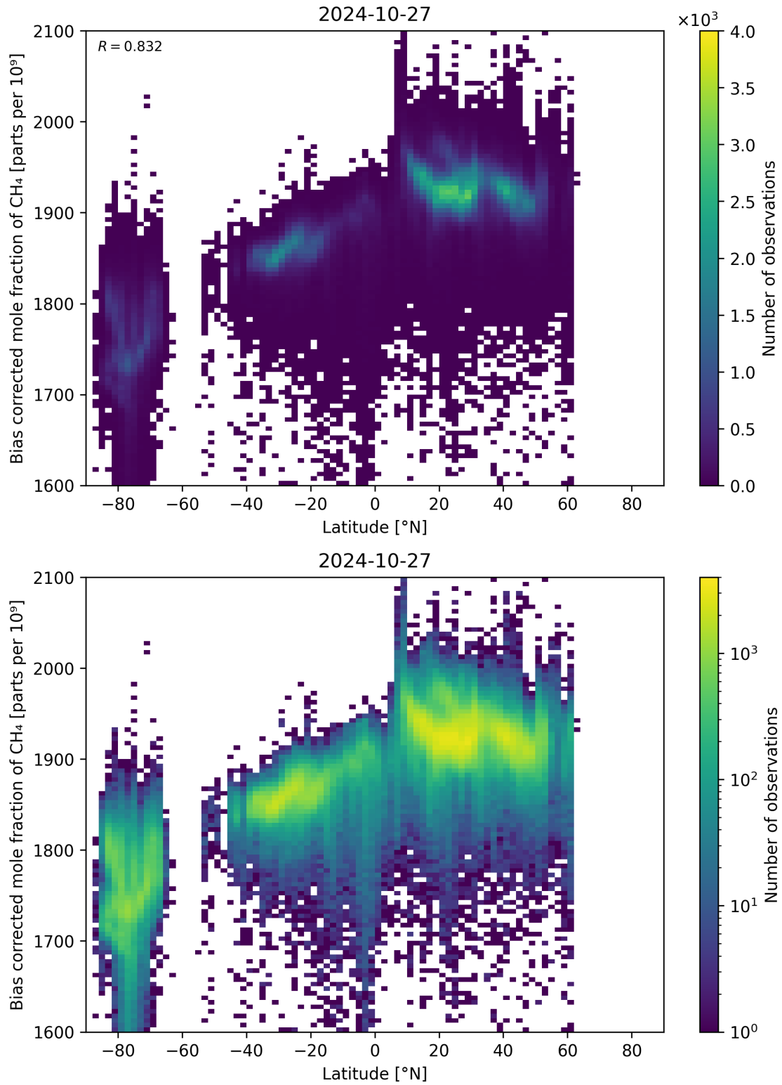
Figure 58: Scatter density plot of “Latitude” against “Bias corrected mole fraction of CH 4 ” for 2024-10-26 to 2024-10-28.
