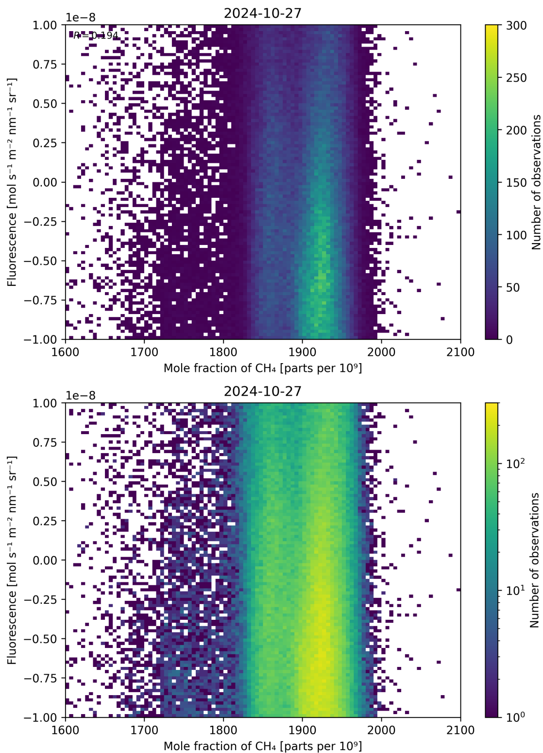
Figure 73: Scatter density plot of “Mole fraction of CH 4 ” against “Fluorescence” for 2024-10-26 to 2024-10-28.
