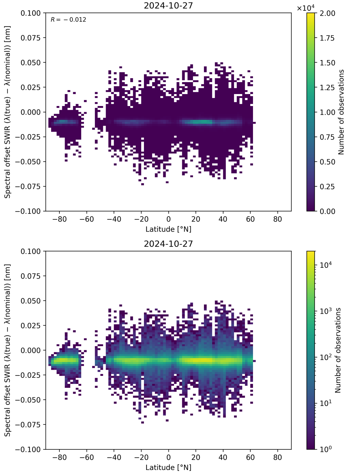
Figure 62: Scatter density plot of “Latitude” against “Spectral offset SWIR ( \lambda_{\text{true}} - \lambda_{\text{nominal}} )” for 2024-10-26 to 2024-10-28.
