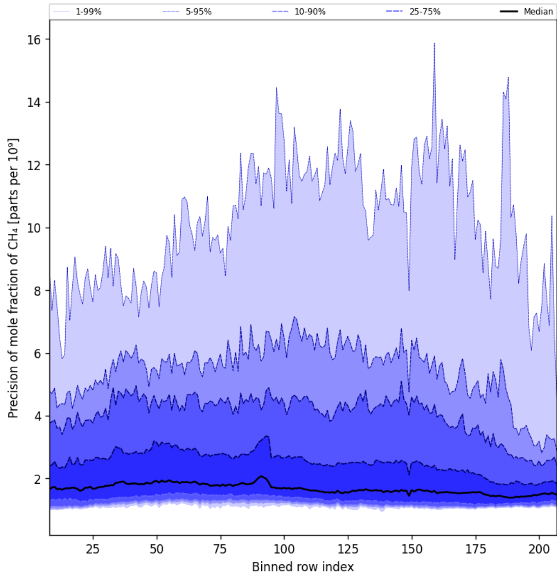
Figure 35: Along track statistics of “Precision of mole fraction of CH 4 ” for 2024-10-26 to 2024-10-28
