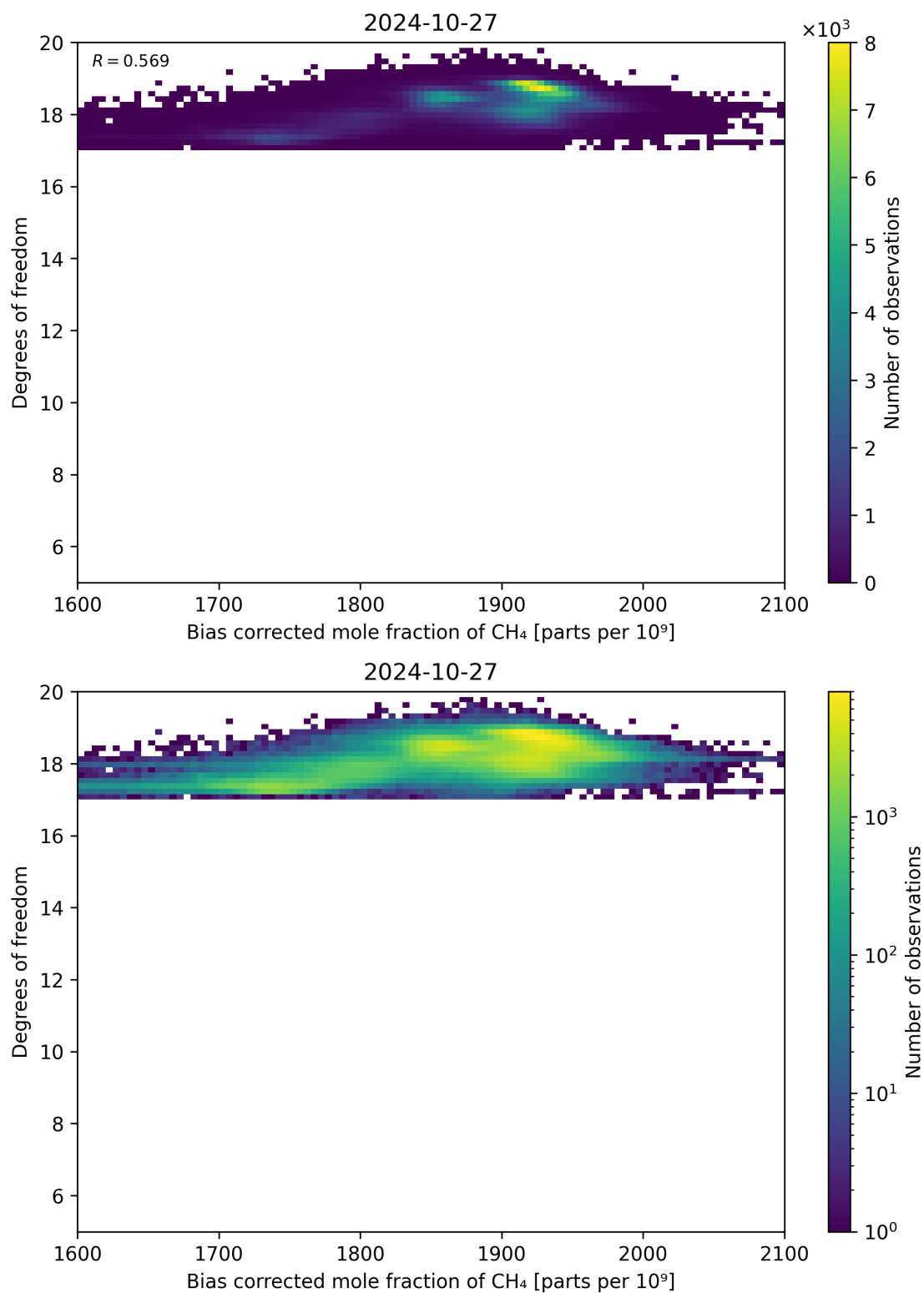
Figure 65: Scatter density plot of “Bias corrected mole fraction of CH 4 ” against “Degrees of freedom” for 2024-10-26 to 2024-10-28.
