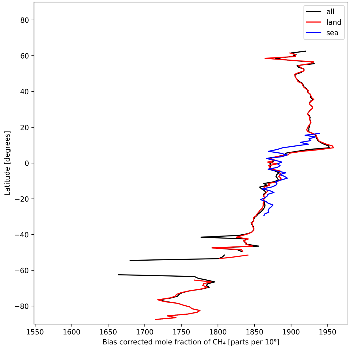
Figure 14: Zonal average of “Bias corrected mole fraction of CH 4 ” for 2024-10-26 to 2024-10-28.
