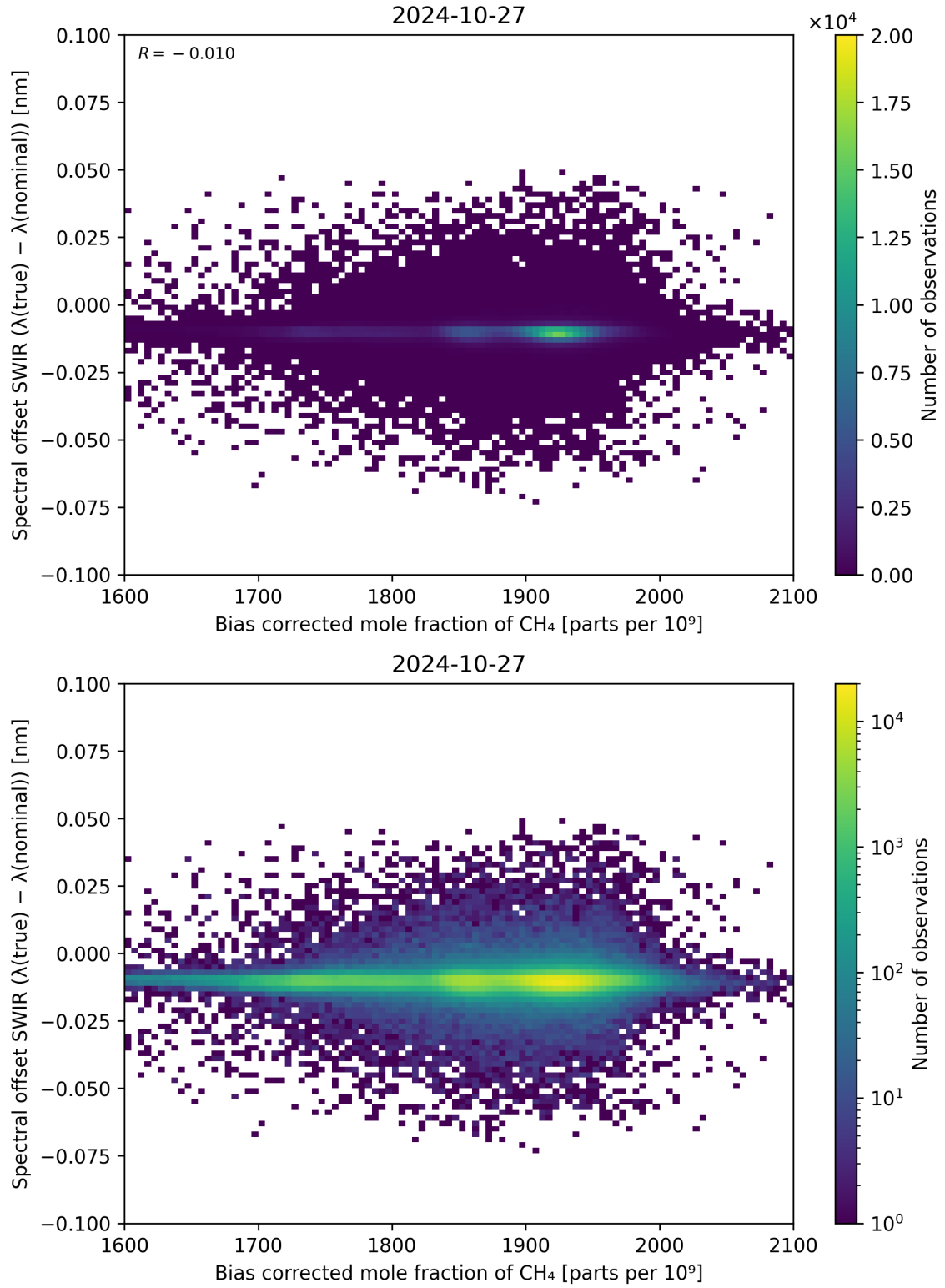
Figure 69: Scatter density plot of “Bias corrected mole fraction of CH 4 ” against “Spectral offset SWIR ( \lambda_{\text{true}} - \lambda_{\text{nominal}} )” for 2024-10-26 to 2024-10-28.
