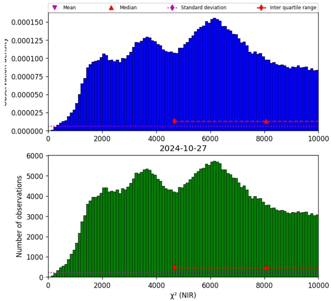
Figure 29: Histogram of “ \chi^2 (NIR)” for 2024-10-26 to 2024-10-28
