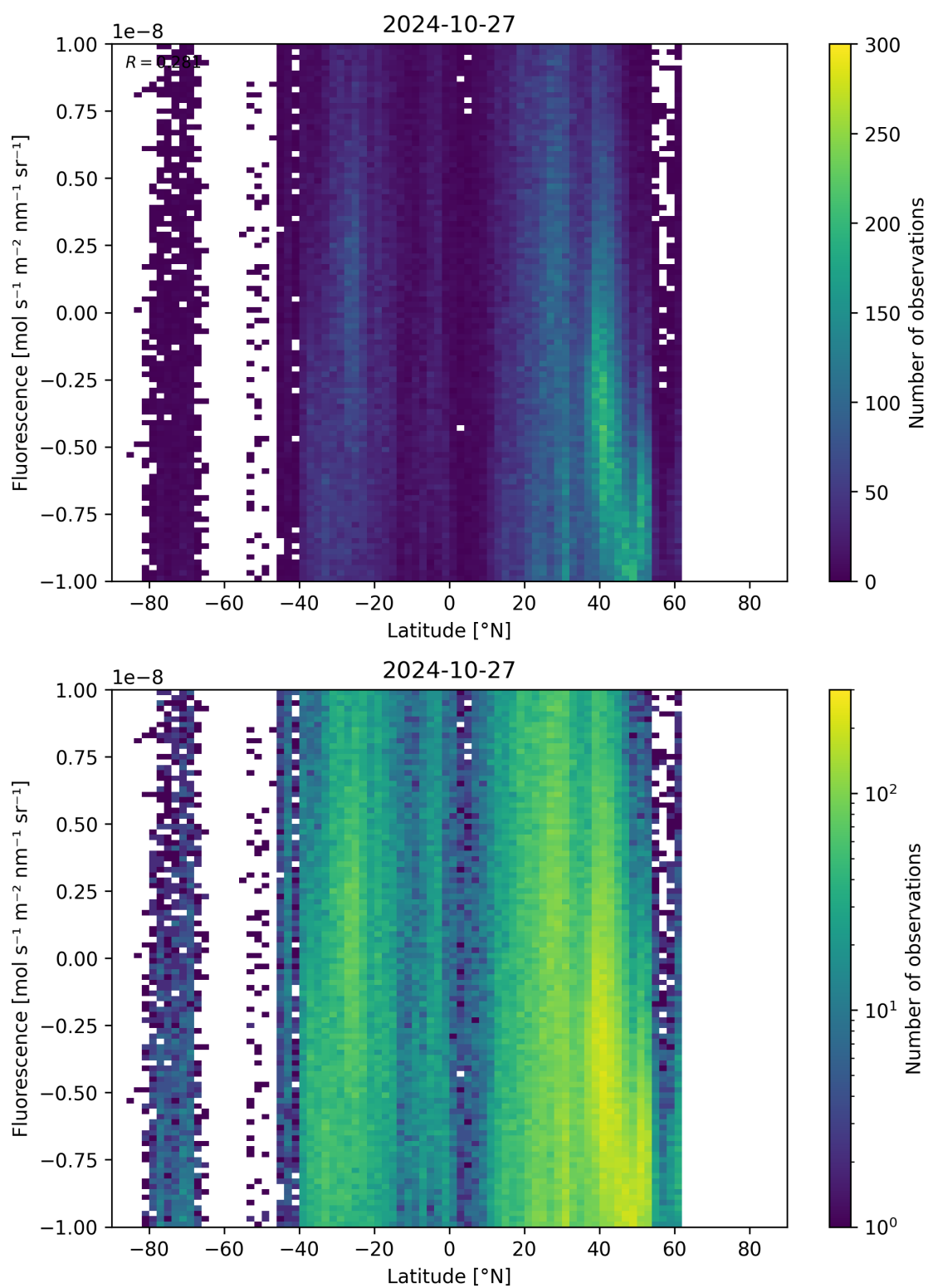
Figure 56: Scatter density plot of “Latitude” against “Fluorescence” for 2024-10-26 to 2024-10-28.
