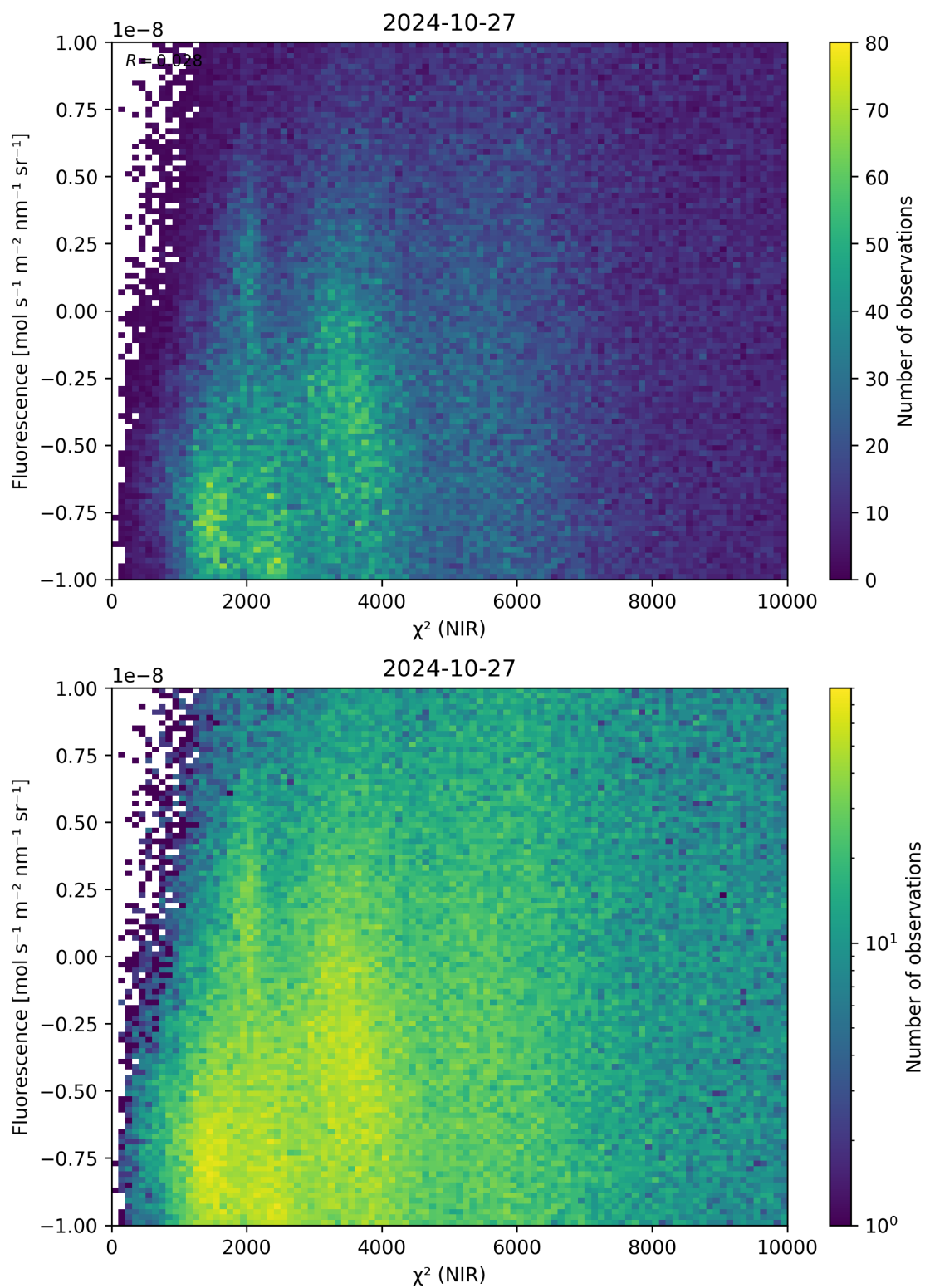
Figure 45: Scatter density plot of “ \chi^2 (NIR)” against “Fluorescence” for 2024-10-26 to 2024-10-28.
