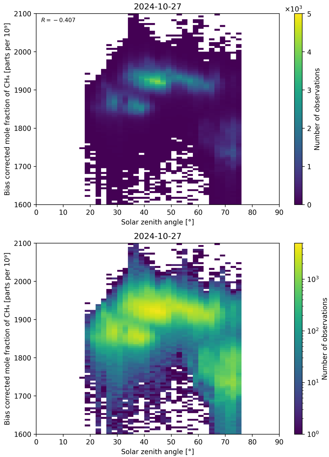
Figure 100: Scatter density plot of “Solar zenith angle” against “Bias corrected mole fraction of CH 4 ” for 2024-10-26 to 2024-10-28.
