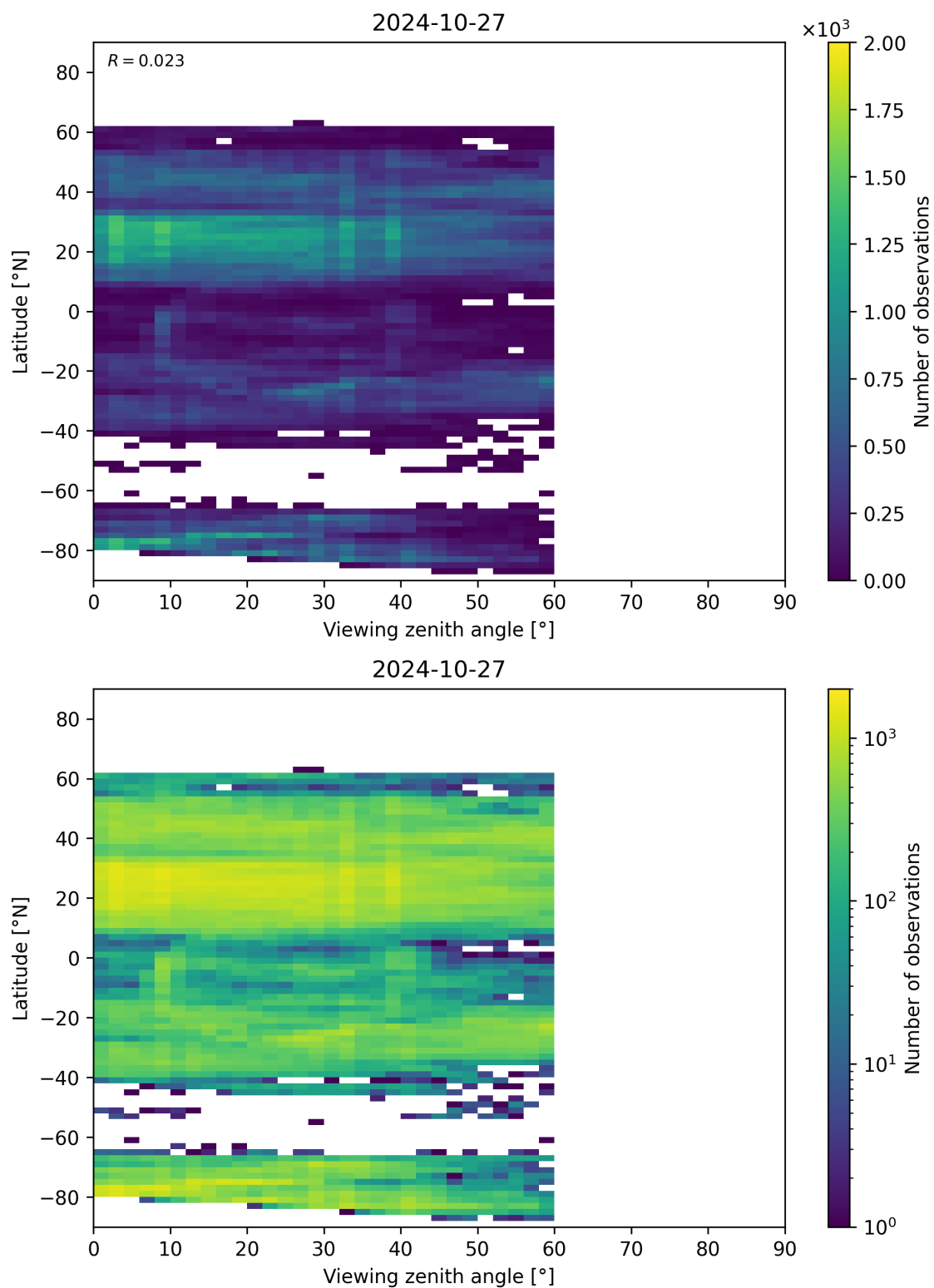
Figure 109: Scatter density plot of “Viewing zenith angle” against “Latitude” for 2024-10-26 to 2024-10-28.
