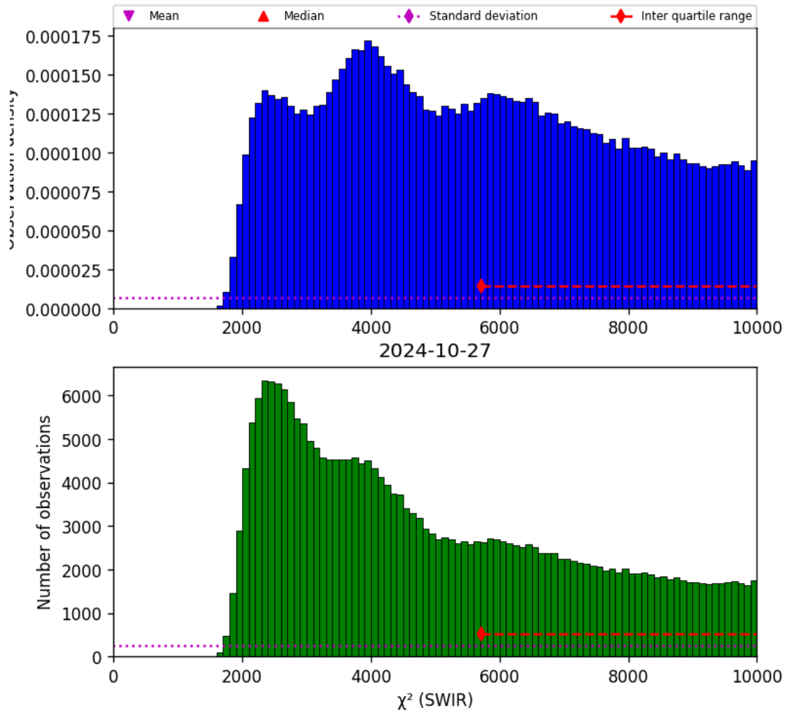
Figure 28: Histogram of “ \chi^2 (SWIR)” for 2024-10-26 to 2024-10-28
