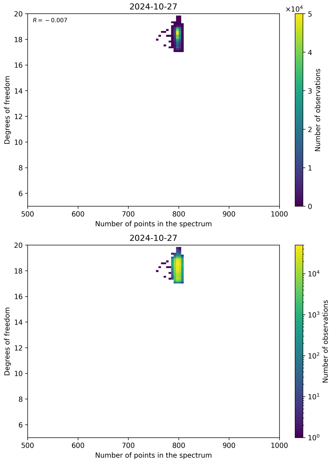
Figure 90: Scatter density plot of “Number of points in the spectrum” against “Degrees of freedom” for 2024-10-26 to 2024-10-28.
