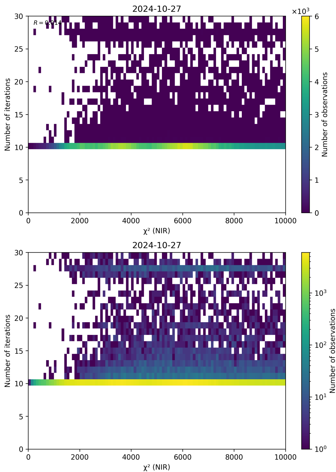
Figure 46: Scatter density plot of “ \chi^2 (NIR)” against “Number of iterations” for 2024-10-26 to 2024-10-28.
