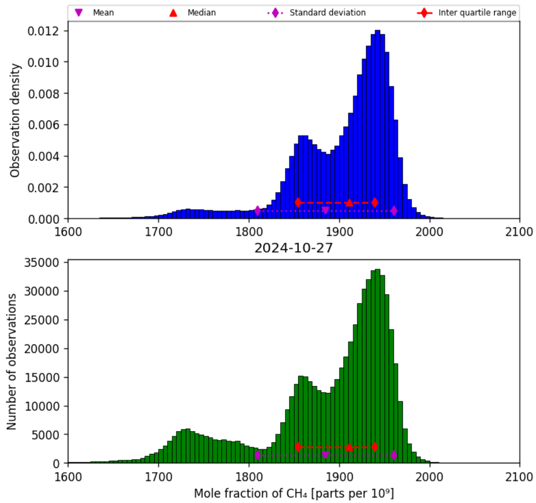
Figure 23: Histogram of “Mole fraction of CH 4 ” for 2024-10-26 to 2024-10-28
