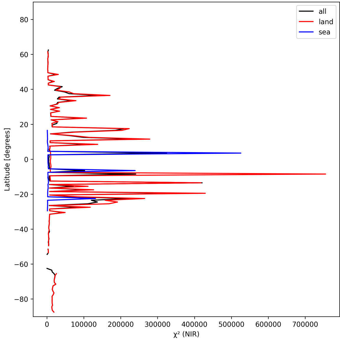
Figure 18: Zonal average of “ \chi^2 (NIR)” for 2024-10-26 to 2024-10-28.
