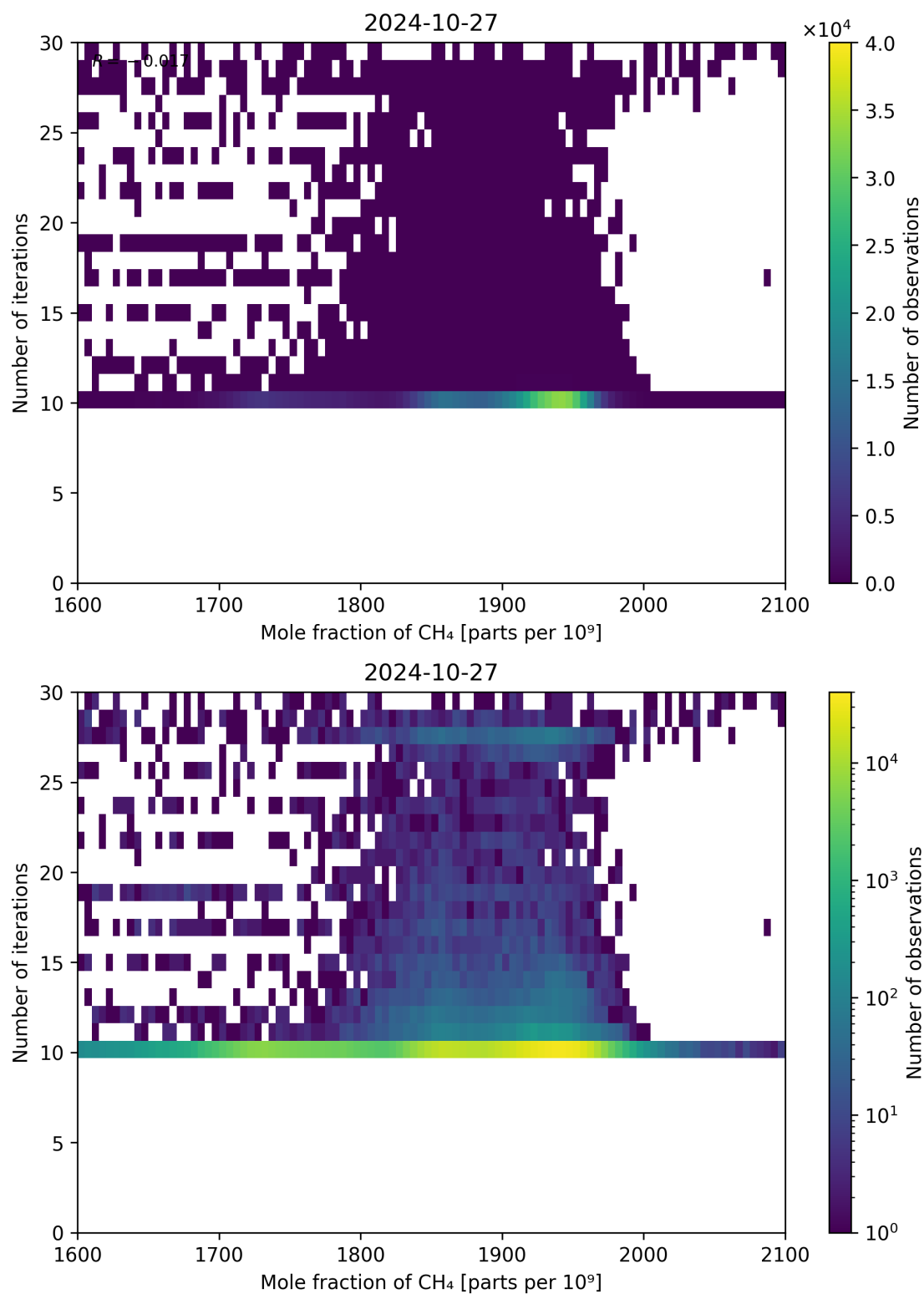
Figure 76: Scatter density plot of “Mole fraction of CH 4 ” against “Number of iterations” for 2024-10-26 to 2024-10-28.
