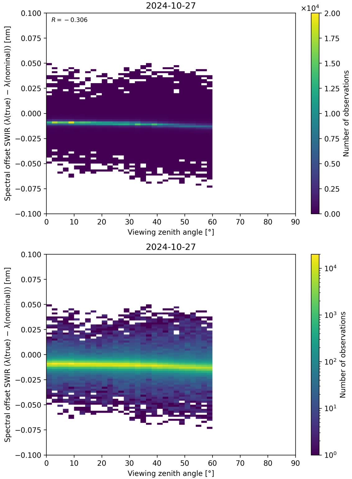
Figure 116: Scatter density plot of “Viewing zenith angle” against “Spectral offset SWIR ( \lambda_{\text{true}} - \lambda_{\text{nominal}} )” for 2024-10-26 to 2024-10-28.
