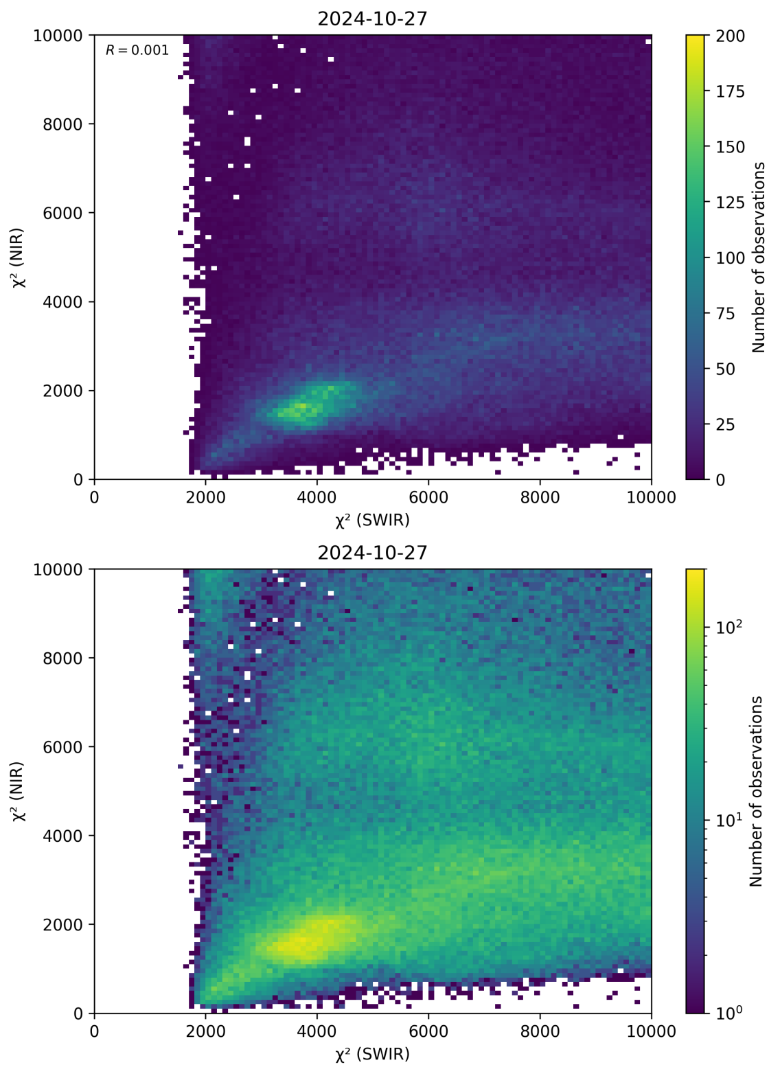
Figure 47: Scatter density plot of “ \chi^2 (SWIR)” against “ \chi^2 (NIR)” for 2024-10-26 to 2024-10-28.
