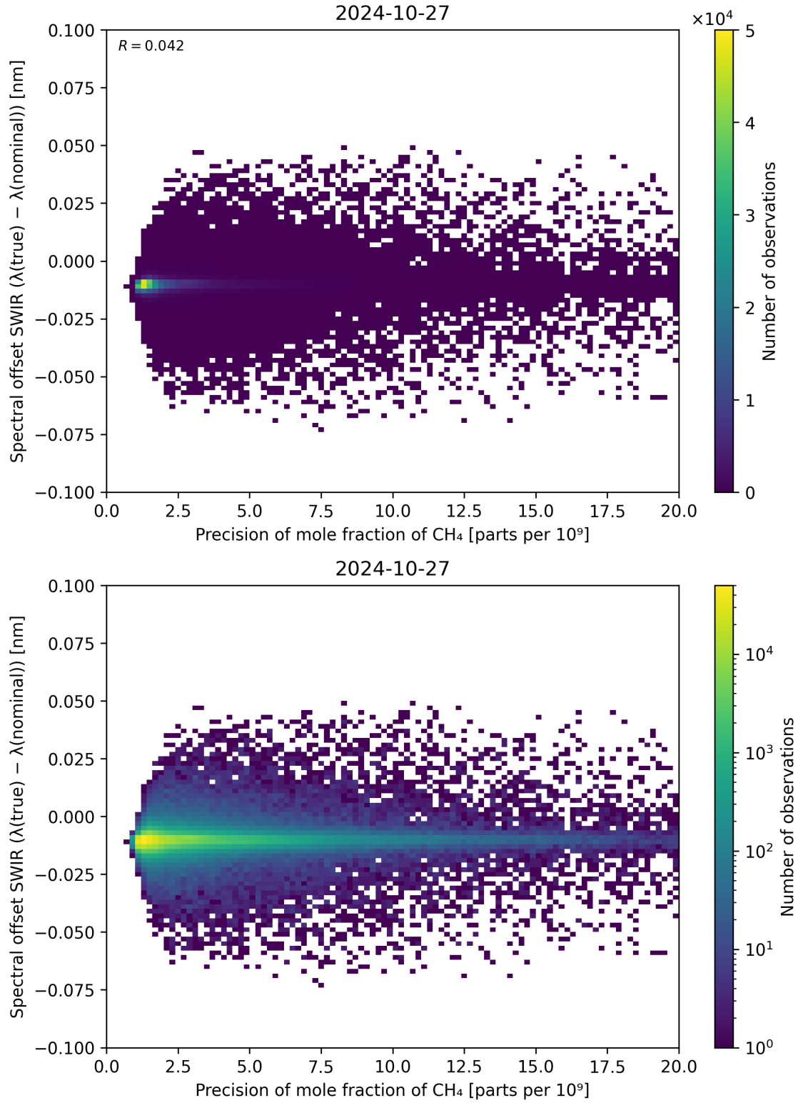
Figure 85: Scatter density plot of “Precision of mole fraction of CH 4 ” against “Spectral offset SWIR ( \lambda_{\text{true}} - \lambda_{\text{nominal}} )” for 2024-10-26 to 2024-10-28.
