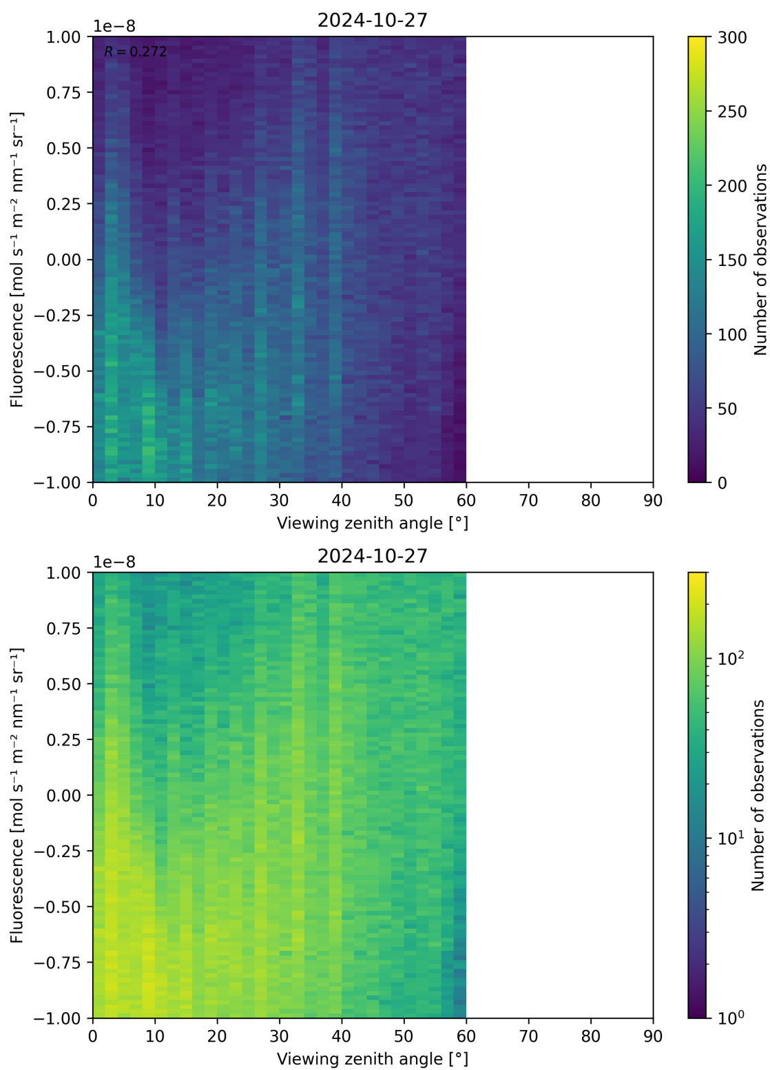
Figure 108: Scatter density plot of “Viewing zenith angle” against “Fluorescence” for 2024-10-26 to 2024-10-28.
