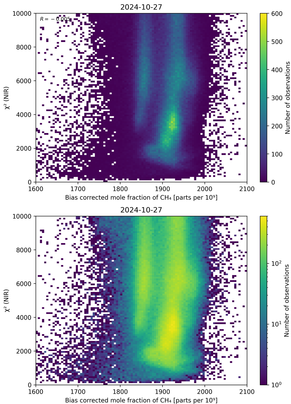
Figure 63: Scatter density plot of “Bias corrected mole fraction of CH 4 ” against “ \chi^2 (NIR)” for 2024-10-26 to 2024-10-28.
