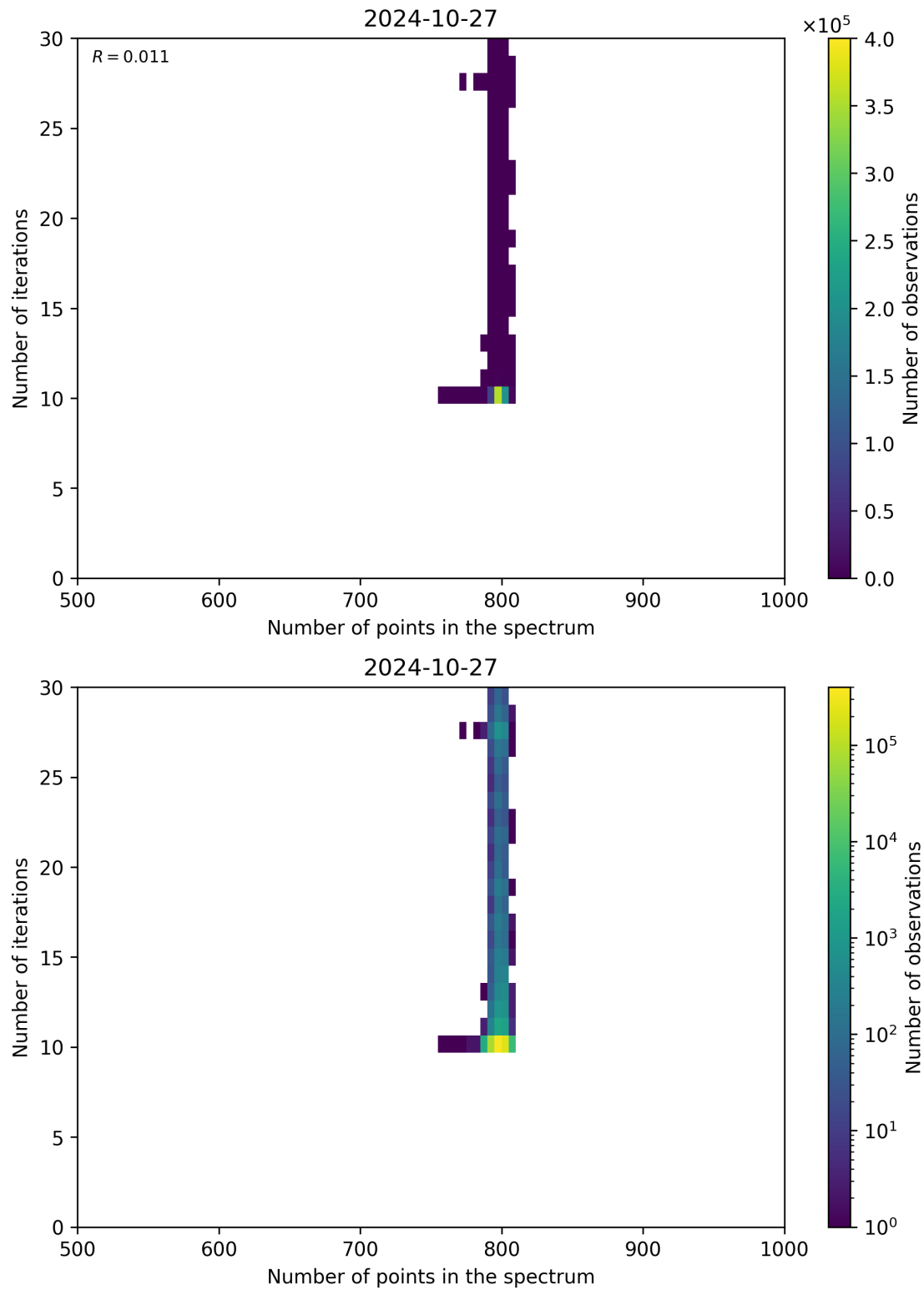
Figure 92: Scatter density plot of “Number of points in the spectrum” against “Number of iterations” for 2024-10-26 to 2024-10-28.
