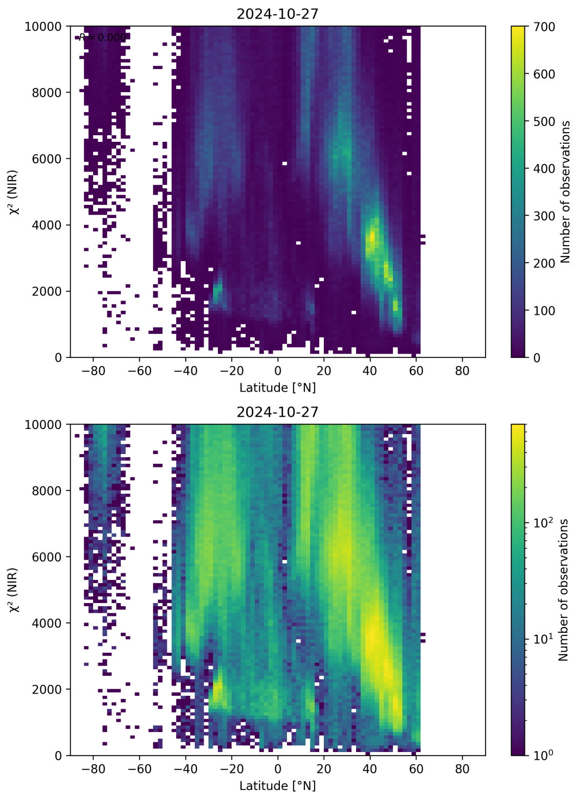
Figure 53: Scatter density plot of “Latitude” against “ \chi^2 (NIR)” for 2024-10-26 to 2024-10-28.
