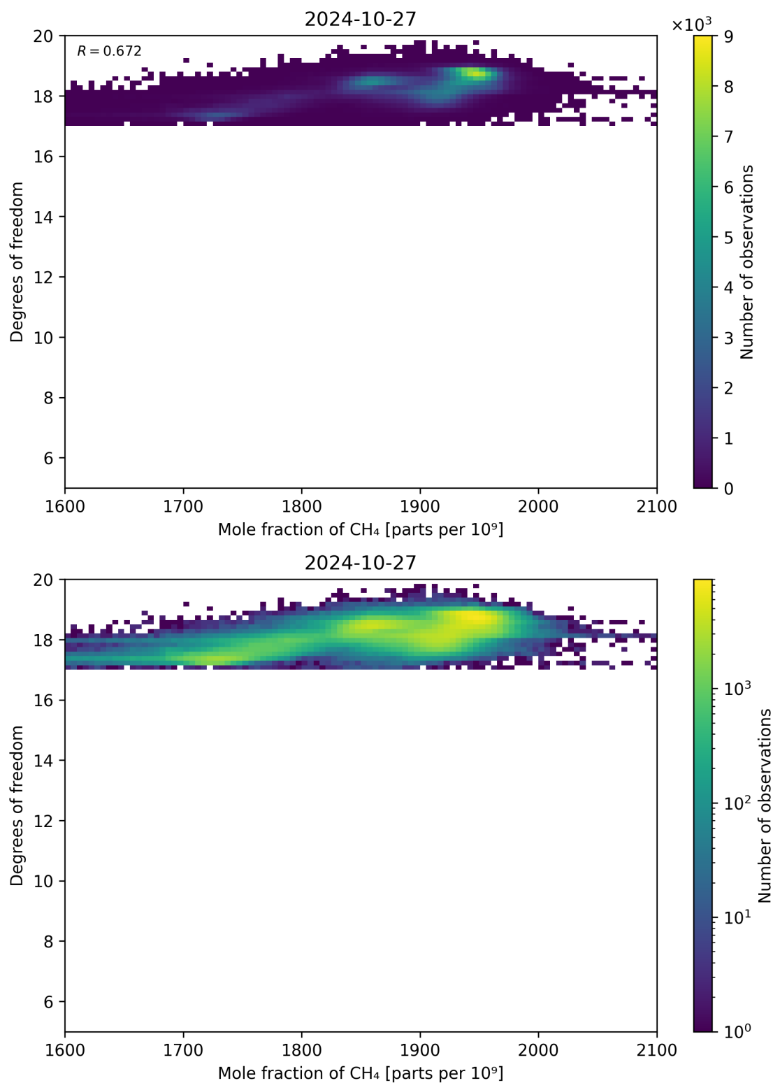
Figure 72: Scatter density plot of “Mole fraction of CH 4 ” against “Degrees of freedom” for 2024-10-26 to 2024-10-28.
