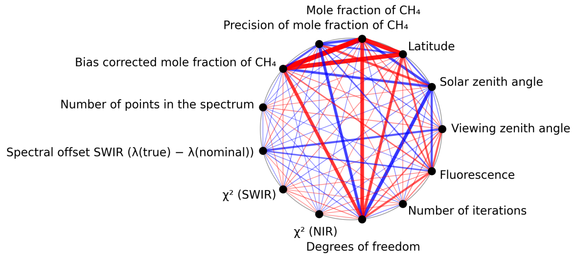
Figure 1: Map of correlation graph for 2024-10-26 to 2024-10-28.
