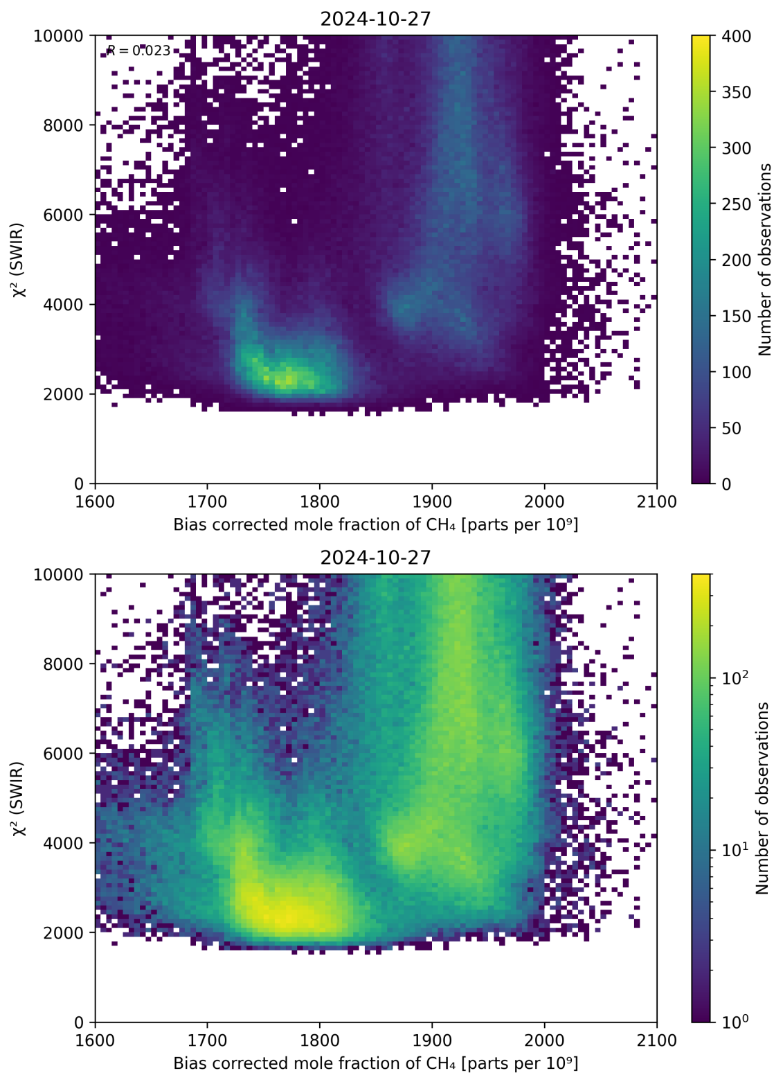
Figure 64: Scatter density plot of “Bias corrected mole fraction of \text{CH}_4 ” against “ \chi^2 (SWIR)” for 2024-10-26 to 2024-10-28.
