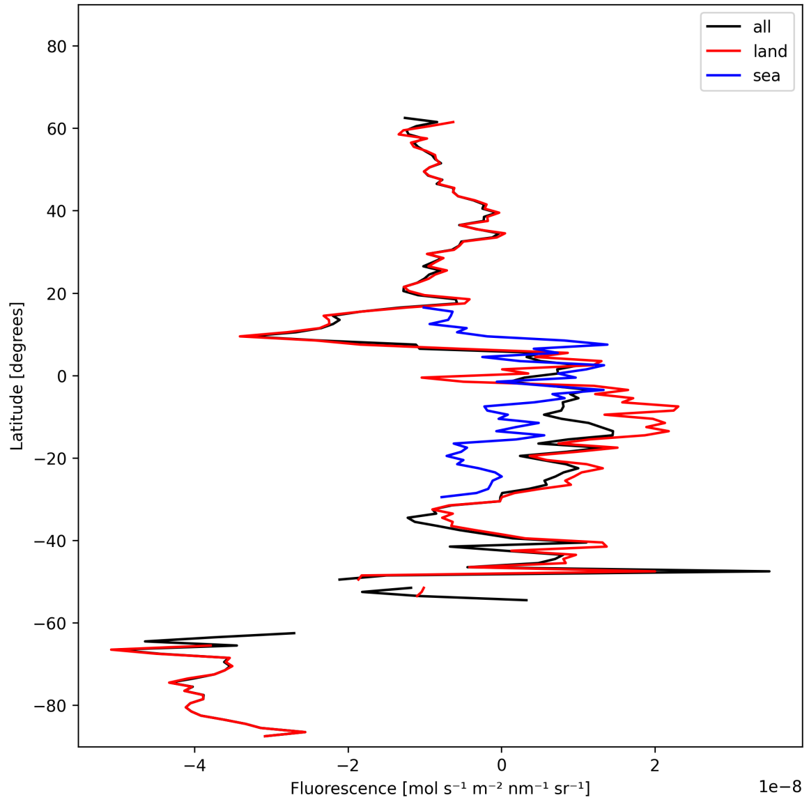
Figure 21: Zonal average of “Fluorescence” for 2024-10-26 to 2024-10-28.
