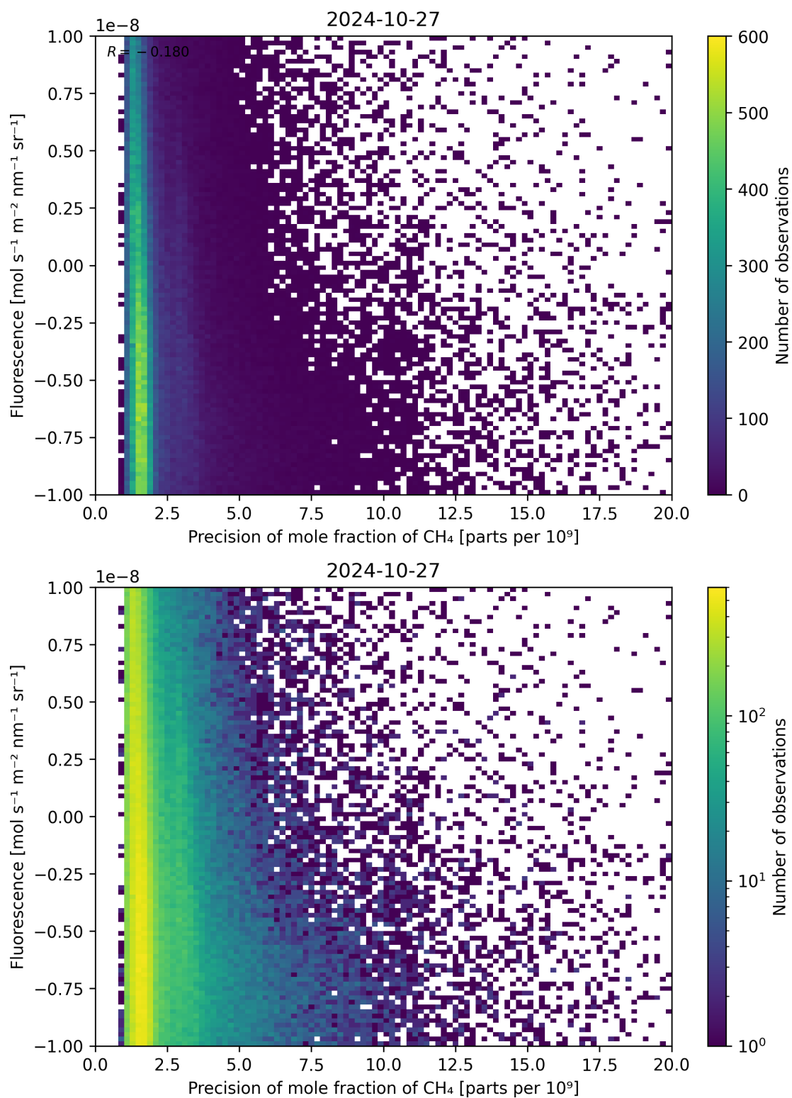
Figure 81: Scatter density plot of “Precision of mole fraction of \text{CH}_4 ” against “Fluorescence” for 2024-10-26 to 2024-10-28.
