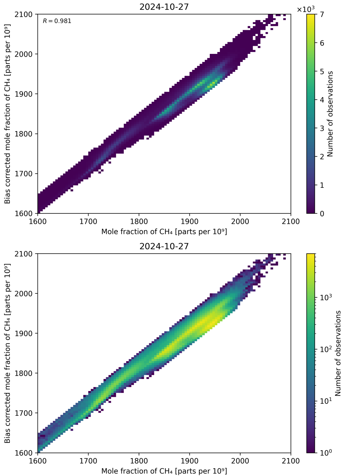
Figure 74: Scatter density plot of “Mole fraction of CH 4 ” against “Bias corrected mole fraction of CH 4 ” for 2024-10-26 to 2024-10-28.
