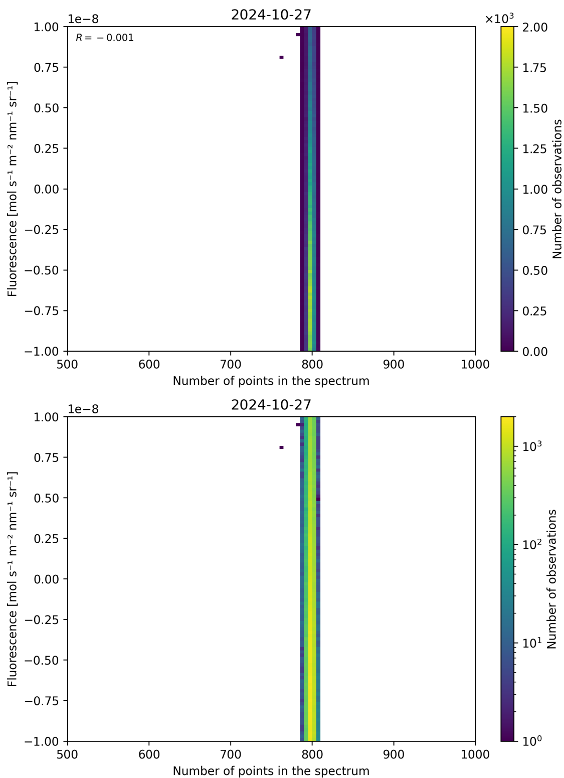
Figure 91: Scatter density plot of “Number of points in the spectrum” against “Fluorescence” for 2024-10-26 to 2024-10-28.
