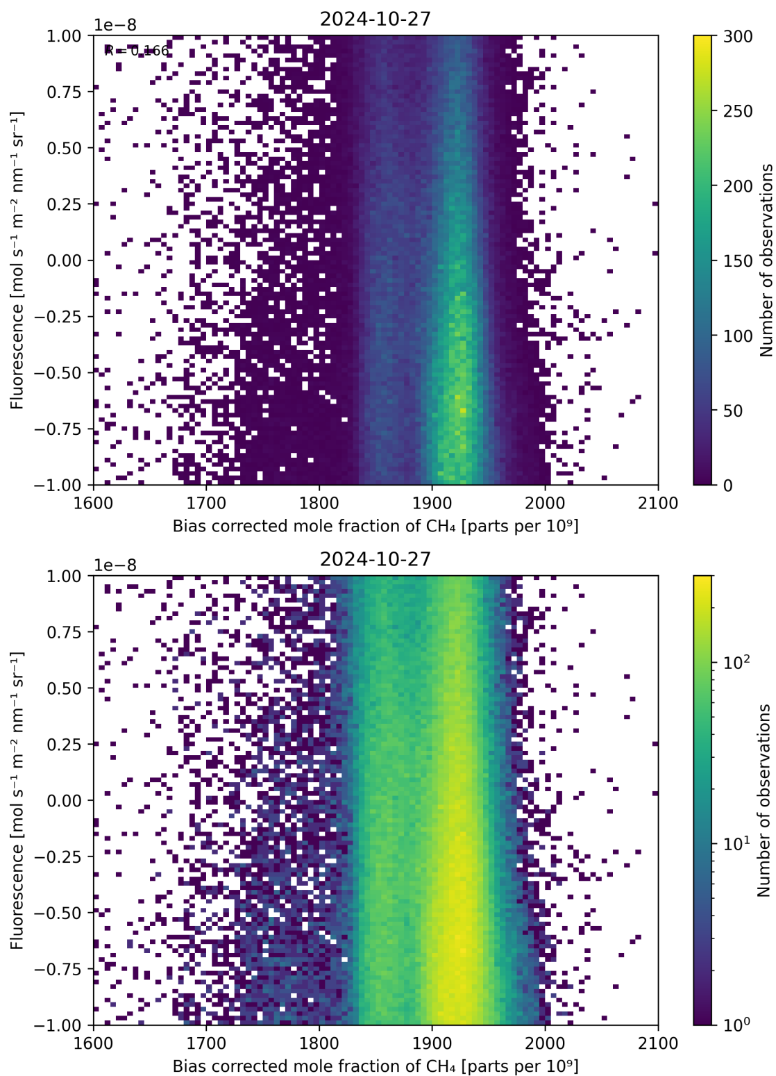
Figure 66: Scatter density plot of “Bias corrected mole fraction of \text{CH}_4 ” against “Fluorescence” for 2024-10-26 to 2024-10-28.
