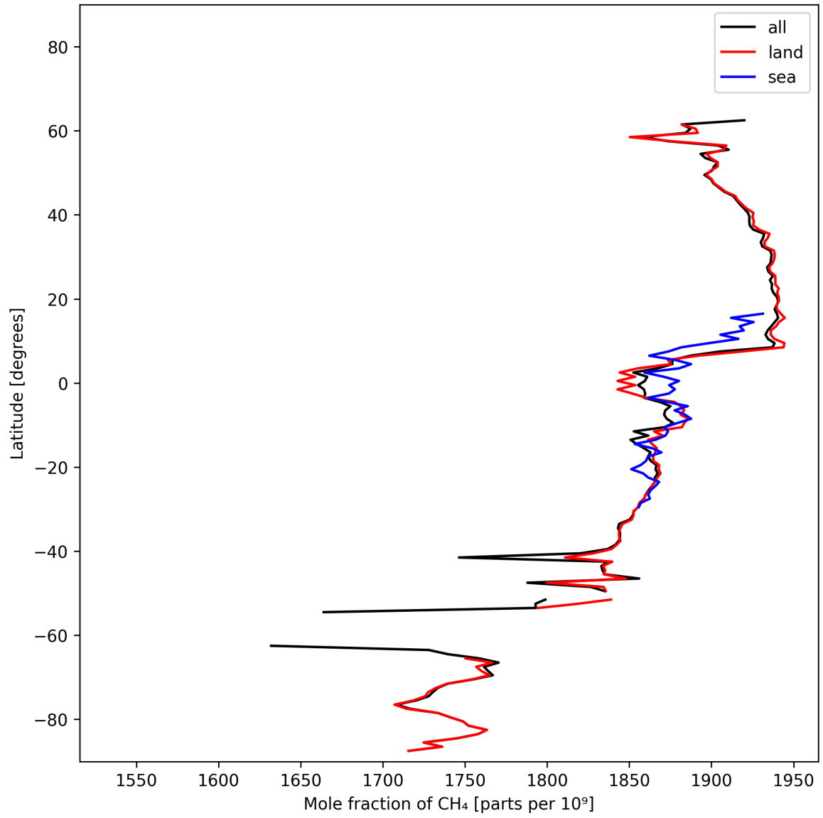
Figure 12: Zonal average of “Mole fraction of \text{CH}_4 ” for 2024-10-26 to 2024-10-28.
