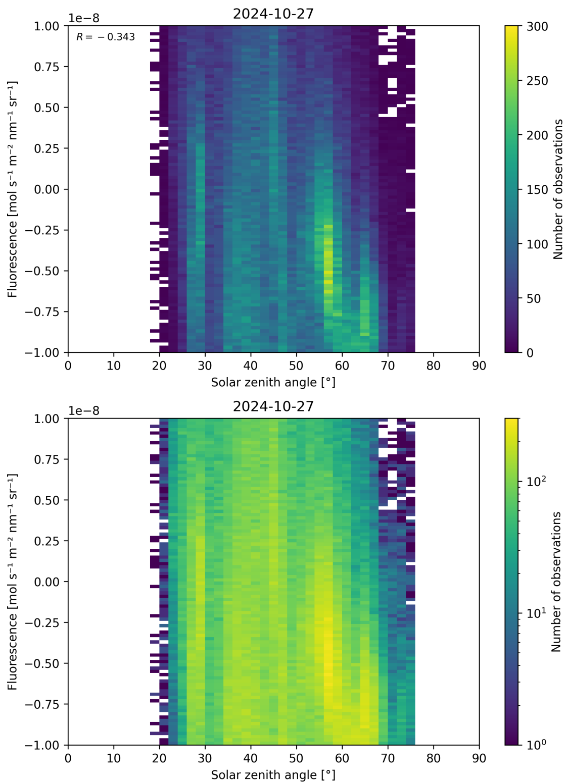
Figure 97: Scatter density plot of “Solar zenith angle” against “Fluorescence” for 2024-10-26 to 2024-10-28.
