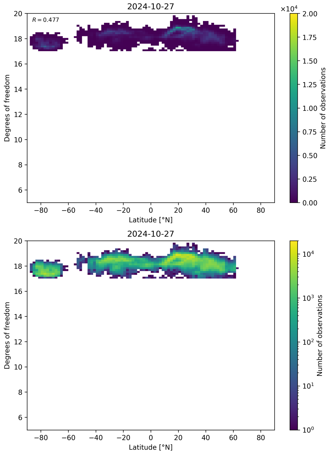
Figure 55: Scatter density plot of “Latitude” against “Degrees of freedom” for 2024-10-26 to 2024-10-28.
