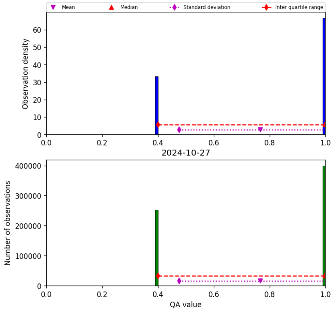
Figure 22: Histogram of “QA value” for 2024-10-26 to 2024-10-28
