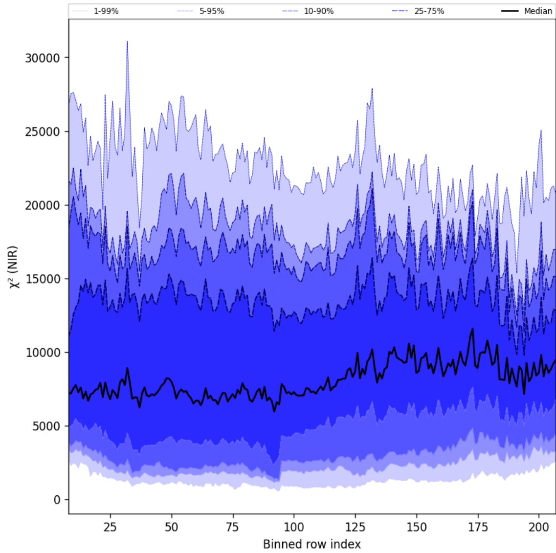
Figure 40: Along track statistics of “ \chi^2 (NIR)” for 2024-10-26 to 2024-10-28
