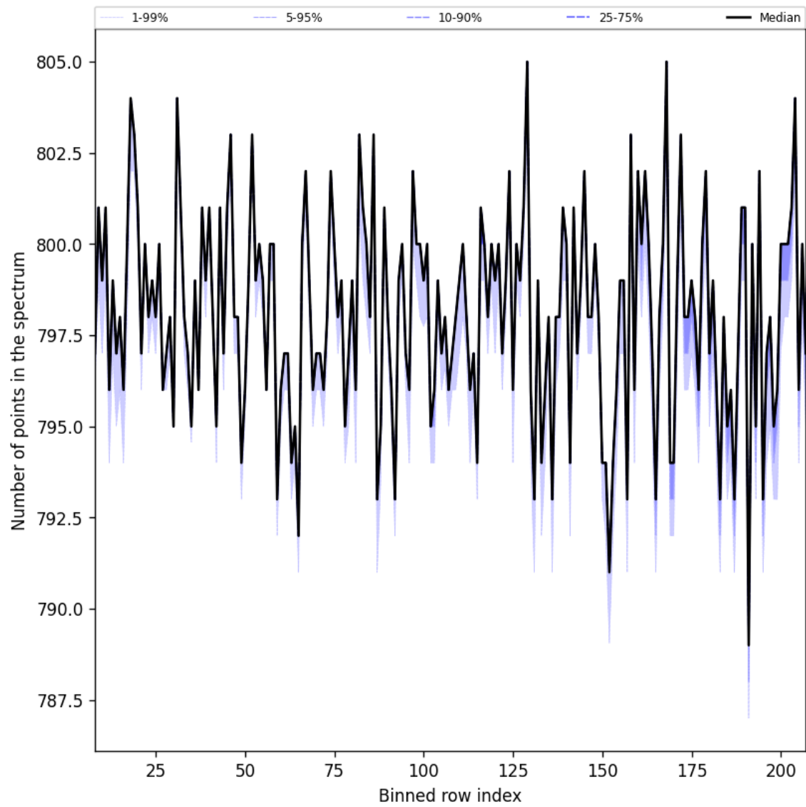
Figure 37: Along track statistics of “Number of points in the spectrum” for 2024-10-26 to 2024-10-28
