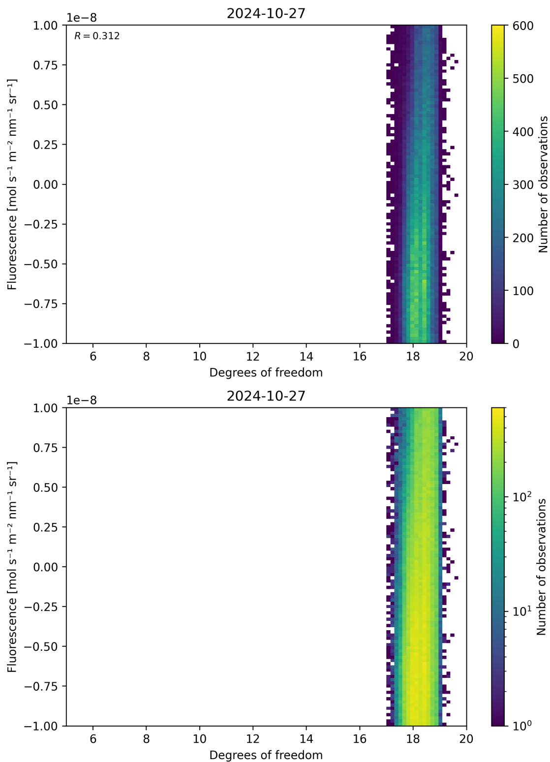
Figure 51: Scatter density plot of “Degrees of freedom” against “Fluorescence” for 2024-10-26 to 2024-10-28.
