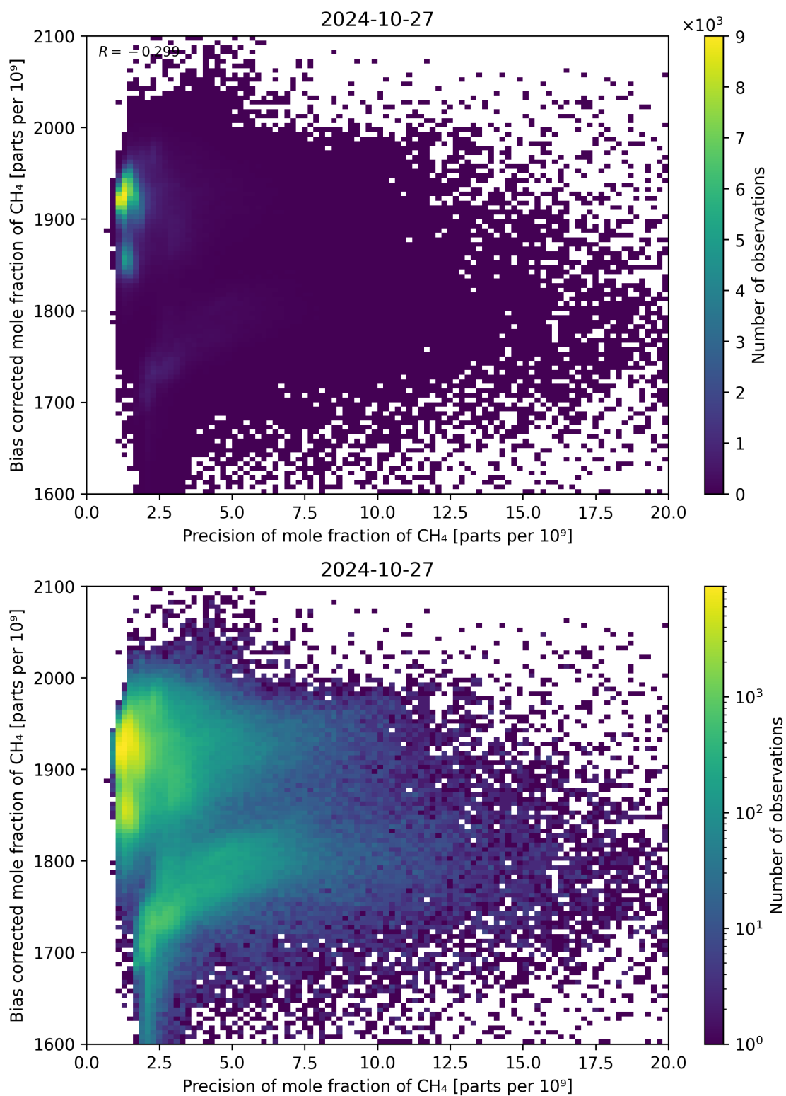
Figure 82: Scatter density plot of “Precision of mole fraction of CH 4 ” against “Bias corrected mole fraction of CH 4 ” for 2024-10-26 to 2024-10-28.
