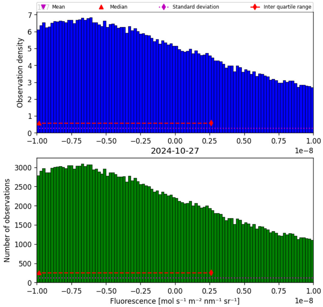
Figure 32: Histogram of “Fluorescence” for 2024-10-26 to 2024-10-28
