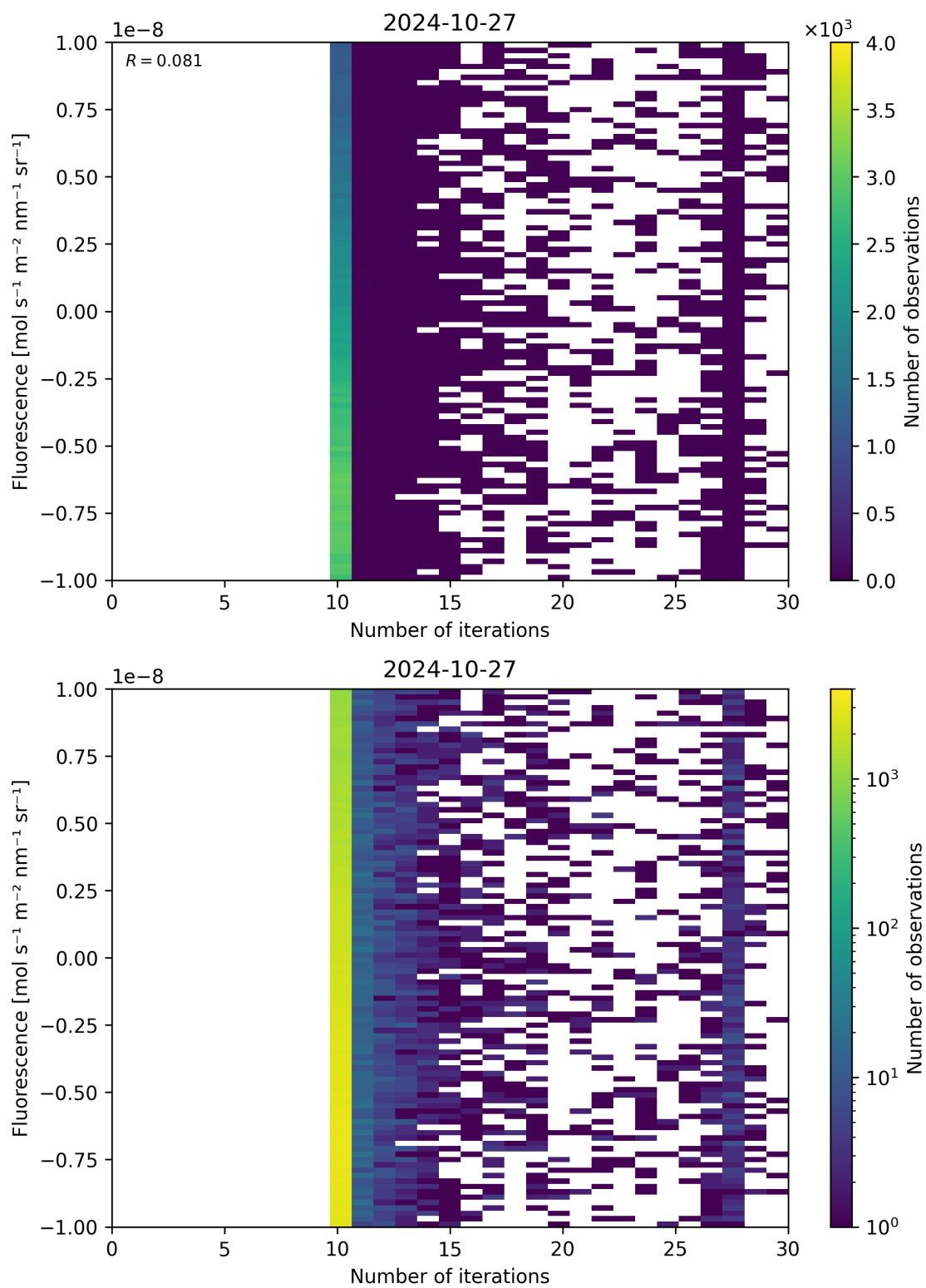
Figure 87: Scatter density plot of “Number of iterations” against “Fluorescence” for 2024-10-26 to 2024-10-28.
