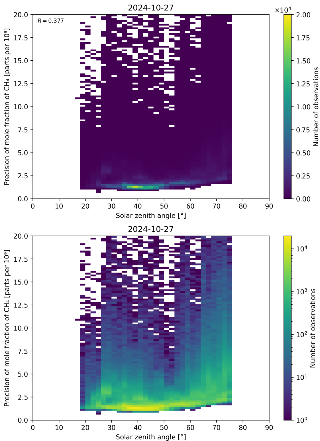
Figure 101: Scatter density plot of “Solar zenith angle” against “Precision of mole fraction of \text{CH}_4 ” for 2024-10-26 to 2024-10-28.
