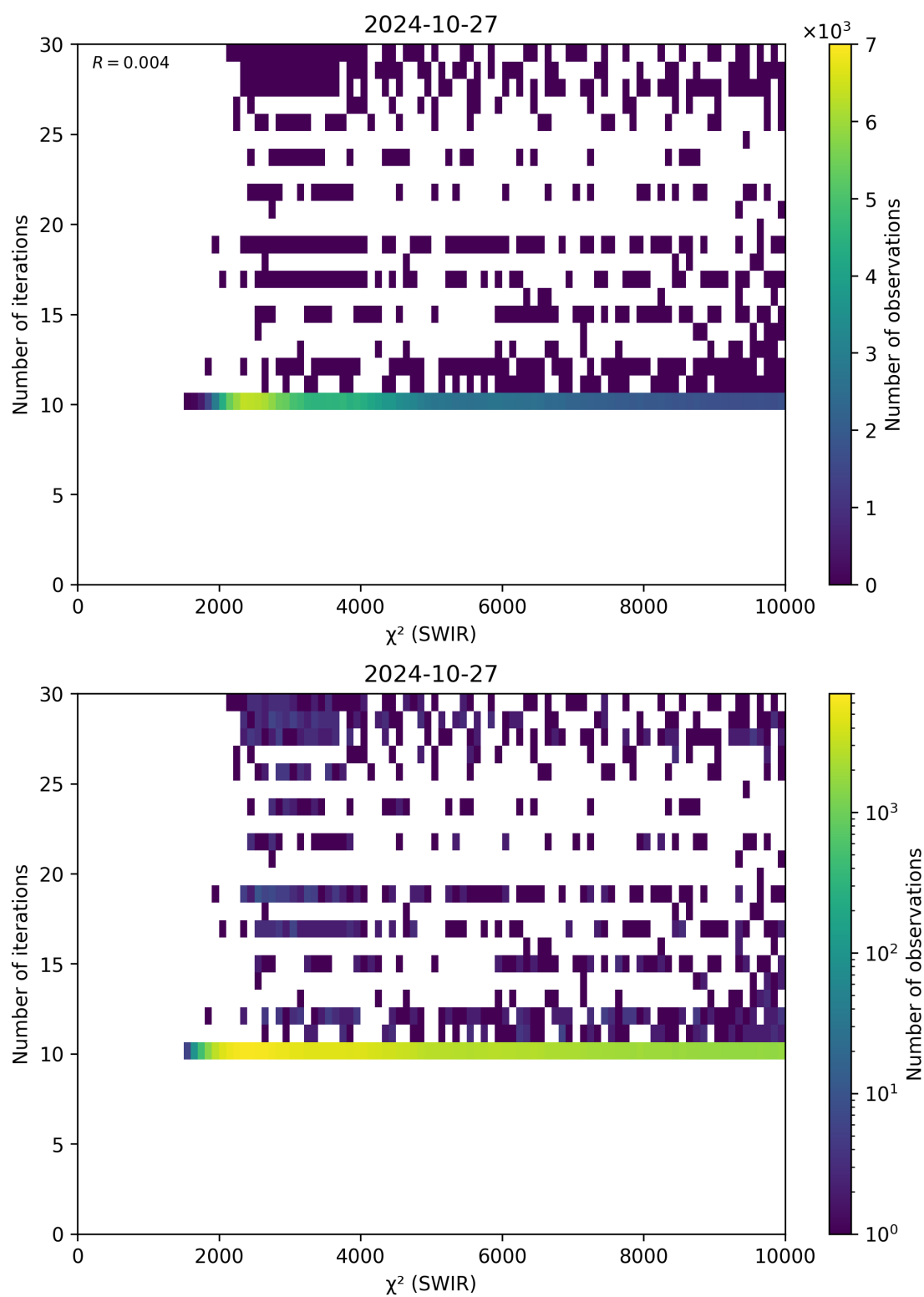
Figure 50: Scatter density plot of “ \chi^2 (SWIR)” against “Number of iterations” for 2024-10-26 to 2024-10-28.
