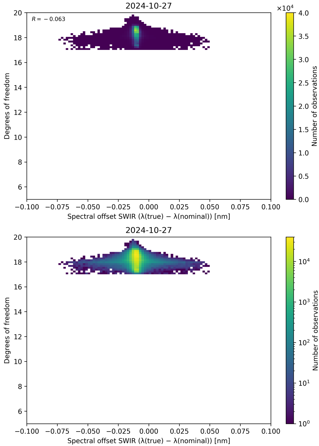
Figure 119: Scatter density plot of “Spectral offset SWIR ( \lambda_{\text{true}} - \lambda_{\text{nominal}} )” against “Degrees of freedom” for 2024-10-26 to 2024-10-28.
