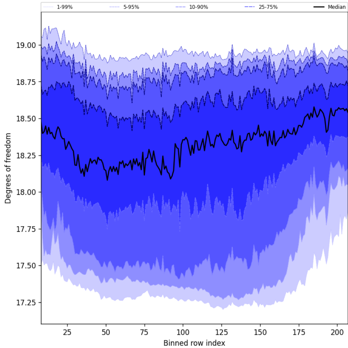
Figure 41: Along track statistics of “Degrees of freedom” for 2024-10-26 to 2024-10-28
