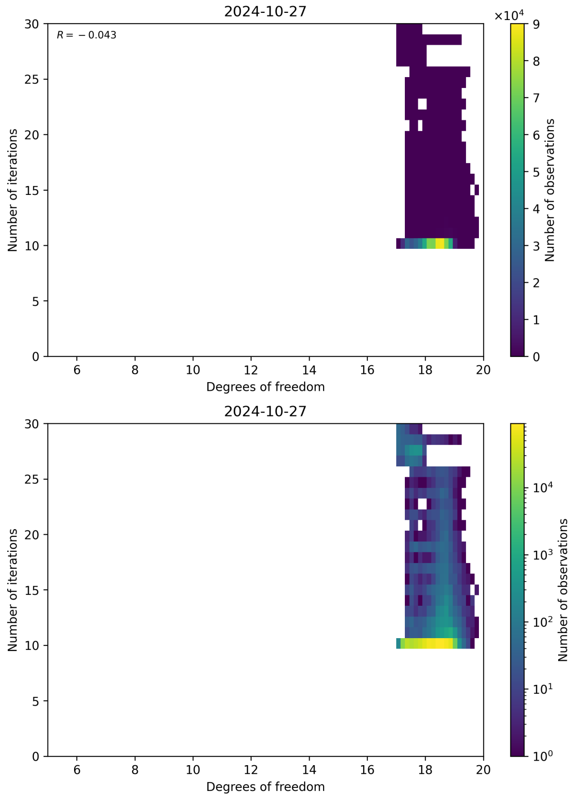
Figure 52: Scatter density plot of “Degrees of freedom” against “Number of iterations” for 2024-10-26 to 2024-10-28.
