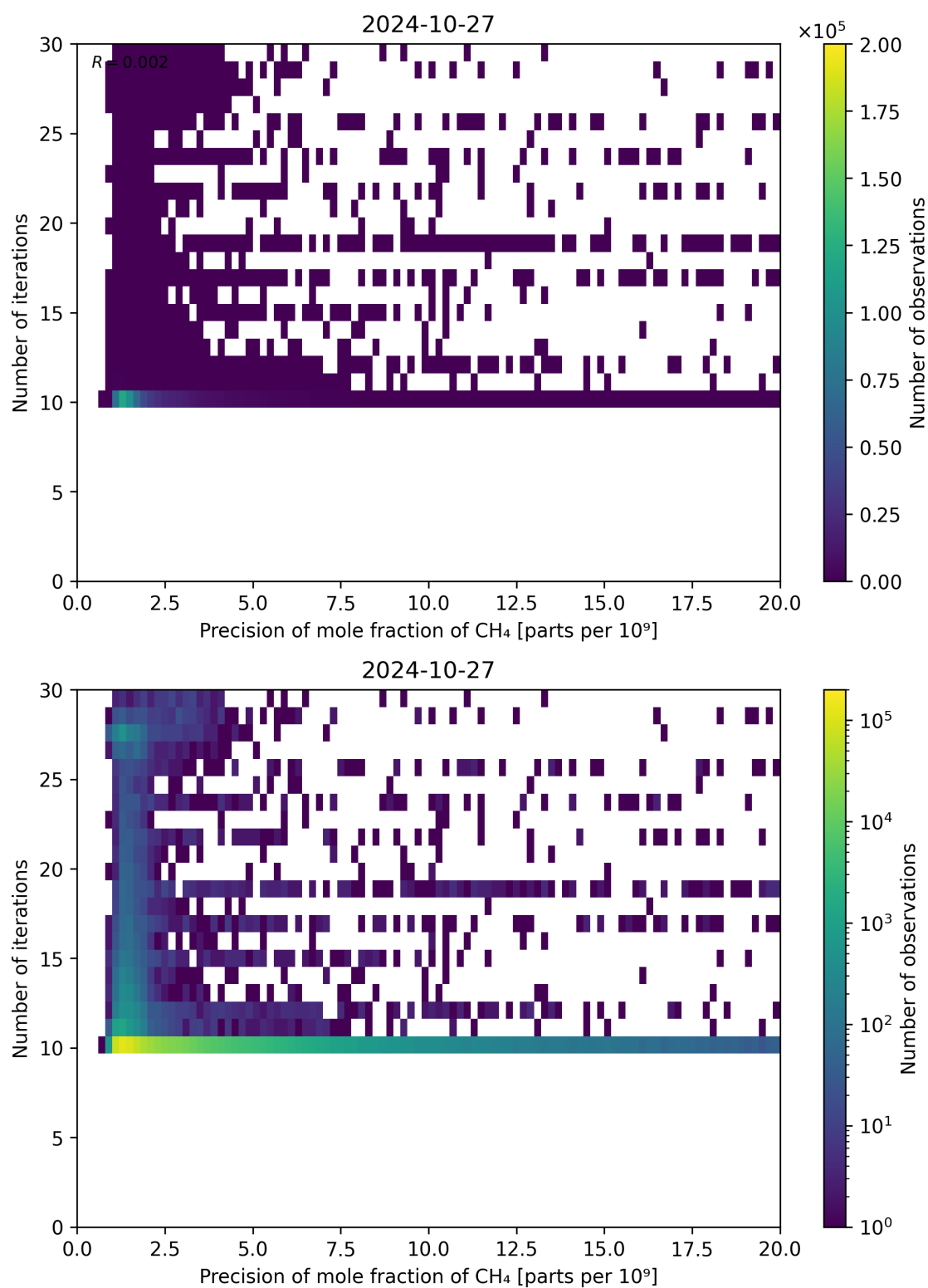
Figure 83: Scatter density plot of “Precision of mole fraction of CH 4 ” against “Number of iterations” for 2024-10-26 to 2024-10-28.
