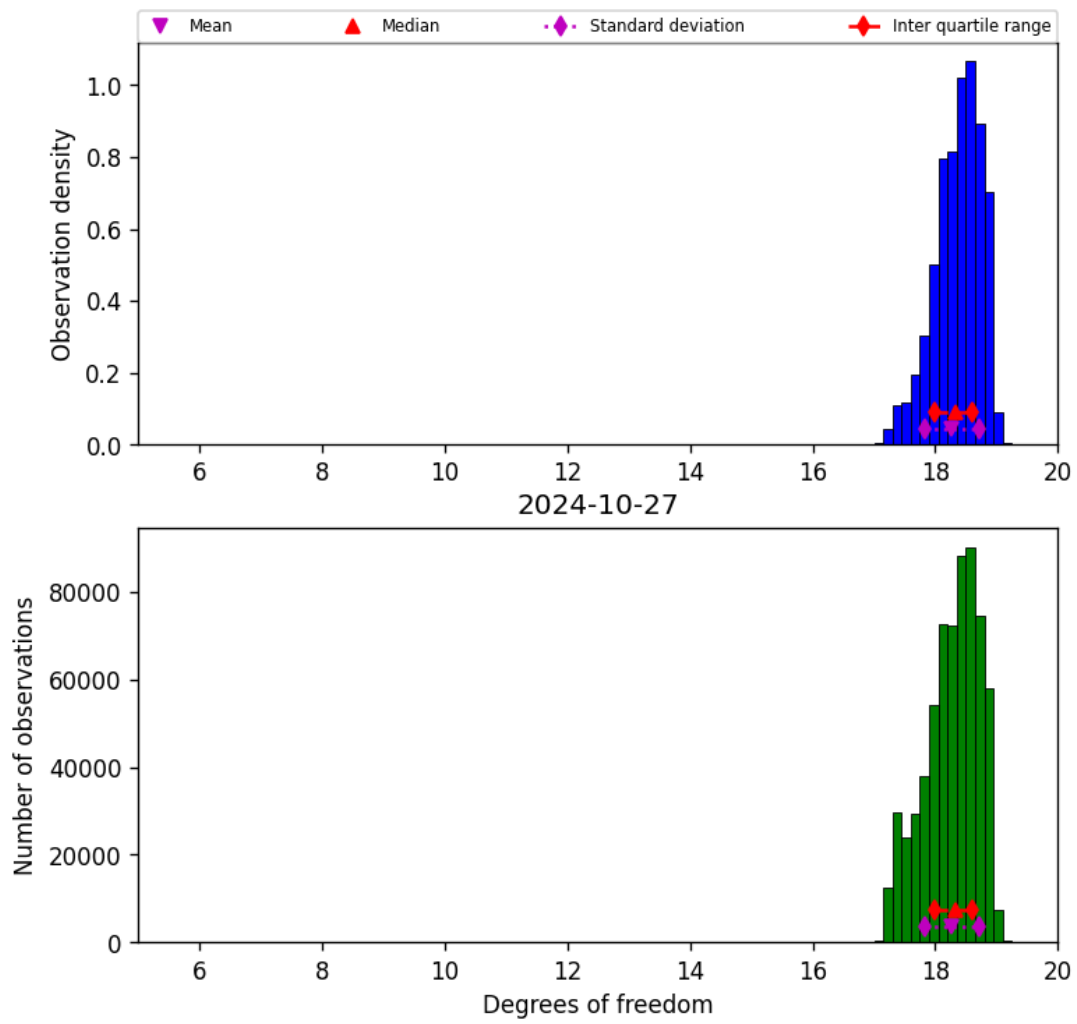
Figure 30: Histogram of “Degrees of freedom” for 2024-10-26 to 2024-10-28
