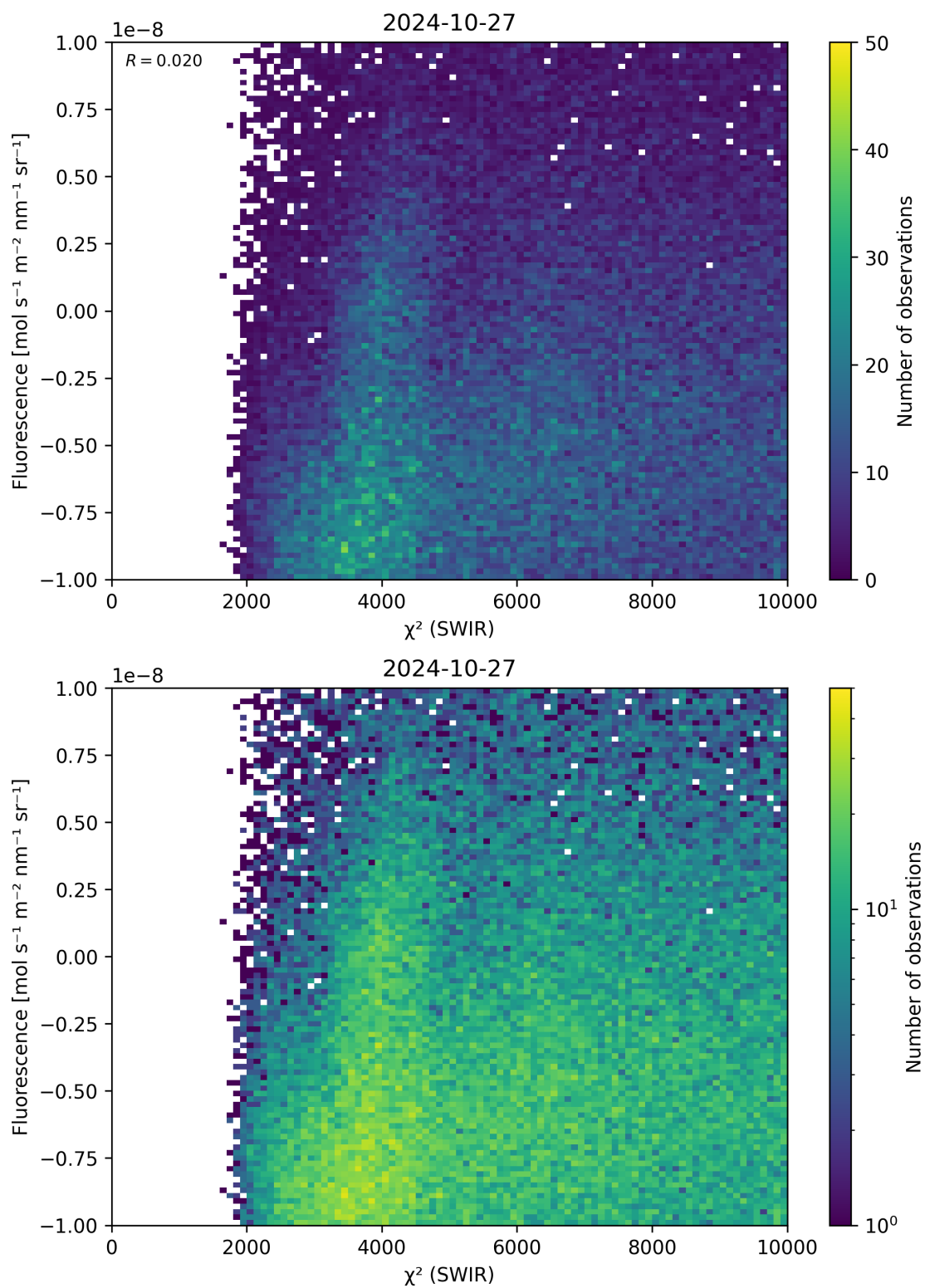
Figure 49: Scatter density plot of “ \chi^2 (SWIR)” against “Fluorescence” for 2024-10-26 to 2024-10-28.
