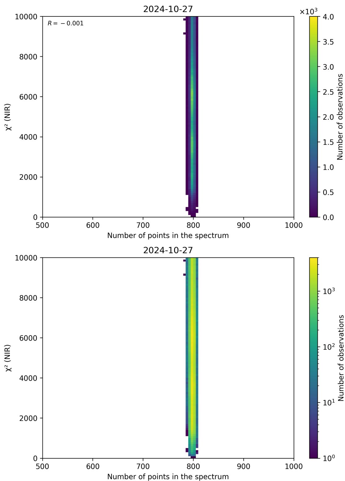
Figure 88: Scatter density plot of “Number of points in the spectrum” against “ \chi^2 (NIR)” for 2024-10-26 to 2024-10-28.
