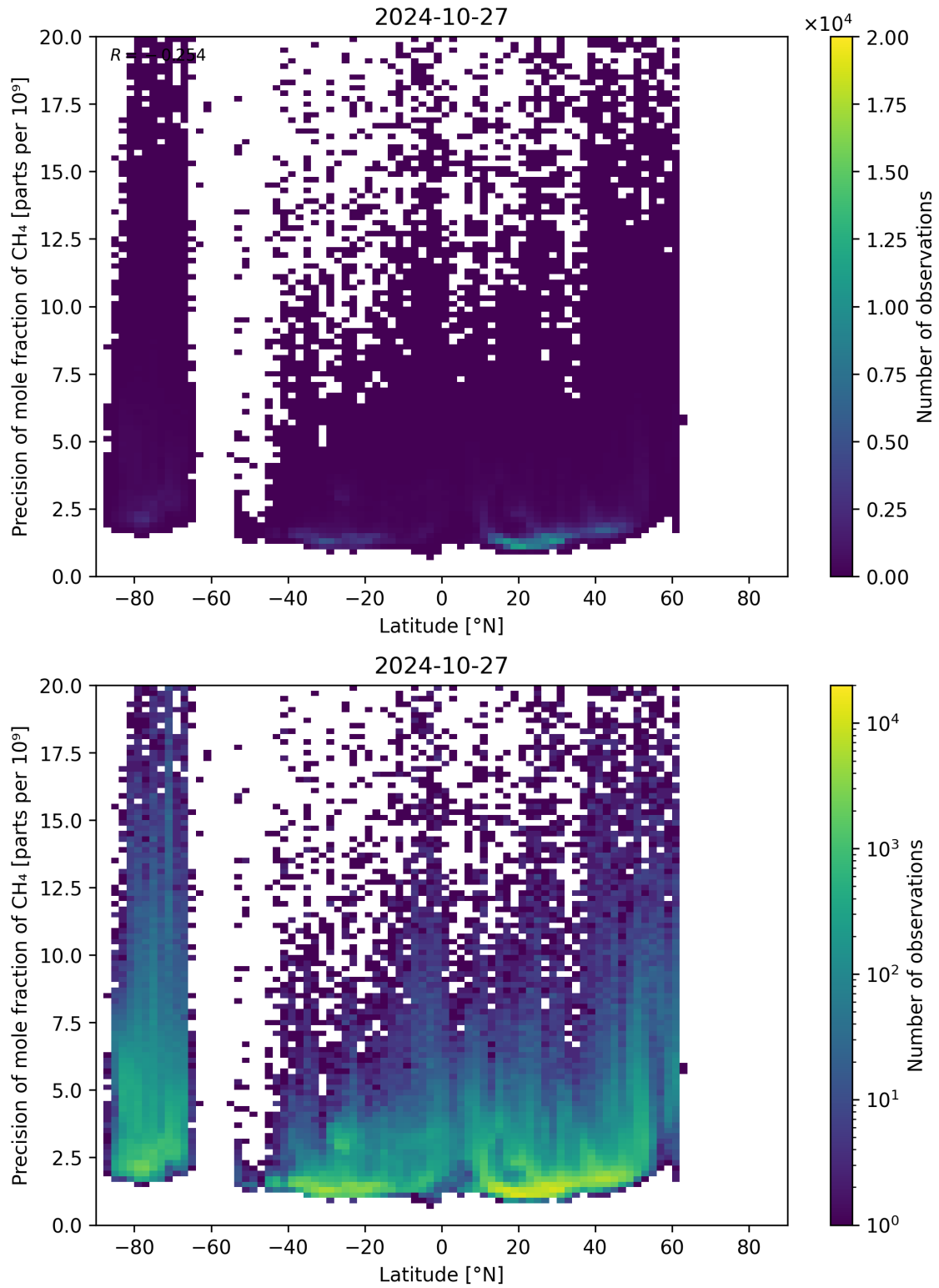
Figure 59: Scatter density plot of “Latitude” against “Precision of mole fraction of CH 4 ” for 2024-10-26 to 2024-10-28.
