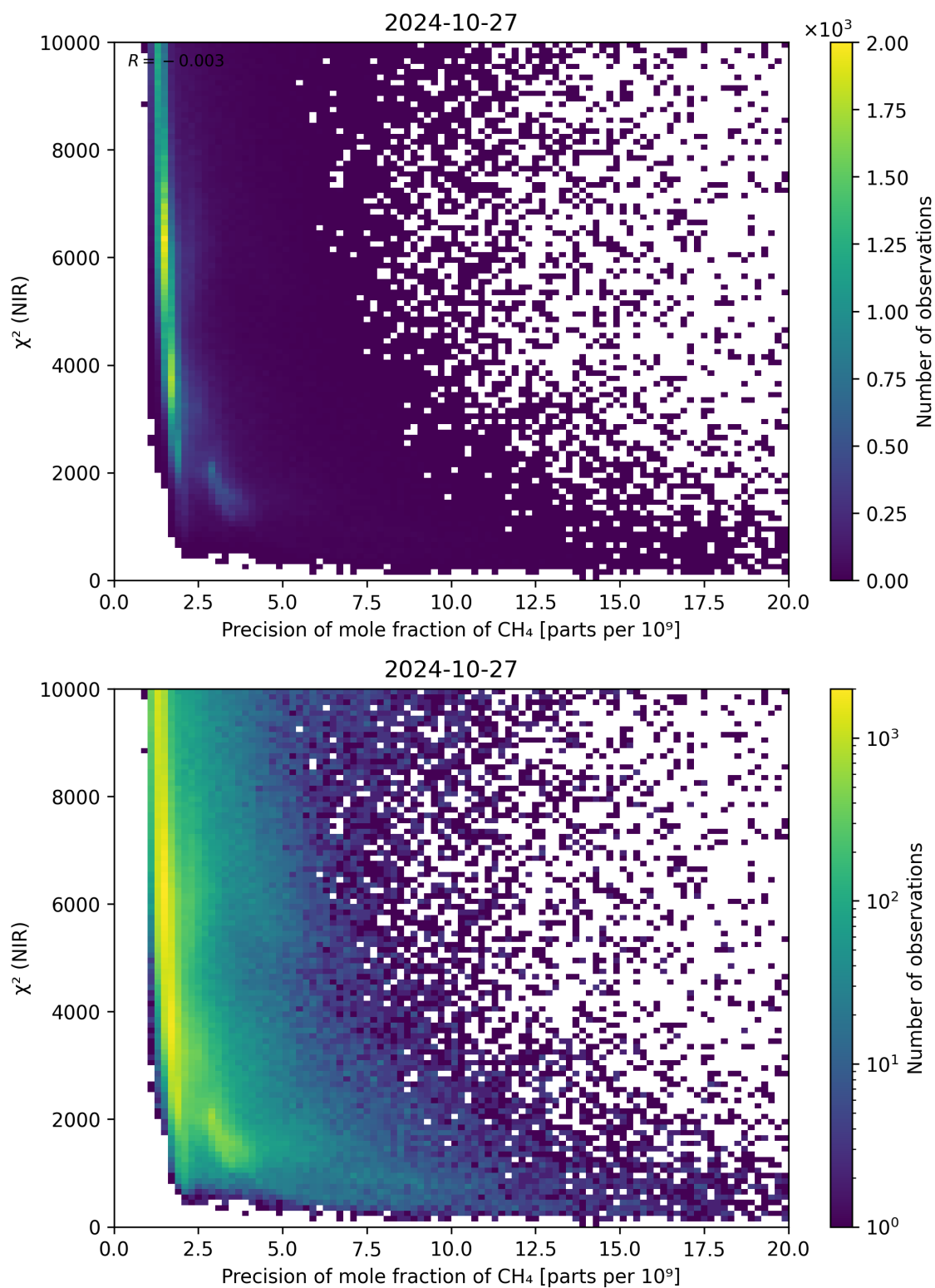
Figure 78: Scatter density plot of “Precision of mole fraction of \text{CH}_4 ” against “ \chi^2 (NIR)” for 2024-10-26 to 2024-10-28.
