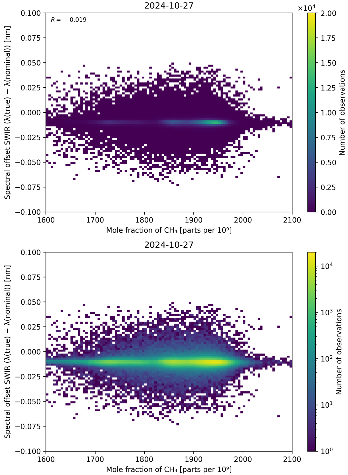
Figure 86: Scatter density plot of “Mole fraction of \text{CH}_4 ” against “Spectral offset SWIR ( \lambda_{\text{true}} - \lambda_{\text{nominal}} )” for 2024-10-26 to 2024-10-28.
