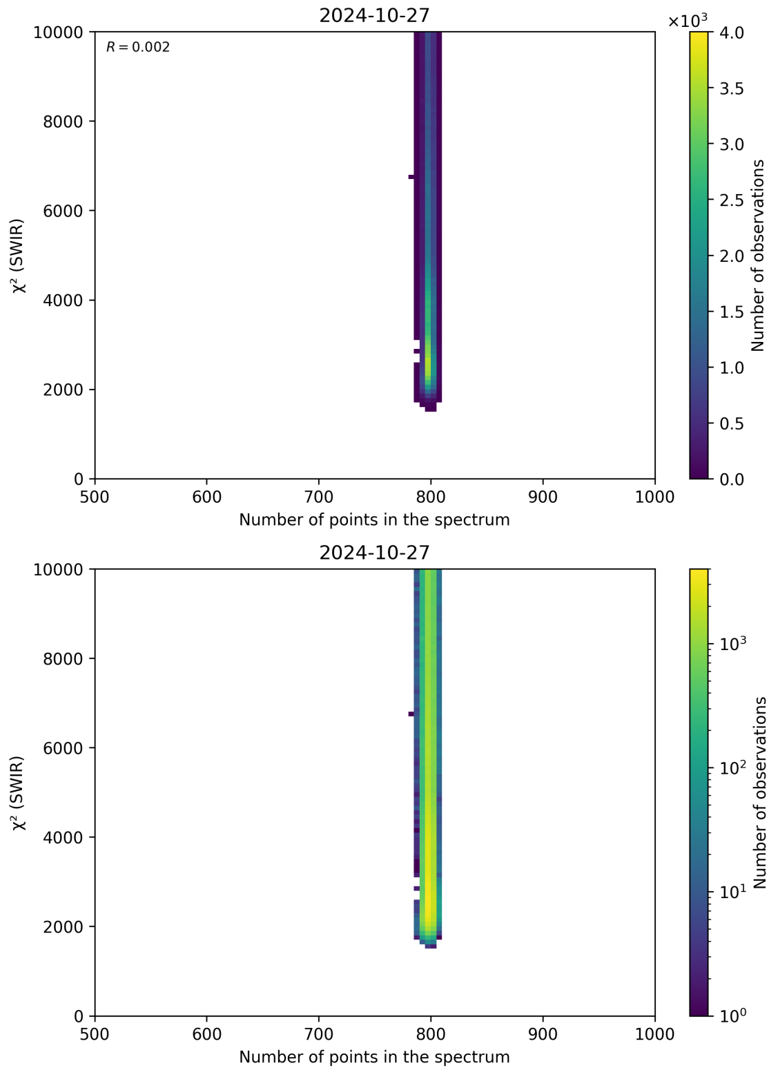
Figure 89: Scatter density plot of “Number of points in the spectrum” against “ \chi^2 (SWIR)” for 2024-10-26 to 2024-10-28.
