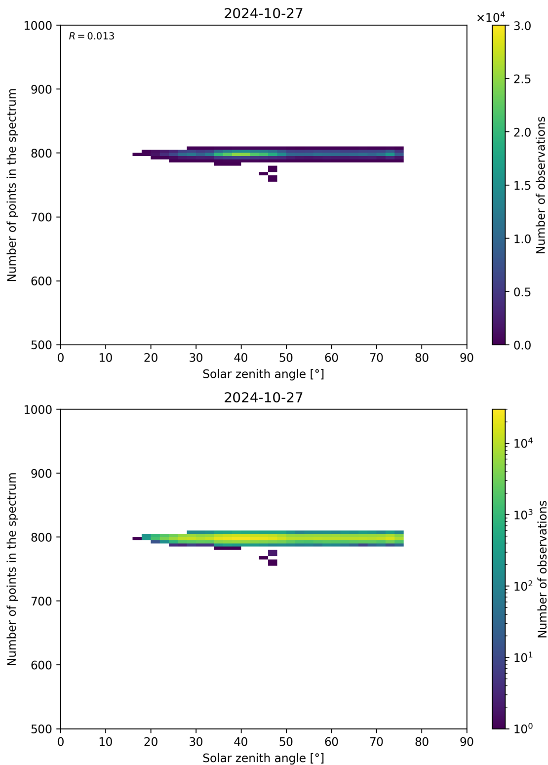
Figure 103: Scatter density plot of “Solar zenith angle” against “Number of points in the spectrum” for 2024-10-26 to 2024-10-28.
