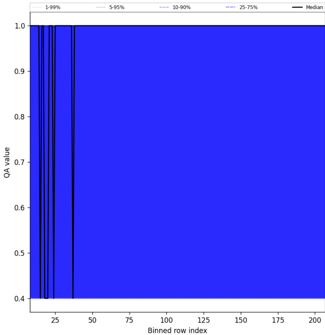
Figure 33: Along track statistics of “QA value” for 2024-10-26 to 2024-10-28
