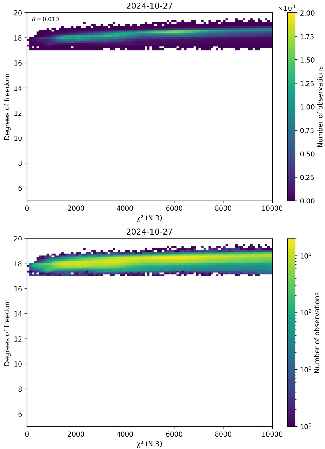
Figure 44: Scatter density plot of “ \chi^2 (NIR)” against “Degrees of freedom” for 2024-10-26 to 2024-10-28.
