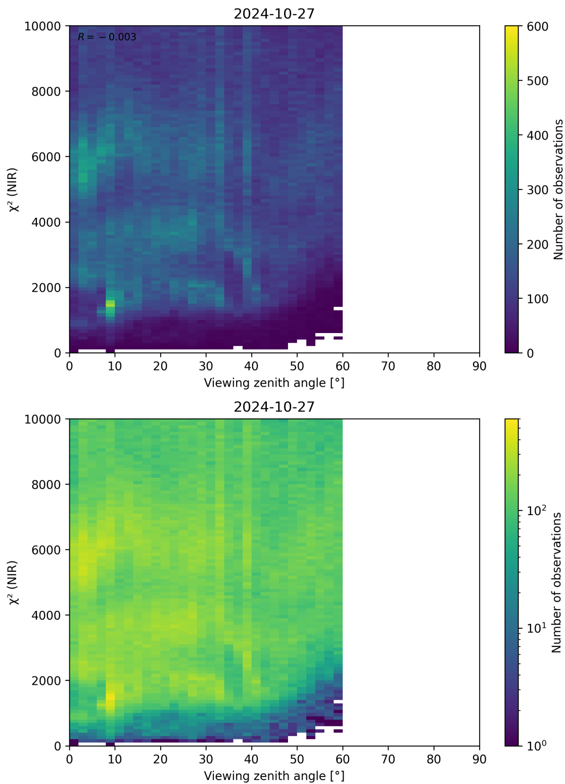
Figure 105: Scatter density plot of “Viewing zenith angle” against “ \chi^2 (NIR)” for 2024-10-26 to 2024-10-28.
