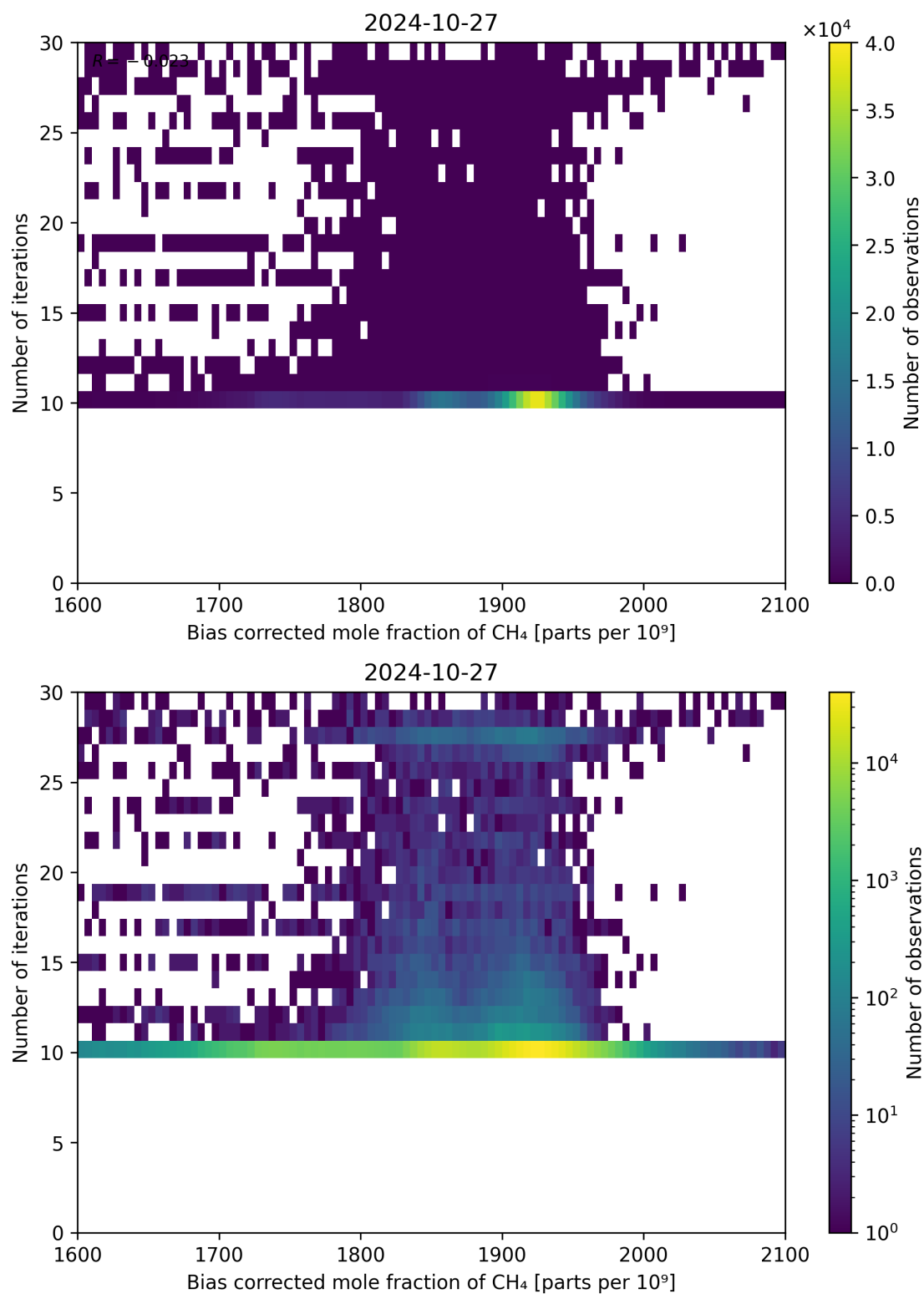
Figure 67: Scatter density plot of “Bias corrected mole fraction of \text{CH}_4 ” against “Number of iterations” for 2024-10-26 to 2024-10-28.
