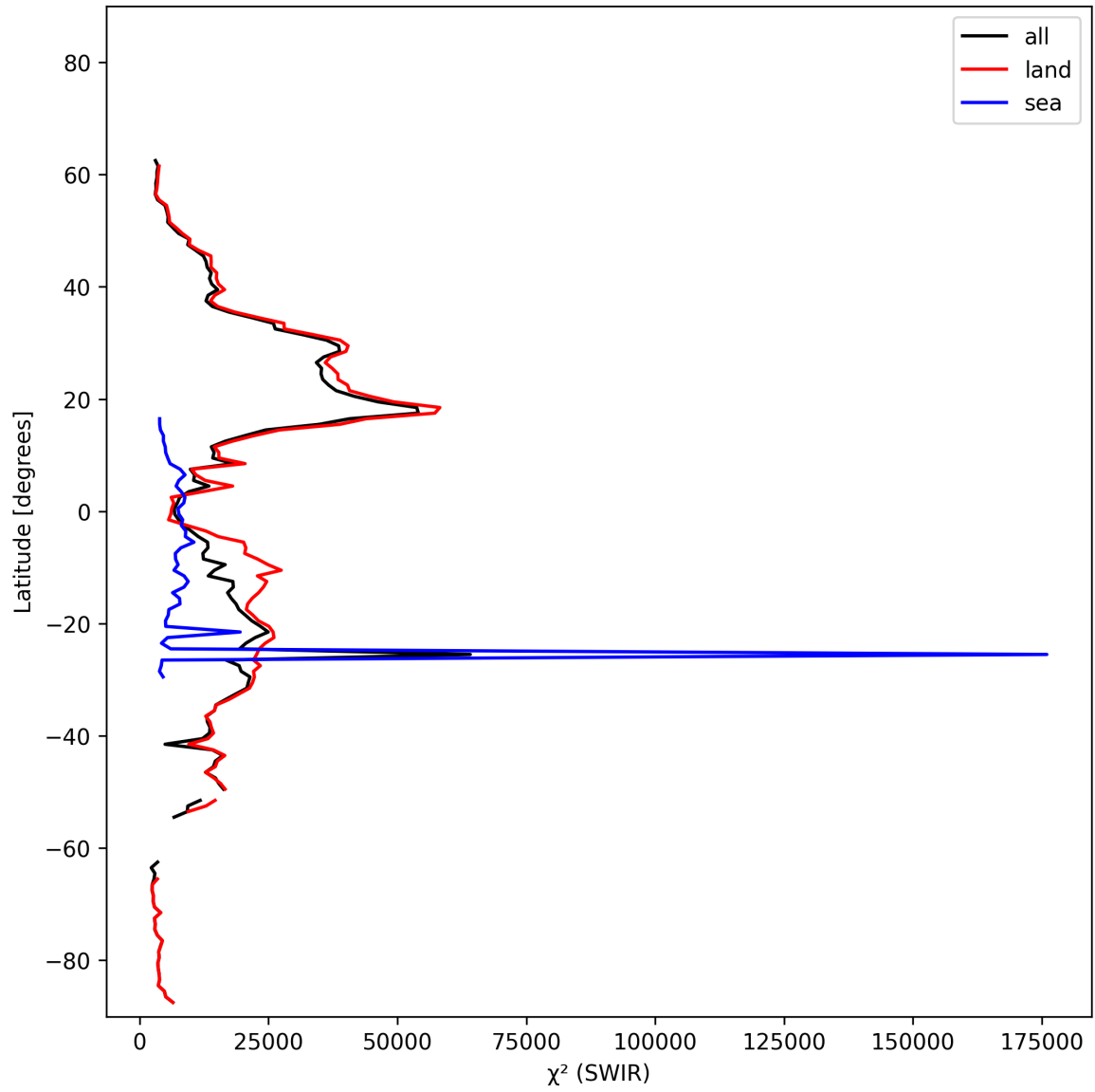
Figure 17: Zonal average of “ \chi^2 (SWIR)” for 2024-10-26 to 2024-10-28.
