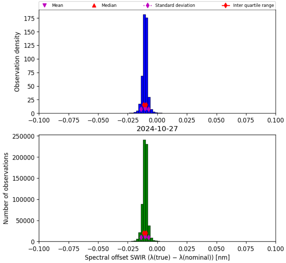
Figure 27: Histogram of “Spectral offset SWIR ( \lambda_{\text{true}} - \lambda_{\text{nominal}} )” for 2024-10-26 to 2024-10-28
