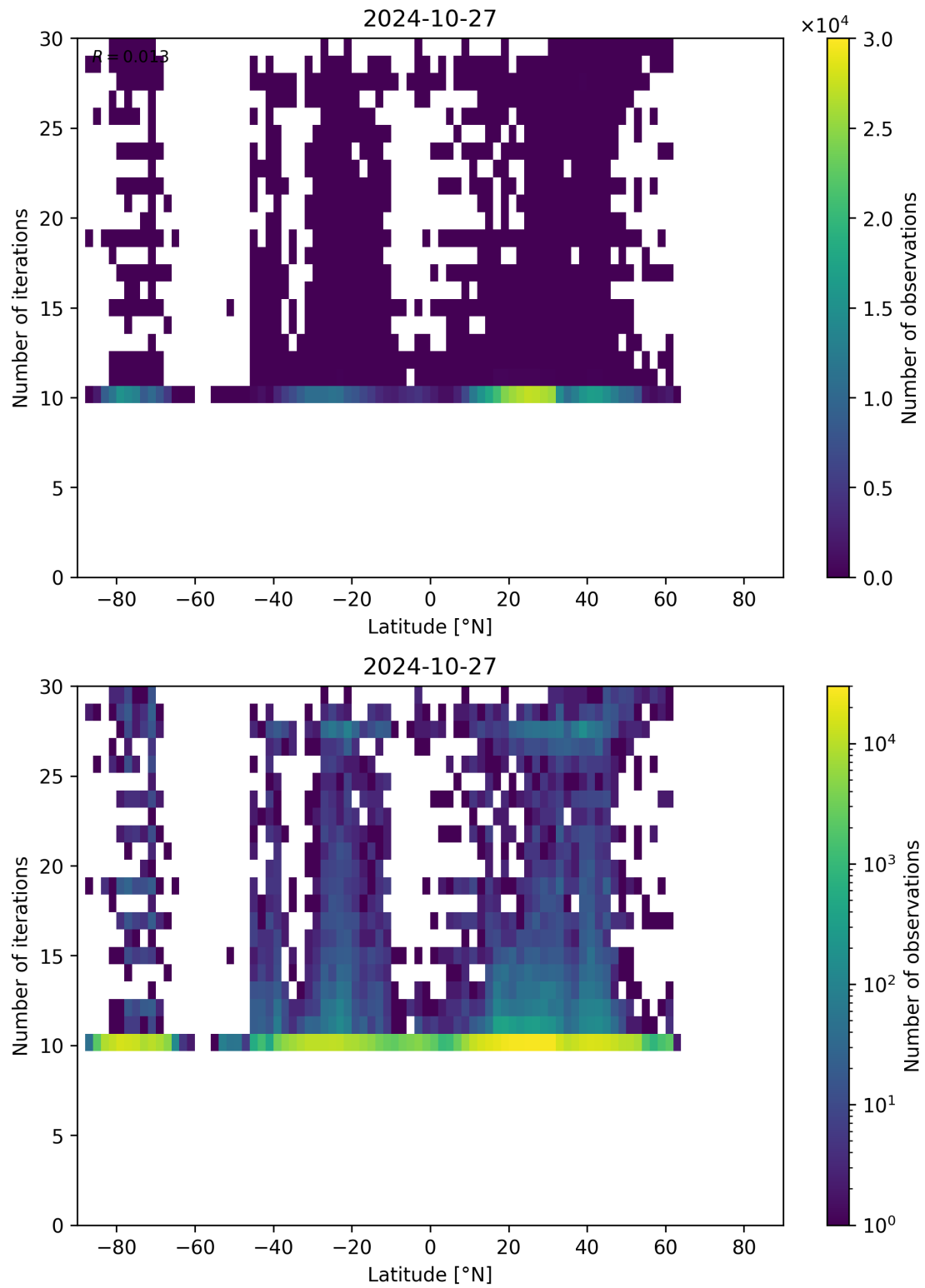
Figure 60: Scatter density plot of “Latitude” against “Number of iterations” for 2024-10-26 to 2024-10-28.
