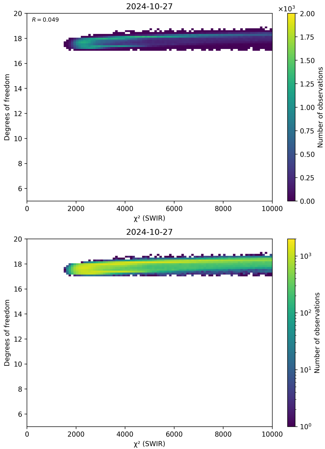
Figure 48: Scatter density plot of “ \chi^2 (SWIR)” against “Degrees of freedom” for 2024-10-26 to 2024-10-28.
