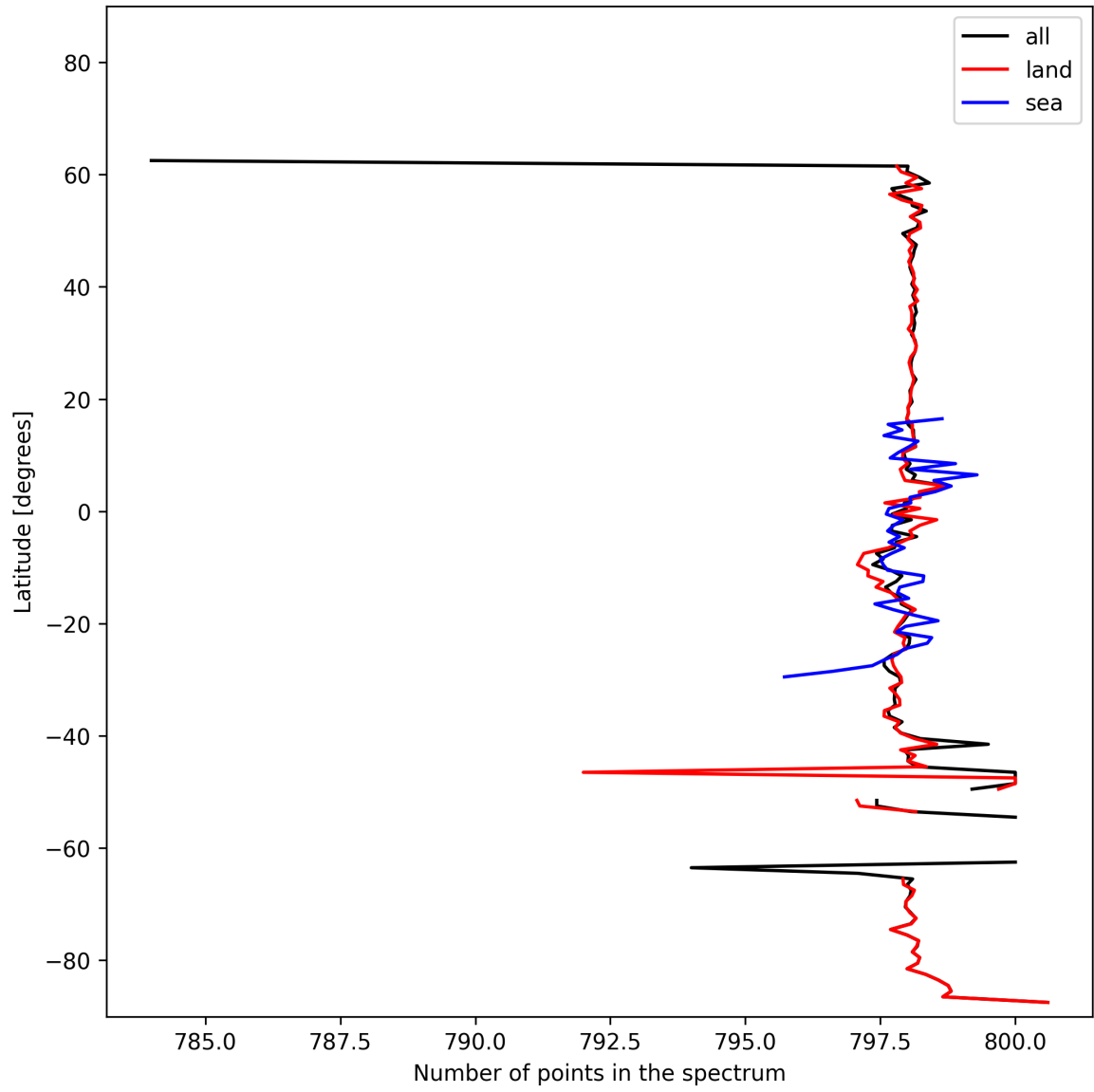
Figure 15: Zonal average of “Number of points in the spectrum” for 2024-10-26 to 2024-10-28.
