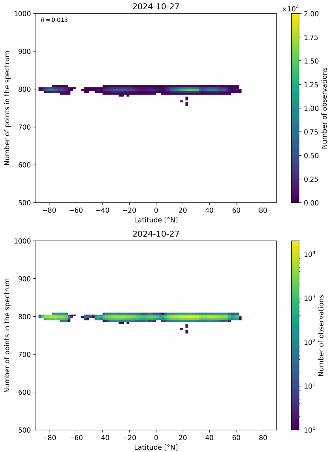
Figure 61: Scatter density plot of “Latitude” against “Number of points in the spectrum” for 2024-10-26 to 2024-10-28.
