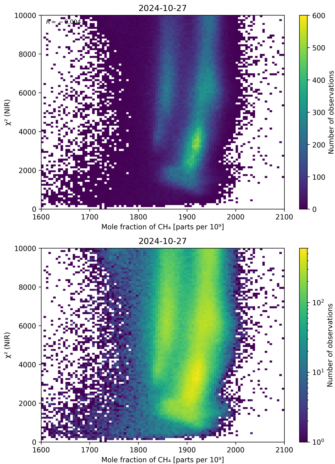
Figure 70: Scatter density plot of “Mole fraction of CH 4 ” against “ \chi^2 (NIR)” for 2024-10-26 to 2024-10-28.
