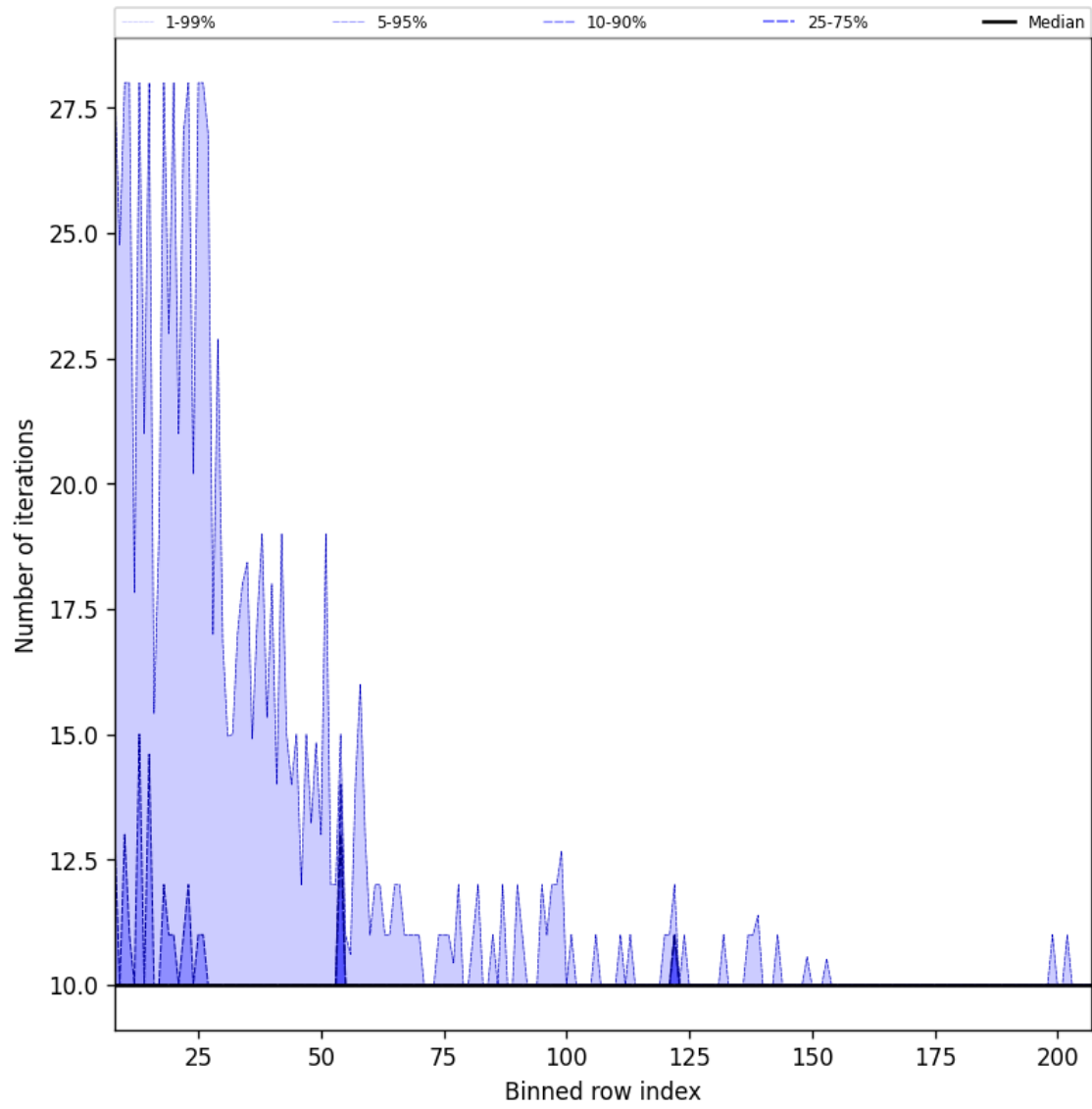
Figure 42: Along track statistics of “Number of iterations” for 2024-10-26 to 2024-10-28
