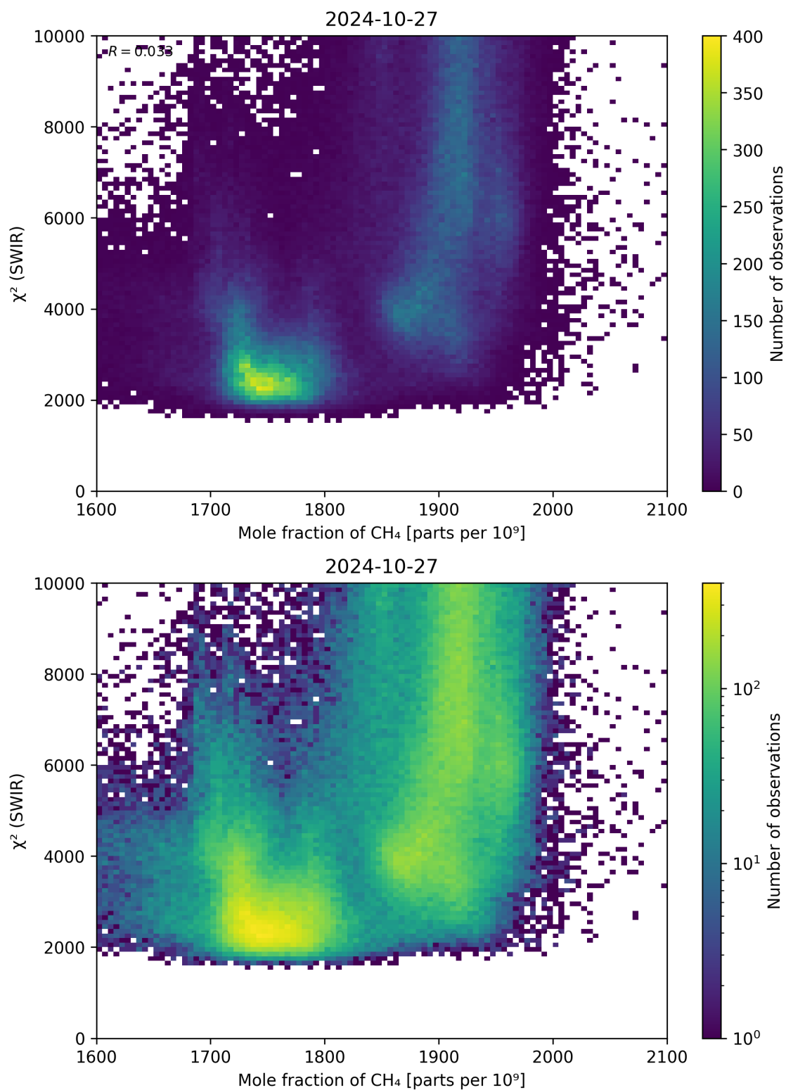
Figure 71: Scatter density plot of “Mole fraction of \text{CH}_4 ” against “ \chi^2 (SWIR)” for 2024-10-26 to 2024-10-28.
