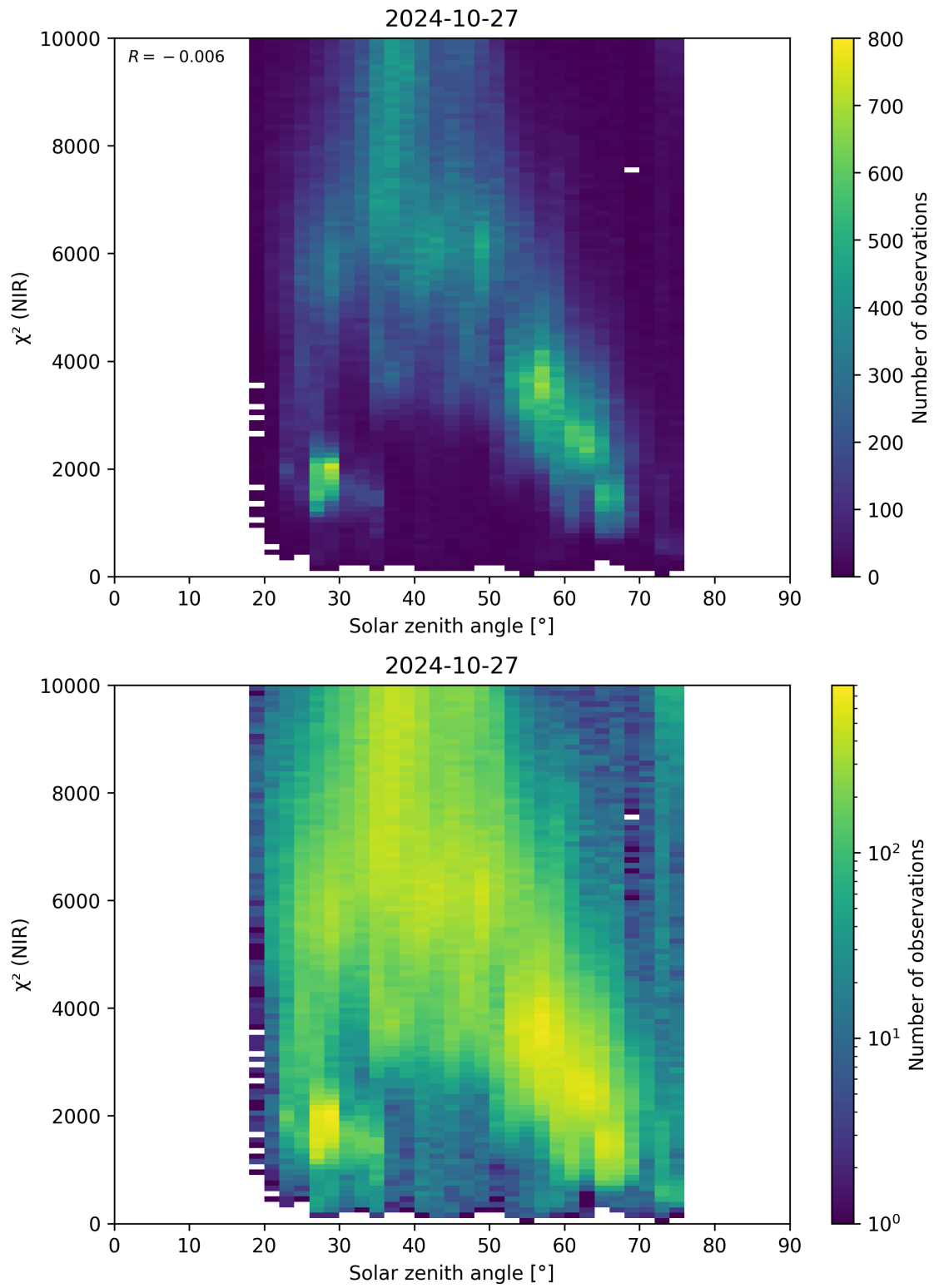
Figure 94: Scatter density plot of “Solar zenith angle” against “ \chi^2 (NIR)” for 2024-10-26 to 2024-10-28.
