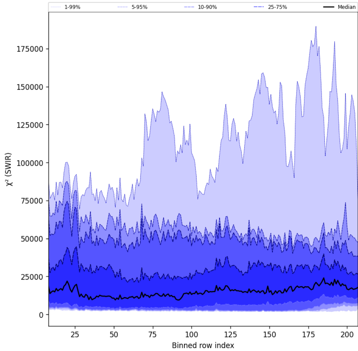
Figure 39: Along track statistics of “ \chi^2 (SWIR)” for 2024-10-26 to 2024-10-28
