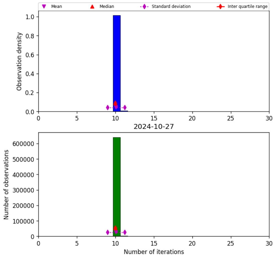
Figure 31: Histogram of “Number of iterations” for 2024-10-26 to 2024-10-28
