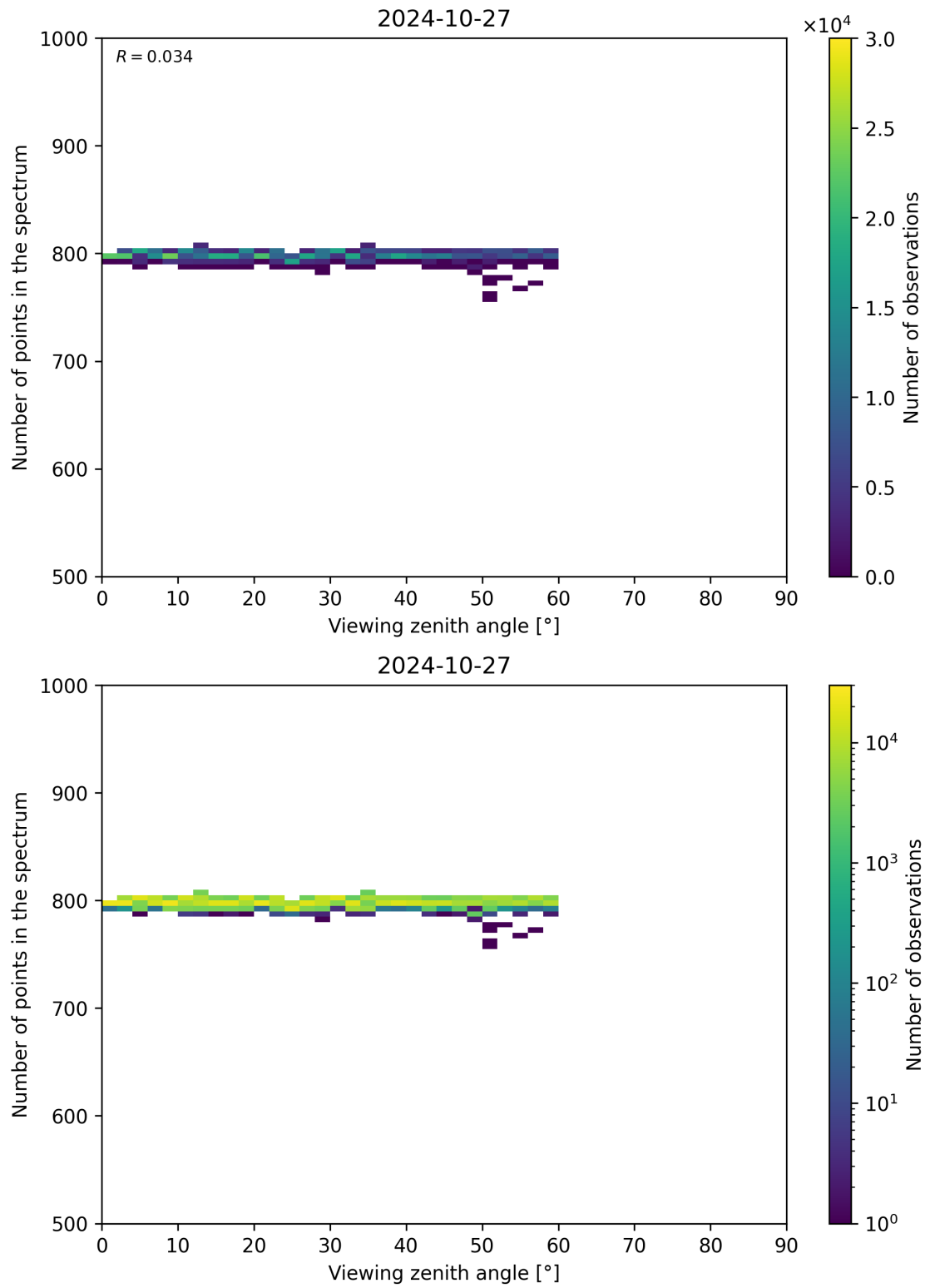
Figure 114: Scatter density plot of “Viewing zenith angle” against “Number of points in the spectrum” for 2024-10-26 to 2024-10-28.
