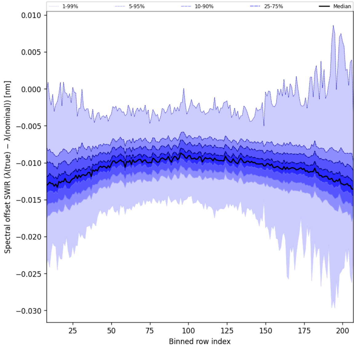
Figure 38: Along track statistics of “Spectral offset SWIR ( \lambda_{\text{true}} - \lambda_{\text{nominal}} )” for 2024-10-26 to 2024-10-28
