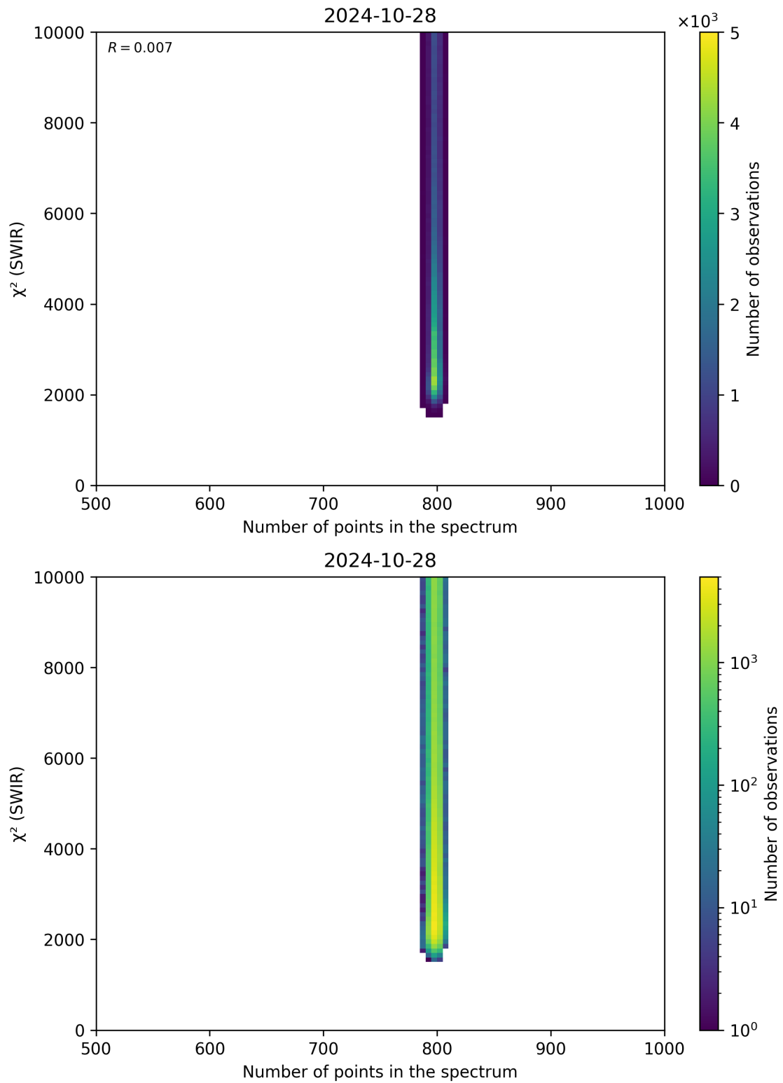
Figure 89: Scatter density plot of “Number of points in the spectrum” against “ \chi^2 (SWIR)” for 2024-10-27 to 2024-10-29.
