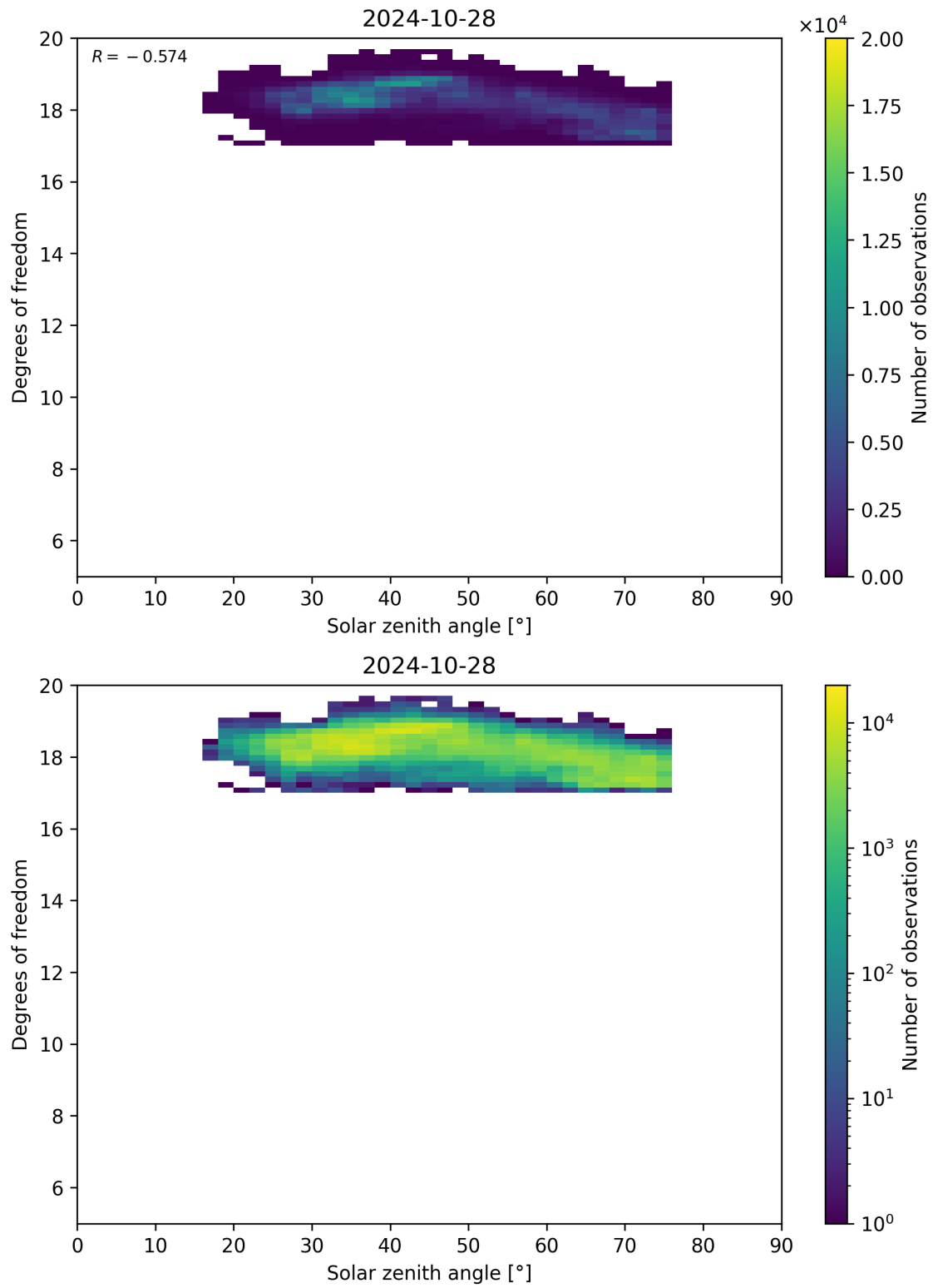
Figure 96: Scatter density plot of “Solar zenith angle” against “Degrees of freedom” for 2024-10-27 to 2024-10-29.
