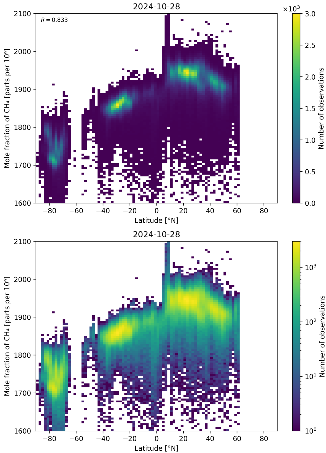
Figure 57: Scatter density plot of “Latitude” against “Mole fraction of CH 4 ” for 2024-10-27 to 2024-10-29.
