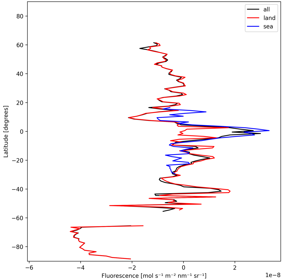
Figure 21: Zonal average of “Fluorescence” for 2024-10-27 to 2024-10-29.
