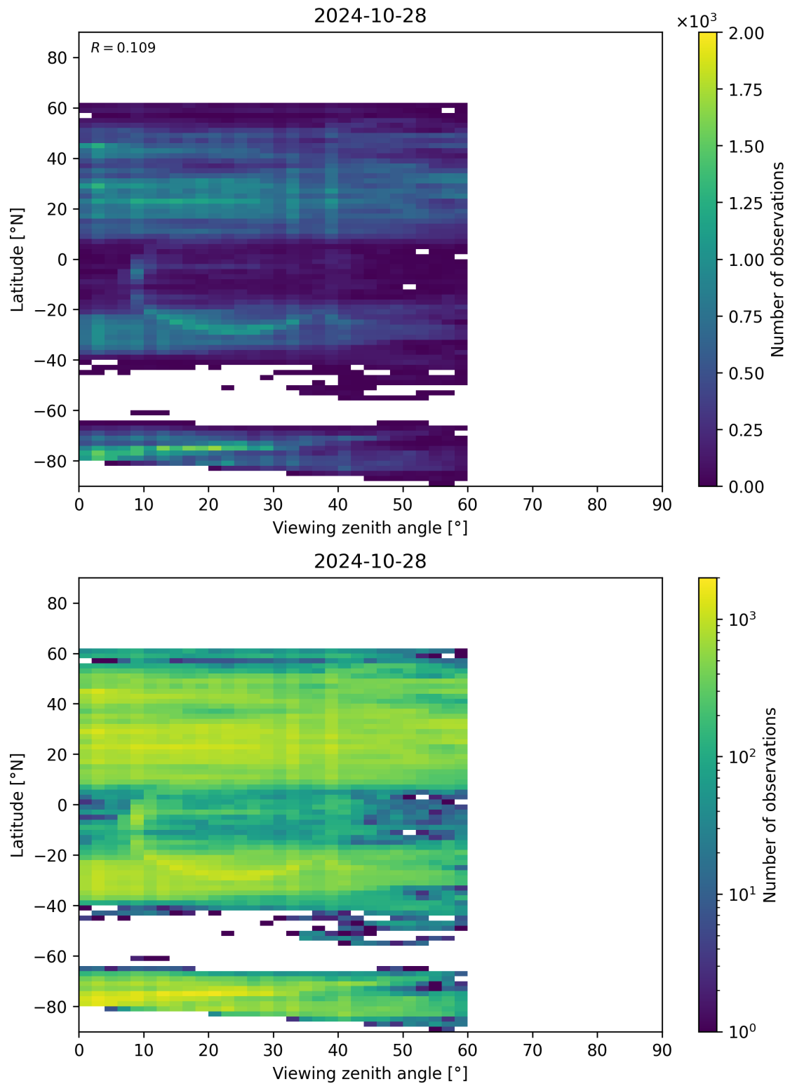
Figure 109: Scatter density plot of “Viewing zenith angle” against “Latitude” for 2024-10-27 to 2024-10-29.
