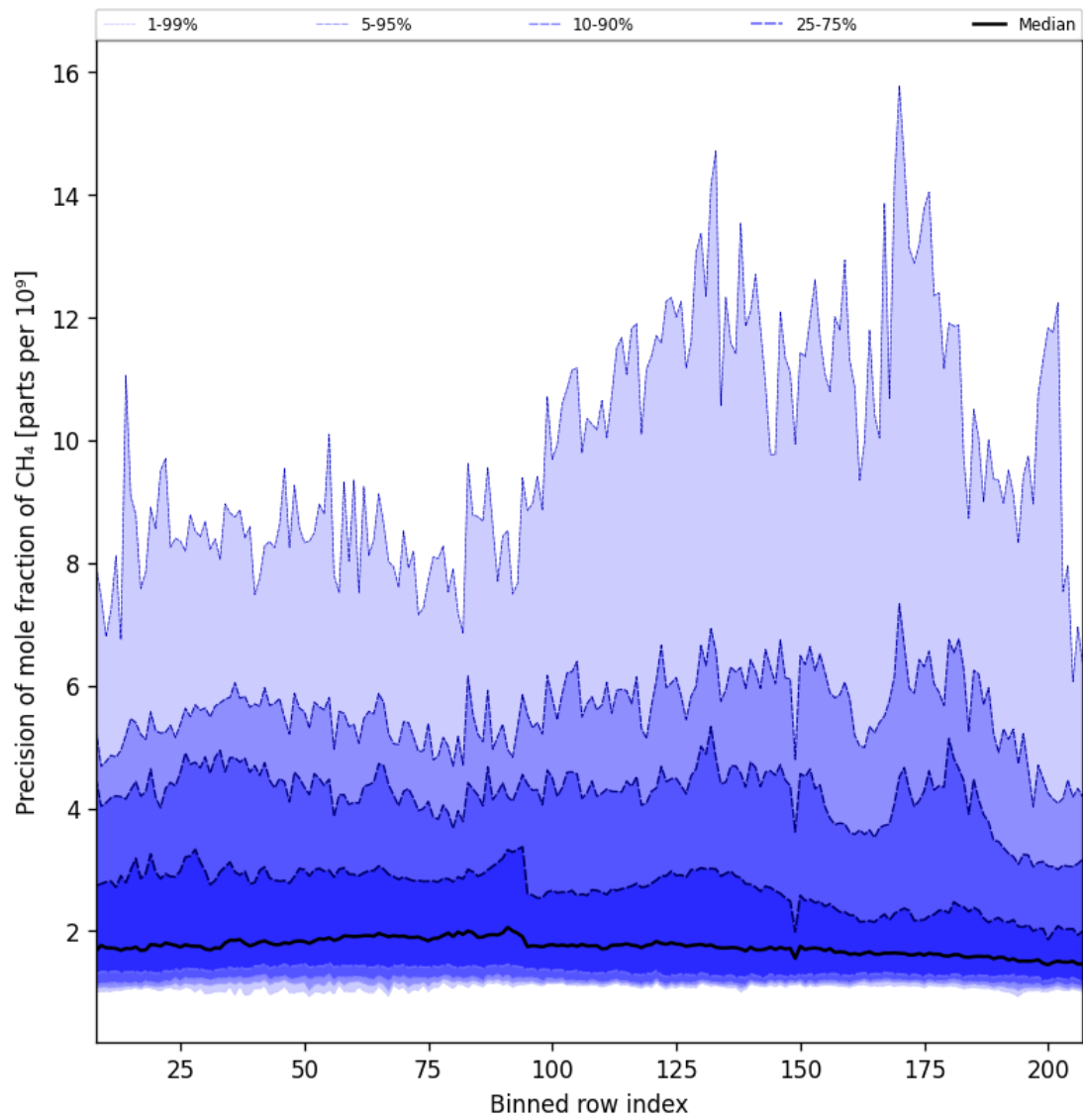
Figure 35: Along track statistics of “Precision of mole fraction of CH 4 ” for 2024-10-27 to 2024-10-29
