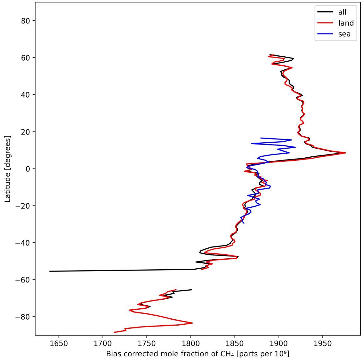
Figure 14: Zonal average of “Bias corrected mole fraction of CH 4 ” for 2024-10-27 to 2024-10-29.
