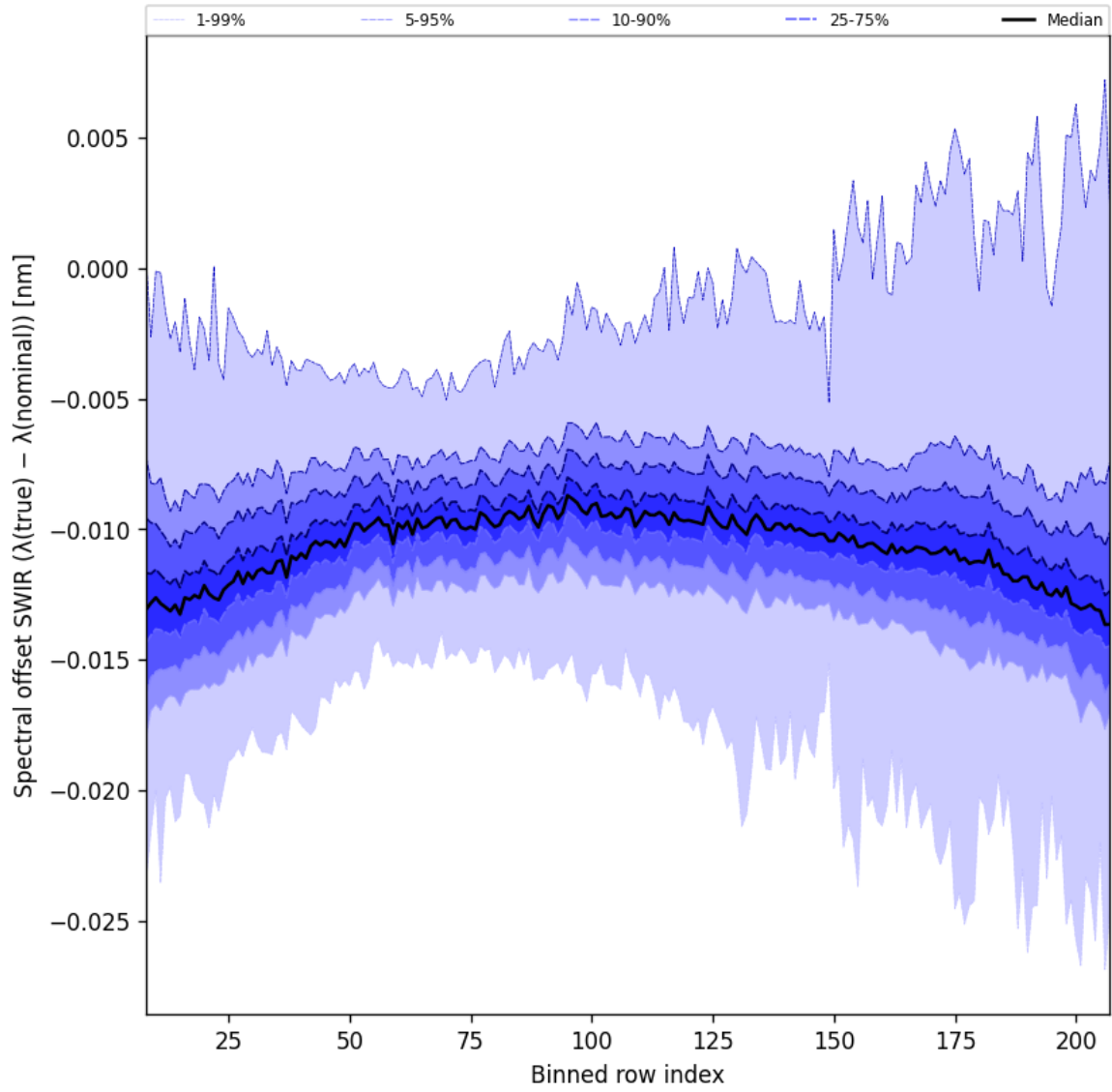
Figure 38: Along track statistics of “Spectral offset SWIR ( \lambda_{\text{true}} - \lambda_{\text{nominal}} )” for 2024-10-27 to 2024-10-29
