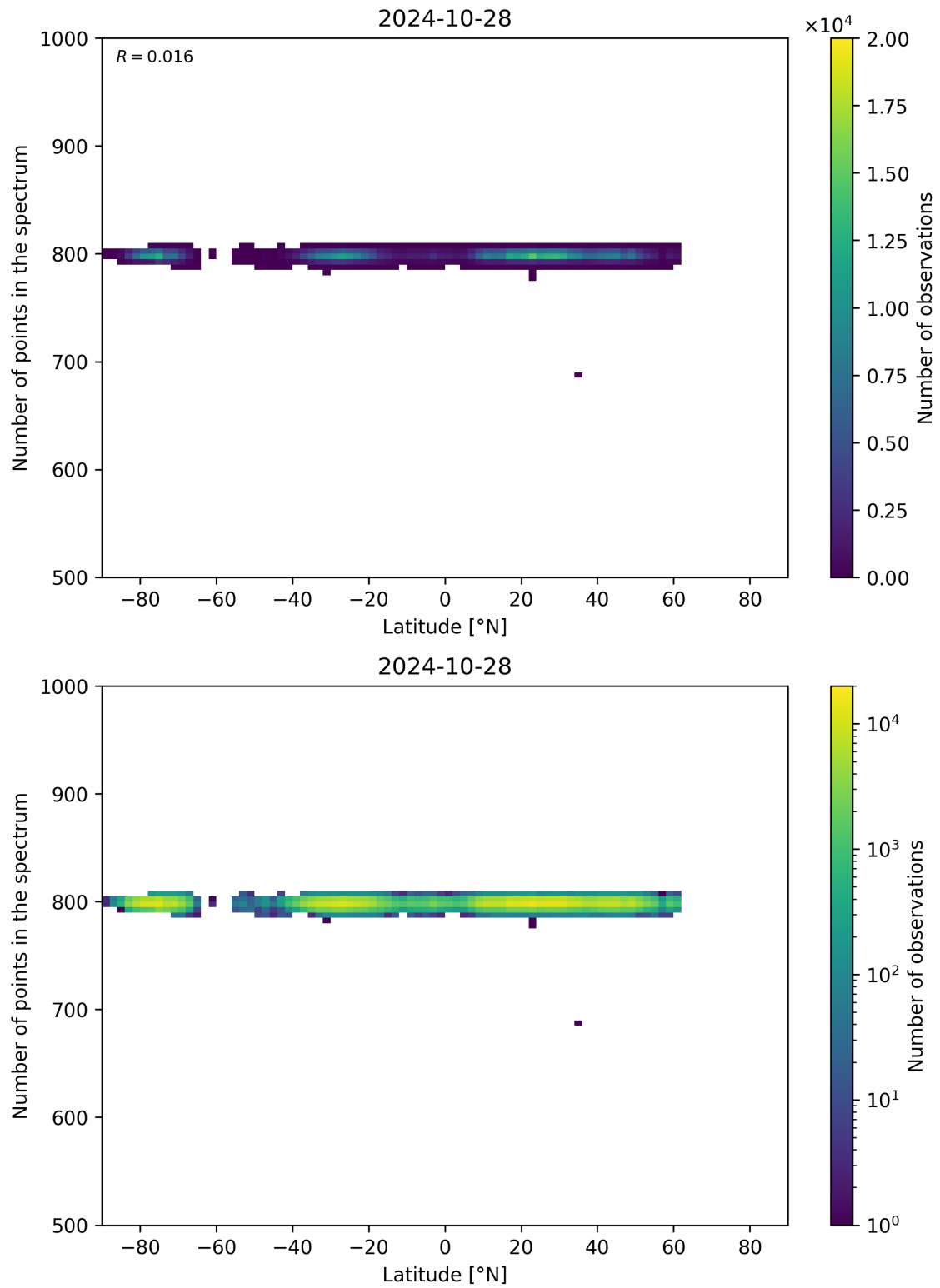
Figure 61: Scatter density plot of “Latitude” against “Number of points in the spectrum” for 2024-10-27 to 2024-10-29.
