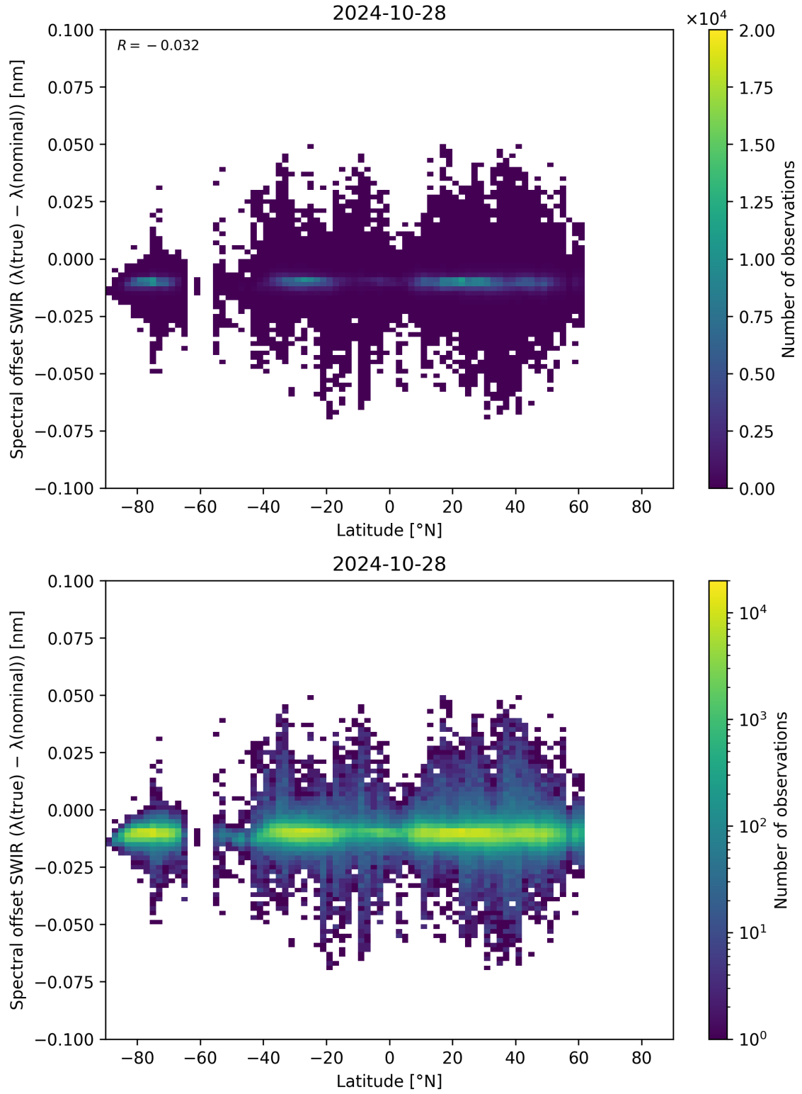
Figure 62: Scatter density plot of “Latitude” against “Spectral offset SWIR ( \lambda_{\text{true}} - \lambda_{\text{nominal}} )” for 2024-10-27 to 2024-10-29.
