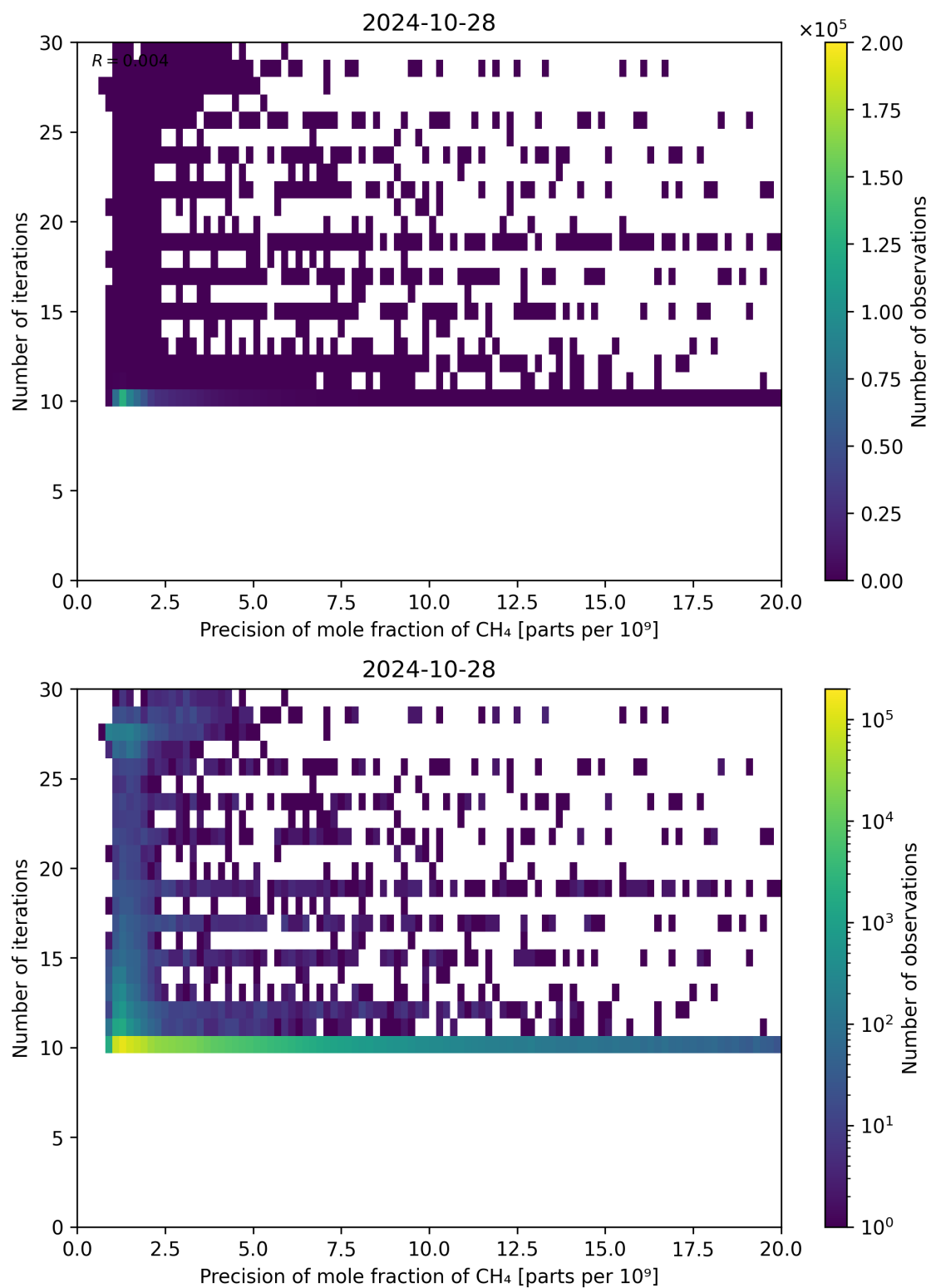
Figure 83: Scatter density plot of “Precision of mole fraction of \text{CH}_4 ” against “Number of iterations” for 2024-10-27 to 2024-10-29.
