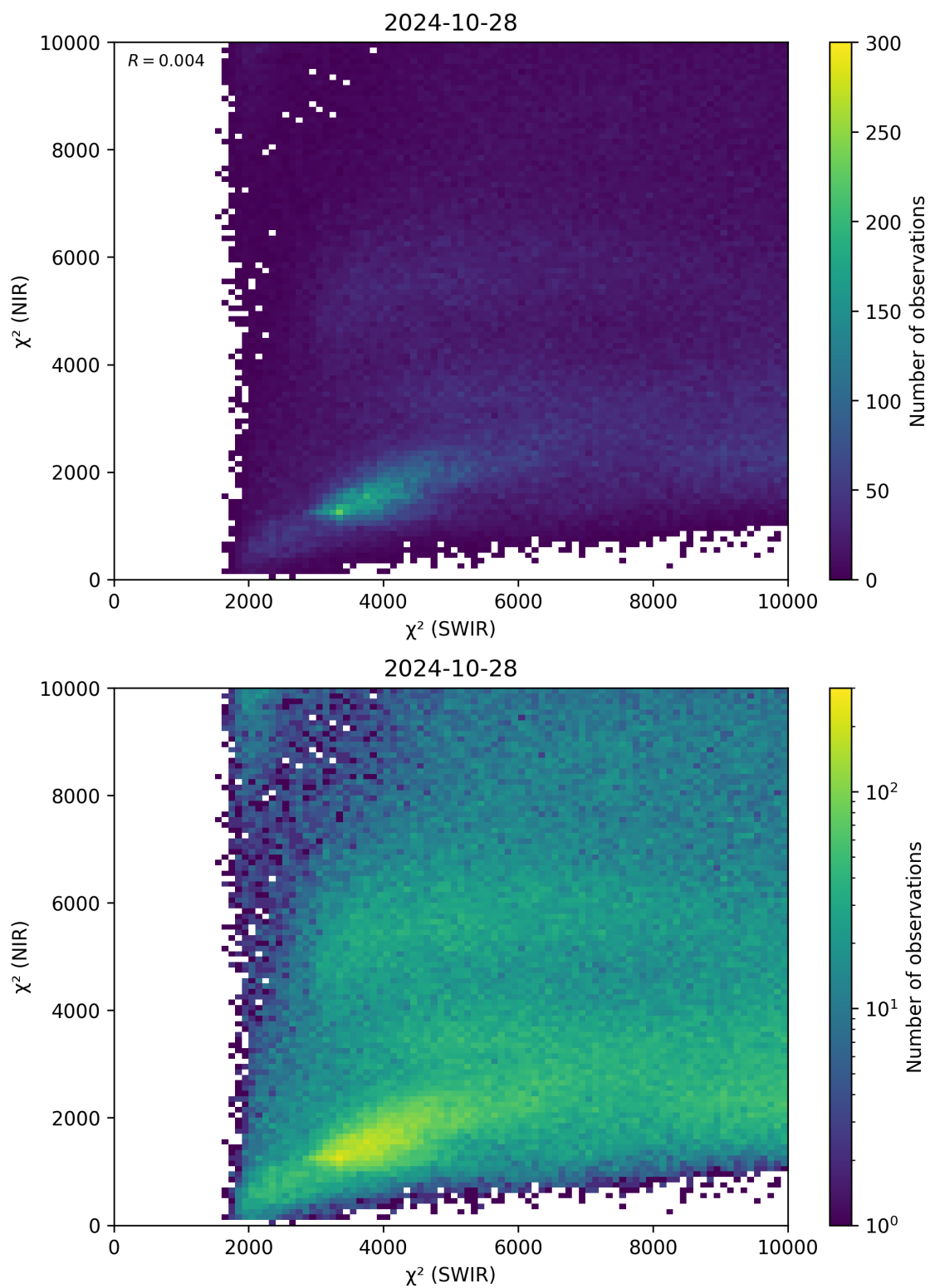
Figure 47: Scatter density plot of “ \chi^2 (SWIR)” against “ \chi^2 (NIR)” for 2024-10-27 to 2024-10-29.
