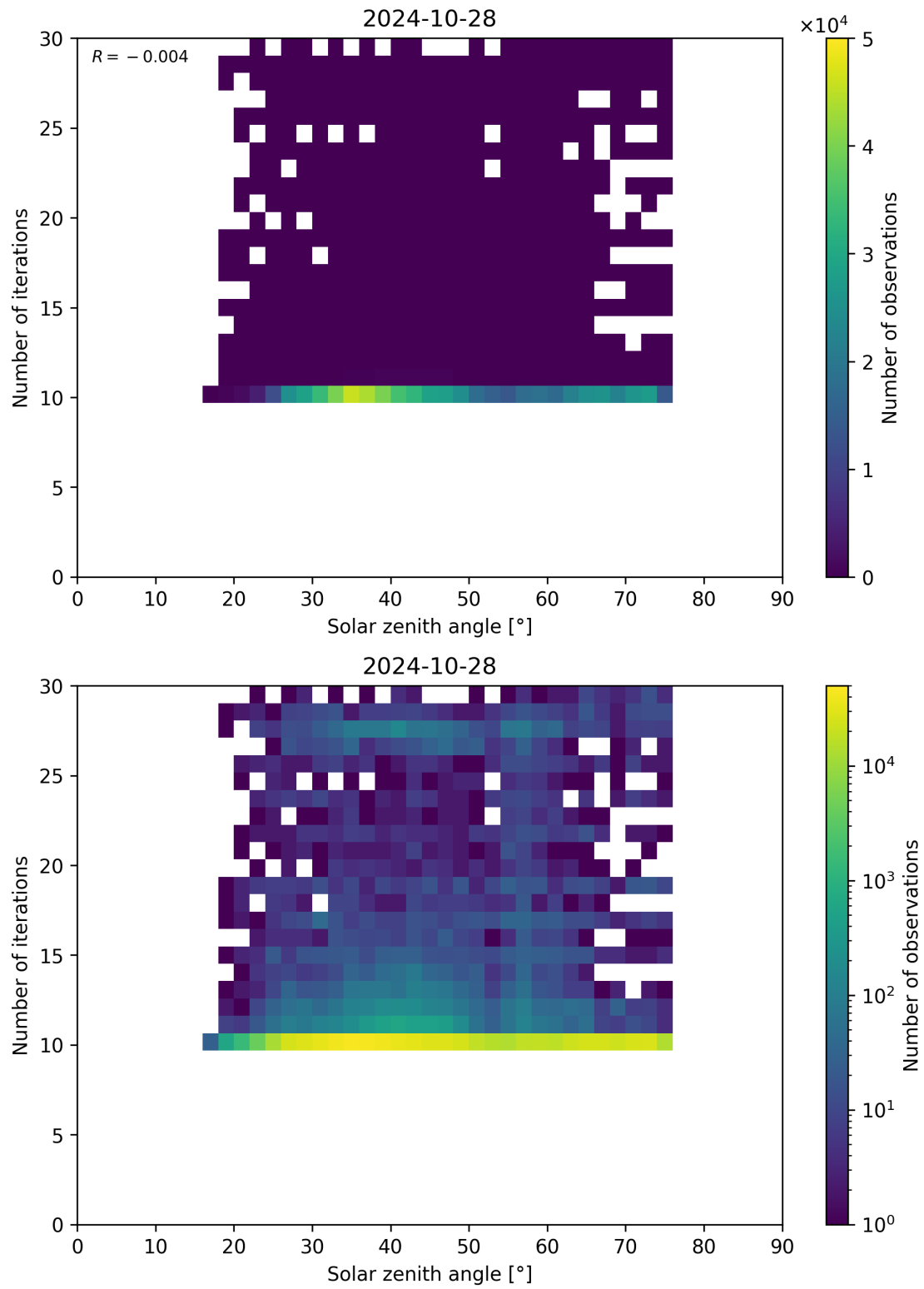
Figure 102: Scatter density plot of “Solar zenith angle” against “Number of iterations” for 2024-10-27 to 2024-10-29.
