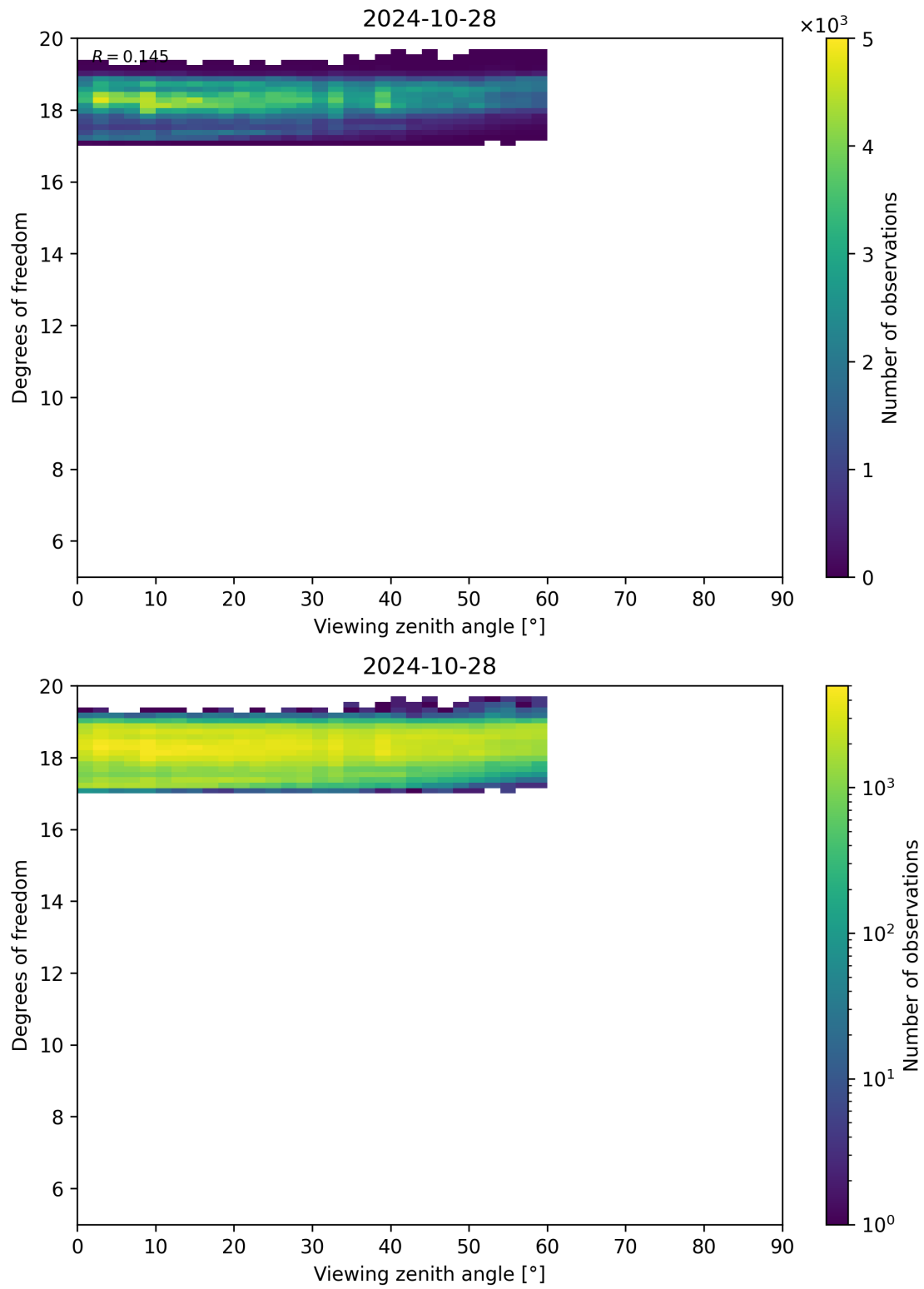
Figure 107: Scatter density plot of “Viewing zenith angle” against “Degrees of freedom” for 2024-10-27 to 2024-10-29.
