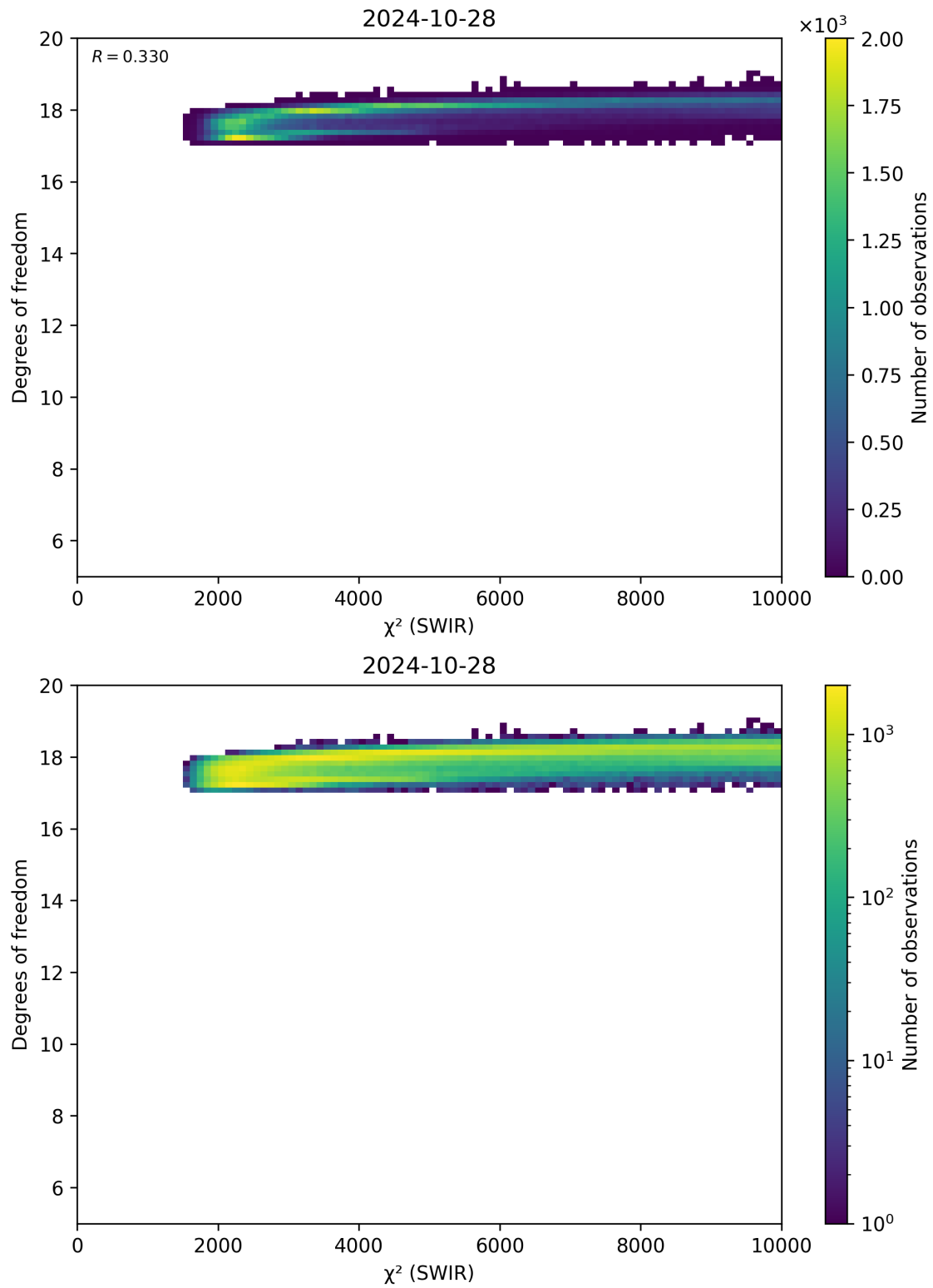
Figure 48: Scatter density plot of “ \chi^2 (SWIR)” against “Degrees of freedom” for 2024-10-27 to 2024-10-29.
