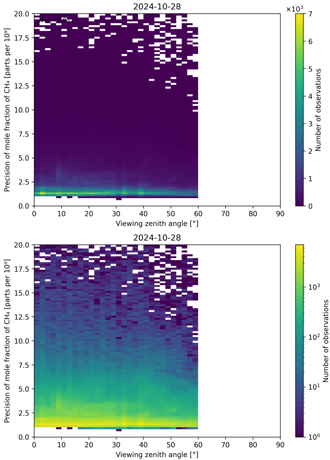
Figure 112: Scatter density plot of “Viewing zenith angle” against “Precision of mole fraction of CH 4 ” for 2024-10-27 to 2024-10-29.
