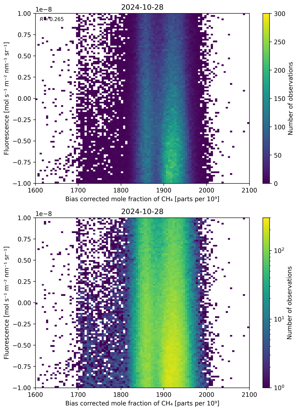
Figure 66: Scatter density plot of “Bias corrected mole fraction of \text{CH}_4 ” against “Fluorescence” for 2024-10-27 to 2024-10-29.
