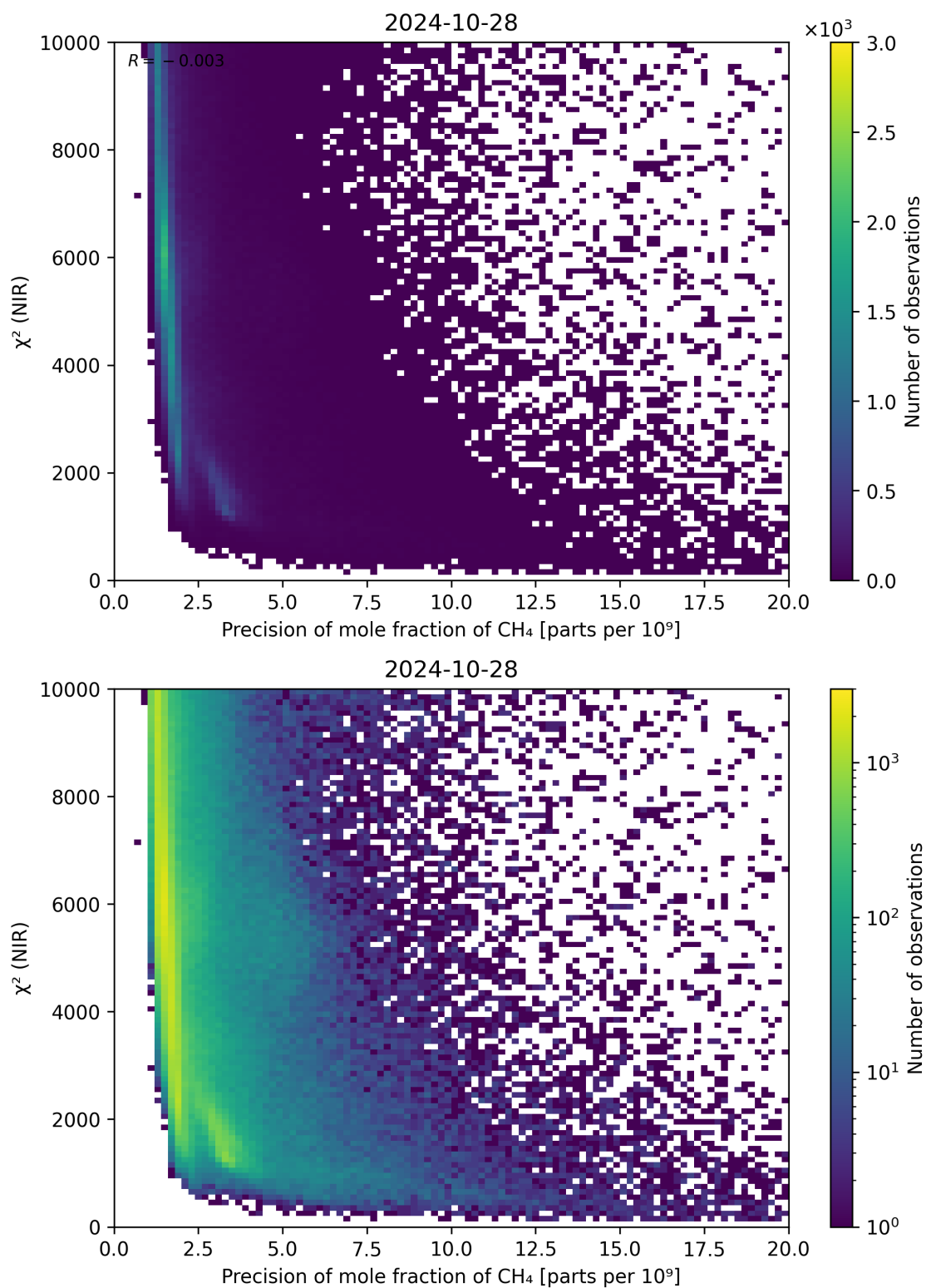
Figure 78: Scatter density plot of “Precision of mole fraction of CH 4 ” against “ \chi^2 (NIR)” for 2024-10-27 to 2024-10-29.
