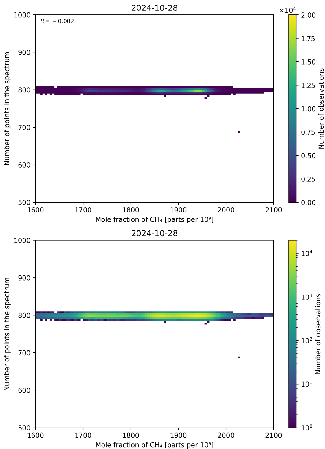
Figure 77: Scatter density plot of “Mole fraction of CH 4 ” against “Number of points in the spectrum” for 2024-10-27 to 2024-10-29.
