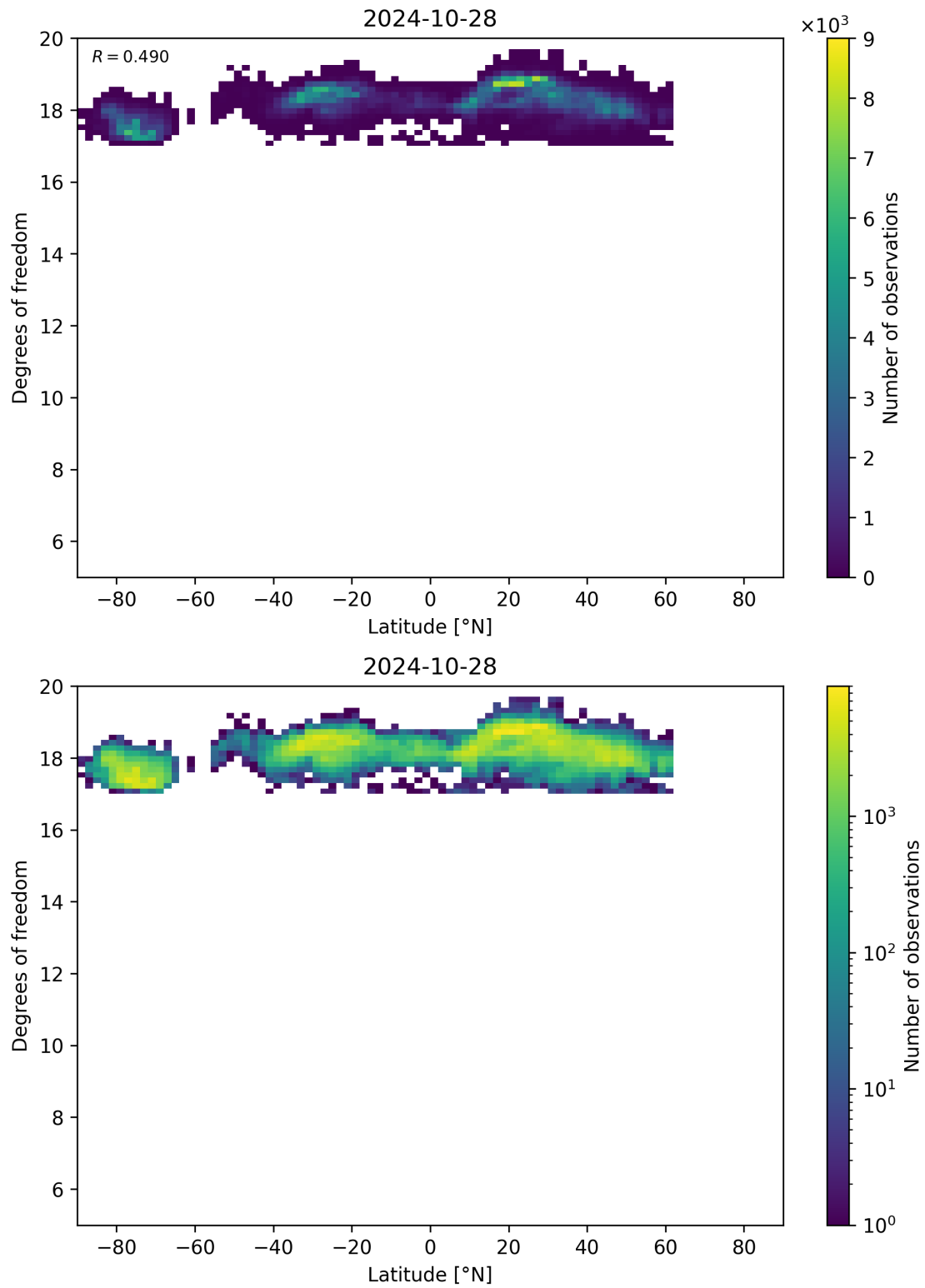
Figure 55: Scatter density plot of “Latitude” against “Degrees of freedom” for 2024-10-27 to 2024-10-29.
