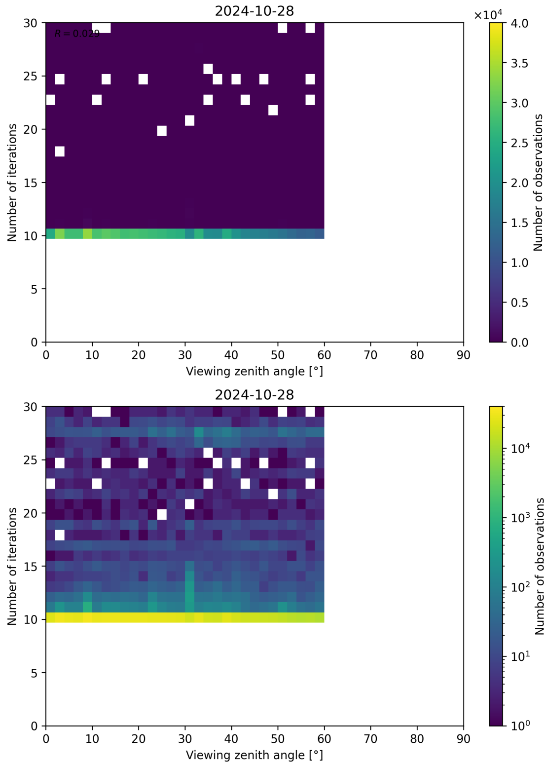
Figure 113: Scatter density plot of “Viewing zenith angle” against “Number of iterations” for 2024-10-27 to 2024-10-29.
