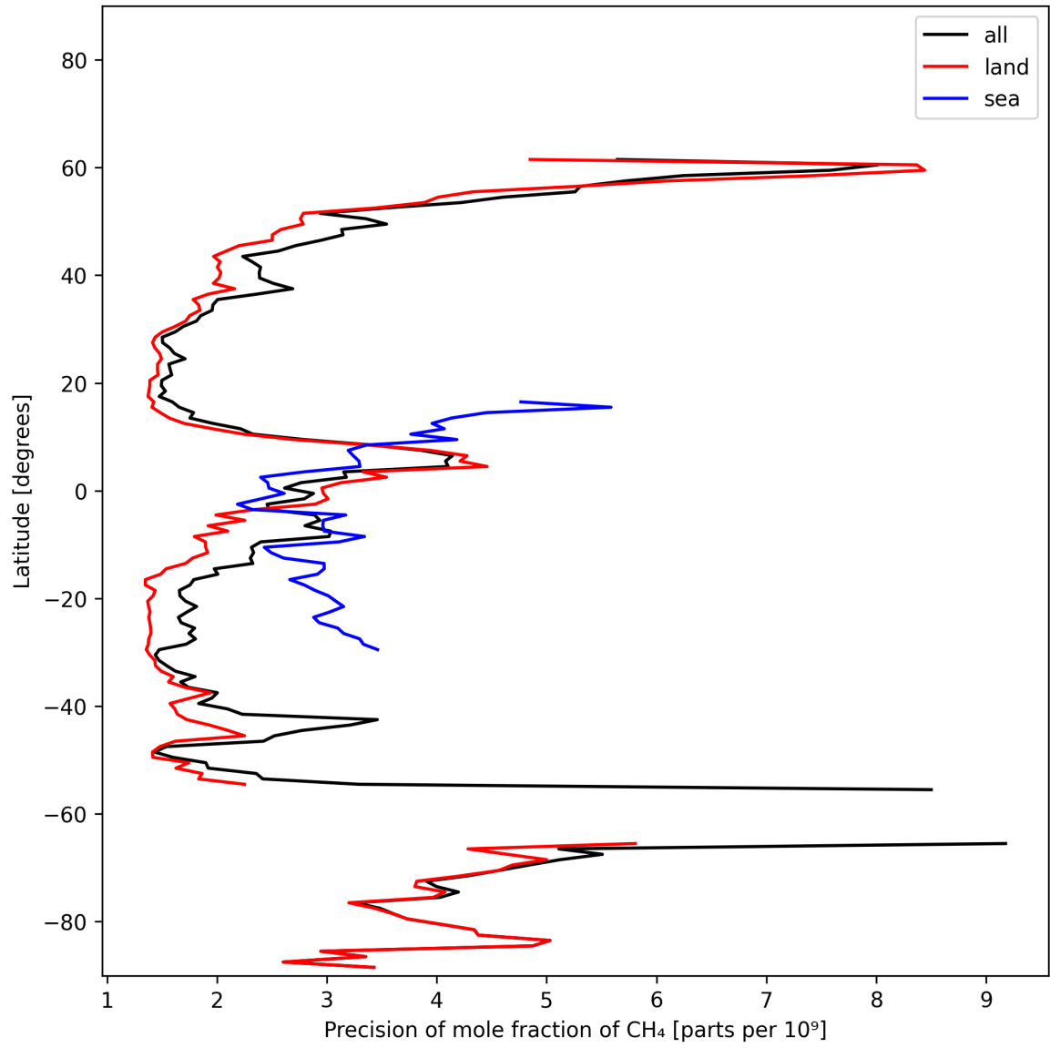
Figure 13: Zonal average of “Precision of mole fraction of CH 4 ” for 2024-10-27 to 2024-10-29.
