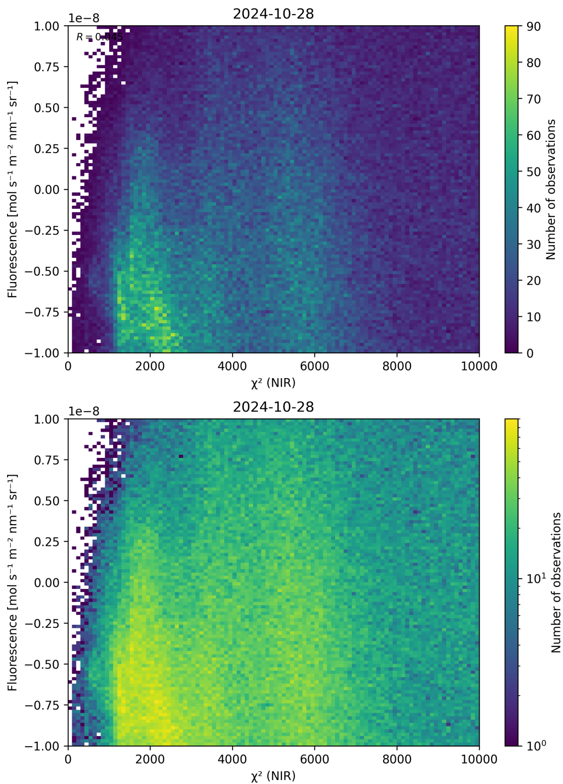
Figure 45: Scatter density plot of “ \chi^2 (NIR)” against “Fluorescence” for 2024-10-27 to 2024-10-29.
