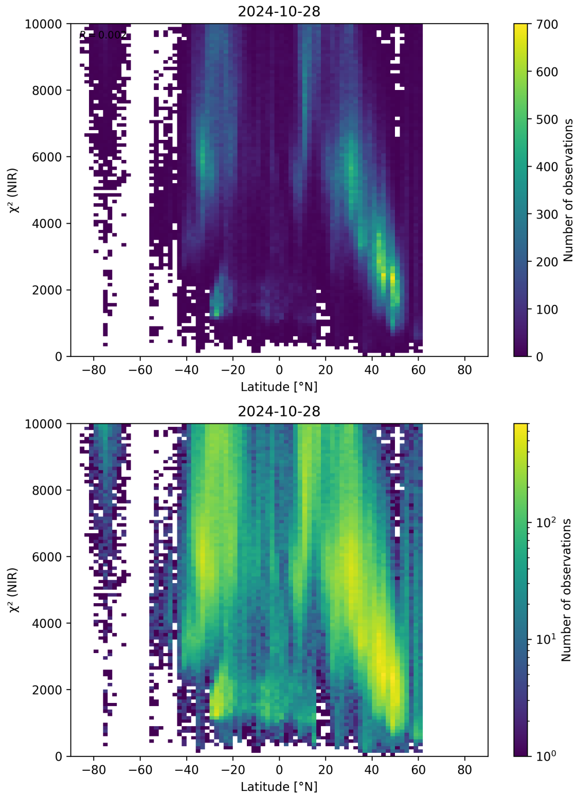
Figure 53: Scatter density plot of “Latitude” against “ \chi^2 (NIR)” for 2024-10-27 to 2024-10-29.
