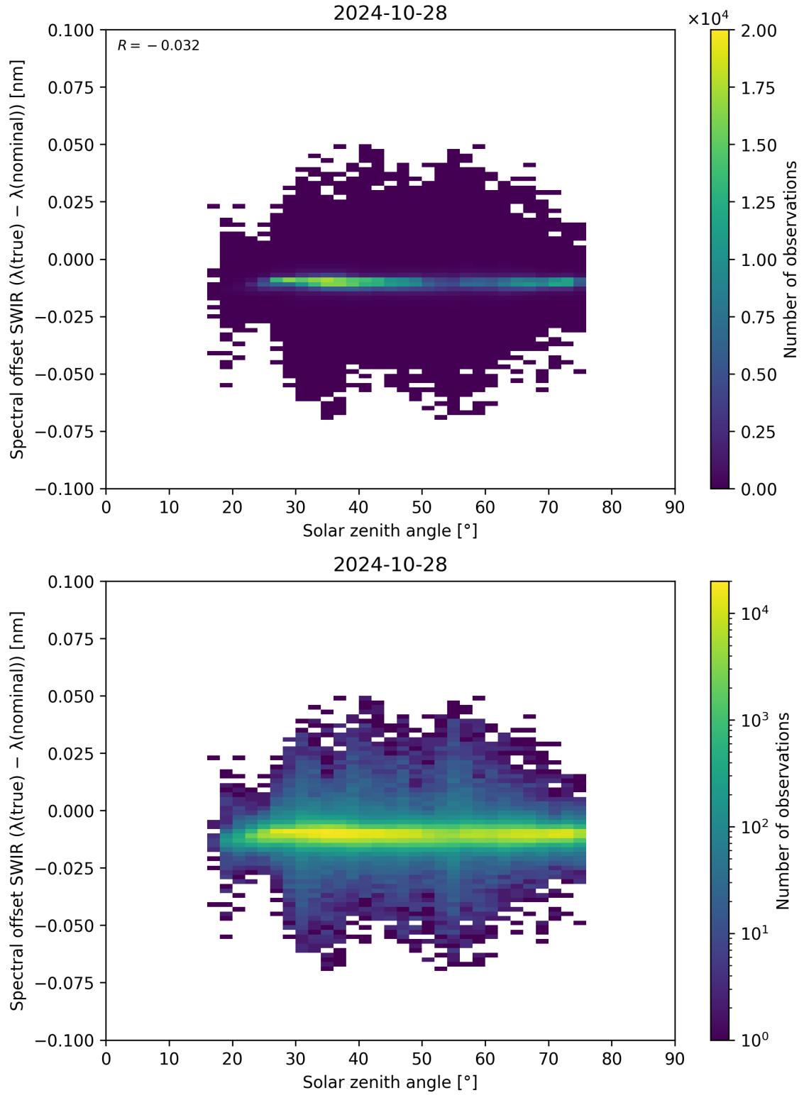
Figure 104: Scatter density plot of “Solar zenith angle” against “Spectral offset SWIR ( \lambda_{\text{true}} - \lambda_{\text{nominal}} )” for 2024-10-27 to 2024-10-29.
