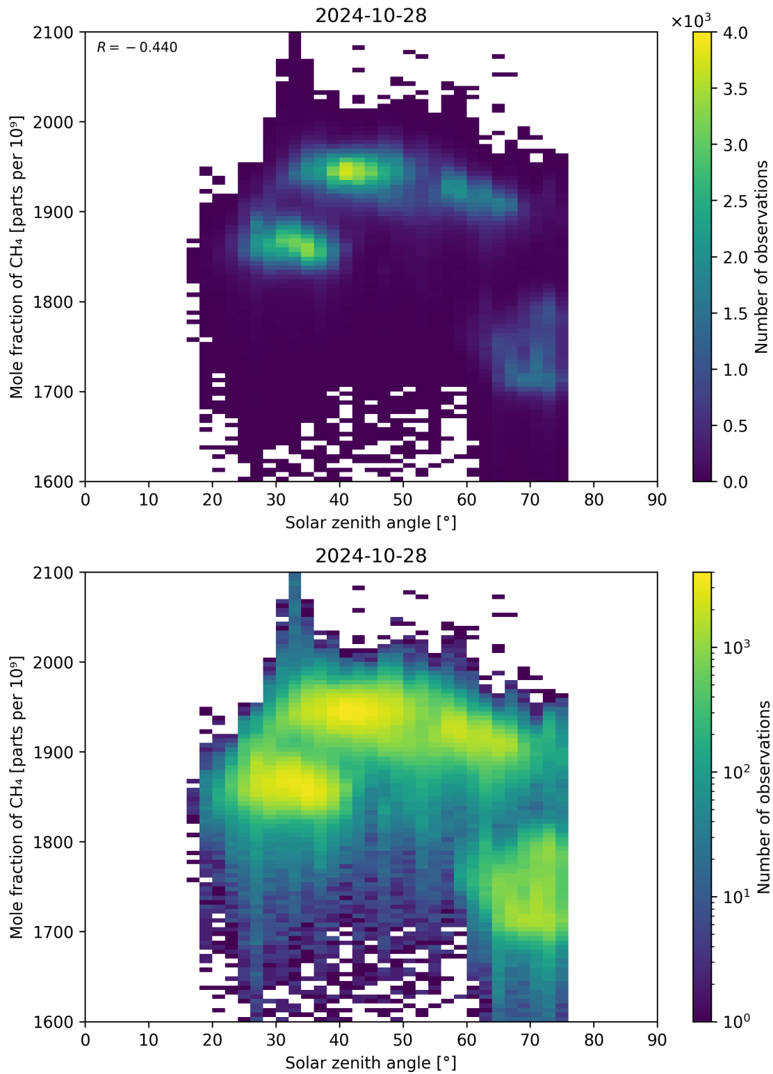
Figure 99: Scatter density plot of “Solar zenith angle” against “Mole fraction of CH 4 ” for 2024-10-27 to 2024-10-29.
