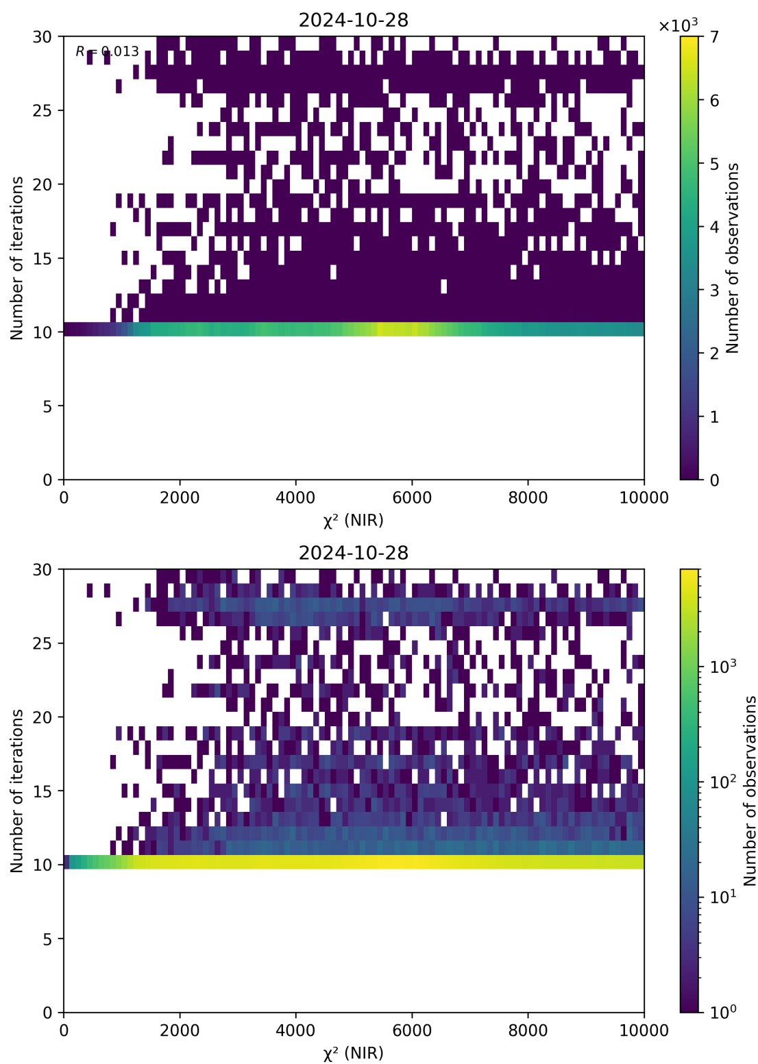
Figure 46: Scatter density plot of “ \chi^2 (NIR)” against “Number of iterations” for 2024-10-27 to 2024-10-29.
