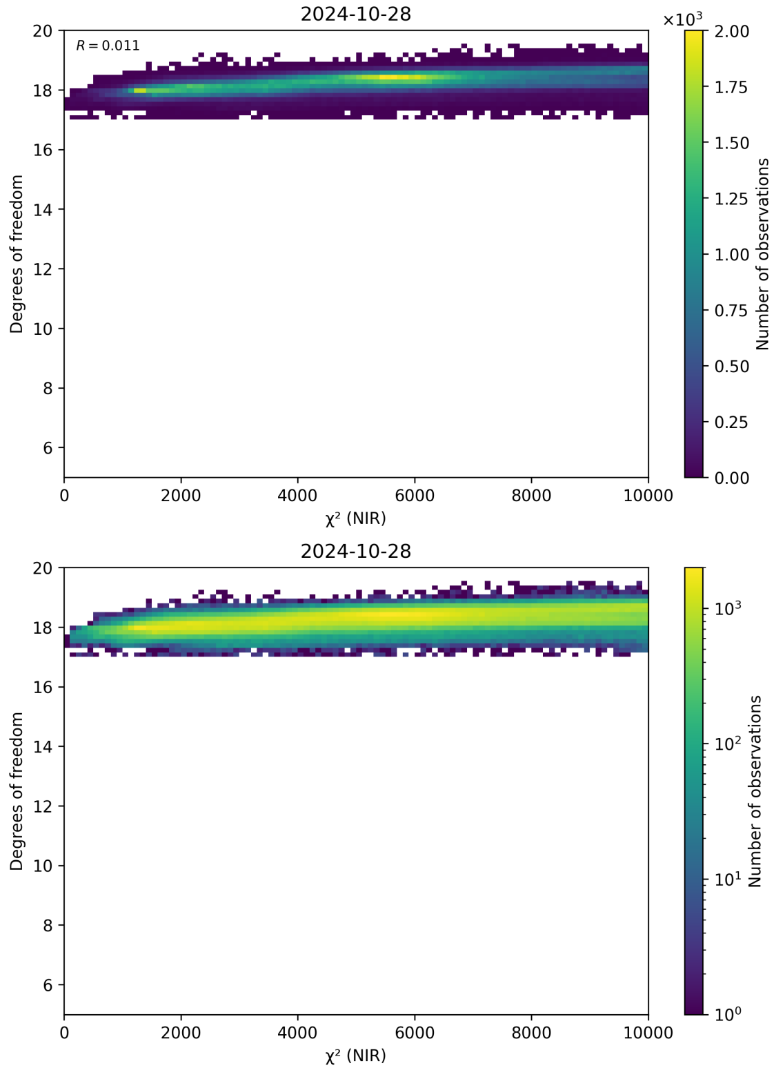
Figure 44: Scatter density plot of “ \chi^2 (NIR)” against “Degrees of freedom” for 2024-10-27 to 2024-10-29.
