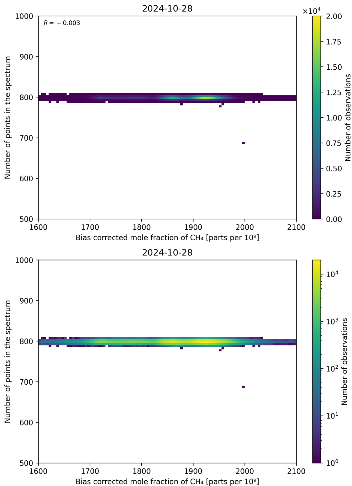
Figure 68: Scatter density plot of “Bias corrected mole fraction of CH 4 ” against “Number of points in the spectrum” for 2024-10-27 to 2024-10-29.
