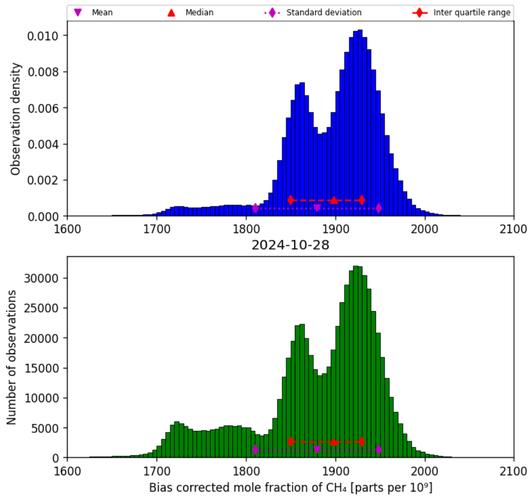
Figure 25: Histogram of “Bias corrected mole fraction of CH 4 ” for 2024-10-27 to 2024-10-29
