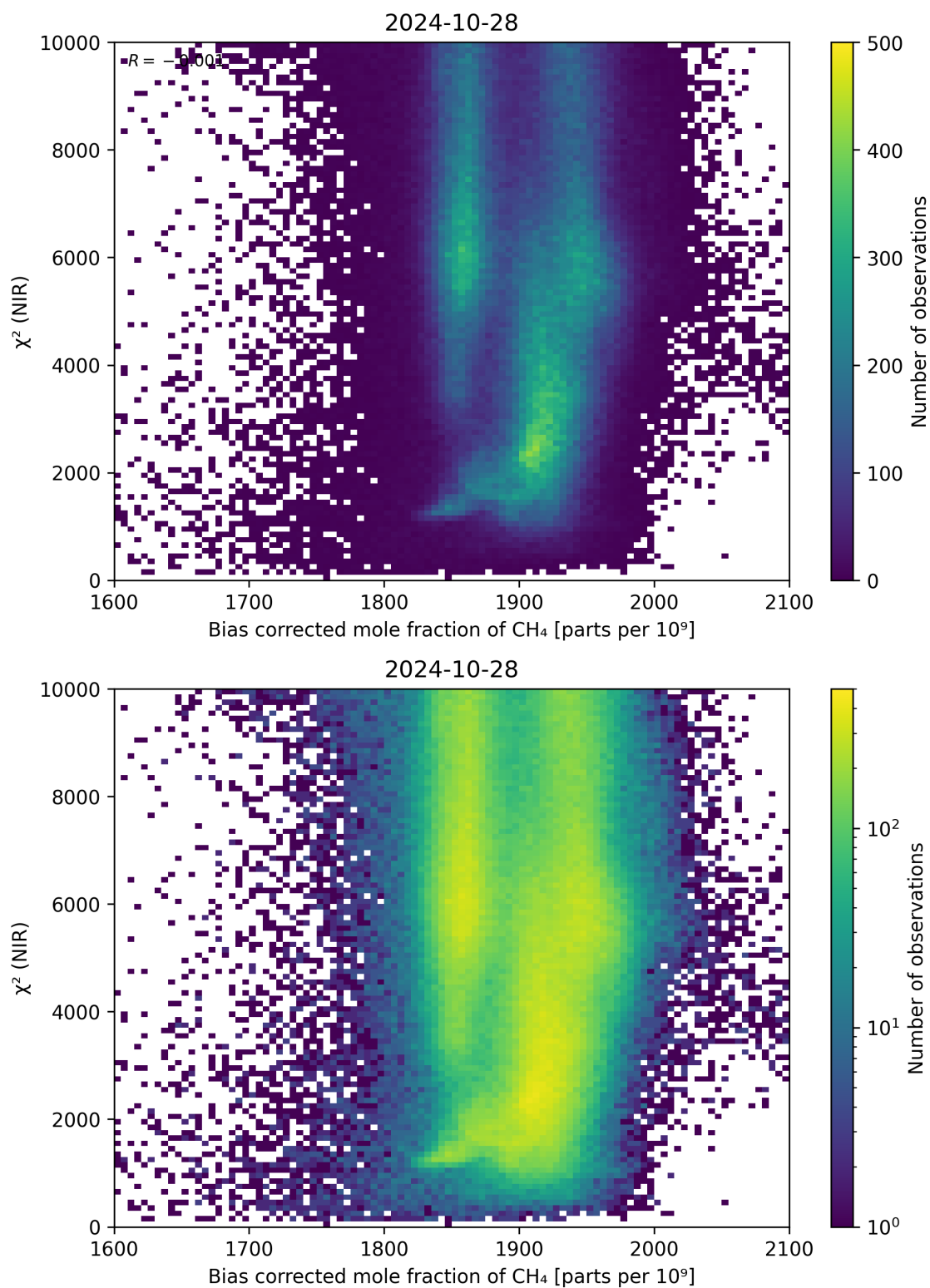
Figure 63: Scatter density plot of “Bias corrected mole fraction of \text{CH}_4 ” against “ \chi^2 (NIR)” for 2024-10-27 to 2024-10-29.
