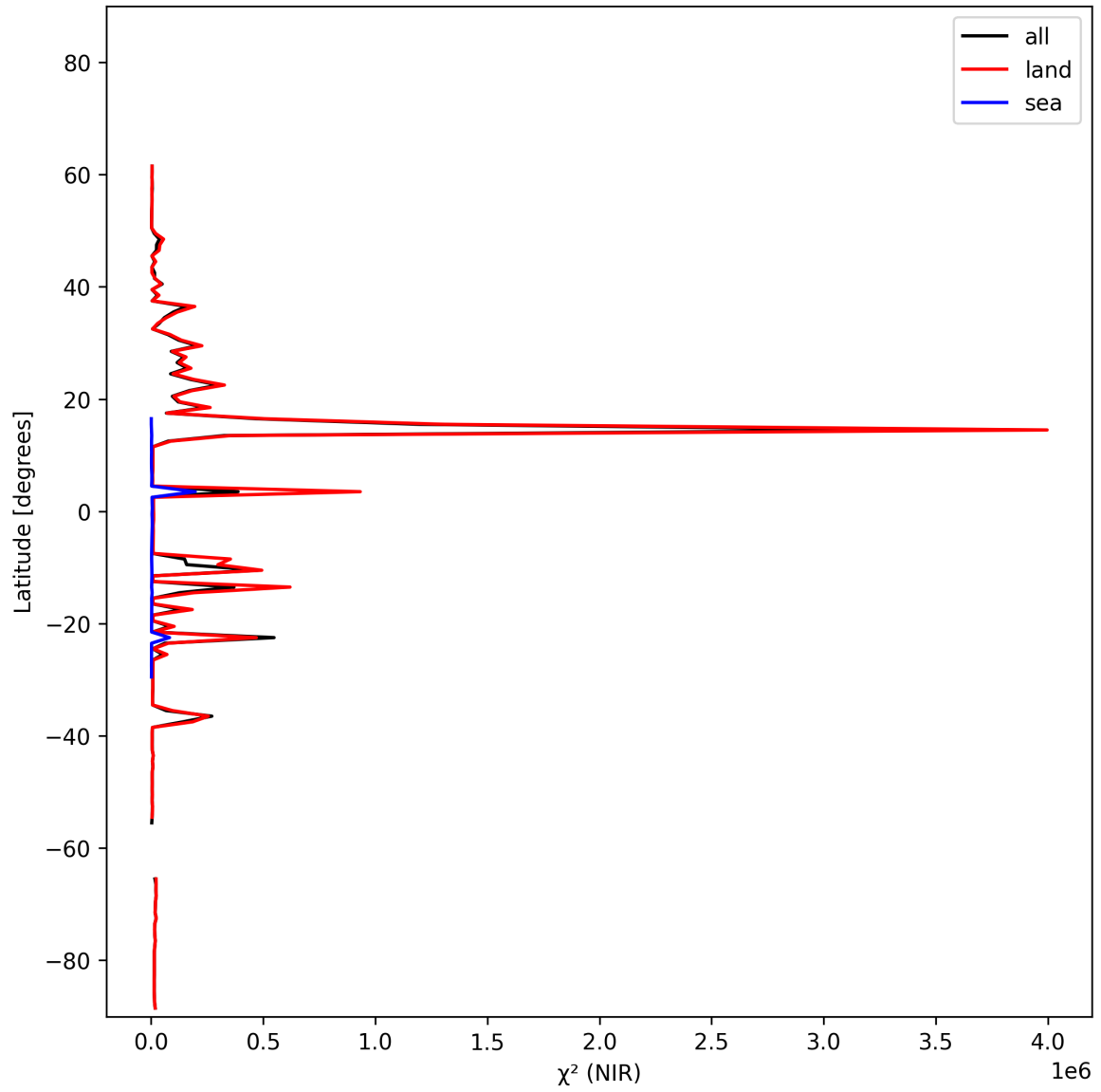
Figure 18: Zonal average of “ \chi^2 (NIR)” for 2024-10-27 to 2024-10-29.
