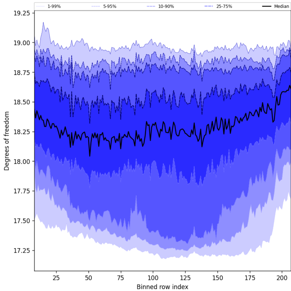
Figure 41: Along track statistics of “Degrees of freedom” for 2024-10-27 to 2024-10-29
