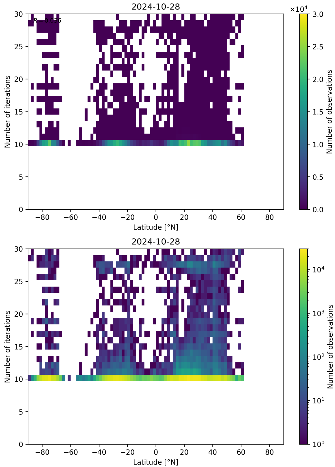
Figure 60: Scatter density plot of “Latitude” against “Number of iterations” for 2024-10-27 to 2024-10-29.
