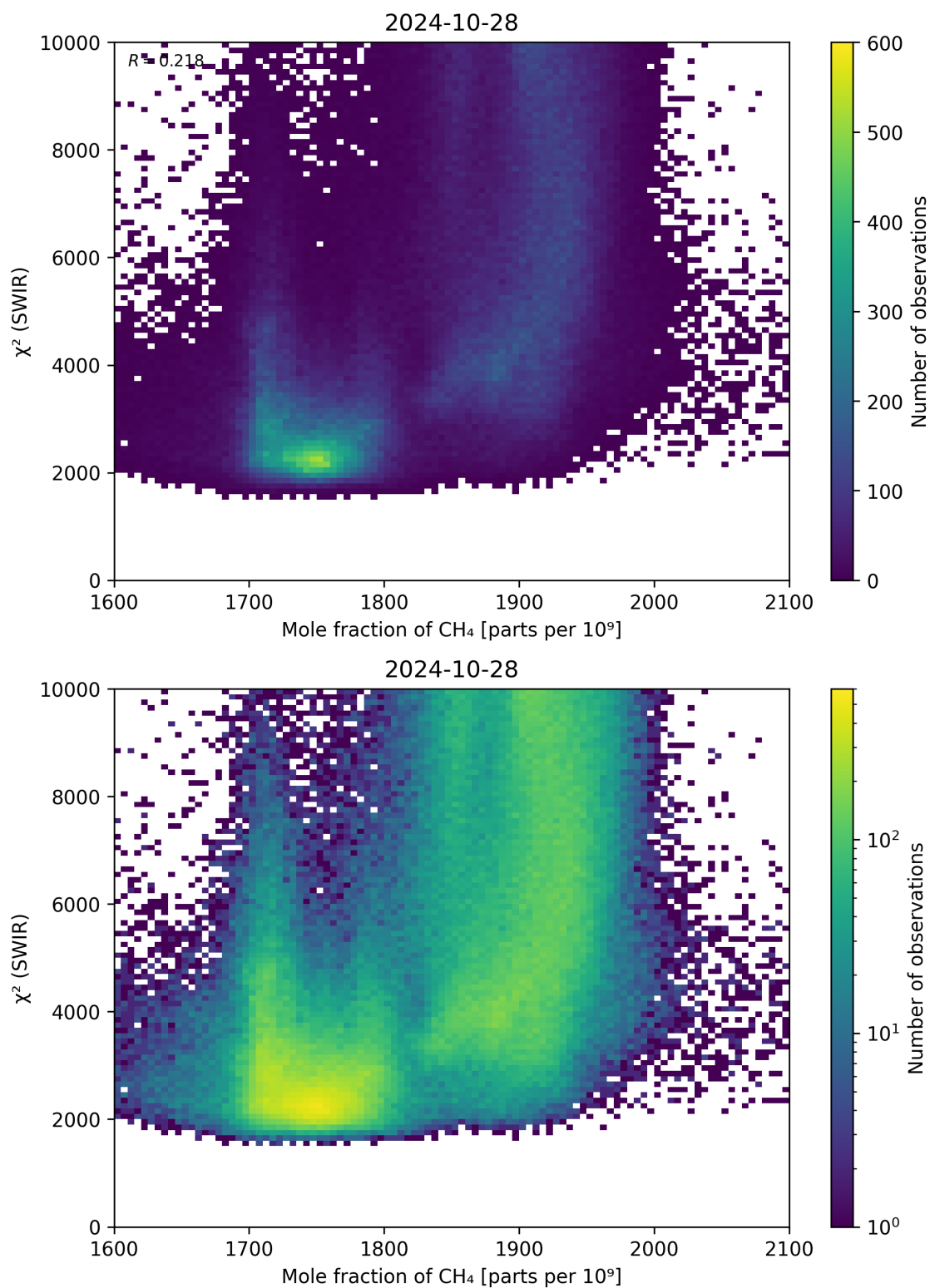
Figure 71: Scatter density plot of “Mole fraction of CH 4 ” against “ \chi^2 (SWIR)” for 2024-10-27 to 2024-10-29.
