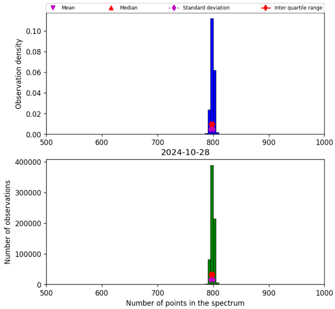
Figure 26: Histogram of “Number of points in the spectrum” for 2024-10-27 to 2024-10-29
