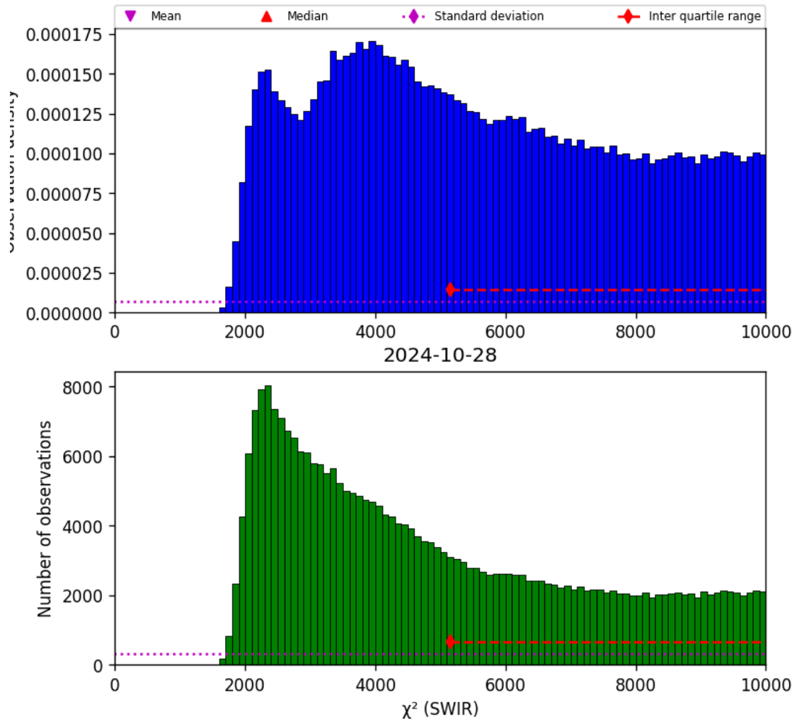
Figure 28: Histogram of “ \chi^2 (SWIR)” for 2024-10-27 to 2024-10-29
