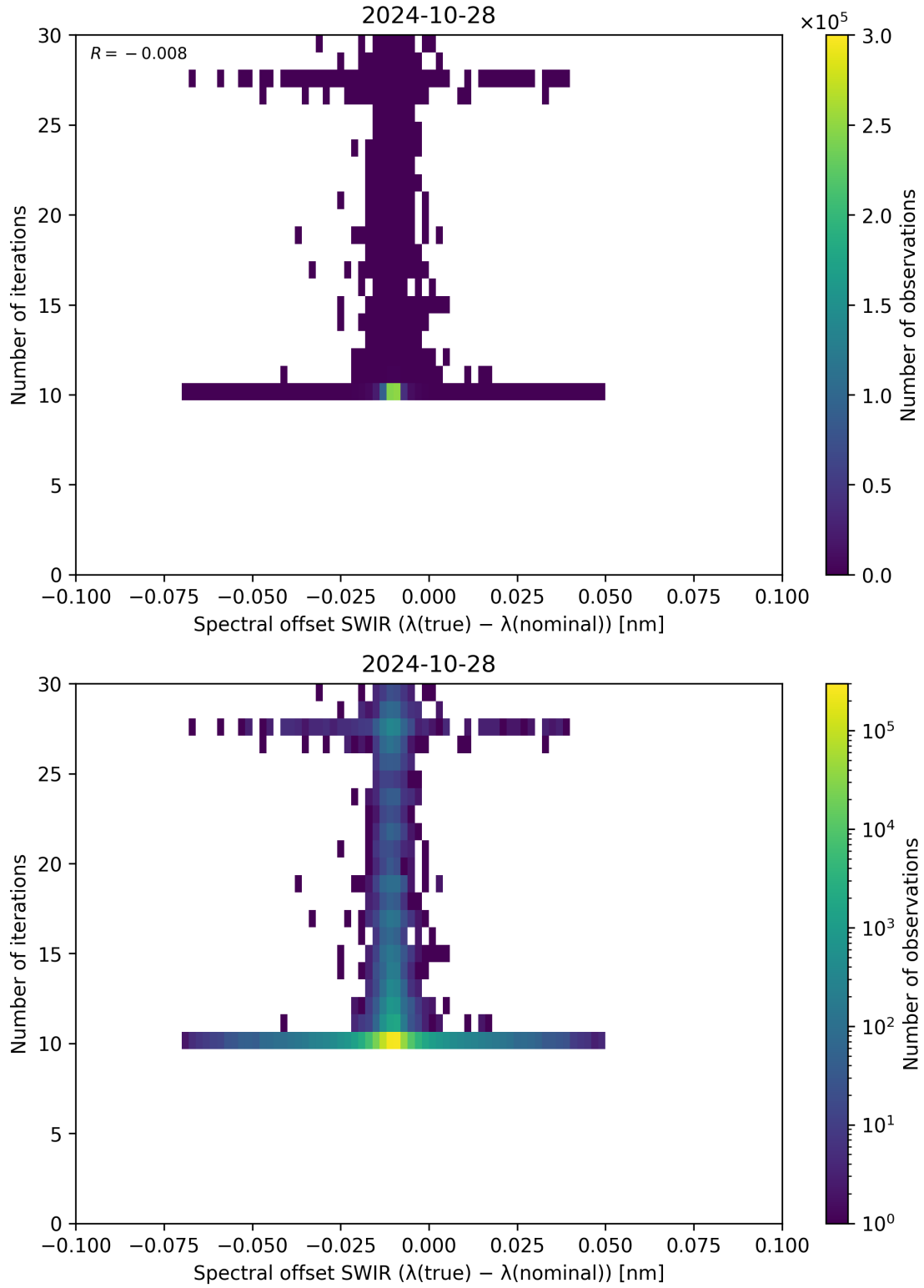
Figure 121: Scatter density plot of “Spectral offset SWIR ( \lambda_{\text{true}} - \lambda_{\text{nominal}} )” against “Number of iterations” for 2024-10-27 to 2024-10-29.
