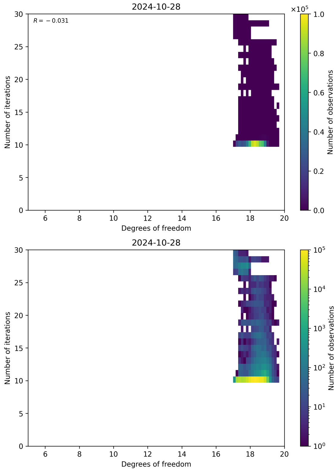
Figure 52: Scatter density plot of “Degrees of freedom” against “Number of iterations” for 2024-10-27 to 2024-10-29.
