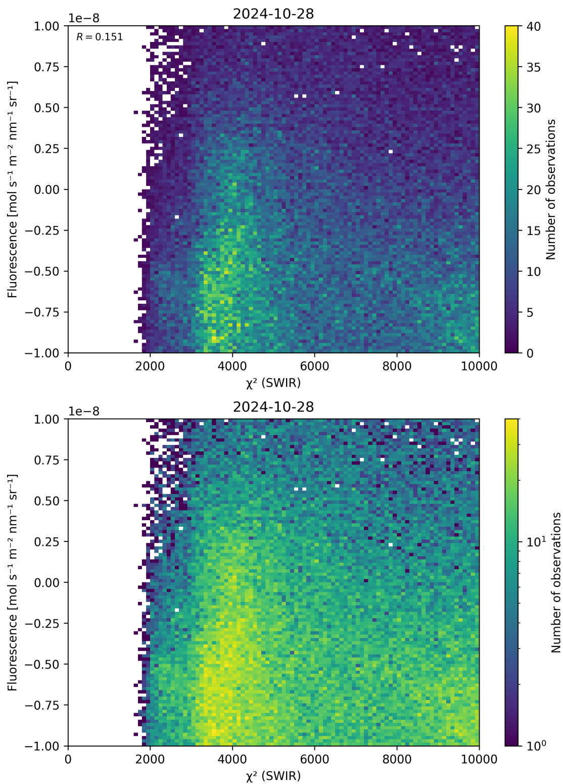
Figure 49: Scatter density plot of “ \chi^2 (SWIR)” against “Fluorescence” for 2024-10-27 to 2024-10-29.
