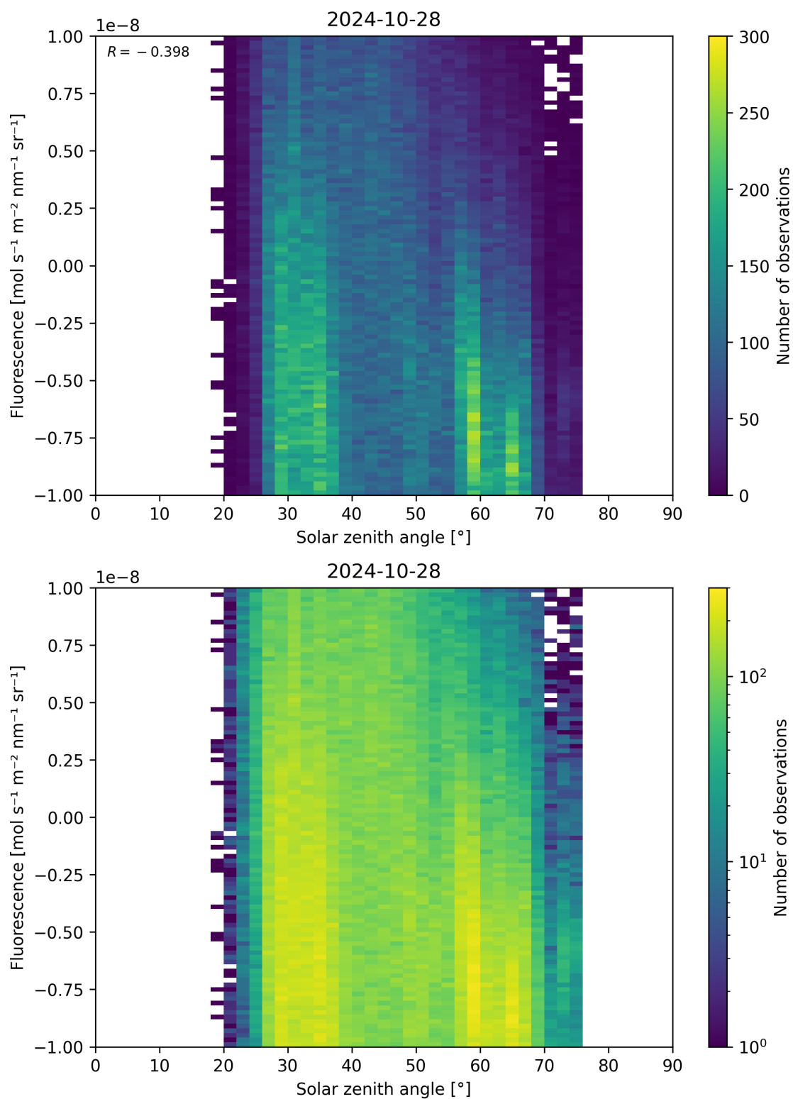
Figure 97: Scatter density plot of “Solar zenith angle” against “Fluorescence” for 2024-10-27 to 2024-10-29.
