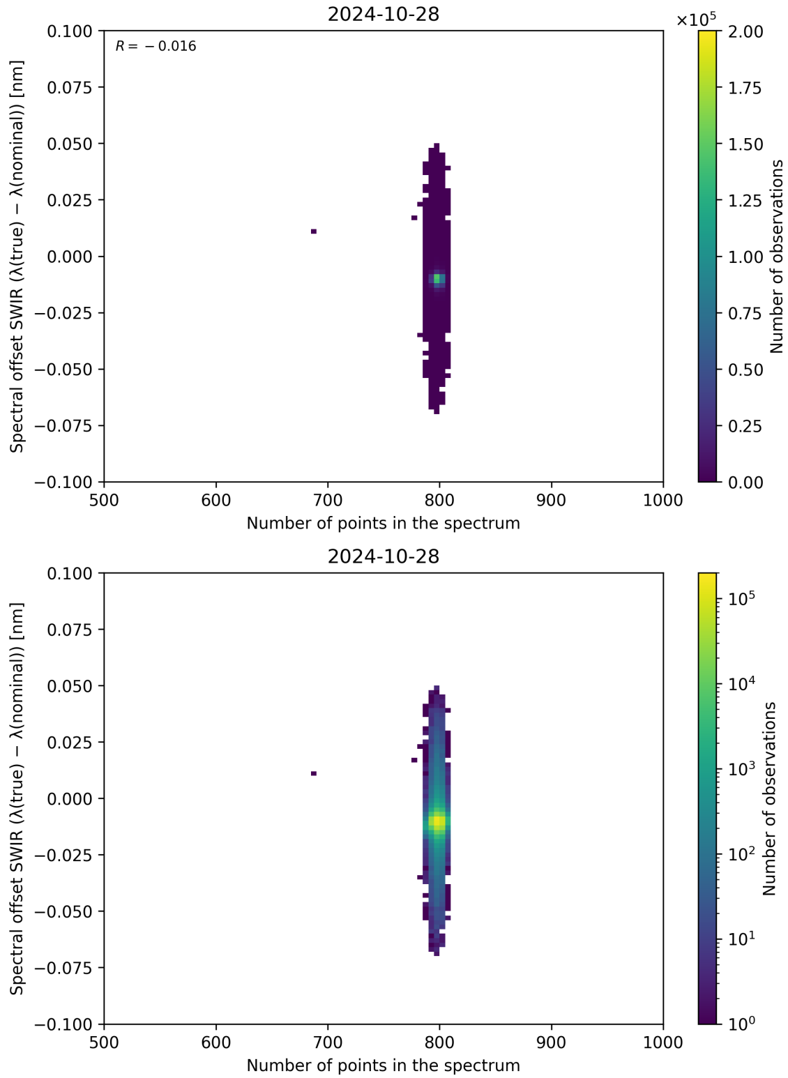
Figure 93: Scatter density plot of “Number of points in the spectrum” against “Spectral offset SWIR ( \lambda_{\text{true}} - \lambda_{\text{nominal}} )” for 2024-10-27 to 2024-10-29.
