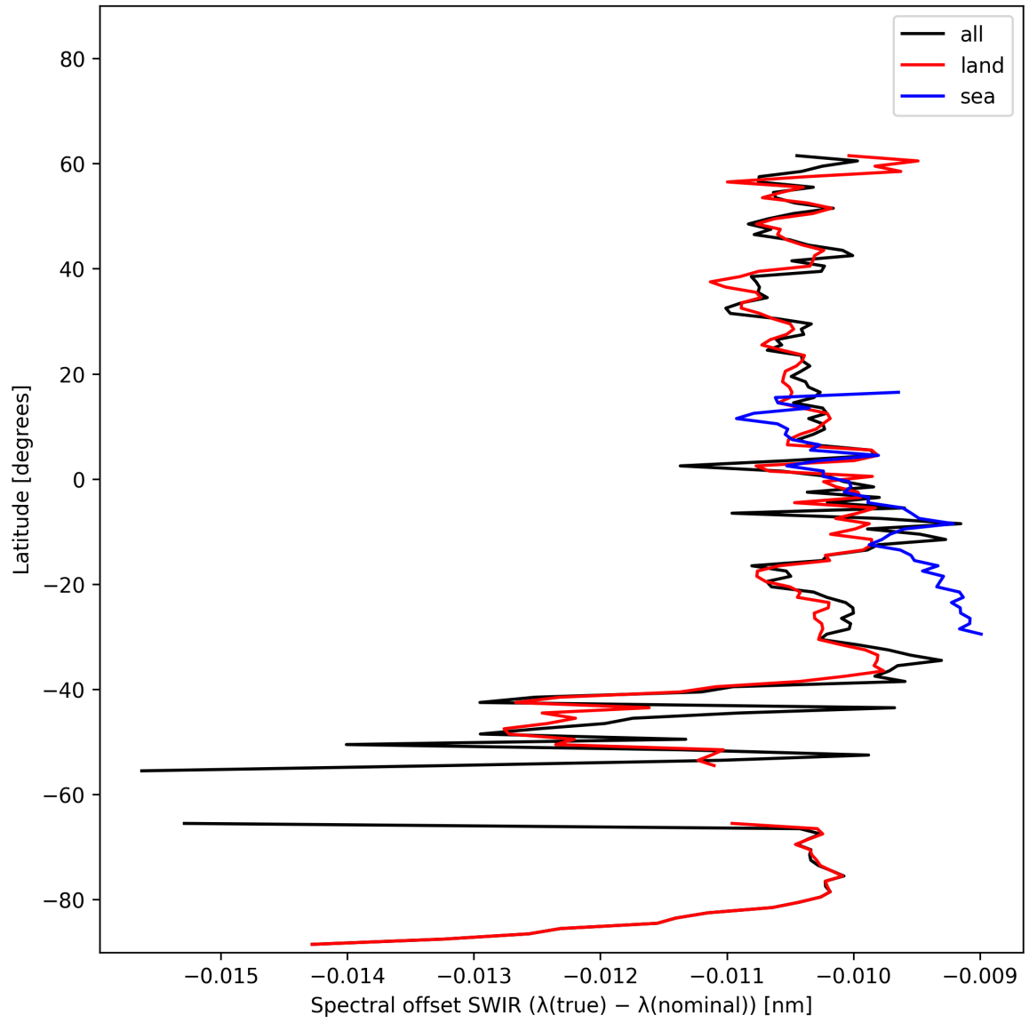
Figure 16: Zonal average of “Spectral offset SWIR ( \lambda_{\text{true}} - \lambda_{\text{nominal}} )” for 2024-10-27 to 2024-10-29.
