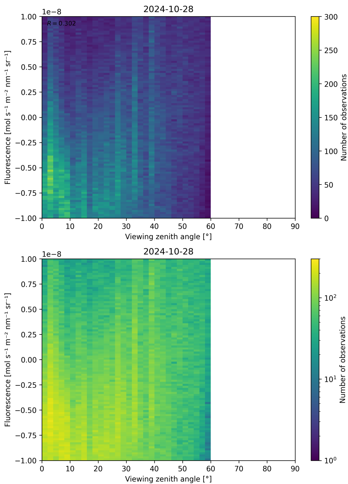
Figure 108: Scatter density plot of “Viewing zenith angle” against “Fluorescence” for 2024-10-27 to 2024-10-29.
