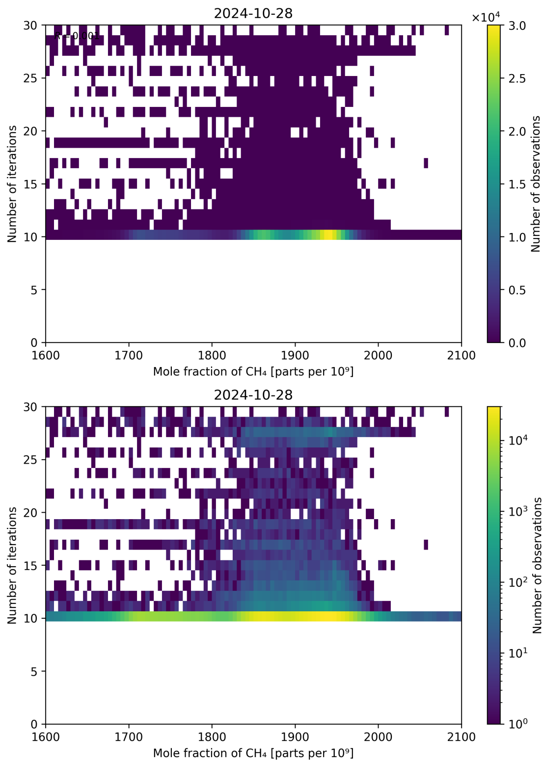
Figure 76: Scatter density plot of “Mole fraction of CH 4 ” against “Number of iterations” for 2024-10-27 to 2024-10-29.
