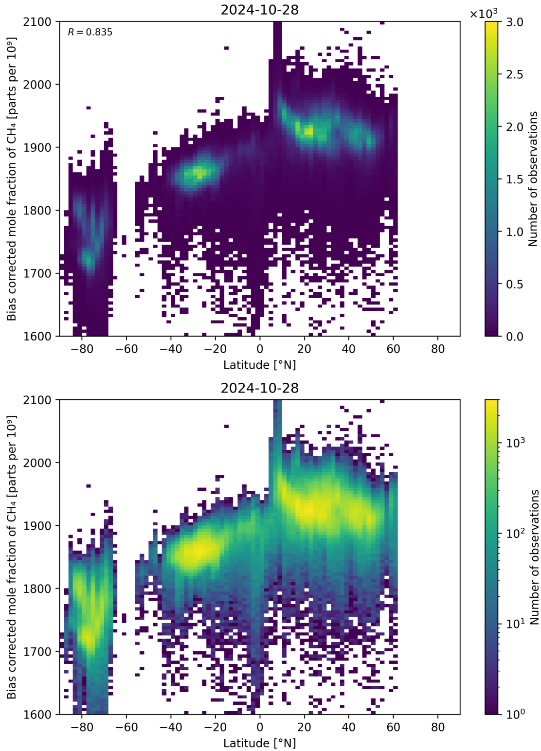
Figure 58: Scatter density plot of “Latitude” against “Bias corrected mole fraction of \text{CH}_4 ” for 2024-10-27 to 2024-10-29.
