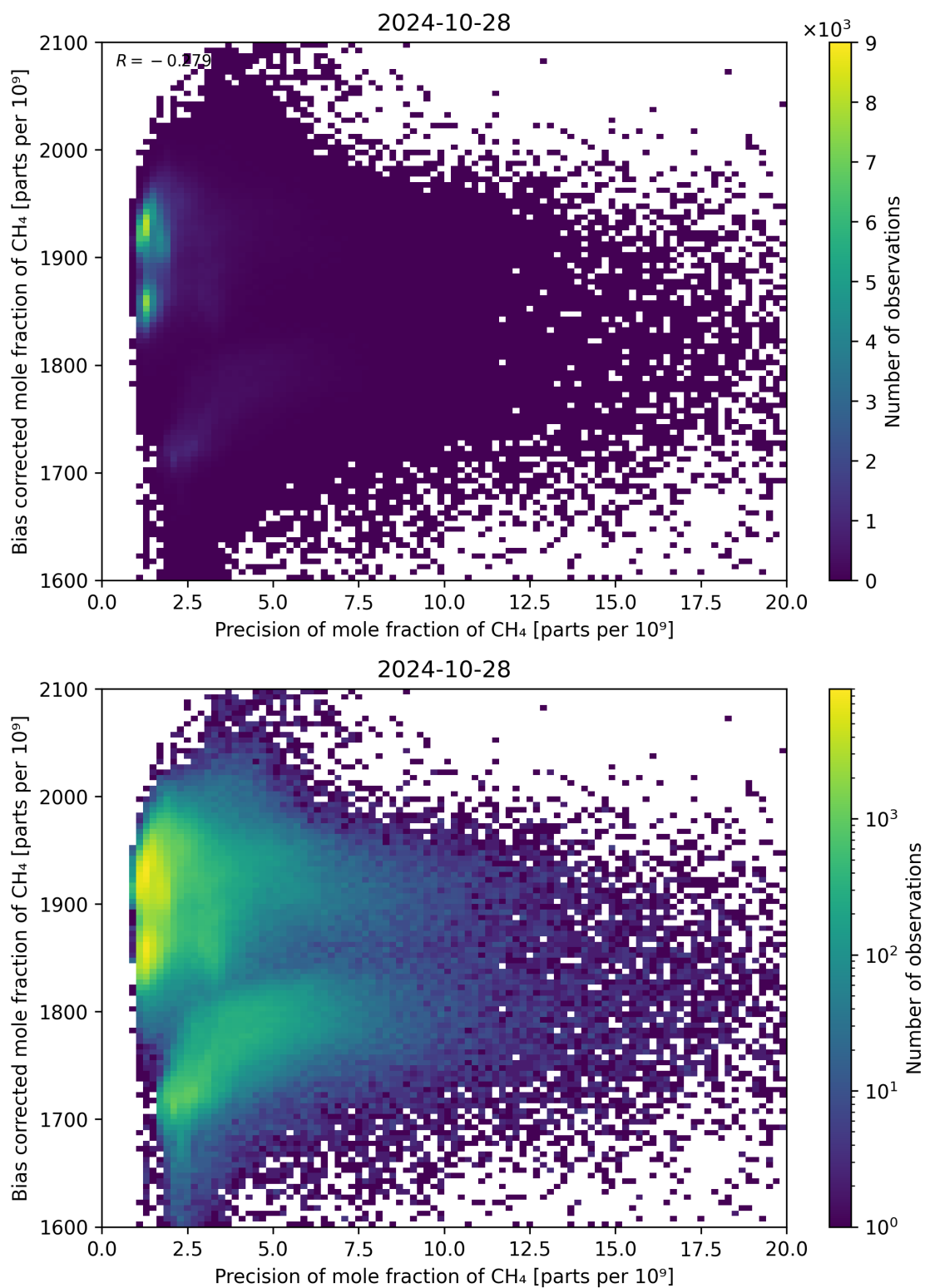
Figure 82: Scatter density plot of “Precision of mole fraction of CH 4 ” against “Bias corrected mole fraction of CH 4 ” for 2024-10-27 to 2024-10-29.
