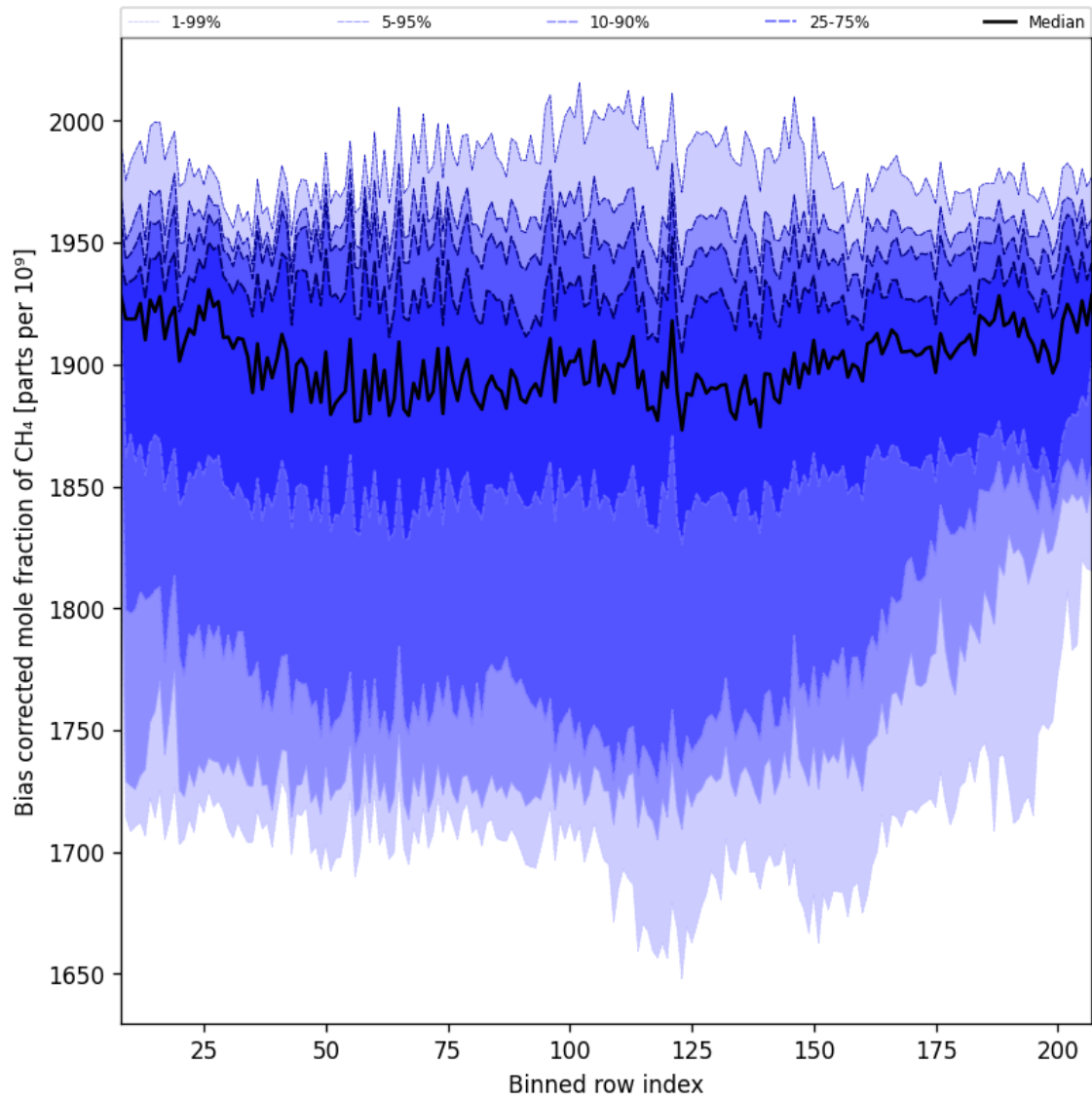
Figure 36: Along track statistics of “Bias corrected mole fraction of CH 4 ” for 2024-10-27 to 2024-10-29
