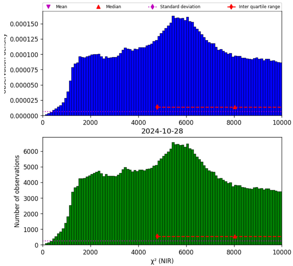
Figure 29: Histogram of “ \chi^2 (NIR)” for 2024-10-27 to 2024-10-29
