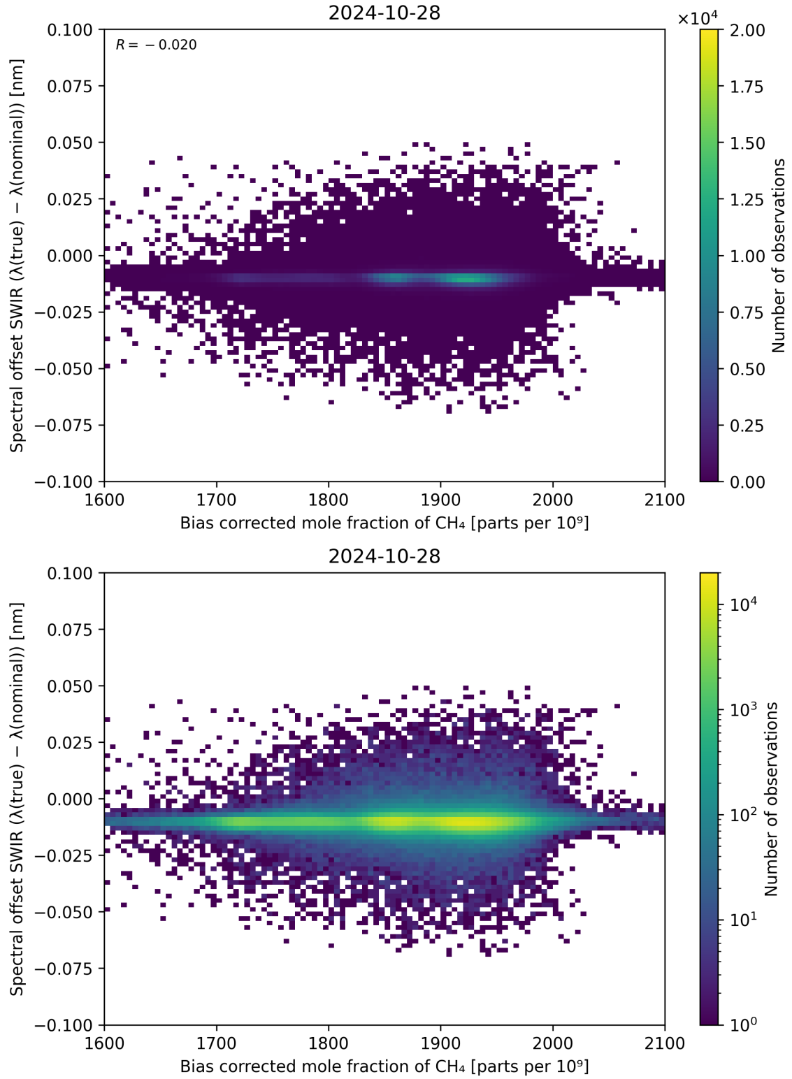
Figure 69: Scatter density plot of “Bias corrected mole fraction of \text{CH}_4 ” against “Spectral offset SWIR ( \lambda_{\text{true}} - \lambda_{\text{nominal}} )” for 2024-10-27 to 2024-10-29.
