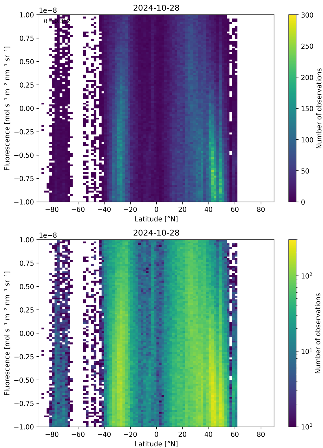
Figure 56: Scatter density plot of “Latitude” against “Fluorescence” for 2024-10-27 to 2024-10-29.
