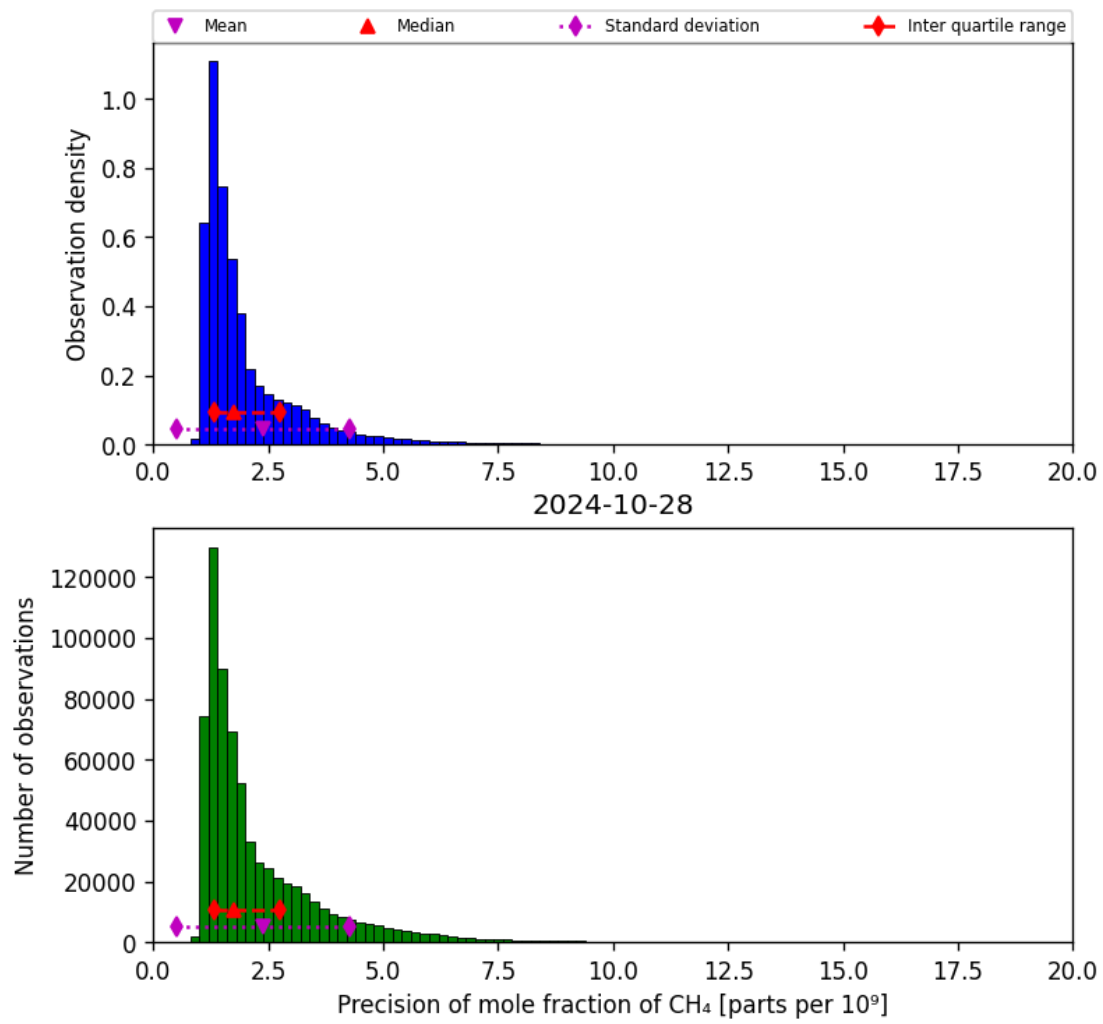
Figure 24: Histogram of “Precision of mole fraction of CH 4 ” for 2024-10-27 to 2024-10-29
