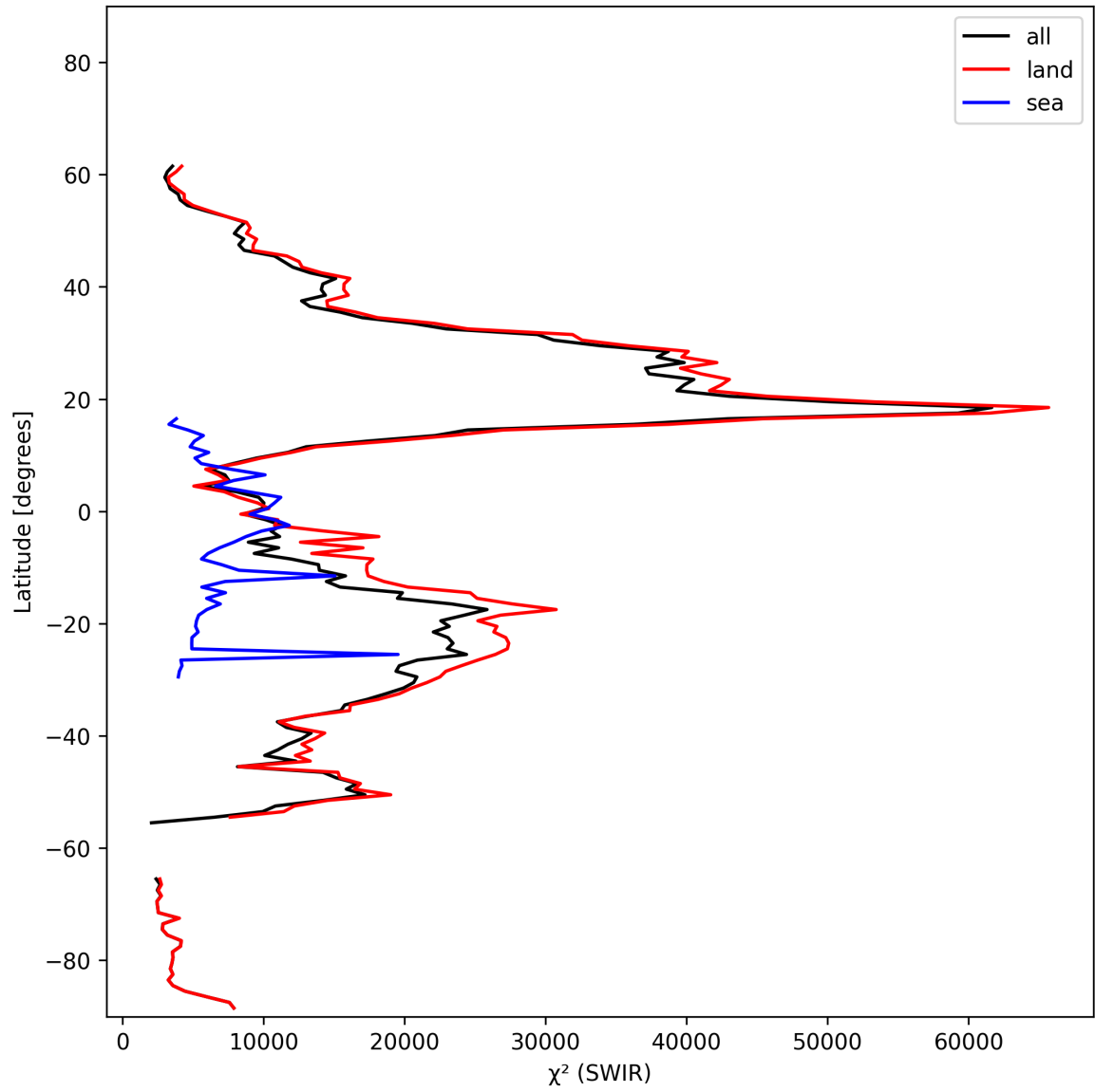
Figure 17: Zonal average of “ \chi^2 (SWIR)” for 2024-10-27 to 2024-10-29.
