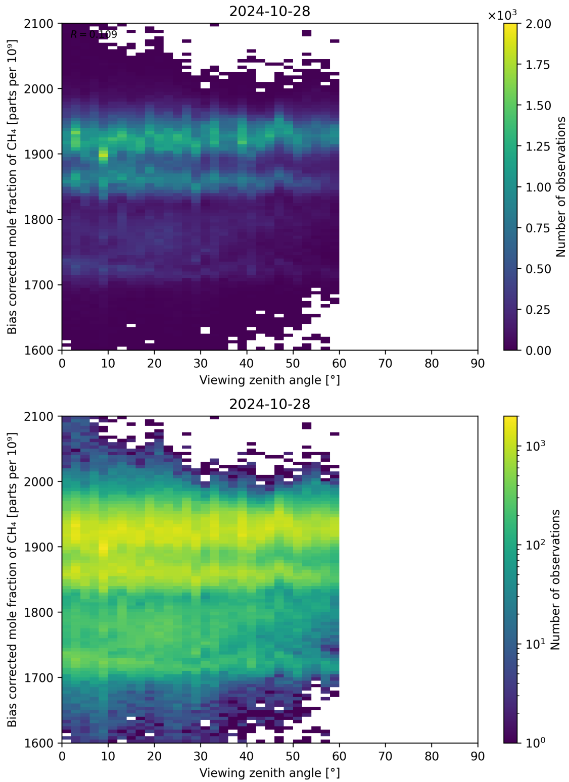
Figure 111: Scatter density plot of “Viewing zenith angle” against “Bias corrected mole fraction of CH 4 ” for 2024-10-27 to 2024-10-29.
