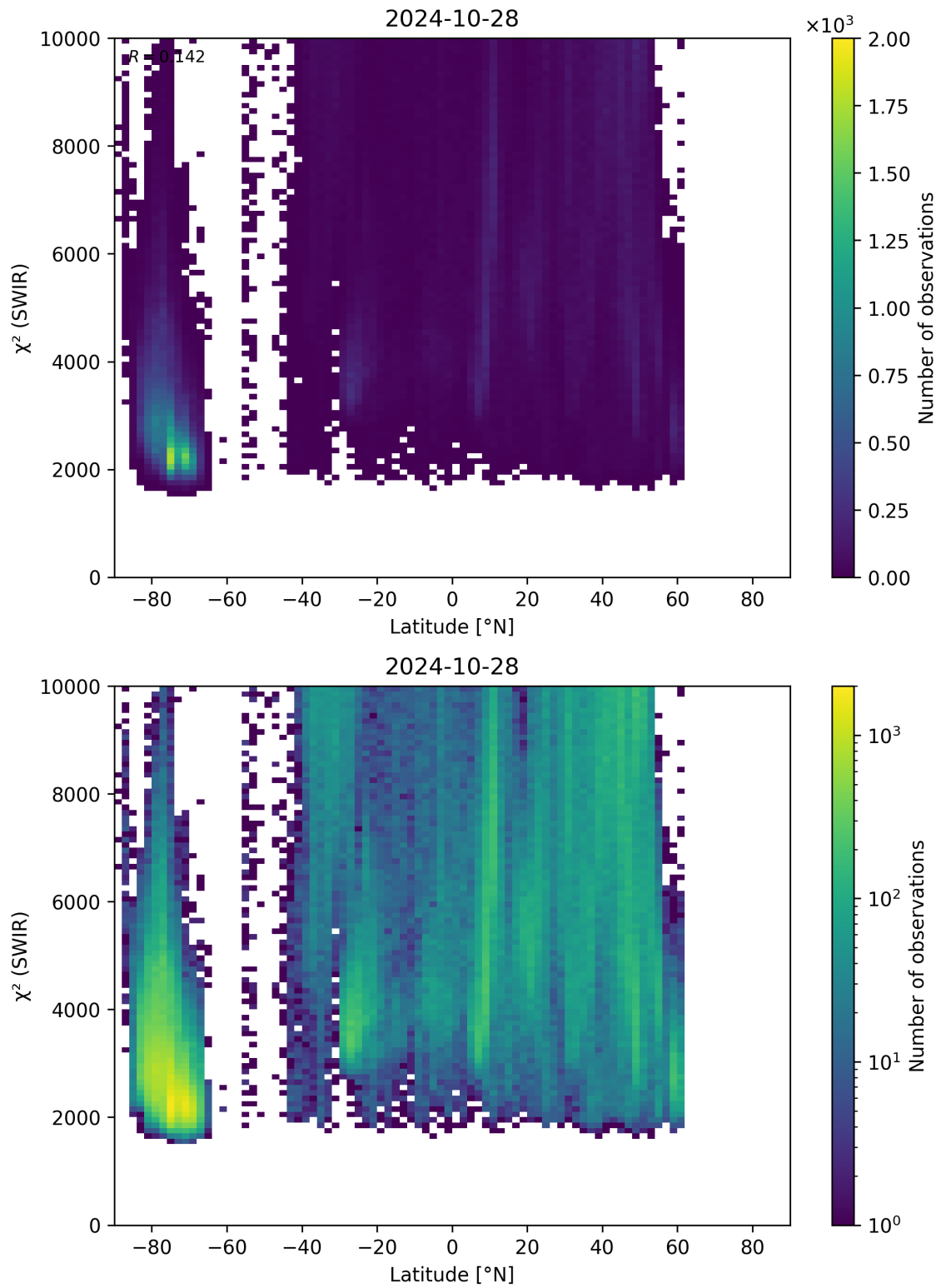
Figure 54: Scatter density plot of “Latitude” against “ \chi^2 (SWIR)” for 2024-10-27 to 2024-10-29.
