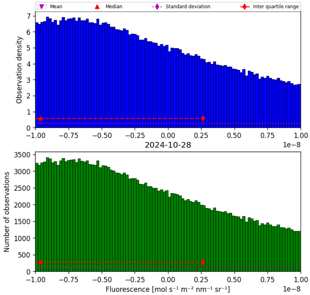
Figure 32: Histogram of “Fluorescence” for 2024-10-27 to 2024-10-29
