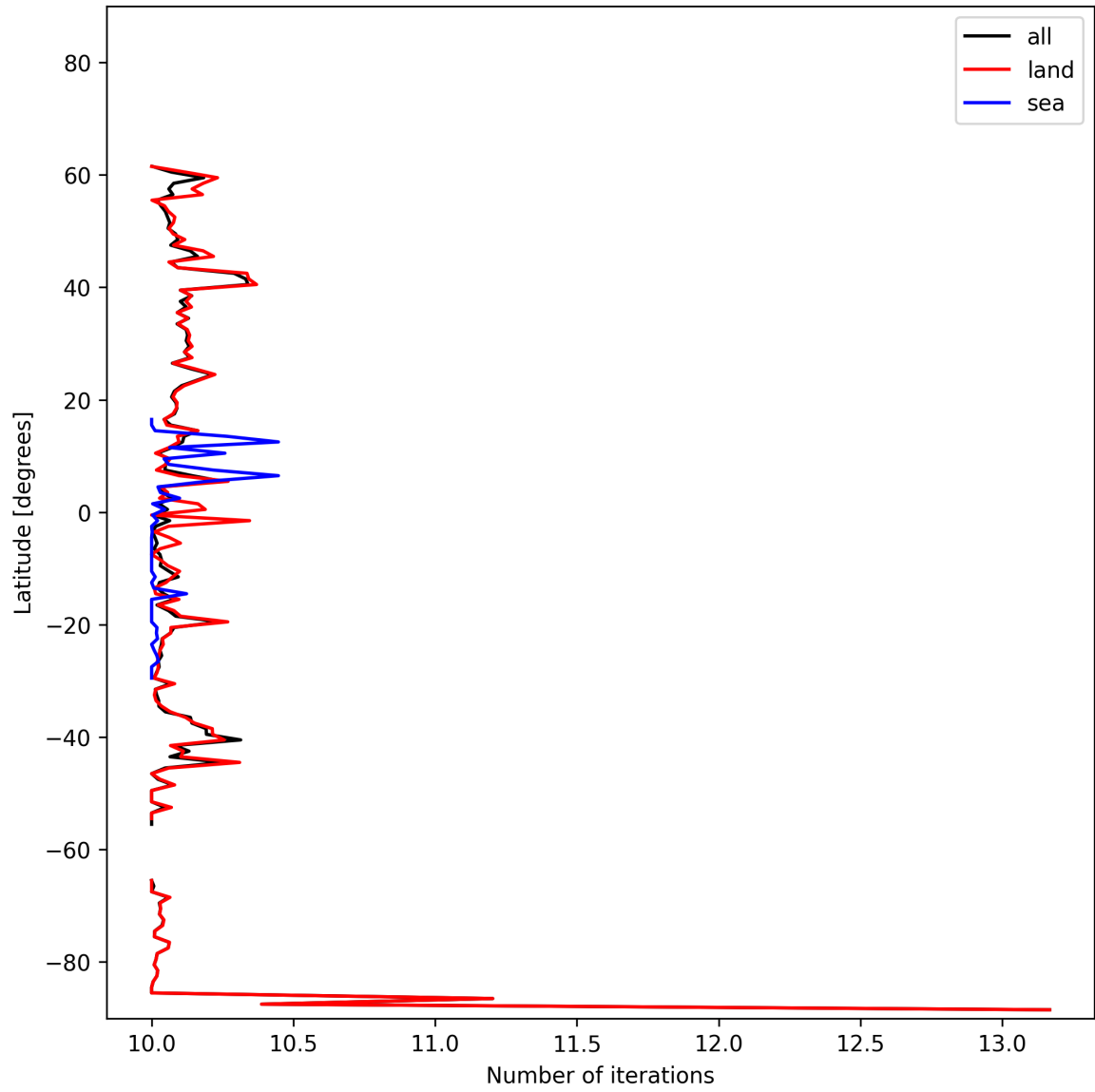
Figure 20: Zonal average of “Number of iterations” for 2024-10-27 to 2024-10-29.
