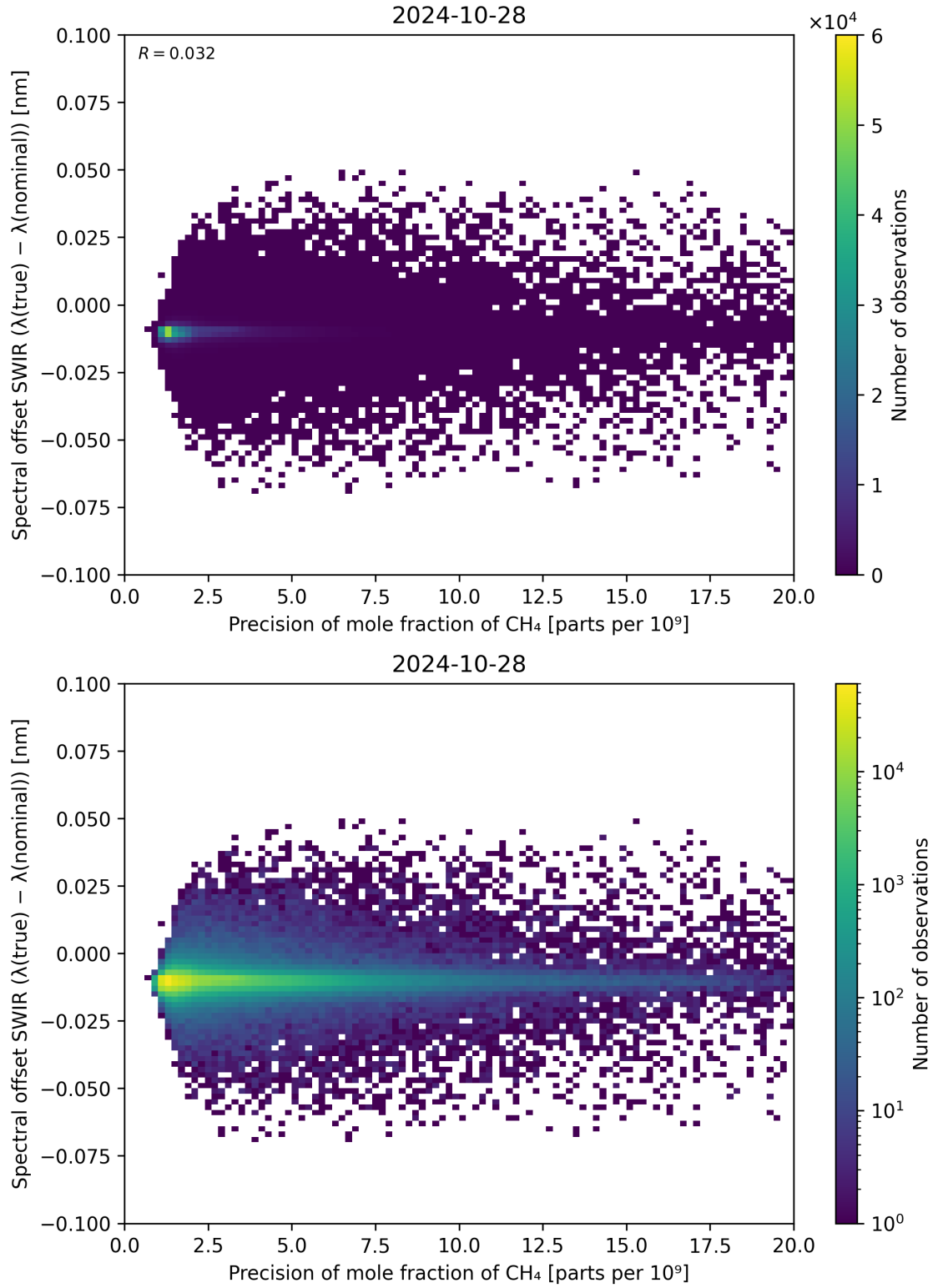
Figure 85: Scatter density plot of “Precision of mole fraction of \text{CH}_4 ” against “Spectral offset SWIR ( \lambda_{\text{true}} - \lambda_{\text{nominal}} )” for 2024-10-27 to 2024-10-29.
