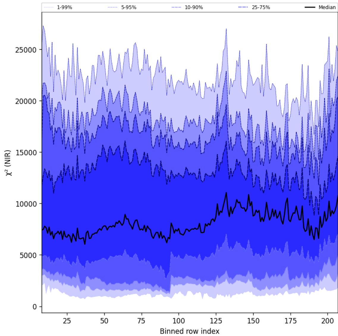
Figure 40: Along track statistics of “ \chi^2 (NIR)” for 2024-10-27 to 2024-10-29
