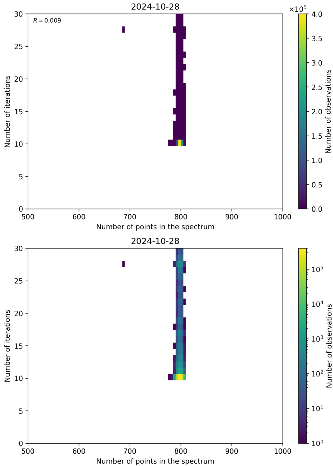
Figure 92: Scatter density plot of “Number of points in the spectrum” against “Number of iterations” for 2024-10-27 to 2024-10-29.
