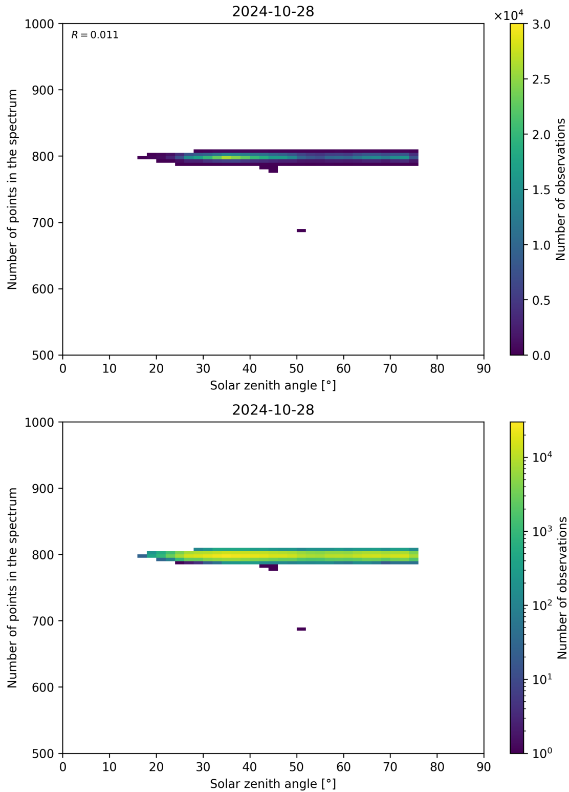
Figure 103: Scatter density plot of “Solar zenith angle” against “Number of points in the spectrum” for 2024-10-27 to 2024-10-29.
