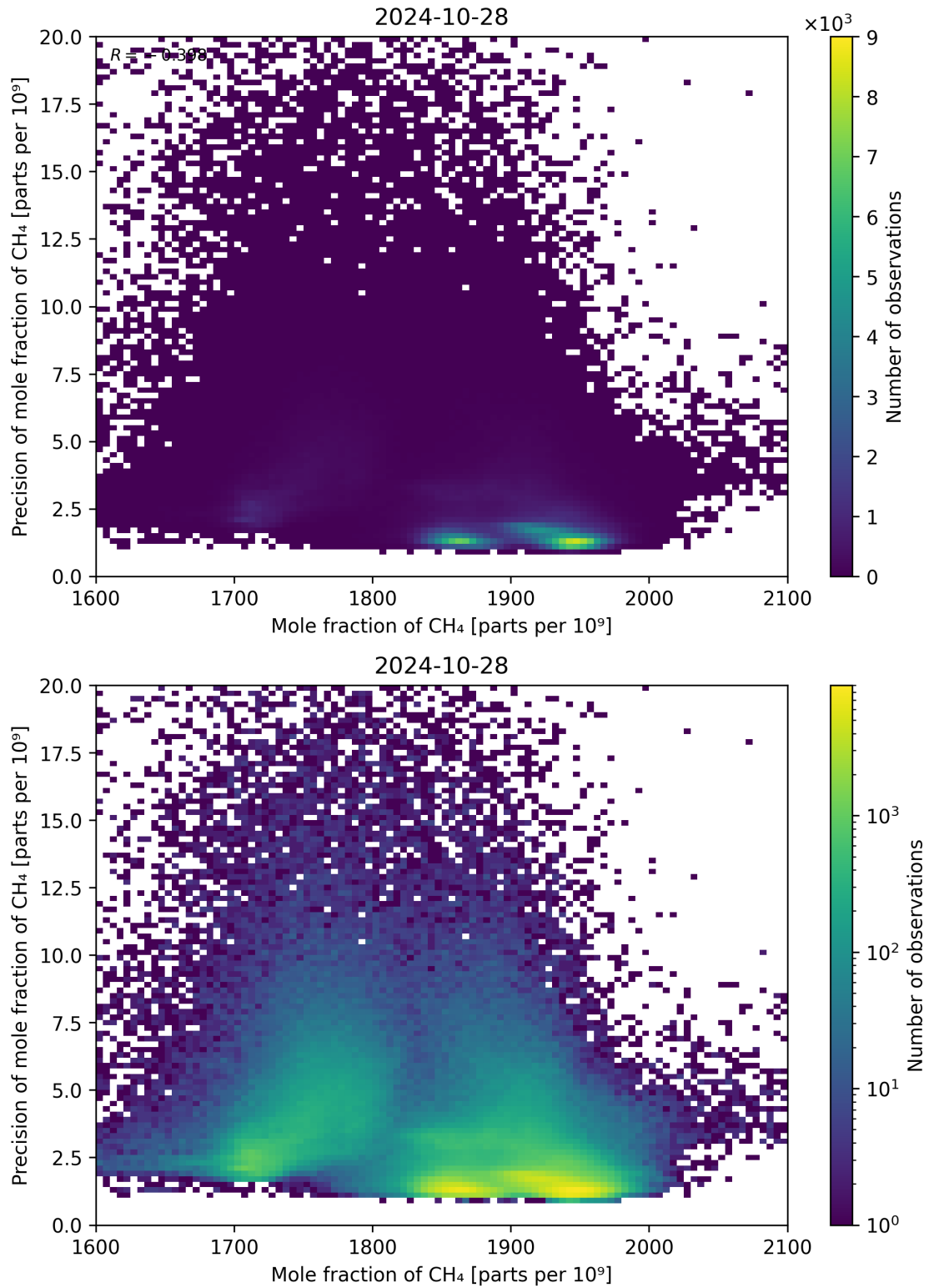
Figure 75: Scatter density plot of “Mole fraction of CH 4 ” against “Precision of mole fraction of CH 4 ” for 2024-10-27 to 2024-10-29.
