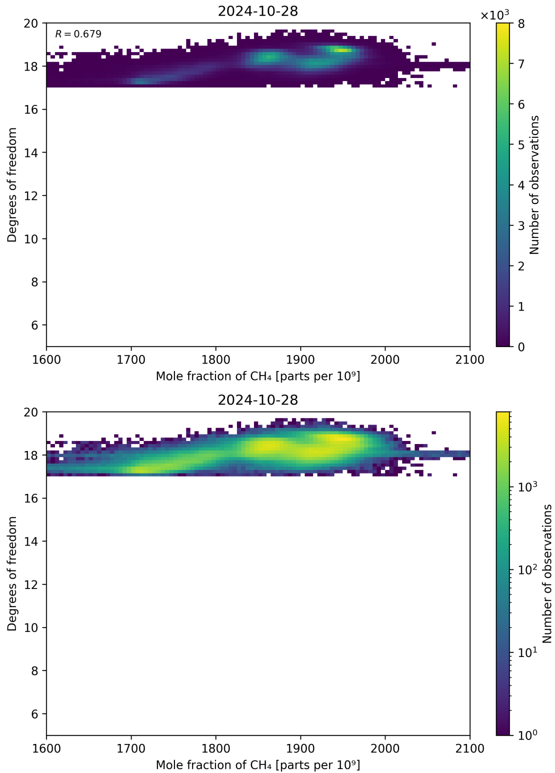
Figure 72: Scatter density plot of “Mole fraction of CH 4 ” against “Degrees of freedom” for 2024-10-27 to 2024-10-29.
