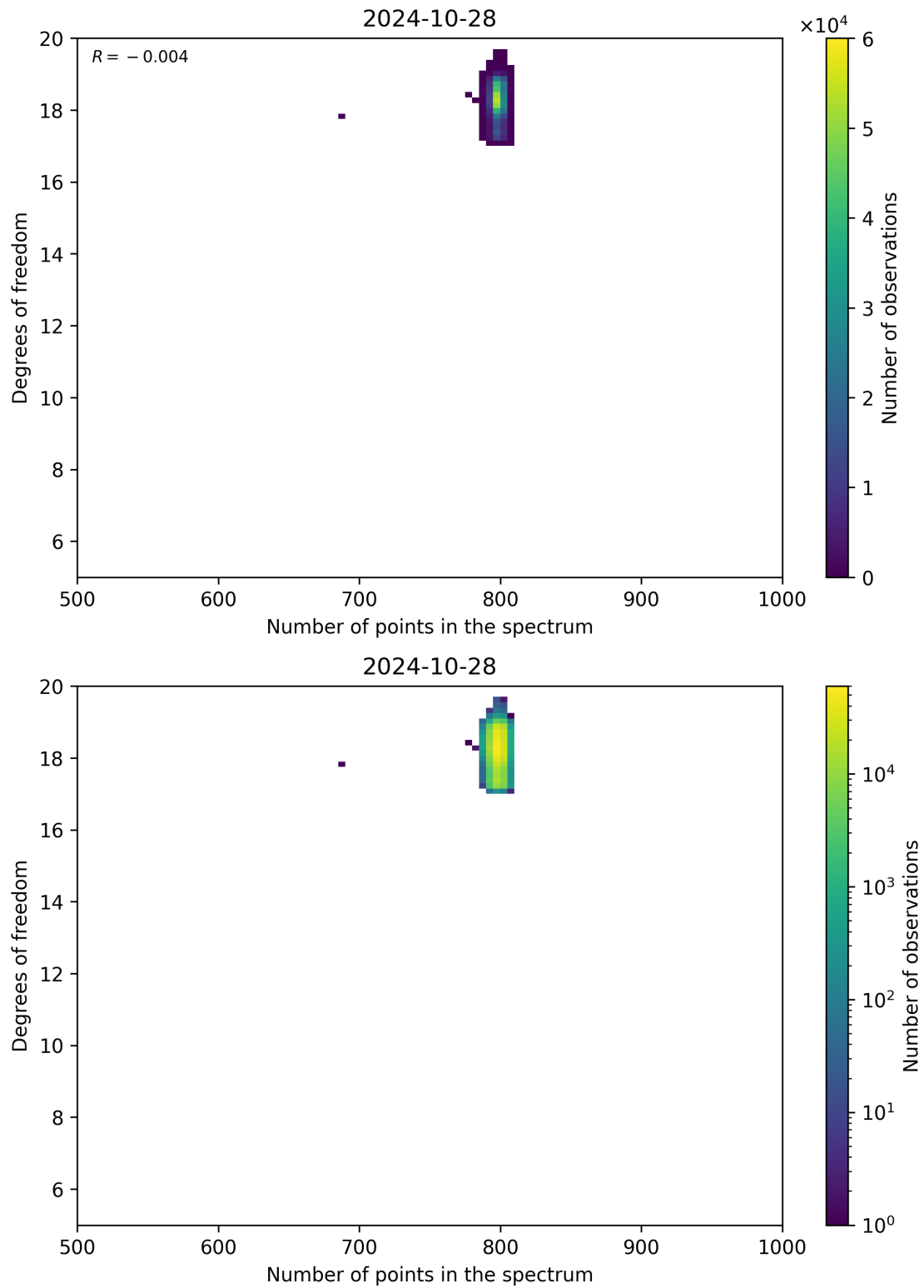
Figure 90: Scatter density plot of “Number of points in the spectrum” against “Degrees of freedom” for 2024-10-27 to 2024-10-29.
