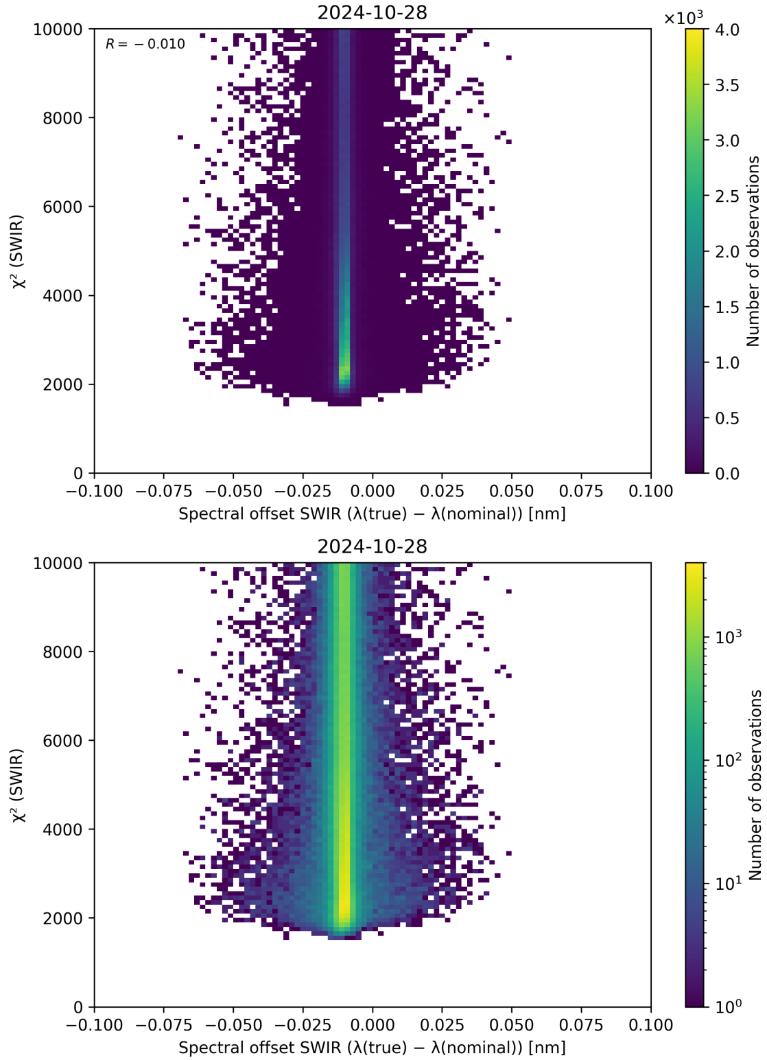
Figure 118: Scatter density plot of “Spectral offset SWIR ( \lambda_{\text{true}} - \lambda_{\text{nominal}} )” against “ \chi^2 (SWIR)” for 2024-10-27 to 2024-10-29.
