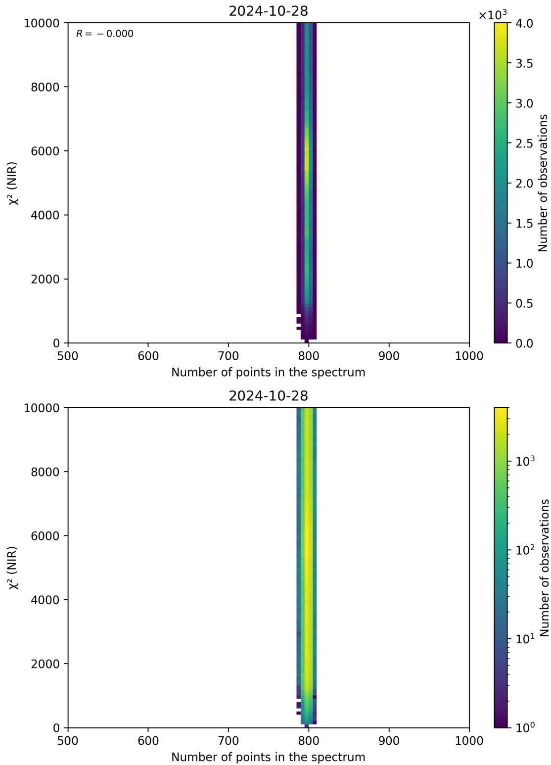
Figure 88: Scatter density plot of “Number of points in the spectrum” against “ \chi^2 (NIR)” for 2024-10-27 to 2024-10-29.
