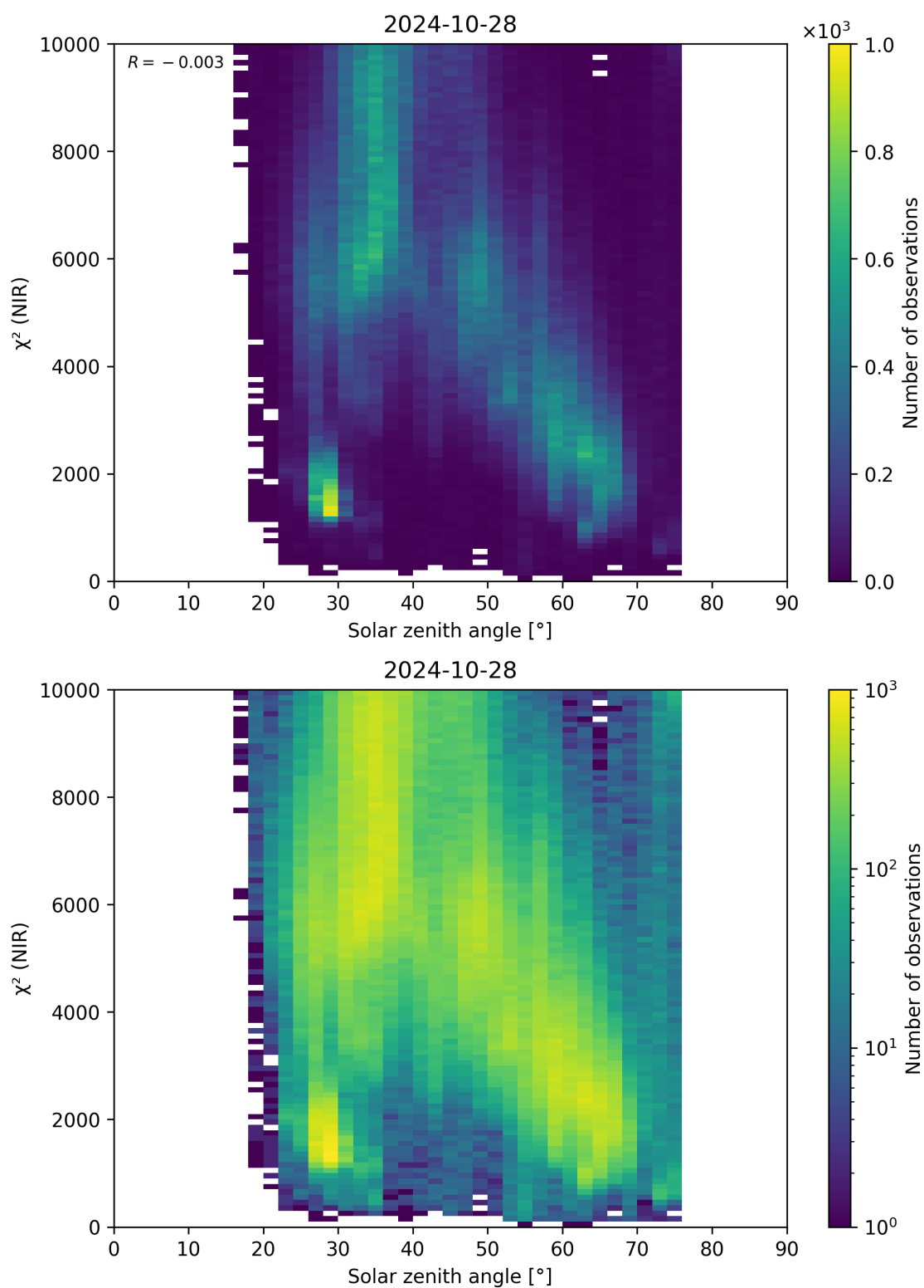
Figure 94: Scatter density plot of “Solar zenith angle” against “ \chi^2 (NIR)” for 2024-10-27 to 2024-10-29.
