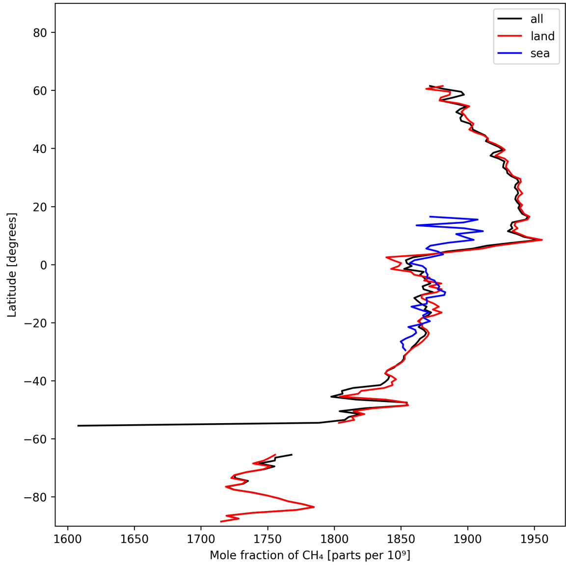
Figure 12: Zonal average of “Mole fraction of \text{CH}_4 ” for 2024-10-27 to 2024-10-29.
