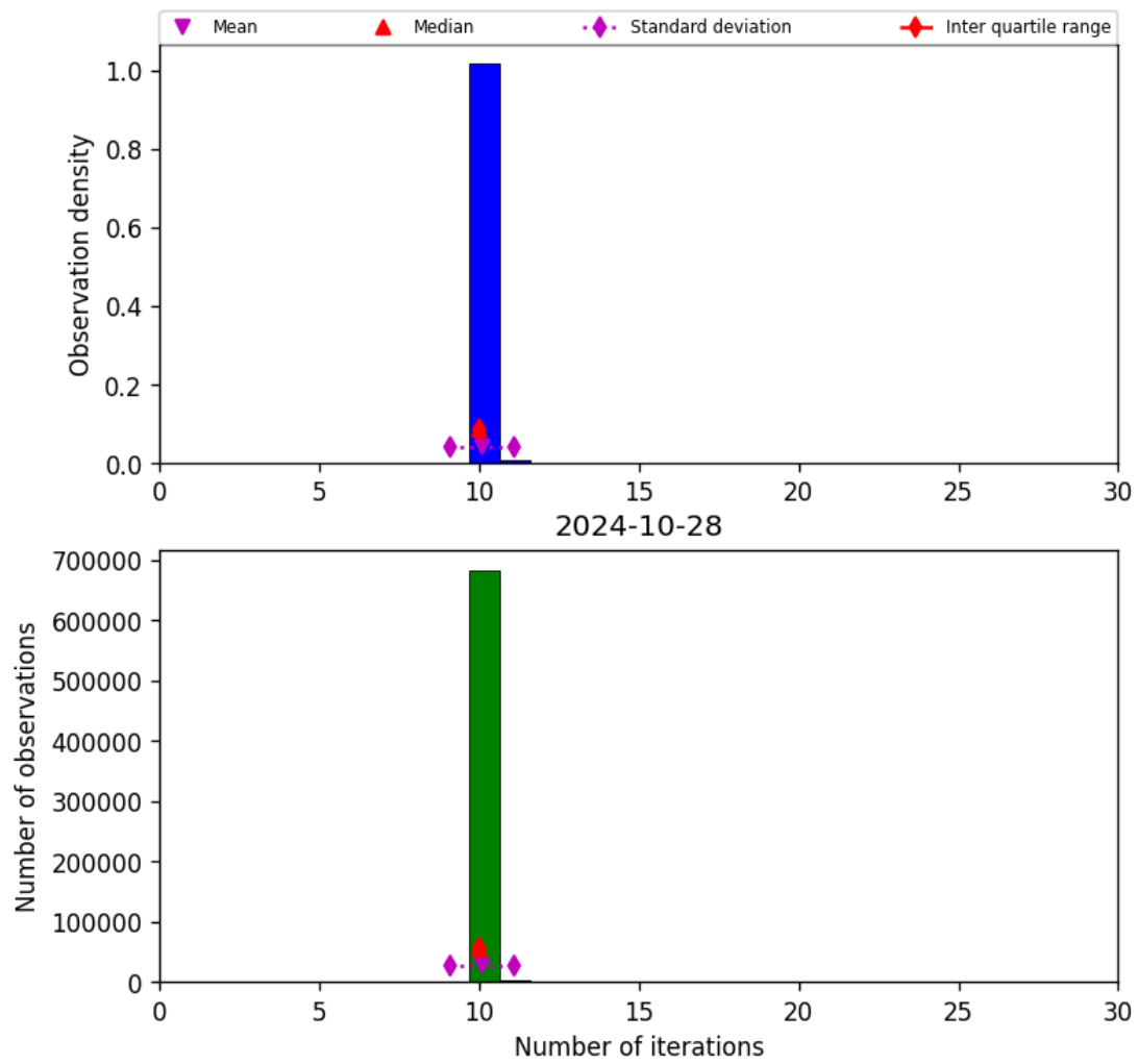
Figure 31: Histogram of “Number of iterations” for 2024-10-27 to 2024-10-29
