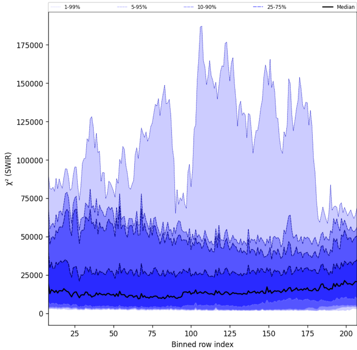
Figure 39: Along track statistics of “ \chi^2 (SWIR)” for 2024-10-27 to 2024-10-29
