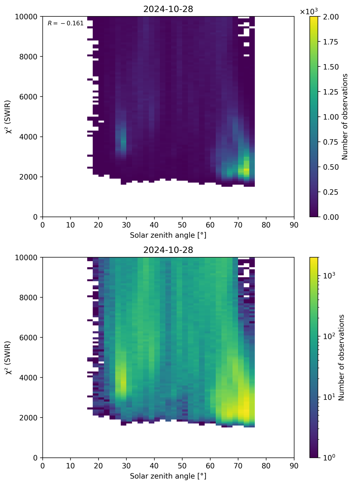
Figure 95: Scatter density plot of “Solar zenith angle” against “ \chi^2 (SWIR)” for 2024-10-27 to 2024-10-29.
