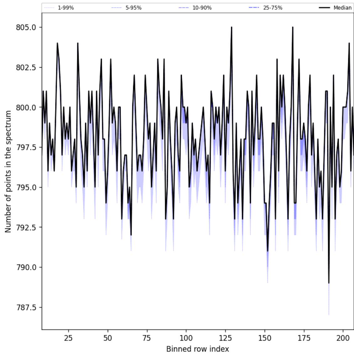
Figure 37: Along track statistics of “Number of points in the spectrum” for 2024-10-27 to 2024-10-29
