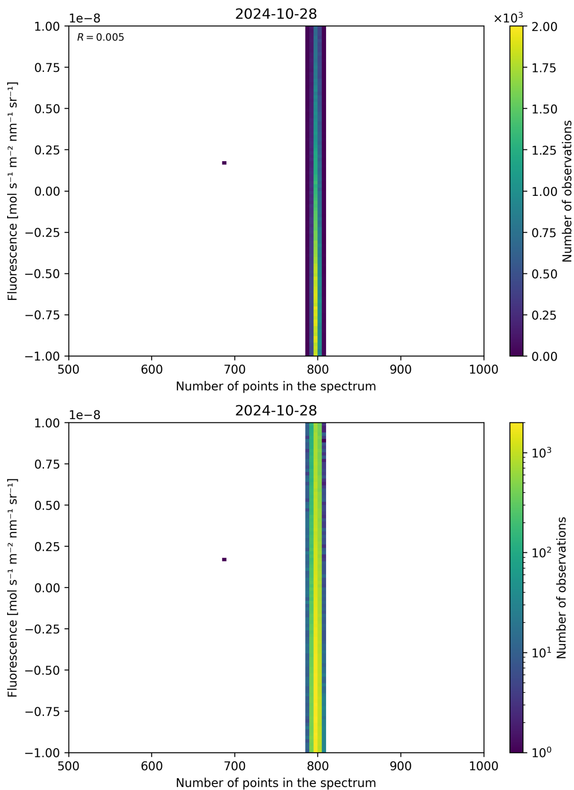
Figure 91: Scatter density plot of “Number of points in the spectrum” against “Fluorescence” for 2024-10-27 to 2024-10-29.
