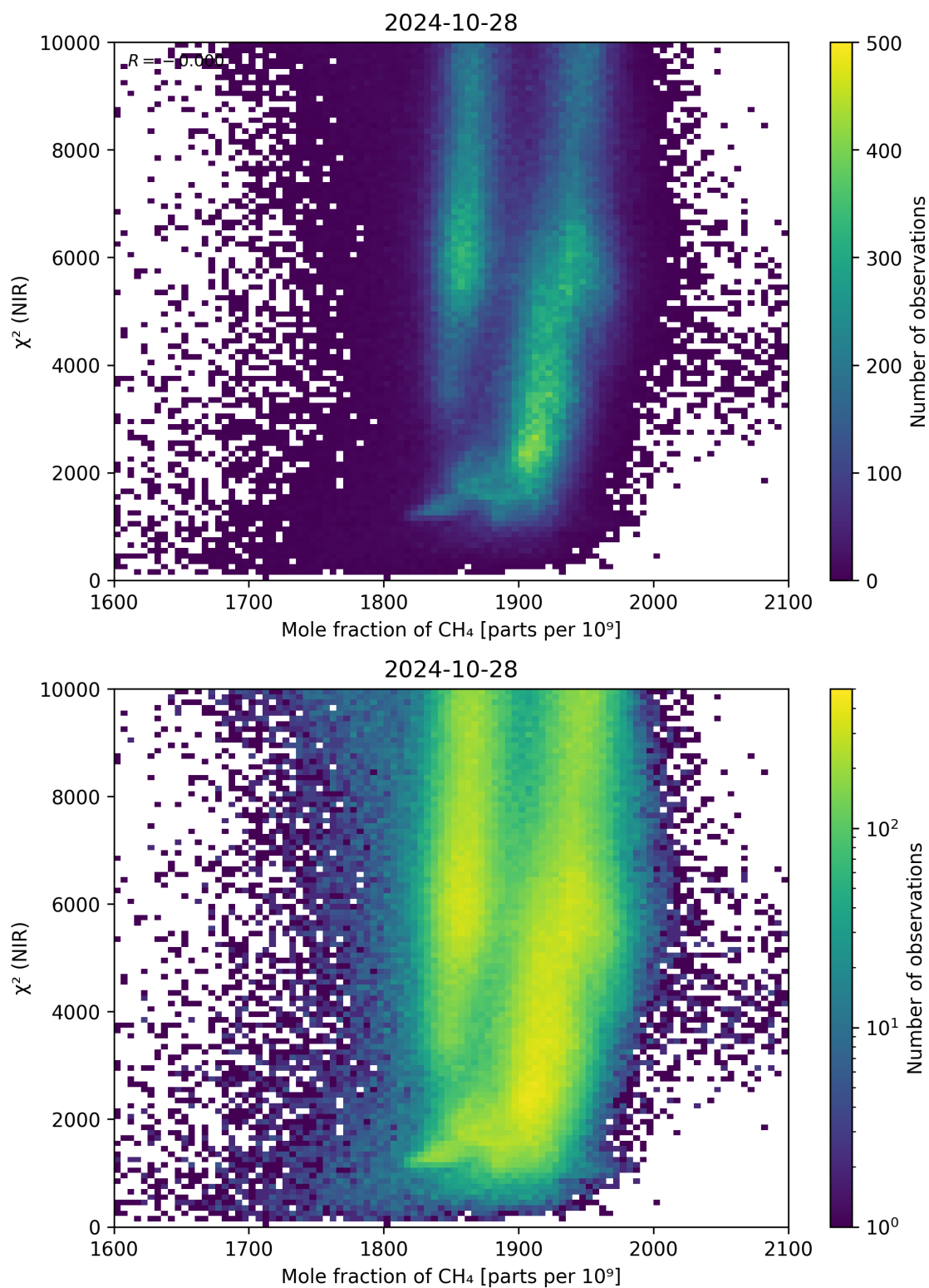
Figure 70: Scatter density plot of “Mole fraction of CH 4 ” against “ \chi^2 (NIR)” for 2024-10-27 to 2024-10-29.
