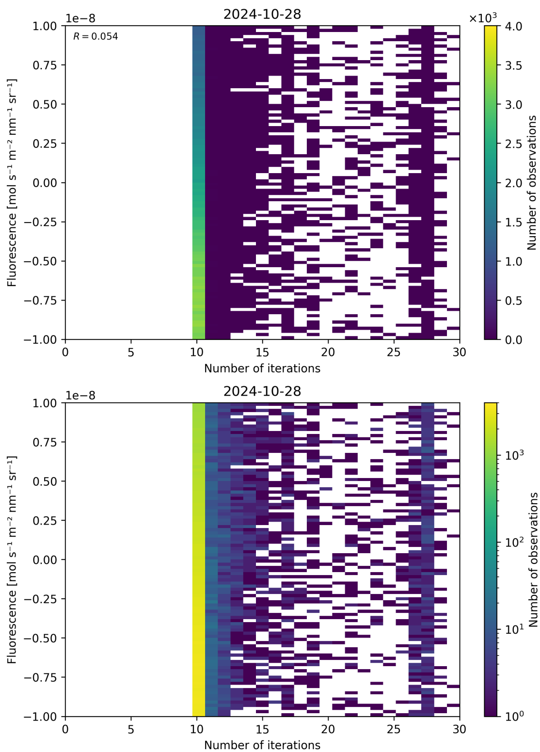
Figure 87: Scatter density plot of “Number of iterations” against “Fluorescence” for 2024-10-27 to 2024-10-29.
