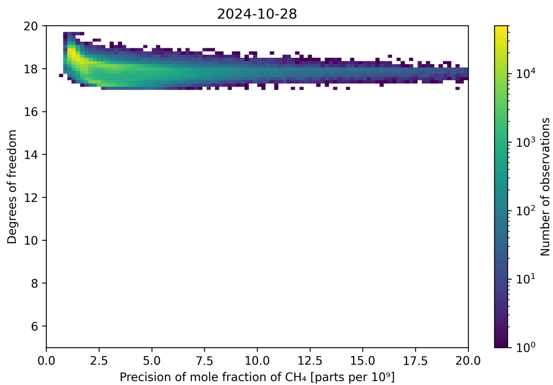
Figure 80: Scatter density plot of “Precision of mole fraction of \text{CH}_4 ” against “Degrees of freedom” for 2024-10-27 to 2024-10-29.
