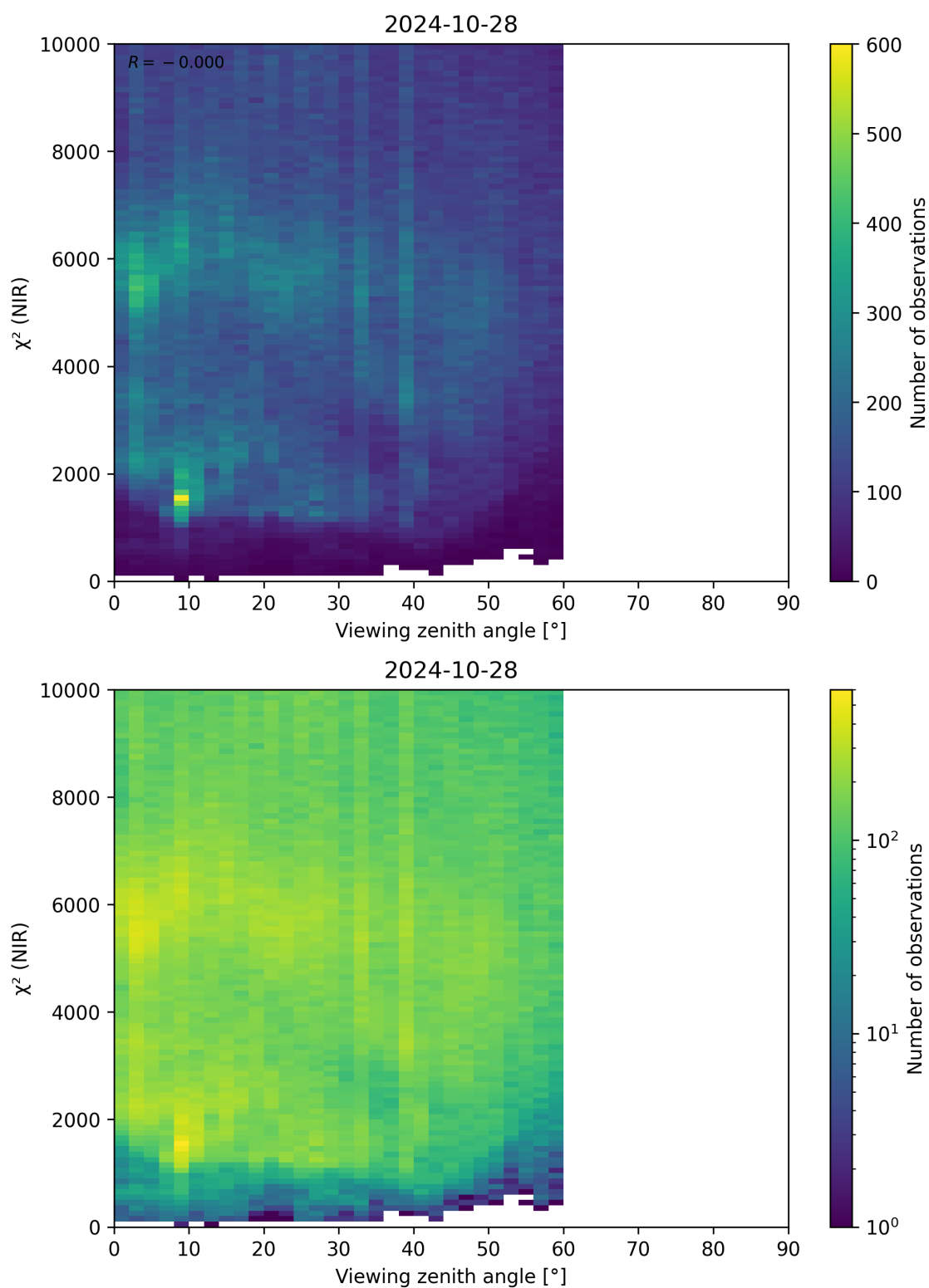
Figure 105: Scatter density plot of “Viewing zenith angle” against “ \chi^2 (NIR)” for 2024-10-27 to 2024-10-29.
