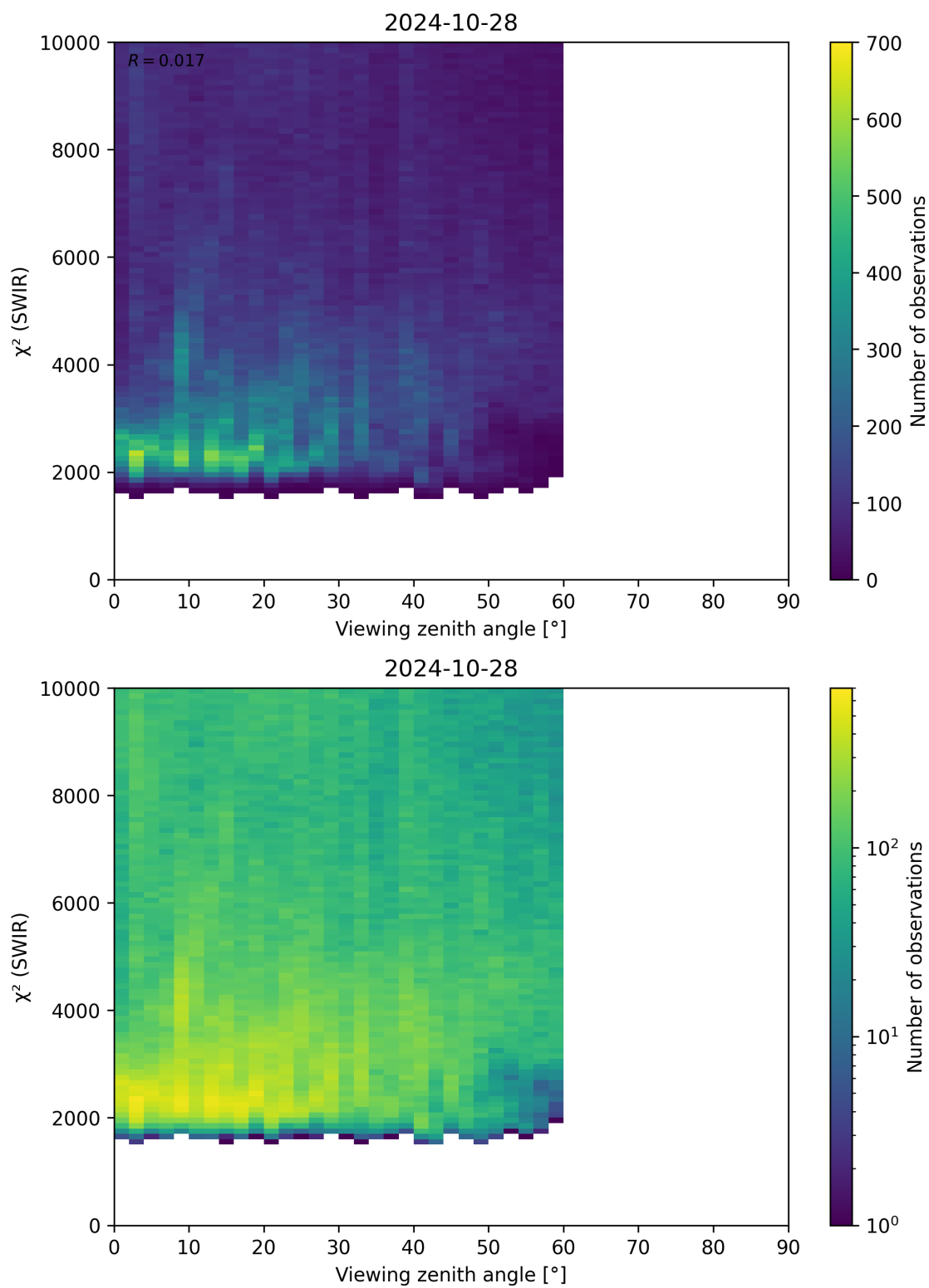
Figure 106: Scatter density plot of “Viewing zenith angle” against “ \chi^2 (SWIR)” for 2024-10-27 to 2024-10-29.
