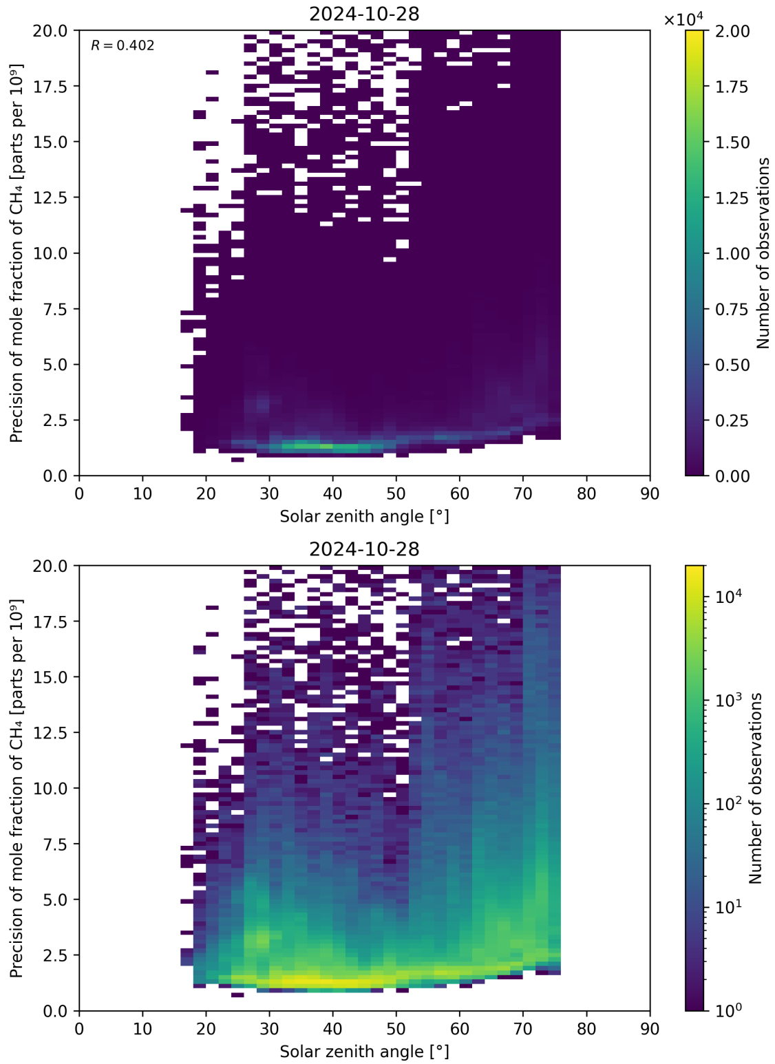
Figure 101: Scatter density plot of “Solar zenith angle” against “Precision of mole fraction of \text{CH}_4 ” for 2024-10-27 to 2024-10-29.
