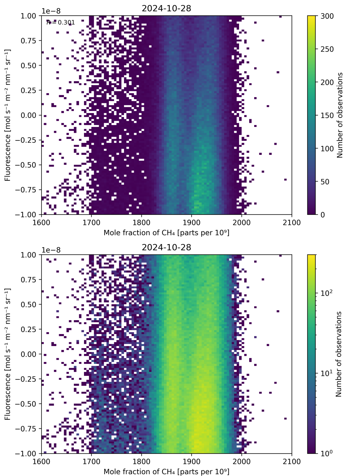
Figure 73: Scatter density plot of “Mole fraction of \text{CH}_4 ” against “Fluorescence” for 2024-10-27 to 2024-10-29.
