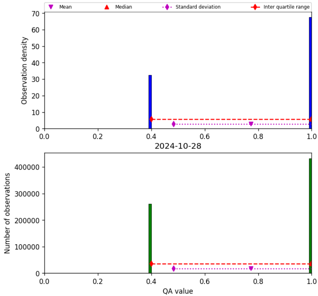
Figure 22: Histogram of “QA value” for 2024-10-27 to 2024-10-29
