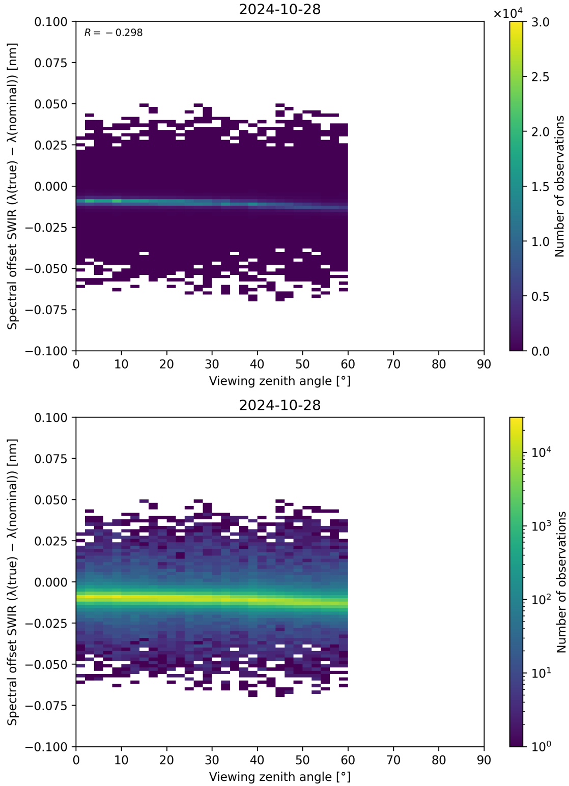
Figure 116: Scatter density plot of “Viewing zenith angle” against “Spectral offset SWIR ( \lambda_{\text{true}} - \lambda_{\text{nominal}} )” for 2024-10-27 to 2024-10-29.
