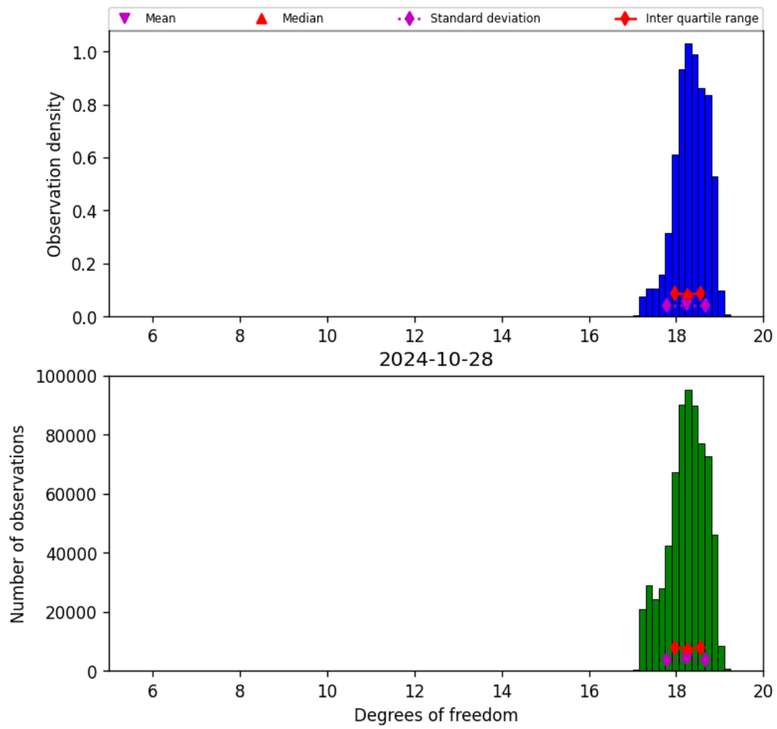
Figure 30: Histogram of “Degrees of freedom” for 2024-10-27 to 2024-10-29
