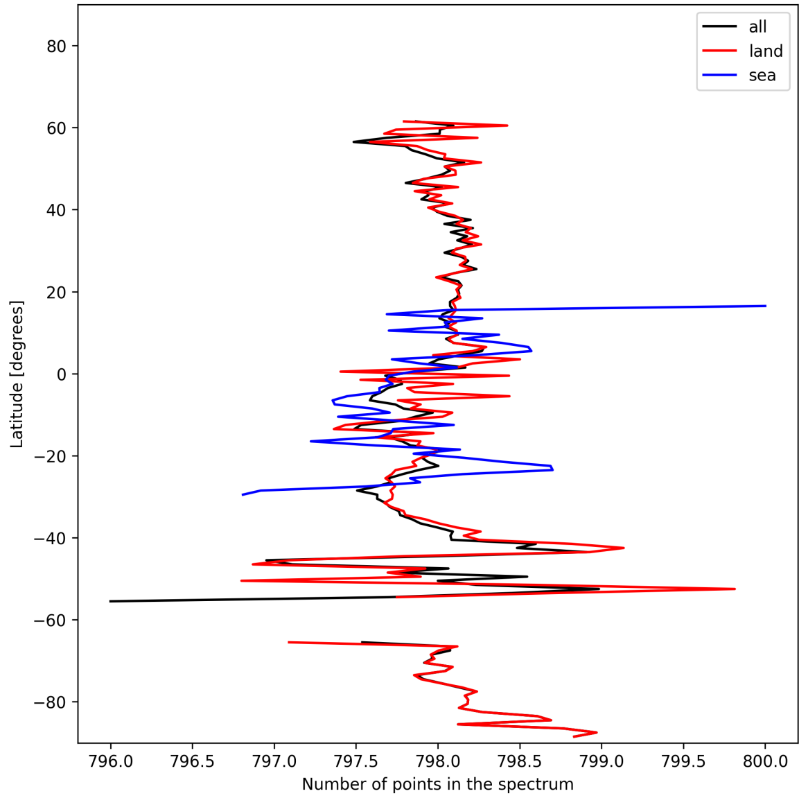
Figure 15: Zonal average of “Number of points in the spectrum” for 2024-10-27 to 2024-10-29.
