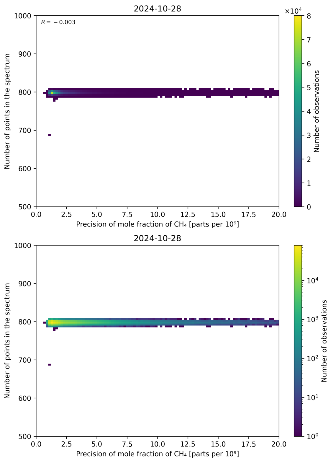
Figure 84: Scatter density plot of “Precision of mole fraction of CH 4 ” against “Number of points in the spectrum” for 2024-10-27 to 2024-10-29.
