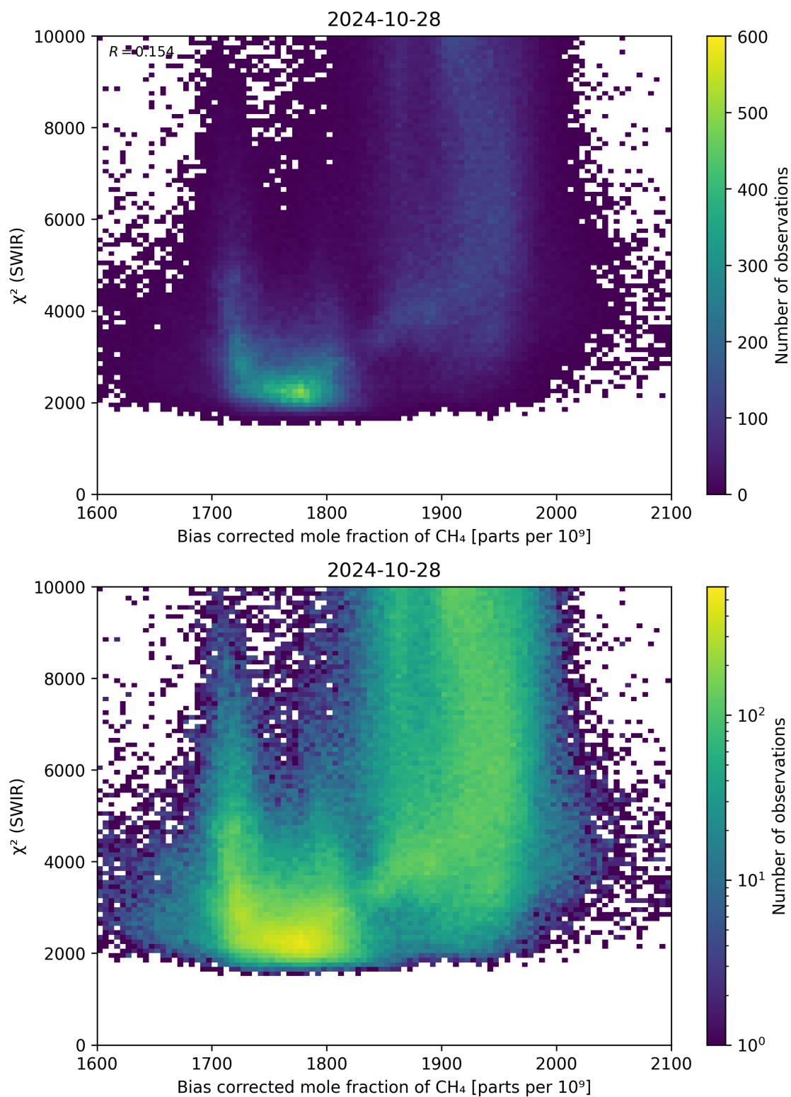
Figure 64: Scatter density plot of “Bias corrected mole fraction of \text{CH}_4 ” against “ \chi^2 (SWIR)” for 2024-10-27 to 2024-10-29.
