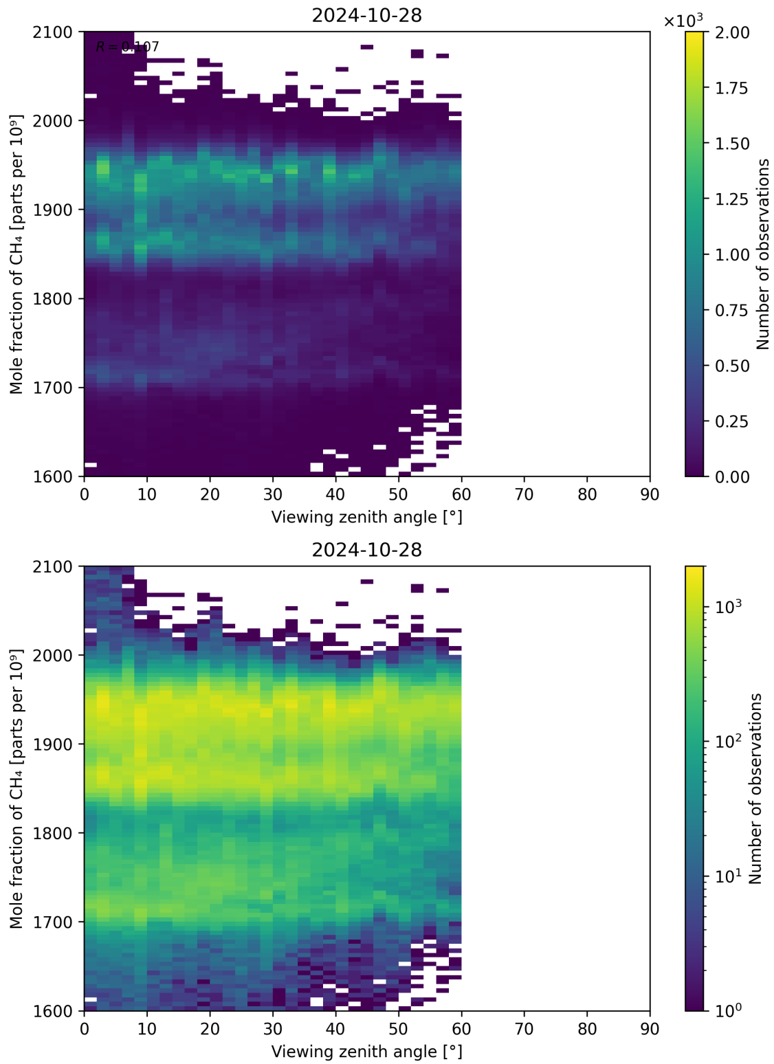
Figure 110: Scatter density plot of “Viewing zenith angle” against “Mole fraction of CH 4 ” for 2024-10-27 to 2024-10-29.
