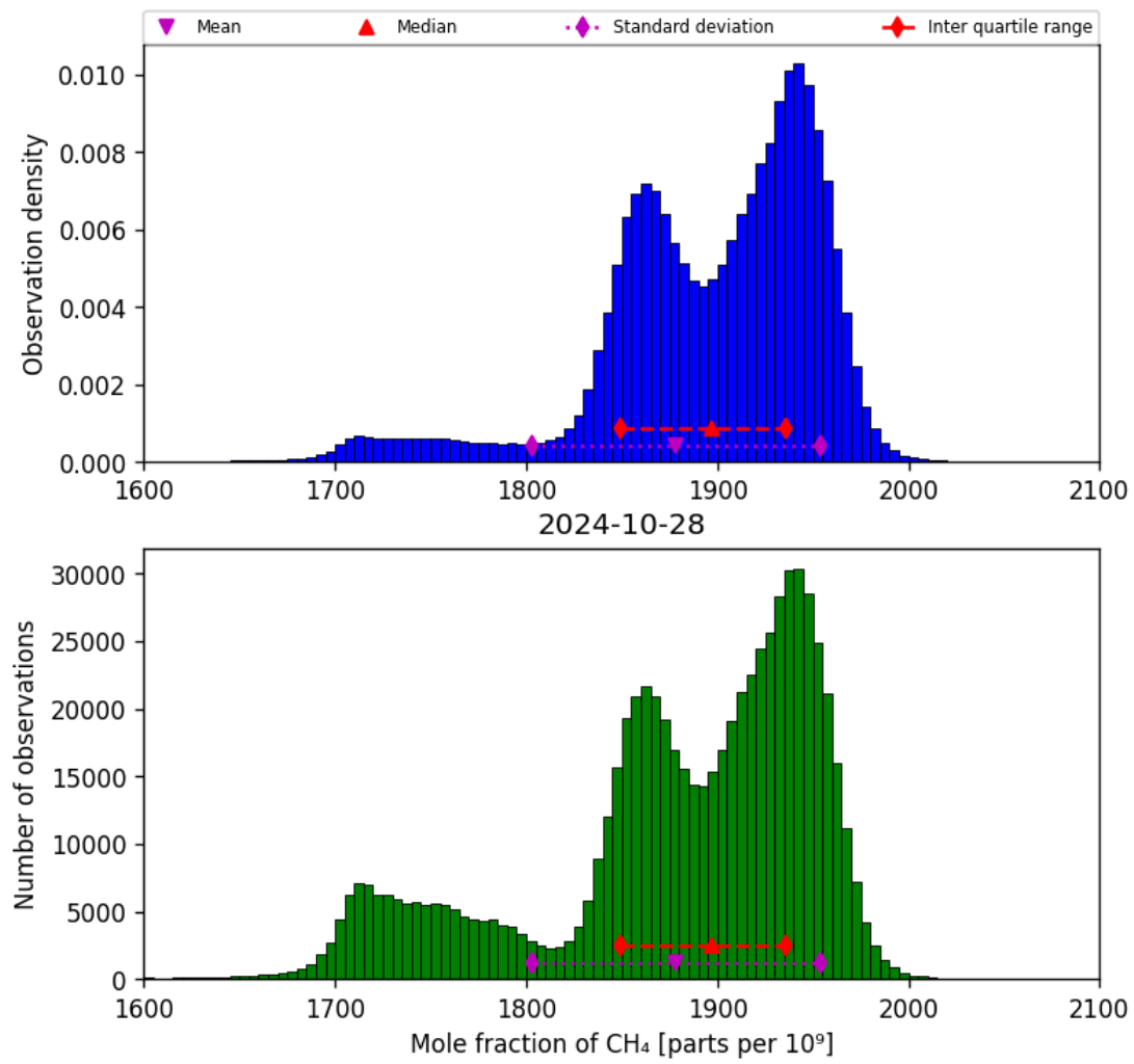
Figure 23: Histogram of “Mole fraction of CH 4 ” for 2024-10-27 to 2024-10-29
