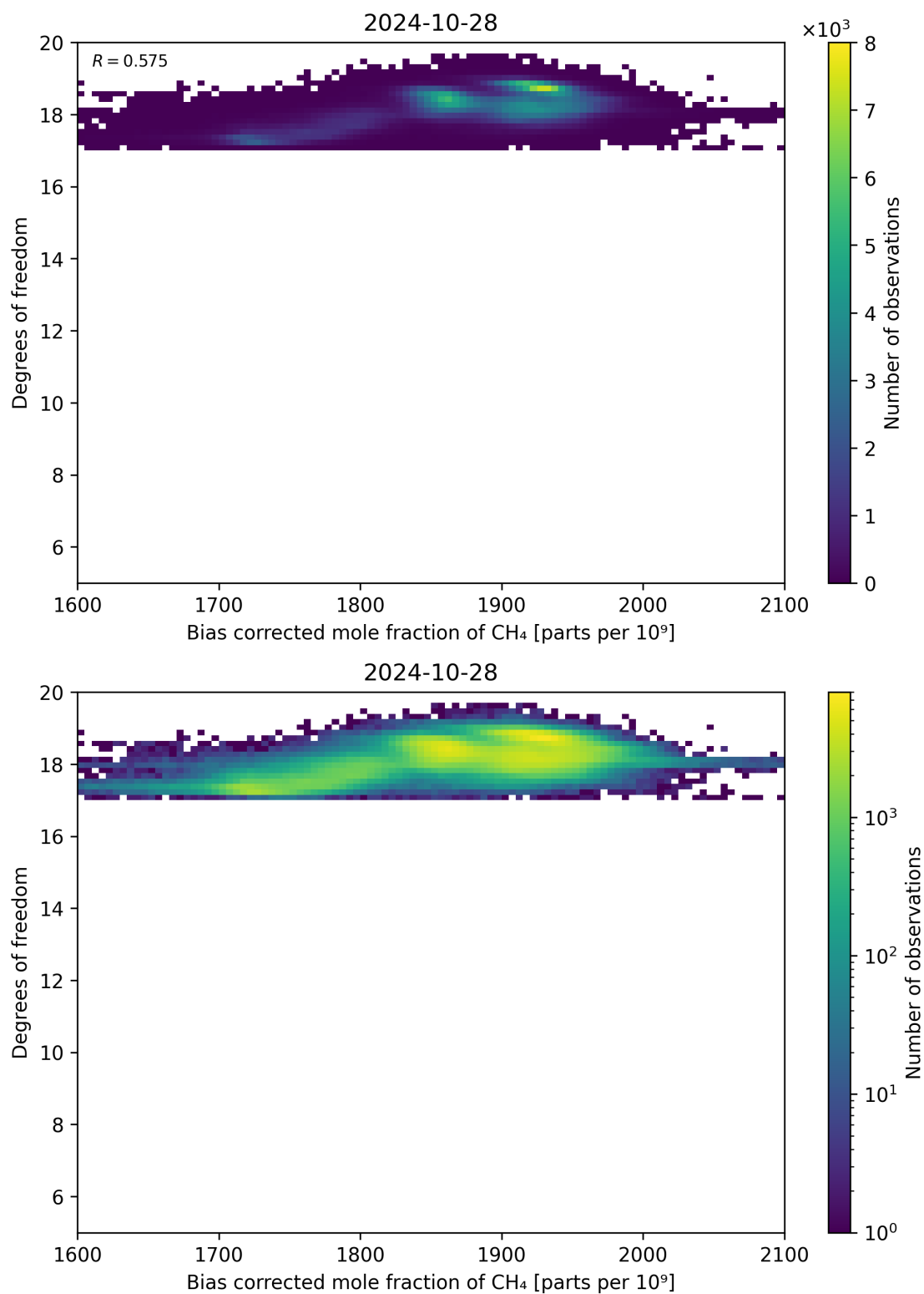
Figure 65: Scatter density plot of “Bias corrected mole fraction of CH 4 ” against “Degrees of freedom” for 2024-10-27 to 2024-10-29.
