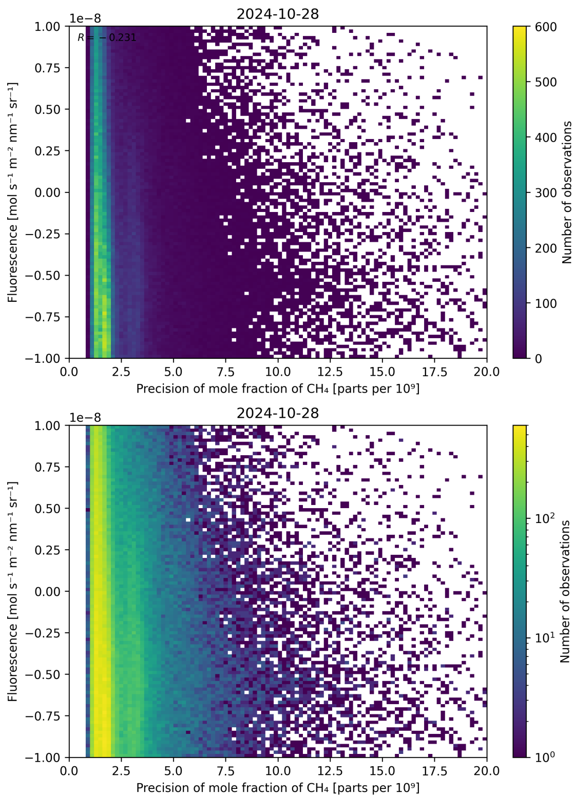
Figure 81: Scatter density plot of “Precision of mole fraction of \text{CH}_4 ” against “Fluorescence” for 2024-10-27 to 2024-10-29.
