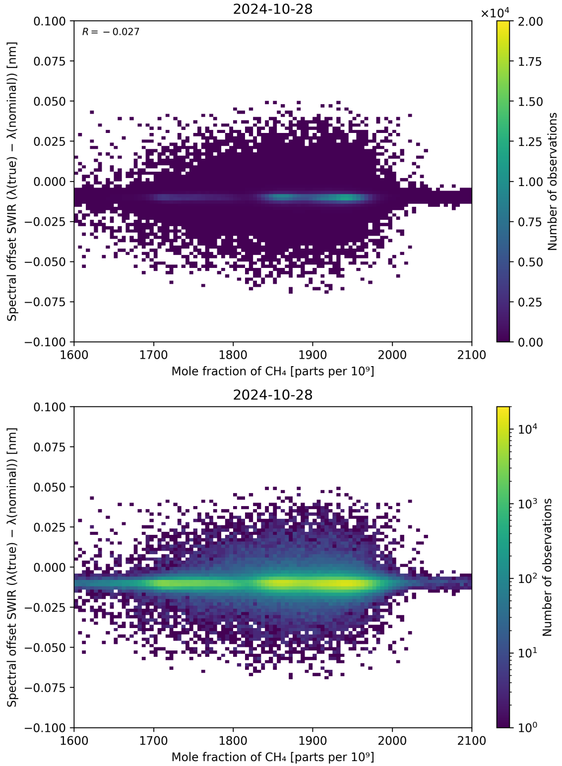
Figure 86: Scatter density plot of “Mole fraction of CH 4 ” against “Spectral offset SWIR ( \lambda_{\text{true}} - \lambda_{\text{nominal}} )” for 2024-10-27 to 2024-10-29.
