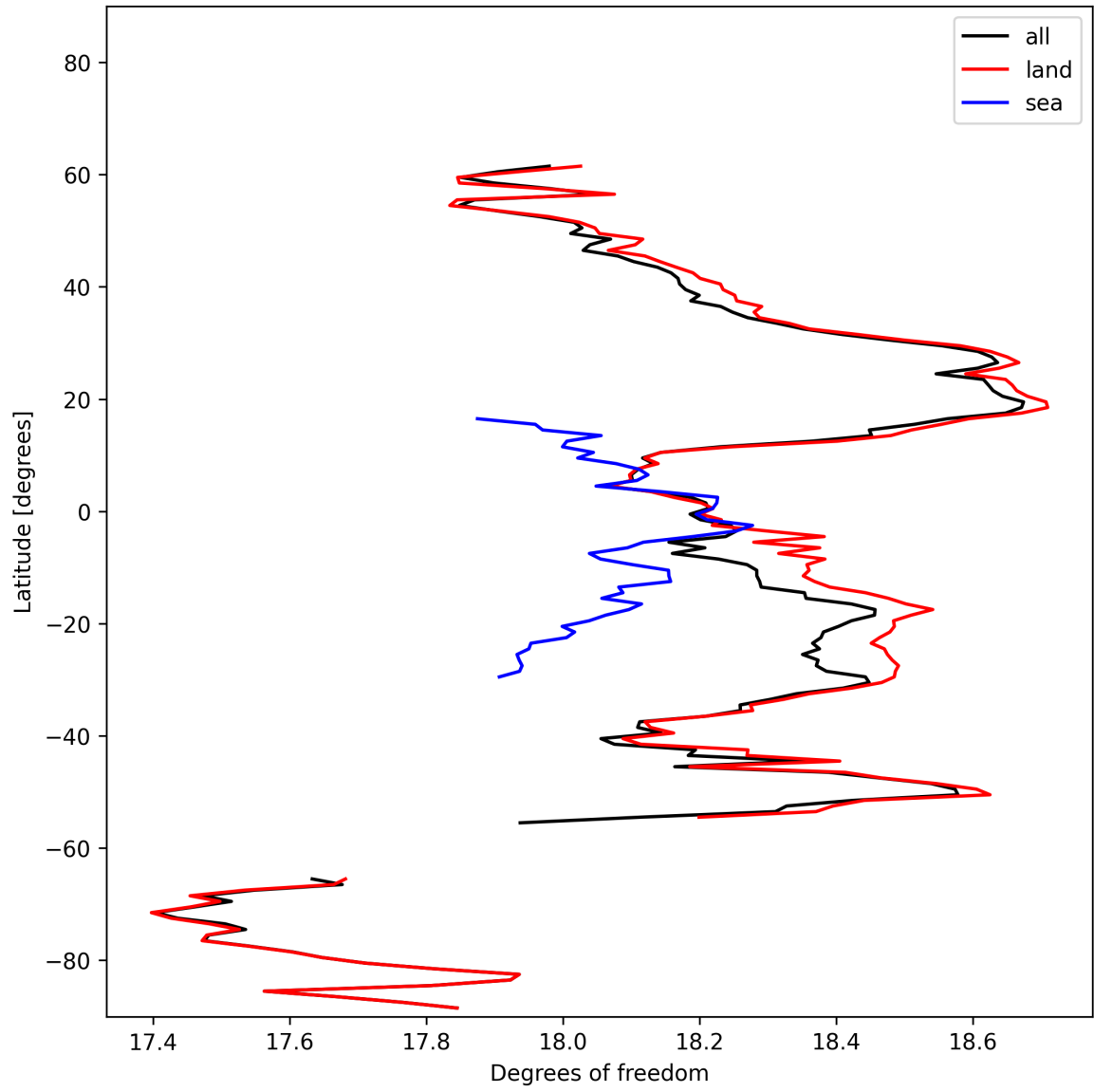
Figure 19: Zonal average of “Degrees of freedom” for 2024-10-27 to 2024-10-29.
