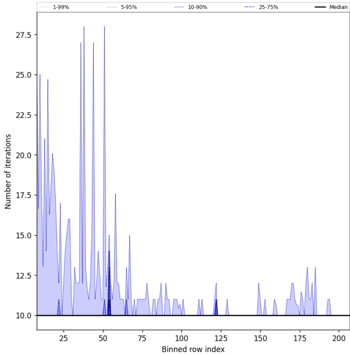
Figure 42: Along track statistics of “Number of iterations” for 2024-10-27 to 2024-10-29
