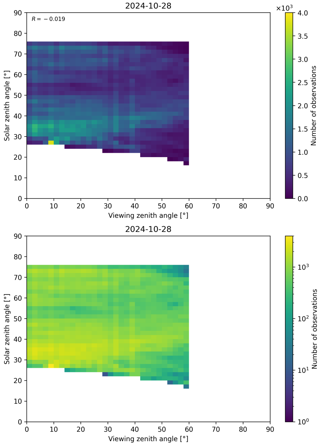
Figure 115: Scatter density plot of “Viewing zenith angle” against “Solar zenith angle” for 2024-10-27 to 2024-10-29.
