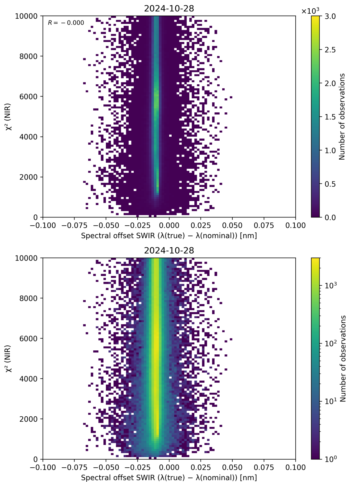
Figure 117: Scatter density plot of “Spectral offset SWIR ( \lambda_{\text{true}} - \lambda_{\text{nominal}} )” against “ \chi^2 (NIR)” for 2024-10-27 to 2024-10-29.
