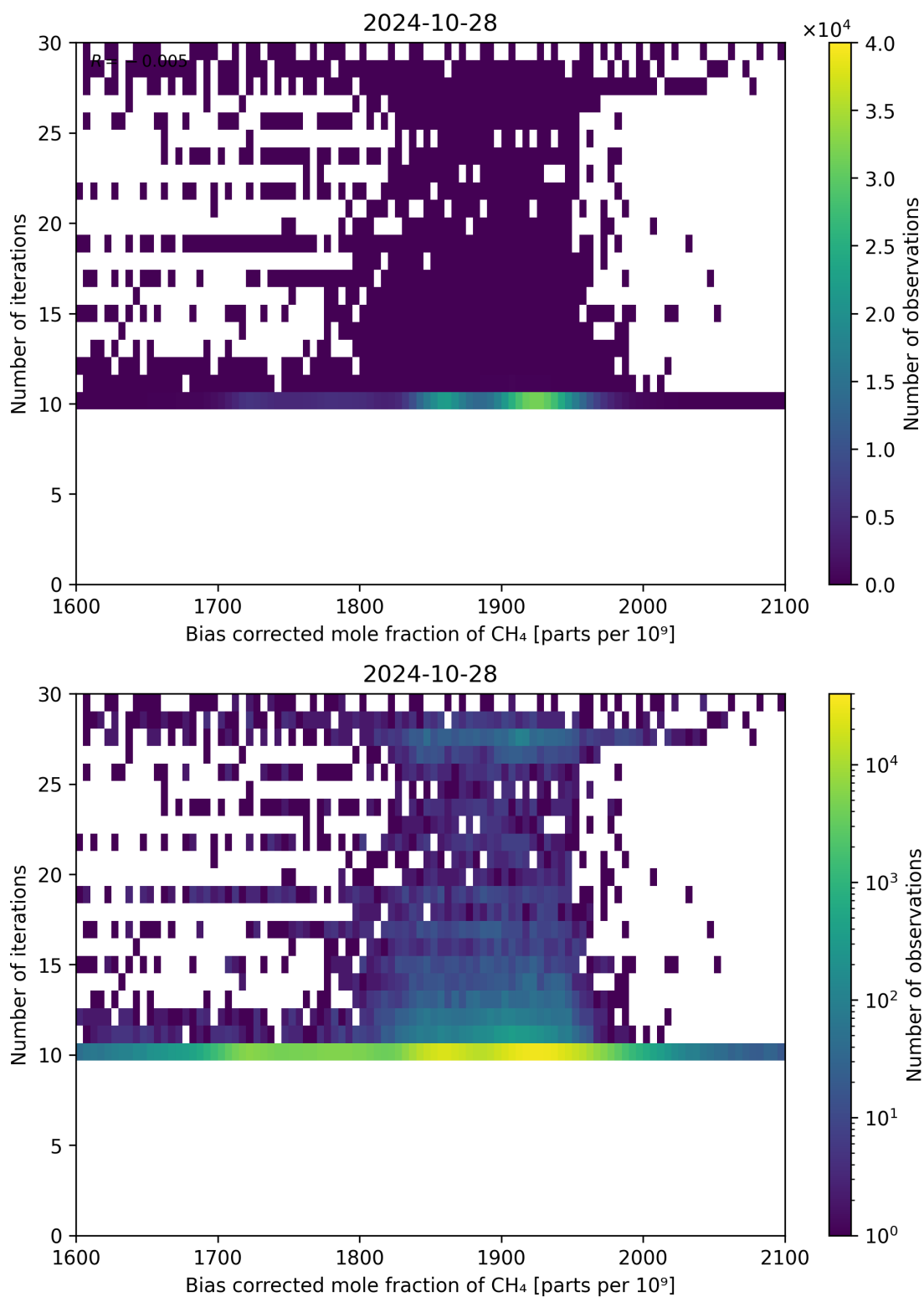
Figure 67: Scatter density plot of “Bias corrected mole fraction of \text{CH}_4 ” against “Number of iterations” for 2024-10-27 to 2024-10-29.
