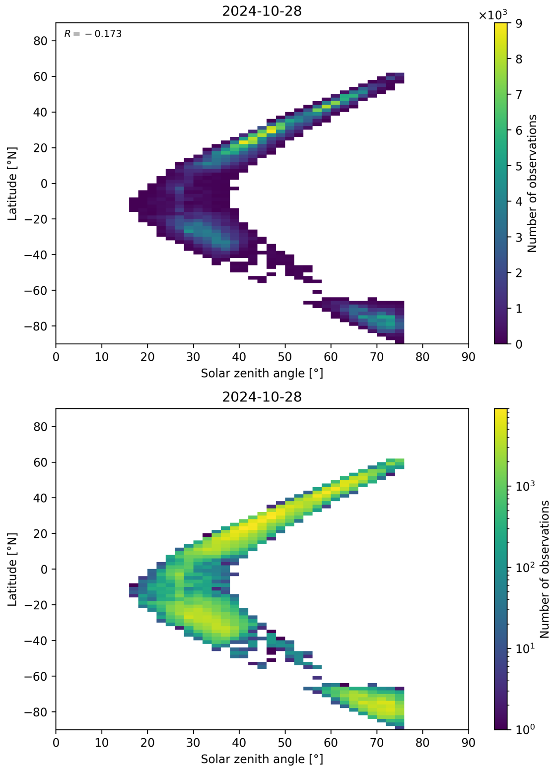
Figure 98: Scatter density plot of “Solar zenith angle” against “Latitude” for 2024-10-27 to 2024-10-29.
