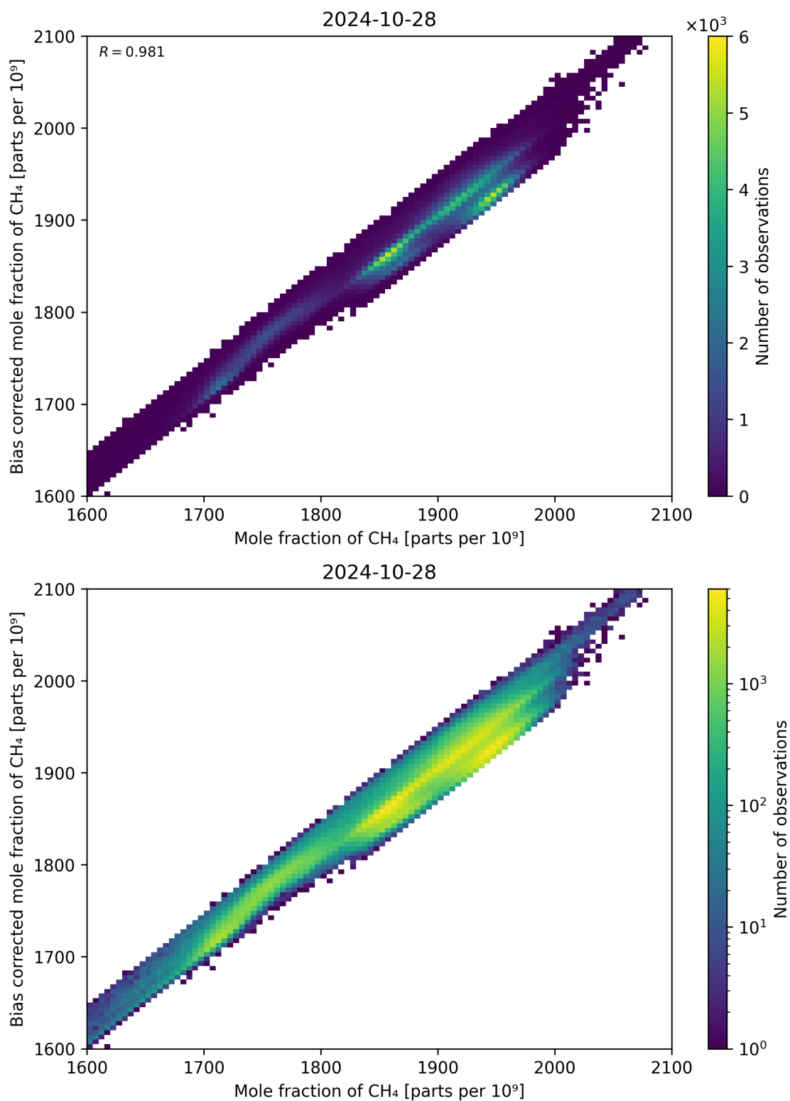
Figure 74: Scatter density plot of “Mole fraction of CH 4 ” against “Bias corrected mole fraction of CH 4 ” for 2024-10-27 to 2024-10-29.
