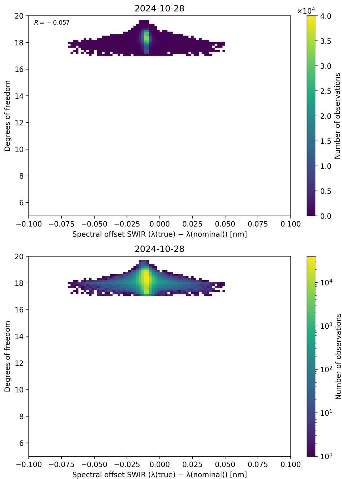
Figure 119: Scatter density plot of “Spectral offset SWIR ( \lambda_{\text{true}} - \lambda_{\text{nominal}} )” against “Degrees of freedom” for 2024-10-27 to 2024-10-29.
