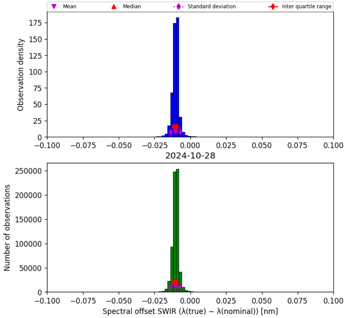
Figure 27: Histogram of “Spectral offset SWIR ( \lambda_{\text{true}} - \lambda_{\text{nominal}} )” for 2024-10-27 to 2024-10-29
