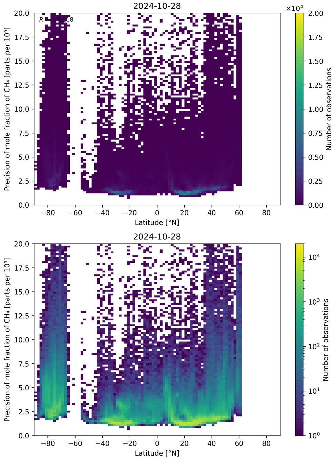
Figure 59: Scatter density plot of “Latitude” against “Precision of mole fraction of CH 4 ” for 2024-10-27 to 2024-10-29.
