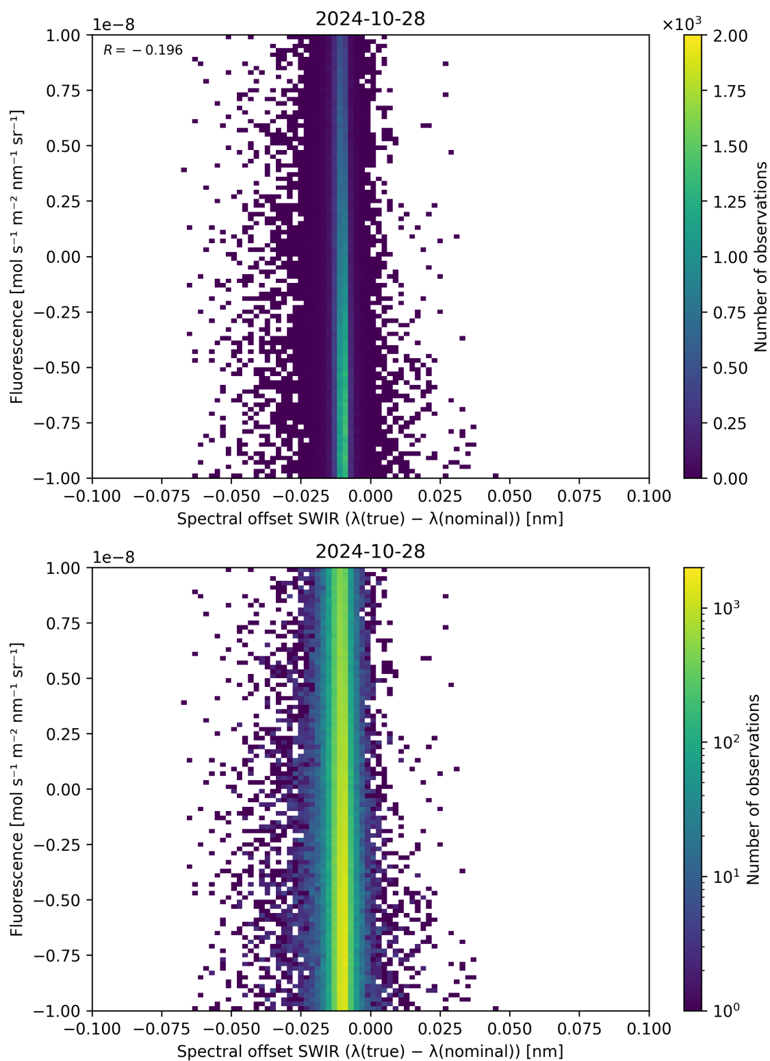
Figure 120: Scatter density plot of “Spectral offset SWIR ( \lambda_{\text{true}} - \lambda_{\text{nominal}} )” against “Fluorescence” for 2024-10-27 to 2024-10-29.
