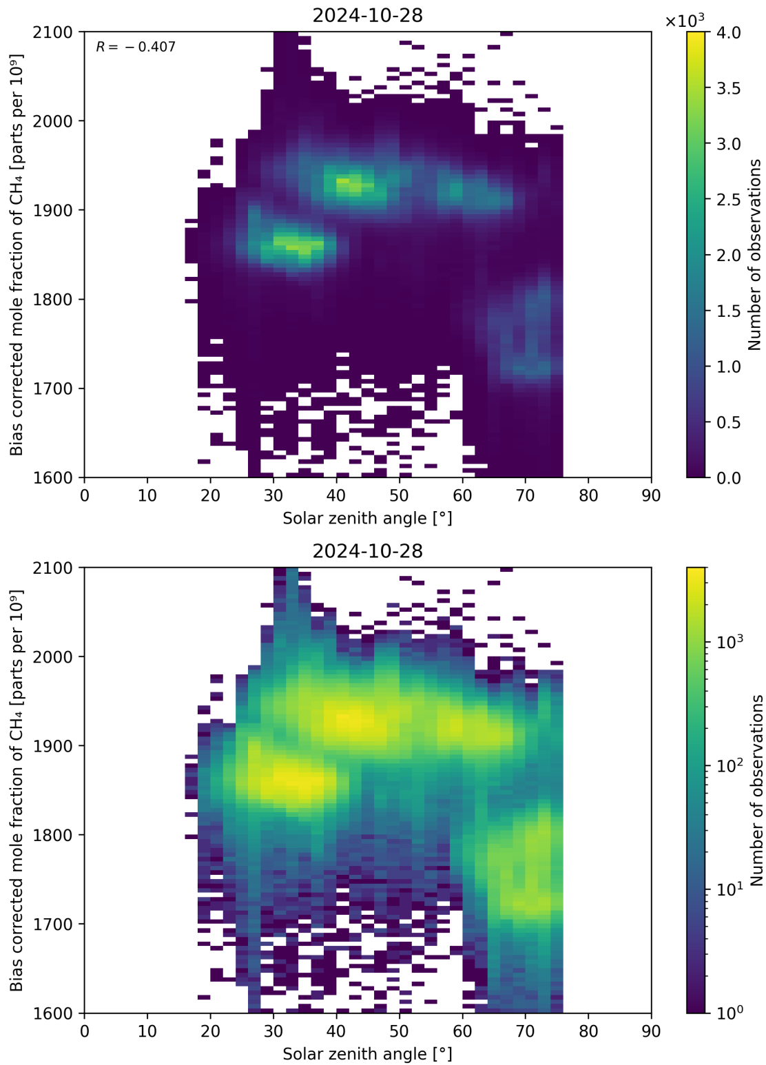
Figure 100: Scatter density plot of “Solar zenith angle” against “Bias corrected mole fraction of CH 4 ” for 2024-10-27 to 2024-10-29.
