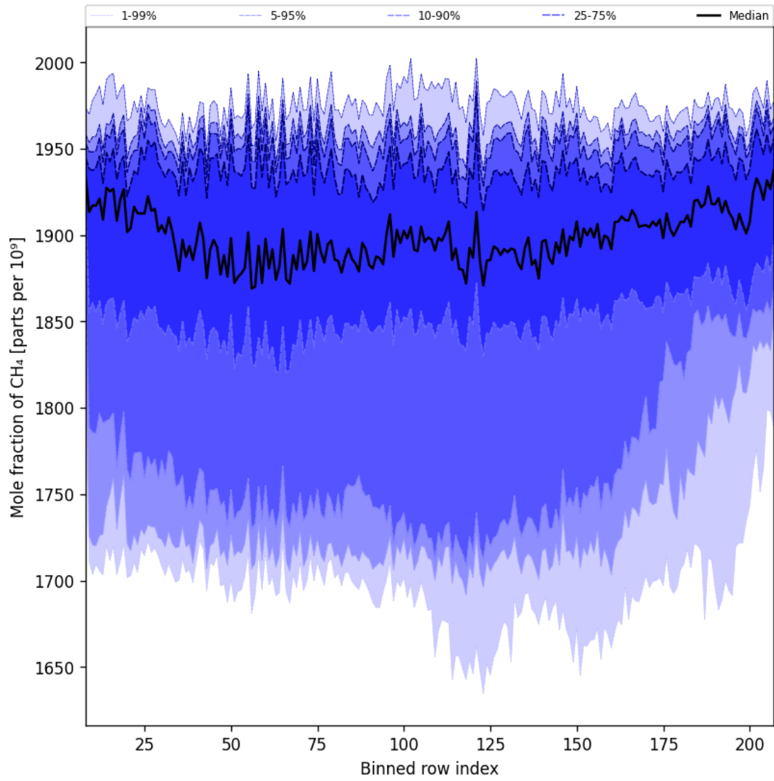
Figure 34: Along track statistics of “Mole fraction of CH 4 ” for 2024-10-27 to 2024-10-29
