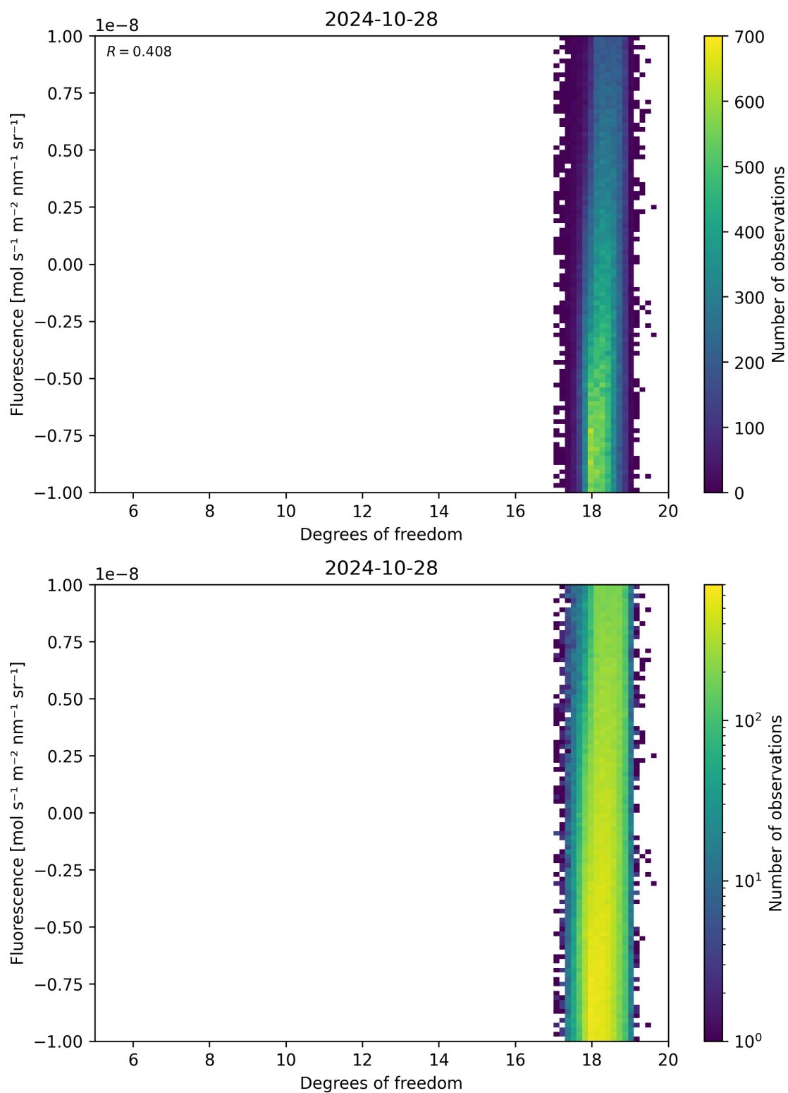
Figure 51: Scatter density plot of “Degrees of freedom” against “Fluorescence” for 2024-10-27 to 2024-10-29.
