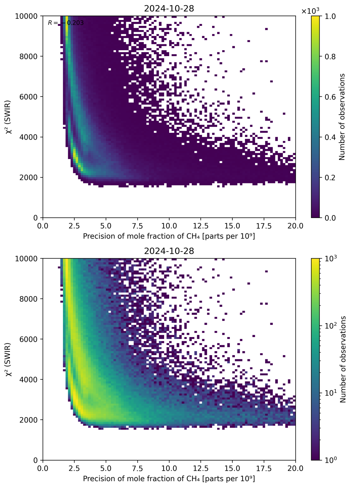
Figure 79: Scatter density plot of “Precision of mole fraction of \text{CH}_4 ” against “ \chi^2 (SWIR)” for 2024-10-27 to 2024-10-29.
