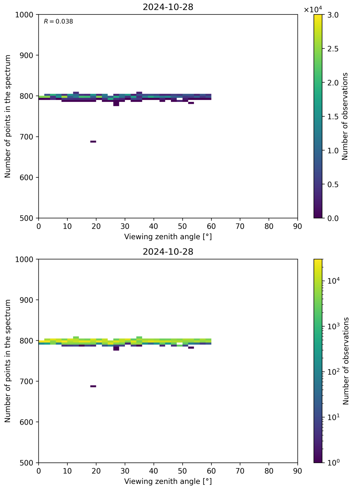
Figure 114: Scatter density plot of “Viewing zenith angle” against “Number of points in the spectrum” for 2024-10-27 to 2024-10-29.
