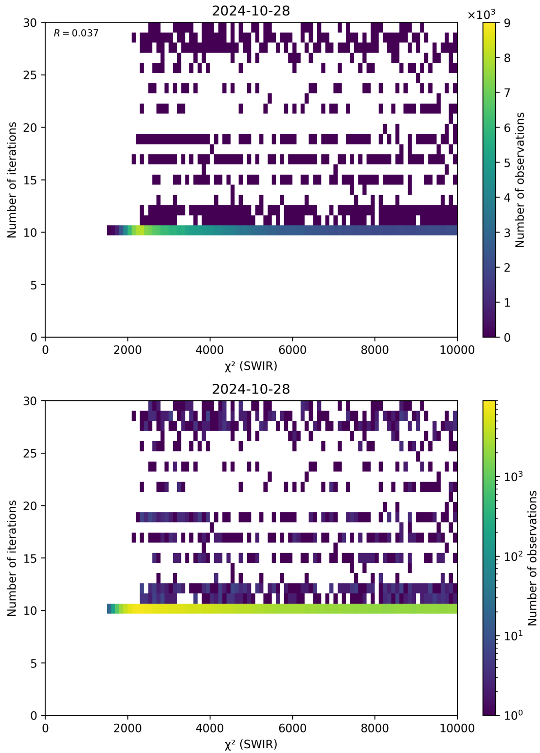
Figure 50: Scatter density plot of “ \chi^2 (SWIR)” against “Number of iterations” for 2024-10-27 to 2024-10-29.
