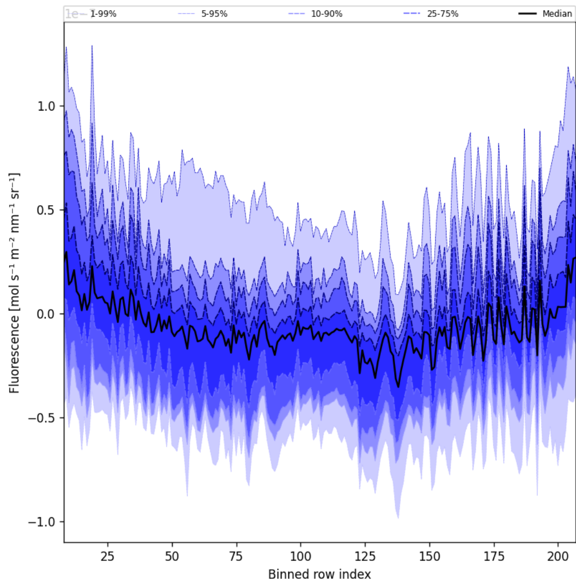
Figure 43: Along track statistics of “Fluorescence” for 2024-10-27 to 2024-10-29
