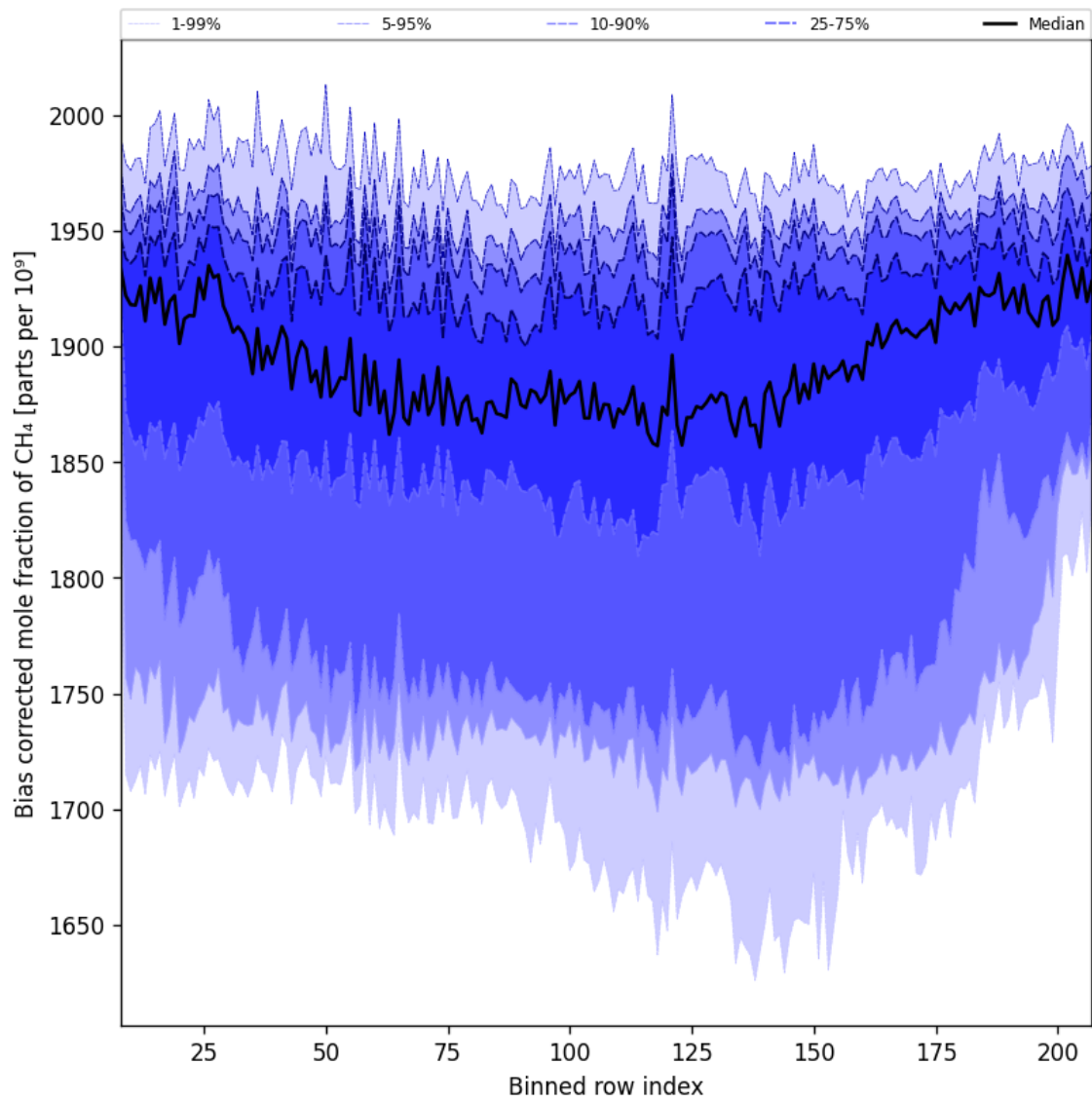
Figure 36: Along track statistics of “Bias corrected mole fraction of \text{CH}_4 ” for 2024-10-29 to 2024-10-30
