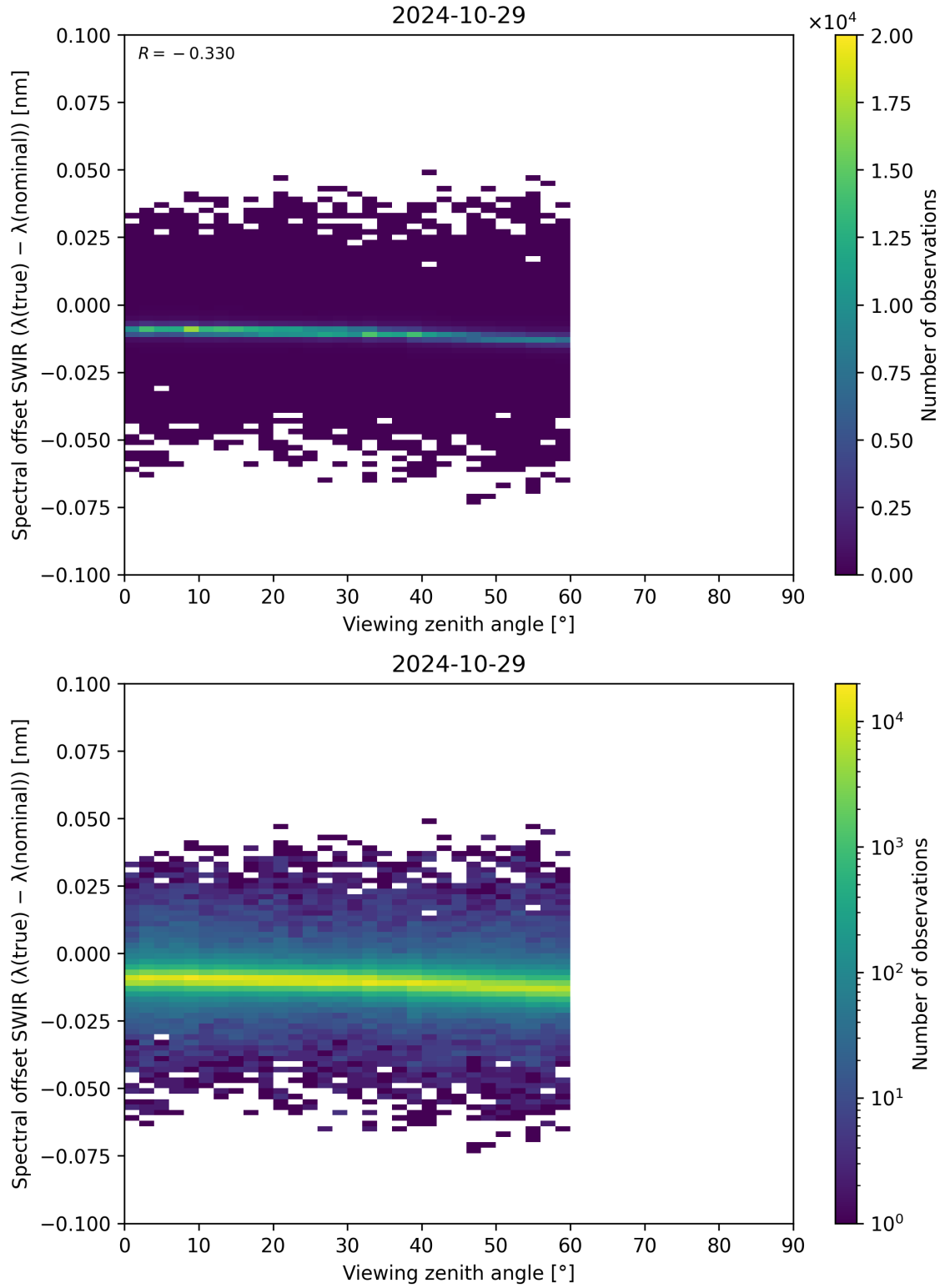
Figure 116: Scatter density plot of “Viewing zenith angle” against “Spectral offset SWIR ( \lambda_{\text{true}} - \lambda_{\text{nominal}} )” for 2024-10-29 to 2024-10-30.
