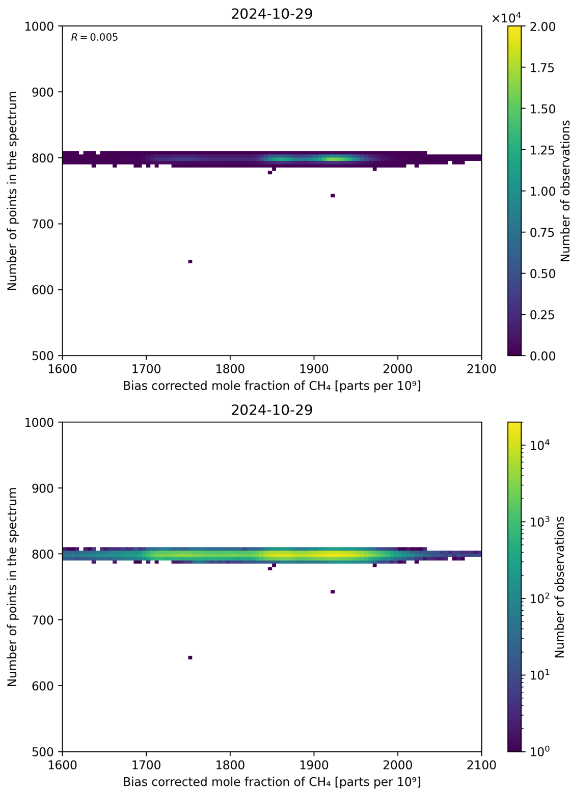
Figure 68: Scatter density plot of “Bias corrected mole fraction of CH 4 ” against “Number of points in the spectrum” for 2024-10-29 to 2024-10-30.
