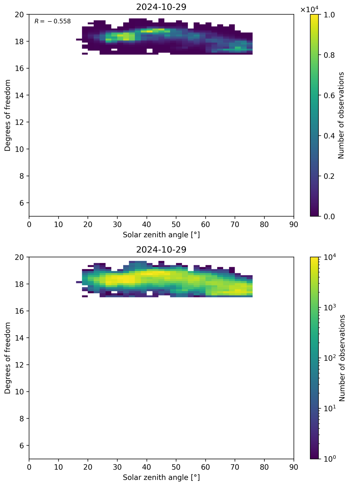
Figure 96: Scatter density plot of “Solar zenith angle” against “Degrees of freedom” for 2024-10-29 to 2024-10-30.
