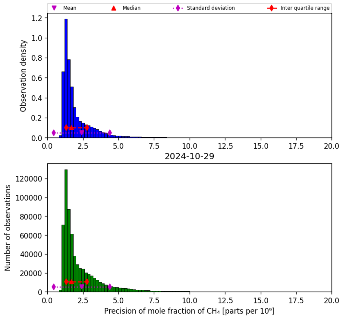
Figure 24: Histogram of “Precision of mole fraction of CH 4 ” for 2024-10-29 to 2024-10-30
