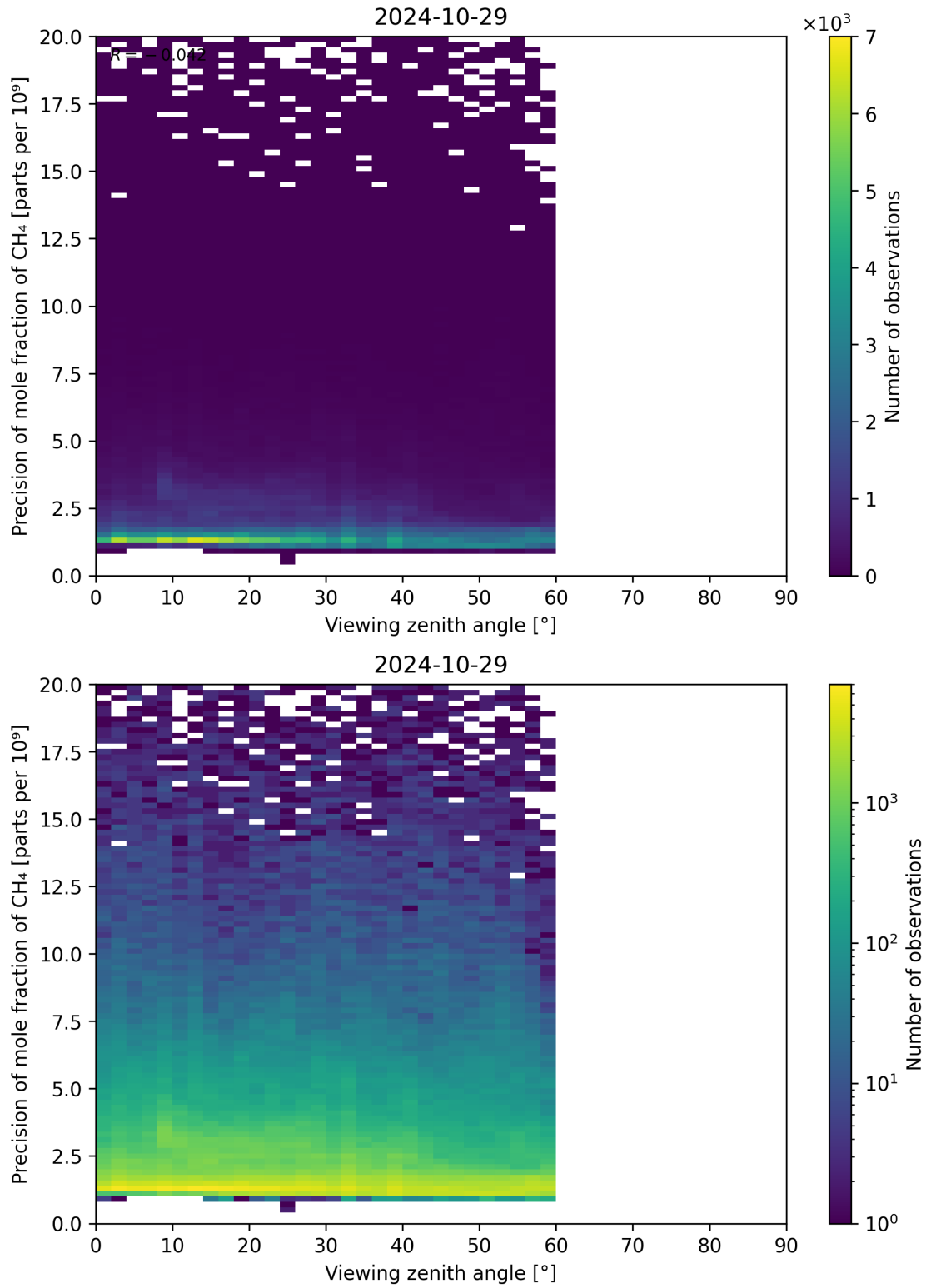
Figure 112: Scatter density plot of “Viewing zenith angle” against “Precision of mole fraction of CH 4 ” for 2024-10-29 to 2024-10-30.
