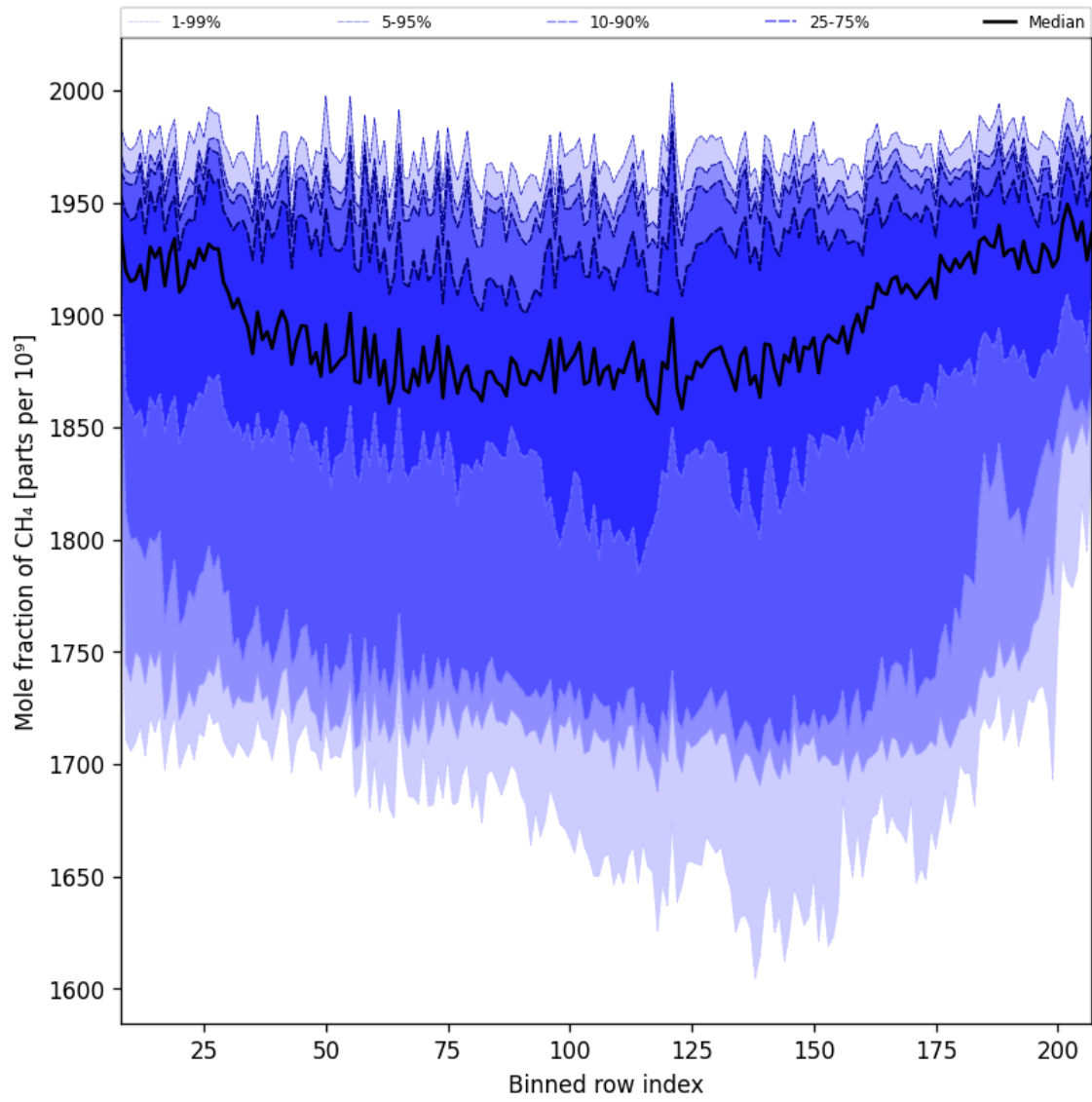
Figure 34: Along track statistics of “Mole fraction of CH 4 ” for 2024-10-29 to 2024-10-30
