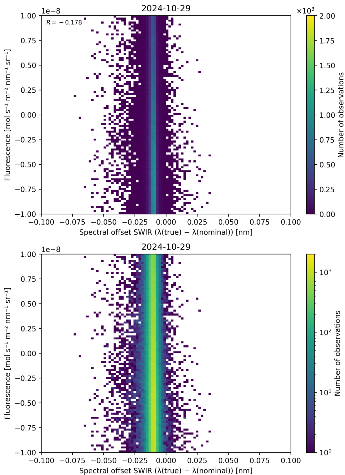
Figure 120: Scatter density plot of “Spectral offset SWIR ( \lambda_{\text{true}} - \lambda_{\text{nominal}} )” against “Fluorescence” for 2024-10-29 to 2024-10-30.
