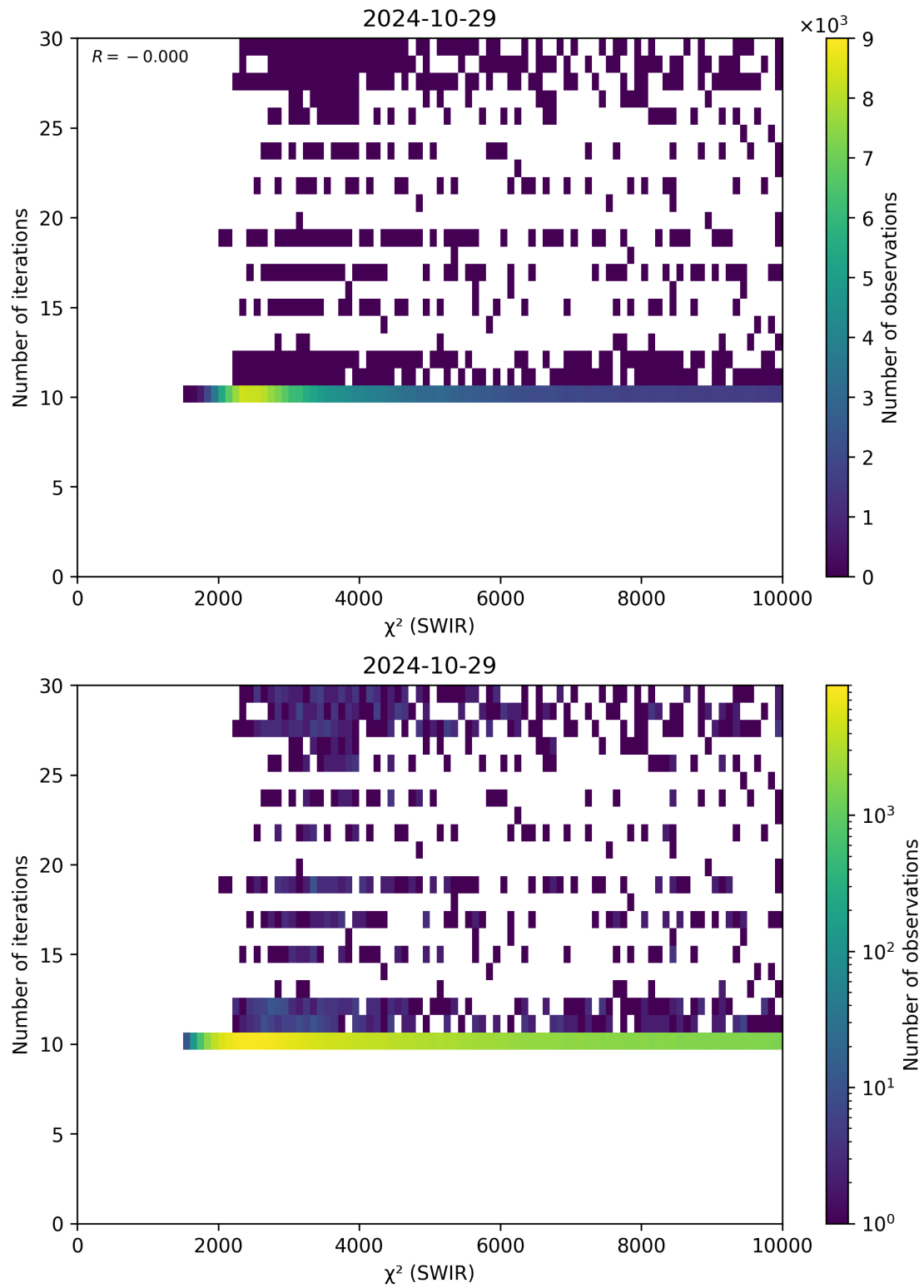
Figure 50: Scatter density plot of “ \chi^2 (SWIR)” against “Number of iterations” for 2024-10-29 to 2024-10-30.
