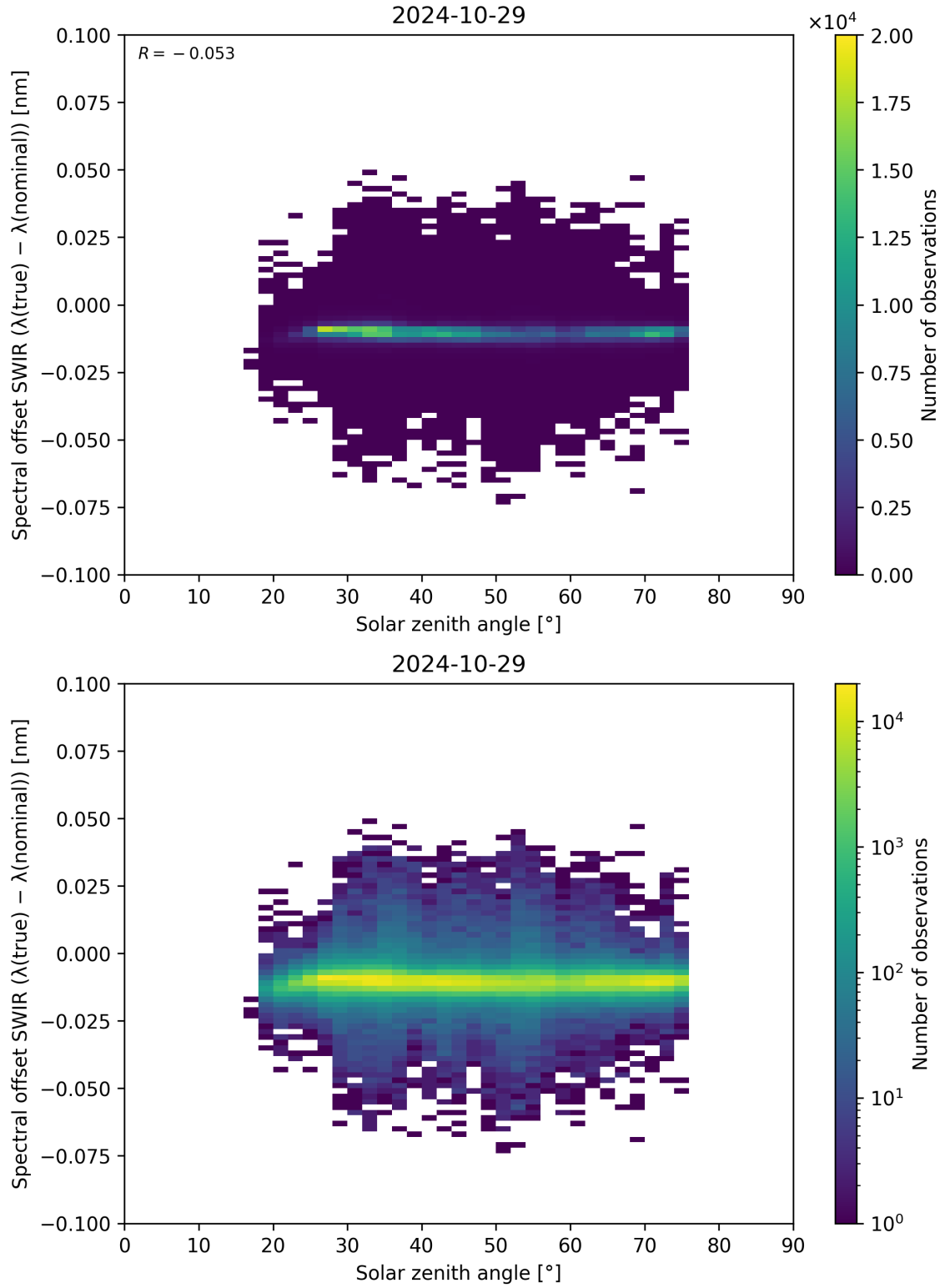
Figure 104: Scatter density plot of “Solar zenith angle” against “Spectral offset SWIR ( \lambda_{\text{true}} - \lambda_{\text{nominal}} )” for 2024-10-29 to 2024-10-30.
