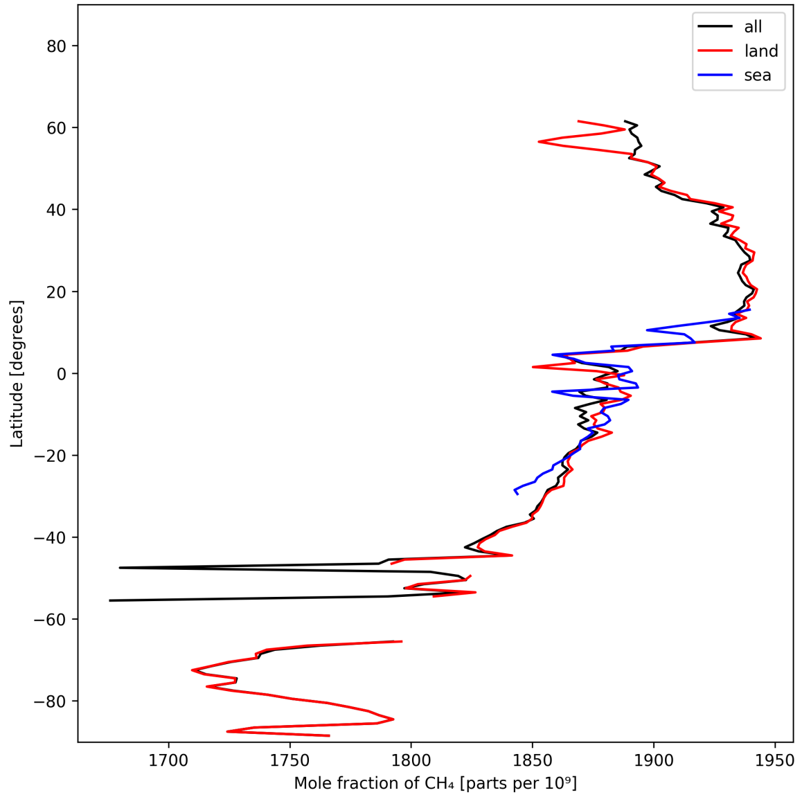
Figure 12: Zonal average of “Mole fraction of CH 4 ” for 2024-10-29 to 2024-10-30.
