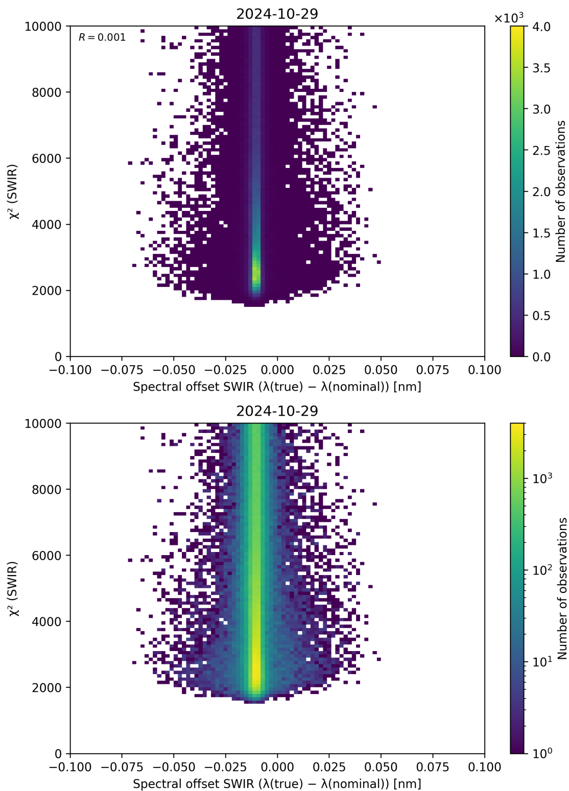
Figure 118: Scatter density plot of “Spectral offset SWIR ( \lambda_{\text{true}} - \lambda_{\text{nominal}} )” against “ \chi^2 (SWIR)” for 2024-10-29 to 2024-10-30.
