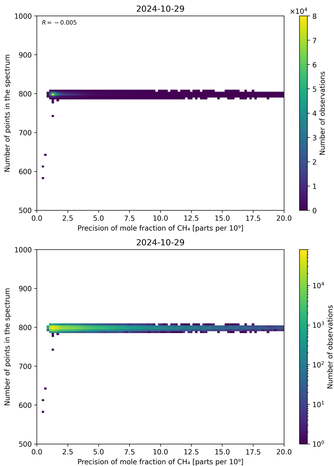
Figure 84: Scatter density plot of “Precision of mole fraction of CH 4 ” against “Number of points in the spectrum” for 2024-10-29 to 2024-10-30.
