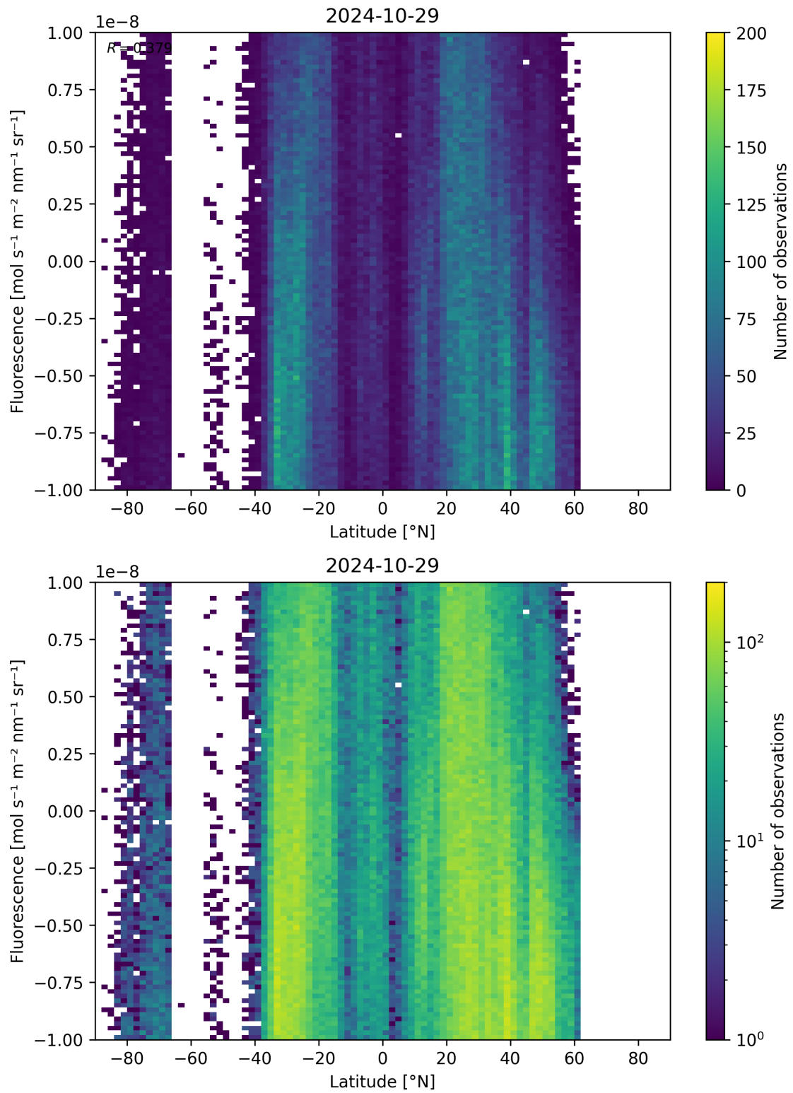
Figure 56: Scatter density plot of “Latitude” against “Fluorescence” for 2024-10-29 to 2024-10-30.
