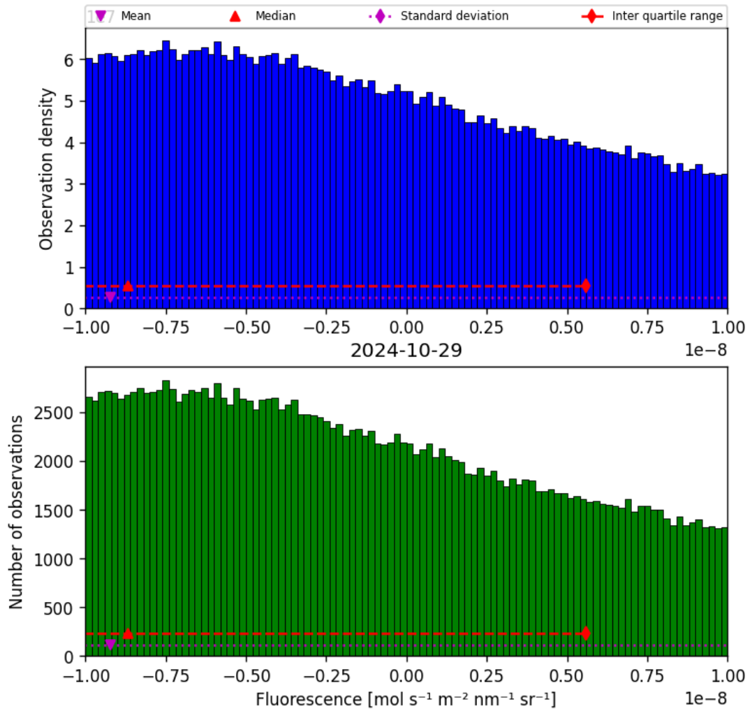
Figure 32: Histogram of “Fluorescence” for 2024-10-29 to 2024-10-30
