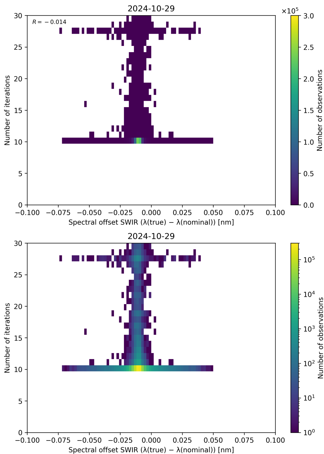
Figure 121: Scatter density plot of “Spectral offset SWIR ( \lambda_{\text{true}} - \lambda_{\text{nominal}} )” against “Number of iterations” for 2024-10-29 to 2024-10-30.
