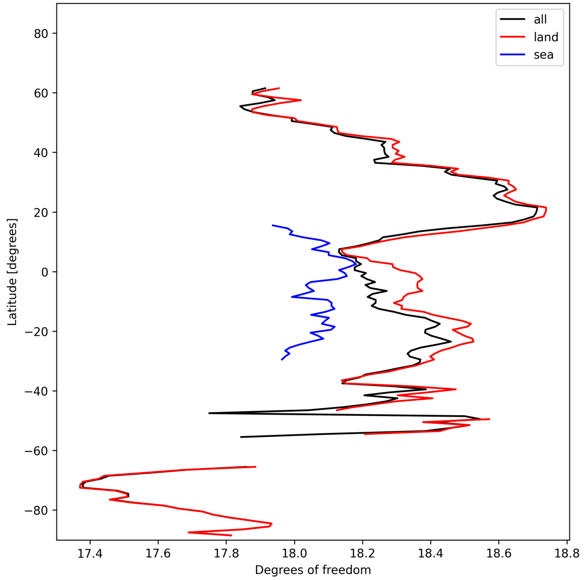
Figure 19: Zonal average of “Degrees of freedom” for 2024-10-29 to 2024-10-30.
