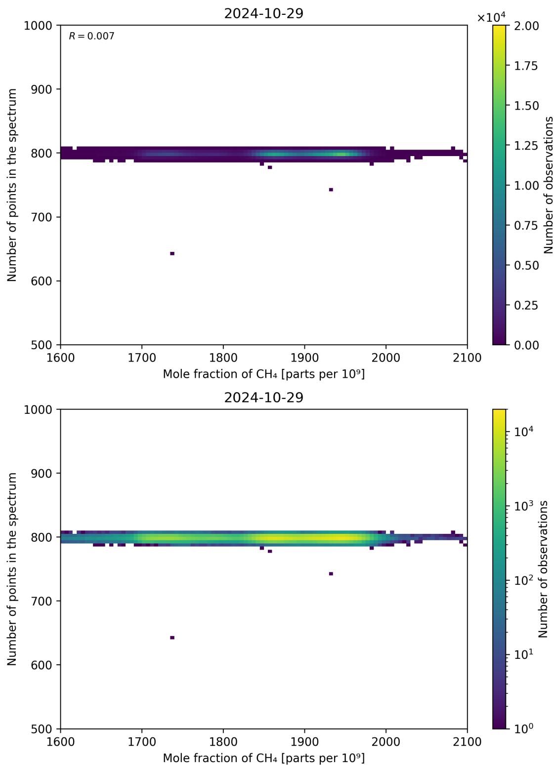
Figure 77: Scatter density plot of “Mole fraction of CH 4 ” against “Number of points in the spectrum” for 2024-10-29 to 2024-10-30.
