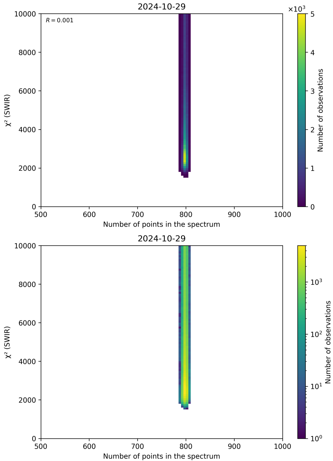
Figure 89: Scatter density plot of “Number of points in the spectrum” against “ \chi^2 (SWIR)” for 2024-10-29 to 2024-10-30.
