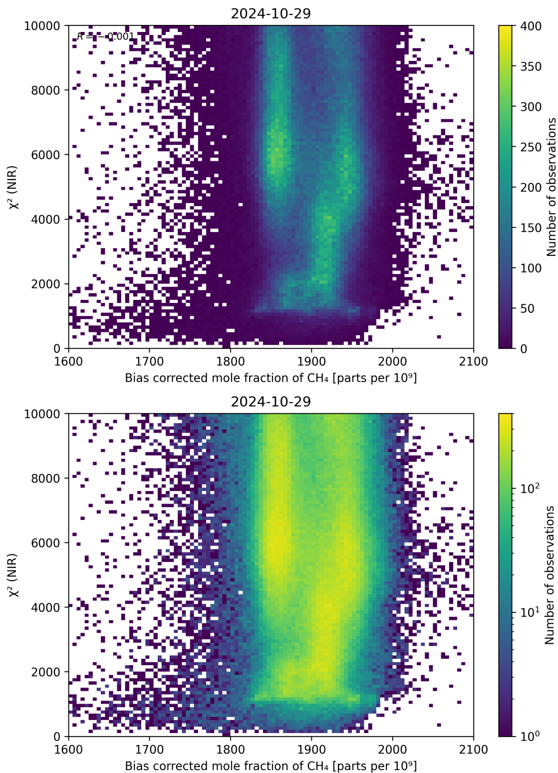
Figure 63: Scatter density plot of “Bias corrected mole fraction of CH 4 ” against “ \chi^2 (NIR)” for 2024-10-29 to 2024-10-30.
