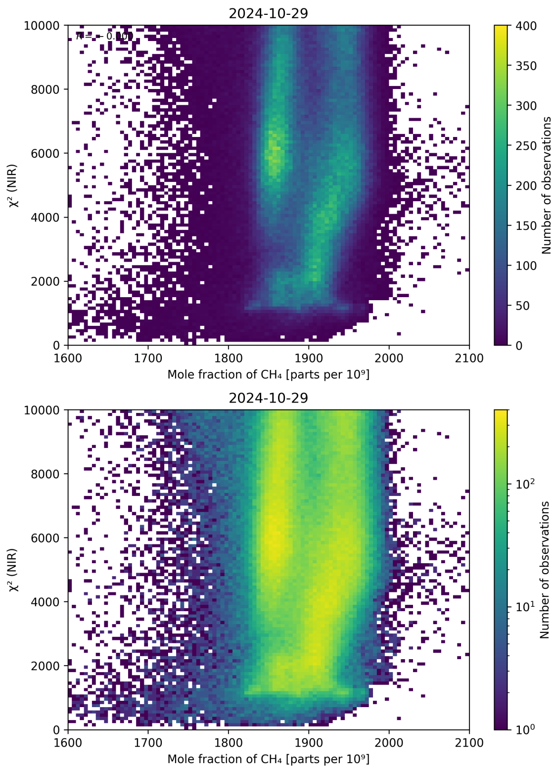
Figure 70: Scatter density plot of “Mole fraction of \text{CH}_4 ” against “ \chi^2 (NIR)” for 2024-10-29 to 2024-10-30.
