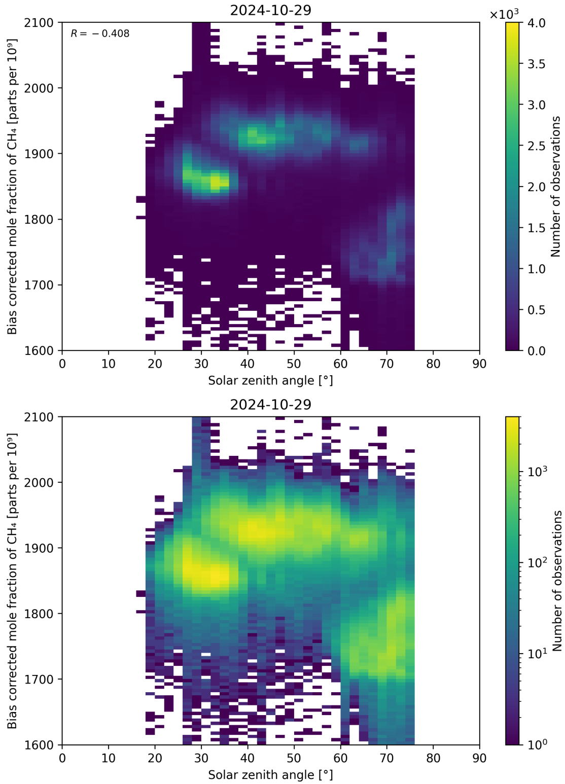
Figure 100: Scatter density plot of “Solar zenith angle” against “Bias corrected mole fraction of CH 4 ” for 2024-10-29 to 2024-10-30.
