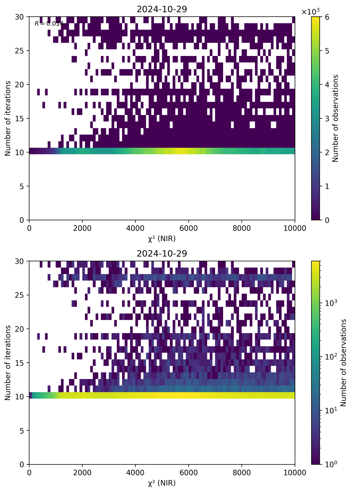
Figure 46: Scatter density plot of “ \chi^2 (NIR)” against “Number of iterations” for 2024-10-29 to 2024-10-30.
