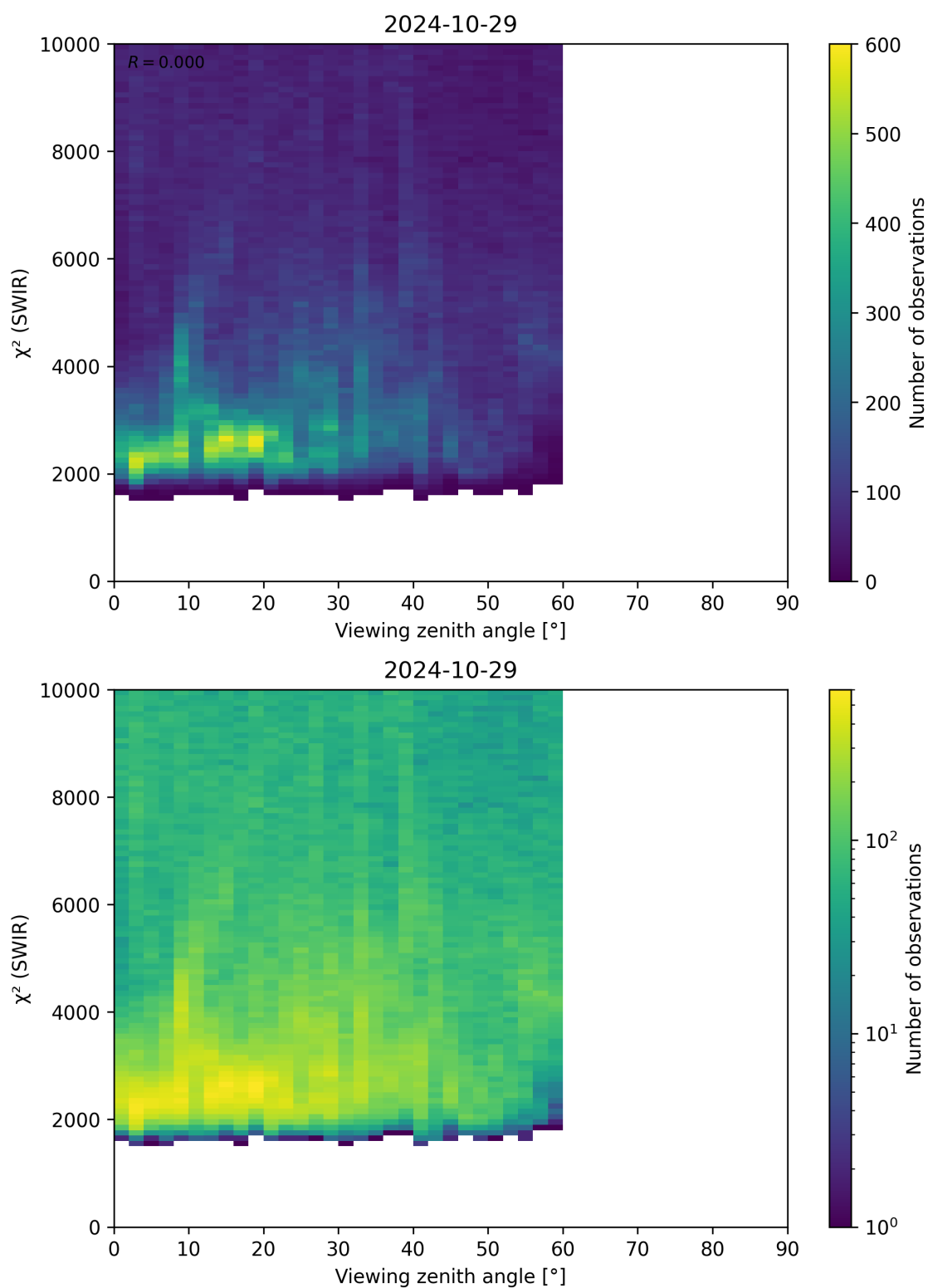
Figure 106: Scatter density plot of “Viewing zenith angle” against “ \chi^2 (SWIR)” for 2024-10-29 to 2024-10-30.
