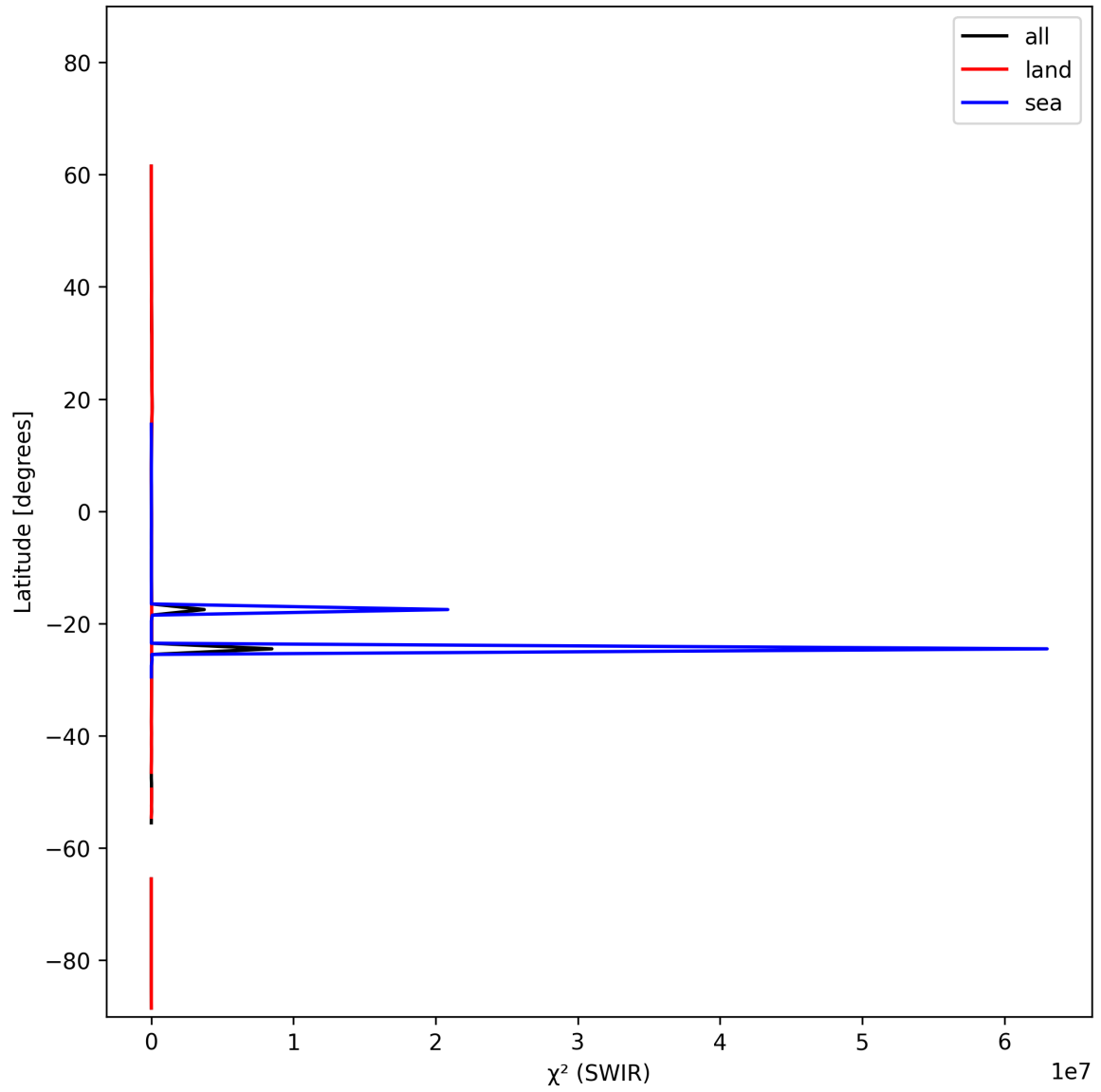
Figure 17: Zonal average of “ \chi^2 (SWIR)” for 2024-10-29 to 2024-10-30.
