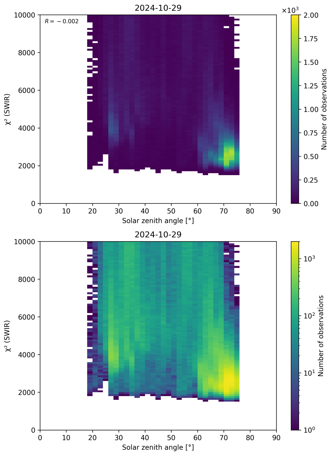
Figure 95: Scatter density plot of “Solar zenith angle” against “ \chi^2 (SWIR)” for 2024-10-29 to 2024-10-30.
