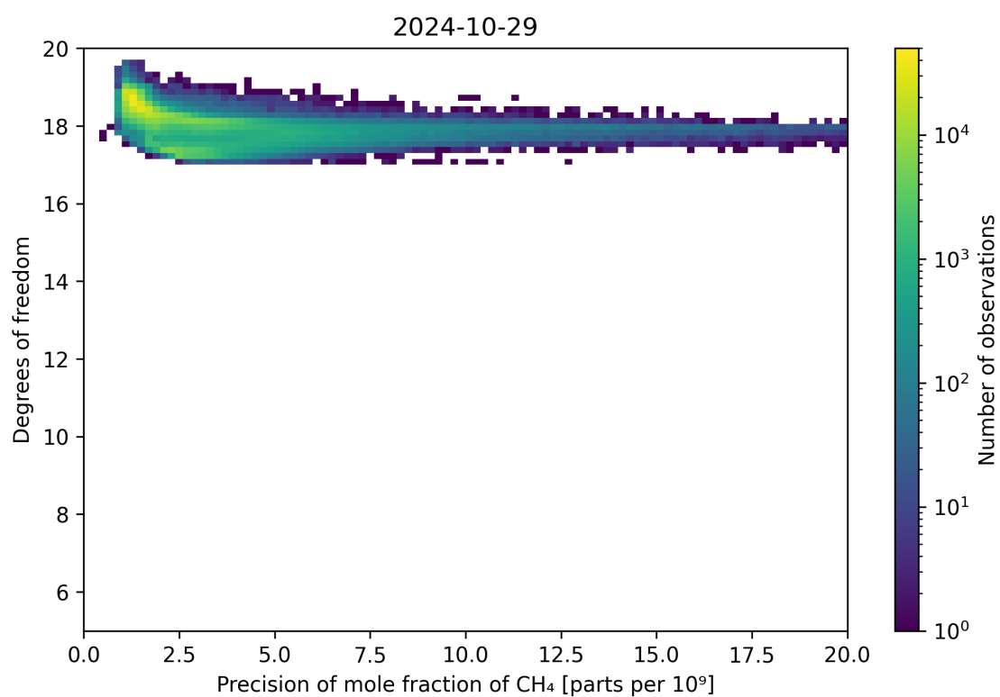
Figure 80: Scatter density plot of “Precision of mole fraction of CH 4 ” against “Degrees of freedom” for 2024-10-29 to 2024-10-30.
