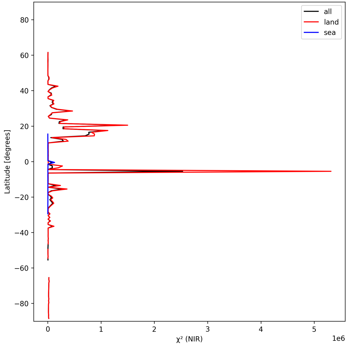
Figure 18: Zonal average of “ \chi^2 (NIR)” for 2024-10-29 to 2024-10-30.
