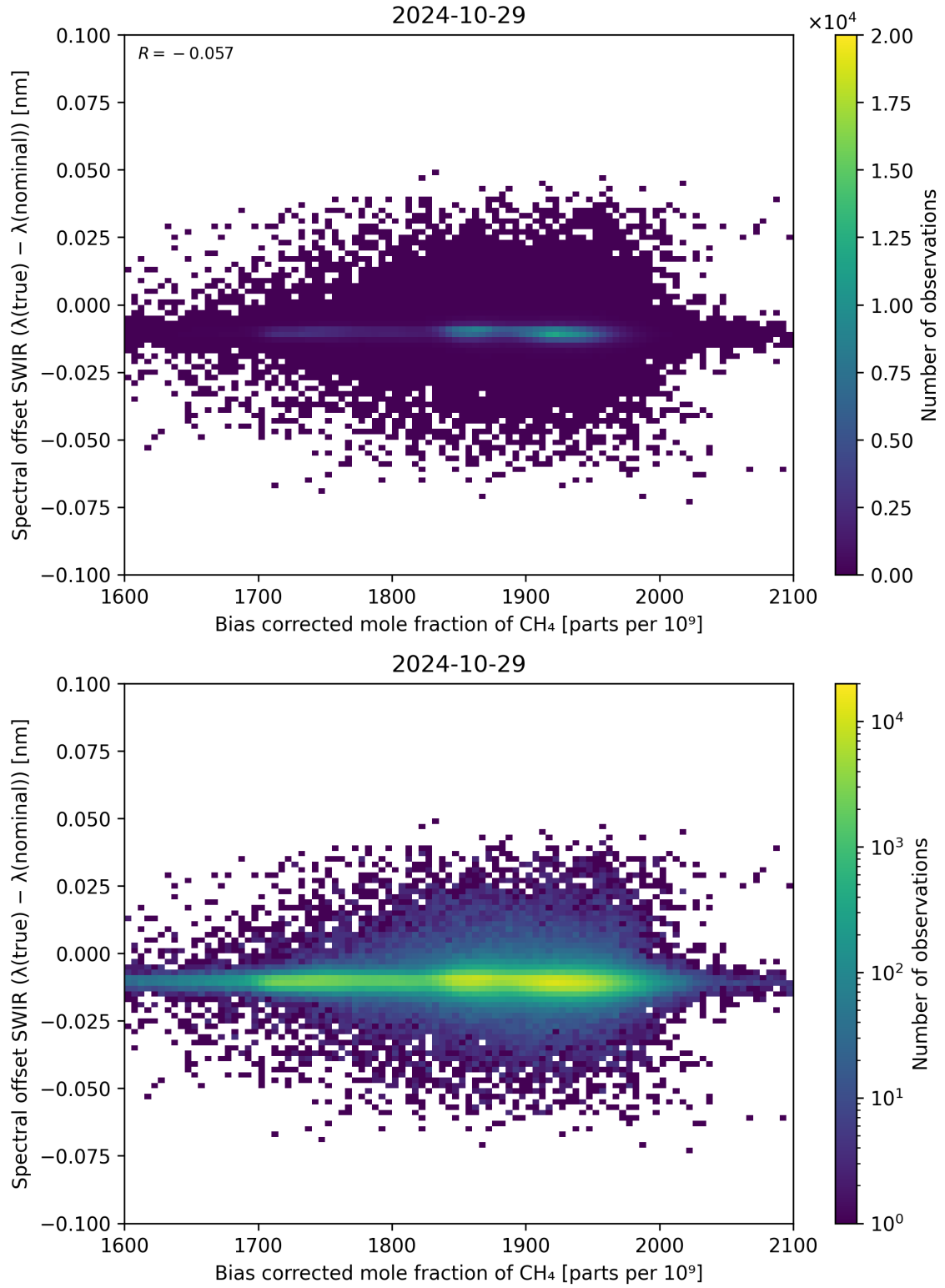
Figure 69: Scatter density plot of “Bias corrected mole fraction of \text{CH}_4 ” against “Spectral offset SWIR ( \lambda_{\text{true}} - \lambda_{\text{nominal}} )” for 2024-10-29 to 2024-10-30.
