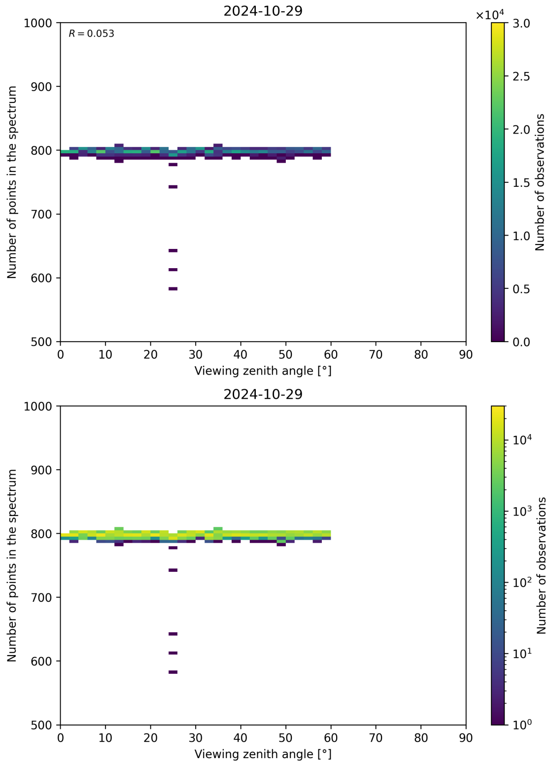
Figure 114: Scatter density plot of “Viewing zenith angle” against “Number of points in the spectrum” for 2024-10-29 to 2024-10-30.
