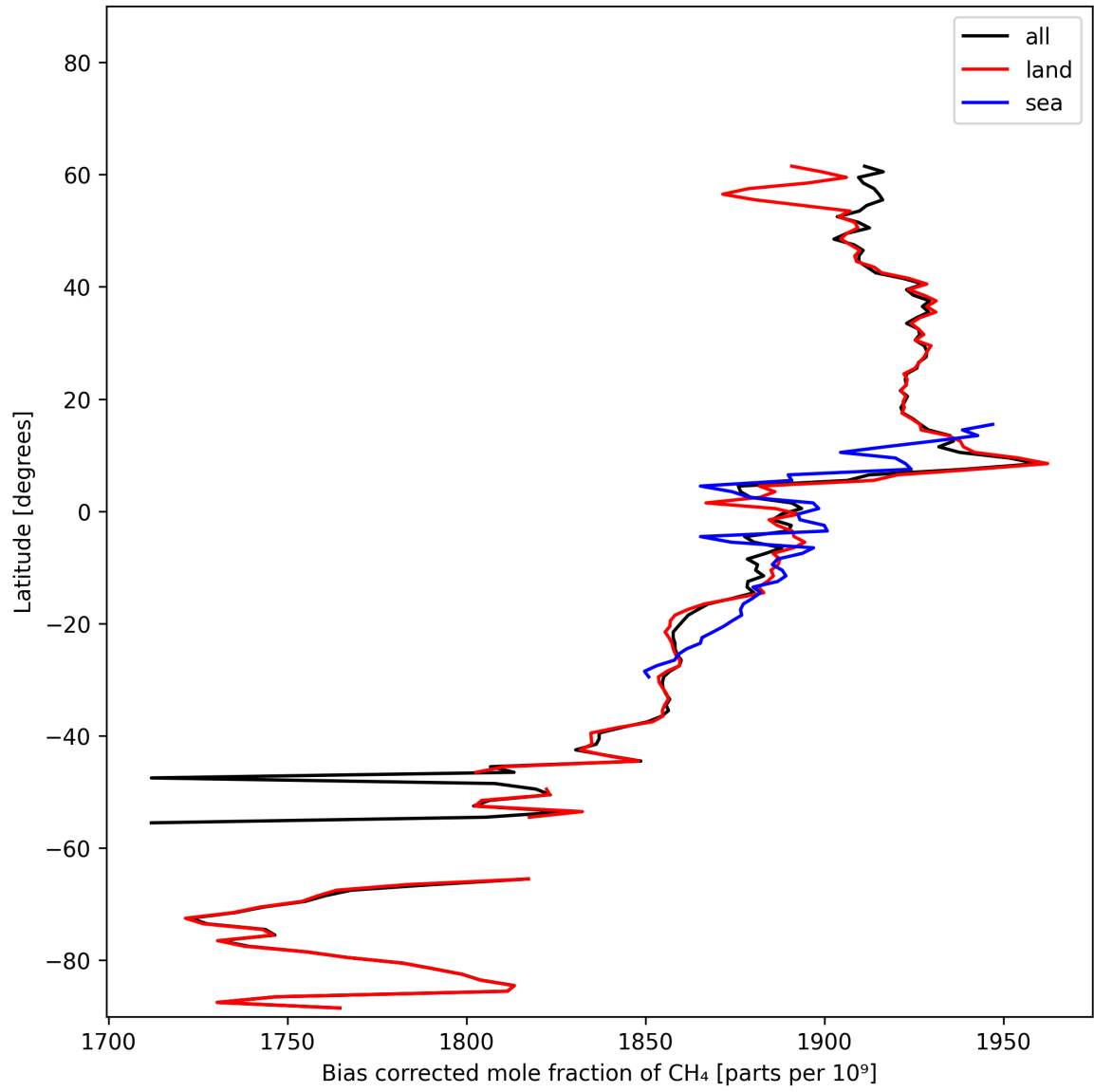
Figure 14: Zonal average of “Bias corrected mole fraction of \text{CH}_4 ” for 2024-10-29 to 2024-10-30.
