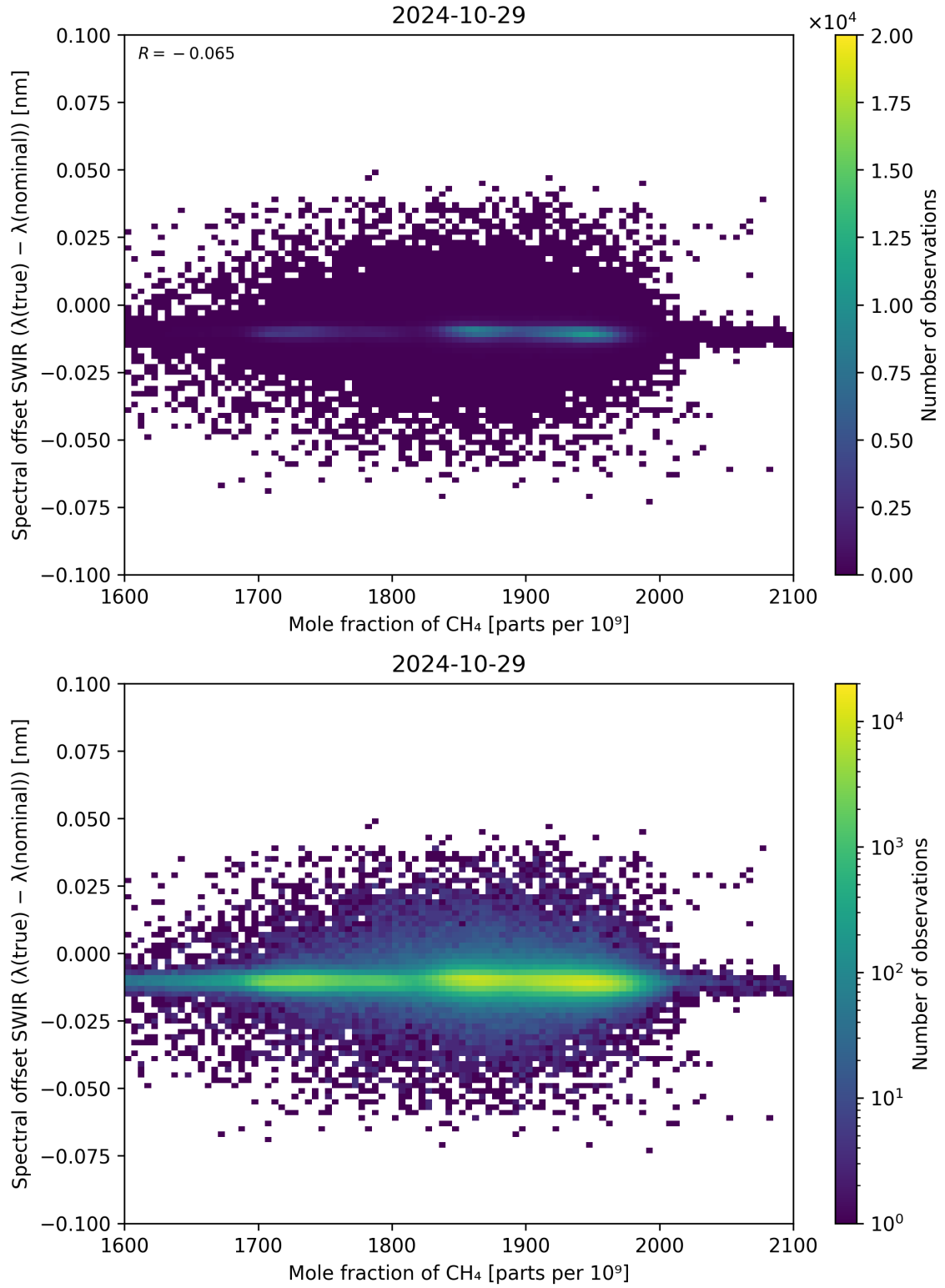
Figure 86: Scatter density plot of “Mole fraction of \text{CH}_4 ” against “Spectral offset SWIR ( \lambda_{\text{true}} - \lambda_{\text{nominal}} )” for 2024-10-29 to 2024-10-30.
