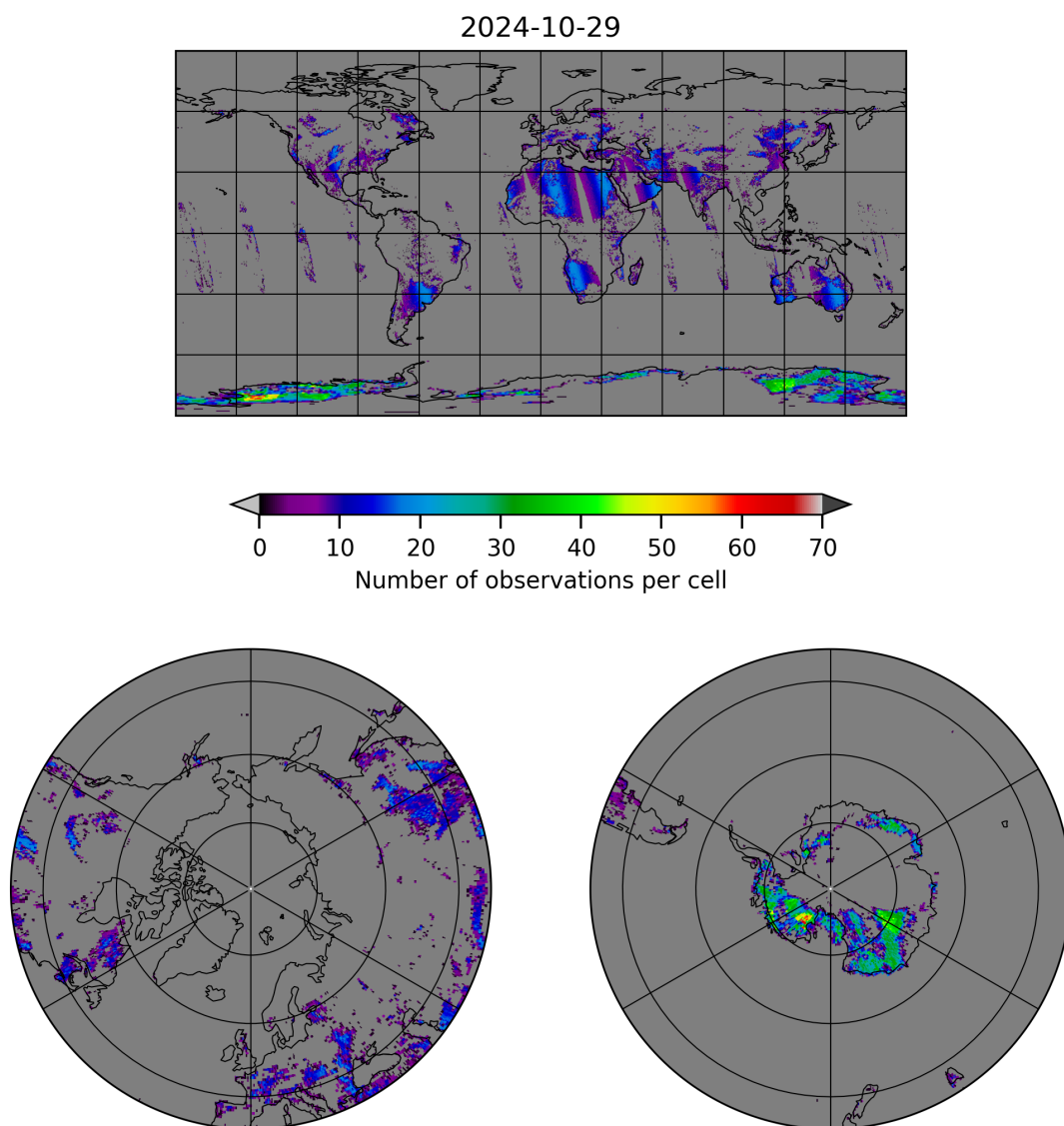
Figure 10: Map of the number of observations for 2024-10-29 to 2024-10-30
