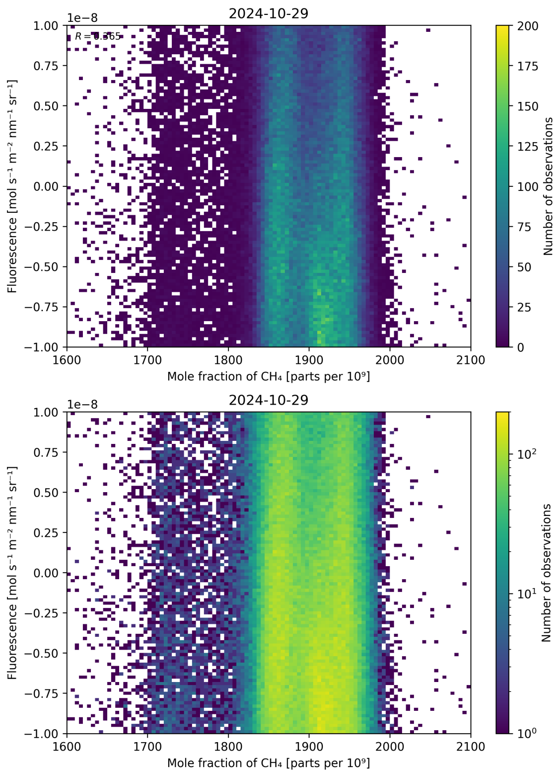
Figure 73: Scatter density plot of “Mole fraction of \text{CH}_4 ” against “Fluorescence” for 2024-10-29 to 2024-10-30.
