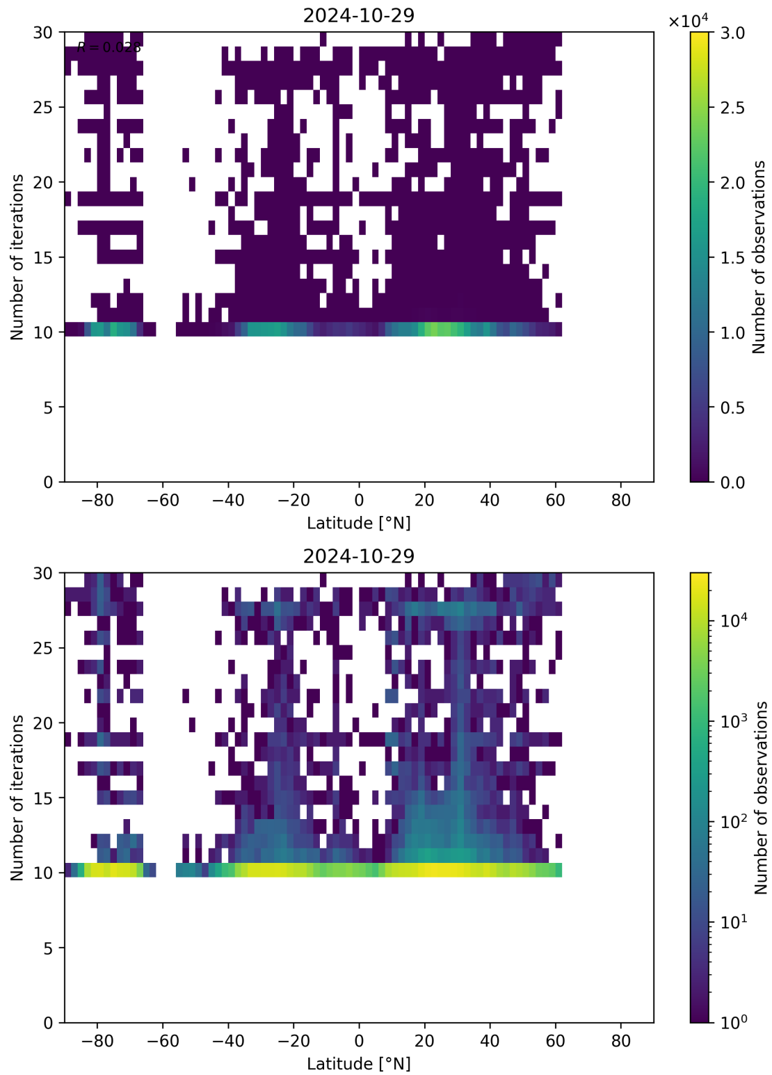
Figure 60: Scatter density plot of “Latitude” against “Number of iterations” for 2024-10-29 to 2024-10-30.
