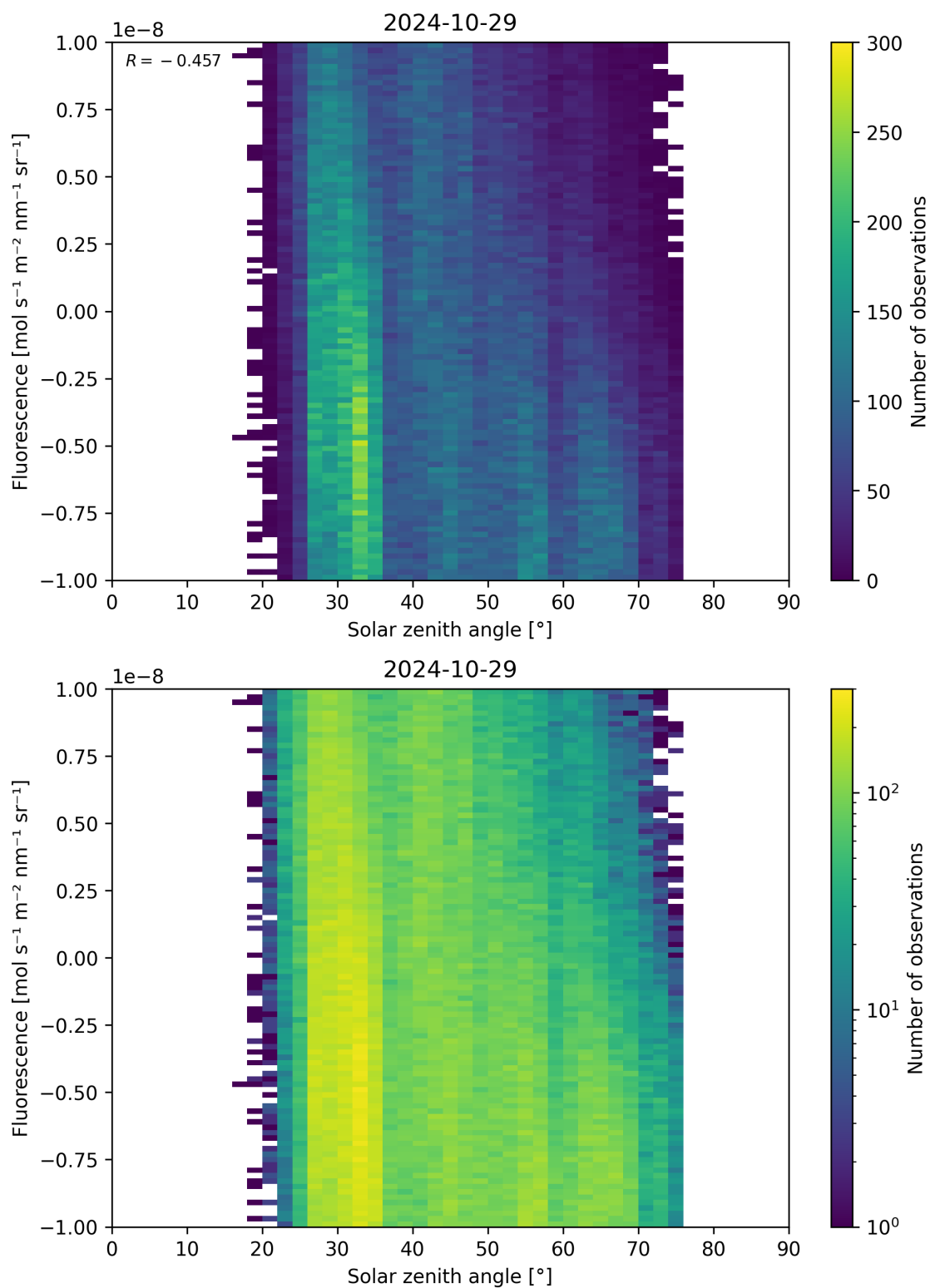
Figure 97: Scatter density plot of “Solar zenith angle” against “Fluorescence” for 2024-10-29 to 2024-10-30.
