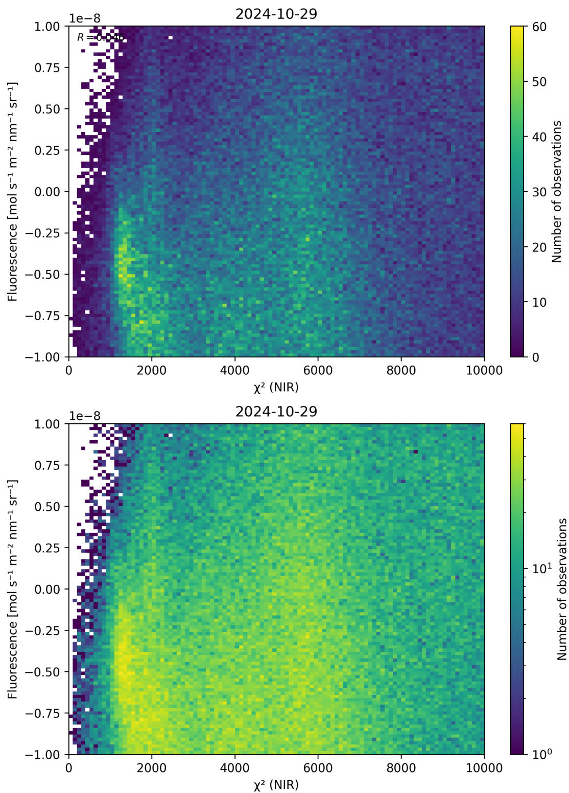
Figure 45: Scatter density plot of “ \chi^2 (NIR)” against “Fluorescence” for 2024-10-29 to 2024-10-30.
