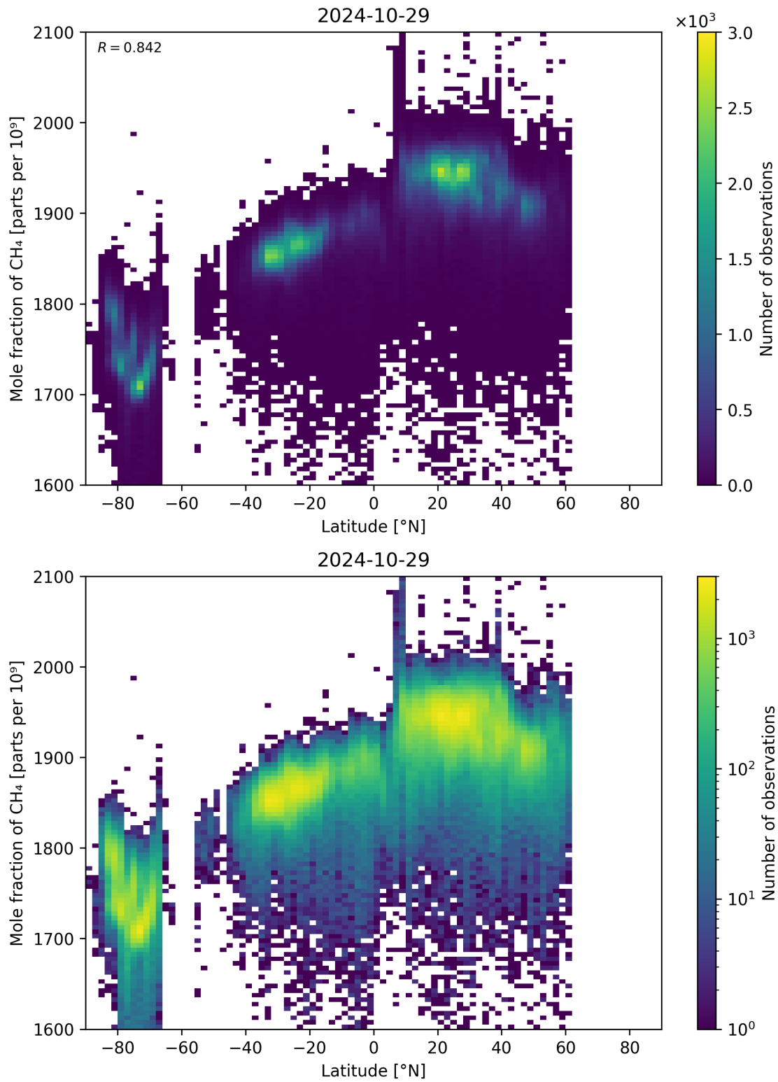
Figure 57: Scatter density plot of “Latitude” against “Mole fraction of \text{CH}_4 ” for 2024-10-29 to 2024-10-30.
