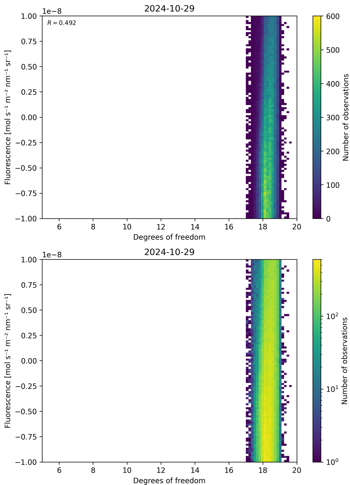
Figure 51: Scatter density plot of “Degrees of freedom” against “Fluorescence” for 2024-10-29 to 2024-10-30.
