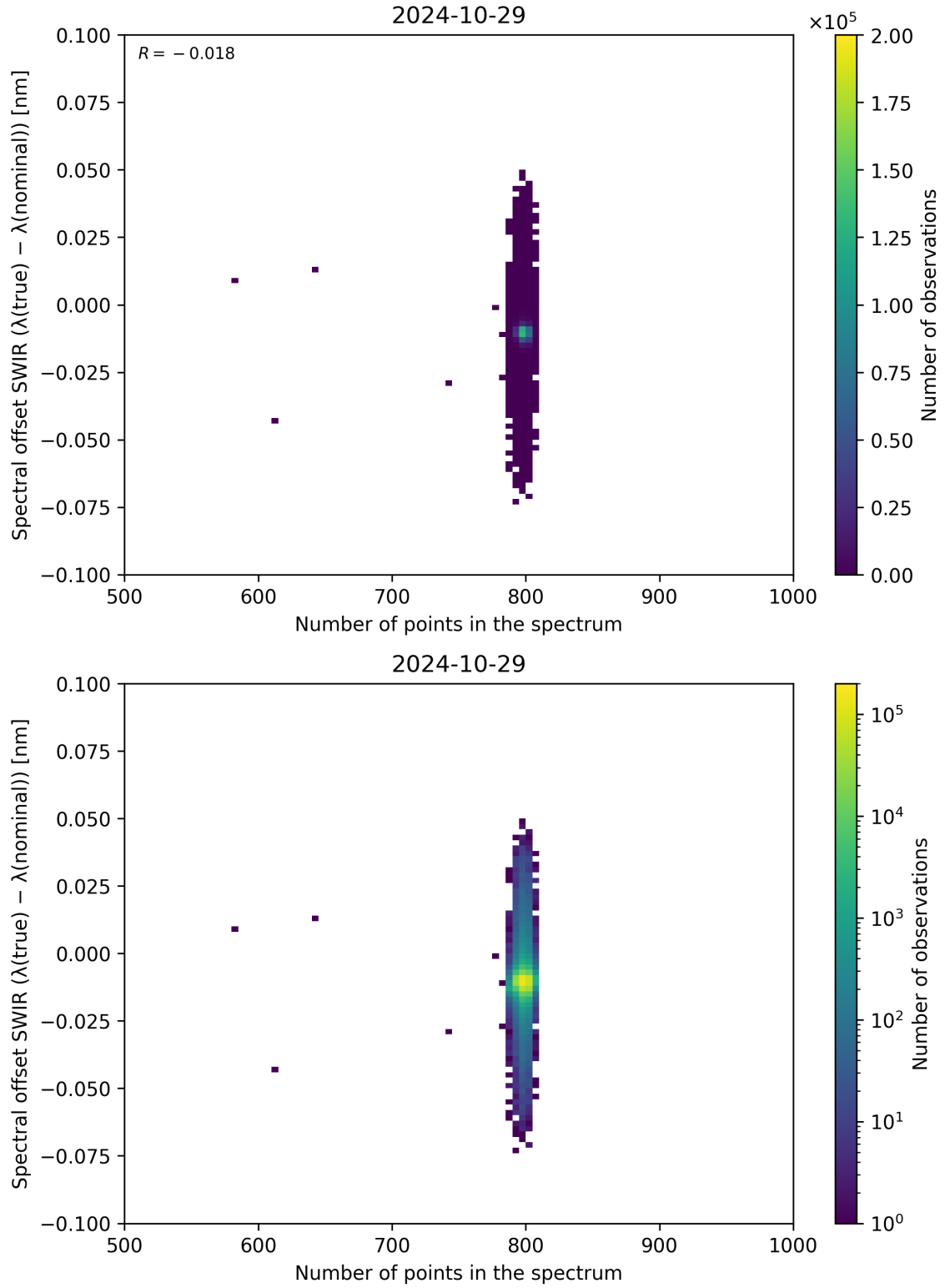
Figure 93: Scatter density plot of “Number of points in the spectrum” against “Spectral offset SWIR ( \lambda_{\text{true}} - \lambda_{\text{nominal}} )” for 2024-10-29 to 2024-10-30.
