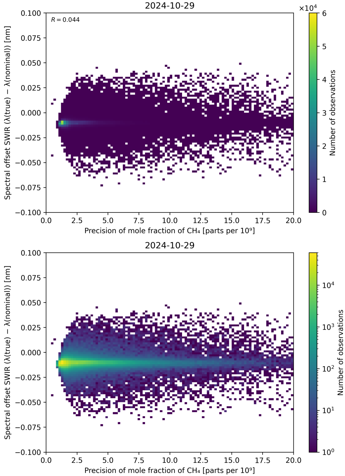
Figure 85: Scatter density plot of “Precision of mole fraction of \text{CH}_4 ” against “Spectral offset SWIR ( \lambda_{\text{true}} - \lambda_{\text{nominal}} )” for 2024-10-29 to 2024-10-30.
