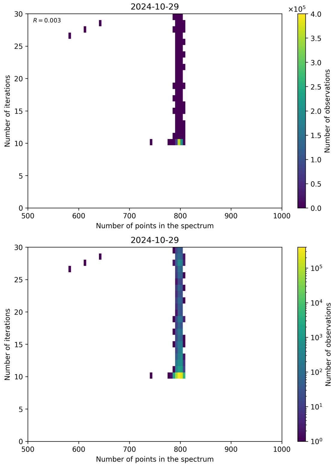
Figure 92: Scatter density plot of “Number of points in the spectrum” against “Number of iterations” for 2024-10-29 to 2024-10-30.
