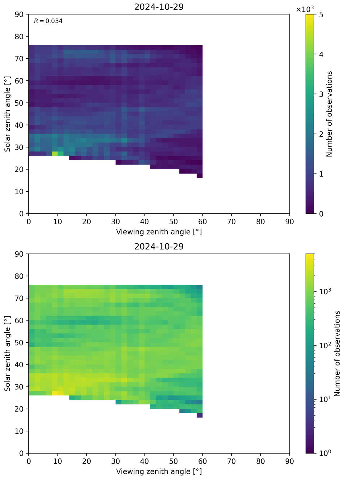
Figure 115: Scatter density plot of “Viewing zenith angle” against “Solar zenith angle” for 2024-10-29 to 2024-10-30.
