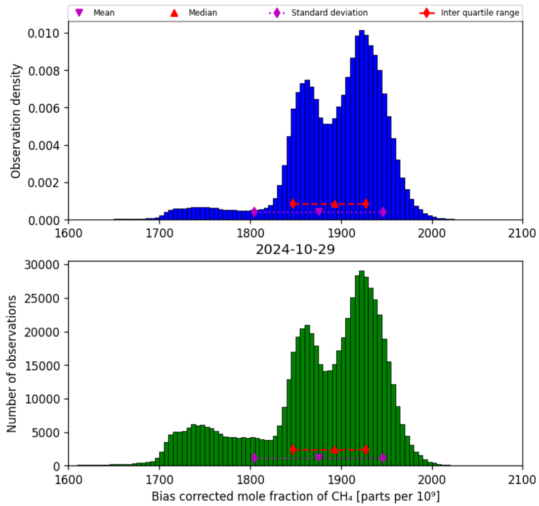
Figure 25: Histogram of “Bias corrected mole fraction of CH 4 ” for 2024-10-29 to 2024-10-30
