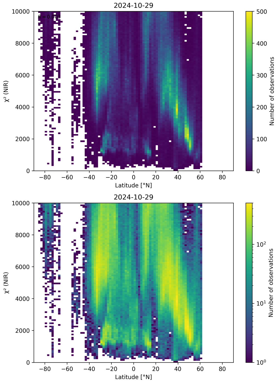
Figure 53: Scatter density plot of “Latitude” against “ \chi^2 (NIR)” for 2024-10-29 to 2024-10-30.
