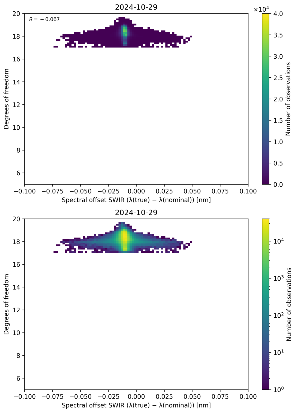
Figure 119: Scatter density plot of “Spectral offset SWIR ( \lambda_{\text{true}} - \lambda_{\text{nominal}} )” against “Degrees of freedom” for 2024-10-29 to 2024-10-30.
