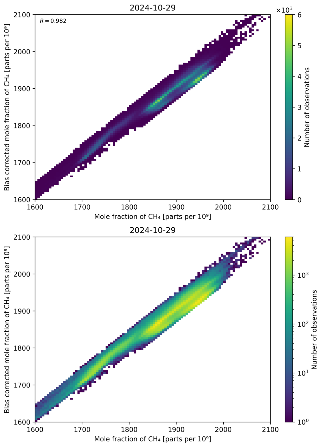
Figure 74: Scatter density plot of “Mole fraction of CH 4 ” against “Bias corrected mole fraction of CH 4 ” for 2024-10-29 to 2024-10-30.
