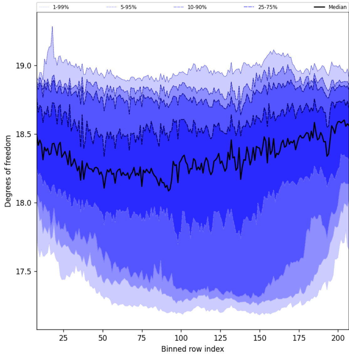
Figure 41: Along track statistics of “Degrees of freedom” for 2024-10-29 to 2024-10-30
