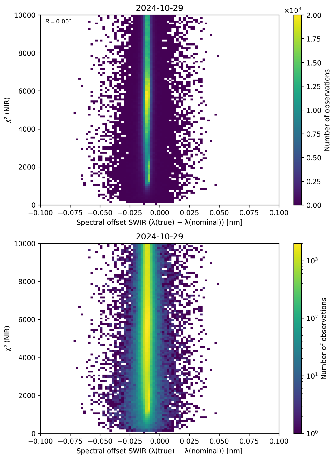
Figure 117: Scatter density plot of “Spectral offset SWIR ( \lambda_{\text{true}} - \lambda_{\text{nominal}} )” against “ \chi^2 (NIR)” for 2024-10-29 to 2024-10-30.
