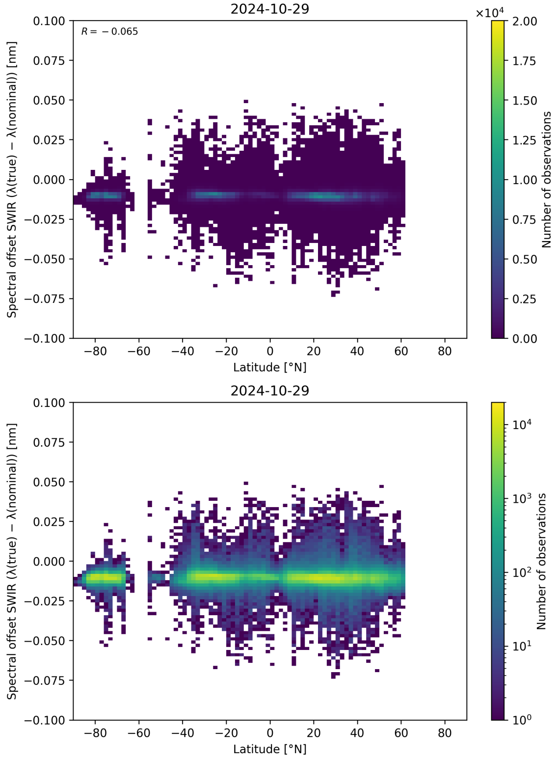
Figure 62: Scatter density plot of “Latitude” against “Spectral offset SWIR ( \lambda_{\text{true}} - \lambda_{\text{nominal}} )” for 2024-10-29 to 2024-10-30.
