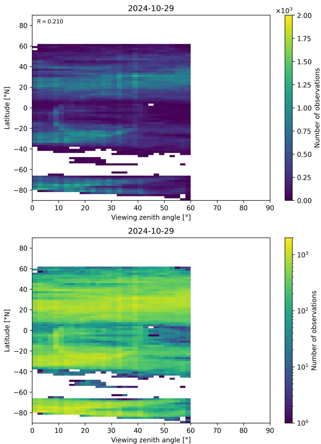
Figure 109: Scatter density plot of “Viewing zenith angle” against “Latitude” for 2024-10-29 to 2024-10-30.
