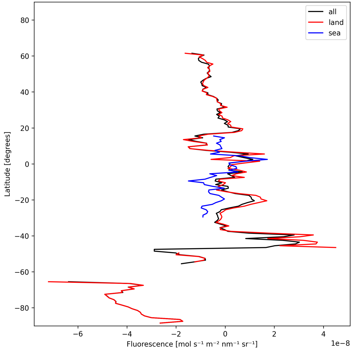
Figure 21: Zonal average of “Fluorescence” for 2024-10-29 to 2024-10-30.
