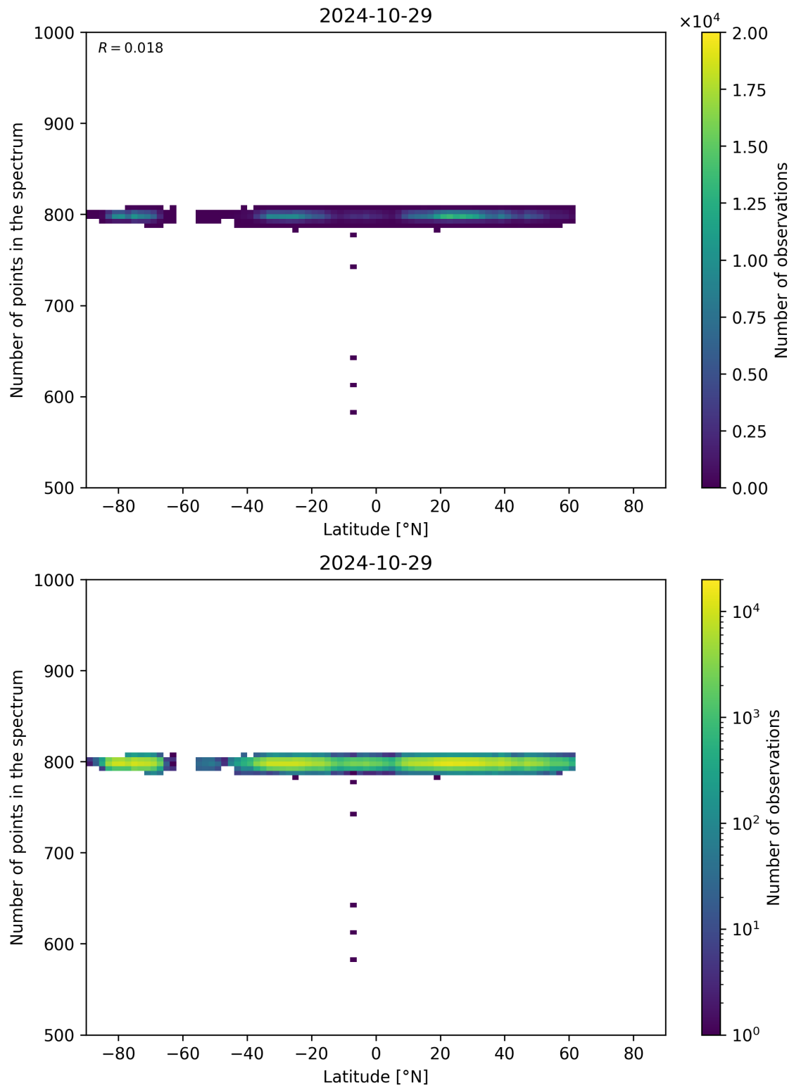
Figure 61: Scatter density plot of “Latitude” against “Number of points in the spectrum” for 2024-10-29 to 2024-10-30.
