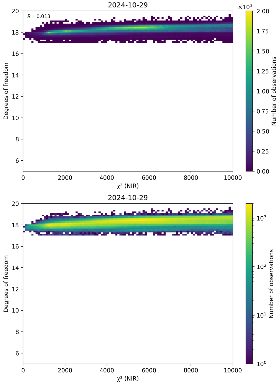
Figure 44: Scatter density plot of “ \chi^2 (NIR)” against “Degrees of freedom” for 2024-10-29 to 2024-10-30.
