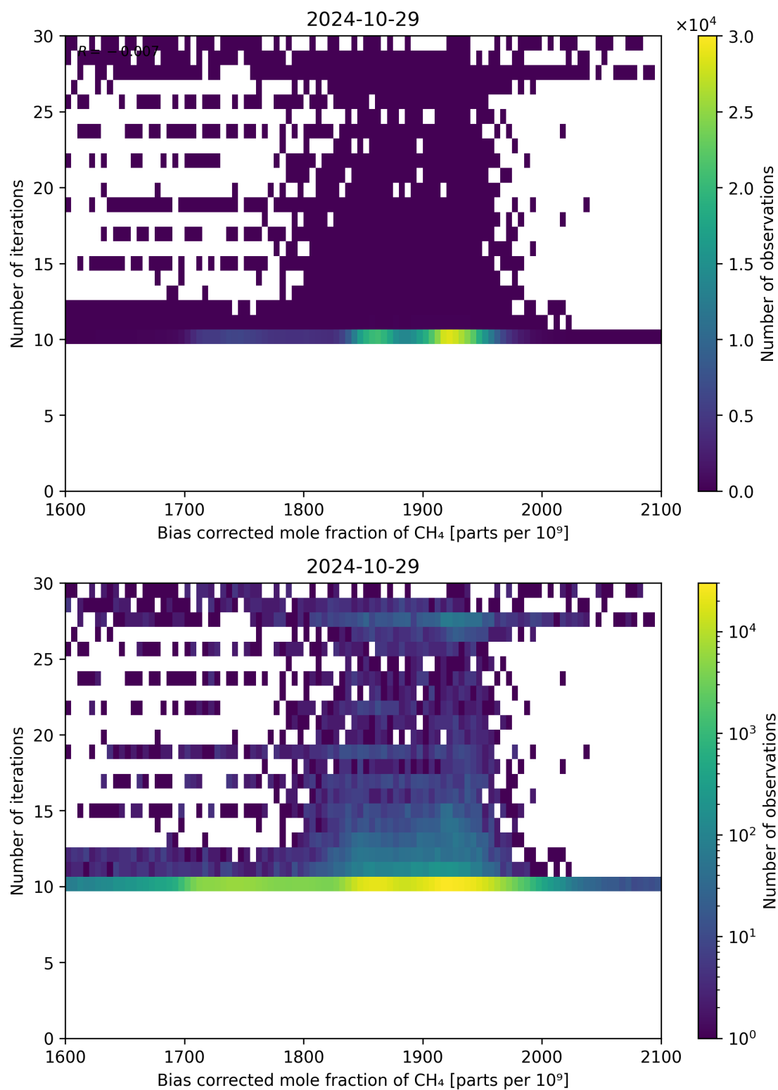
Figure 67: Scatter density plot of “Bias corrected mole fraction of CH 4 ” against “Number of iterations” for 2024-10-29 to 2024-10-30.
