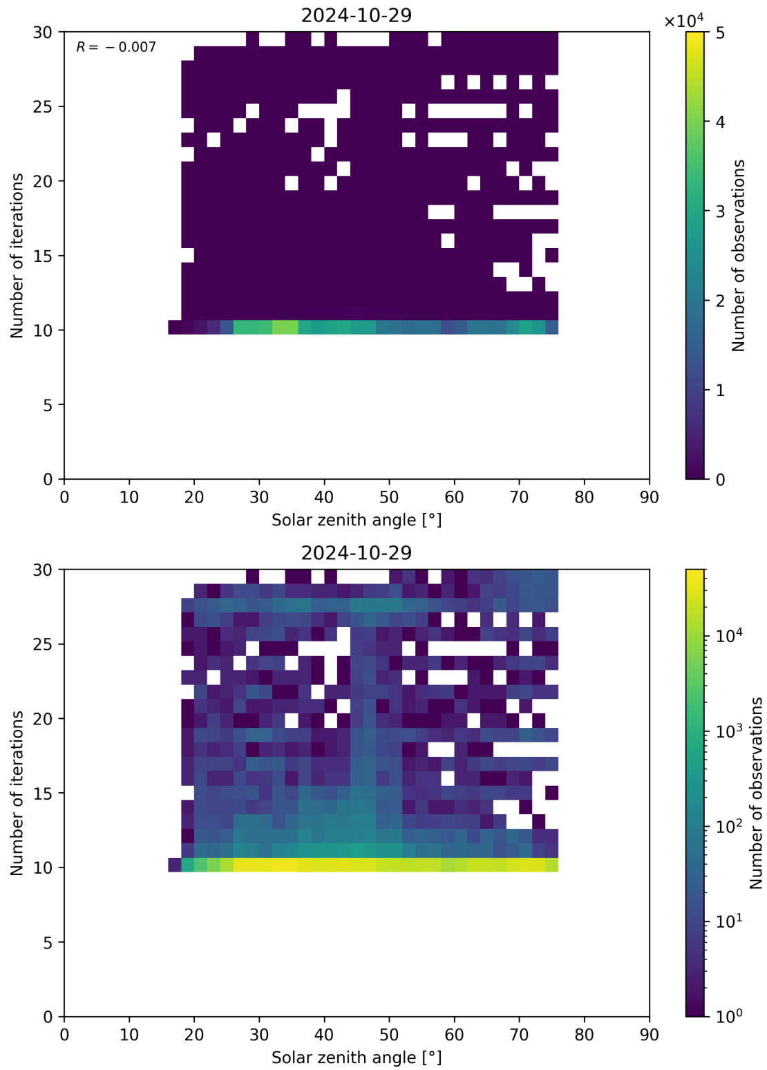
Figure 102: Scatter density plot of “Solar zenith angle” against “Number of iterations” for 2024-10-29 to 2024-10-30.
