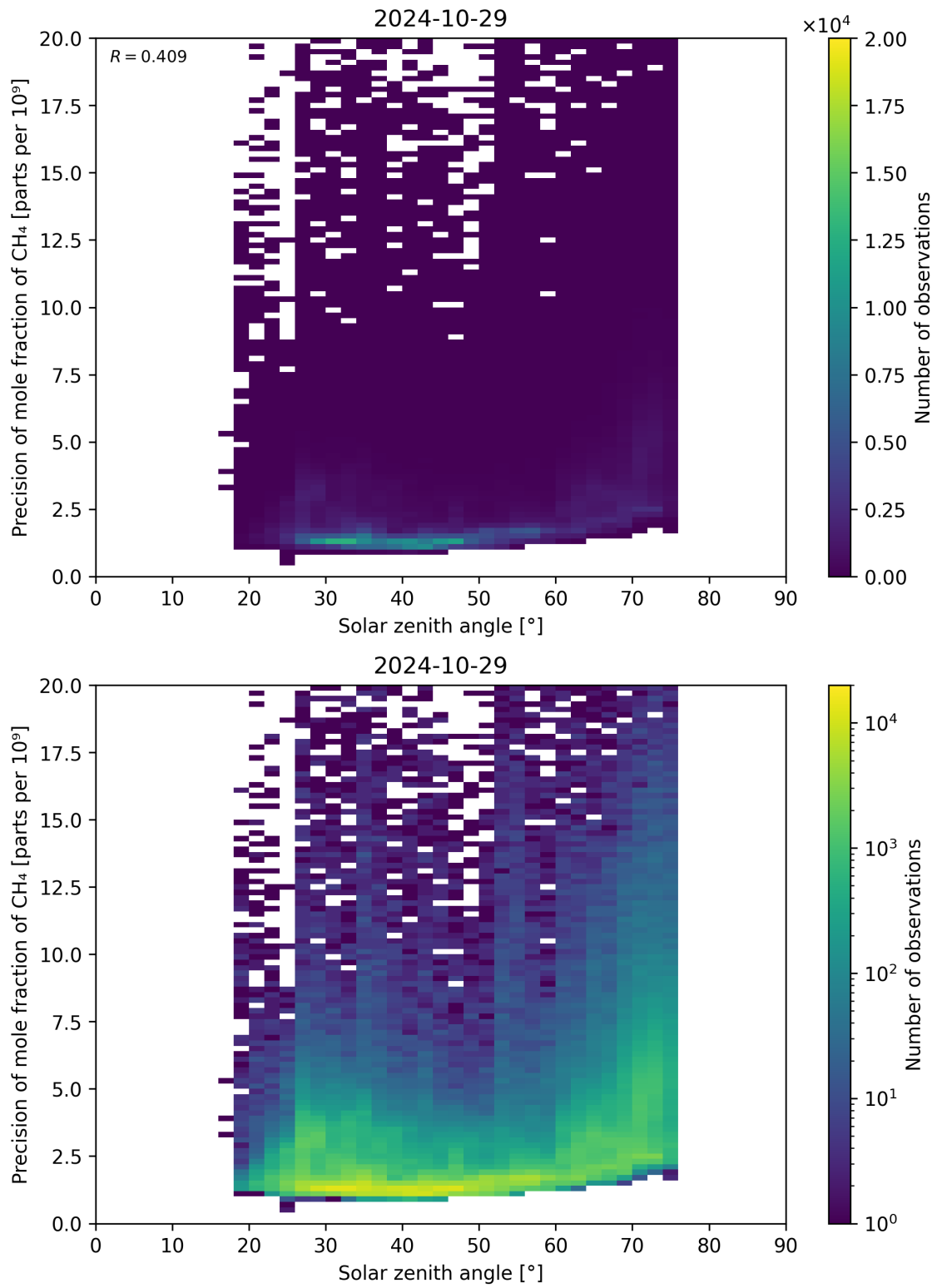
Figure 101: Scatter density plot of “Solar zenith angle” against “Precision of mole fraction of \text{CH}_4 ” for 2024-10-29 to 2024-10-30.
