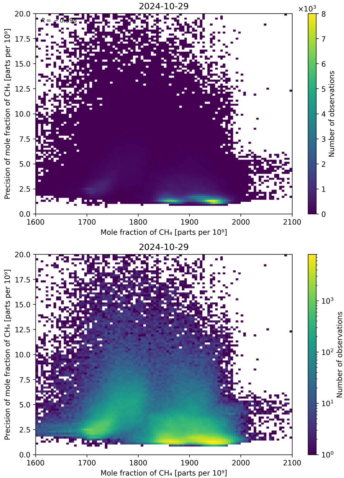
Figure 75: Scatter density plot of “Mole fraction of CH 4 ” against “Precision of mole fraction of CH 4 ” for 2024-10-29 to 2024-10-30.
