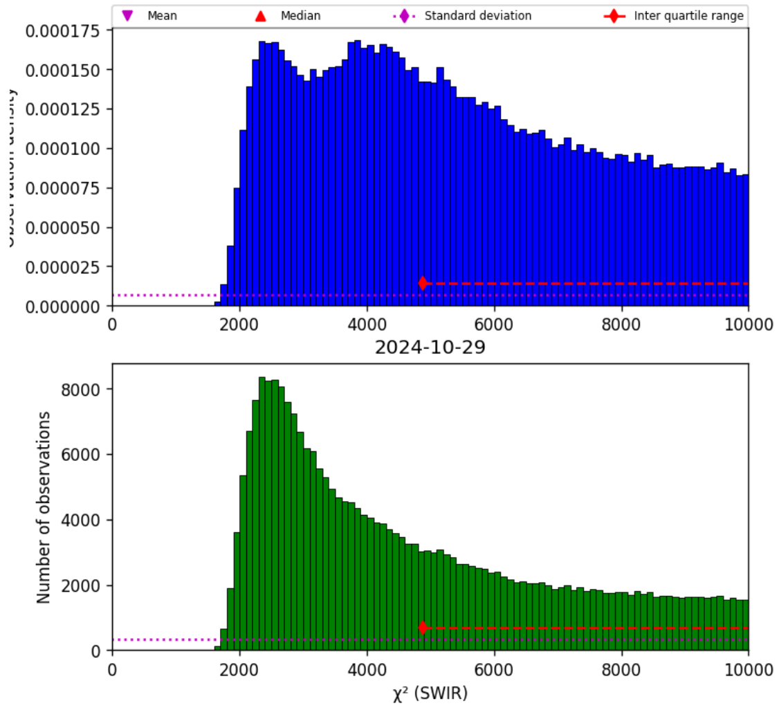
Figure 28: Histogram of “ \chi^2 (SWIR)” for 2024-10-29 to 2024-10-30
