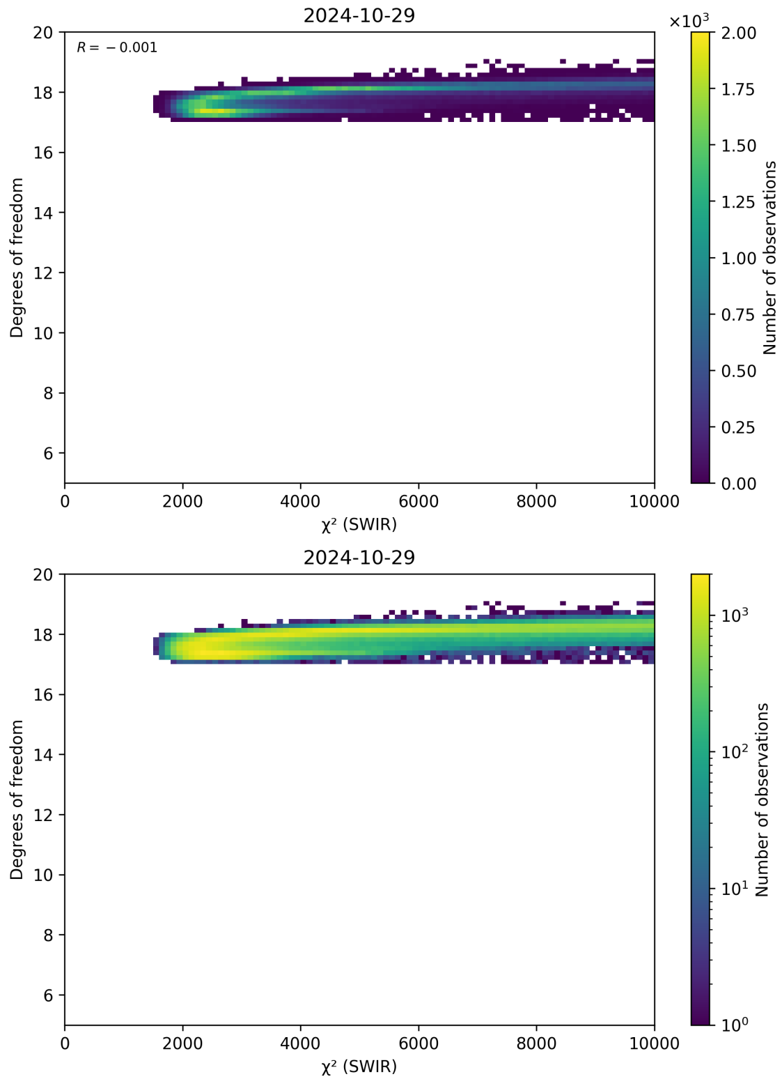
Figure 48: Scatter density plot of “ \chi^2 (SWIR)” against “Degrees of freedom” for 2024-10-29 to 2024-10-30.
