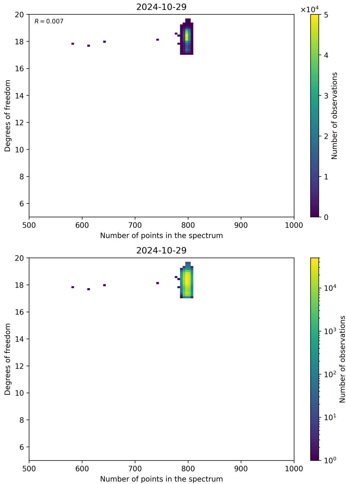
Figure 90: Scatter density plot of “Number of points in the spectrum” against “Degrees of freedom” for 2024-10-29 to 2024-10-30.
