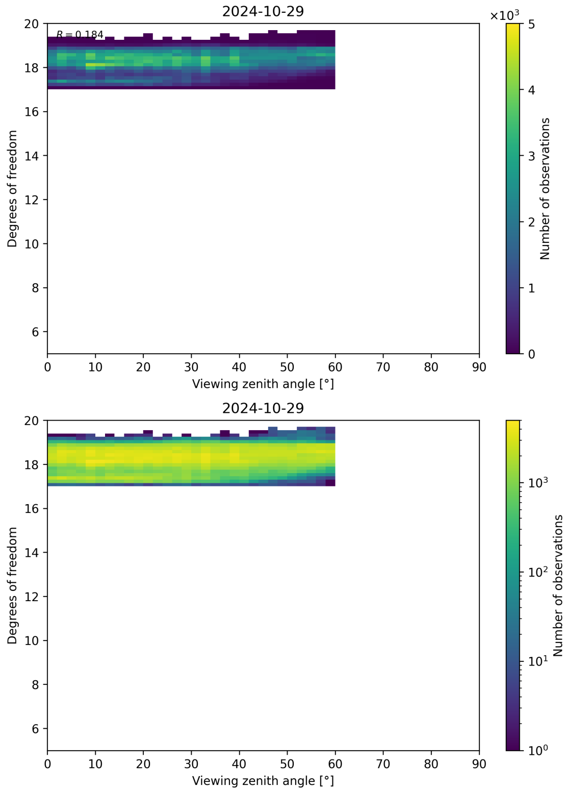
Figure 107: Scatter density plot of “Viewing zenith angle” against “Degrees of freedom” for 2024-10-29 to 2024-10-30.
