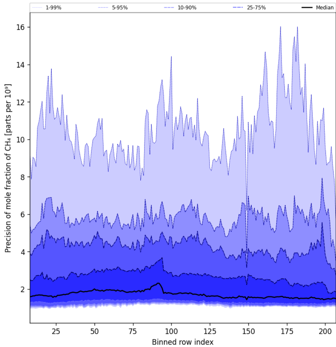
Figure 35: Along track statistics of “Precision of mole fraction of CH 4 ” for 2024-10-29 to 2024-10-30
