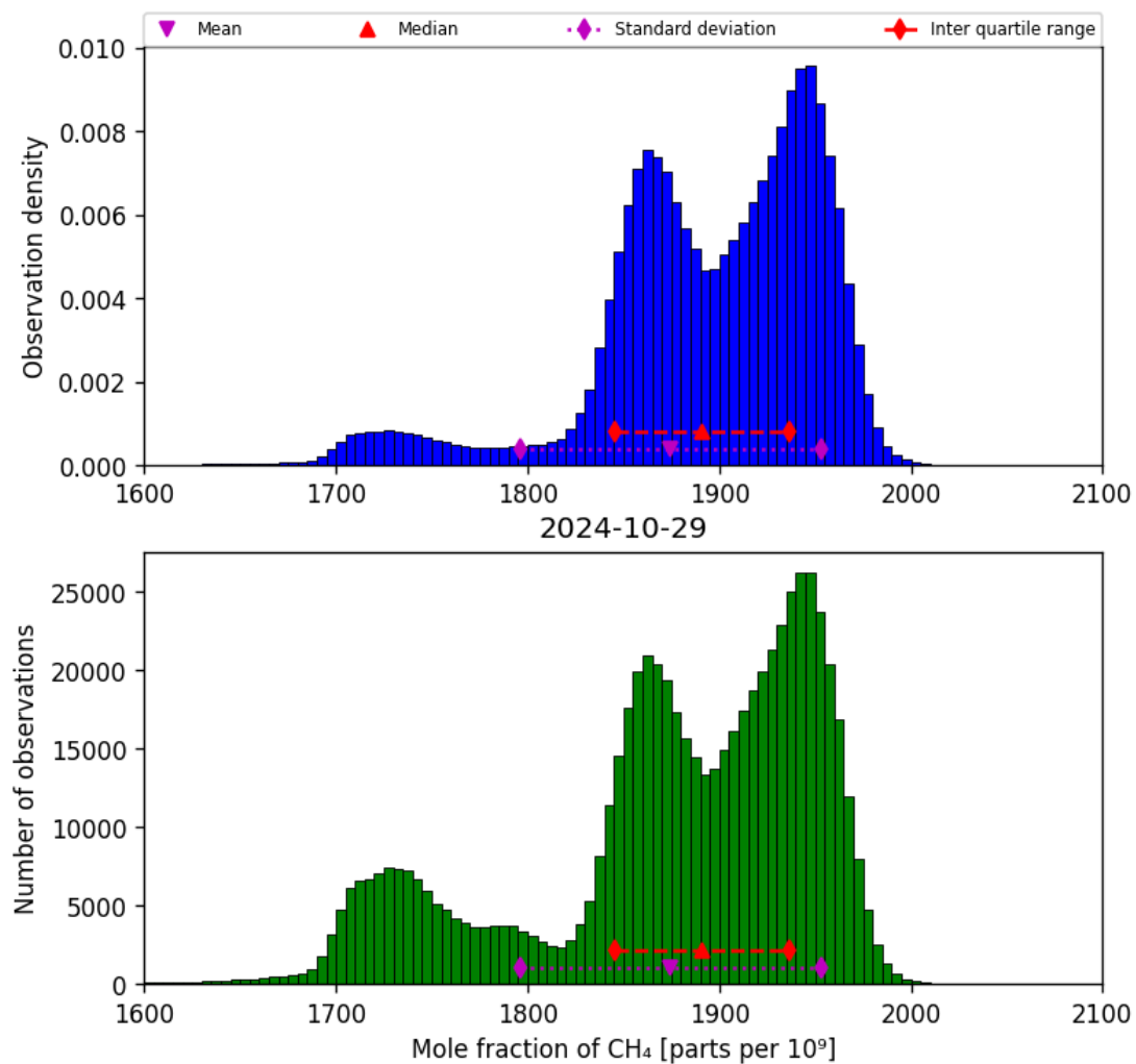
Figure 23: Histogram of “Mole fraction of CH 4 ” for 2024-10-29 to 2024-10-30
