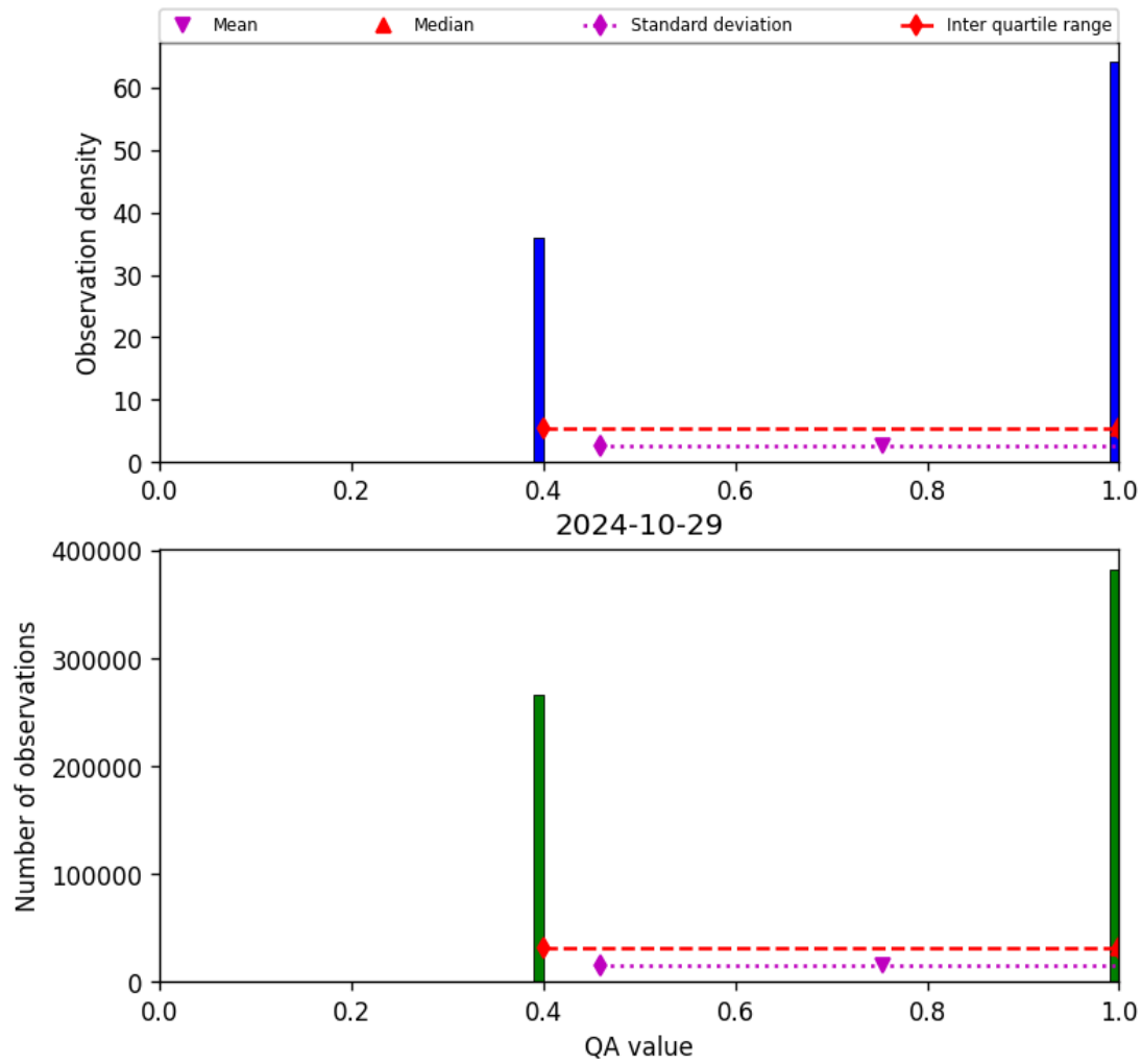
Figure 22: Histogram of “QA value” for 2024-10-29 to 2024-10-30
