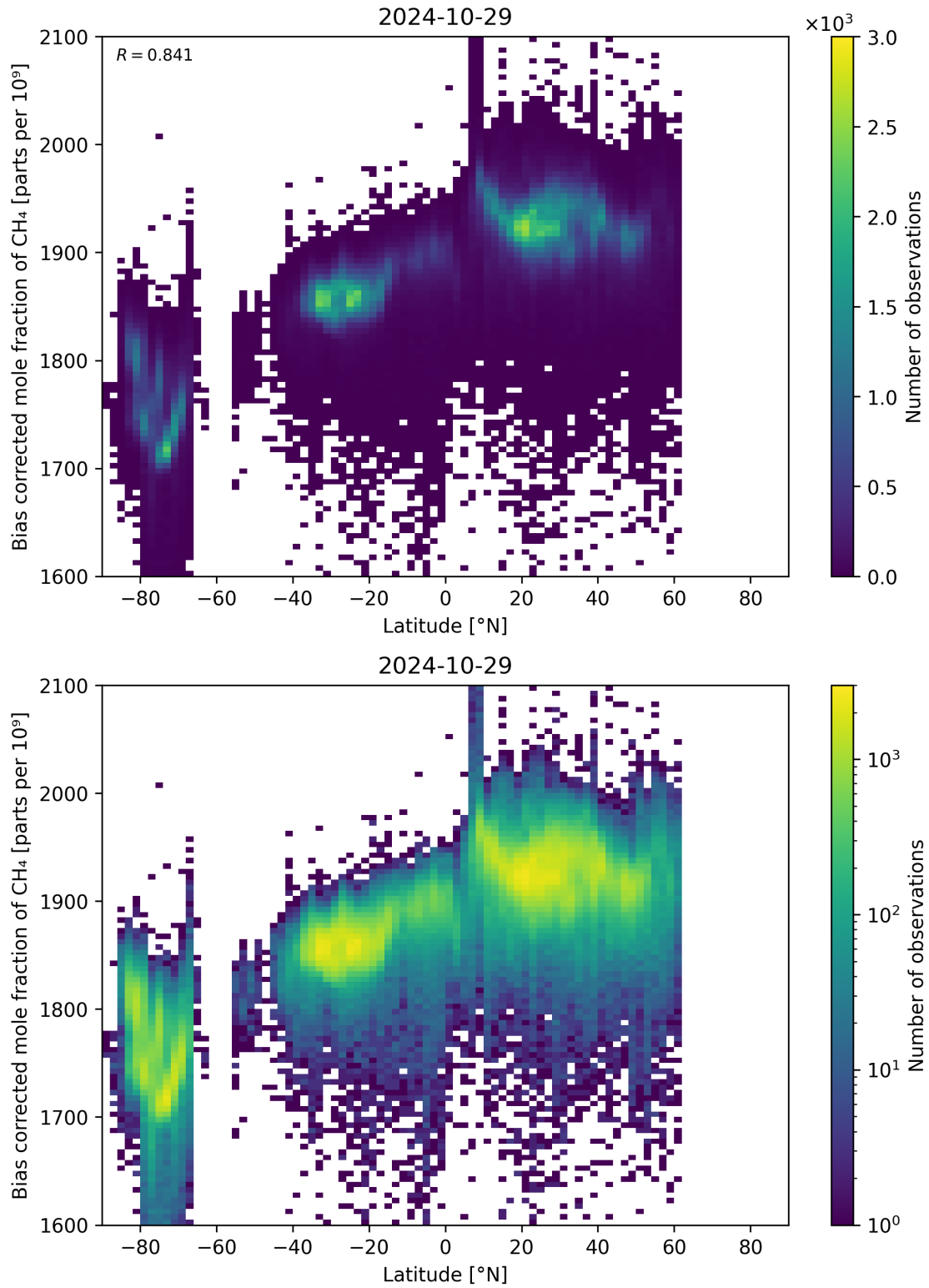
Figure 58: Scatter density plot of “Latitude” against “Bias corrected mole fraction of \text{CH}_4 ” for 2024-10-29 to 2024-10-30.
