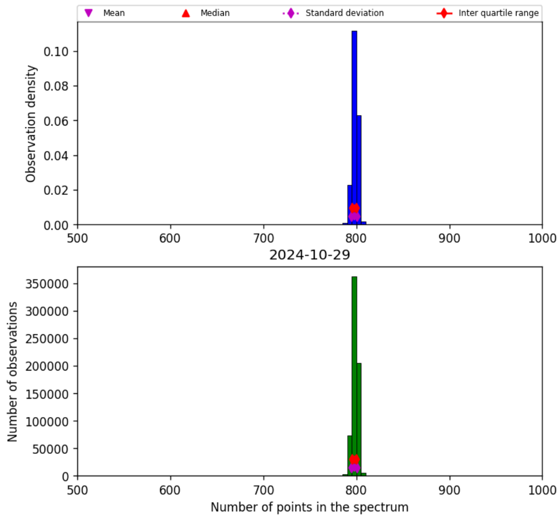
Figure 26: Histogram of “Number of points in the spectrum” for 2024-10-29 to 2024-10-30
