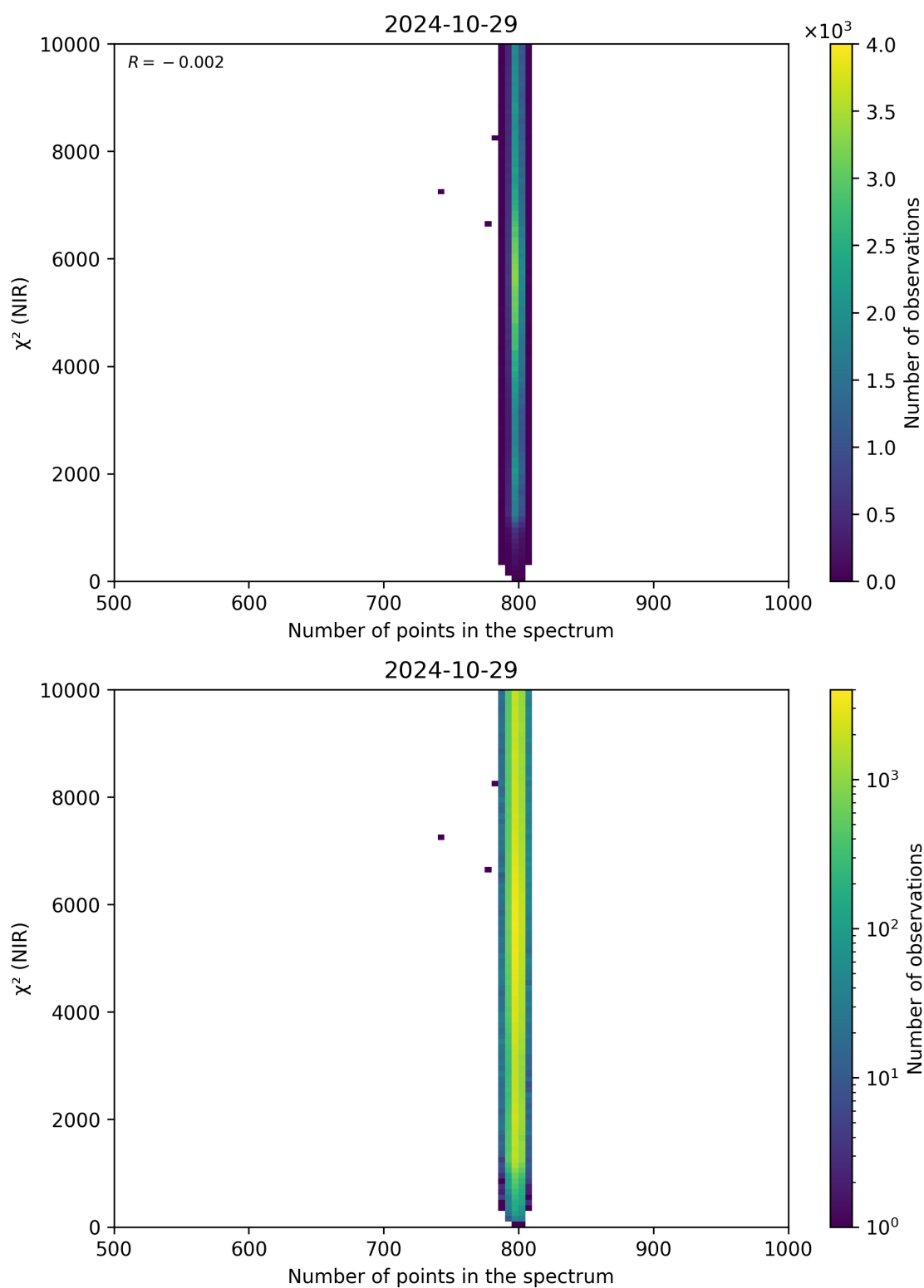
Figure 88: Scatter density plot of “Number of points in the spectrum” against “ \chi^2 (NIR)” for 2024-10-29 to 2024-10-30.
