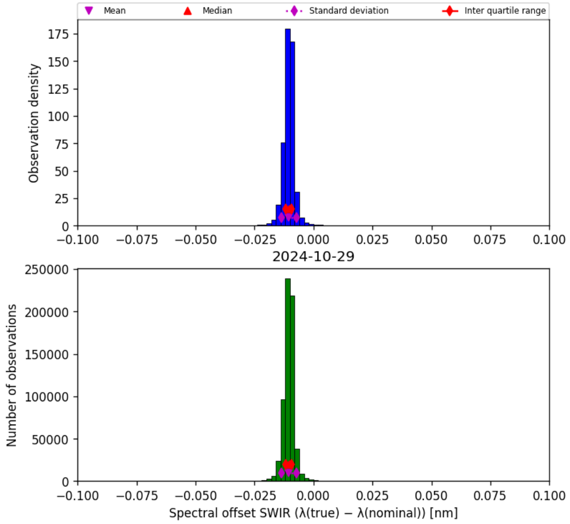
Figure 27: Histogram of “Spectral offset SWIR ( \lambda_{\text{true}} - \lambda_{\text{nominal}} )” for 2024-10-29 to 2024-10-30
