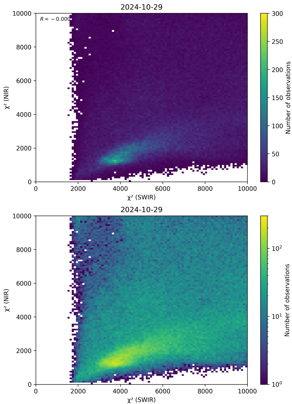
Figure 47: Scatter density plot of “ \chi^2 (SWIR)” against “ \chi^2 (NIR)” for 2024-10-29 to 2024-10-30.
