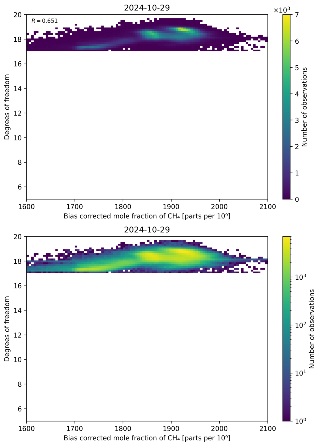
Figure 65: Scatter density plot of “Bias corrected mole fraction of CH 4 ” against “Degrees of freedom” for 2024-10-29 to 2024-10-30.
