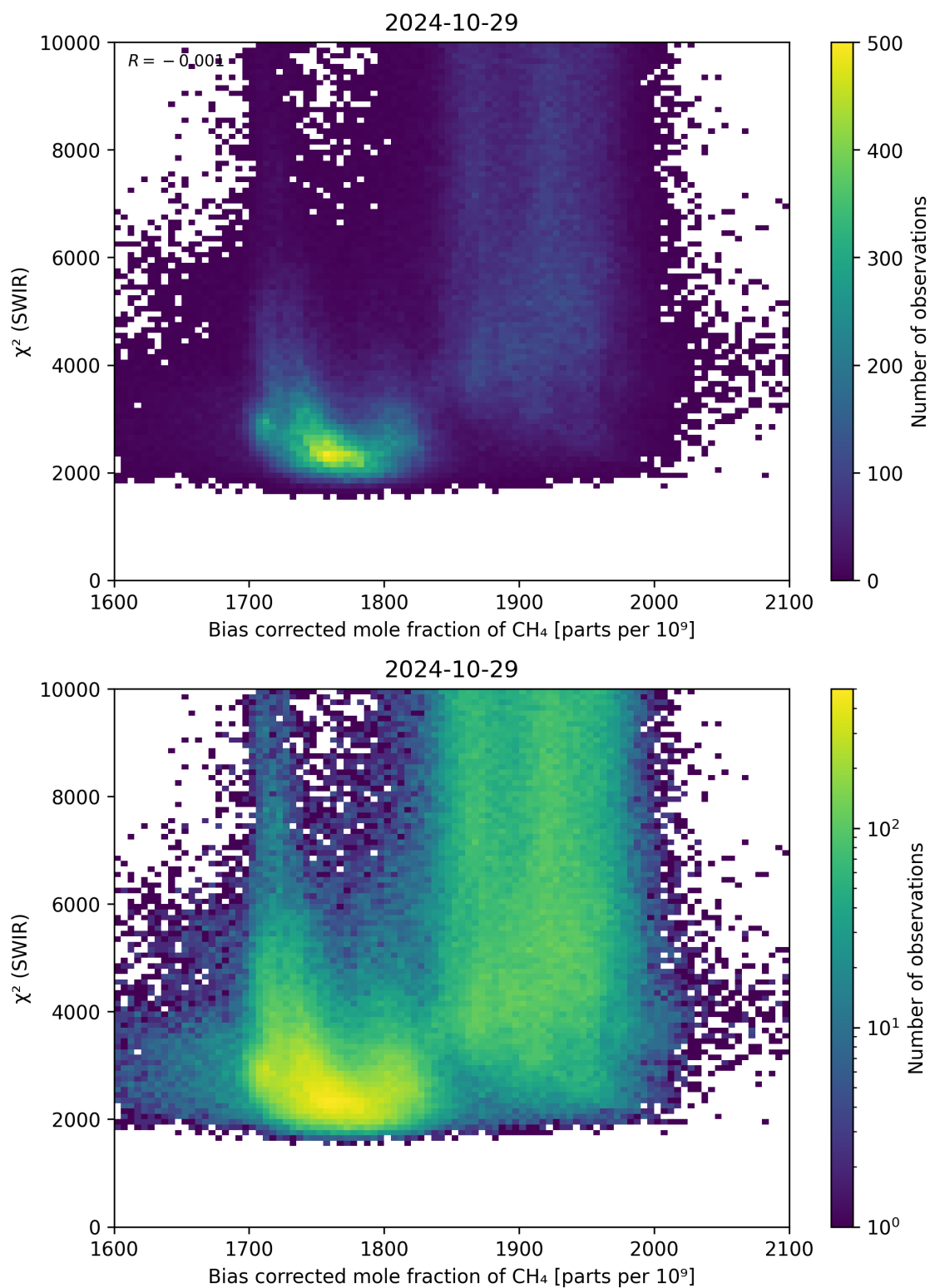
Figure 64: Scatter density plot of “Bias corrected mole fraction of \text{CH}_4 ” against “ \chi^2 (SWIR)” for 2024-10-29 to 2024-10-30.
