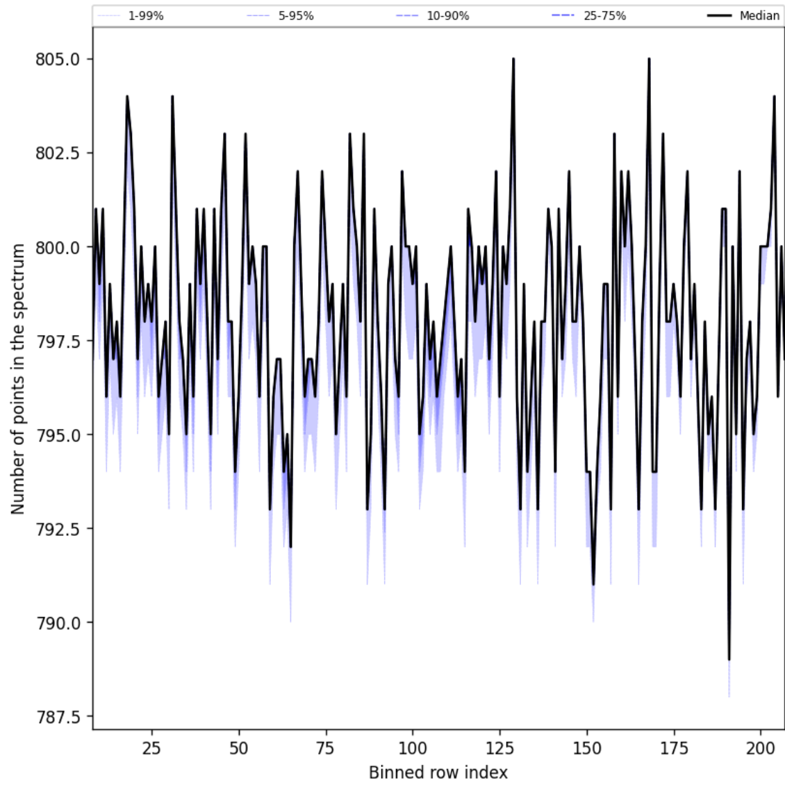
Figure 37: Along track statistics of “Number of points in the spectrum” for 2024-10-29 to 2024-10-30
