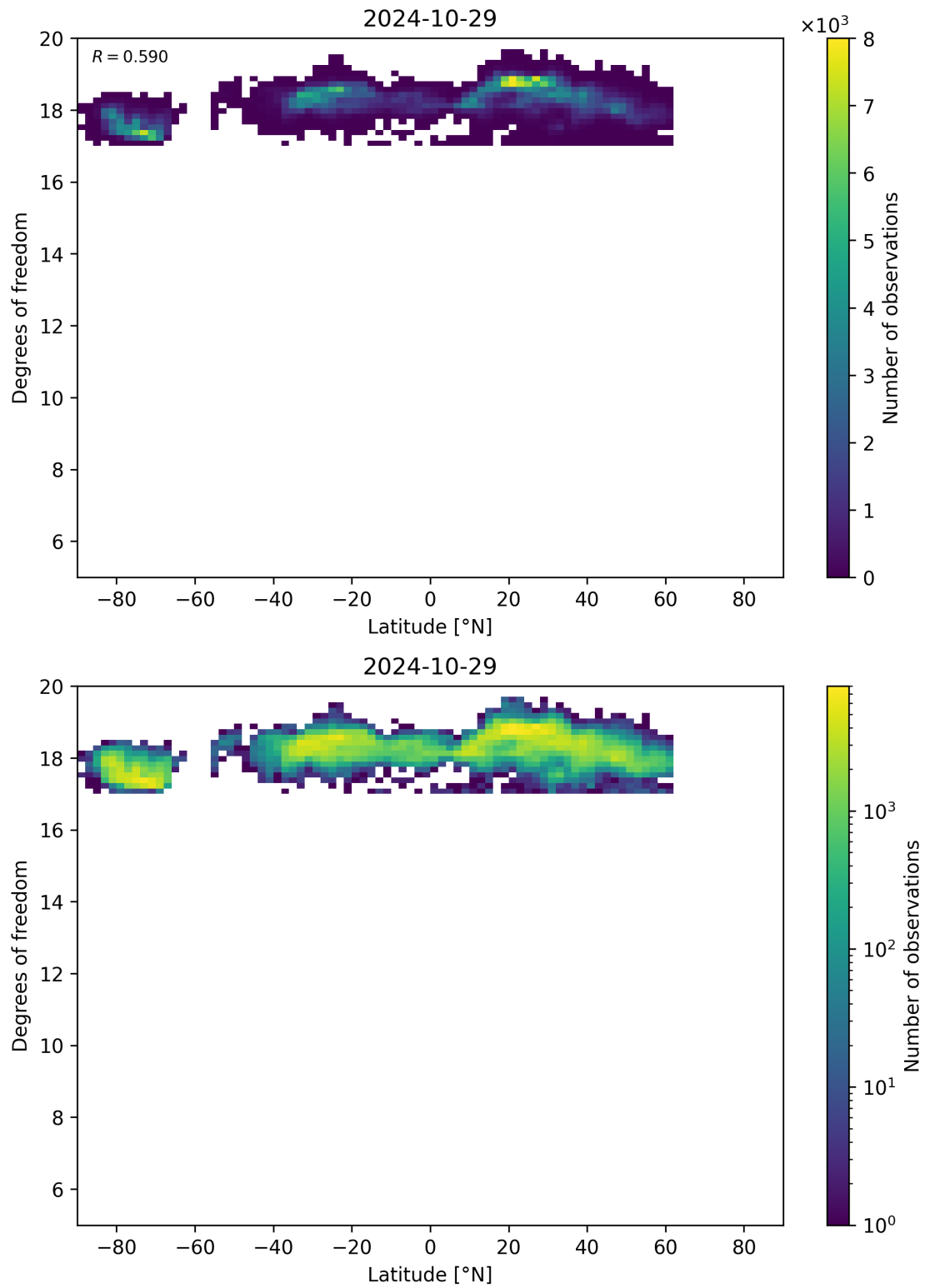
Figure 55: Scatter density plot of “Latitude” against “Degrees of freedom” for 2024-10-29 to 2024-10-30.
