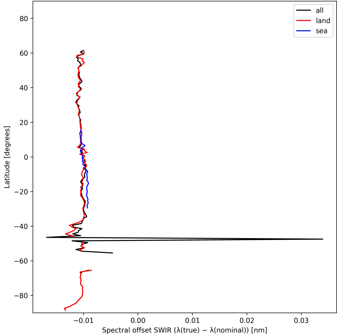
Figure 16: Zonal average of “Spectral offset SWIR ( \lambda_{\text{true}} - \lambda_{\text{nominal}} )” for 2024-10-29 to 2024-10-30.
