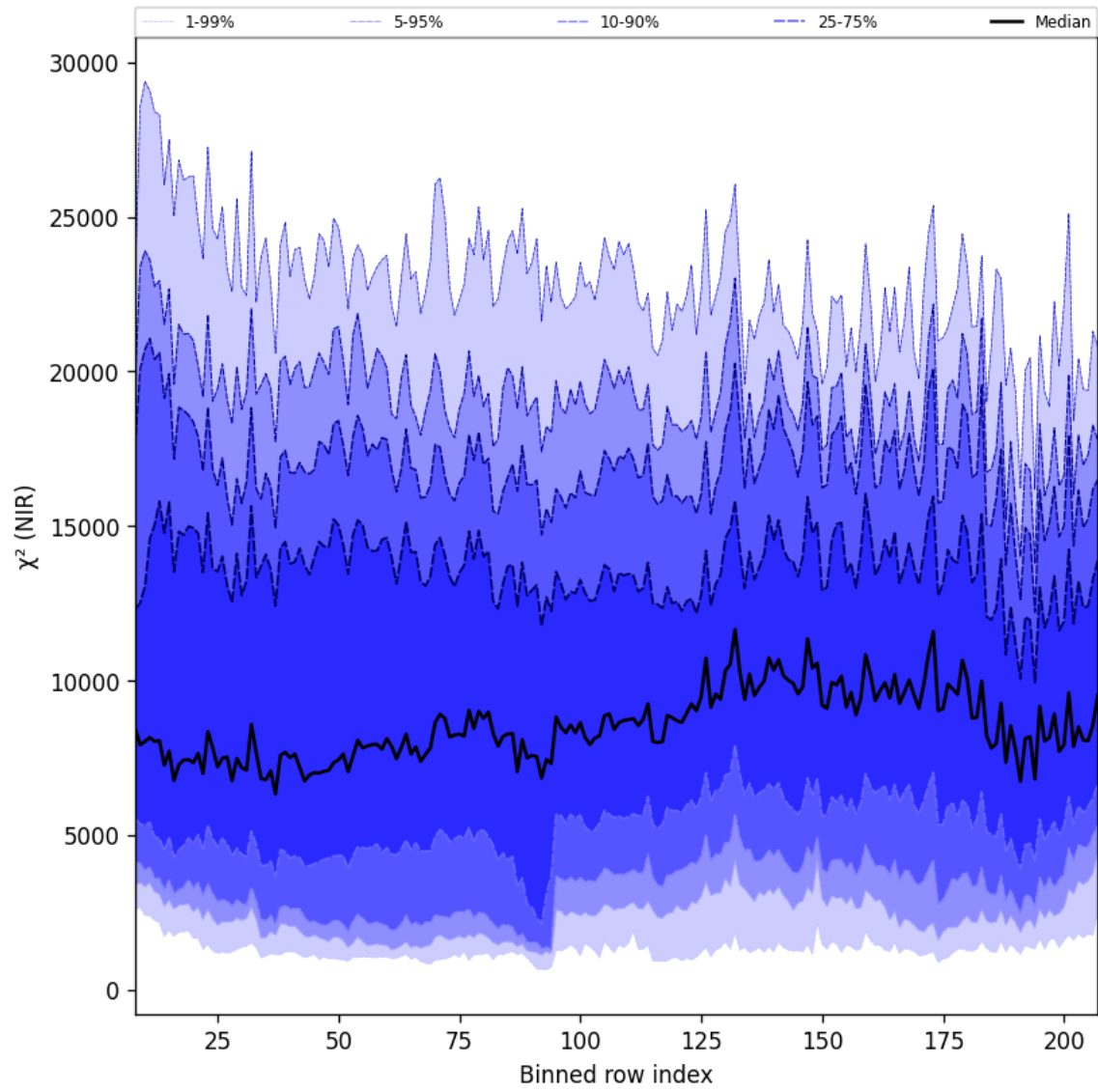
Figure 40: Along track statistics of “ \chi^2 (NIR)” for 2024-10-29 to 2024-10-30
