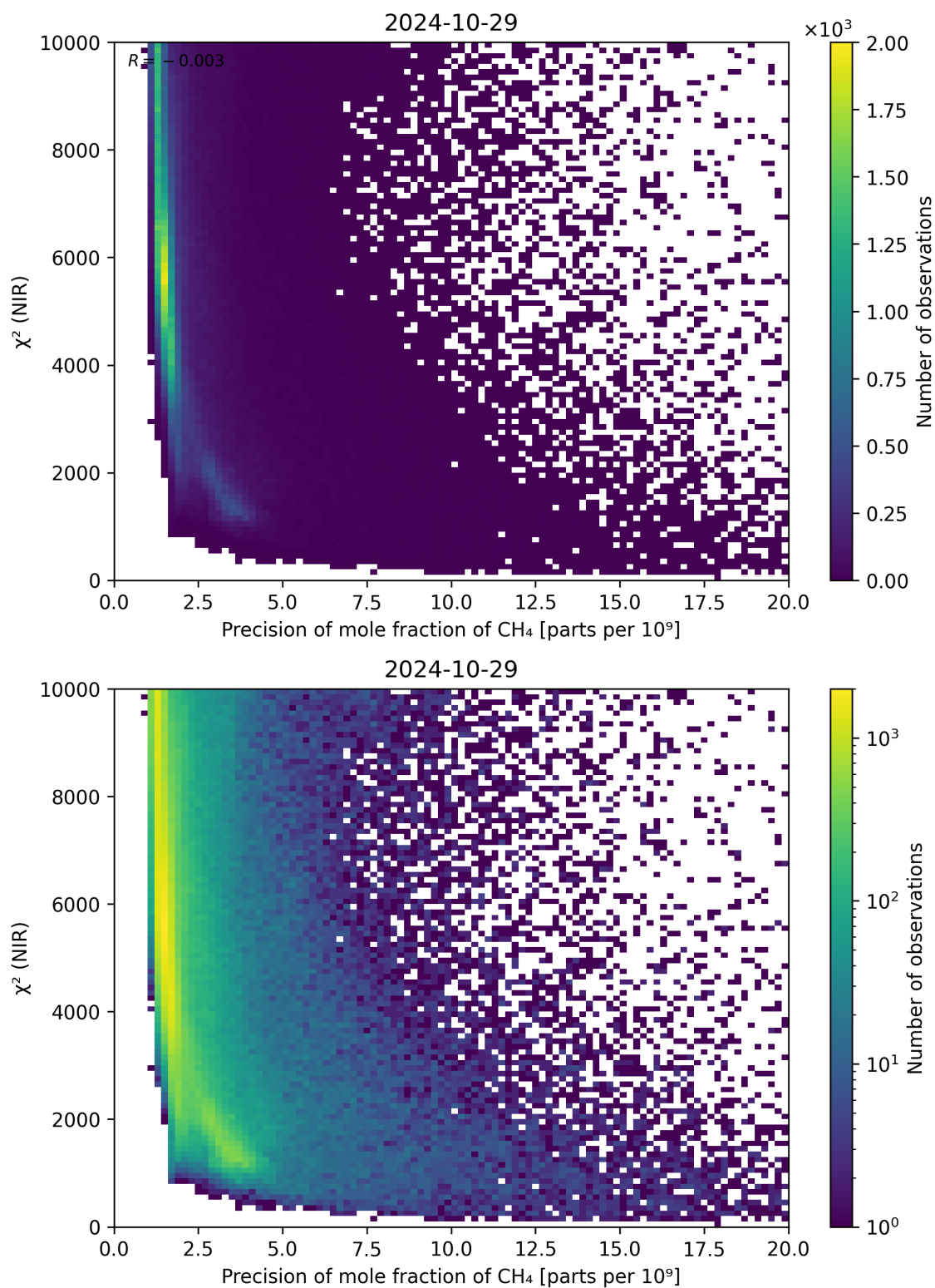
Figure 78: Scatter density plot of “Precision of mole fraction of CH 4 ” against “ \chi^2 (NIR)” for 2024-10-29 to 2024-10-30.
