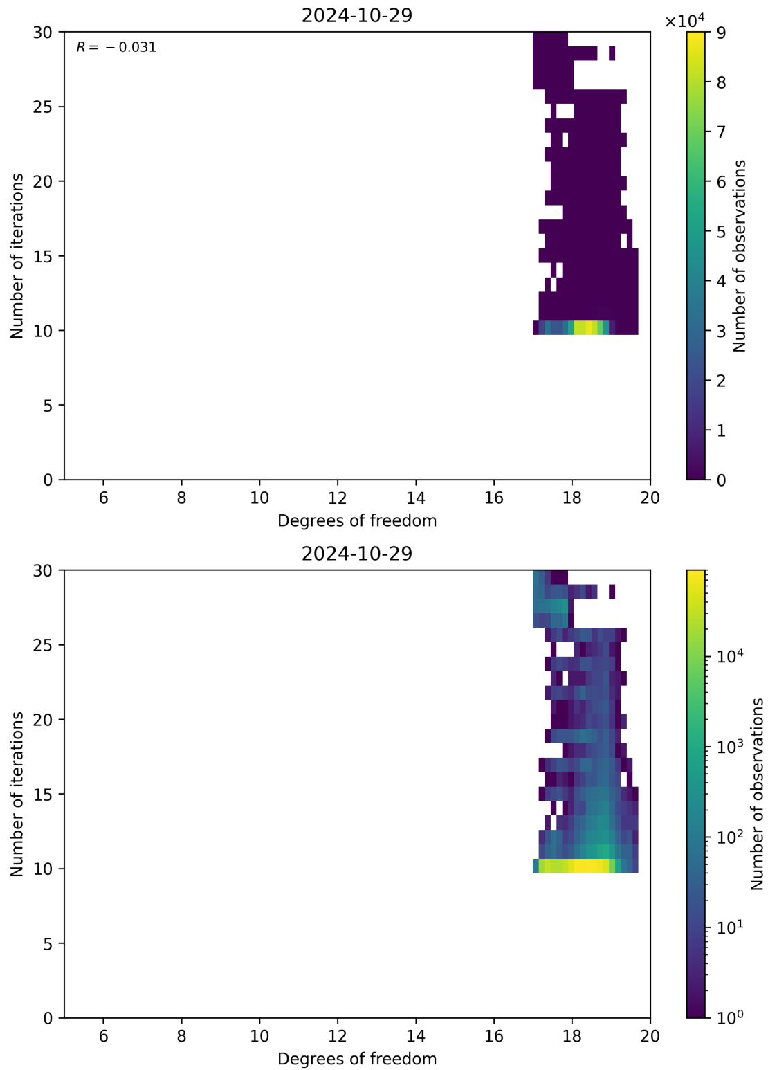
Figure 52: Scatter density plot of “Degrees of freedom” against “Number of iterations” for 2024-10-29 to 2024-10-30.
