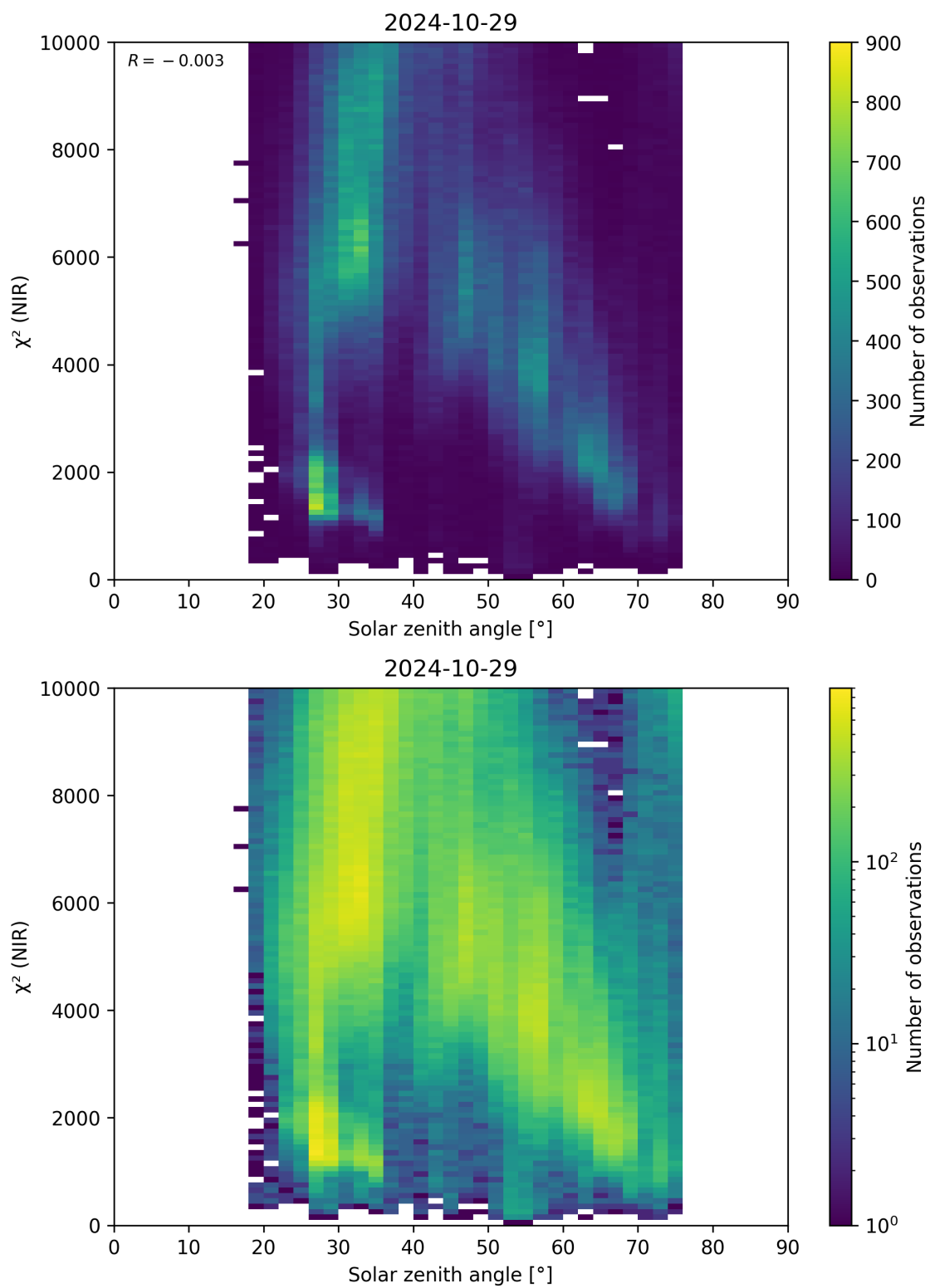
Figure 94: Scatter density plot of “Solar zenith angle” against “ \chi^2 (NIR)” for 2024-10-29 to 2024-10-30.
