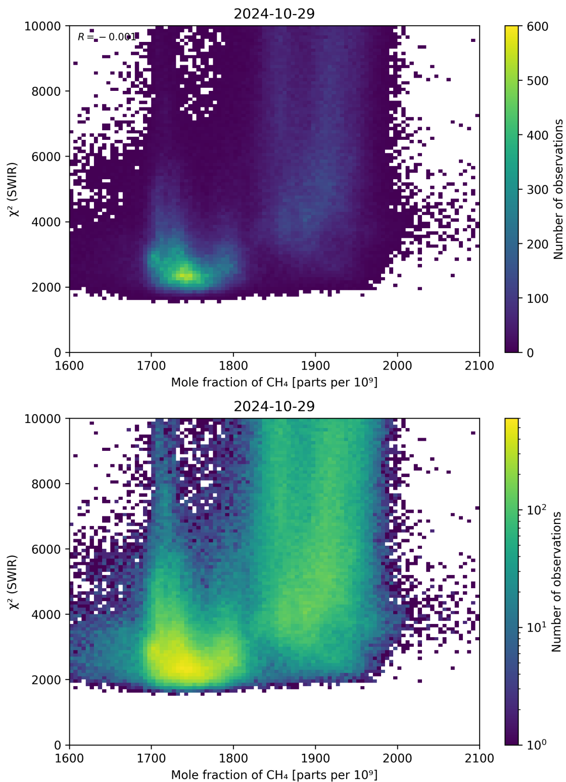
Figure 71: Scatter density plot of “Mole fraction of \text{CH}_4 ” against “ \chi^2 (SWIR)” for 2024-10-29 to 2024-10-30.
