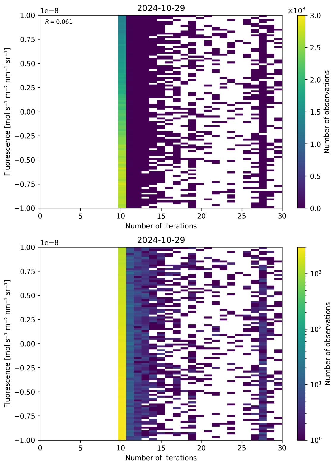
Figure 87: Scatter density plot of “Number of iterations” against “Fluorescence” for 2024-10-29 to 2024-10-30.
