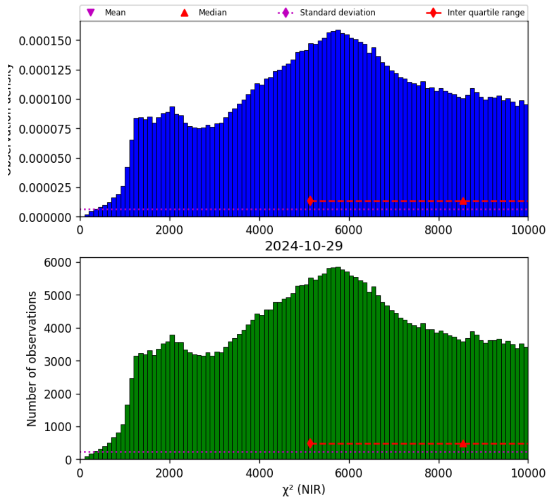
Figure 29: Histogram of “ \chi^2 (NIR)” for 2024-10-29 to 2024-10-30
