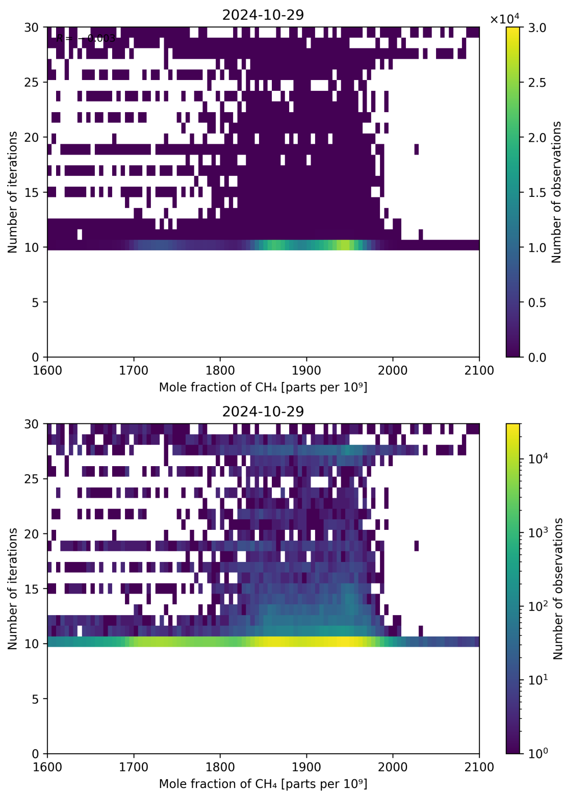
Figure 76: Scatter density plot of “Mole fraction of CH 4 ” against “Number of iterations” for 2024-10-29 to 2024-10-30.
