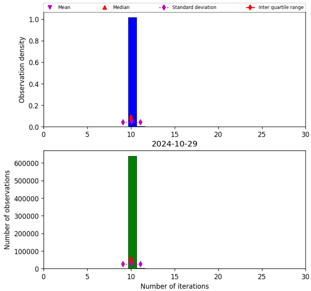
Figure 31: Histogram of “Number of iterations” for 2024-10-29 to 2024-10-30
