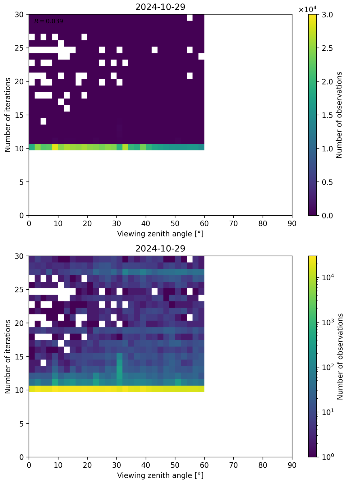
Figure 113: Scatter density plot of “Viewing zenith angle” against “Number of iterations” for 2024-10-29 to 2024-10-30.
