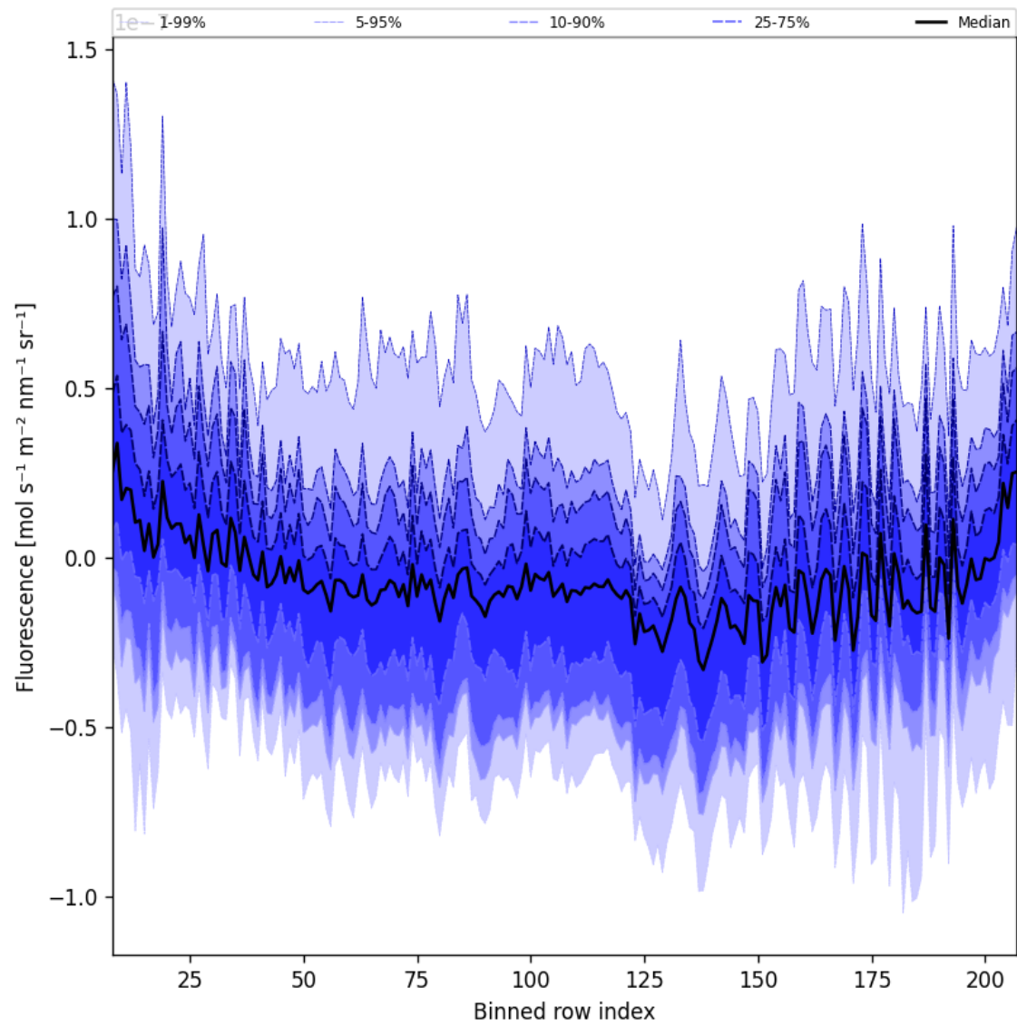
Figure 43: Along track statistics of “Fluorescence” for 2024-10-29 to 2024-10-30
