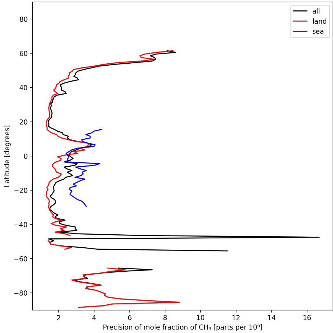
Figure 13: Zonal average of “Precision of mole fraction of CH 4 ” for 2024-10-29 to 2024-10-30.
