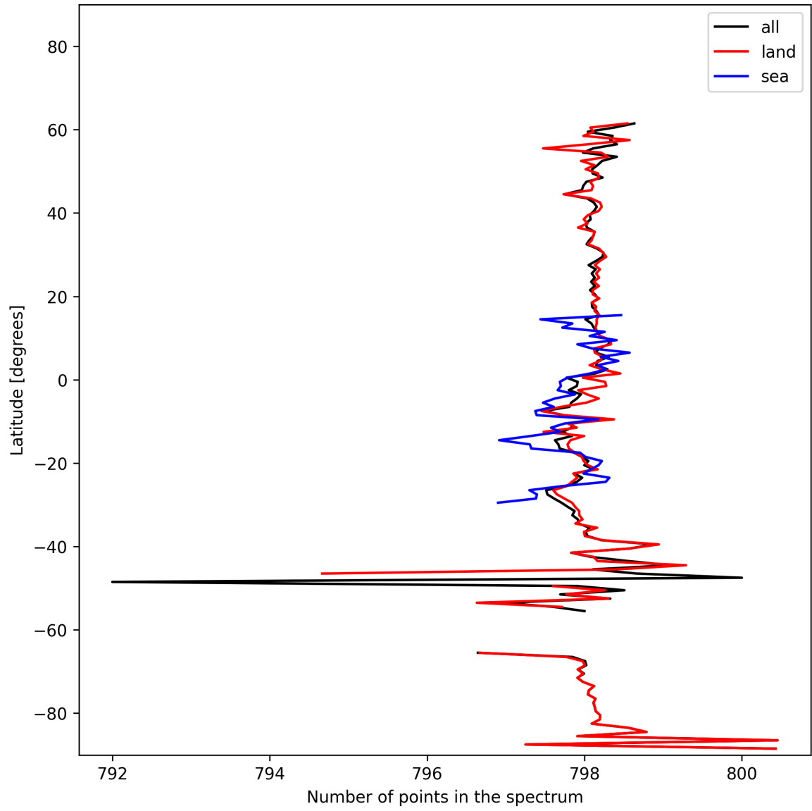
Figure 15: Zonal average of “Number of points in the spectrum” for 2024-10-29 to 2024-10-30.
