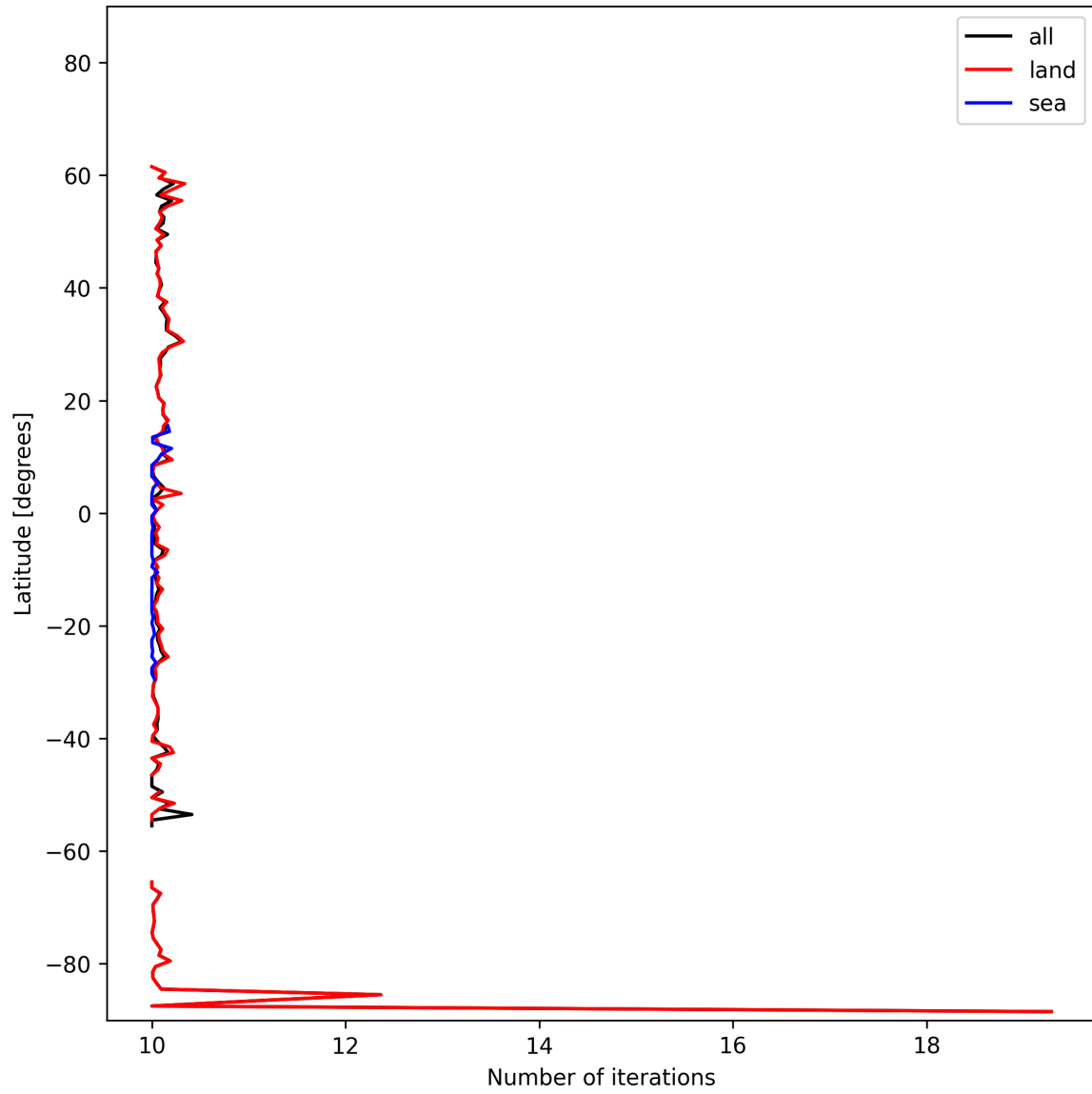
Figure 20: Zonal average of “Number of iterations” for 2024-10-29 to 2024-10-30.
