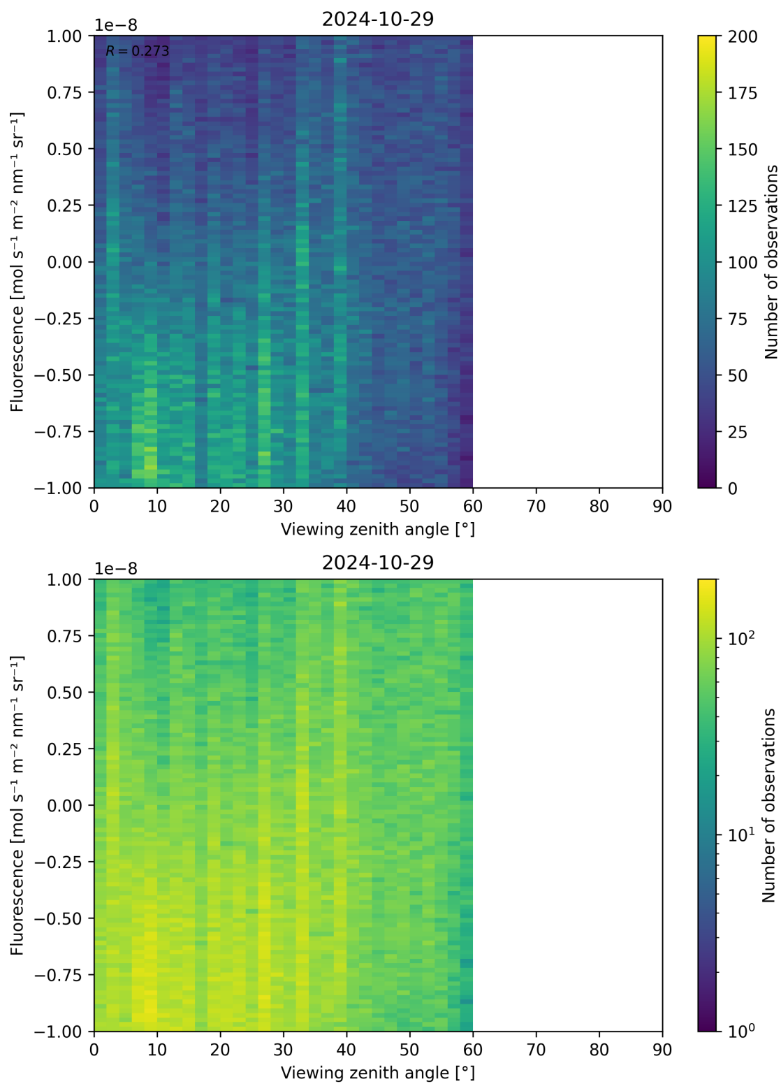
Figure 108: Scatter density plot of “Viewing zenith angle” against “Fluorescence” for 2024-10-29 to 2024-10-30.
