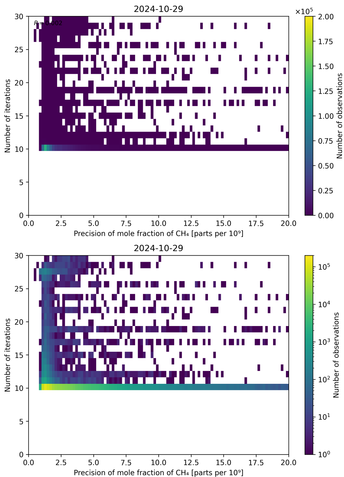
Figure 83: Scatter density plot of “Precision of mole fraction of CH 4 ” against “Number of iterations” for 2024-10-29 to 2024-10-30.
