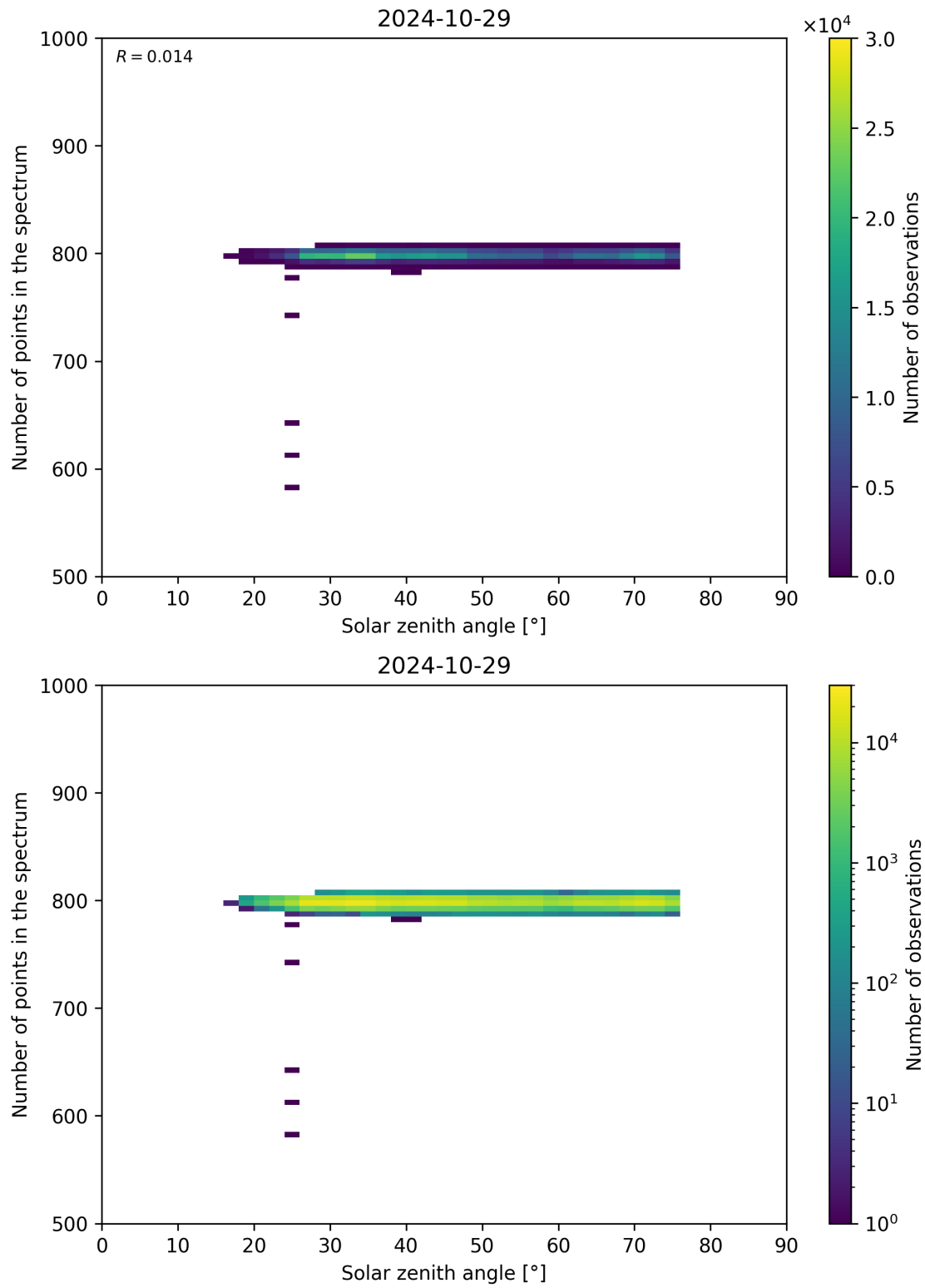
Figure 103: Scatter density plot of “Solar zenith angle” against “Number of points in the spectrum” for 2024-10-29 to 2024-10-30.
