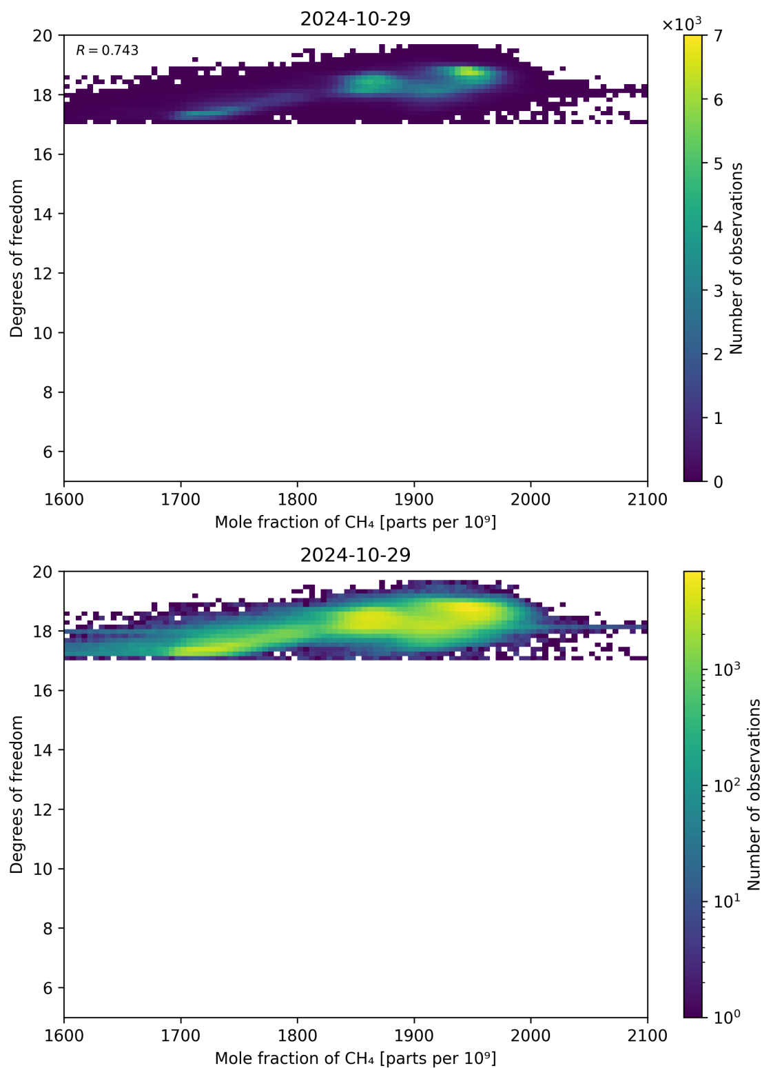
Figure 72: Scatter density plot of “Mole fraction of CH 4 ” against “Degrees of freedom” for 2024-10-29 to 2024-10-30.
