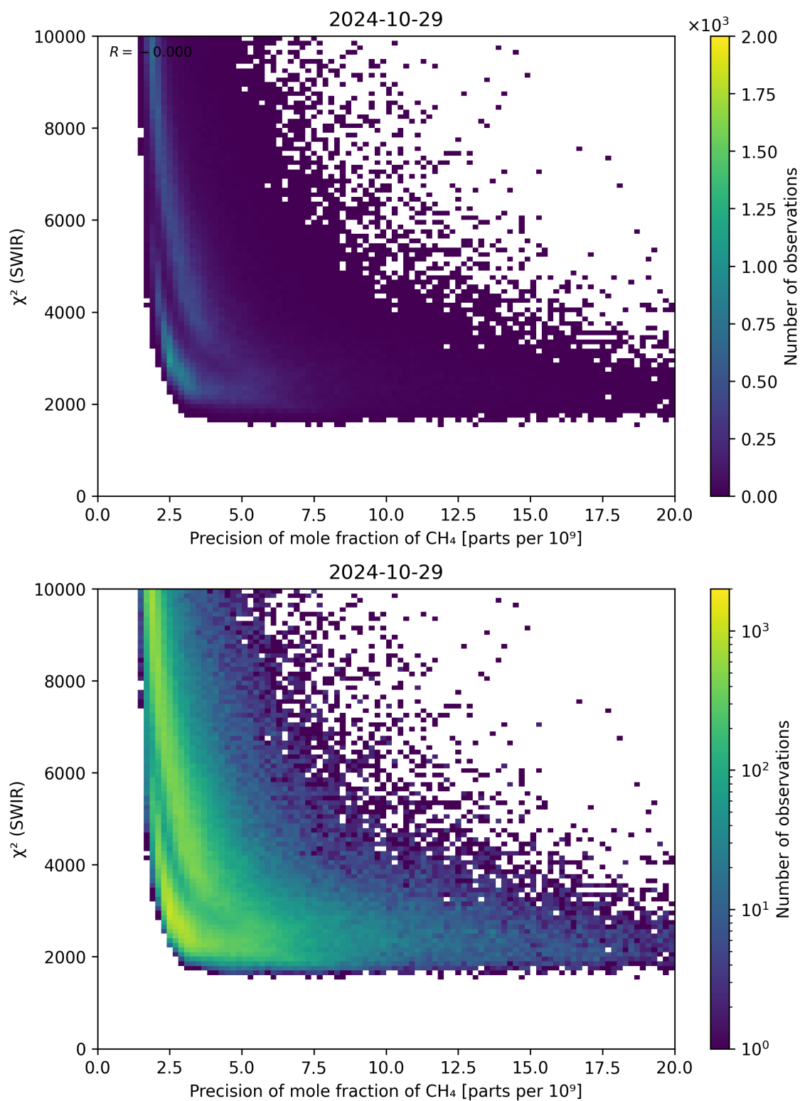
Figure 79: Scatter density plot of “Precision of mole fraction of \text{CH}_4 ” against “ \chi^2 (SWIR)” for 2024-10-29 to 2024-10-30.
