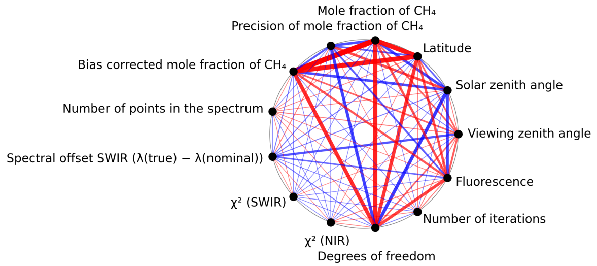
Figure 1: Map of correlation graph for 2024-10-29 to 2024-10-30.
