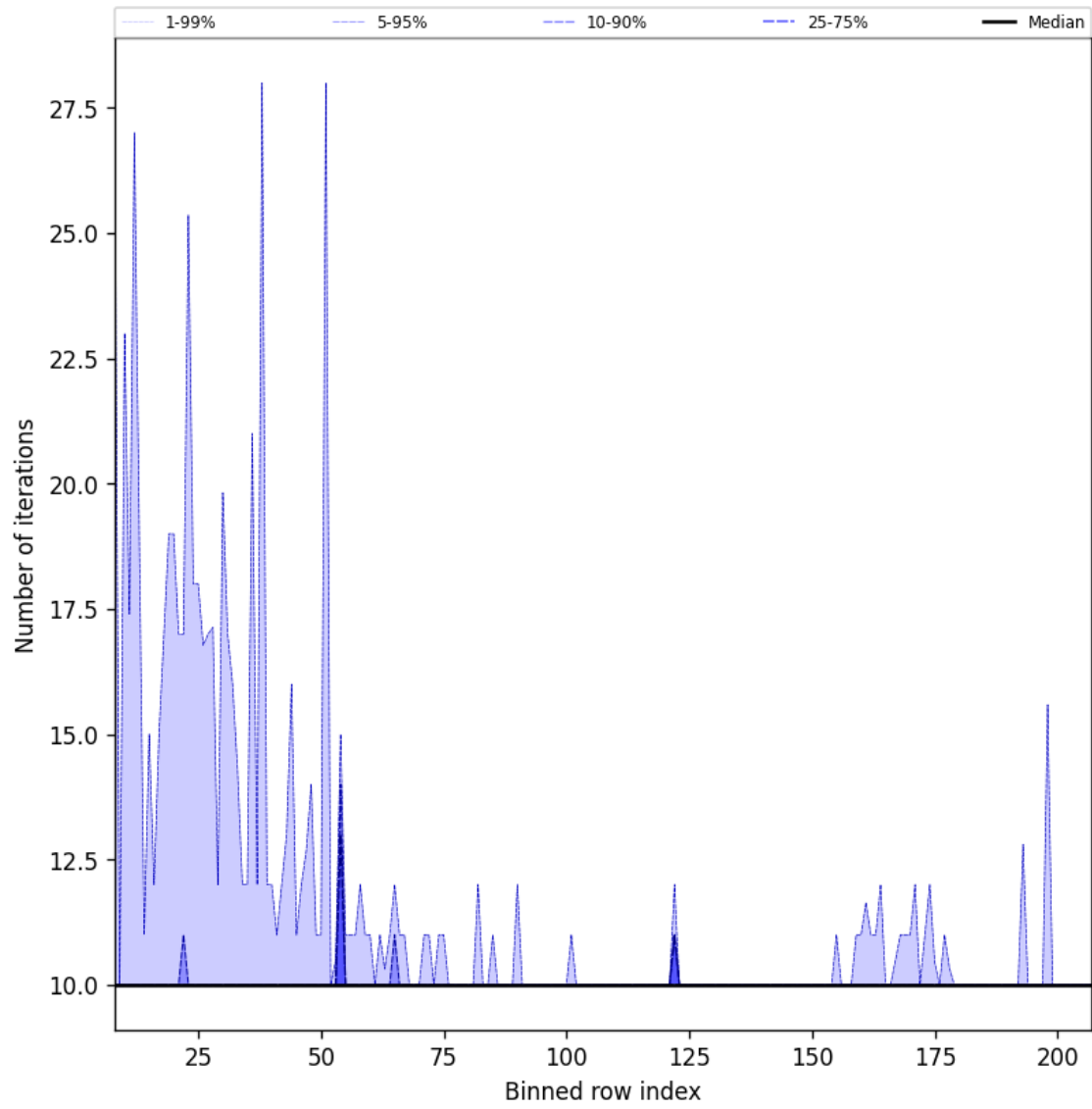
Figure 42: Along track statistics of “Number of iterations” for 2024-10-29 to 2024-10-30
