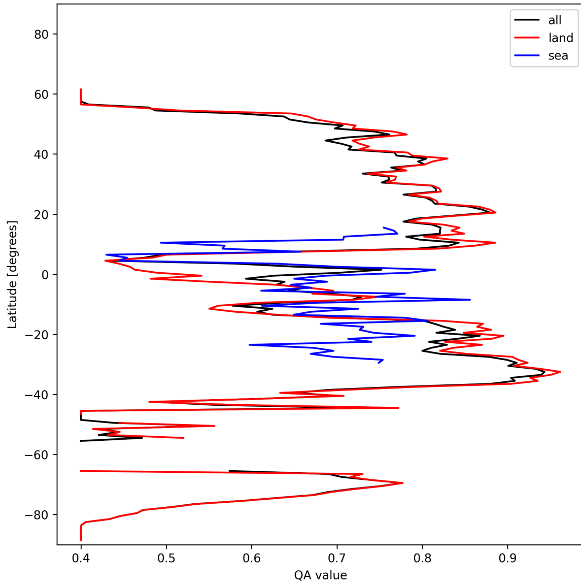
Figure 11: Zonal average of “QA value” for 2024-10-29 to 2024-10-30.
