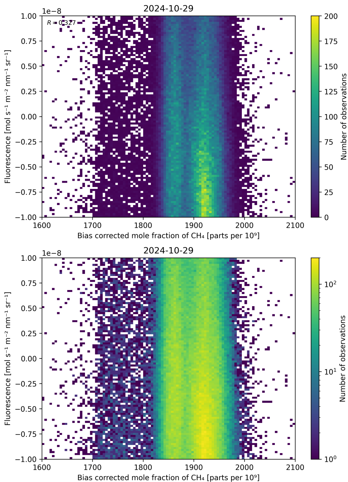
Figure 66: Scatter density plot of “Bias corrected mole fraction of \text{CH}_4 ” against “Fluorescence” for 2024-10-29 to 2024-10-30.
