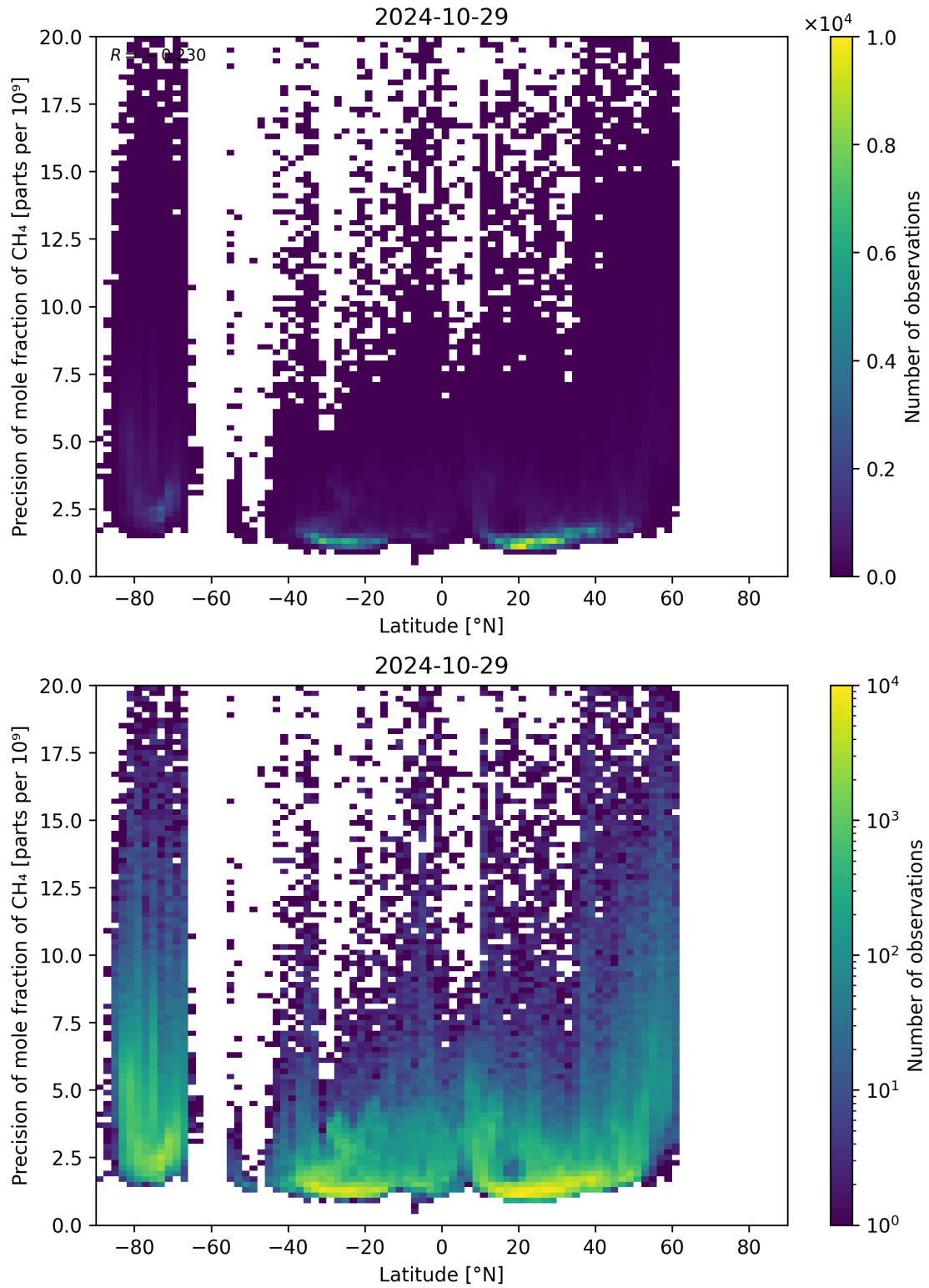
Figure 59: Scatter density plot of “Latitude” against “Precision of mole fraction of CH 4 ” for 2024-10-29 to 2024-10-30.
