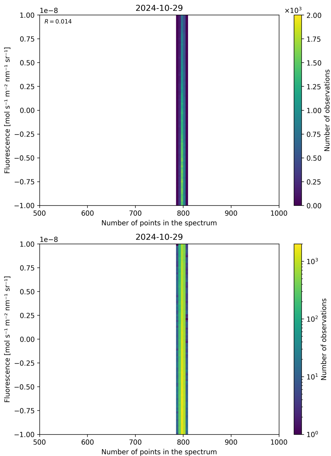
Figure 91: Scatter density plot of “Number of points in the spectrum” against “Fluorescence” for 2024-10-29 to 2024-10-30.
