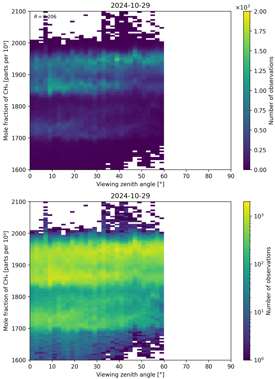
Figure 110: Scatter density plot of “Viewing zenith angle” against “Mole fraction of CH 4 ” for 2024-10-29 to 2024-10-30.
