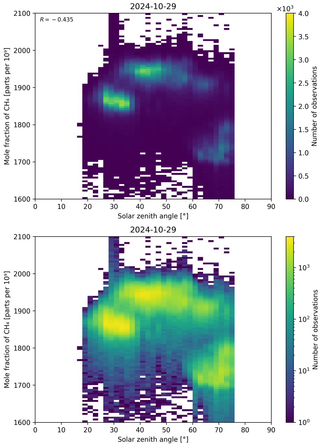
Figure 99: Scatter density plot of “Solar zenith angle” against “Mole fraction of CH 4 ” for 2024-10-29 to 2024-10-30.
