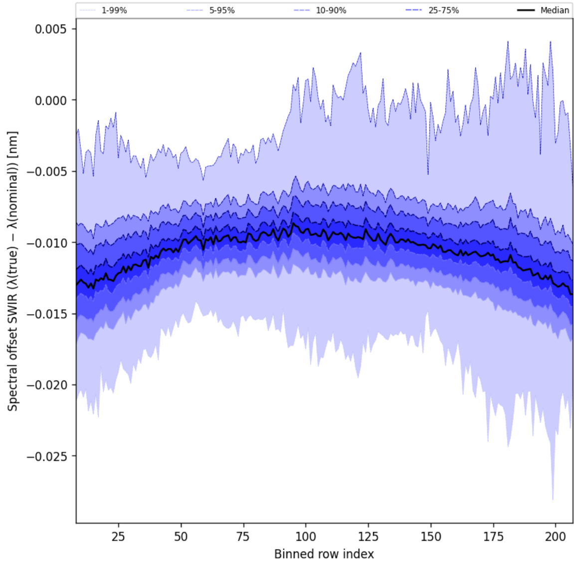
Figure 38: Along track statistics of “Spectral offset SWIR ( \lambda_{\text{true}} - \lambda_{\text{nominal}} )” for 2024-10-29 to 2024-10-30
