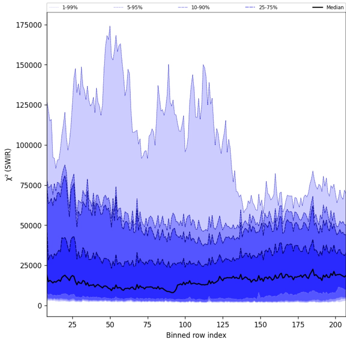
Figure 39: Along track statistics of “ \chi^2 (SWIR)” for 2024-10-29 to 2024-10-30
