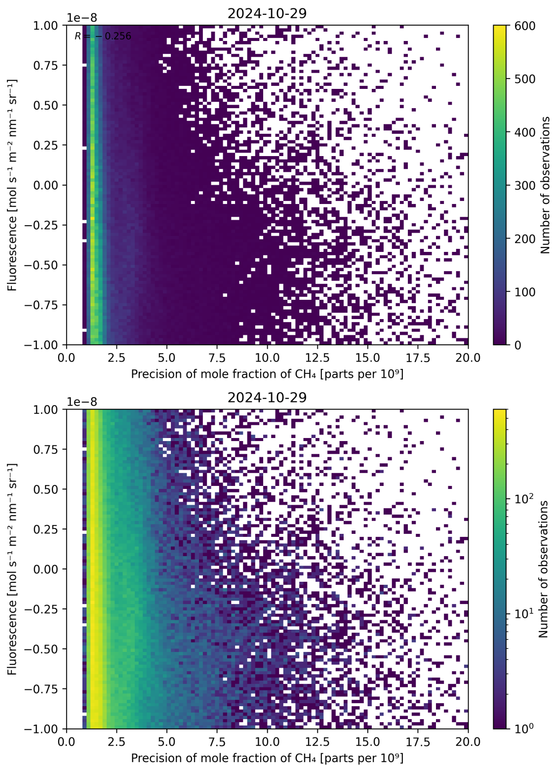
Figure 81: Scatter density plot of “Precision of mole fraction of CH 4 ” against “Fluorescence” for 2024-10-29 to 2024-10-30.
