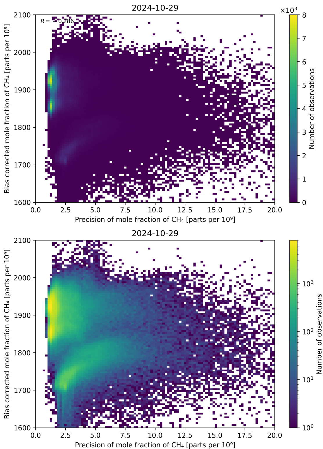
Figure 82: Scatter density plot of “Precision of mole fraction of CH 4 ” against “Bias corrected mole fraction of CH 4 ” for 2024-10-29 to 2024-10-30.
