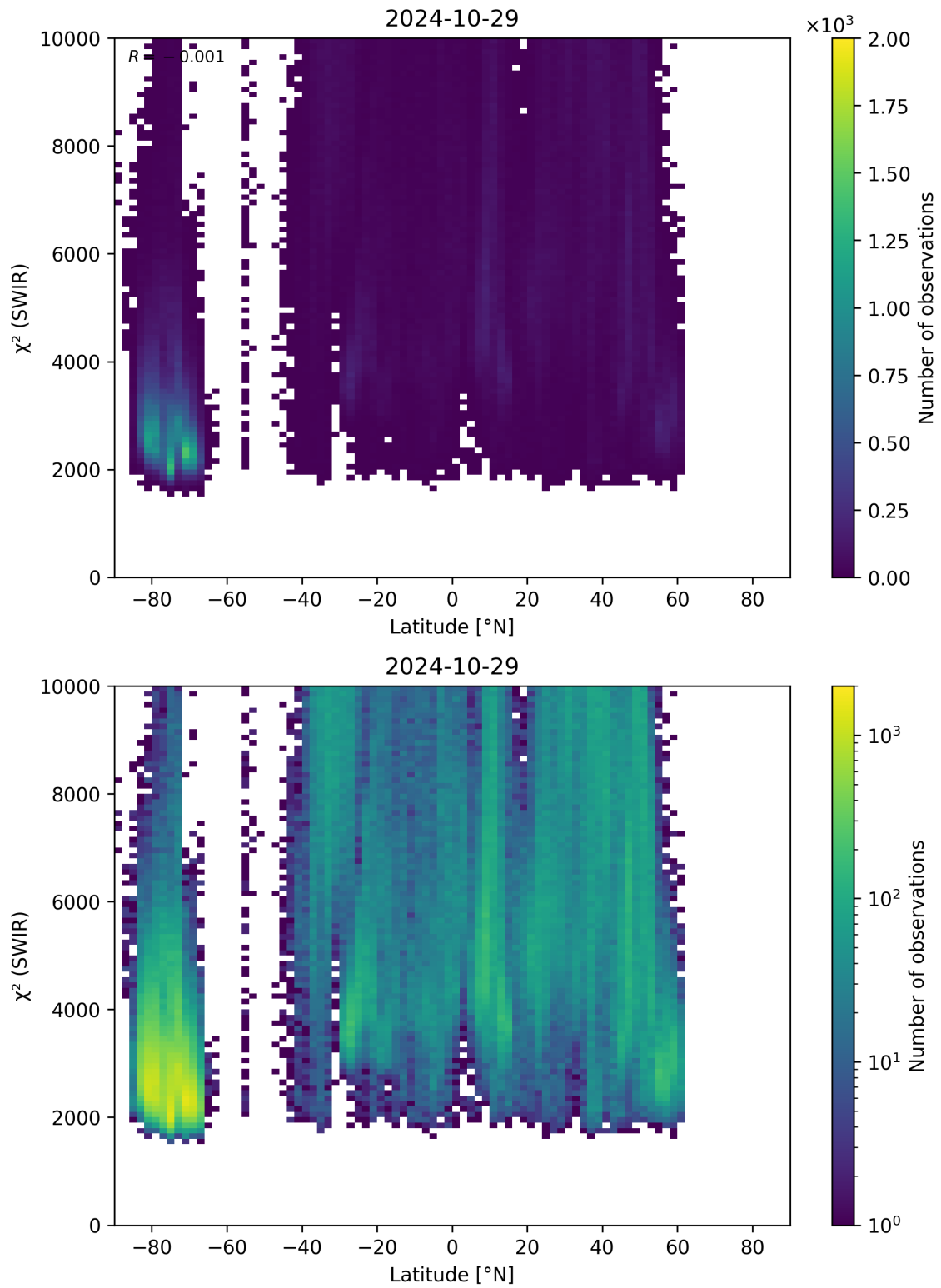
Figure 54: Scatter density plot of “Latitude” against “ \chi^2 (SWIR)” for 2024-10-29 to 2024-10-30.
