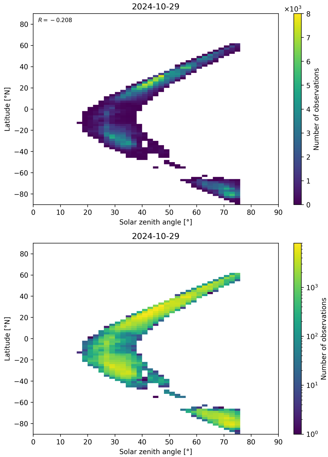
Figure 98: Scatter density plot of “Solar zenith angle” against “Latitude” for 2024-10-29 to 2024-10-30.
