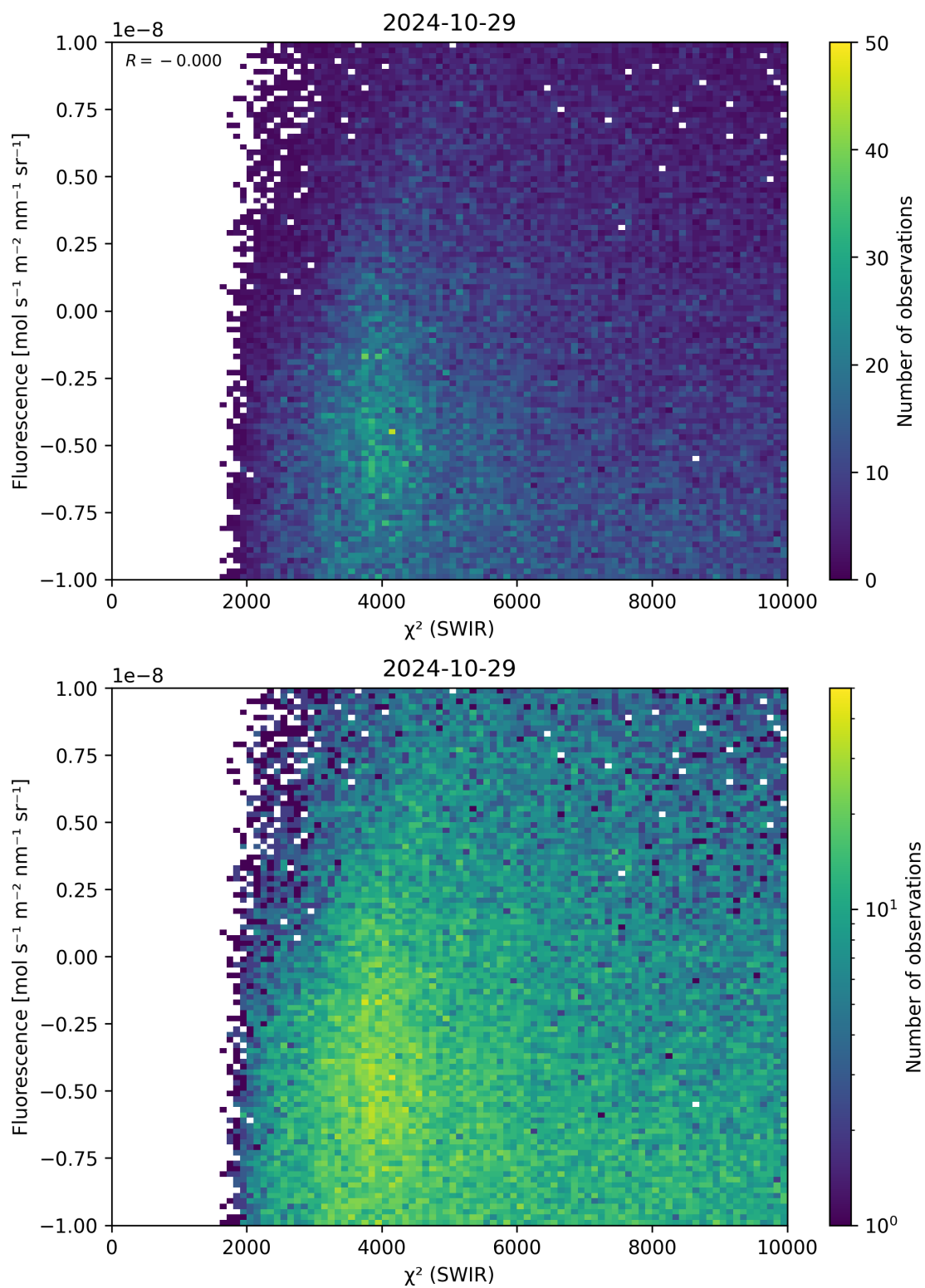
Figure 49: Scatter density plot of “ \chi^2 (SWIR)” against “Fluorescence” for 2024-10-29 to 2024-10-30.
