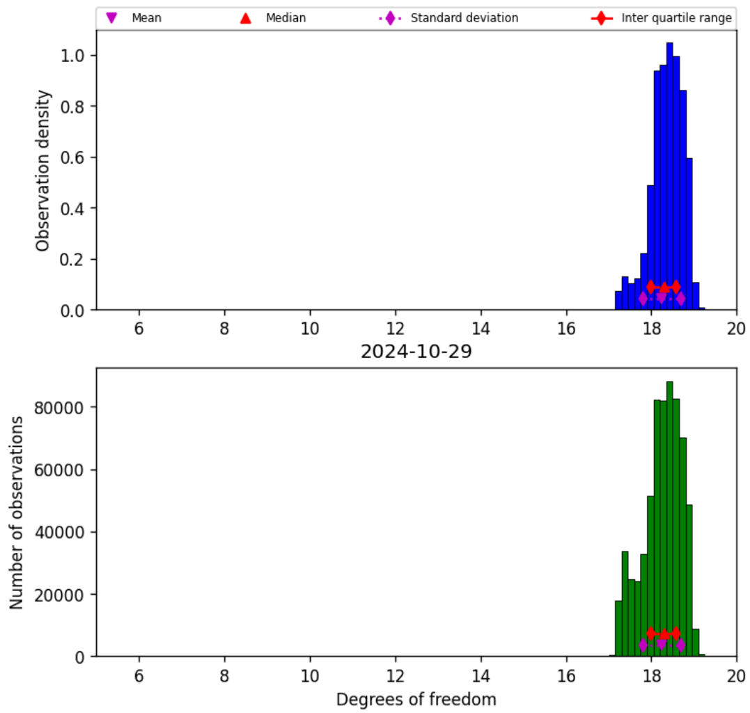
Figure 30: Histogram of “Degrees of freedom” for 2024-10-29 to 2024-10-30
