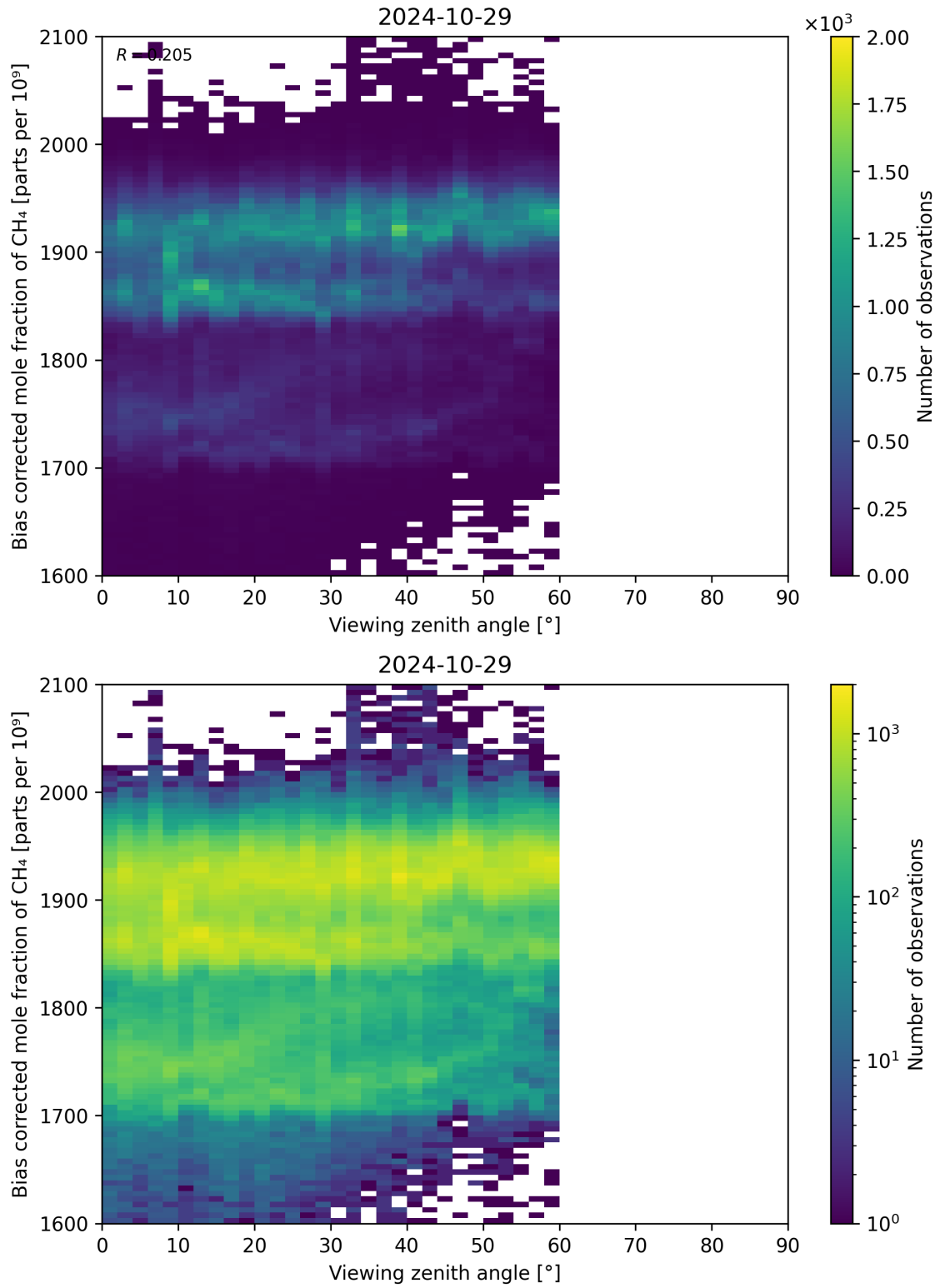
Figure 111: Scatter density plot of “Viewing zenith angle” against “Bias corrected mole fraction of CH 4 ” for 2024-10-29 to 2024-10-30.
