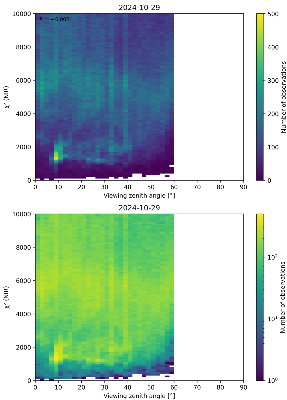
Figure 105: Scatter density plot of “Viewing zenith angle” against “ \chi^2 (NIR)” for 2024-10-29 to 2024-10-30.
