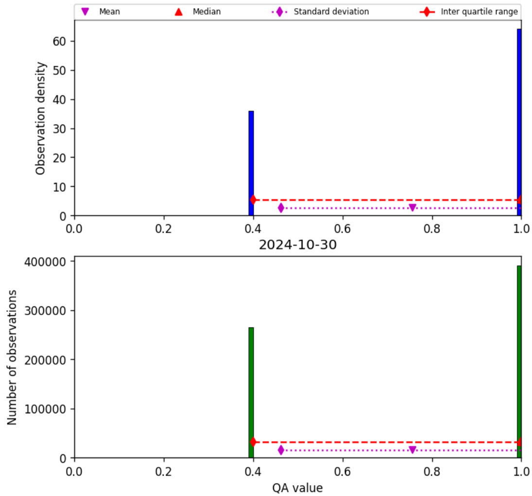
Figure 22: Histogram of “QA value” for 2024-10-30 to 2024-10-31
