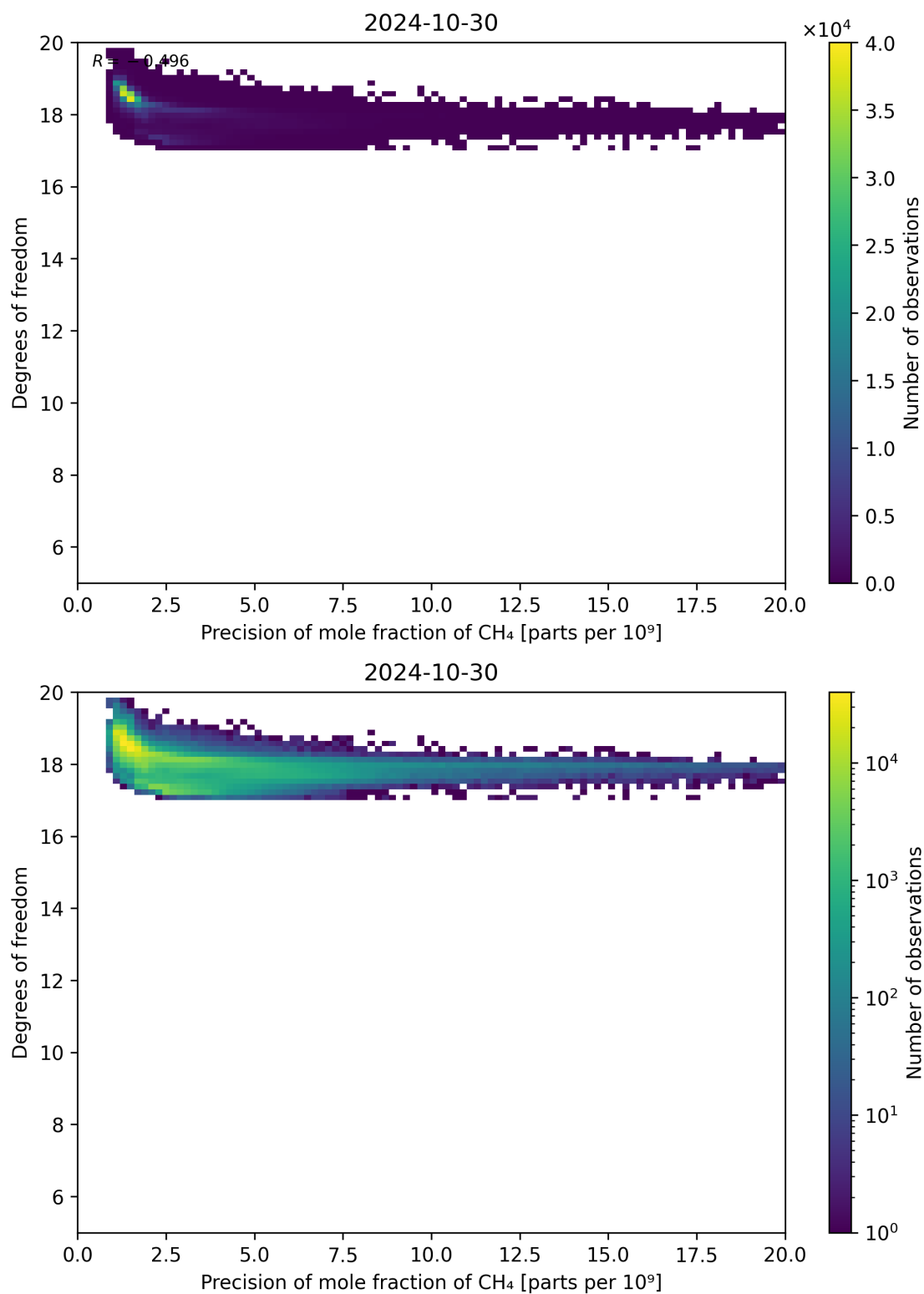
Figure 80: Scatter density plot of “Precision of mole fraction of CH 4 ” against “Degrees of freedom” for 2024-10-30 to 2024-10-31.
