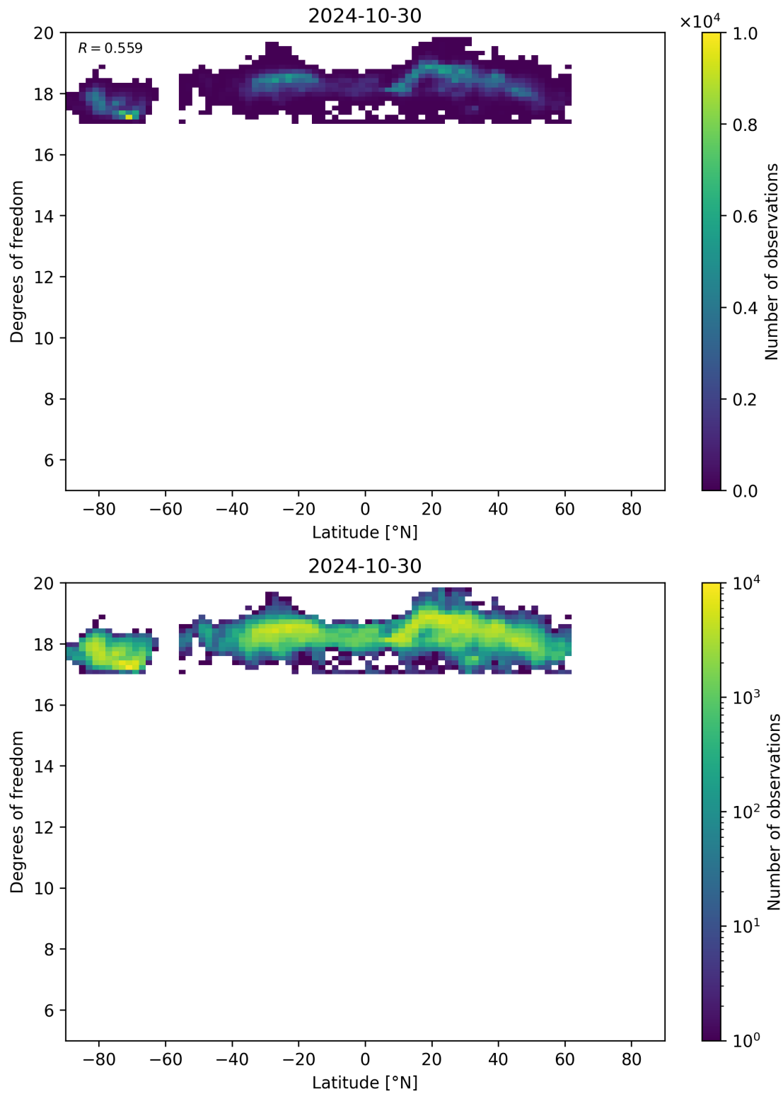
Figure 55: Scatter density plot of “Latitude” against “Degrees of freedom” for 2024-10-30 to 2024-10-31.
