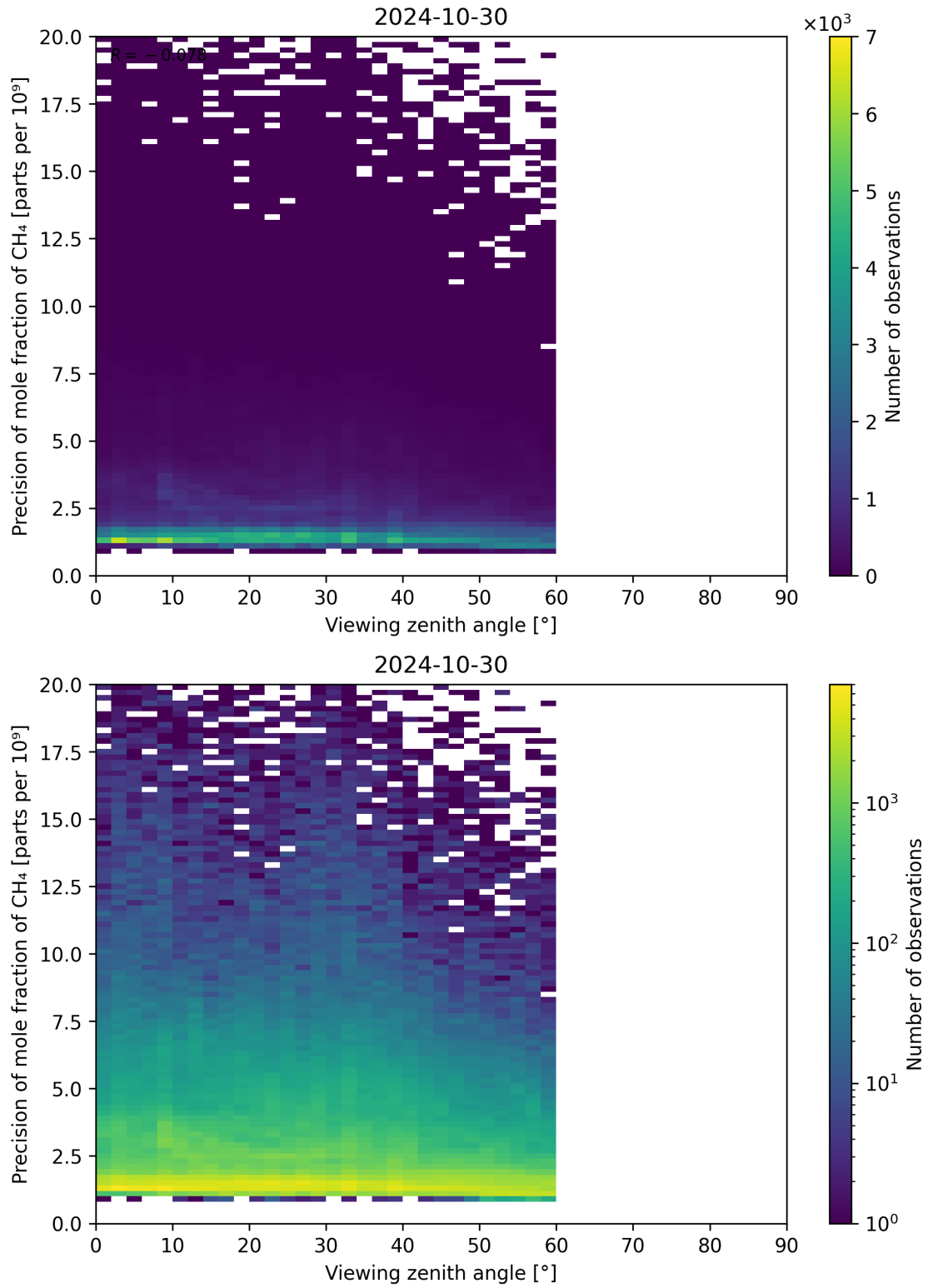
Figure 112: Scatter density plot of “Viewing zenith angle” against “Precision of mole fraction of CH 4 ” for 2024-10-30 to 2024-10-31.
