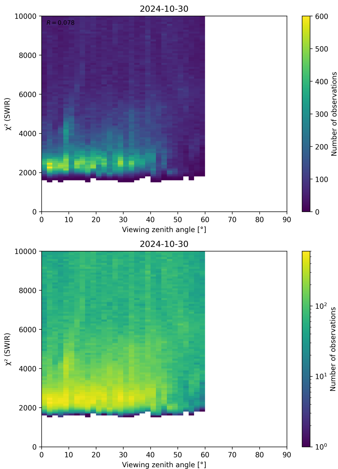
Figure 106: Scatter density plot of “Viewing zenith angle” against “ \chi^2 (SWIR)” for 2024-10-30 to 2024-10-31.
