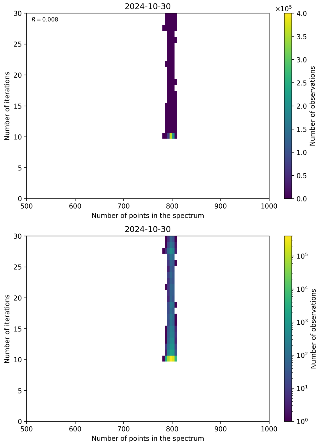
Figure 92: Scatter density plot of “Number of points in the spectrum” against “Number of iterations” for 2024-10-30 to 2024-10-31.
