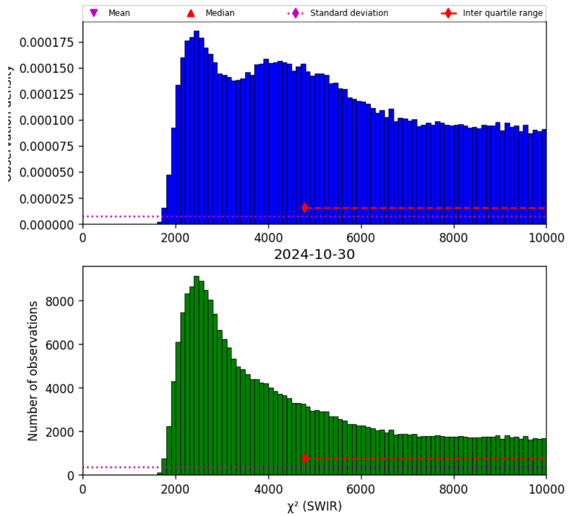
Figure 28: Histogram of “ \chi^2 (SWIR)” for 2024-10-30 to 2024-10-31
