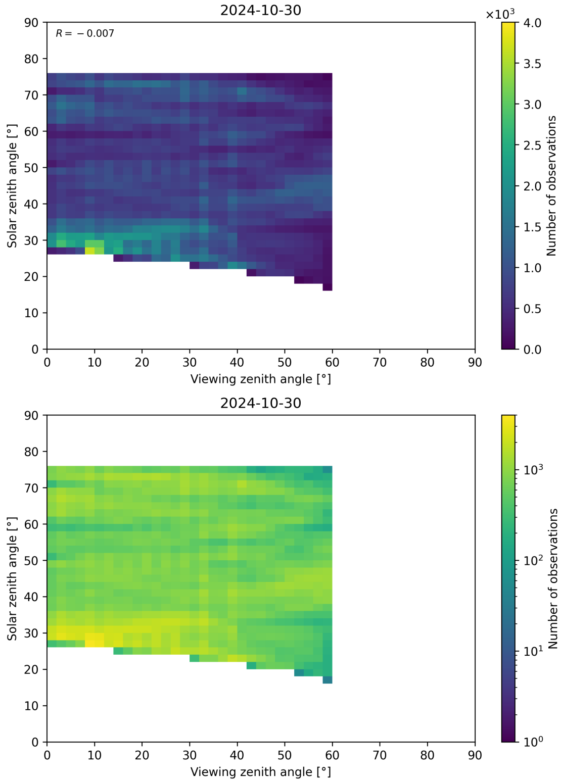
Figure 115: Scatter density plot of “Viewing zenith angle” against “Solar zenith angle” for 2024-10-30 to 2024-10-31.
