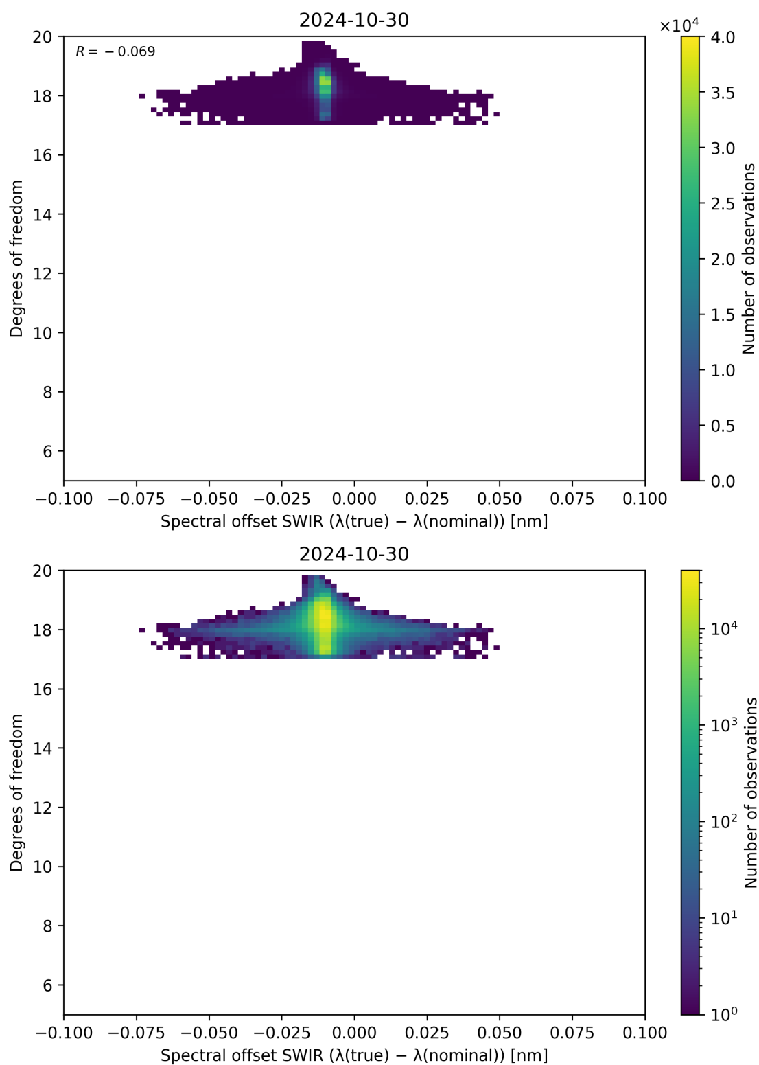
Figure 119: Scatter density plot of “Spectral offset SWIR ( \lambda_{\text{true}} - \lambda_{\text{nominal}} )” against “Degrees of freedom” for 2024-10-30 to 2024-10-31.
