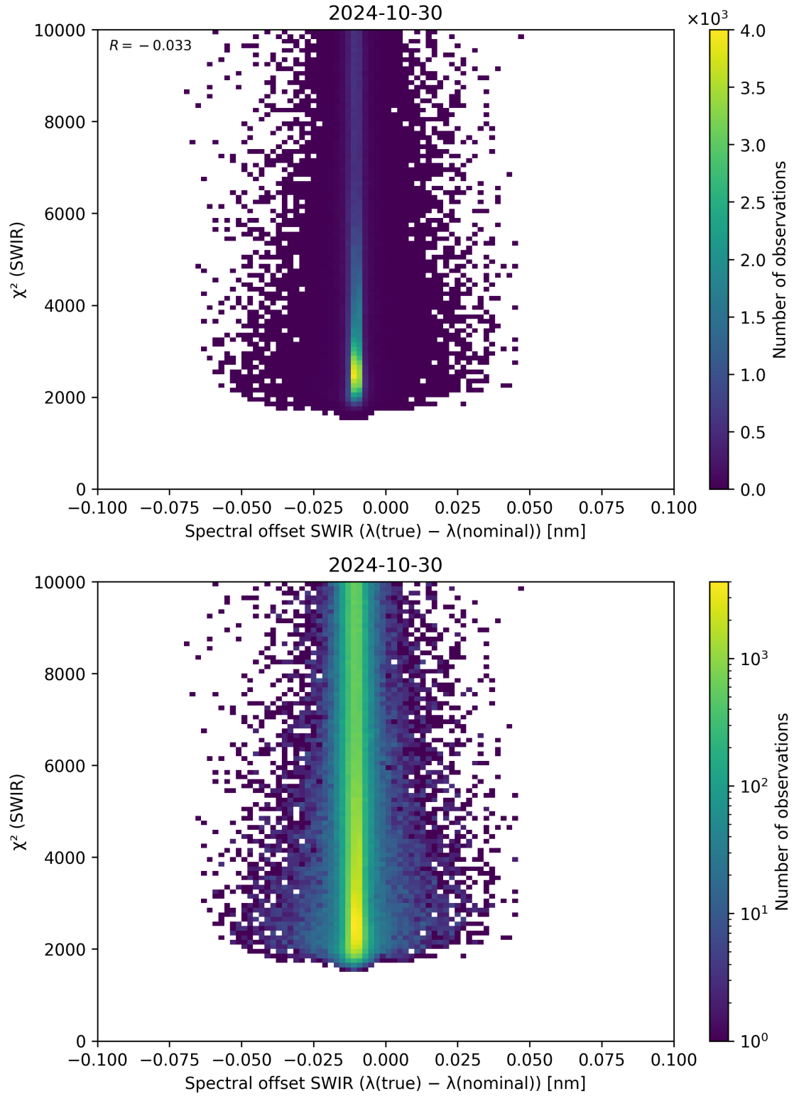
Figure 118: Scatter density plot of “Spectral offset SWIR ( \lambda_{\text{true}} - \lambda_{\text{nominal}} )” against “ \chi^2 (SWIR)” for 2024-10-30 to 2024-10-31.
