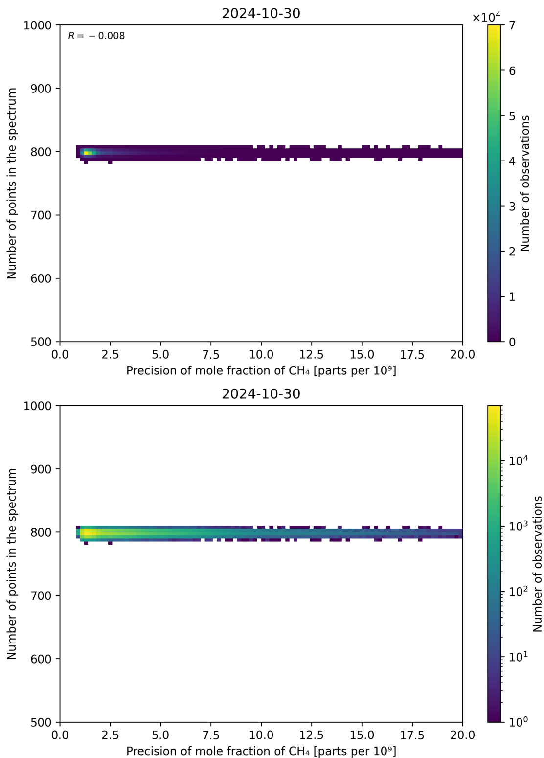
Figure 84: Scatter density plot of “Precision of mole fraction of CH 4 ” against “Number of points in the spectrum” for 2024-10-30 to 2024-10-31.
