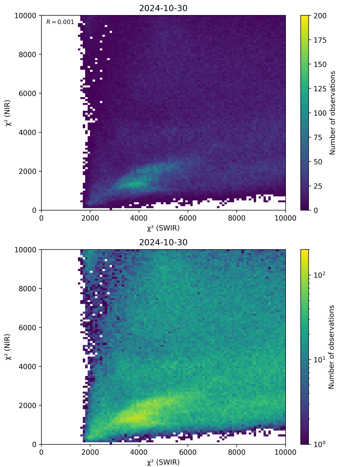
Figure 47: Scatter density plot of “ \chi^2 (SWIR)” against “ \chi^2 (NIR)” for 2024-10-30 to 2024-10-31.
