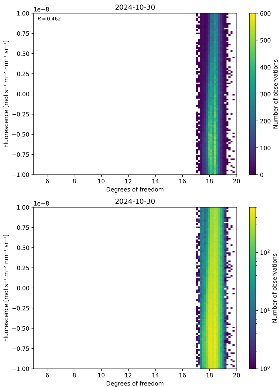
Figure 51: Scatter density plot of “Degrees of freedom” against “Fluorescence” for 2024-10-30 to 2024-10-31.
