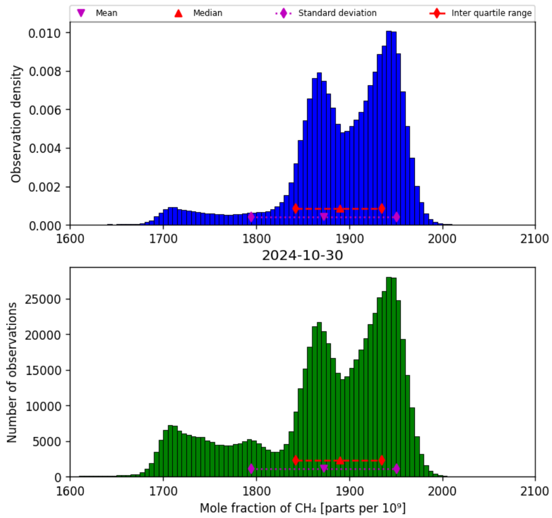
Figure 23: Histogram of “Mole fraction of CH 4 ” for 2024-10-30 to 2024-10-31
