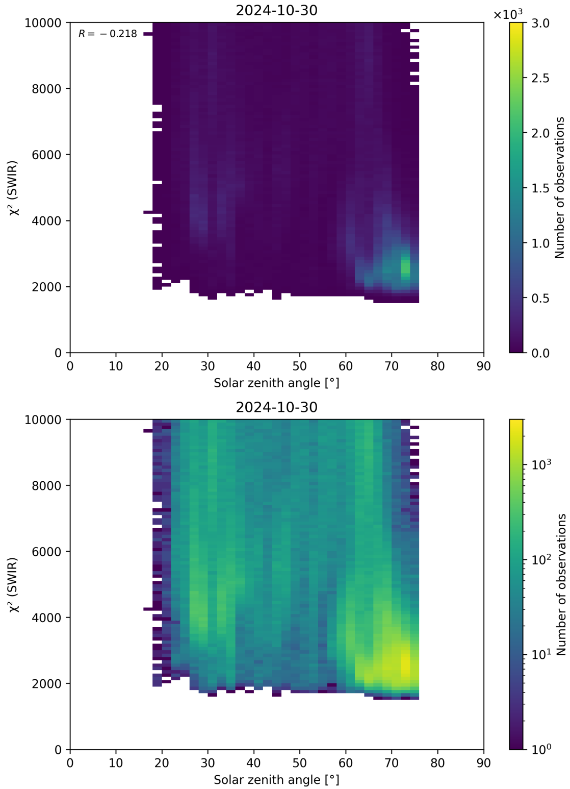
Figure 95: Scatter density plot of “Solar zenith angle” against “ \chi^2 (SWIR)” for 2024-10-30 to 2024-10-31.
