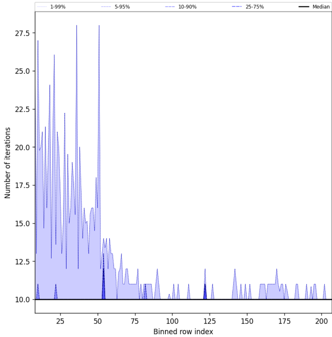
Figure 42: Along track statistics of “Number of iterations” for 2024-10-30 to 2024-10-31
