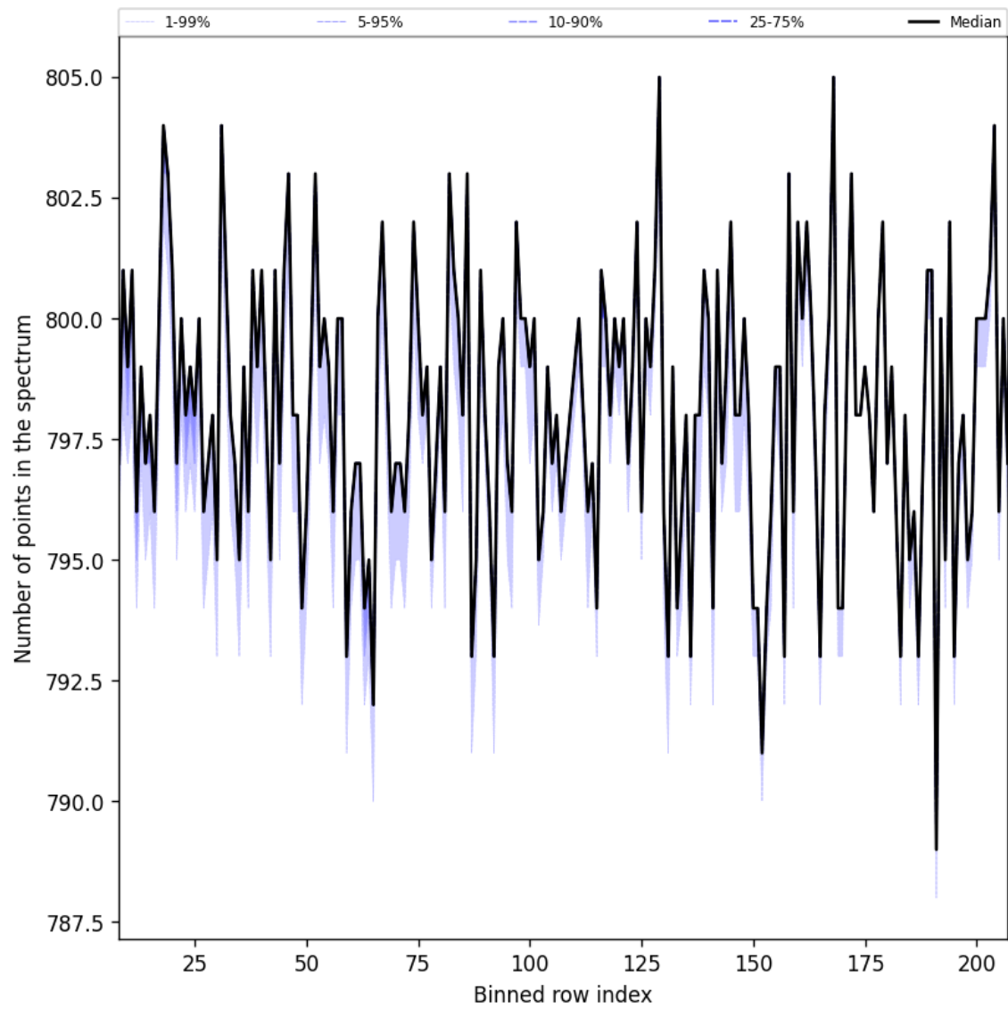
Figure 37: Along track statistics of “Number of points in the spectrum” for 2024-10-30 to 2024-10-31
