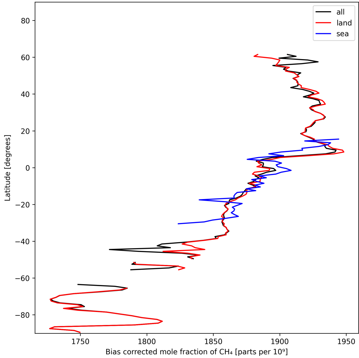
Figure 14: Zonal average of “Bias corrected mole fraction of CH 4 ” for 2024-10-30 to 2024-10-31.
