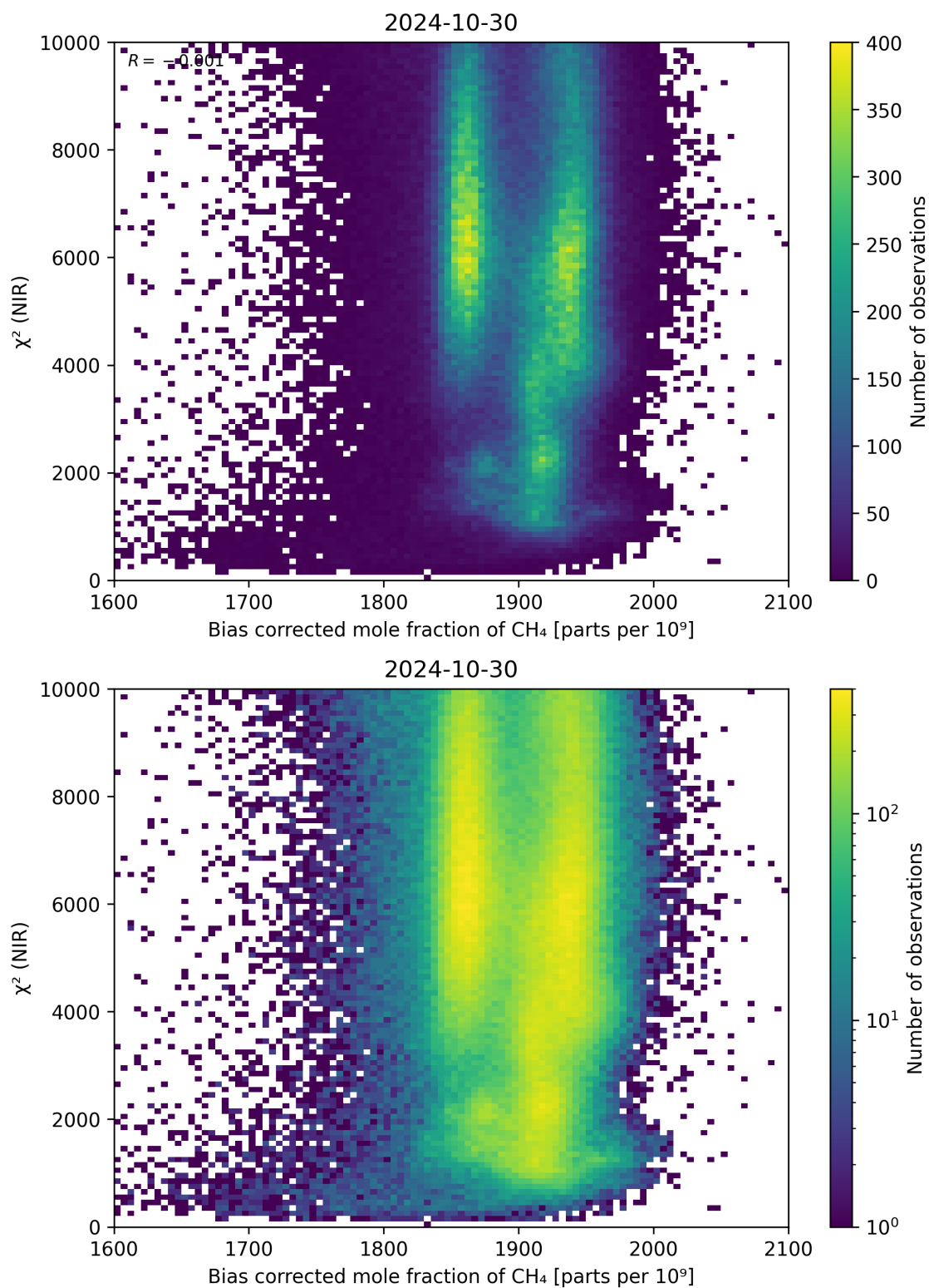
Figure 63: Scatter density plot of “Bias corrected mole fraction of \text{CH}_4 ” against “ \chi^2 (NIR)” for 2024-10-30 to 2024-10-31.
