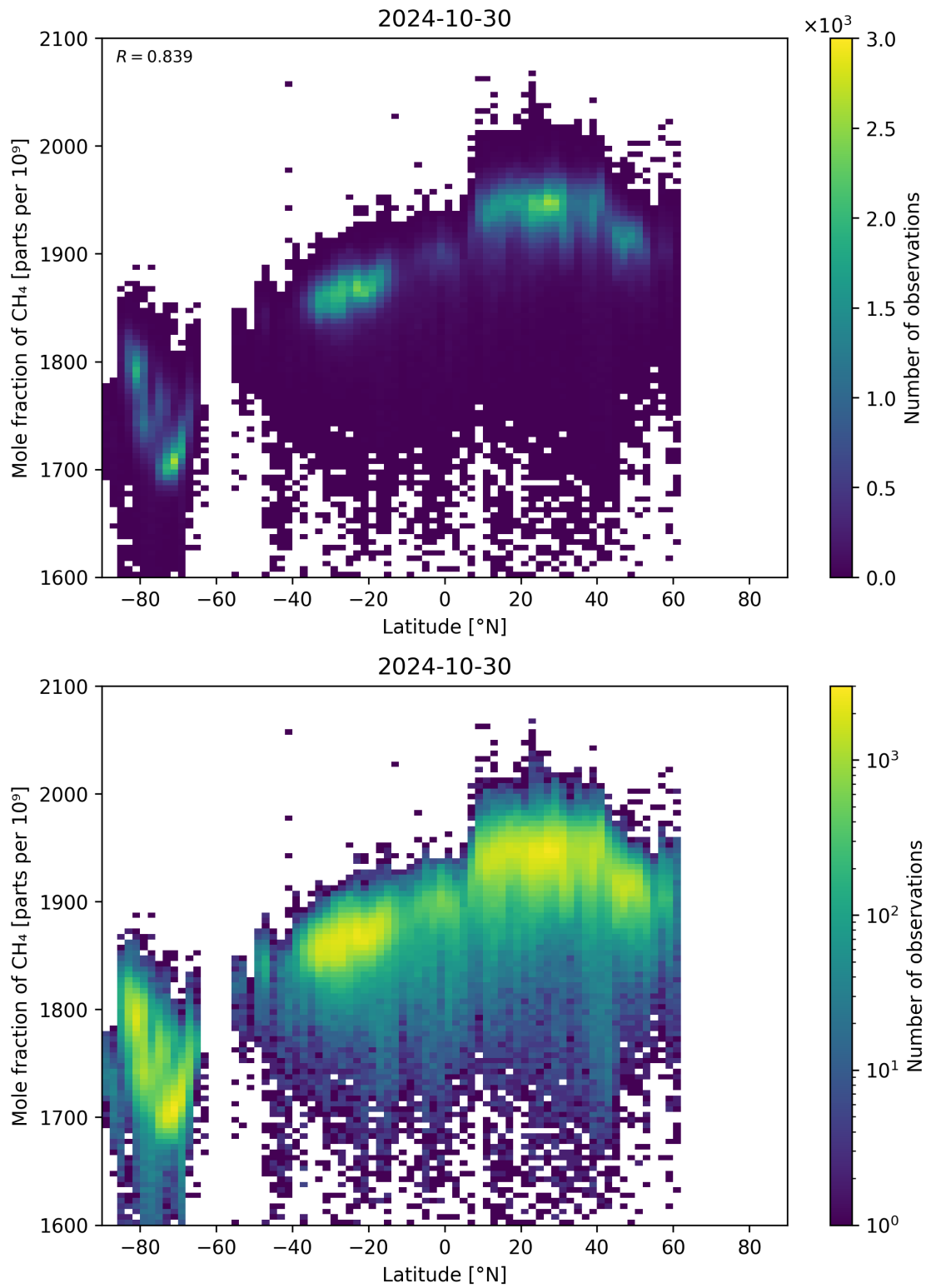
Figure 57: Scatter density plot of “Latitude” against “Mole fraction of CH 4 ” for 2024-10-30 to 2024-10-31.
