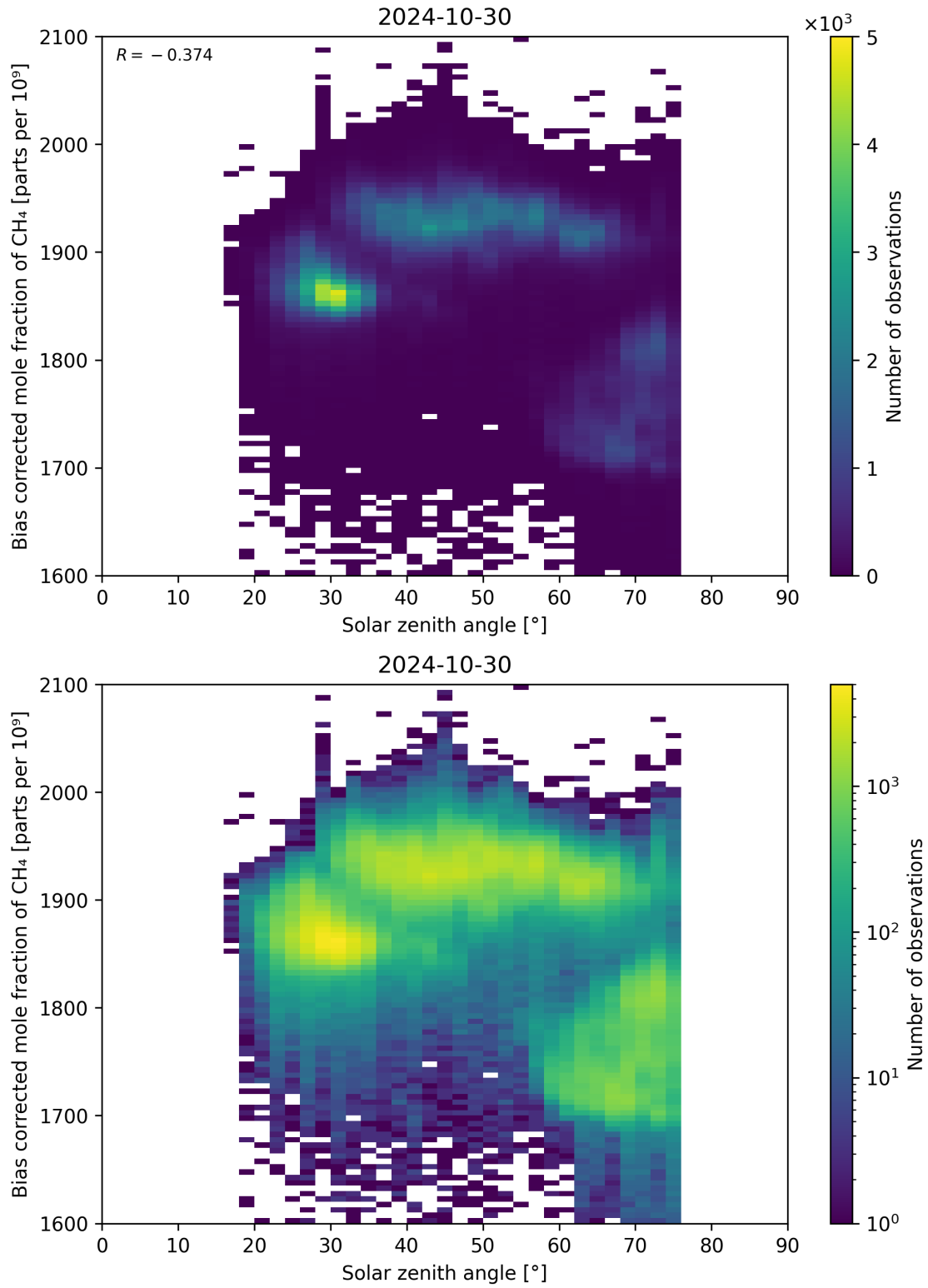
Figure 100: Scatter density plot of “Solar zenith angle” against “Bias corrected mole fraction of CH 4 ” for 2024-10-30 to 2024-10-31.
