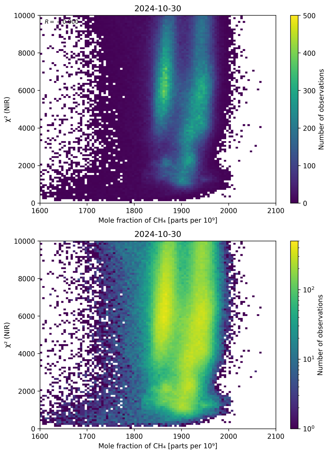
Figure 70: Scatter density plot of “Mole fraction of \text{CH}_4 ” against “ \chi^2 (NIR)” for 2024-10-30 to 2024-10-31.
