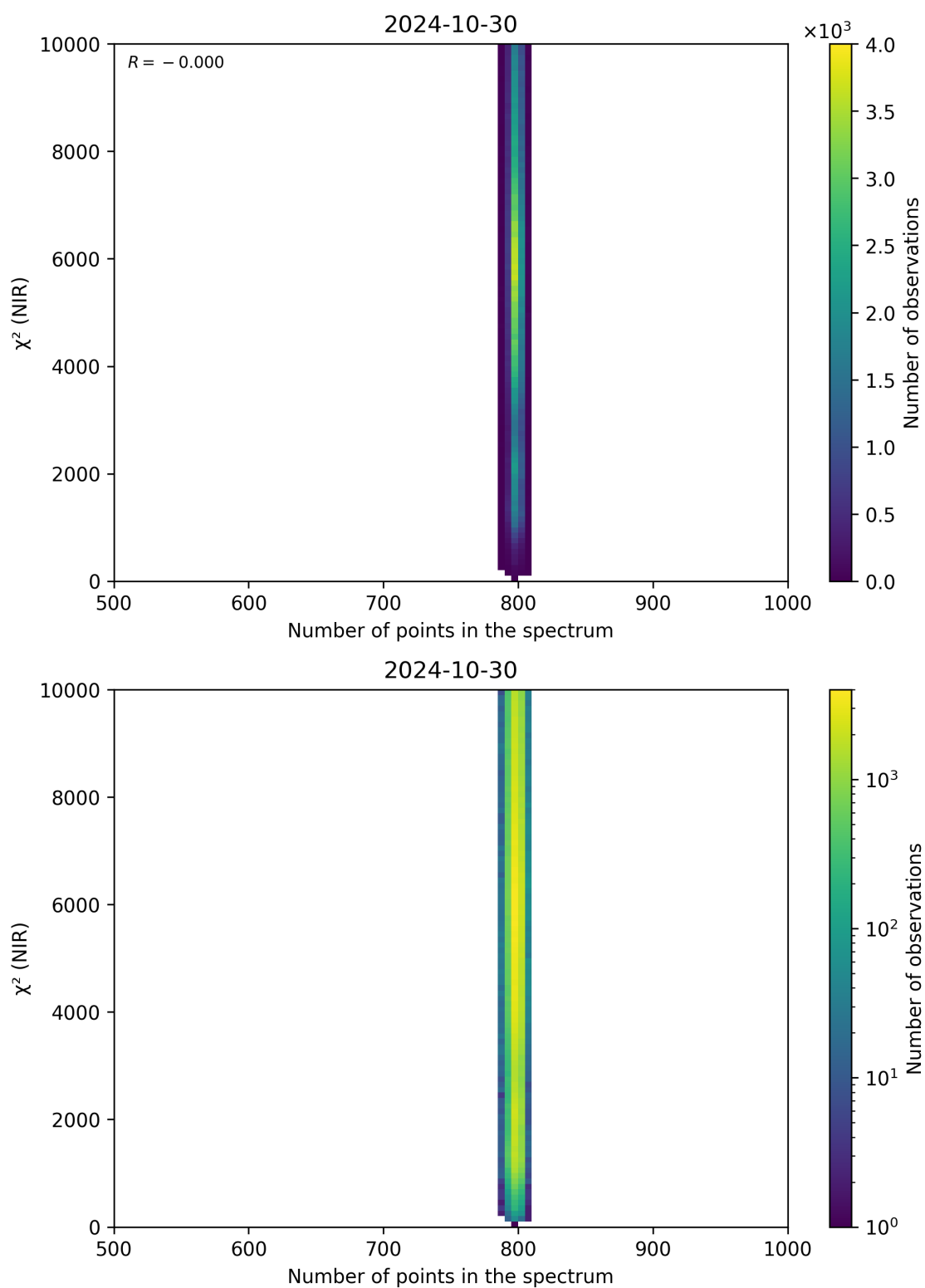
Figure 88: Scatter density plot of “Number of points in the spectrum” against “ \chi^2 (NIR)” for 2024-10-30 to 2024-10-31.
