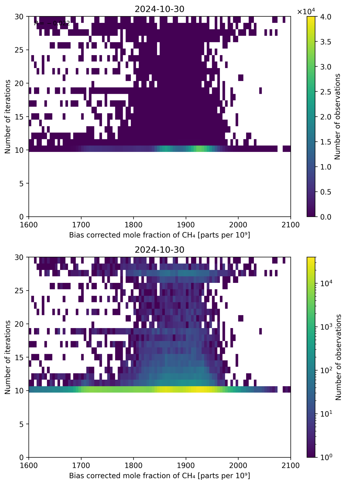
Figure 67: Scatter density plot of “Bias corrected mole fraction of CH 4 ” against “Number of iterations” for 2024-10-30 to 2024-10-31.
