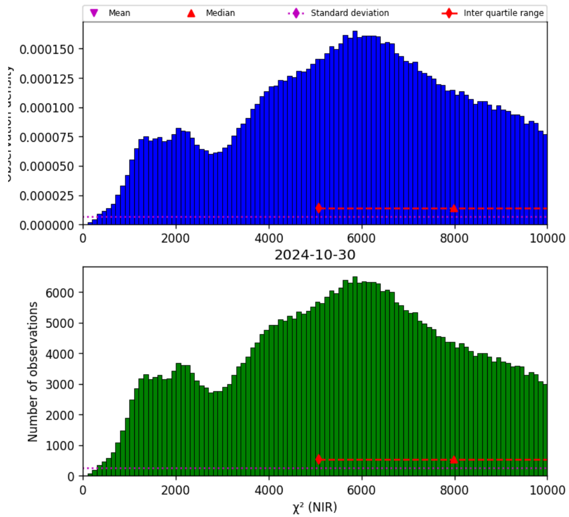
Figure 29: Histogram of “ \chi^2 (NIR)” for 2024-10-30 to 2024-10-31
