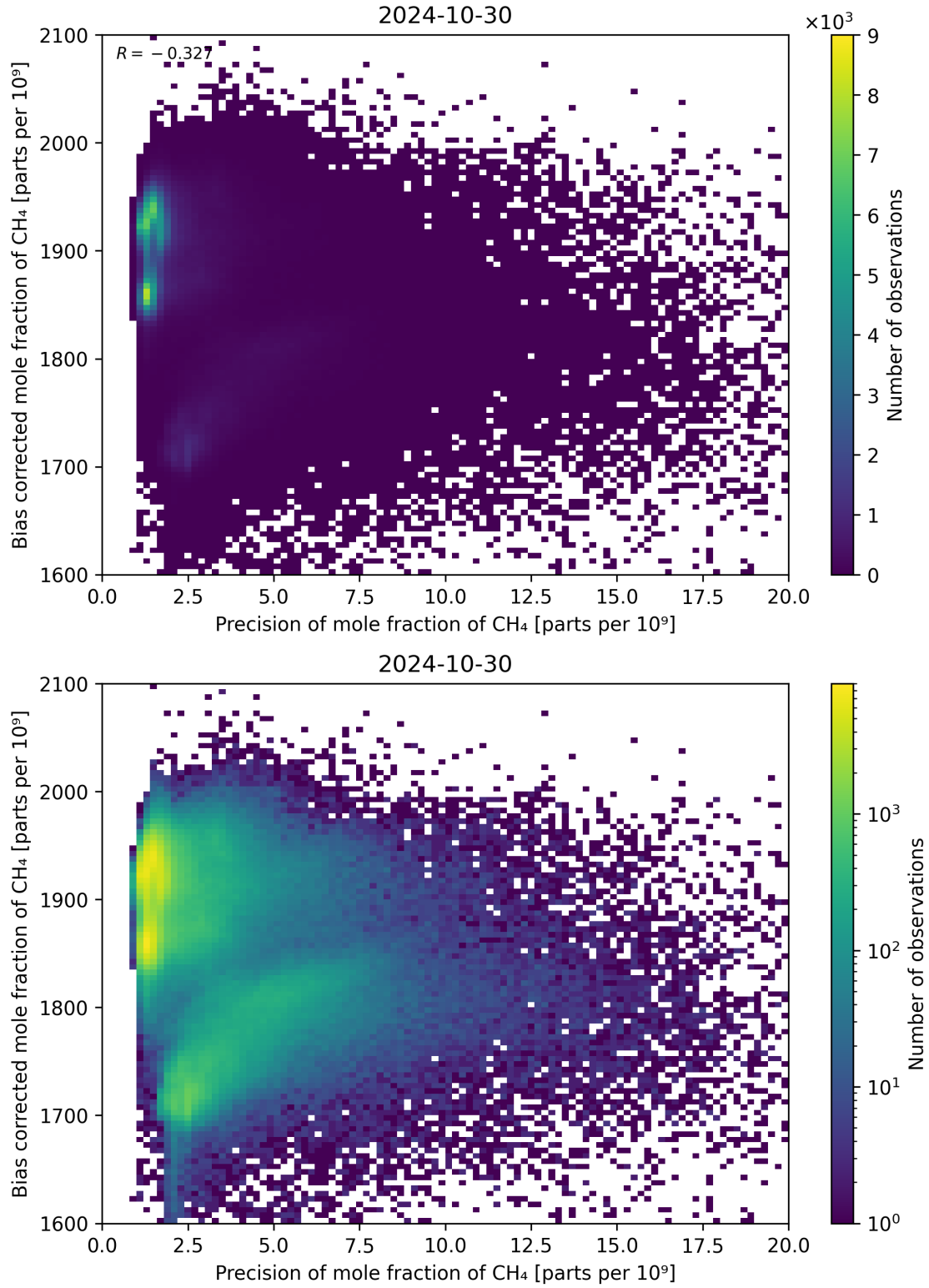
Figure 82: Scatter density plot of “Precision of mole fraction of CH 4 ” against “Bias corrected mole fraction of CH 4 ” for 2024-10-30 to 2024-10-31.
