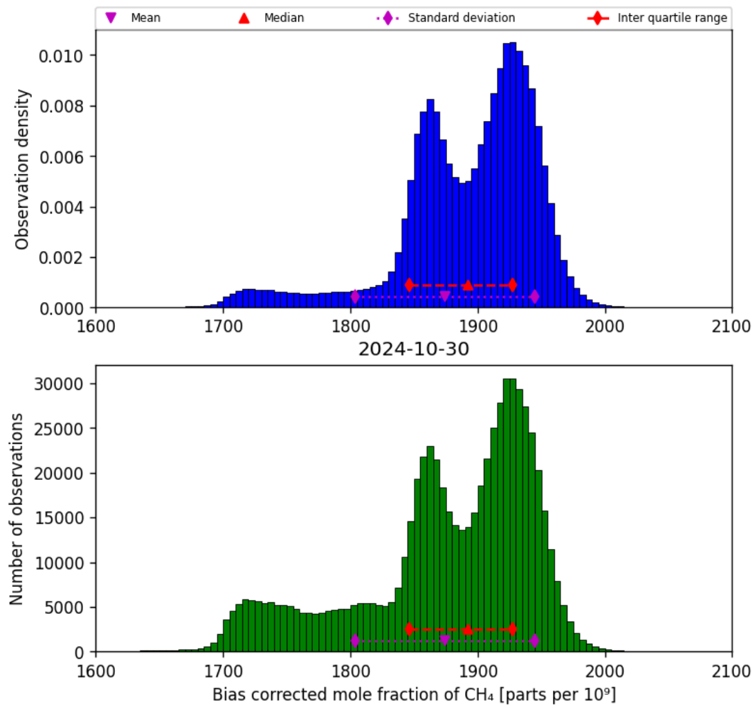
Figure 25: Histogram of “Bias corrected mole fraction of CH 4 ” for 2024-10-30 to 2024-10-31
