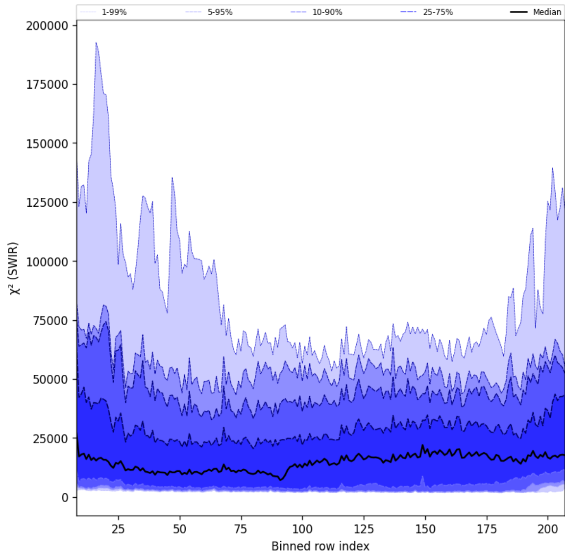
Figure 39: Along track statistics of “ \chi^2 (SWIR)” for 2024-10-30 to 2024-10-31
