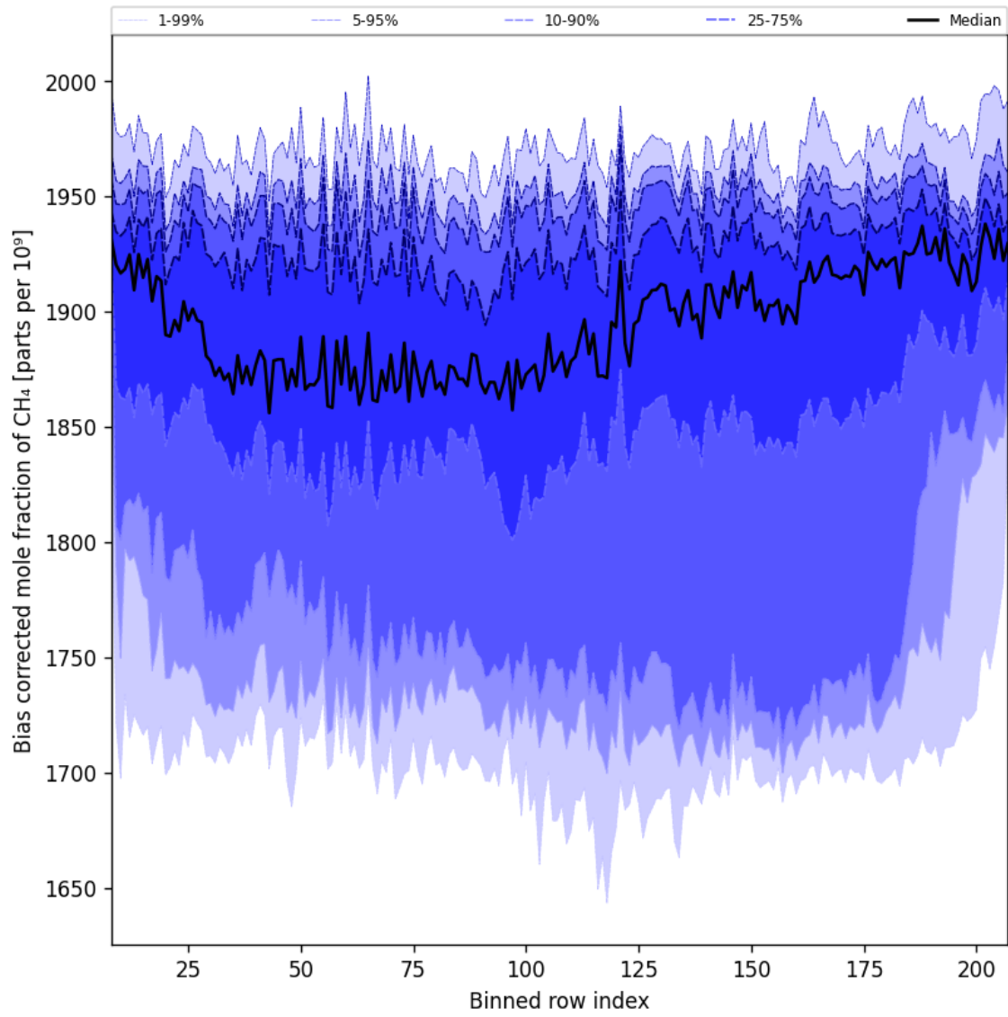
Figure 36: Along track statistics of “Bias corrected mole fraction of CH 4 ” for 2024-10-30 to 2024-10-31
