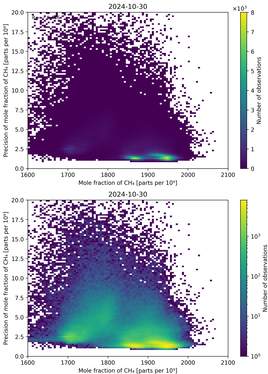
Figure 75: Scatter density plot of “Mole fraction of CH 4 ” against “Precision of mole fraction of CH 4 ” for 2024-10-30 to 2024-10-31.
