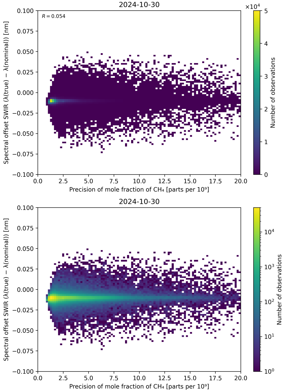
Figure 85: Scatter density plot of “Precision of mole fraction of \text{CH}_4 ” against “Spectral offset SWIR ( \lambda_{\text{true}} - \lambda_{\text{nominal}} )” for 2024-10-30 to 2024-10-31.
