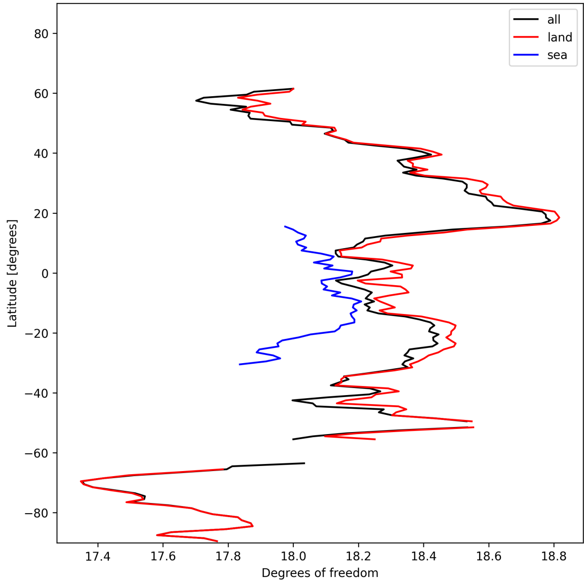
Figure 19: Zonal average of “Degrees of freedom” for 2024-10-30 to 2024-10-31.
