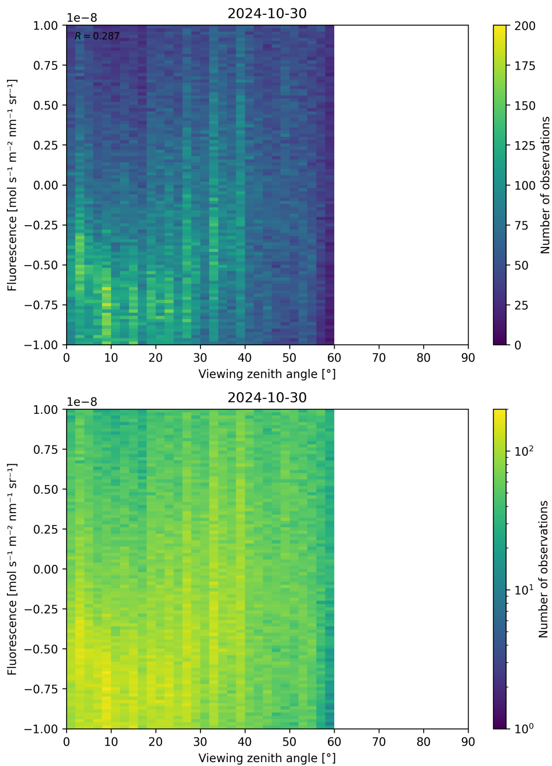
Figure 108: Scatter density plot of “Viewing zenith angle” against “Fluorescence” for 2024-10-30 to 2024-10-31.
