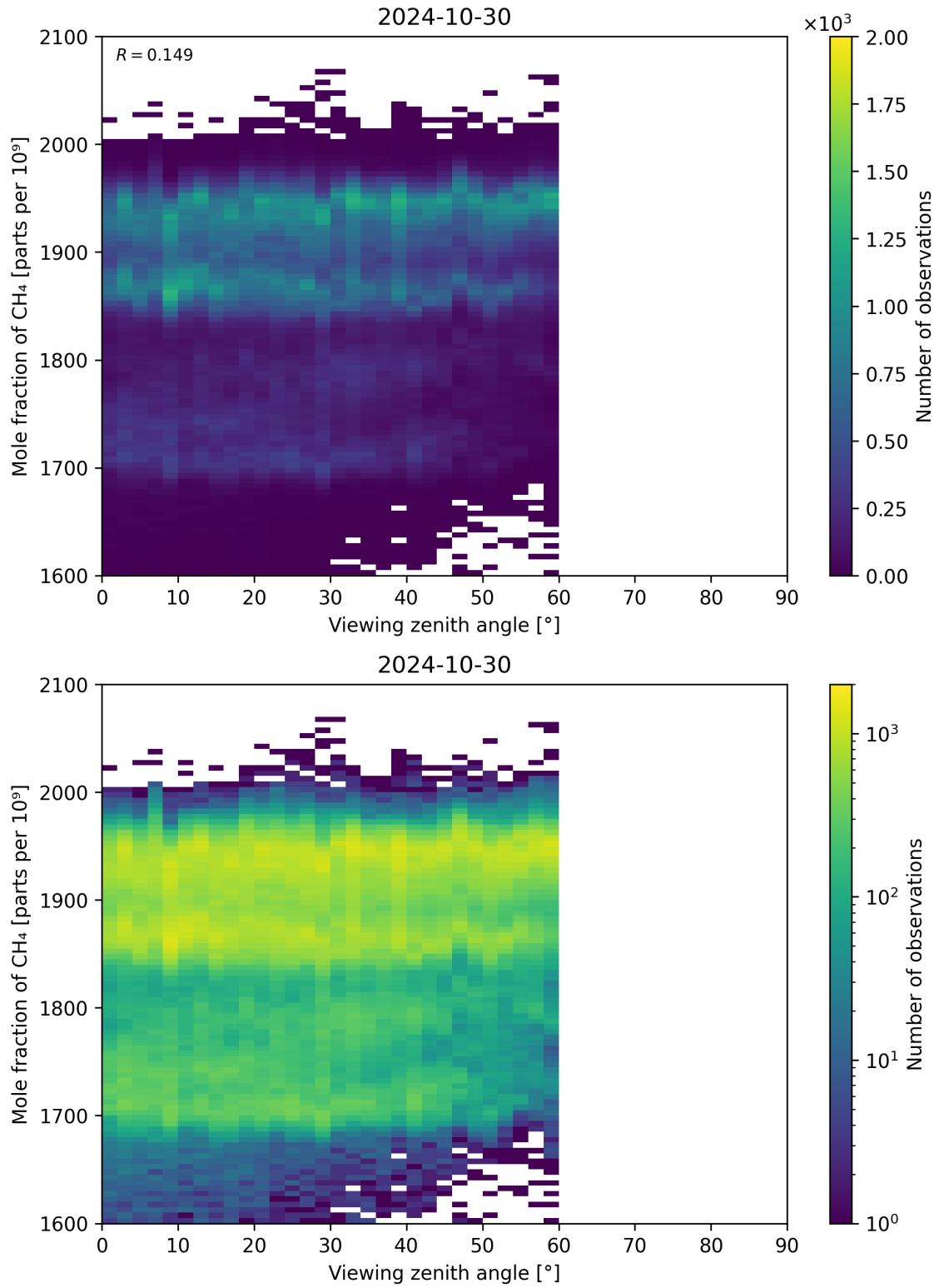
Figure 110: Scatter density plot of “Viewing zenith angle” against “Mole fraction of \text{CH}_4 ” for 2024-10-30 to 2024-10-31.
