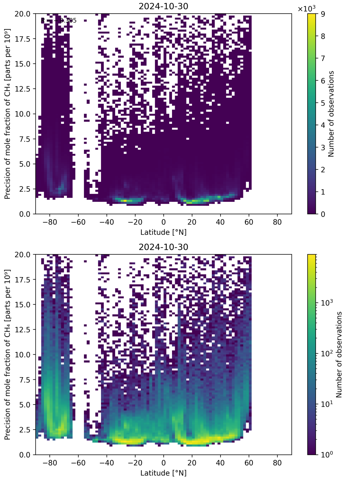
Figure 59: Scatter density plot of “Latitude” against “Precision of mole fraction of CH 4 ” for 2024-10-30 to 2024-10-31.
