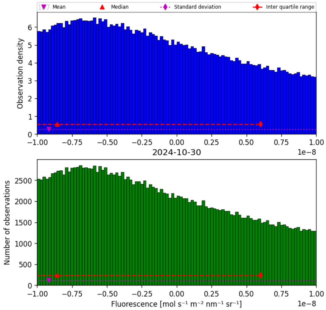
Figure 32: Histogram of “Fluorescence” for 2024-10-30 to 2024-10-31
