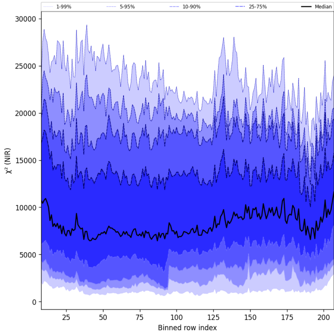
Figure 40: Along track statistics of “ \chi^2 (NIR)” for 2024-10-30 to 2024-10-31
