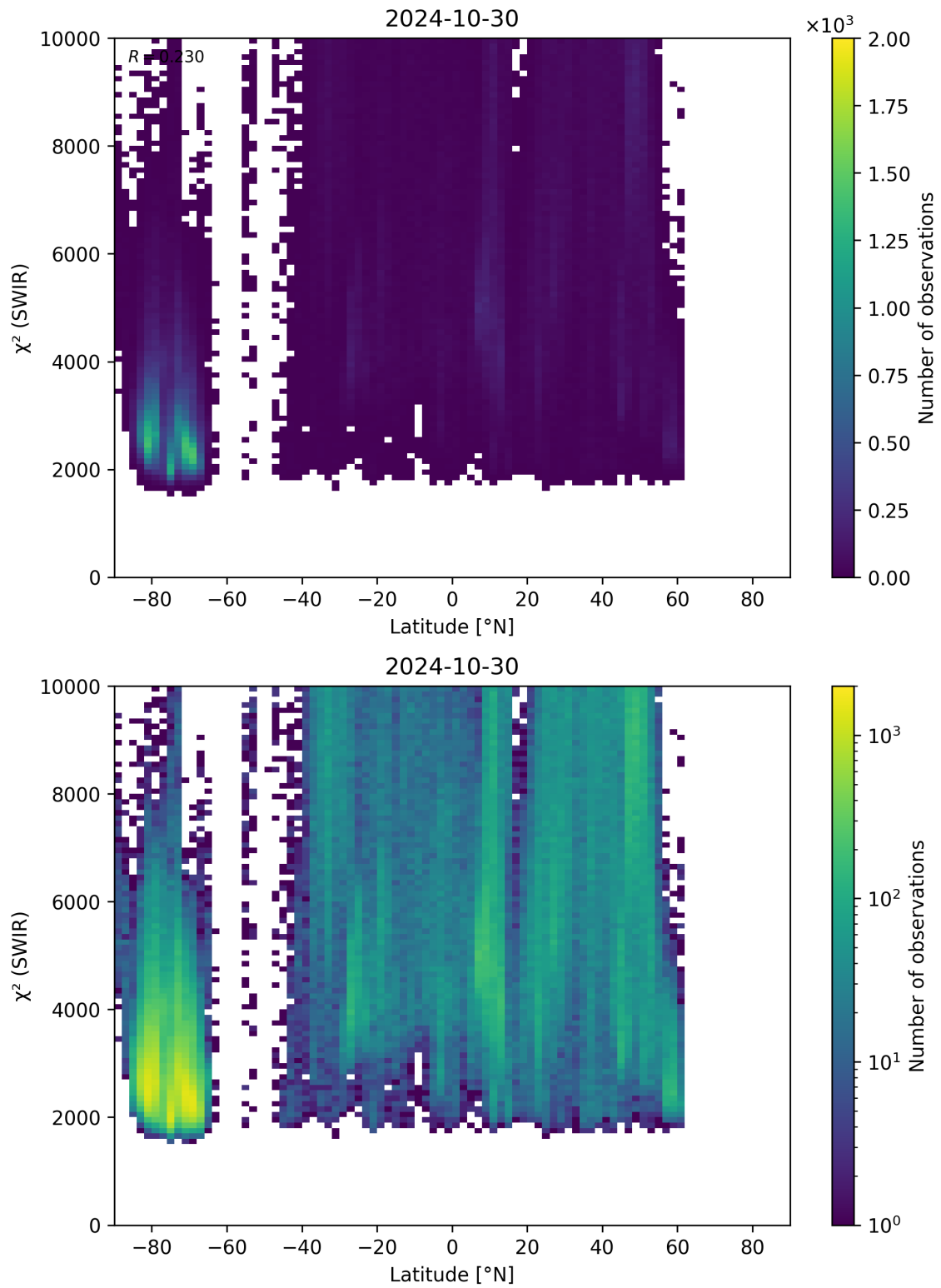
Figure 54: Scatter density plot of “Latitude” against “ \chi^2 (SWIR)” for 2024-10-30 to 2024-10-31.
