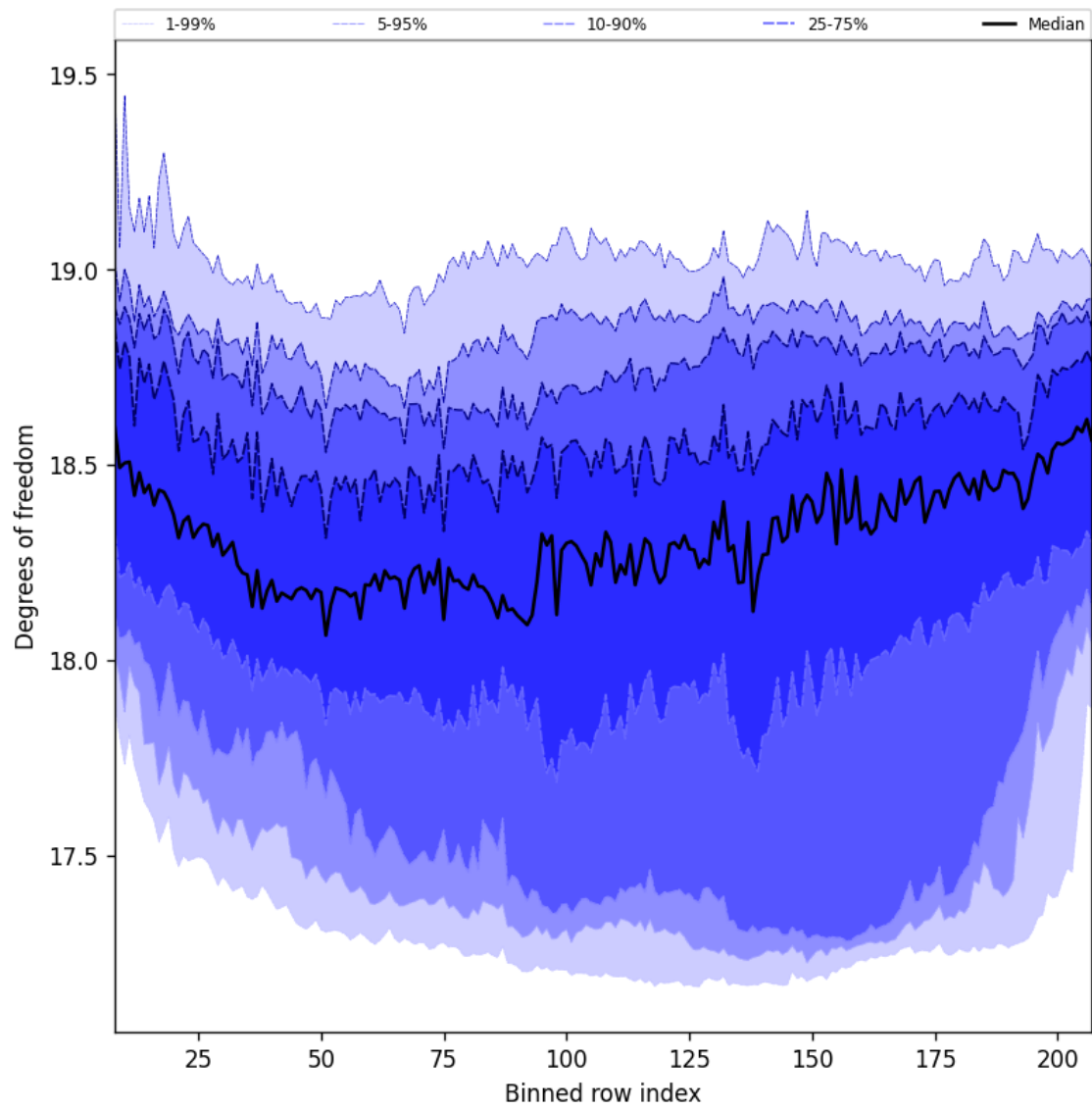
Figure 41: Along track statistics of “Degrees of freedom” for 2024-10-30 to 2024-10-31
