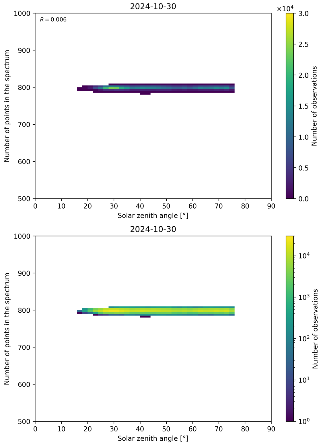
Figure 103: Scatter density plot of “Solar zenith angle” against “Number of points in the spectrum” for 2024-10-30 to 2024-10-31.
