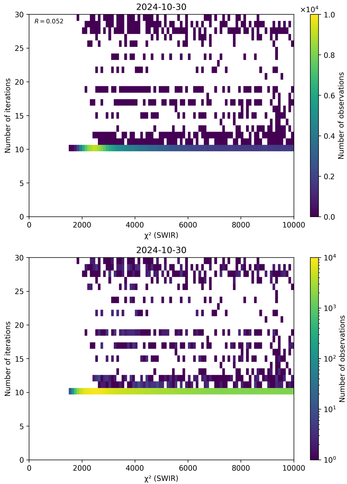
Figure 50: Scatter density plot of “ \chi^2 (SWIR)” against “Number of iterations” for 2024-10-30 to 2024-10-31.
