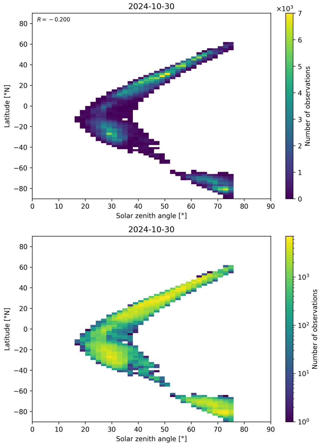
Figure 98: Scatter density plot of “Solar zenith angle” against “Latitude” for 2024-10-30 to 2024-10-31.
