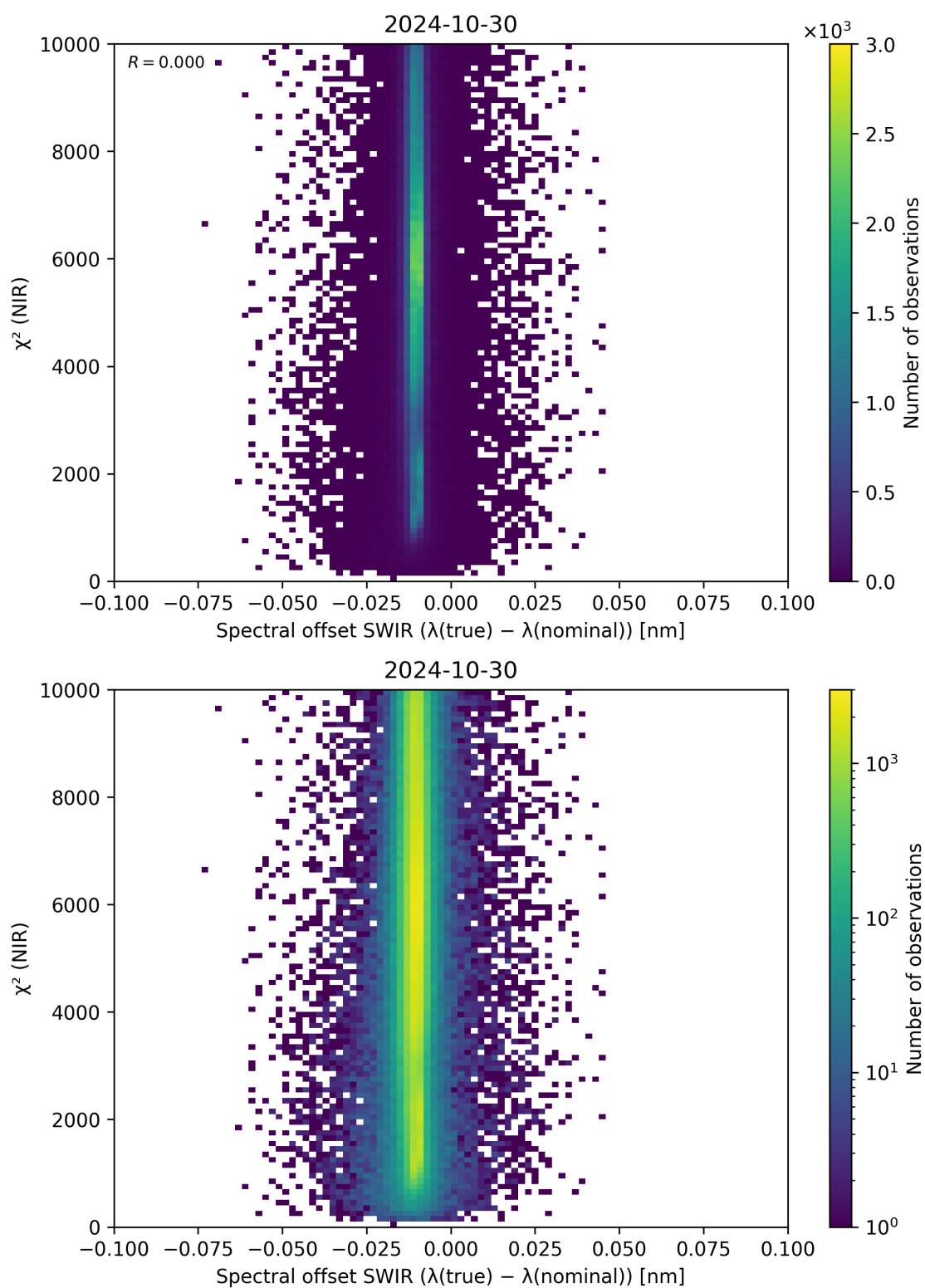
Figure 117: Scatter density plot of “Spectral offset SWIR ( \lambda_{\text{true}} - \lambda_{\text{nominal}} )” against “ \chi^2 (NIR)” for 2024-10-30 to 2024-10-31.
