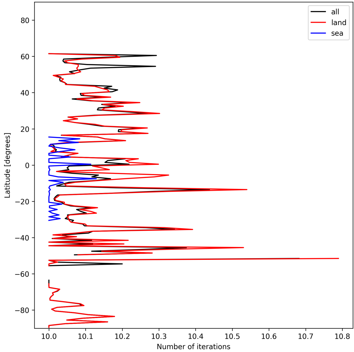
Figure 20: Zonal average of “Number of iterations” for 2024-10-30 to 2024-10-31.
