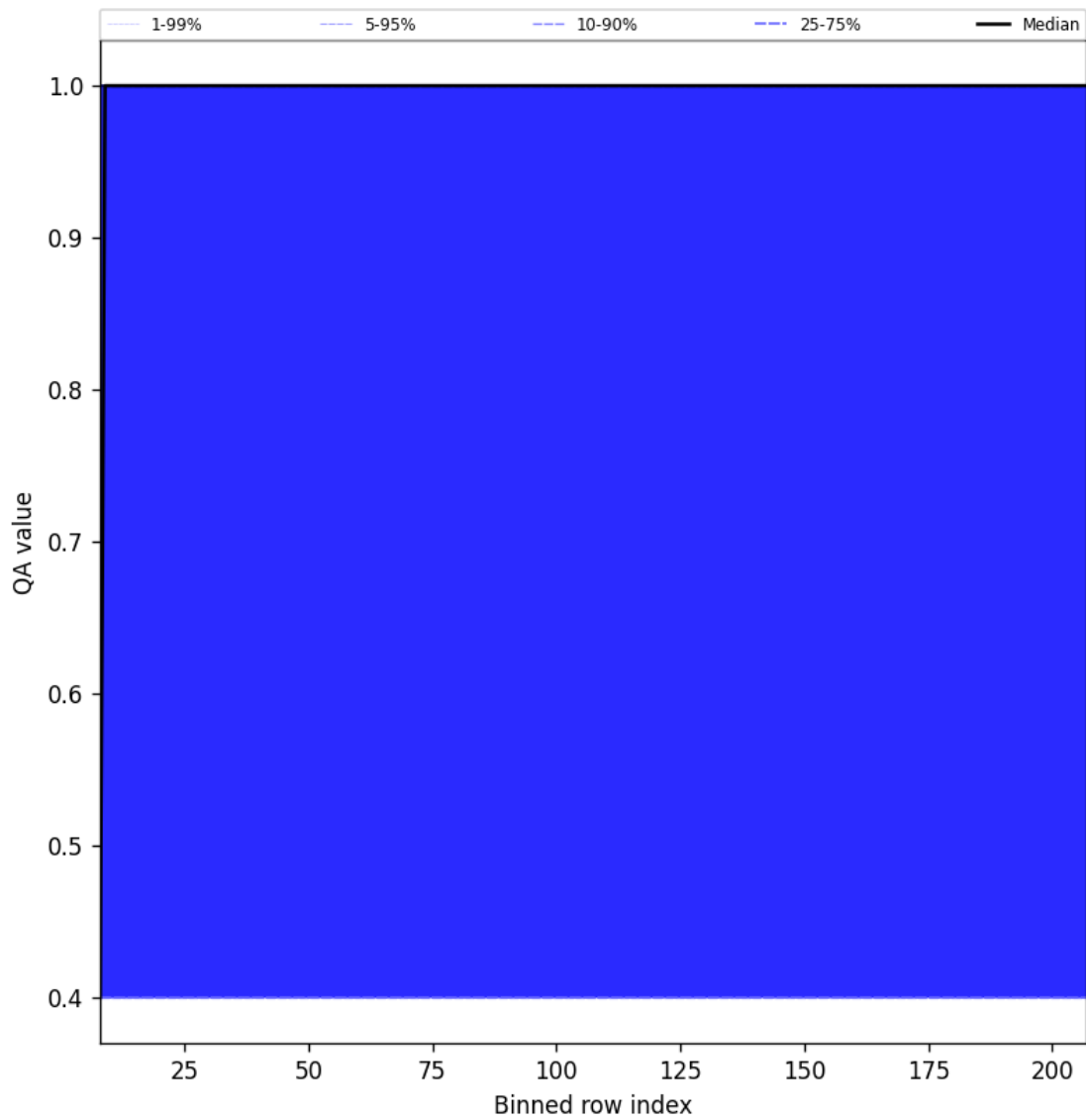
Figure 33: Along track statistics of “QA value” for 2024-10-30 to 2024-10-31
