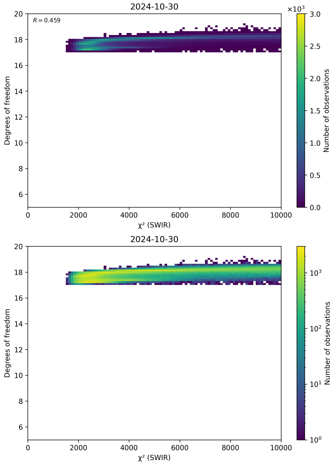
Figure 48: Scatter density plot of “ \chi^2 (SWIR)” against “Degrees of freedom” for 2024-10-30 to 2024-10-31.
