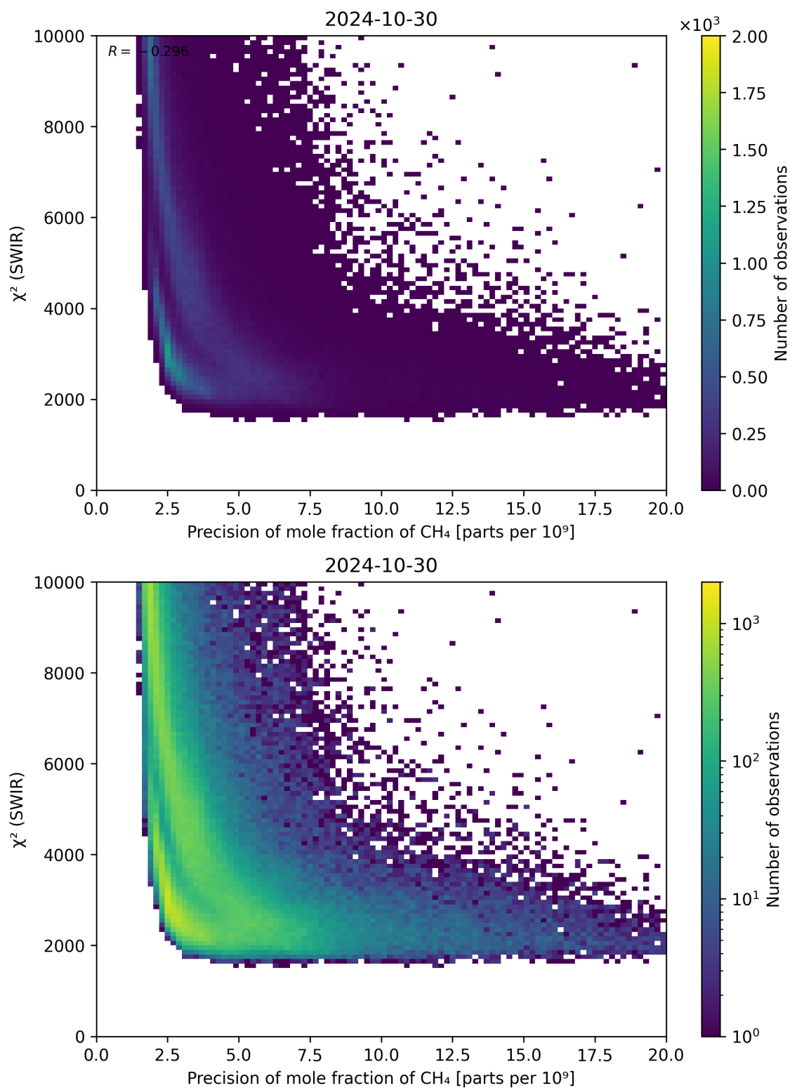
Figure 79: Scatter density plot of “Precision of mole fraction of \text{CH}_4 ” against “ \chi^2 (SWIR)” for 2024-10-30 to 2024-10-31.
