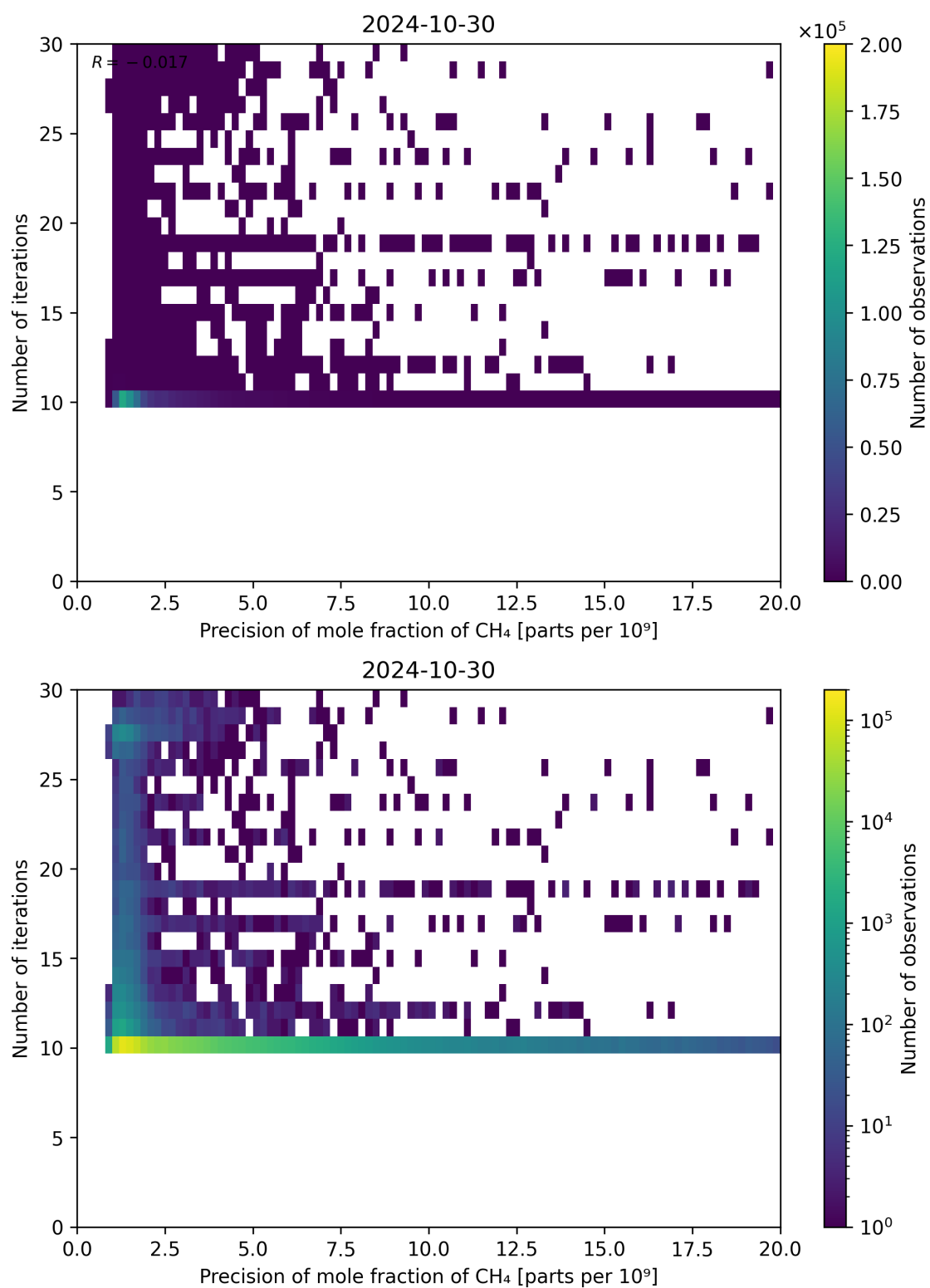
Figure 83: Scatter density plot of “Precision of mole fraction of CH 4 ” against “Number of iterations” for 2024-10-30 to 2024-10-31.
