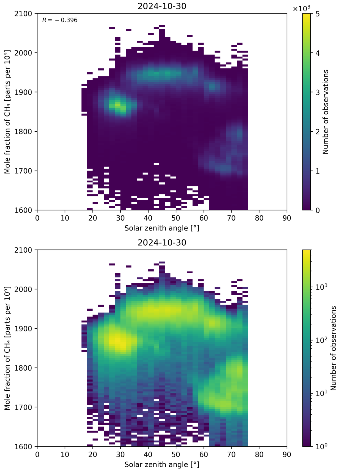
Figure 99: Scatter density plot of “Solar zenith angle” against “Mole fraction of \text{CH}_4 ” for 2024-10-30 to 2024-10-31.
