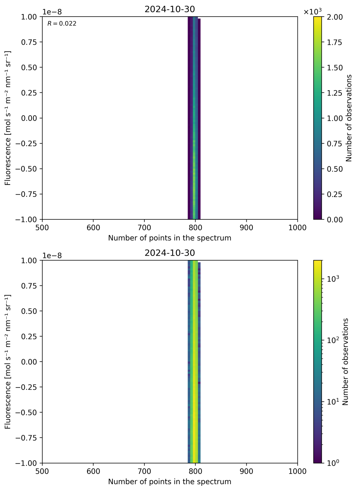
Figure 91: Scatter density plot of “Number of points in the spectrum” against “Fluorescence” for 2024-10-30 to 2024-10-31.
