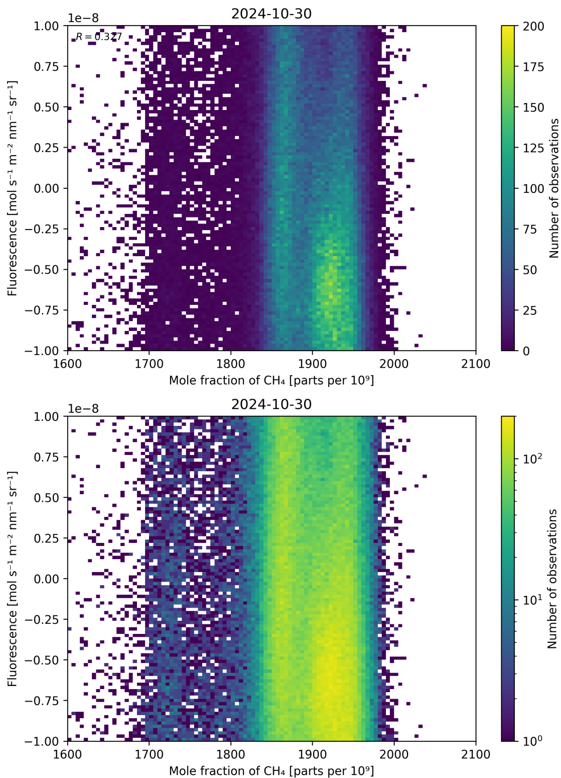
Figure 73: Scatter density plot of “Mole fraction of \text{CH}_4 ” against “Fluorescence” for 2024-10-30 to 2024-10-31.
