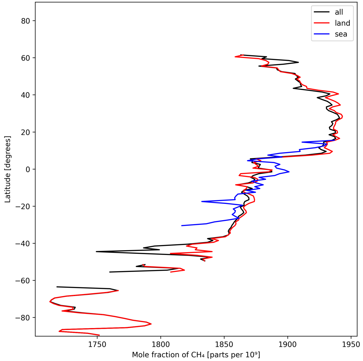
Figure 12: Zonal average of “Mole fraction of CH 4 ” for 2024-10-30 to 2024-10-31.
