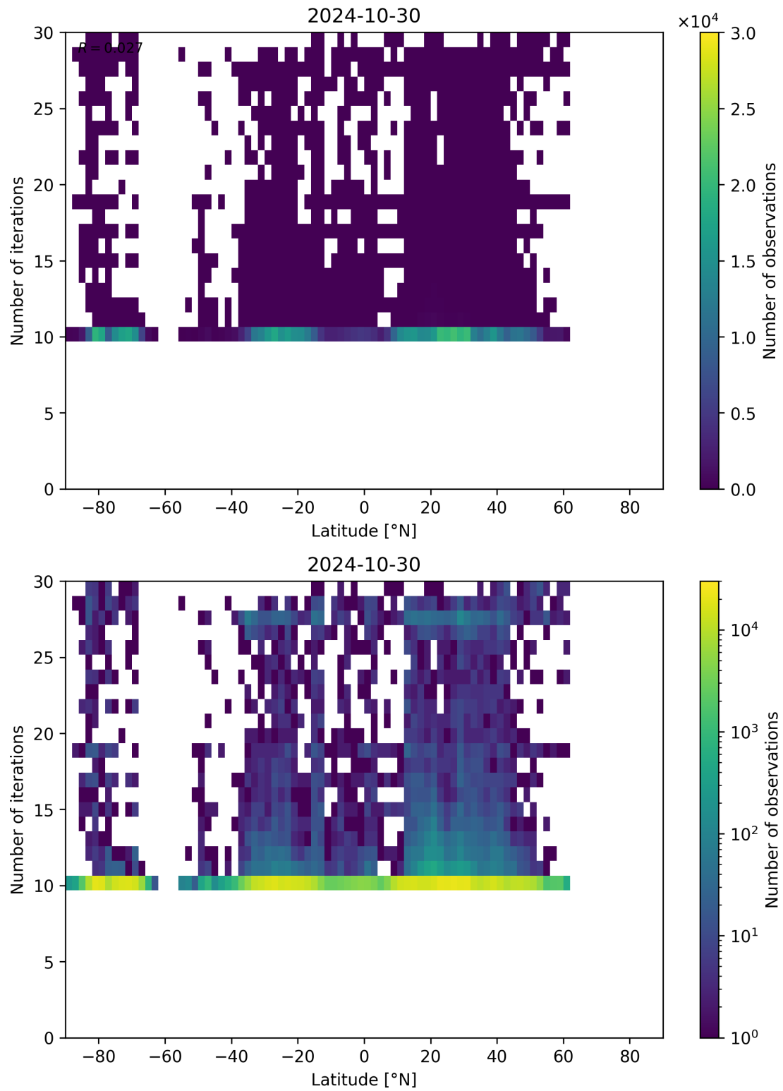
Figure 60: Scatter density plot of “Latitude” against “Number of iterations” for 2024-10-30 to 2024-10-31.
