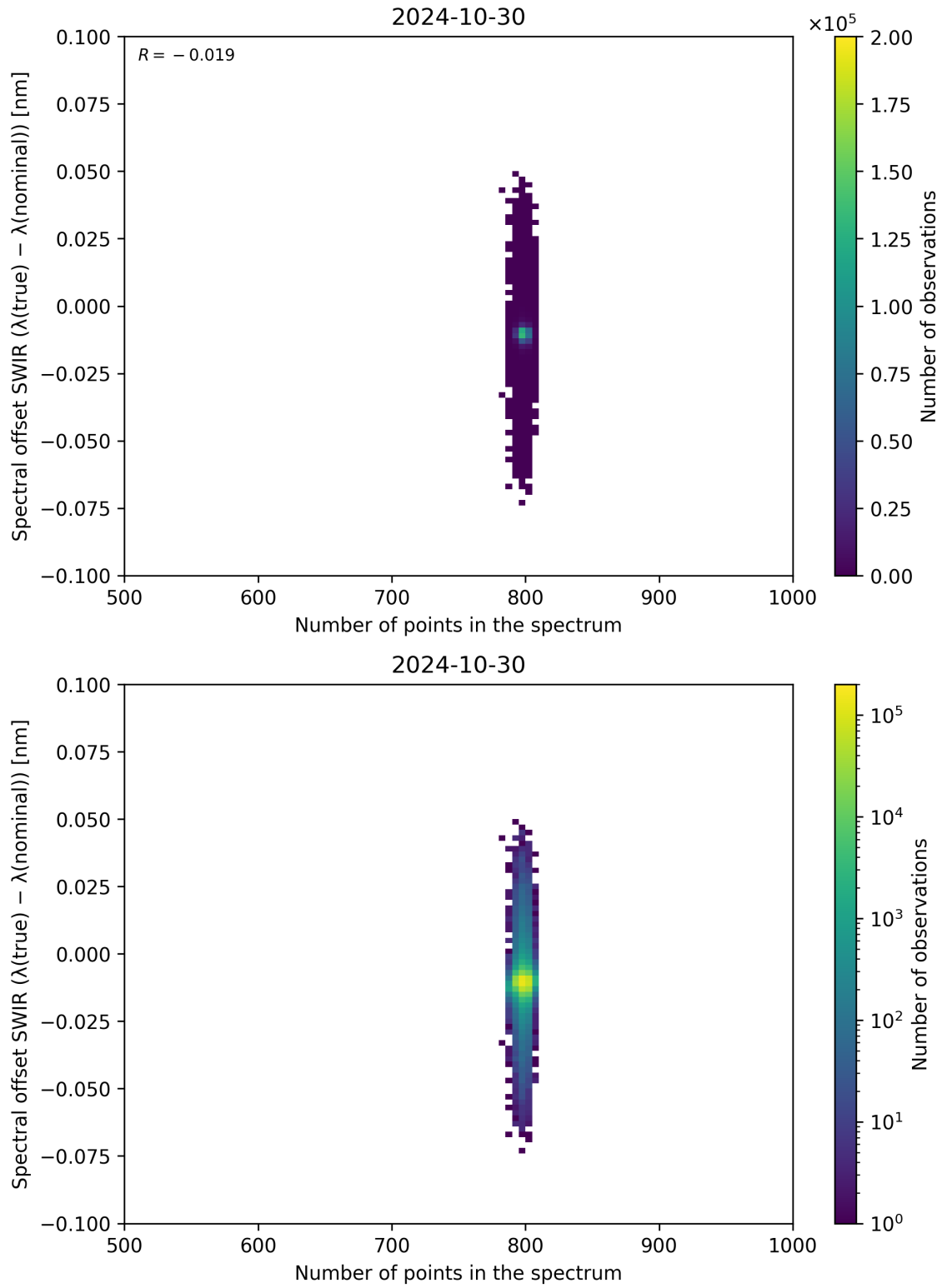
Figure 93: Scatter density plot of “Number of points in the spectrum” against “Spectral offset SWIR ( \lambda_{\text{true}} - \lambda_{\text{nominal}} )” for 2024-10-30 to 2024-10-31.
