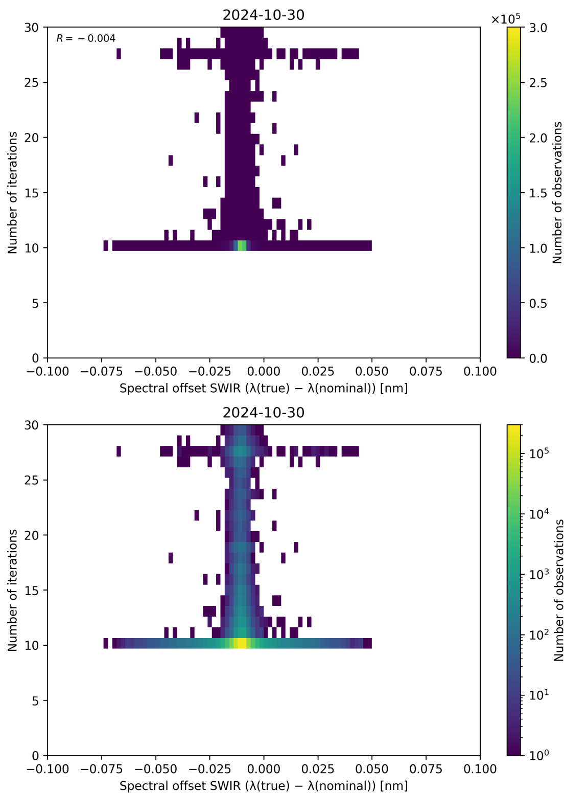
Figure 121: Scatter density plot of “Spectral offset SWIR ( \lambda_{\text{true}} - \lambda_{\text{nominal}} )” against “Number of iterations” for 2024-10-30 to 2024-10-31.
