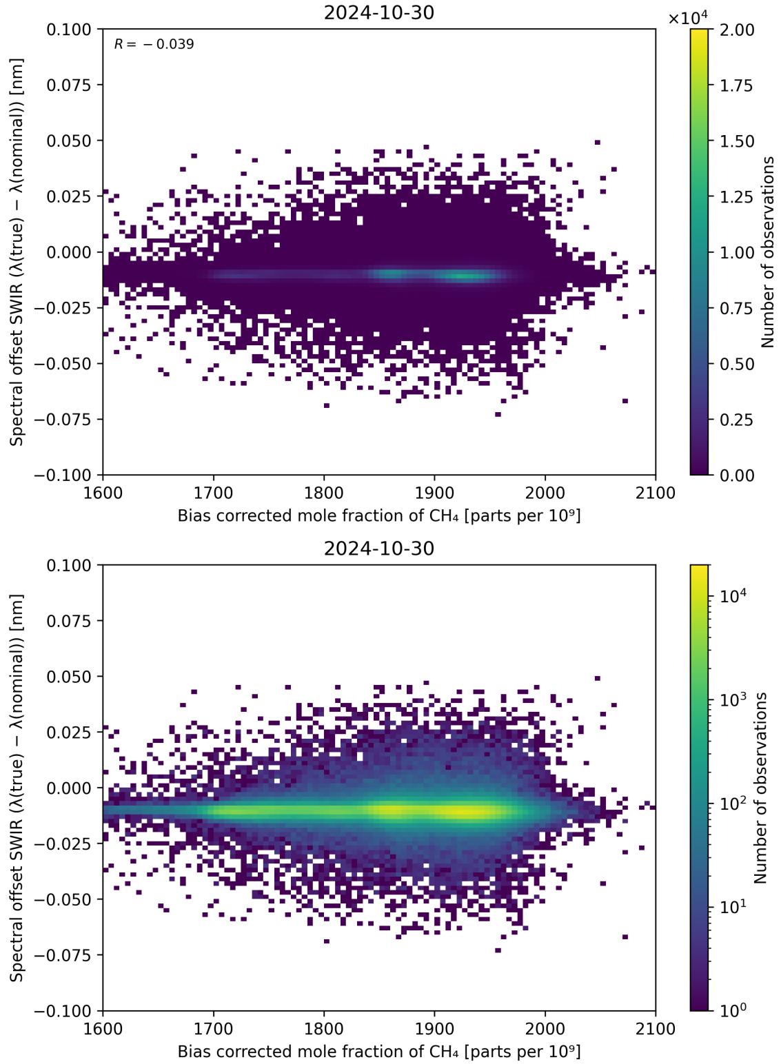
Figure 69: Scatter density plot of “Bias corrected mole fraction of \text{CH}_4 ” against “Spectral offset SWIR ( \lambda_{\text{true}} - \lambda_{\text{nominal}} )” for 2024-10-30 to 2024-10-31.
