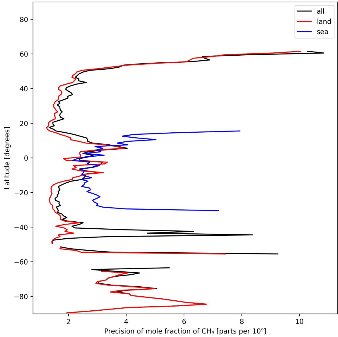
Figure 13: Zonal average of “Precision of mole fraction of CH 4 ” for 2024-10-30 to 2024-10-31.
