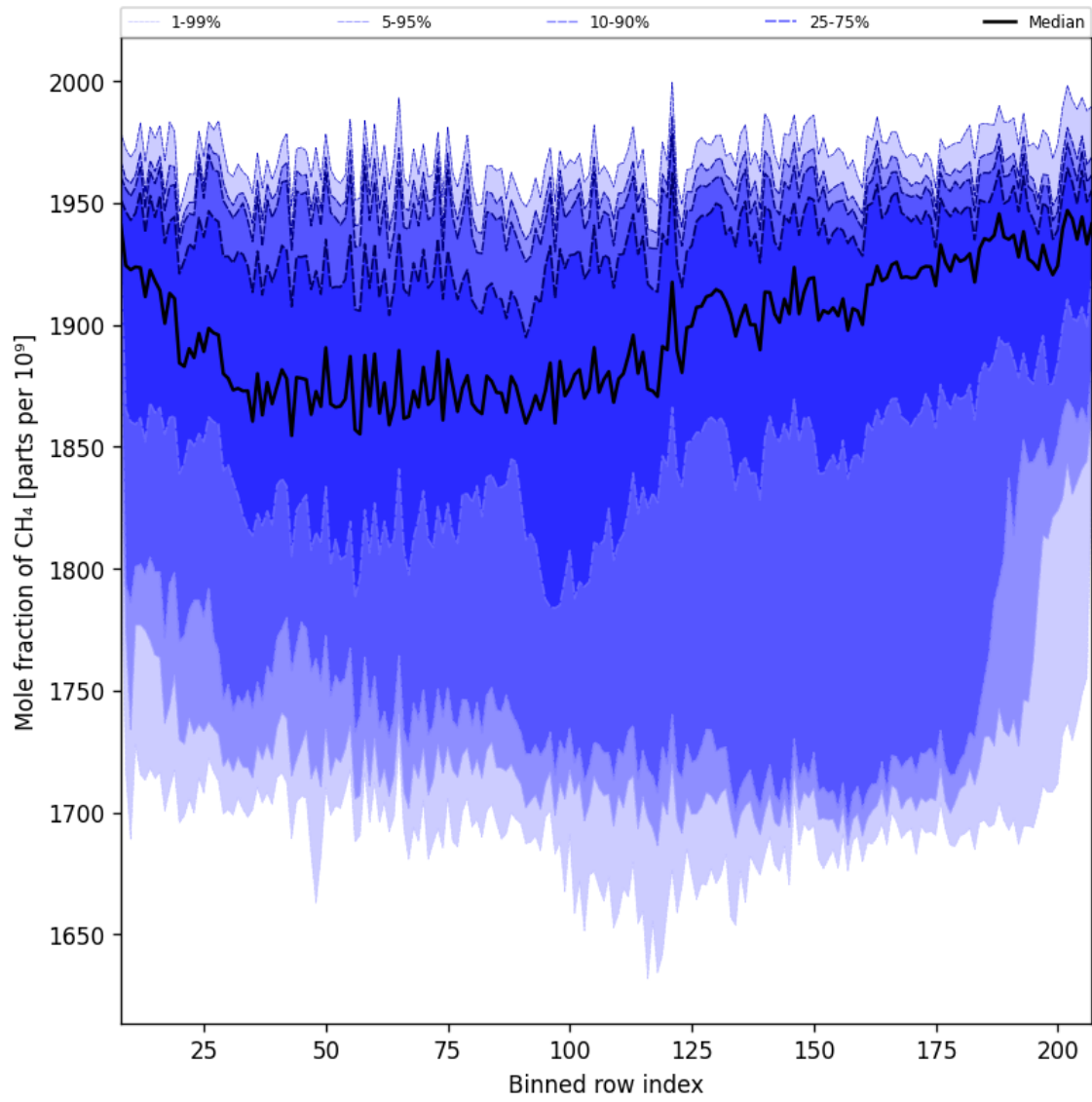
Figure 34: Along track statistics of “Mole fraction of CH 4 ” for 2024-10-30 to 2024-10-31
