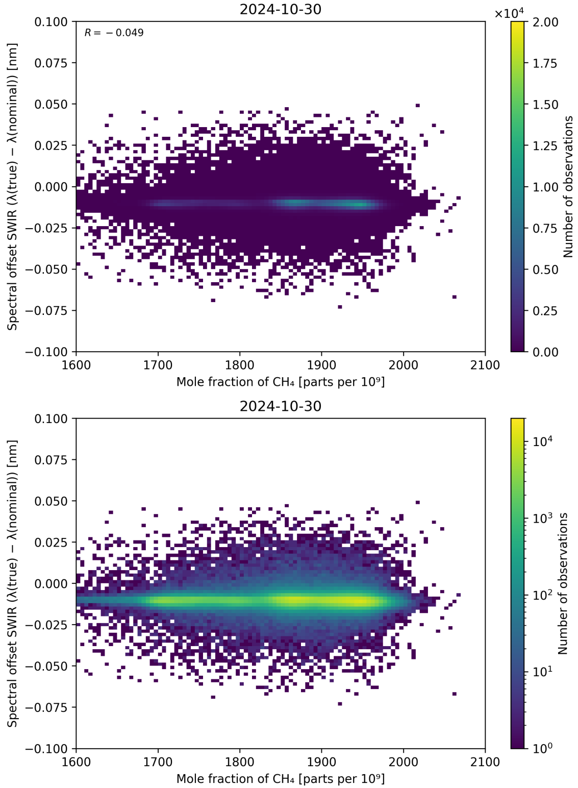
Figure 86: Scatter density plot of “Mole fraction of \text{CH}_4 ” against “Spectral offset SWIR ( \lambda_{\text{true}} - \lambda_{\text{nominal}} )” for 2024-10-30 to 2024-10-31.
