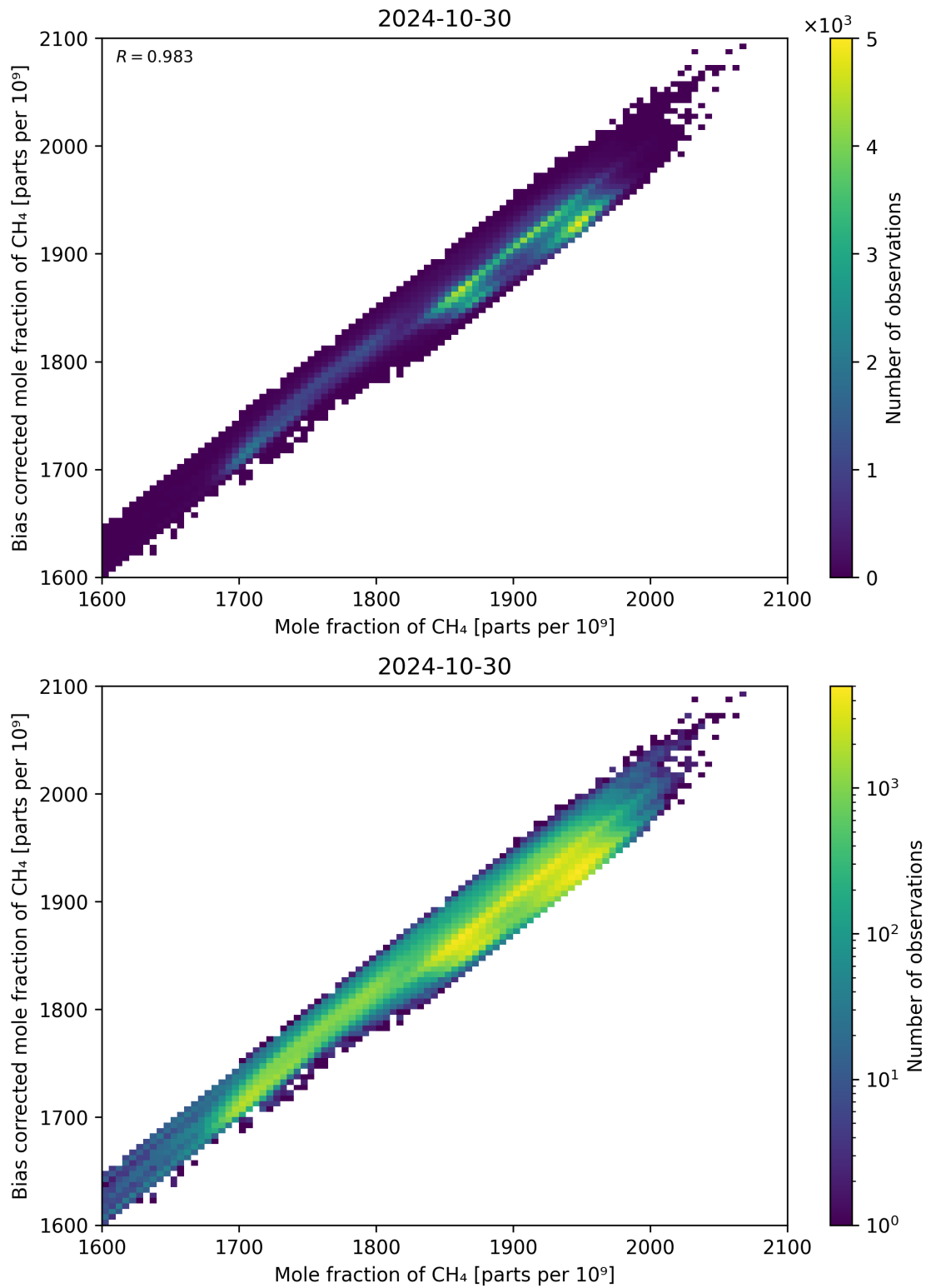
Figure 74: Scatter density plot of “Mole fraction of CH 4 ” against “Bias corrected mole fraction of CH 4 ” for 2024-10-30 to 2024-10-31.
