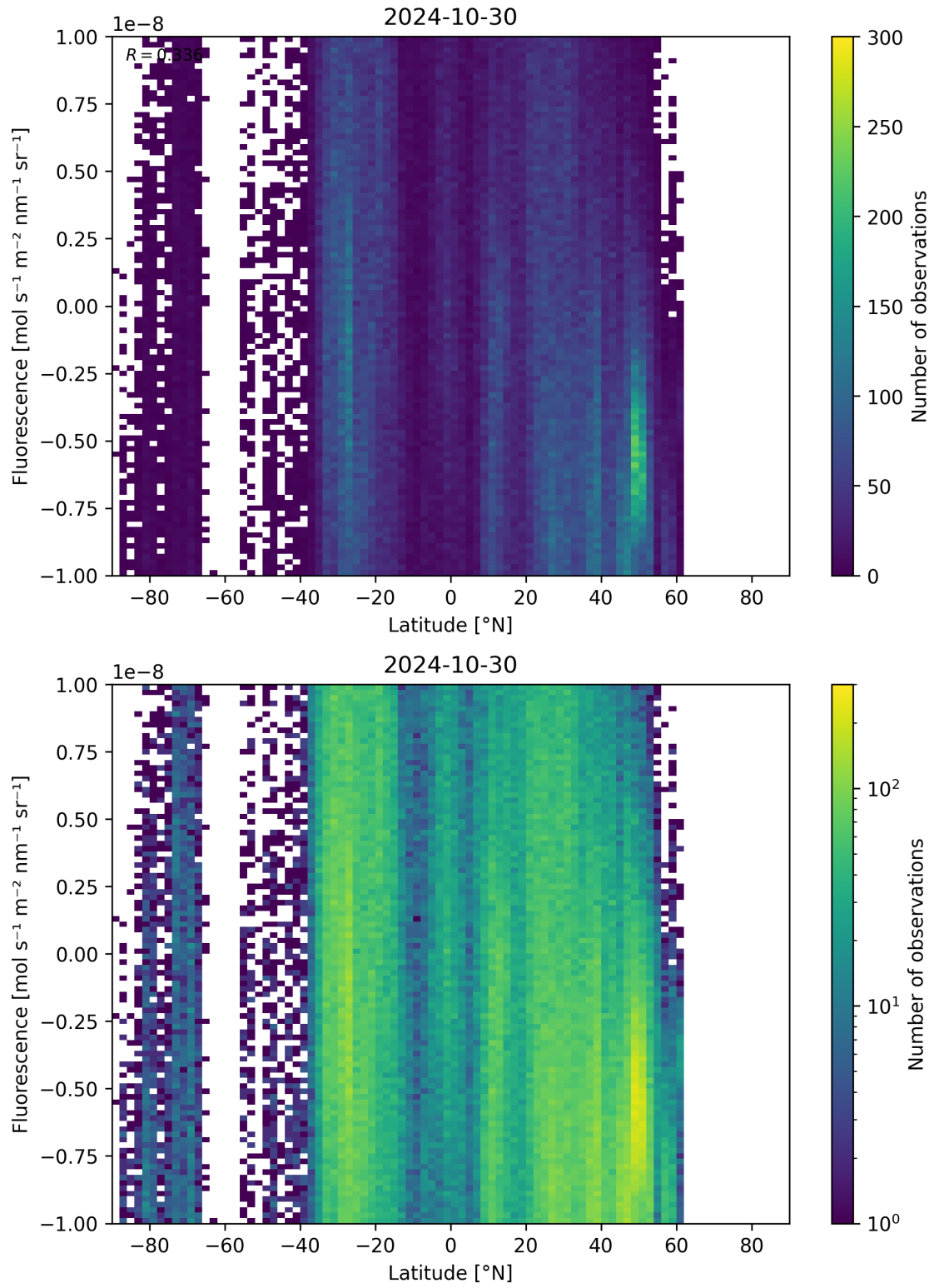
Figure 56: Scatter density plot of “Latitude” against “Fluorescence” for 2024-10-30 to 2024-10-31.
