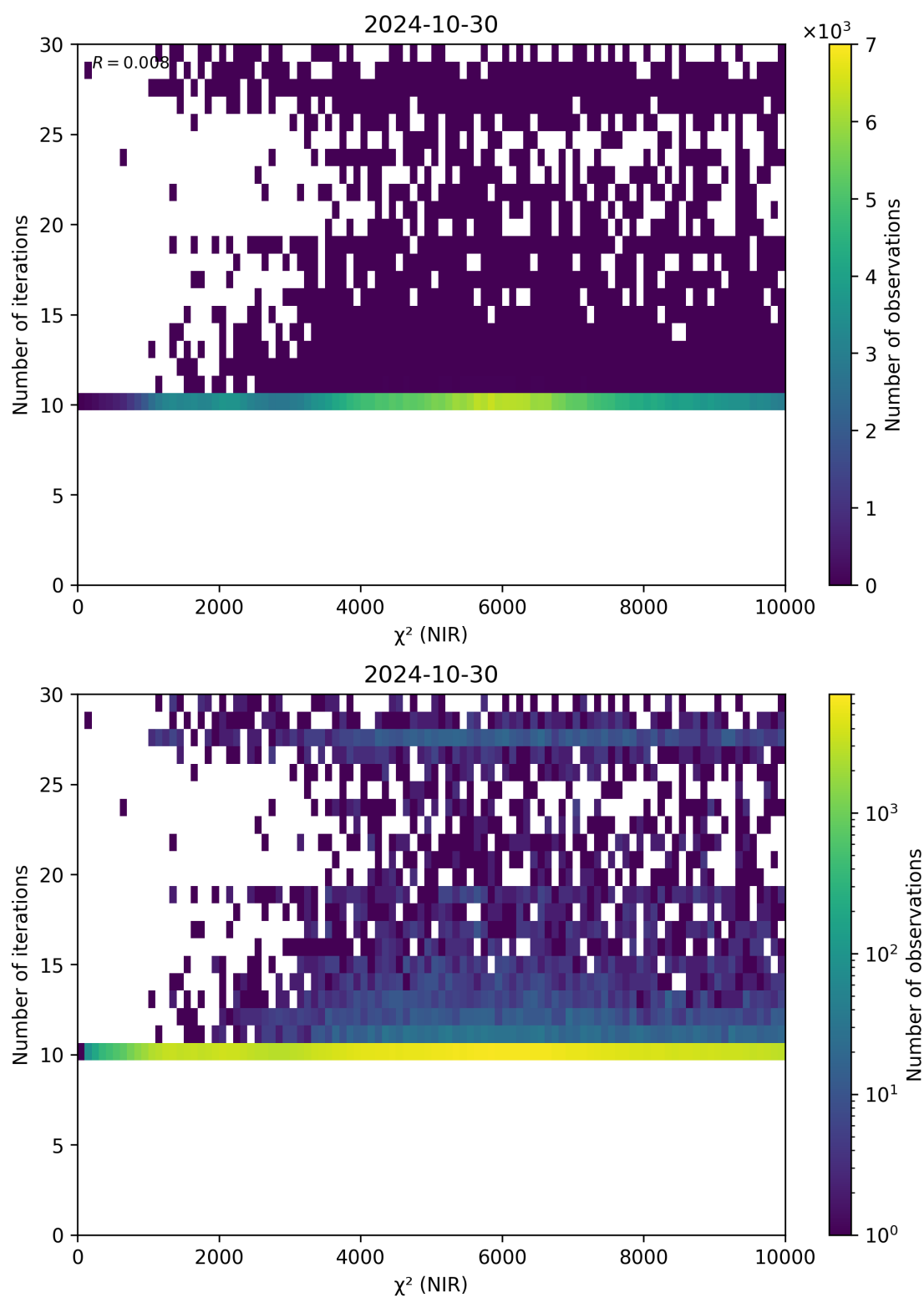
Figure 46: Scatter density plot of “ \chi^2 (NIR)” against “Number of iterations” for 2024-10-30 to 2024-10-31.
