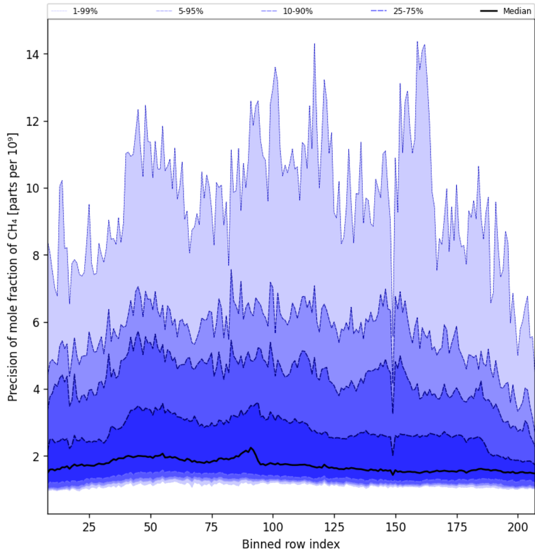
Figure 35: Along track statistics of “Precision of mole fraction of CH 4 ” for 2024-10-30 to 2024-10-31
