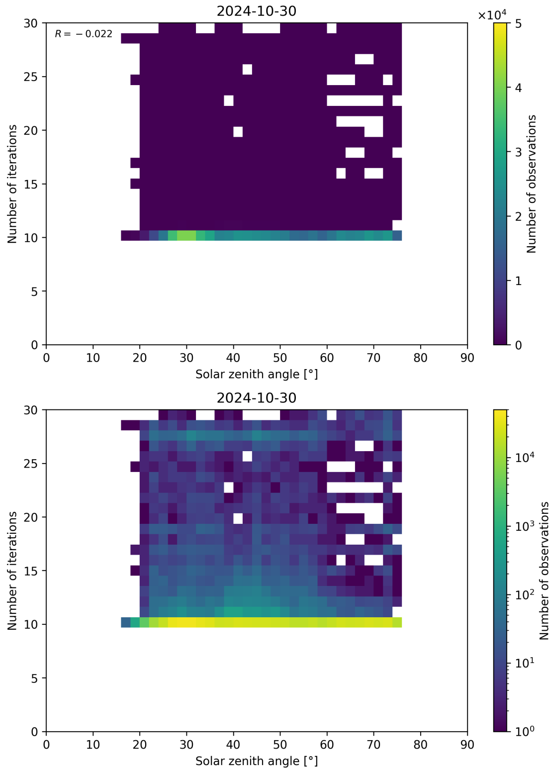
Figure 102: Scatter density plot of “Solar zenith angle” against “Number of iterations” for 2024-10-30 to 2024-10-31.
