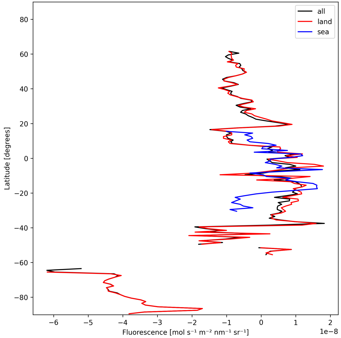
Figure 21: Zonal average of “Fluorescence” for 2024-10-30 to 2024-10-31.
