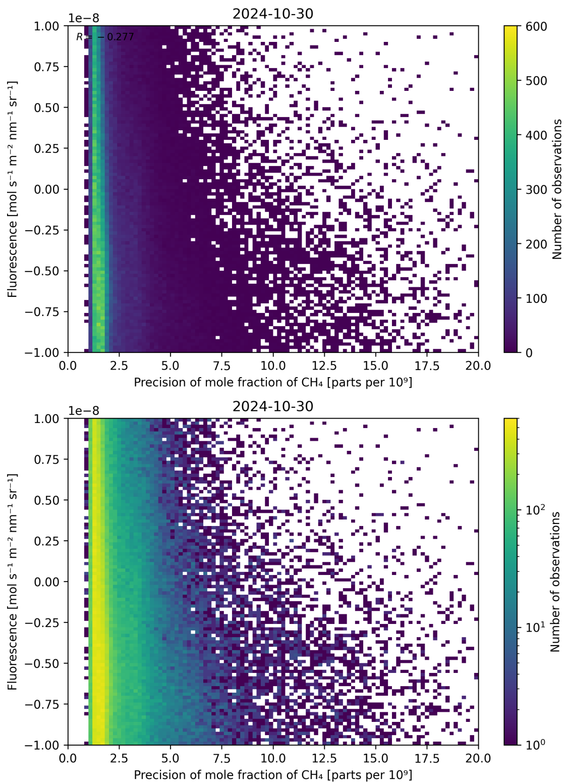
Figure 81: Scatter density plot of “Precision of mole fraction of \text{CH}_4 ” against “Fluorescence” for 2024-10-30 to 2024-10-31.
