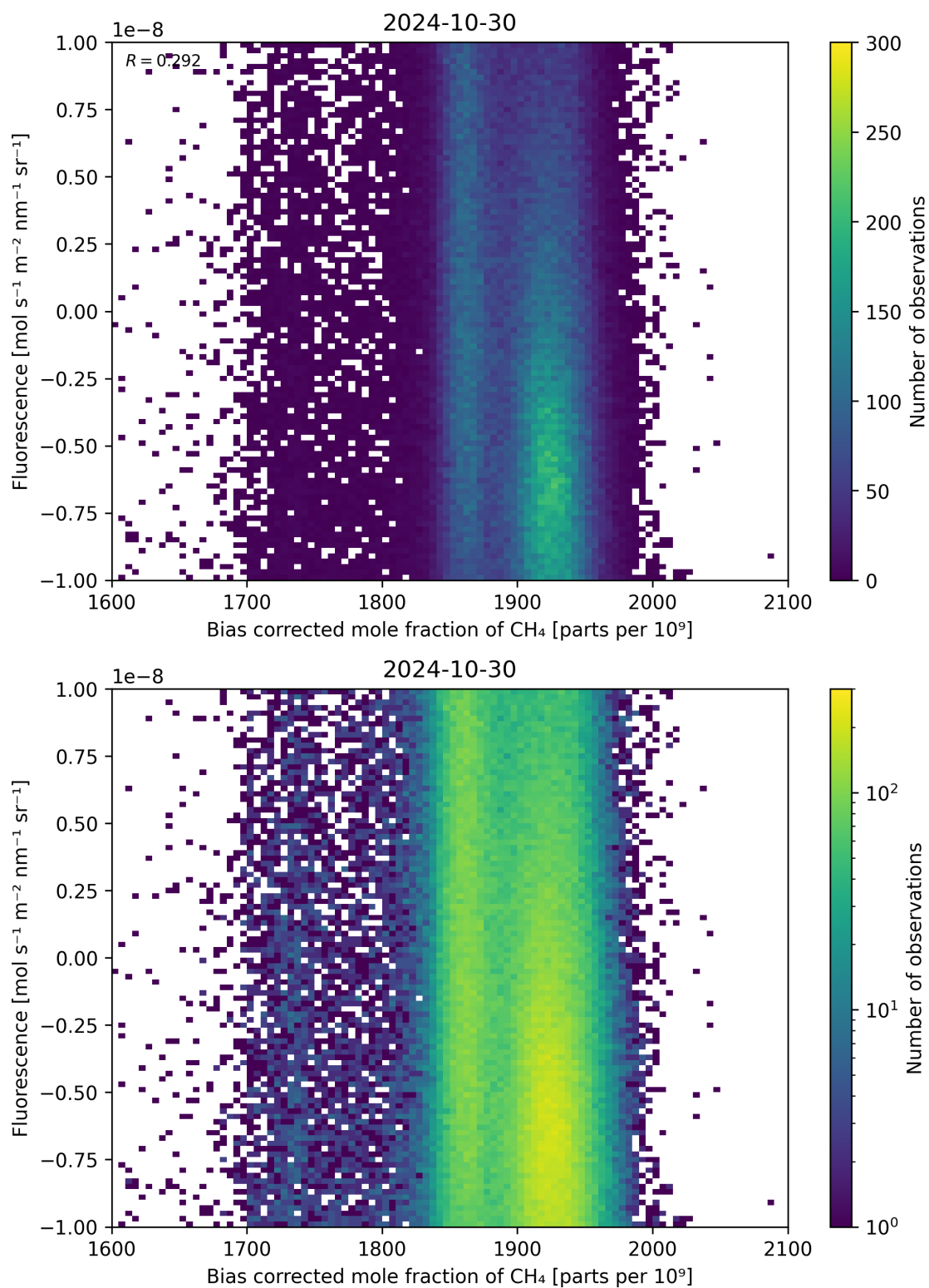
Figure 66: Scatter density plot of “Bias corrected mole fraction of \text{CH}_4 ” against “Fluorescence” for 2024-10-30 to 2024-10-31.
