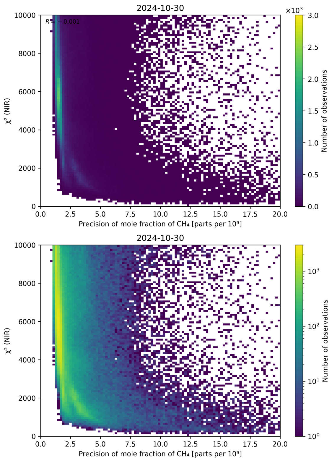
Figure 78: Scatter density plot of “Precision of mole fraction of \text{CH}_4 ” against “ \chi^2 (NIR)” for 2024-10-30 to 2024-10-31.
