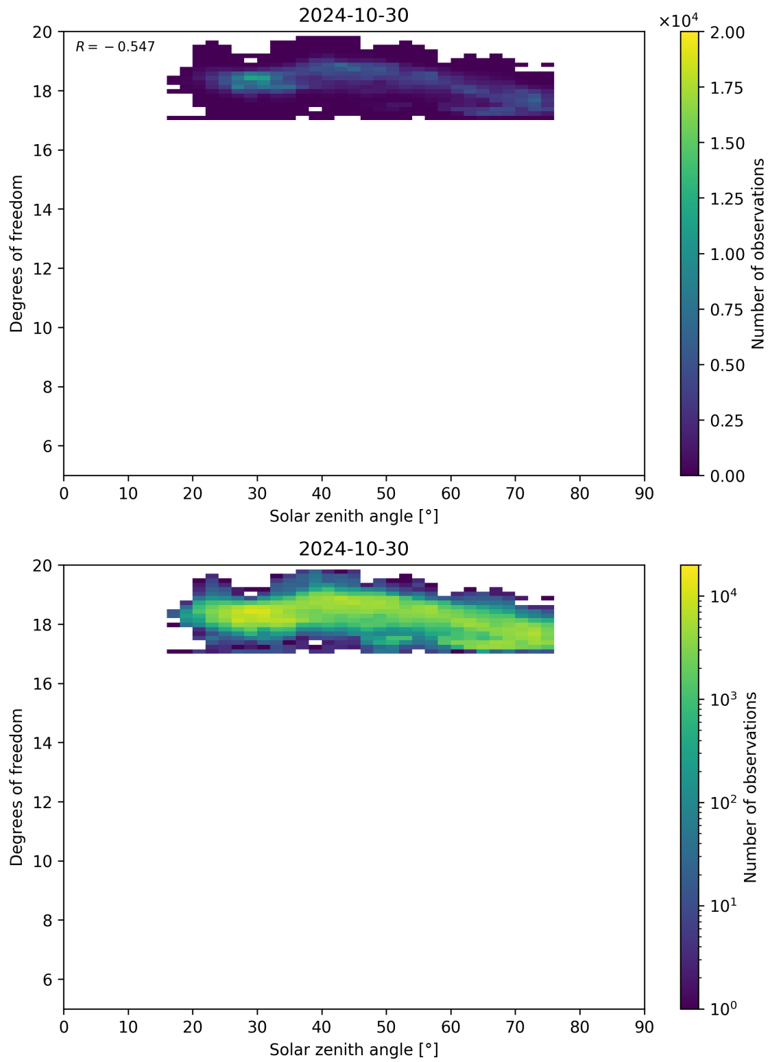
Figure 96: Scatter density plot of “Solar zenith angle” against “Degrees of freedom” for 2024-10-30 to 2024-10-31.
