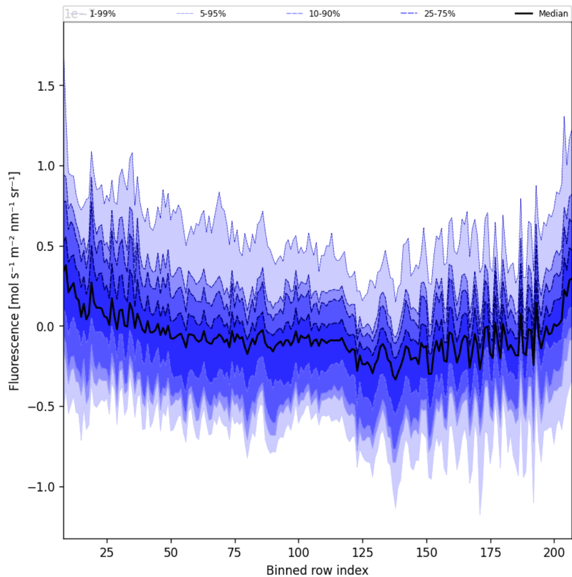
Figure 43: Along track statistics of “Fluorescence” for 2024-10-30 to 2024-10-31
