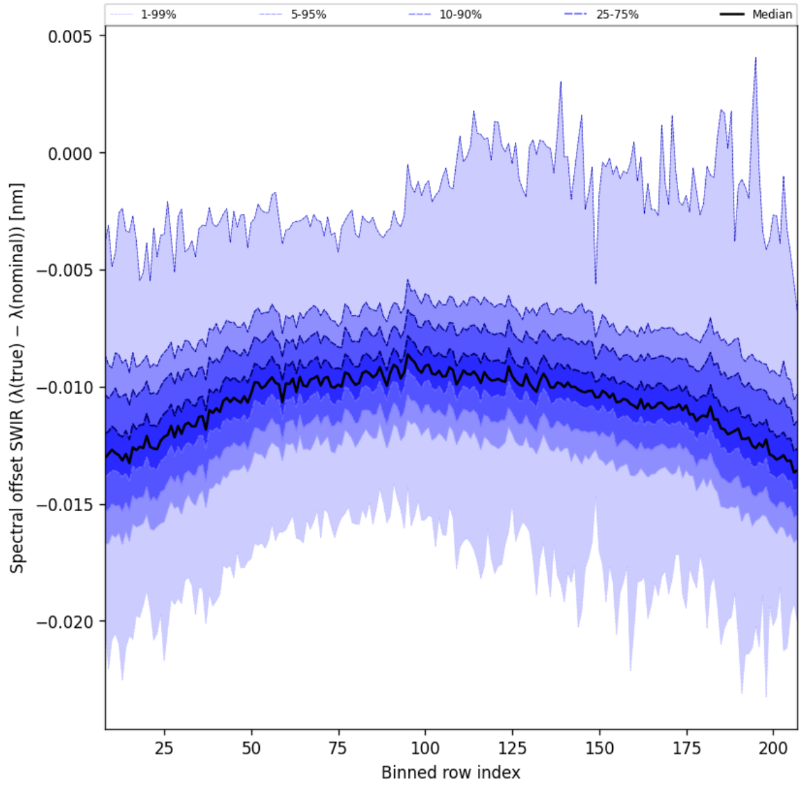
Figure 38: Along track statistics of “Spectral offset SWIR ( \lambda_{\text{true}} - \lambda_{\text{nominal}} )” for 2024-10-30 to 2024-10-31
