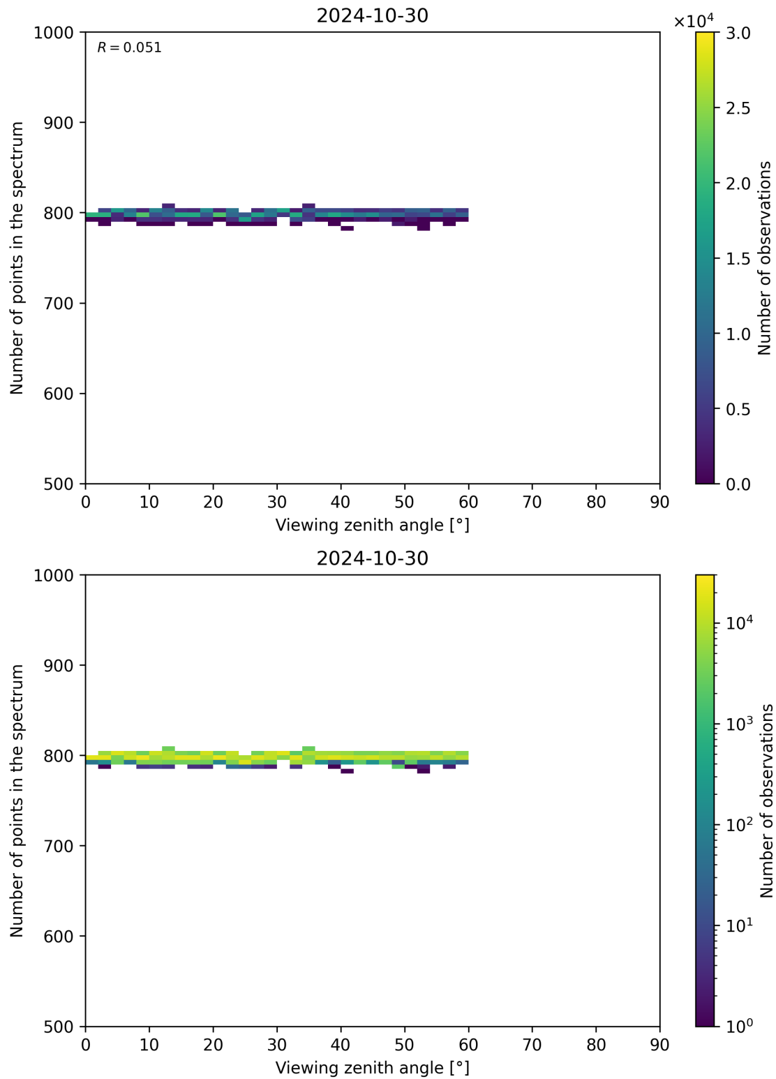
Figure 114: Scatter density plot of “Viewing zenith angle” against “Number of points in the spectrum” for 2024-10-30 to 2024-10-31.
