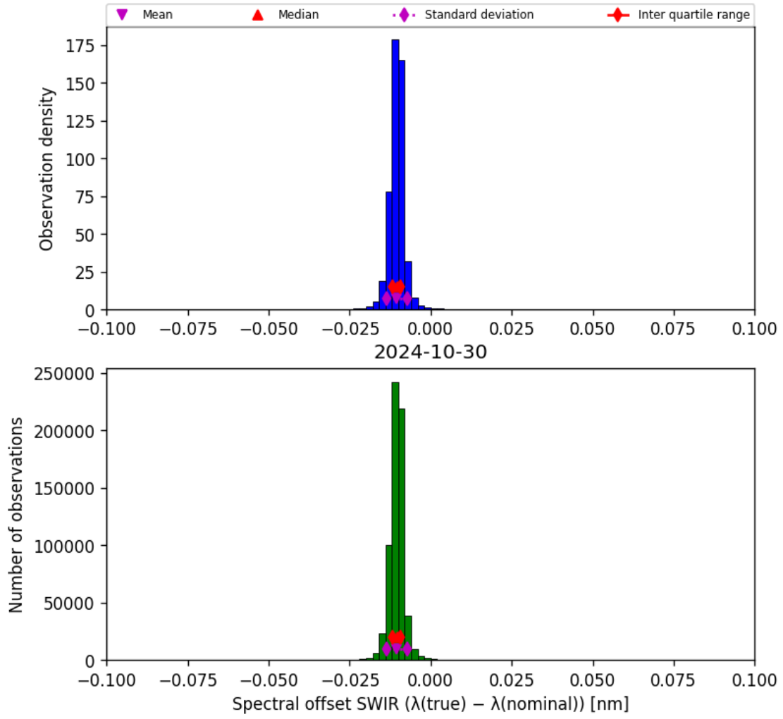
Figure 27: Histogram of “Spectral offset SWIR ( \lambda_{\text{true}} - \lambda_{\text{nominal}} )” for 2024-10-30 to 2024-10-31
