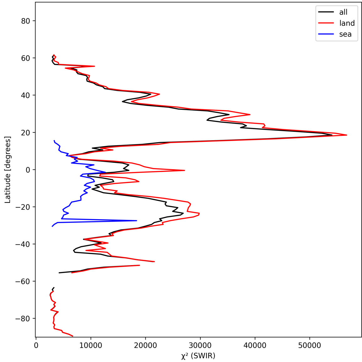
Figure 17: Zonal average of “ \chi^2 (SWIR)” for 2024-10-30 to 2024-10-31.
