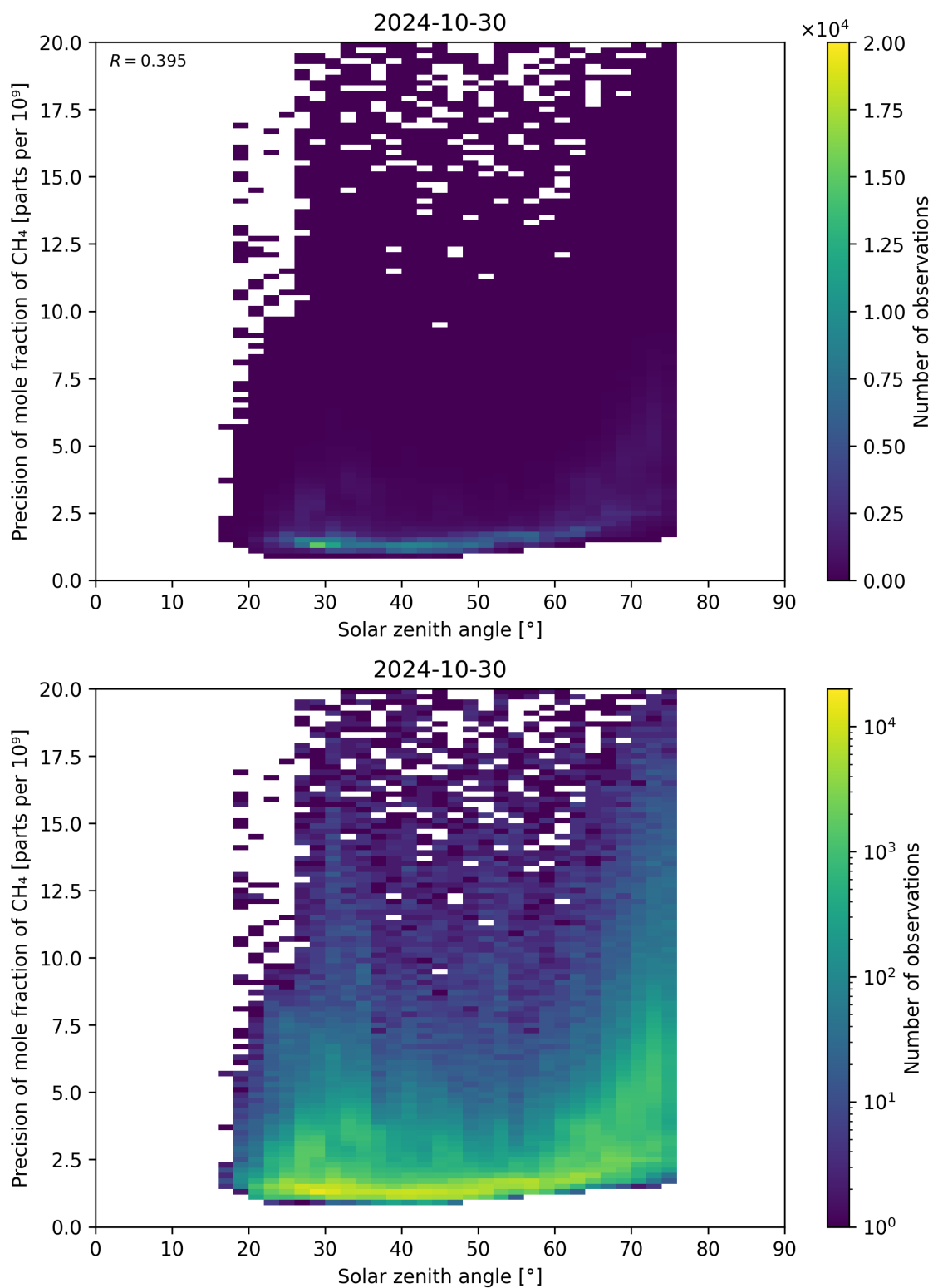
Figure 101: Scatter density plot of “Solar zenith angle” against “Precision of mole fraction of \text{CH}_4 ” for 2024-10-30 to 2024-10-31.
