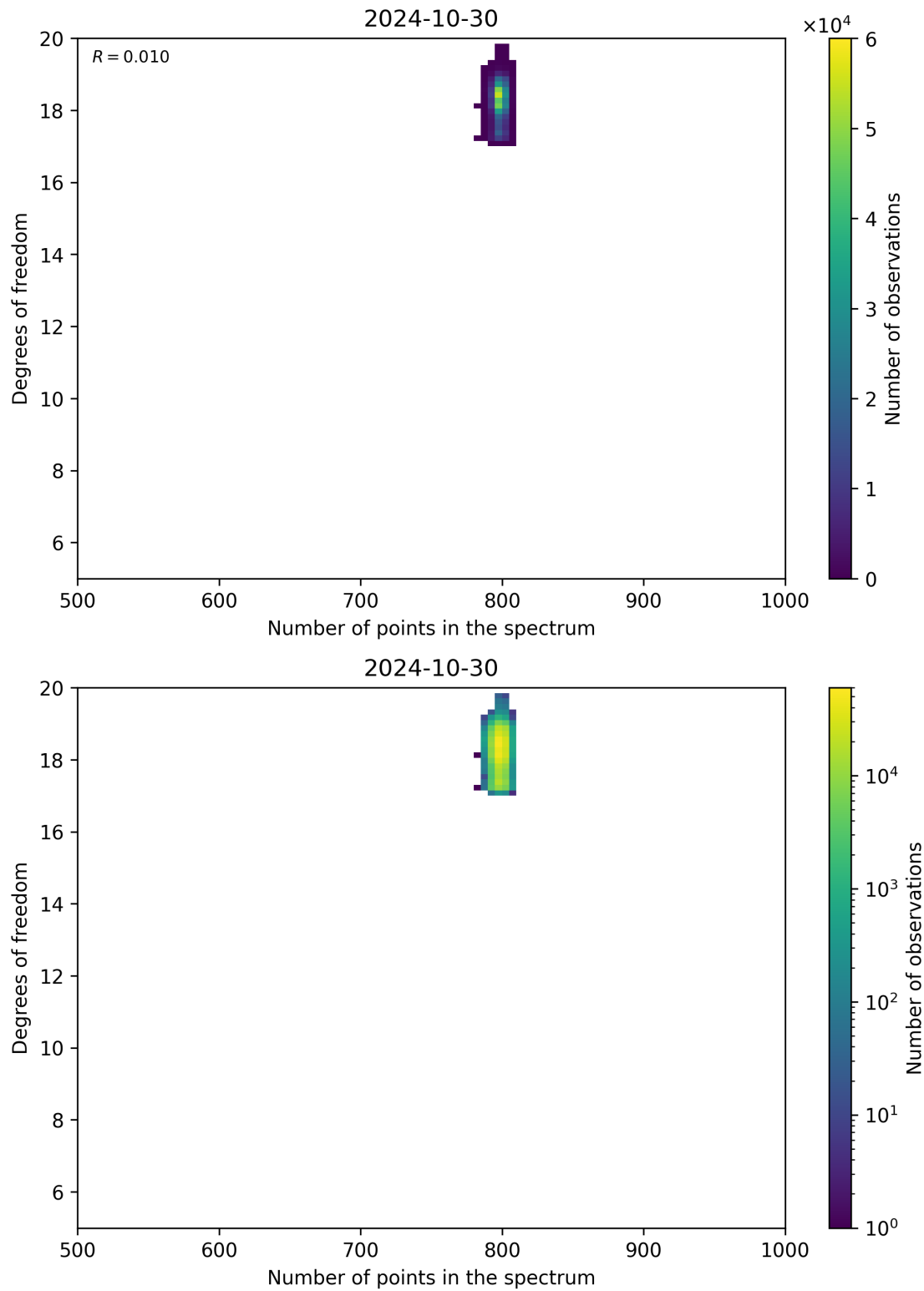
Figure 90: Scatter density plot of “Number of points in the spectrum” against “Degrees of freedom” for 2024-10-30 to 2024-10-31.
