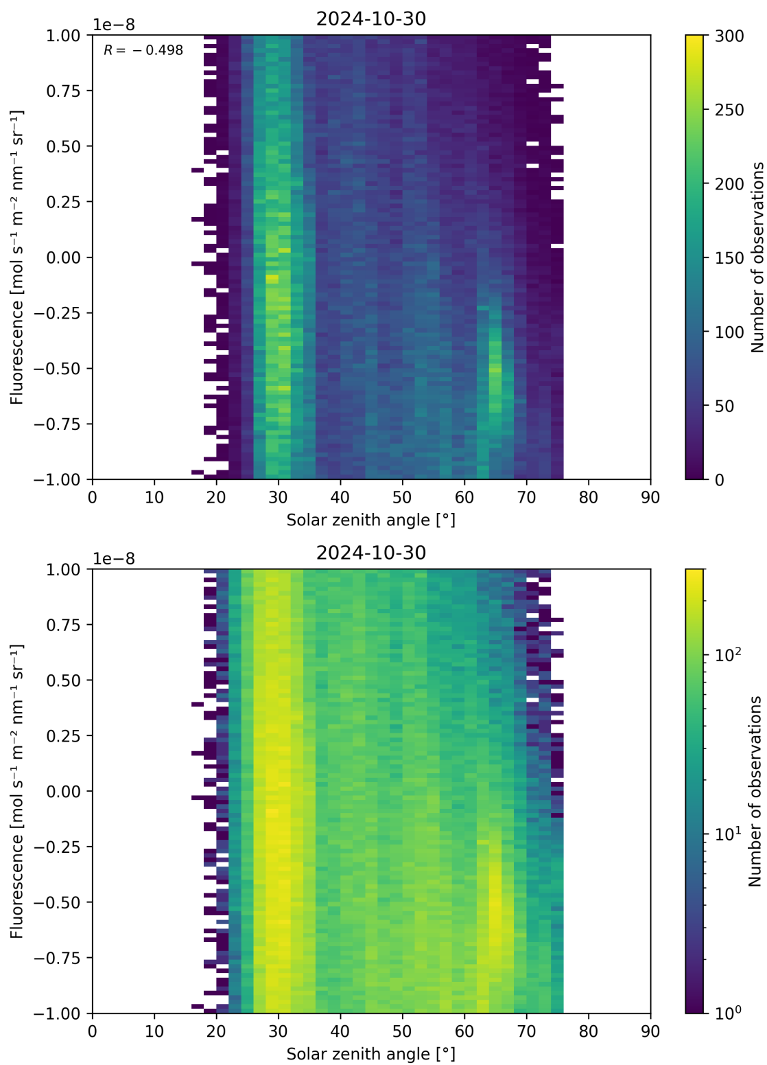
Figure 97: Scatter density plot of “Solar zenith angle” against “Fluorescence” for 2024-10-30 to 2024-10-31.
