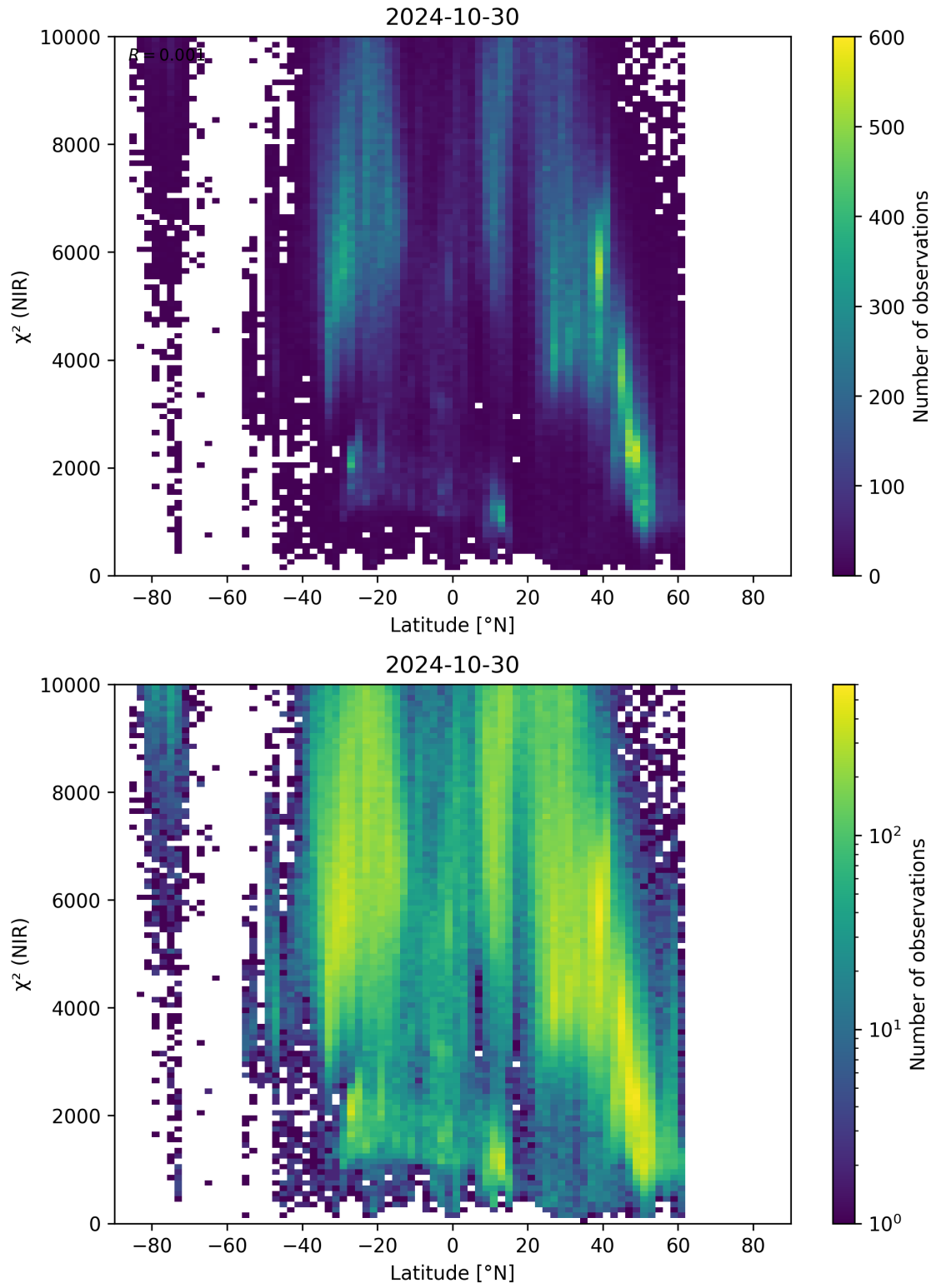
Figure 53: Scatter density plot of “Latitude” against “ \chi^2 (NIR)” for 2024-10-30 to 2024-10-31.
