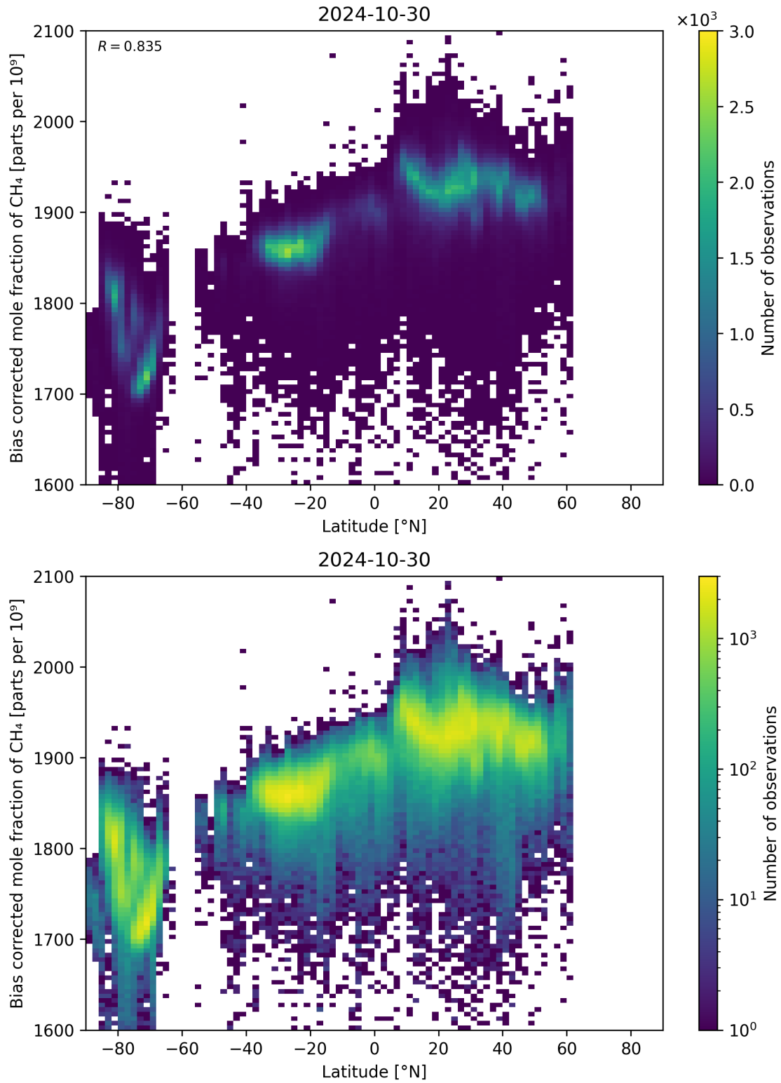
Figure 58: Scatter density plot of “Latitude” against “Bias corrected mole fraction of CH 4 ” for 2024-10-30 to 2024-10-31.
