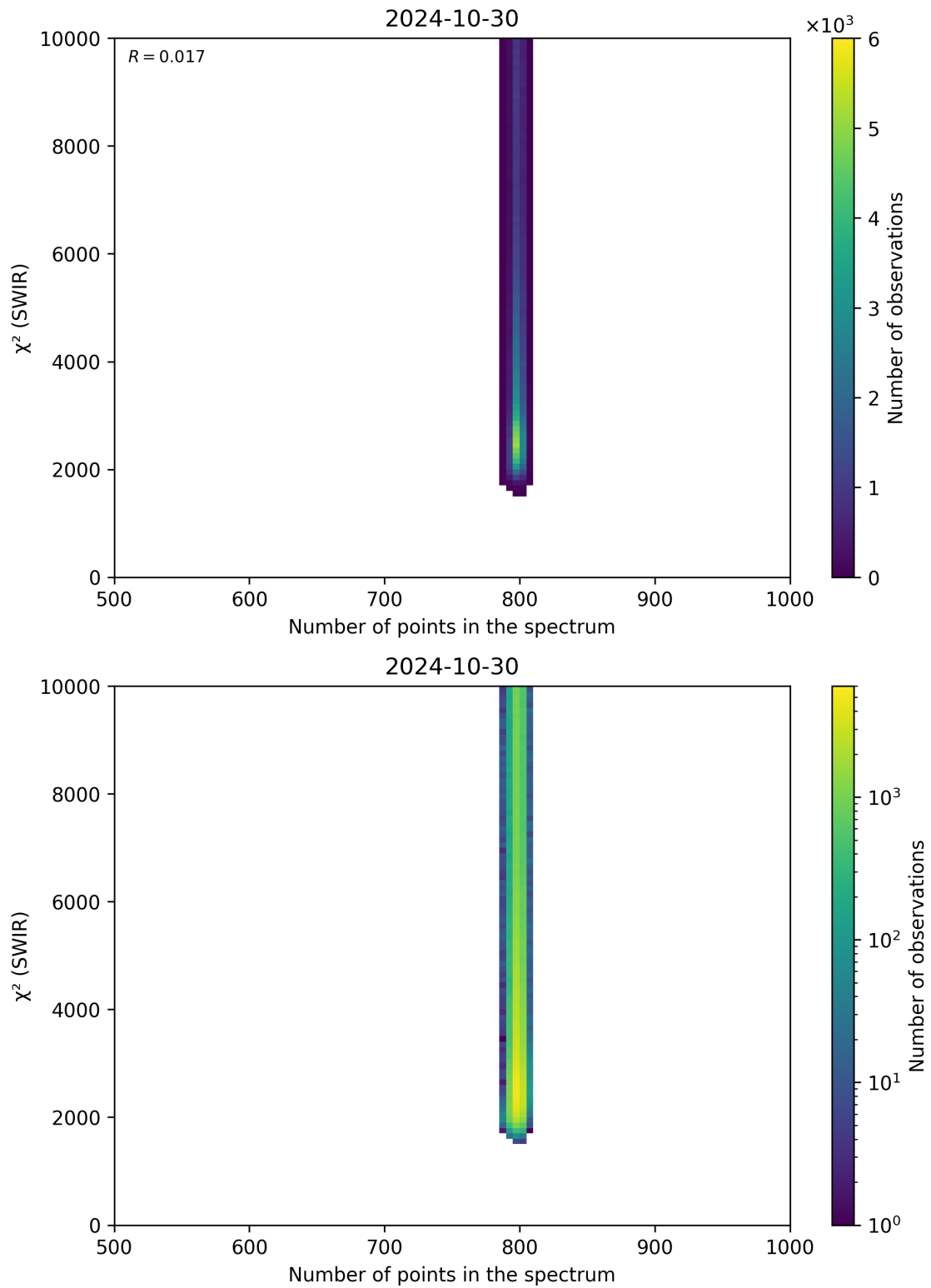
Figure 89: Scatter density plot of “Number of points in the spectrum” against “ \chi^2 (SWIR)” for 2024-10-30 to 2024-10-31.
