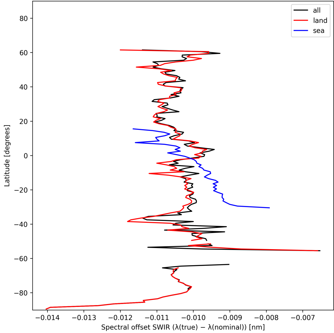
Figure 16: Zonal average of “Spectral offset SWIR ( \lambda_{\text{true}} - \lambda_{\text{nominal}} )” for 2024-10-30 to 2024-10-31.
