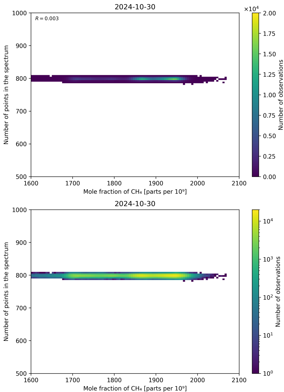
Figure 77: Scatter density plot of “Mole fraction of CH 4 ” against “Number of points in the spectrum” for 2024-10-30 to 2024-10-31.
