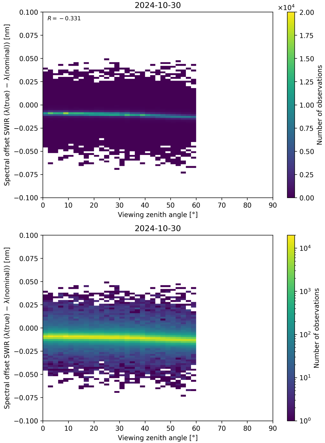
Figure 116: Scatter density plot of “Viewing zenith angle” against “Spectral offset SWIR ( \lambda_{\text{true}} - \lambda_{\text{nominal}} )” for 2024-10-30 to 2024-10-31.
