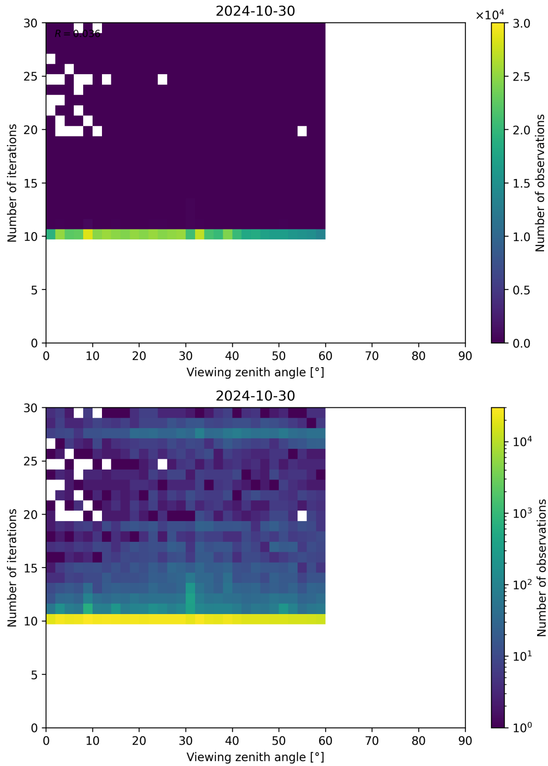
Figure 113: Scatter density plot of “Viewing zenith angle” against “Number of iterations” for 2024-10-30 to 2024-10-31.
