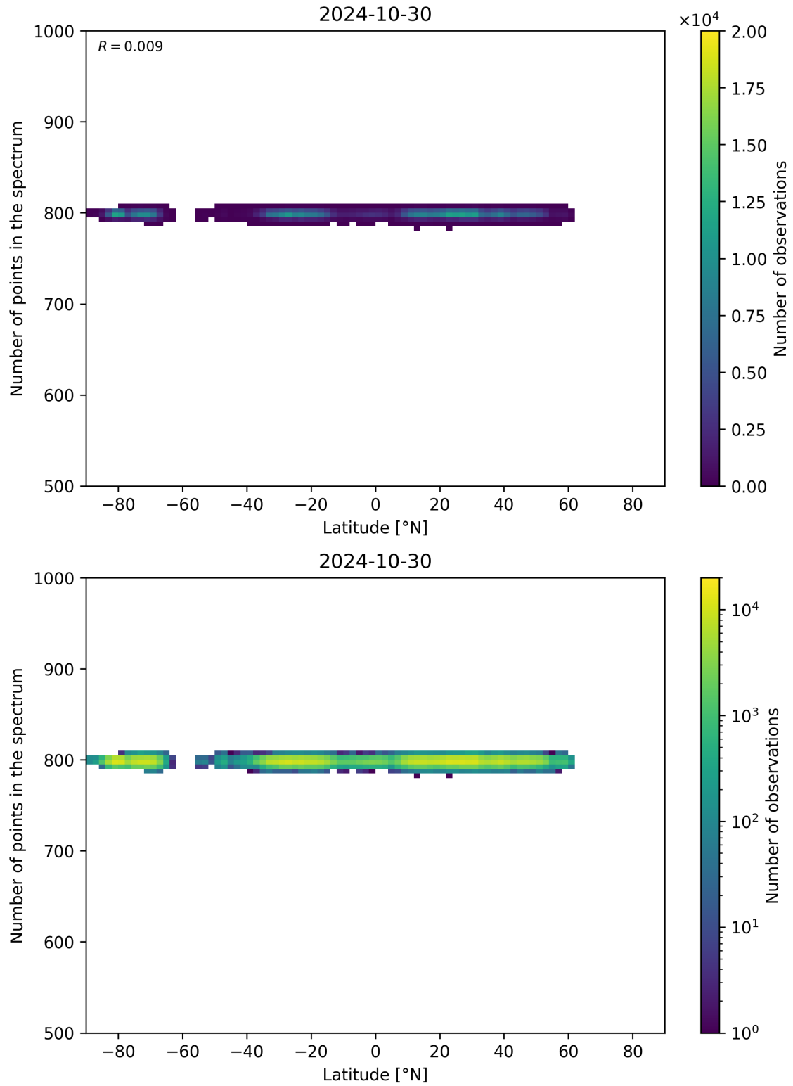
Figure 61: Scatter density plot of “Latitude” against “Number of points in the spectrum” for 2024-10-30 to 2024-10-31.
