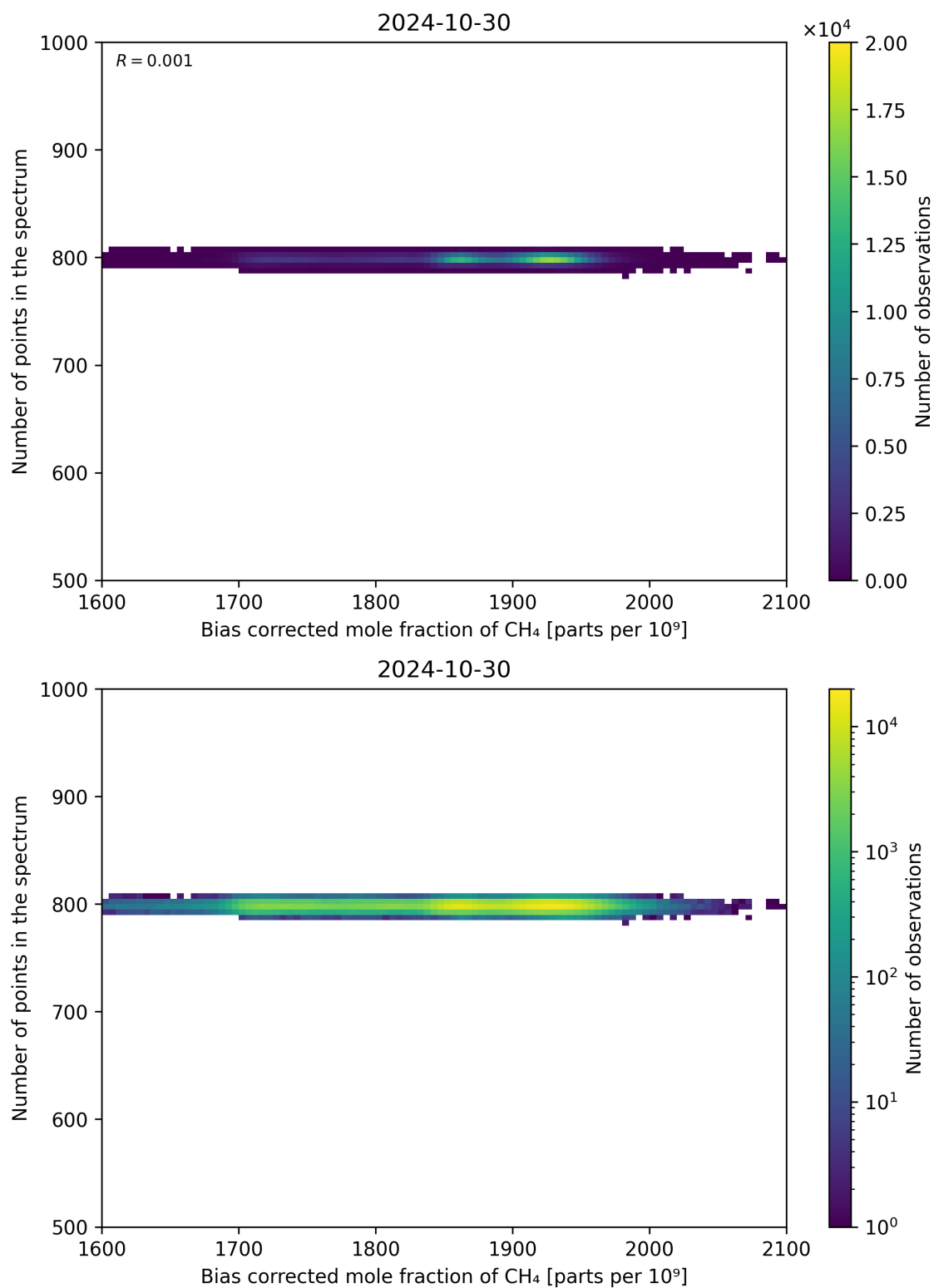
Figure 68: Scatter density plot of “Bias corrected mole fraction of CH 4 ” against “Number of points in the spectrum” for 2024-10-30 to 2024-10-31.
