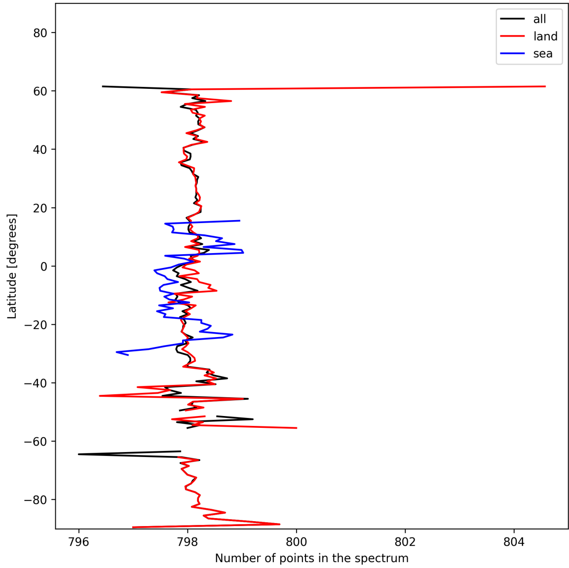
Figure 15: Zonal average of “Number of points in the spectrum” for 2024-10-30 to 2024-10-31.
