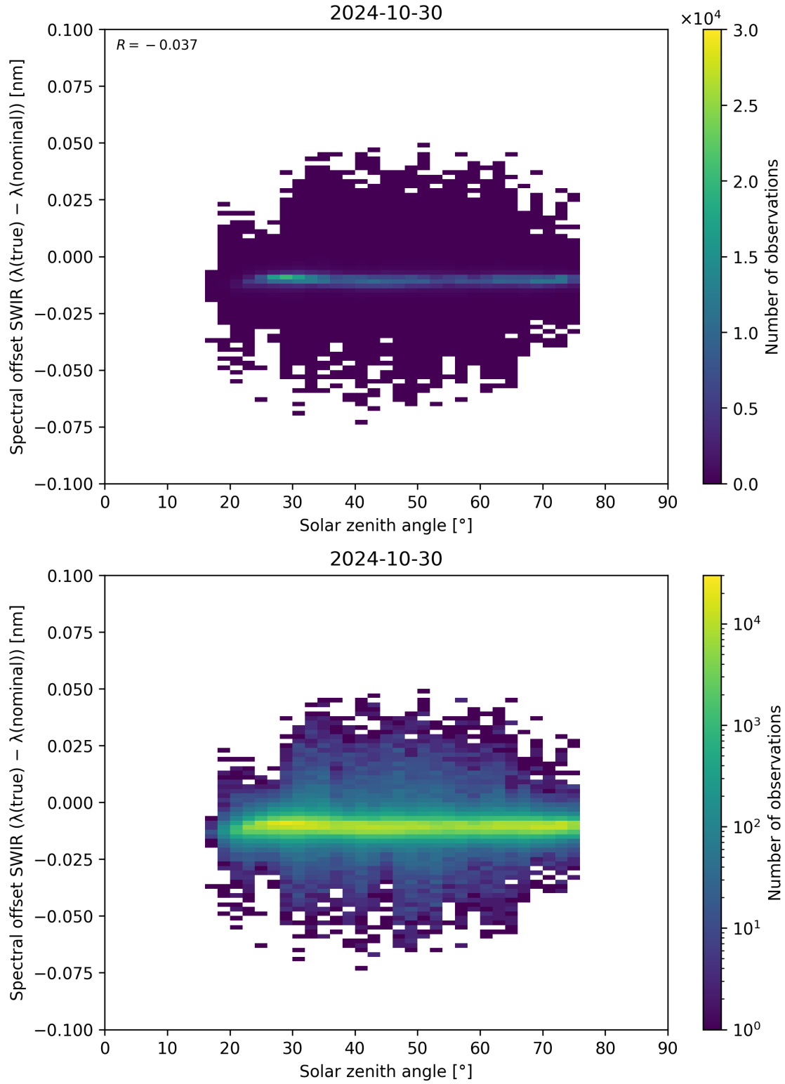
Figure 104: Scatter density plot of “Solar zenith angle” against “Spectral offset SWIR ( \lambda_{\text{true}} - \lambda_{\text{nominal}} )” for 2024-10-30 to 2024-10-31.
