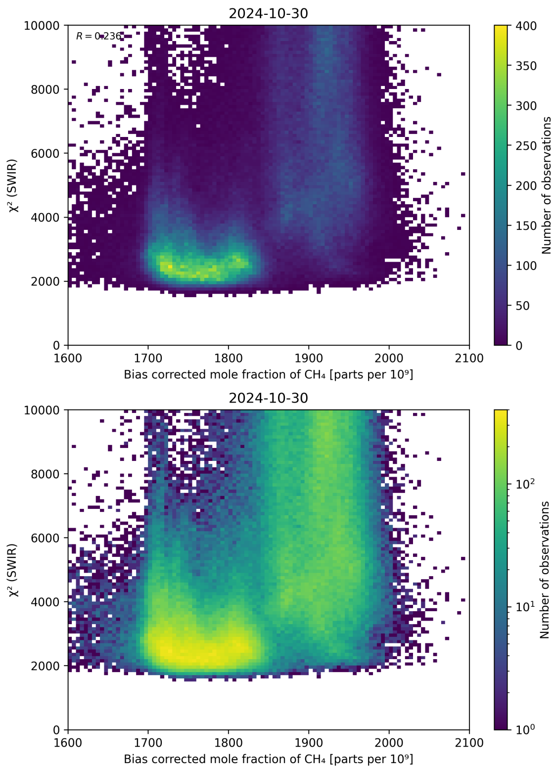
Figure 64: Scatter density plot of “Bias corrected mole fraction of \text{CH}_4 ” against “ \chi^2 (SWIR)” for 2024-10-30 to 2024-10-31.
