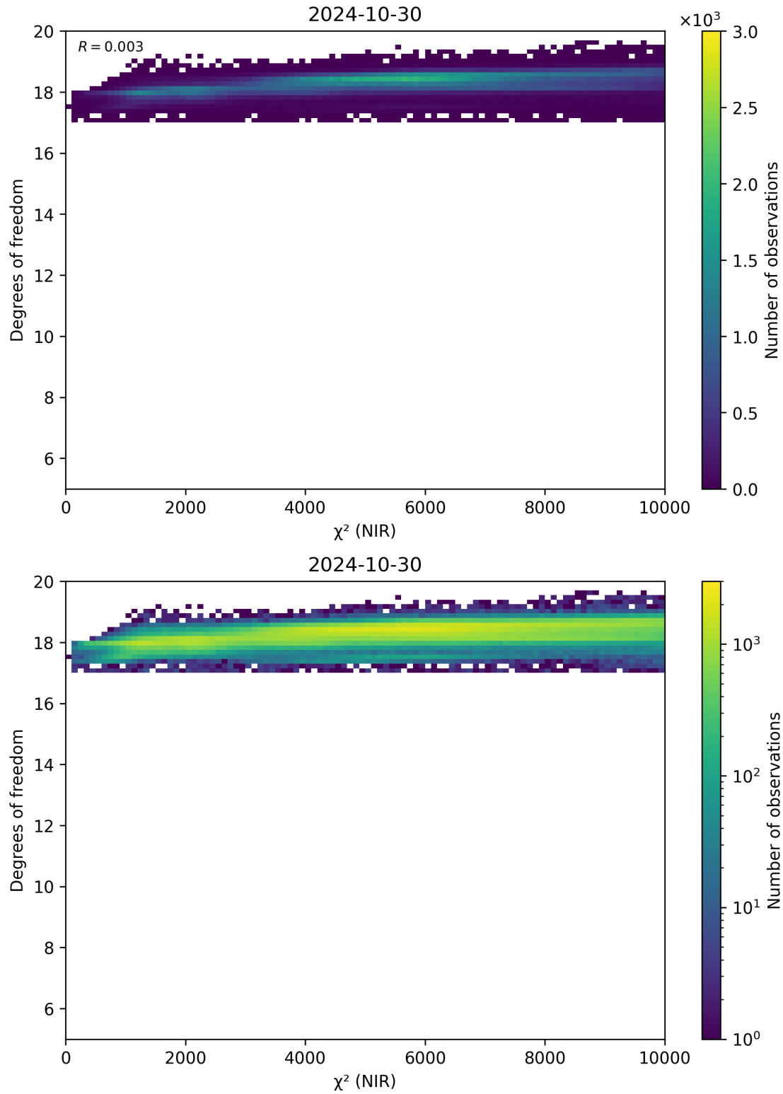
Figure 44: Scatter density plot of “ \chi^2 (NIR)” against “Degrees of freedom” for 2024-10-30 to 2024-10-31.
