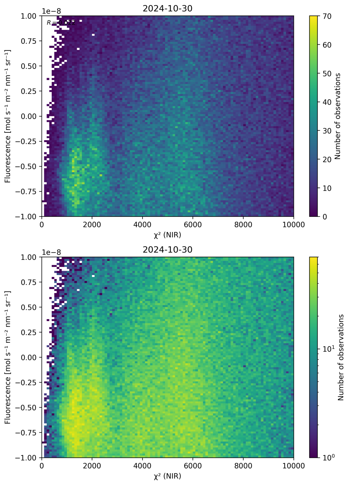
Figure 45: Scatter density plot of “ \chi^2 (NIR)” against “Fluorescence” for 2024-10-30 to 2024-10-31.
