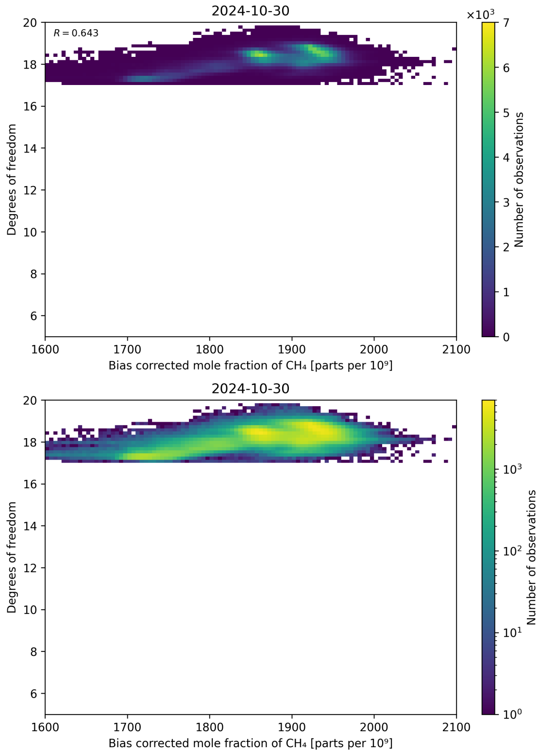
Figure 65: Scatter density plot of “Bias corrected mole fraction of CH 4 ” against “Degrees of freedom” for 2024-10-30 to 2024-10-31.
