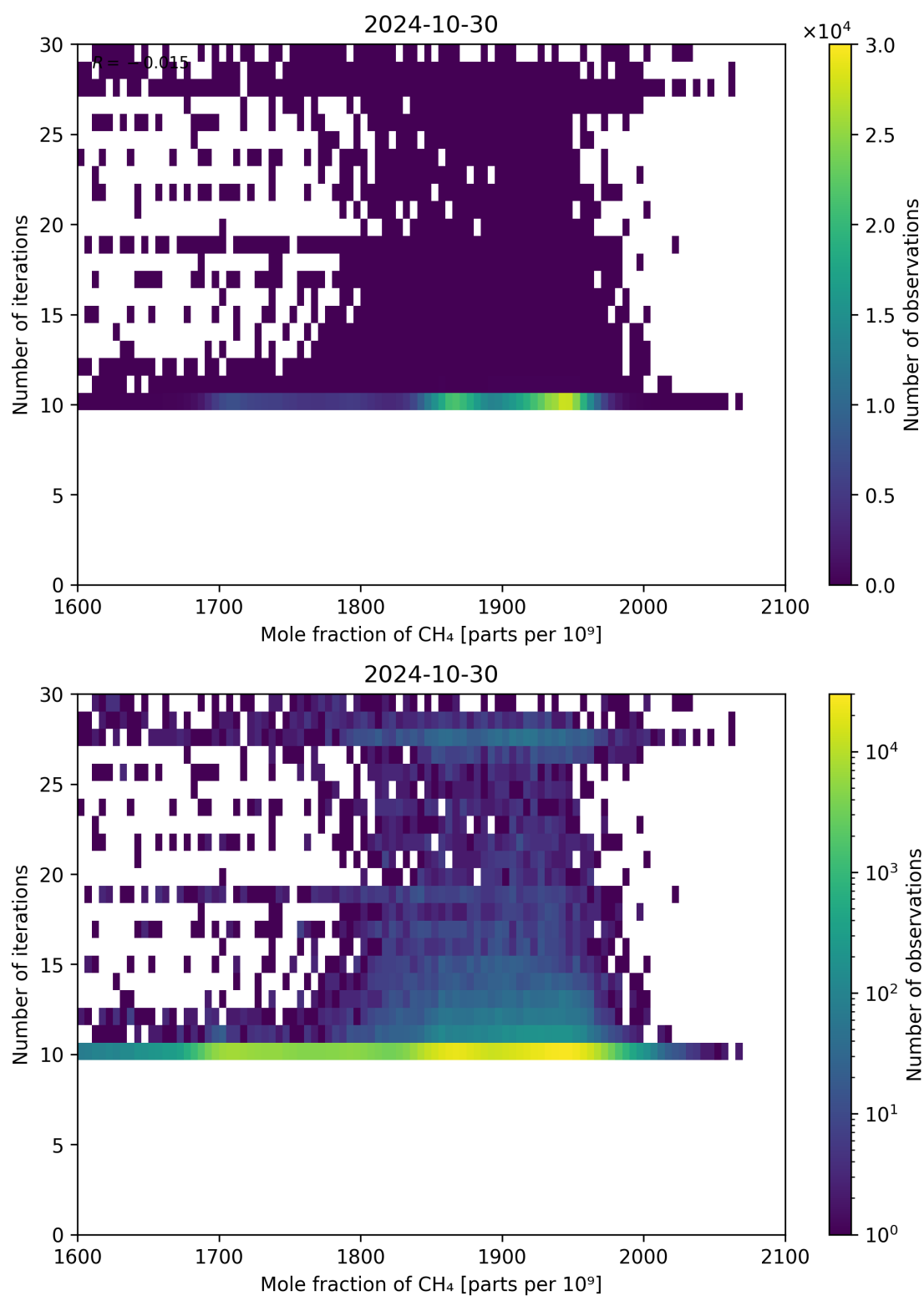
Figure 76: Scatter density plot of “Mole fraction of CH 4 ” against “Number of iterations” for 2024-10-30 to 2024-10-31.
