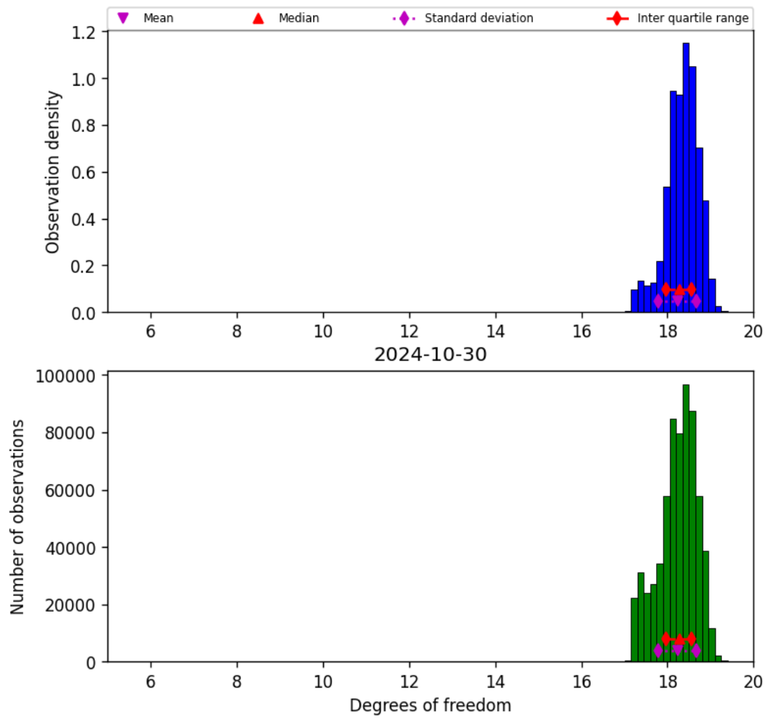
Figure 30: Histogram of “Degrees of freedom” for 2024-10-30 to 2024-10-31
