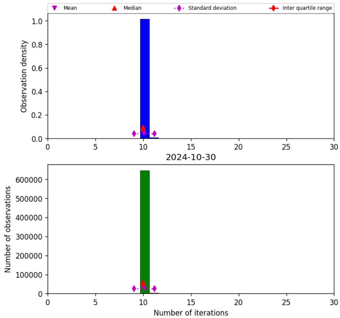
Figure 31: Histogram of “Number of iterations” for 2024-10-30 to 2024-10-31
