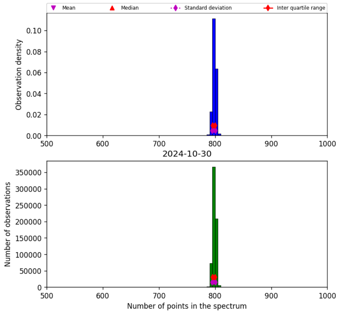
Figure 26: Histogram of “Number of points in the spectrum” for 2024-10-30 to 2024-10-31
