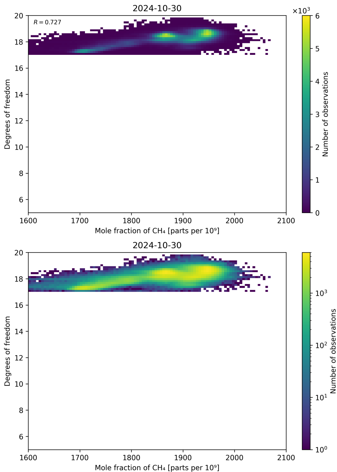
Figure 72: Scatter density plot of “Mole fraction of CH 4 ” against “Degrees of freedom” for 2024-10-30 to 2024-10-31.
