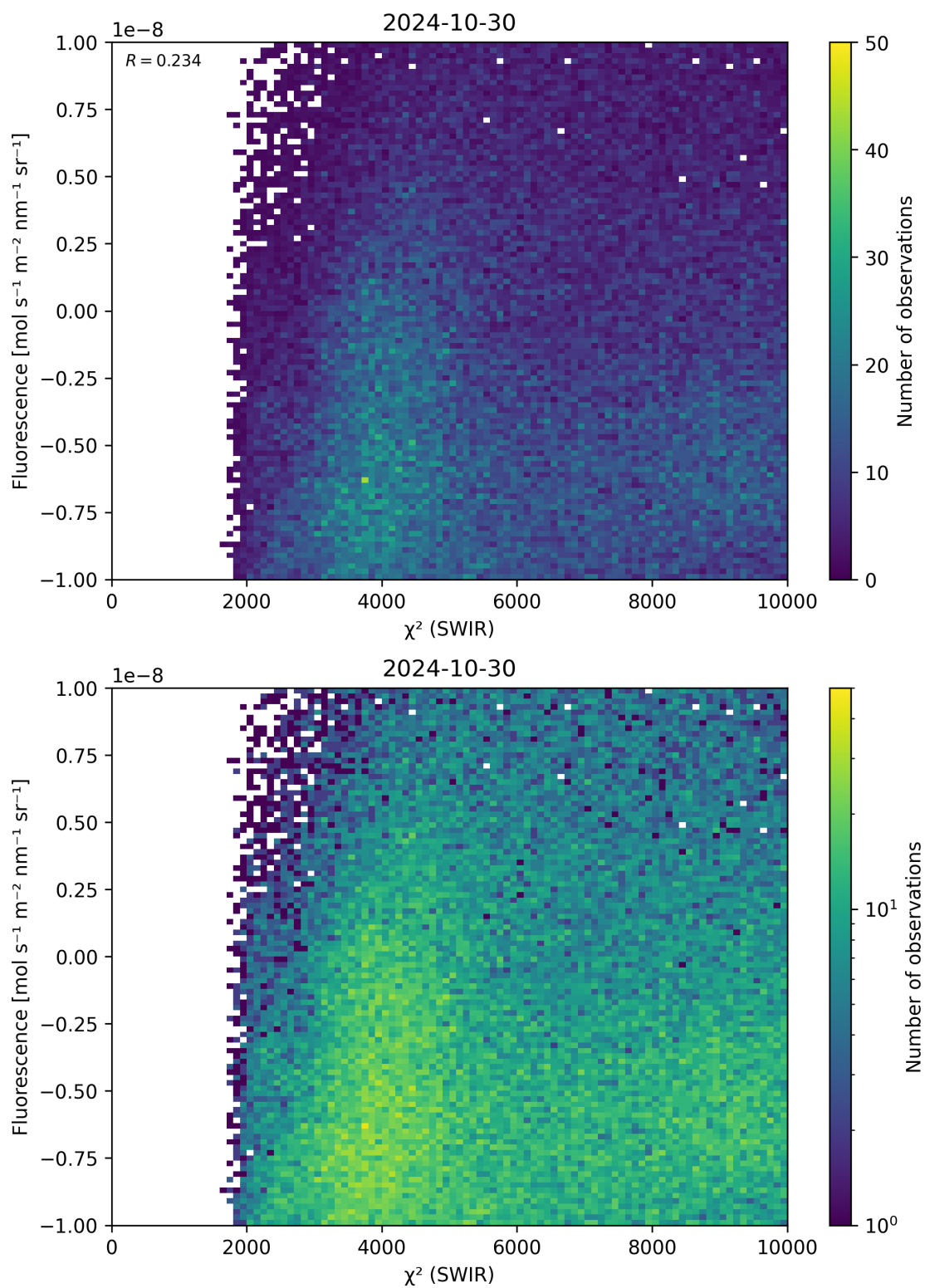
Figure 49: Scatter density plot of “ \chi^2 (SWIR)” against “Fluorescence” for 2024-10-30 to 2024-10-31.
