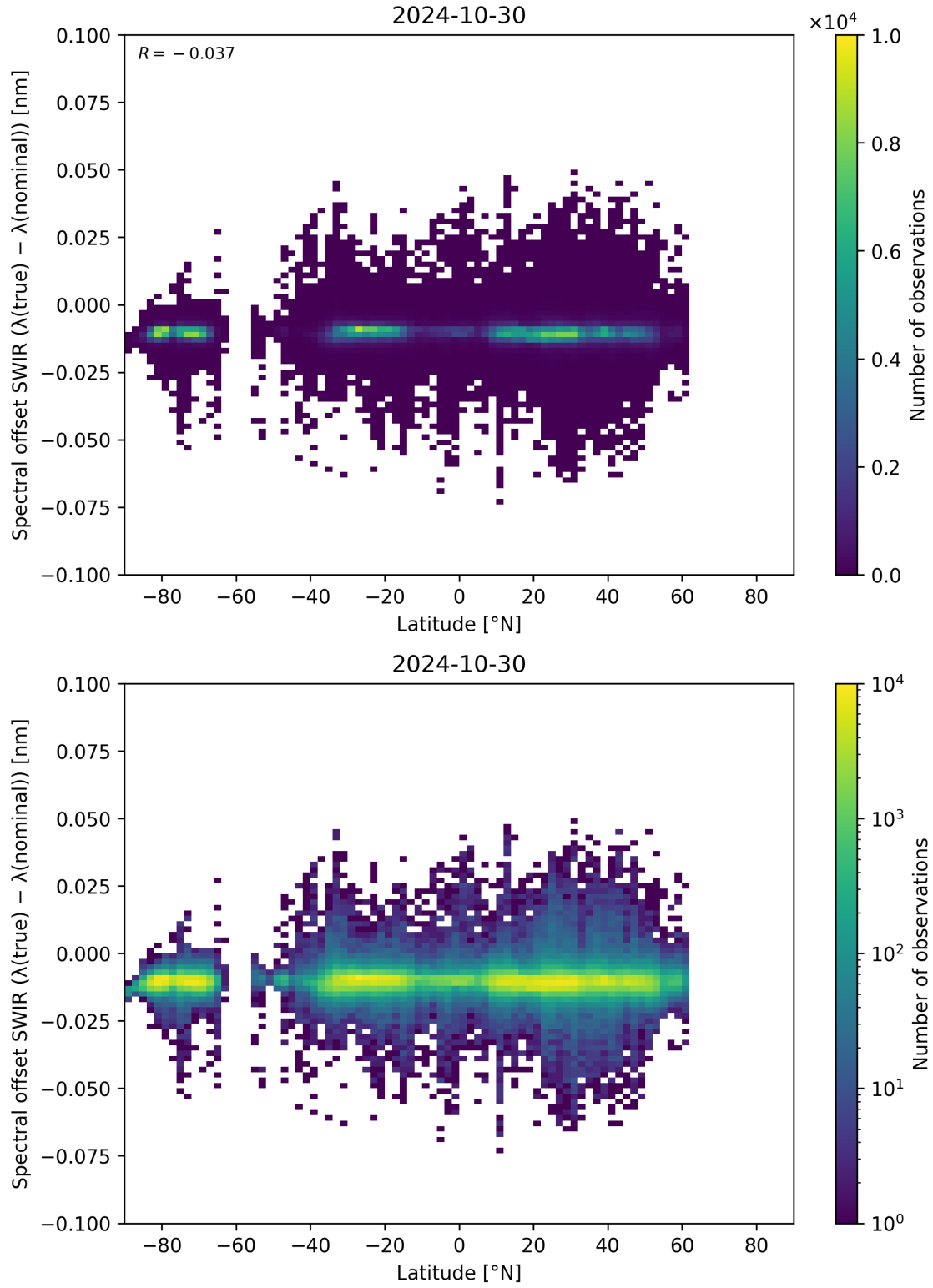
Figure 62: Scatter density plot of “Latitude” against “Spectral offset SWIR ( \lambda_{\text{true}} - \lambda_{\text{nominal}} )” for 2024-10-30 to 2024-10-31.
