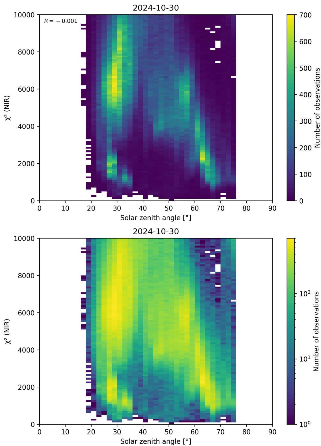
Figure 94: Scatter density plot of “Solar zenith angle” against “ \chi^2 (NIR)” for 2024-10-30 to 2024-10-31.
