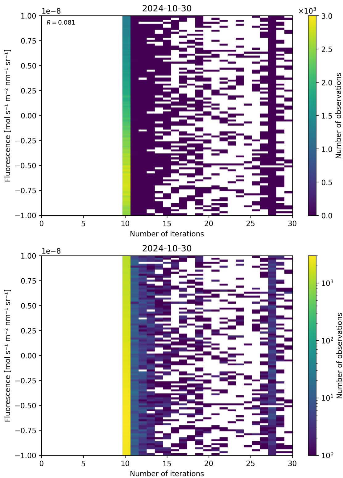
Figure 87: Scatter density plot of "Number of iterations" against "Fluorescence" for 2024-10-30 to 2024-10-31.
