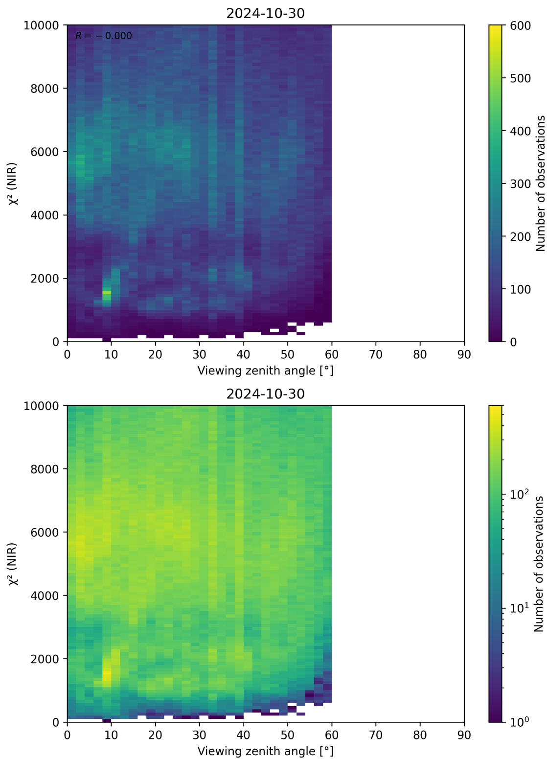
Figure 105: Scatter density plot of “Viewing zenith angle” against “ \chi^2 (NIR)” for 2024-10-30 to 2024-10-31.
