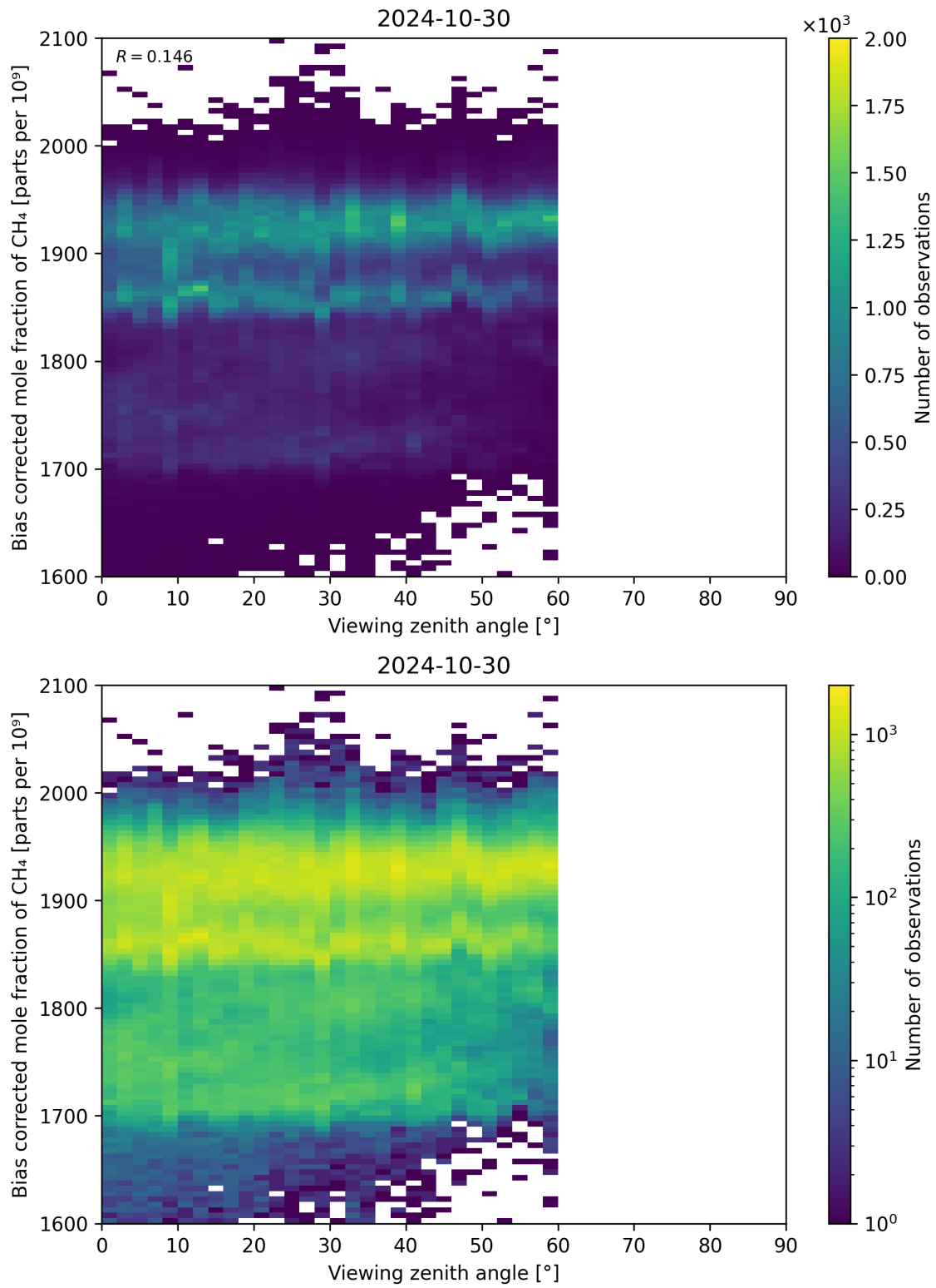
Figure 111: Scatter density plot of “Viewing zenith angle” against “Bias corrected mole fraction of CH 4 ” for 2024-10-30 to 2024-10-31.
