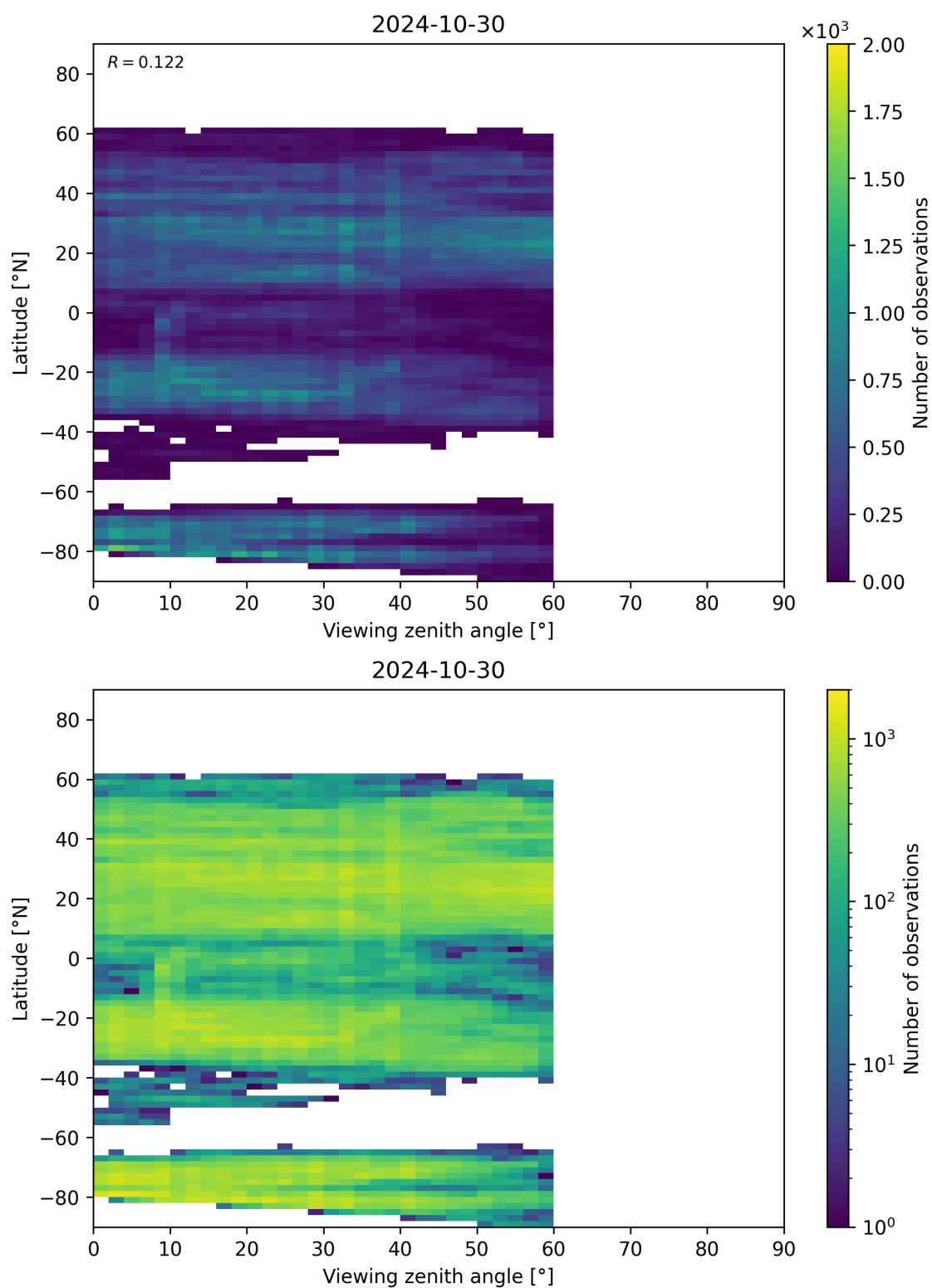
Figure 109: Scatter density plot of “Viewing zenith angle” against “Latitude” for 2024-10-30 to 2024-10-31.
