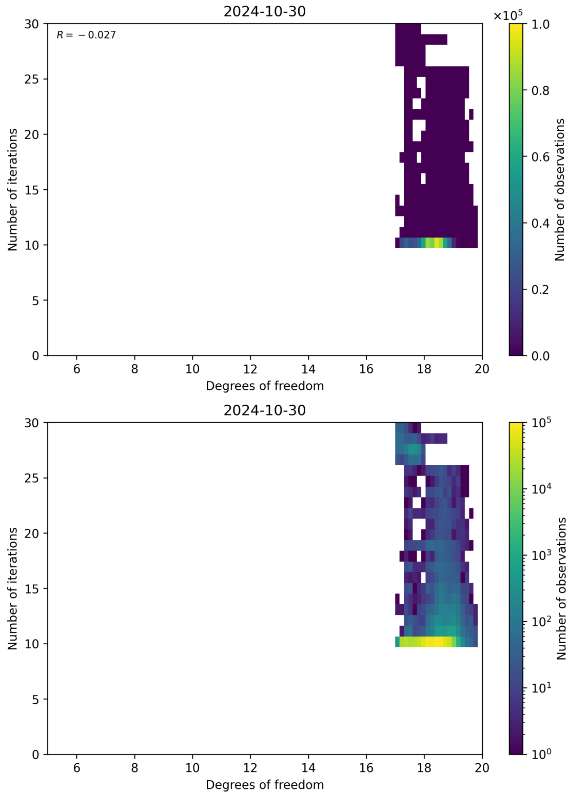
Figure 52: Scatter density plot of “Degrees of freedom” against “Number of iterations” for 2024-10-30 to 2024-10-31.
