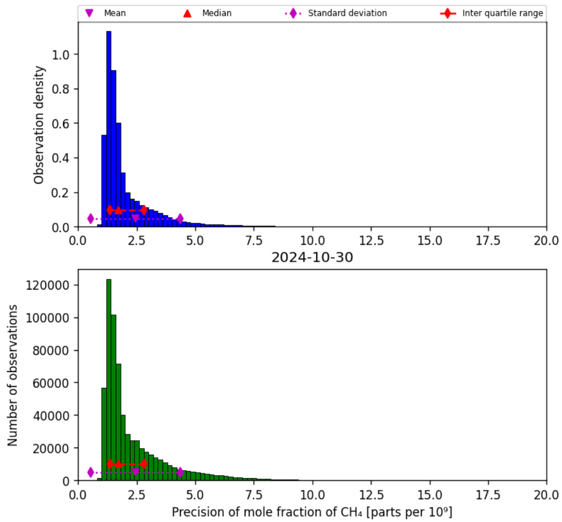
Figure 24: Histogram of “Precision of mole fraction of CH 4 ” for 2024-10-30 to 2024-10-31
