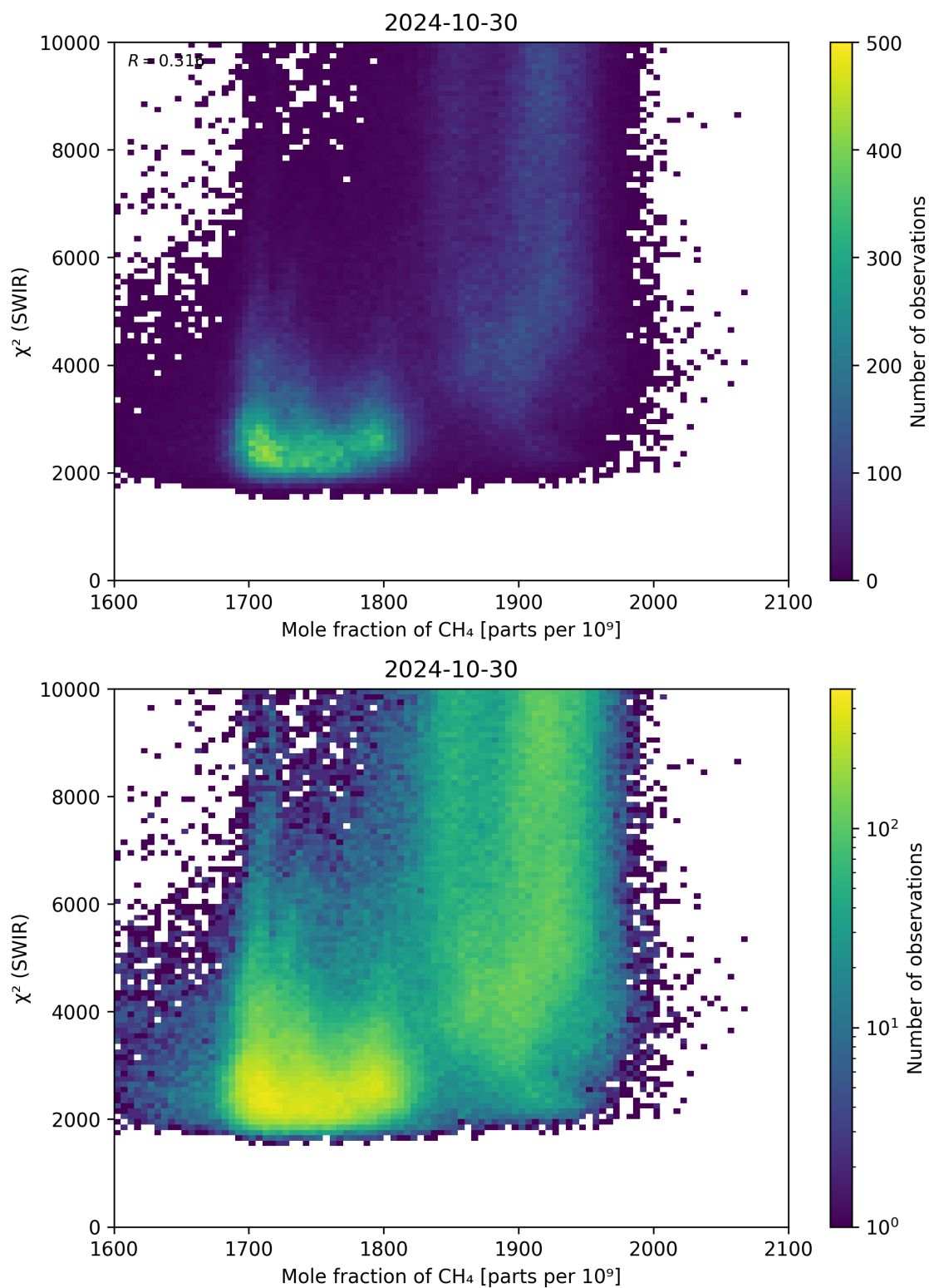
Figure 71: Scatter density plot of “Mole fraction of \text{CH}_4 ” against “ \chi^2 (SWIR)” for 2024-10-30 to 2024-10-31.
