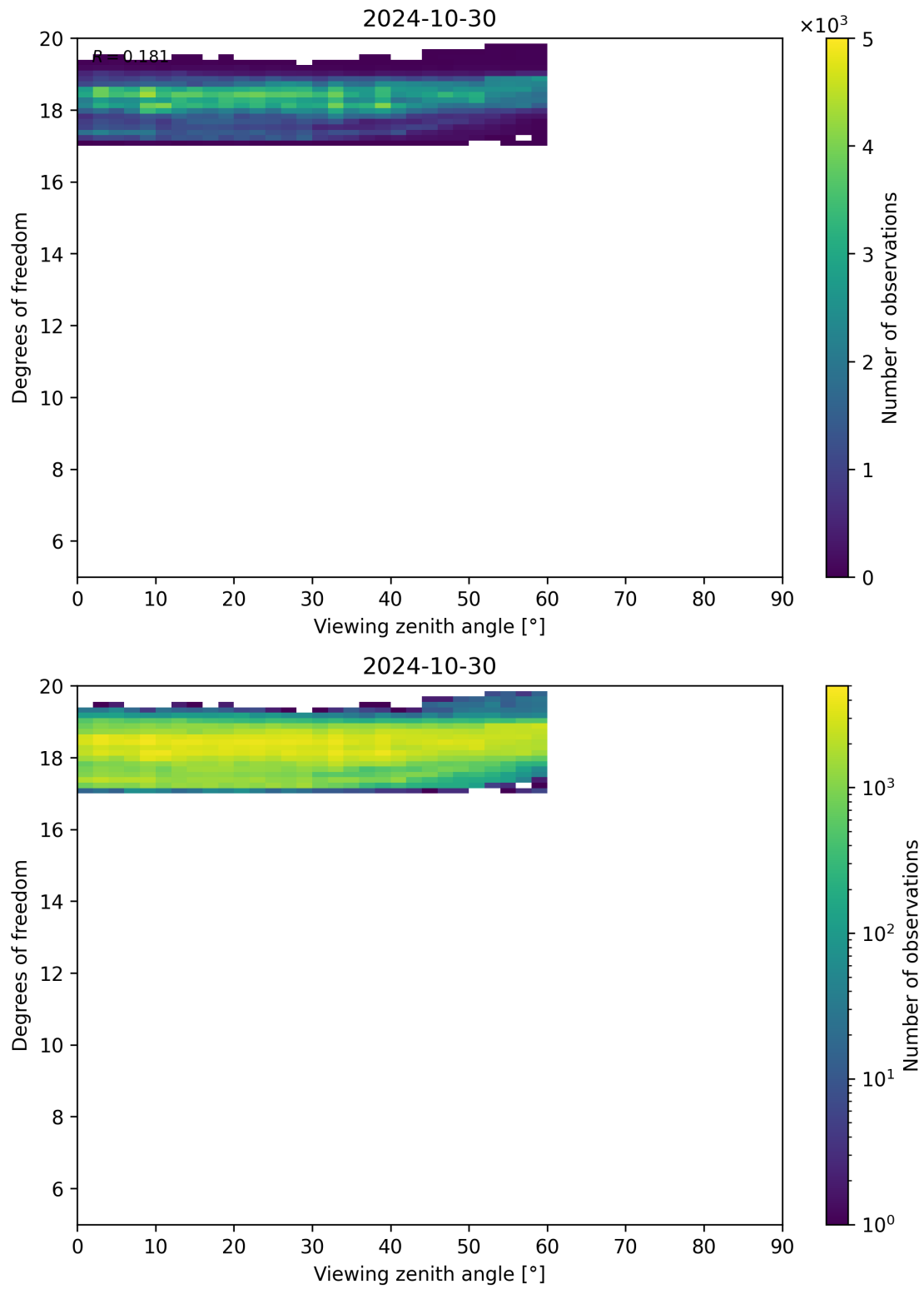
Figure 107: Scatter density plot of “Viewing zenith angle” against “Degrees of freedom” for 2024-10-30 to 2024-10-31.
