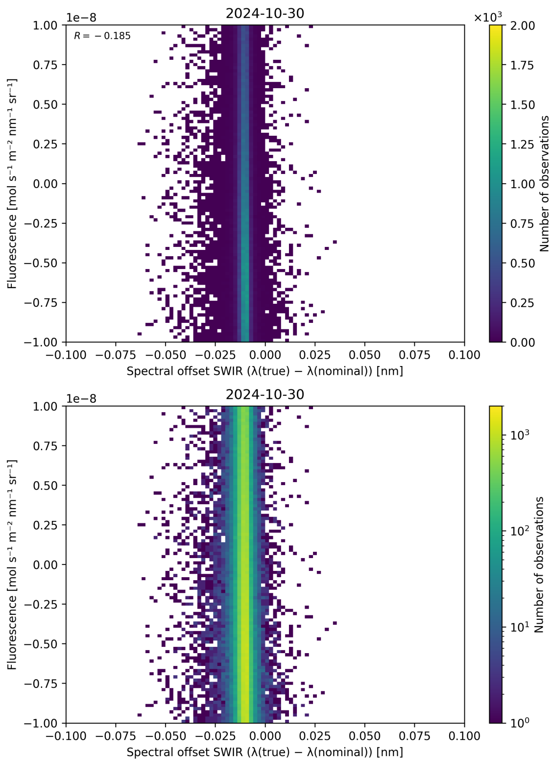
Figure 120: Scatter density plot of “Spectral offset SWIR ( \lambda_{\text{true}} - \lambda_{\text{nominal}} )” against “Fluorescence” for 2024-10-30 to 2024-10-31.
