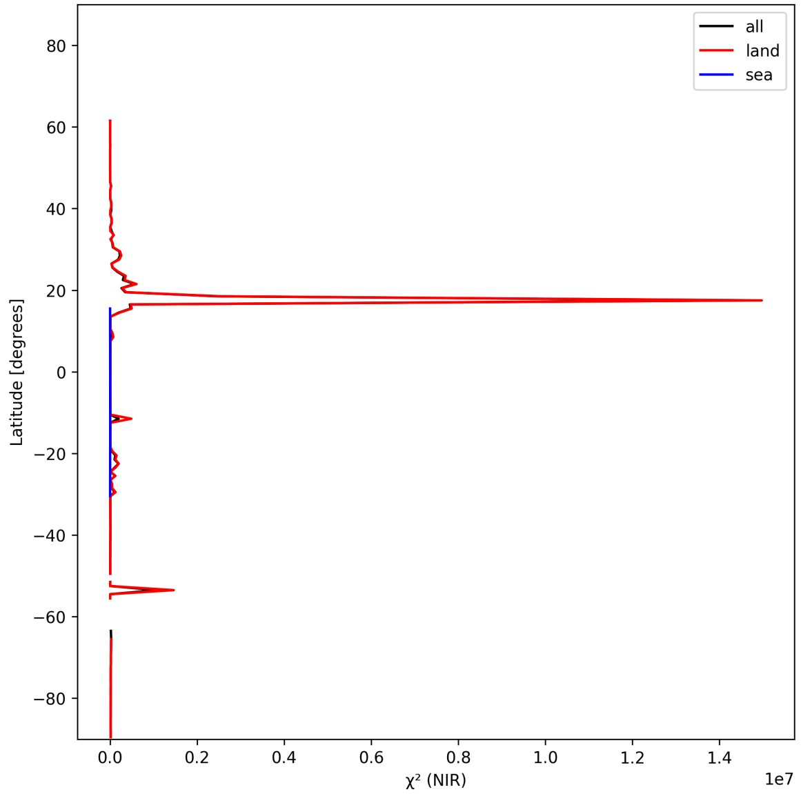
Figure 18: Zonal average of “ \chi^2 (NIR)” for 2024-10-30 to 2024-10-31.
