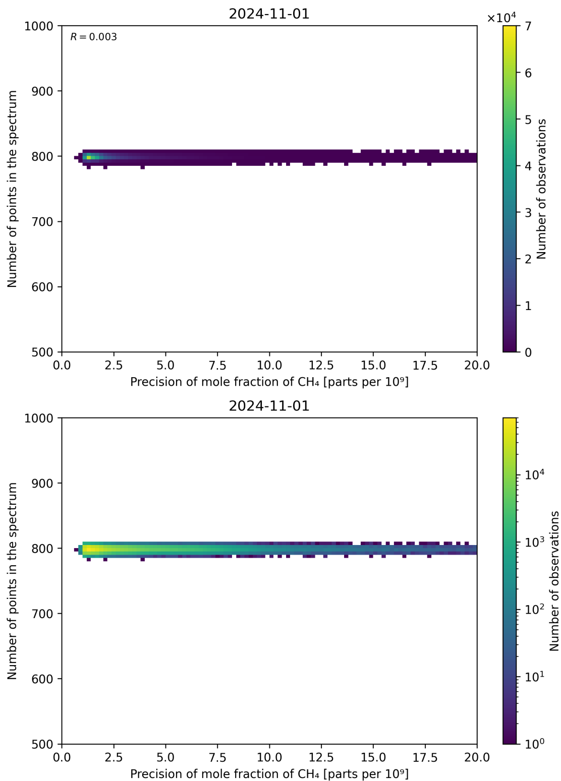
Figure 84: Scatter density plot of “Precision of mole fraction of CH 4 ” against “Number of points in the spectrum” for 2024-10-31 to 2024-11-02.
