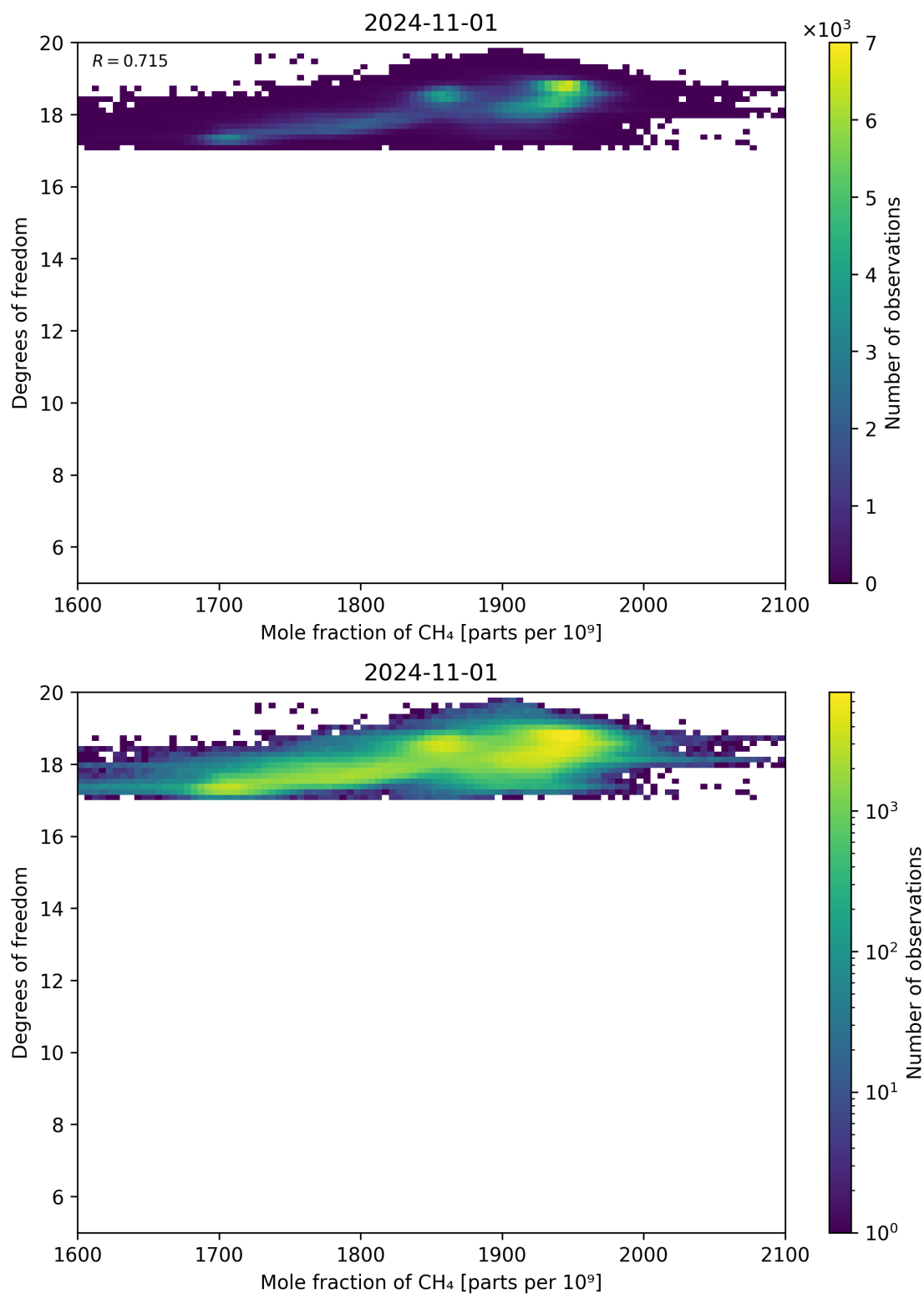
Figure 72: Scatter density plot of “Mole fraction of CH 4 ” against “Degrees of freedom” for 2024-10-31 to 2024-11-02.
