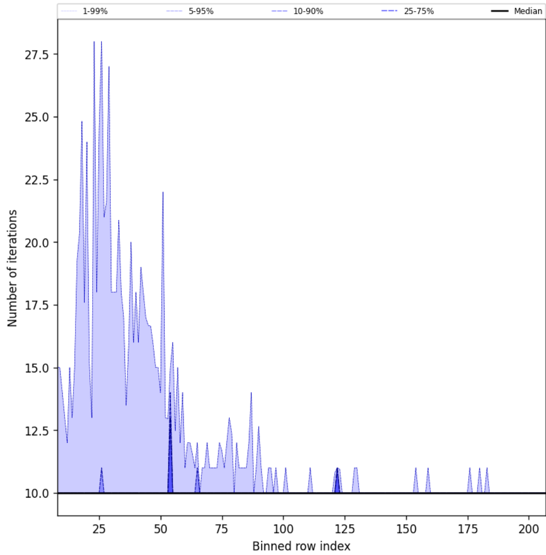
Figure 42: Along track statistics of “Number of iterations” for 2024-10-31 to 2024-11-02
