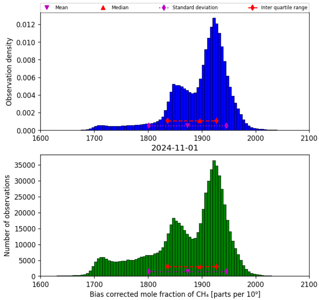
Figure 25: Histogram of “Bias corrected mole fraction of CH 4 ” for 2024-10-31 to 2024-11-02
