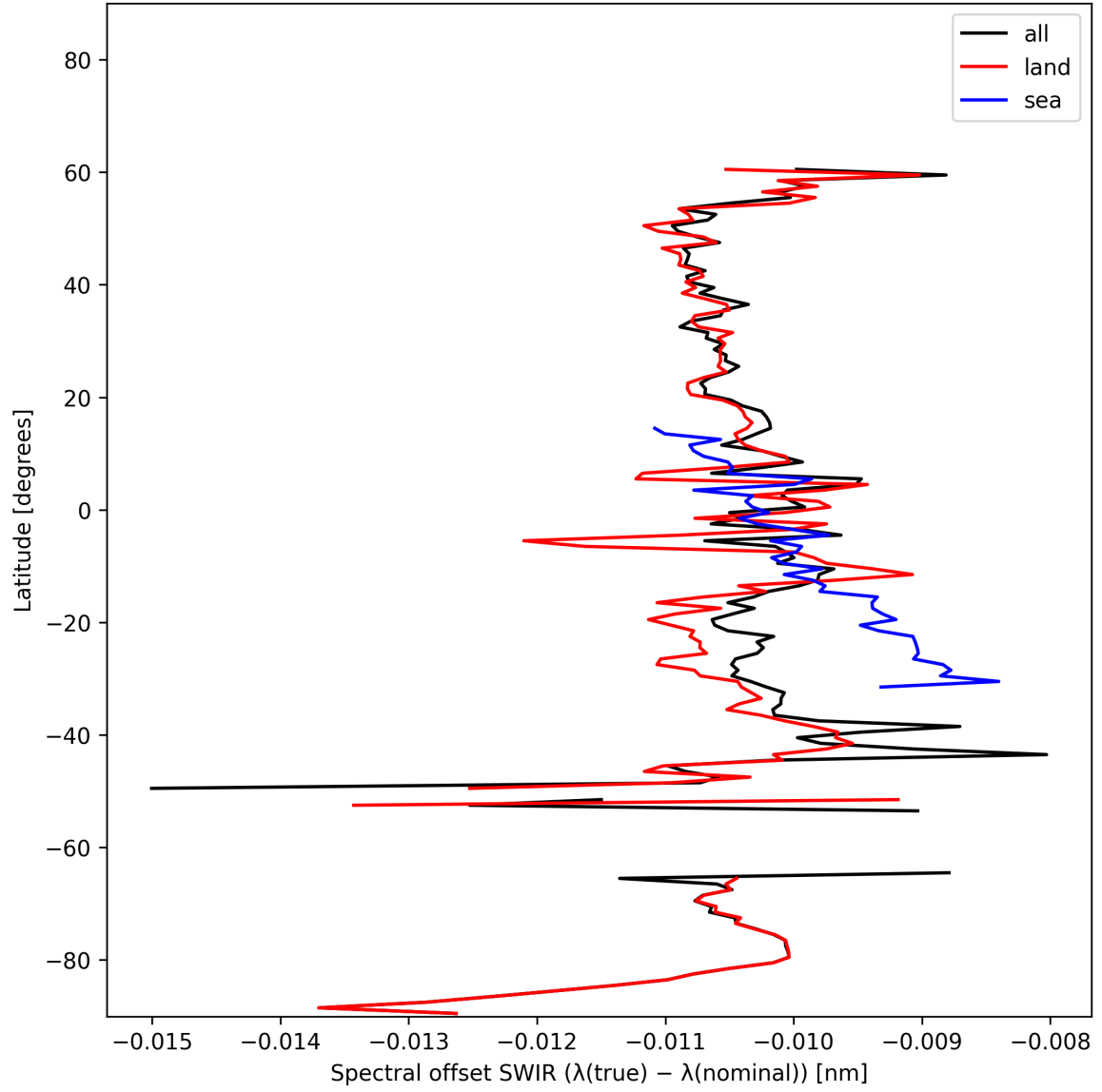
Figure 16: Zonal average of “Spectral offset SWIR ( \lambda_{\text{true}} - \lambda_{\text{nominal}} )” for 2024-10-31 to 2024-11-02.
