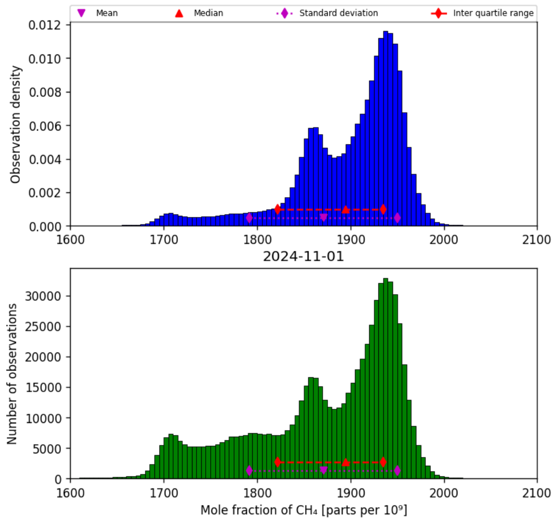
Figure 23: Histogram of “Mole fraction of CH 4 ” for 2024-10-31 to 2024-11-02
