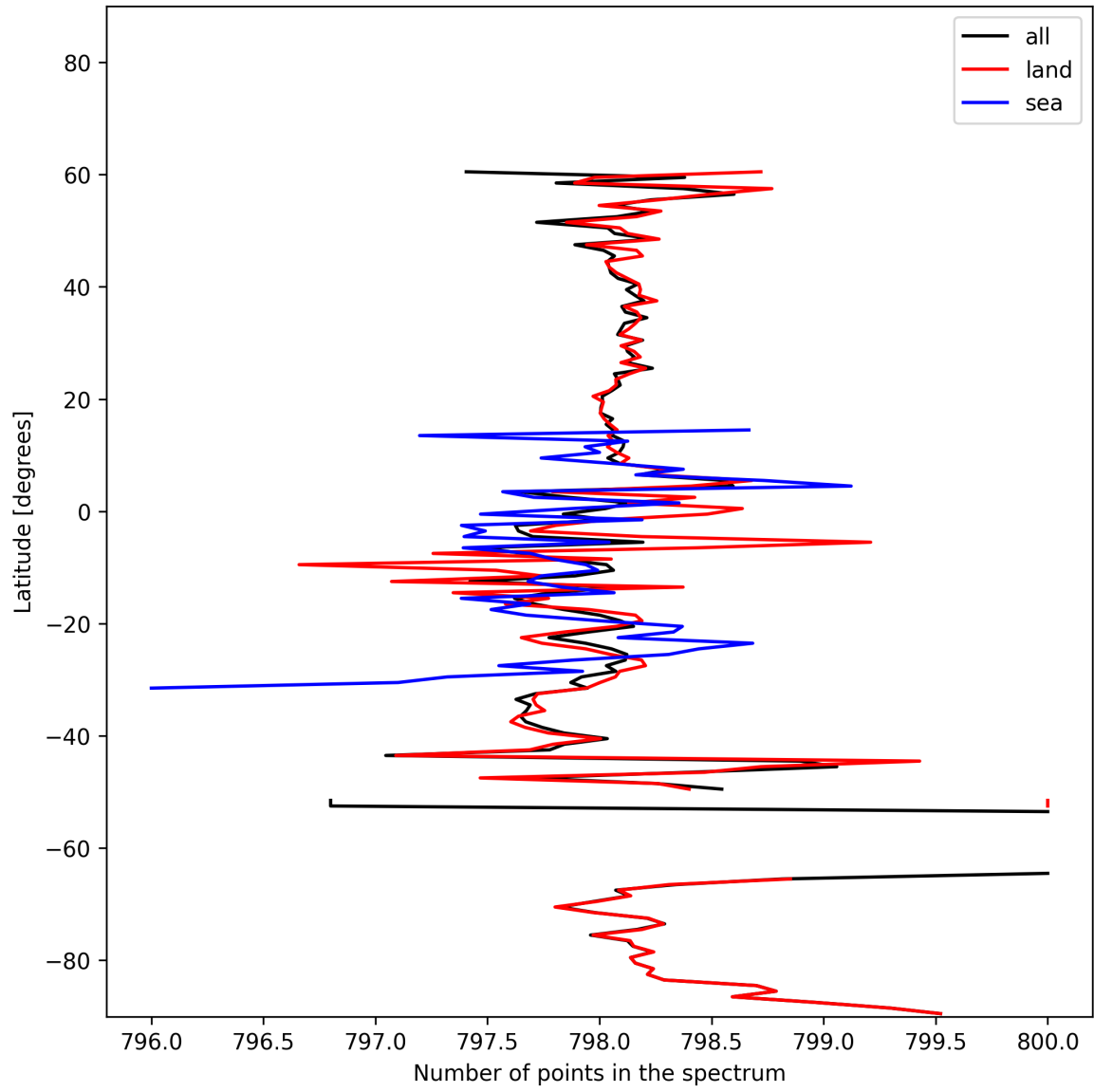
Figure 15: Zonal average of “Number of points in the spectrum” for 2024-10-31 to 2024-11-02.
