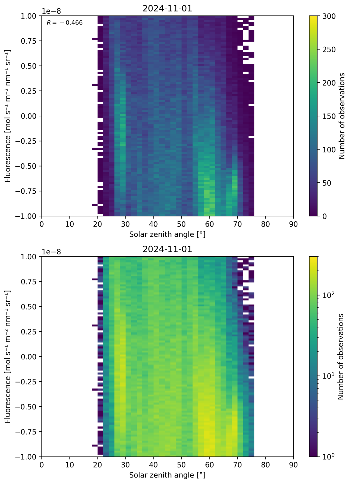
Figure 97: Scatter density plot of “Solar zenith angle” against “Fluorescence” for 2024-10-31 to 2024-11-02.
