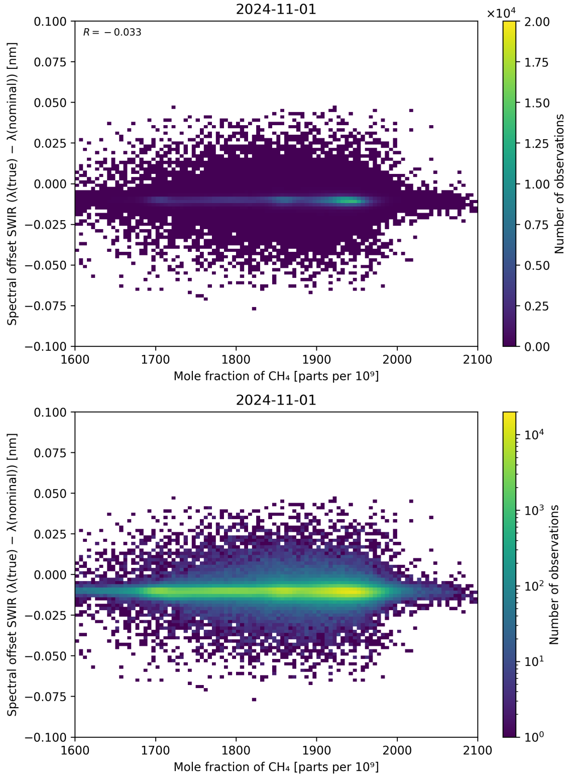
Figure 86: Scatter density plot of “Mole fraction of CH 4 ” against “Spectral offset SWIR ( \lambda_{\text{true}} - \lambda_{\text{nominal}} )” for 2024-10-31 to 2024-11-02.
