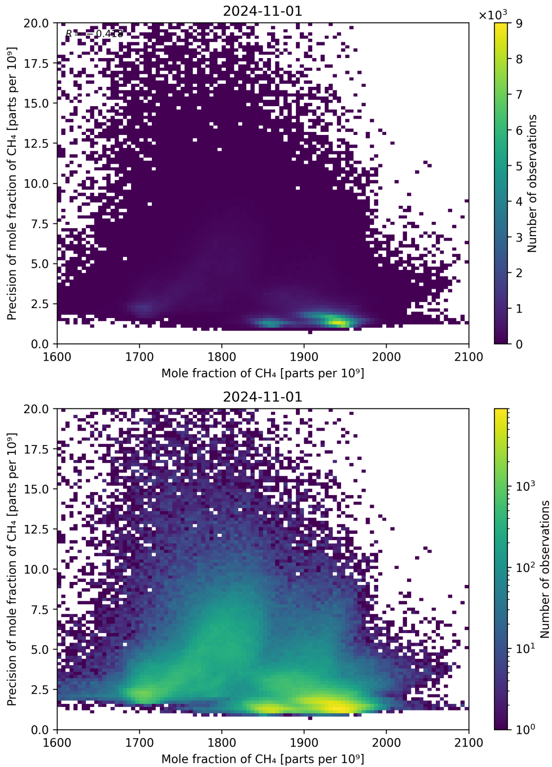
Figure 75: Scatter density plot of “Mole fraction of CH 4 ” against “Precision of mole fraction of CH 4 ” for 2024-10-31 to 2024-11-02.
