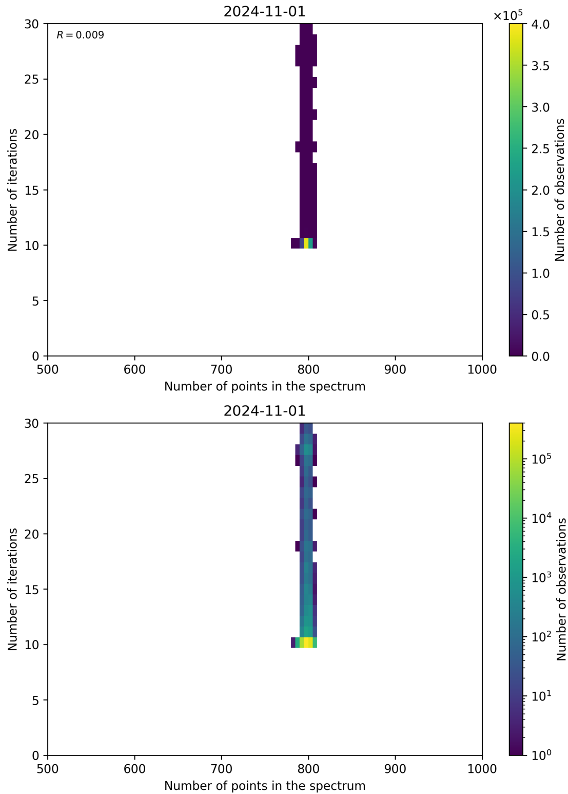
Figure 92: Scatter density plot of “Number of points in the spectrum” against “Number of iterations” for 2024-10-31 to 2024-11-02.
