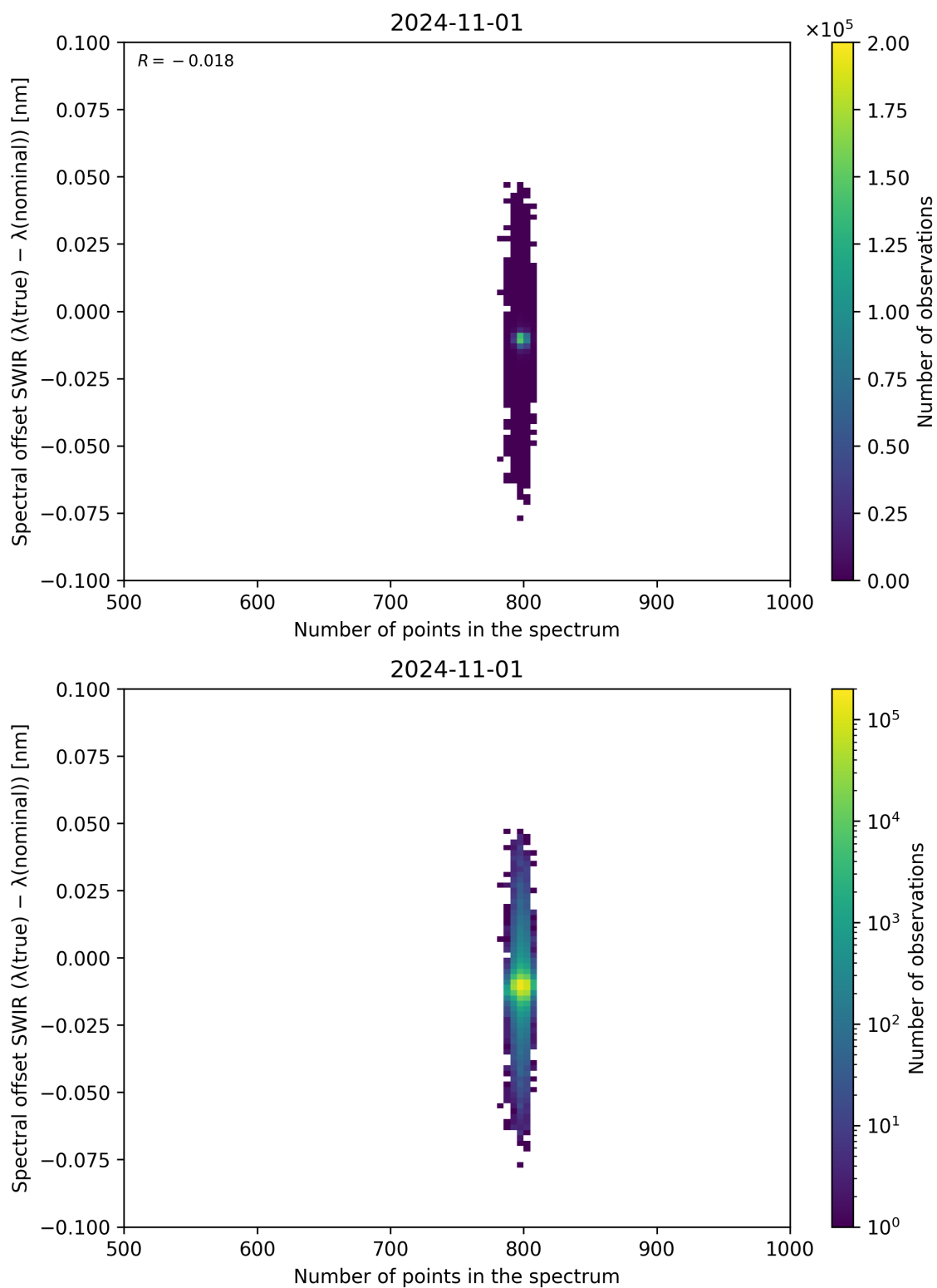
Figure 93: Scatter density plot of “Number of points in the spectrum” against “Spectral offset SWIR ( \lambda_{\text{true}} - \lambda_{\text{nominal}} )” for 2024-10-31 to 2024-11-02.
