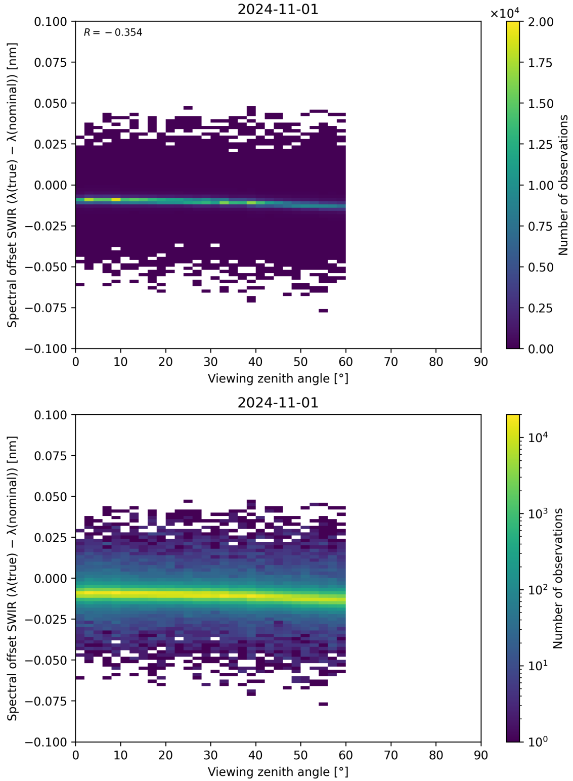
Figure 116: Scatter density plot of “Viewing zenith angle” against “Spectral offset SWIR ( \lambda_{\text{true}} - \lambda_{\text{nominal}} )” for 2024-10-31 to 2024-11-02.
