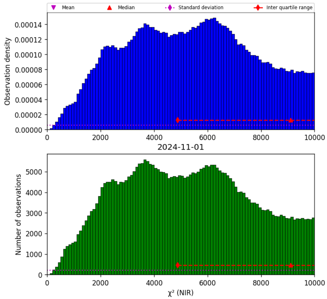
Figure 29: Histogram of “ \chi^2 (NIR)” for 2024-10-31 to 2024-11-02
