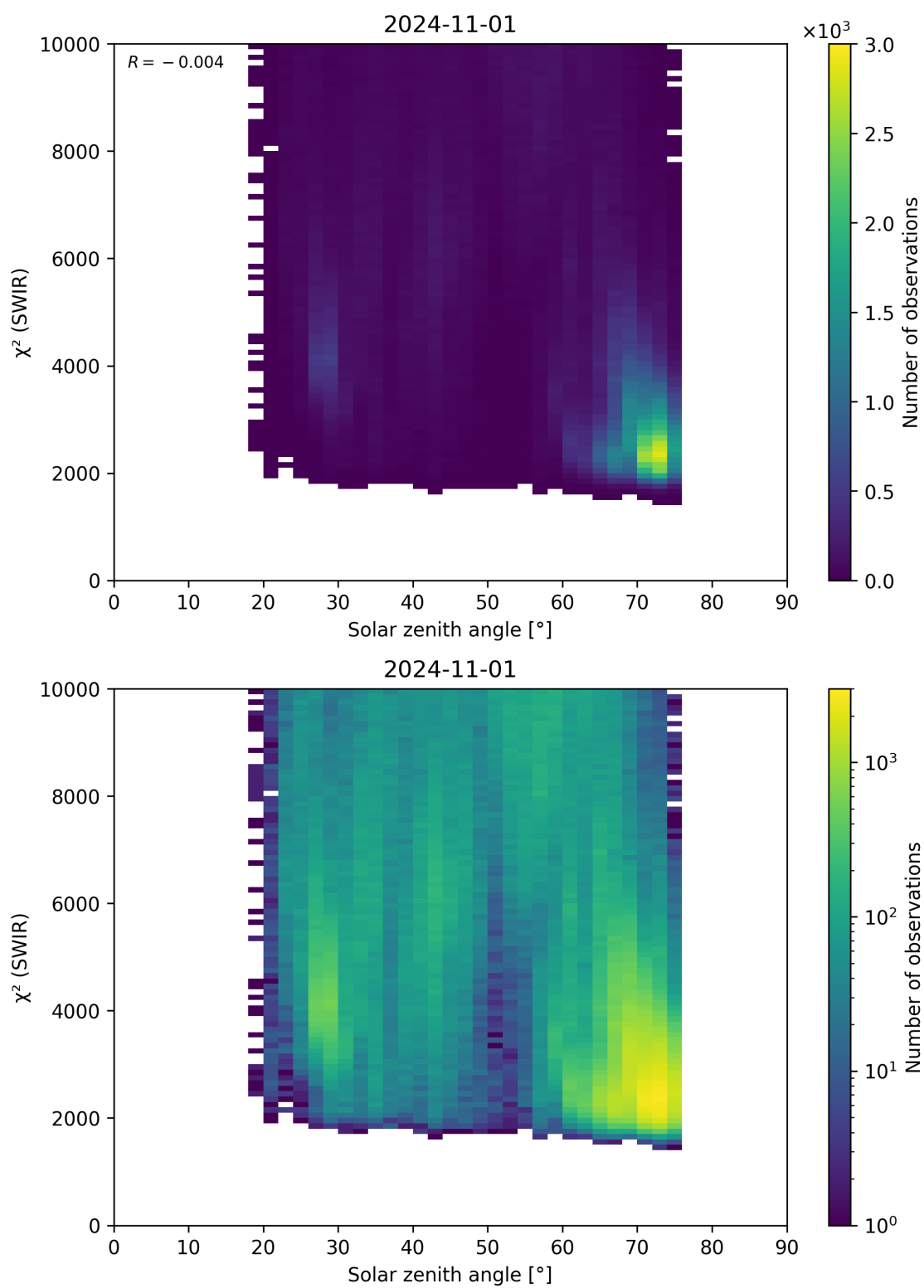
Figure 95: Scatter density plot of “Solar zenith angle” against “ \chi^2 (SWIR)” for 2024-10-31 to 2024-11-02.
