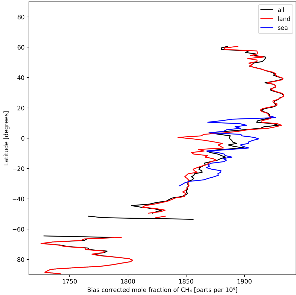
Figure 14: Zonal average of “Bias corrected mole fraction of CH 4 ” for 2024-10-31 to 2024-11-02.
