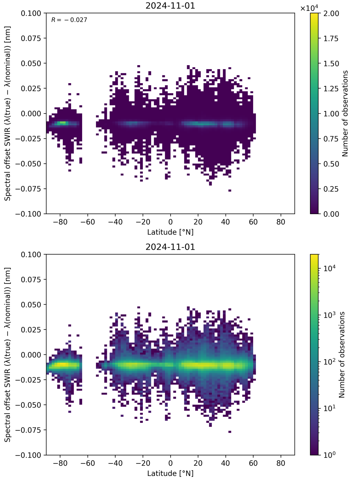
Figure 62: Scatter density plot of “Latitude” against “Spectral offset SWIR ( \lambda_{\text{true}} - \lambda_{\text{nominal}} )” for 2024-10-31 to 2024-11-02.
