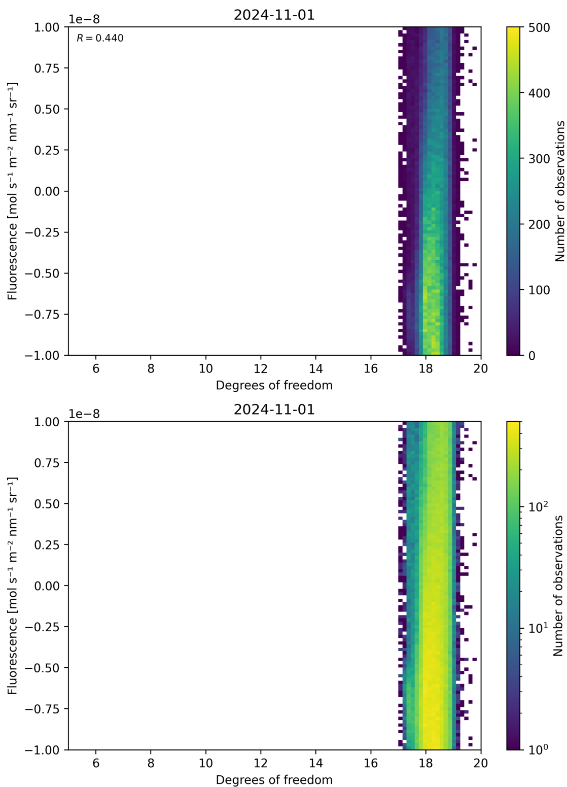
Figure 51: Scatter density plot of “Degrees of freedom” against “Fluorescence” for 2024-10-31 to 2024-11-02.
