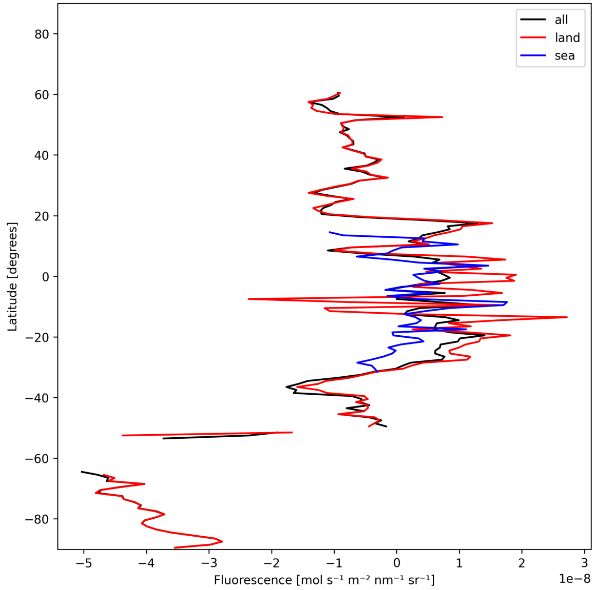
Figure 21: Zonal average of “Fluorescence” for 2024-10-31 to 2024-11-02.
