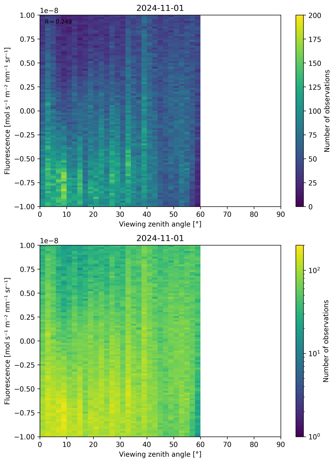
Figure 108: Scatter density plot of “Viewing zenith angle” against “Fluorescence” for 2024-10-31 to 2024-11-02.
