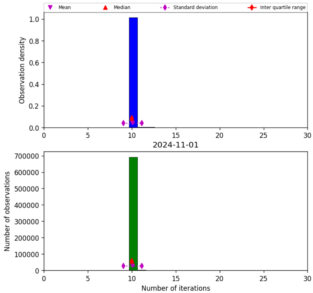
Figure 31: Histogram of “Number of iterations” for 2024-10-31 to 2024-11-02
