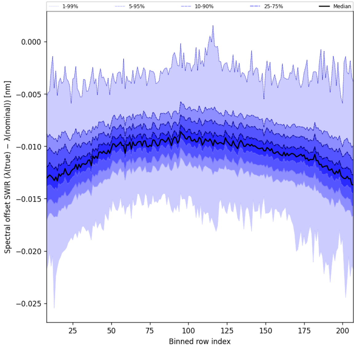
Figure 38: Along track statistics of “Spectral offset SWIR ( \lambda_{\text{true}} - \lambda_{\text{nominal}} )” for 2024-10-31 to 2024-11-02
