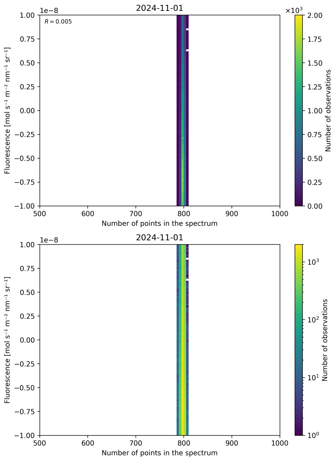
Figure 91: Scatter density plot of “Number of points in the spectrum” against “Fluorescence” for 2024-10-31 to 2024-11-02.
