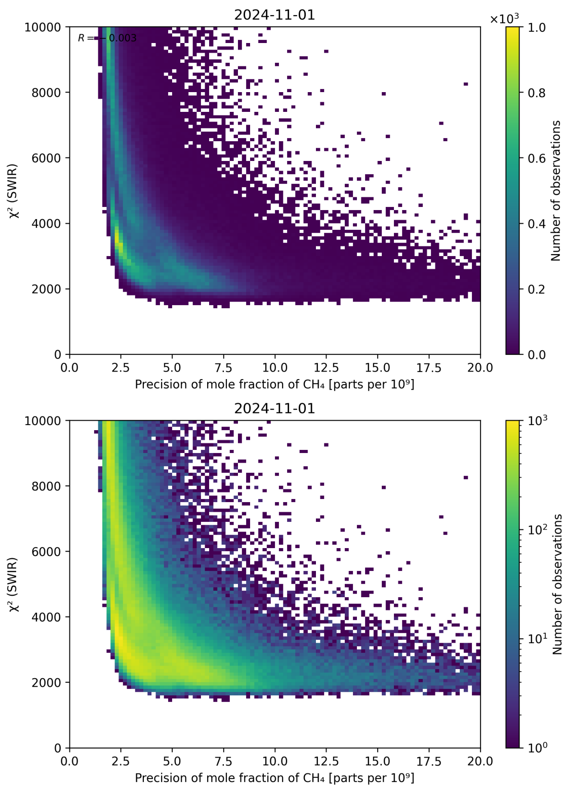
Figure 79: Scatter density plot of “Precision of mole fraction of \text{CH}_4 ” against “ \chi^2 (SWIR)” for 2024-10-31 to 2024-11-02.
