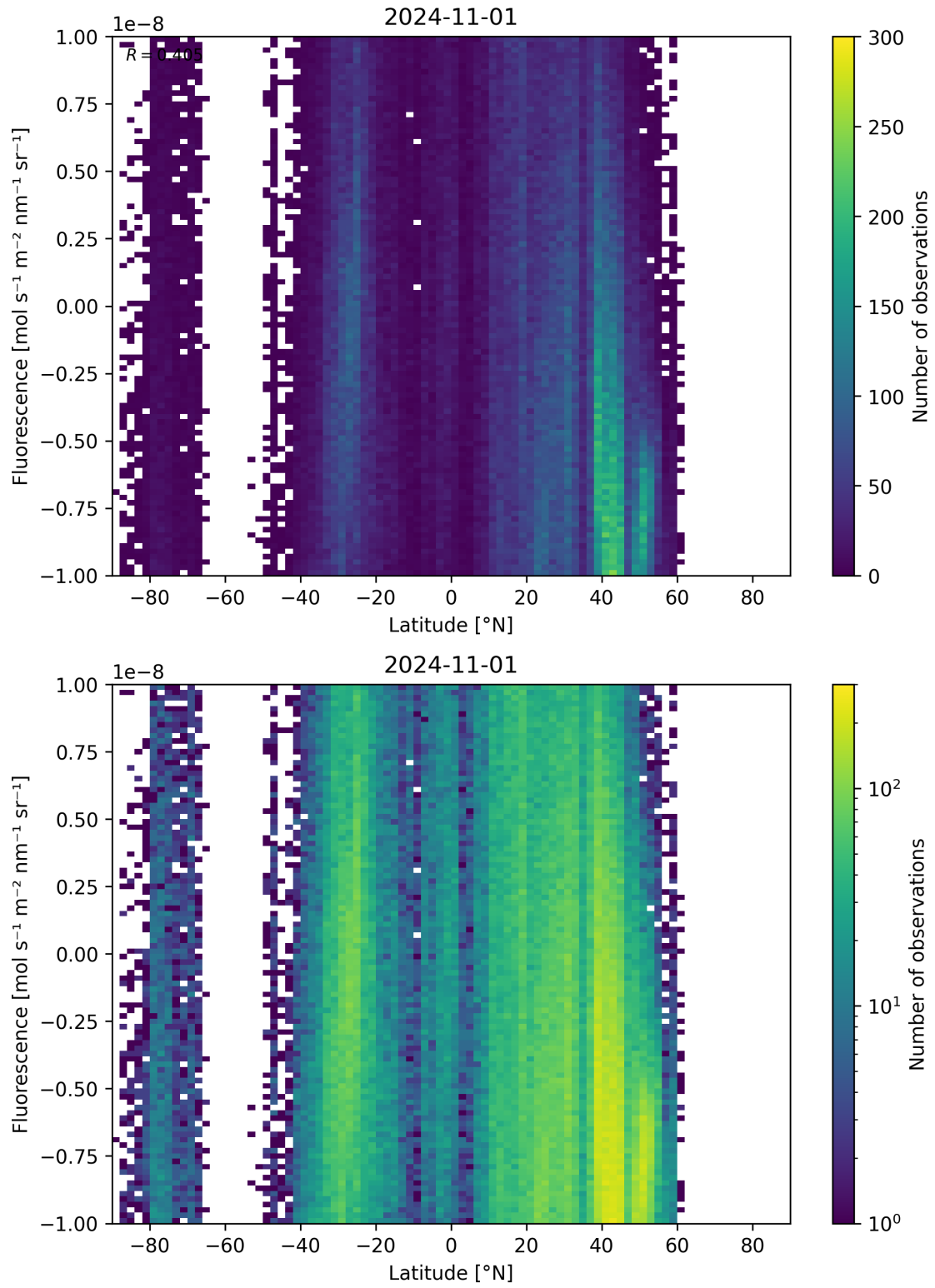
Figure 56: Scatter density plot of “Latitude” against “Fluorescence” for 2024-10-31 to 2024-11-02.
