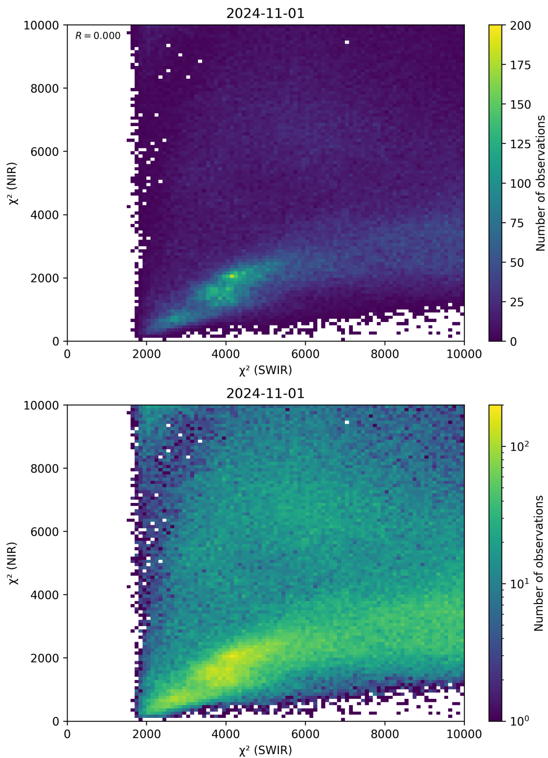
Figure 47: Scatter density plot of “ \chi^2 (SWIR)” against “ \chi^2 (NIR)” for 2024-10-31 to 2024-11-02.
