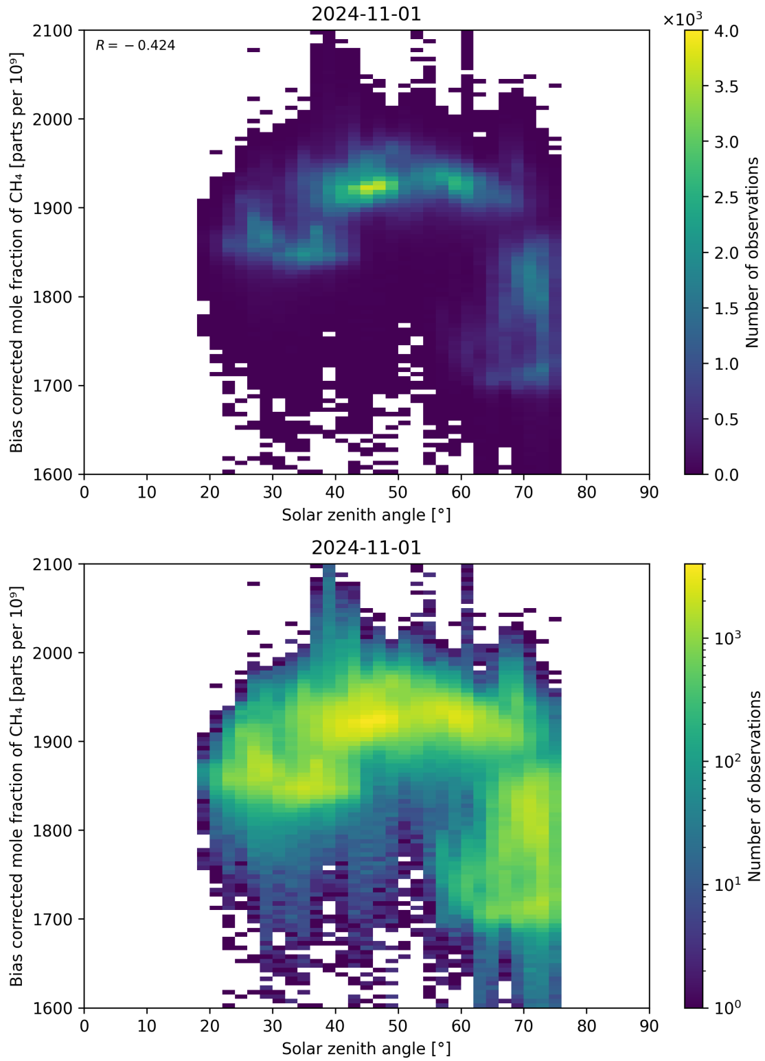
Figure 100: Scatter density plot of “Solar zenith angle” against “Bias corrected mole fraction of CH 4 ” for 2024-10-31 to 2024-11-02.
