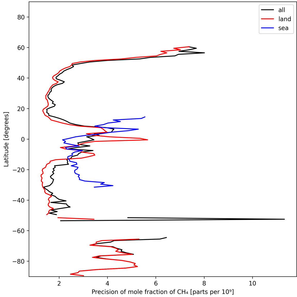
Figure 13: Zonal average of “Precision of mole fraction of CH 4 ” for 2024-10-31 to 2024-11-02.
