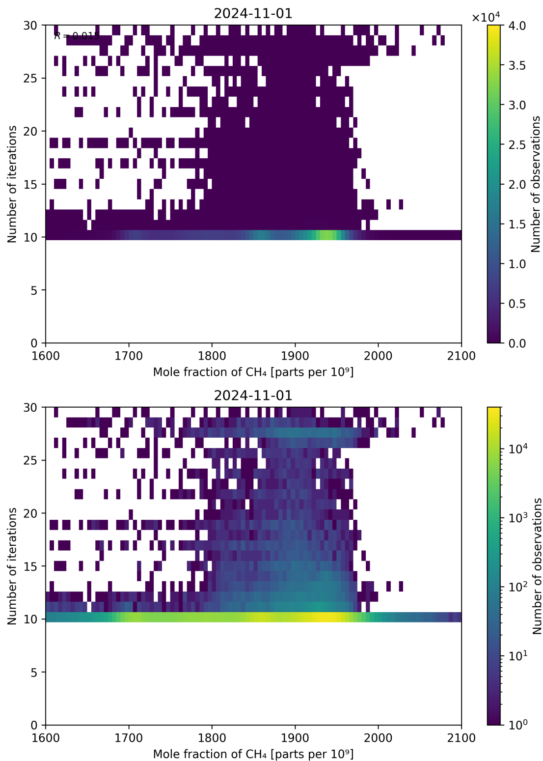
Figure 76: Scatter density plot of “Mole fraction of CH 4 ” against “Number of iterations” for 2024-10-31 to 2024-11-02.
