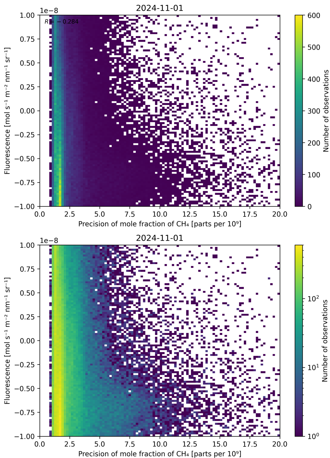
Figure 81: Scatter density plot of “Precision of mole fraction of CH 4 ” against “Fluorescence” for 2024-10-31 to 2024-11-02.
