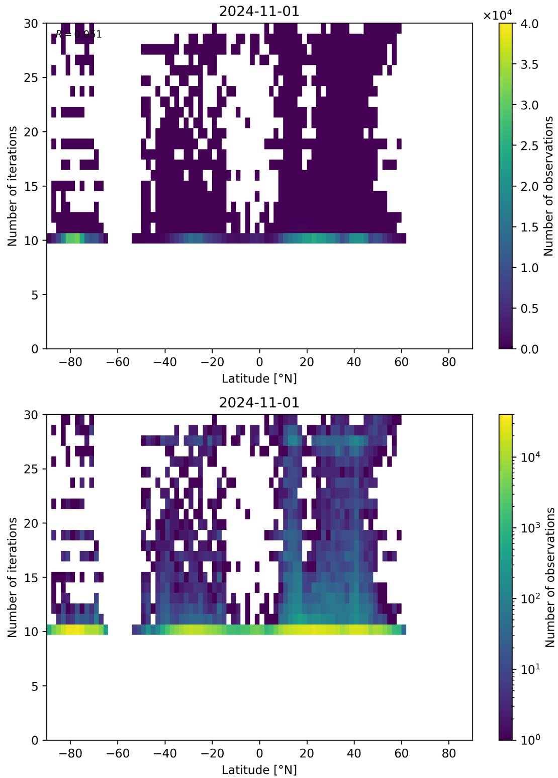
Figure 60: Scatter density plot of “Latitude” against “Number of iterations” for 2024-10-31 to 2024-11-02.
