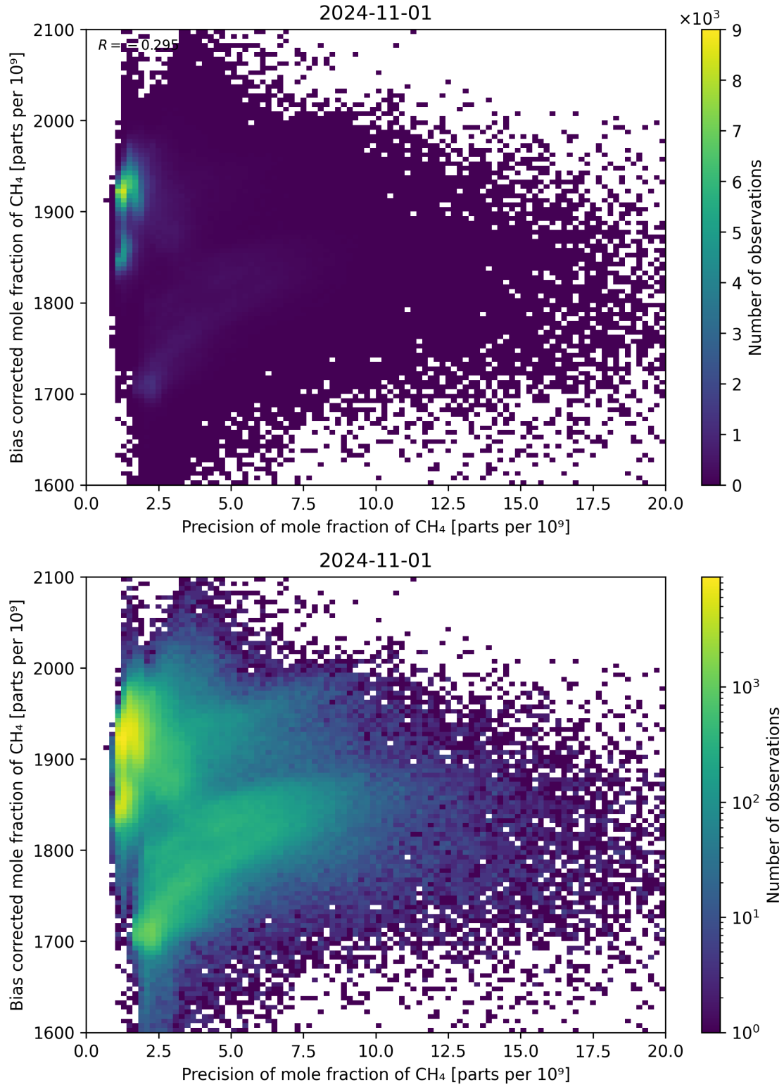
Figure 82: Scatter density plot of “Precision of mole fraction of CH 4 ” against “Bias corrected mole fraction of CH 4 ” for 2024-10-31 to 2024-11-02.
