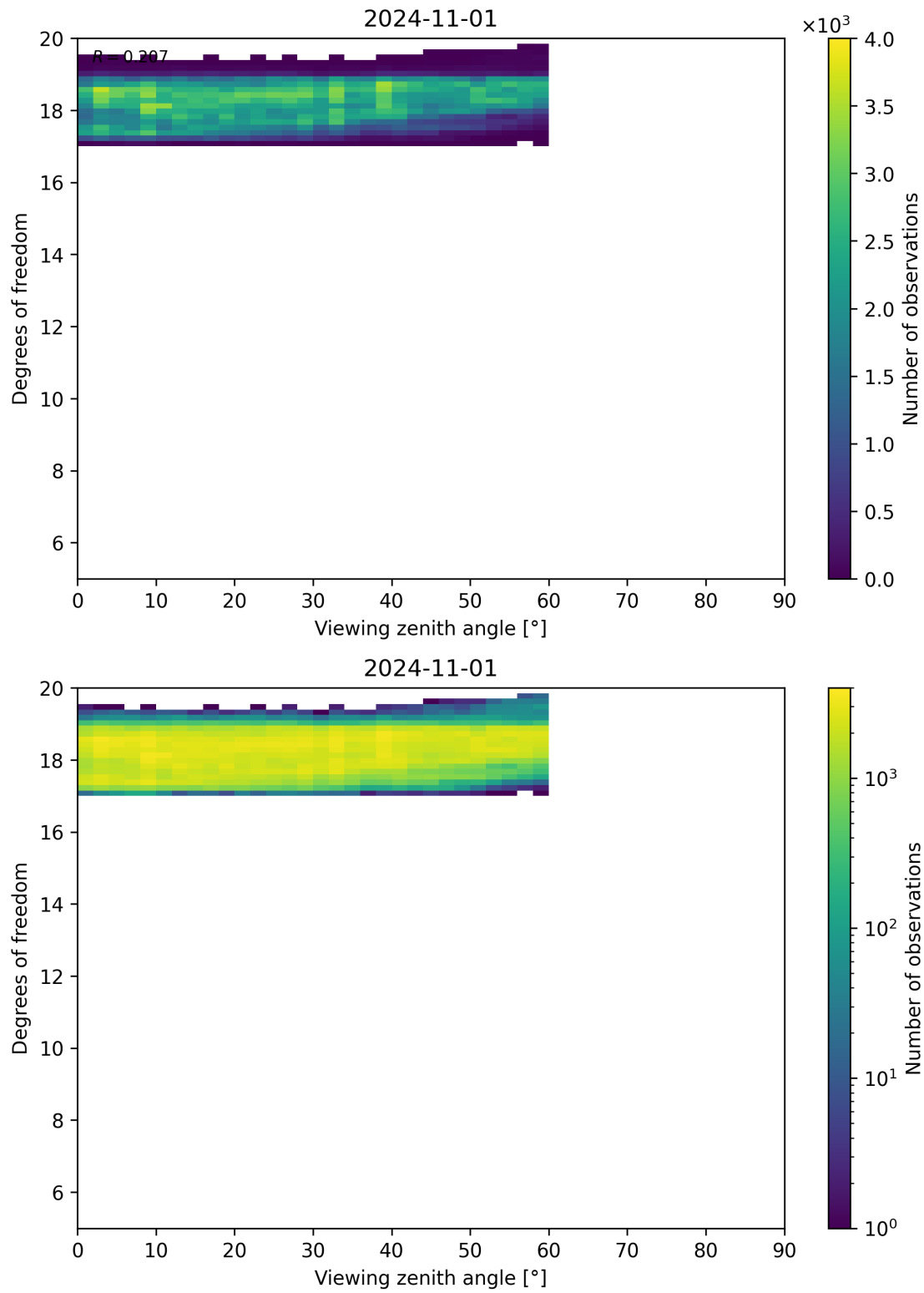
Figure 107: Scatter density plot of “Viewing zenith angle” against “Degrees of freedom” for 2024-10-31 to 2024-11-02.
