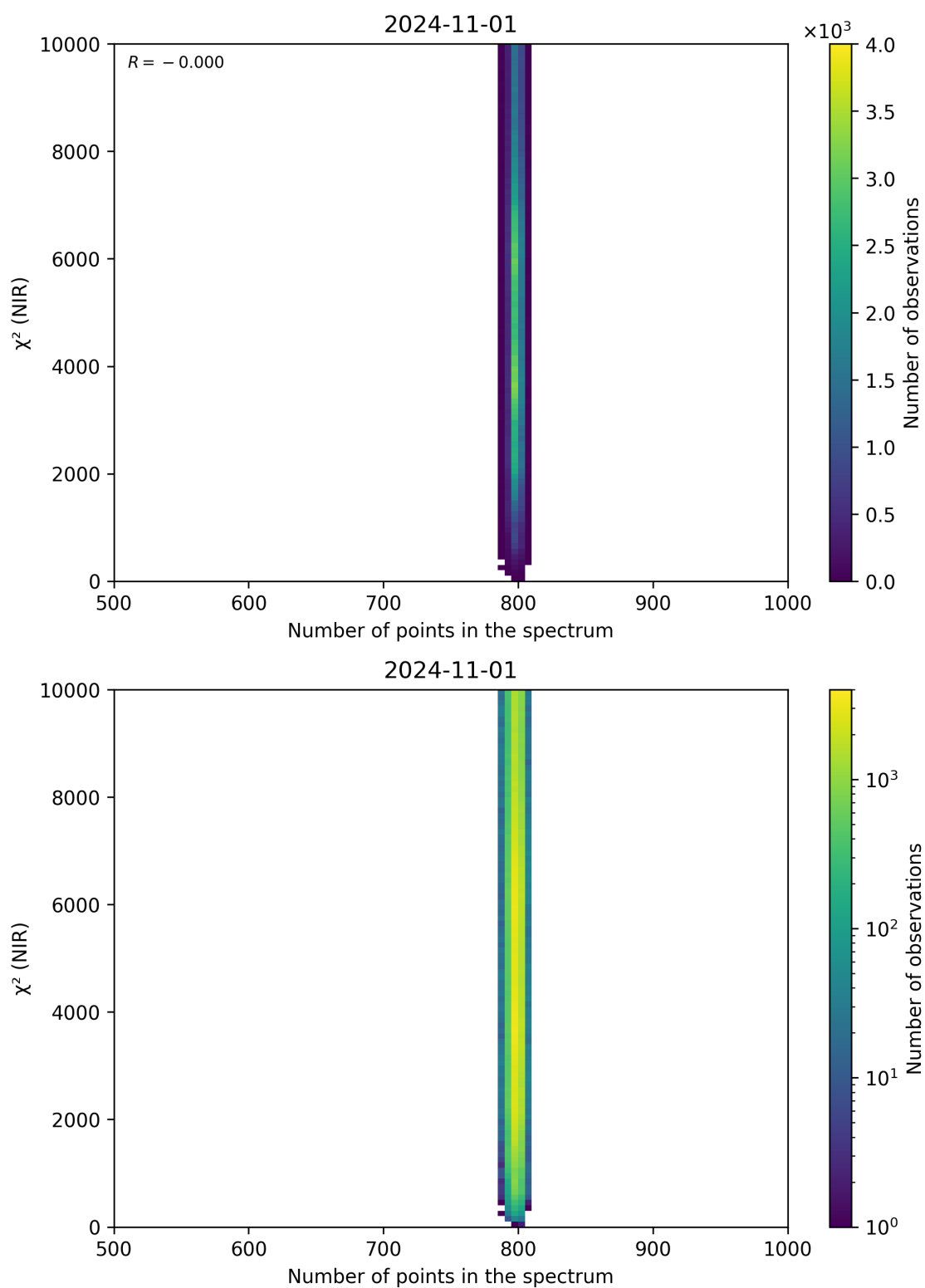
Figure 88: Scatter density plot of “Number of points in the spectrum” against “ \chi^2 (NIR)” for 2024-10-31 to 2024-11-02.
