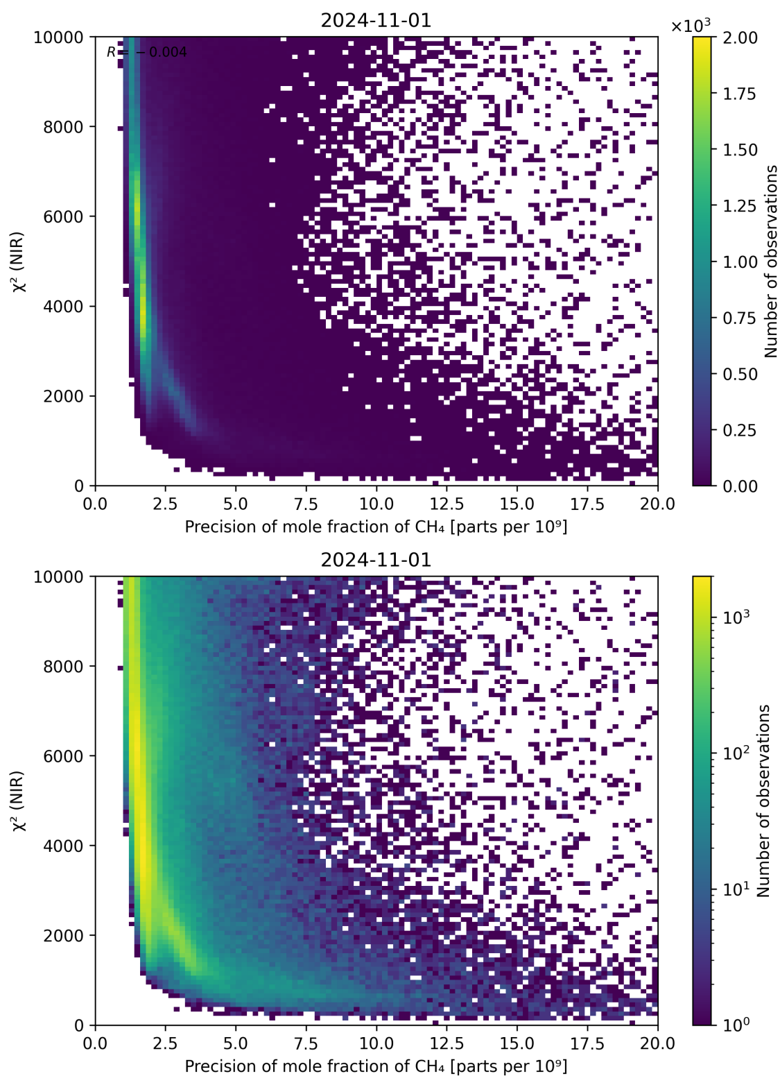
Figure 78: Scatter density plot of “Precision of mole fraction of CH 4 ” against “ \chi^2 (NIR)” for 2024-10-31 to 2024-11-02.
