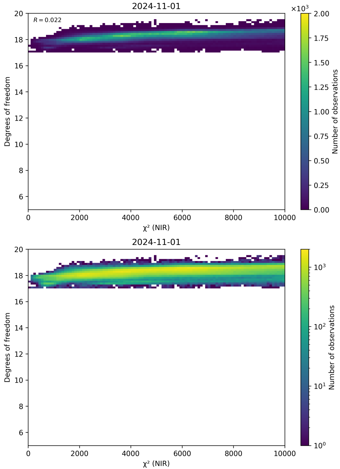
Figure 44: Scatter density plot of “ \chi^2 (NIR)” against “Degrees of freedom” for 2024-10-31 to 2024-11-02.
