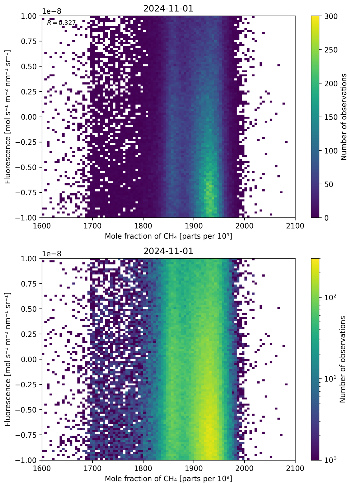
Figure 73: Scatter density plot of “Mole fraction of \text{CH}_4 ” against “Fluorescence” for 2024-10-31 to 2024-11-02.
