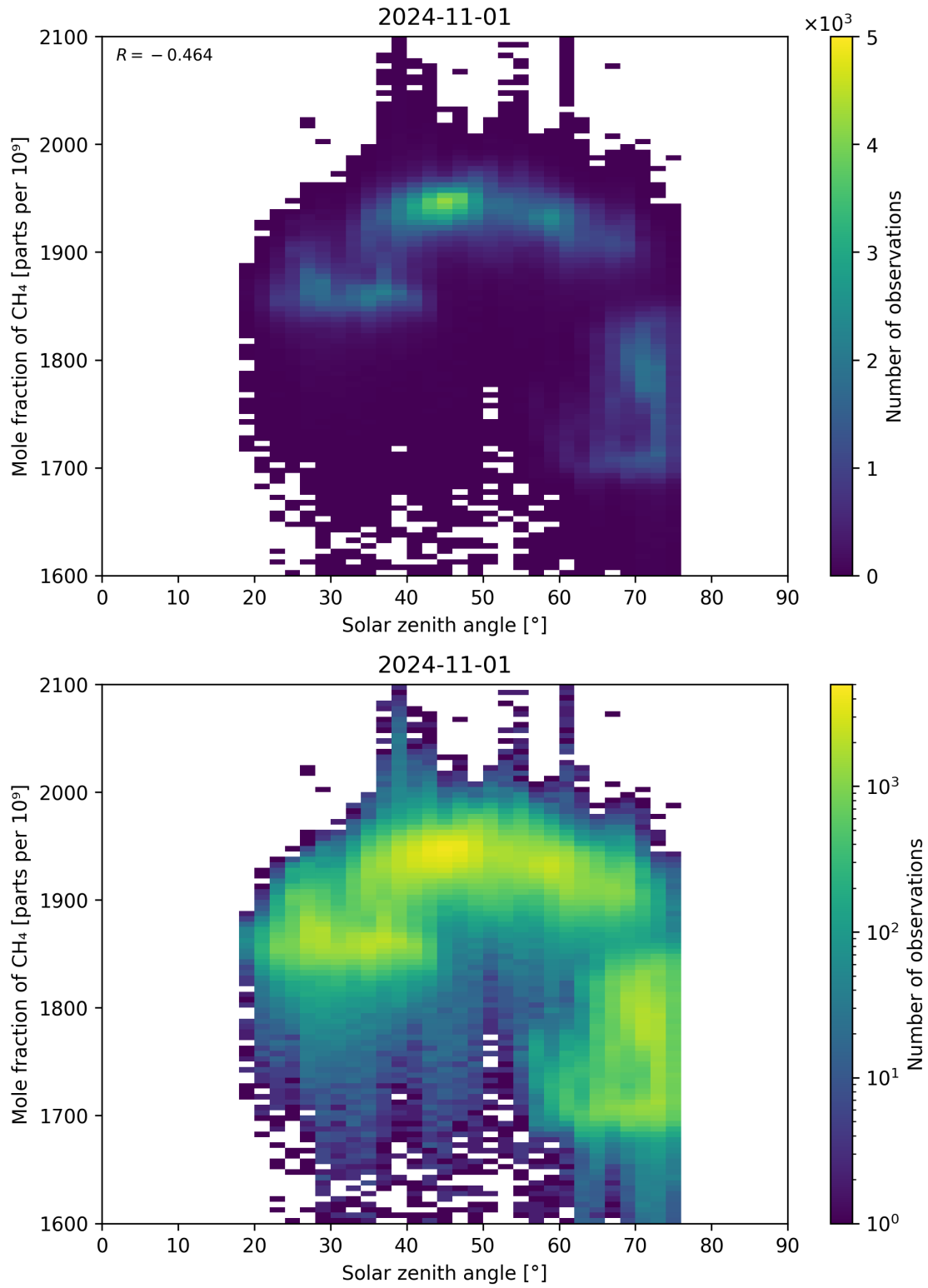
Figure 99: Scatter density plot of “Solar zenith angle” against “Mole fraction of CH 4 ” for 2024-10-31 to 2024-11-02.
