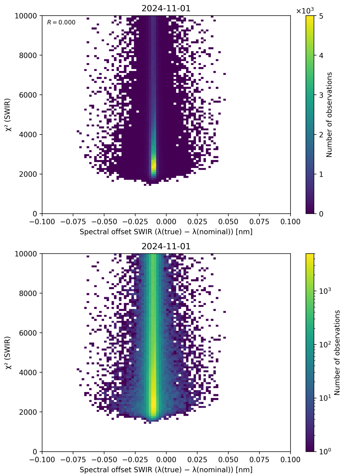
Figure 118: Scatter density plot of “Spectral offset SWIR ( \lambda_{\text{true}} - \lambda_{\text{nominal}} )” against “ \chi^2 (SWIR)” for 2024-10-31 to 2024-11-02.
