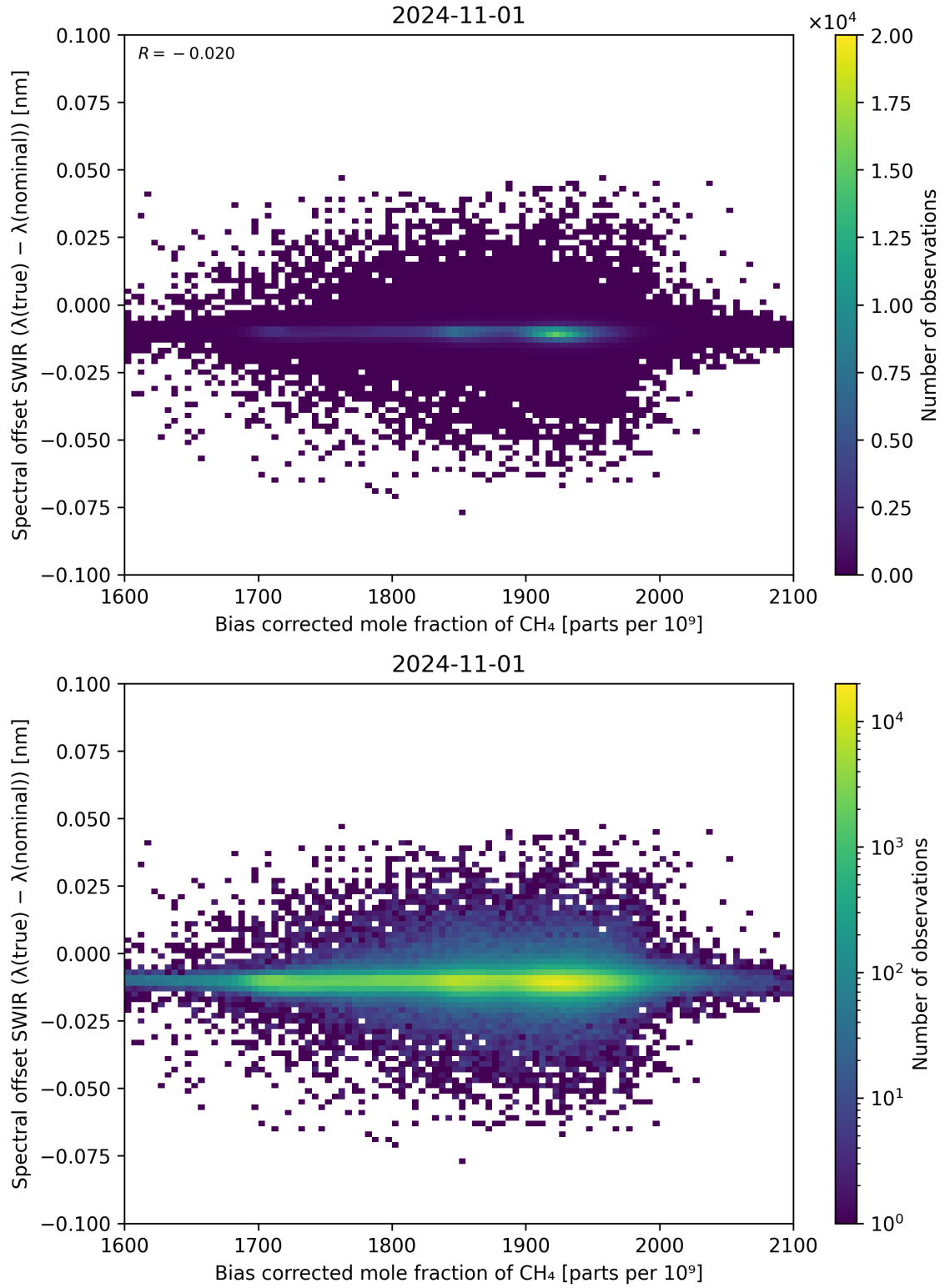
Figure 69: Scatter density plot of “Bias corrected mole fraction of \text{CH}_4 ” against “Spectral offset SWIR ( \lambda_{\text{true}} - \lambda_{\text{nominal}} )” for 2024-10-31 to 2024-11-02.
