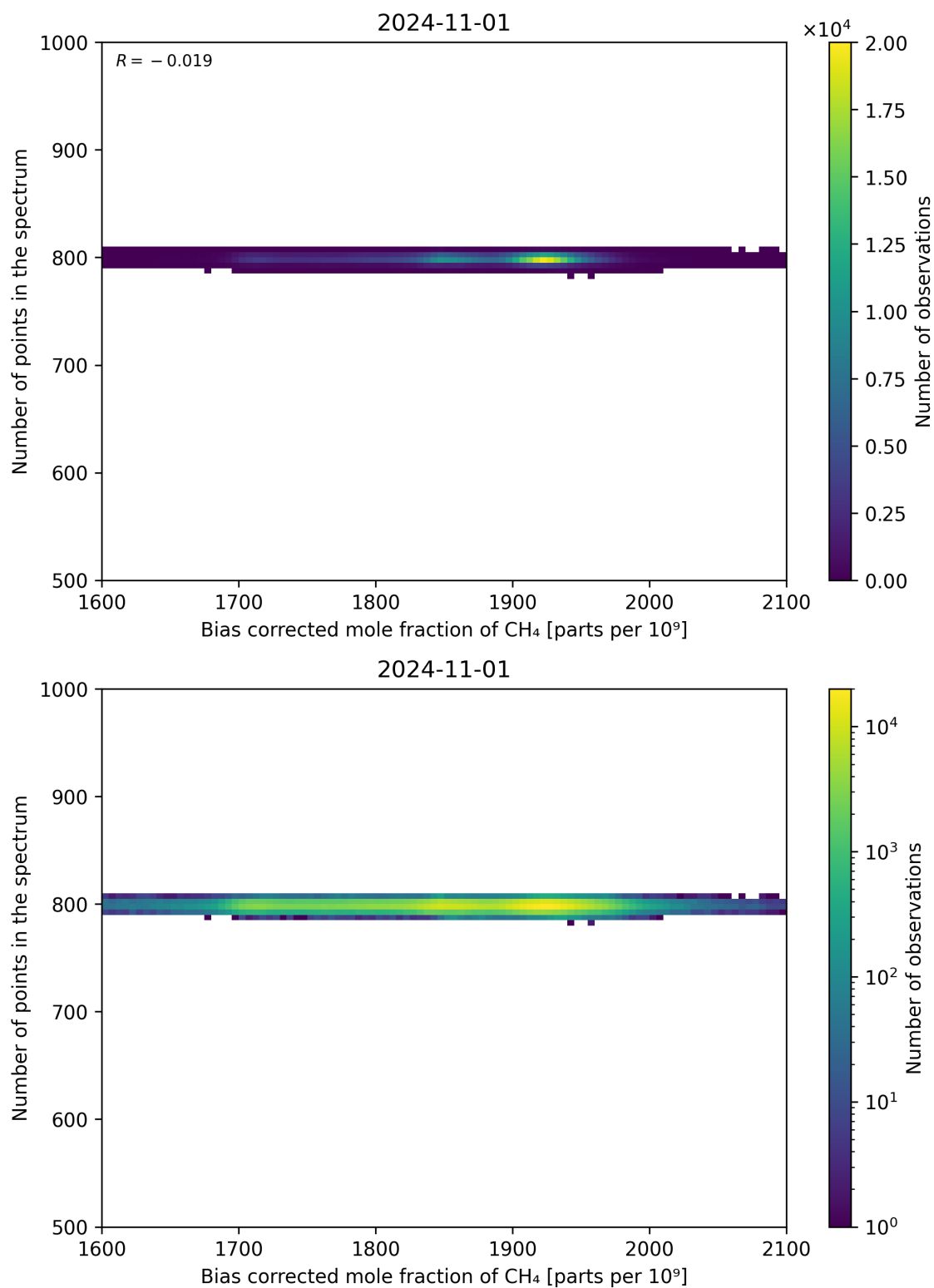
Figure 68: Scatter density plot of “Bias corrected mole fraction of CH 4 ” against “Number of points in the spectrum” for 2024-10-31 to 2024-11-02.
