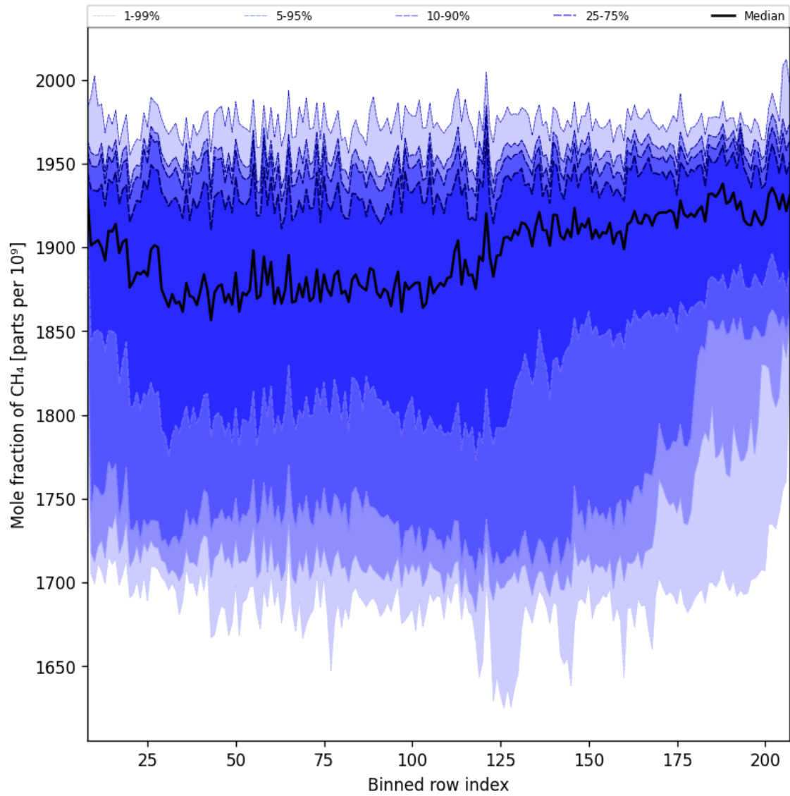
Figure 34: Along track statistics of “Mole fraction of CH 4 ” for 2024-10-31 to 2024-11-02
