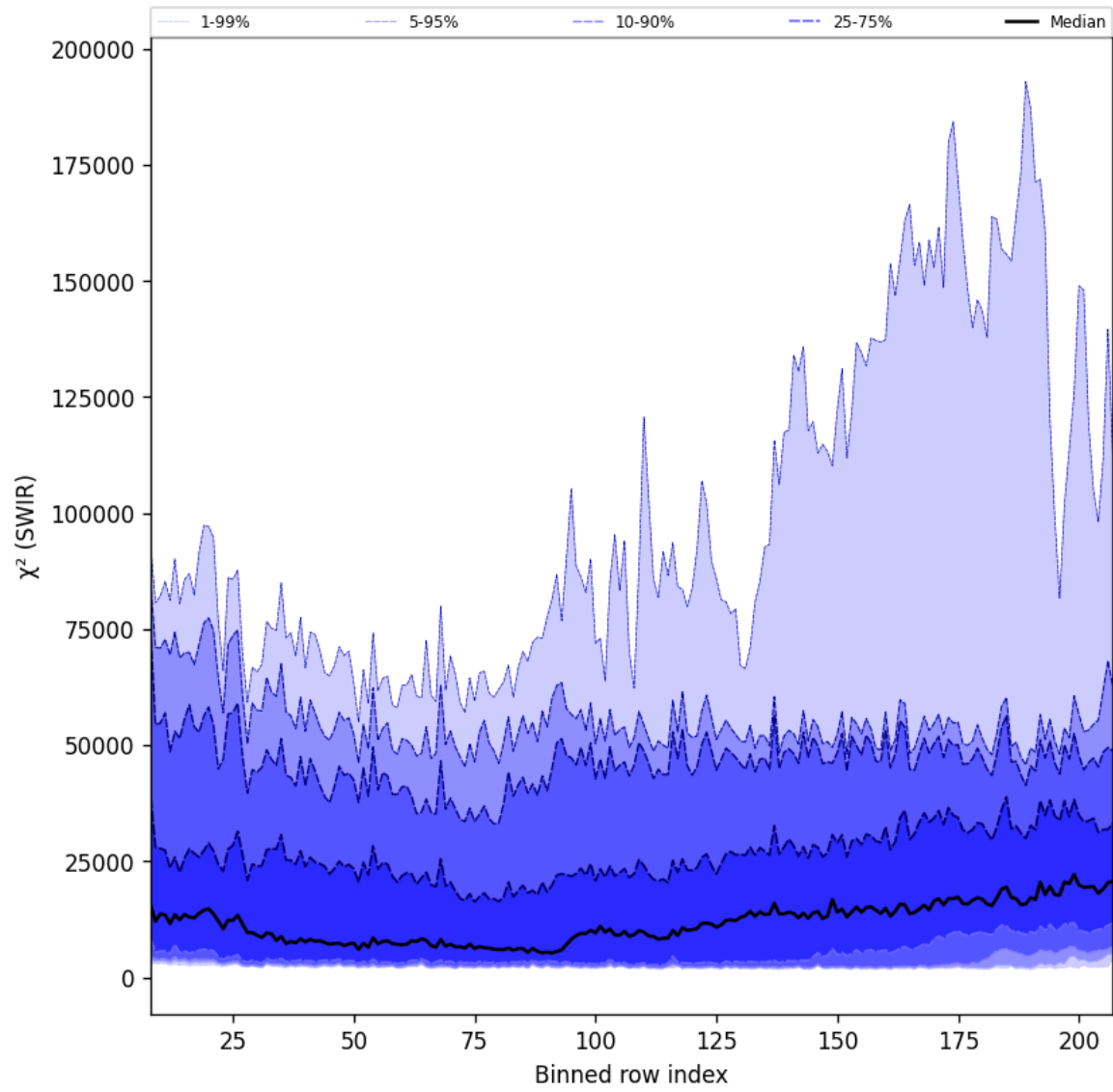
Figure 39: Along track statistics of “ \chi^2 (SWIR)” for 2024-10-31 to 2024-11-02
