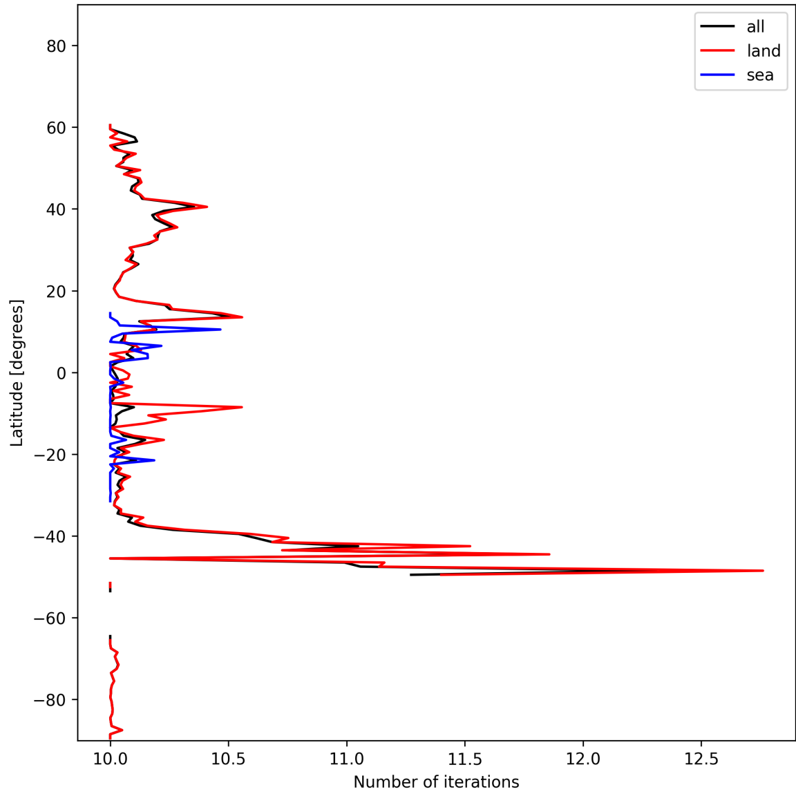
Figure 20: Zonal average of “Number of iterations” for 2024-10-31 to 2024-11-02.
