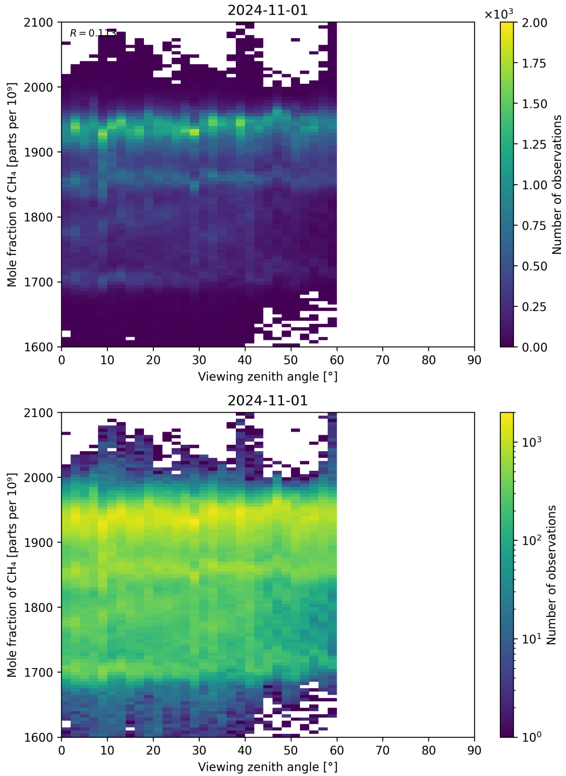
Figure 110: Scatter density plot of “Viewing zenith angle” against “Mole fraction of CH 4 ” for 2024-10-31 to 2024-11-02.
