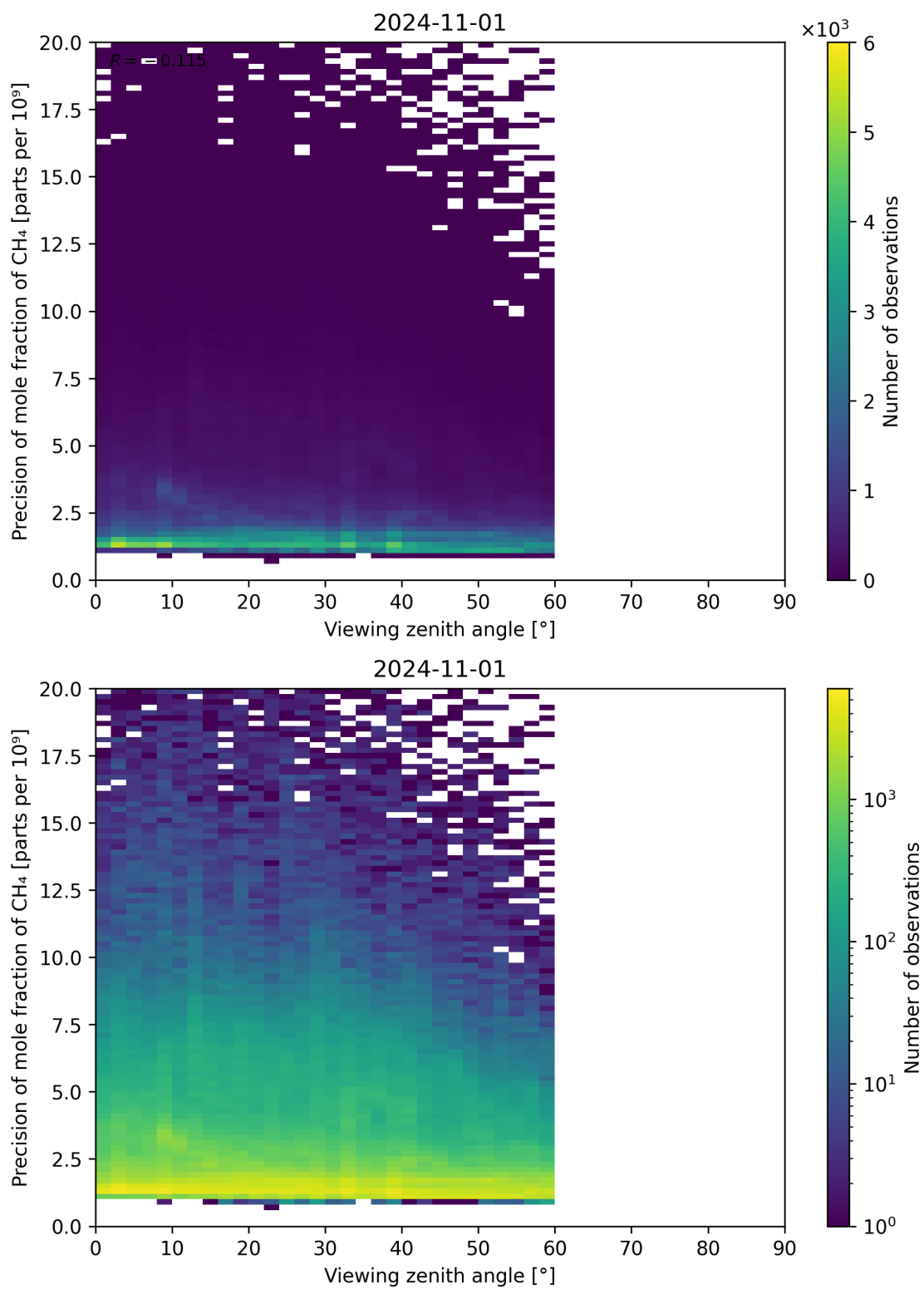
Figure 112: Scatter density plot of “Viewing zenith angle” against “Precision of mole fraction of CH 4 ” for 2024-10-31 to 2024-11-02.
