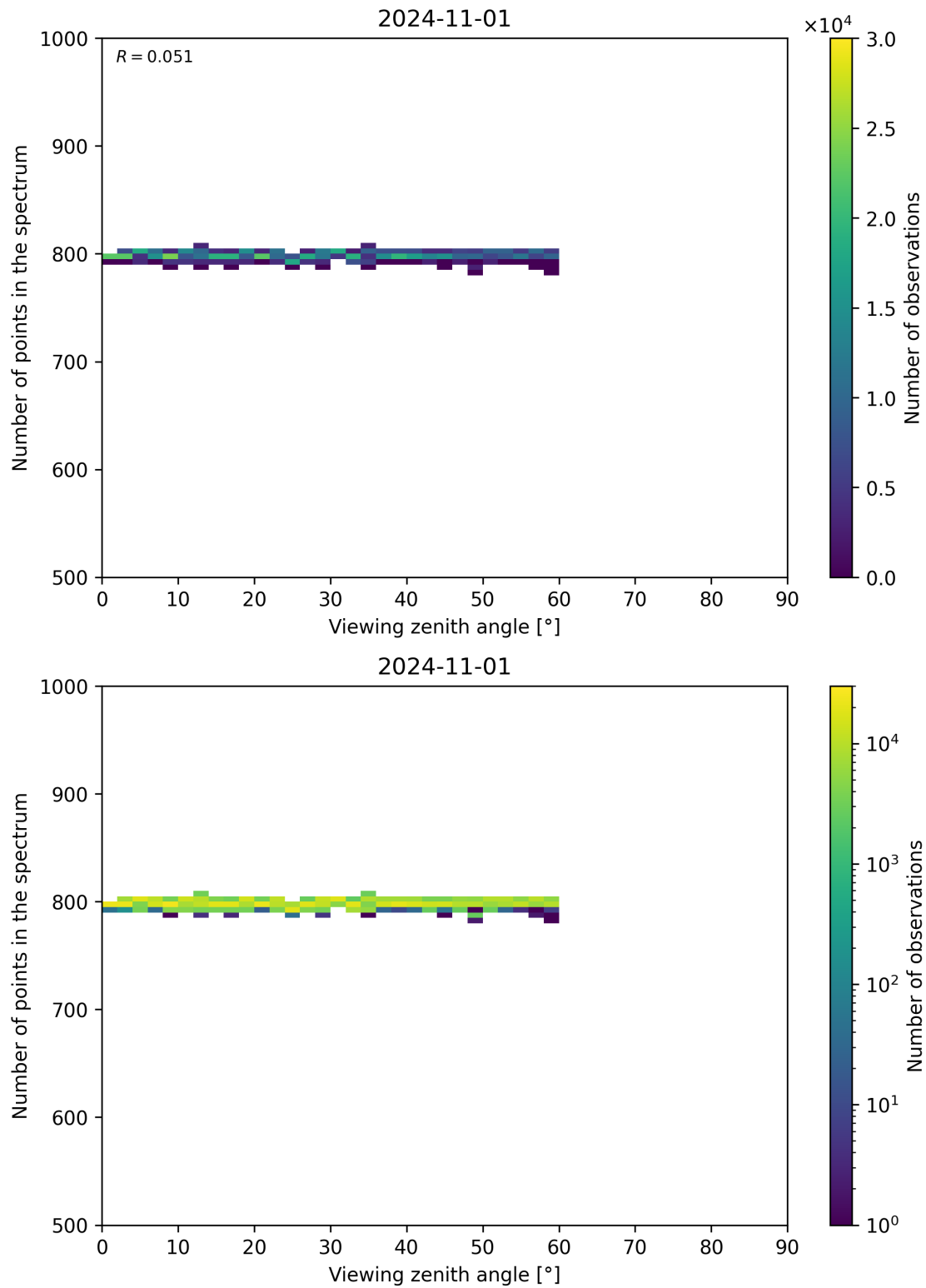
Figure 114: Scatter density plot of “Viewing zenith angle” against “Number of points in the spectrum” for 2024-10-31 to 2024-11-02.
