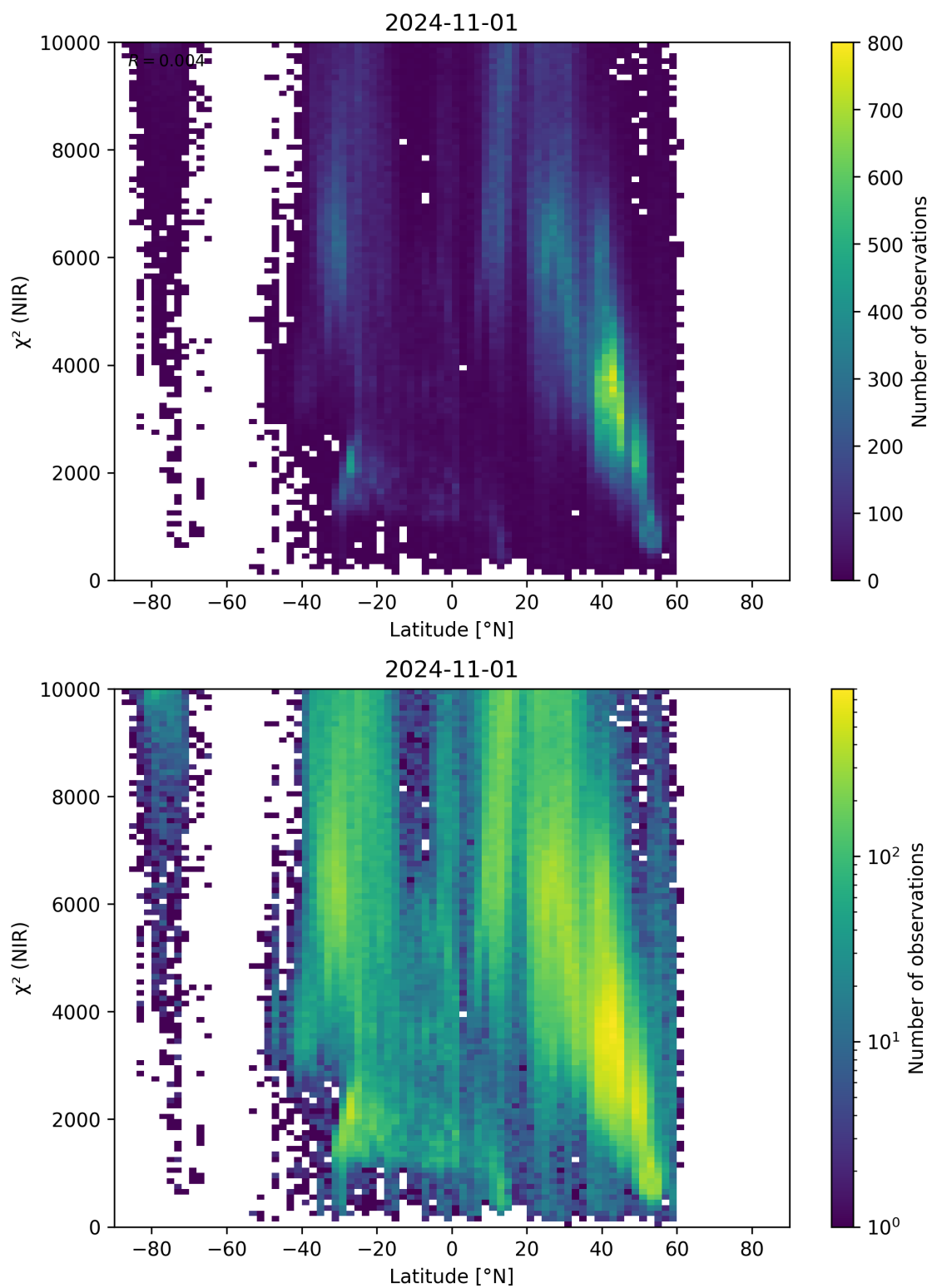
Figure 53: Scatter density plot of “Latitude” against “ \chi^2 (NIR)” for 2024-10-31 to 2024-11-02.
