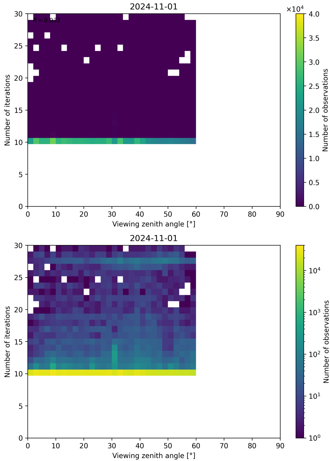
Figure 113: Scatter density plot of “Viewing zenith angle” against “Number of iterations” for 2024-10-31 to 2024-11-02.
