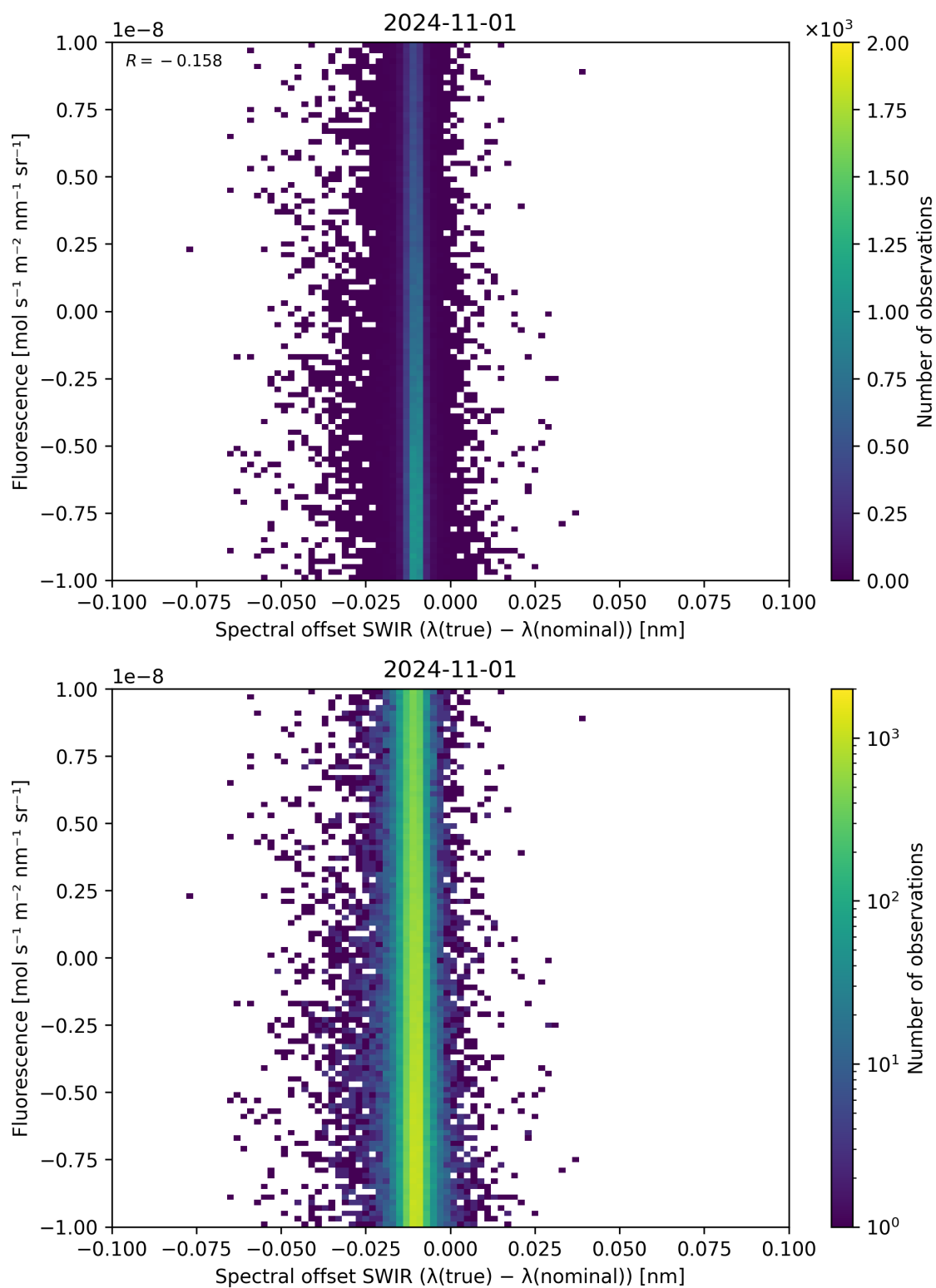
Figure 120: Scatter density plot of “Spectral offset SWIR ( \lambda_{\text{true}} - \lambda_{\text{nominal}} )” against “Fluorescence” for 2024-10-31 to 2024-11-02.
