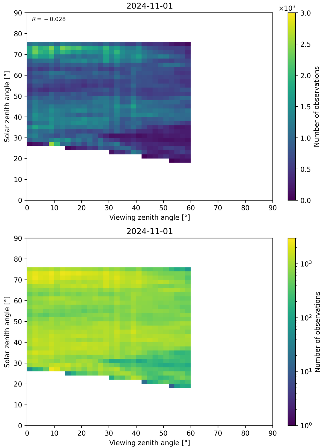
Figure 115: Scatter density plot of “Viewing zenith angle” against “Solar zenith angle” for 2024-10-31 to 2024-11-02.
