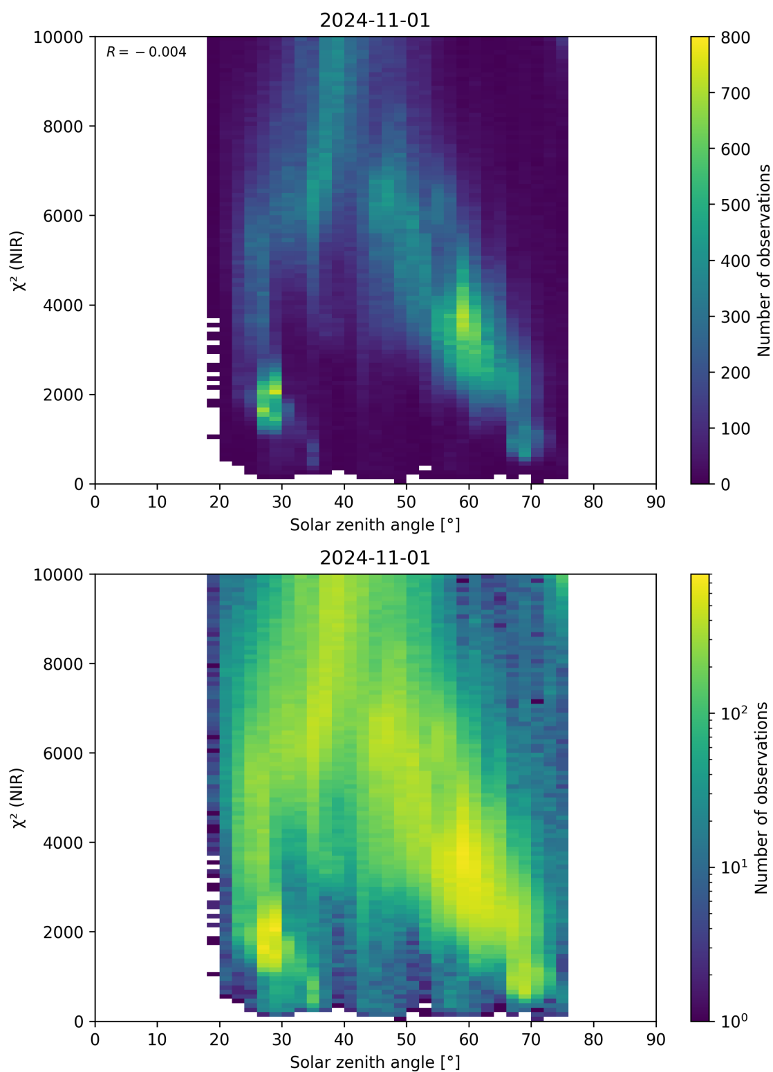
Figure 94: Scatter density plot of “Solar zenith angle” against “ \chi^2 (NIR)” for 2024-10-31 to 2024-11-02.
