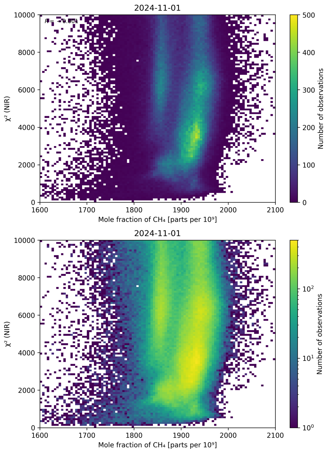
Figure 70: Scatter density plot of “Mole fraction of CH 4 ” against “ \chi^2 (NIR)” for 2024-10-31 to 2024-11-02.
