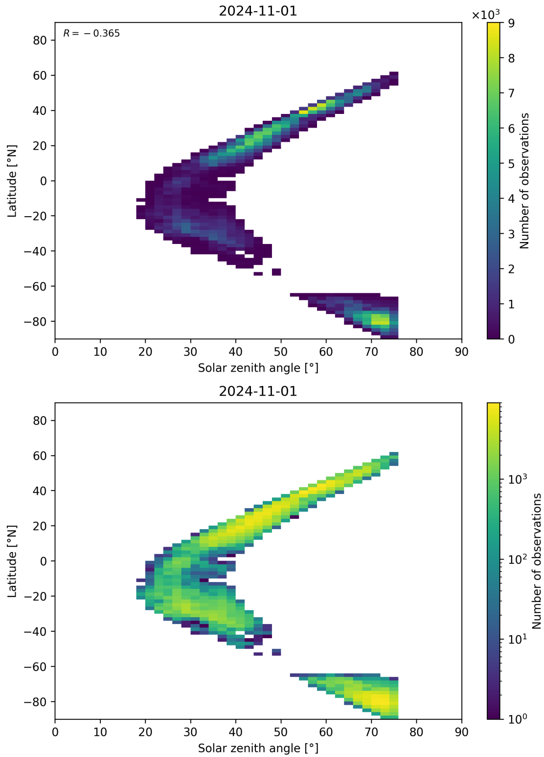
Figure 98: Scatter density plot of “Solar zenith angle” against “Latitude” for 2024-10-31 to 2024-11-02.
