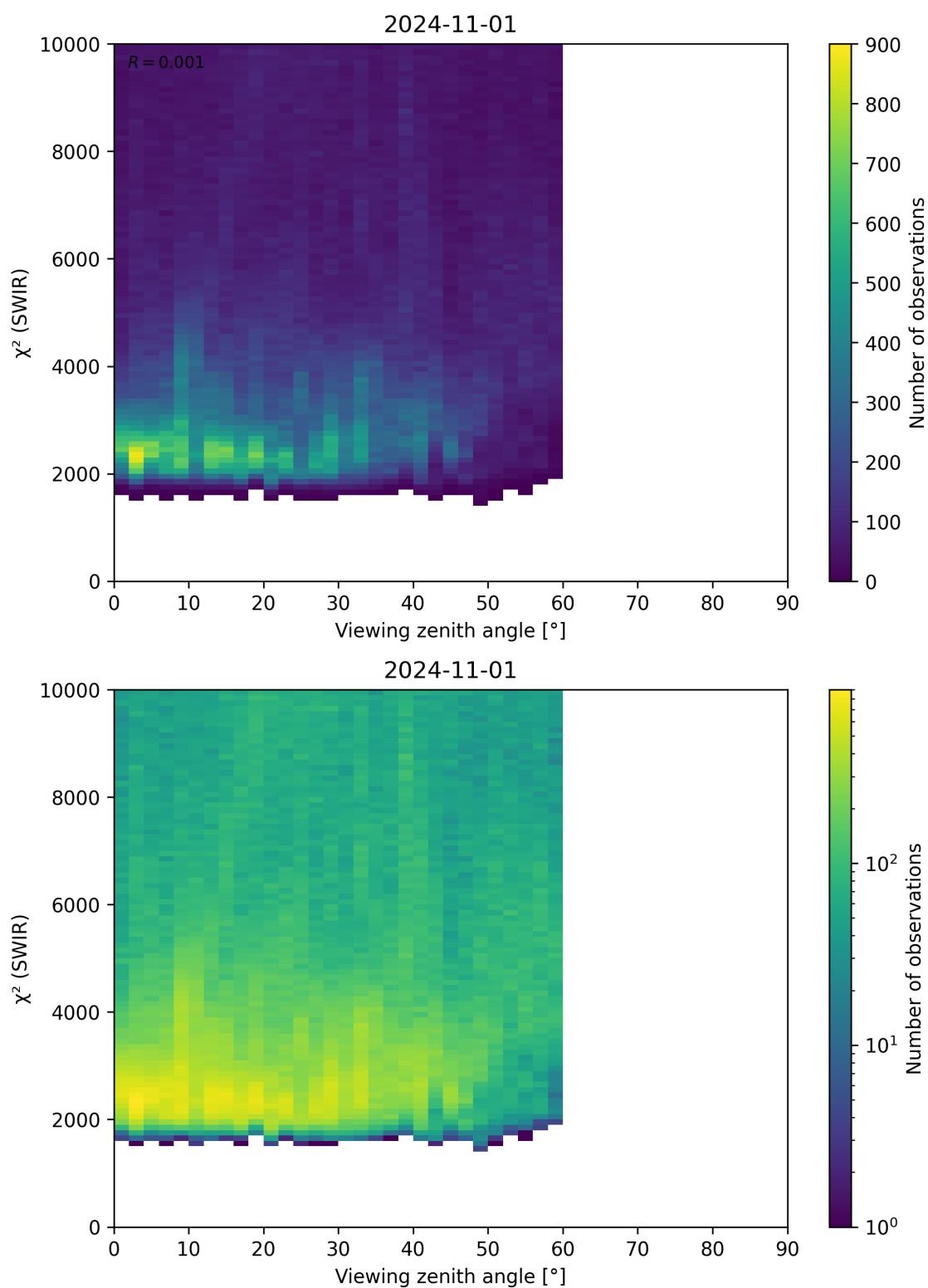
Figure 106: Scatter density plot of “Viewing zenith angle” against “ \chi^2 (SWIR)” for 2024-10-31 to 2024-11-02.
