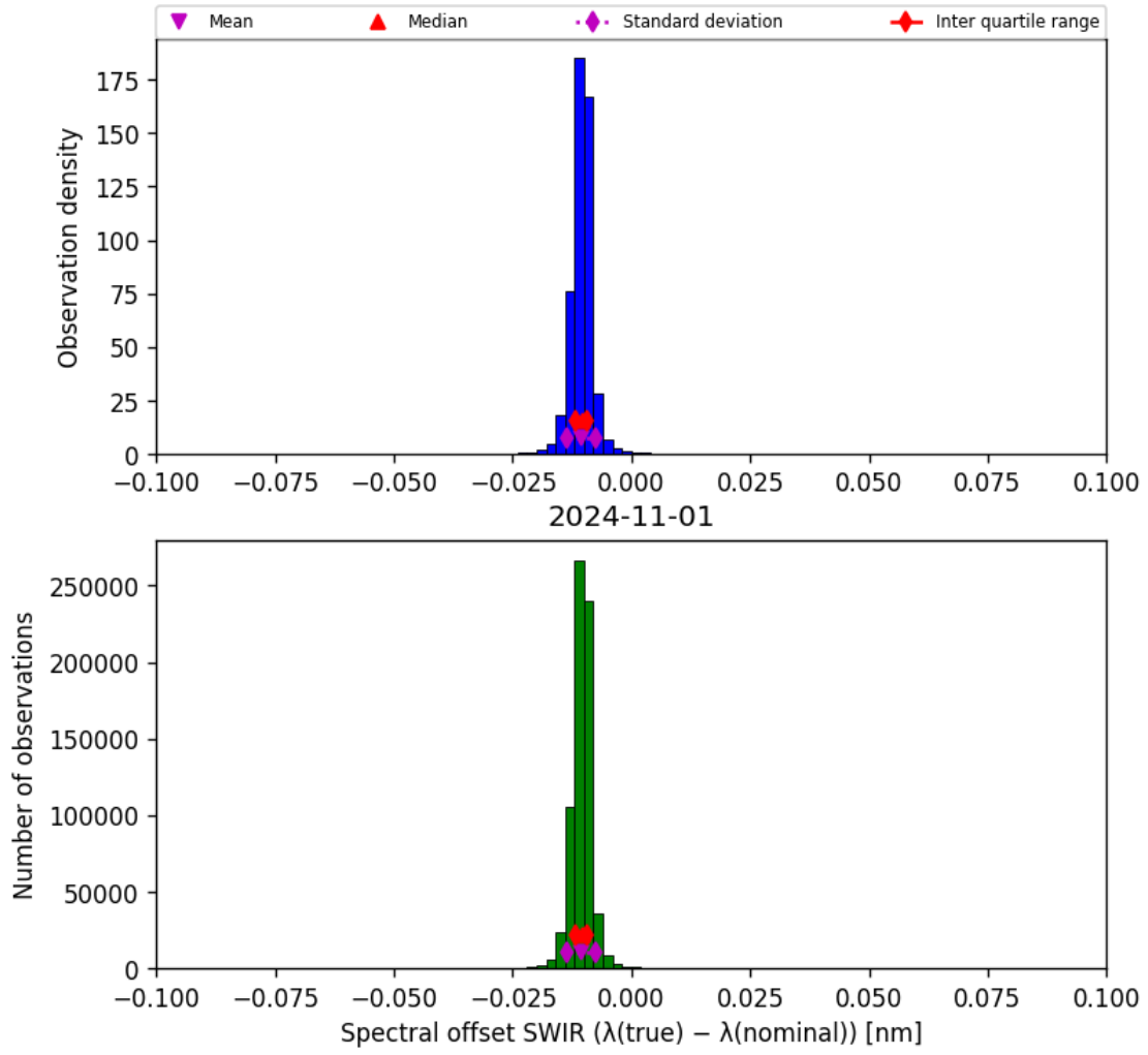
Figure 27: Histogram of “Spectral offset SWIR ( \lambda_{\text{true}} - \lambda_{\text{nominal}} )” for 2024-10-31 to 2024-11-02
