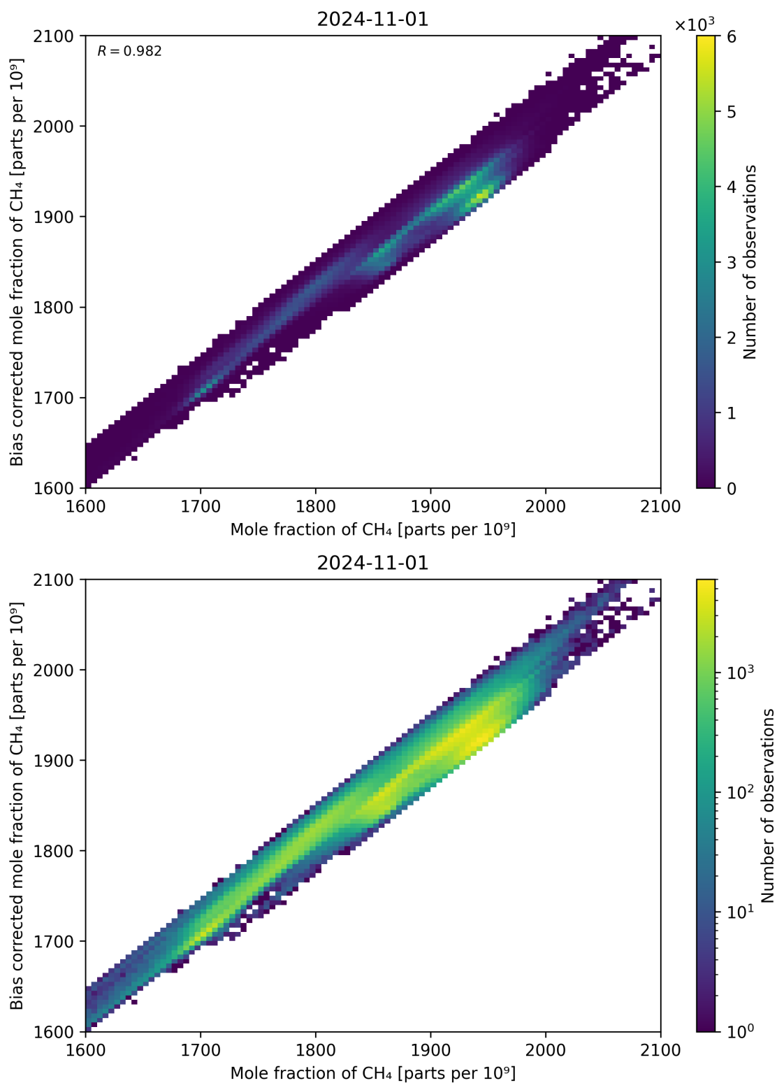
Figure 74: Scatter density plot of “Mole fraction of CH 4 ” against “Bias corrected mole fraction of CH 4 ” for 2024-10-31 to 2024-11-02.
