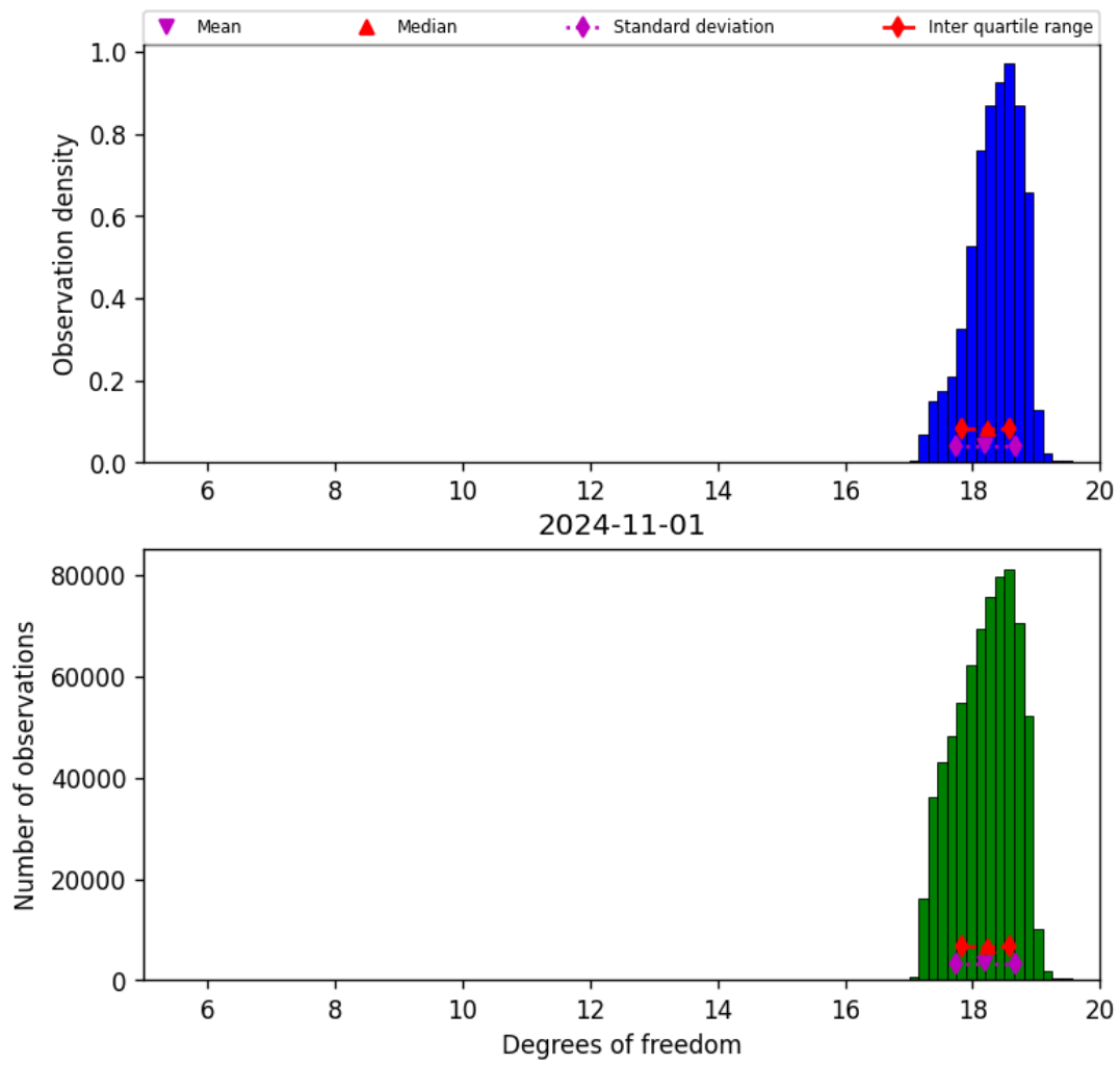
Figure 30: Histogram of “Degrees of freedom” for 2024-10-31 to 2024-11-02
