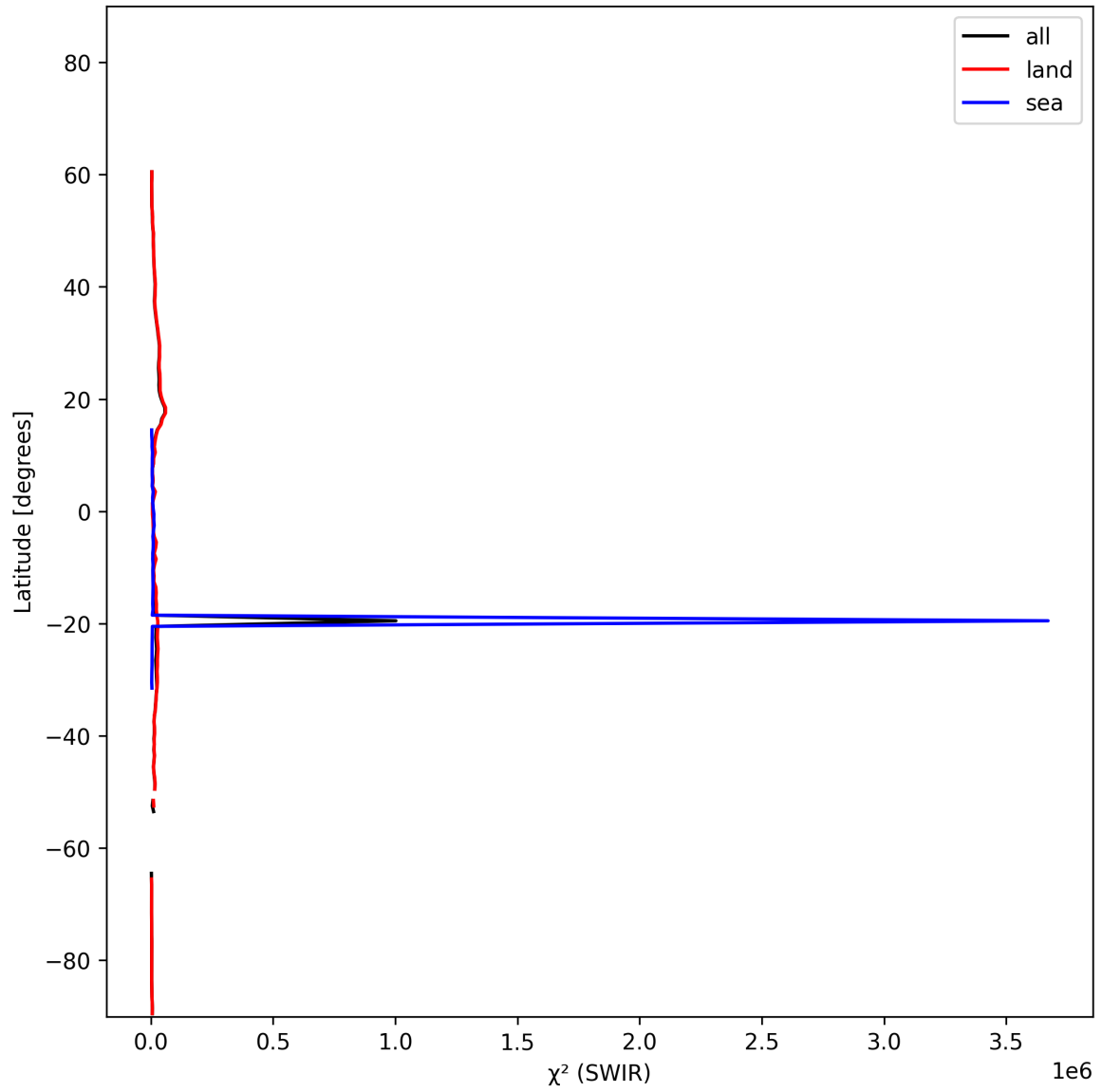
Figure 17: Zonal average of “ \chi^2 (SWIR)” for 2024-10-31 to 2024-11-02.
