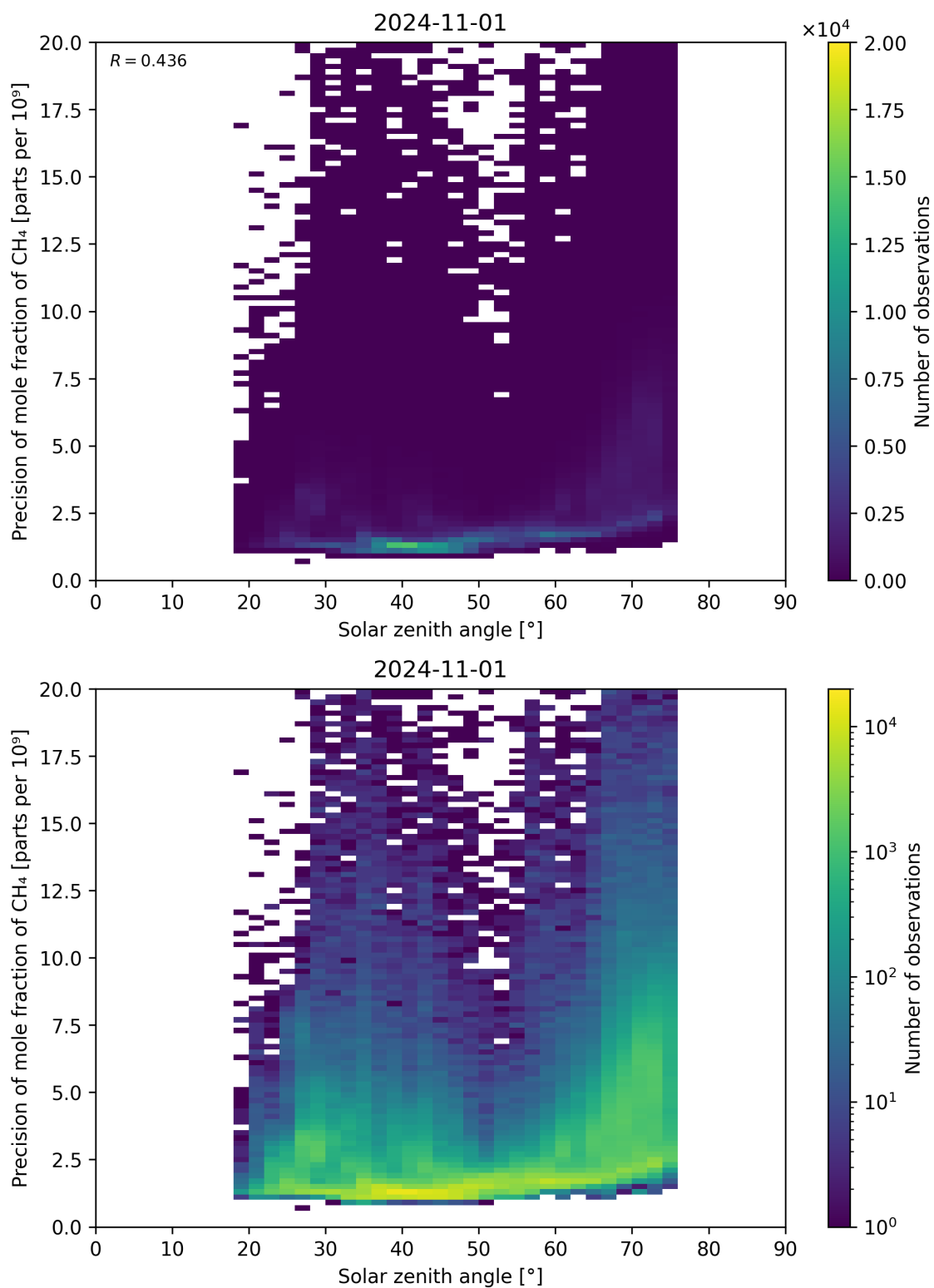
Figure 101: Scatter density plot of “Solar zenith angle” against “Precision of mole fraction of CH 4 ” for 2024-10-31 to 2024-11-02.
