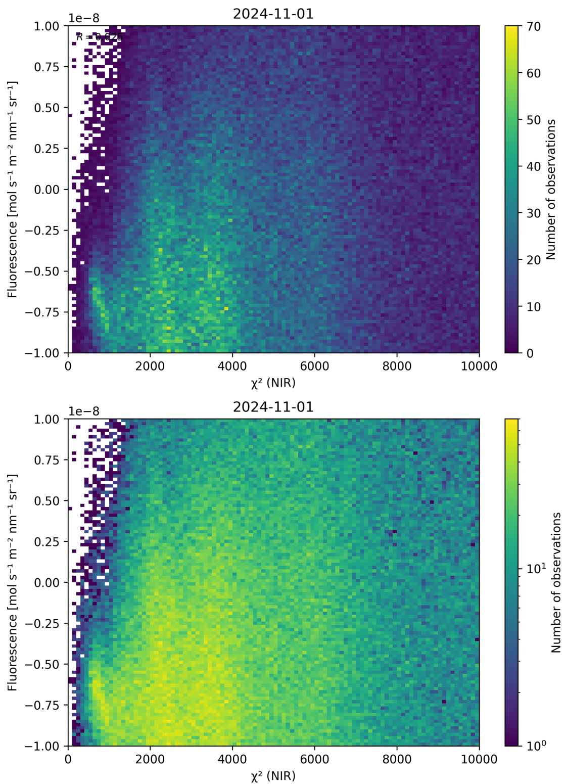
Figure 45: Scatter density plot of “ \chi^2 (NIR)” against “Fluorescence” for 2024-10-31 to 2024-11-02.
