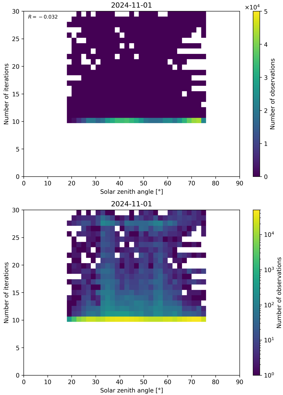
Figure 102: Scatter density plot of “Solar zenith angle” against “Number of iterations” for 2024-10-31 to 2024-11-02.
