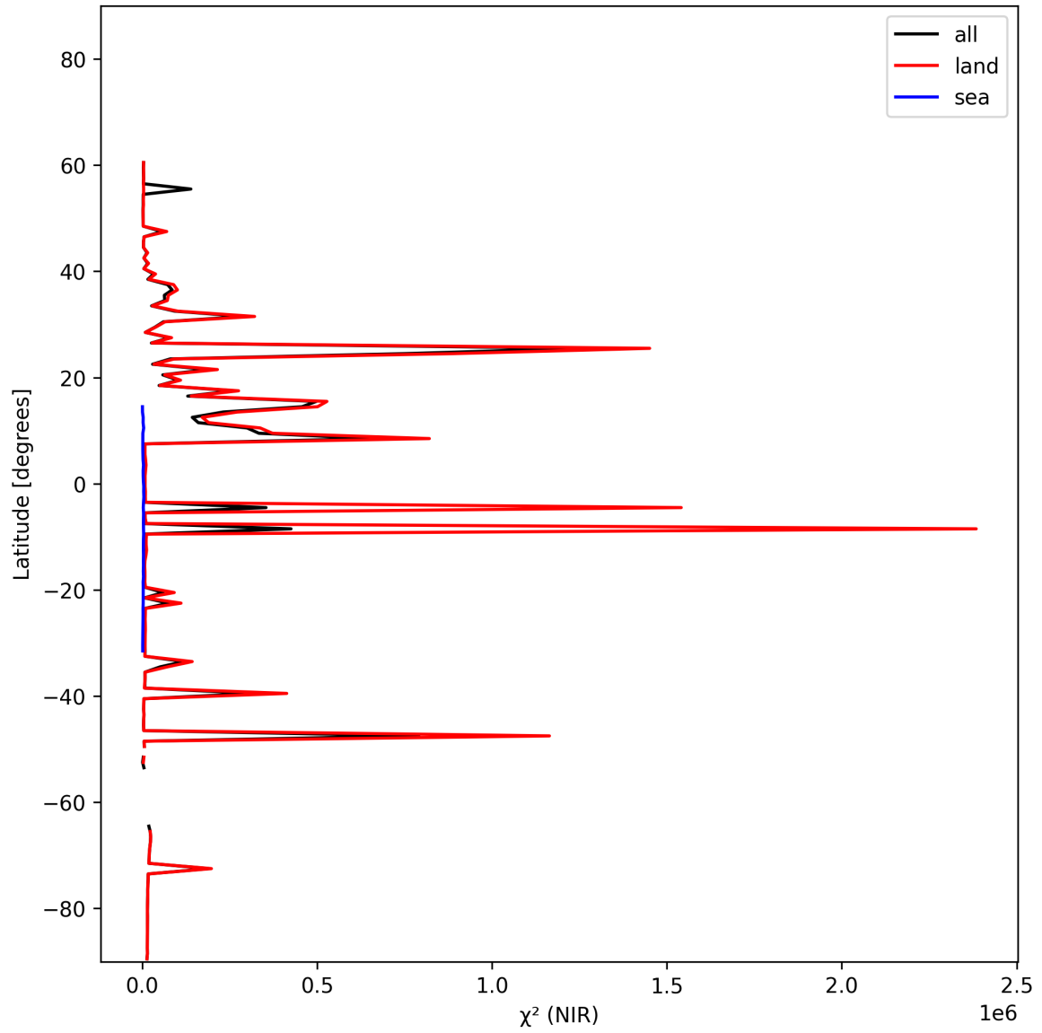
Figure 18: Zonal average of “ \chi^2 (NIR)” for 2024-10-31 to 2024-11-02.
