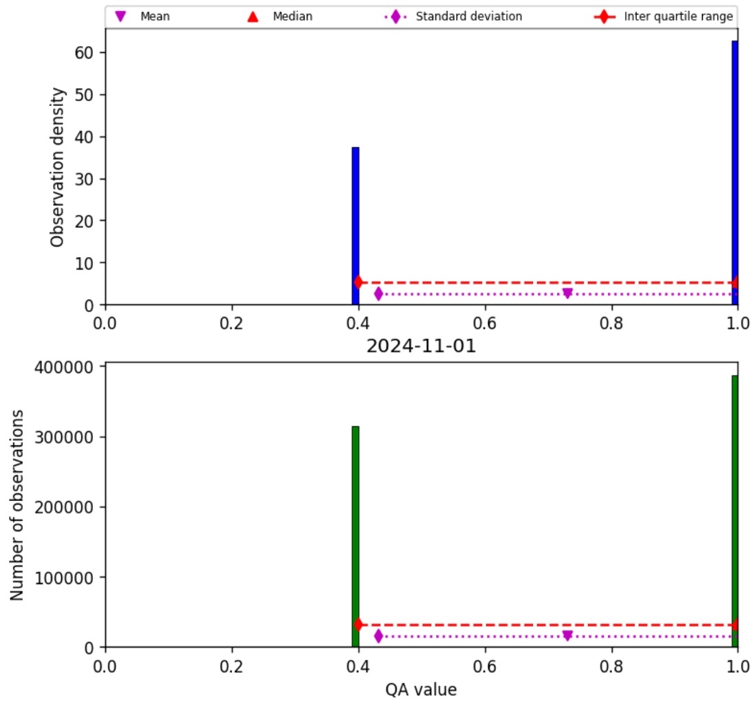
Figure 22: Histogram of “QA value” for 2024-10-31 to 2024-11-02
