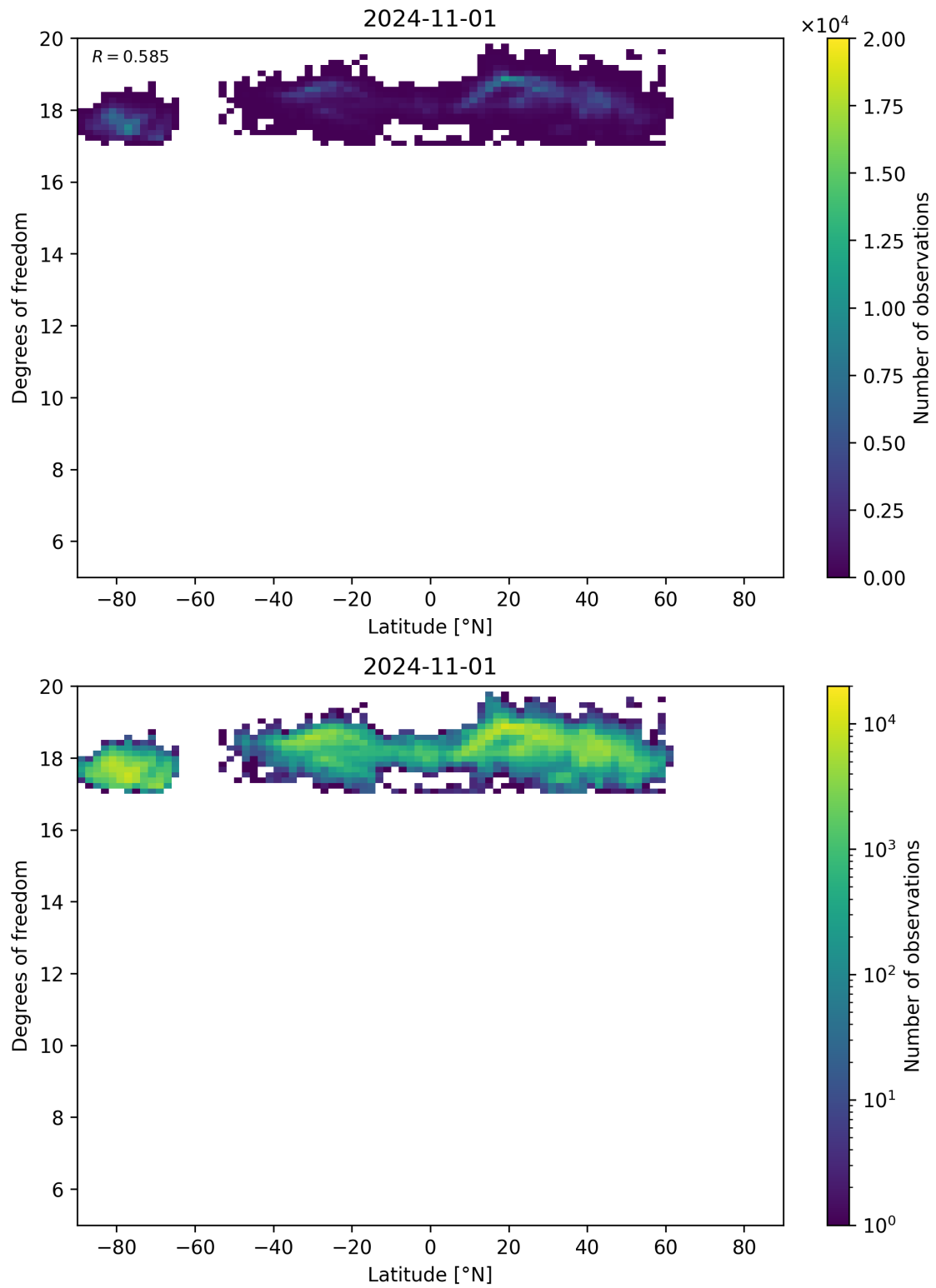
Figure 55: Scatter density plot of “Latitude” against “Degrees of freedom” for 2024-10-31 to 2024-11-02.
