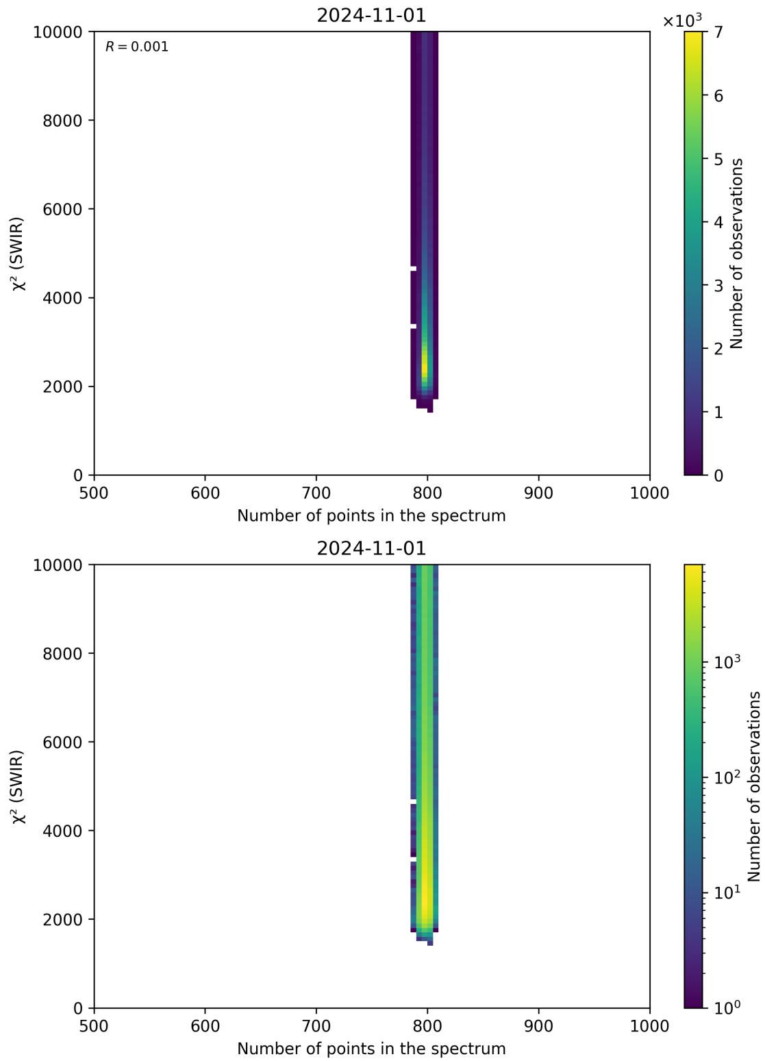
Figure 89: Scatter density plot of “Number of points in the spectrum” against “ \chi^2 (SWIR)” for 2024-10-31 to 2024-11-02.
