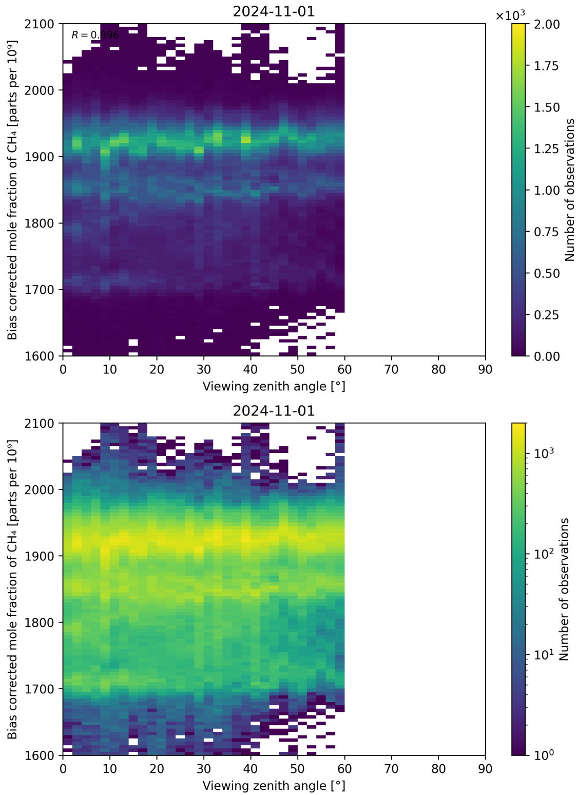
Figure 111: Scatter density plot of “Viewing zenith angle” against “Bias corrected mole fraction of CH 4 ” for 2024-10-31 to 2024-11-02.
