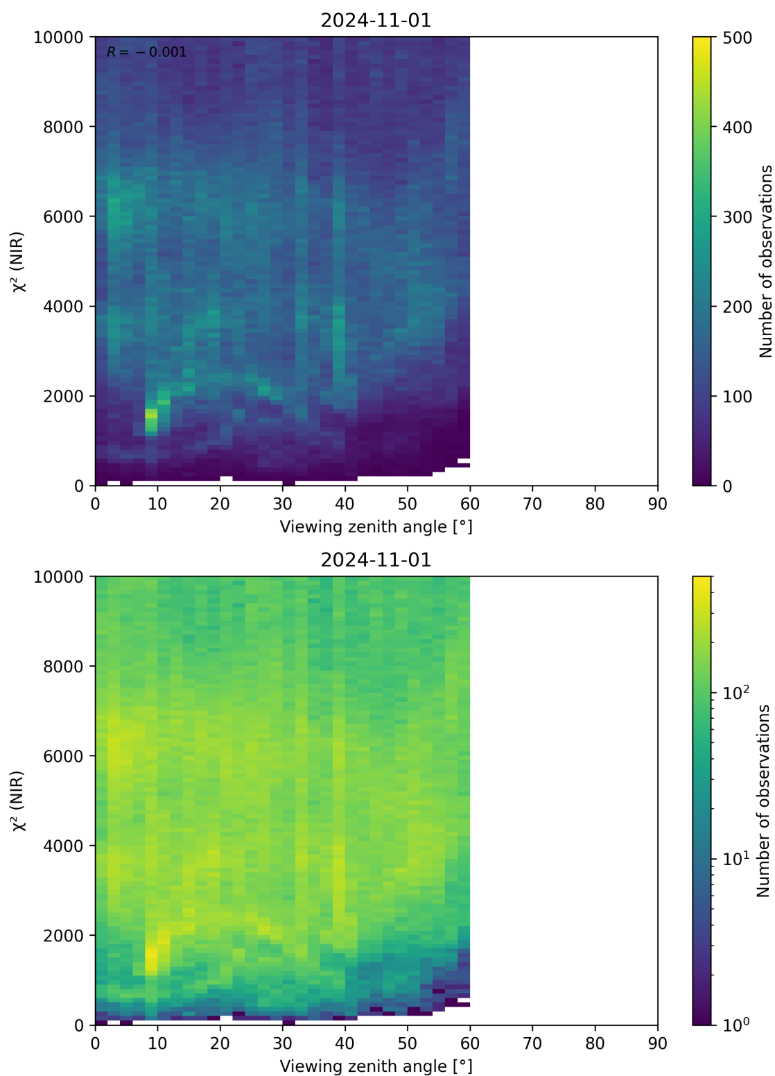
Figure 105: Scatter density plot of “Viewing zenith angle” against “ \chi^2 (NIR)” for 2024-10-31 to 2024-11-02.
