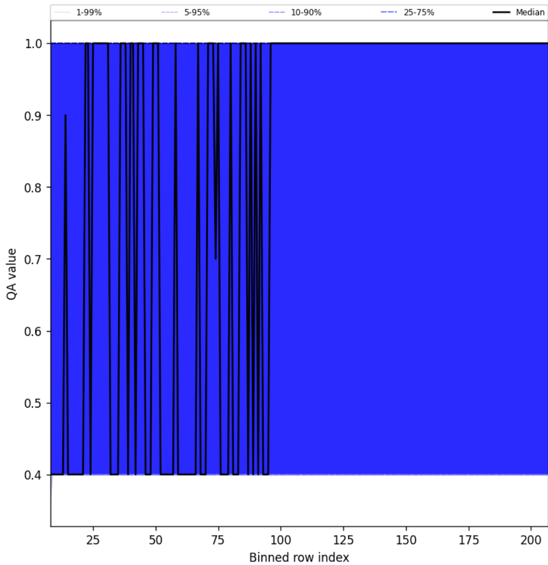
Figure 33: Along track statistics of “QA value” for 2024-10-31 to 2024-11-02
