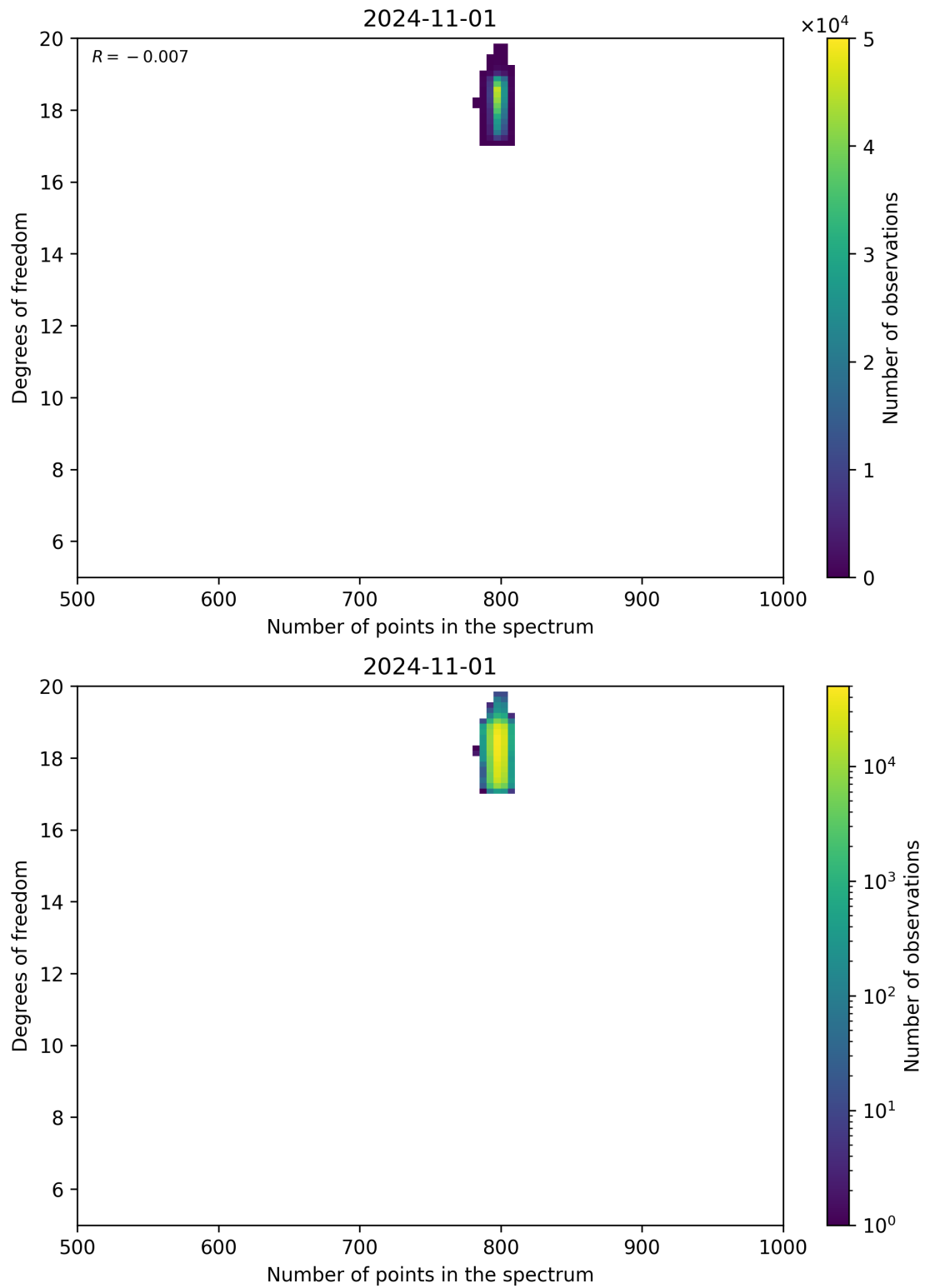
Figure 90: Scatter density plot of “Number of points in the spectrum” against “Degrees of freedom” for 2024-10-31 to 2024-11-02.
