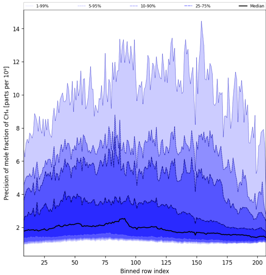
Figure 35: Along track statistics of “Precision of mole fraction of CH 4 ” for 2024-10-31 to 2024-11-02
