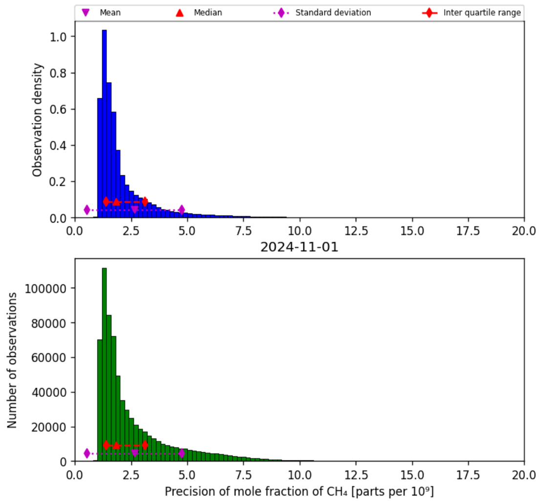
Figure 24: Histogram of “Precision of mole fraction of CH 4 ” for 2024-10-31 to 2024-11-02
