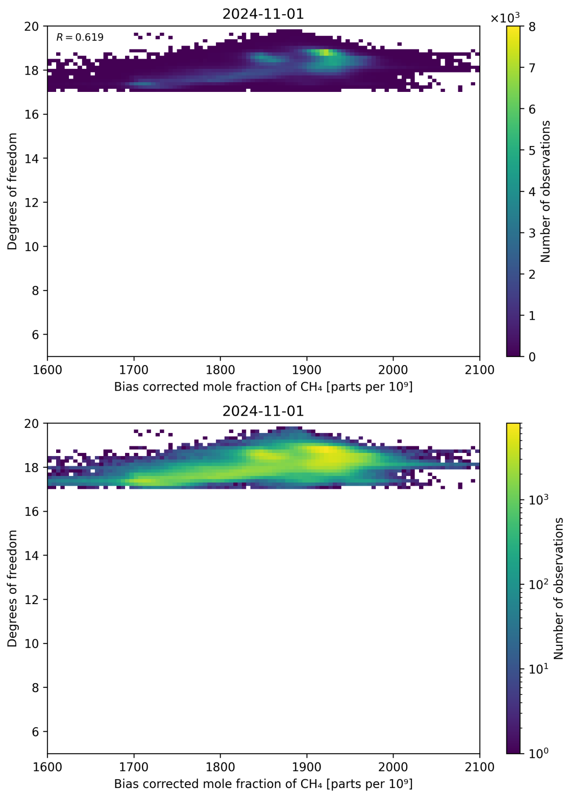
Figure 65: Scatter density plot of “Bias corrected mole fraction of CH 4 ” against “Degrees of freedom” for 2024-10-31 to 2024-11-02.
