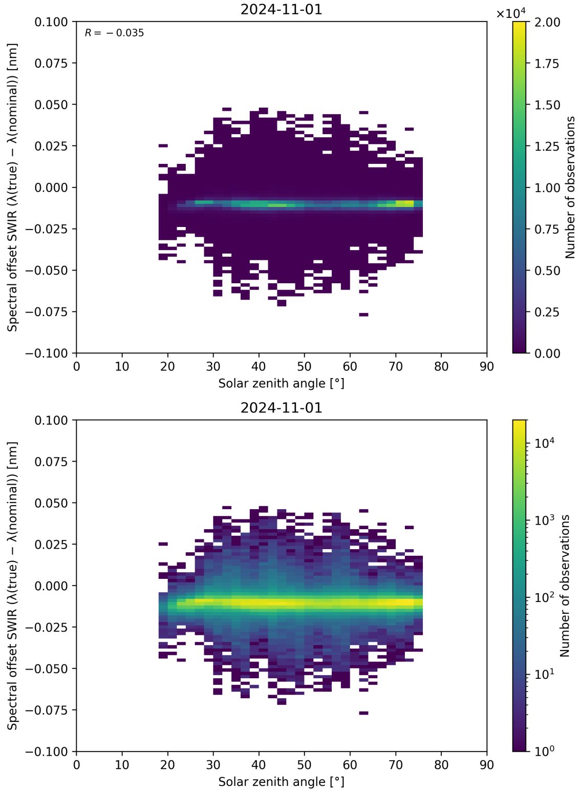
Figure 104: Scatter density plot of “Solar zenith angle” against “Spectral offset SWIR ( \lambda_{\text{true}} - \lambda_{\text{nominal}} )” for 2024-10-31 to 2024-11-02.
