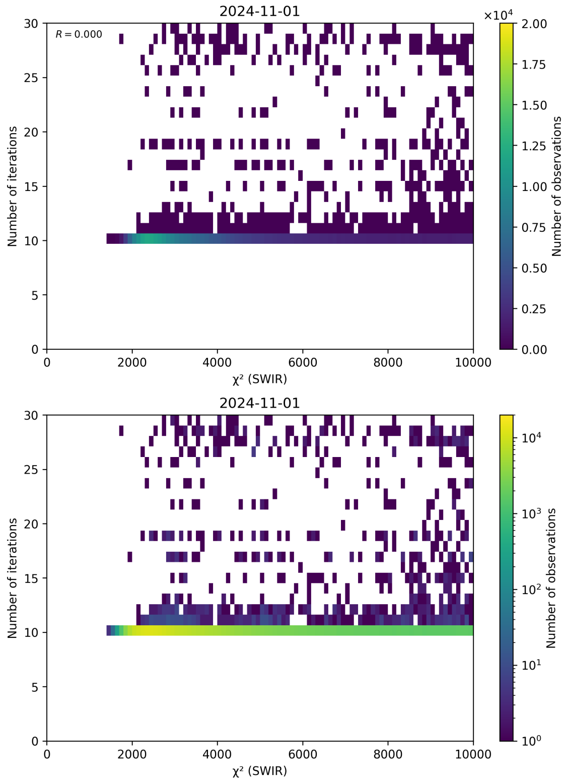
Figure 50: Scatter density plot of “ \chi^2 (SWIR)” against “Number of iterations” for 2024-10-31 to 2024-11-02.
