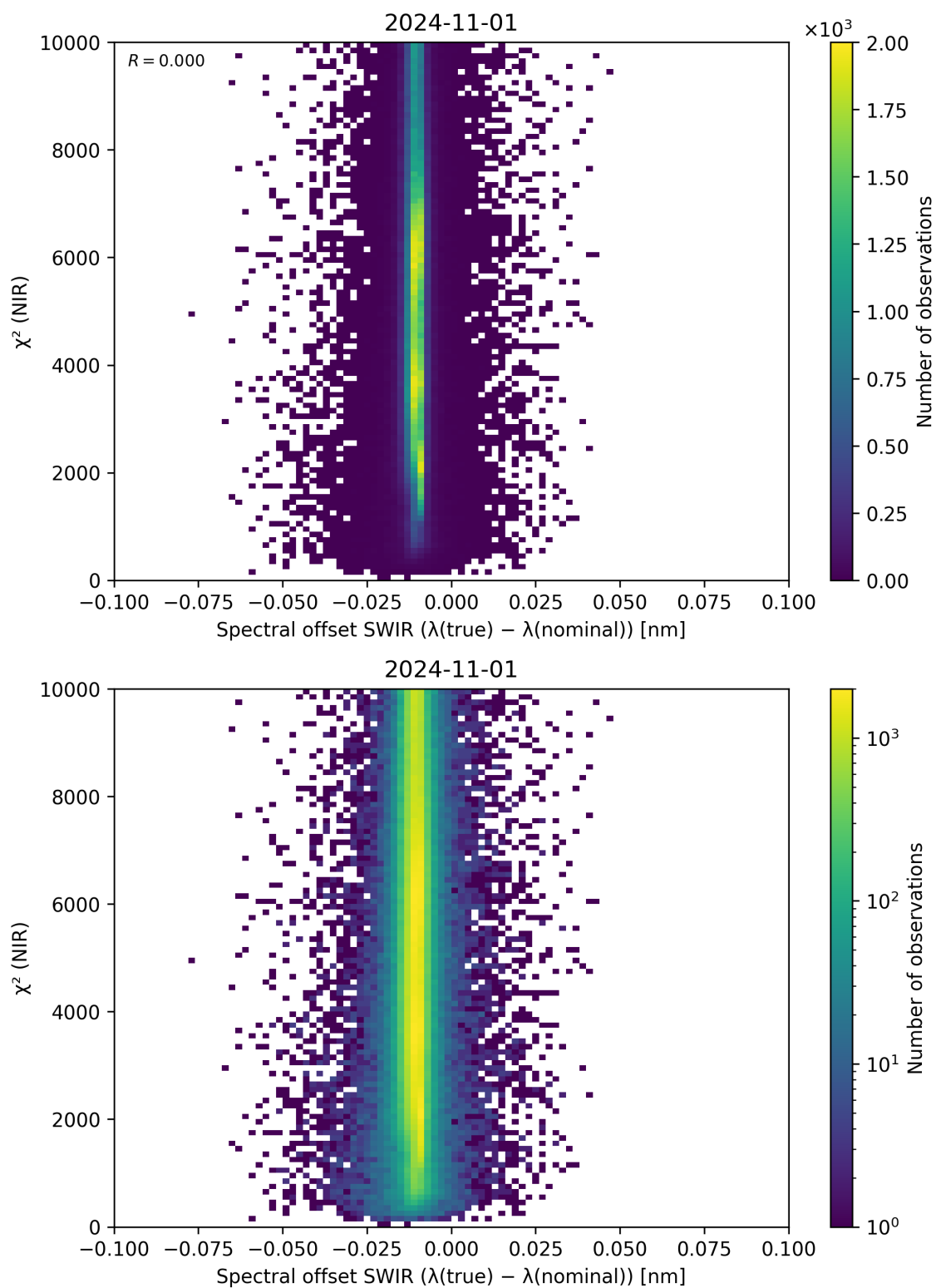
Figure 117: Scatter density plot of “Spectral offset SWIR ( \lambda_{\text{true}} - \lambda_{\text{nominal}} )” against “ \chi^2 (NIR)” for 2024-10-31 to 2024-11-02.
