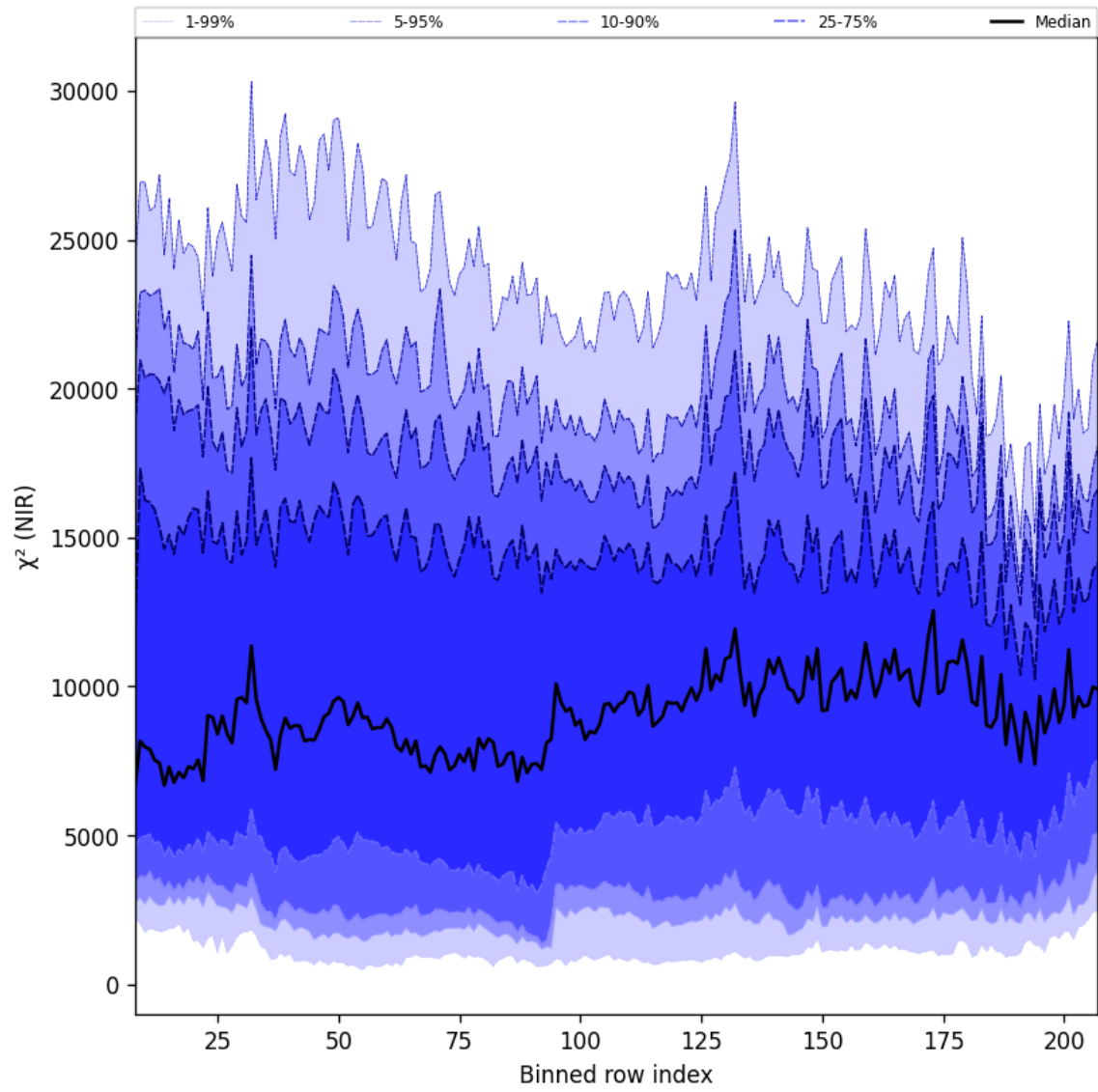
Figure 40: Along track statistics of “ \chi^2 (NIR)” for 2024-10-31 to 2024-11-02
