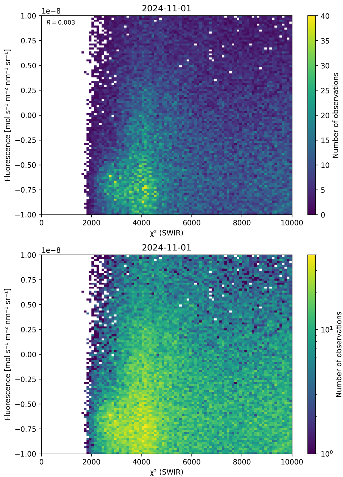
Figure 49: Scatter density plot of “ \chi^2 (SWIR)” against “Fluorescence” for 2024-10-31 to 2024-11-02.
