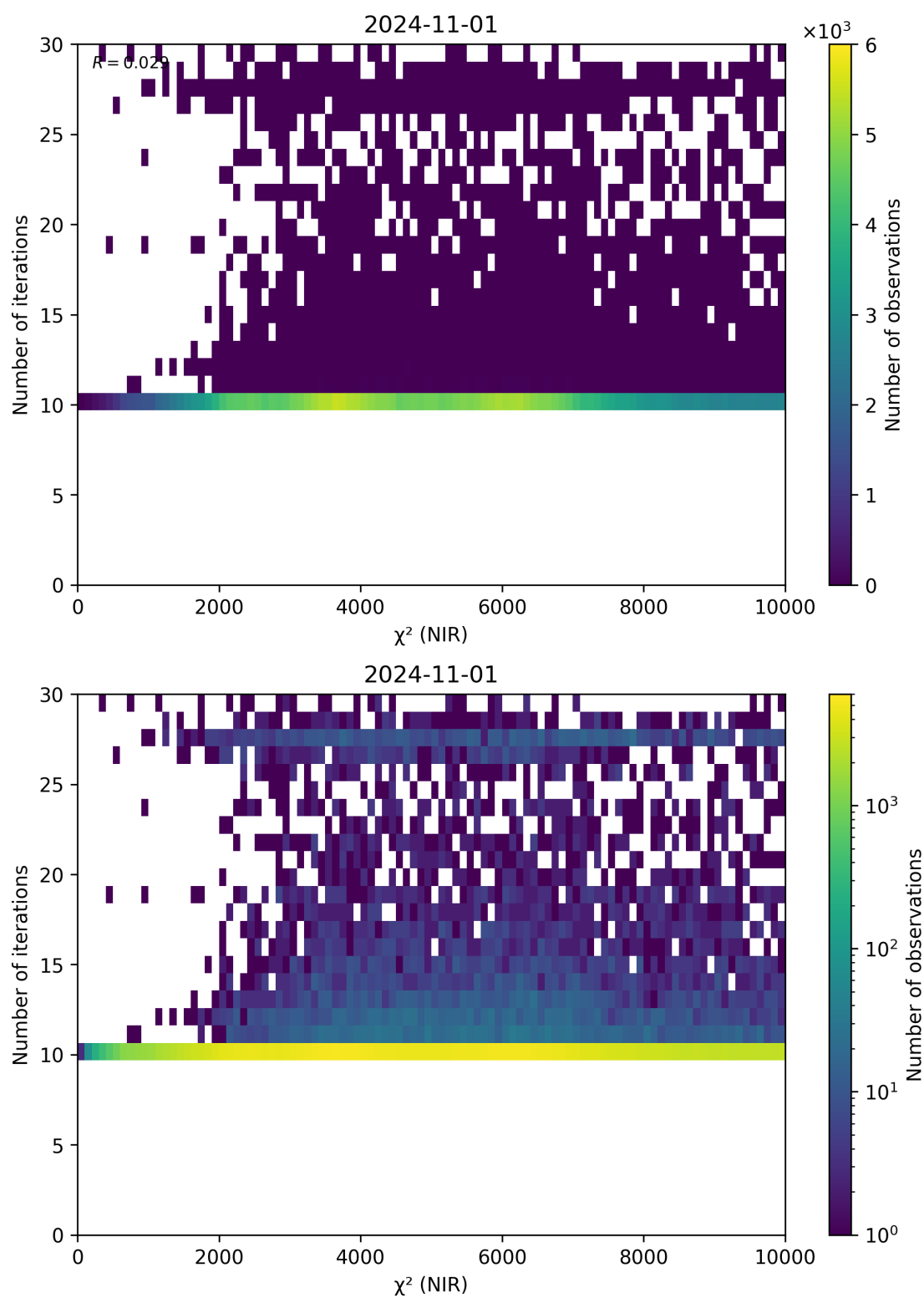
Figure 46: Scatter density plot of “ \chi^2 (NIR)” against “Number of iterations” for 2024-10-31 to 2024-11-02.
