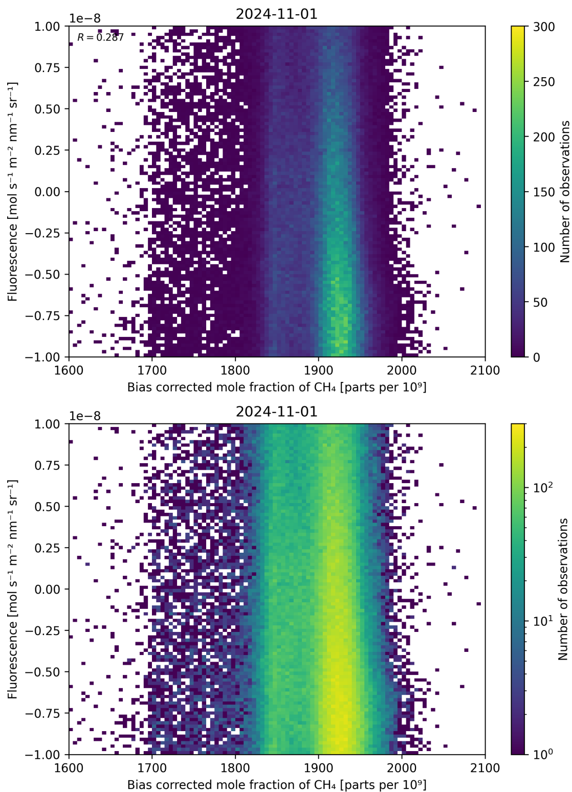
Figure 66: Scatter density plot of “Bias corrected mole fraction of \text{CH}_4 ” against “Fluorescence” for 2024-10-31 to 2024-11-02.
