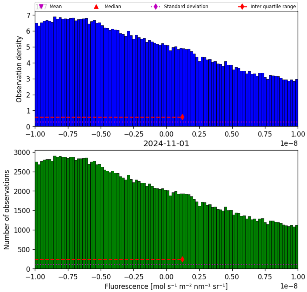
Figure 32: Histogram of “Fluorescence” for 2024-10-31 to 2024-11-02
