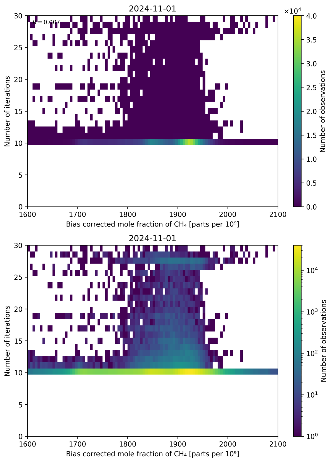
Figure 67: Scatter density plot of “Bias corrected mole fraction of CH 4 ” against “Number of iterations” for 2024-10-31 to 2024-11-02.
