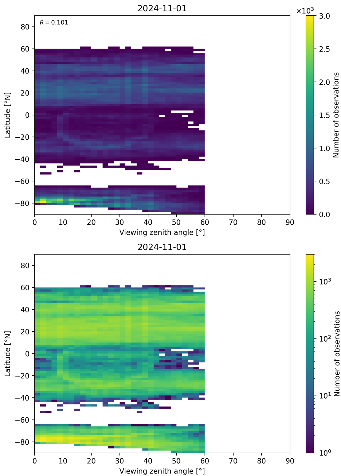
Figure 109: Scatter density plot of “Viewing zenith angle” against “Latitude” for 2024-10-31 to 2024-11-02.
