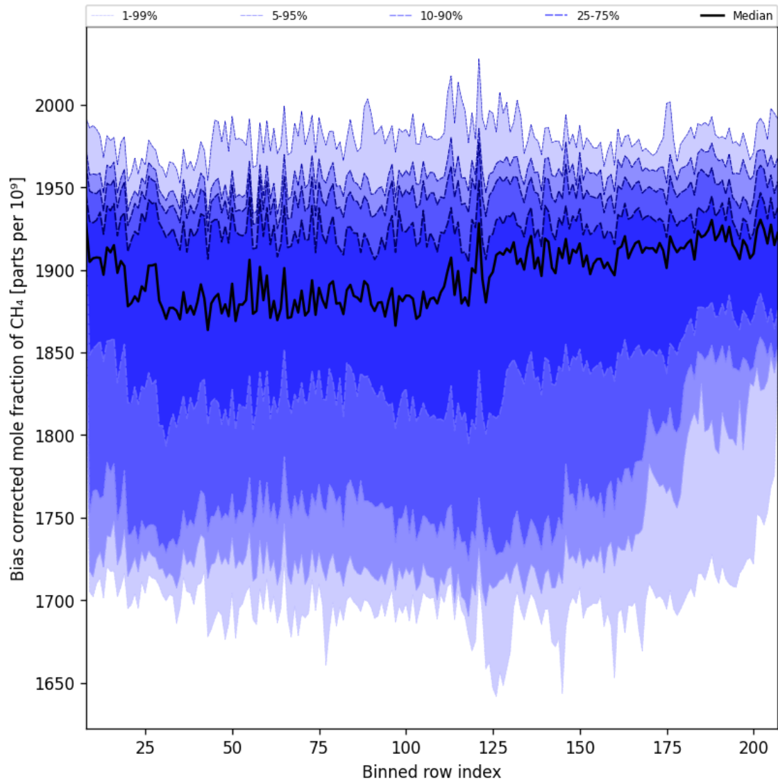
Figure 36: Along track statistics of “Bias corrected mole fraction of \text{CH}_4 ” for 2024-10-31 to 2024-11-02
