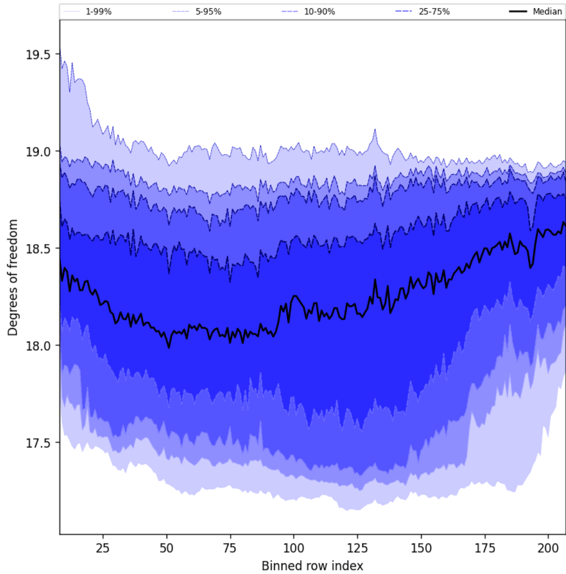
Figure 41: Along track statistics of “Degrees of freedom” for 2024-10-31 to 2024-11-02
