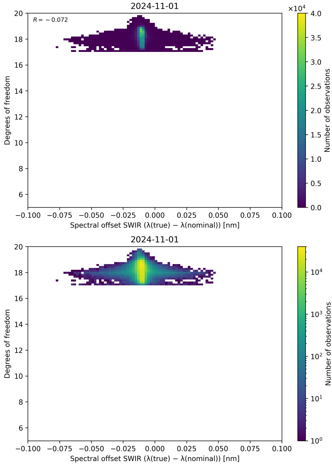
Figure 119: Scatter density plot of “Spectral offset SWIR ( \lambda_{\text{true}} - \lambda_{\text{nominal}} )” against “Degrees of freedom” for 2024-10-31 to 2024-11-02.
