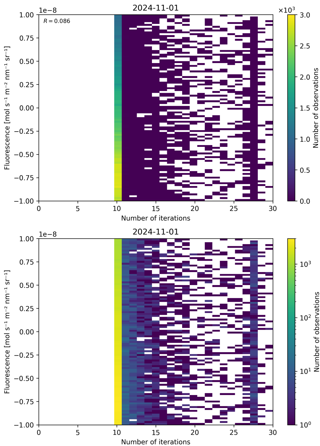
Figure 87: Scatter density plot of “Number of iterations” against “Fluorescence” for 2024-10-31 to 2024-11-02.
