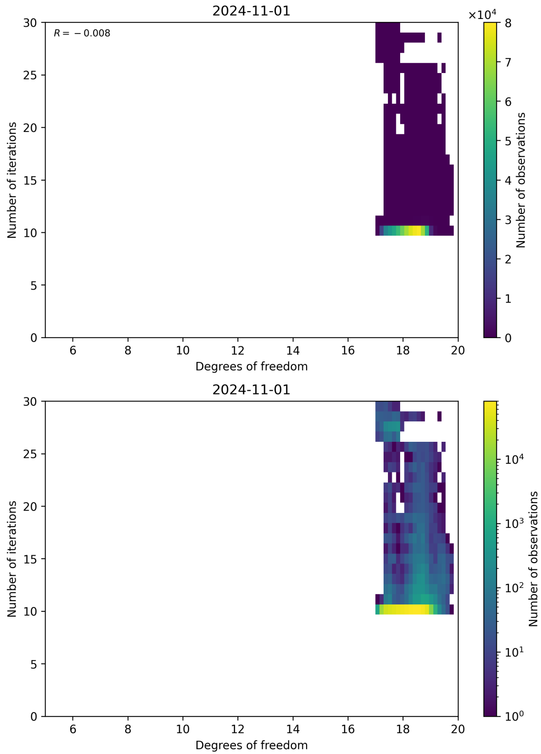
Figure 52: Scatter density plot of “Degrees of freedom” against “Number of iterations” for 2024-10-31 to 2024-11-02.
