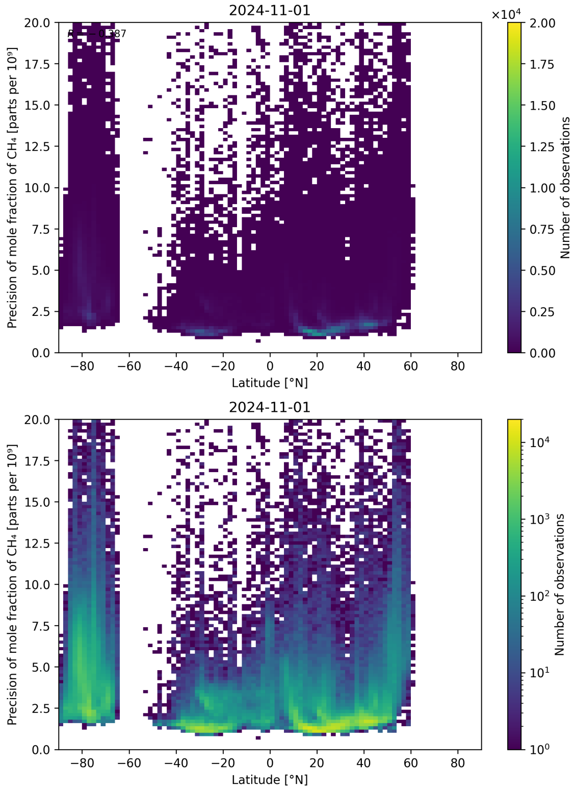
Figure 59: Scatter density plot of “Latitude” against “Precision of mole fraction of CH 4 ” for 2024-10-31 to 2024-11-02.
