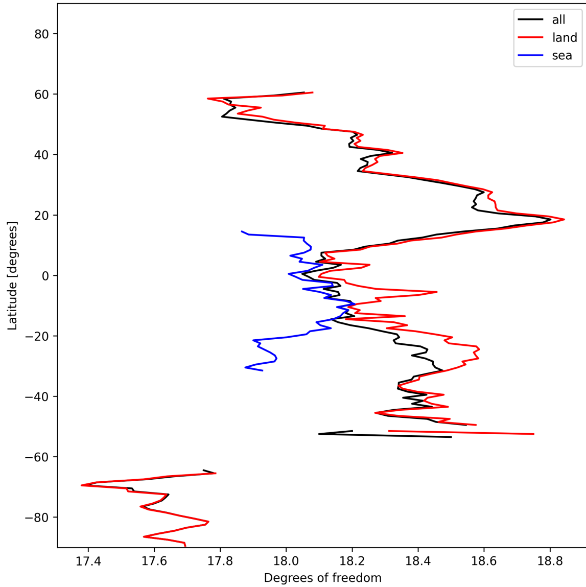
Figure 19: Zonal average of “Degrees of freedom” for 2024-10-31 to 2024-11-02.
