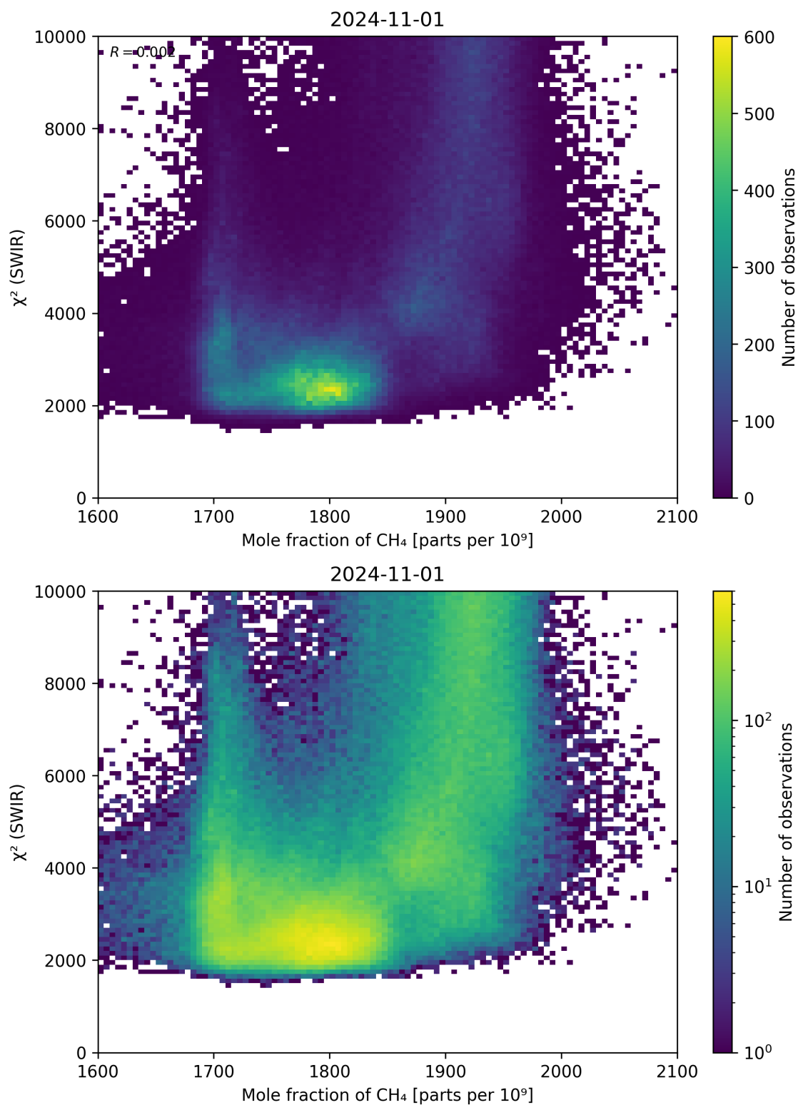
Figure 71: Scatter density plot of “Mole fraction of \text{CH}_4 ” against “ \chi^2 (SWIR)” for 2024-10-31 to 2024-11-02.
