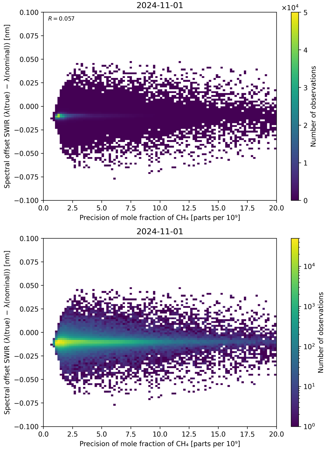
Figure 85: Scatter density plot of “Precision of mole fraction of \text{CH}_4 ” against “Spectral offset SWIR ( \lambda_{\text{true}} - \lambda_{\text{nominal}} )” for 2024-10-31 to 2024-11-02.
