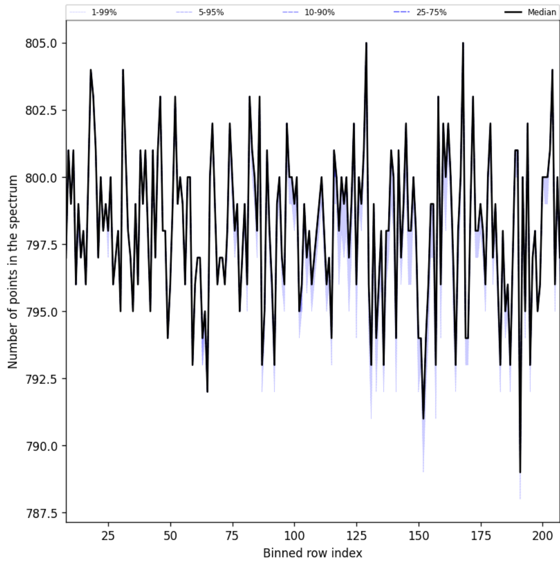
Figure 37: Along track statistics of “Number of points in the spectrum” for 2024-10-31 to 2024-11-02
