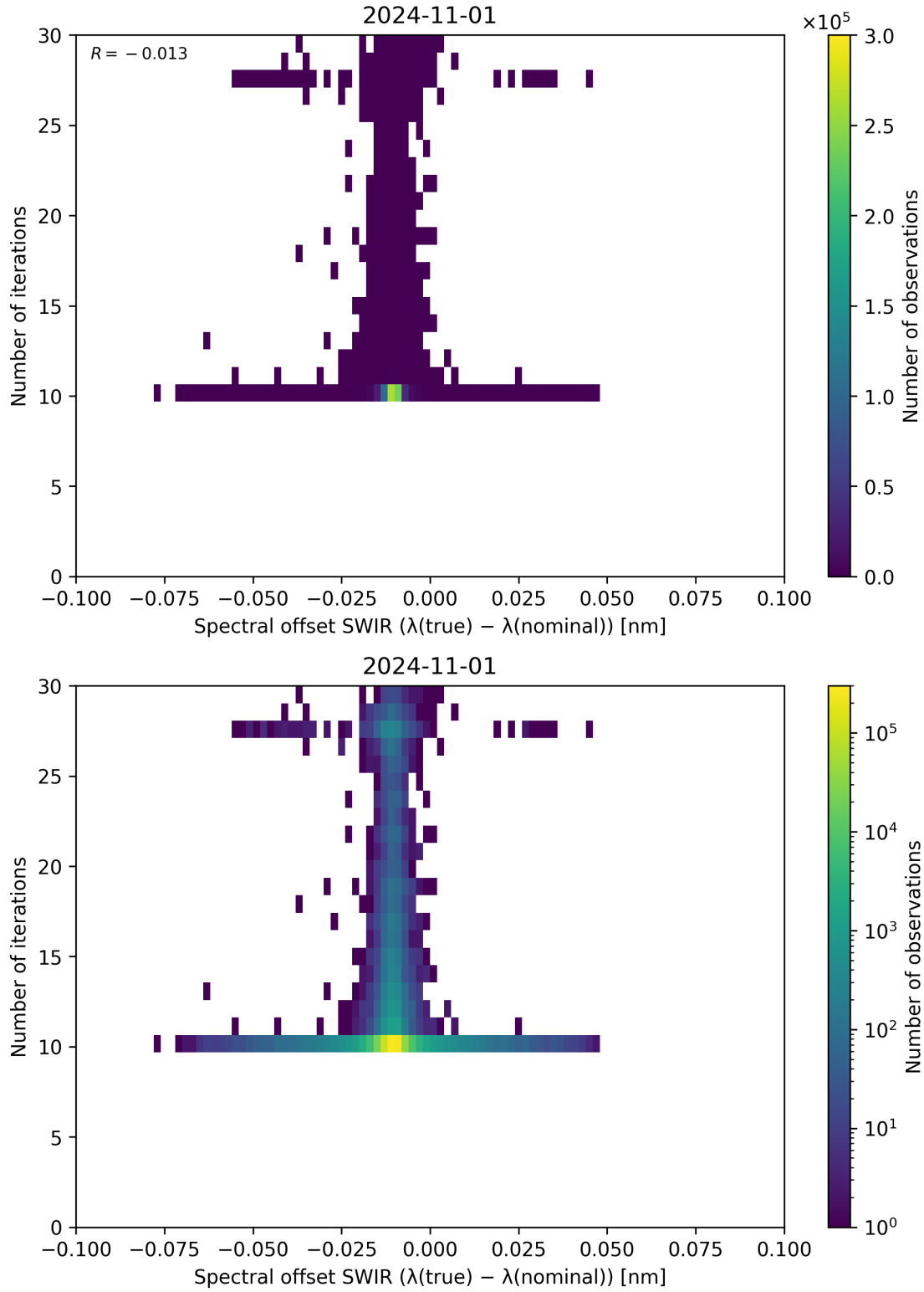
Figure 121: Scatter density plot of “Spectral offset SWIR ( \lambda_{\text{true}} - \lambda_{\text{nominal}} )” against “Number of iterations” for 2024-10-31 to 2024-11-02.
