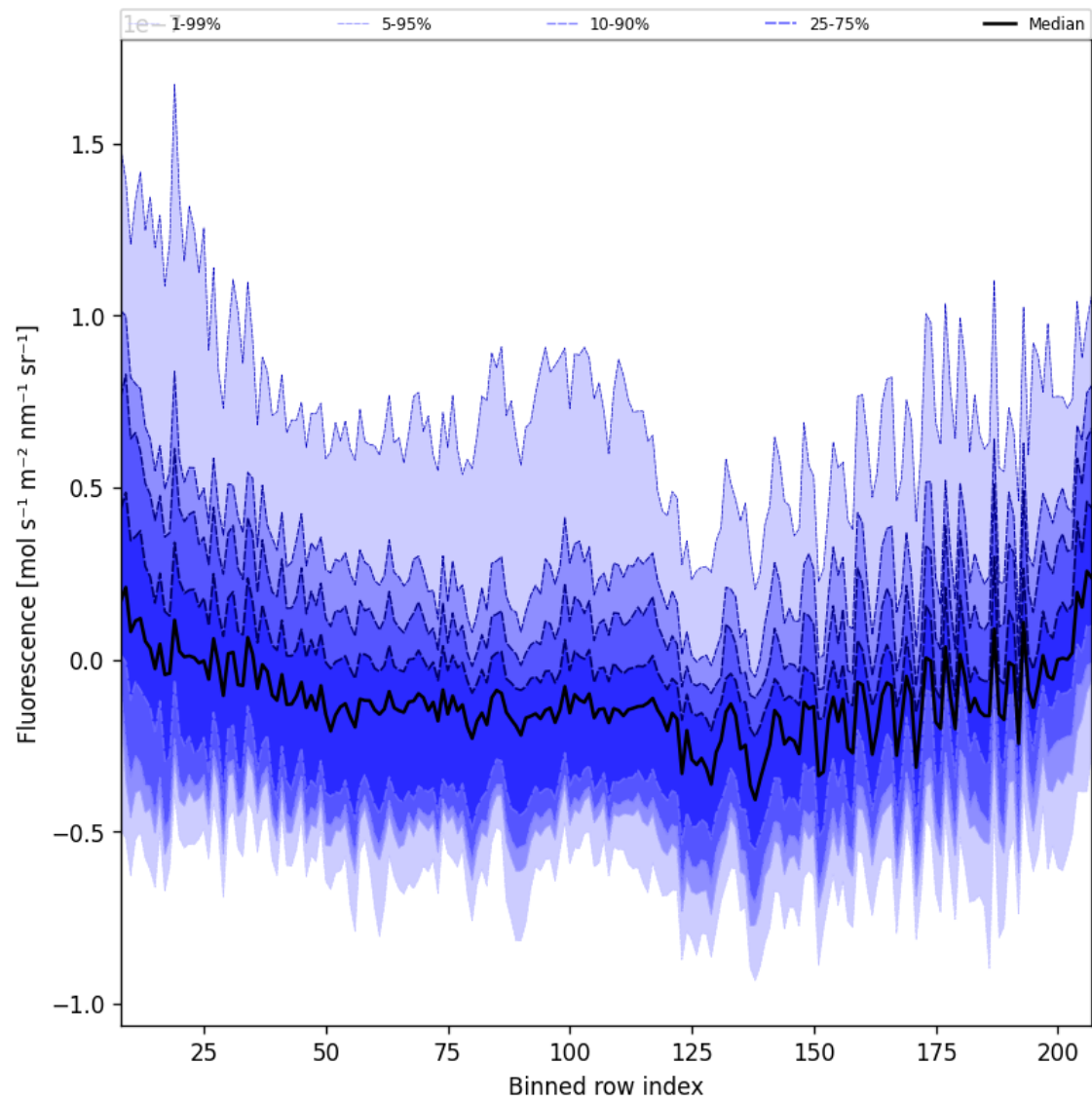
Figure 43: Along track statistics of “Fluorescence” for 2024-10-31 to 2024-11-02
