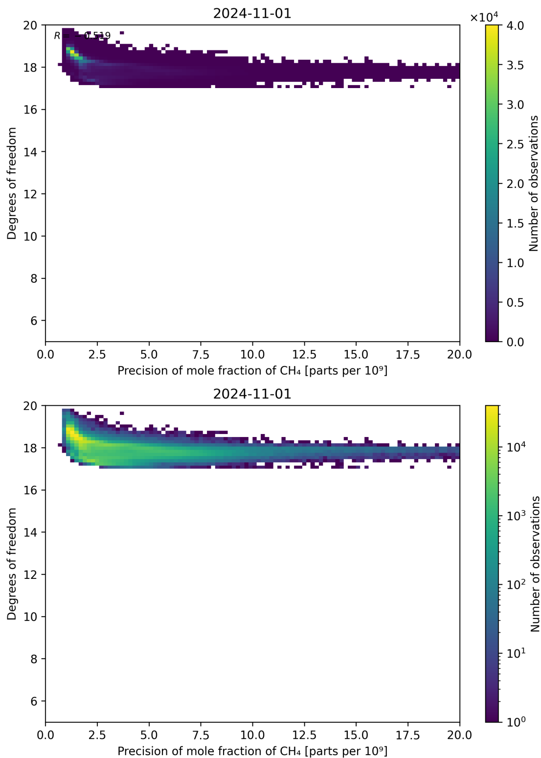
Figure 80: Scatter density plot of “Precision of mole fraction of CH 4 ” against “Degrees of freedom” for 2024-10-31 to 2024-11-02.
