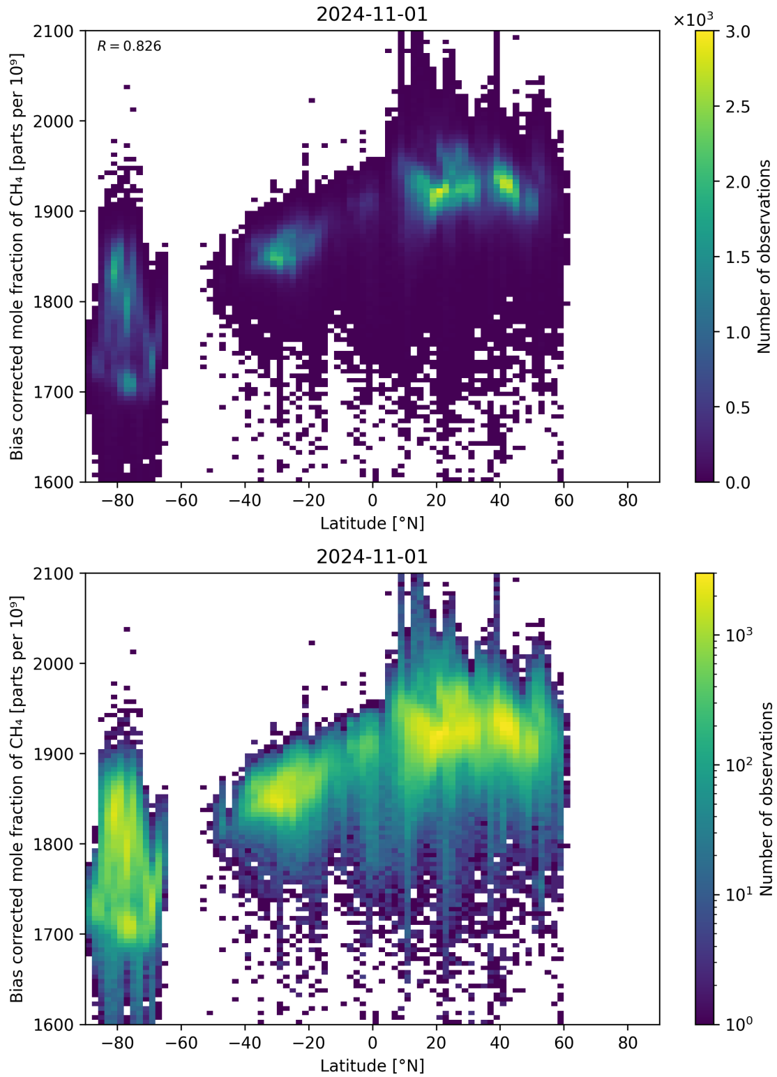
Figure 58: Scatter density plot of “Latitude” against “Bias corrected mole fraction of \text{CH}_4 ” for 2024-10-31 to 2024-11-02.
