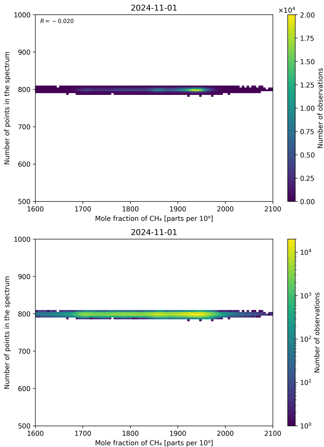
Figure 77: Scatter density plot of “Mole fraction of CH 4 ” against “Number of points in the spectrum” for 2024-10-31 to 2024-11-02.
