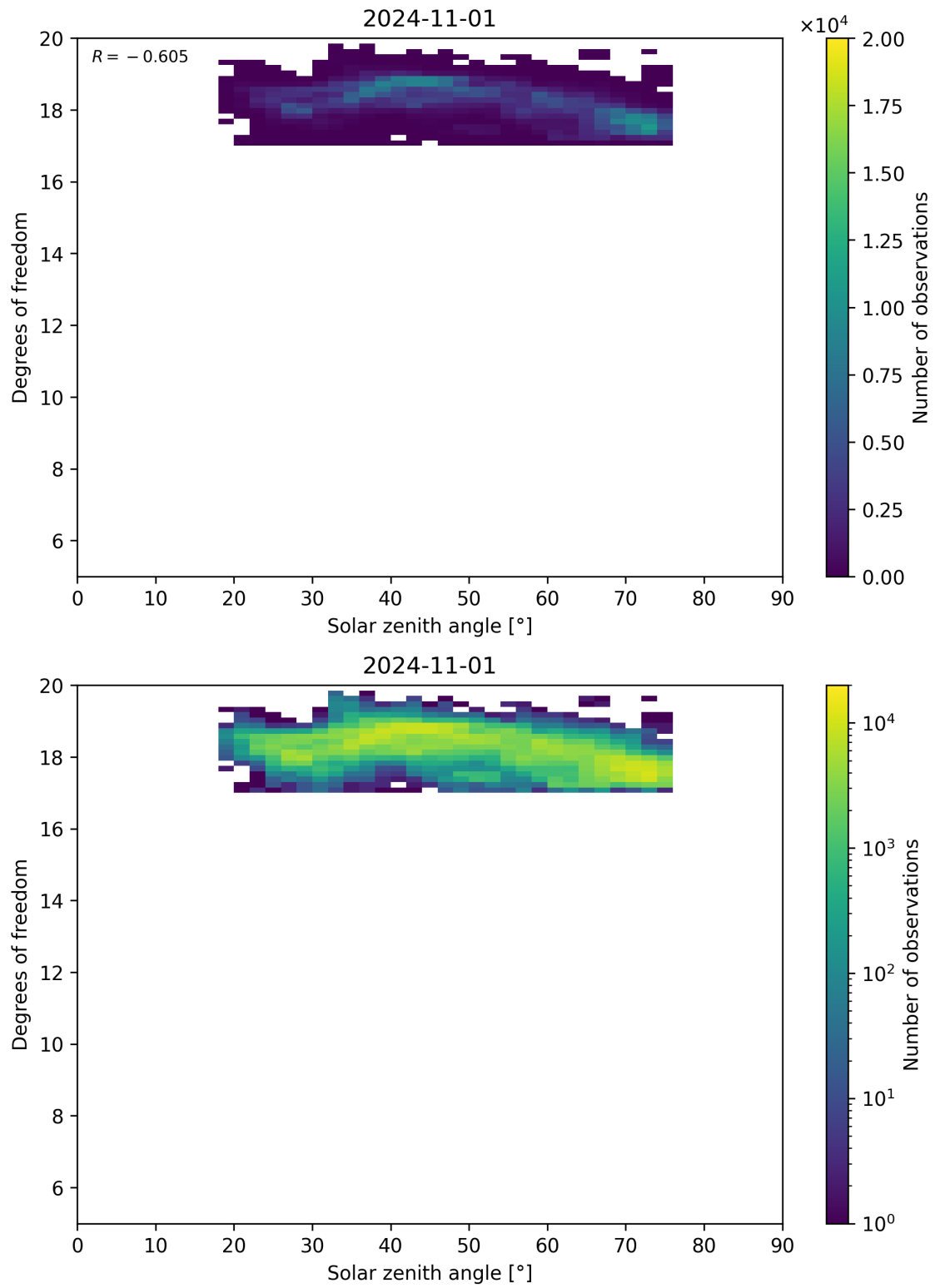
Figure 96: Scatter density plot of “Solar zenith angle” against “Degrees of freedom” for 2024-10-31 to 2024-11-02.
