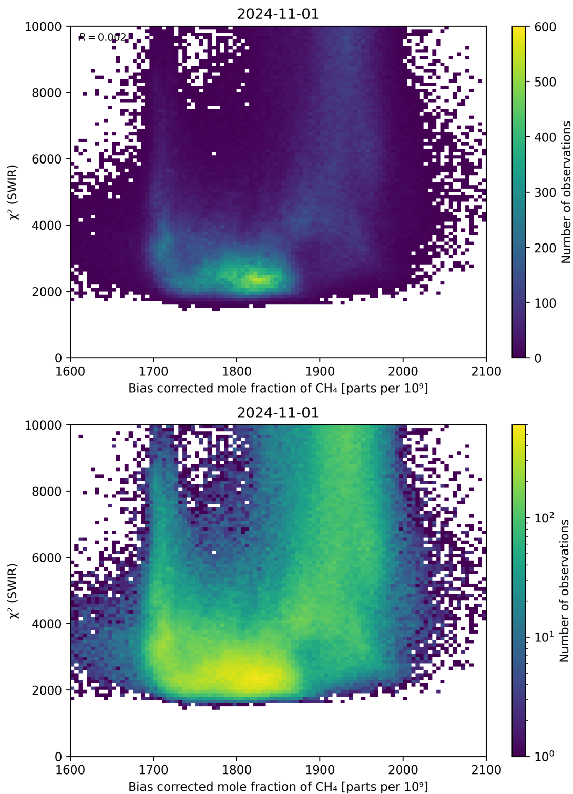
Figure 64: Scatter density plot of “Bias corrected mole fraction of \text{CH}_4 ” against “ \chi^2 (SWIR)” for 2024-10-31 to 2024-11-02.
