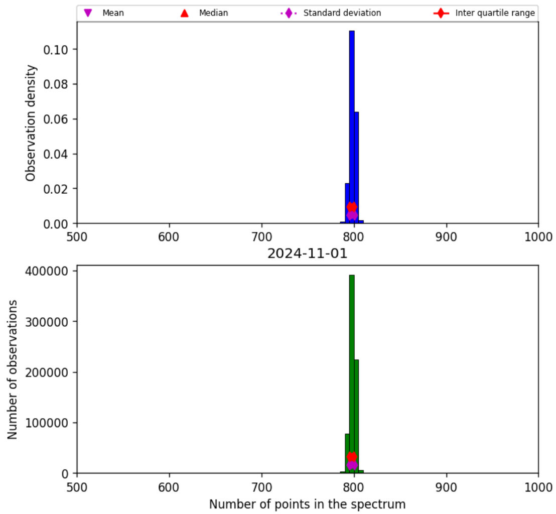
Figure 26: Histogram of “Number of points in the spectrum” for 2024-10-31 to 2024-11-02
