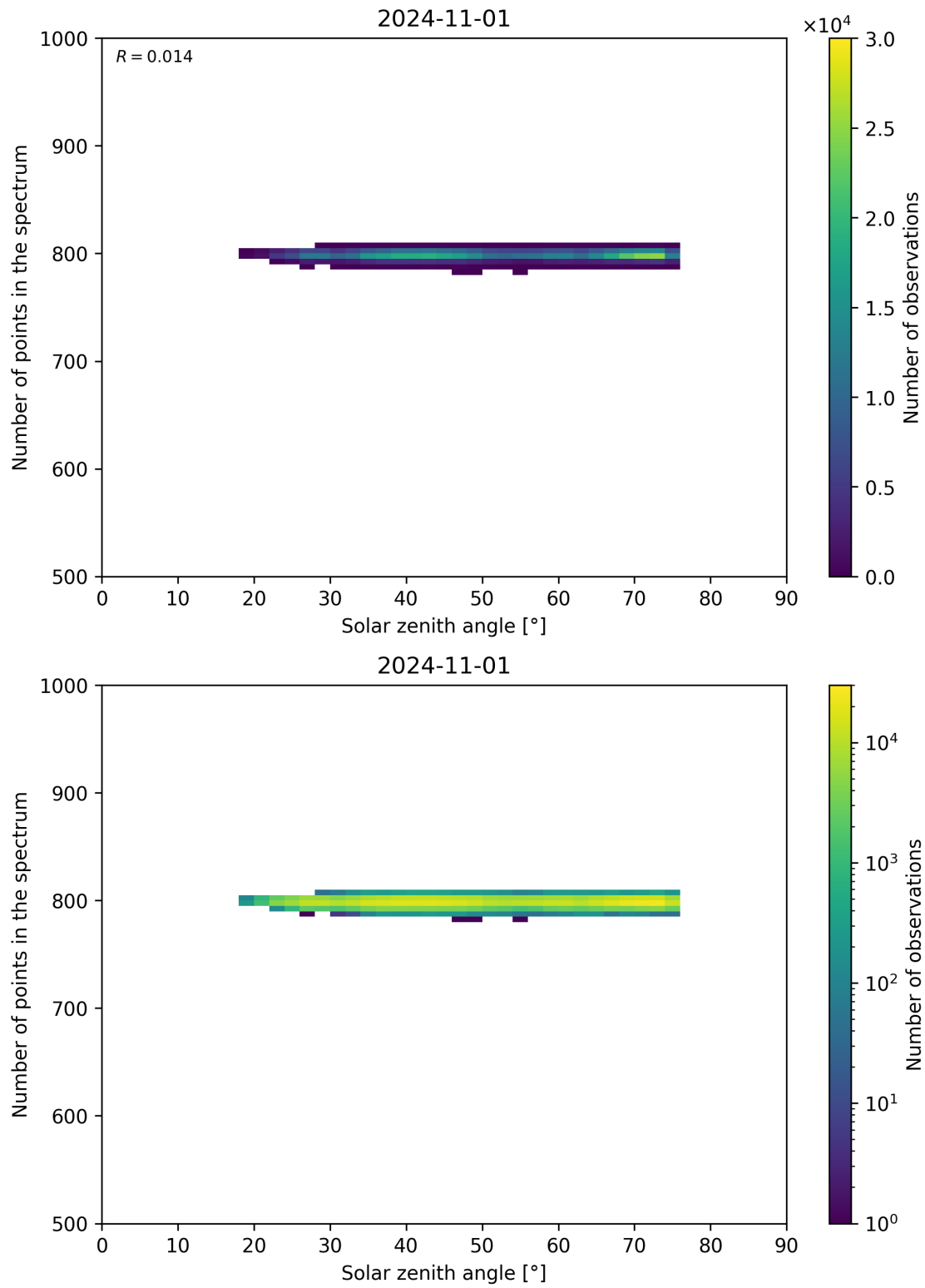
Figure 103: Scatter density plot of “Solar zenith angle” against “Number of points in the spectrum” for 2024-10-31 to 2024-11-02.
