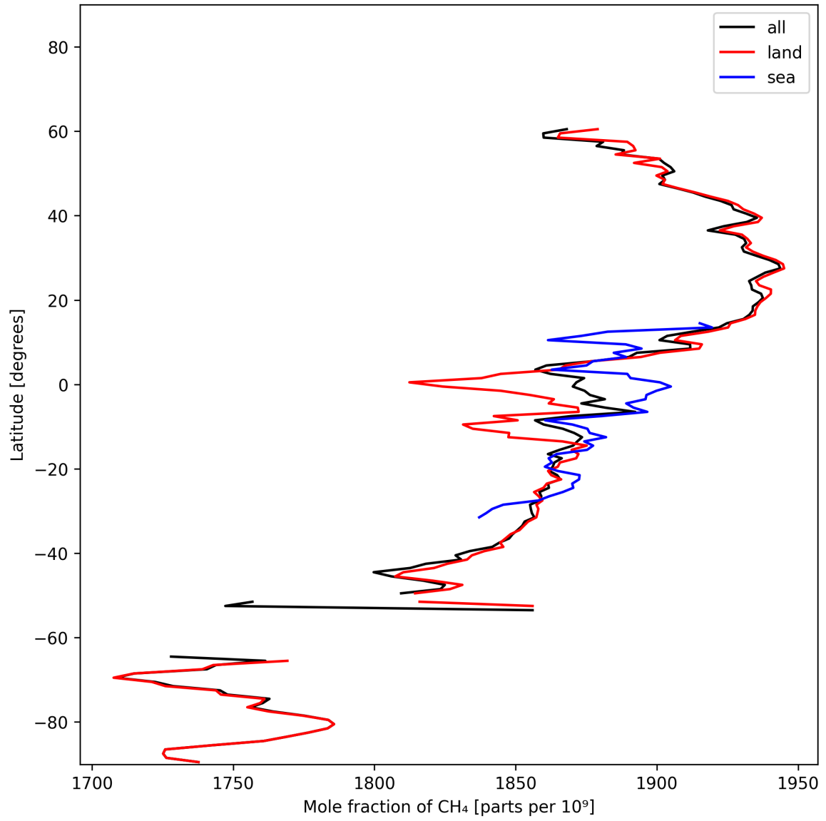
Figure 12: Zonal average of “Mole fraction of \text{CH}_4 ” for 2024-10-31 to 2024-11-02.
