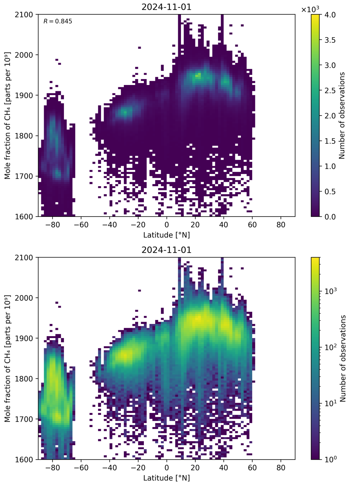
Figure 57: Scatter density plot of “Latitude” against “Mole fraction of CH 4 ” for 2024-10-31 to 2024-11-02.
