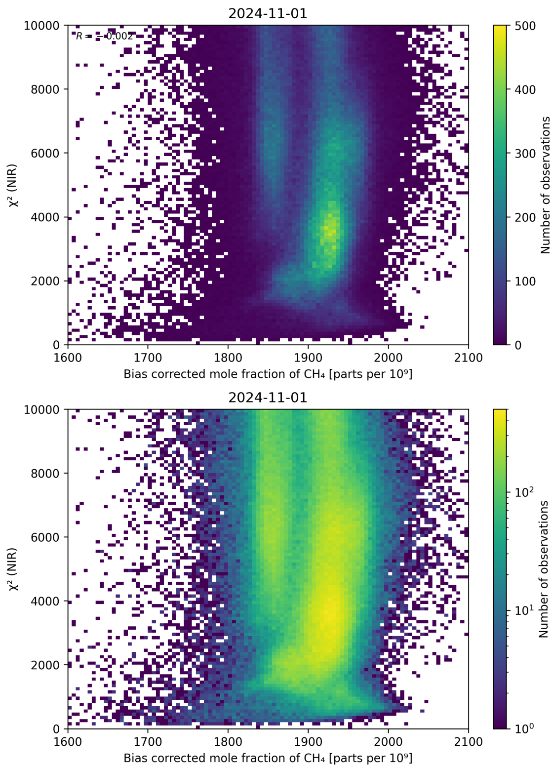
Figure 63: Scatter density plot of “Bias corrected mole fraction of CH 4 ” against “ \chi^2 (NIR)” for 2024-10-31 to 2024-11-02.
