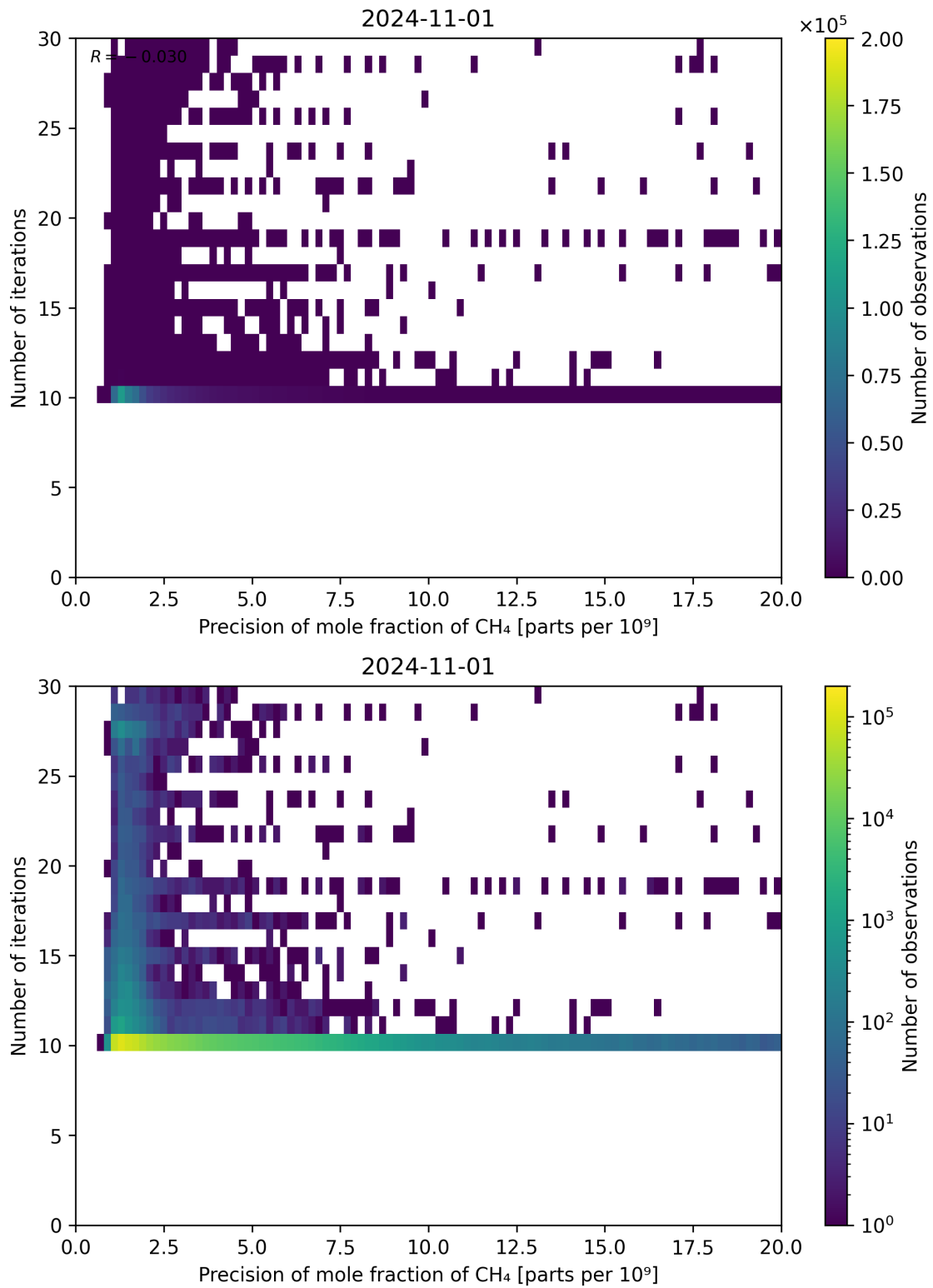
Figure 83: Scatter density plot of “Precision of mole fraction of CH 4 ” against “Number of iterations” for 2024-10-31 to 2024-11-02.
