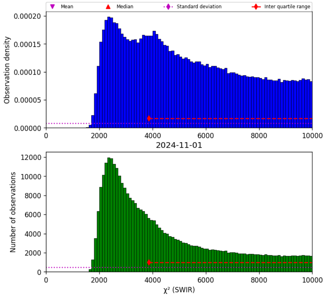
Figure 28: Histogram of " \chi^2 (SWIR)" for 2024-10-31 to 2024-11-02
