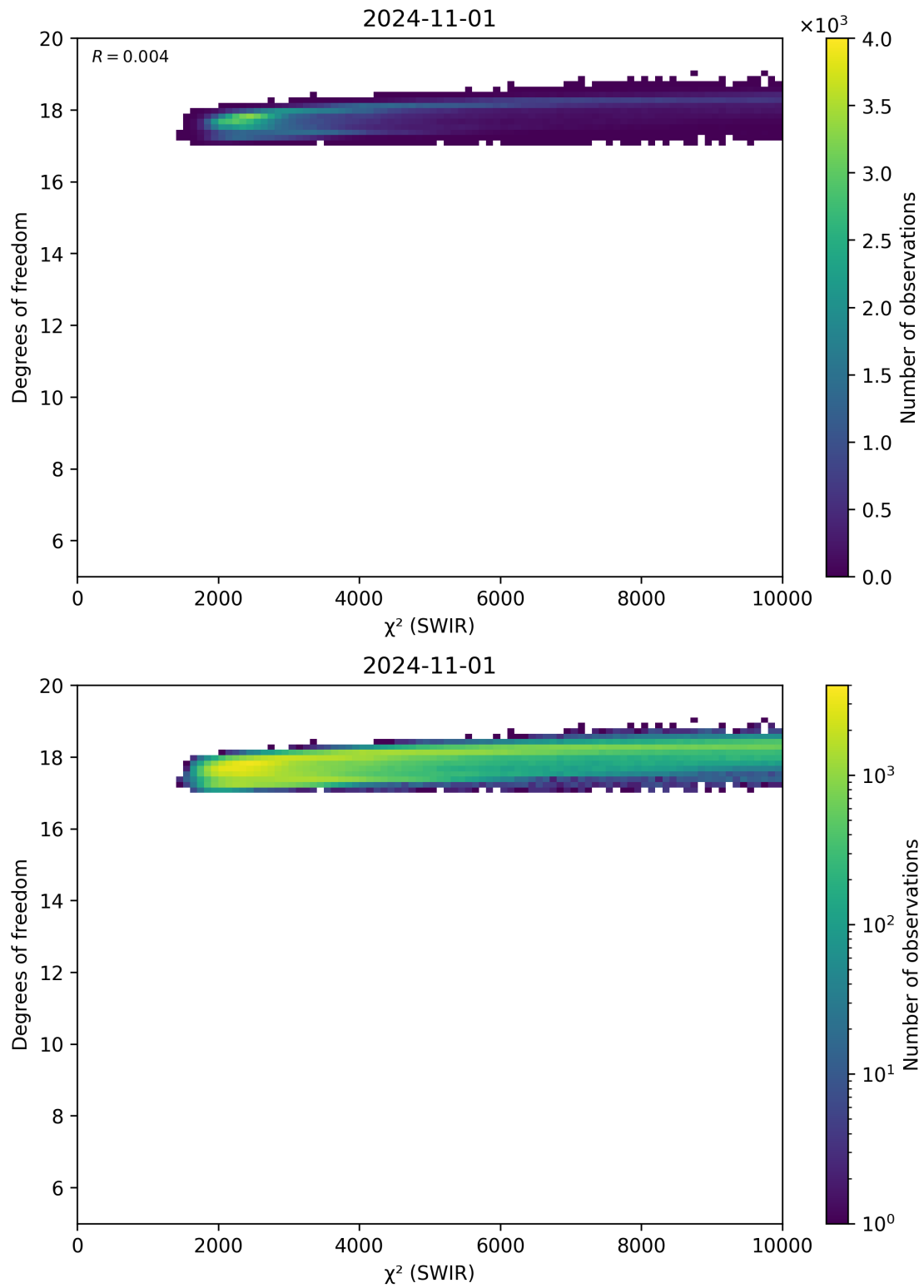
Figure 48: Scatter density plot of “ \chi^2 (SWIR)” against “Degrees of freedom” for 2024-10-31 to 2024-11-02.
