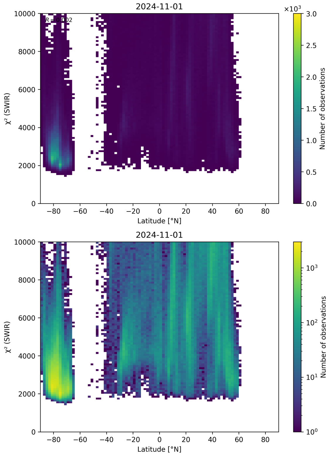
Figure 54: Scatter density plot of “Latitude” against “ \chi^2 (SWIR)” for 2024-10-31 to 2024-11-02.
