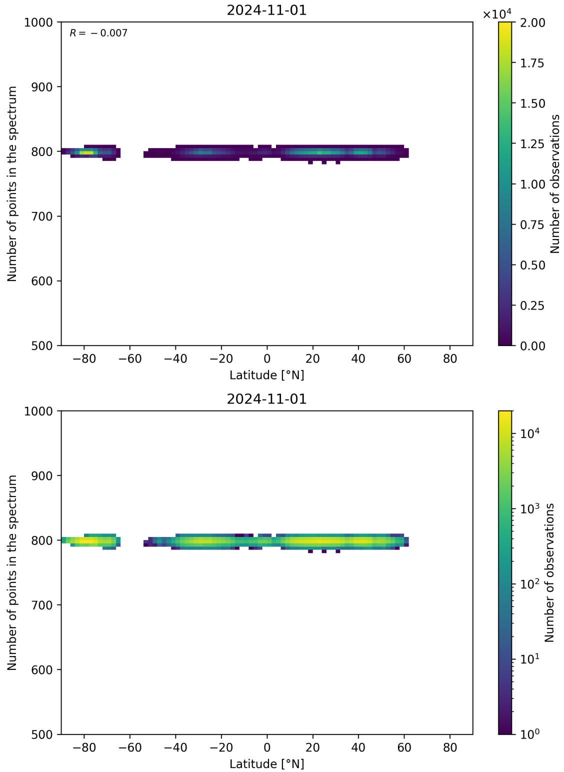
Figure 61: Scatter density plot of “Latitude” against “Number of points in the spectrum” for 2024-10-31 to 2024-11-02.
