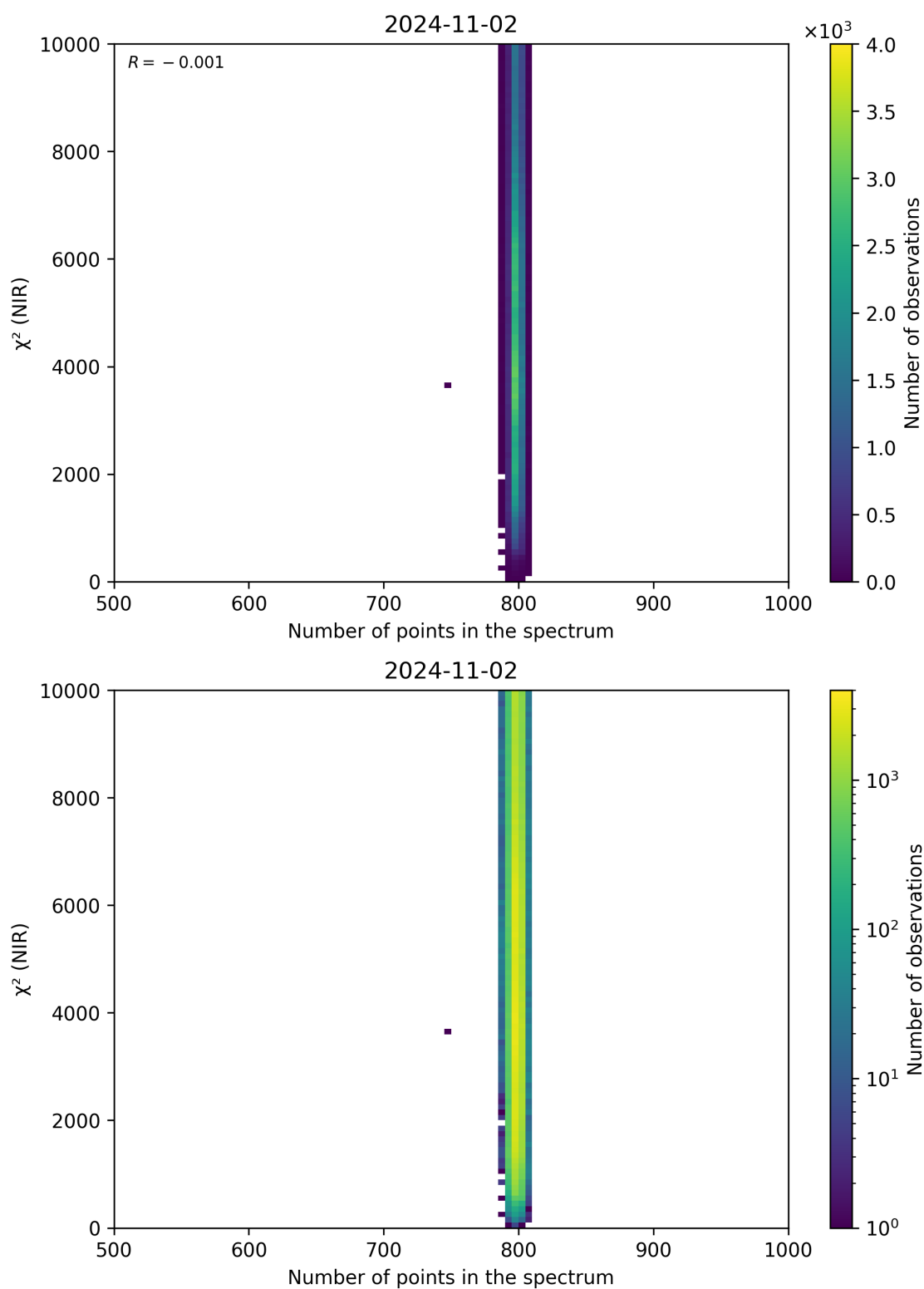
Figure 88: Scatter density plot of “Number of points in the spectrum” against “ \chi^2 (NIR)” for 2024-11-01 to 2024-11-03.
