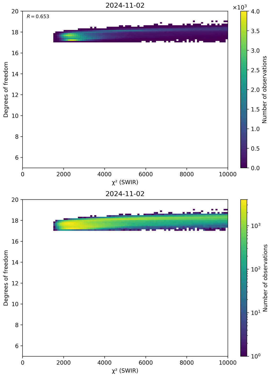
Figure 48: Scatter density plot of “ \chi^2 (SWIR)” against “Degrees of freedom” for 2024-11-01 to 2024-11-03.
