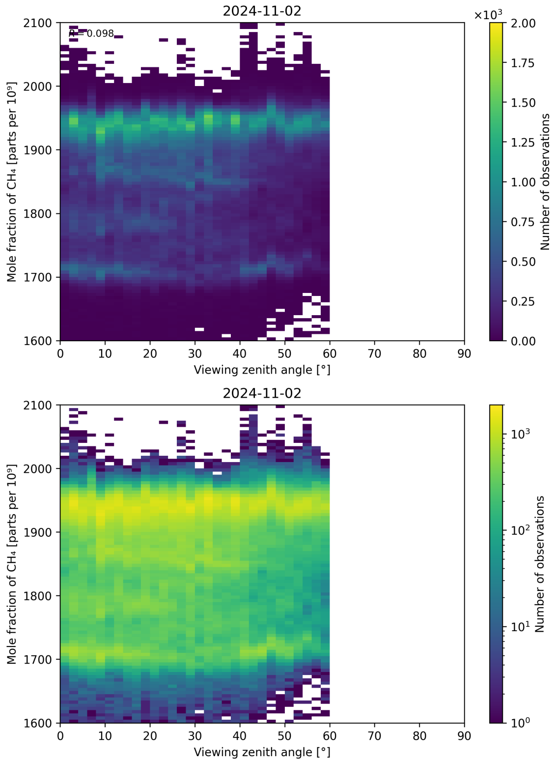
Figure 110: Scatter density plot of “Viewing zenith angle” against “Mole fraction of CH 4 ” for 2024-11-01 to 2024-11-03.
