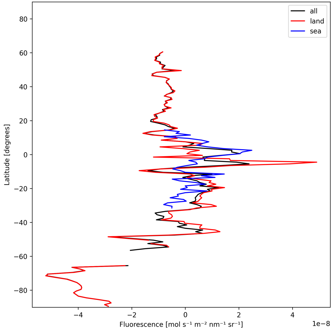
Figure 21: Zonal average of “Fluorescence” for 2024-11-01 to 2024-11-03.
