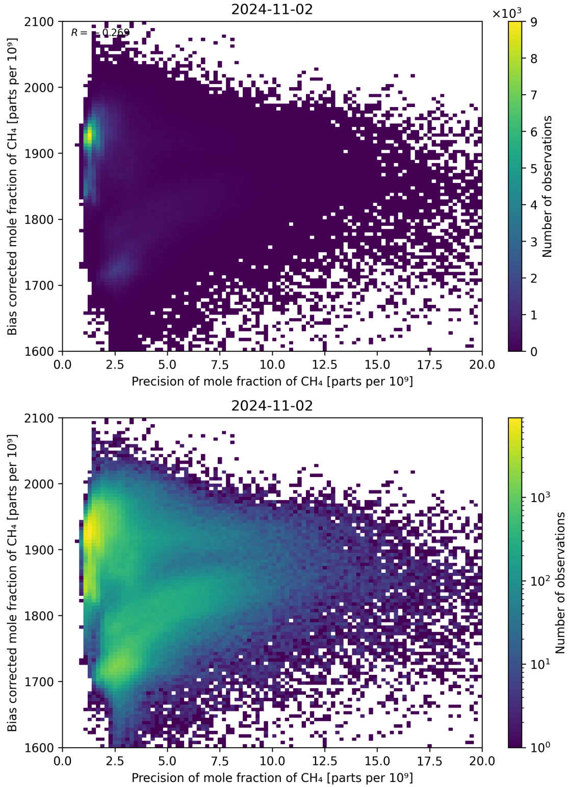
Figure 82: Scatter density plot of “Precision of mole fraction of CH 4 ” against “Bias corrected mole fraction of CH 4 ” for 2024-11-01 to 2024-11-03.
