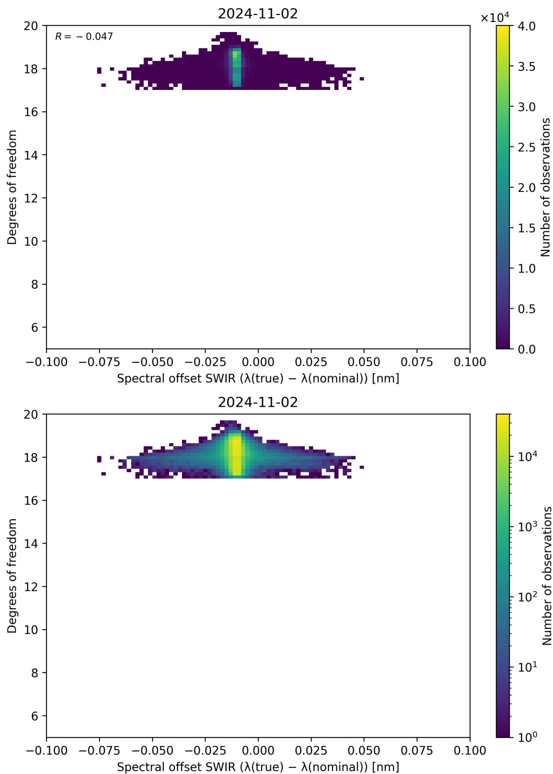
Figure 119: Scatter density plot of “Spectral offset SWIR ( \lambda_{\text{true}} - \lambda_{\text{nominal}} )” against “Degrees of freedom” for 2024-11-01 to 2024-11-03.
