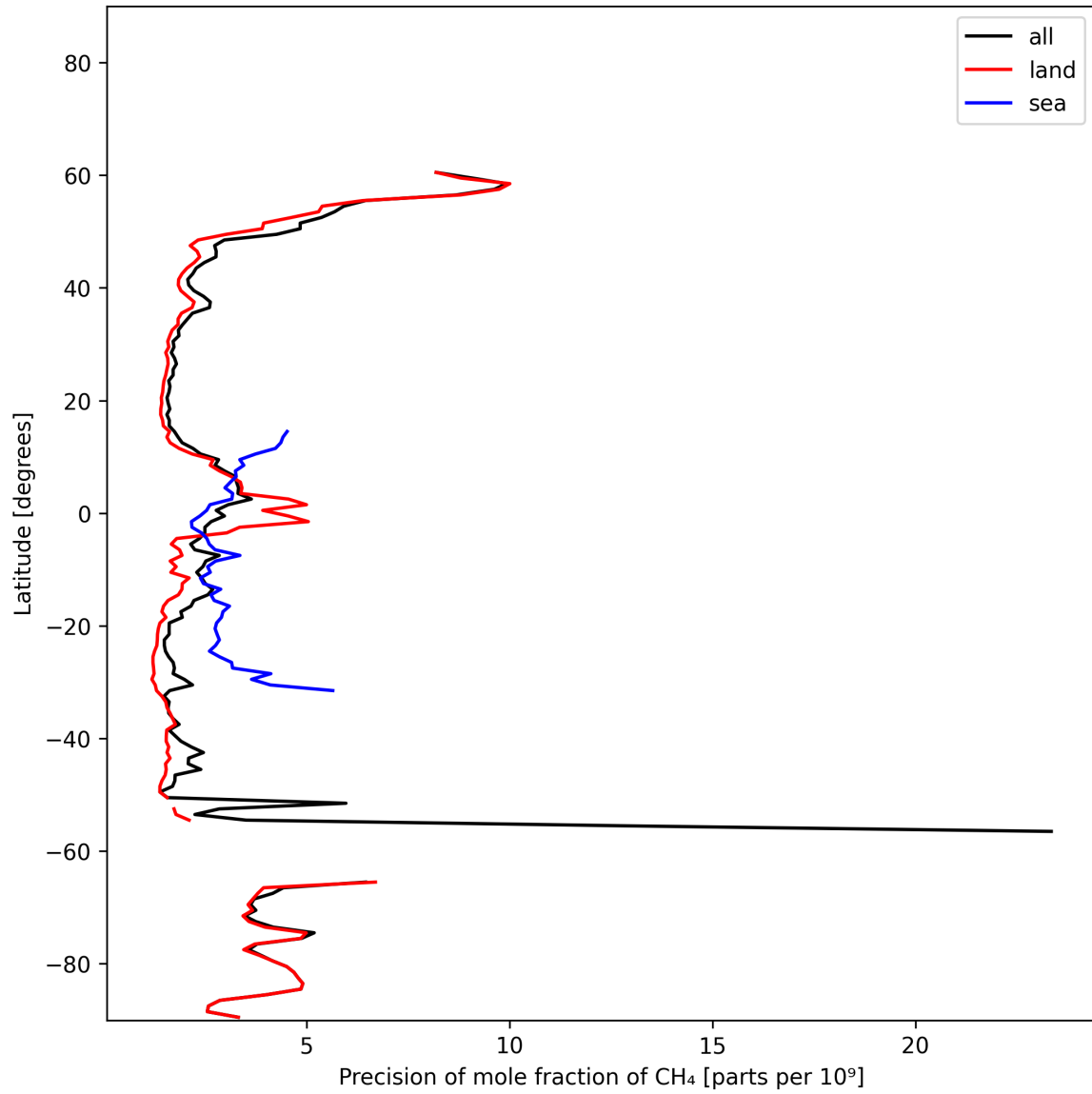
Figure 13: Zonal average of “Precision of mole fraction of CH 4 ” for 2024-11-01 to 2024-11-03.
