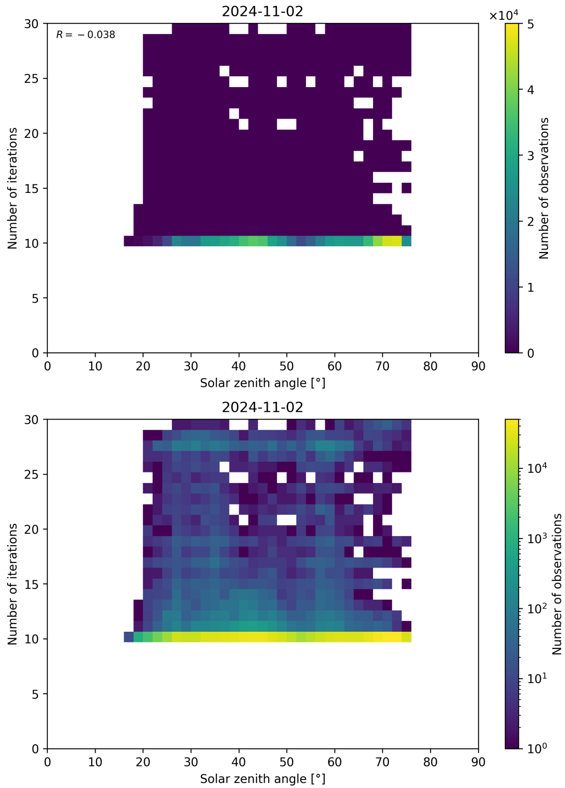
Figure 102: Scatter density plot of “Solar zenith angle” against “Number of iterations” for 2024-11-01 to 2024-11-03.
