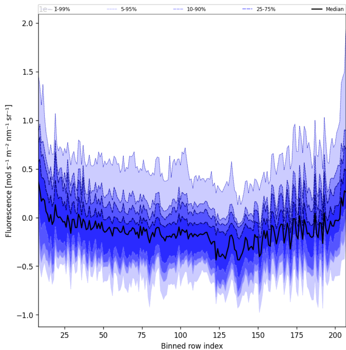
Figure 43: Along track statistics of “Fluorescence” for 2024-11-01 to 2024-11-03
