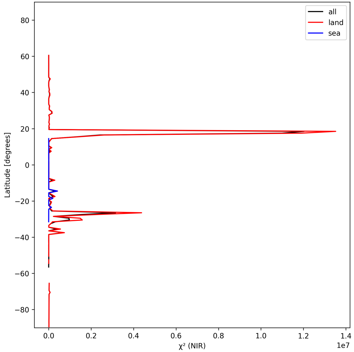
Figure 18: Zonal average of “ \chi^2 (NIR)” for 2024-11-01 to 2024-11-03.
