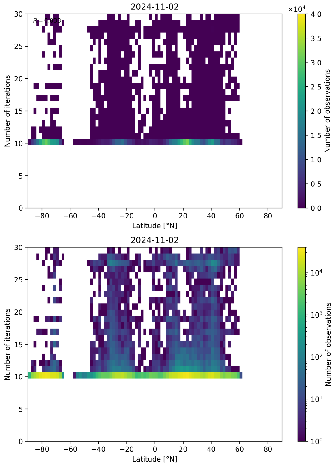
Figure 60: Scatter density plot of “Latitude” against “Number of iterations” for 2024-11-01 to 2024-11-03.
