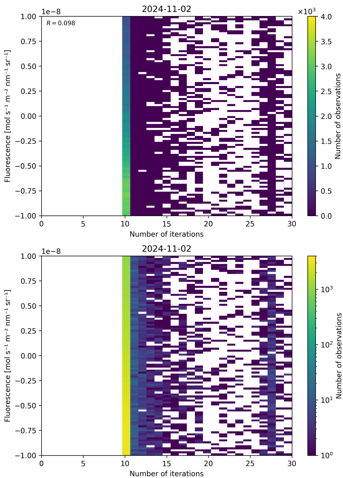
Figure 87: Scatter density plot of “Number of iterations” against “Fluorescence” for 2024-11-01 to 2024-11-03.
