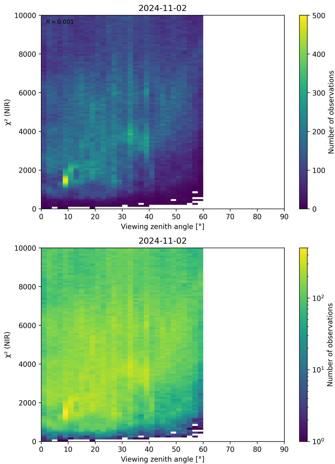
Figure 105: Scatter density plot of “Viewing zenith angle” against “ \chi^2 (NIR)” for 2024-11-01 to 2024-11-03.
