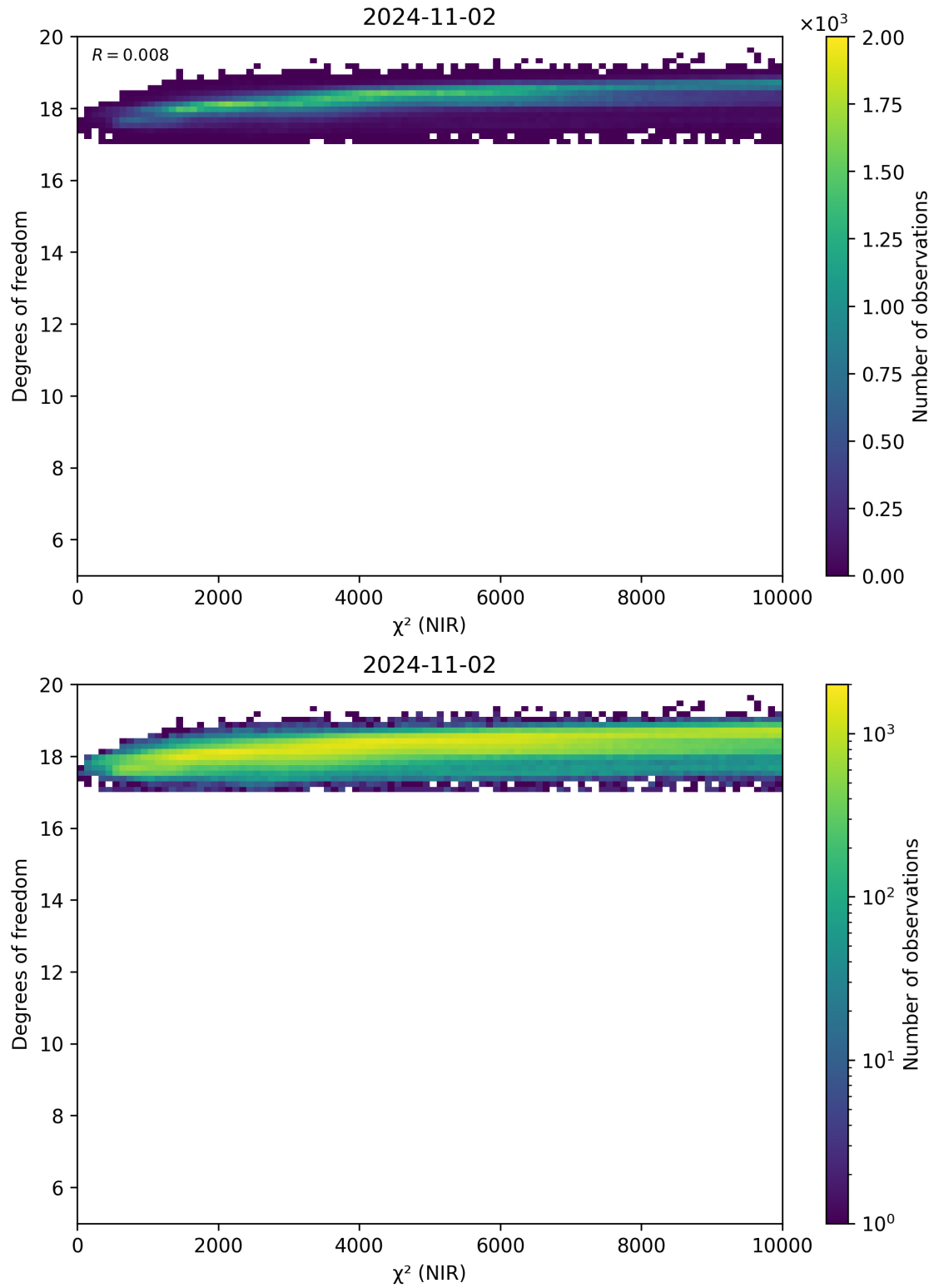
Figure 44: Scatter density plot of “ \chi^2 (NIR)” against “Degrees of freedom” for 2024-11-01 to 2024-11-03.
