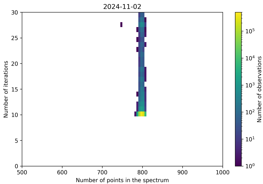
Figure 92: Scatter density plot of “Number of points in the spectrum” against “Number of iterations” for 2024-11-01 to 2024-11-03.
