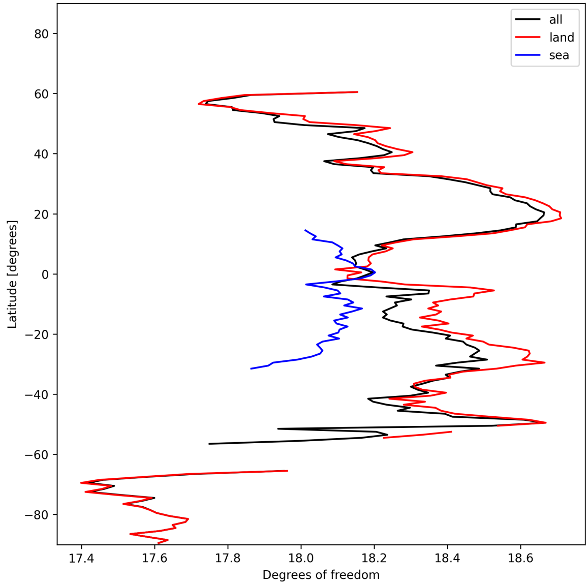
Figure 19: Zonal average of “Degrees of freedom” for 2024-11-01 to 2024-11-03.
