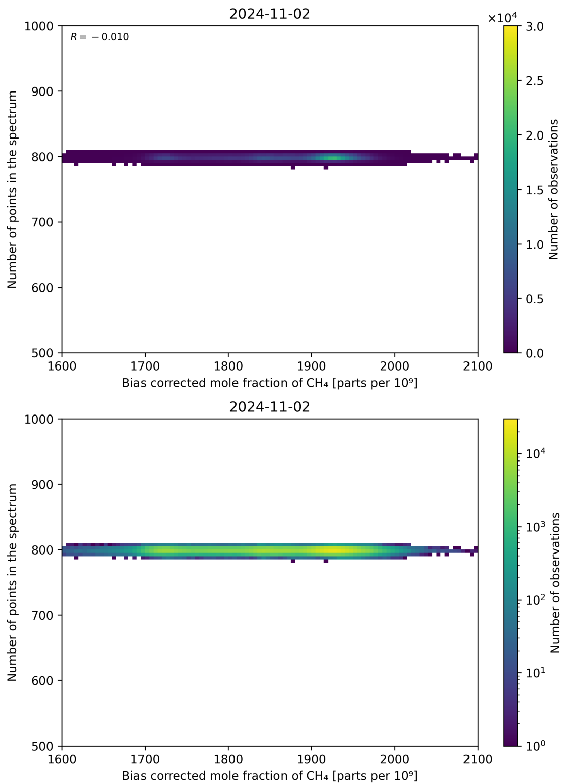
Figure 68: Scatter density plot of “Bias corrected mole fraction of CH 4 ” against “Number of points in the spectrum” for 2024-11-01 to 2024-11-03.
