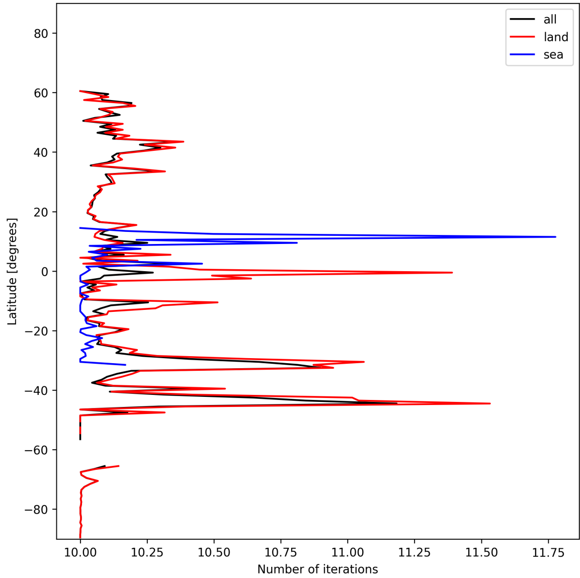
Figure 20: Zonal average of “Number of iterations” for 2024-11-01 to 2024-11-03.
