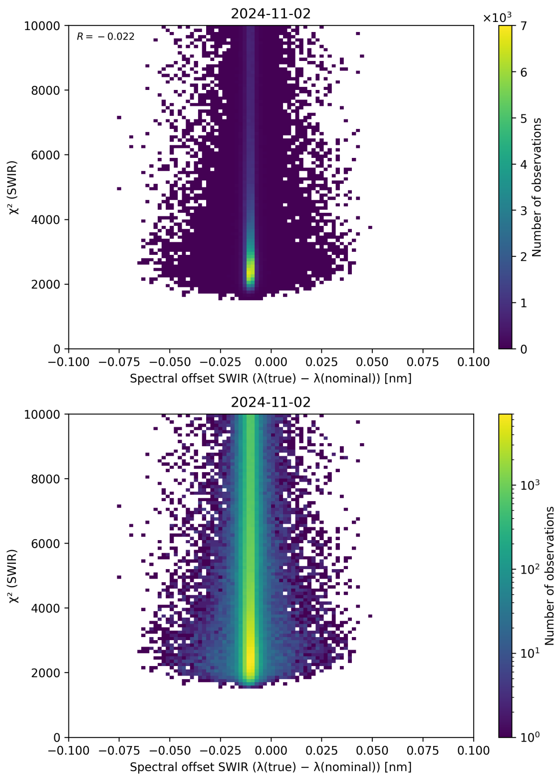
Figure 118: Scatter density plot of “Spectral offset SWIR ( \lambda_{\text{true}} - \lambda_{\text{nominal}} )” against “ \chi^2 (SWIR)” for 2024-11-01 to 2024-11-03.
