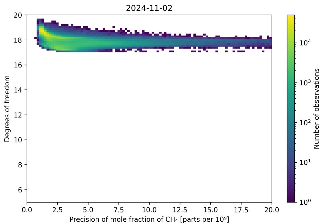
Figure 80: Scatter density plot of “Precision of mole fraction of CH 4 ” against “Degrees of freedom” for 2024-11-01 to 2024-11-03.
