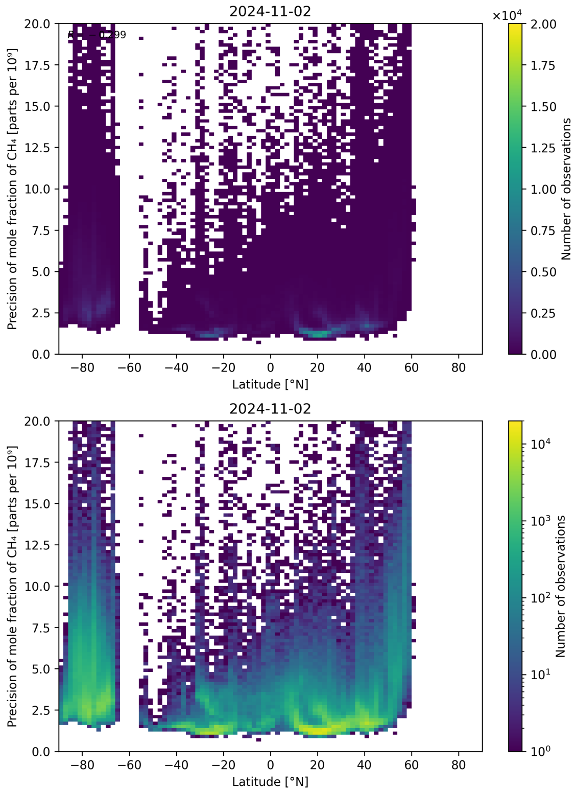
Figure 59: Scatter density plot of “Latitude” against “Precision of mole fraction of CH 4 ” for 2024-11-01 to 2024-11-03.
