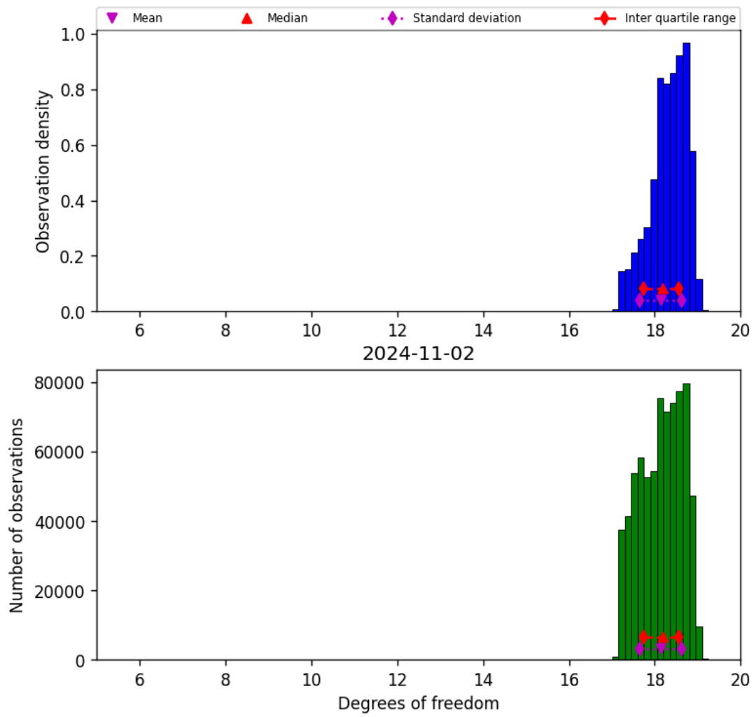
Figure 30: Histogram of “Degrees of freedom” for 2024-11-01 to 2024-11-03
