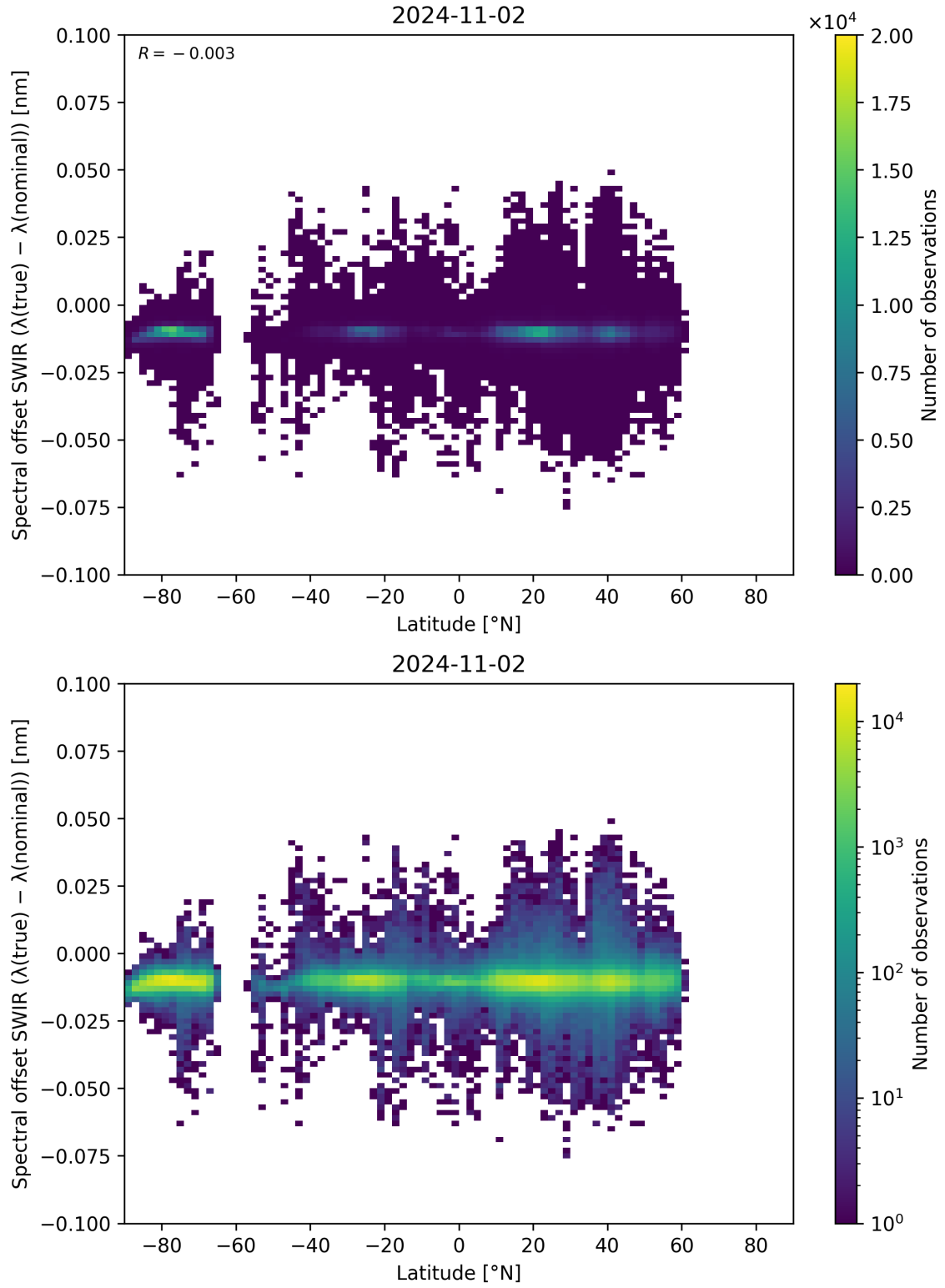
Figure 62: Scatter density plot of “Latitude” against “Spectral offset SWIR ( \lambda_{\text{true}} - \lambda_{\text{nominal}} )” for 2024-11-01 to 2024-11-03.
