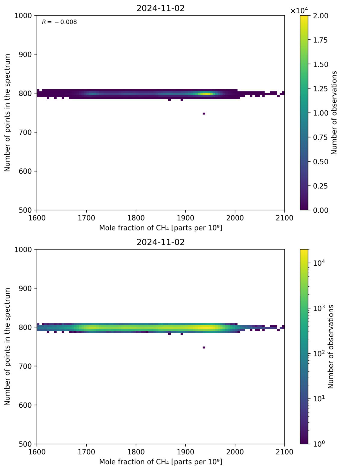
Figure 77: Scatter density plot of “Mole fraction of CH 4 ” against “Number of points in the spectrum” for 2024-11-01 to 2024-11-03.
