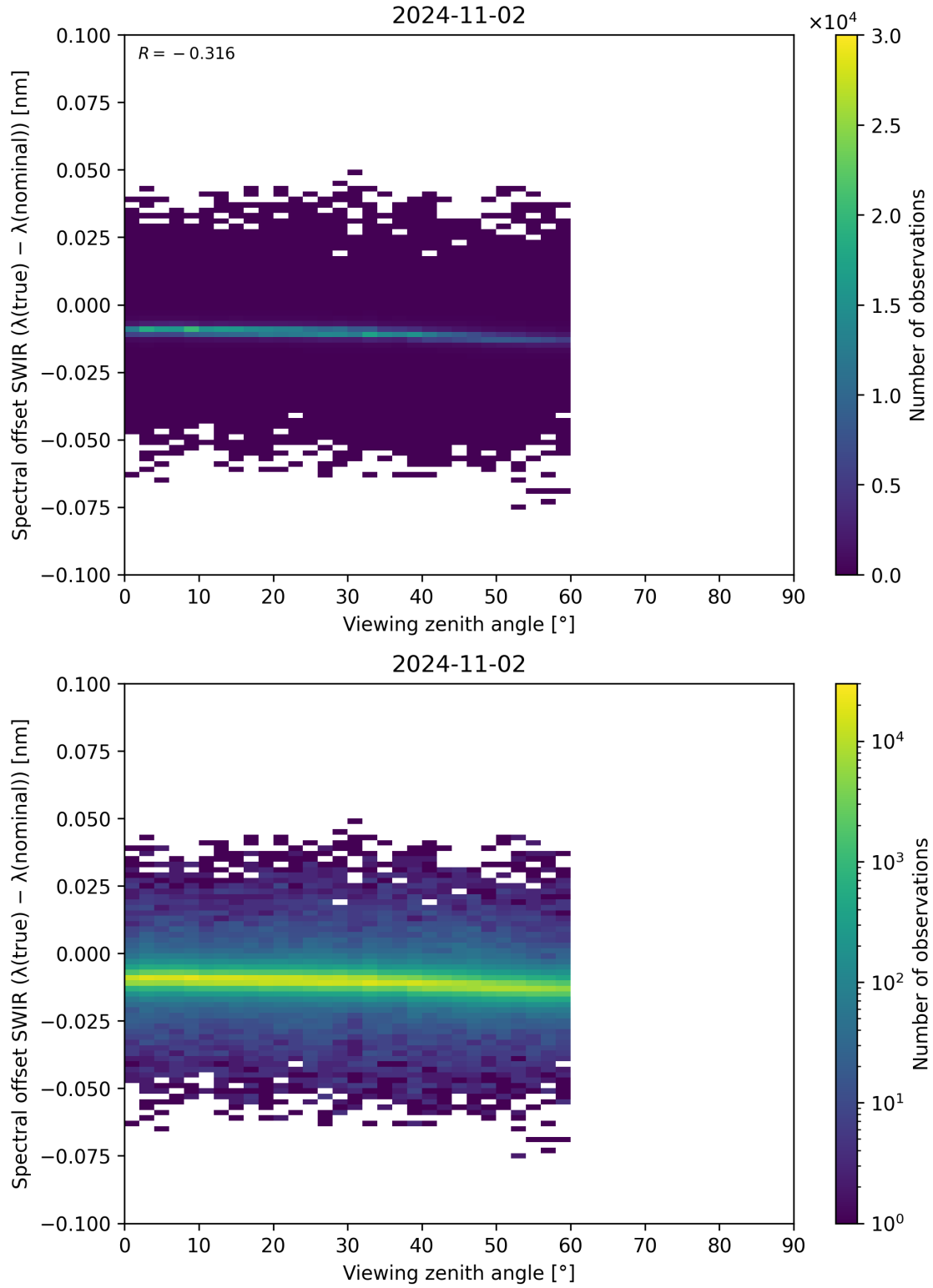
Figure 116: Scatter density plot of “Viewing zenith angle” against “Spectral offset SWIR ( \lambda_{\text{true}} - \lambda_{\text{nominal}} )” for 2024-11-01 to 2024-11-03.
