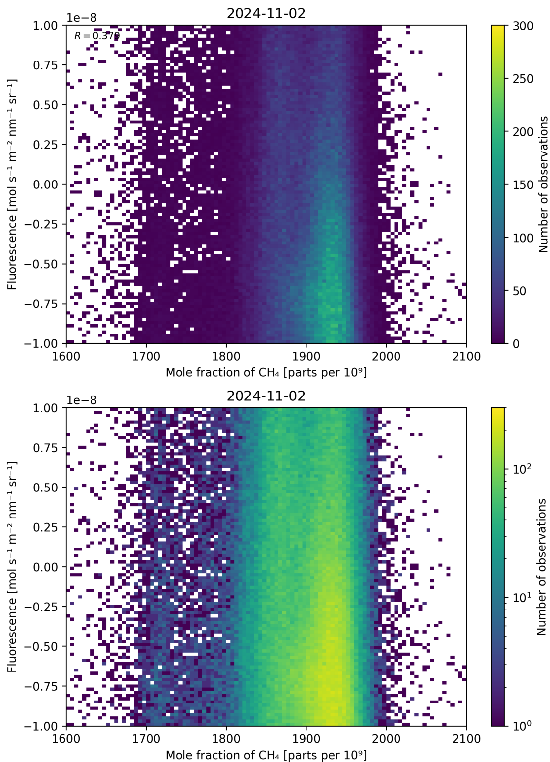
Figure 73: Scatter density plot of “Mole fraction of \text{CH}_4 ” against “Fluorescence” for 2024-11-01 to 2024-11-03.
