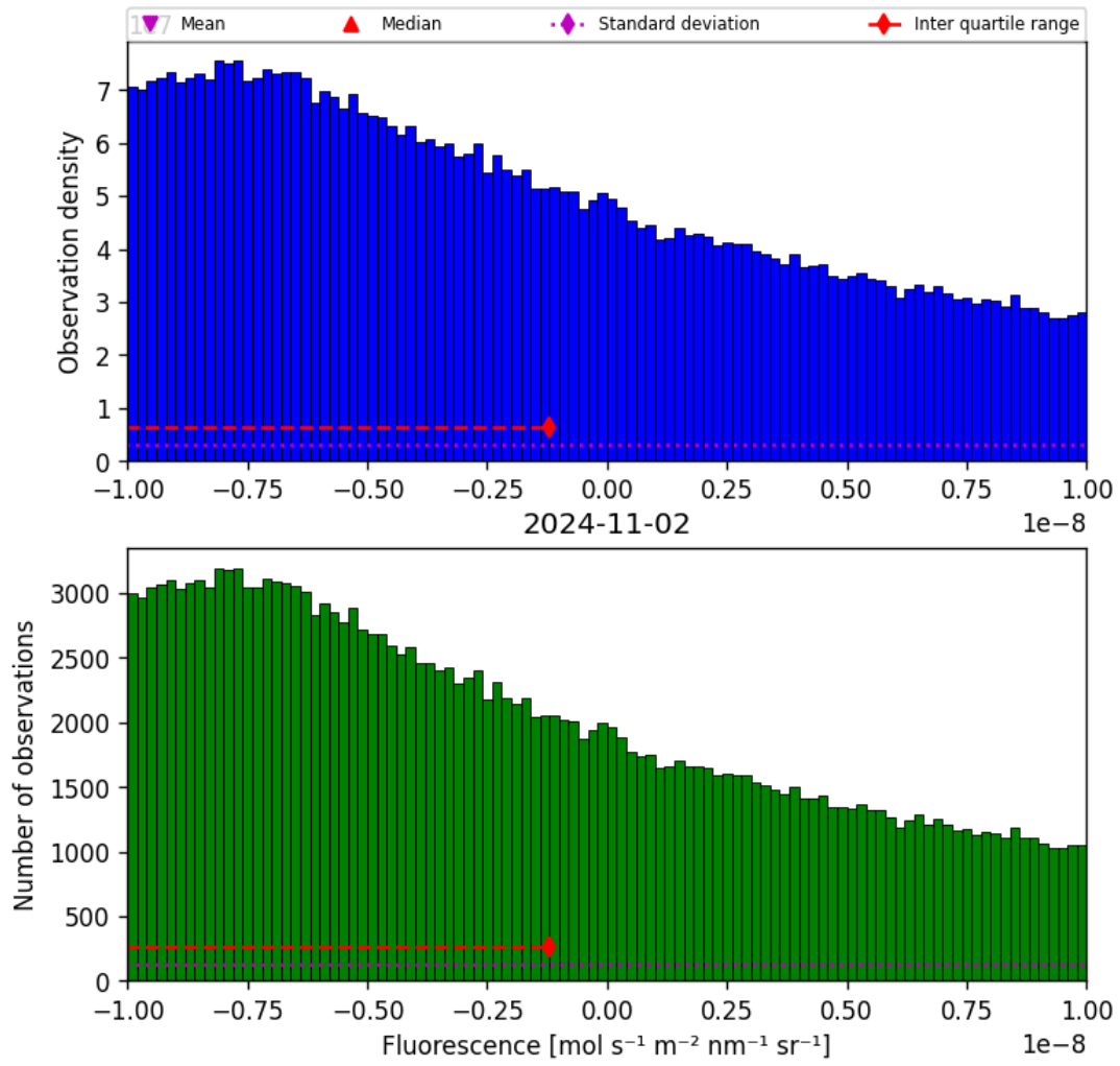
Figure 32: Histogram of “Fluorescence” for 2024-11-01 to 2024-11-03
