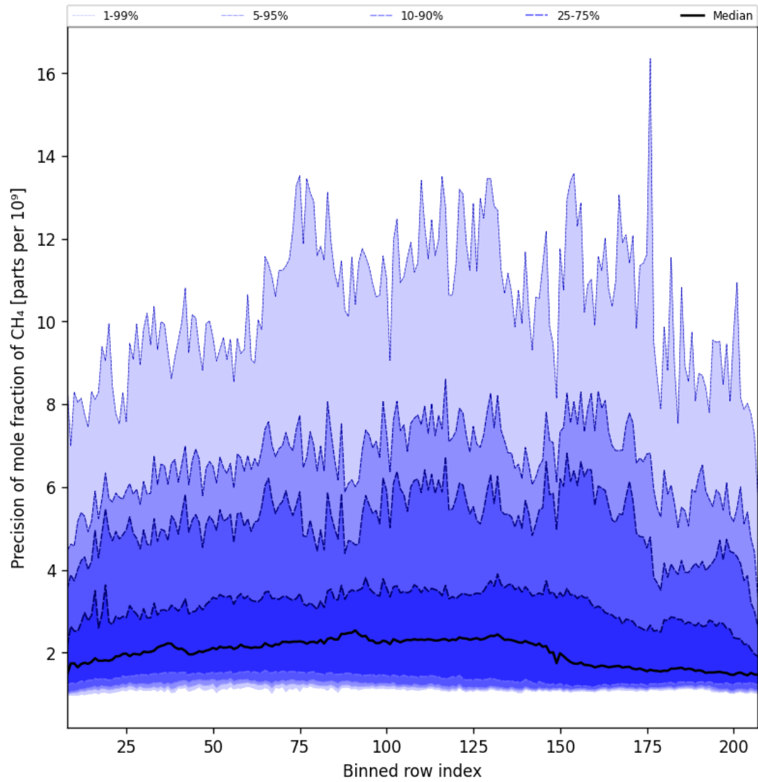
Figure 35: Along track statistics of “Precision of mole fraction of CH 4 ” for 2024-11-01 to 2024-11-03
