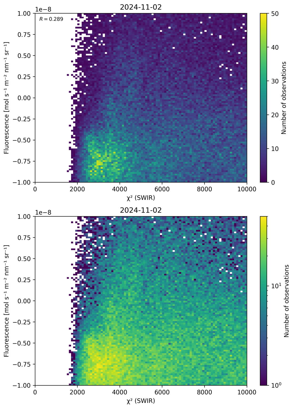
Figure 49: Scatter density plot of “ \chi^2 (SWIR)” against “Fluorescence” for 2024-11-01 to 2024-11-03.
