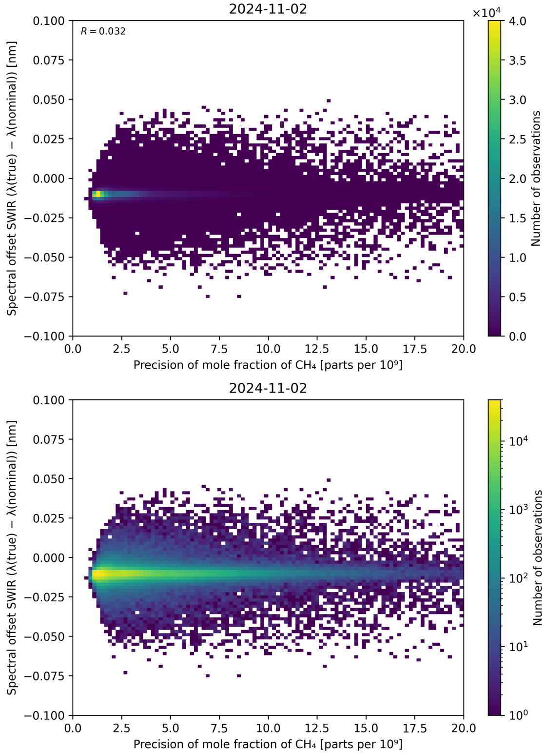
Figure 85: Scatter density plot of “Precision of mole fraction of CH 4 ” against “Spectral offset SWIR ( \lambda_{\text{true}} - \lambda_{\text{nominal}} )” for 2024-11-01 to 2024-11-03.
