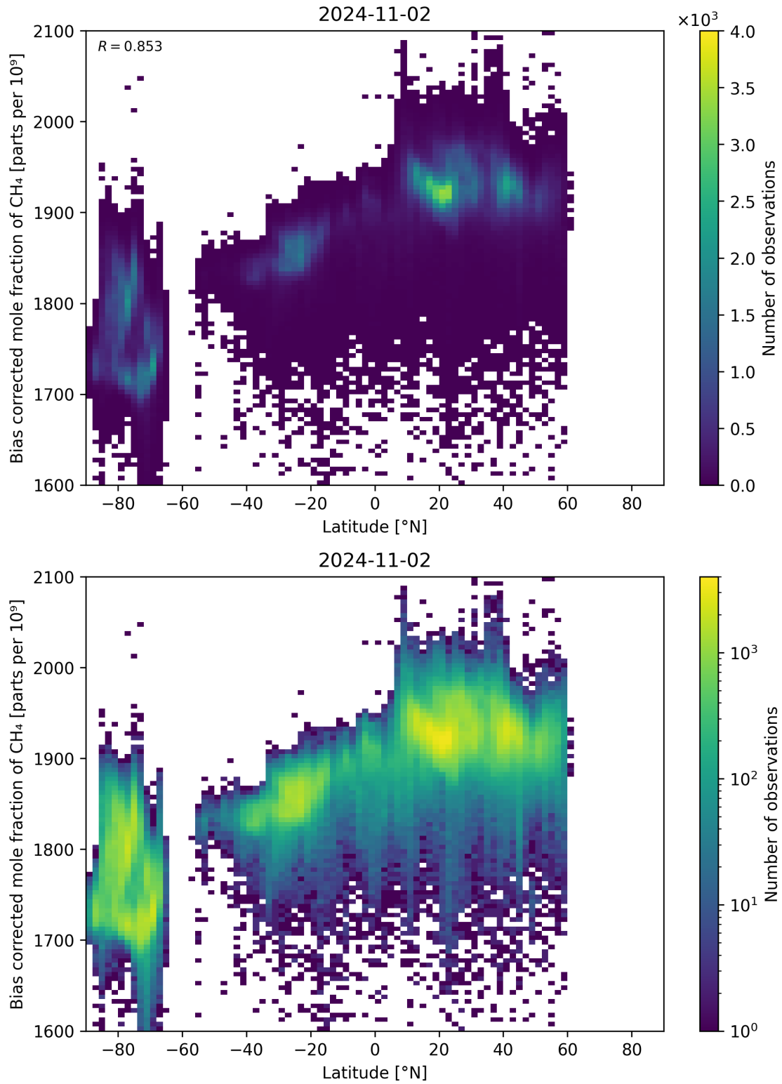
Figure 58: Scatter density plot of “Latitude” against “Bias corrected mole fraction of CH 4 ” for 2024-11-01 to 2024-11-03.
