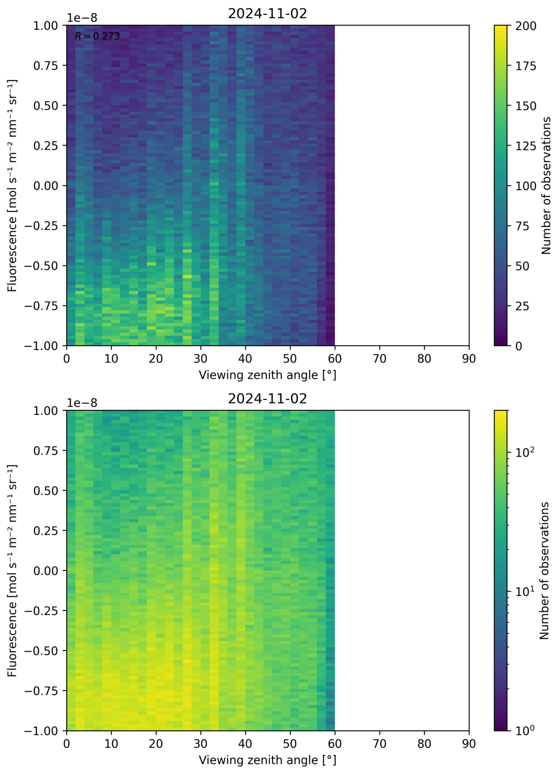
Figure 108: Scatter density plot of “Viewing zenith angle” against “Fluorescence” for 2024-11-01 to 2024-11-03.
