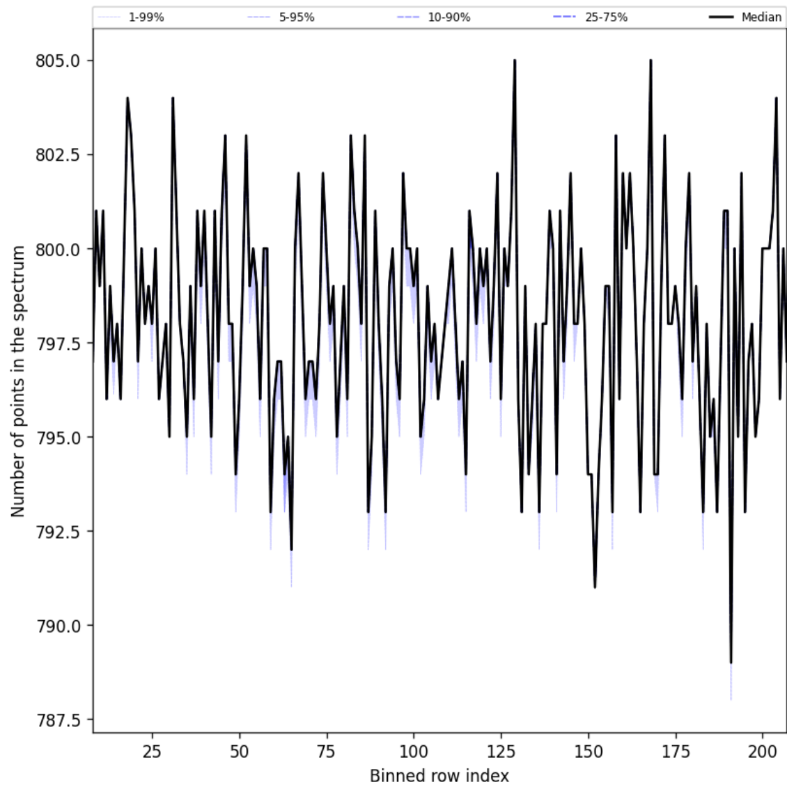
Figure 37: Along track statistics of “Number of points in the spectrum” for 2024-11-01 to 2024-11-03
