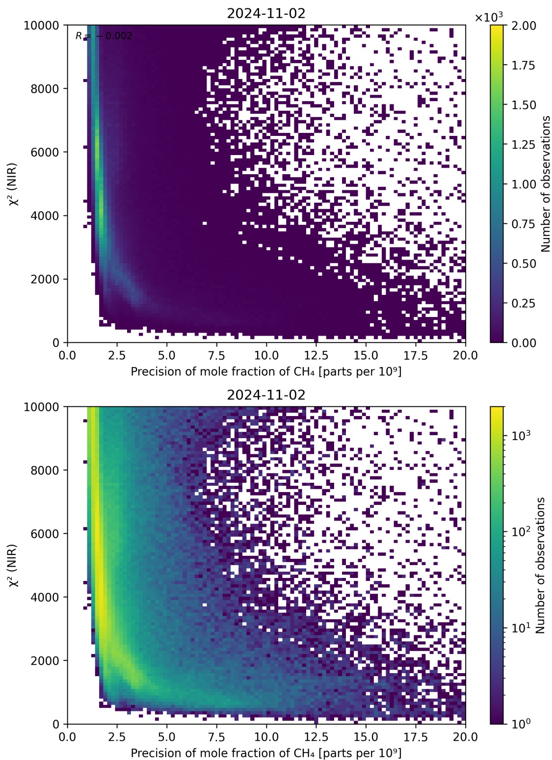
Figure 78: Scatter density plot of “Precision of mole fraction of CH 4 ” against “ \chi^2 (NIR)” for 2024-11-01 to 2024-11-03.
