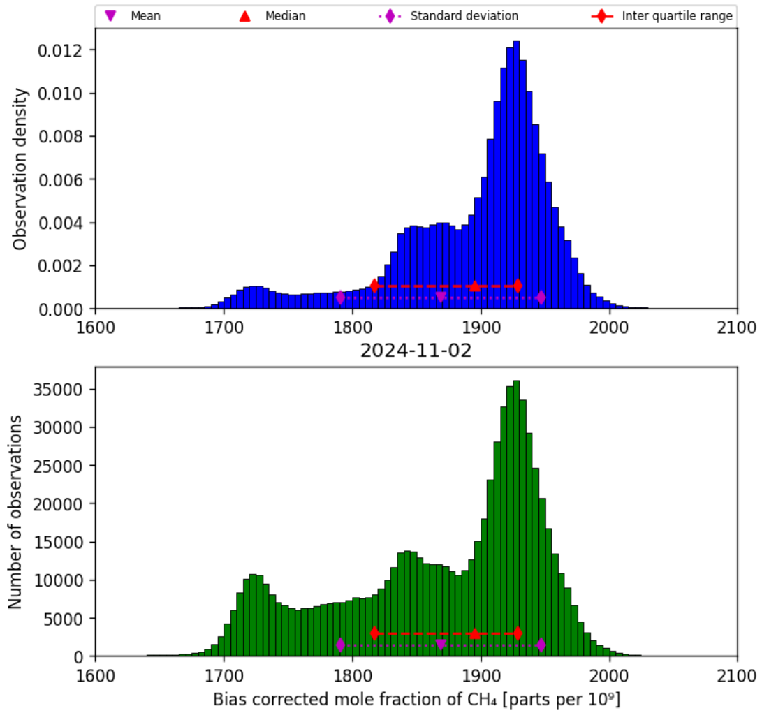
Figure 25: Histogram of “Bias corrected mole fraction of CH 4 ” for 2024-11-01 to 2024-11-03
