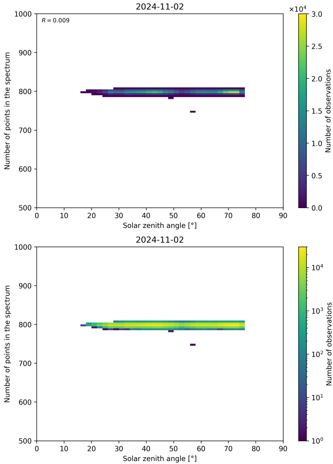
Figure 103: Scatter density plot of “Solar zenith angle” against “Number of points in the spectrum” for 2024-11-01 to 2024-11-03.
