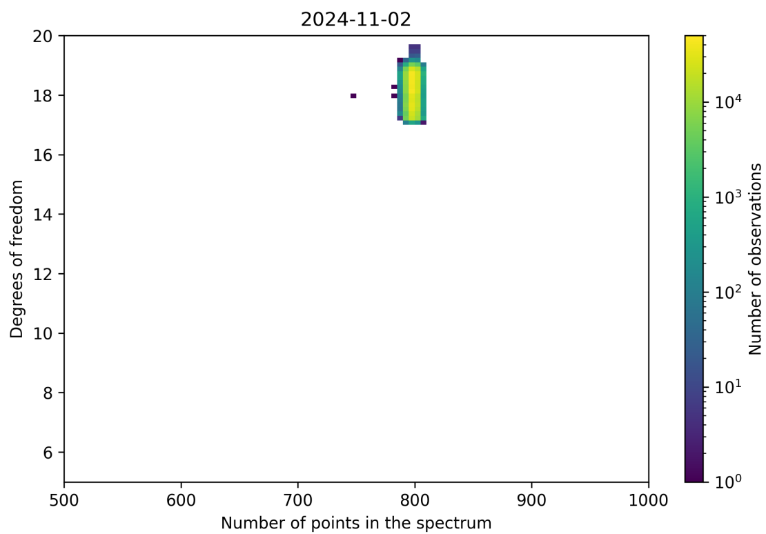
Figure 90: Scatter density plot of “Number of points in the spectrum” against “Degrees of freedom” for 2024-11-01 to 2024-11-03.
