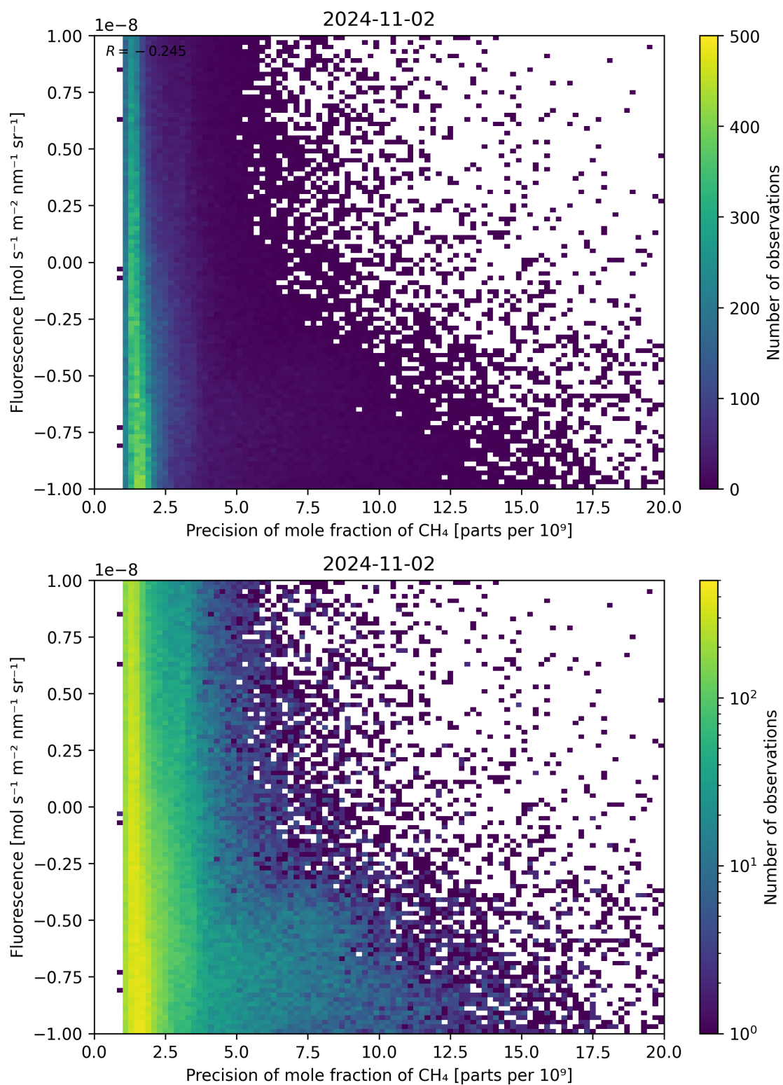
Figure 81: Scatter density plot of “Precision of mole fraction of \text{CH}_4 ” against “Fluorescence” for 2024-11-01 to 2024-11-03.
