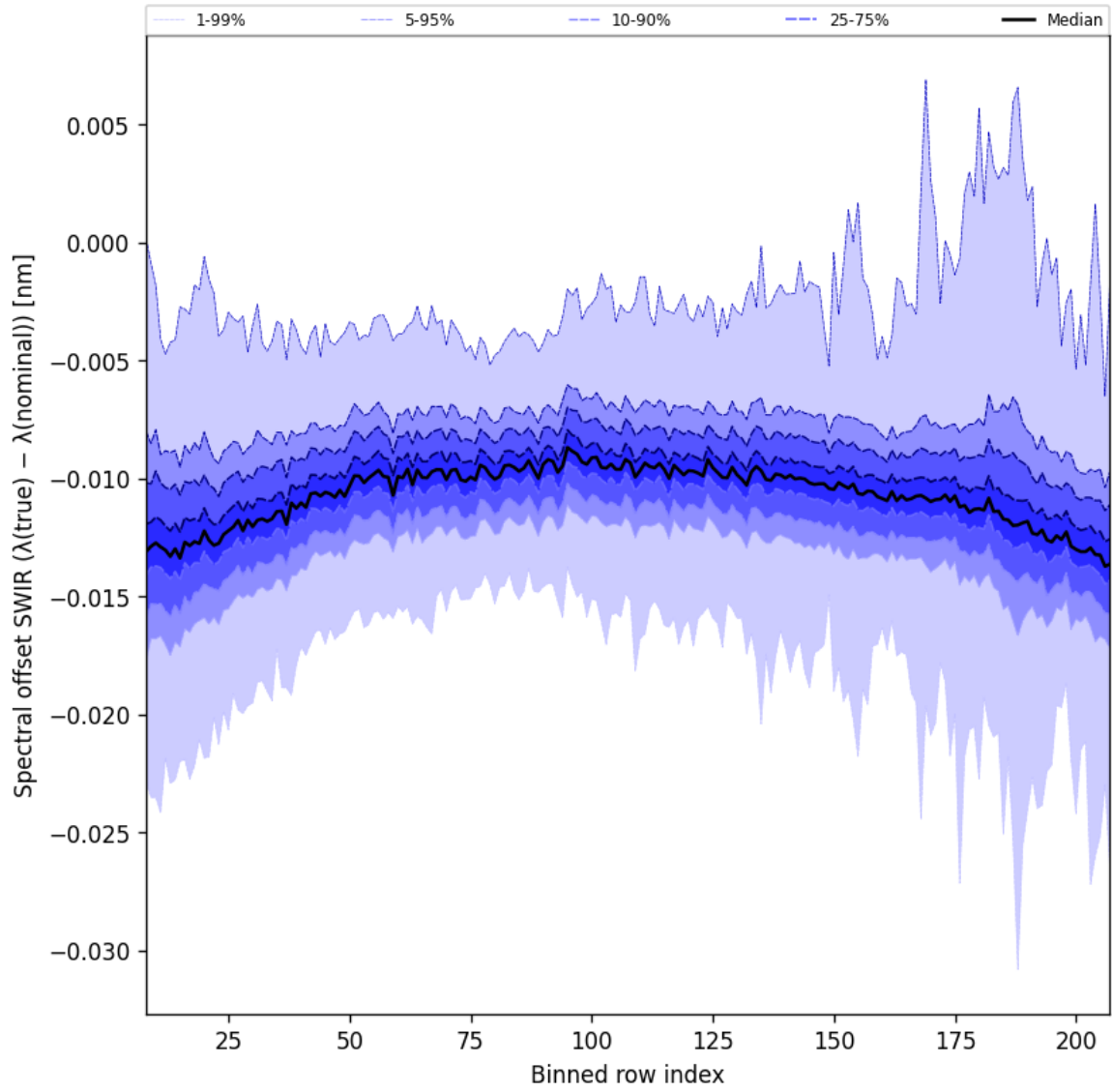
Figure 38: Along track statistics of “Spectral offset SWIR ( \lambda_{\text{true}} - \lambda_{\text{nominal}} )” for 2024-11-01 to 2024-11-03
