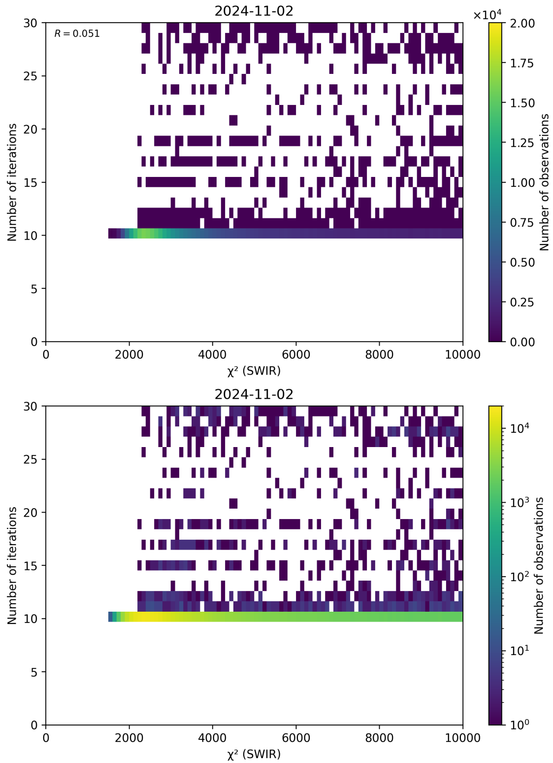
Figure 50: Scatter density plot of “ \chi^2 (SWIR)” against “Number of iterations” for 2024-11-01 to 2024-11-03.
