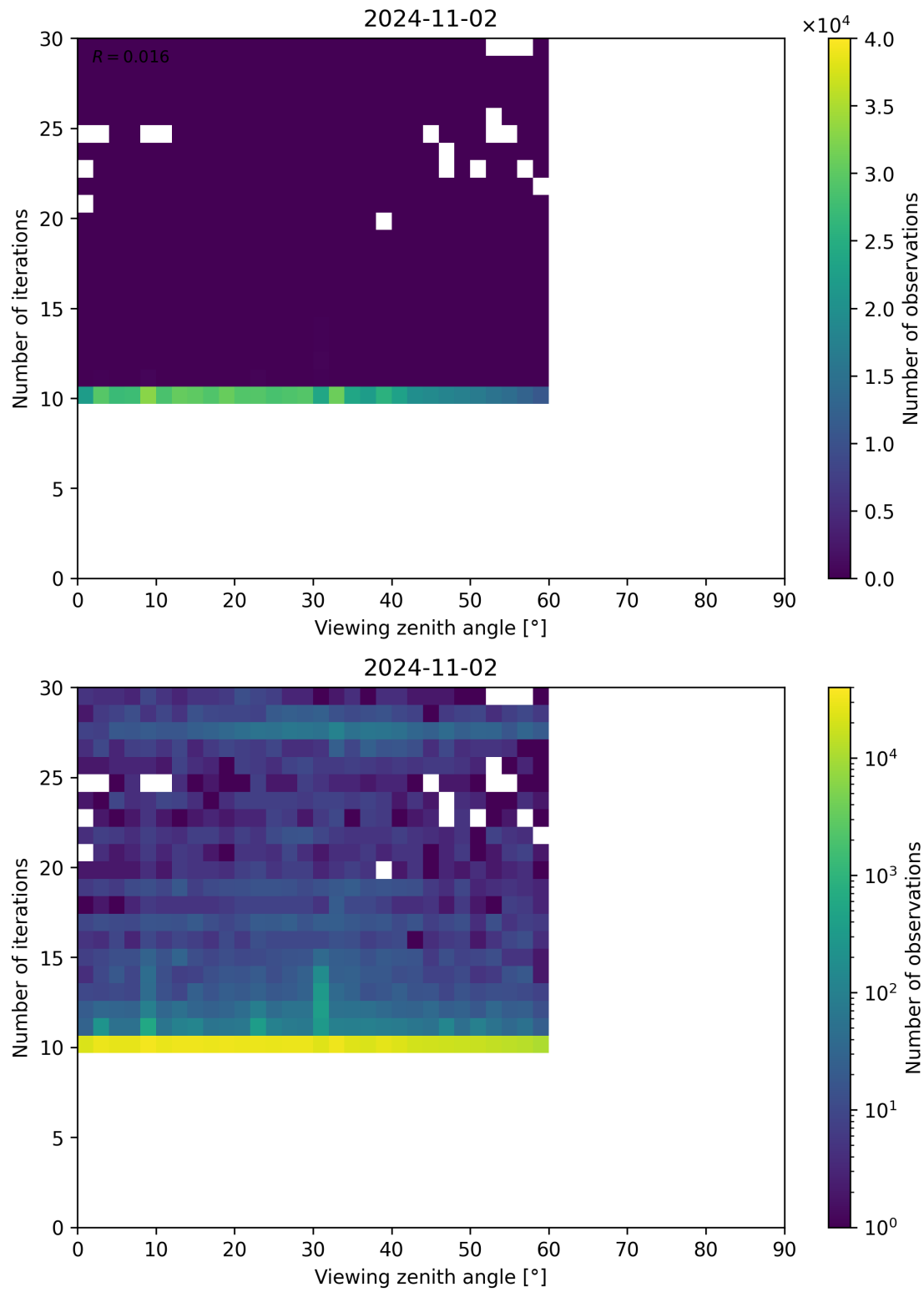
Figure 113: Scatter density plot of “Viewing zenith angle” against “Number of iterations” for 2024-11-01 to 2024-11-03.
