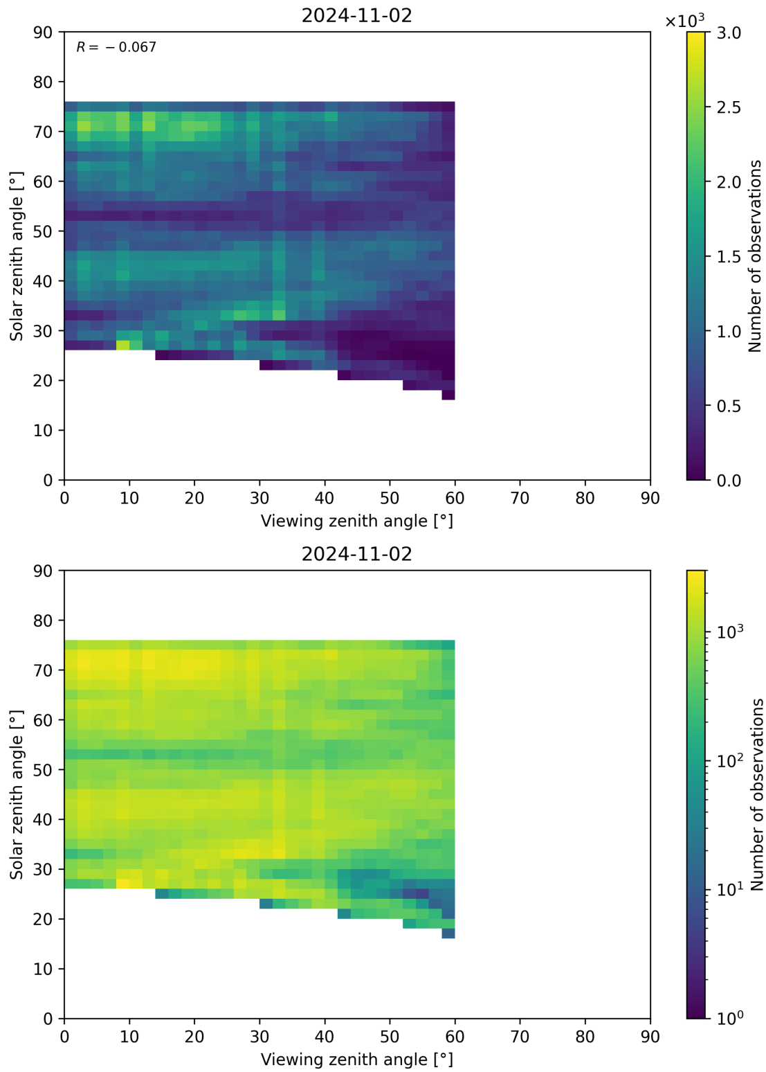
Figure 115: Scatter density plot of “Viewing zenith angle” against “Solar zenith angle” for 2024-11-01 to 2024-11-03.
