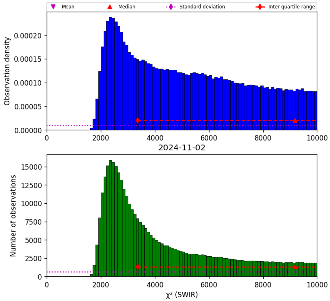
Figure 28: Histogram of “ \chi^2 (SWIR)” for 2024-11-01 to 2024-11-03
