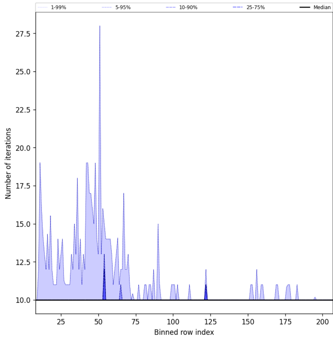
Figure 42: Along track statistics of “Number of iterations” for 2024-11-01 to 2024-11-03
