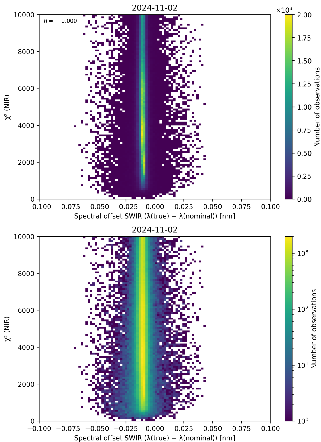
Figure 117: Scatter density plot of “Spectral offset SWIR ( \lambda_{\text{true}} - \lambda_{\text{nominal}} )” against “ \chi^2 (NIR)” for 2024-11-01 to 2024-11-03.
