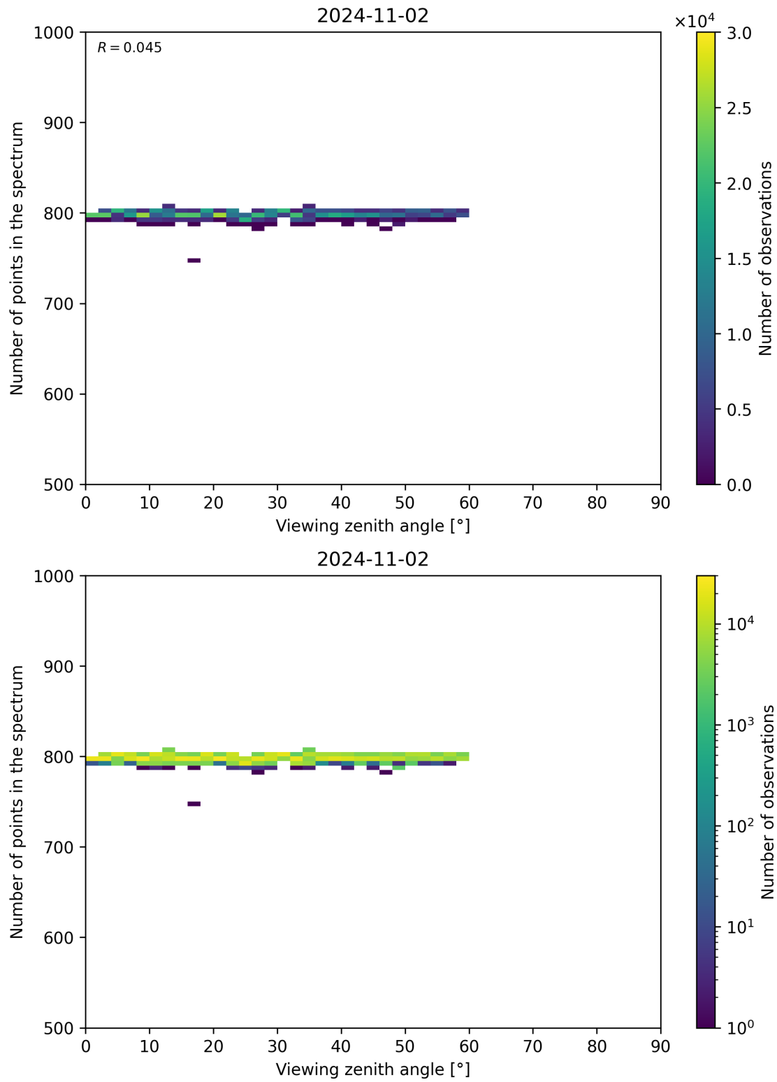
Figure 114: Scatter density plot of “Viewing zenith angle” against “Number of points in the spectrum” for 2024-11-01 to 2024-11-03.
