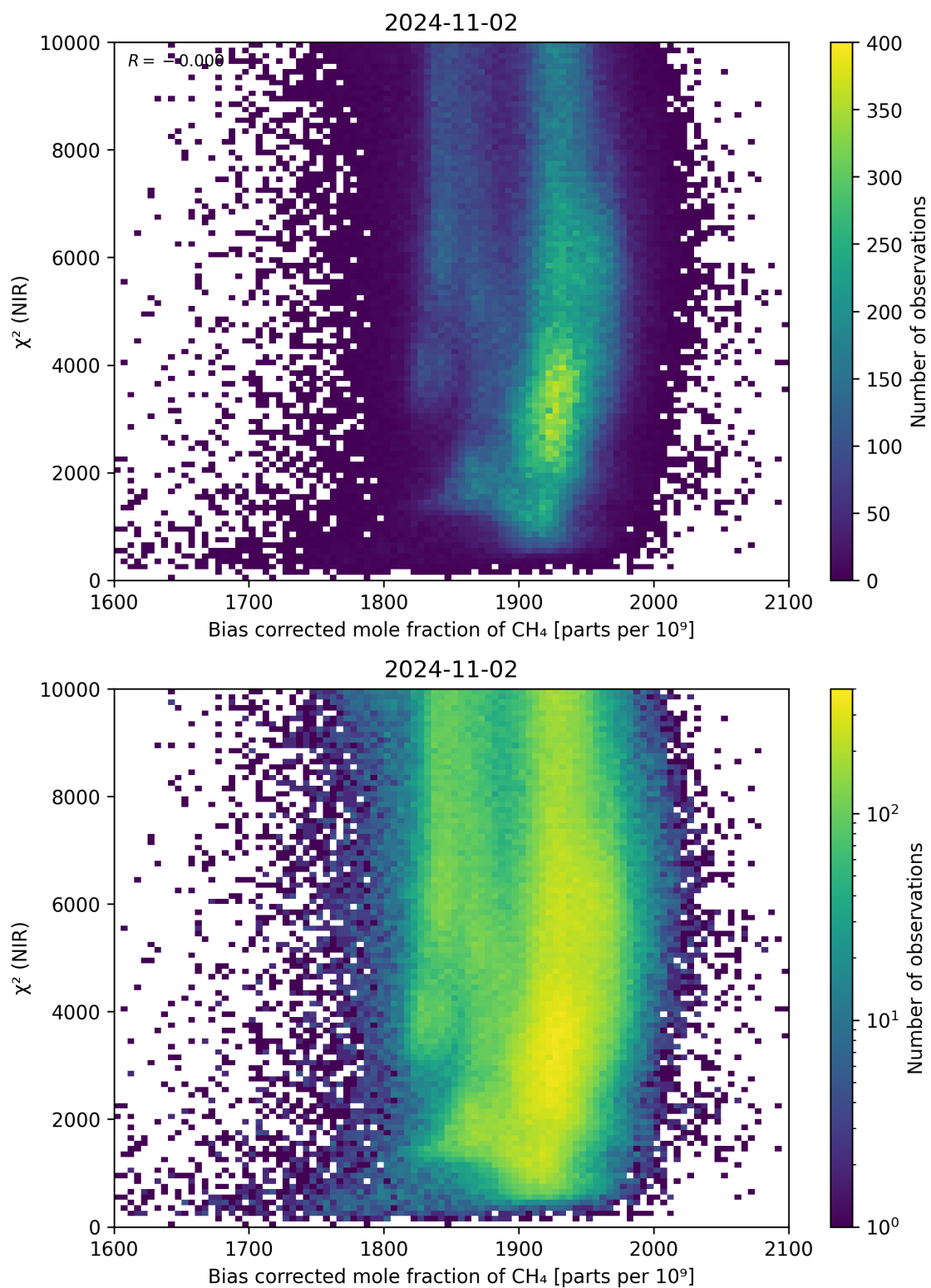
Figure 63: Scatter density plot of “Bias corrected mole fraction of CH 4 ” against “ \chi^2 (NIR)” for 2024-11-01 to 2024-11-03.
