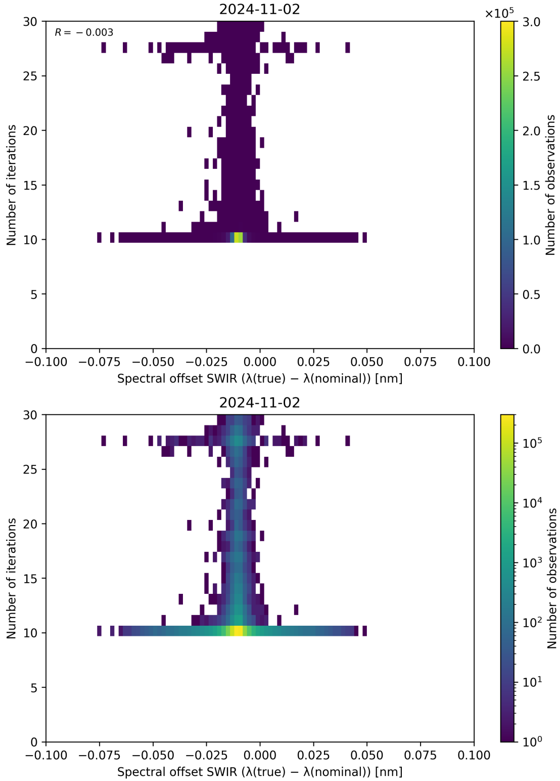
Figure 121: Scatter density plot of “Spectral offset SWIR ( \lambda_{\text{true}} - \lambda_{\text{nominal}} )” against “Number of iterations” for 2024-11-01 to 2024-11-03.
