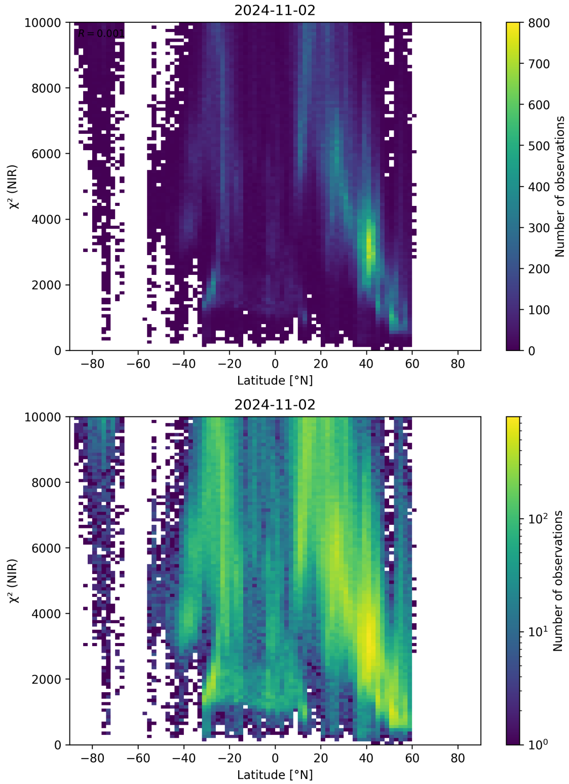
Figure 53: Scatter density plot of “Latitude” against “ \chi^2 (NIR)” for 2024-11-01 to 2024-11-03.
