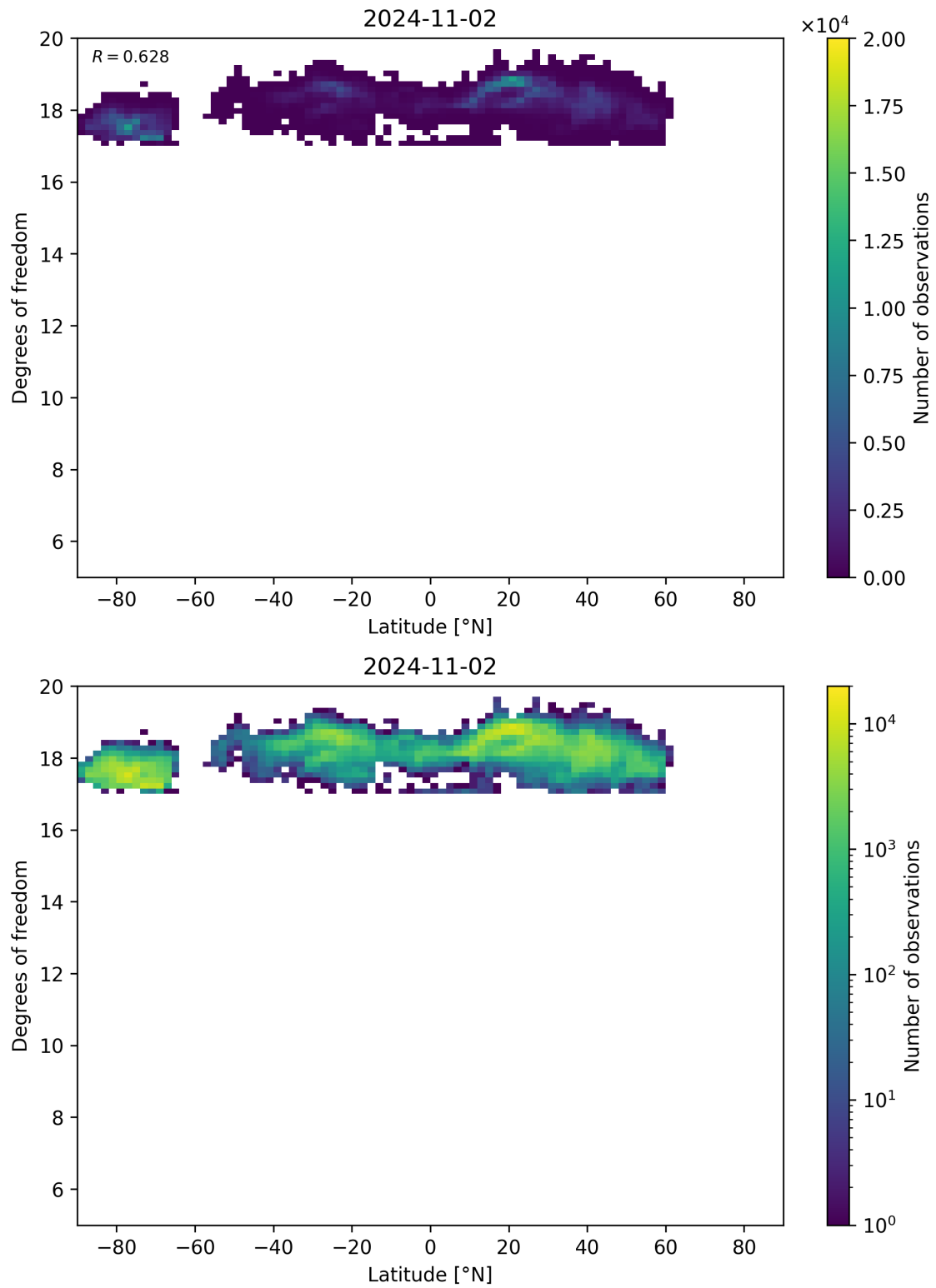
Figure 55: Scatter density plot of “Latitude” against “Degrees of freedom” for 2024-11-01 to 2024-11-03.
