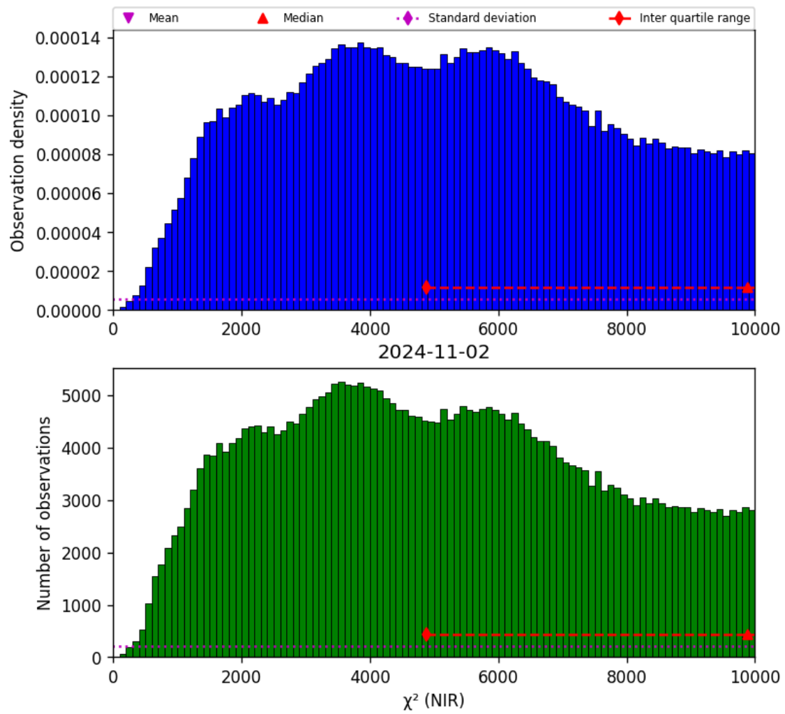
Figure 29: Histogram of “ \chi^2 (NIR)” for 2024-11-01 to 2024-11-03
