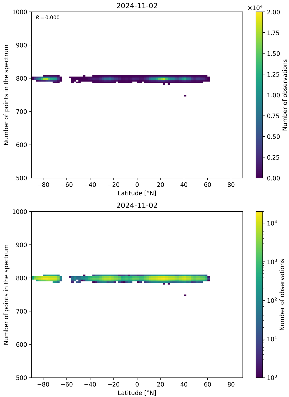
Figure 61: Scatter density plot of “Latitude” against “Number of points in the spectrum” for 2024-11-01 to 2024-11-03.
