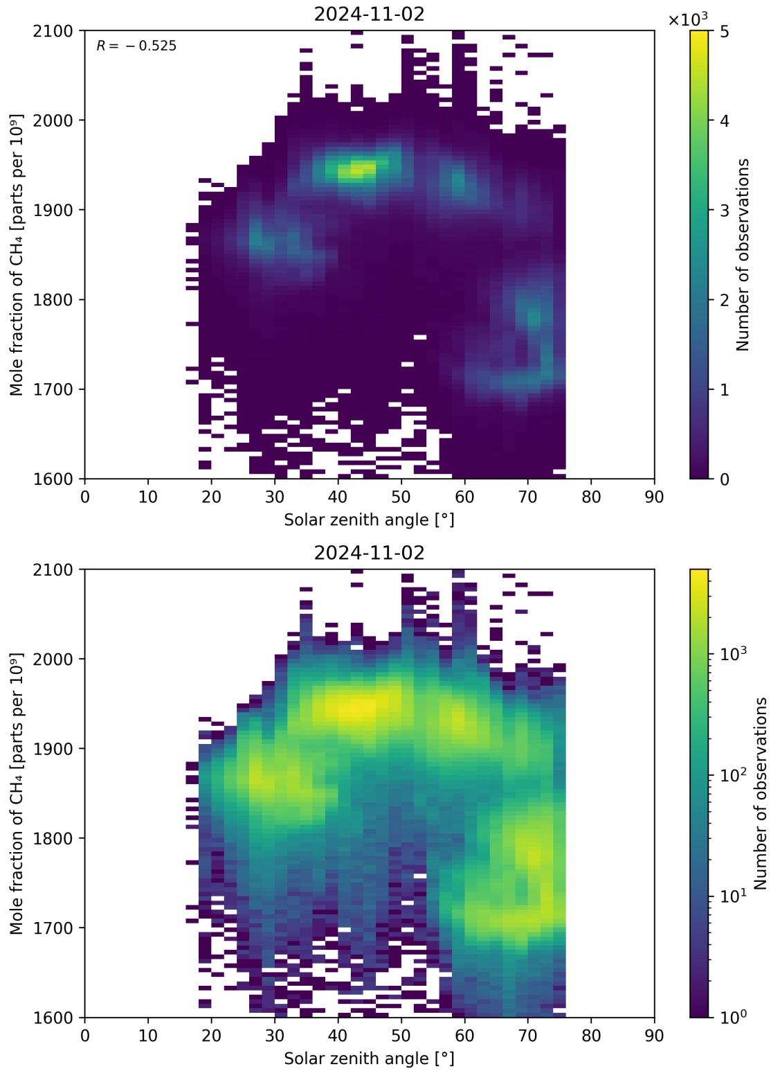
Figure 99: Scatter density plot of “Solar zenith angle” against “Mole fraction of CH 4 ” for 2024-11-01 to 2024-11-03.
