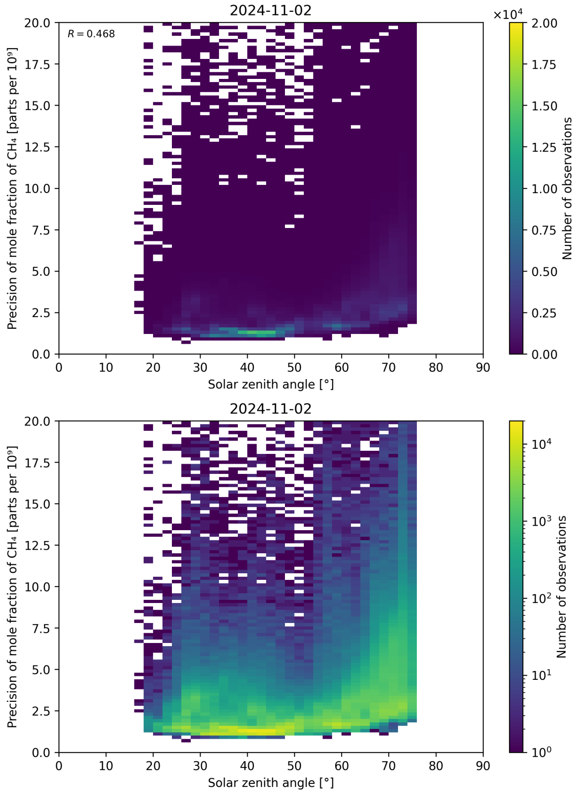
Figure 101: Scatter density plot of “Solar zenith angle” against “Precision of mole fraction of \text{CH}_4 ” for 2024-11-01 to 2024-11-03.
