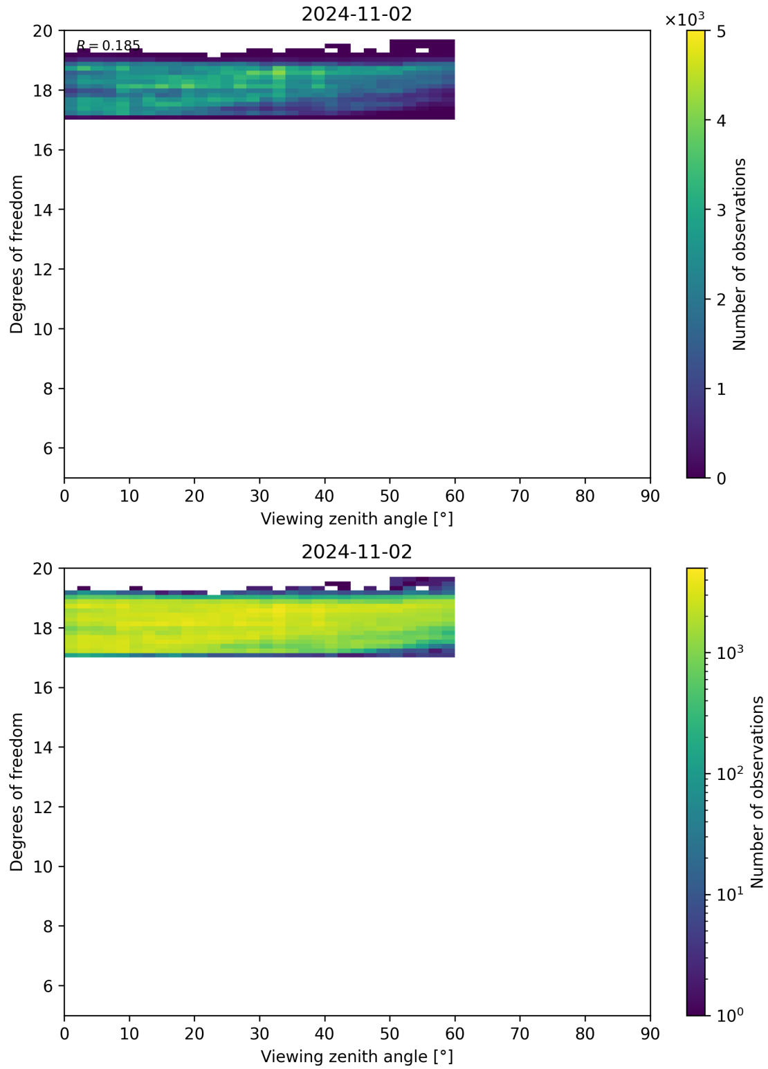
Figure 107: Scatter density plot of “Viewing zenith angle” against “Degrees of freedom” for 2024-11-01 to 2024-11-03.
