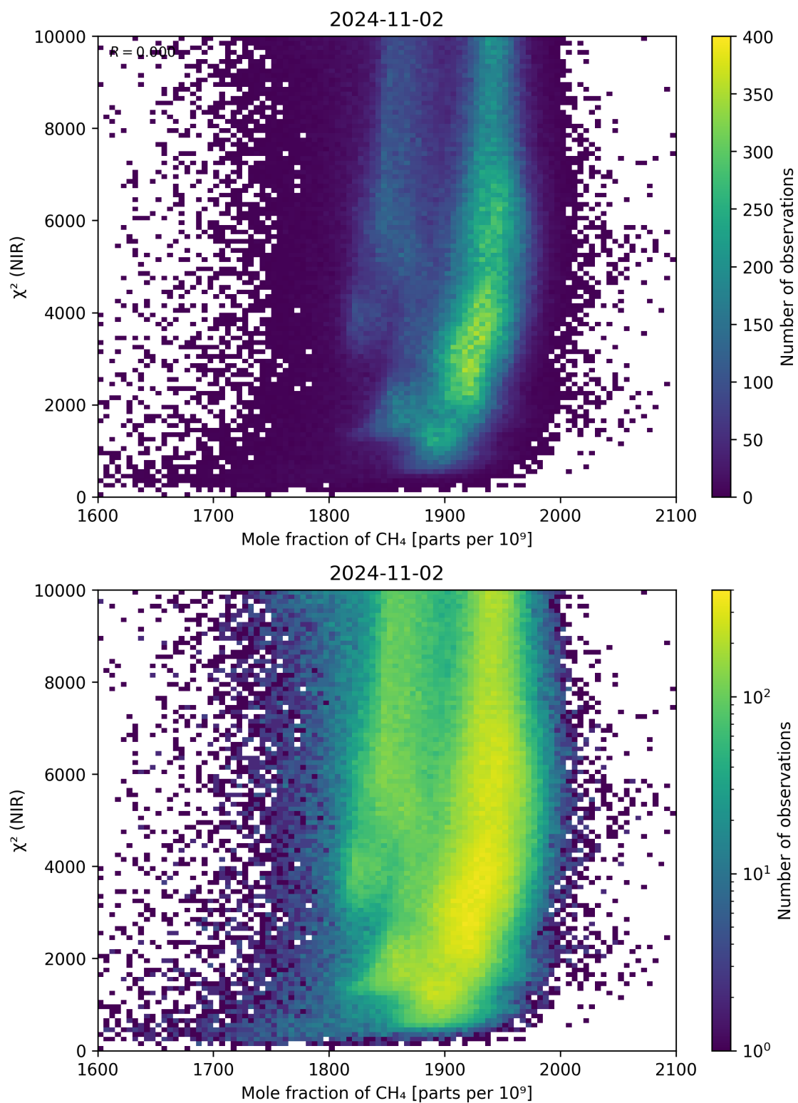
Figure 70: Scatter density plot of “Mole fraction of \text{CH}_4 ” against “ \chi^2 (NIR)” for 2024-11-01 to 2024-11-03.
