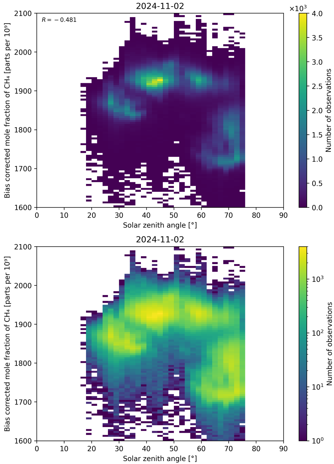
Figure 100: Scatter density plot of “Solar zenith angle” against “Bias corrected mole fraction of CH 4 ” for 2024-11-01 to 2024-11-03.
