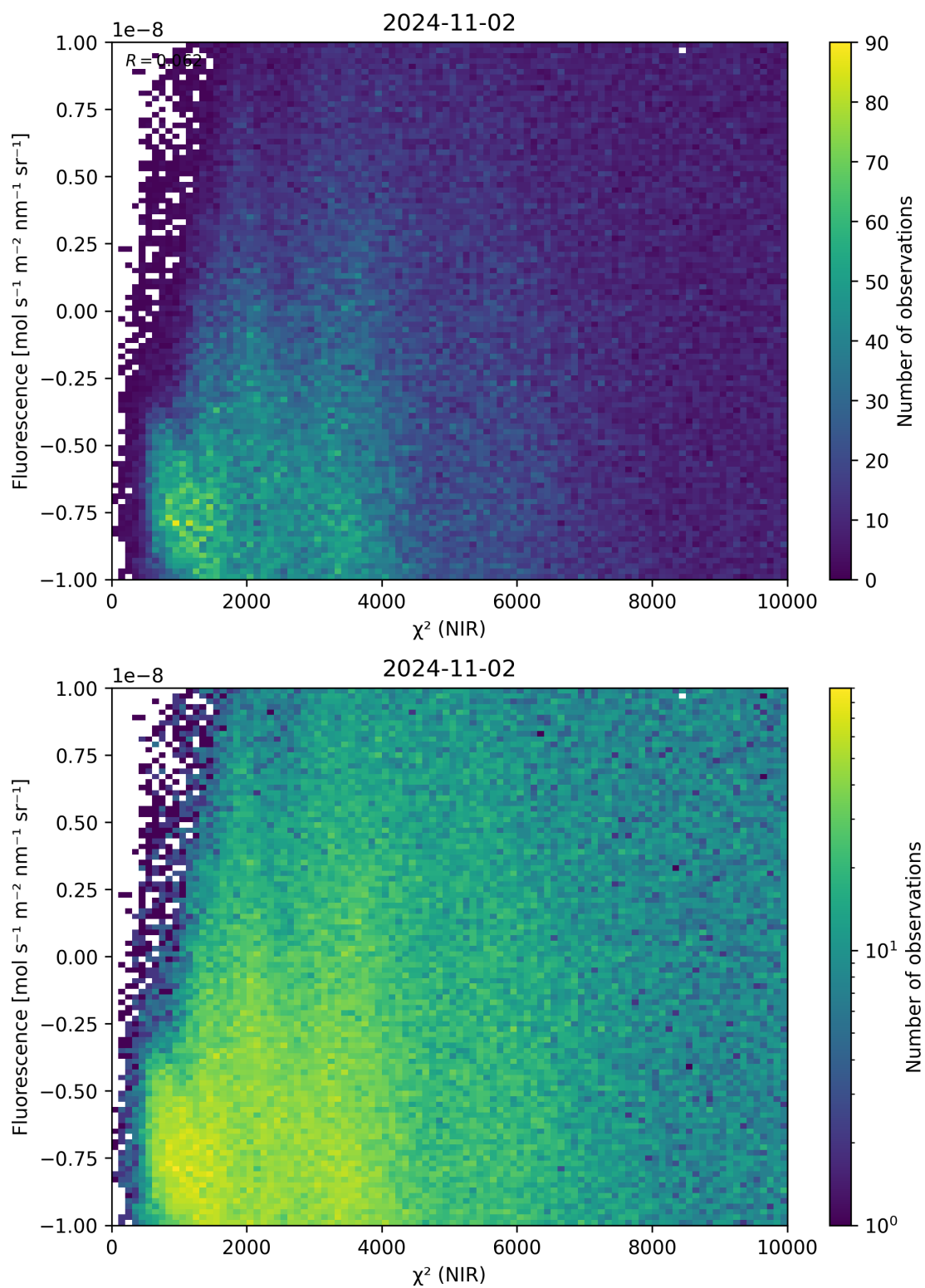
Figure 45: Scatter density plot of “ \chi^2 (NIR)” against “Fluorescence” for 2024-11-01 to 2024-11-03.
