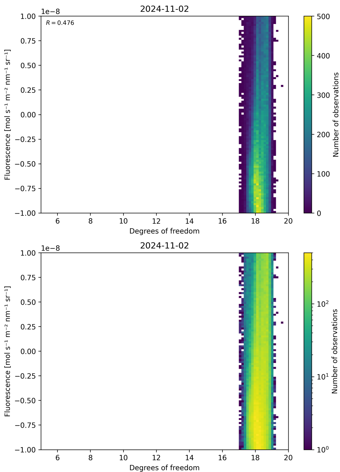
Figure 51: Scatter density plot of “Degrees of freedom” against “Fluorescence” for 2024-11-01 to 2024-11-03.
