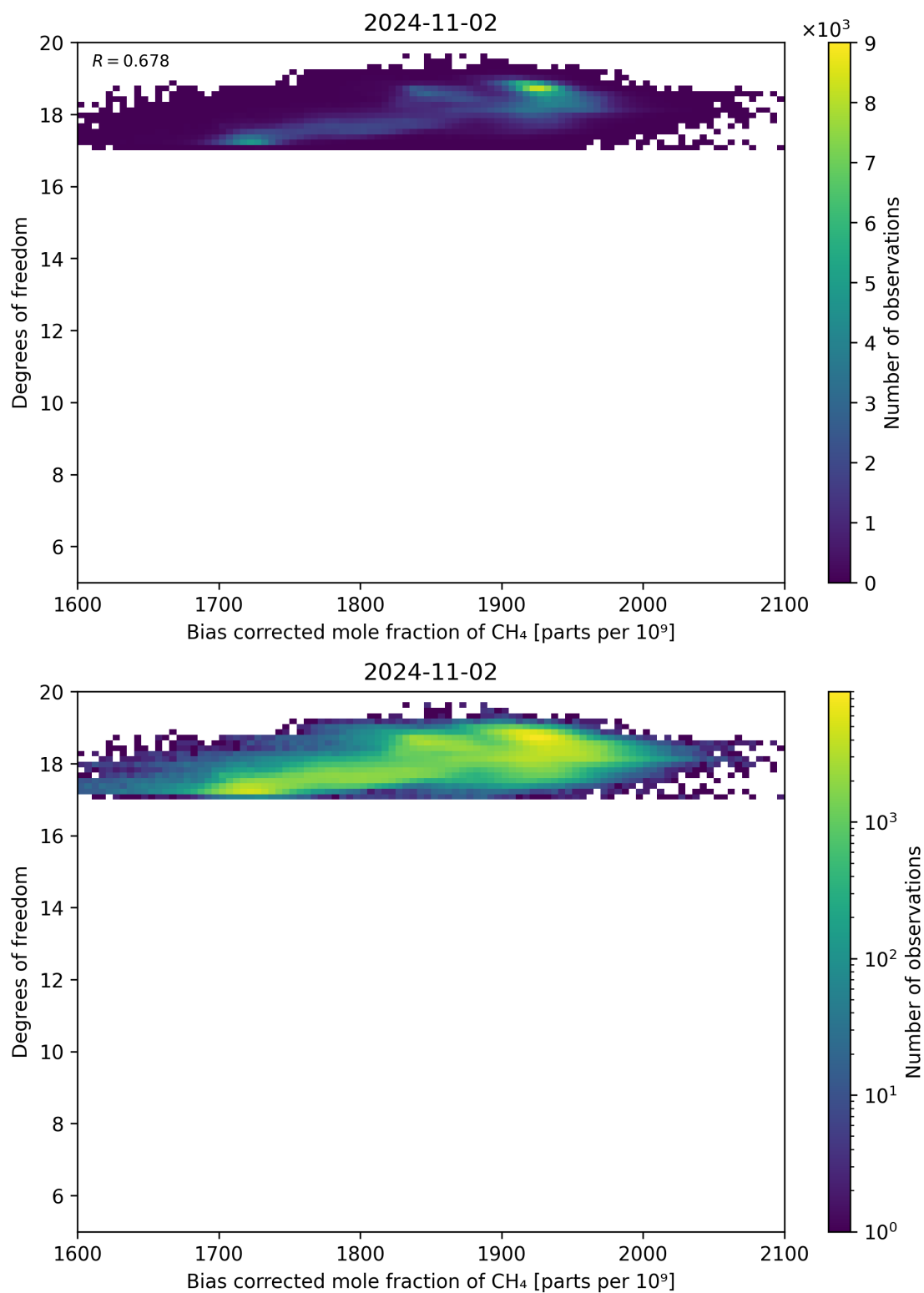
Figure 65: Scatter density plot of “Bias corrected mole fraction of CH 4 ” against “Degrees of freedom” for 2024-11-01 to 2024-11-03.
