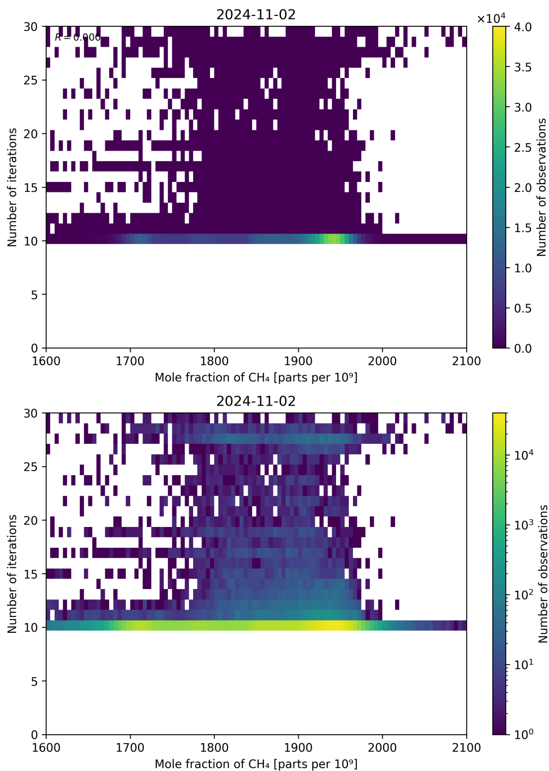
Figure 76: Scatter density plot of “Mole fraction of CH 4 ” against “Number of iterations” for 2024-11-01 to 2024-11-03.
