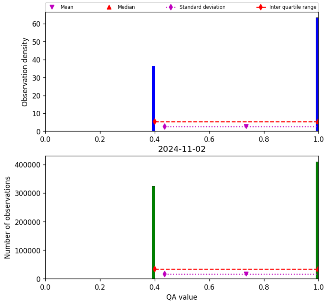
Figure 22: Histogram of “QA value” for 2024-11-01 to 2024-11-03
