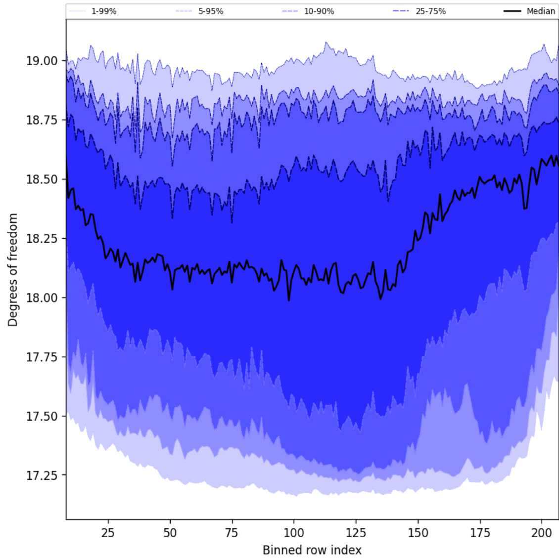
Figure 41: Along track statistics of “Degrees of freedom” for 2024-11-01 to 2024-11-03
