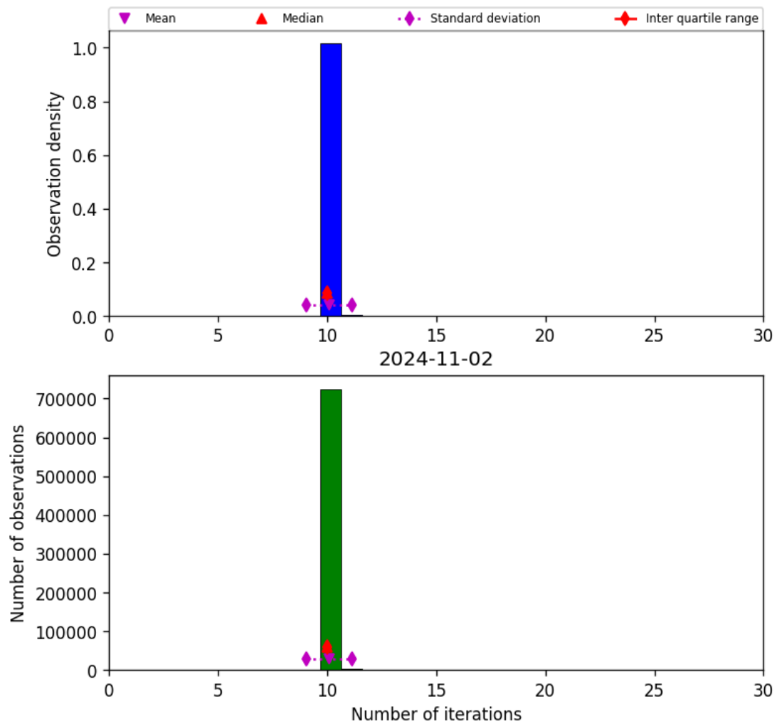
Figure 31: Histogram of “Number of iterations” for 2024-11-01 to 2024-11-03
