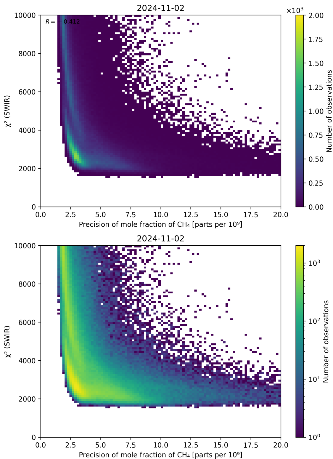
Figure 79: Scatter density plot of “Precision of mole fraction of \text{CH}_4 ” against “ \chi^2 (SWIR)” for 2024-11-01 to 2024-11-03.
