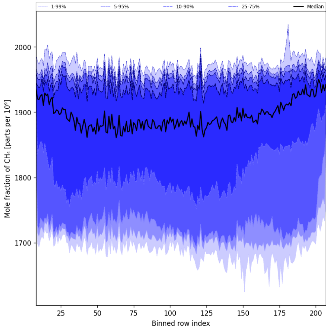
Figure 34: Along track statistics of “Mole fraction of CH 4 ” for 2024-11-01 to 2024-11-03
