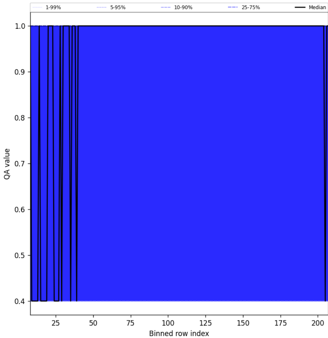
Figure 33: Along track statistics of “QA value” for 2024-11-01 to 2024-11-03
