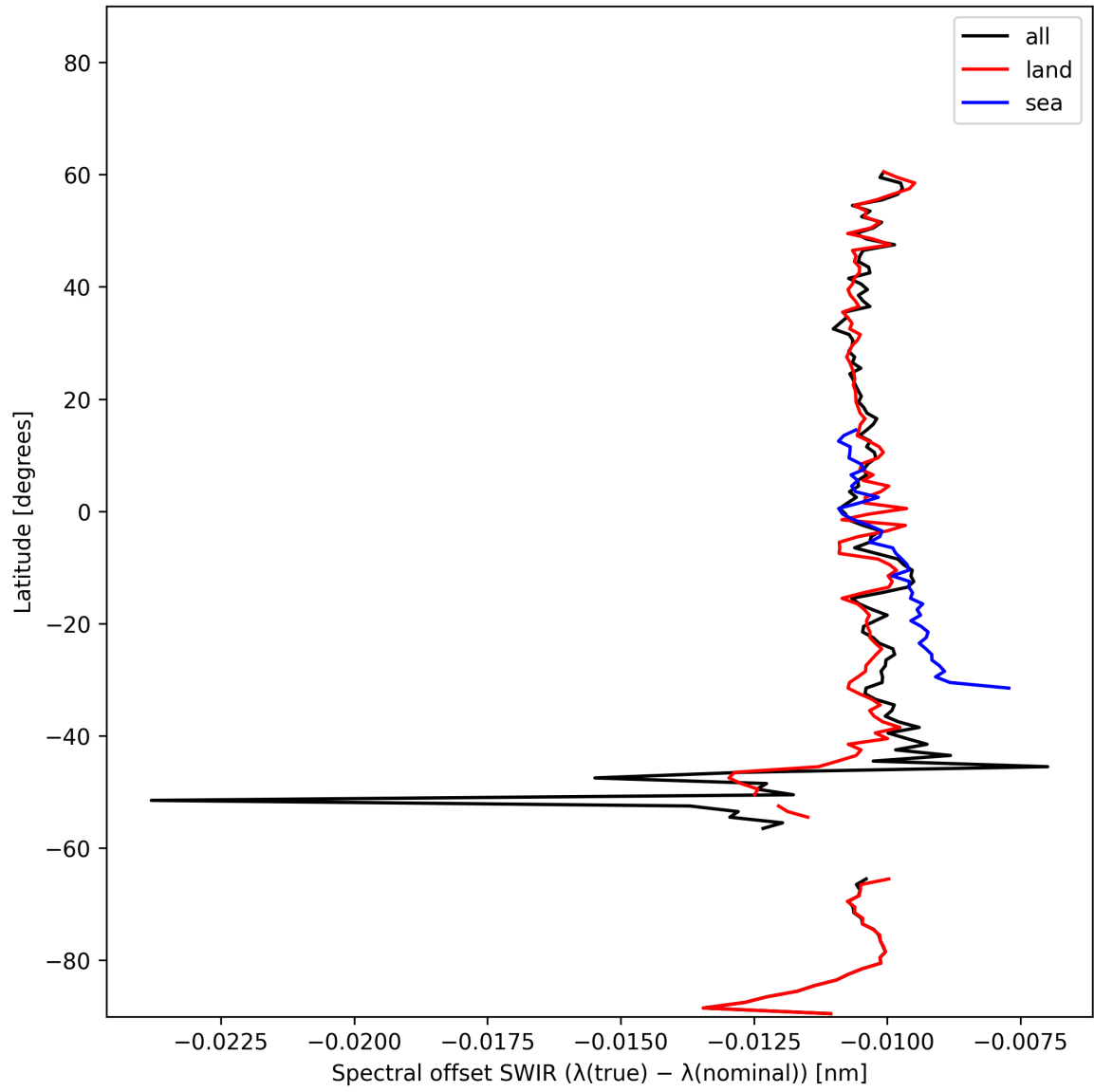
Figure 16: Zonal average of “Spectral offset SWIR ( \lambda_{\text{true}} - \lambda_{\text{nominal}} )” for 2024-11-01 to 2024-11-03.
