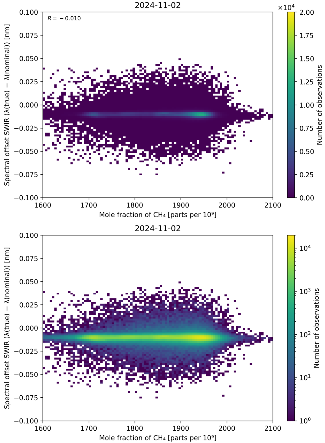
Figure 86: Scatter density plot of “Mole fraction of CH 4 ” against “Spectral offset SWIR ( \lambda_{\text{true}} - \lambda_{\text{nominal}} )” for 2024-11-01 to 2024-11-03.
