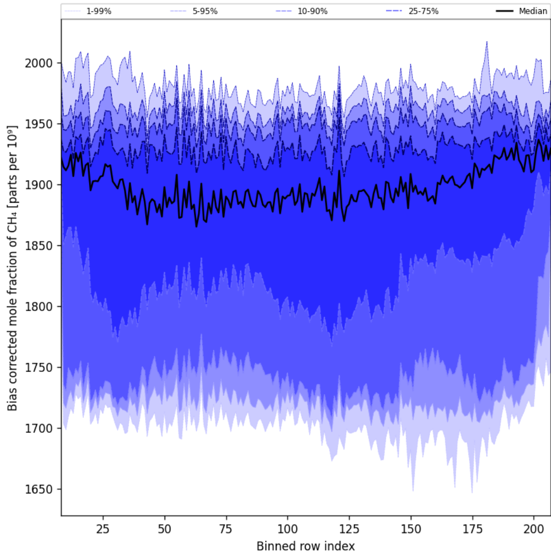
Figure 36: Along track statistics of “Bias corrected mole fraction of CH 4 ” for 2024-11-01 to 2024-11-03
