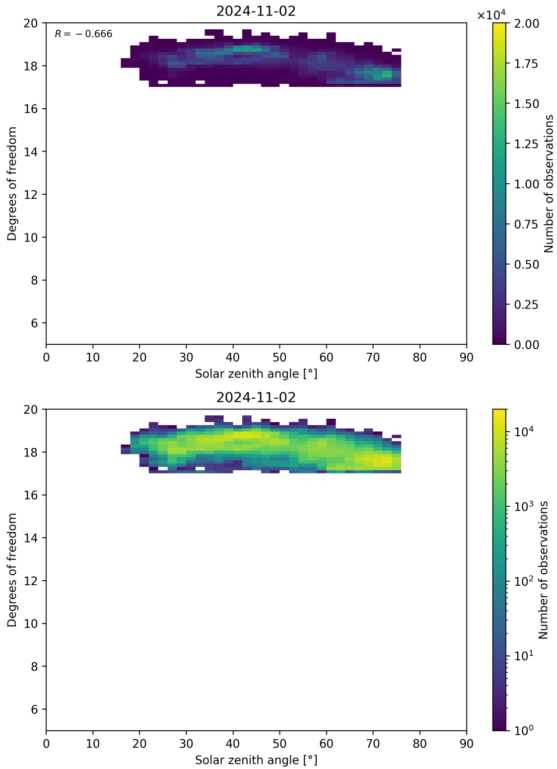
Figure 96: Scatter density plot of “Solar zenith angle” against “Degrees of freedom” for 2024-11-01 to 2024-11-03.
