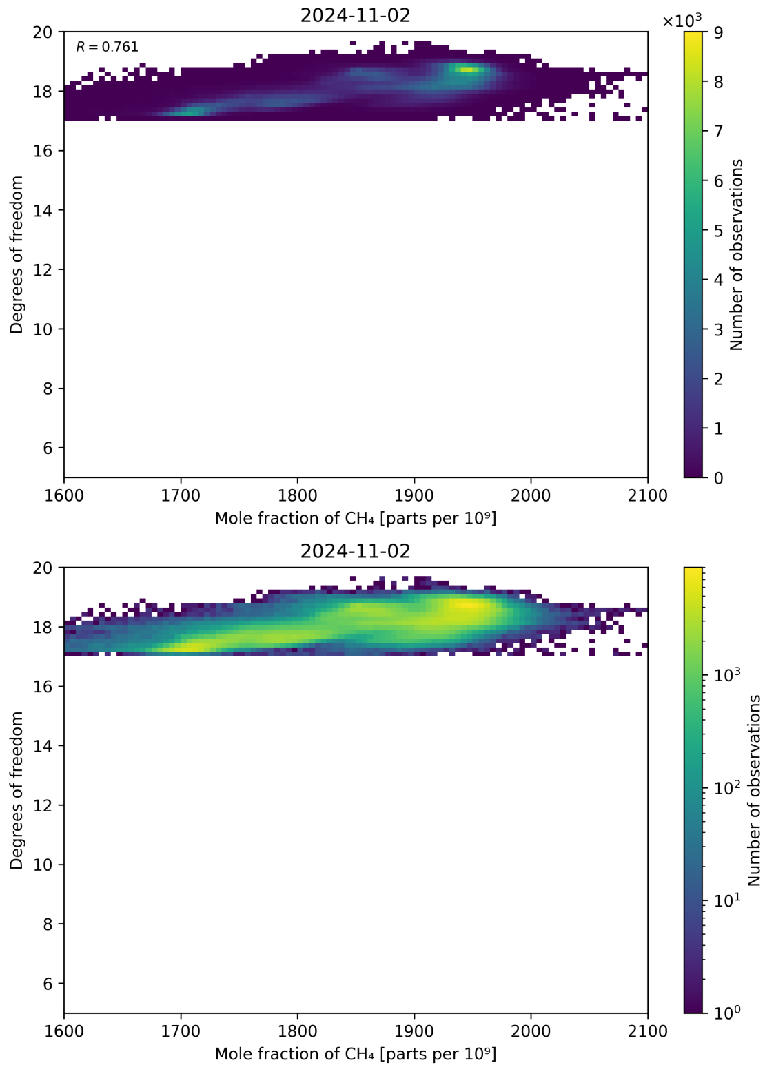
Figure 72: Scatter density plot of “Mole fraction of CH 4 ” against “Degrees of freedom” for 2024-11-01 to 2024-11-03.
