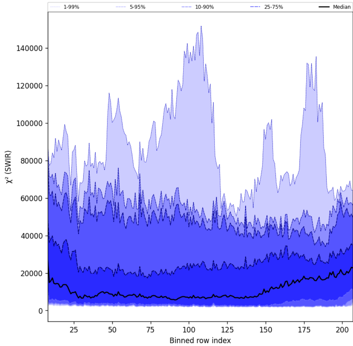
Figure 39: Along track statistics of “ \chi^2 (SWIR)” for 2024-11-01 to 2024-11-03
