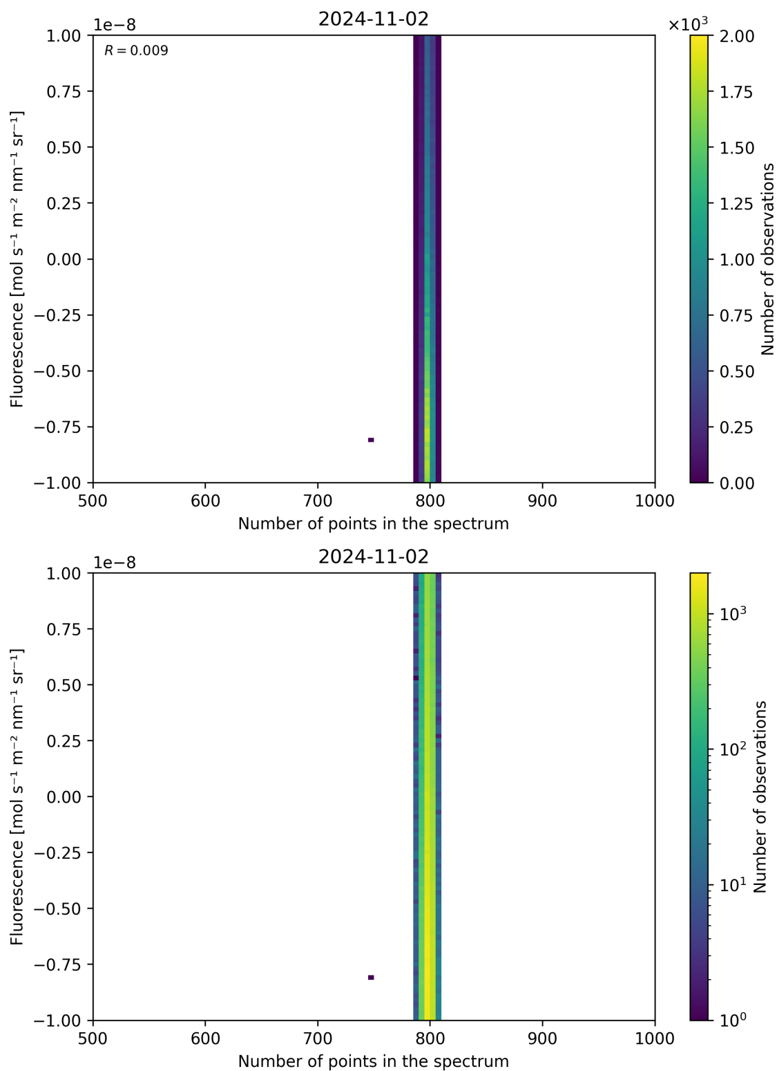
Figure 91: Scatter density plot of “Number of points in the spectrum” against “Fluorescence” for 2024-11-01 to 2024-11-03.
