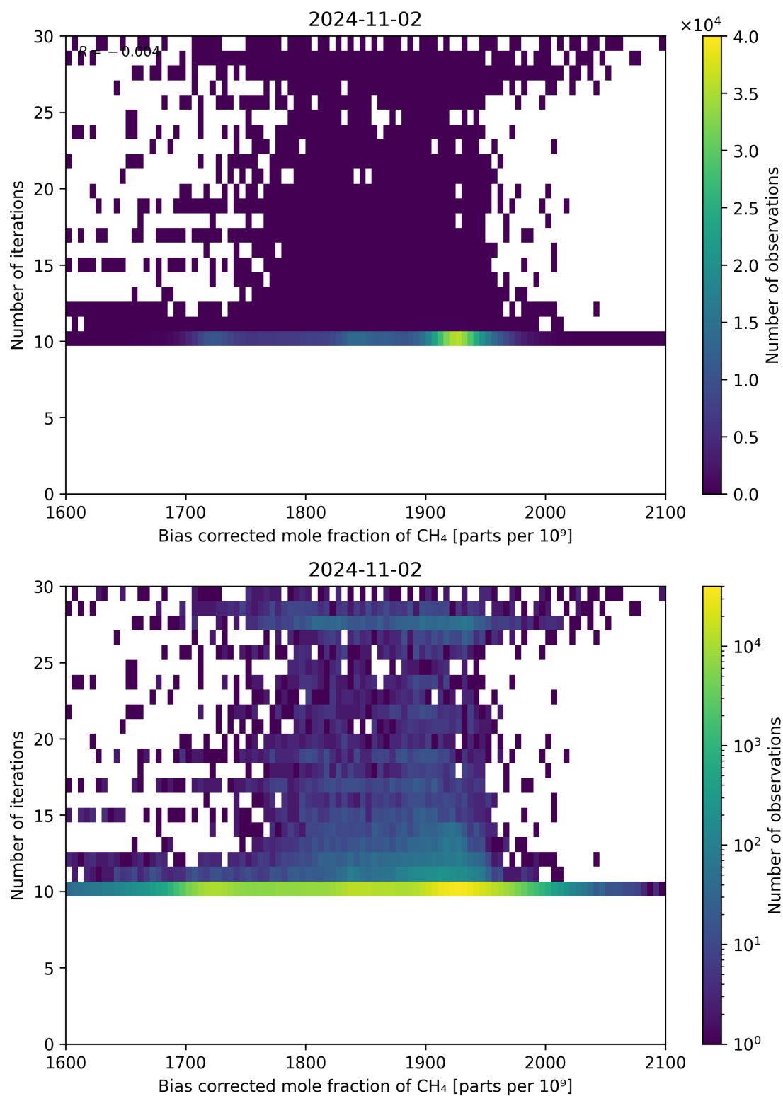
Figure 67: Scatter density plot of “Bias corrected mole fraction of CH 4 ” against “Number of iterations” for 2024-11-01 to 2024-11-03.
