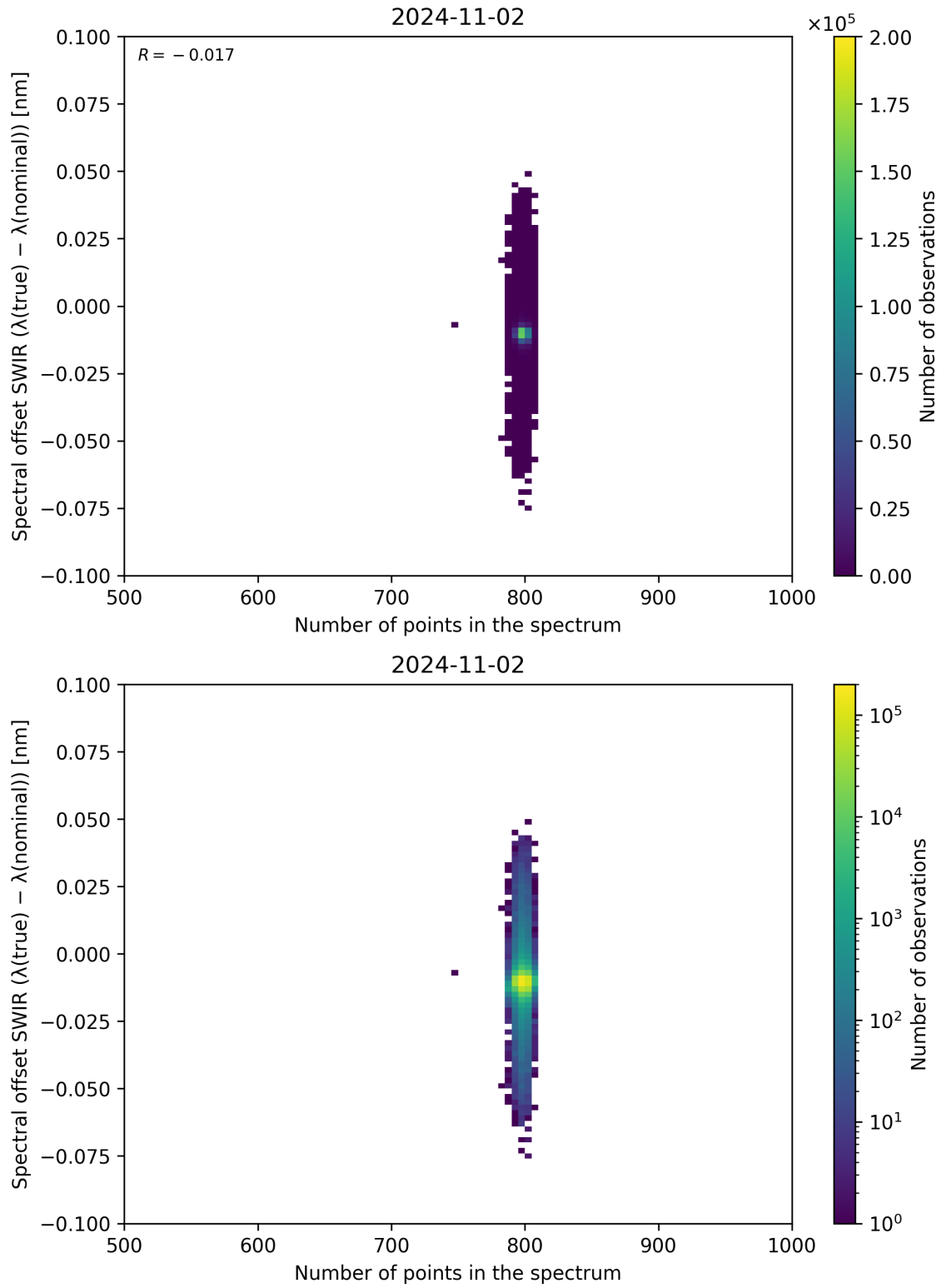
Figure 93: Scatter density plot of “Number of points in the spectrum” against “Spectral offset SWIR ( \lambda_{\text{true}} - \lambda_{\text{nominal}} )” for 2024-11-01 to 2024-11-03.
