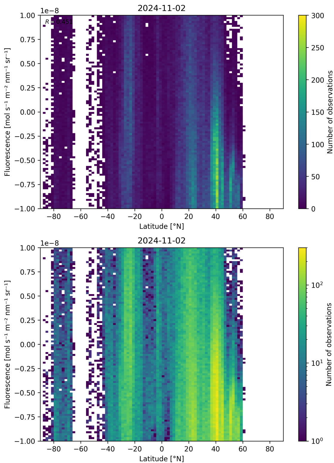
Figure 56: Scatter density plot of “Latitude” against “Fluorescence” for 2024-11-01 to 2024-11-03.
