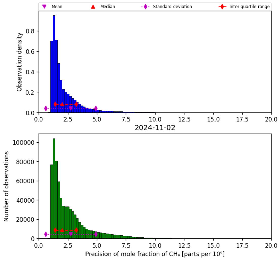
Figure 24: Histogram of “Precision of mole fraction of CH 4 ” for 2024-11-01 to 2024-11-03
