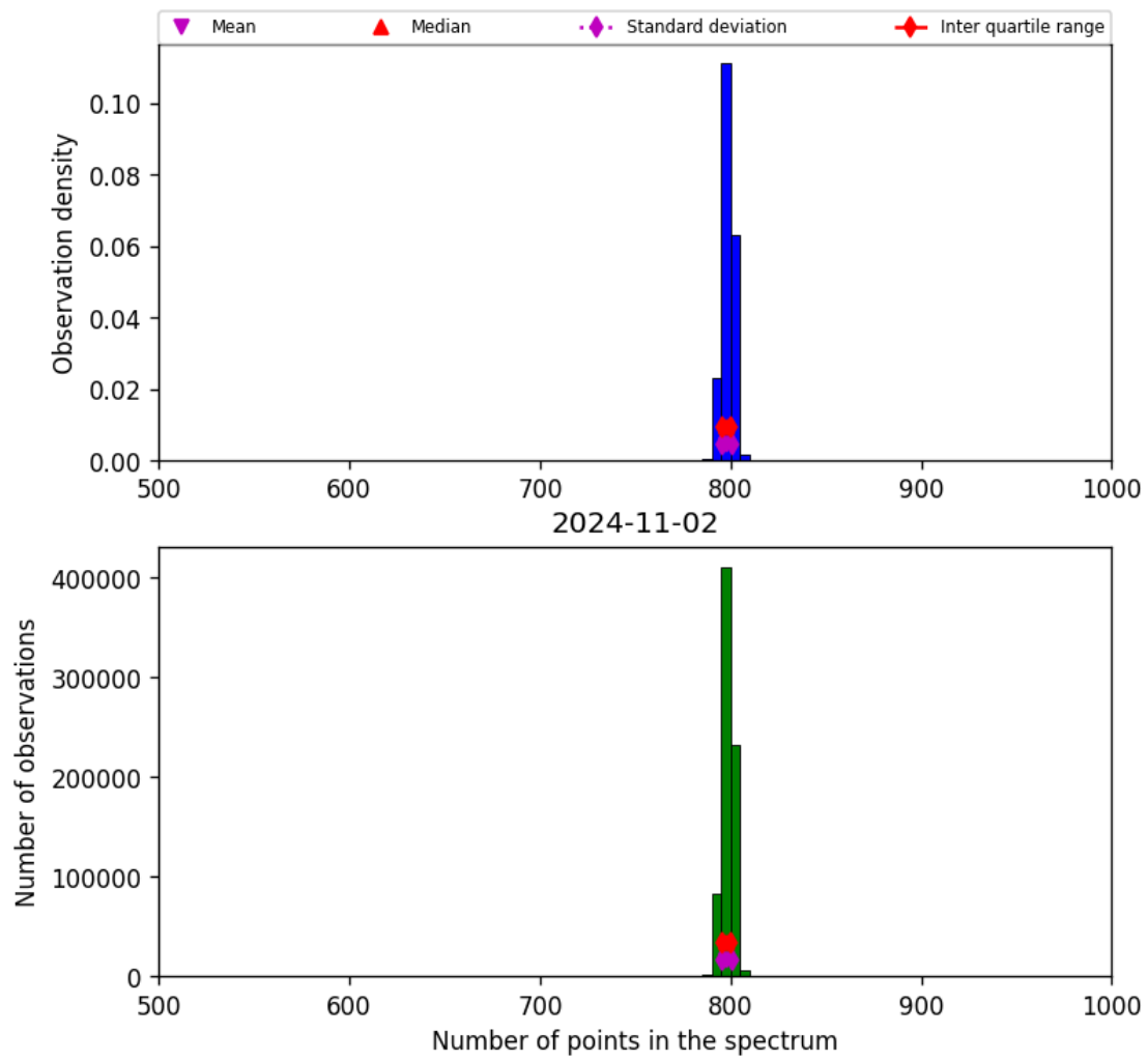
Figure 26: Histogram of “Number of points in the spectrum” for 2024-11-01 to 2024-11-03
