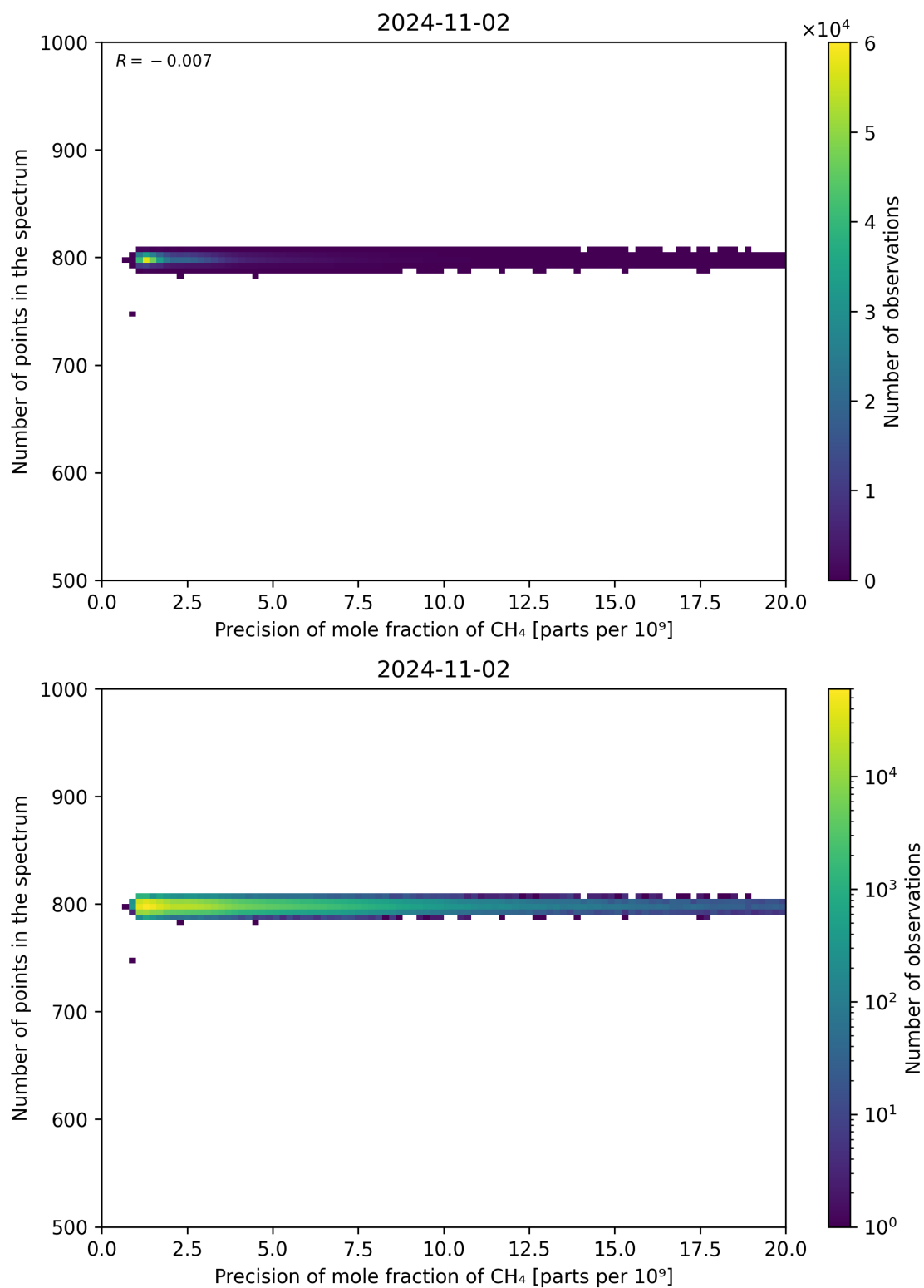
Figure 84: Scatter density plot of “Precision of mole fraction of CH 4 ” against “Number of points in the spectrum” for 2024-11-01 to 2024-11-03.
