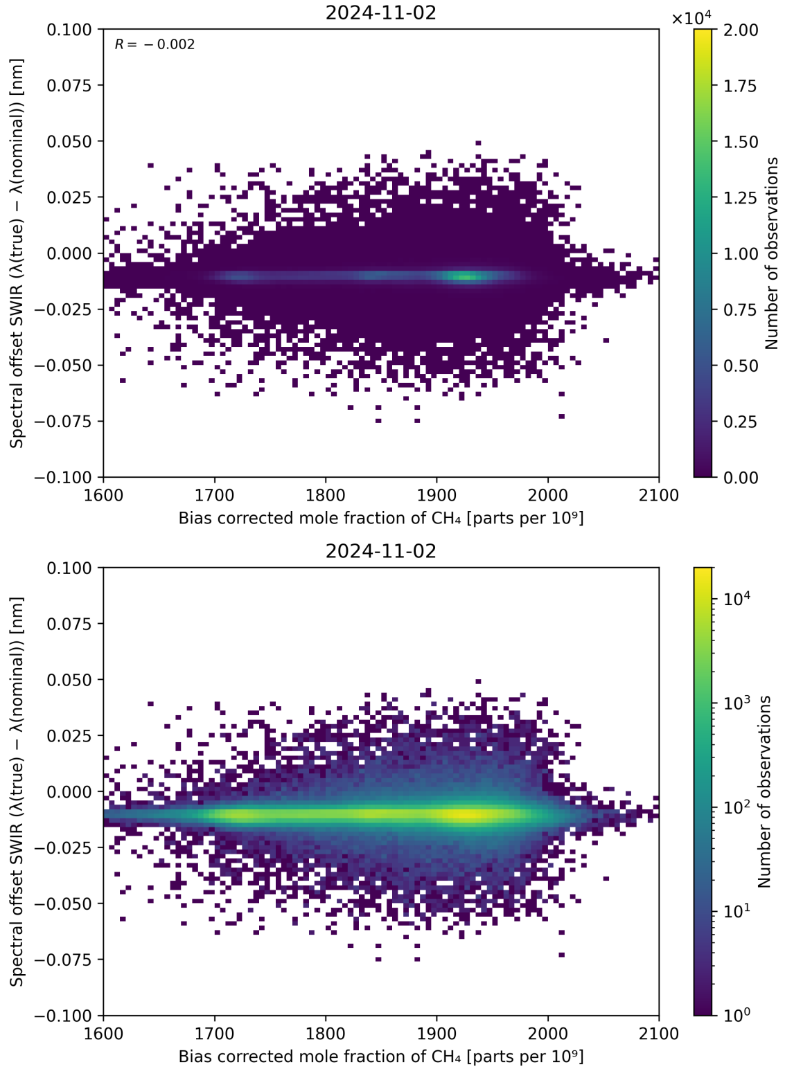
Figure 69: Scatter density plot of “Bias corrected mole fraction of \text{CH}_4 ” against “Spectral offset SWIR ( \lambda_{\text{true}} - \lambda_{\text{nominal}} )” for 2024-11-01 to 2024-11-03.
