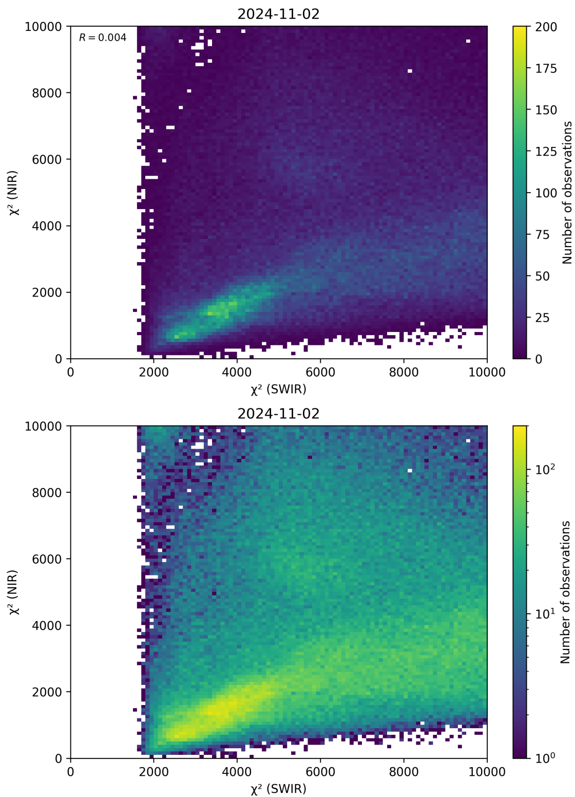
Figure 47: Scatter density plot of “ \chi^2 (SWIR)” against “ \chi^2 (NIR)” for 2024-11-01 to 2024-11-03.
