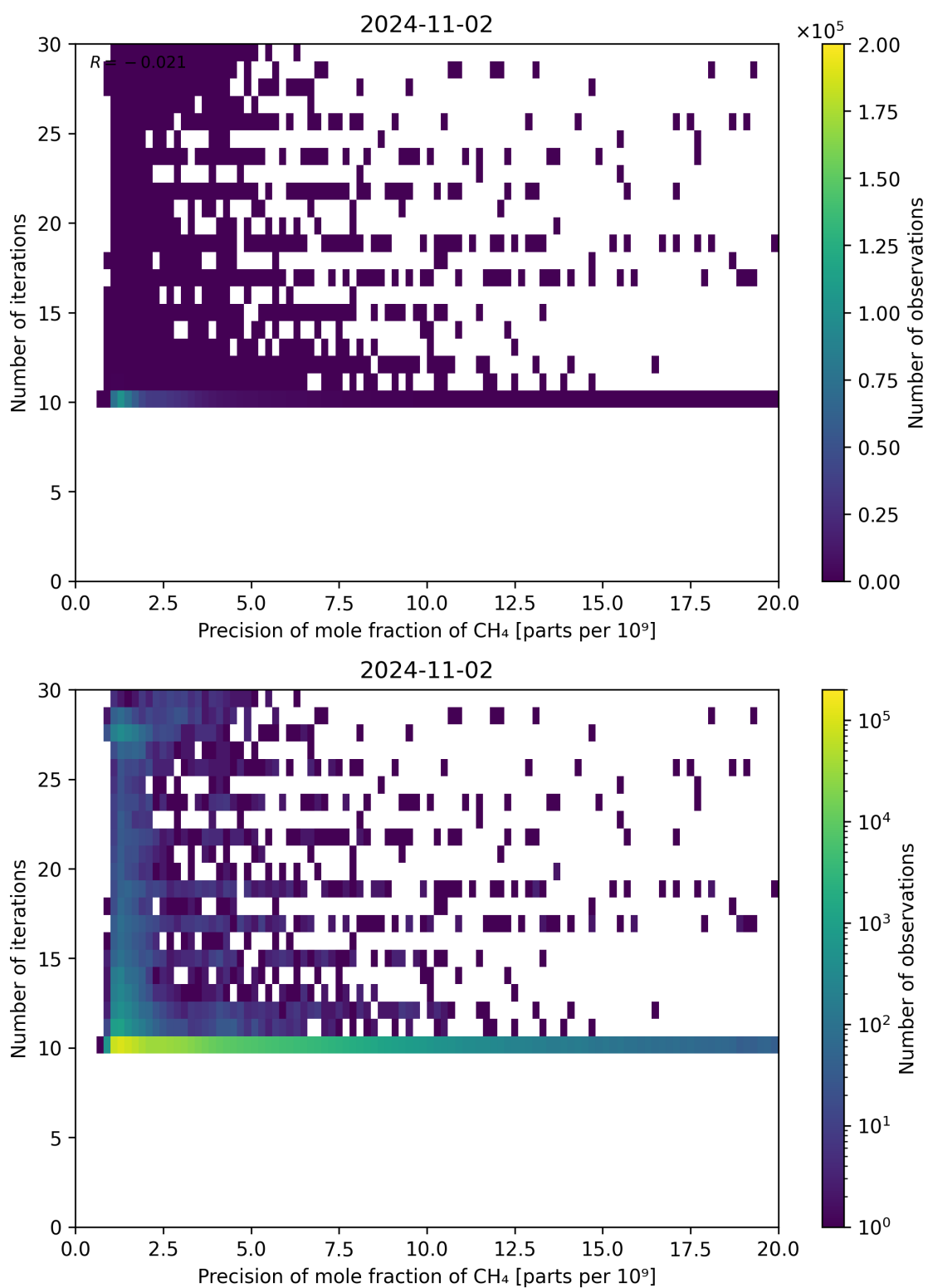
Figure 83: Scatter density plot of “Precision of mole fraction of CH 4 ” against “Number of iterations” for 2024-11-01 to 2024-11-03.
