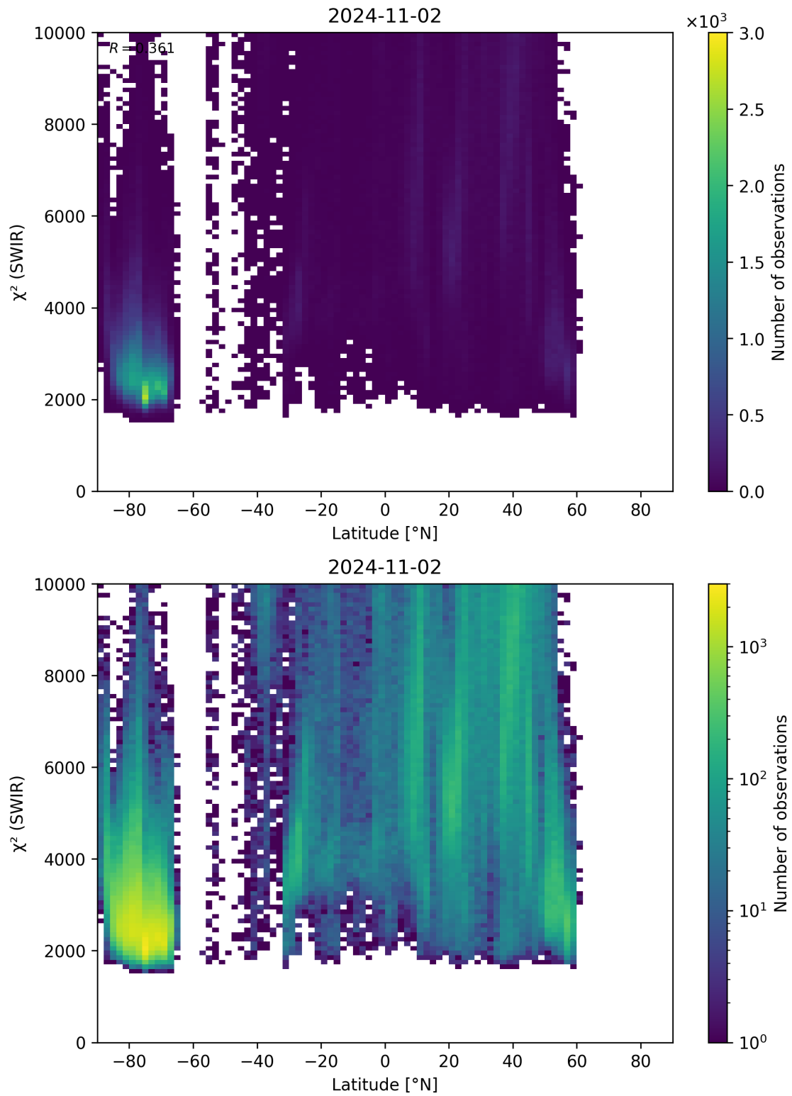
Figure 54: Scatter density plot of “Latitude” against “ \chi^2 (SWIR)” for 2024-11-01 to 2024-11-03.
