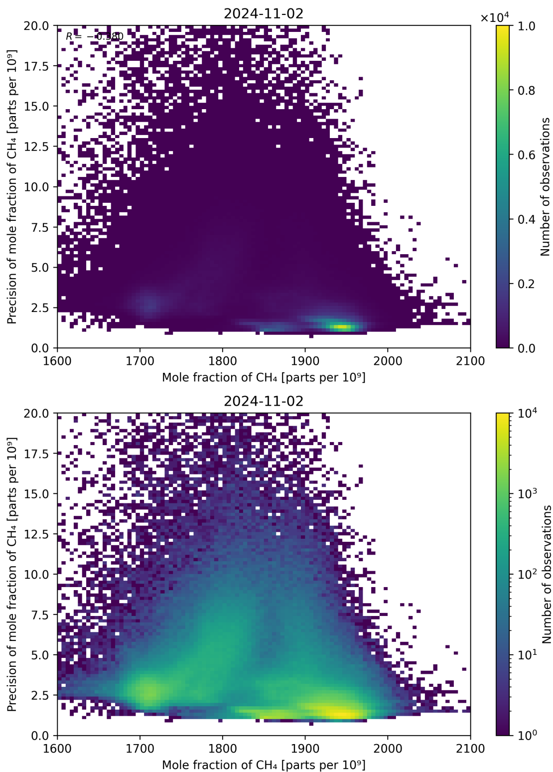
Figure 75: Scatter density plot of “Mole fraction of CH 4 ” against “Precision of mole fraction of CH 4 ” for 2024-11-01 to 2024-11-03.
