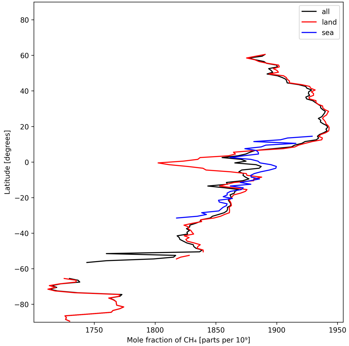
Figure 12: Zonal average of “Mole fraction of CH 4 ” for 2024-11-01 to 2024-11-03.
