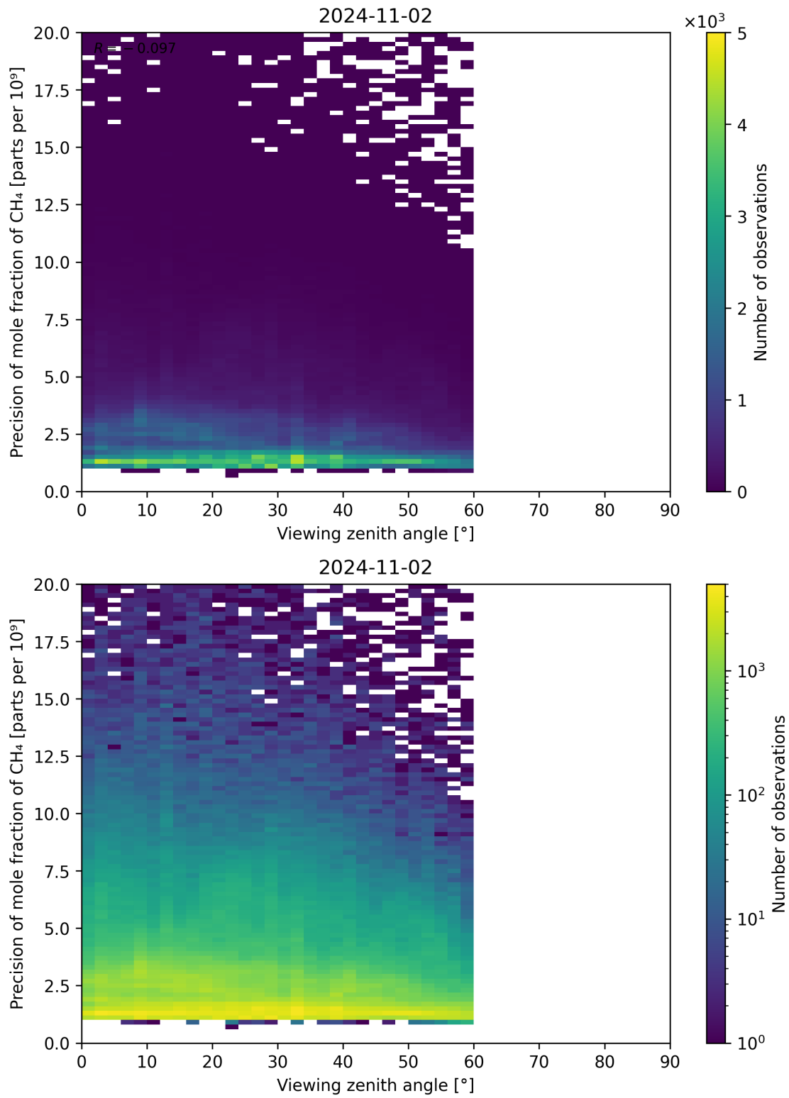
Figure 112: Scatter density plot of “Viewing zenith angle” against “Precision of mole fraction of CH 4 ” for 2024-11-01 to 2024-11-03.
