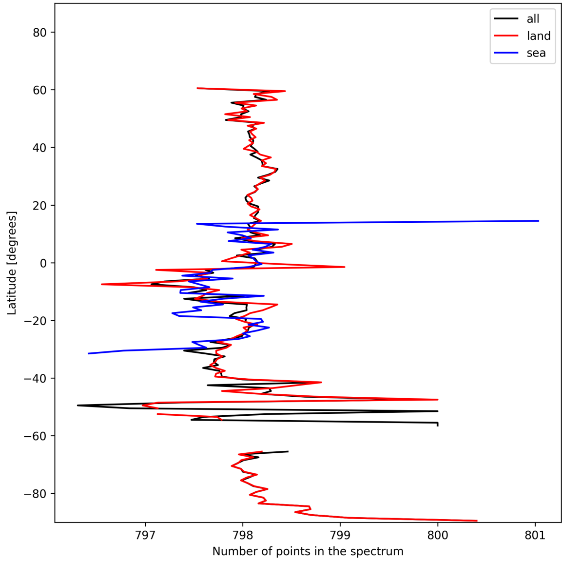
Figure 15: Zonal average of “Number of points in the spectrum” for 2024-11-01 to 2024-11-03.
