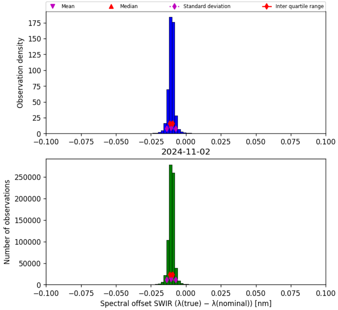
Figure 27: Histogram of “Spectral offset SWIR ( \lambda_{\text{true}} - \lambda_{\text{nominal}} )” for 2024-11-01 to 2024-11-03
