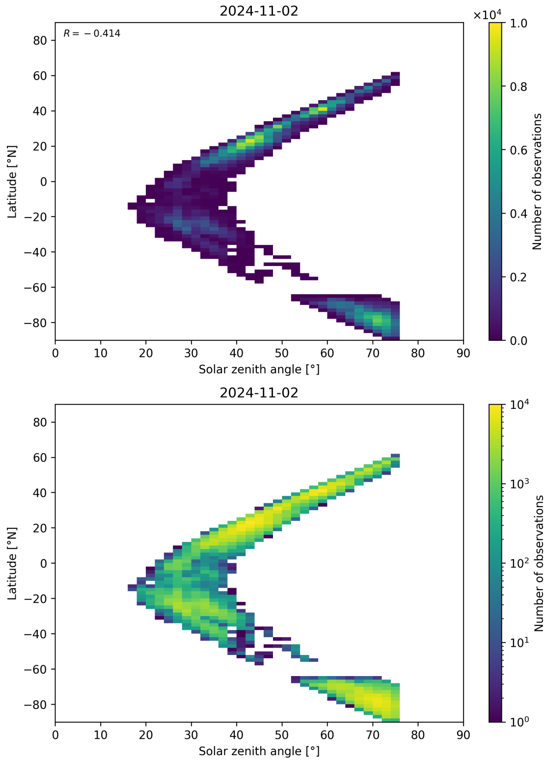
Figure 98: Scatter density plot of “Solar zenith angle” against “Latitude” for 2024-11-01 to 2024-11-03.
