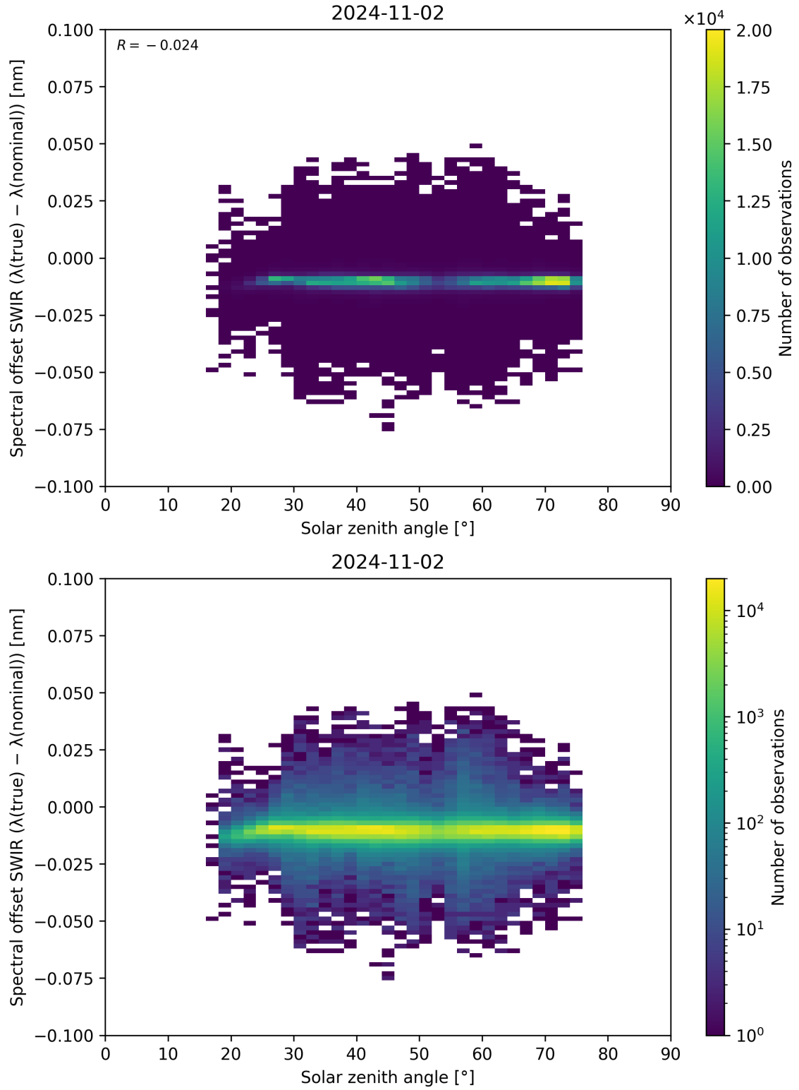
Figure 104: Scatter density plot of “Solar zenith angle” against “Spectral offset SWIR ( \lambda_{\text{true}} - \lambda_{\text{nominal}} )” for 2024-11-01 to 2024-11-03.
