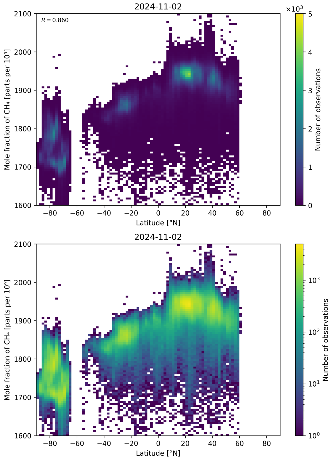
Figure 57: Scatter density plot of “Latitude” against “Mole fraction of CH 4 ” for 2024-11-01 to 2024-11-03.
