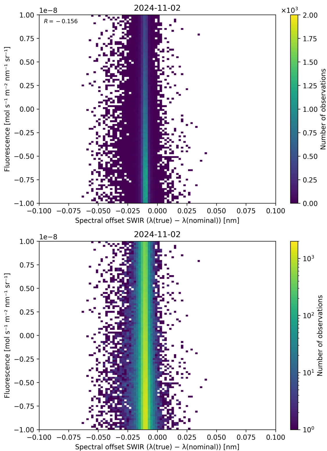
Figure 120: Scatter density plot of “Spectral offset SWIR ( \lambda_{\text{true}} - \lambda_{\text{nominal}} )” against “Fluorescence” for 2024-11-01 to 2024-11-03.
