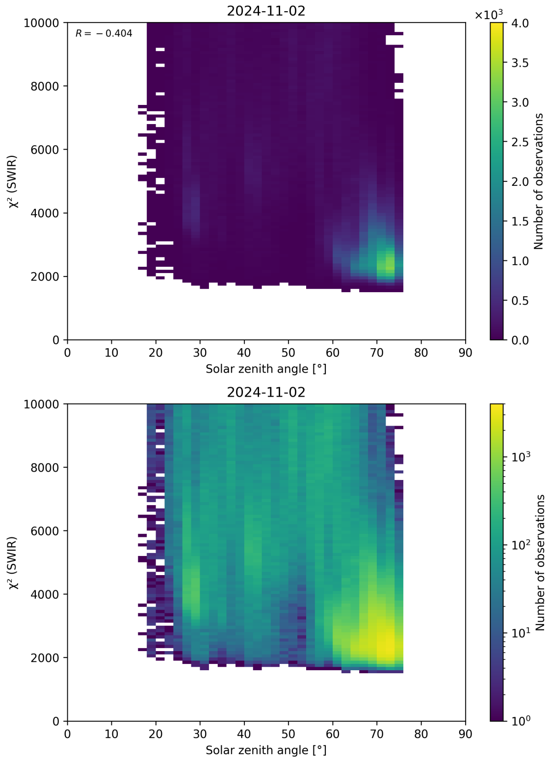
Figure 95: Scatter density plot of “Solar zenith angle” against “ \chi^2 (SWIR)” for 2024-11-01 to 2024-11-03.
