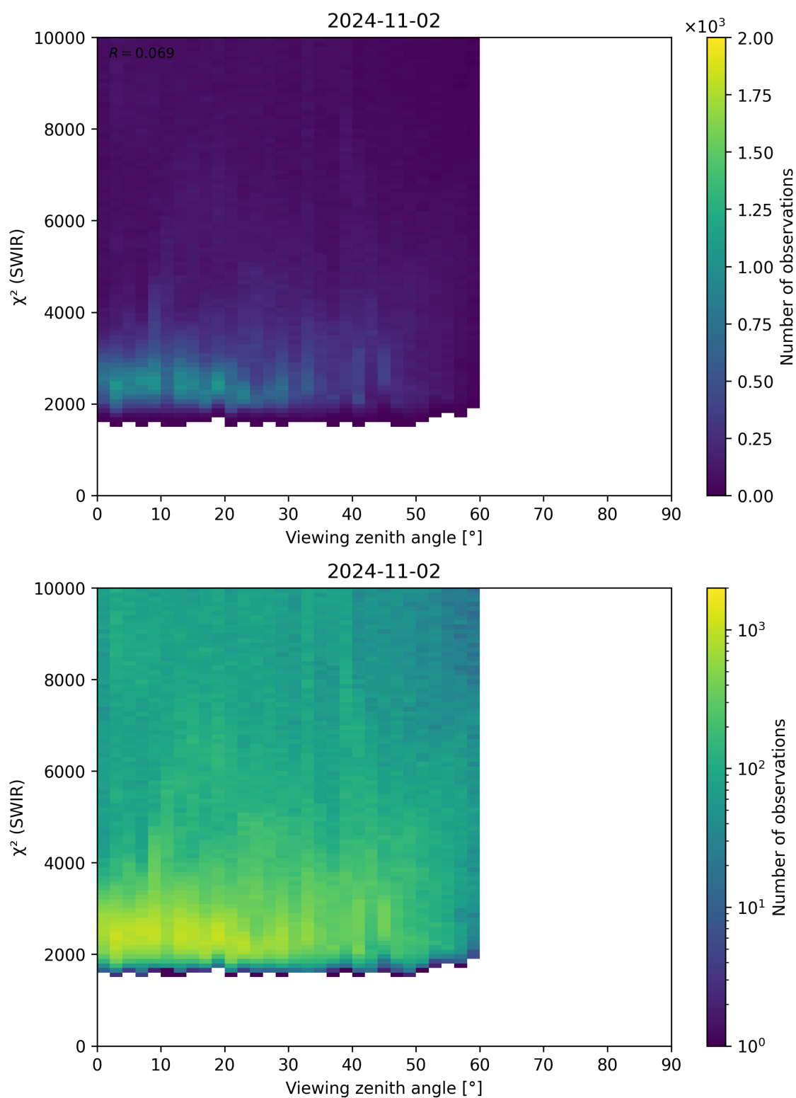
Figure 106: Scatter density plot of “Viewing zenith angle” against “ \chi^2 (SWIR)” for 2024-11-01 to 2024-11-03.
