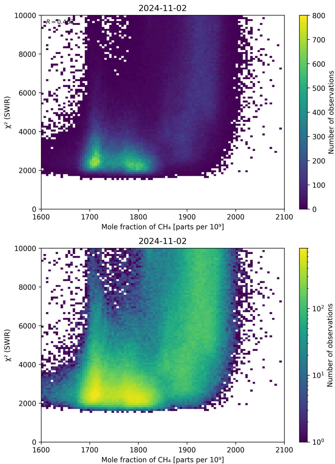
Figure 71: Scatter density plot of “Mole fraction of \text{CH}_4 ” against “ \chi^2 (SWIR)” for 2024-11-01 to 2024-11-03.
