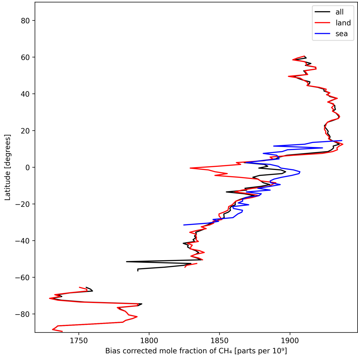
Figure 14: Zonal average of “Bias corrected mole fraction of CH 4 ” for 2024-11-01 to 2024-11-03.
