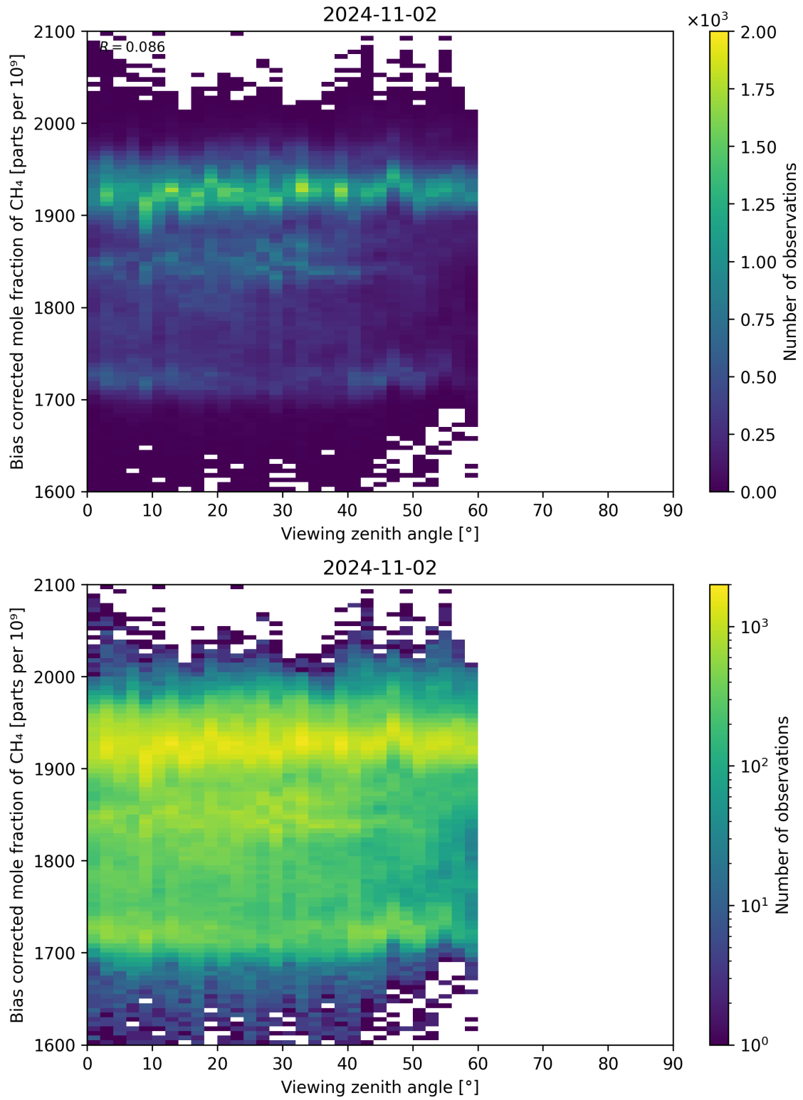
Figure 111: Scatter density plot of “Viewing zenith angle” against “Bias corrected mole fraction of CH 4 ” for 2024-11-01 to 2024-11-03.
