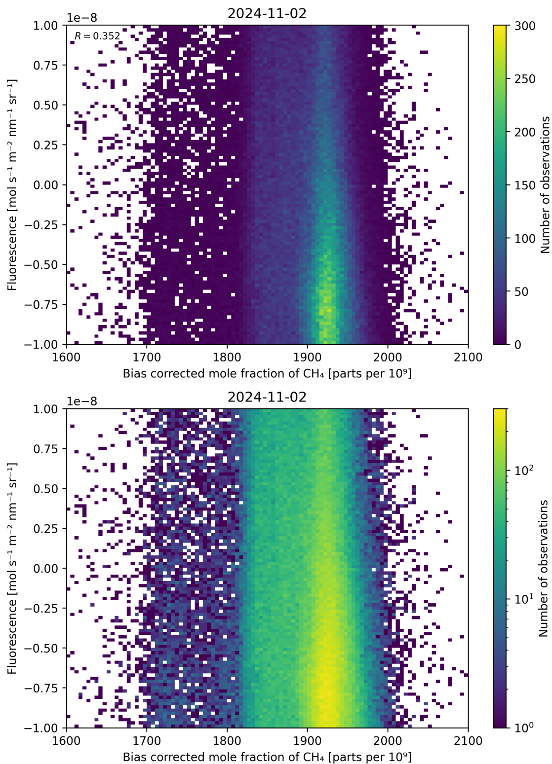
Figure 66: Scatter density plot of “Bias corrected mole fraction of \text{CH}_4 ” against “Fluorescence” for 2024-11-01 to 2024-11-03.
