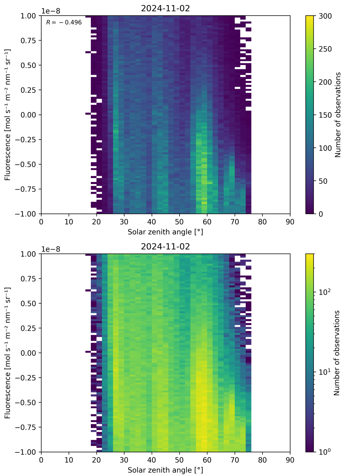
Figure 97: Scatter density plot of “Solar zenith angle” against “Fluorescence” for 2024-11-01 to 2024-11-03.
