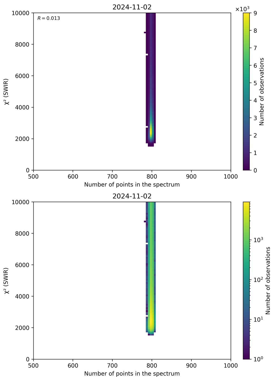
Figure 89: Scatter density plot of “Number of points in the spectrum” against “ \chi^2 (SWIR)” for 2024-11-01 to 2024-11-03.
