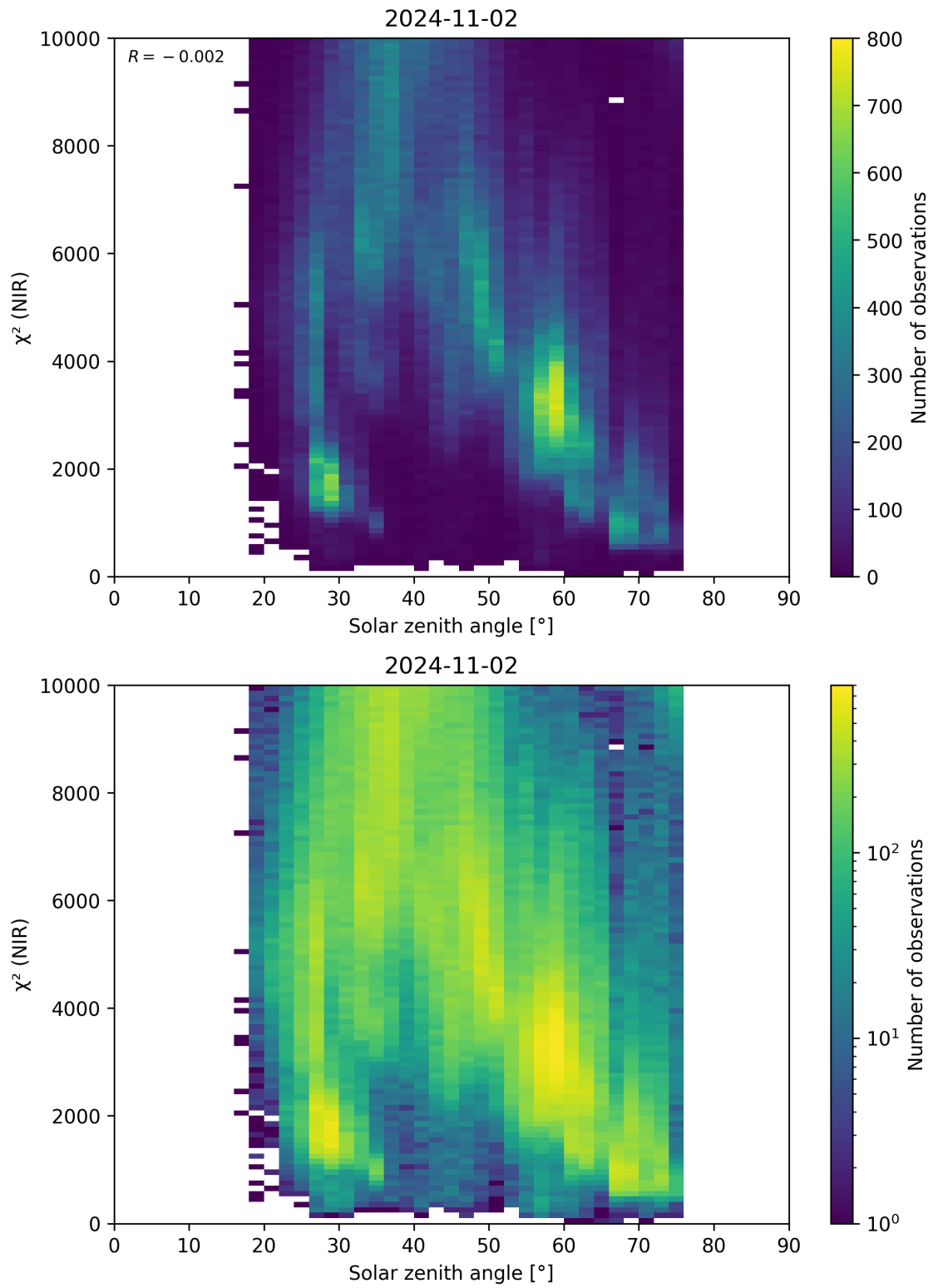
Figure 94: Scatter density plot of “Solar zenith angle” against “ \chi^2 (NIR)” for 2024-11-01 to 2024-11-03.
