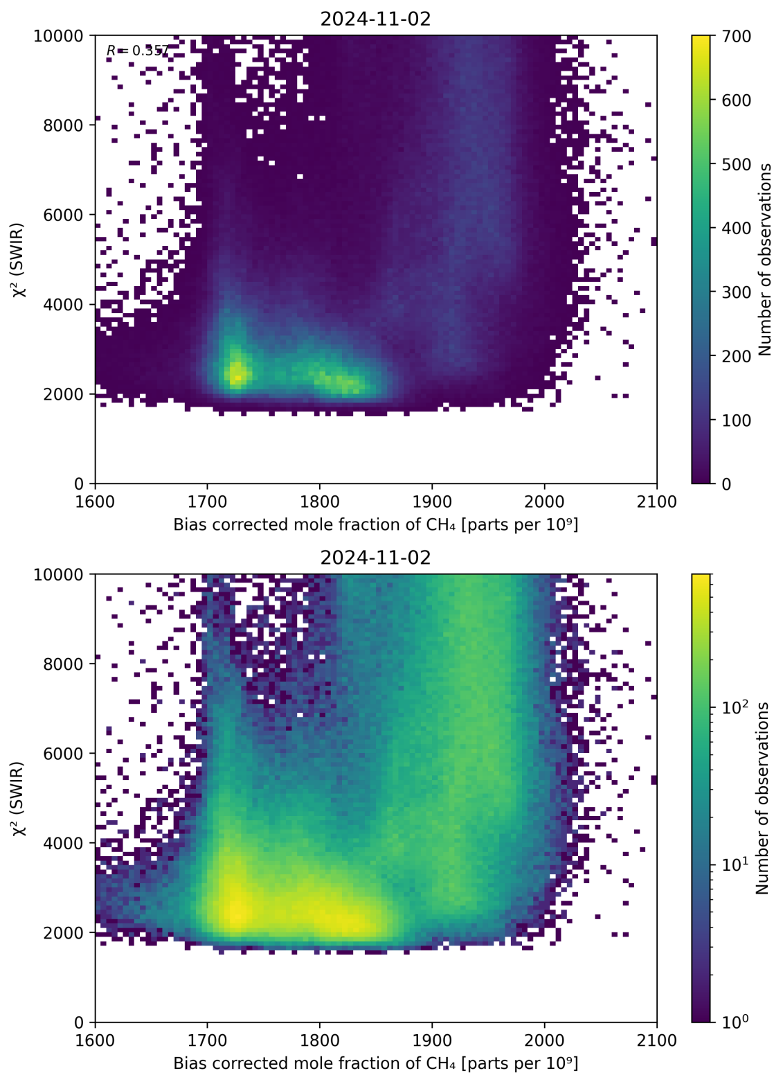
Figure 64: Scatter density plot of “Bias corrected mole fraction of \text{CH}_4 ” against “ \chi^2 (SWIR)” for 2024-11-01 to 2024-11-03.
