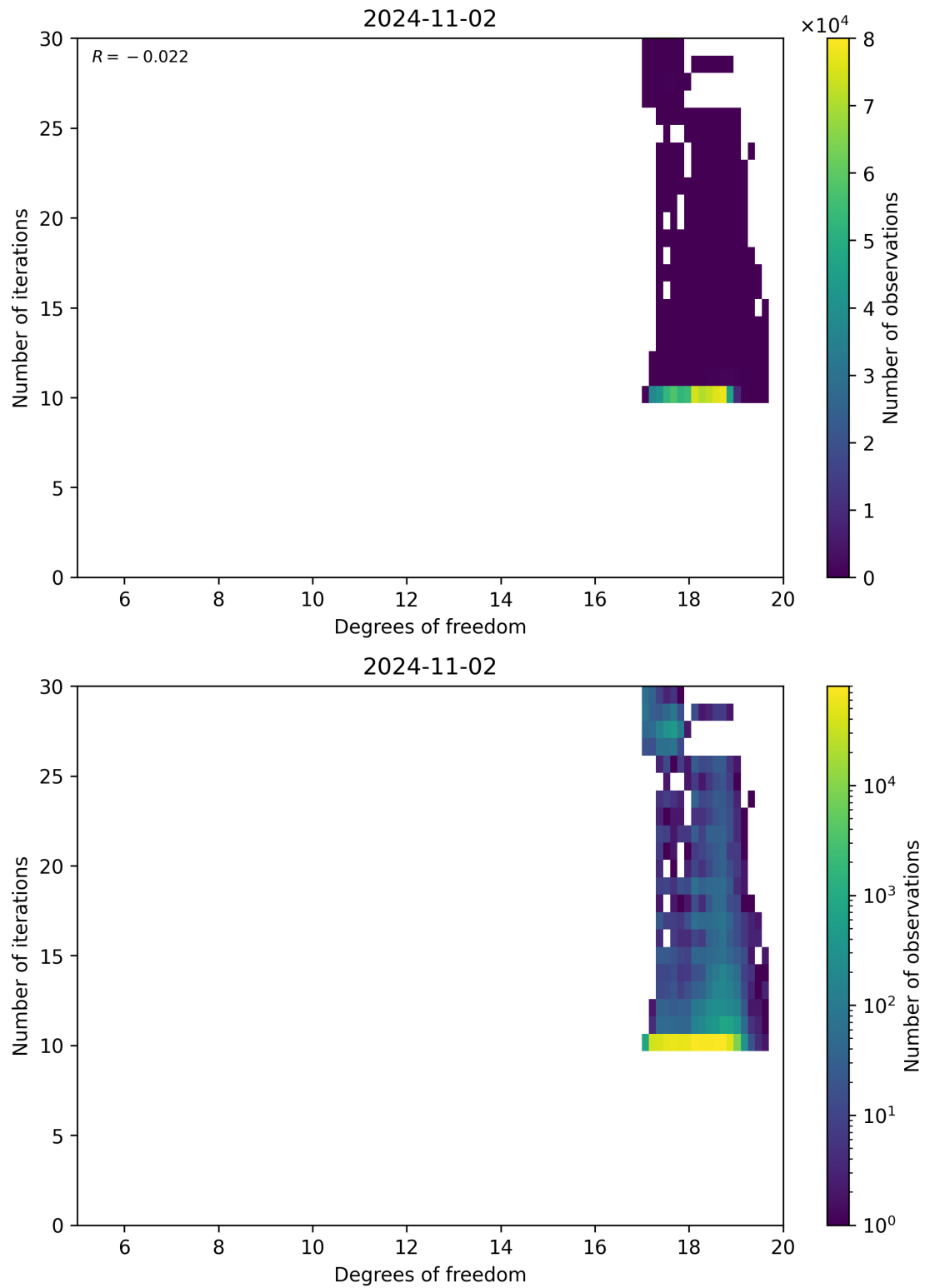
Figure 52: Scatter density plot of “Degrees of freedom” against “Number of iterations” for 2024-11-01 to 2024-11-03.
