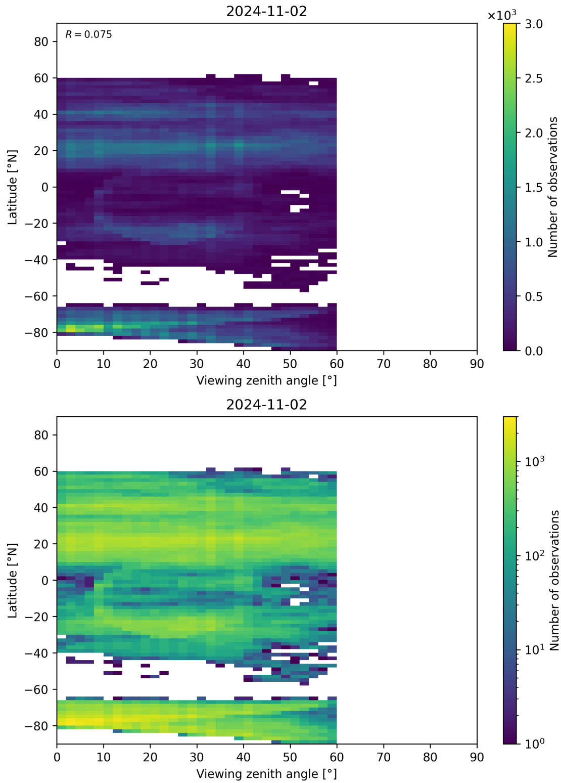
Figure 109: Scatter density plot of “Viewing zenith angle” against “Latitude” for 2024-11-01 to 2024-11-03.
