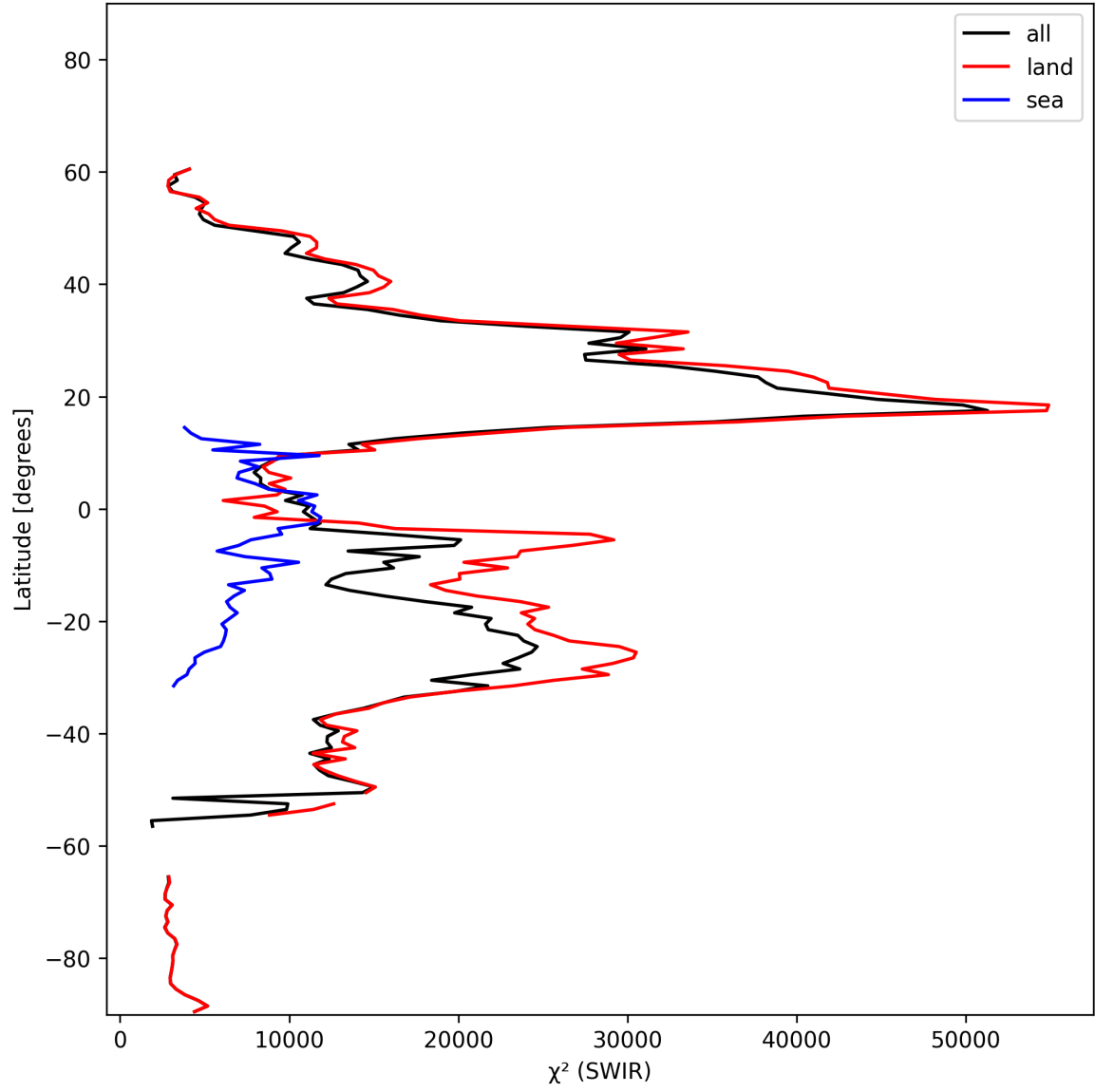
Figure 17: Zonal average of “ \chi^2 (SWIR)” for 2024-11-01 to 2024-11-03.
