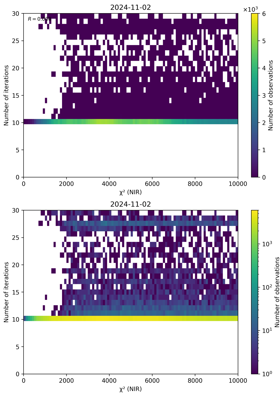
Figure 46: Scatter density plot of “ \chi^2 (NIR)” against “Number of iterations” for 2024-11-01 to 2024-11-03.
