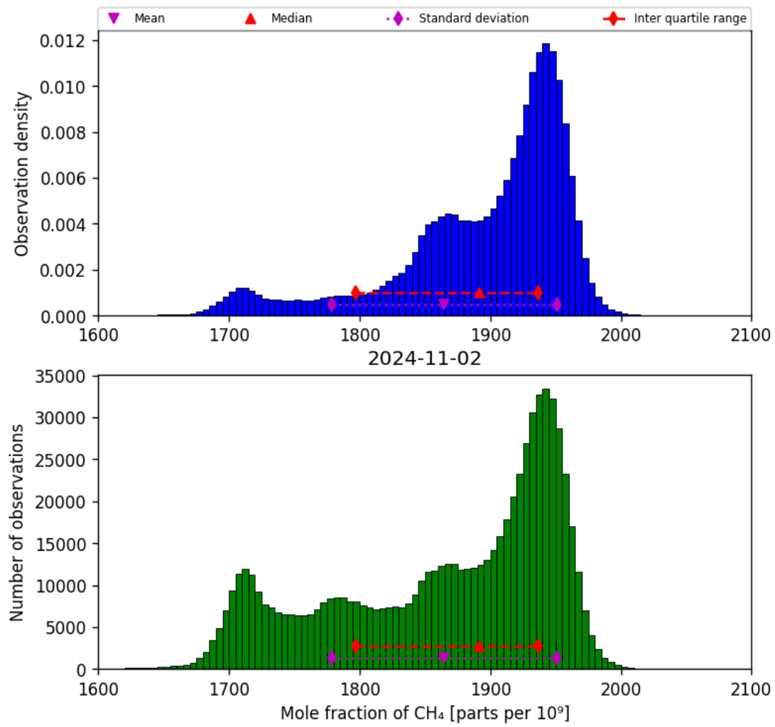
Figure 23: Histogram of “Mole fraction of CH 4 ” for 2024-11-01 to 2024-11-03
