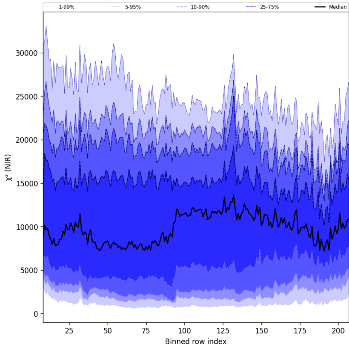
Figure 40: Along track statistics of “ \chi^2 (NIR)” for 2024-11-01 to 2024-11-03
