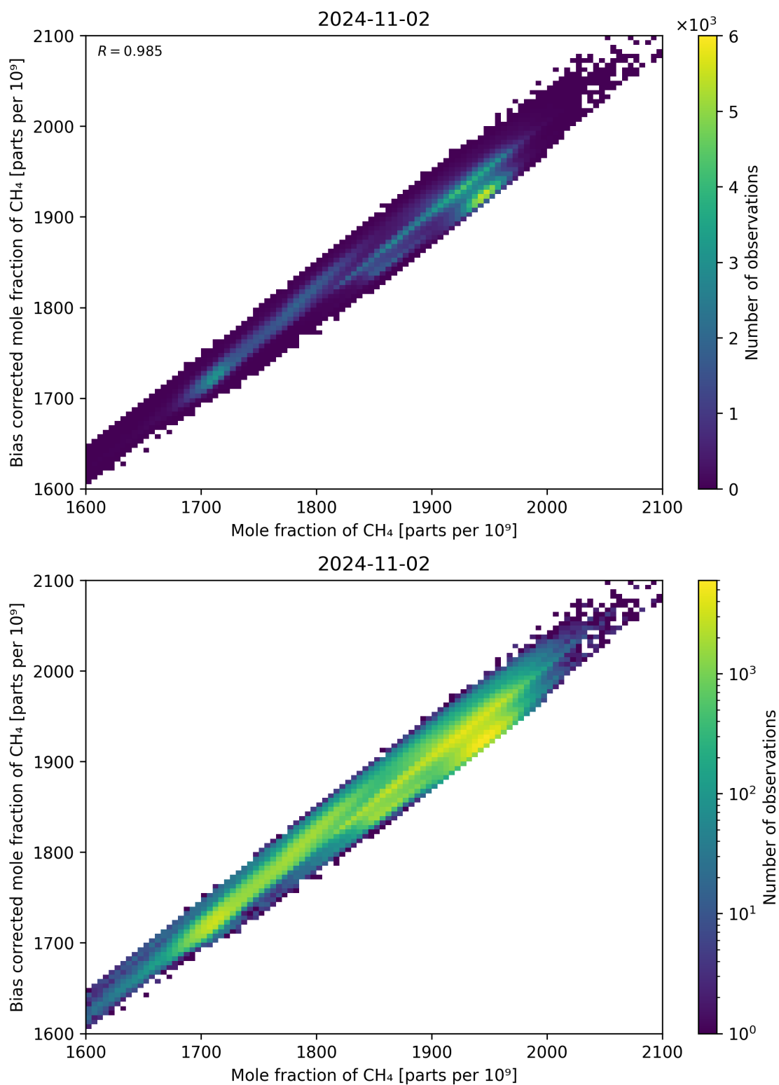
Figure 74: Scatter density plot of “Mole fraction of CH 4 ” against “Bias corrected mole fraction of CH 4 ” for 2024-11-01 to 2024-11-03.
