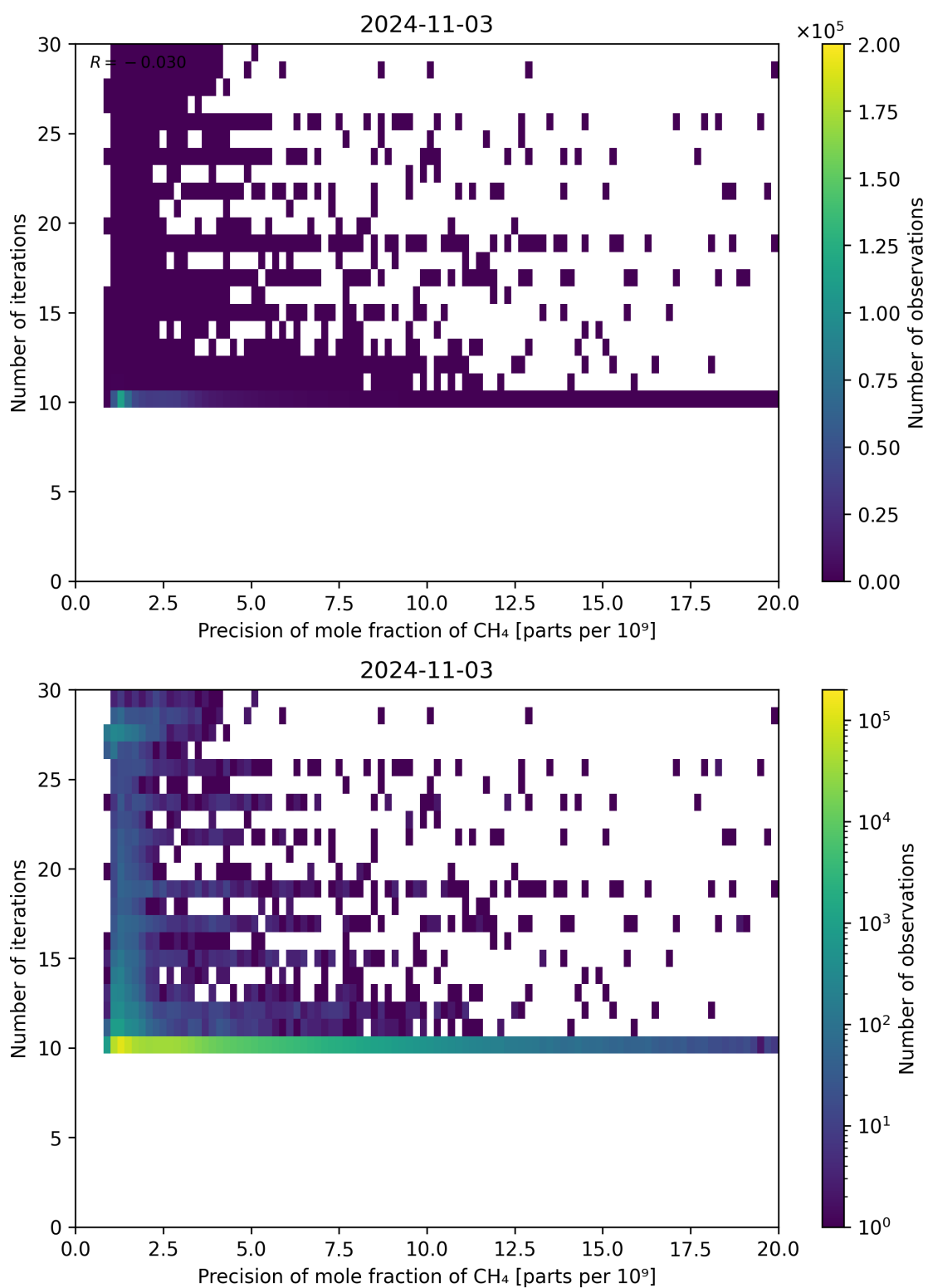
Figure 83: Scatter density plot of “Precision of mole fraction of CH 4 ” against “Number of iterations” for 2024-11-02 to 2024-11-04.
