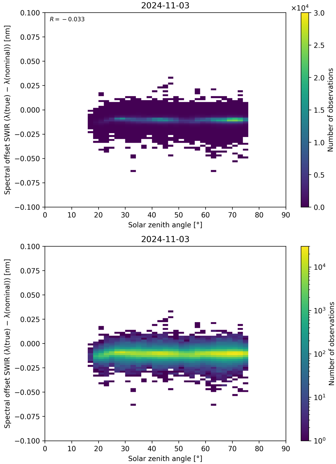
Figure 104: Scatter density plot of “Solar zenith angle” against “Spectral offset SWIR ( \lambda_{\text{true}} - \lambda_{\text{nominal}} )” for 2024-11-02 to 2024-11-04.
