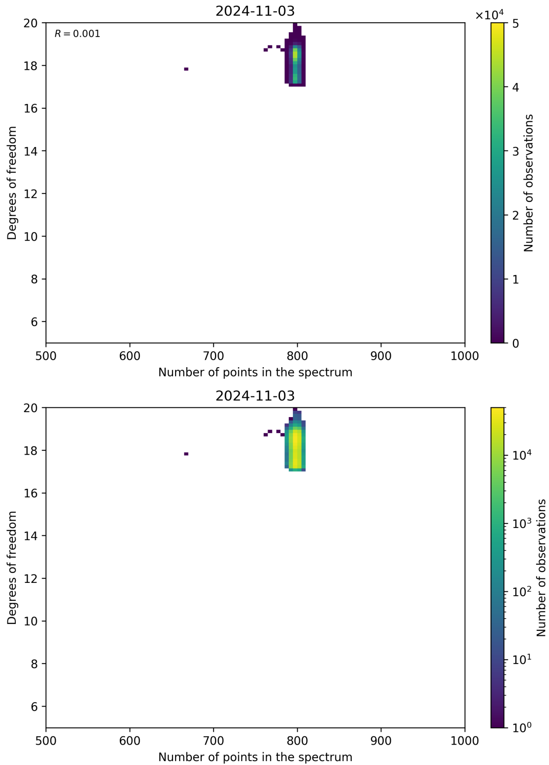
Figure 90: Scatter density plot of “Number of points in the spectrum” against “Degrees of freedom” for 2024-11-02 to 2024-11-04.
