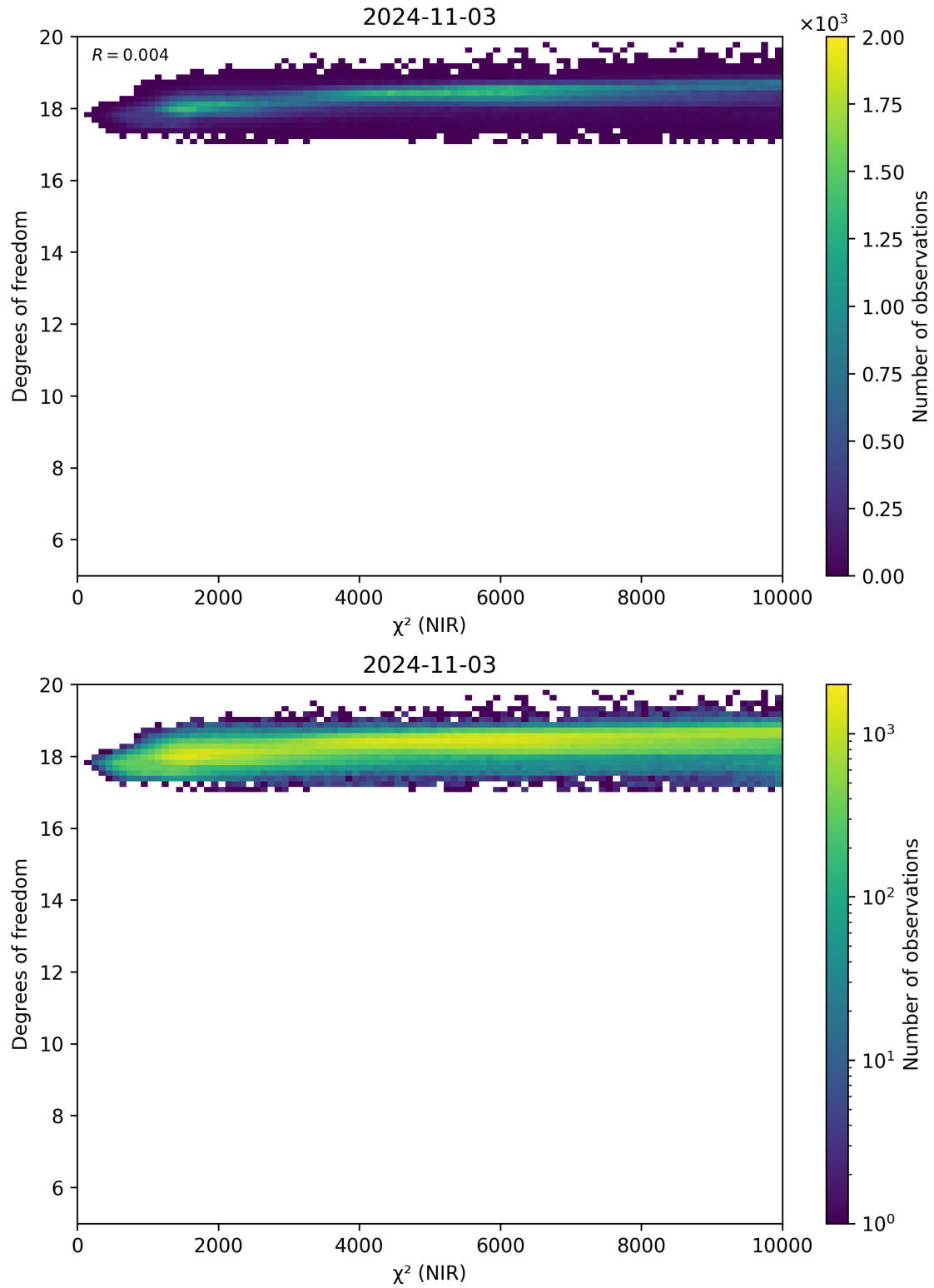
Figure 44: Scatter density plot of “ \chi^2 (NIR)” against “Degrees of freedom” for 2024-11-02 to 2024-11-04.
