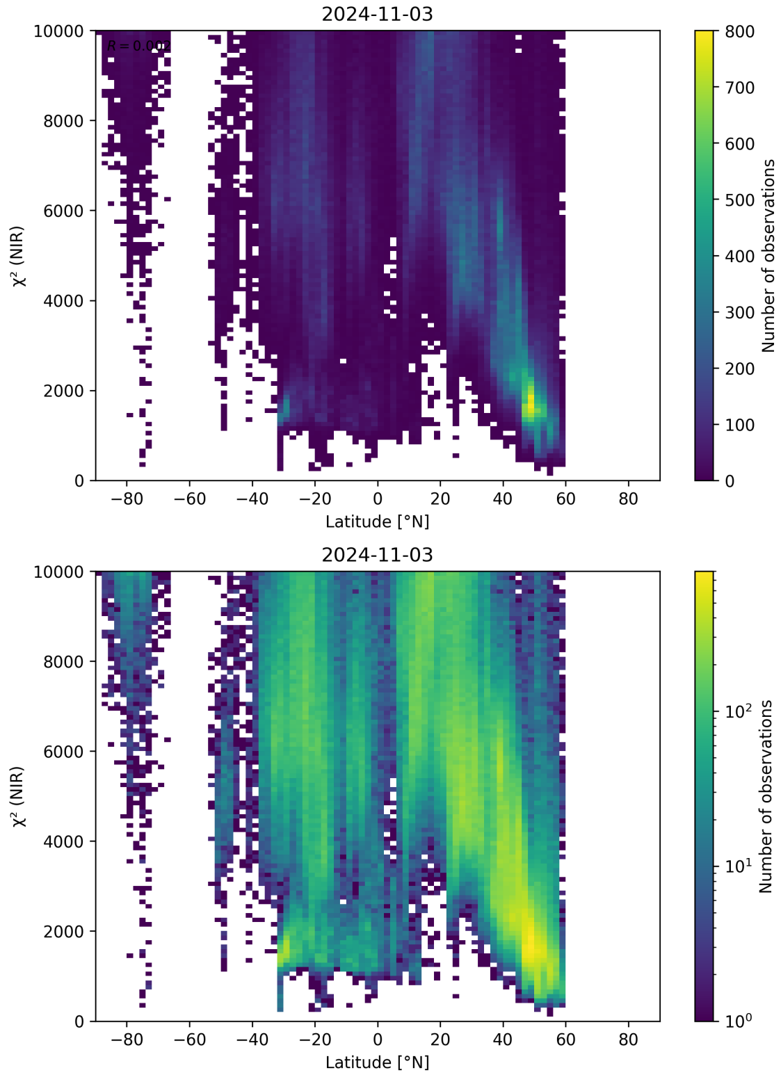
Figure 53: Scatter density plot of “Latitude” against “ \chi^2 (NIR)” for 2024-11-02 to 2024-11-04.
