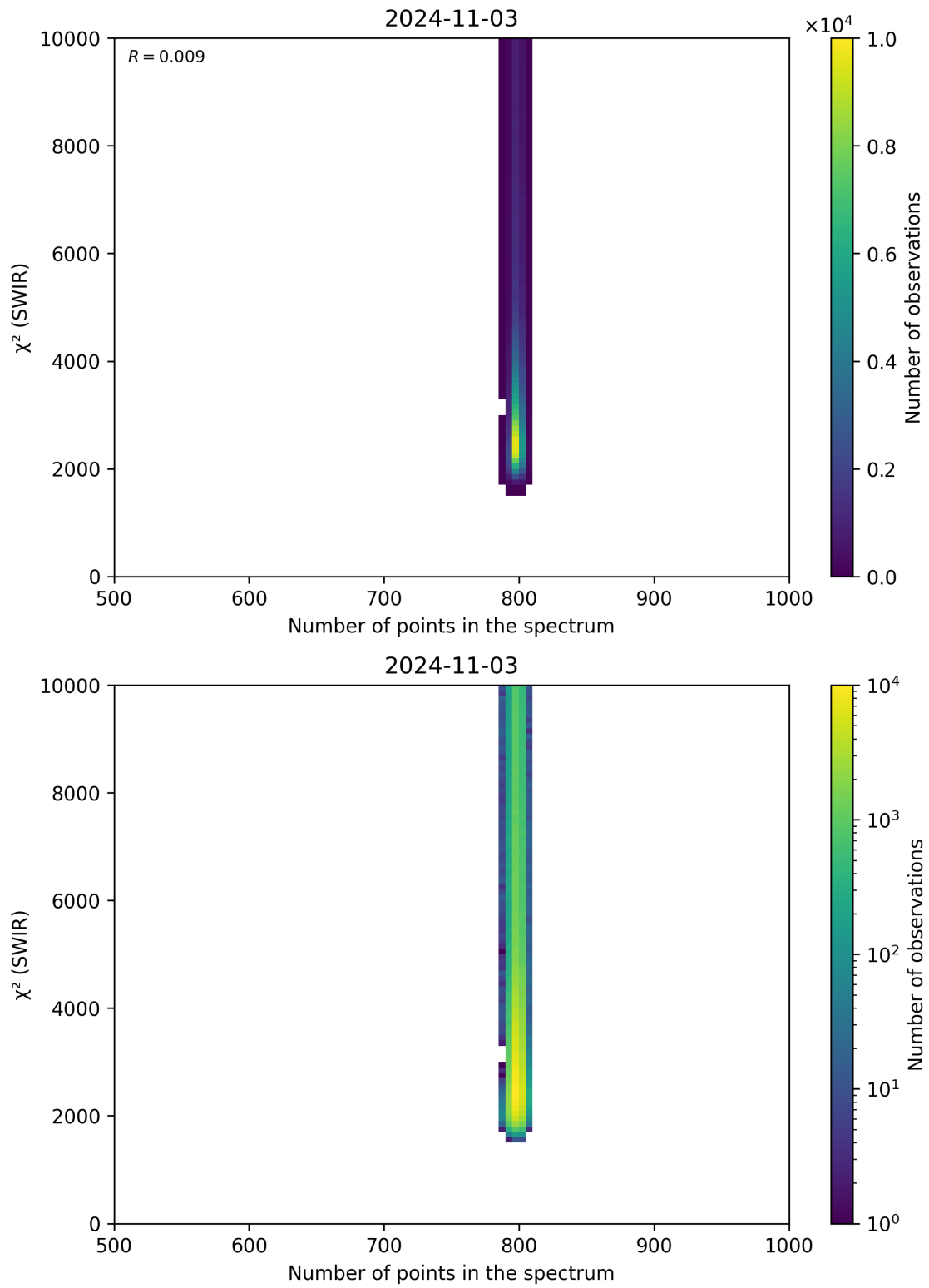
Figure 89: Scatter density plot of “Number of points in the spectrum” against “ \chi^2 (SWIR)” for 2024-11-02 to 2024-11-04.
