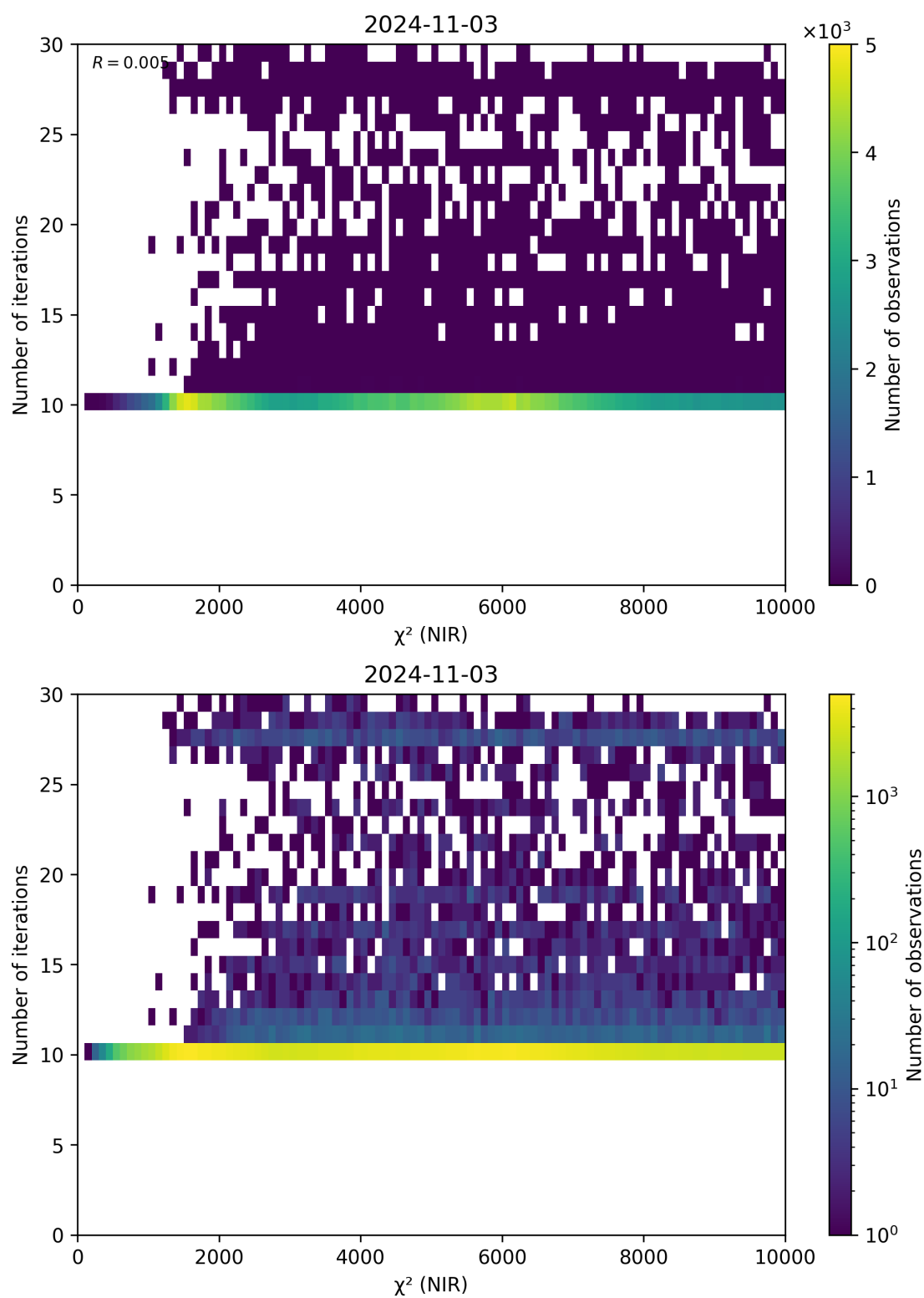
Figure 46: Scatter density plot of “ \chi^2 (NIR)” against “Number of iterations” for 2024-11-02 to 2024-11-04.
