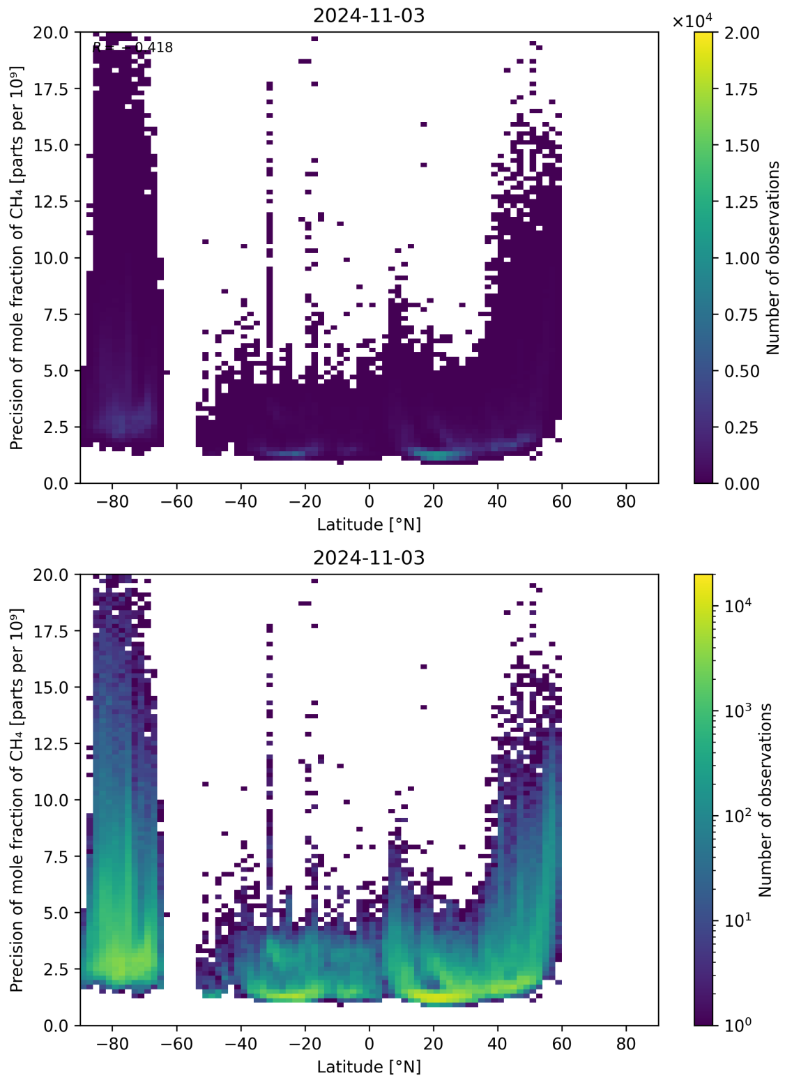
Figure 59: Scatter density plot of “Latitude” against “Precision of mole fraction of CH 4 ” for 2024-11-02 to 2024-11-04.
