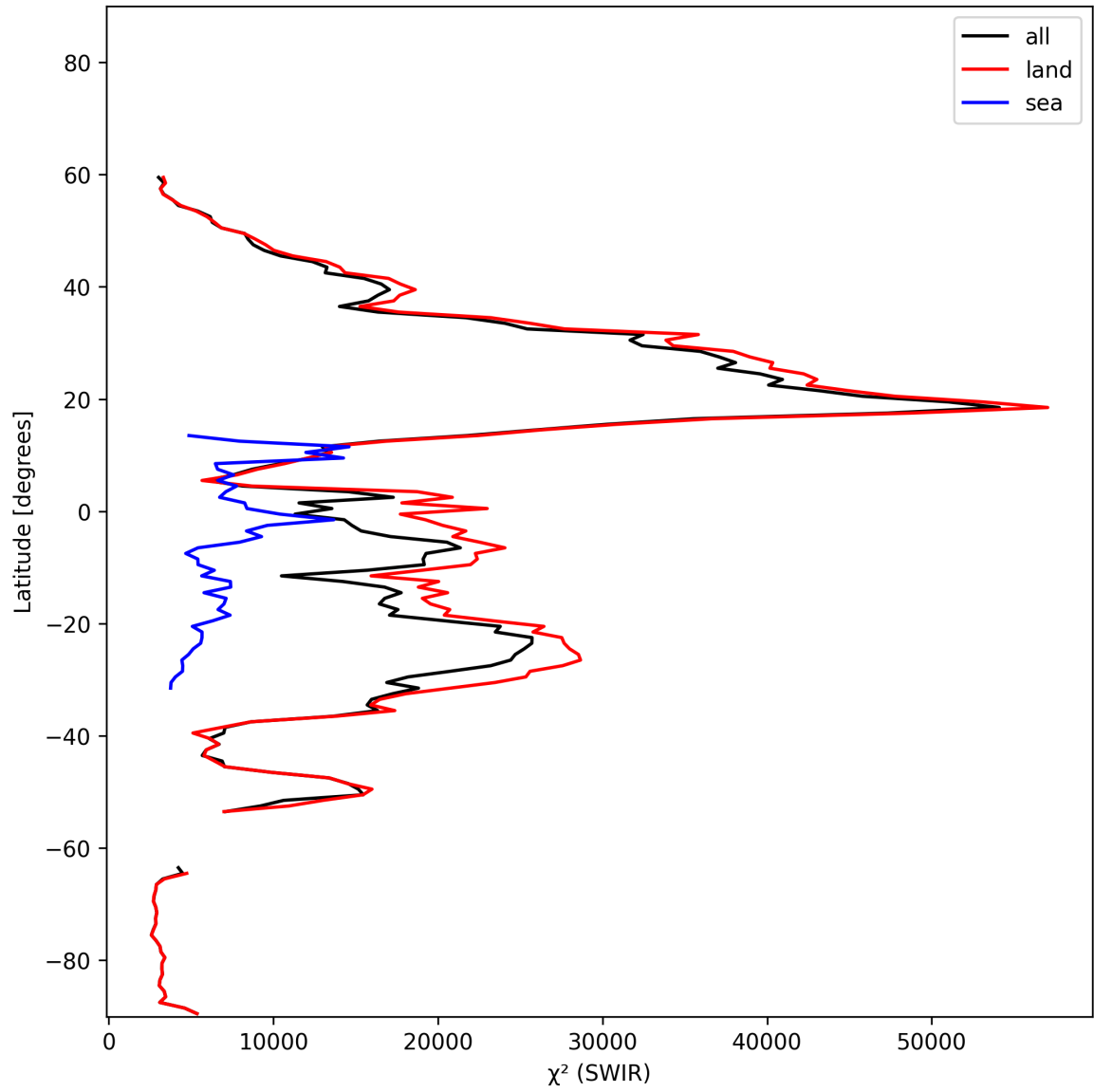
Figure 17: Zonal average of “ \chi^2 (SWIR)” for 2024-11-02 to 2024-11-04.
