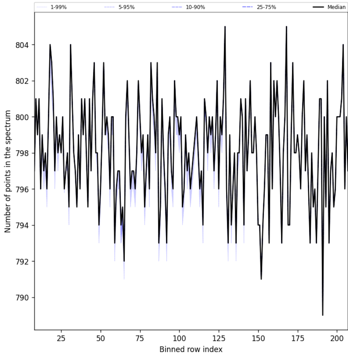
Figure 37: Along track statistics of “Number of points in the spectrum” for 2024-11-02 to 2024-11-04
