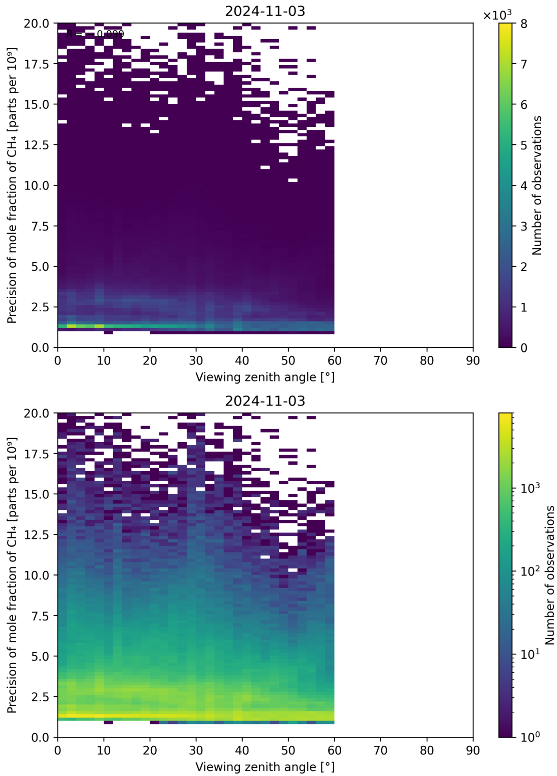
Figure 112: Scatter density plot of “Viewing zenith angle” against “Precision of mole fraction of CH 4 ” for 2024-11-02 to 2024-11-04.
