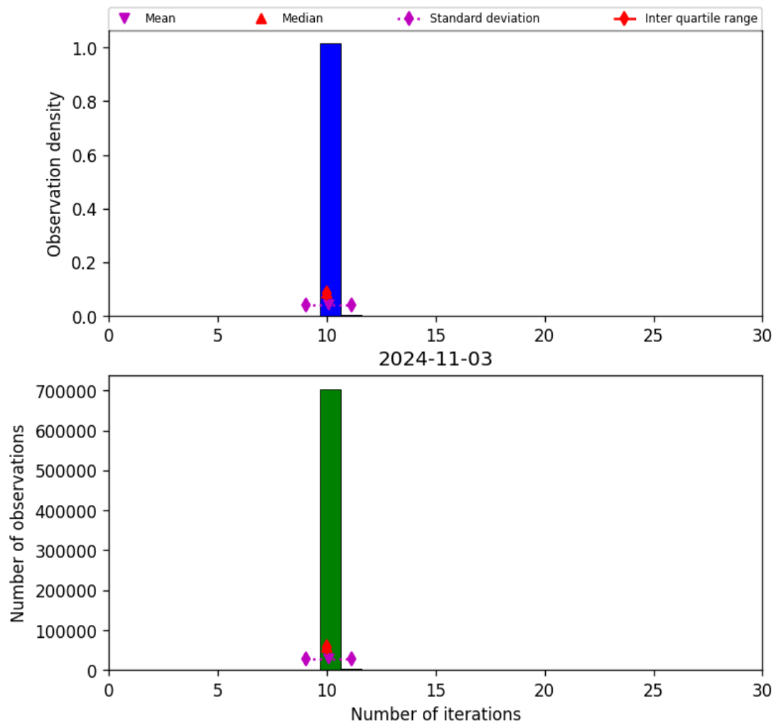
Figure 31: Histogram of “Number of iterations” for 2024-11-02 to 2024-11-04
