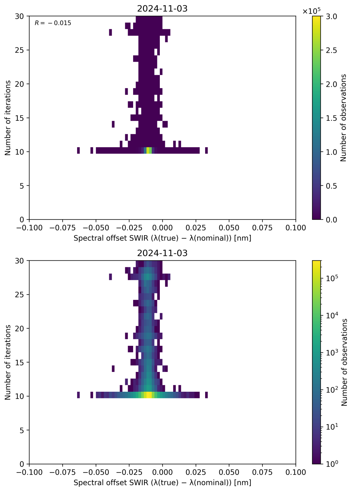
Figure 121: Scatter density plot of “Spectral offset SWIR ( \lambda_{\text{true}} - \lambda_{\text{nominal}} )” against “Number of iterations” for 2024-11-02 to 2024-11-04.
