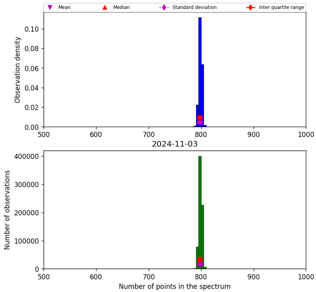
Figure 26: Histogram of “Number of points in the spectrum” for 2024-11-02 to 2024-11-04
