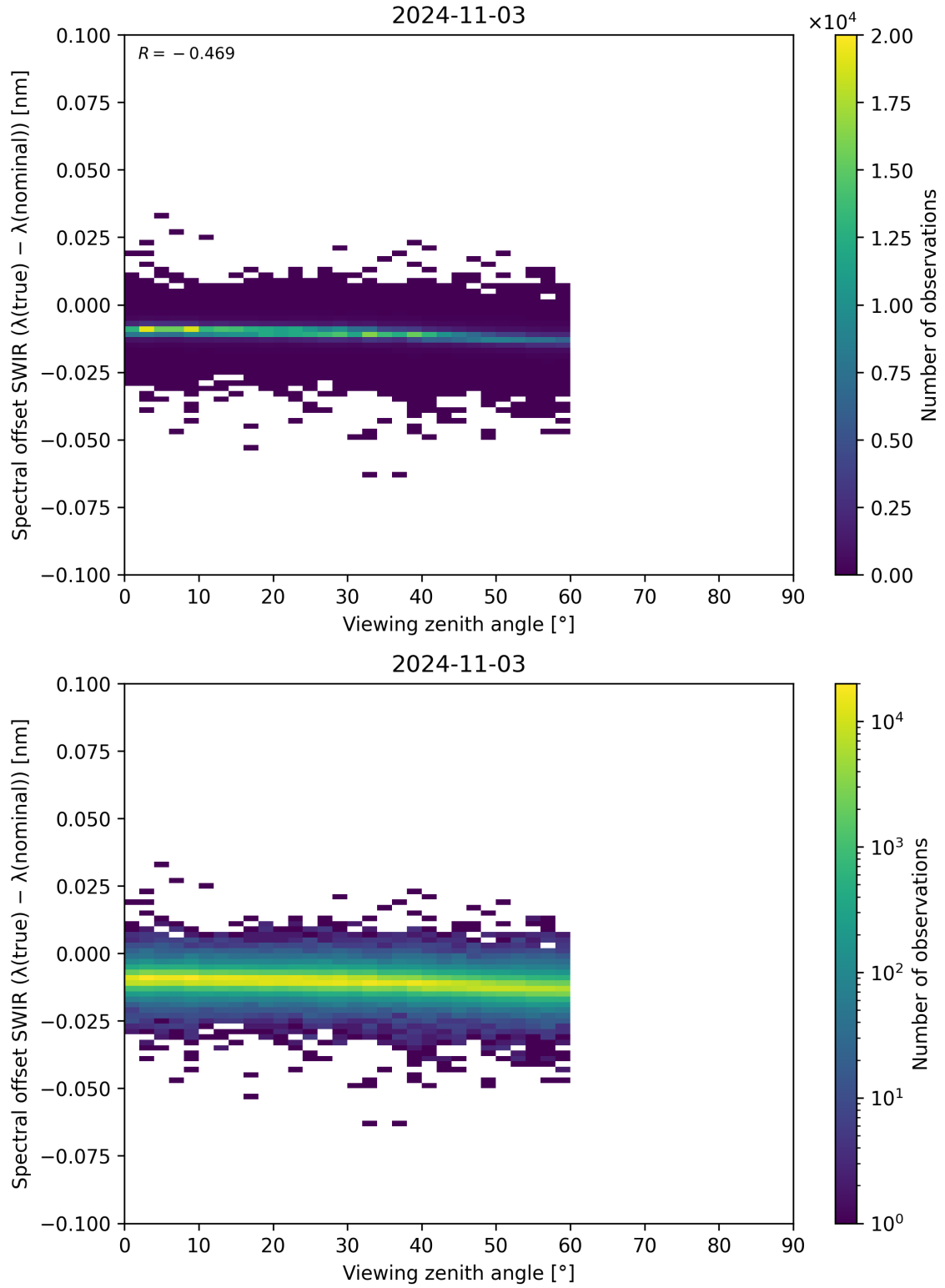
Figure 116: Scatter density plot of “Viewing zenith angle” against “Spectral offset SWIR ( \lambda_{\text{true}} - \lambda_{\text{nominal}} )” for 2024-11-02 to 2024-11-04.
