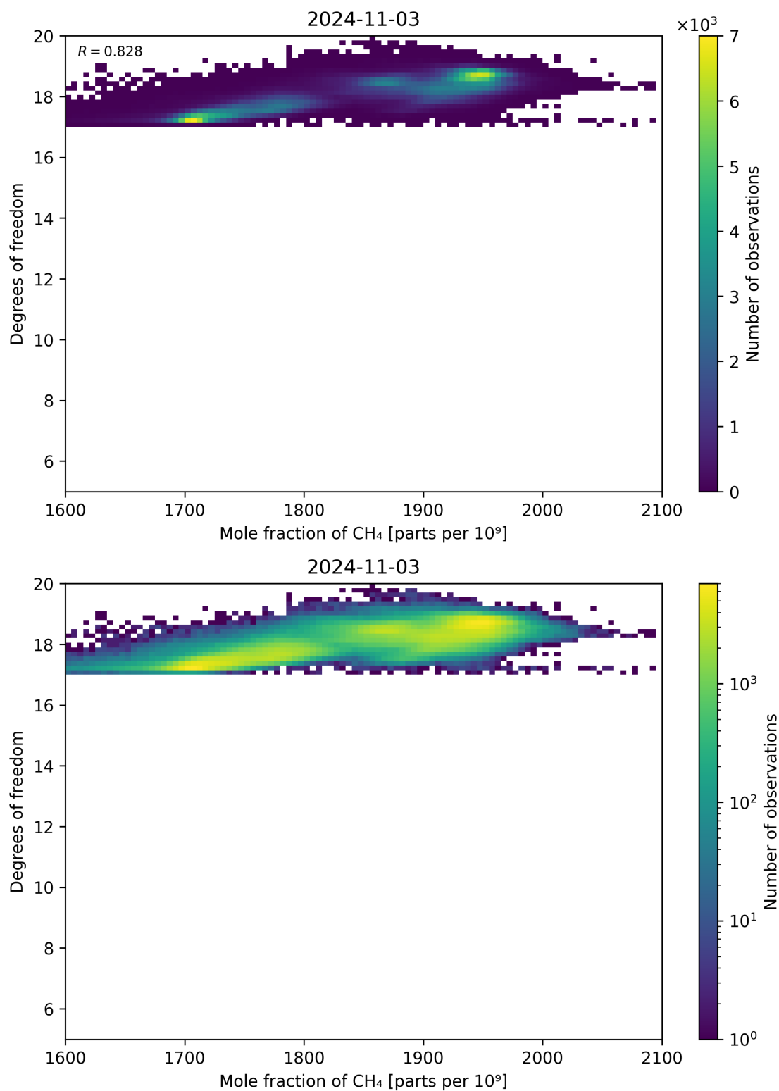
Figure 72: Scatter density plot of “Mole fraction of CH 4 ” against “Degrees of freedom” for 2024-11-02 to 2024-11-04.
