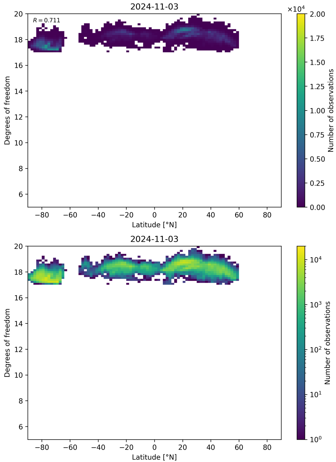
Figure 55: Scatter density plot of “Latitude” against “Degrees of freedom” for 2024-11-02 to 2024-11-04.
