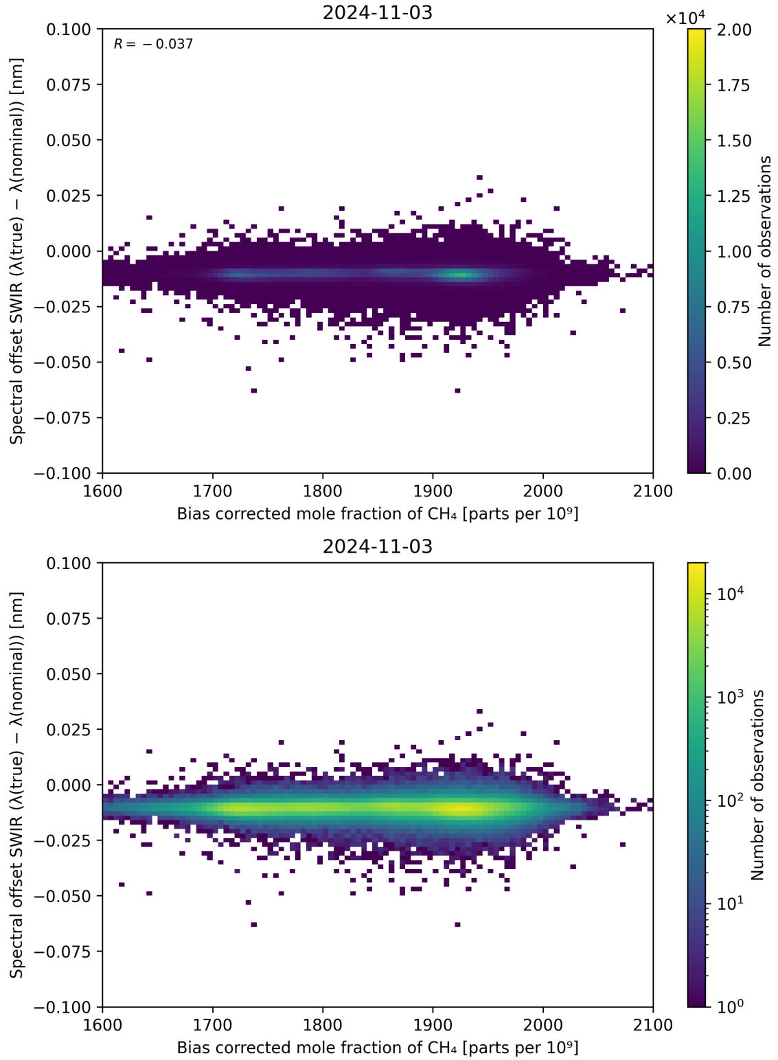
Figure 69: Scatter density plot of “Bias corrected mole fraction of CH 4 ” against “Spectral offset SWIR ( \lambda_{\text{true}} - \lambda_{\text{nominal}} )” for 2024-11-02 to 2024-11-04.
