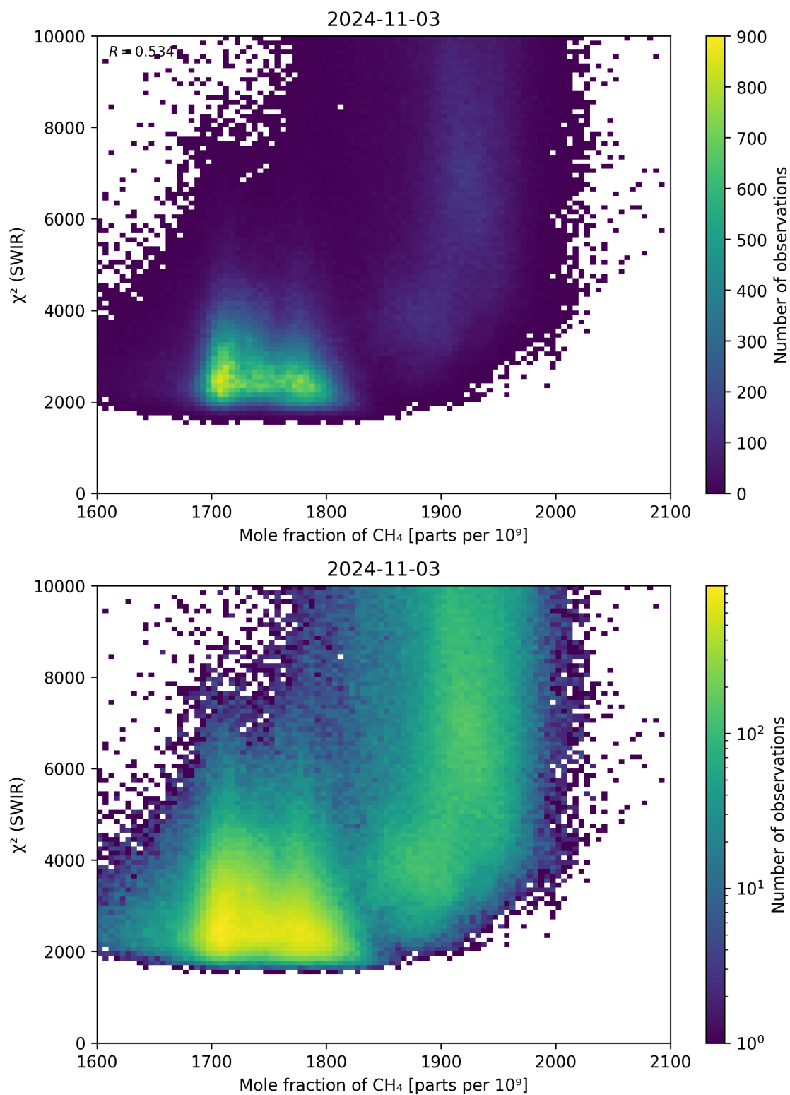
Figure 71: Scatter density plot of “Mole fraction of \text{CH}_4 ” against “ \chi^2 (SWIR)” for 2024-11-02 to 2024-11-04.
