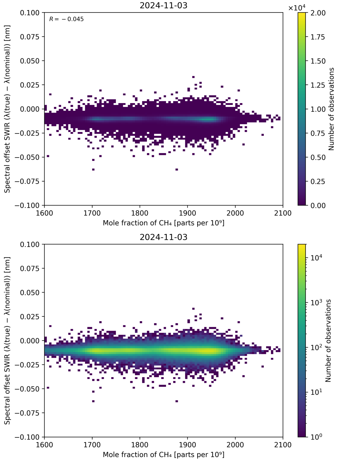
Figure 86: Scatter density plot of “Mole fraction of \text{CH}_4 ” against “Spectral offset SWIR ( \lambda_{\text{true}} - \lambda_{\text{nominal}} )” for 2024-11-02 to 2024-11-04.
