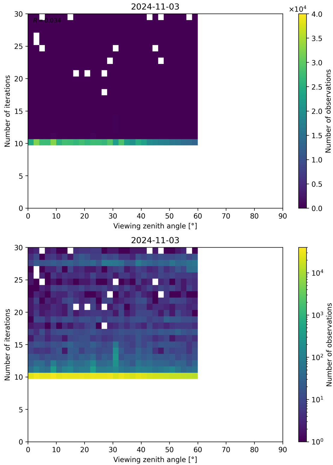
Figure 113: Scatter density plot of “Viewing zenith angle” against “Number of iterations” for 2024-11-02 to 2024-11-04.
