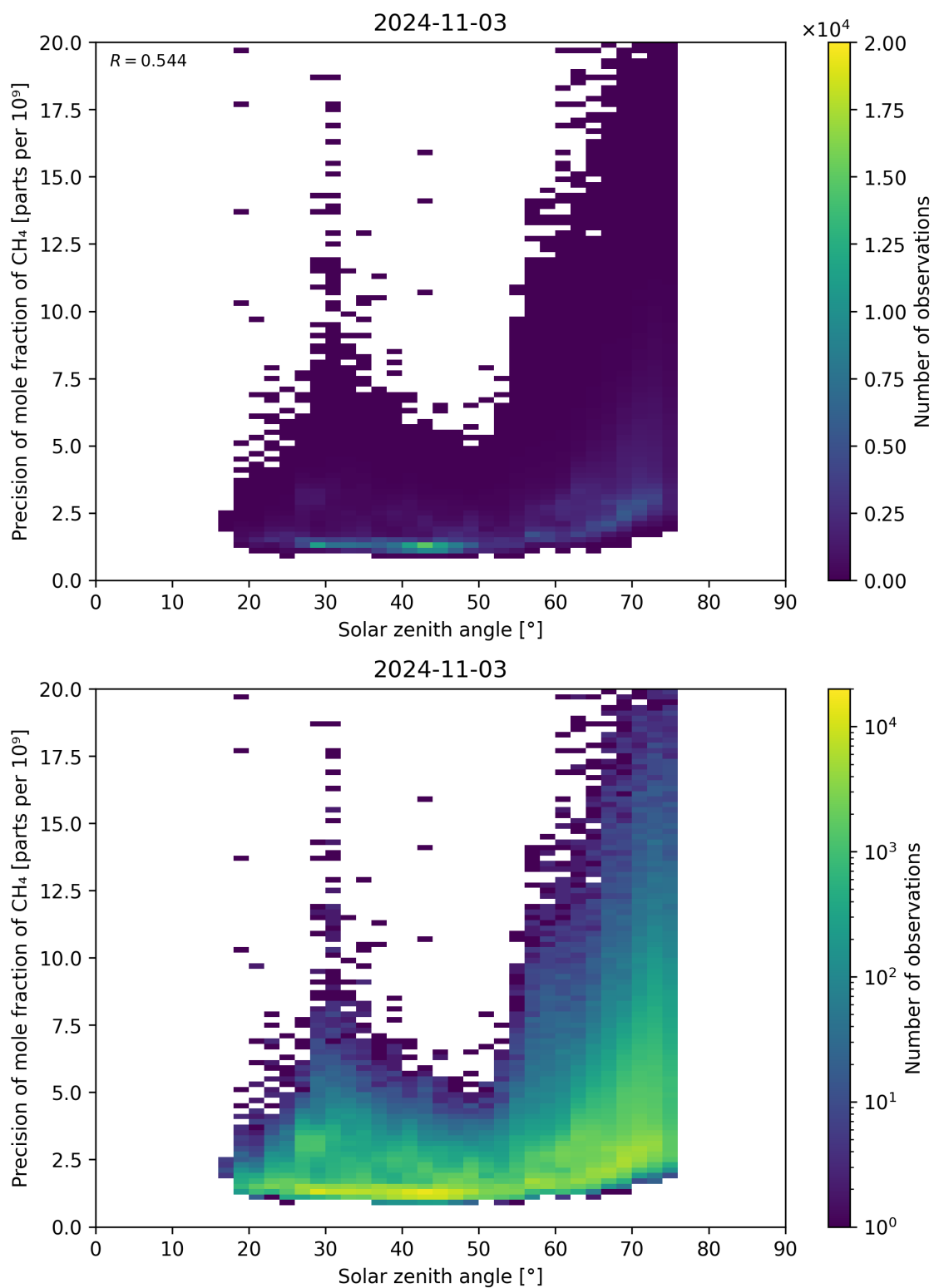
Figure 101: Scatter density plot of “Solar zenith angle” against “Precision of mole fraction of \text{CH}_4 ” for 2024-11-02 to 2024-11-04.
