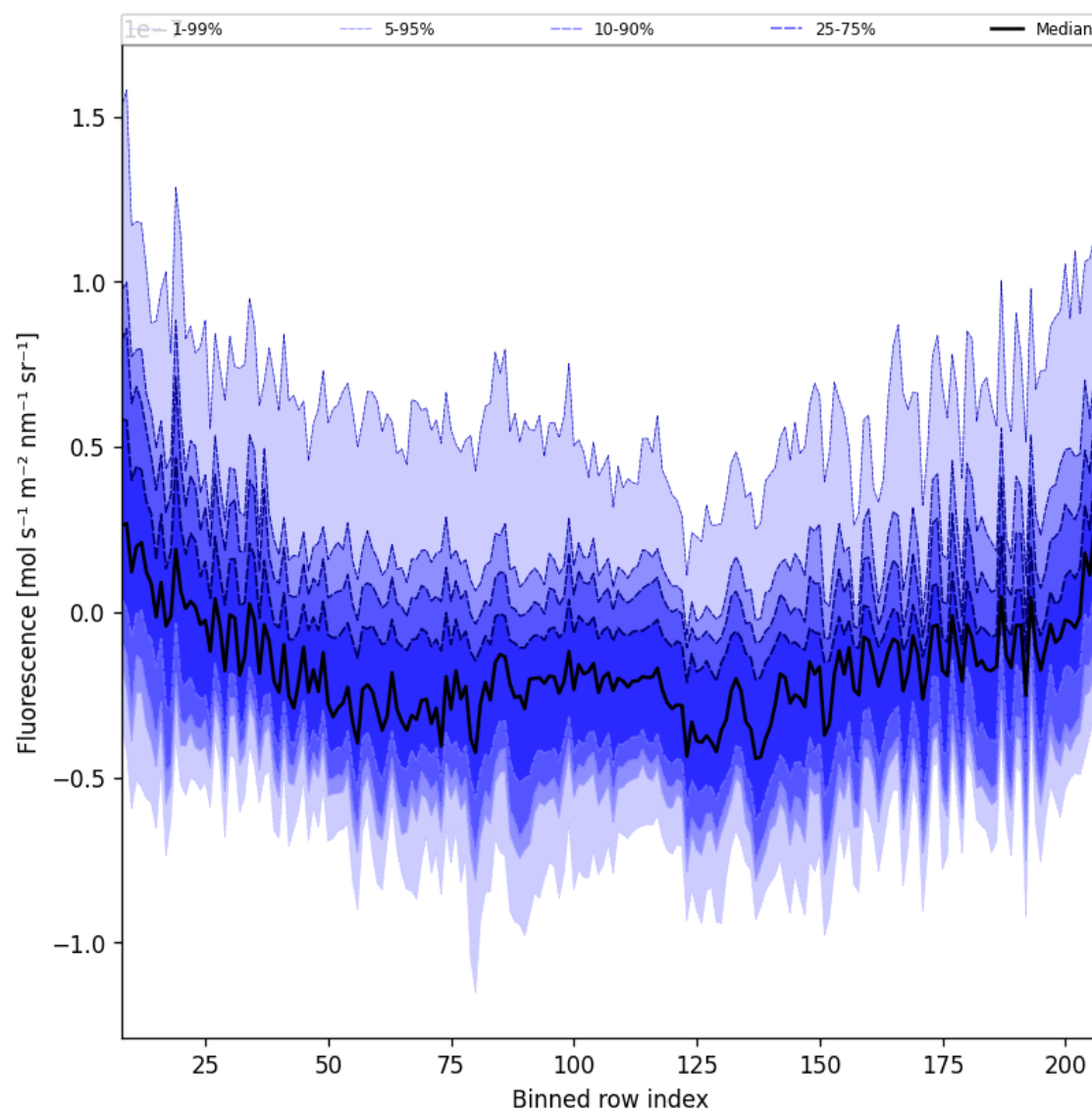
Figure 43: Along track statistics of “Fluorescence” for 2024-11-02 to 2024-11-04
