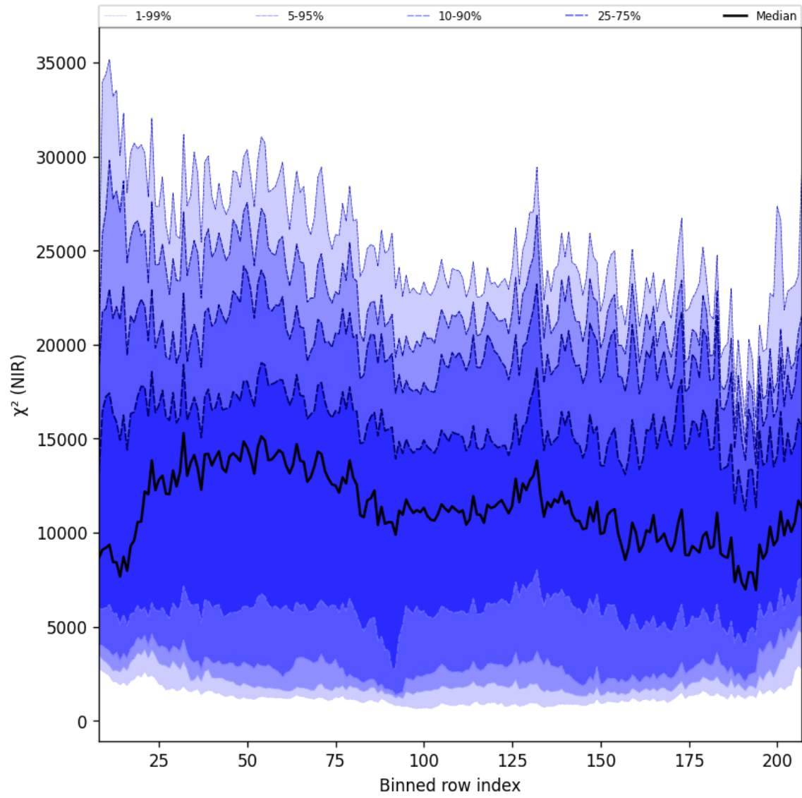
Figure 40: Along track statistics of “ \chi^2 (NIR)” for 2024-11-02 to 2024-11-04
