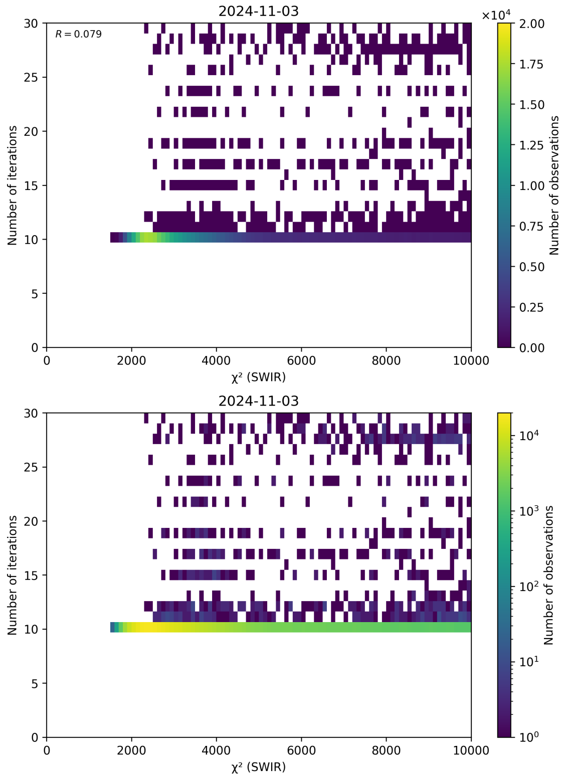
Figure 50: Scatter density plot of “ \chi^2 (SWIR)” against “Number of iterations” for 2024-11-02 to 2024-11-04.
