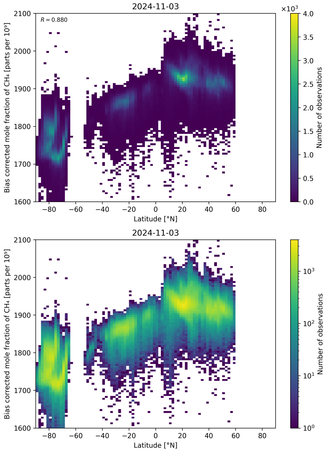
Figure 58: Scatter density plot of “Latitude” against “Bias corrected mole fraction of \text{CH}_4 ” for 2024-11-02 to 2024-11-04.
