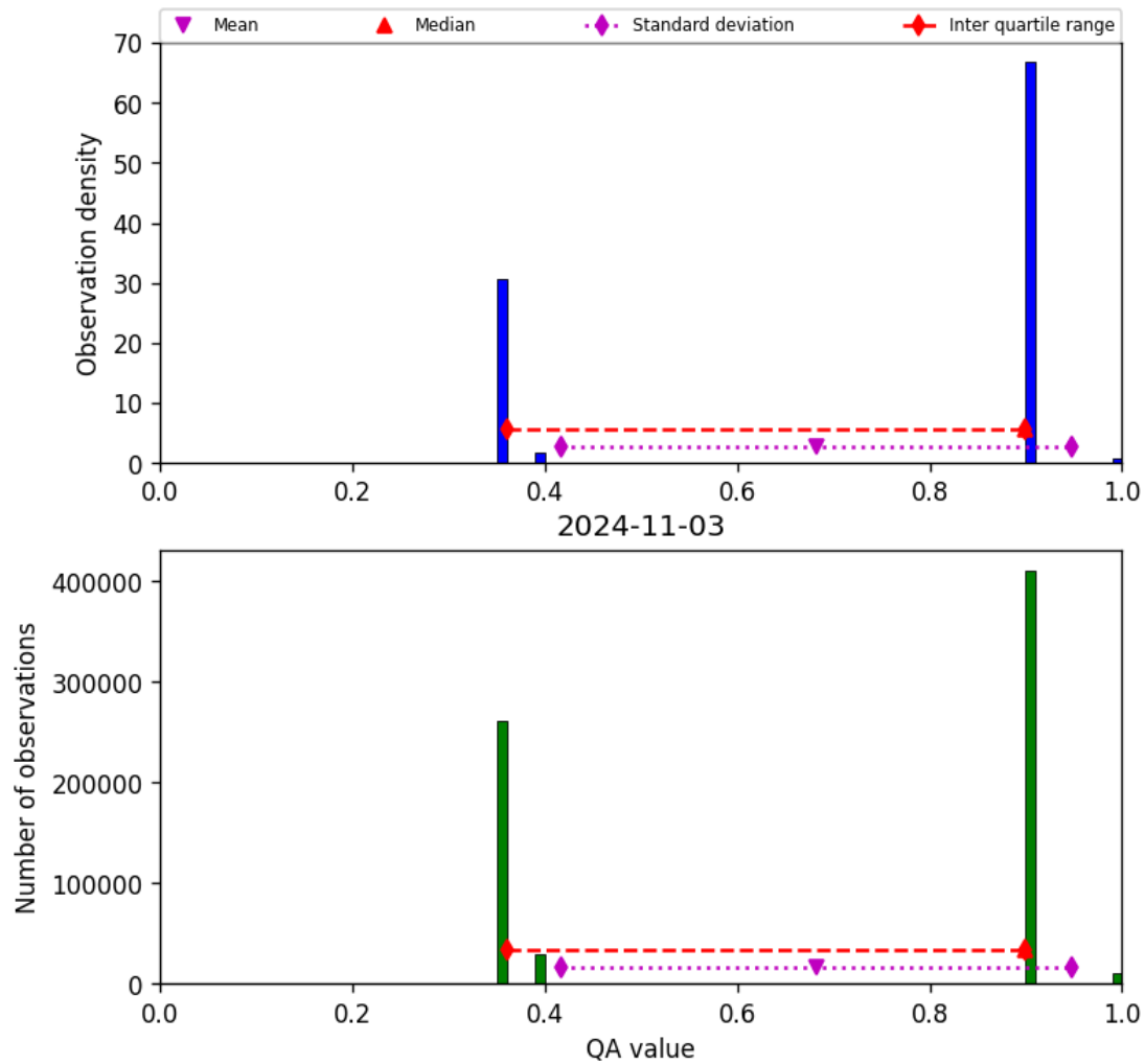
Figure 22: Histogram of “QA value” for 2024-11-02 to 2024-11-04
