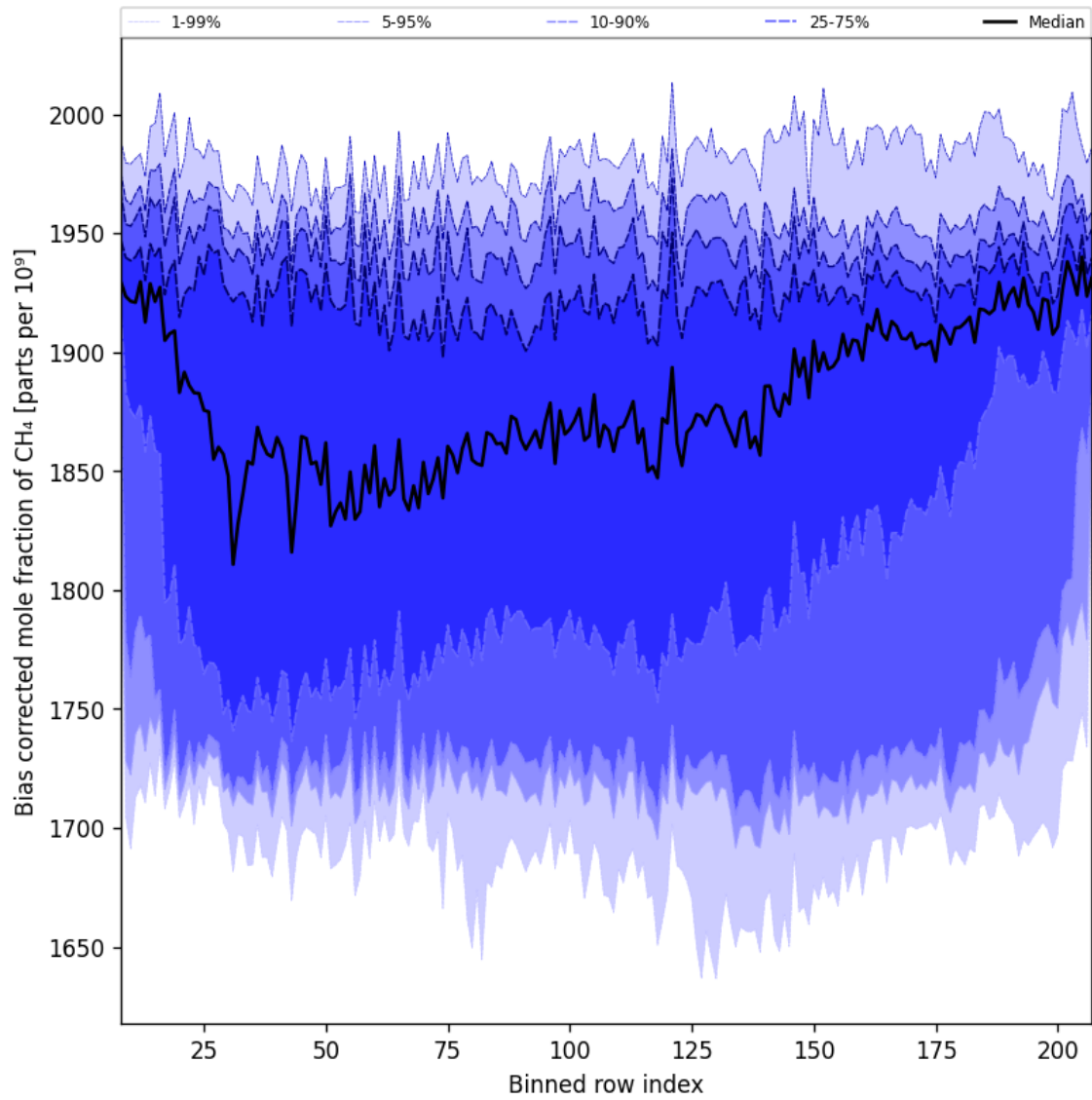
Figure 36: Along track statistics of “Bias corrected mole fraction of CH 4 ” for 2024-11-02 to 2024-11-04
