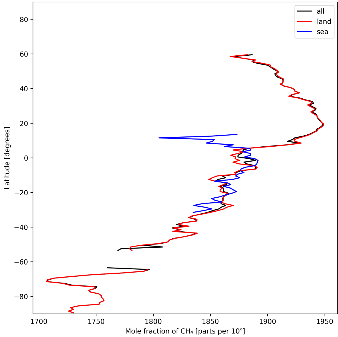
Figure 12: Zonal average of “Mole fraction of CH 4 ” for 2024-11-02 to 2024-11-04.
