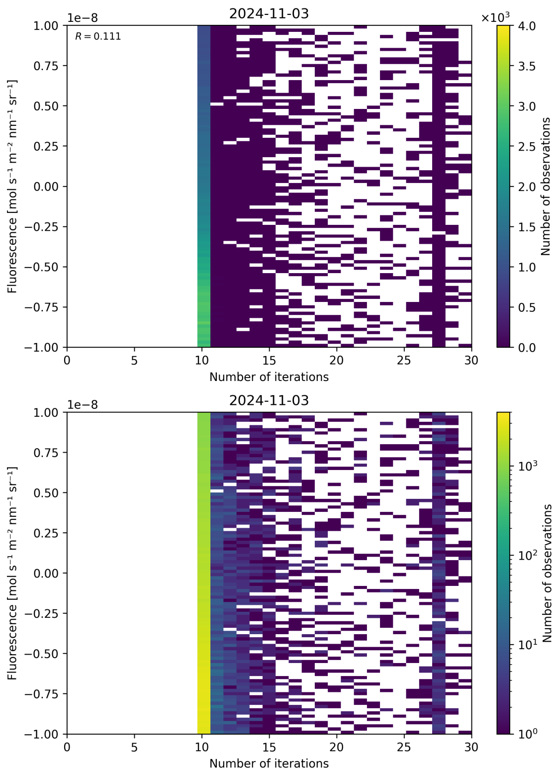
Figure 87: Scatter density plot of “Number of iterations” against “Fluorescence” for 2024-11-02 to 2024-11-04.
