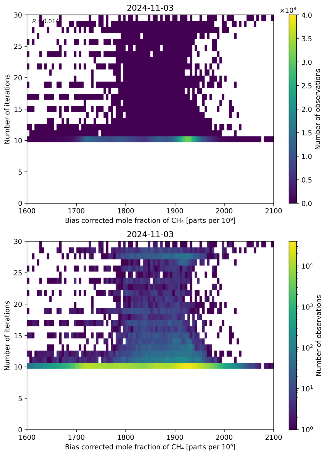
Figure 67: Scatter density plot of “Bias corrected mole fraction of CH 4 ” against “Number of iterations” for 2024-11-02 to 2024-11-04.
