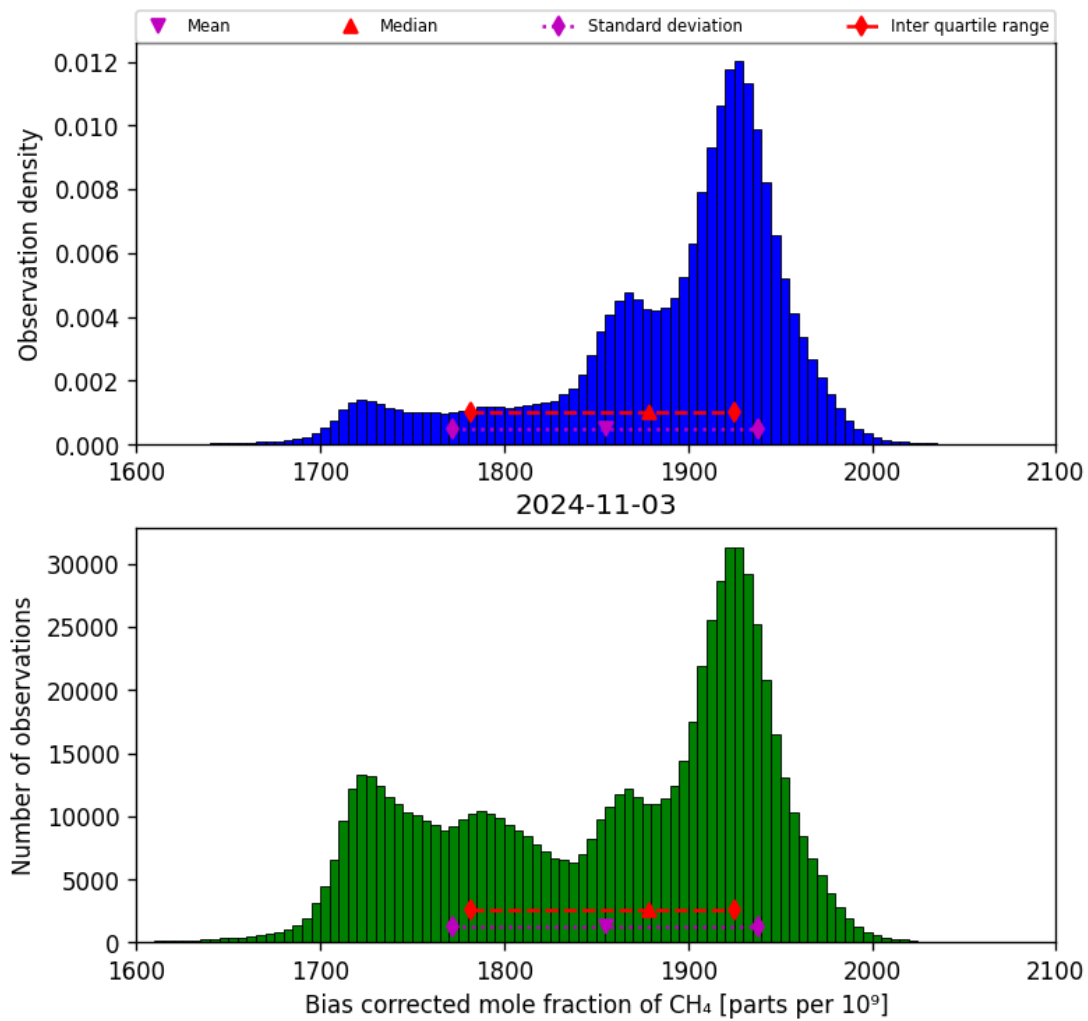
Figure 25: Histogram of “Bias corrected mole fraction of CH 4 ” for 2024-11-02 to 2024-11-04
