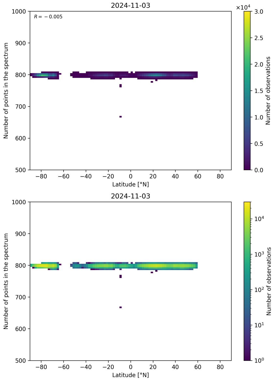
Figure 61: Scatter density plot of “Latitude” against “Number of points in the spectrum” for 2024-11-02 to 2024-11-04.
