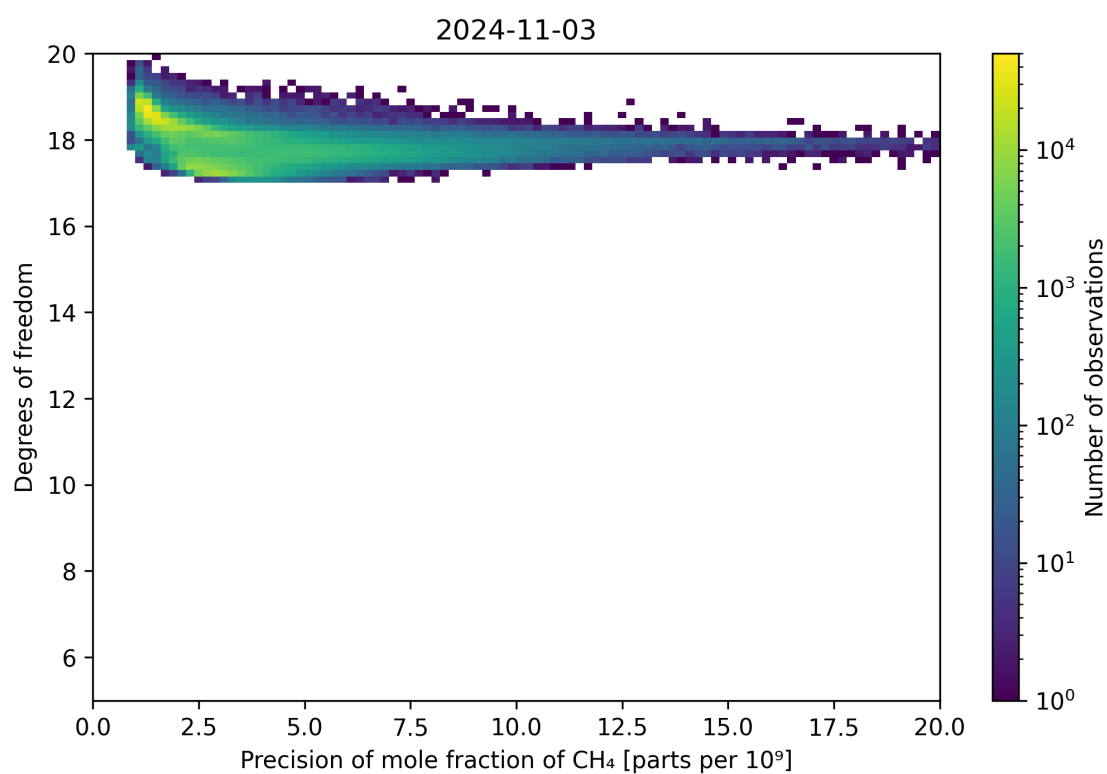
Figure 80: Scatter density plot of “Precision of mole fraction of CH 4 ” against “Degrees of freedom” for 2024-11-02 to 2024-11-04.
