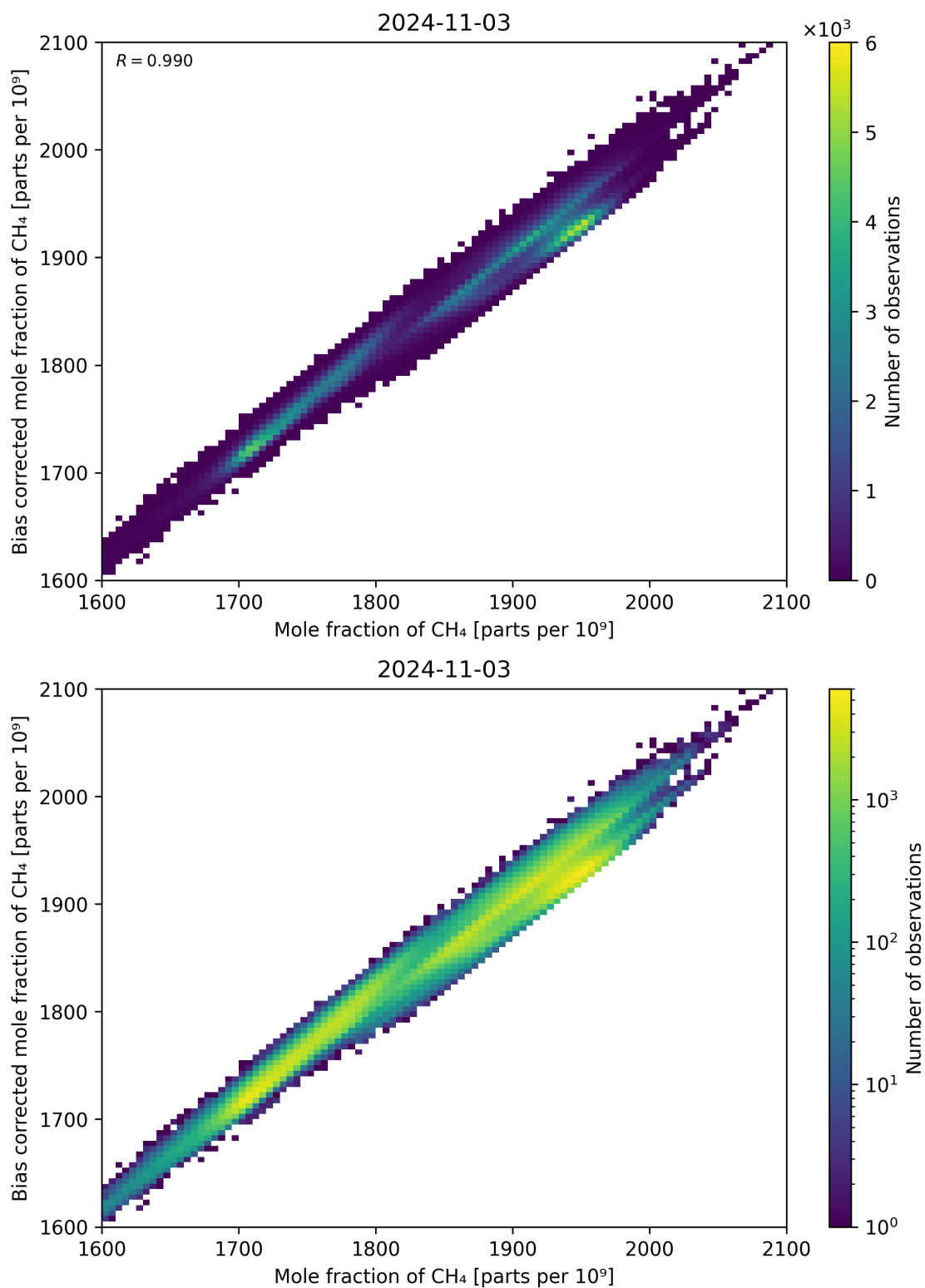
Figure 74: Scatter density plot of “Mole fraction of CH 4 ” against “Bias corrected mole fraction of CH 4 ” for 2024-11-02 to 2024-11-04.
