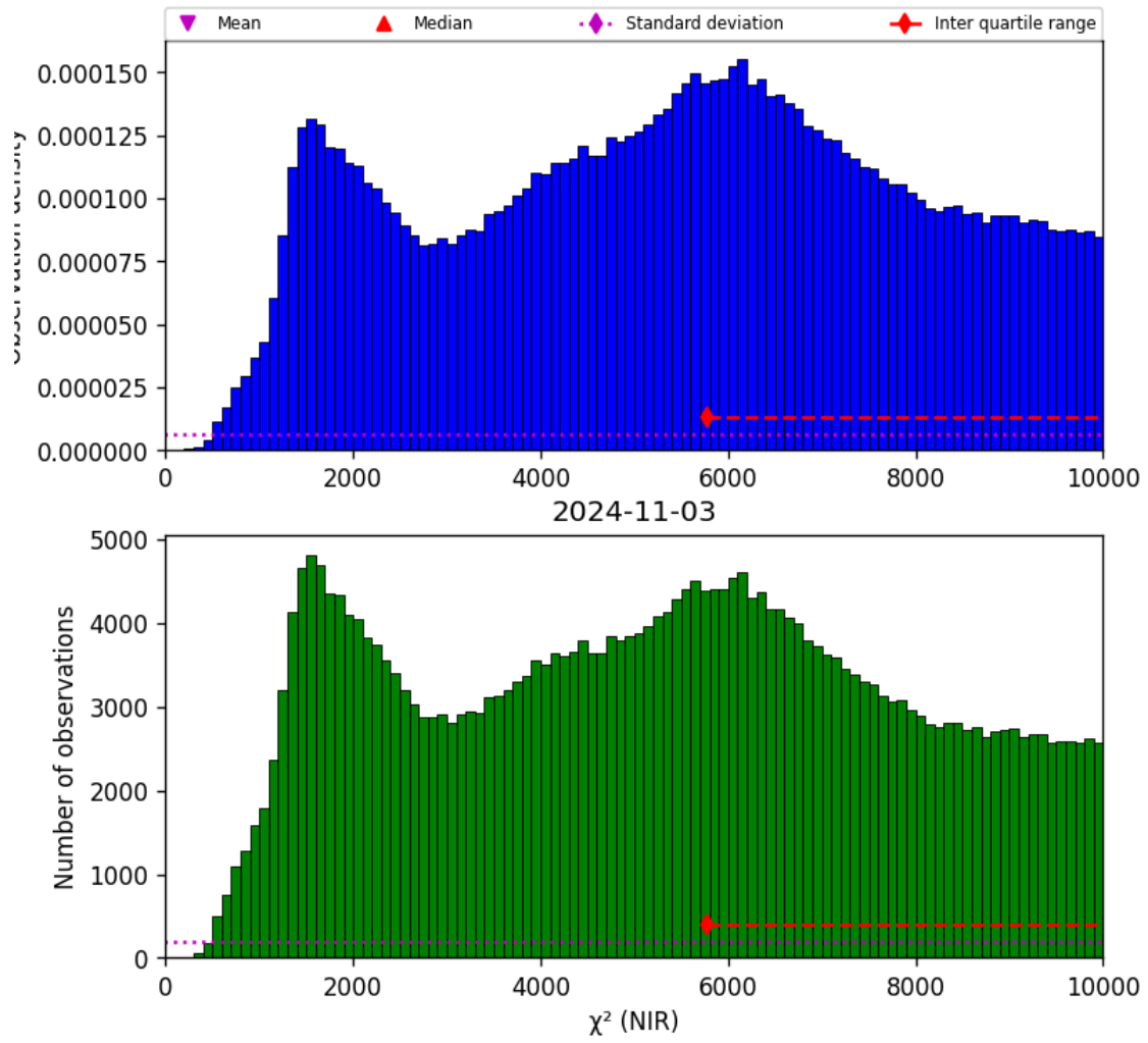
Figure 29: Histogram of “ \chi^2 (NIR)” for 2024-11-02 to 2024-11-04
