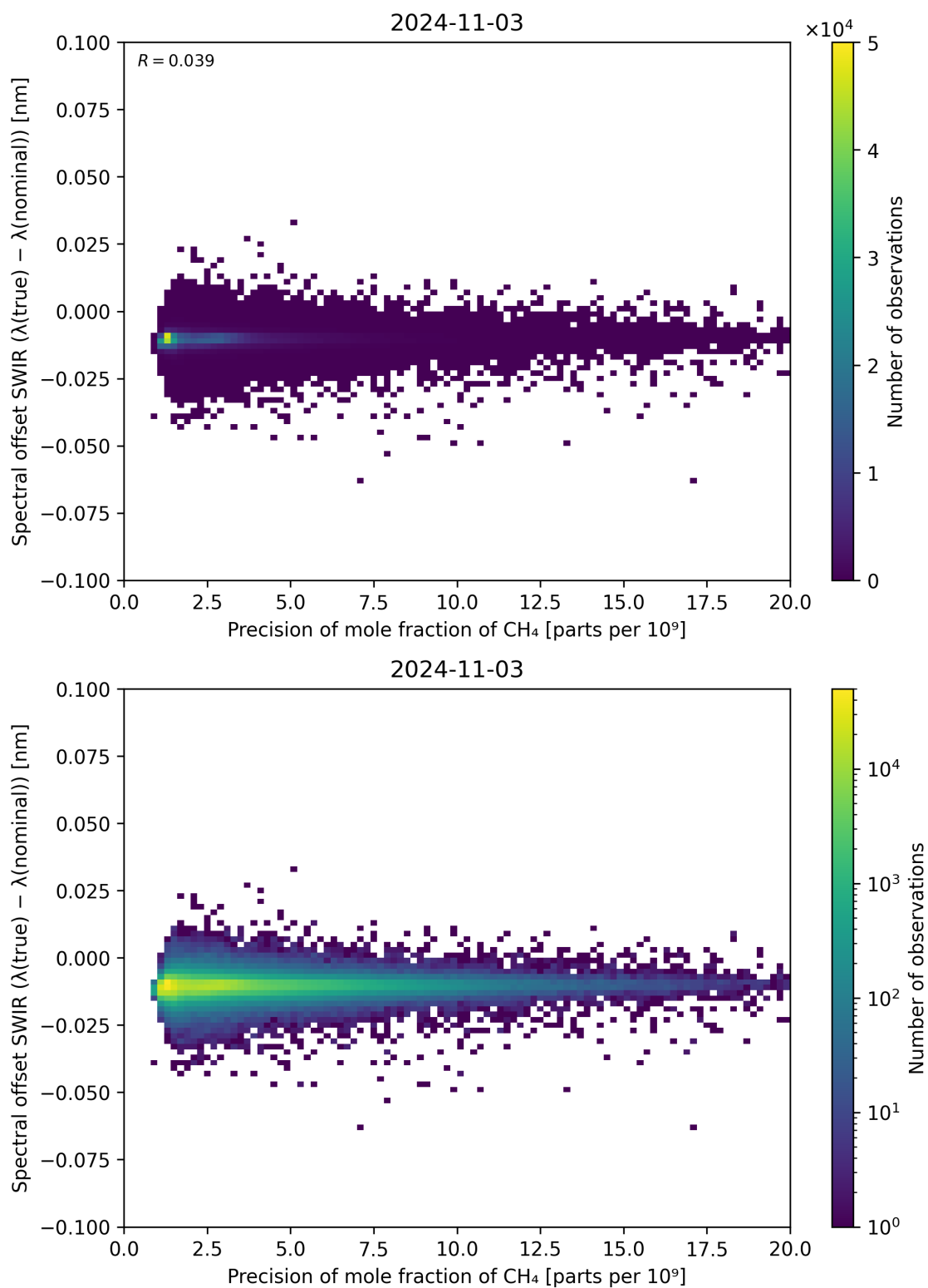
Figure 85: Scatter density plot of “Precision of mole fraction of \text{CH}_4 ” against “Spectral offset SWIR ( \lambda_{\text{true}} - \lambda_{\text{nominal}} )” for 2024-11-02 to 2024-11-04.
