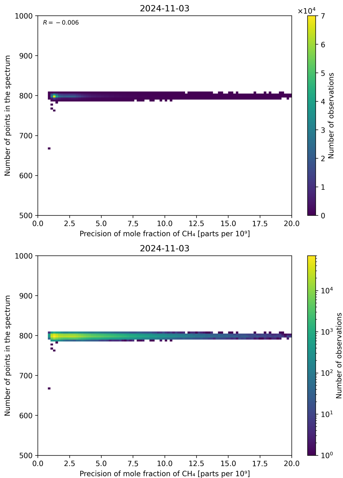
Figure 84: Scatter density plot of “Precision of mole fraction of CH 4 ” against “Number of points in the spectrum” for 2024-11-02 to 2024-11-04.
