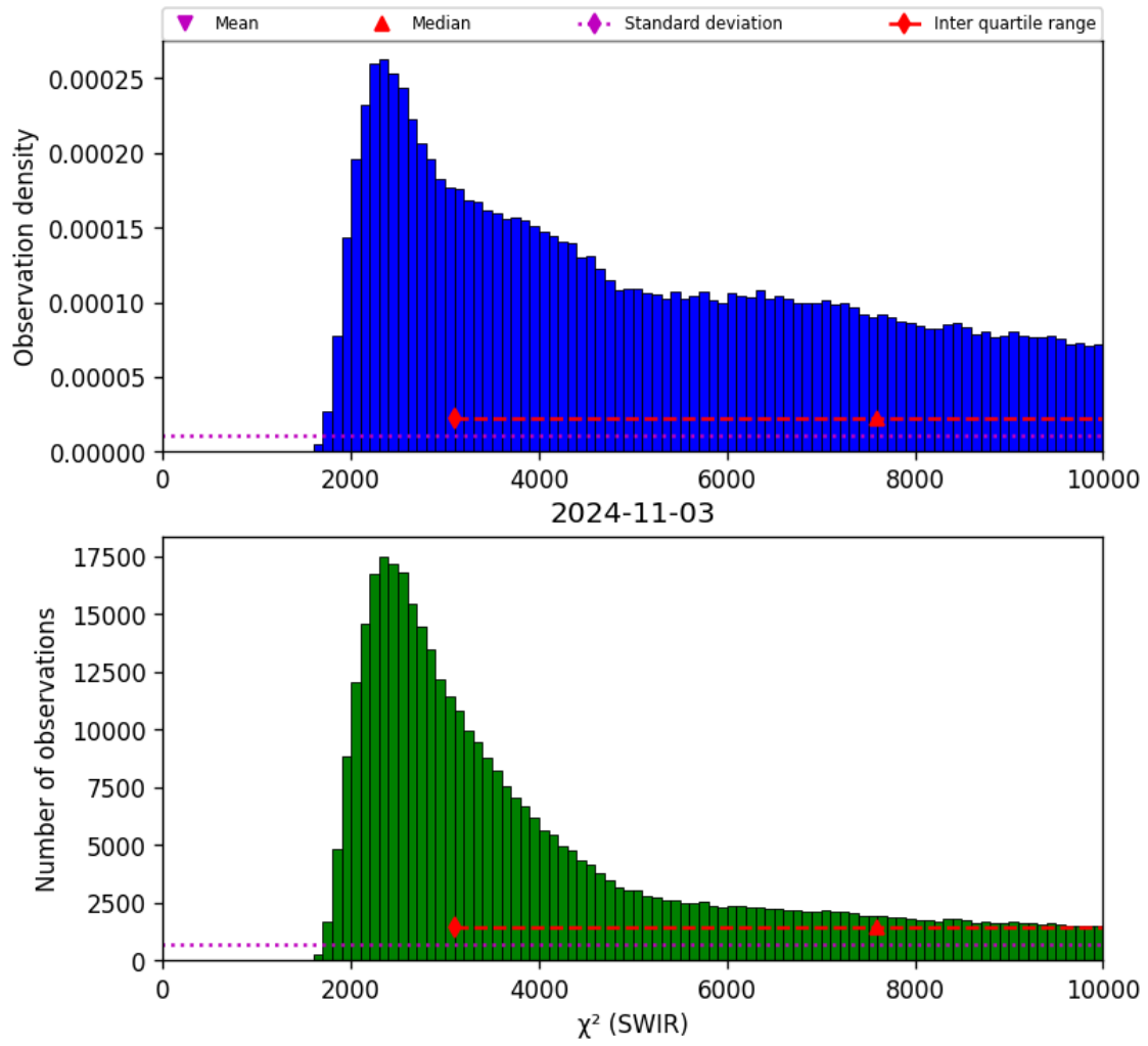
Figure 28: Histogram of “ \chi^2 (SWIR)” for 2024-11-02 to 2024-11-04
