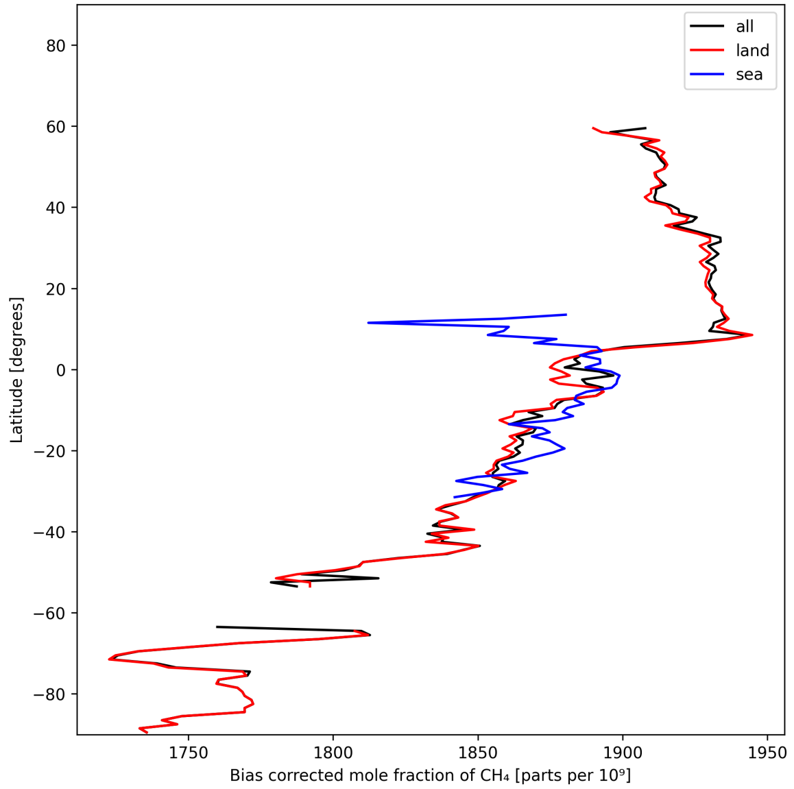
Figure 14: Zonal average of “Bias corrected mole fraction of CH 4 ” for 2024-11-02 to 2024-11-04.
