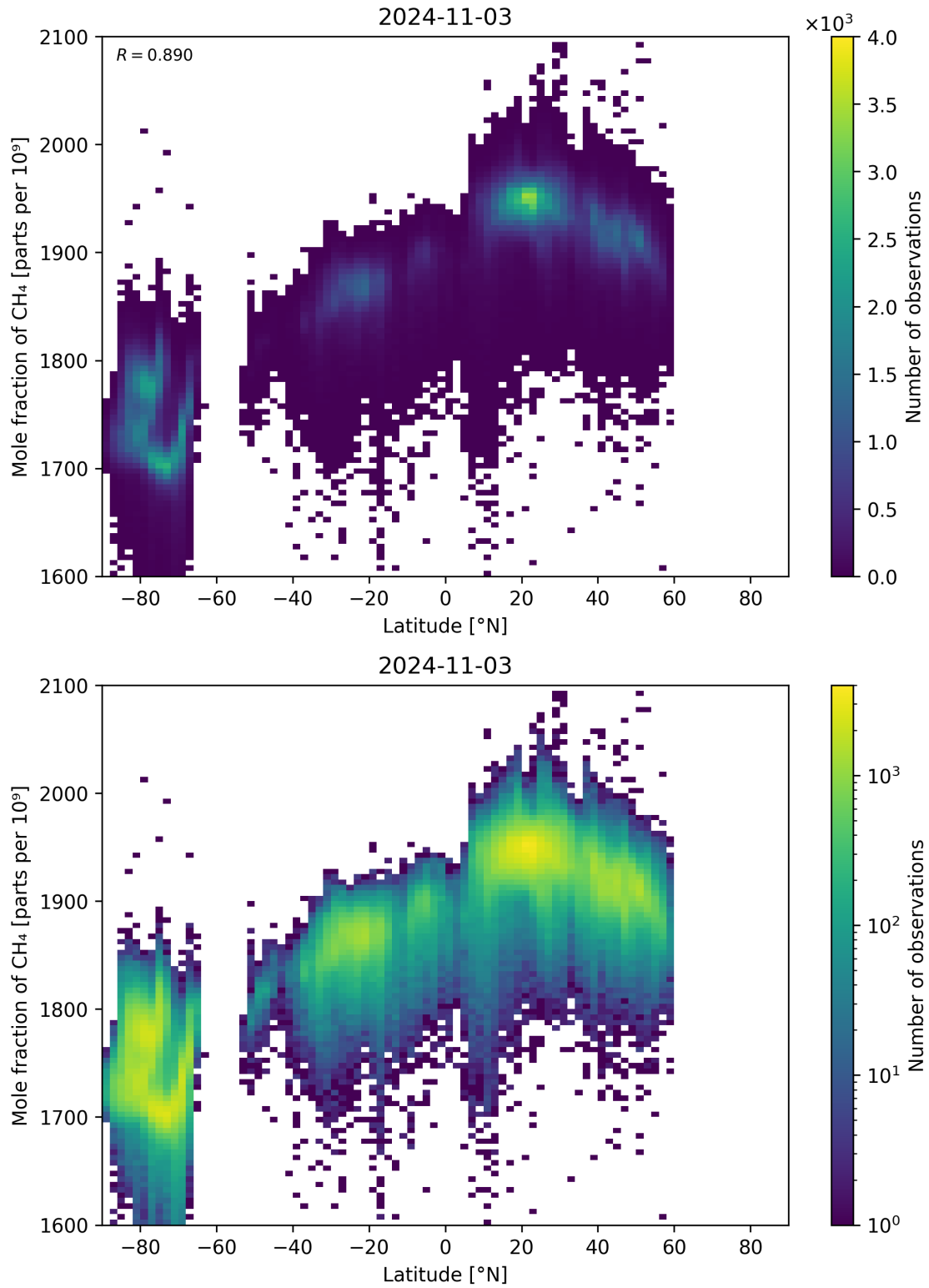
Figure 57: Scatter density plot of “Latitude” against “Mole fraction of CH 4 ” for 2024-11-02 to 2024-11-04.
