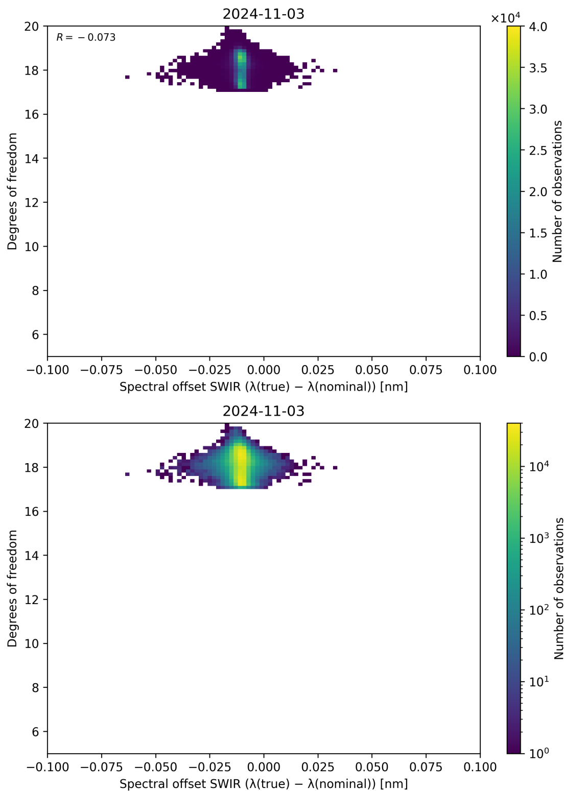
Figure 119: Scatter density plot of “Spectral offset SWIR ( \lambda_{\text{true}} - \lambda_{\text{nominal}} )” against “Degrees of freedom” for 2024-11-02 to 2024-11-04.
