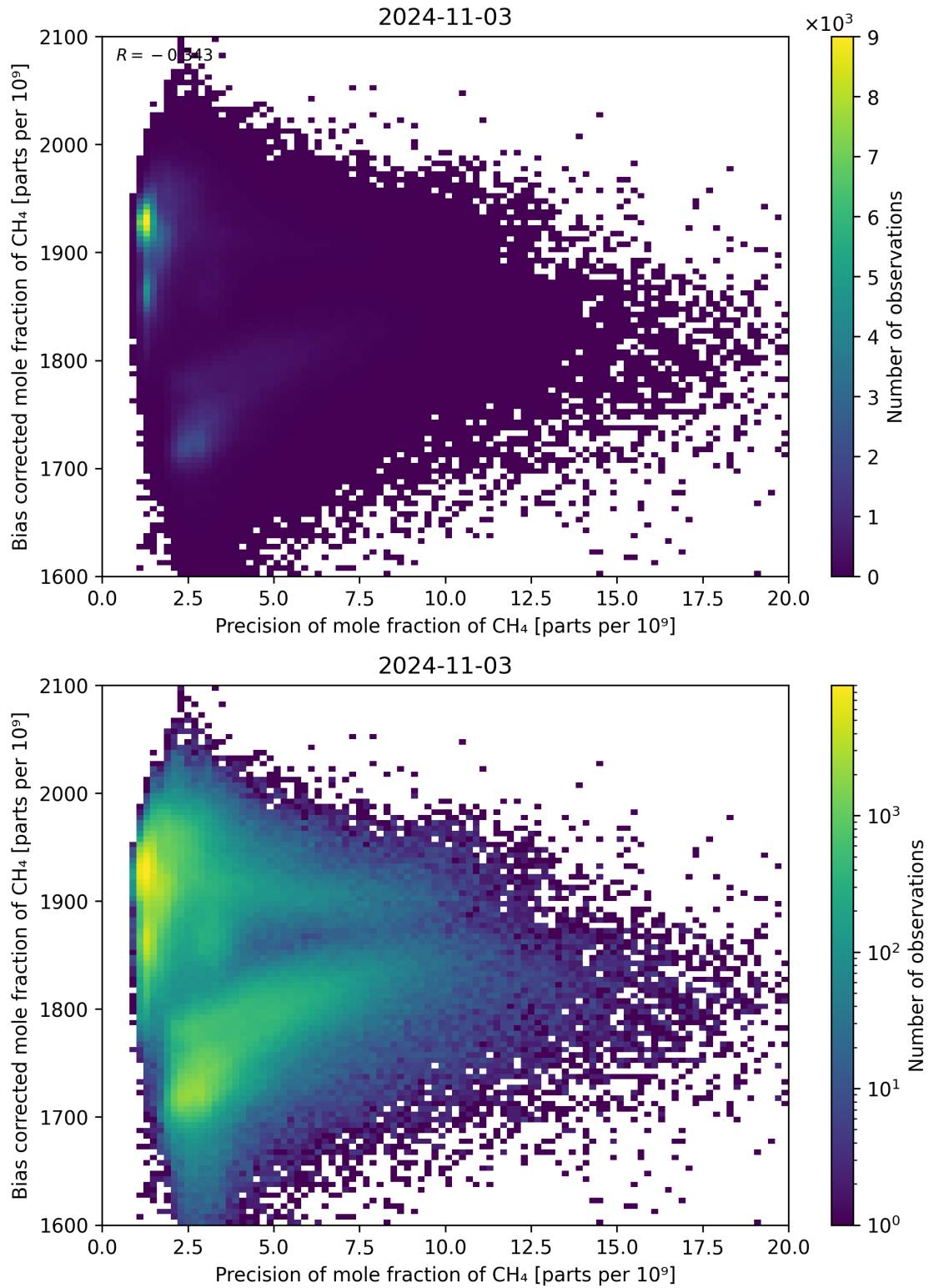
Figure 82: Scatter density plot of “Precision of mole fraction of CH 4 ” against “Bias corrected mole fraction of CH 4 ” for 2024-11-02 to 2024-11-04.
