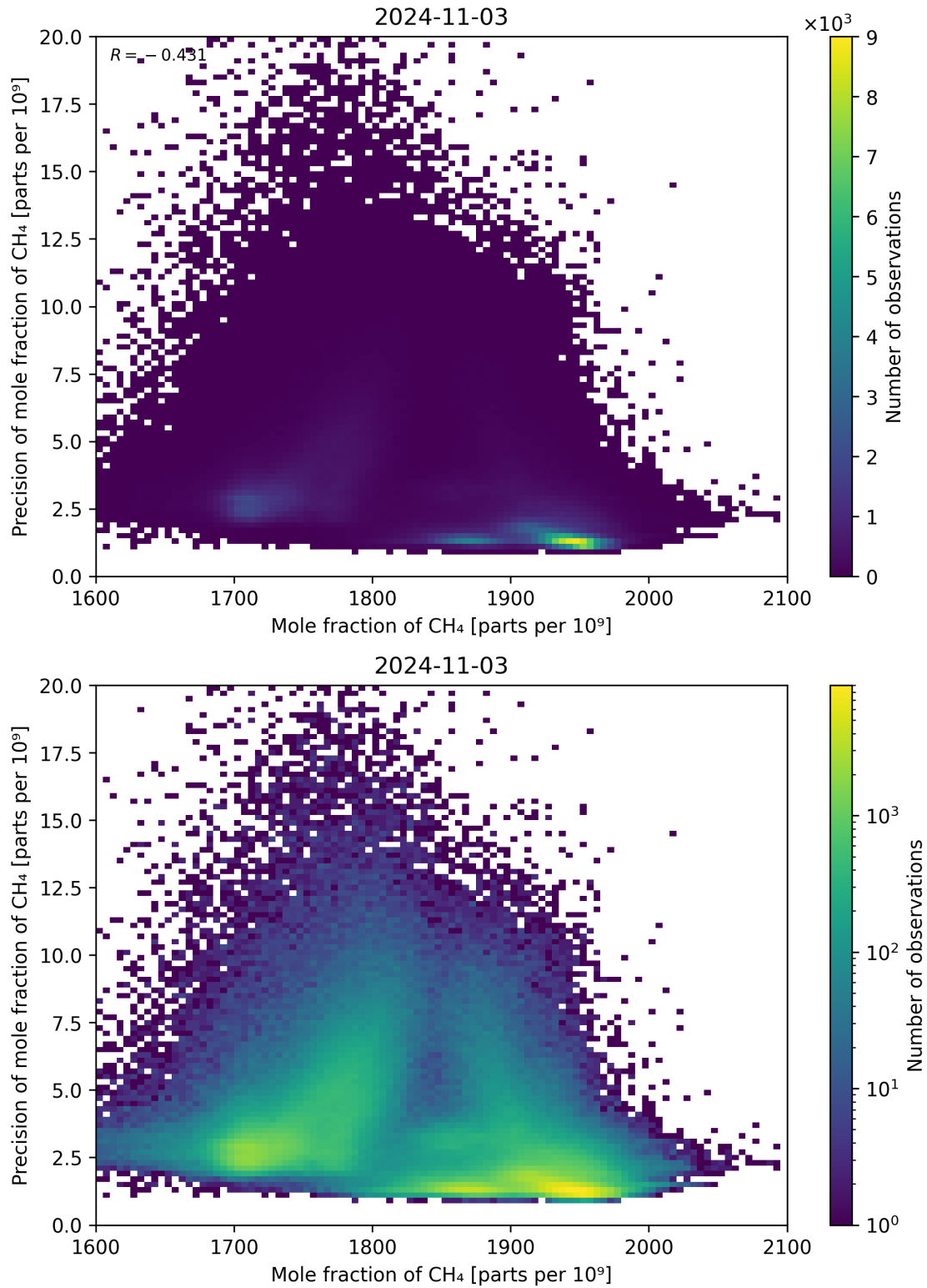
Figure 75: Scatter density plot of “Mole fraction of CH 4 ” against “Precision of mole fraction of CH 4 ” for 2024-11-02 to 2024-11-04.
