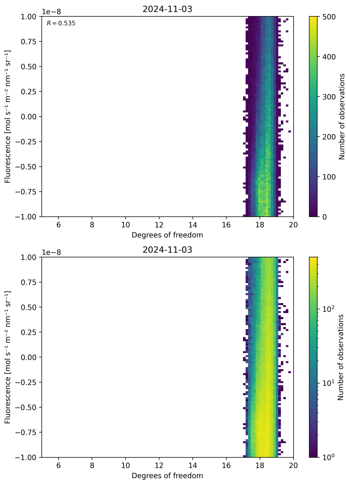
Figure 51: Scatter density plot of “Degrees of freedom” against “Fluorescence” for 2024-11-02 to 2024-11-04.
