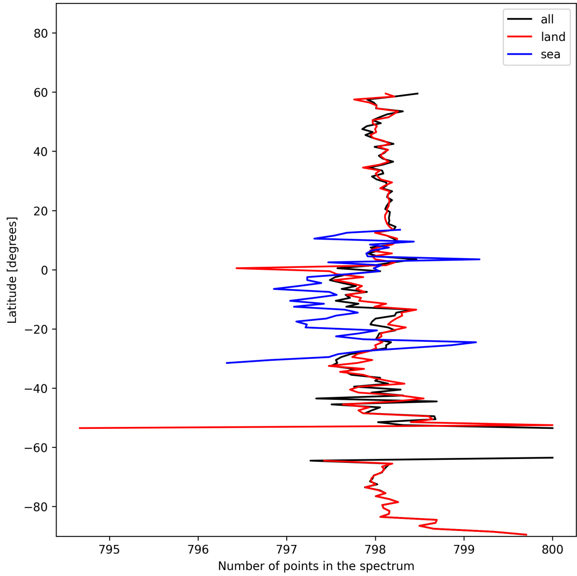
Figure 15: Zonal average of “Number of points in the spectrum” for 2024-11-02 to 2024-11-04.
