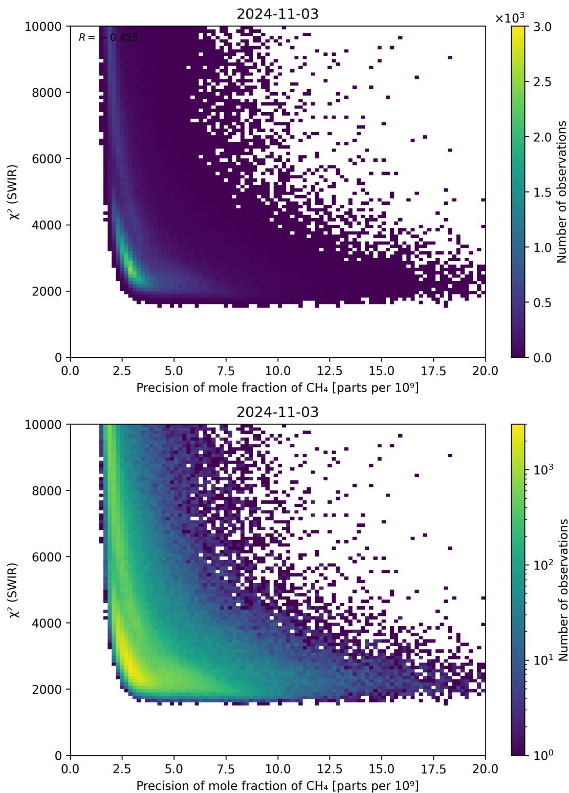
Figure 79: Scatter density plot of “Precision of mole fraction of \text{CH}_4 ” against “ \chi^2 (SWIR)” for 2024-11-02 to 2024-11-04.
