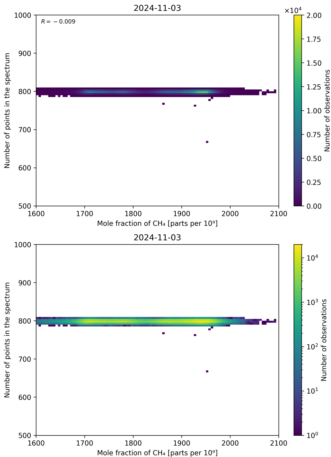
Figure 77: Scatter density plot of “Mole fraction of CH 4 ” against “Number of points in the spectrum” for 2024-11-02 to 2024-11-04.
