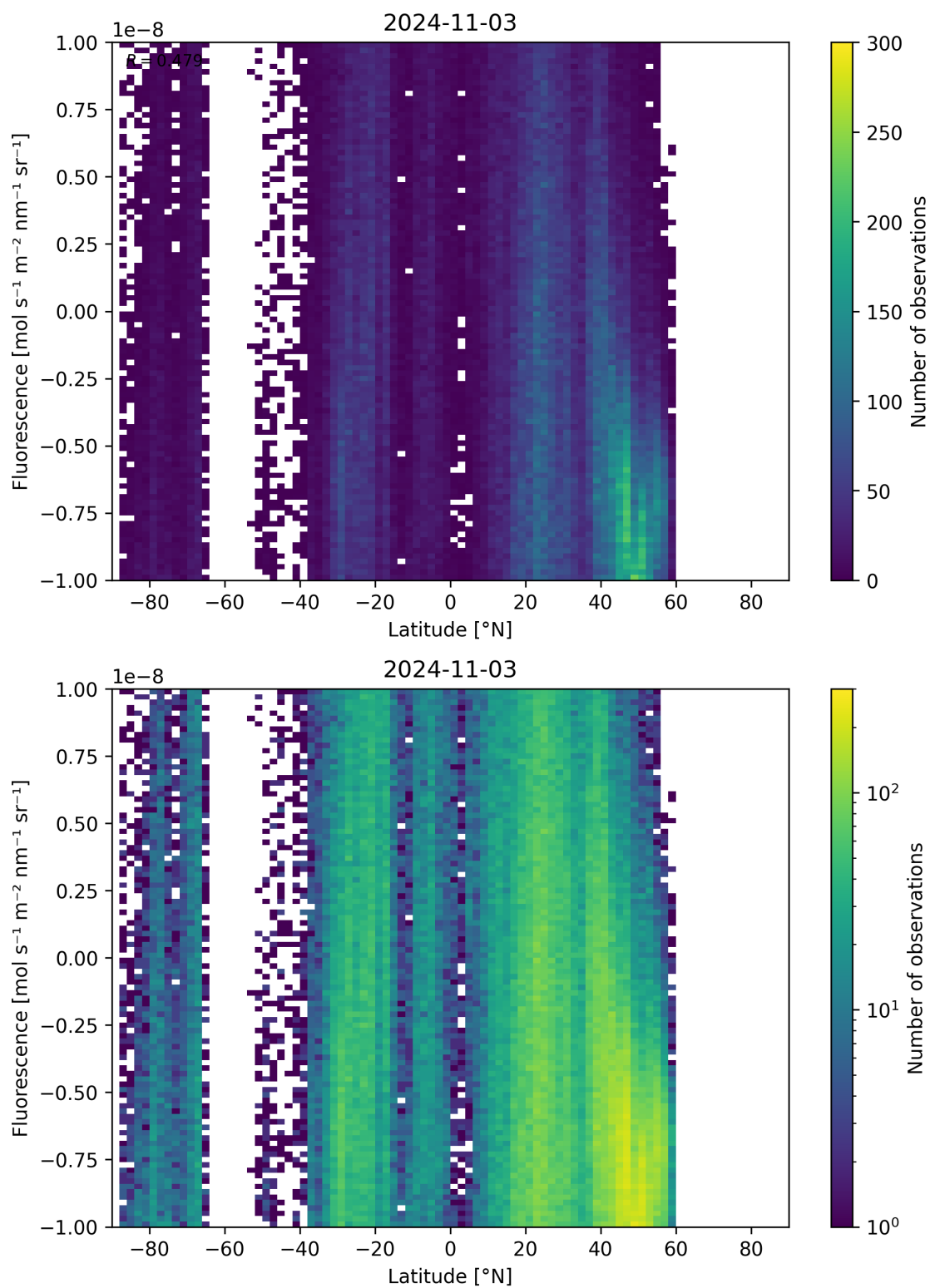
Figure 56: Scatter density plot of “Latitude” against “Fluorescence” for 2024-11-02 to 2024-11-04.
