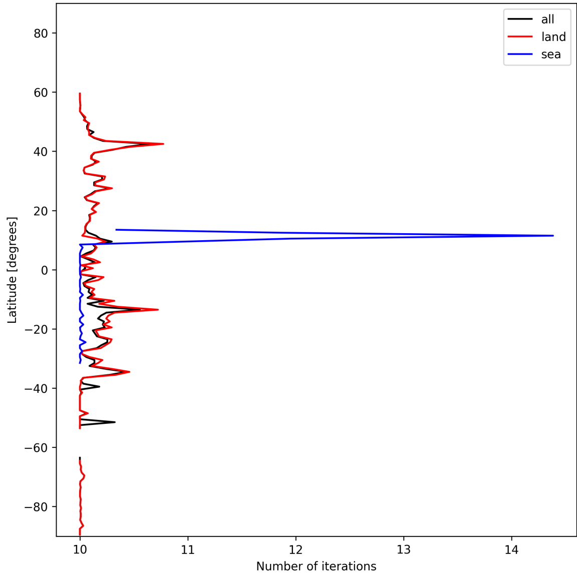
Figure 20: Zonal average of “Number of iterations” for 2024-11-02 to 2024-11-04.
