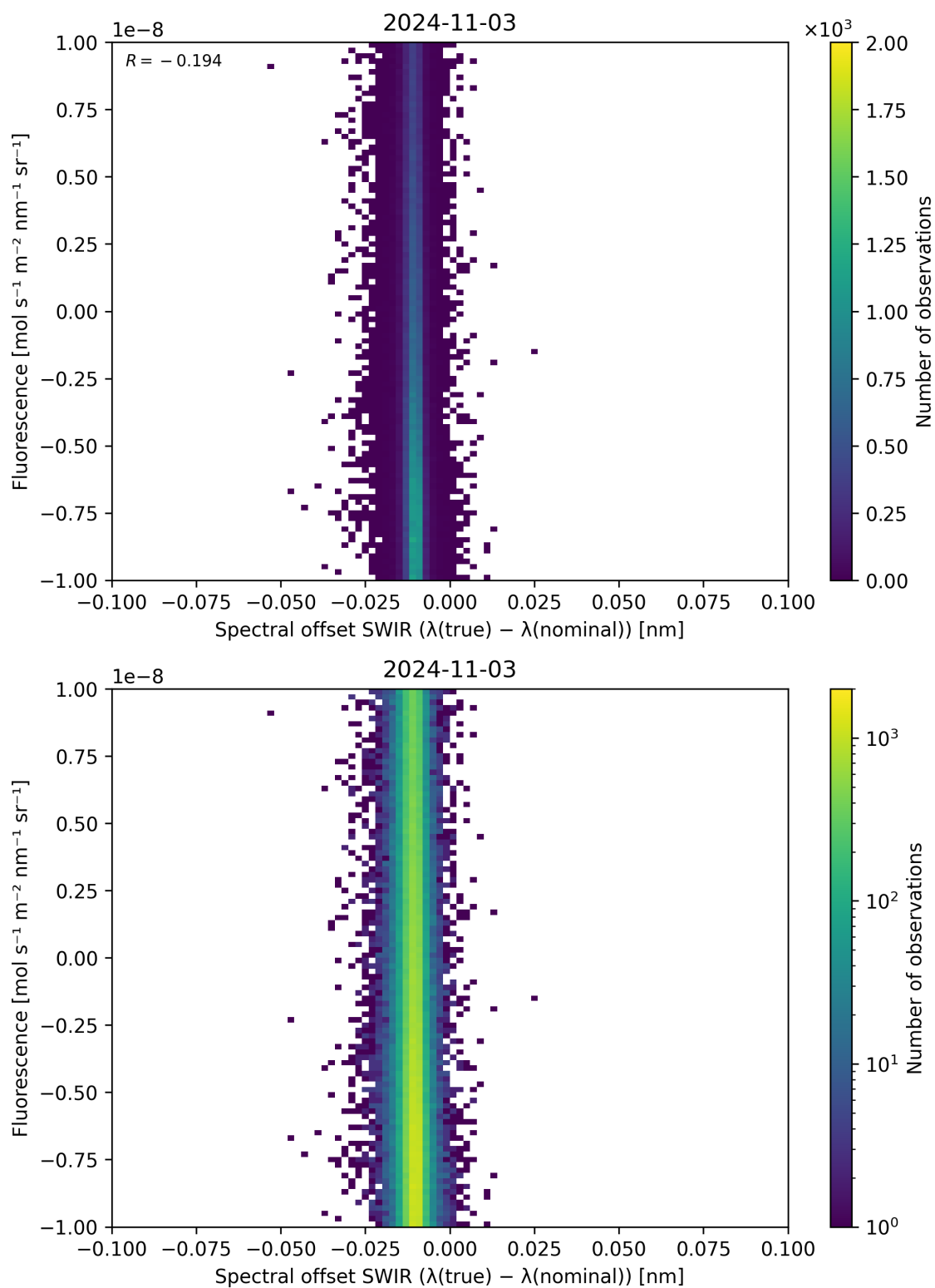
Figure 120: Scatter density plot of “Spectral offset SWIR ( \lambda_{\text{true}} - \lambda_{\text{nominal}} )” against “Fluorescence” for 2024-11-02 to 2024-11-04.
