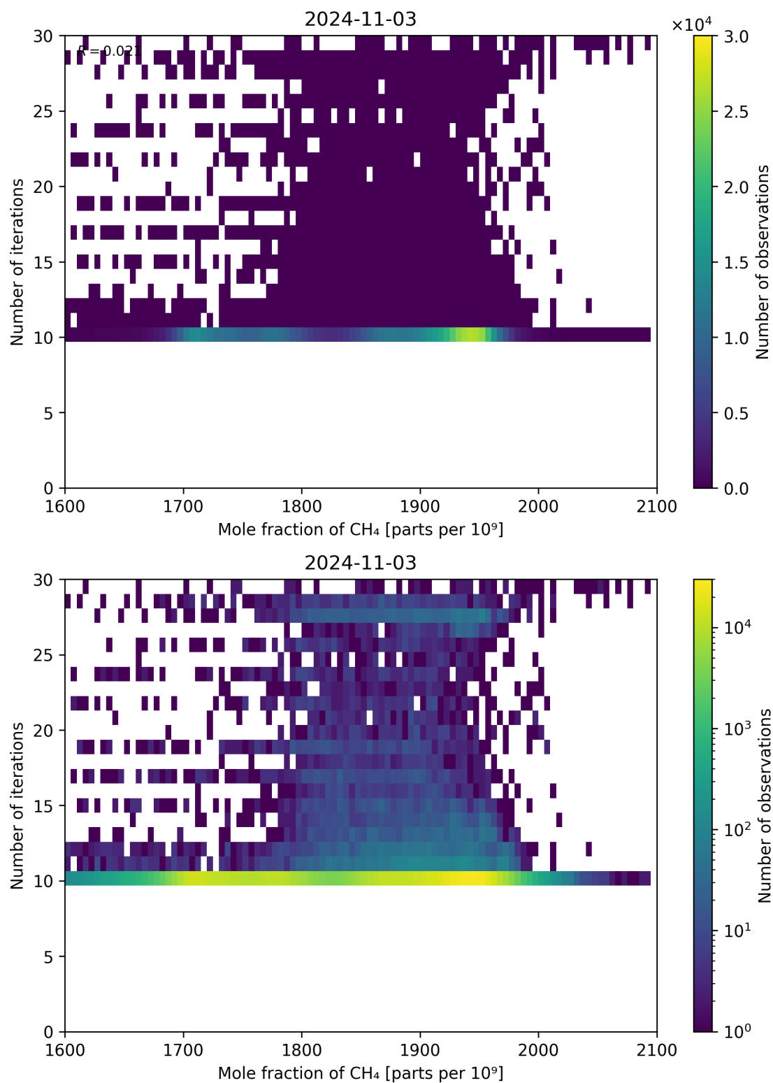
Figure 76: Scatter density plot of “Mole fraction of CH 4 ” against “Number of iterations” for 2024-11-02 to 2024-11-04.
