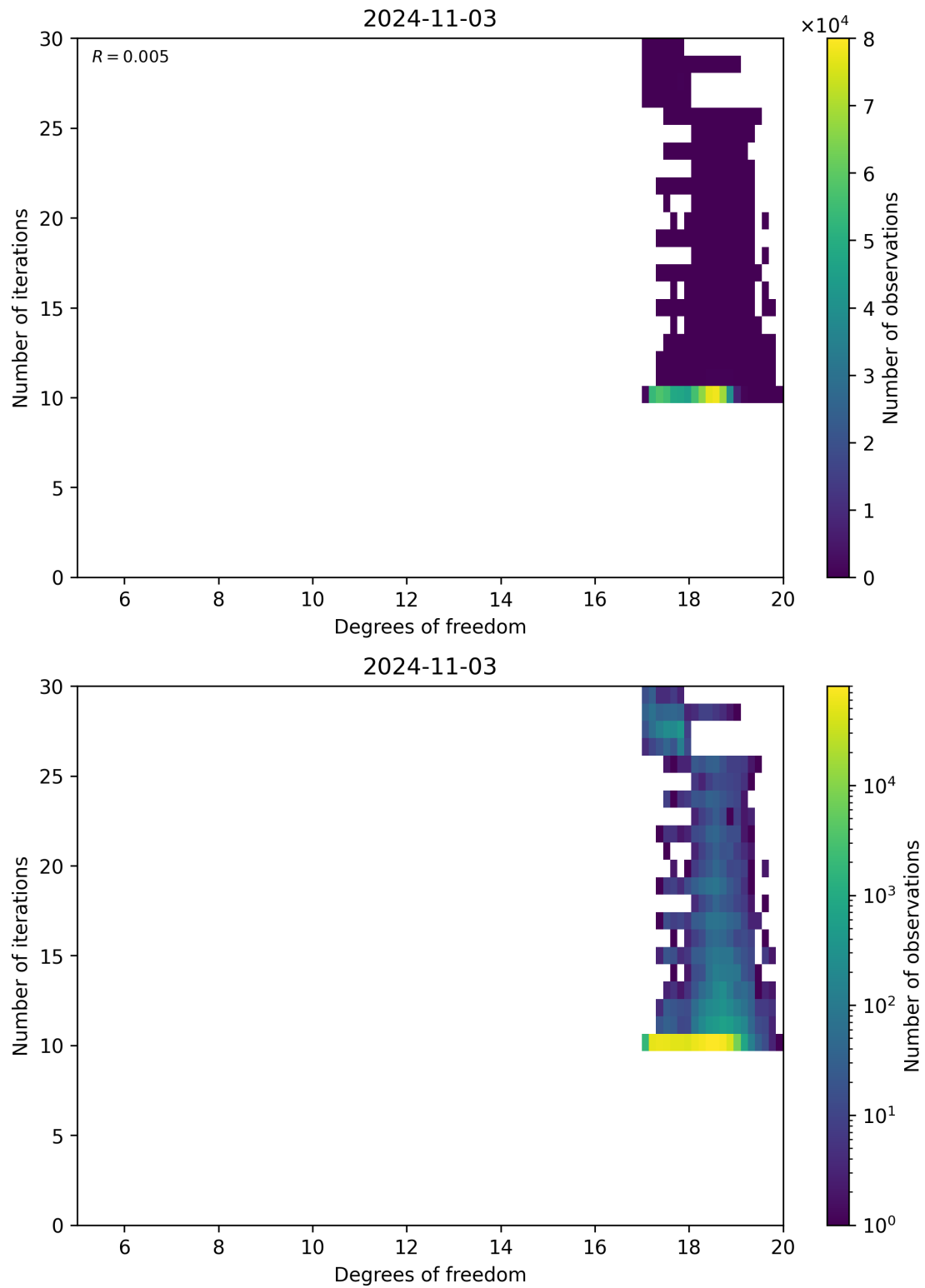
Figure 52: Scatter density plot of “Degrees of freedom” against “Number of iterations” for 2024-11-02 to 2024-11-04.
