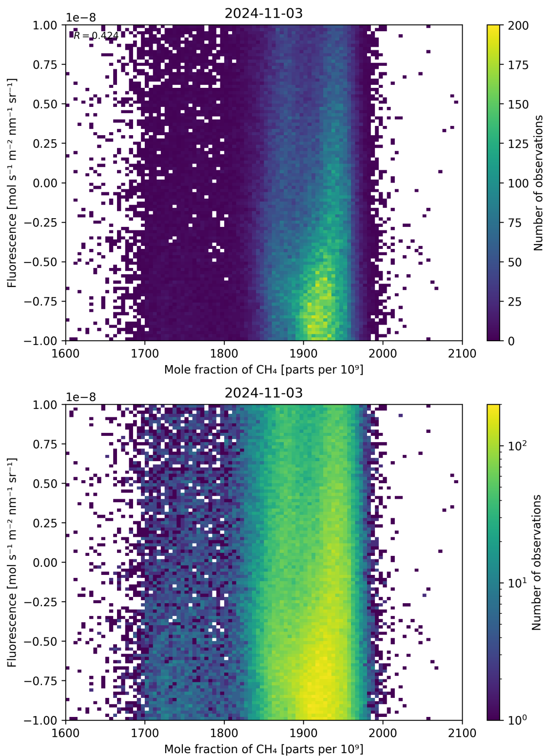
Figure 73: Scatter density plot of “Mole fraction of \text{CH}_4 ” against “Fluorescence” for 2024-11-02 to 2024-11-04.
