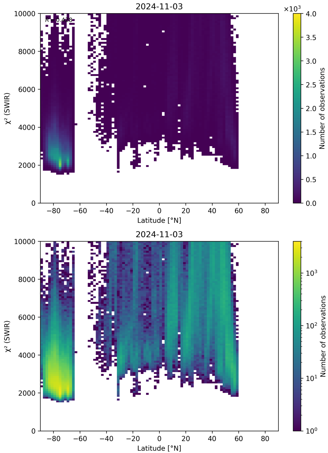
Figure 54: Scatter density plot of “Latitude” against “ \chi^2 (SWIR)” for 2024-11-02 to 2024-11-04.
