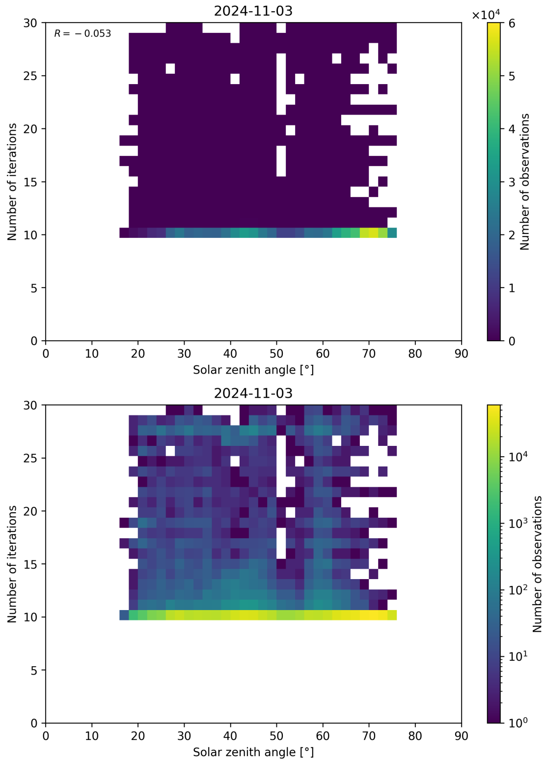
Figure 102: Scatter density plot of “Solar zenith angle” against “Number of iterations” for 2024-11-02 to 2024-11-04.
