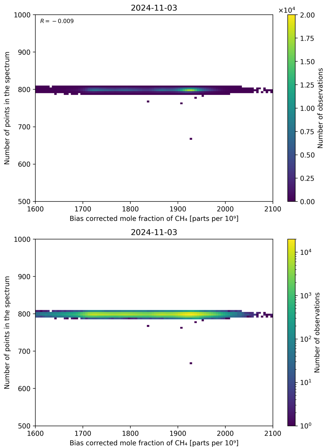
Figure 68: Scatter density plot of “Bias corrected mole fraction of CH 4 ” against “Number of points in the spectrum” for 2024-11-02 to 2024-11-04.
