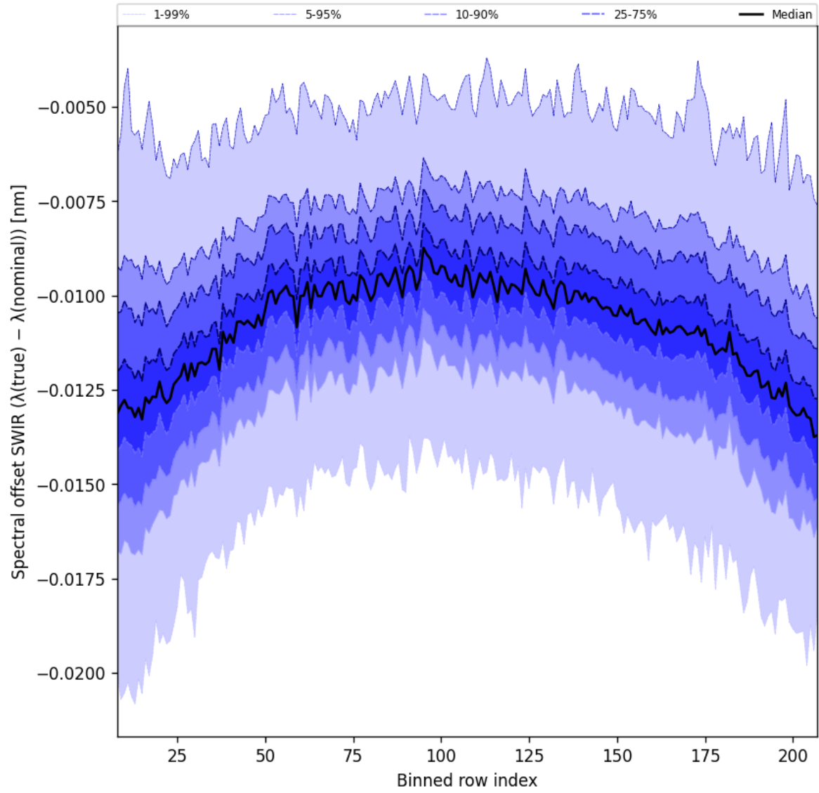
Figure 38: Along track statistics of “Spectral offset SWIR ( \lambda_{\text{true}} - \lambda_{\text{nominal}} )” for 2024-11-02 to 2024-11-04
