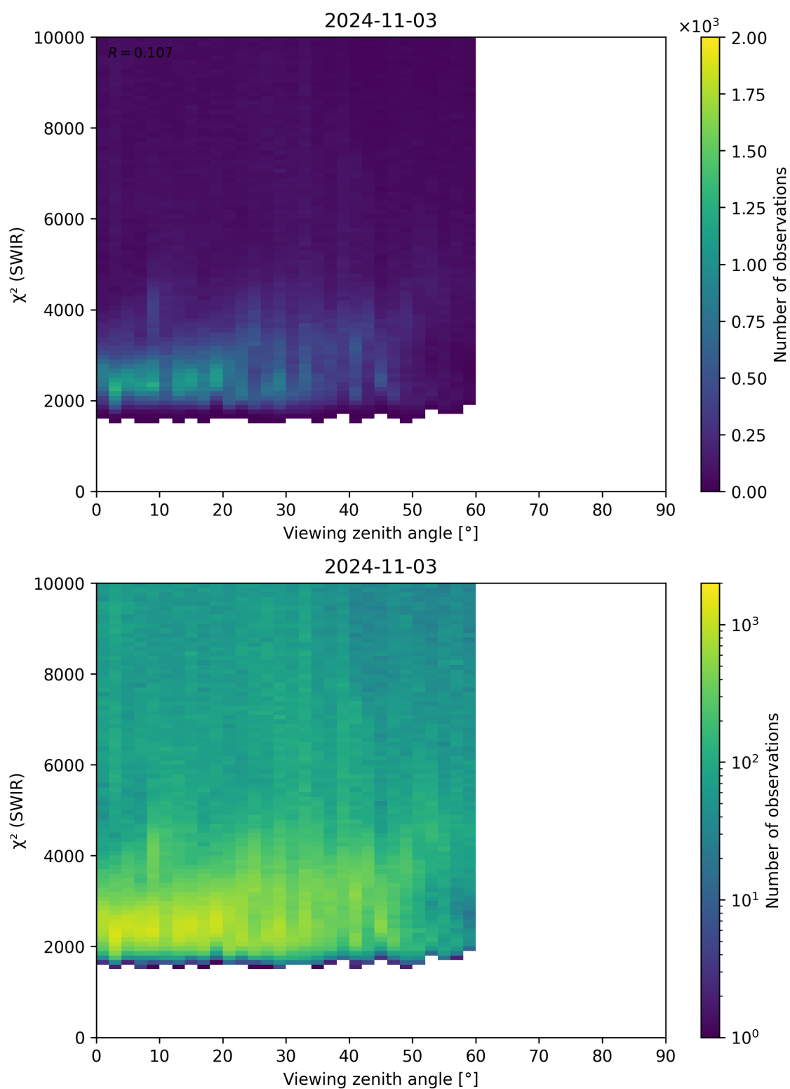
Figure 106: Scatter density plot of “Viewing zenith angle” against “ \chi^2 (SWIR)” for 2024-11-02 to 2024-11-04.
