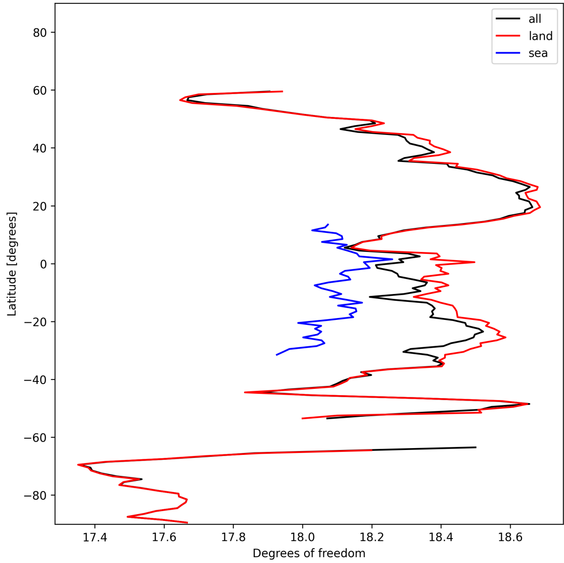
Figure 19: Zonal average of “Degrees of freedom” for 2024-11-02 to 2024-11-04.
