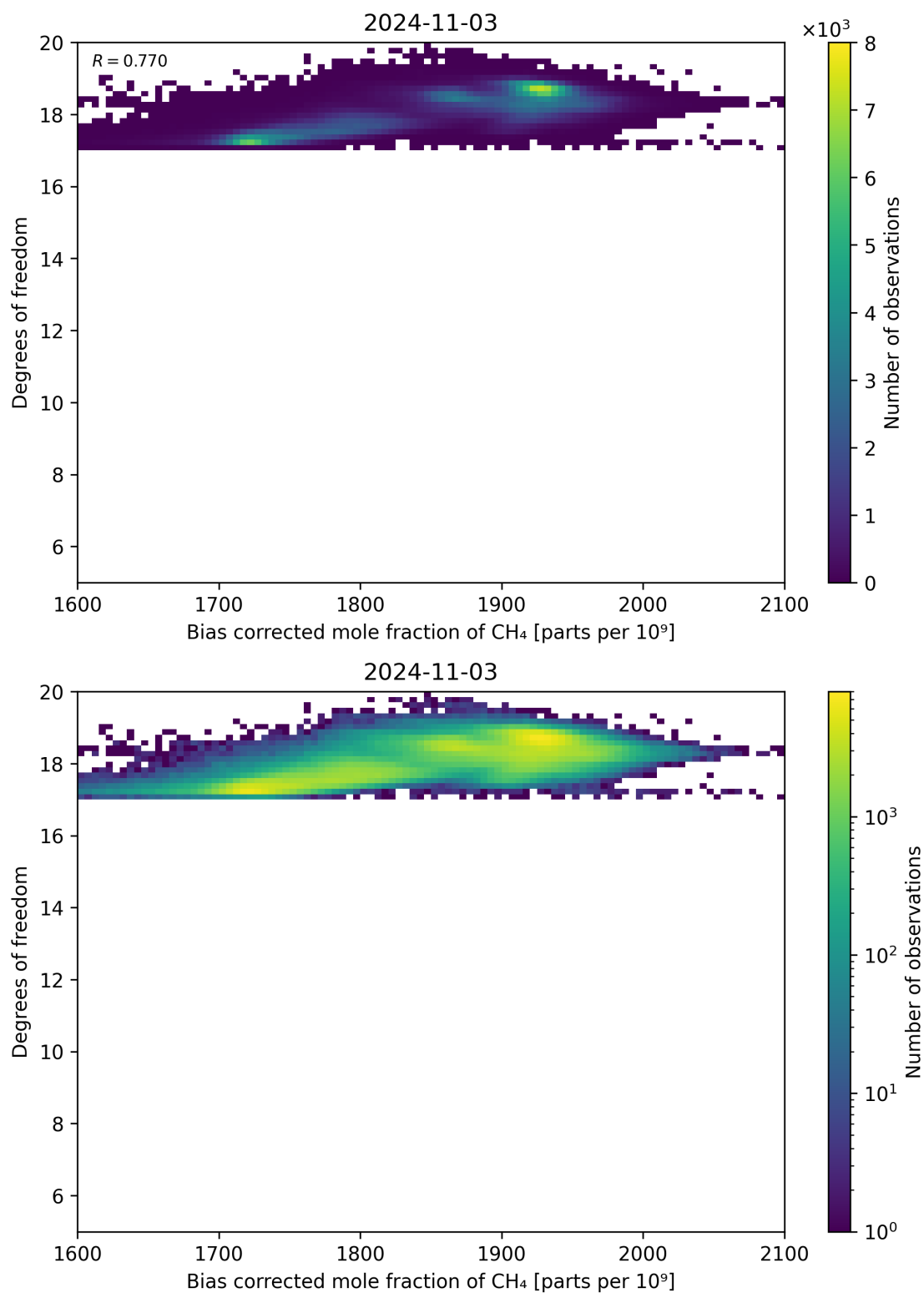
Figure 65: Scatter density plot of “Bias corrected mole fraction of CH 4 ” against “Degrees of freedom” for 2024-11-02 to 2024-11-04.
