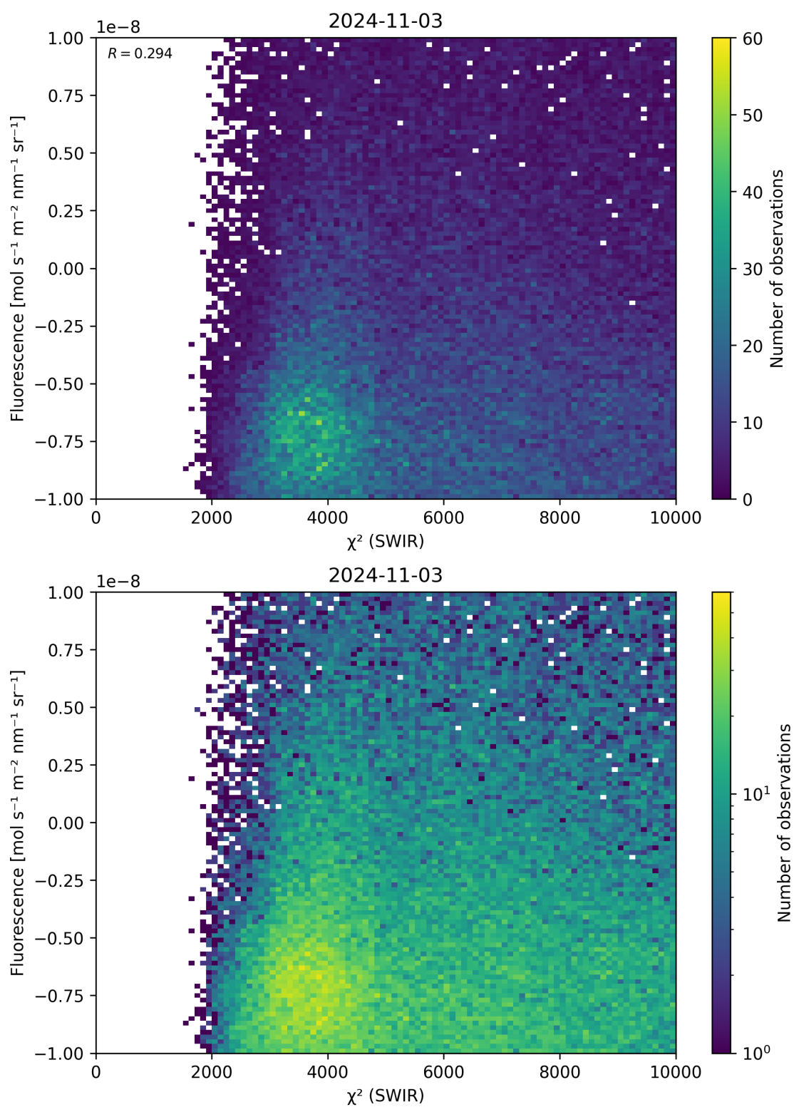
Figure 49: Scatter density plot of “ \chi^2 (SWIR)” against “Fluorescence” for 2024-11-02 to 2024-11-04.
