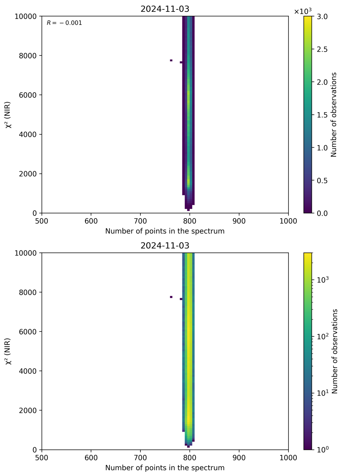
Figure 88: Scatter density plot of “Number of points in the spectrum” against “ \chi^2 (NIR)” for 2024-11-02 to 2024-11-04.
