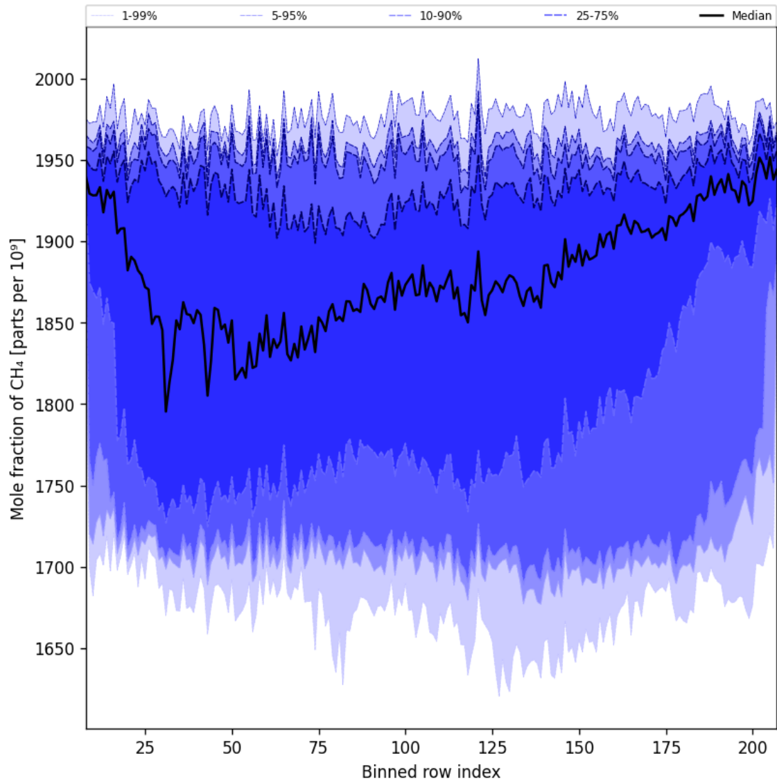
Figure 34: Along track statistics of “Mole fraction of CH 4 ” for 2024-11-02 to 2024-11-04
