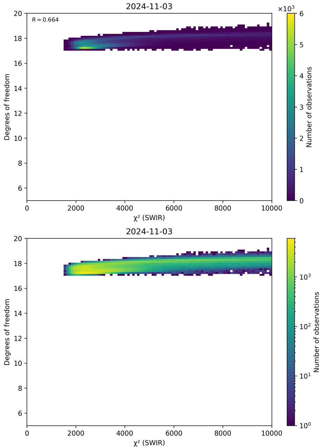
Figure 48: Scatter density plot of “ \chi^2 (SWIR)” against “Degrees of freedom” for 2024-11-02 to 2024-11-04.
