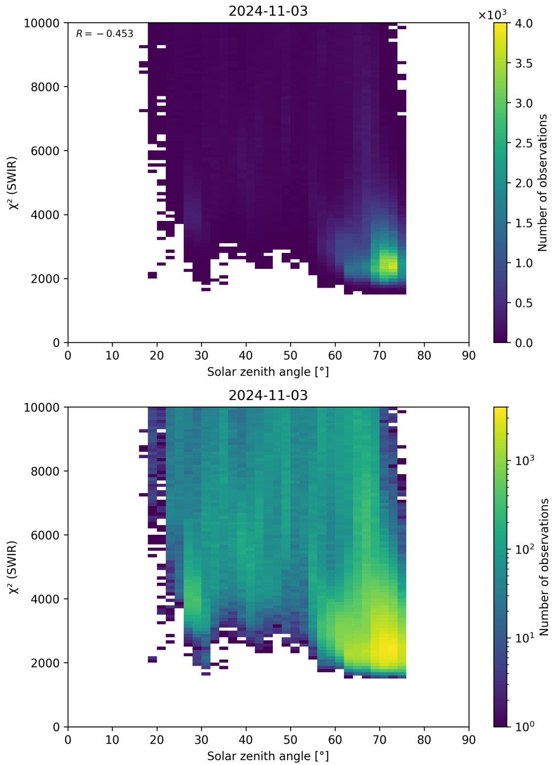
Figure 95: Scatter density plot of “Solar zenith angle” against “ \chi^2 (SWIR)” for 2024-11-02 to 2024-11-04.
