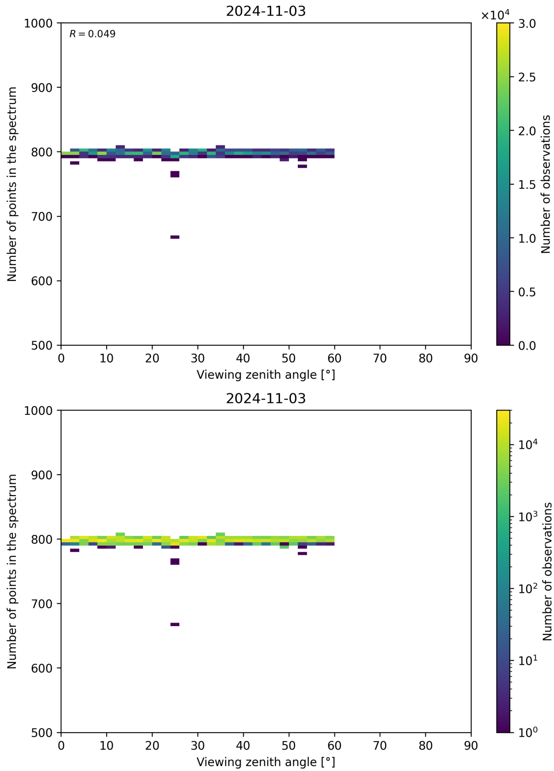
Figure 114: Scatter density plot of “Viewing zenith angle” against “Number of points in the spectrum” for 2024-11-02 to 2024-11-04.
