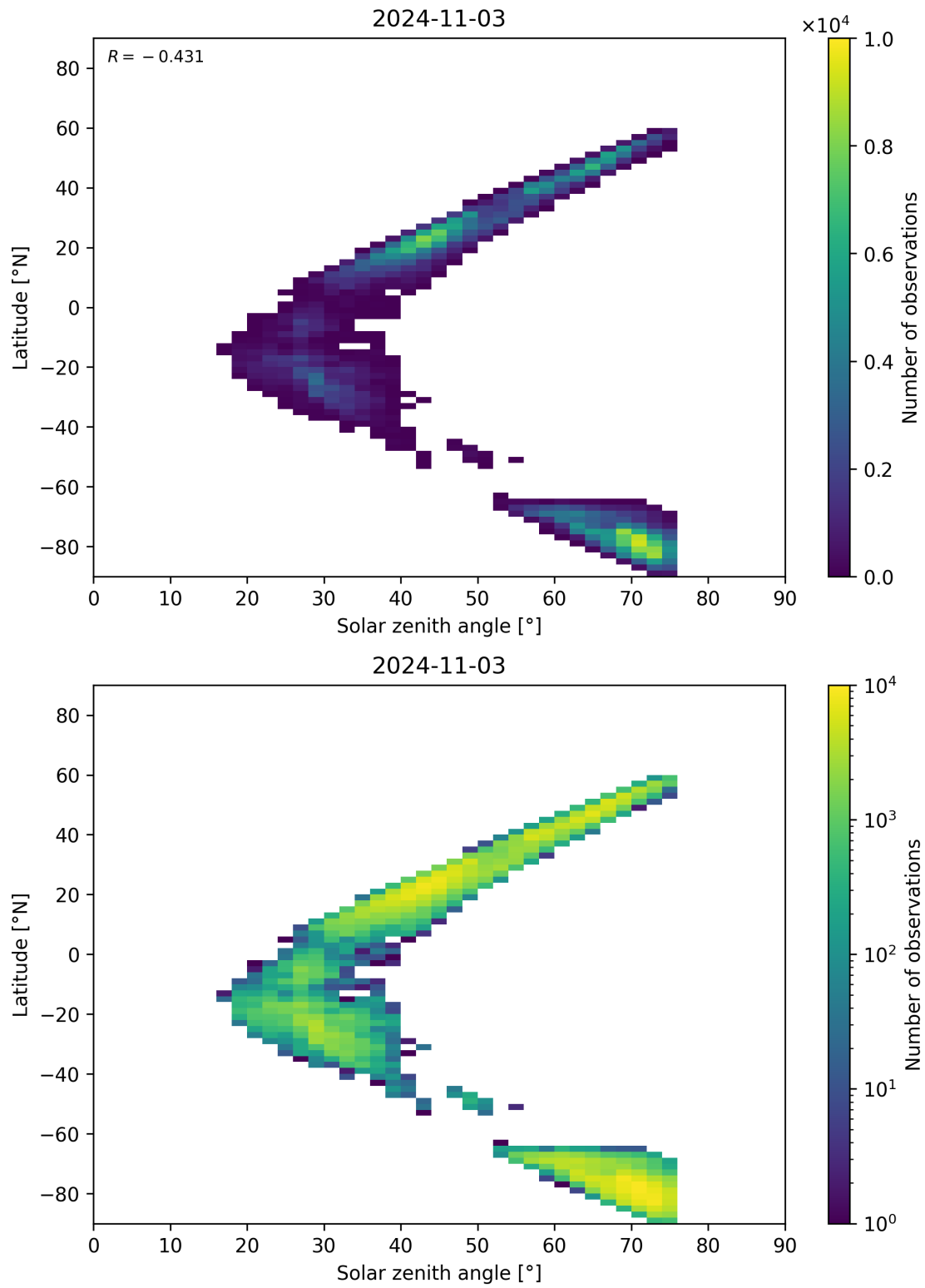
Figure 98: Scatter density plot of “Solar zenith angle” against “Latitude” for 2024-11-02 to 2024-11-04.
