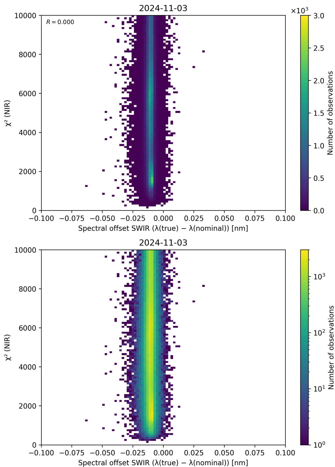
Figure 117: Scatter density plot of “Spectral offset SWIR ( \lambda_{\text{true}} - \lambda_{\text{nominal}} )” against “ \chi^2 (NIR)” for 2024-11-02 to 2024-11-04.
