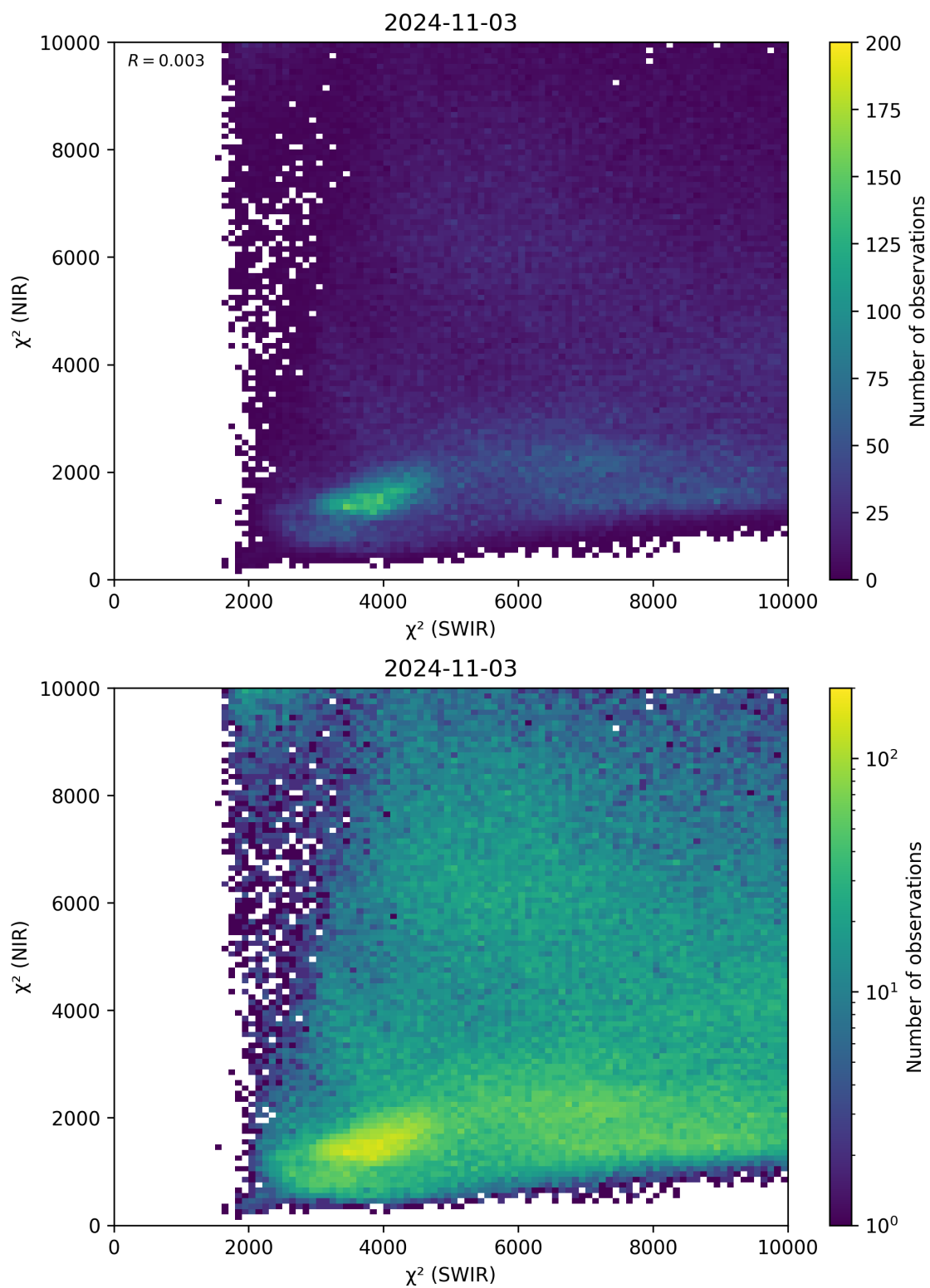
Figure 47: Scatter density plot of “ \chi^2 (SWIR)” against “ \chi^2 (NIR)” for 2024-11-02 to 2024-11-04.
