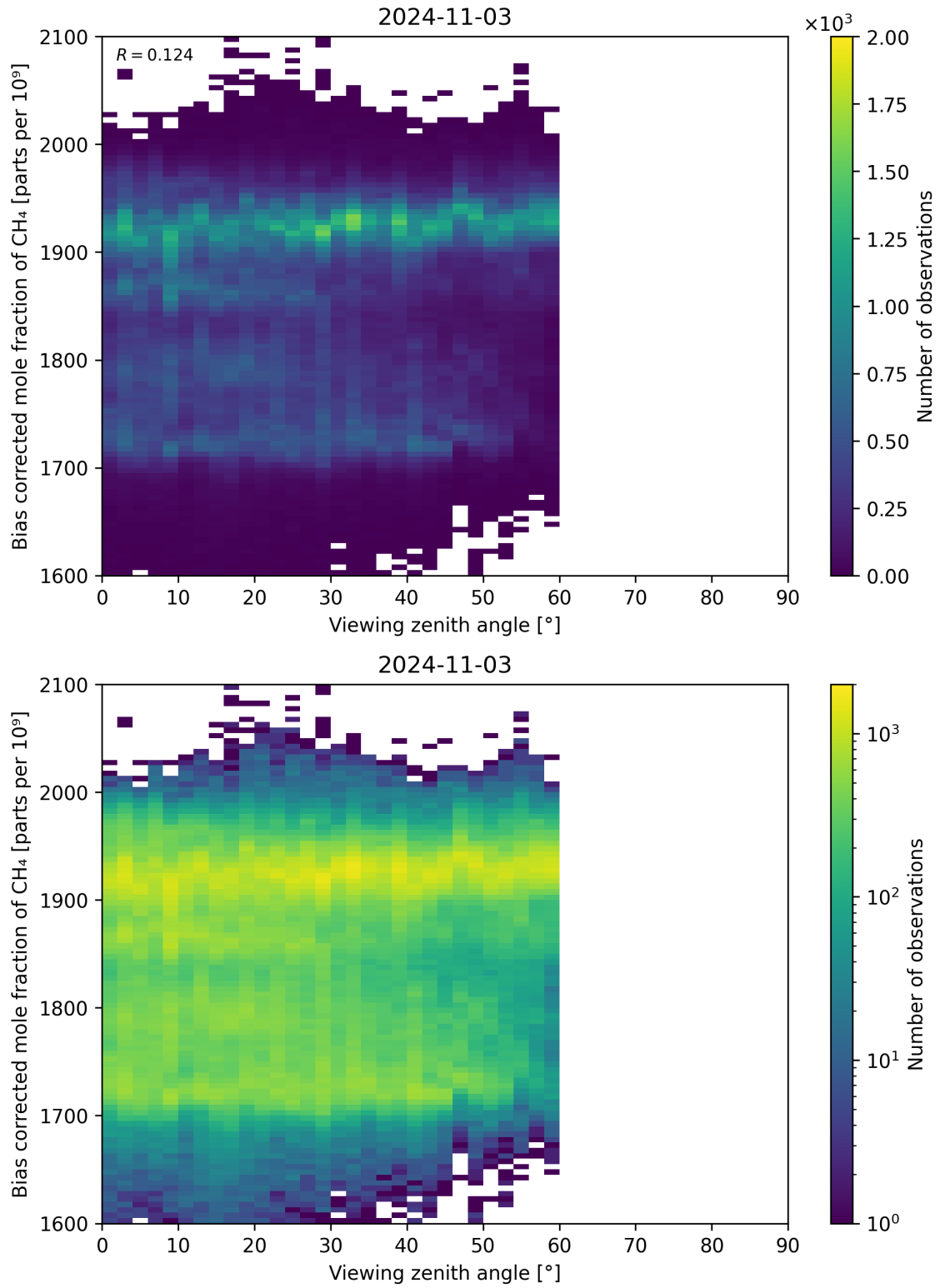
Figure 111: Scatter density plot of “Viewing zenith angle” against “Bias corrected mole fraction of CH 4 ” for 2024-11-02 to 2024-11-04.
