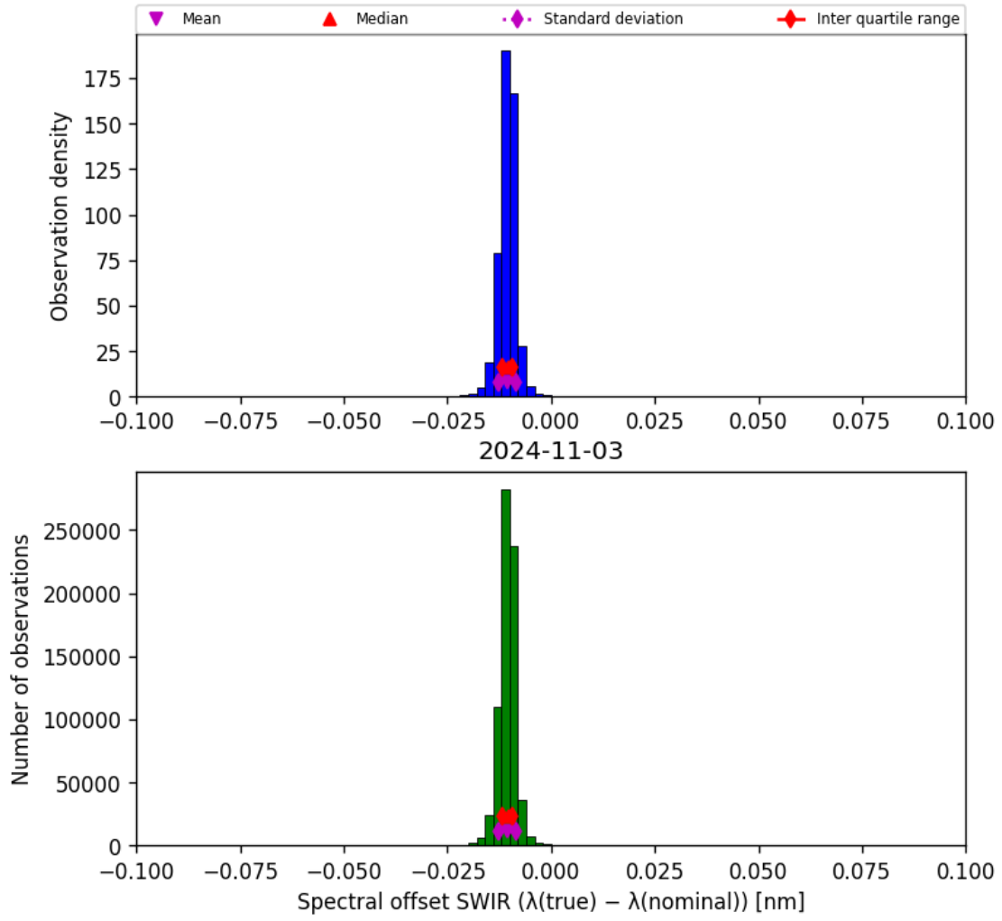
Figure 27: Histogram of “Spectral offset SWIR ( \lambda_{\text{true}} - \lambda_{\text{nominal}} )” for 2024-11-02 to 2024-11-04
