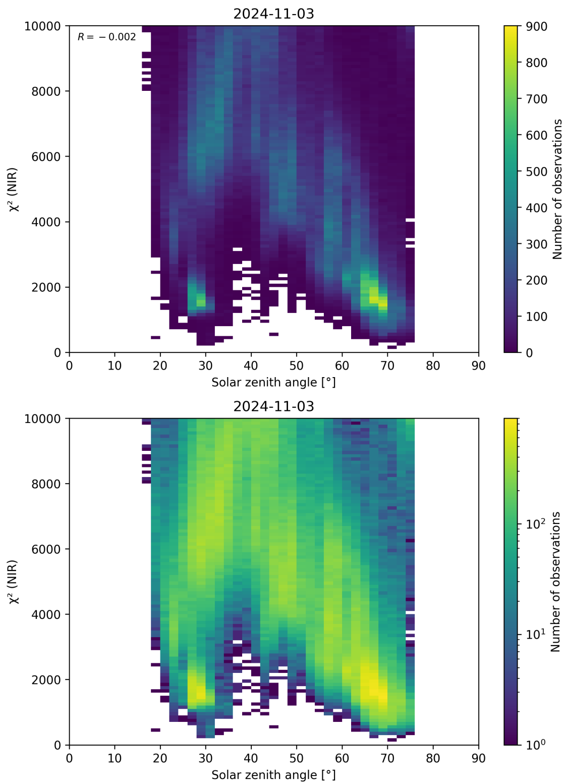
Figure 94: Scatter density plot of “Solar zenith angle” against “ \chi^2 (NIR)” for 2024-11-02 to 2024-11-04.
