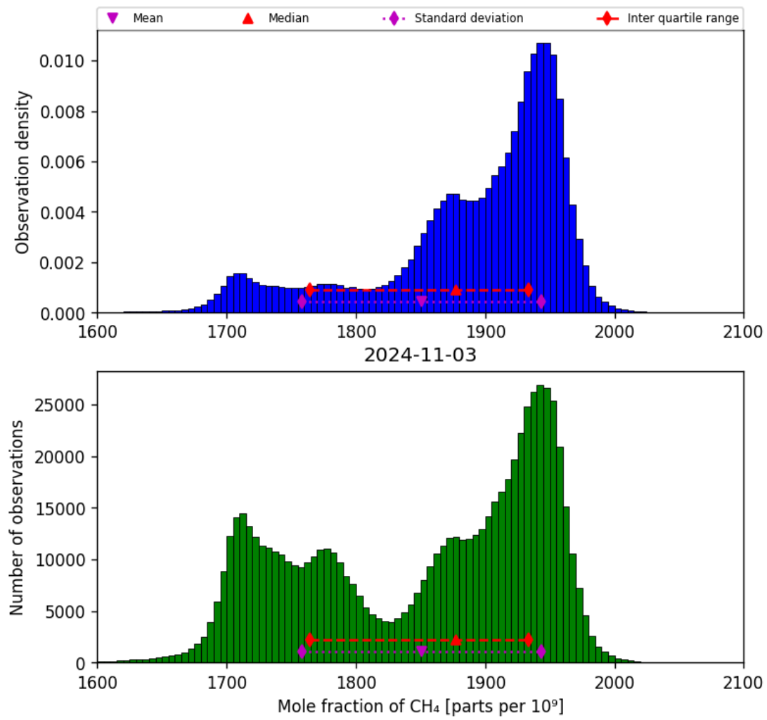
Figure 23: Histogram of “Mole fraction of CH 4 ” for 2024-11-02 to 2024-11-04
