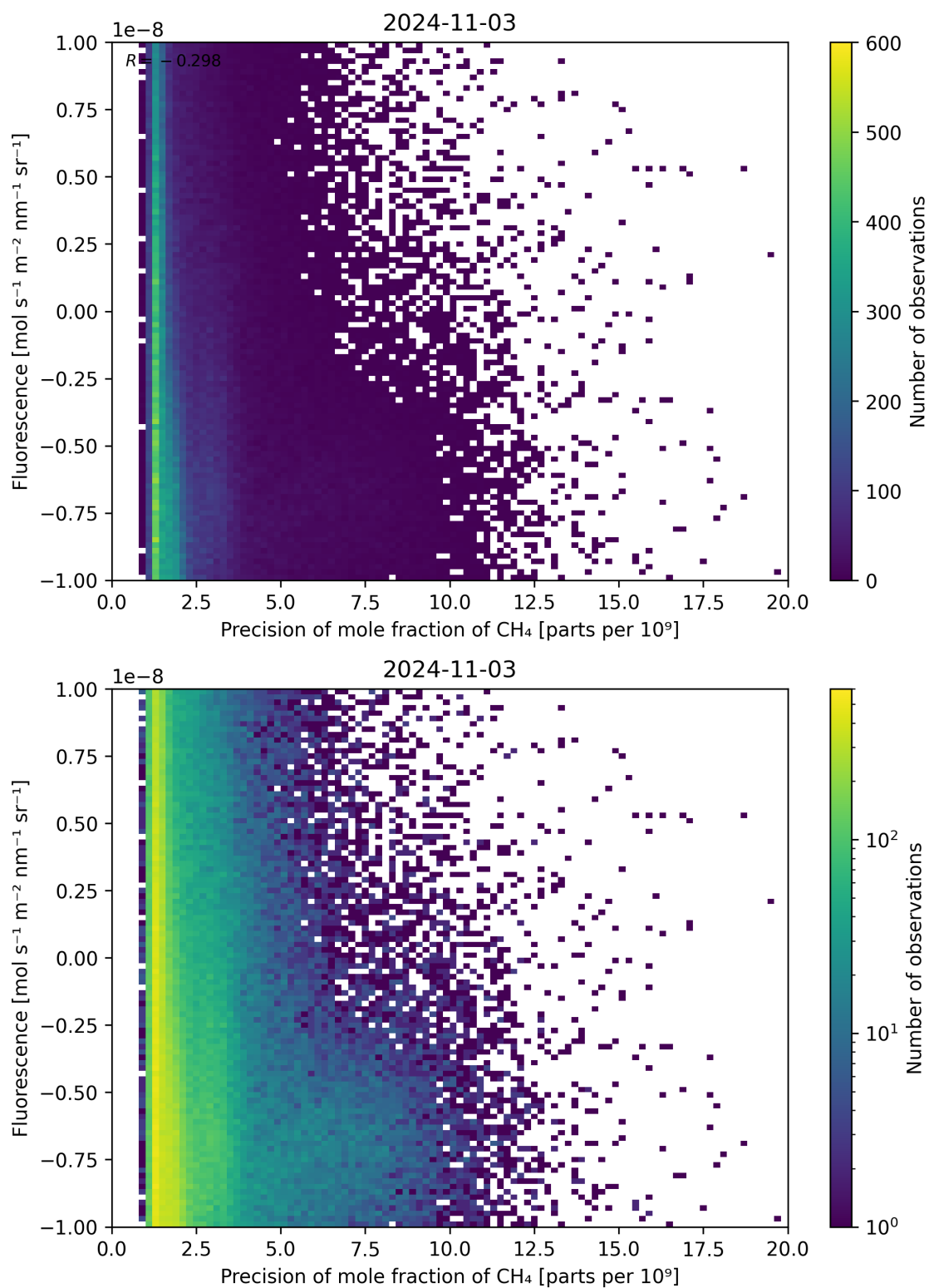
Figure 81: Scatter density plot of “Precision of mole fraction of \text{CH}_4 ” against “Fluorescence” for 2024-11-02 to 2024-11-04.
