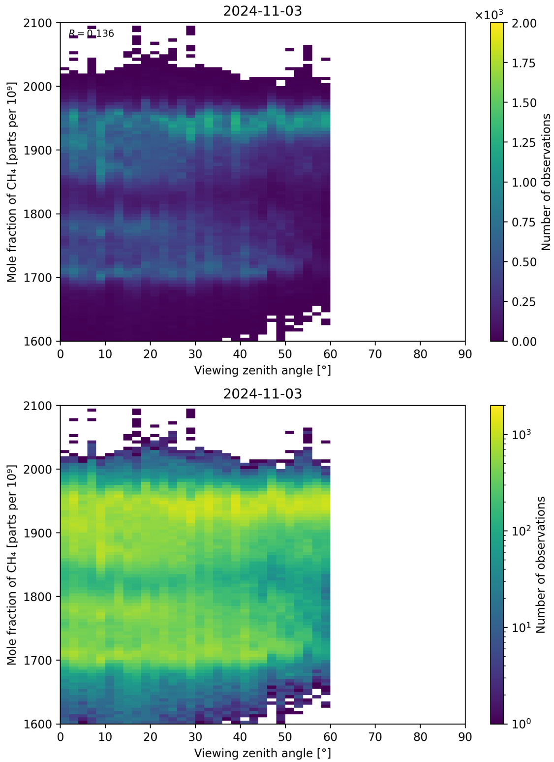
Figure 110: Scatter density plot of “Viewing zenith angle” against “Mole fraction of \text{CH}_4 ” for 2024-11-02 to 2024-11-04.
