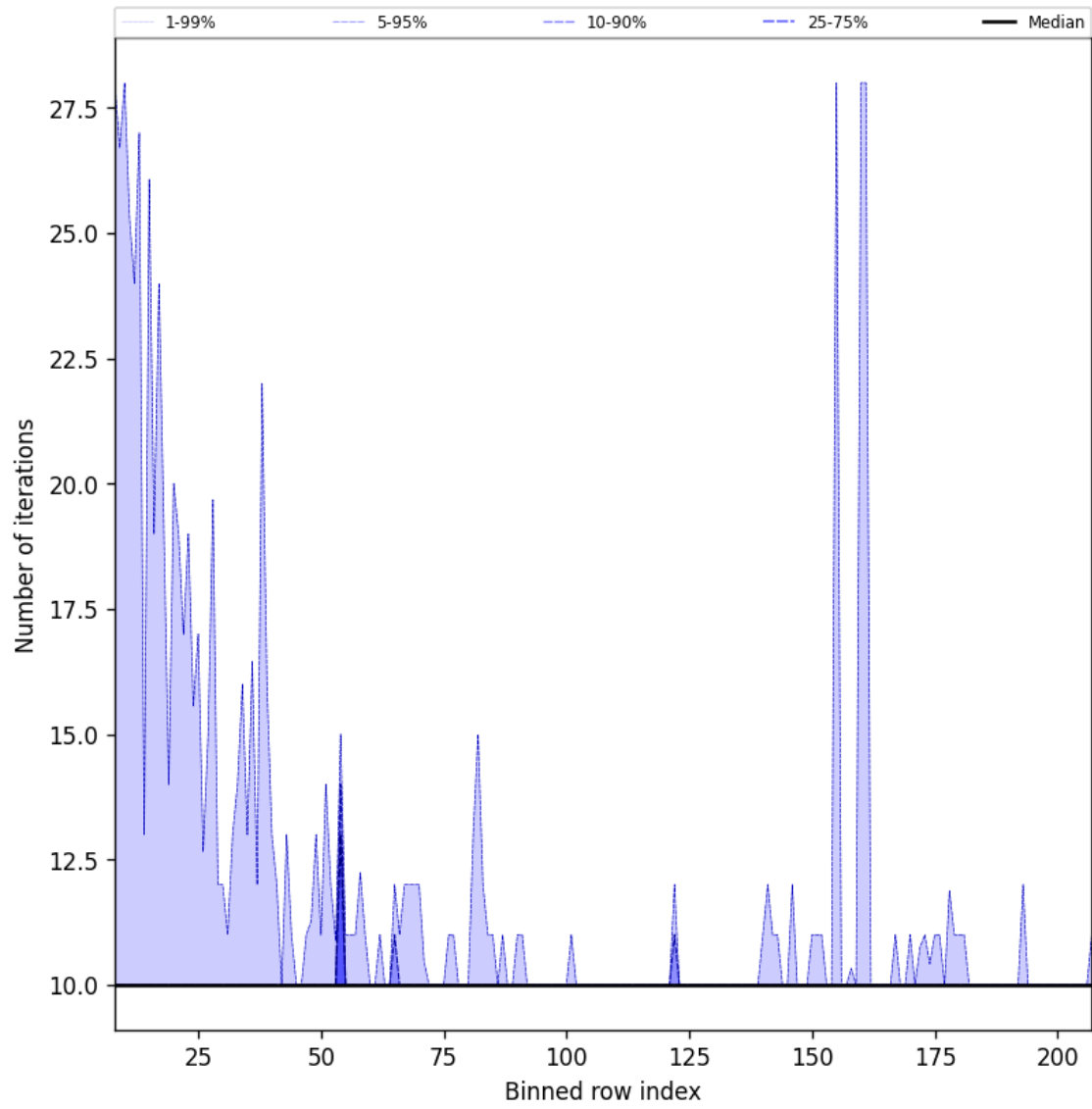
Figure 42: Along track statistics of “Number of iterations” for 2024-11-02 to 2024-11-04
