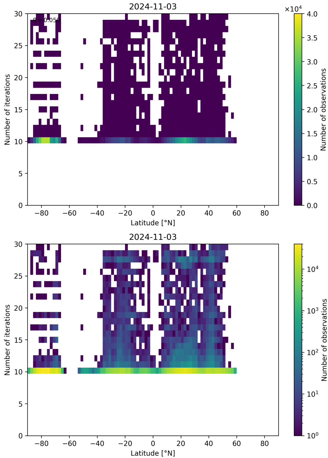
Figure 60: Scatter density plot of “Latitude” against “Number of iterations” for 2024-11-02 to 2024-11-04.
