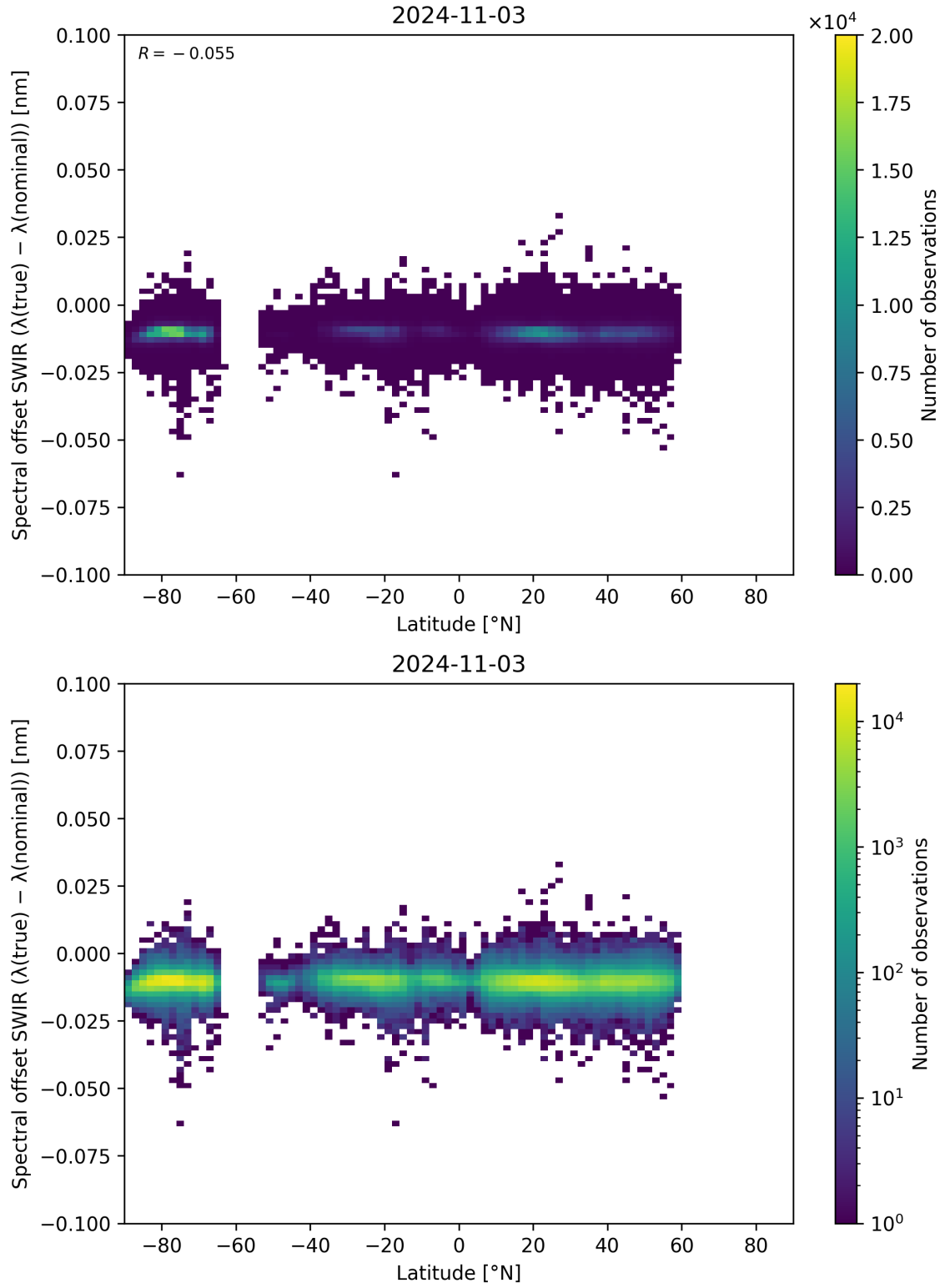
Figure 62: Scatter density plot of “Latitude” against “Spectral offset SWIR ( \lambda_{\text{true}} - \lambda_{\text{nominal}} )” for 2024-11-02 to 2024-11-04.
