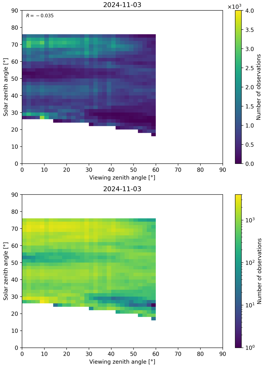
Figure 115: Scatter density plot of “Viewing zenith angle” against “Solar zenith angle” for 2024-11-02 to 2024-11-04.
