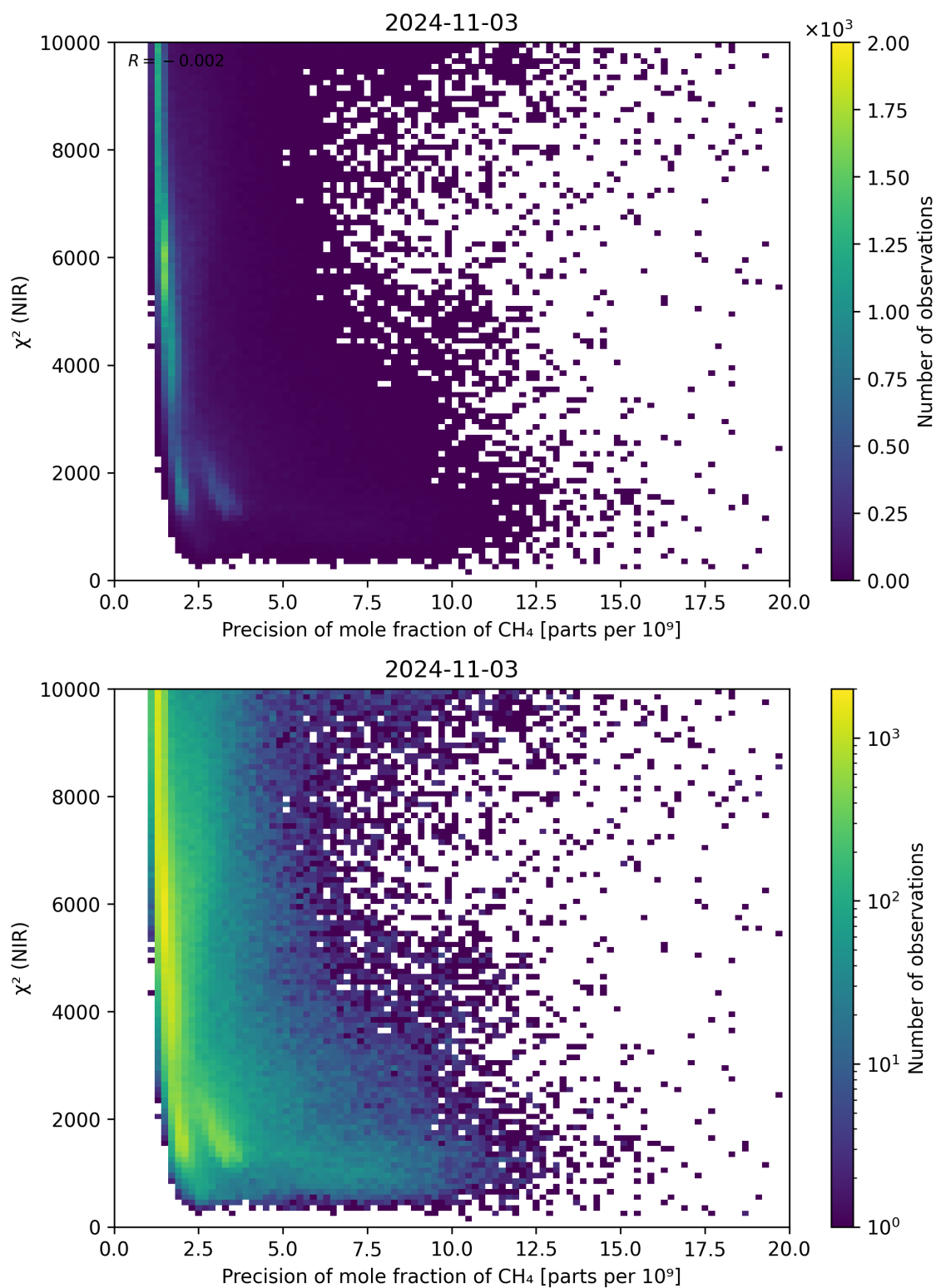
Figure 78: Scatter density plot of “Precision of mole fraction of CH 4 ” against “ \chi^2 (NIR)” for 2024-11-02 to 2024-11-04.
