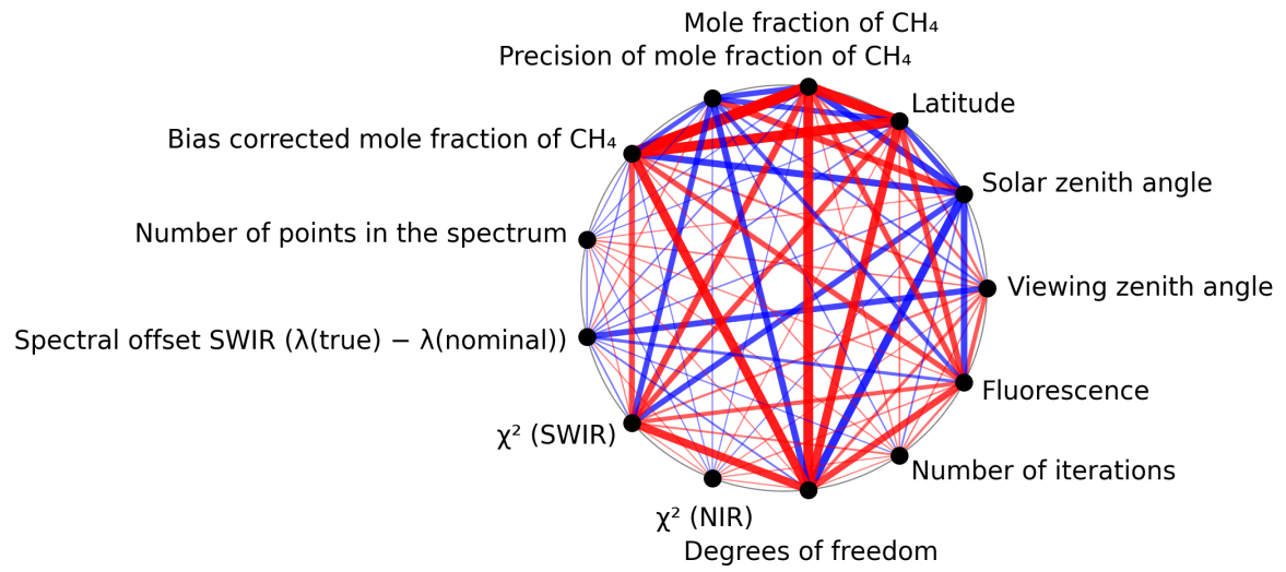
Figure 1: Map of correlation graph for 2024-11-02 to 2024-11-04.
