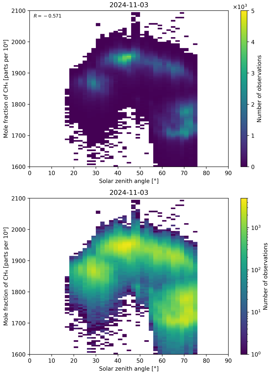
Figure 99: Scatter density plot of “Solar zenith angle” against “Mole fraction of CH 4 ” for 2024-11-02 to 2024-11-04.
