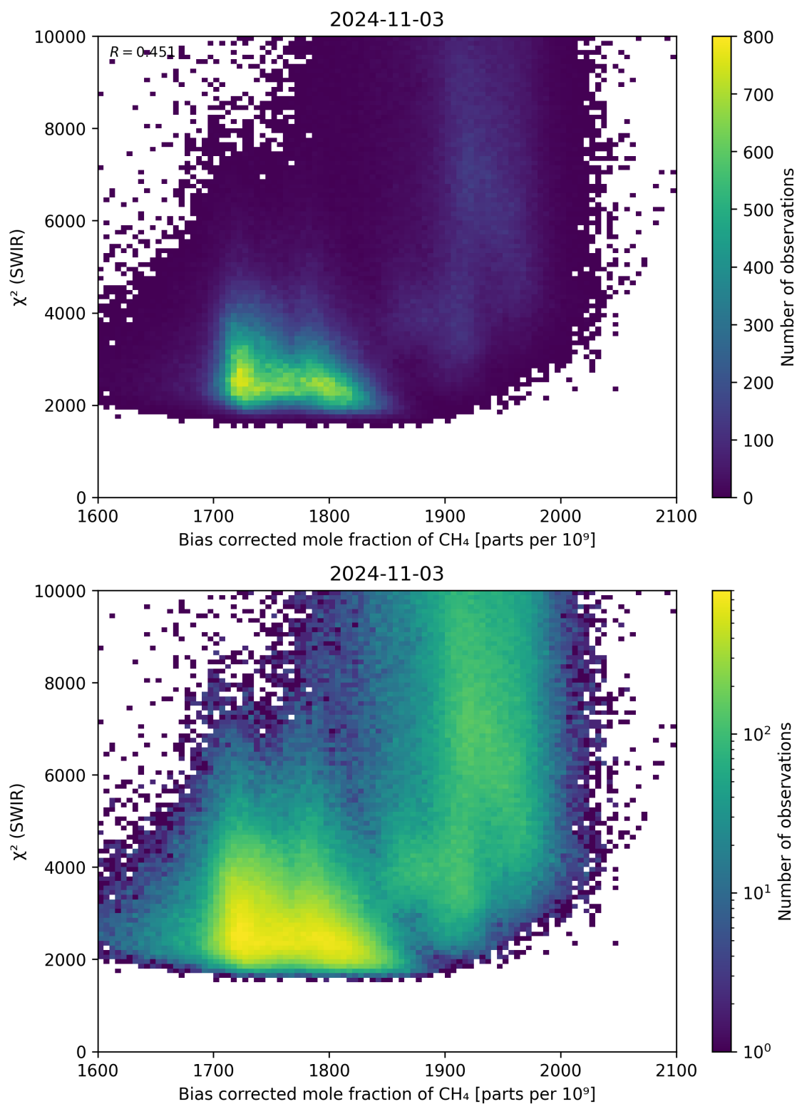
Figure 64: Scatter density plot of “Bias corrected mole fraction of \text{CH}_4 ” against “ \chi^2 (SWIR)” for 2024-11-02 to 2024-11-04.
