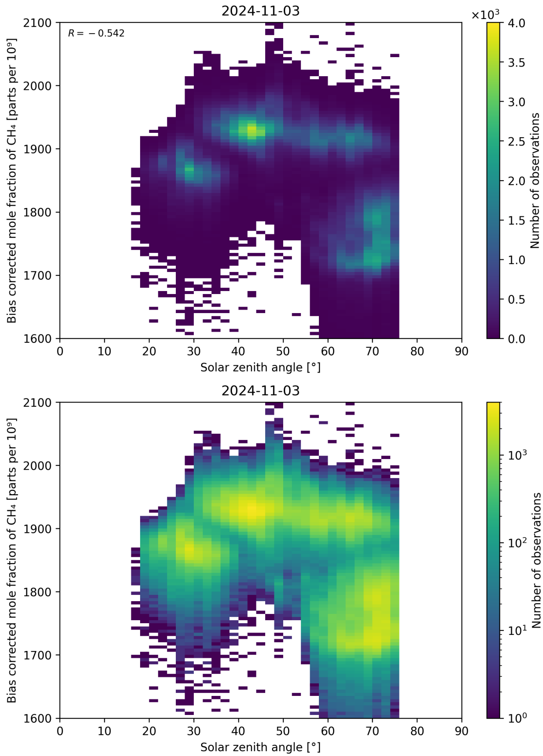
Figure 100: Scatter density plot of “Solar zenith angle” against “Bias corrected mole fraction of CH 4 ” for 2024-11-02 to 2024-11-04.
