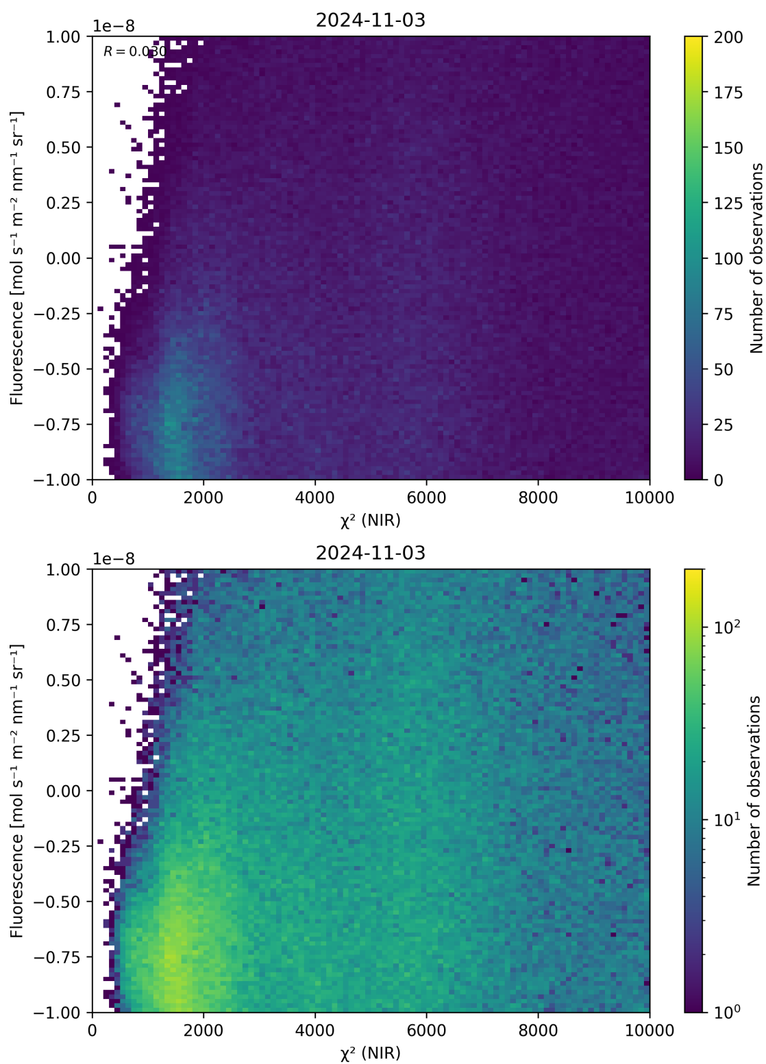
Figure 45: Scatter density plot of “ \chi^2 (NIR)” against “Fluorescence” for 2024-11-02 to 2024-11-04.
