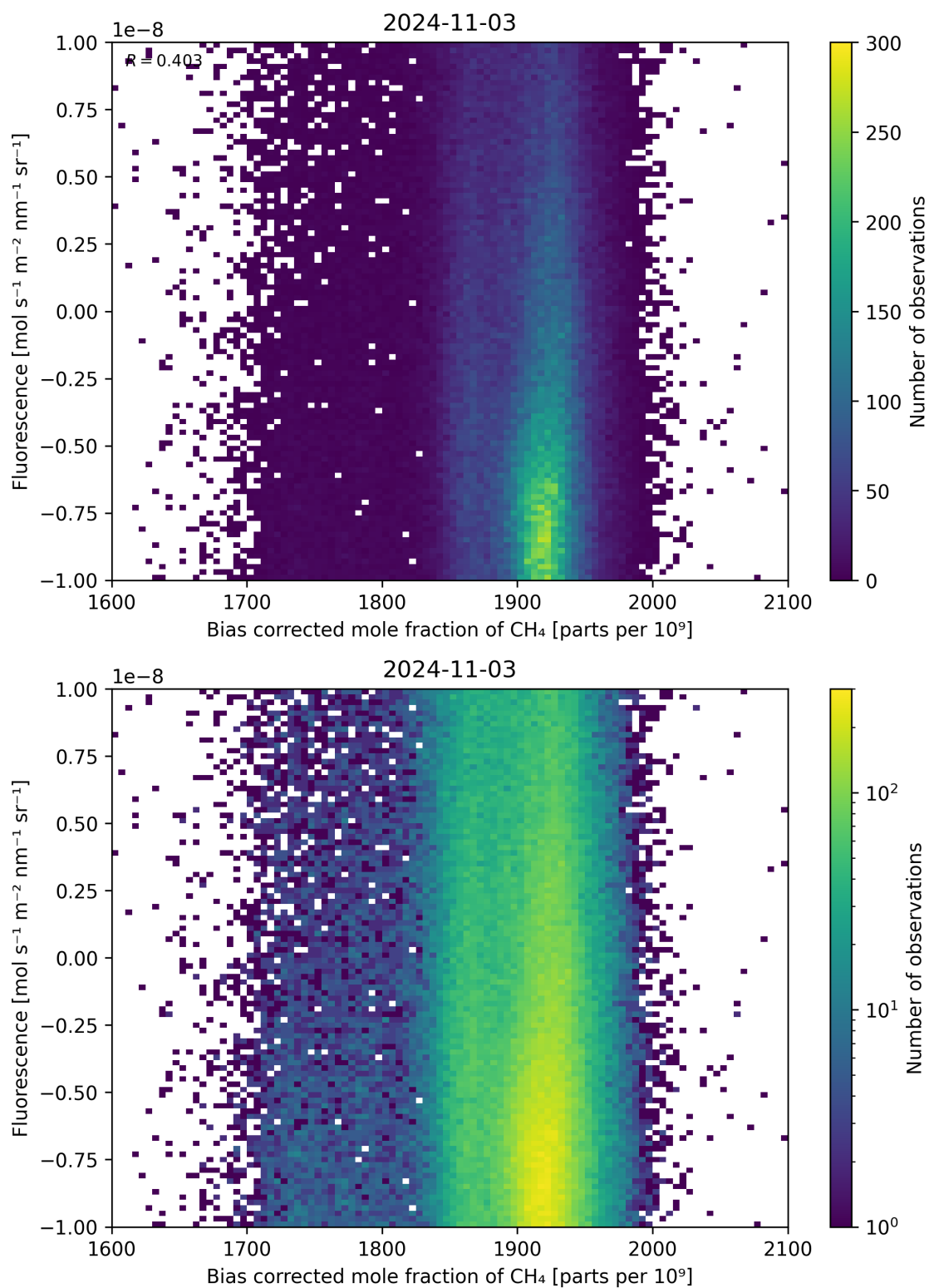
Figure 66: Scatter density plot of “Bias corrected mole fraction of \text{CH}_4 ” against “Fluorescence” for 2024-11-02 to 2024-11-04.
