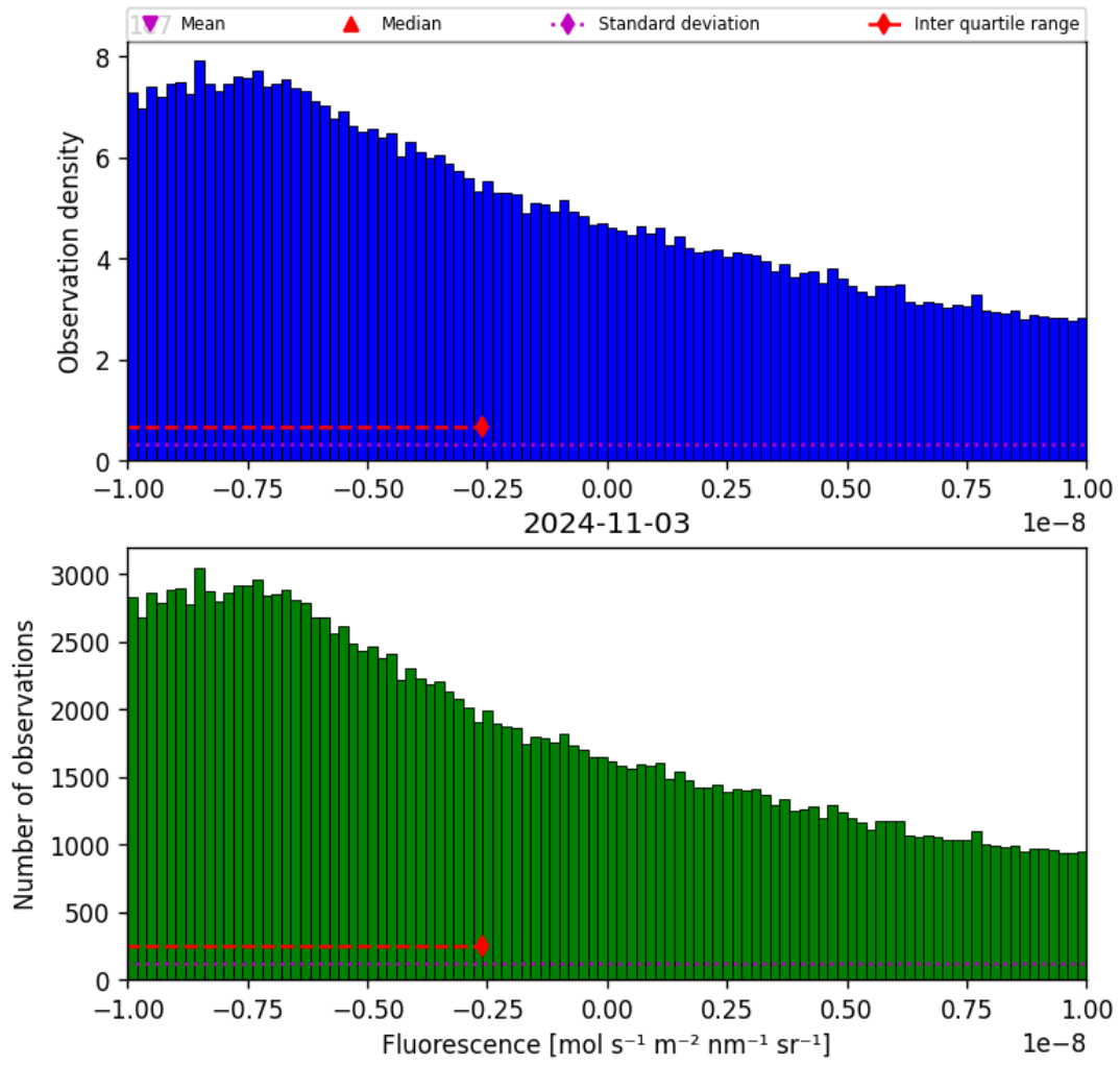
Figure 32: Histogram of “Fluorescence” for 2024-11-02 to 2024-11-04
