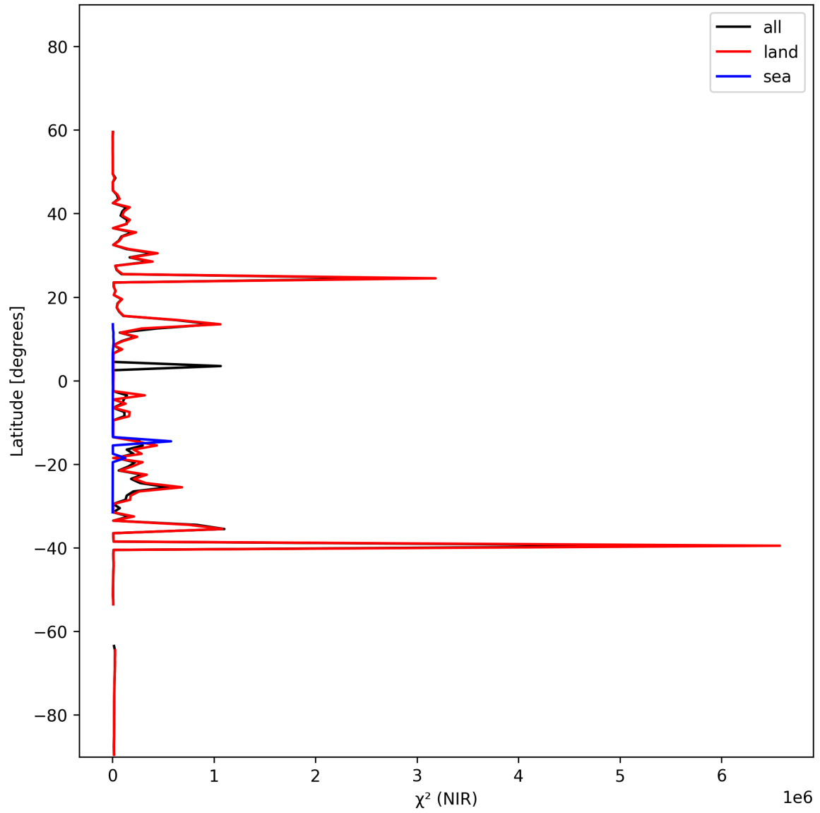
Figure 18: Zonal average of “ \chi^2 (NIR)” for 2024-11-02 to 2024-11-04.
