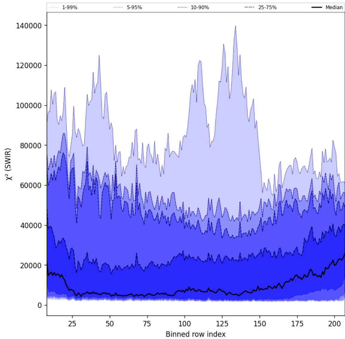
Figure 39: Along track statistics of “ \chi^2 (SWIR)” for 2024-11-02 to 2024-11-04
