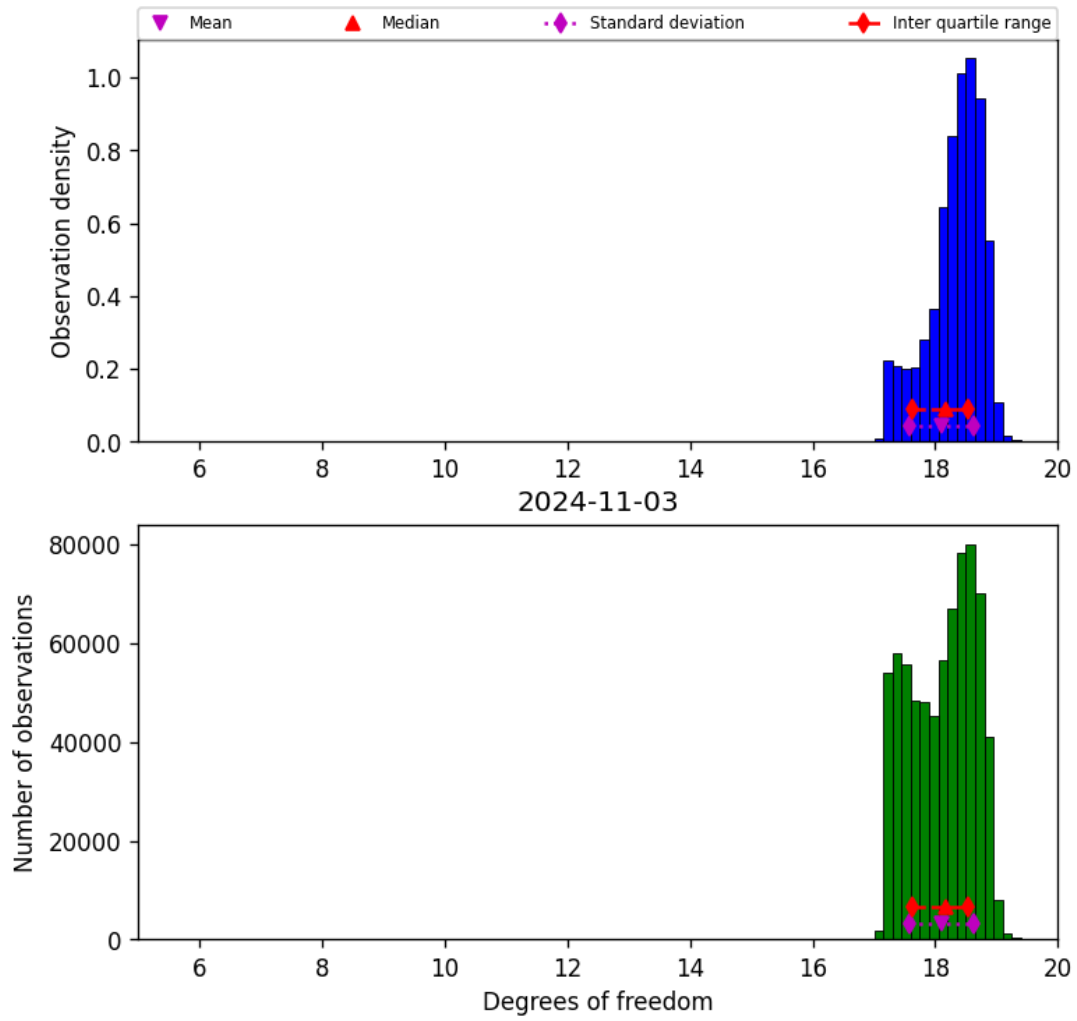
Figure 30: Histogram of “Degrees of freedom” for 2024-11-02 to 2024-11-04
