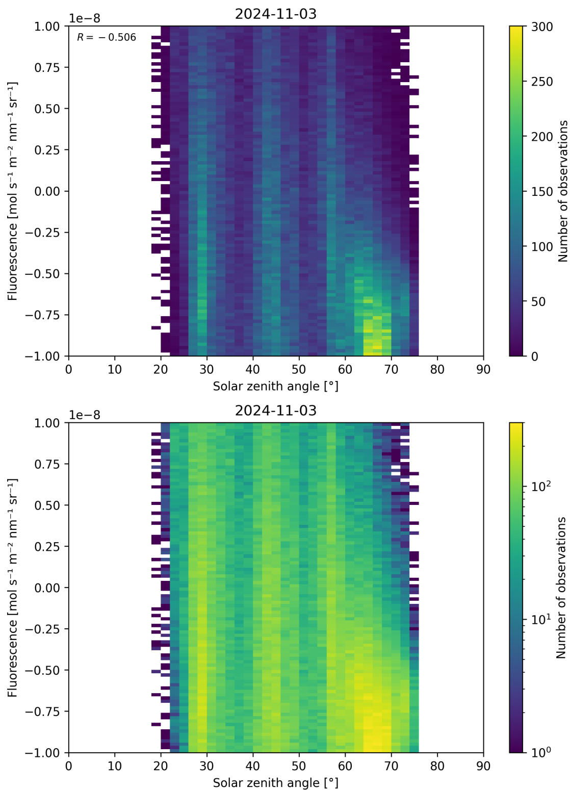
Figure 97: Scatter density plot of “Solar zenith angle” against “Fluorescence” for 2024-11-02 to 2024-11-04.
