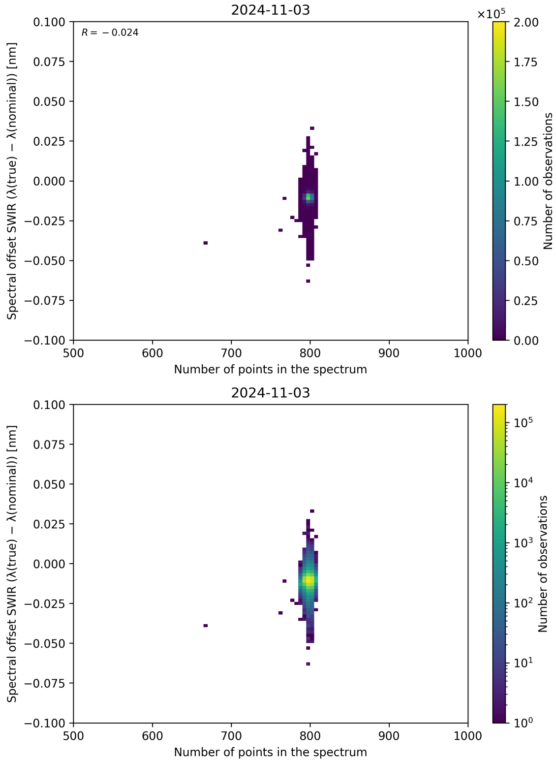
Figure 93: Scatter density plot of “Number of points in the spectrum” against “Spectral offset SWIR ( \lambda_{\text{true}} - \lambda_{\text{nominal}} )” for 2024-11-02 to 2024-11-04.
