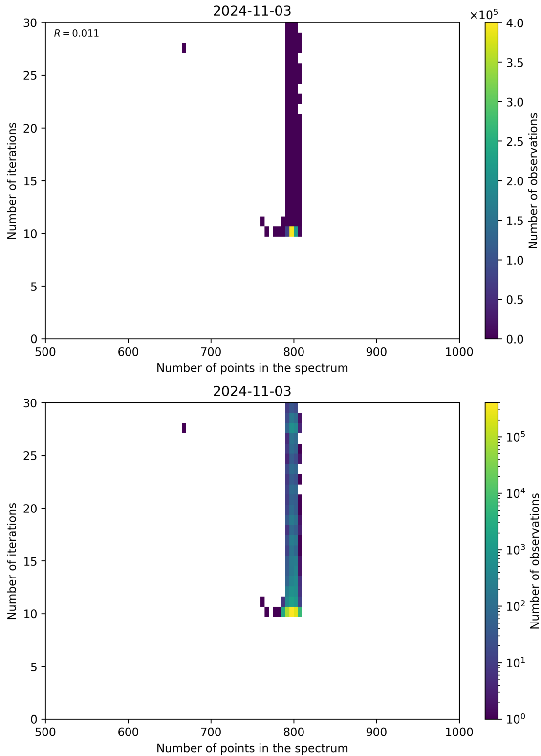
Figure 92: Scatter density plot of “Number of points in the spectrum” against “Number of iterations” for 2024-11-02 to 2024-11-04.
