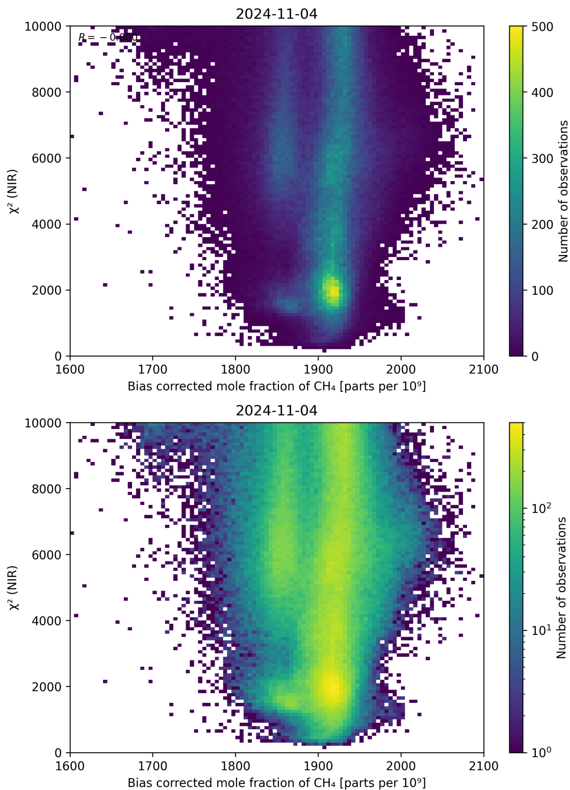
Figure 63: Scatter density plot of “Bias corrected mole fraction of CH 4 ” against “ \chi^2 (NIR)” for 2024-11-04 to 2024-11-05.
