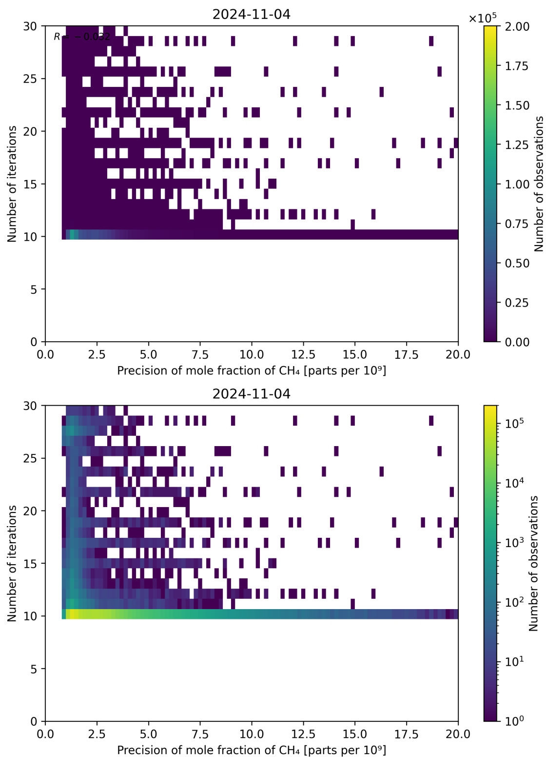
Figure 83: Scatter density plot of “Precision of mole fraction of CH 4 ” against “Number of iterations” for 2024-11-04 to 2024-11-05.
