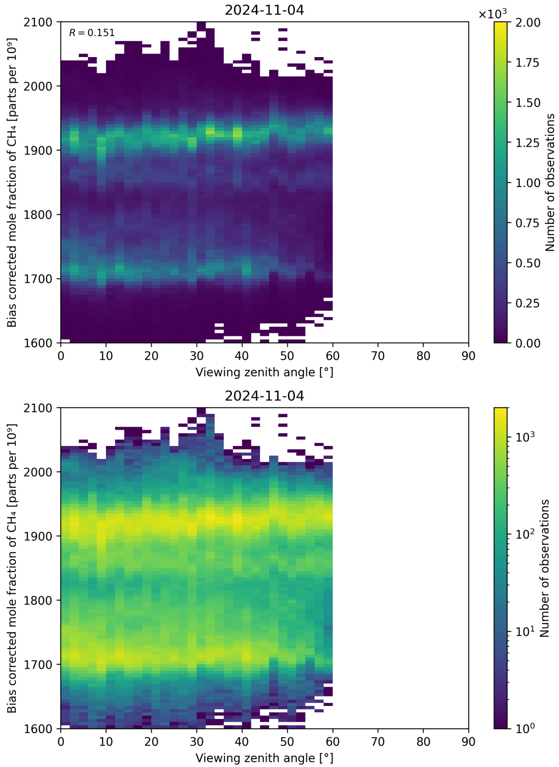
Figure 111: Scatter density plot of “Viewing zenith angle” against “Bias corrected mole fraction of CH 4 ” for 2024-11-04 to 2024-11-05.
