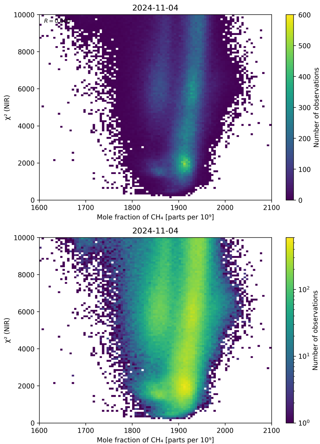
Figure 70: Scatter density plot of “Mole fraction of \text{CH}_4 ” against “ \chi^2 (NIR)” for 2024-11-04 to 2024-11-05.
