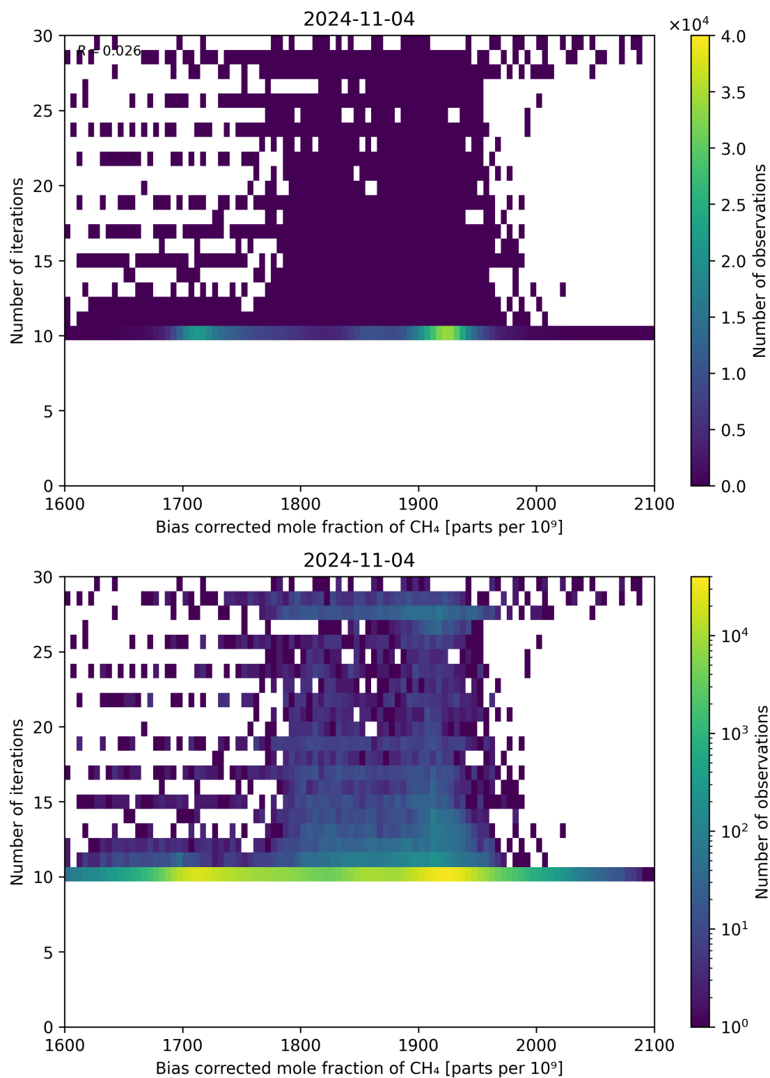
Figure 67: Scatter density plot of “Bias corrected mole fraction of \text{CH}_4 ” against “Number of iterations” for 2024-11-04 to 2024-11-05.
