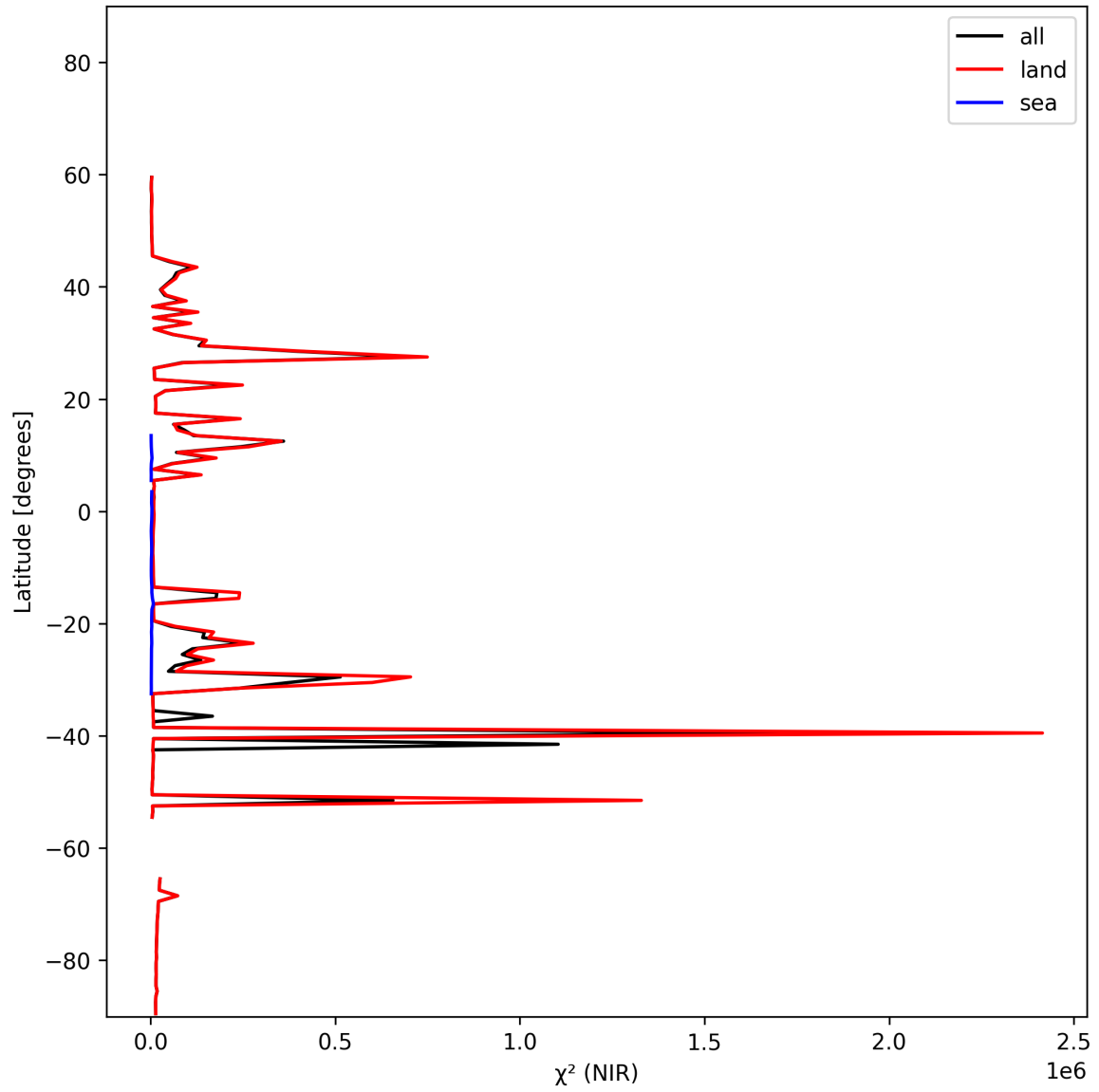
Figure 18: Zonal average of “ \chi^2 (NIR)” for 2024-11-04 to 2024-11-05.
