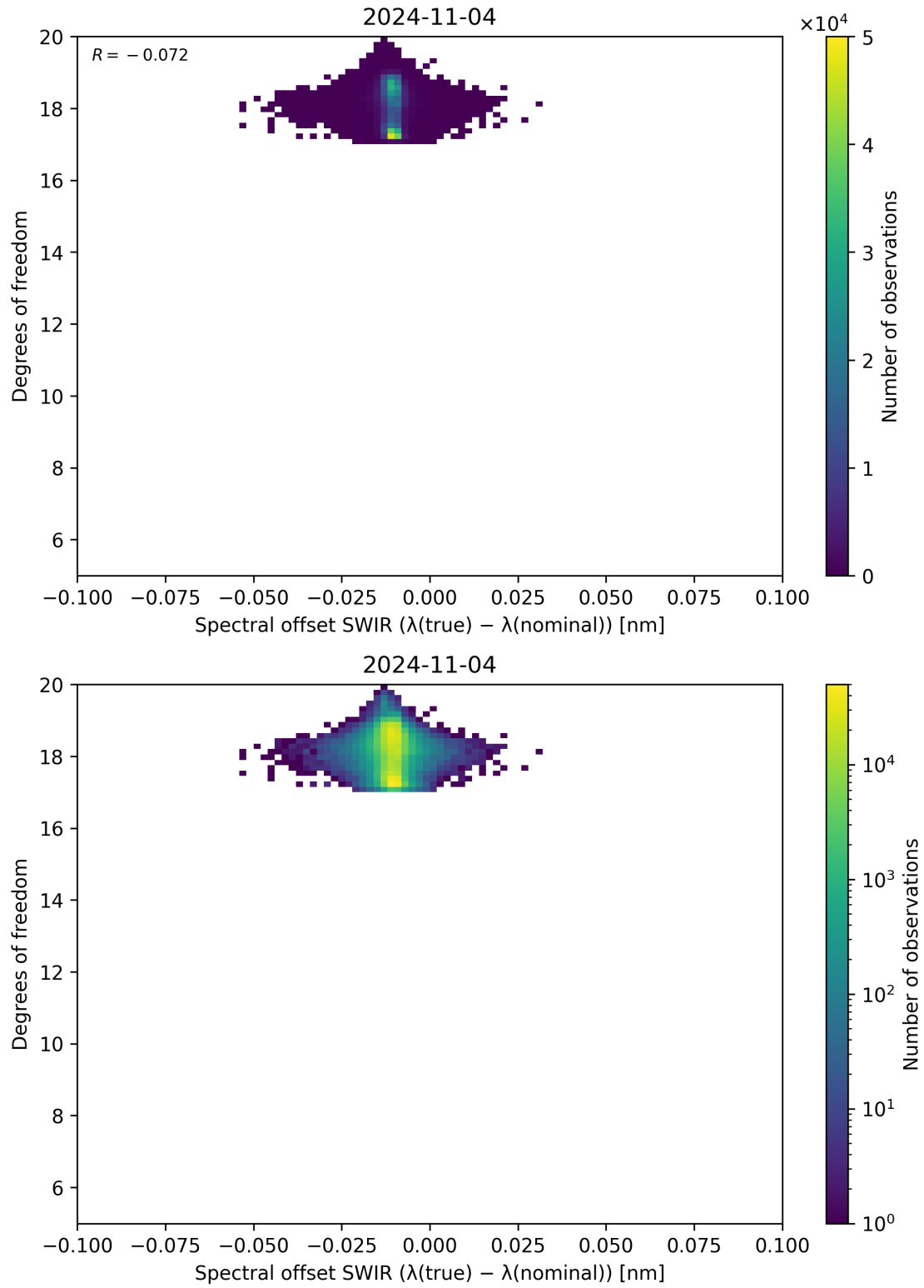
Figure 119: Scatter density plot of “Spectral offset SWIR ( \lambda_{\text{true}} - \lambda_{\text{nominal}} )” against “Degrees of freedom” for 2024-11-04 to 2024-11-05.
