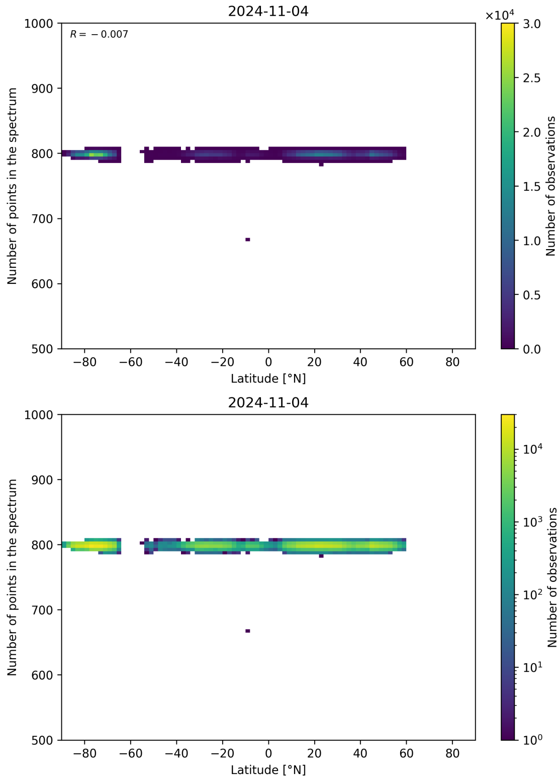
Figure 61: Scatter density plot of “Latitude” against “Number of points in the spectrum” for 2024-11-04 to 2024-11-05.
