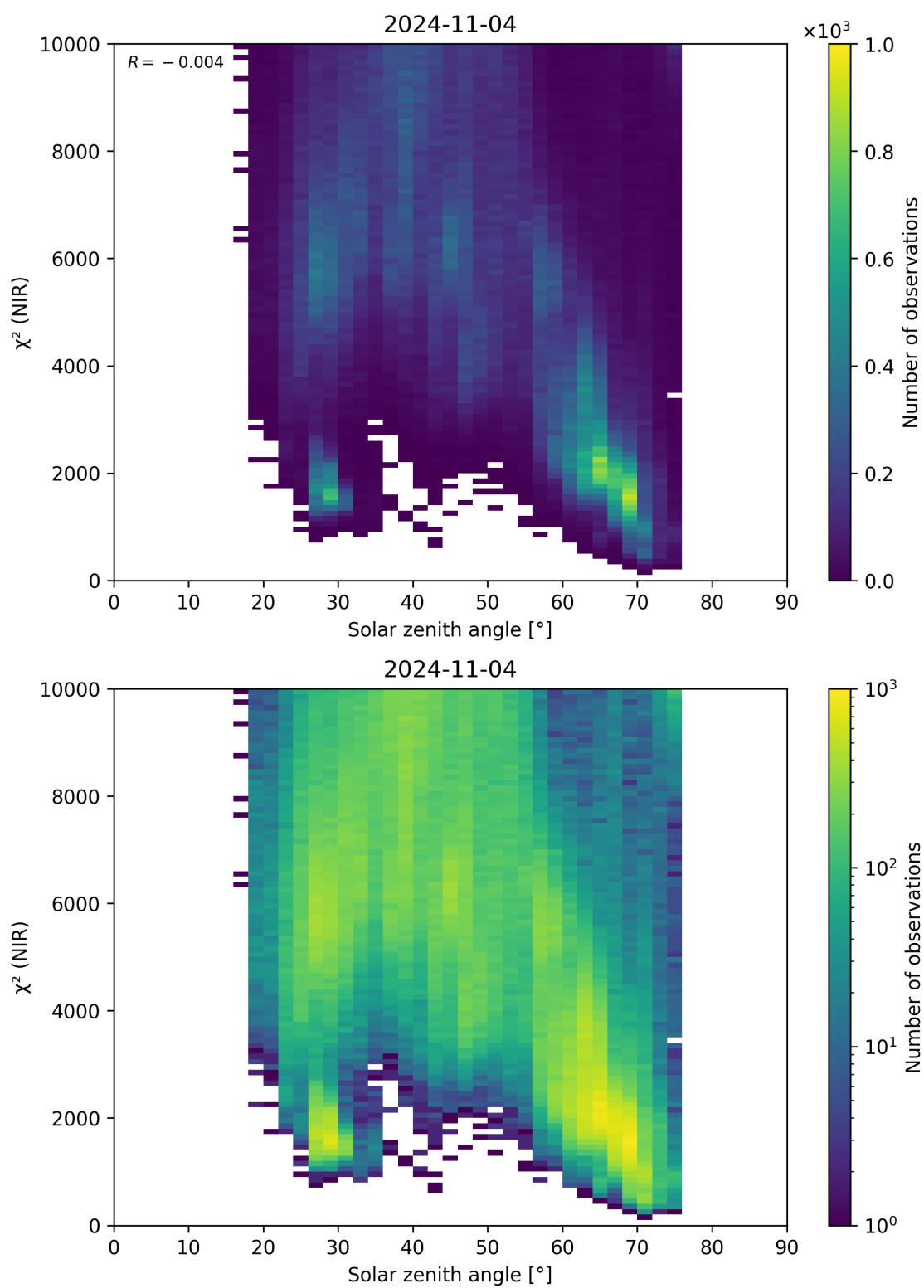
Figure 94: Scatter density plot of “Solar zenith angle” against “ \chi^2 (NIR)” for 2024-11-04 to 2024-11-05.
