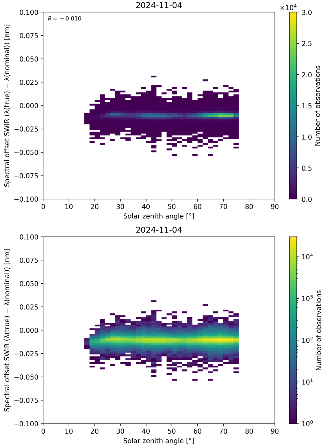
Figure 104: Scatter density plot of “Solar zenith angle” against “Spectral offset SWIR ( \lambda_{\text{true}} - \lambda_{\text{nominal}} )” for 2024-11-04 to 2024-11-05.
