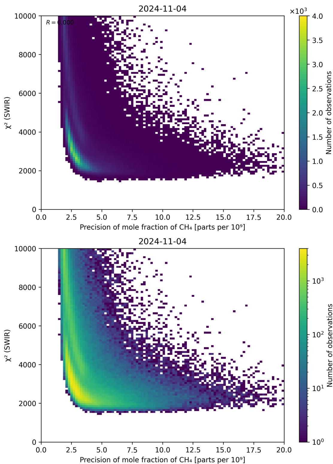
Figure 79: Scatter density plot of “Precision of mole fraction of \text{CH}_4 ” against “ \chi^2 (SWIR)” for 2024-11-04 to 2024-11-05.
