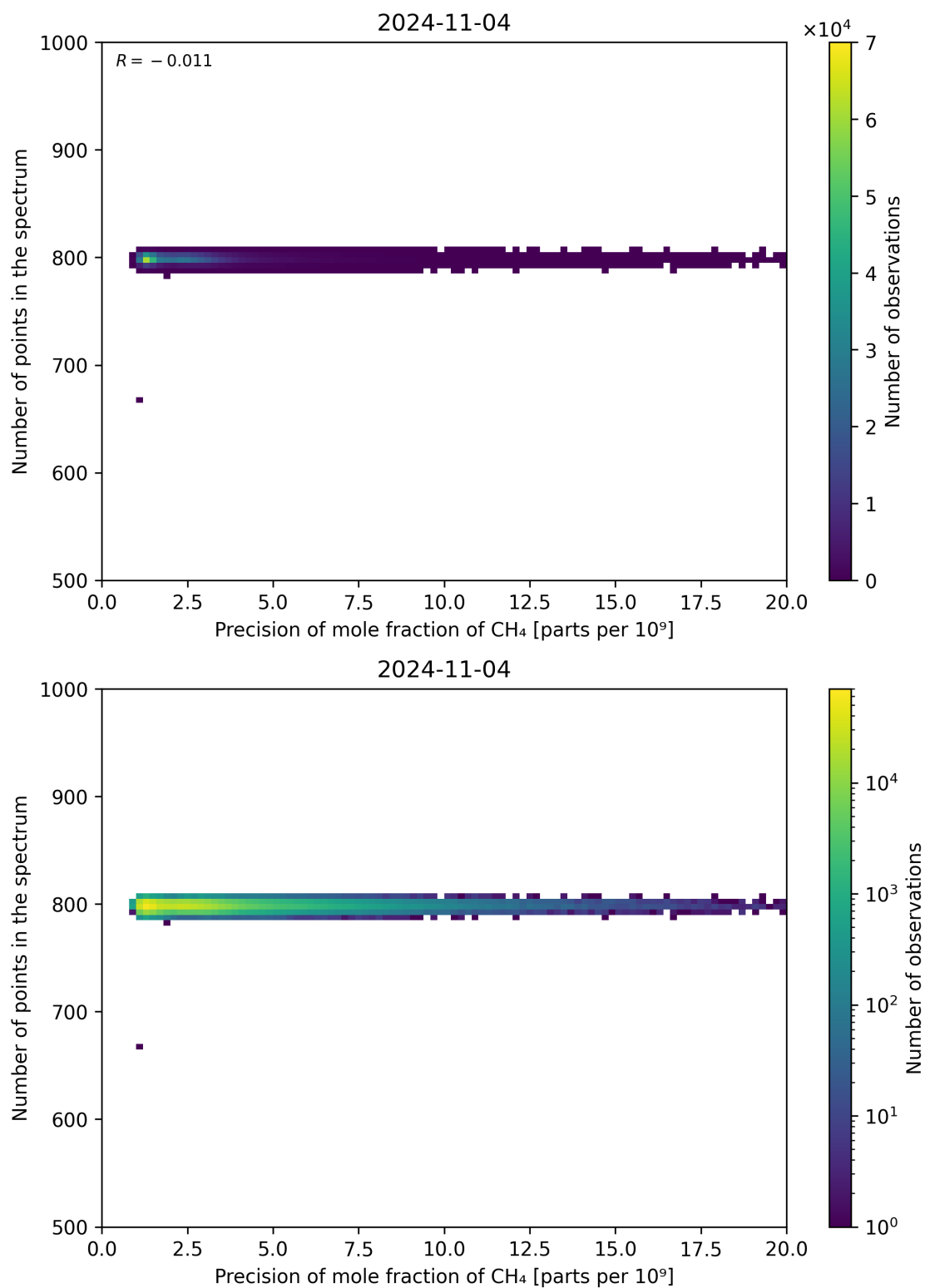
Figure 84: Scatter density plot of “Precision of mole fraction of CH 4 ” against “Number of points in the spectrum” for 2024-11-04 to 2024-11-05.
