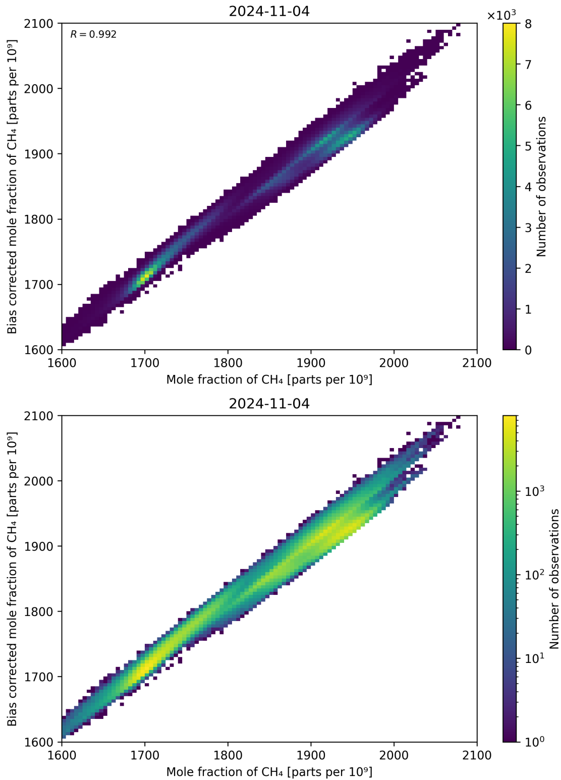
Figure 74: Scatter density plot of “Mole fraction of CH 4 ” against “Bias corrected mole fraction of CH 4 ” for 2024-11-04 to 2024-11-05.
