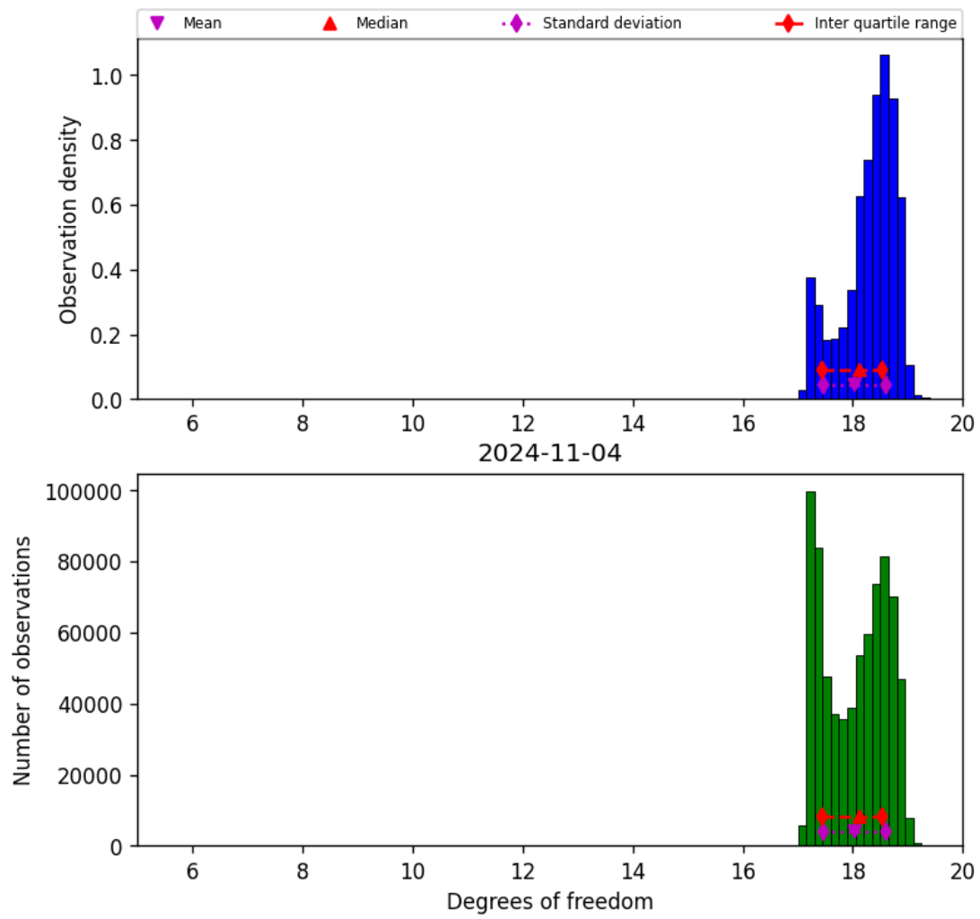
Figure 30: Histogram of “Degrees of freedom” for 2024-11-04 to 2024-11-05
