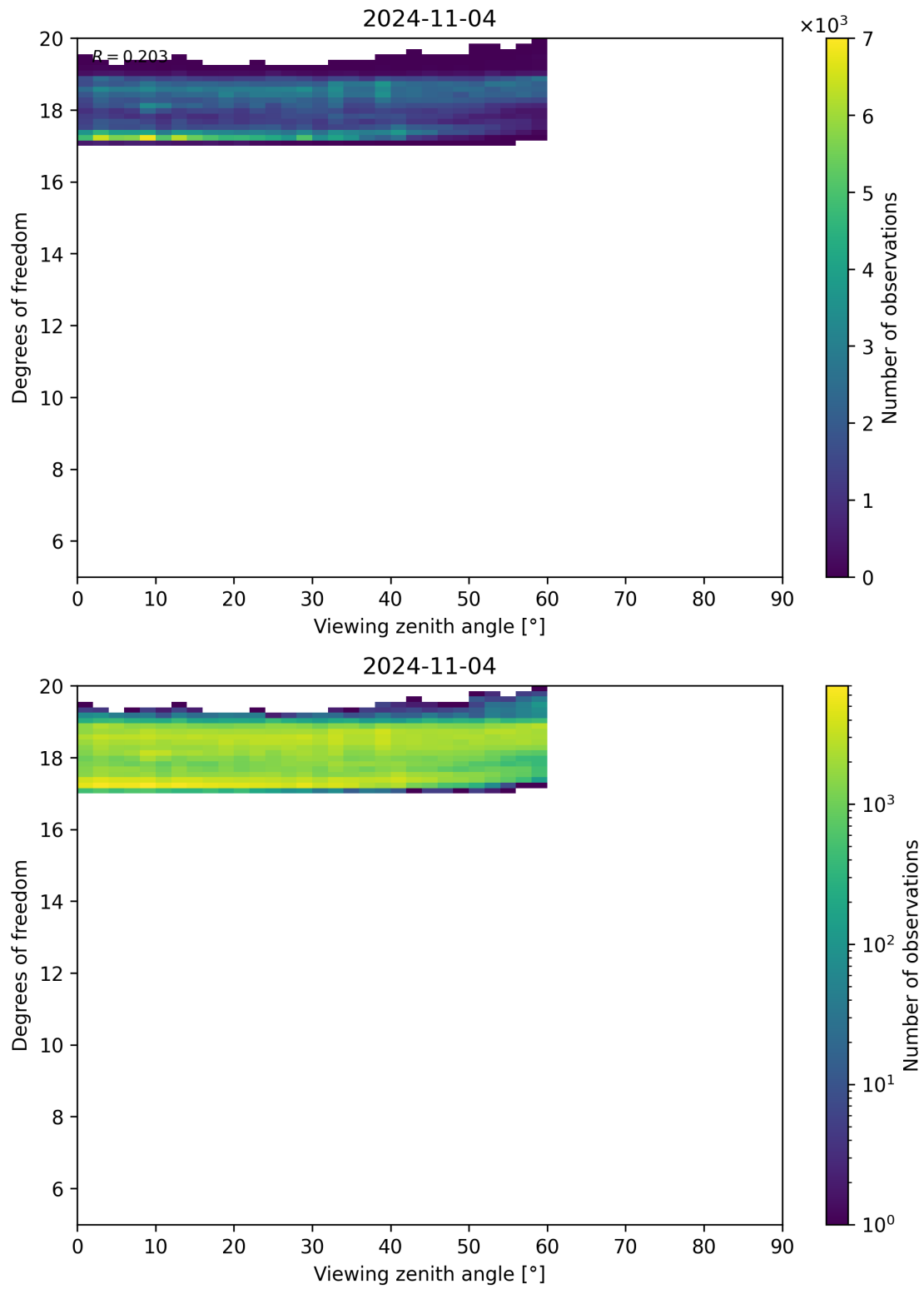
Figure 107: Scatter density plot of “Viewing zenith angle” against “Degrees of freedom” for 2024-11-04 to 2024-11-05.
