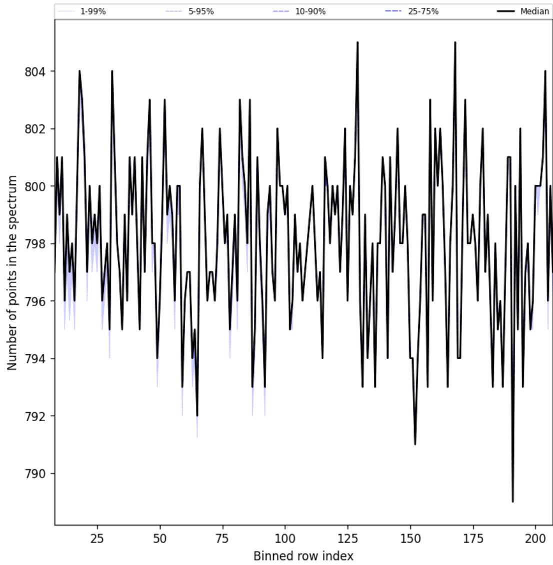
Figure 37: Along track statistics of “Number of points in the spectrum” for 2024-11-04 to 2024-11-05
