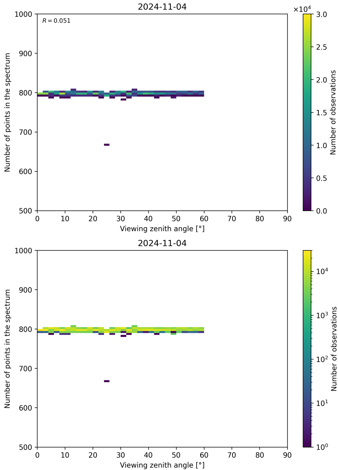
Figure 114: Scatter density plot of “Viewing zenith angle” against “Number of points in the spectrum” for 2024-11-04 to 2024-11-05.
