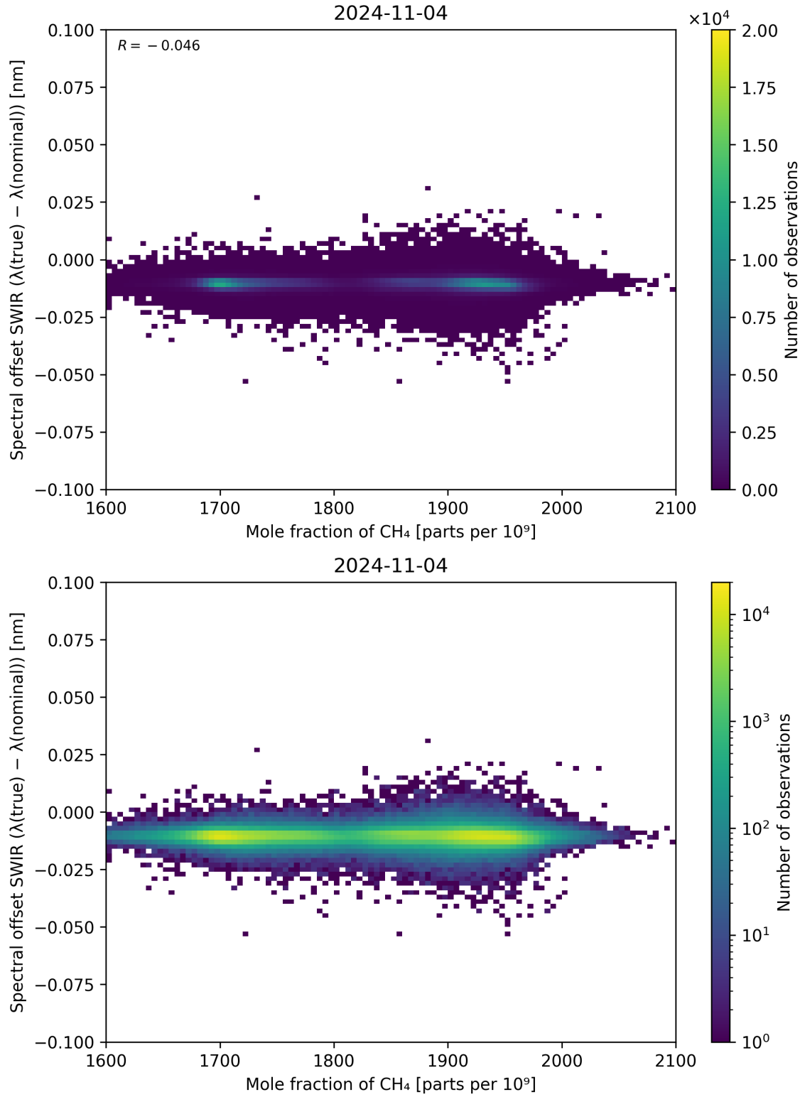
Figure 86: Scatter density plot of “Mole fraction of CH 4 ” against “Spectral offset SWIR ( \lambda_{\text{true}} - \lambda_{\text{nominal}} )” for 2024-11-04 to 2024-11-05.
