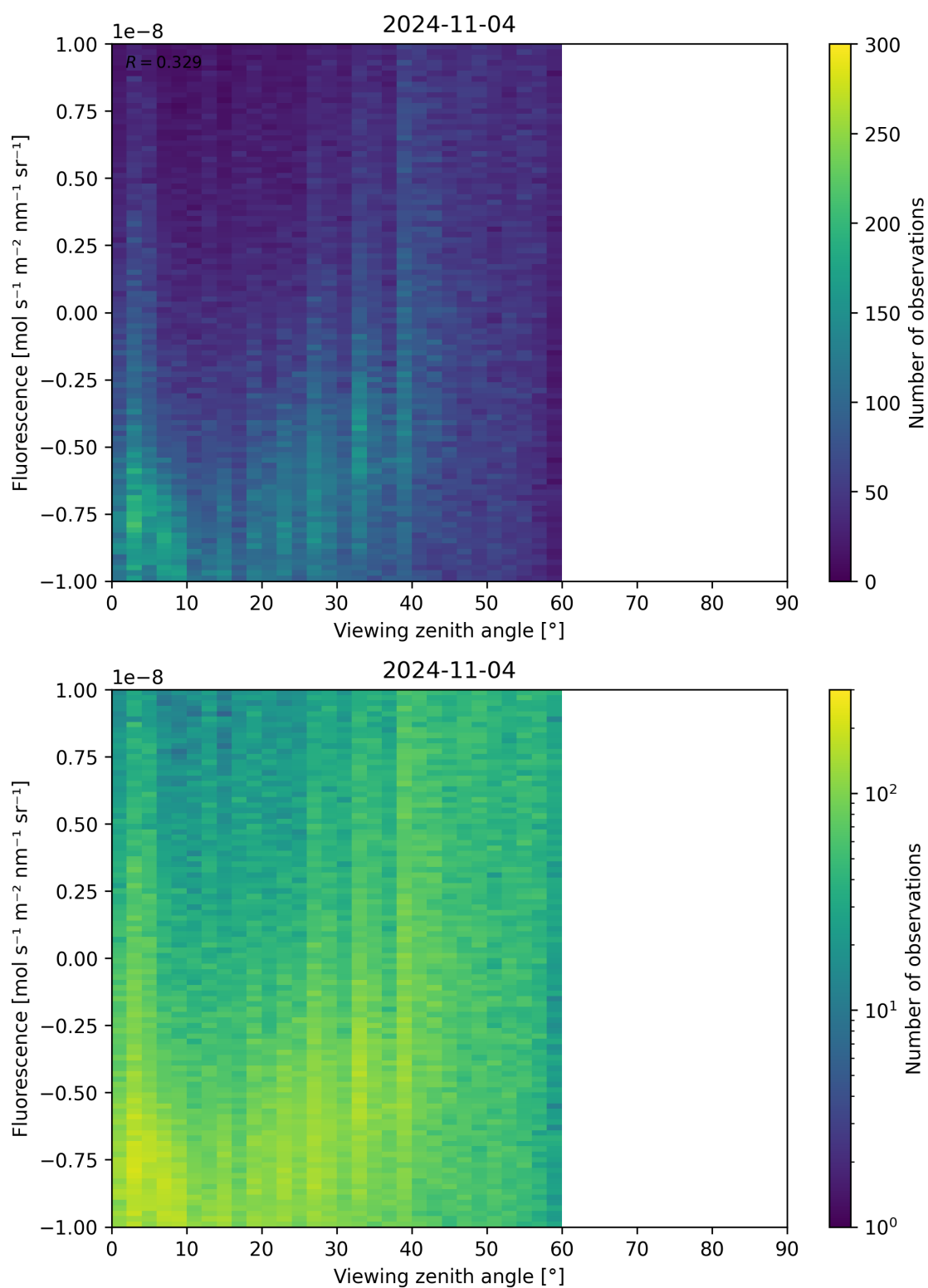
Figure 108: Scatter density plot of “Viewing zenith angle” against “Fluorescence” for 2024-11-04 to 2024-11-05.
