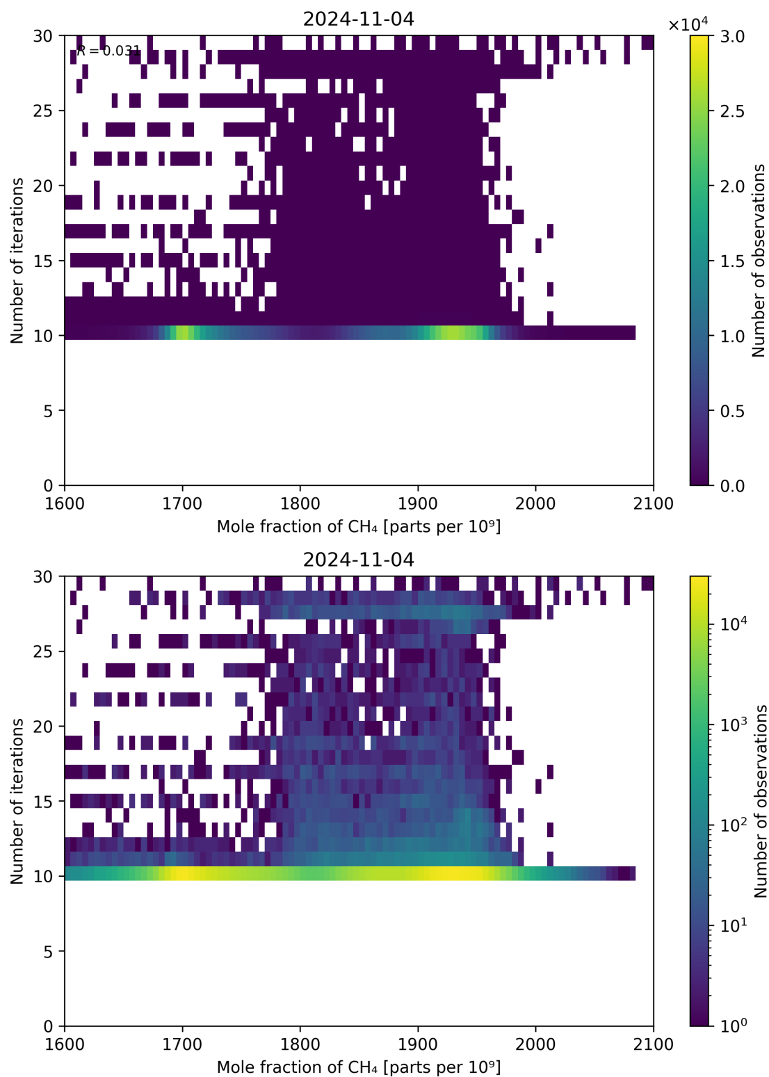
Figure 76: Scatter density plot of “Mole fraction of CH 4 ” against “Number of iterations” for 2024-11-04 to 2024-11-05.
