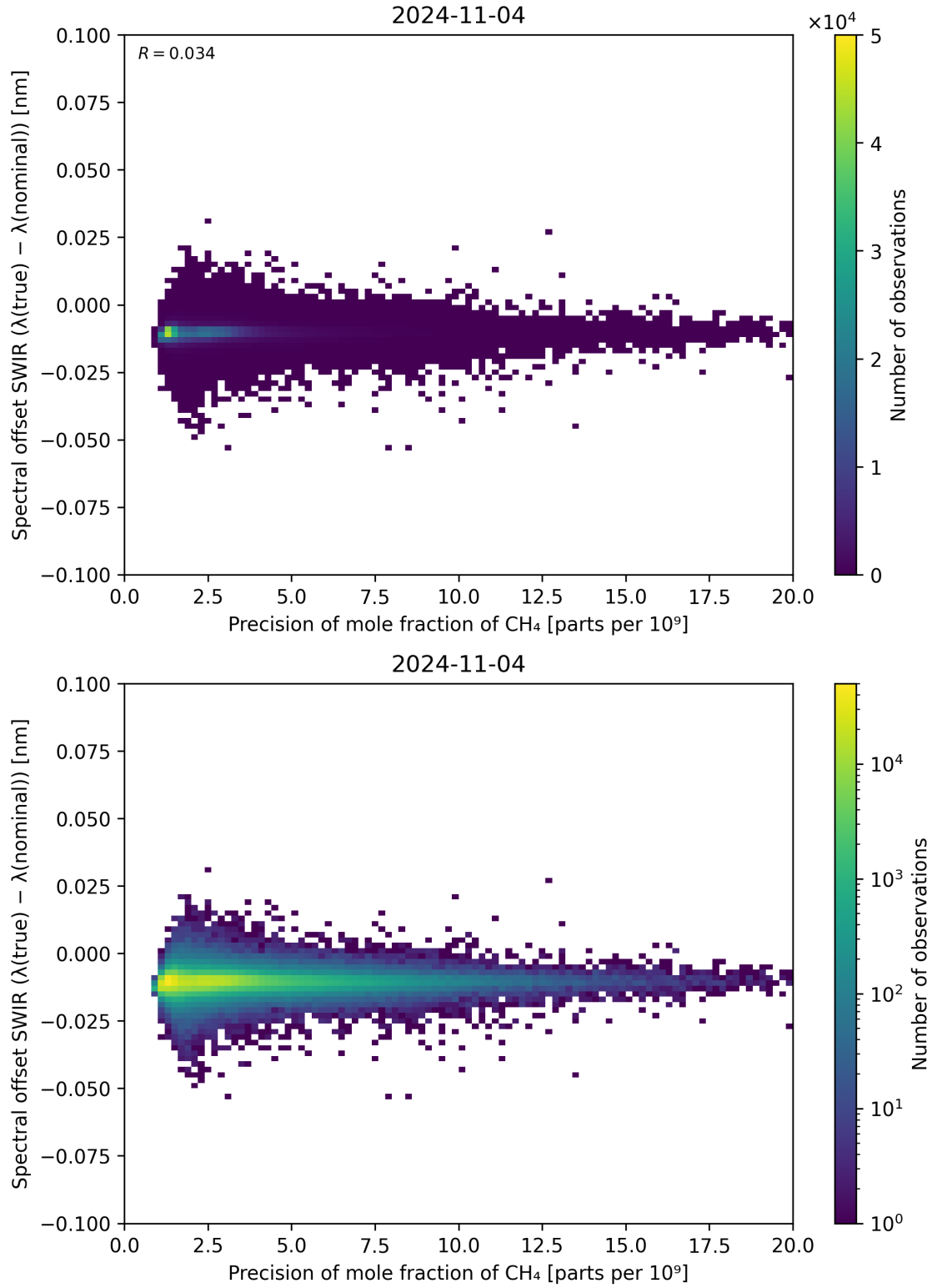
Figure 85: Scatter density plot of “Precision of mole fraction of \text{CH}_4 ” against “Spectral offset SWIR ( \lambda_{\text{true}} - \lambda_{\text{nominal}} )” for 2024-11-04 to 2024-11-05.
