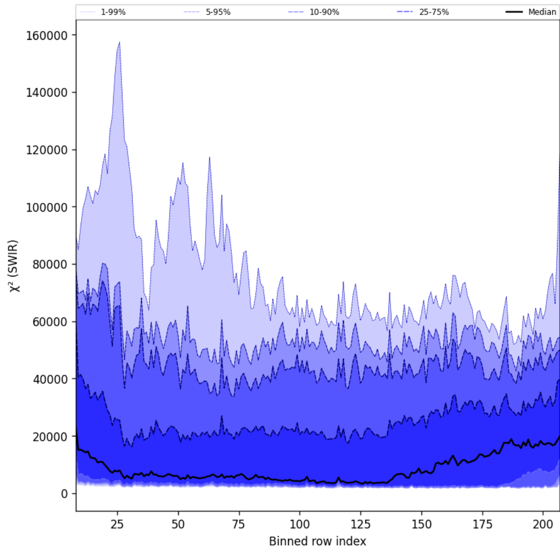
Figure 39: Along track statistics of “ \chi^2 (SWIR)” for 2024-11-04 to 2024-11-05
