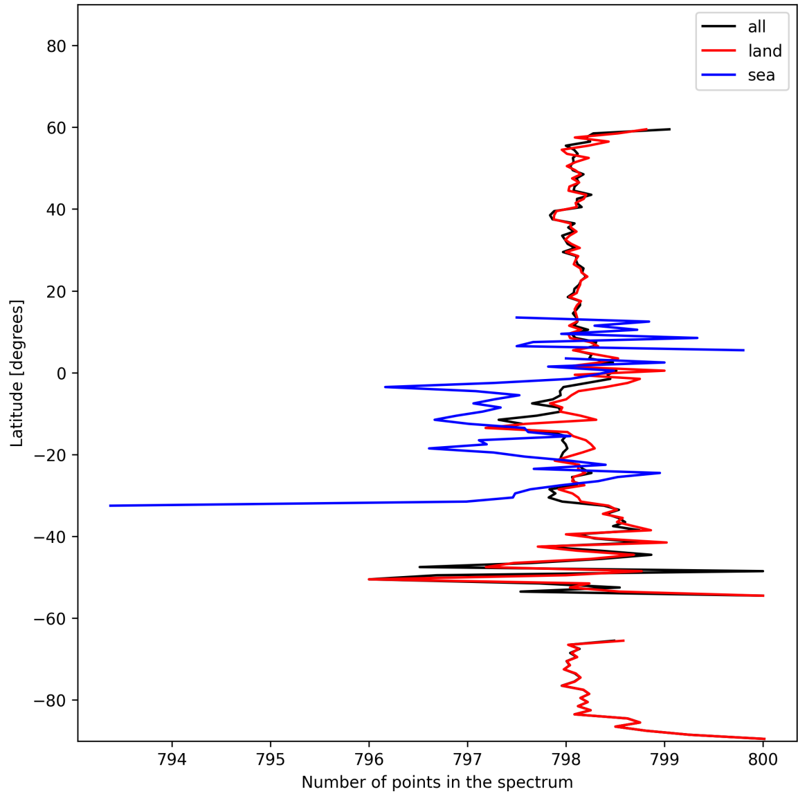
Figure 15: Zonal average of “Number of points in the spectrum” for 2024-11-04 to 2024-11-05.
