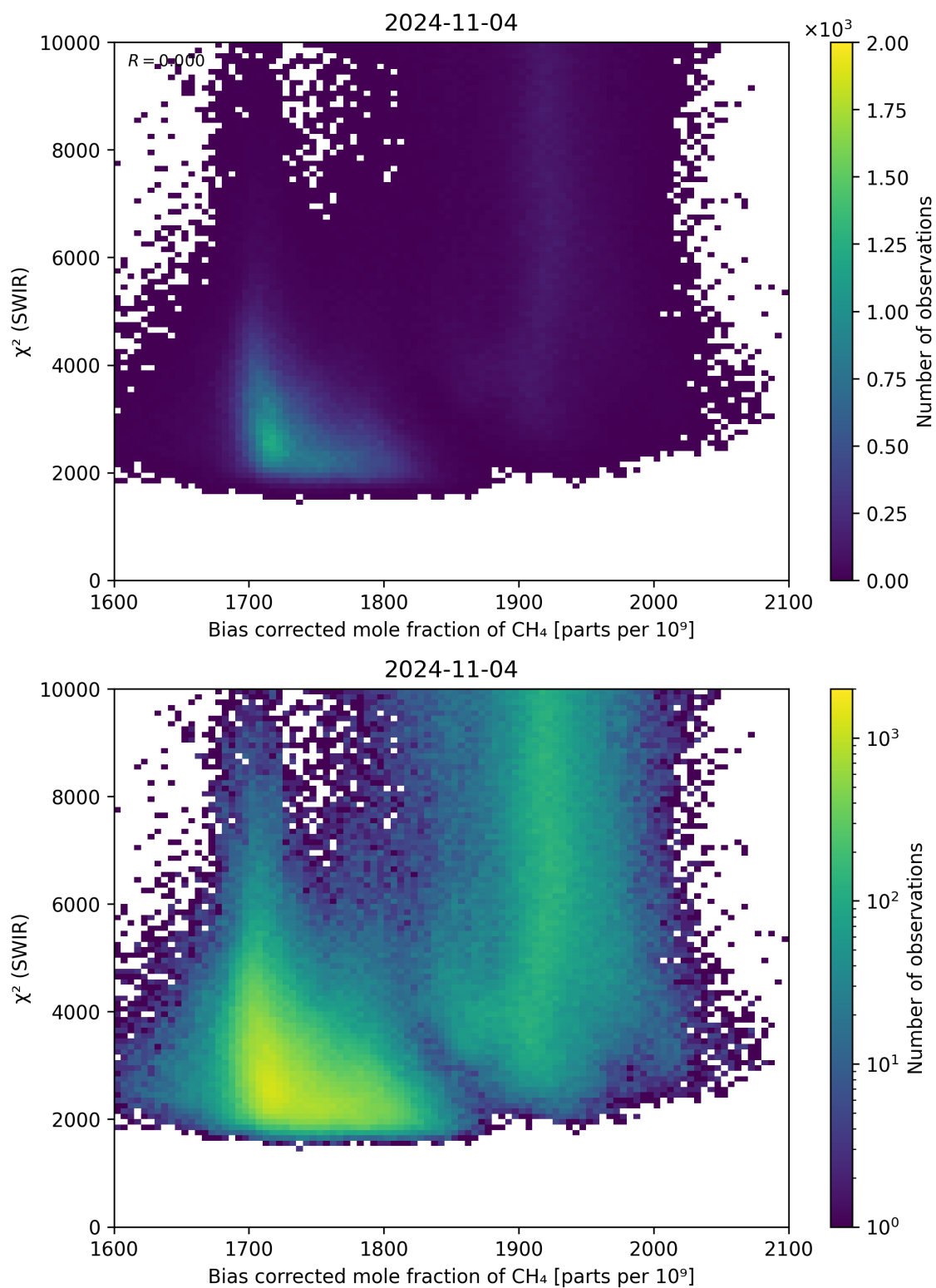
Figure 64: Scatter density plot of “Bias corrected mole fraction of \text{CH}_4 ” against “ \chi^2 (SWIR)” for 2024-11-04 to 2024-11-05.
