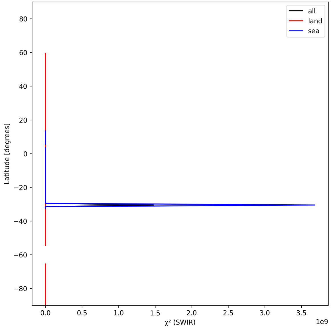
Figure 17: Zonal average of “ \chi^2 (SWIR)” for 2024-11-04 to 2024-11-05.
