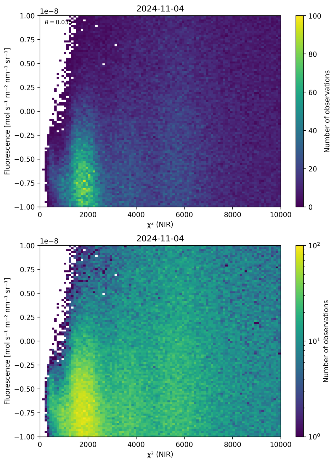
Figure 45: Scatter density plot of “ \chi^2 (NIR)” against “Fluorescence” for 2024-11-04 to 2024-11-05.
