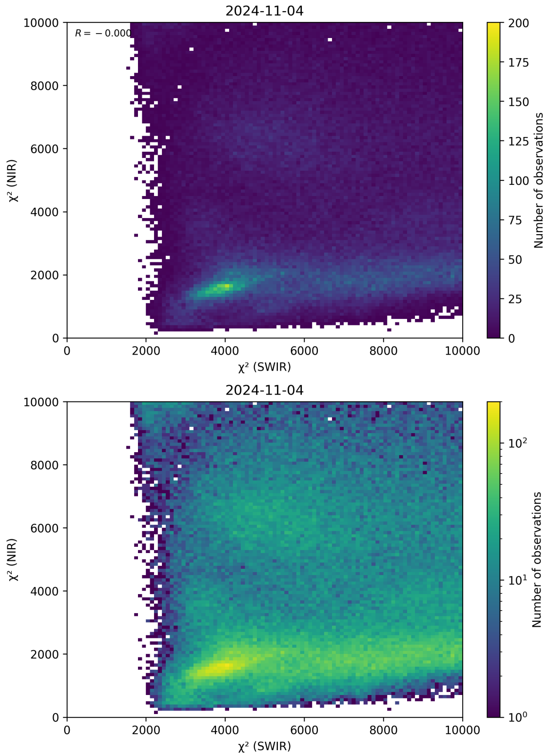
Figure 47: Scatter density plot of “ \chi^2 (SWIR)” against “ \chi^2 (NIR)” for 2024-11-04 to 2024-11-05.
