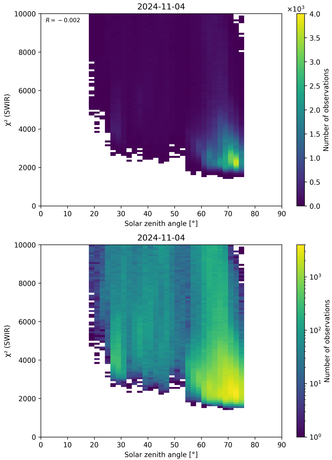
Figure 95: Scatter density plot of “Solar zenith angle” against “ \chi^2 (SWIR)” for 2024-11-04 to 2024-11-05.
