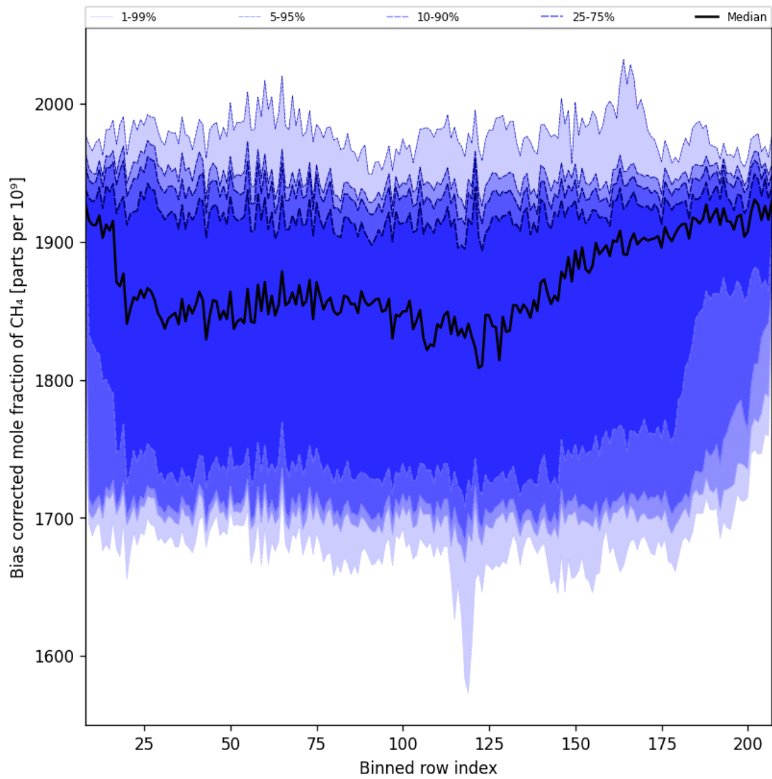
Figure 36: Along track statistics of “Bias corrected mole fraction of CH 4 ” for 2024-11-04 to 2024-11-05
