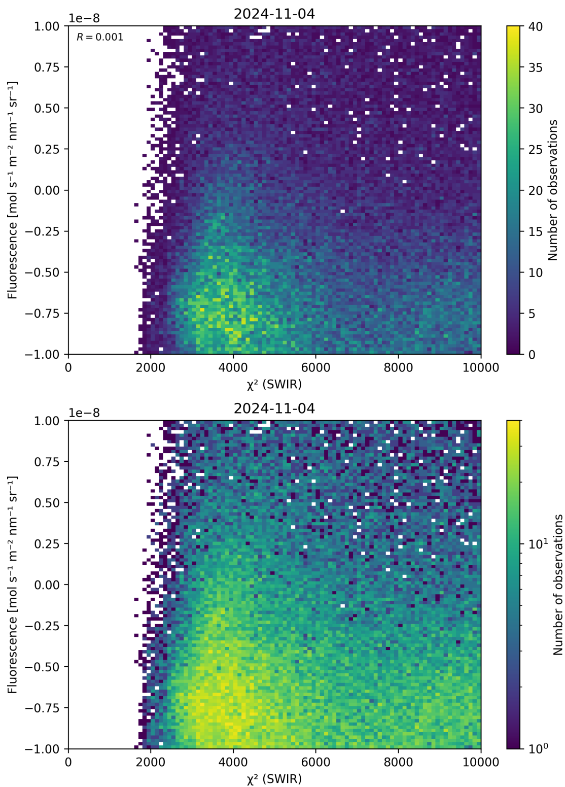
Figure 49: Scatter density plot of “ \chi^2 (SWIR)” against “Fluorescence” for 2024-11-04 to 2024-11-05.
