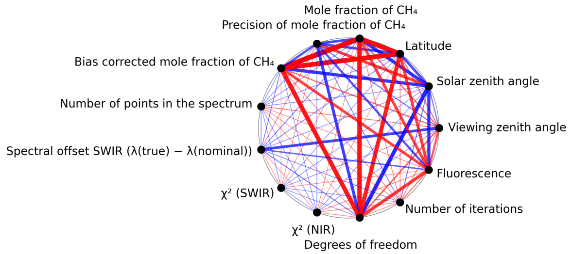
Figure 1: Map of correlation graph for 2024-11-04 to 2024-11-05.
