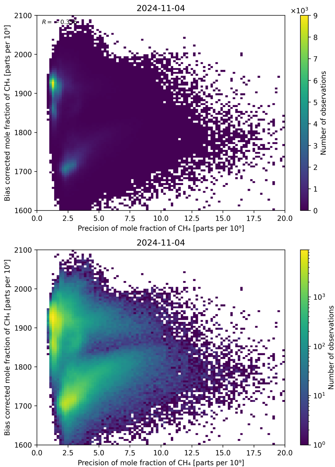
Figure 82: Scatter density plot of “Precision of mole fraction of CH 4 ” against “Bias corrected mole fraction of CH 4 ” for 2024-11-04 to 2024-11-05.
