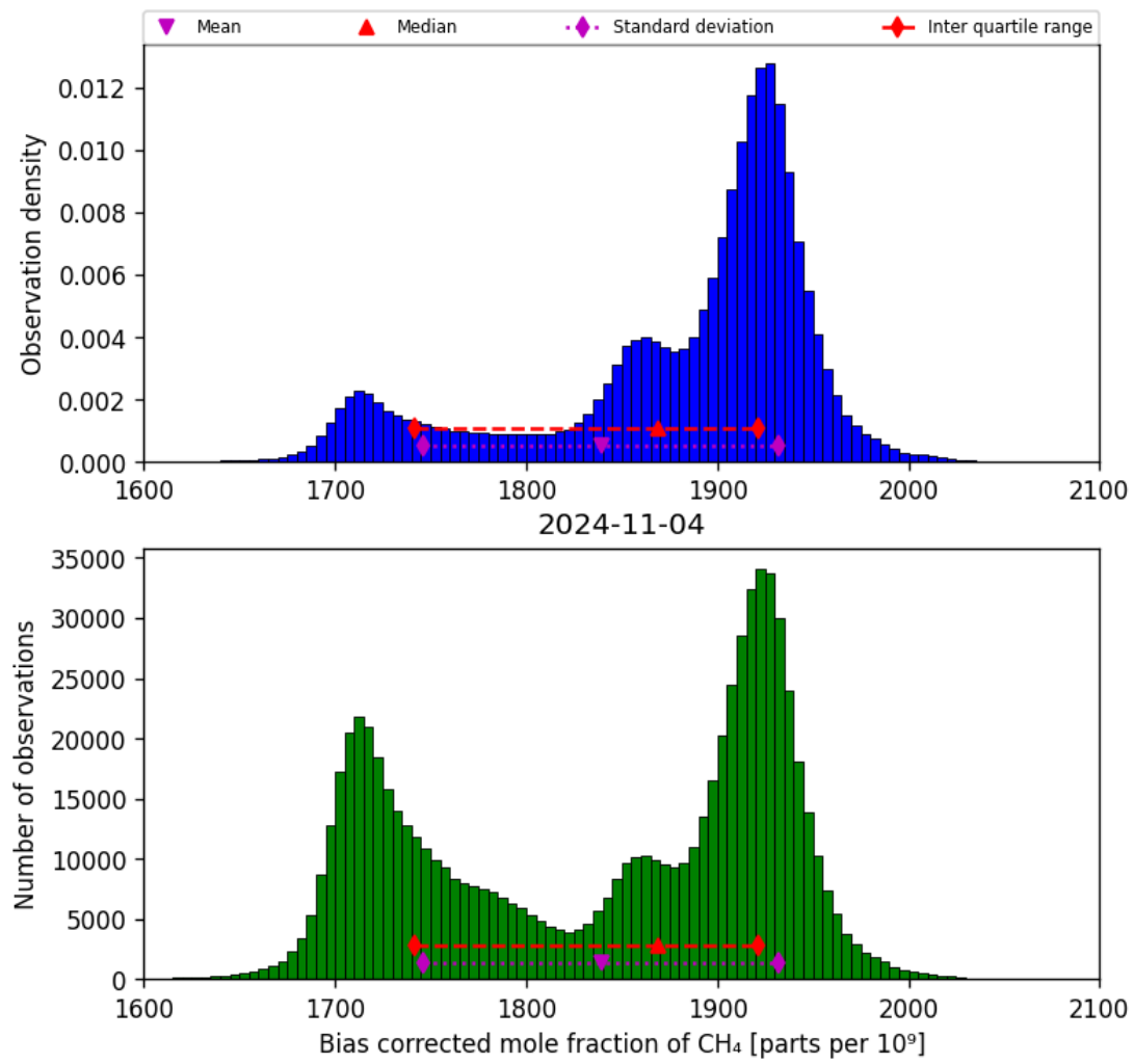
Figure 25: Histogram of “Bias corrected mole fraction of CH 4 ” for 2024-11-04 to 2024-11-05
