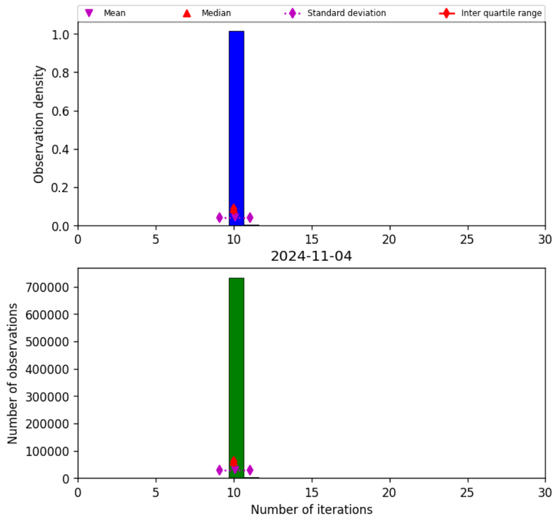
Figure 31: Histogram of “Number of iterations” for 2024-11-04 to 2024-11-05
