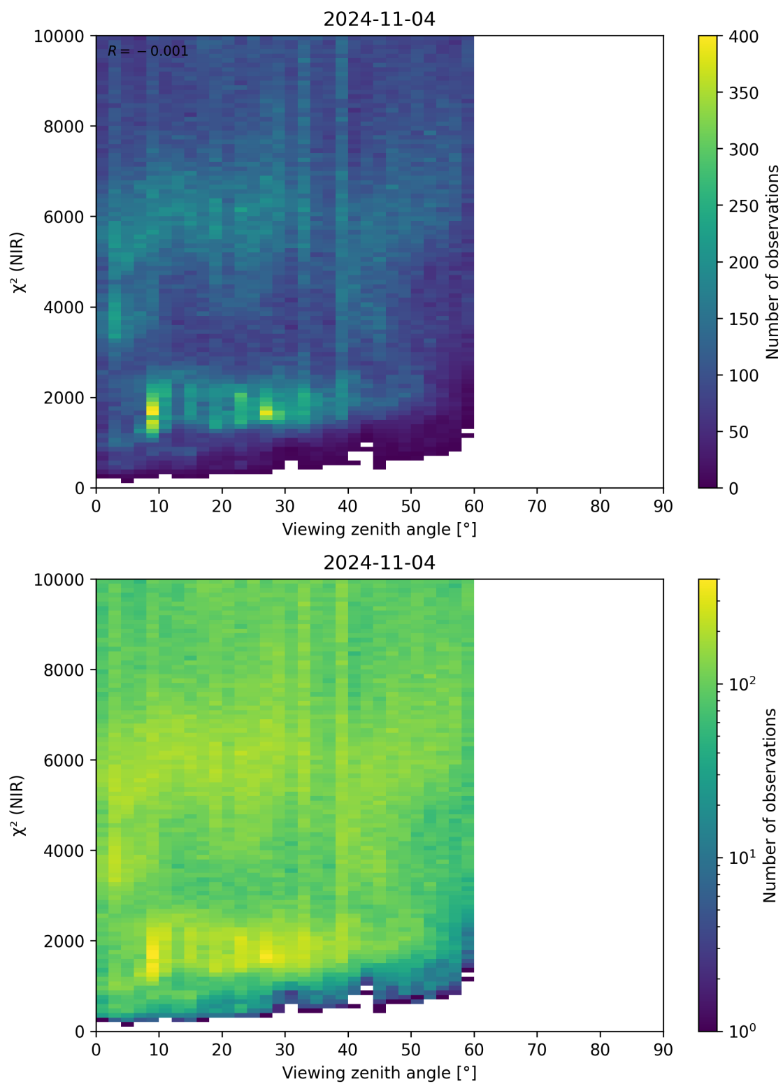
Figure 105: Scatter density plot of “Viewing zenith angle” against “ \chi^2 (NIR)” for 2024-11-04 to 2024-11-05.
