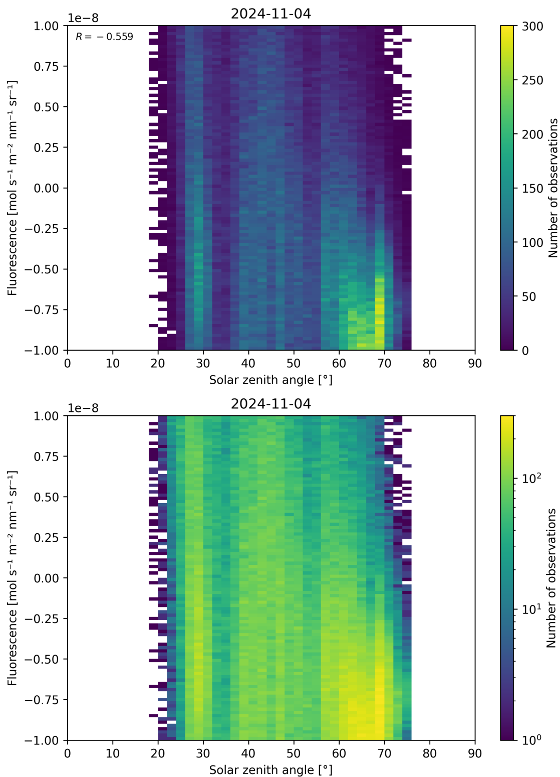
Figure 97: Scatter density plot of “Solar zenith angle” against “Fluorescence” for 2024-11-04 to 2024-11-05.
