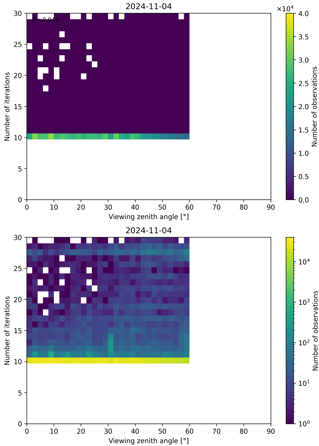
Figure 113: Scatter density plot of “Viewing zenith angle” against “Number of iterations” for 2024-11-04 to 2024-11-05.
