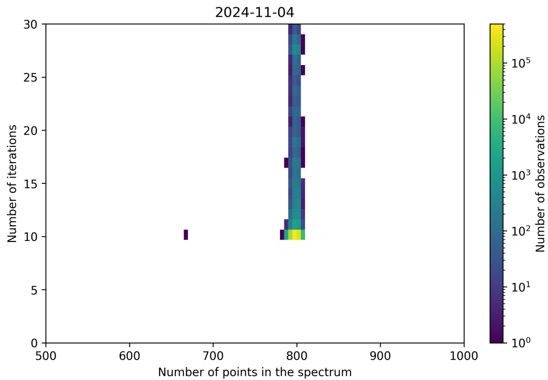
Figure 92: Scatter density plot of “Number of points in the spectrum” against “Number of iterations” for 2024-11-04 to 2024-11-05.
