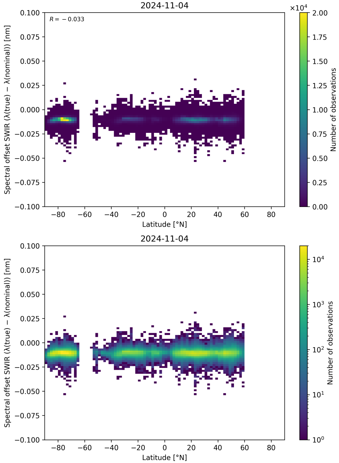
Figure 62: Scatter density plot of “Latitude” against “Spectral offset SWIR ( \lambda_{\text{true}} - \lambda_{\text{nominal}} )” for 2024-11-04 to 2024-11-05.
