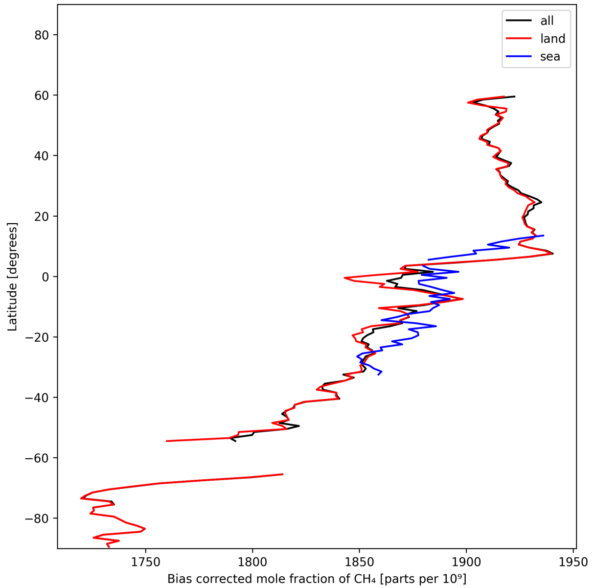
Figure 14: Zonal average of “Bias corrected mole fraction of CH 4 ” for 2024-11-04 to 2024-11-05.
