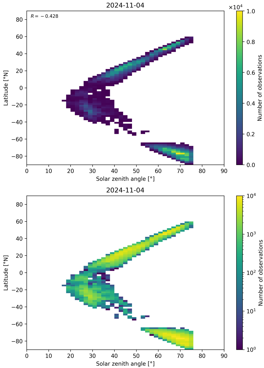
Figure 98: Scatter density plot of “Solar zenith angle” against “Latitude” for 2024-11-04 to 2024-11-05.
