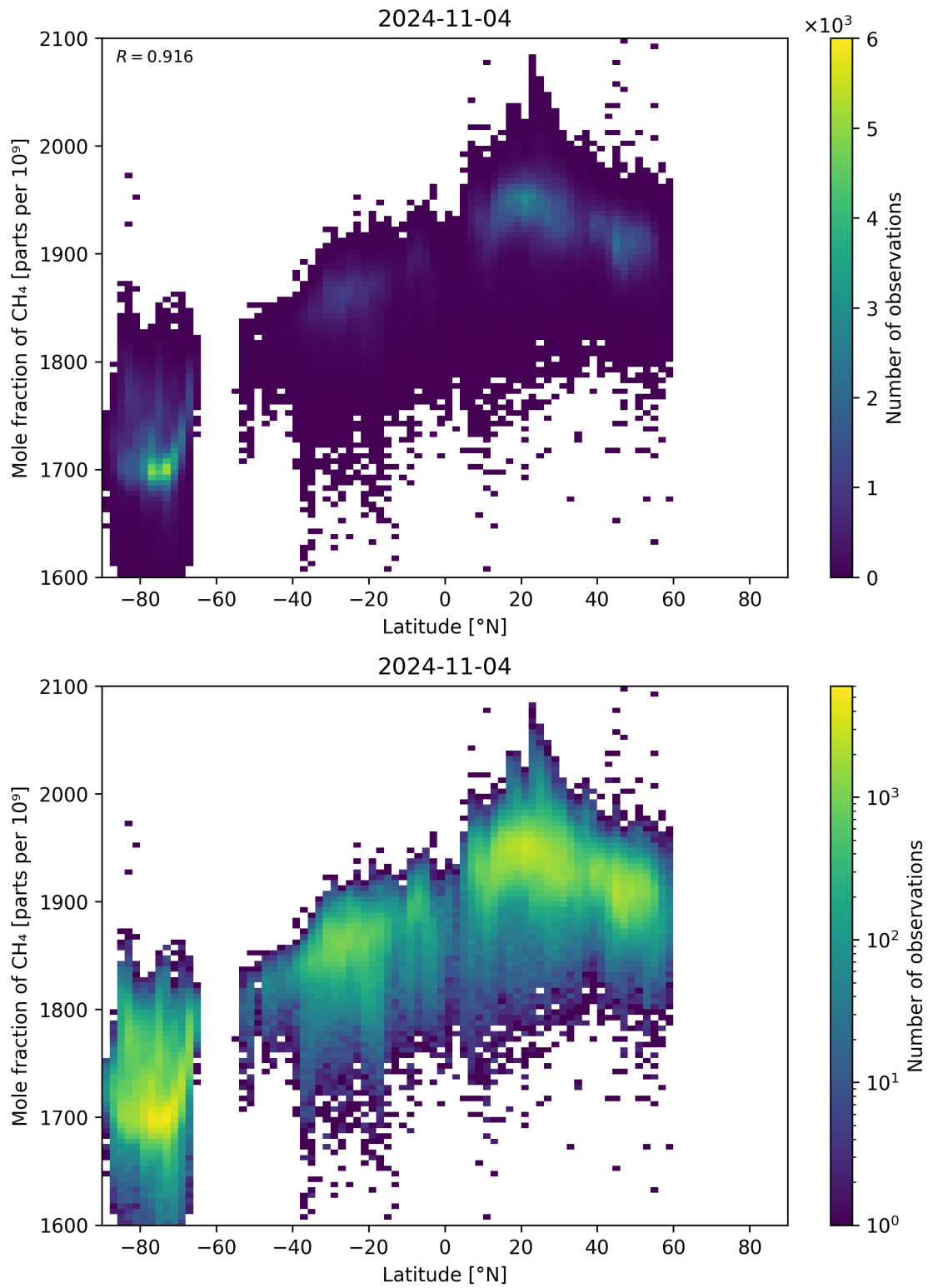
Figure 57: Scatter density plot of “Latitude” against “Mole fraction of CH 4 ” for 2024-11-04 to 2024-11-05.
