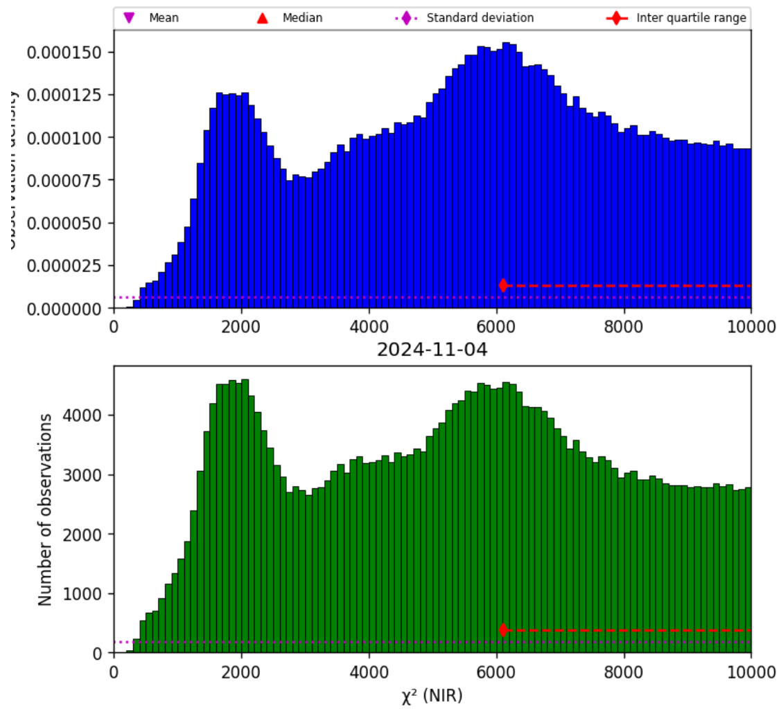
Figure 29: Histogram of “ \chi^2 (NIR)” for 2024-11-04 to 2024-11-05
