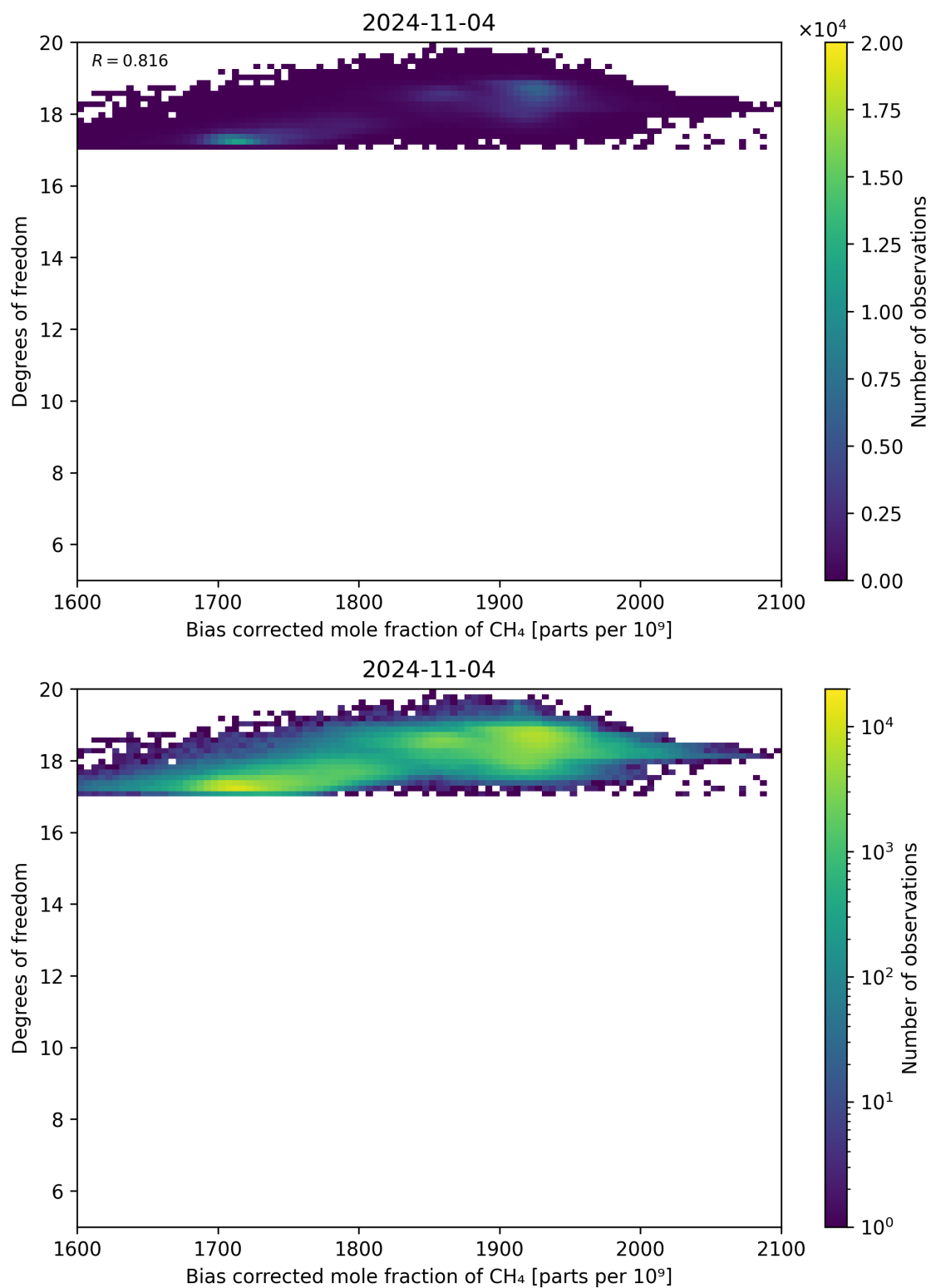
Figure 65: Scatter density plot of “Bias corrected mole fraction of CH 4 ” against “Degrees of freedom” for 2024-11-04 to 2024-11-05.
