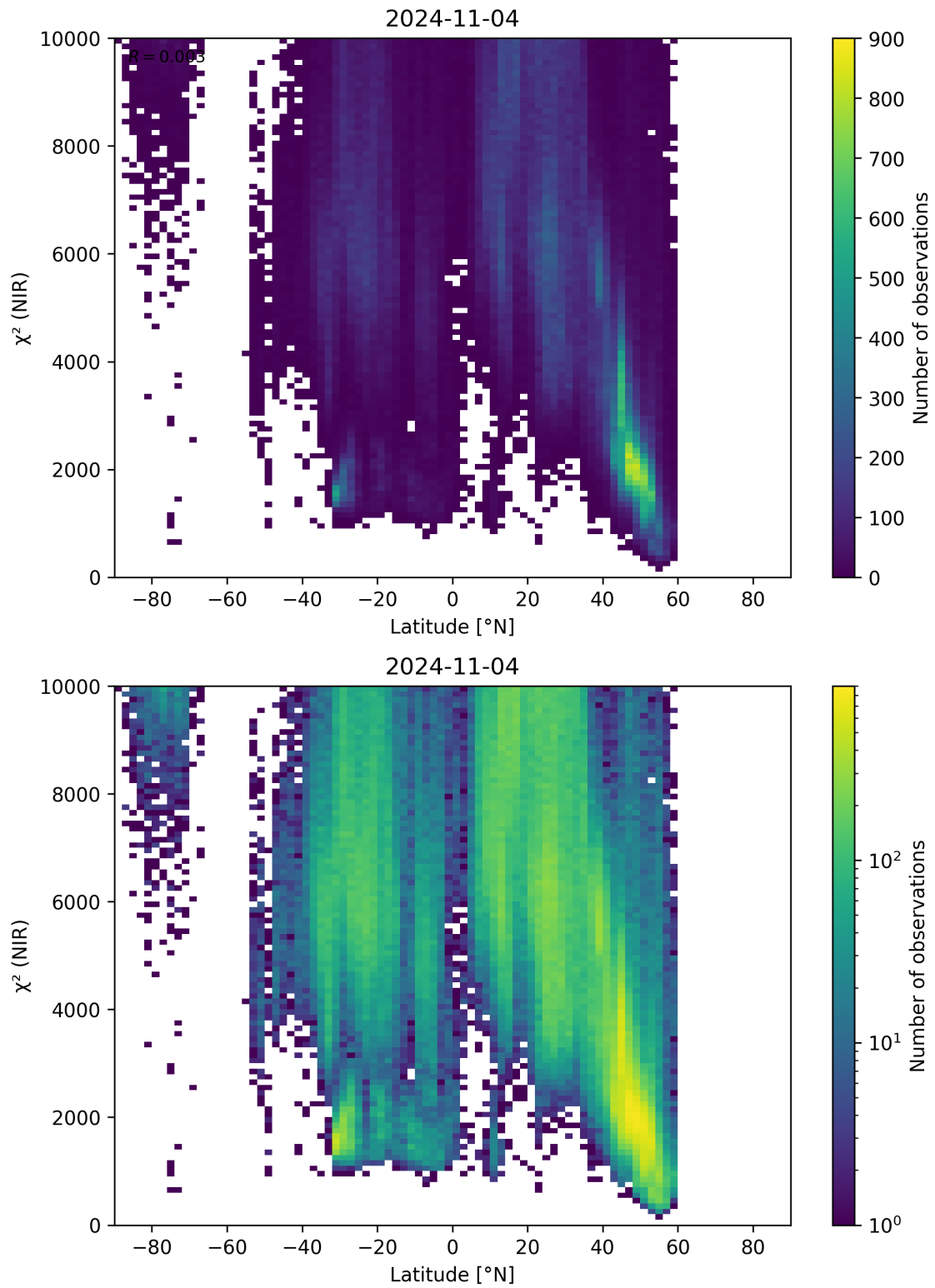
Figure 53: Scatter density plot of “Latitude” against “ \chi^2 (NIR)” for 2024-11-04 to 2024-11-05.
