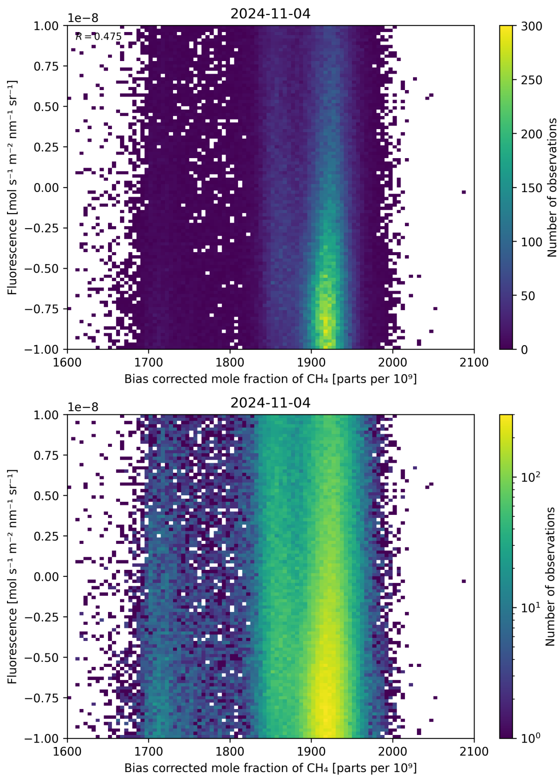
Figure 66: Scatter density plot of “Bias corrected mole fraction of \text{CH}_4 ” against “Fluorescence” for 2024-11-04 to 2024-11-05.
