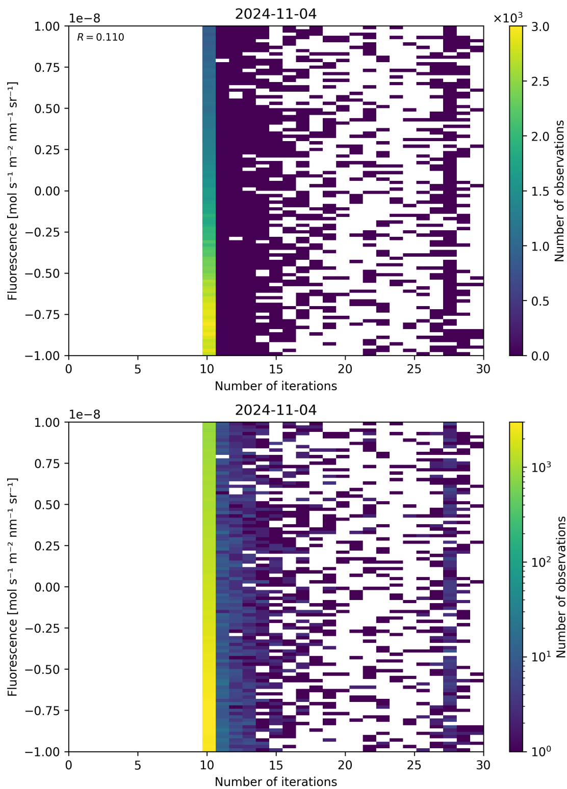
Figure 87: Scatter density plot of “Number of iterations” against “Fluorescence” for 2024-11-04 to 2024-11-05.
