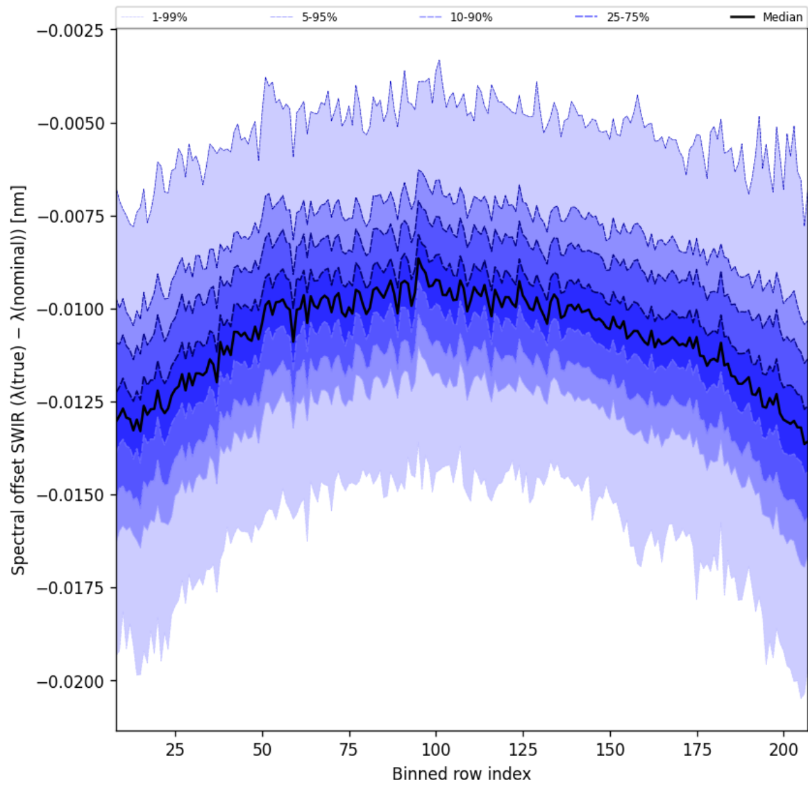
Figure 38: Along track statistics of “Spectral offset SWIR ( \lambda_{\text{true}} - \lambda_{\text{nominal}} )” for 2024-11-04 to 2024-11-05
