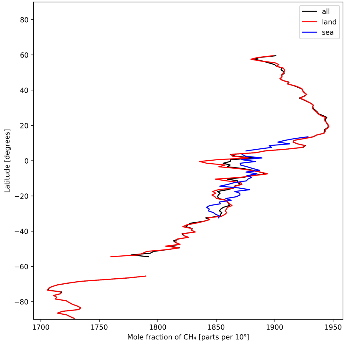
Figure 12: Zonal average of “Mole fraction of CH 4 ” for 2024-11-04 to 2024-11-05.
