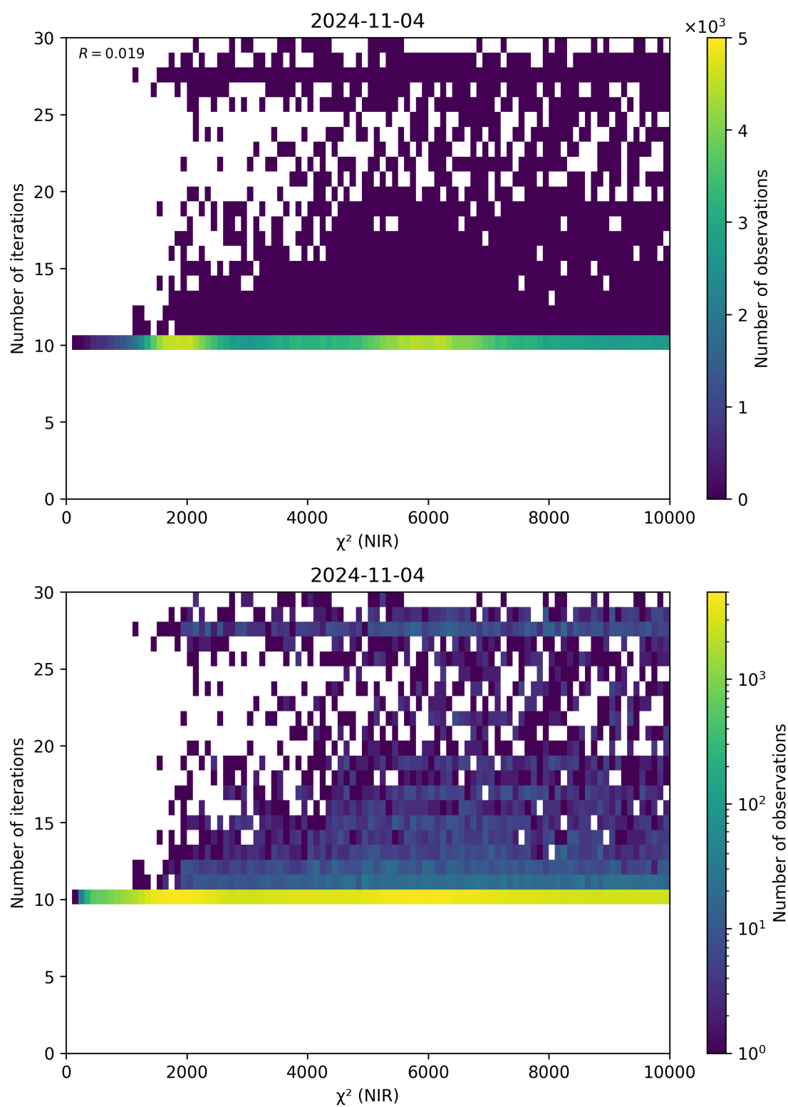
Figure 46: Scatter density plot of “ \chi^2 (NIR)” against “Number of iterations” for 2024-11-04 to 2024-11-05.
