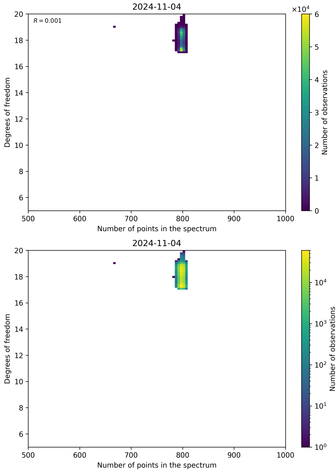
Figure 90: Scatter density plot of “Number of points in the spectrum” against “Degrees of freedom” for 2024-11-04 to 2024-11-05.
