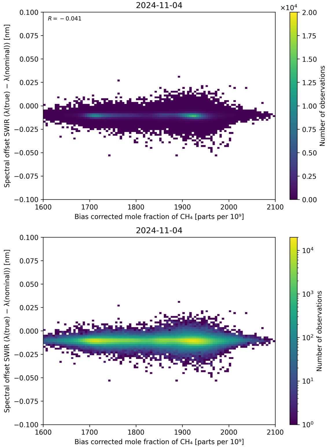
Figure 69: Scatter density plot of “Bias corrected mole fraction of CH 4 ” against “Spectral offset SWIR ( \lambda_{\text{true}} - \lambda_{\text{nominal}} )” for 2024-11-04 to 2024-11-05.
