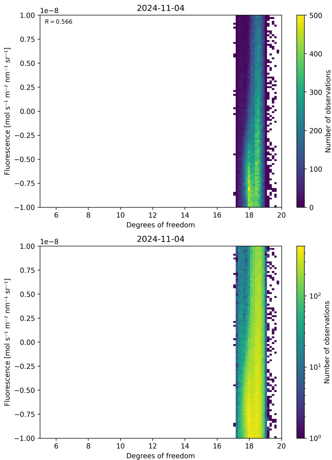
Figure 51: Scatter density plot of “Degrees of freedom” against “Fluorescence” for 2024-11-04 to 2024-11-05.
