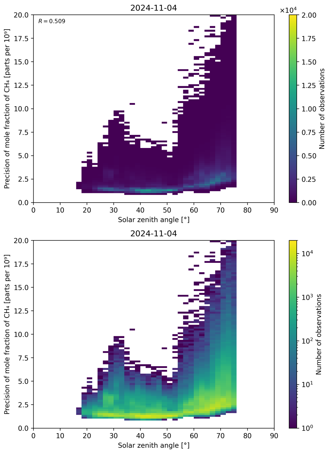
Figure 101: Scatter density plot of “Solar zenith angle” against “Precision of mole fraction of \text{CH}_4 ” for 2024-11-04 to 2024-11-05.
