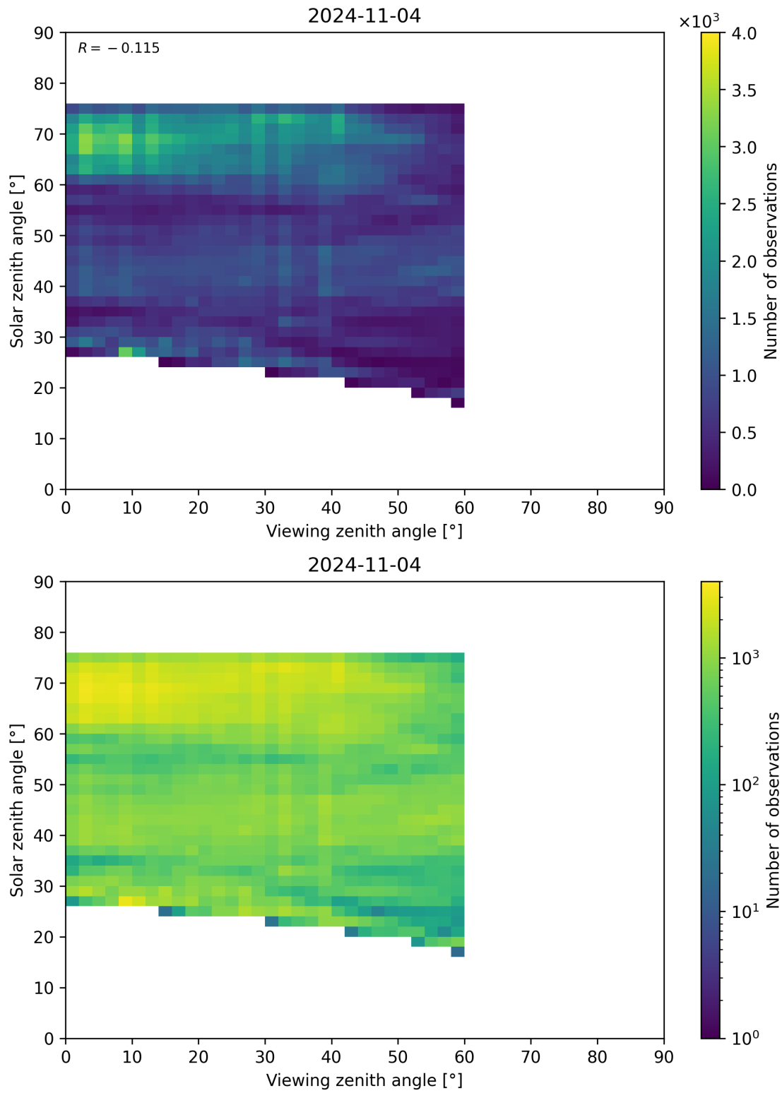
Figure 115: Scatter density plot of “Viewing zenith angle” against “Solar zenith angle” for 2024-11-04 to 2024-11-05.
