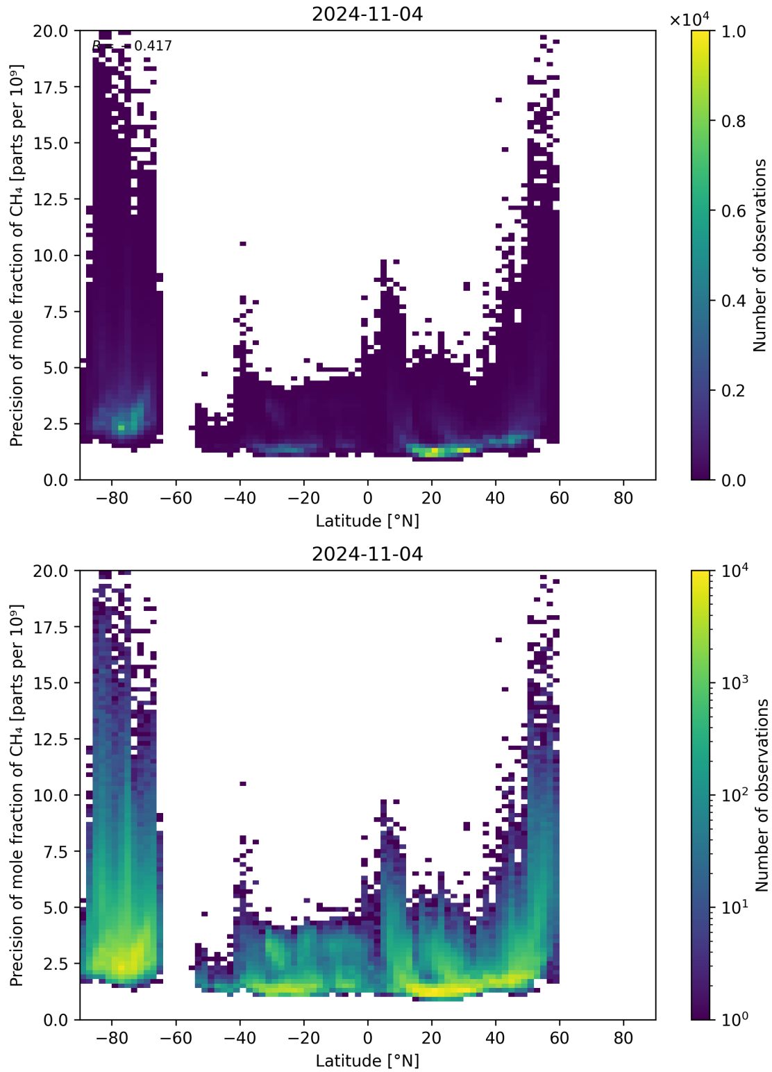
Figure 59: Scatter density plot of “Latitude” against “Precision of mole fraction of CH 4 ” for 2024-11-04 to 2024-11-05.
