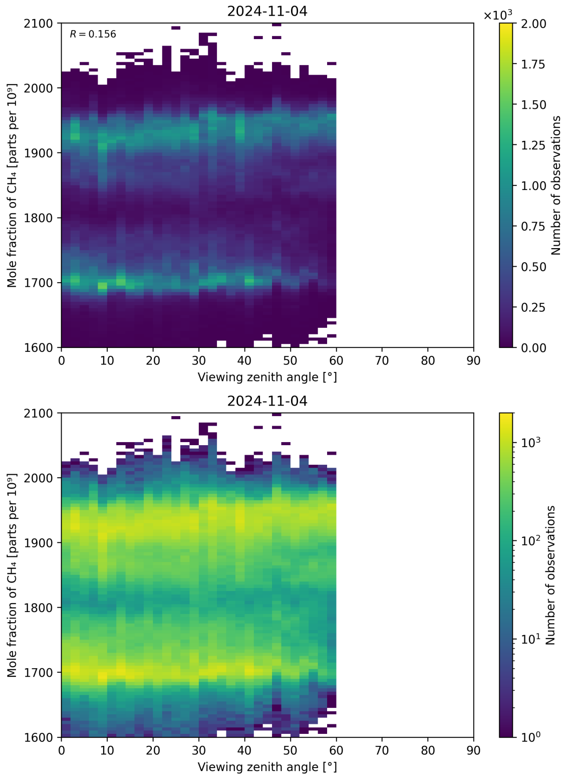
Figure 110: Scatter density plot of “Viewing zenith angle” against “Mole fraction of CH 4 ” for 2024-11-04 to 2024-11-05.
