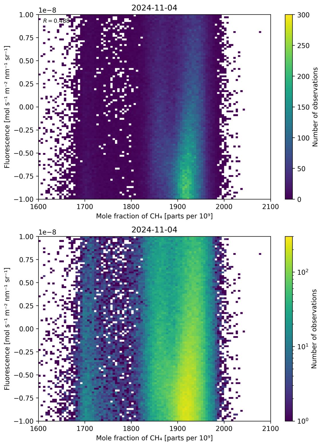
Figure 73: Scatter density plot of “Mole fraction of \text{CH}_4 ” against “Fluorescence” for 2024-11-04 to 2024-11-05.
