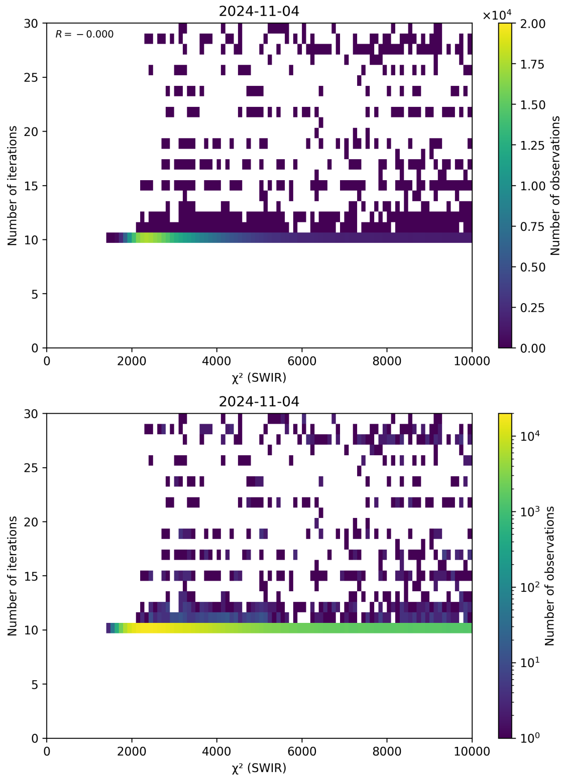
Figure 50: Scatter density plot of “ \chi^2 (SWIR)” against “Number of iterations” for 2024-11-04 to 2024-11-05.
