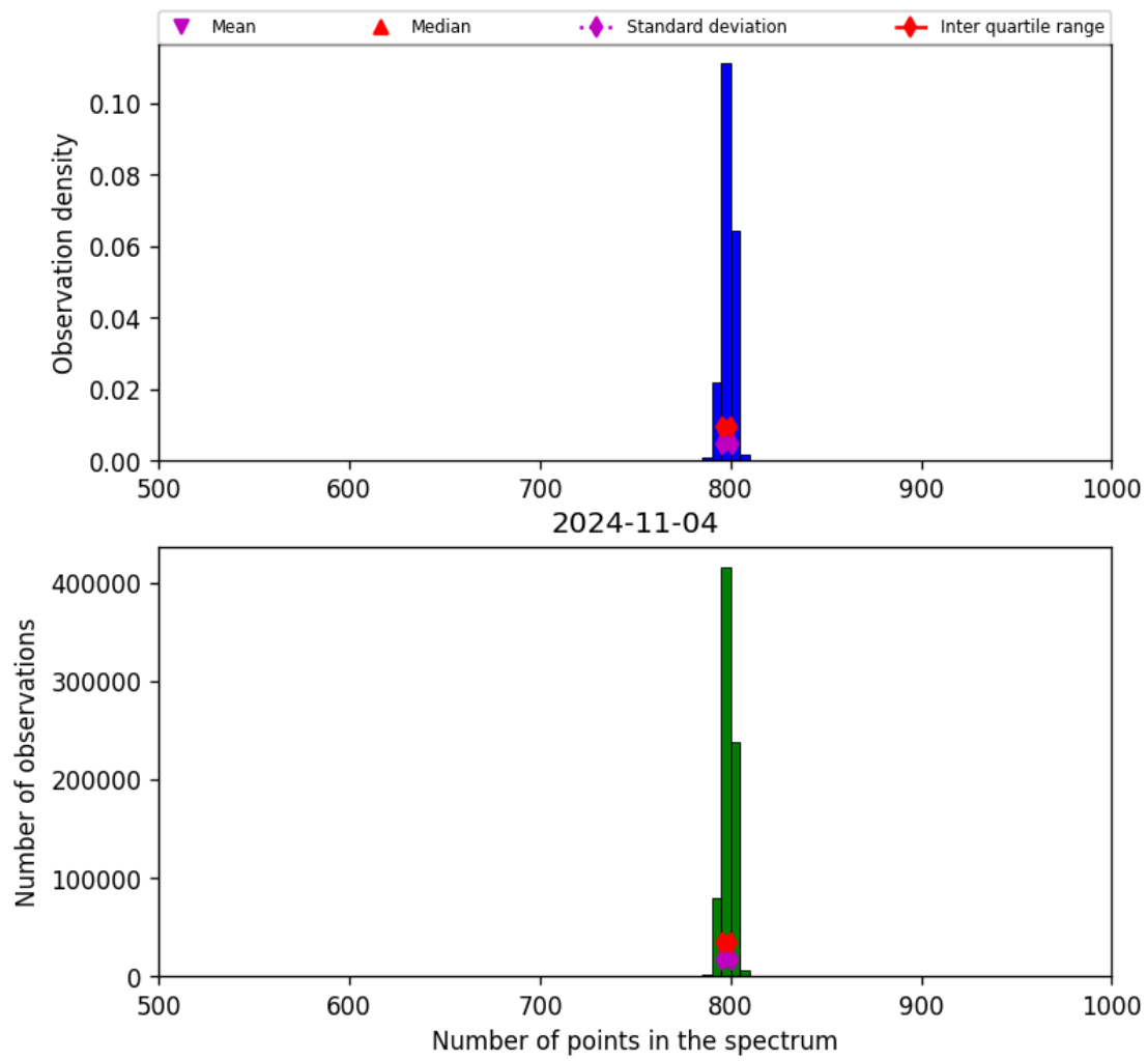
Figure 26: Histogram of “Number of points in the spectrum” for 2024-11-04 to 2024-11-05
