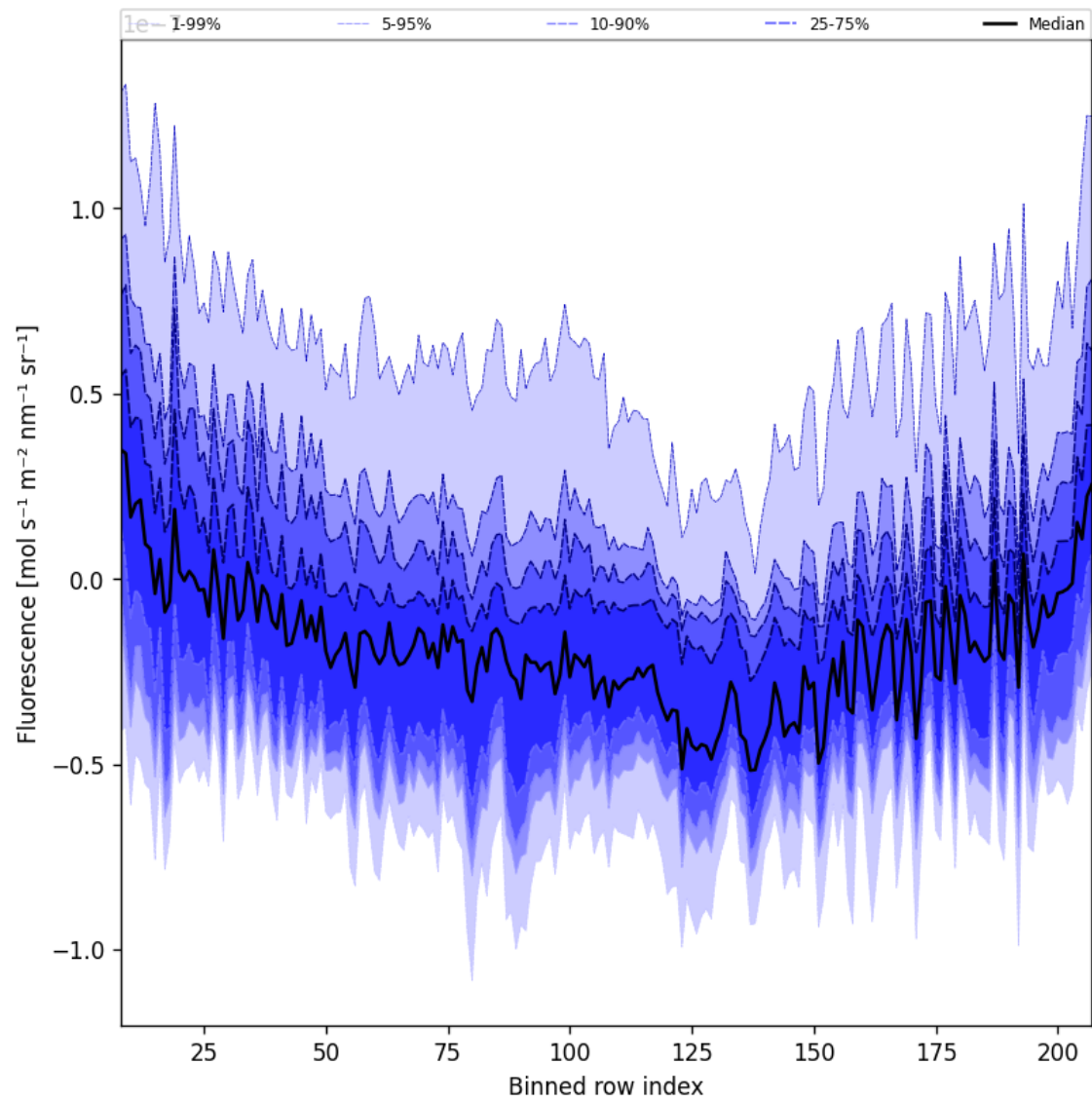
Figure 43: Along track statistics of “Fluorescence” for 2024-11-04 to 2024-11-05
