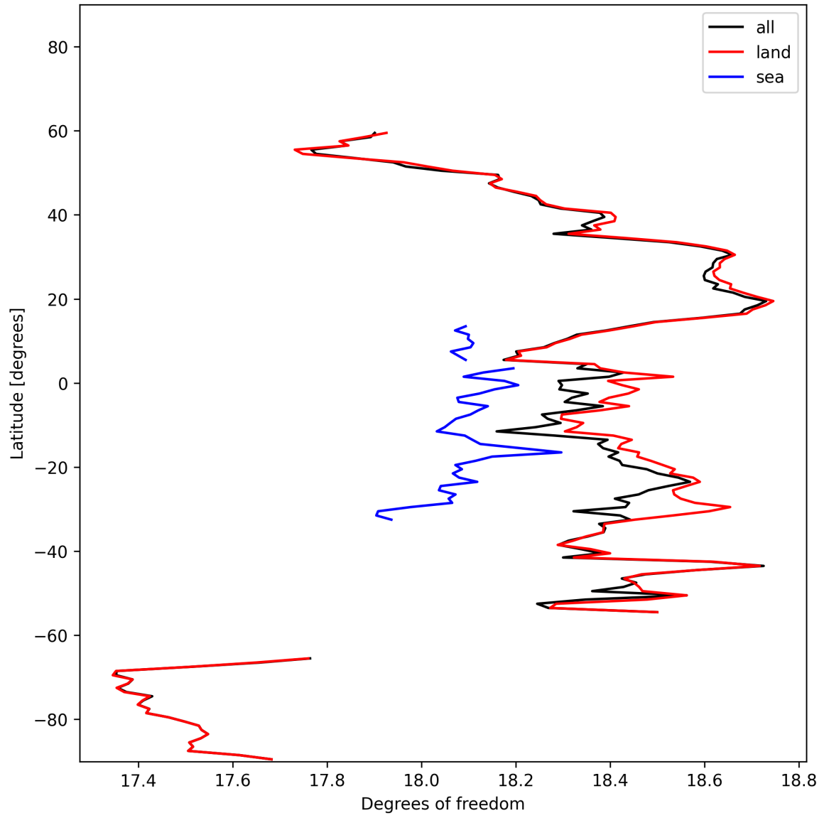
Figure 19: Zonal average of “Degrees of freedom” for 2024-11-04 to 2024-11-05.
