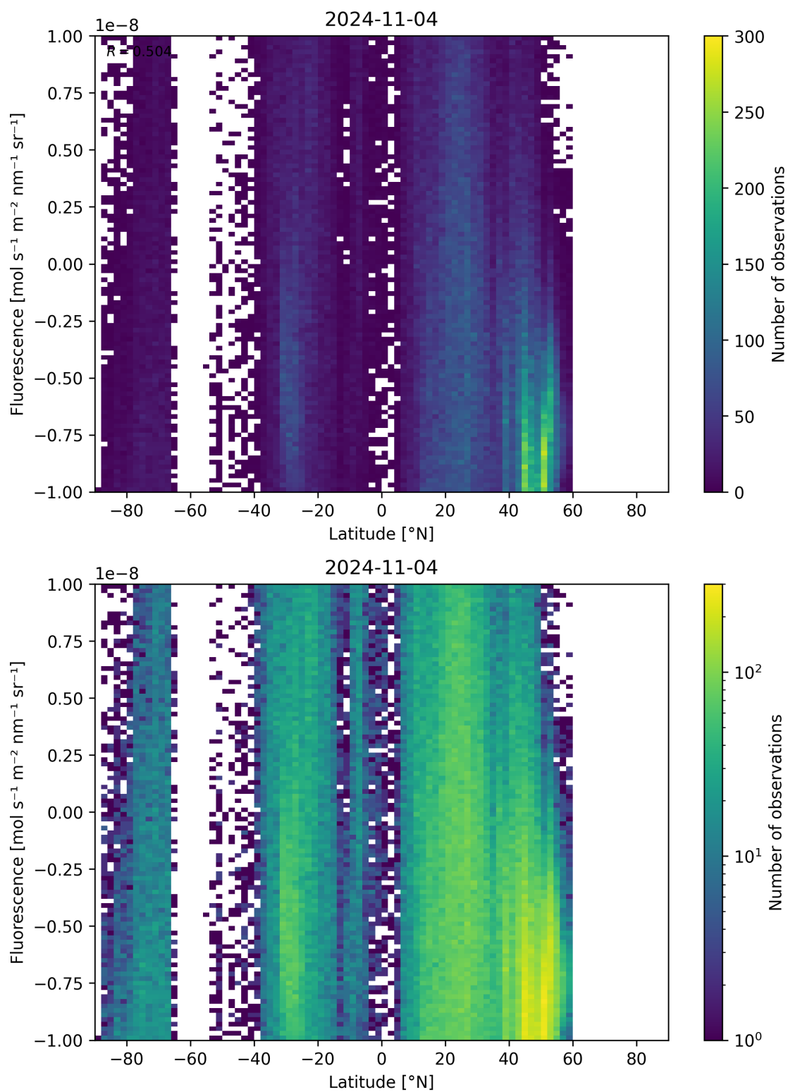
Figure 56: Scatter density plot of “Latitude” against “Fluorescence” for 2024-11-04 to 2024-11-05.
