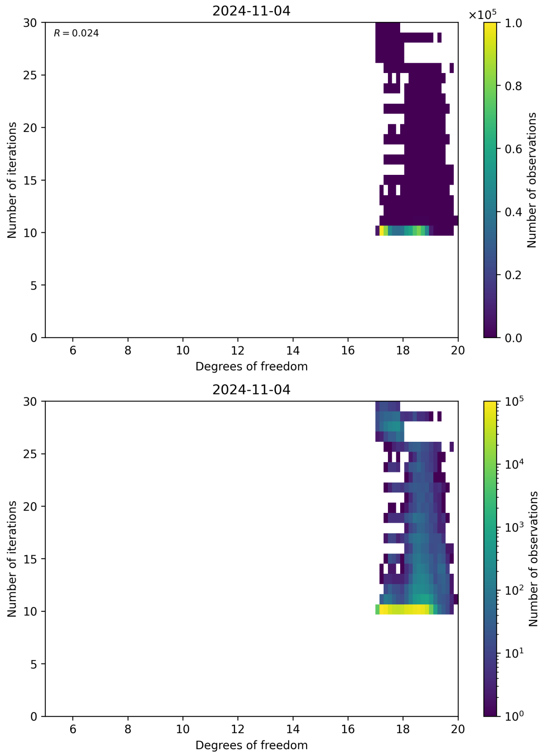
Figure 52: Scatter density plot of “Degrees of freedom” against “Number of iterations” for 2024-11-04 to 2024-11-05.
