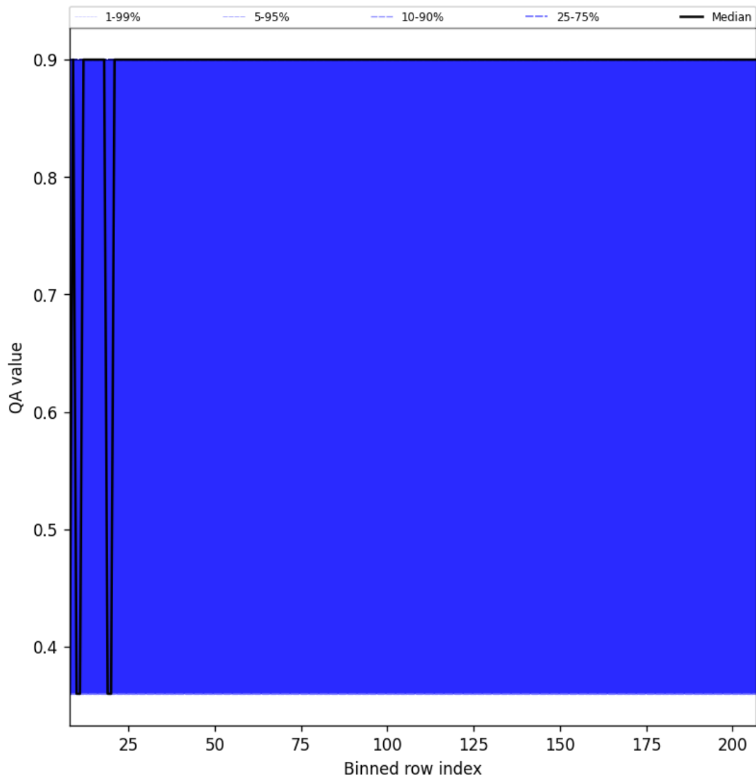
Figure 33: Along track statistics of “QA value” for 2024-11-04 to 2024-11-05
