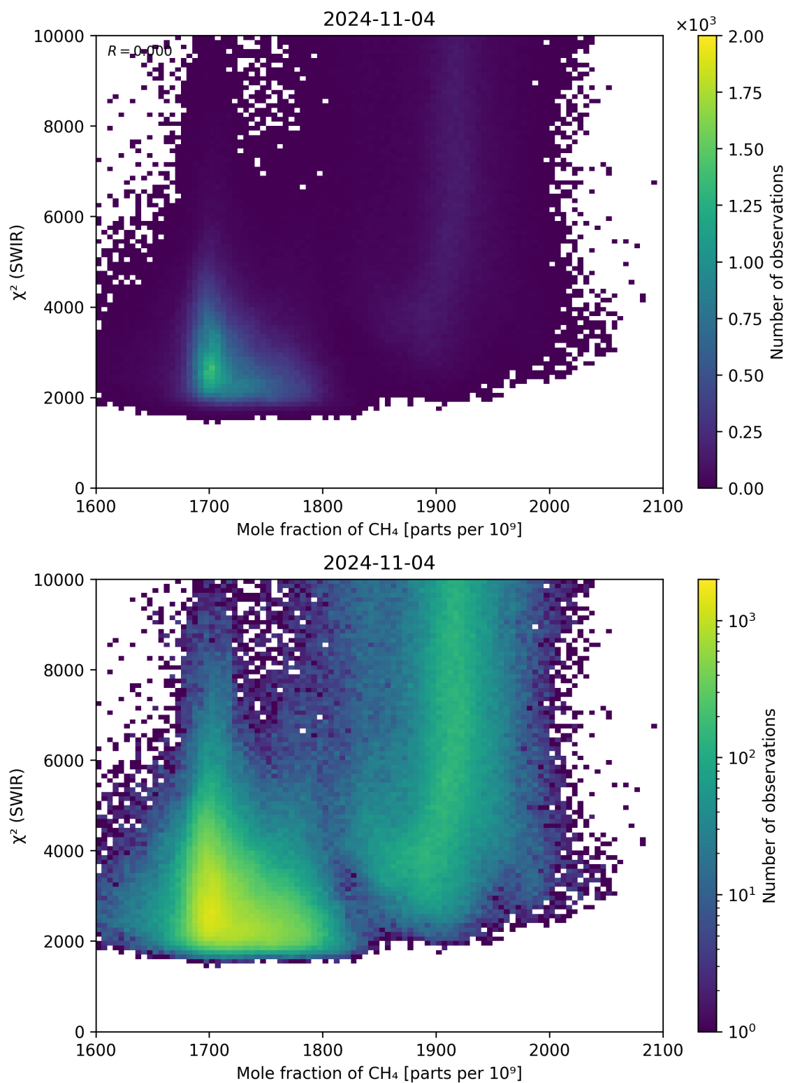
Figure 71: Scatter density plot of “Mole fraction of \text{CH}_4 ” against “ \chi^2 (SWIR)” for 2024-11-04 to 2024-11-05.
