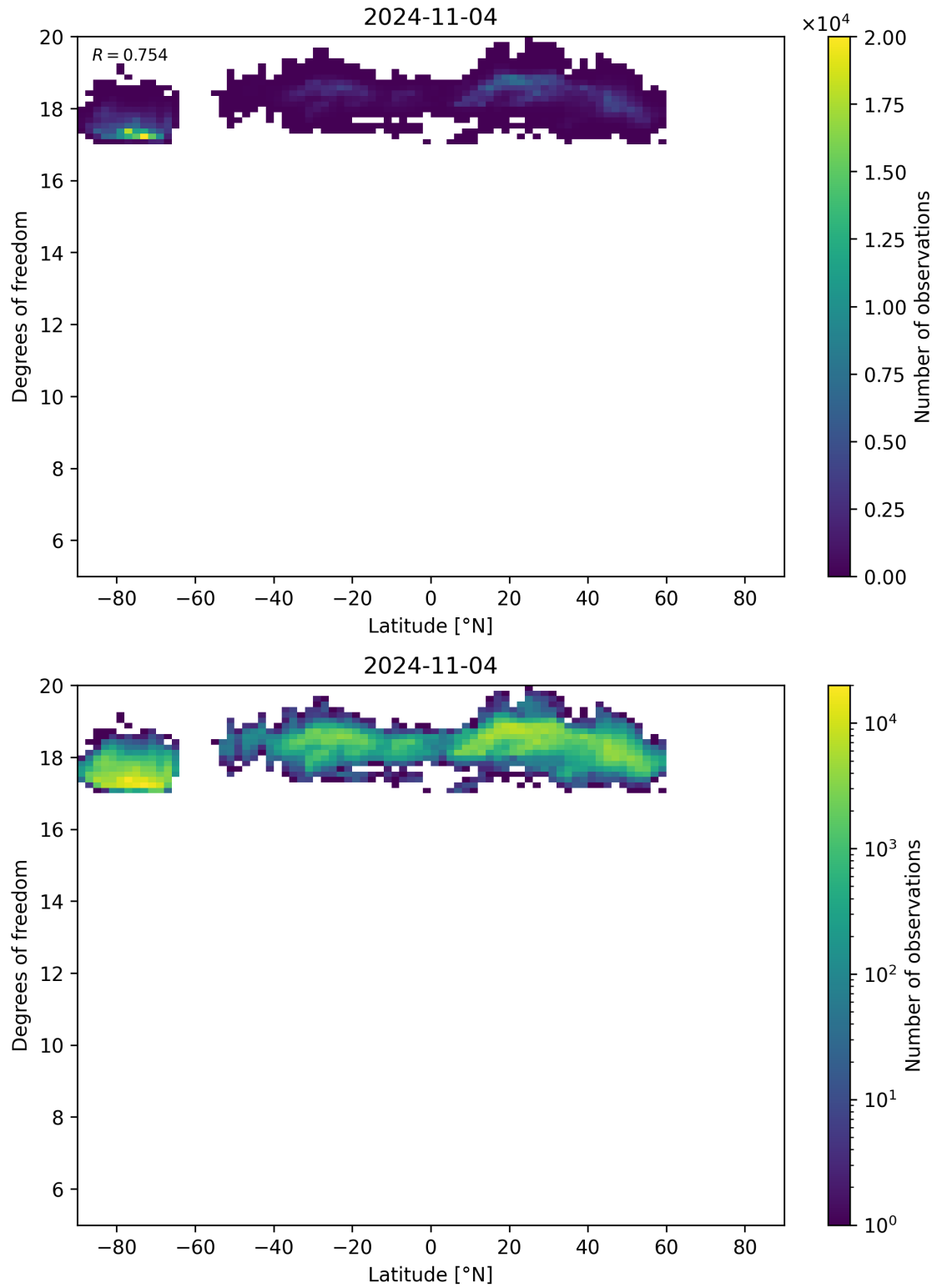
Figure 55: Scatter density plot of “Latitude” against “Degrees of freedom” for 2024-11-04 to 2024-11-05.
