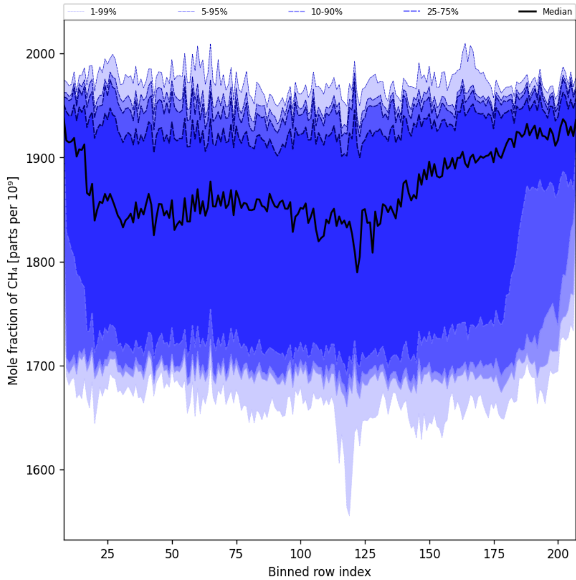
Figure 34: Along track statistics of “Mole fraction of CH 4 ” for 2024-11-04 to 2024-11-05
