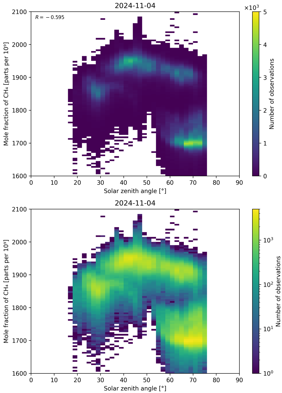
Figure 99: Scatter density plot of “Solar zenith angle” against “Mole fraction of \text{CH}_4 ” for 2024-11-04 to 2024-11-05.
