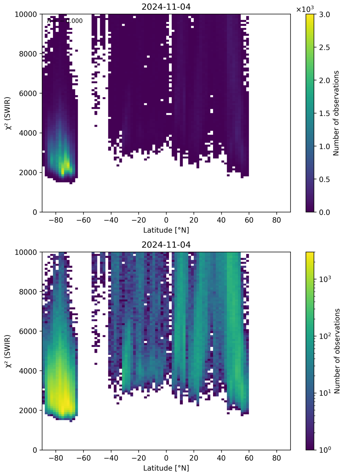
Figure 54: Scatter density plot of “Latitude” against “ \chi^2 (SWIR)” for 2024-11-04 to 2024-11-05.
