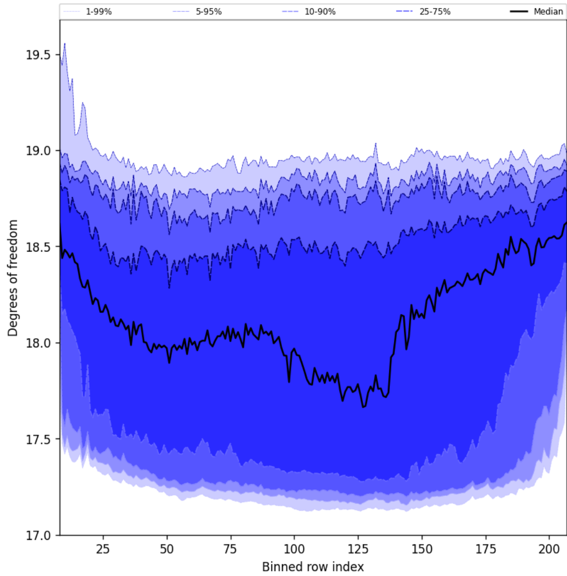
Figure 41: Along track statistics of “Degrees of freedom” for 2024-11-04 to 2024-11-05
