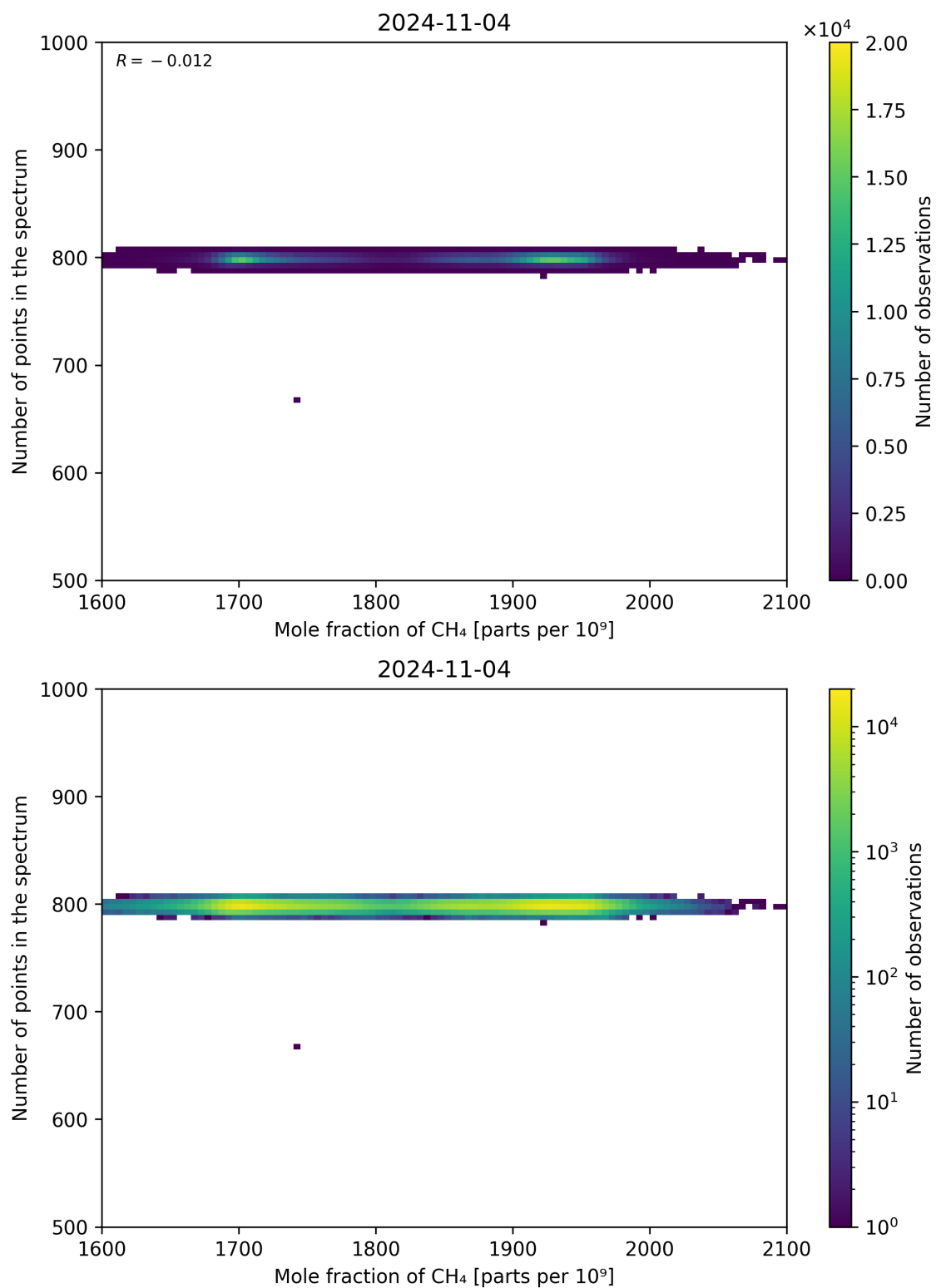
Figure 77: Scatter density plot of “Mole fraction of CH 4 ” against “Number of points in the spectrum” for 2024-11-04 to 2024-11-05.
