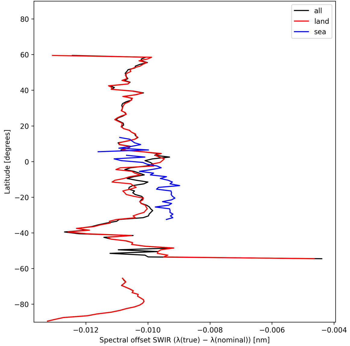
Figure 16: Zonal average of “Spectral offset SWIR ( \lambda_{\text{true}} - \lambda_{\text{nominal}} )” for 2024-11-04 to 2024-11-05.
