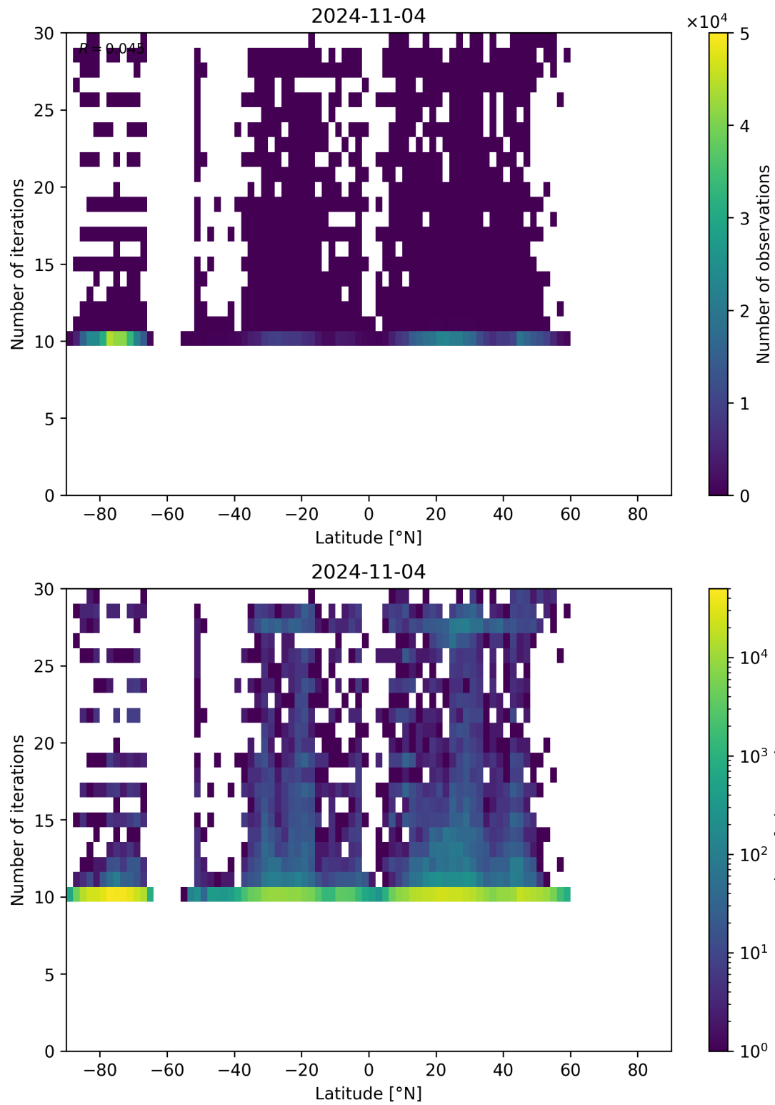
Figure 60: Scatter density plot of “Latitude” against “Number of iterations” for 2024-11-04 to 2024-11-05.
