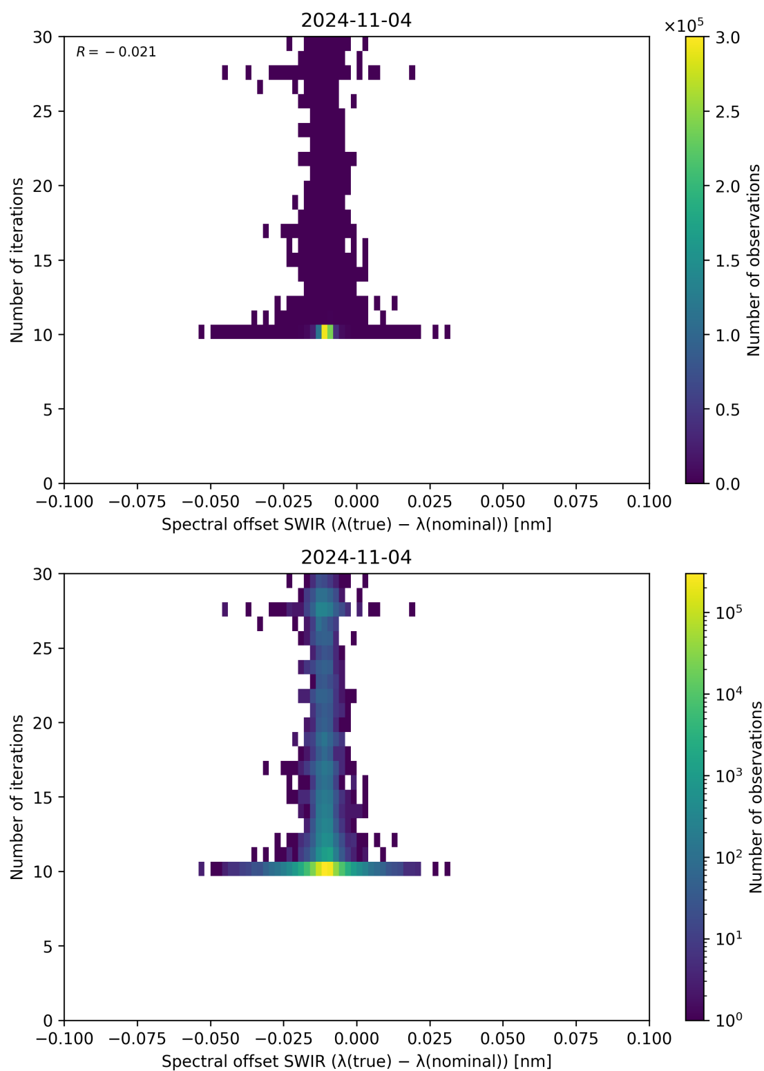
Figure 121: Scatter density plot of “Spectral offset SWIR ( \lambda_{\text{true}} - \lambda_{\text{nominal}} )” against “Number of iterations” for 2024-11-04 to 2024-11-05.
