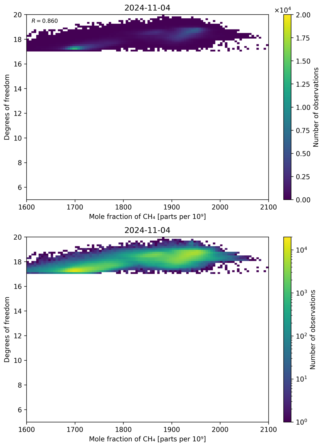
Figure 72: Scatter density plot of “Mole fraction of CH 4 ” against “Degrees of freedom” for 2024-11-04 to 2024-11-05.
