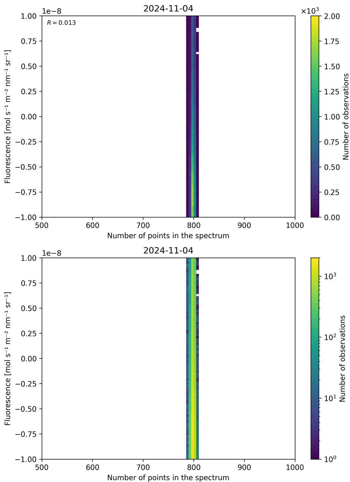
Figure 91: Scatter density plot of “Number of points in the spectrum” against “Fluorescence” for 2024-11-04 to 2024-11-05.
