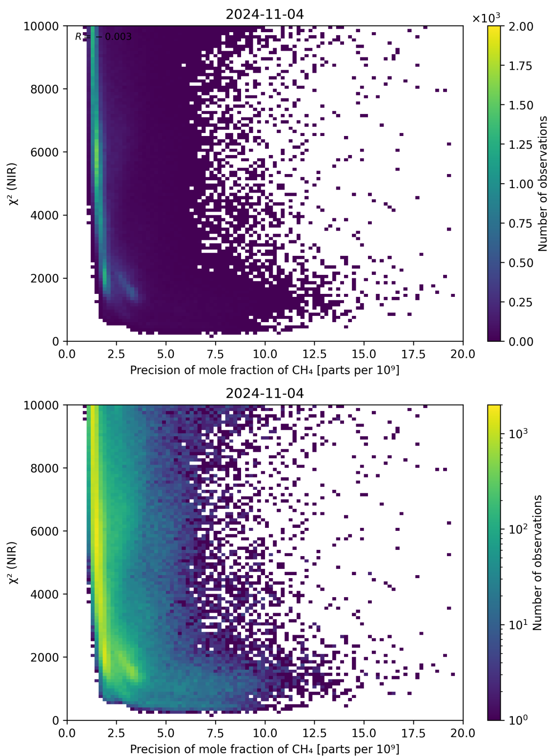
Figure 78: Scatter density plot of “Precision of mole fraction of \text{CH}_4 ” against “ \chi^2 (NIR)” for 2024-11-04 to 2024-11-05.
