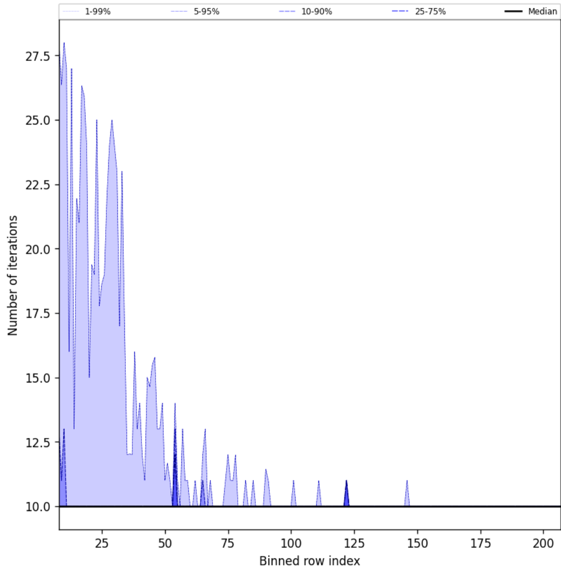
Figure 42: Along track statistics of “Number of iterations” for 2024-11-04 to 2024-11-05
