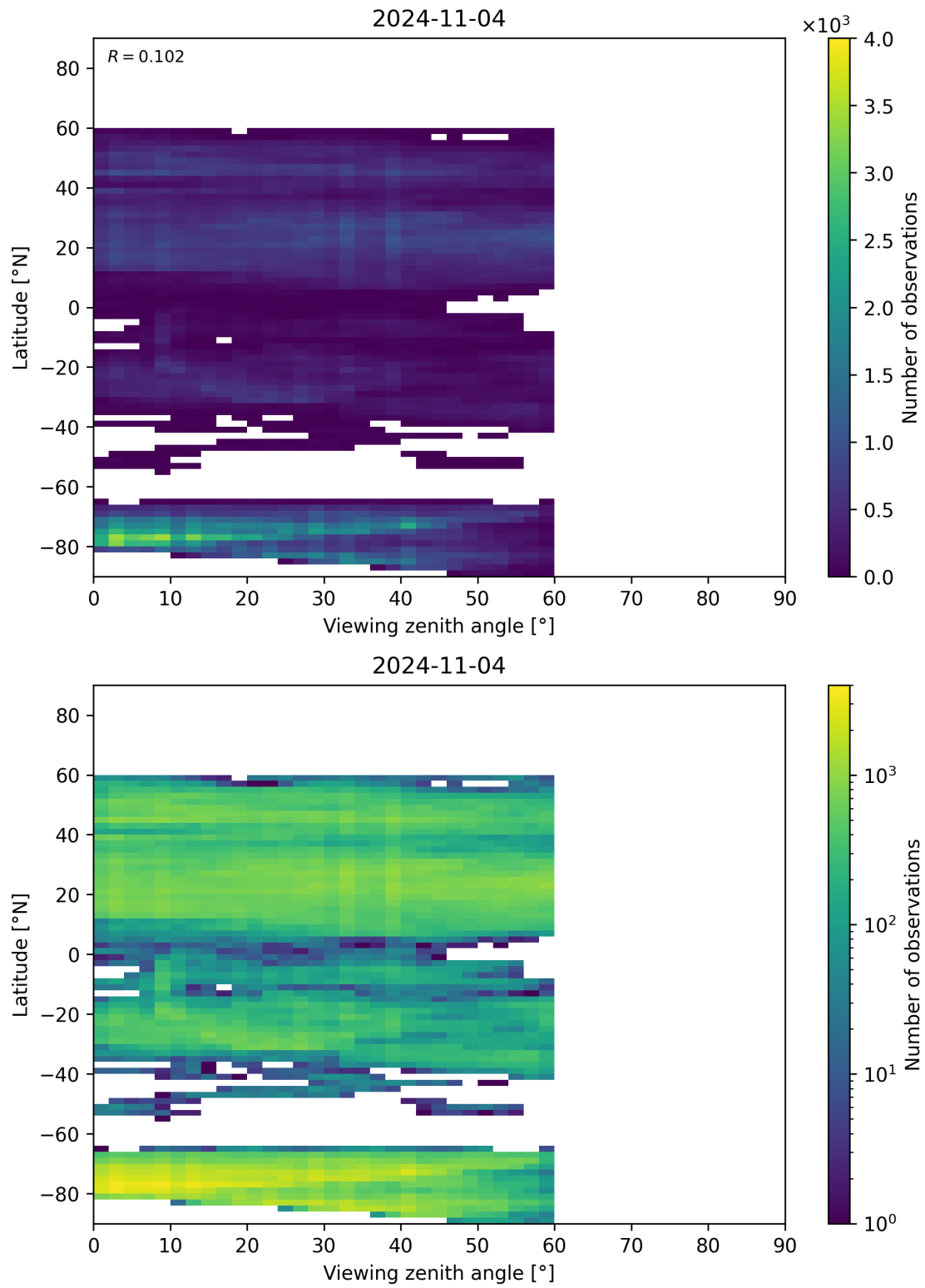
Figure 109: Scatter density plot of “Viewing zenith angle” against “Latitude” for 2024-11-04 to 2024-11-05.
