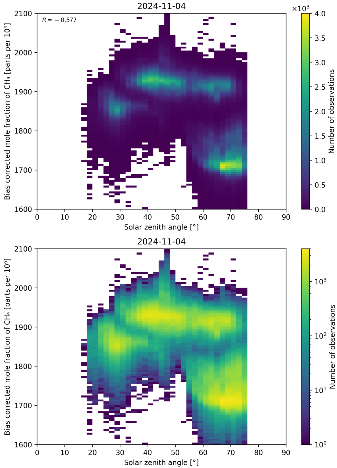
Figure 100: Scatter density plot of “Solar zenith angle” against “Bias corrected mole fraction of CH 4 ” for 2024-11-04 to 2024-11-05.
