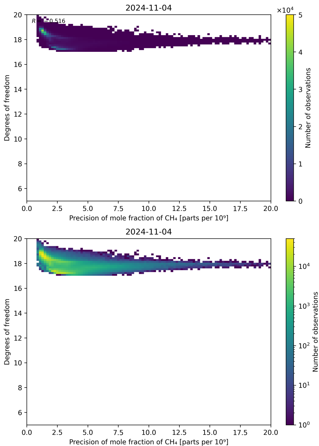
Figure 80: Scatter density plot of “Precision of mole fraction of CH 4 ” against “Degrees of freedom” for 2024-11-04 to 2024-11-05.
