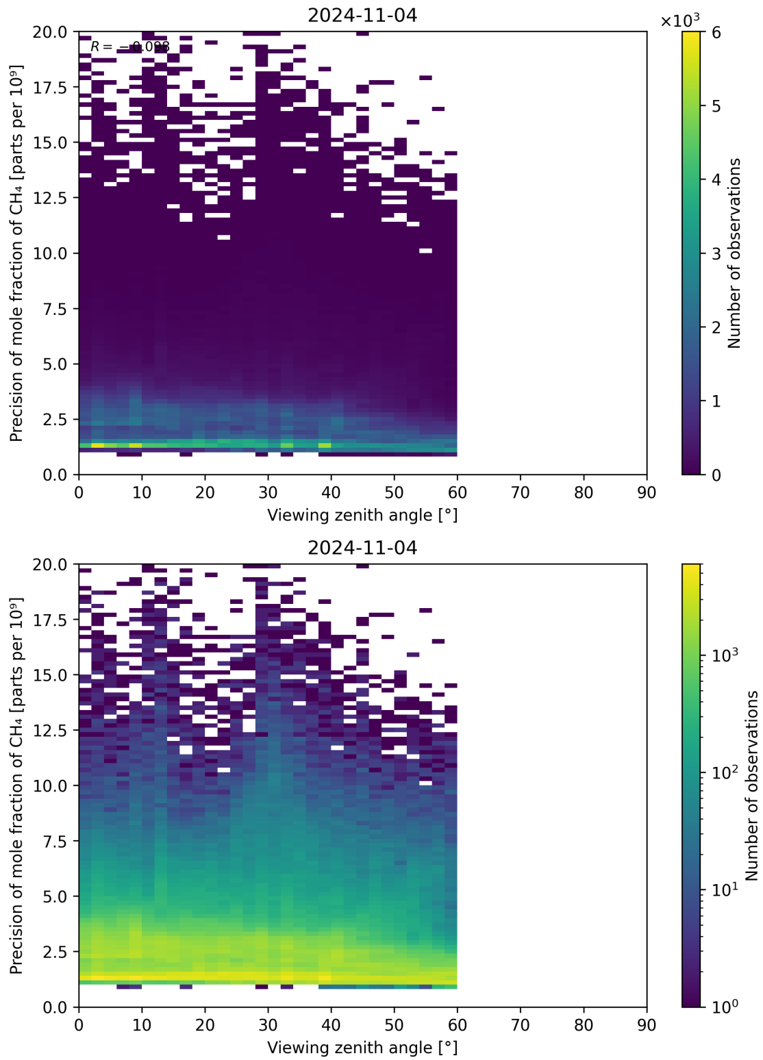
Figure 112: Scatter density plot of “Viewing zenith angle” against “Precision of mole fraction of \text{CH}_4 ” for 2024-11-04 to 2024-11-05.
