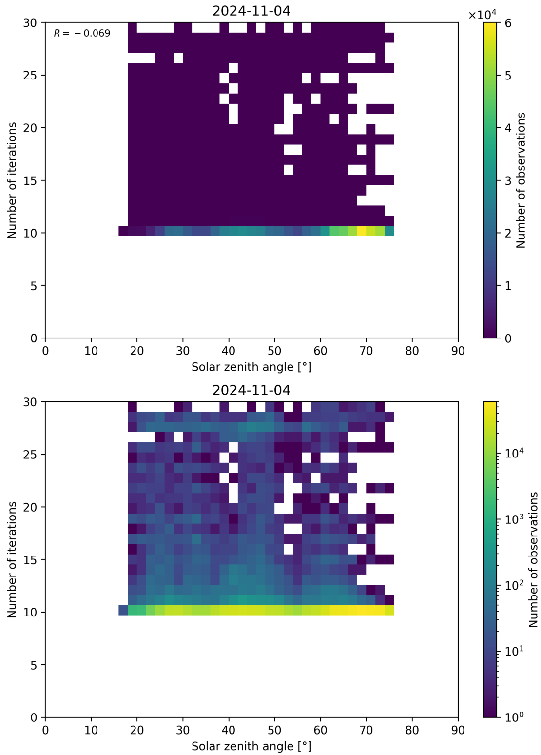
Figure 102: Scatter density plot of “Solar zenith angle” against “Number of iterations” for 2024-11-04 to 2024-11-05.
