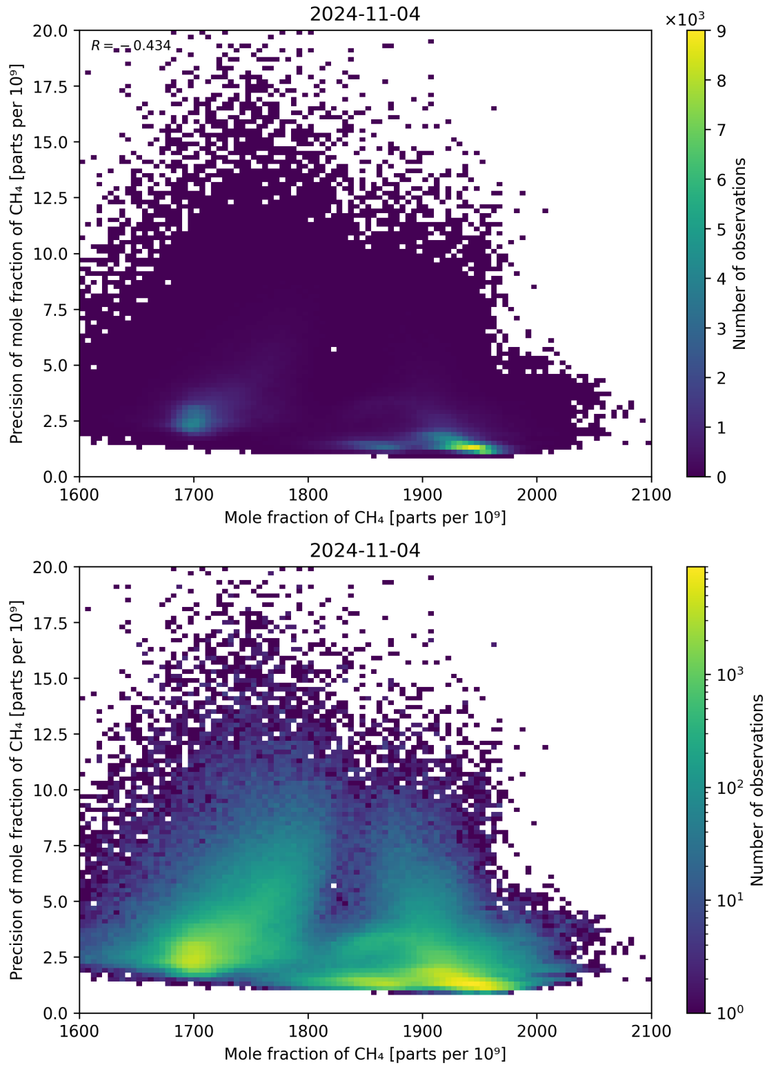
Figure 75: Scatter density plot of “Mole fraction of CH 4 ” against “Precision of mole fraction of CH 4 ” for 2024-11-04 to 2024-11-05.
