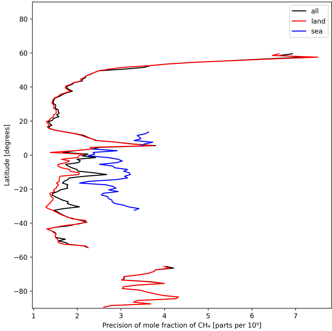
Figure 13: Zonal average of “Precision of mole fraction of CH 4 ” for 2024-11-04 to 2024-11-05.
