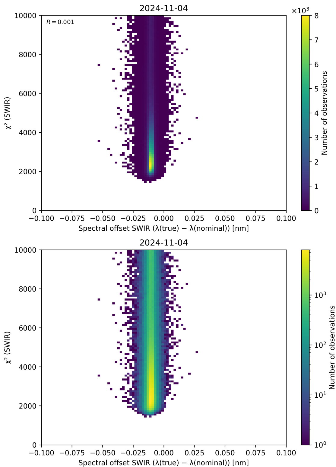
Figure 118: Scatter density plot of “Spectral offset SWIR ( \lambda_{\text{true}} - \lambda_{\text{nominal}} )” against “ \chi^2 (SWIR)” for 2024-11-04 to 2024-11-05.
