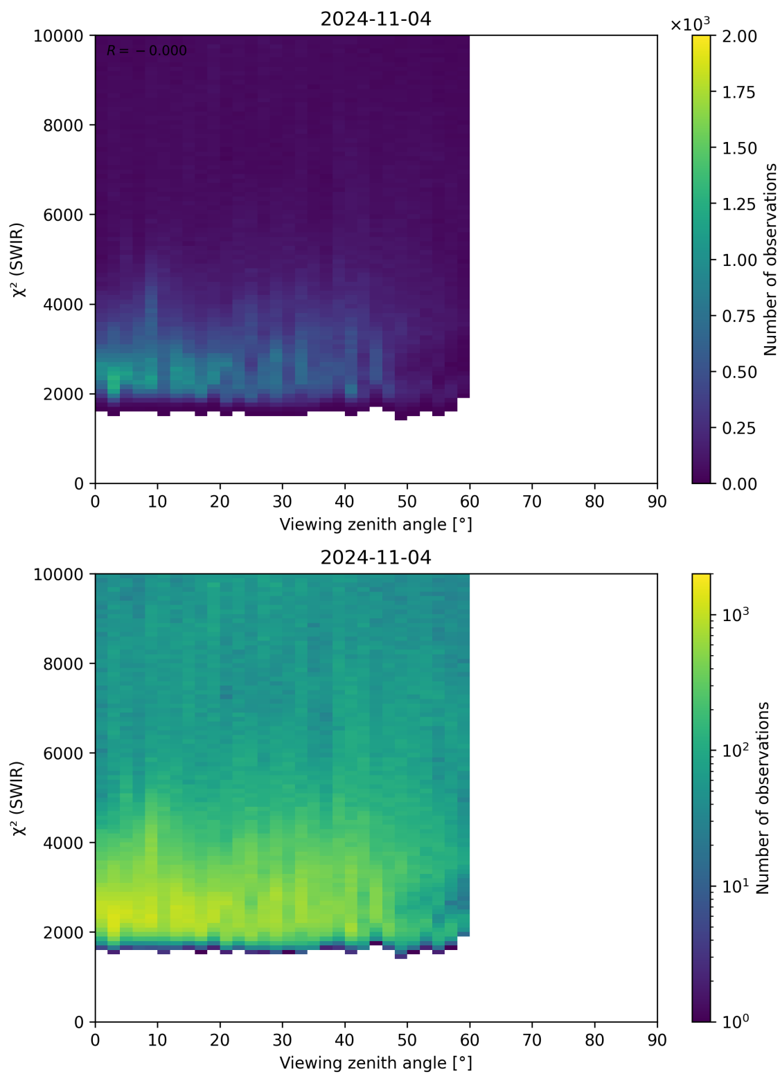
Figure 106: Scatter density plot of “Viewing zenith angle” against “ \chi^2 (SWIR)” for 2024-11-04 to 2024-11-05.
