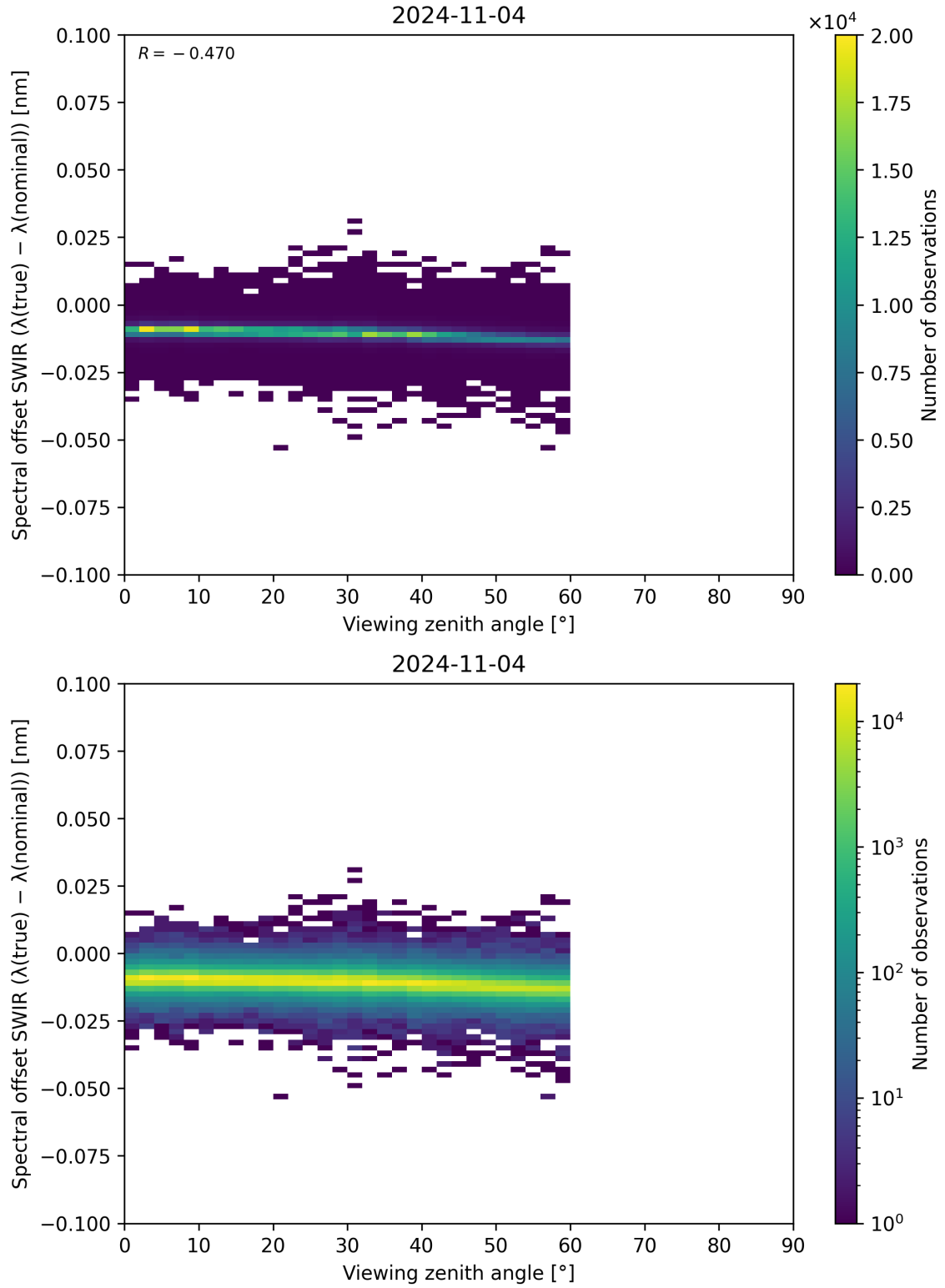
Figure 116: Scatter density plot of “Viewing zenith angle” against “Spectral offset SWIR ( \lambda_{\text{true}} - \lambda_{\text{nominal}} )” for 2024-11-04 to 2024-11-05.
