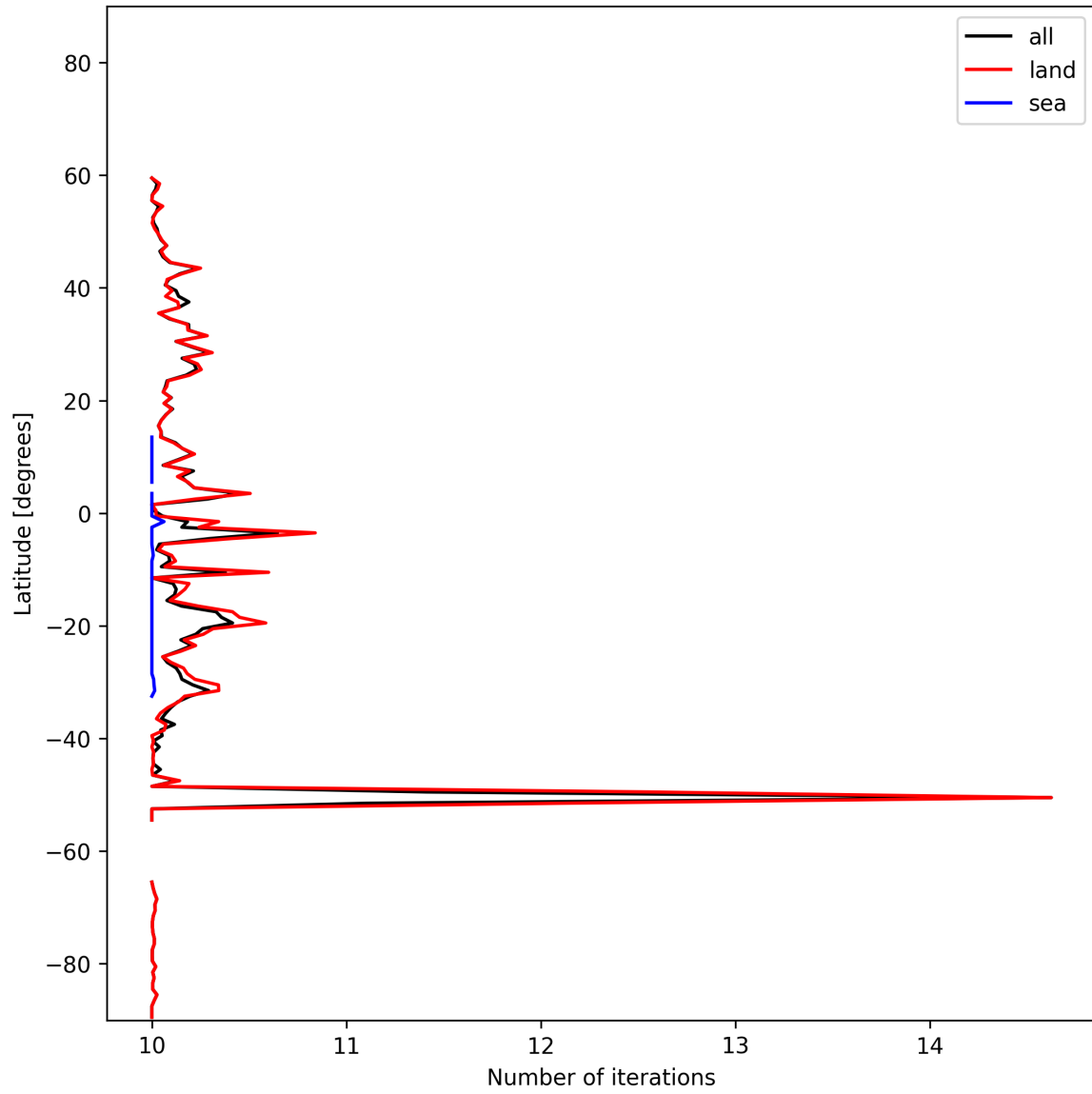
Figure 20: Zonal average of “Number of iterations” for 2024-11-04 to 2024-11-05.
