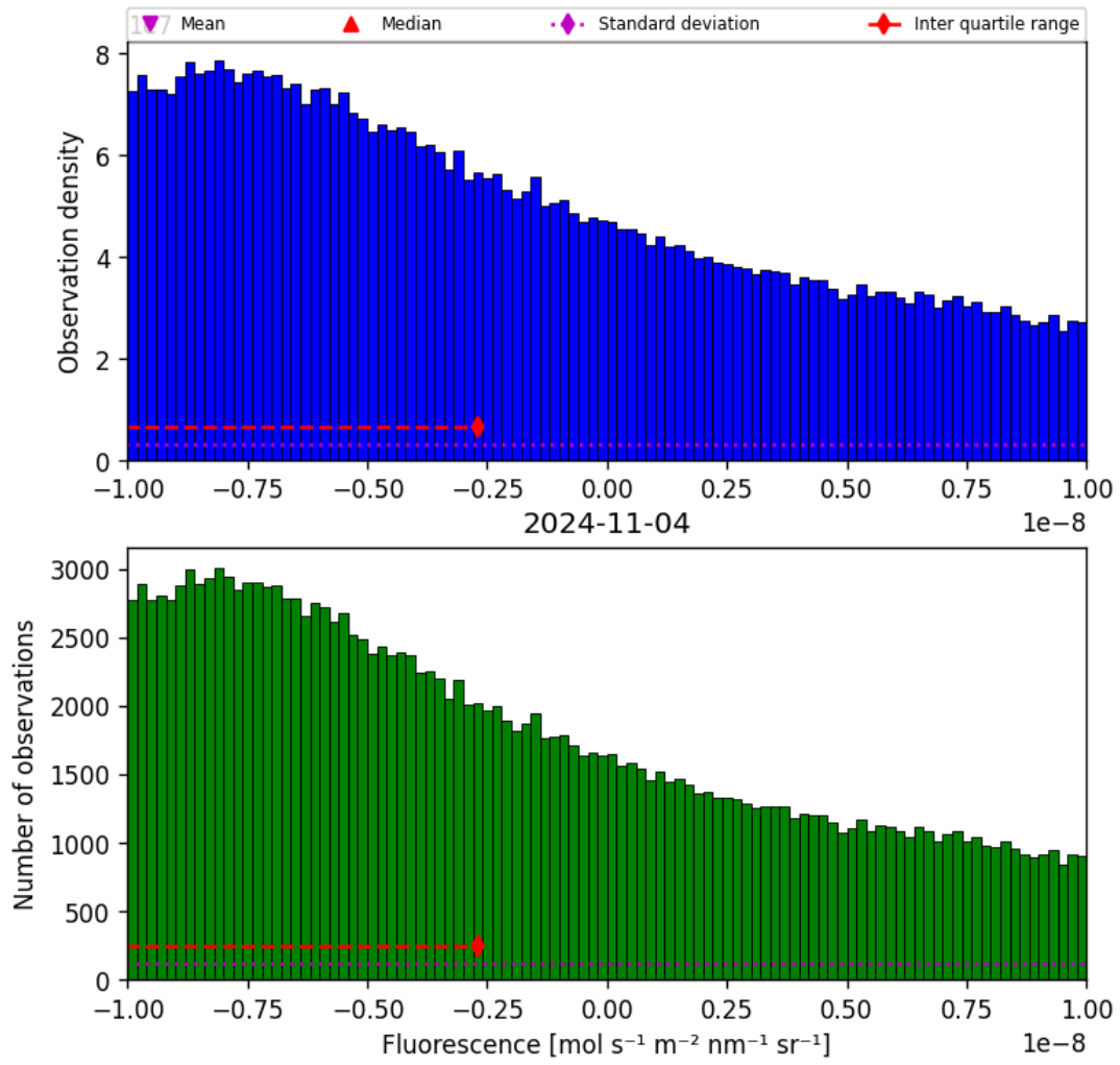
Figure 32: Histogram of “Fluorescence” for 2024-11-04 to 2024-11-05
