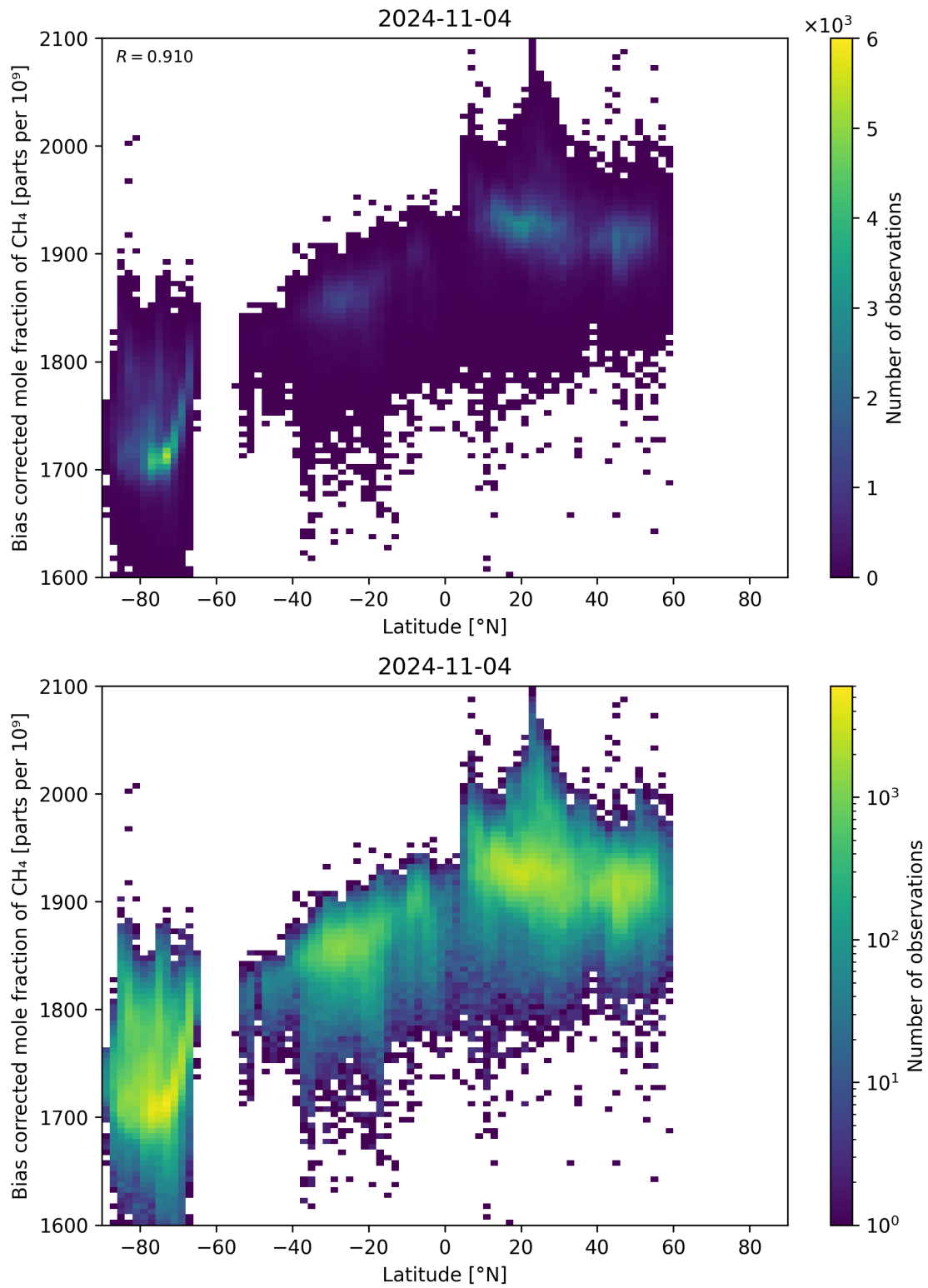
Figure 58: Scatter density plot of “Latitude” against “Bias corrected mole fraction of CH 4 ” for 2024-11-04 to 2024-11-05.
