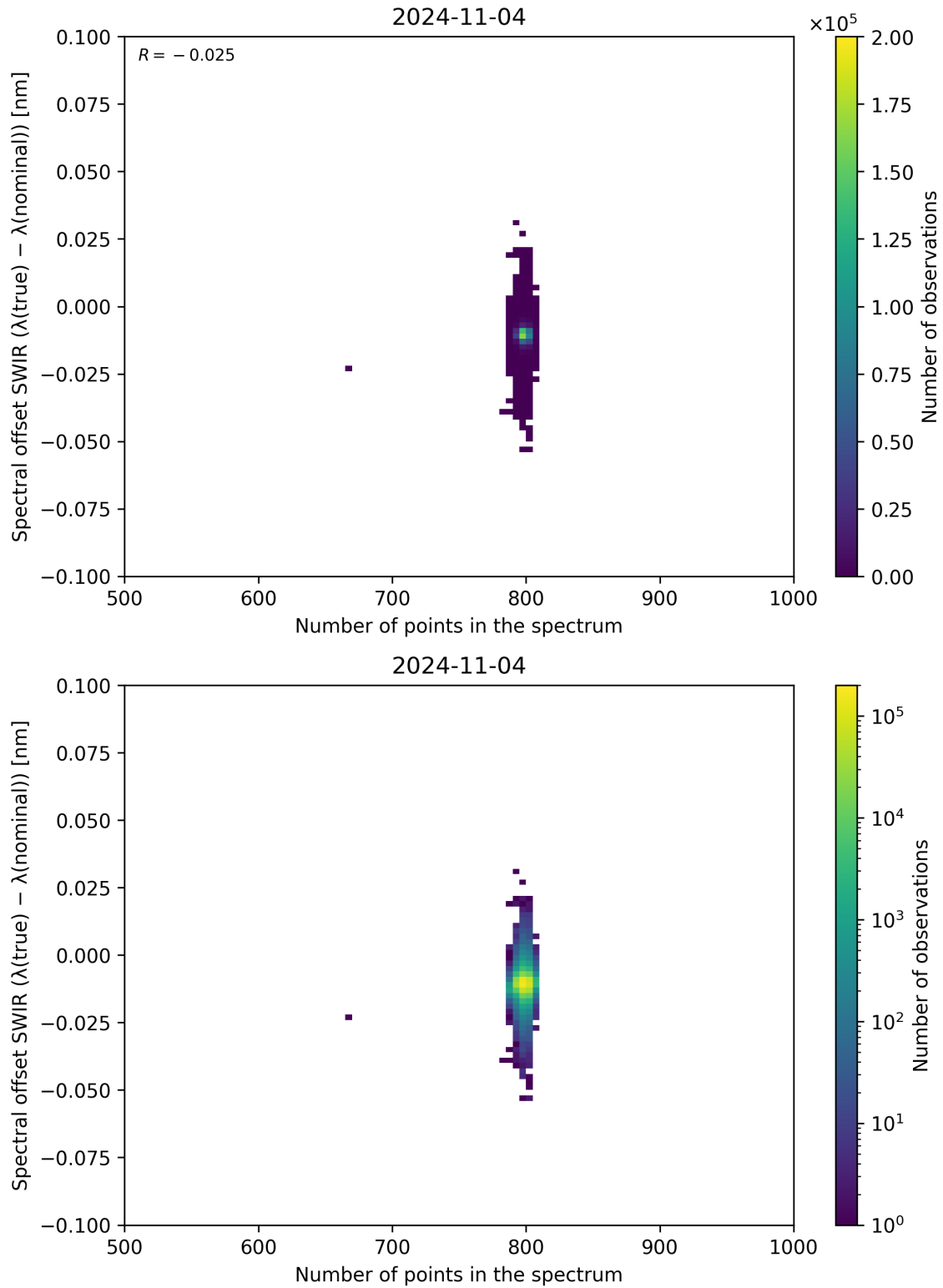
Figure 93: Scatter density plot of “Number of points in the spectrum” against “Spectral offset SWIR ( \lambda_{\text{true}} - \lambda_{\text{nominal}} )” for 2024-11-04 to 2024-11-05.
