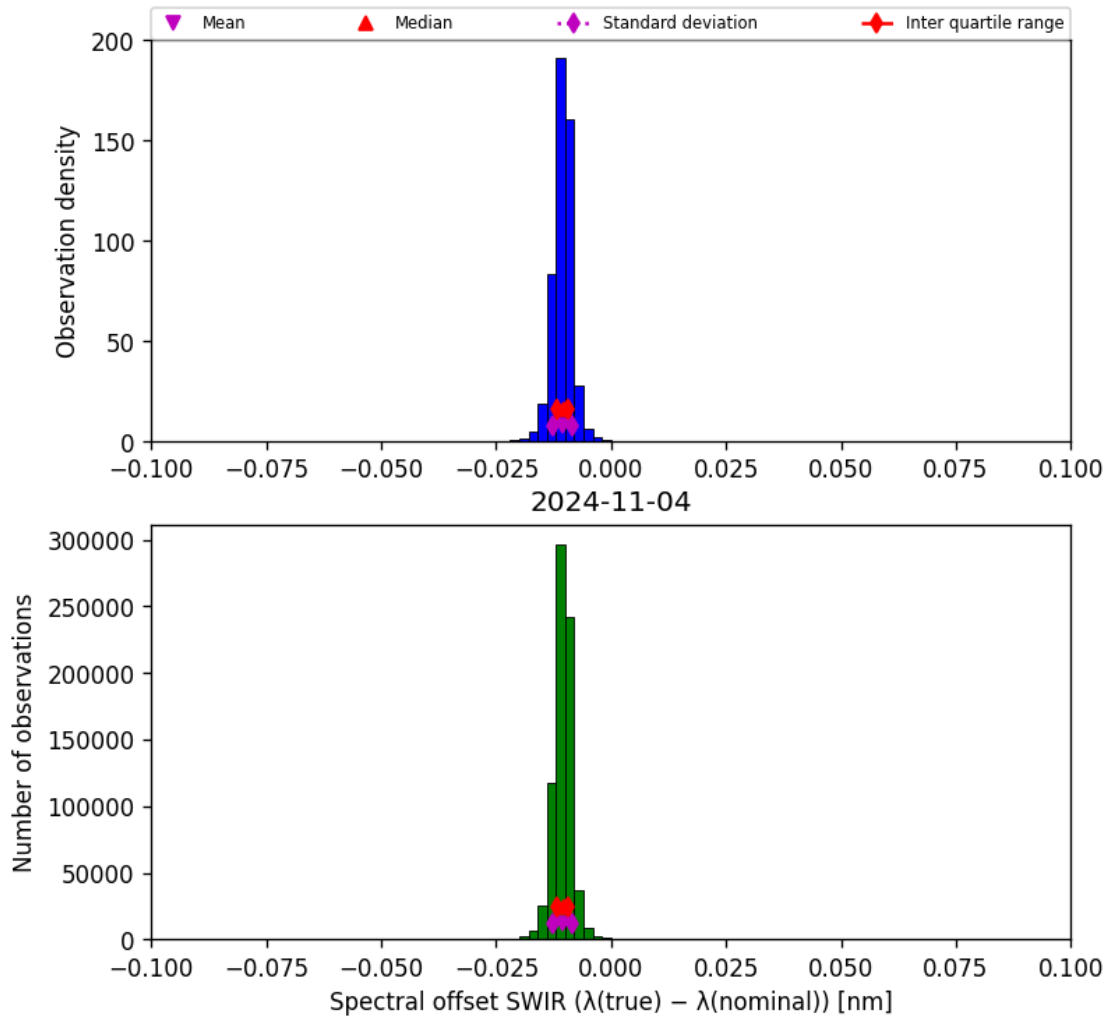
Figure 27: Histogram of “Spectral offset SWIR ( \lambda_{\text{true}} - \lambda_{\text{nominal}} )” for 2024-11-04 to 2024-11-05
