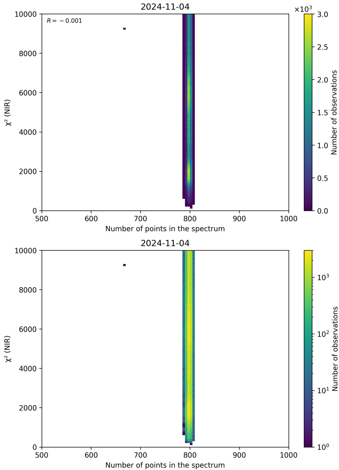
Figure 88: Scatter density plot of “Number of points in the spectrum” against “ \chi^2 (NIR)” for 2024-11-04 to 2024-11-05.
