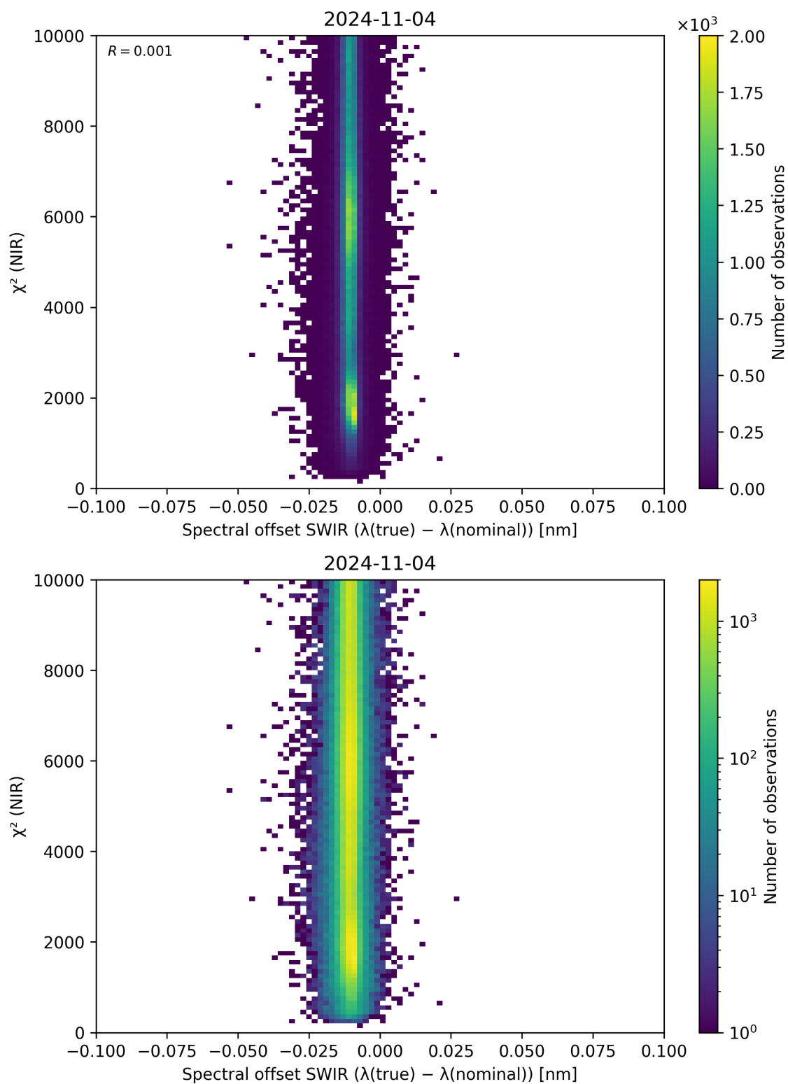
Figure 117: Scatter density plot of “Spectral offset SWIR ( \lambda_{\text{true}} - \lambda_{\text{nominal}} )” against “ \chi^2 (NIR)” for 2024-11-04 to 2024-11-05.
