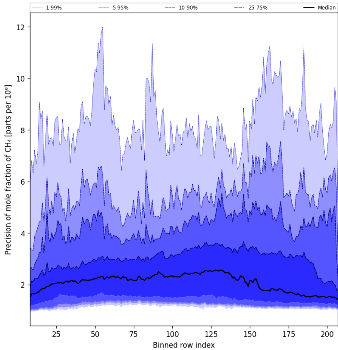
Figure 35: Along track statistics of “Precision of mole fraction of CH 4 ” for 2024-11-04 to 2024-11-05
