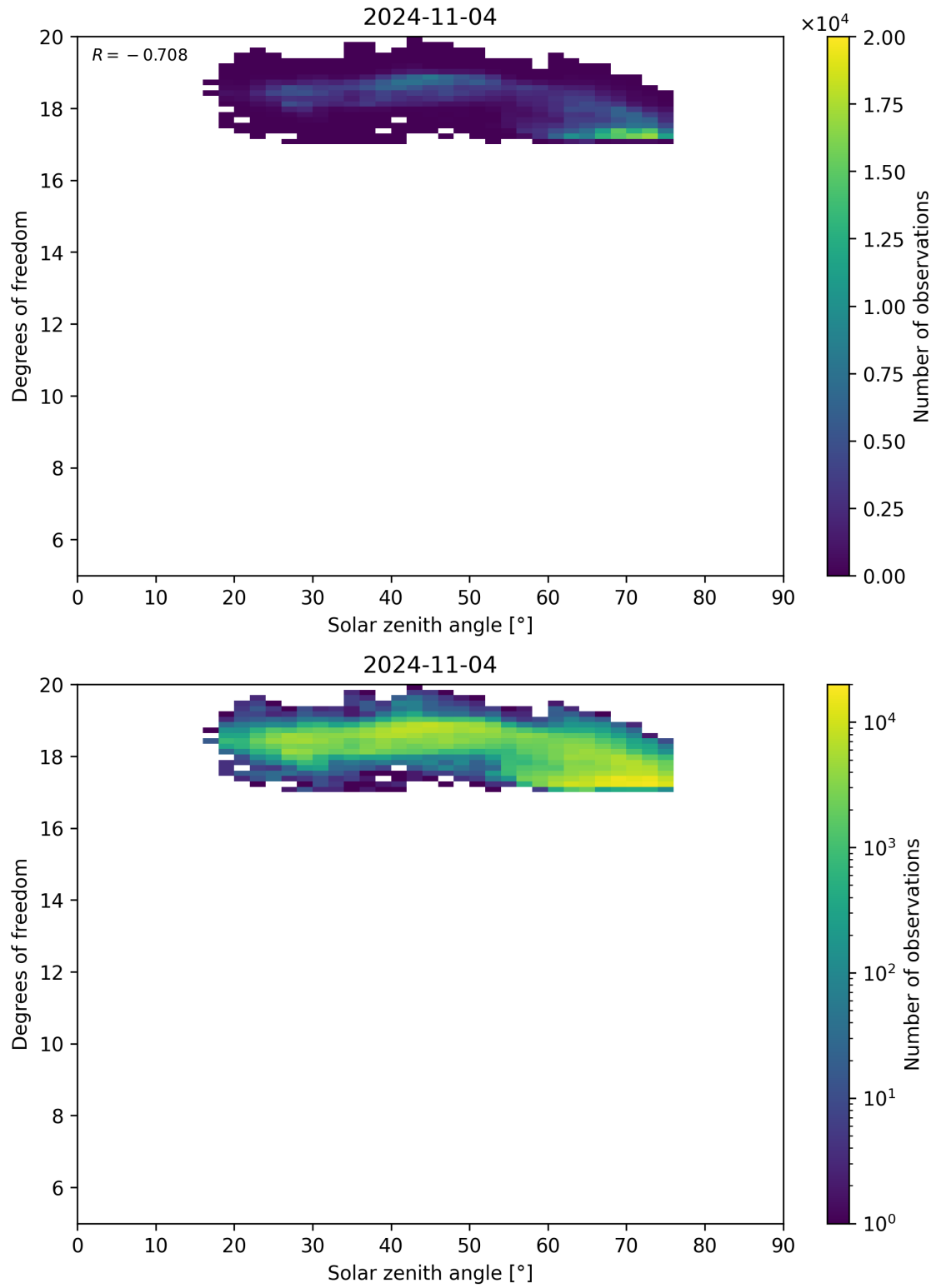
Figure 96: Scatter density plot of “Solar zenith angle” against “Degrees of freedom” for 2024-11-04 to 2024-11-05.
