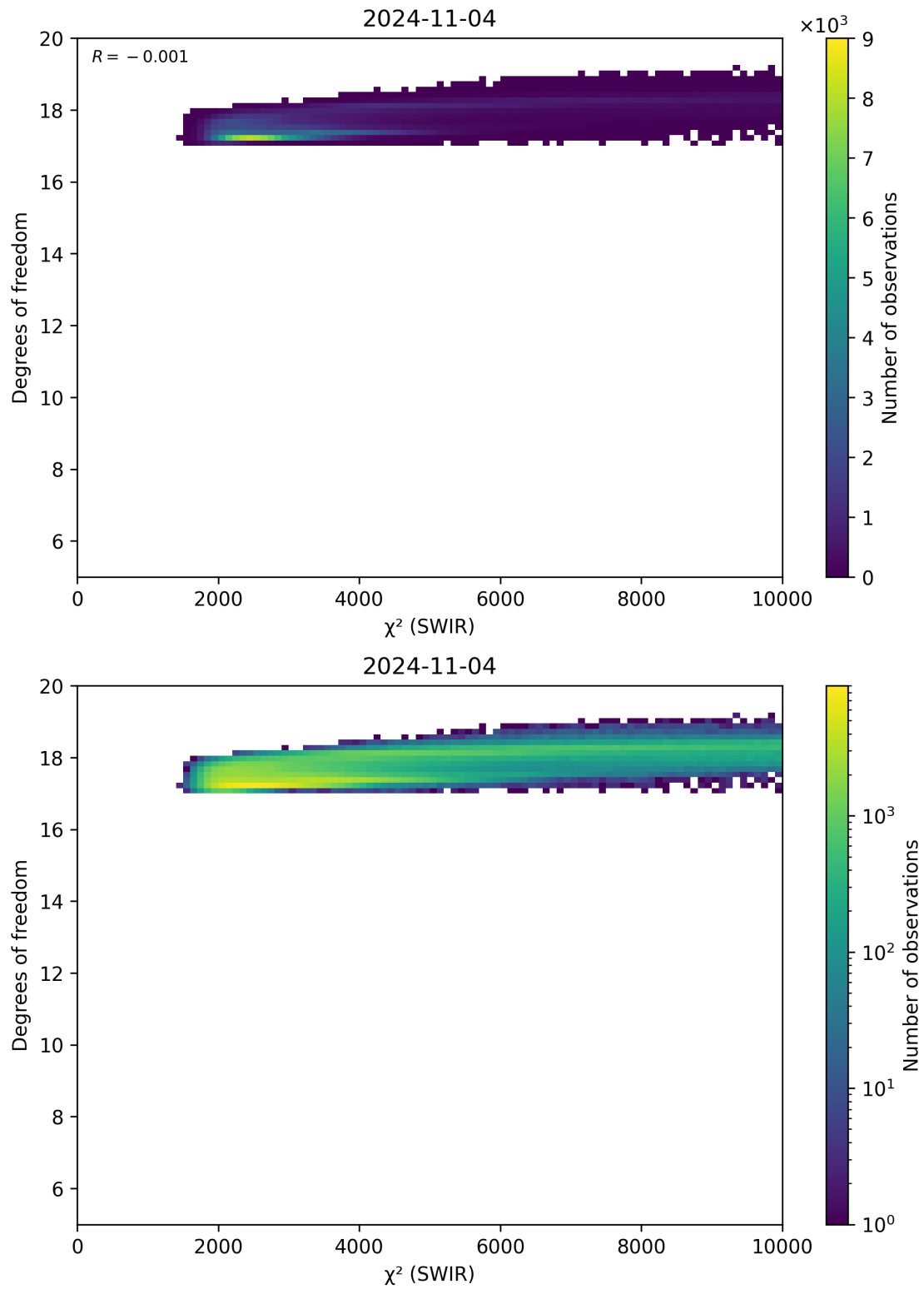
Figure 48: Scatter density plot of “ \chi^2 (SWIR)” against “Degrees of freedom” for 2024-11-04 to 2024-11-05.
