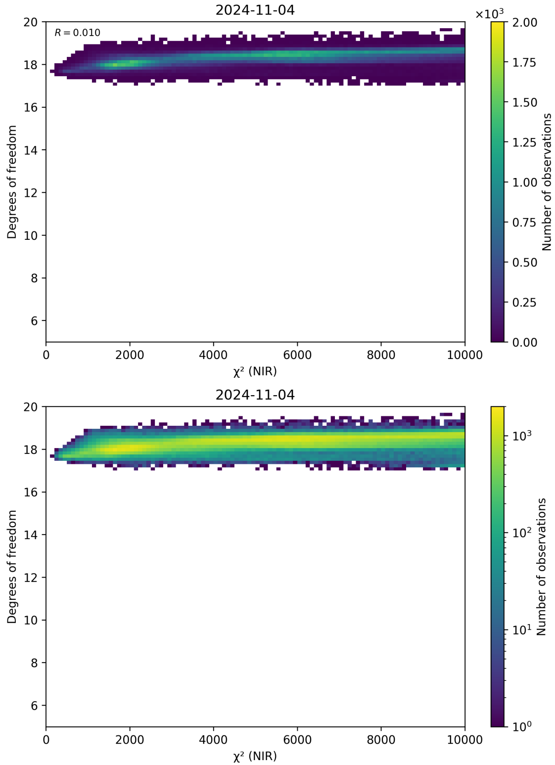
Figure 44: Scatter density plot of “ \chi^2 (NIR)” against “Degrees of freedom” for 2024-11-04 to 2024-11-05.
