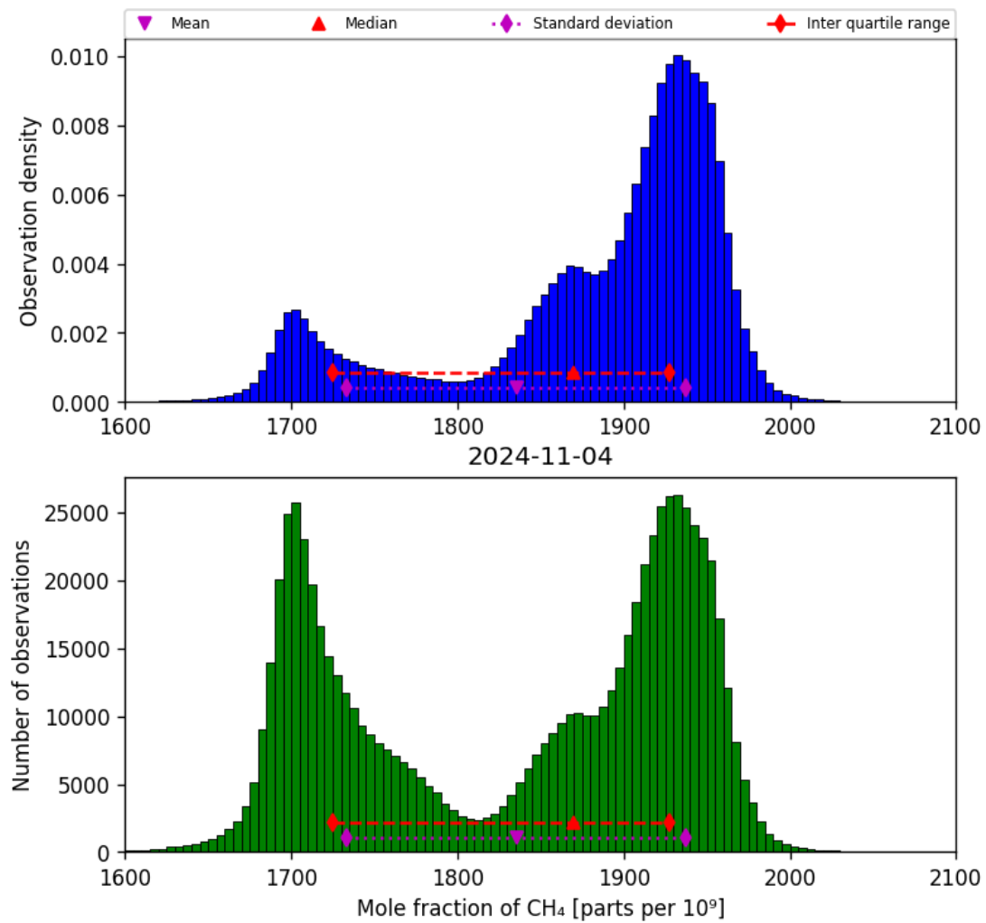
Figure 23: Histogram of “Mole fraction of CH 4 ” for 2024-11-04 to 2024-11-05
