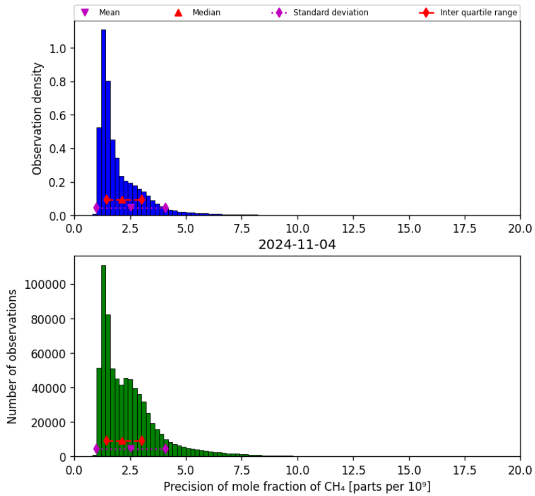
Figure 24: Histogram of “Precision of mole fraction of CH 4 ” for 2024-11-04 to 2024-11-05
