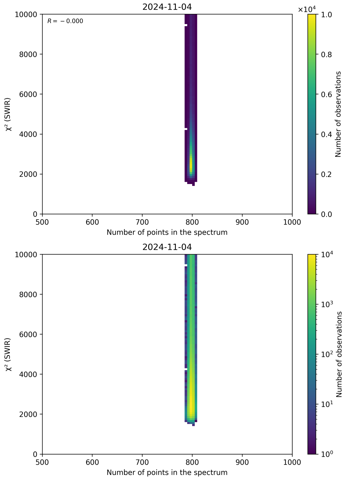
Figure 89: Scatter density plot of “Number of points in the spectrum” against “ \chi^2 (SWIR)” for 2024-11-04 to 2024-11-05.
