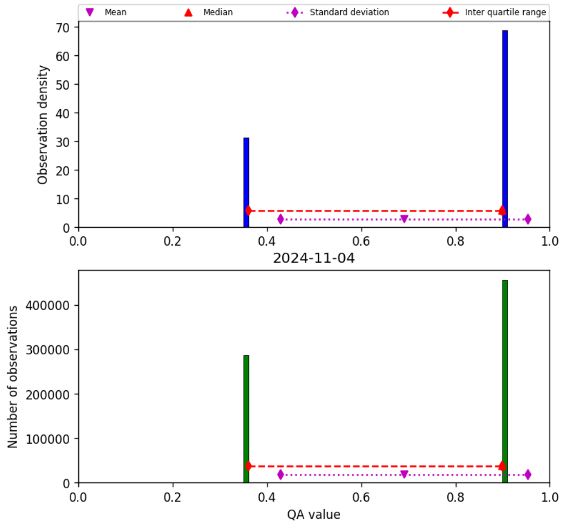
Figure 22: Histogram of “QA value” for 2024-11-04 to 2024-11-05
