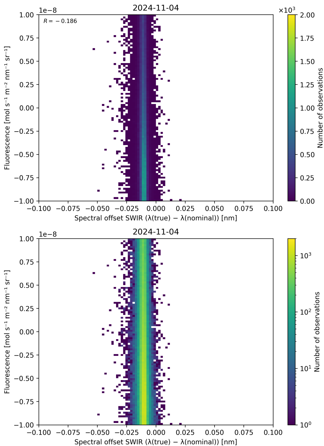
Figure 120: Scatter density plot of “Spectral offset SWIR ( \lambda_{\text{true}} - \lambda_{\text{nominal}} )” against “Fluorescence” for 2024-11-04 to 2024-11-05.
