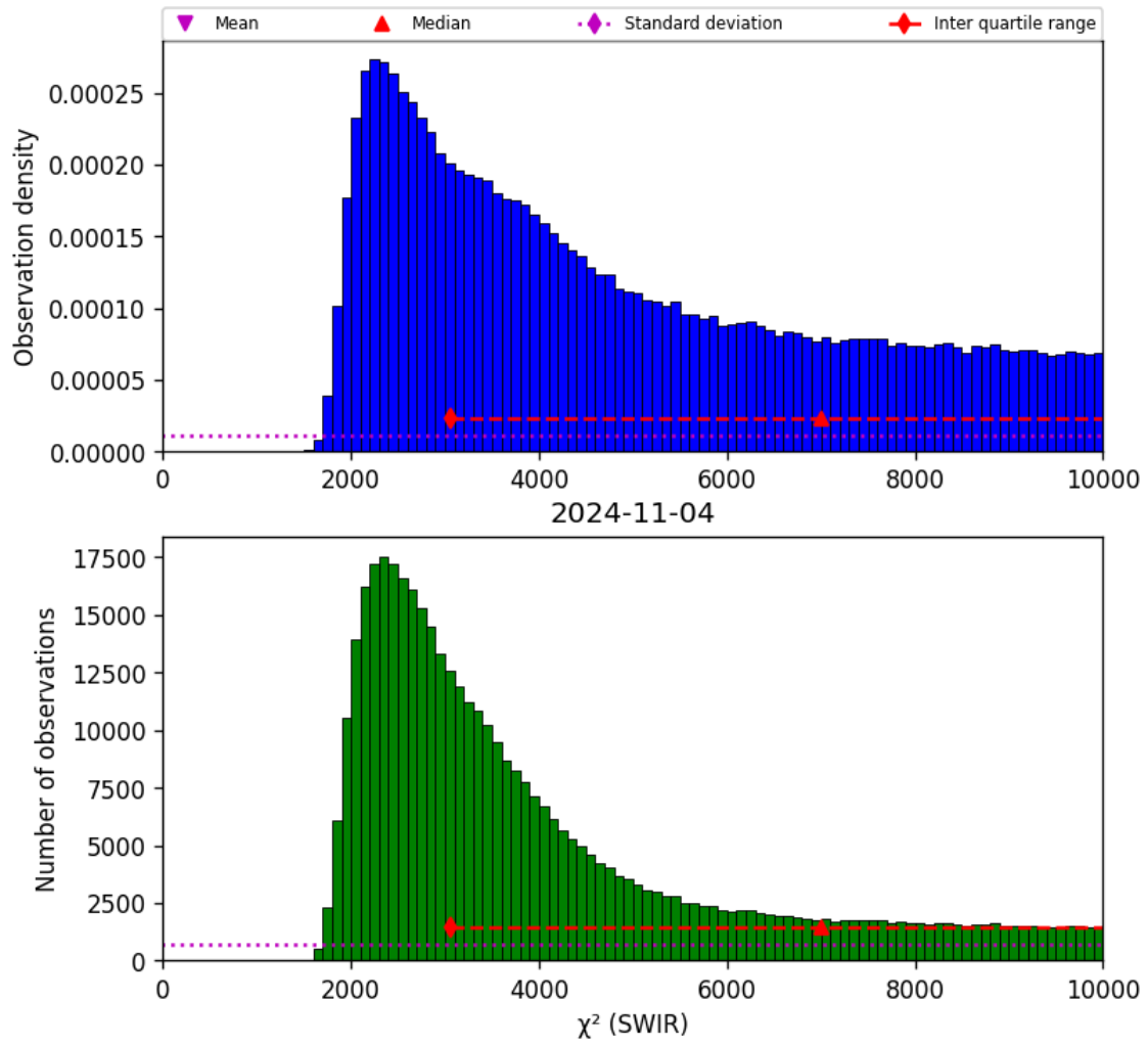
Figure 28: Histogram of “ \chi^2 (SWIR)” for 2024-11-04 to 2024-11-05
