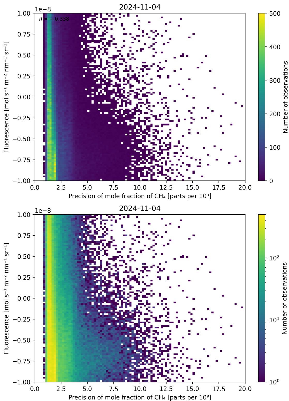
Figure 81: Scatter density plot of “Precision of mole fraction of \text{CH}_4 ” against “Fluorescence” for 2024-11-04 to 2024-11-05.
