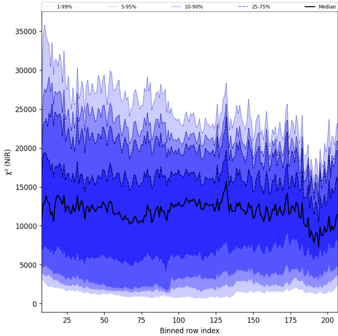
Figure 40: Along track statistics of “ \chi^2 (NIR)” for 2024-11-04 to 2024-11-05
