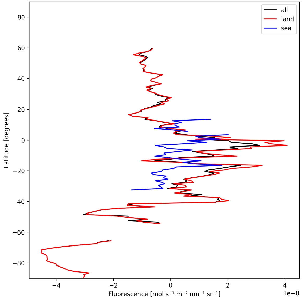
Figure 21: Zonal average of “Fluorescence” for 2024-11-04 to 2024-11-05.
