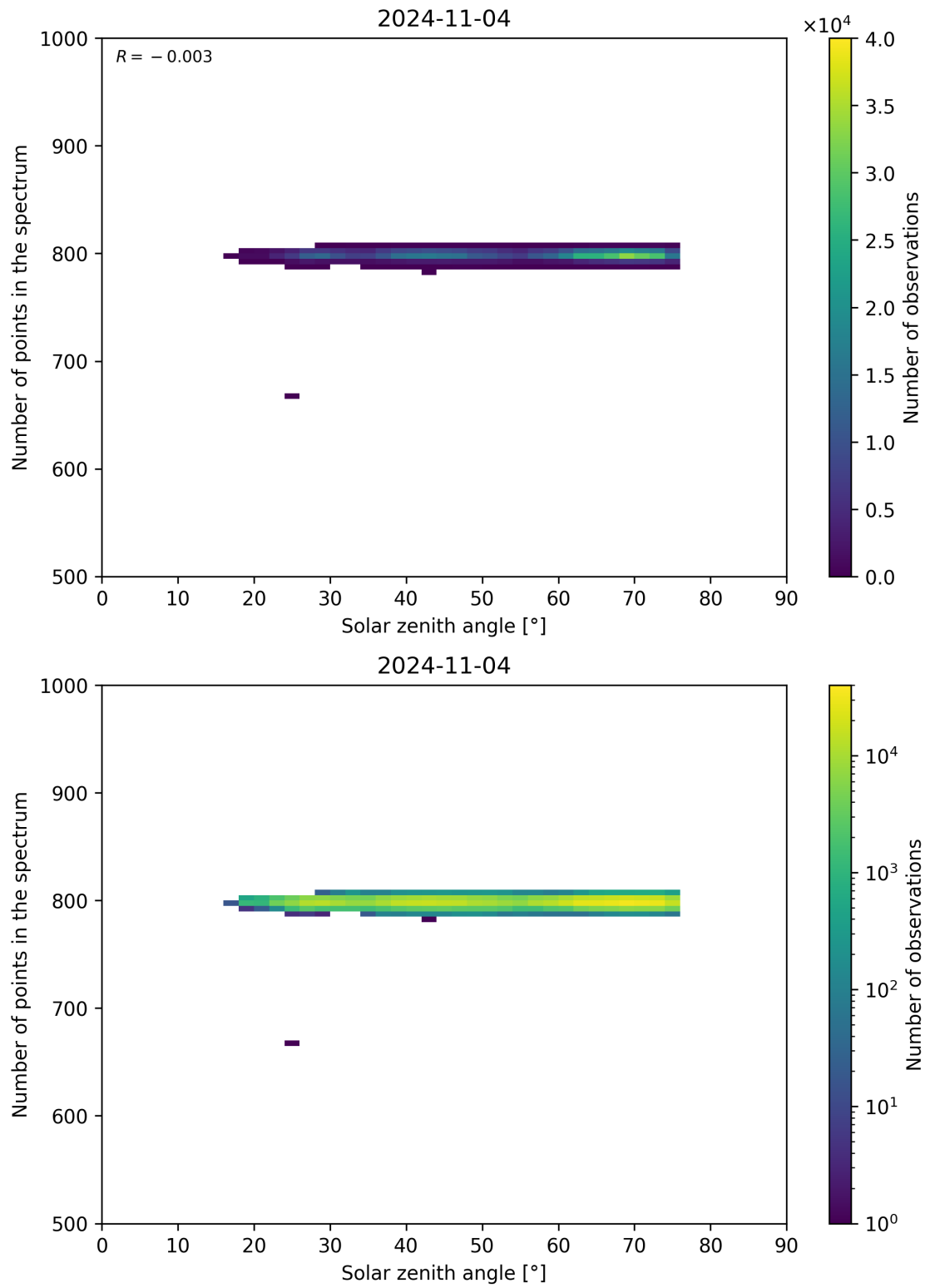
Figure 103: Scatter density plot of “Solar zenith angle” against “Number of points in the spectrum” for 2024-11-04 to 2024-11-05.
