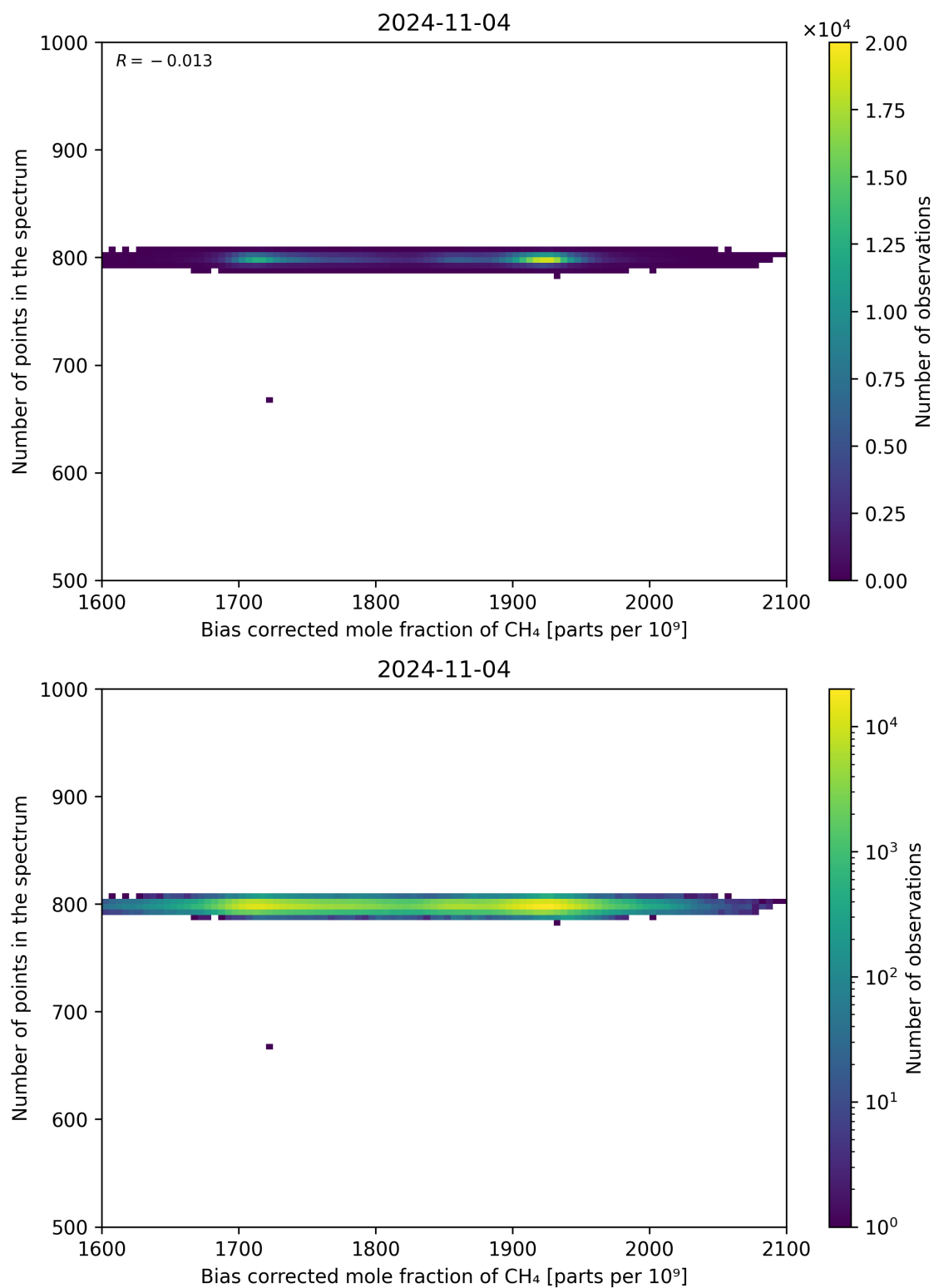
Figure 68: Scatter density plot of “Bias corrected mole fraction of CH 4 ” against “Number of points in the spectrum” for 2024-11-04 to 2024-11-05.
