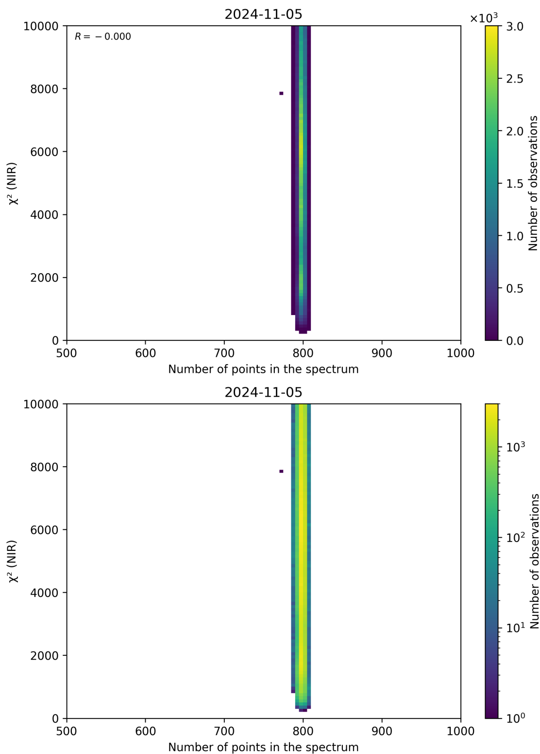
Figure 88: Scatter density plot of “Number of points in the spectrum” against “ \chi^2 (NIR)” for 2024-11-04 to 2024-11-06.
