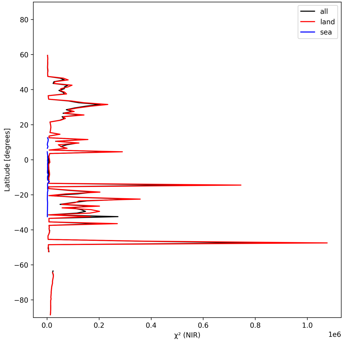
Figure 18: Zonal average of “ \chi^2 (NIR)” for 2024-11-04 to 2024-11-06.
