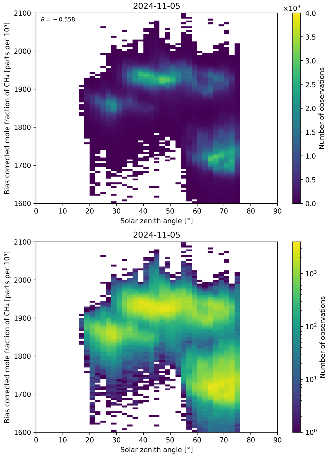
Figure 100: Scatter density plot of “Solar zenith angle” against “Bias corrected mole fraction of CH 4 ” for 2024-11-04 to 2024-11-06.
