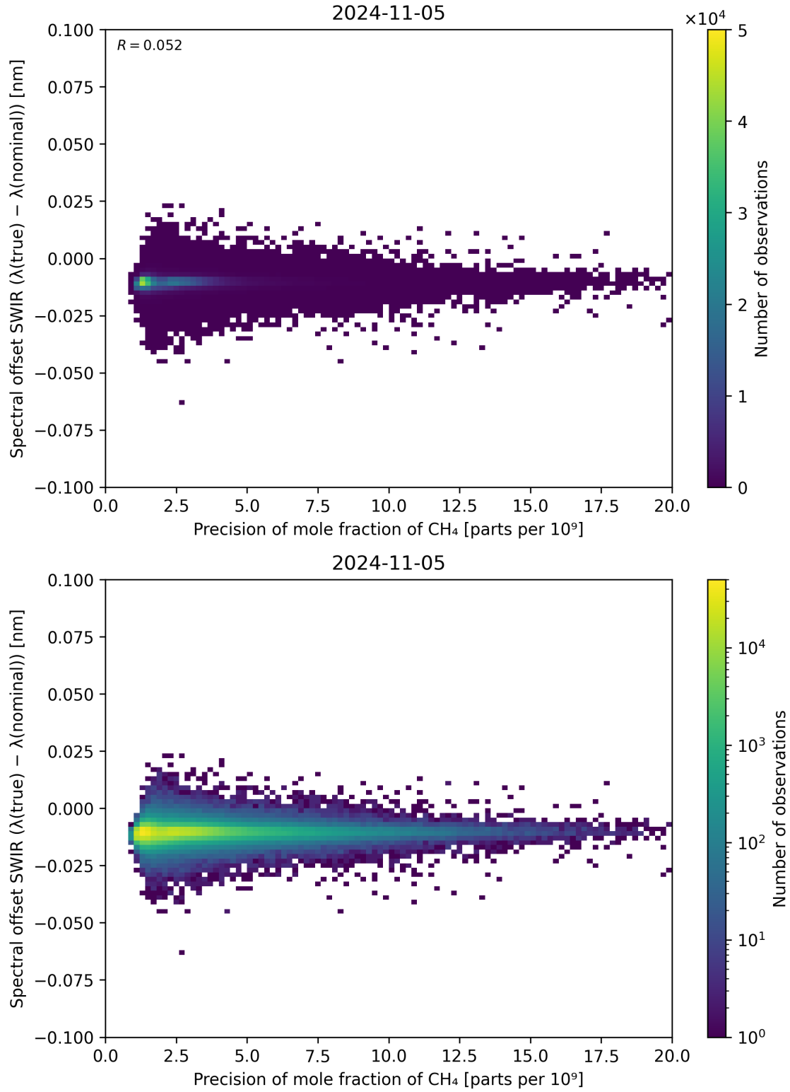
Figure 85: Scatter density plot of “Precision of mole fraction of \text{CH}_4 ” against “Spectral offset SWIR ( \lambda_{\text{true}} - \lambda_{\text{nominal}} )” for 2024-11-04 to 2024-11-06.
