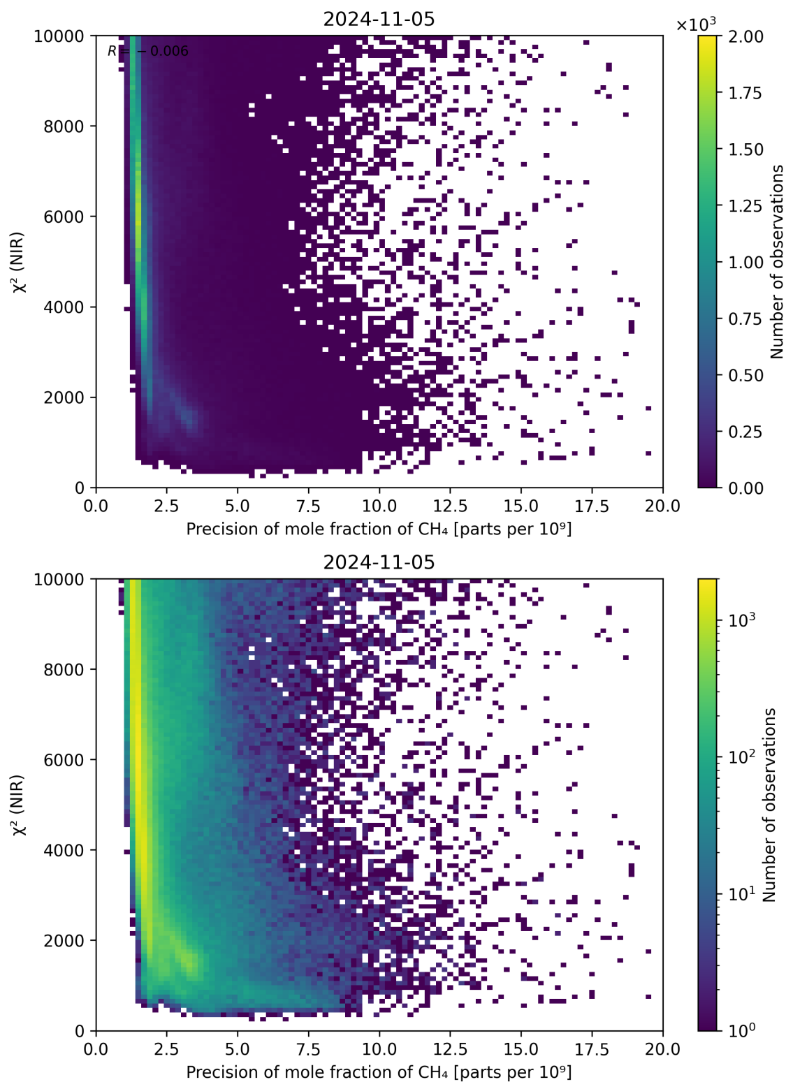
Figure 78: Scatter density plot of “Precision of mole fraction of \text{CH}_4 ” against “ \chi^2 (NIR)” for 2024-11-04 to 2024-11-06.
