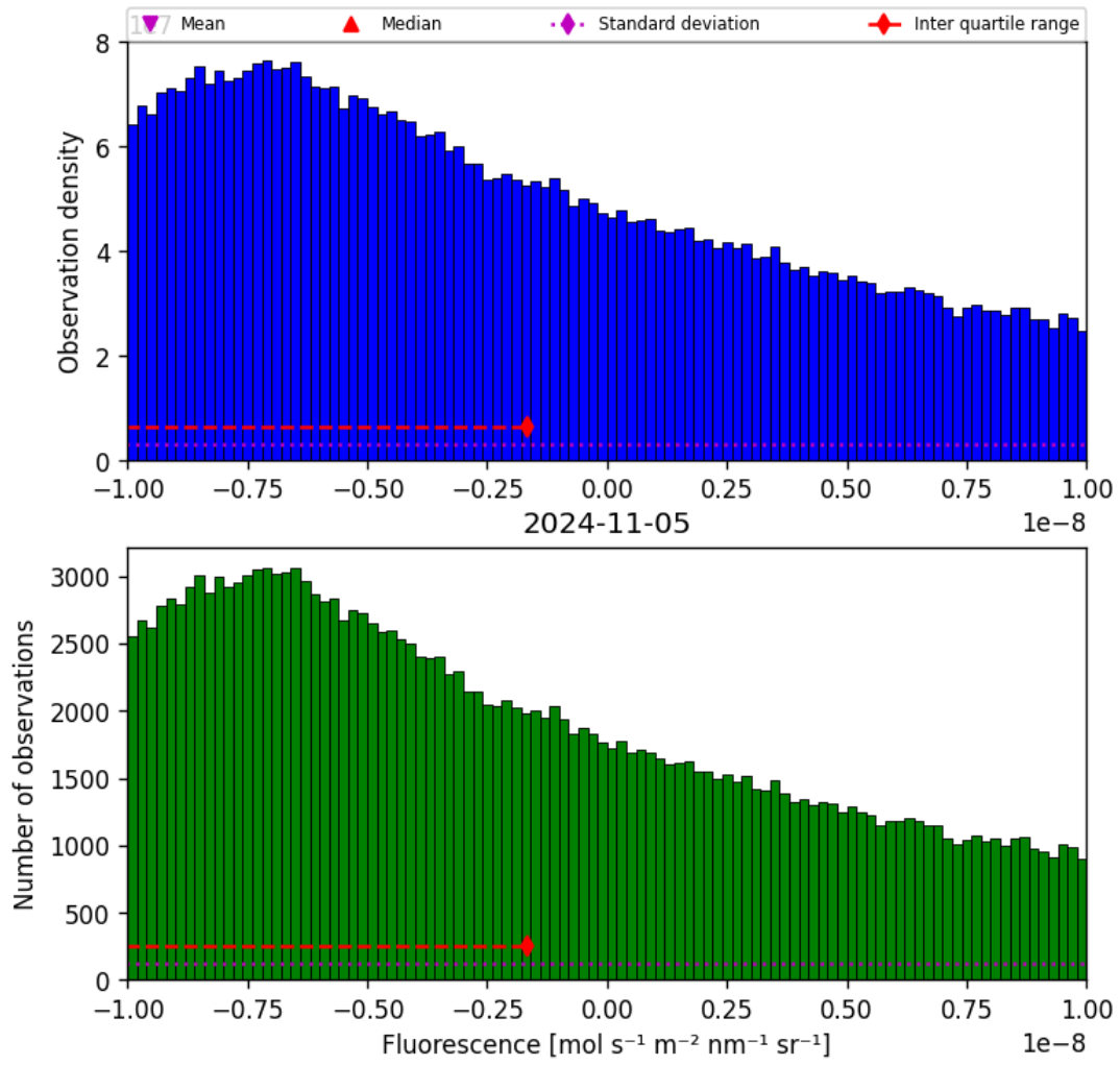
Figure 32: Histogram of “Fluorescence” for 2024-11-04 to 2024-11-06
