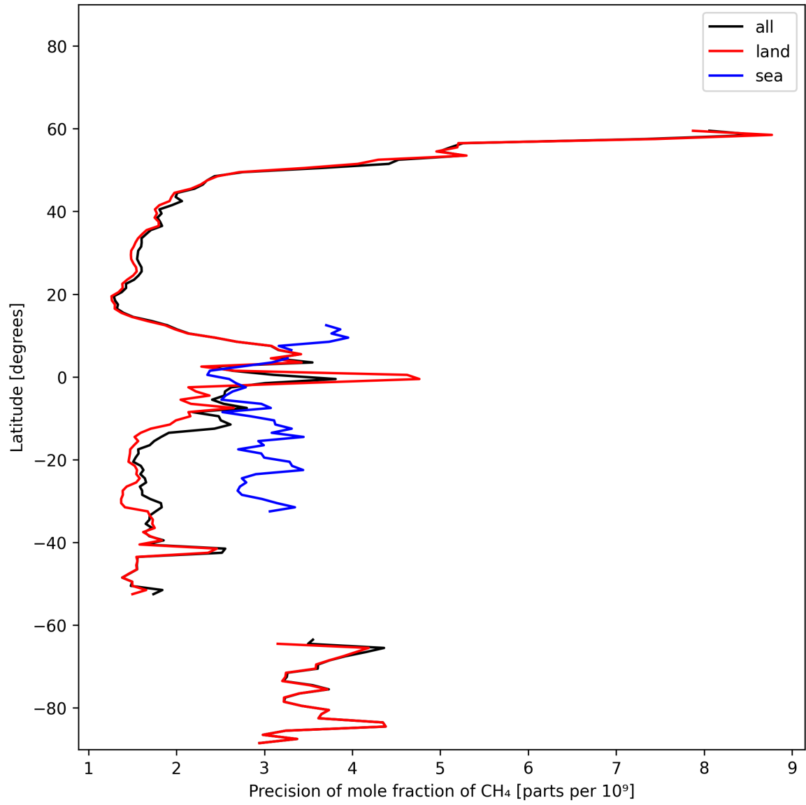
Figure 13: Zonal average of “Precision of mole fraction of CH 4 ” for 2024-11-04 to 2024-11-06.
