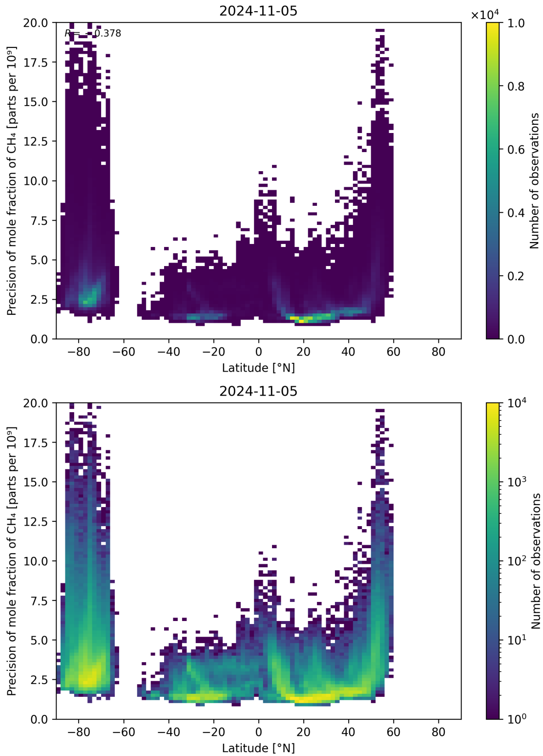
Figure 59: Scatter density plot of “Latitude” against “Precision of mole fraction of CH 4 ” for 2024-11-04 to 2024-11-06.
