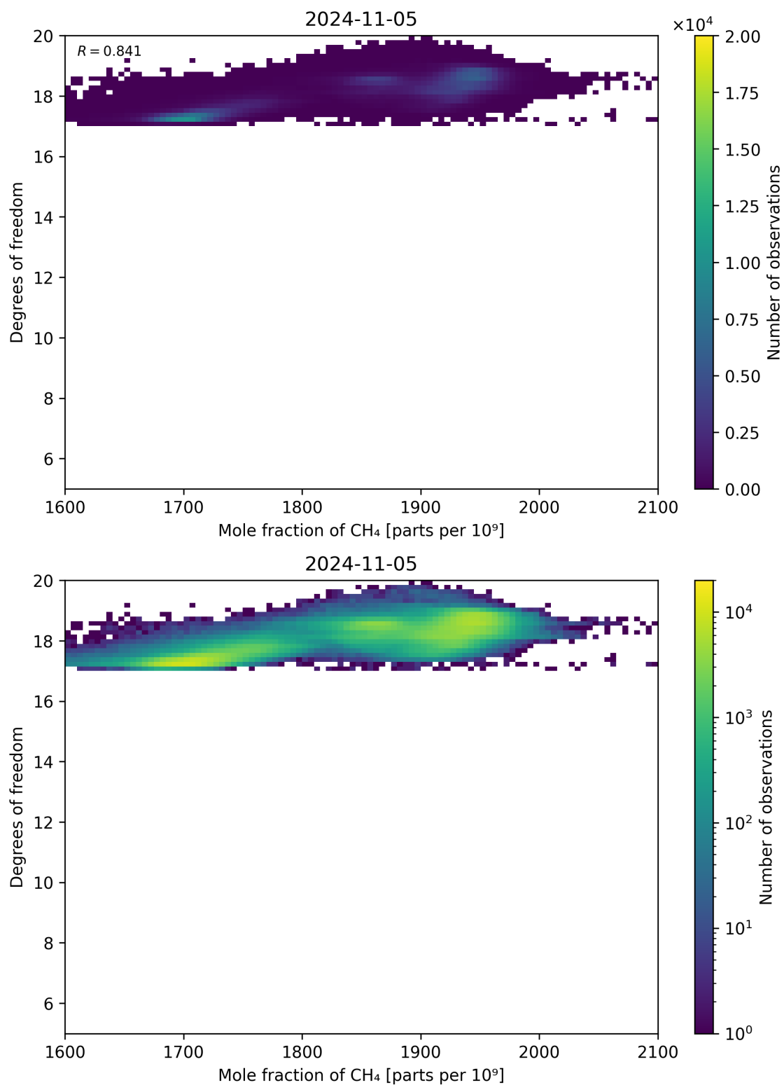
Figure 72: Scatter density plot of “Mole fraction of CH 4 ” against “Degrees of freedom” for 2024-11-04 to 2024-11-06.
