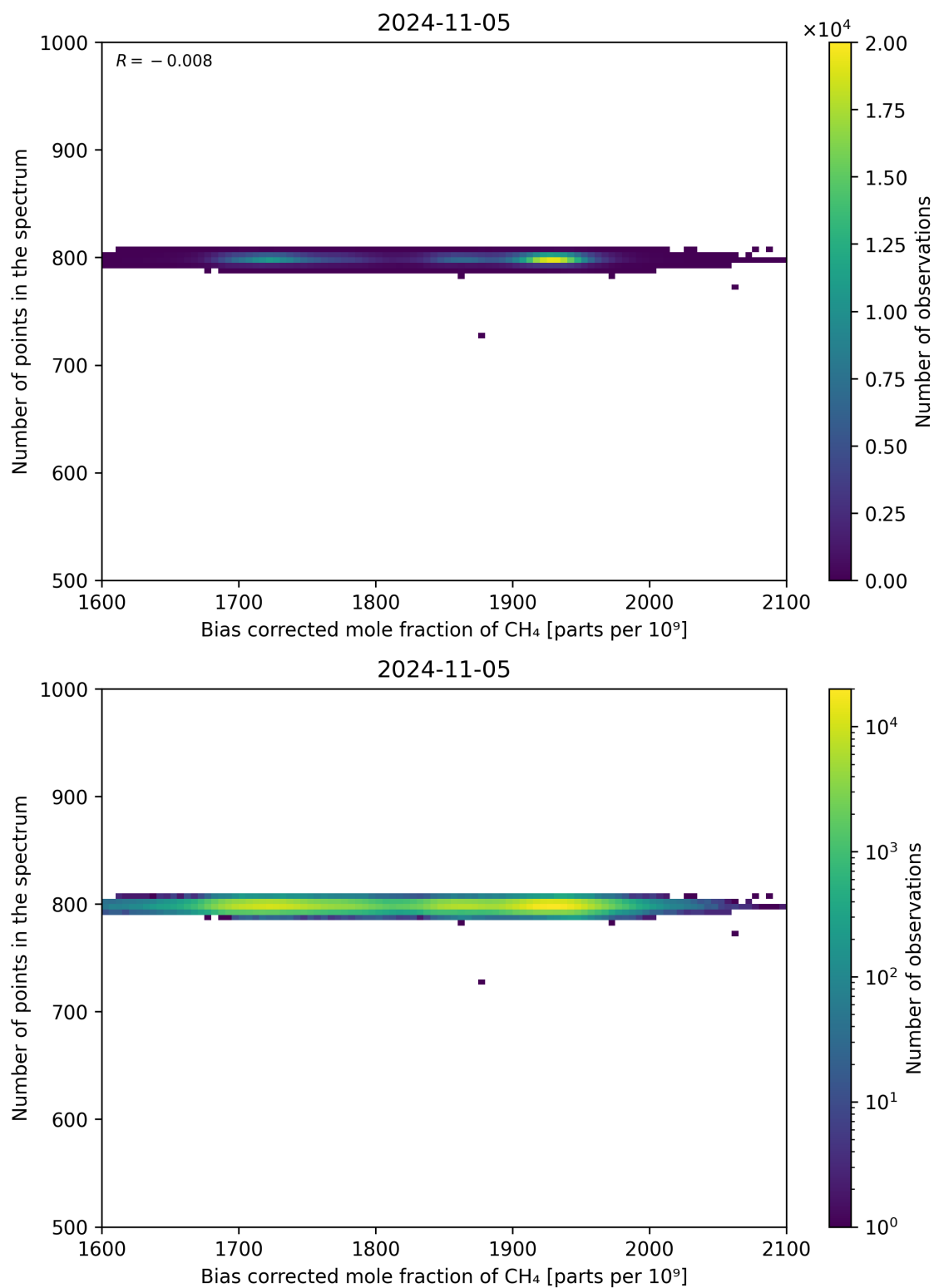
Figure 68: Scatter density plot of “Bias corrected mole fraction of CH 4 ” against “Number of points in the spectrum” for 2024-11-04 to 2024-11-06.
