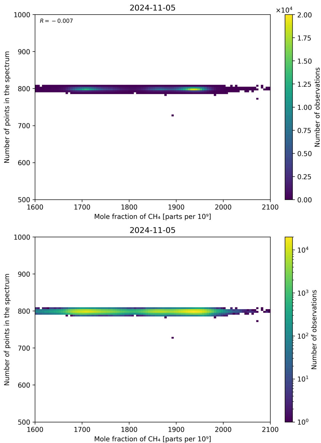
Figure 77: Scatter density plot of “Mole fraction of CH 4 ” against “Number of points in the spectrum” for 2024-11-04 to 2024-11-06.
