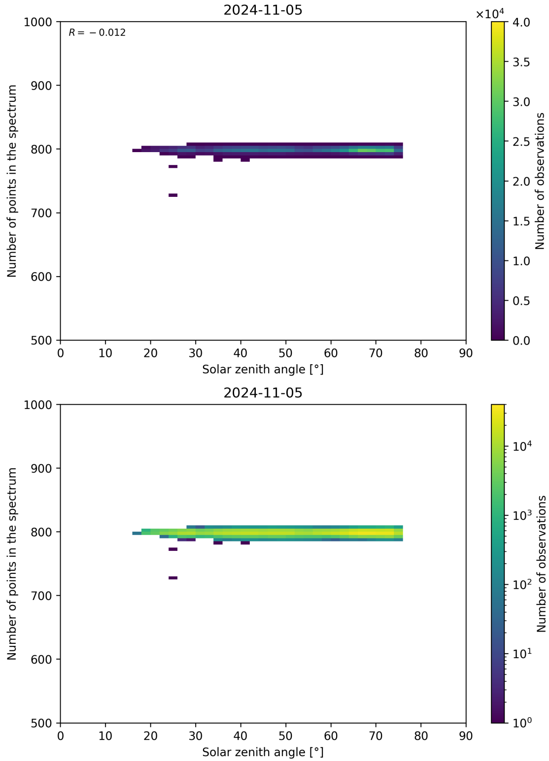
Figure 103: Scatter density plot of “Solar zenith angle” against “Number of points in the spectrum” for 2024-11-04 to 2024-11-06.
