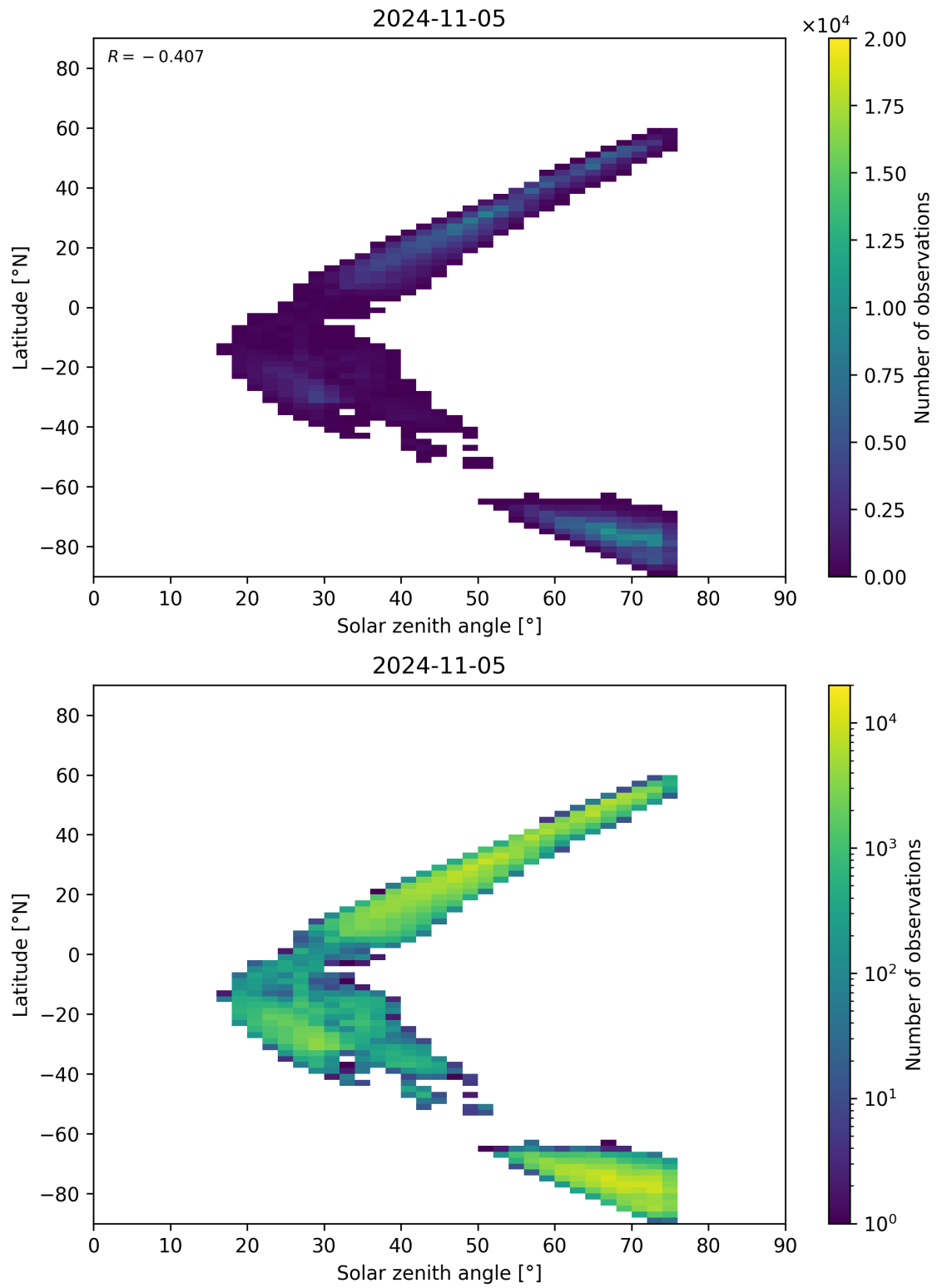
Figure 98: Scatter density plot of “Solar zenith angle” against “Latitude” for 2024-11-04 to 2024-11-06.
