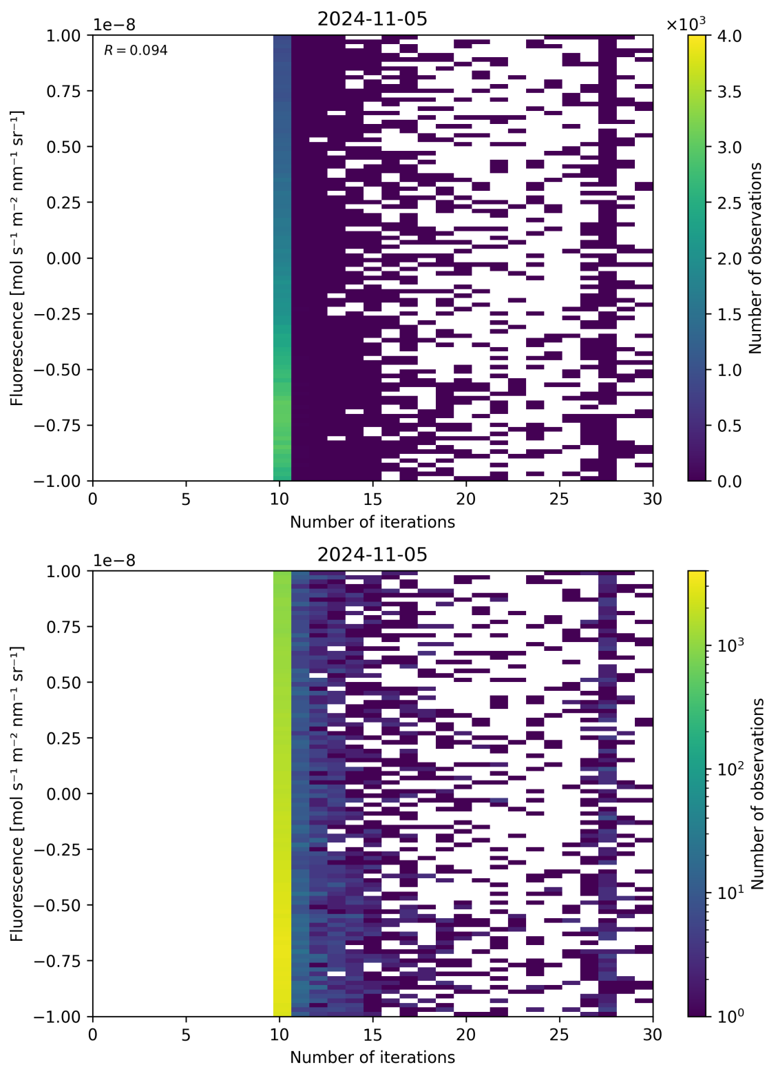
Figure 87: Scatter density plot of “Number of iterations” against “Fluorescence” for 2024-11-04 to 2024-11-06.
