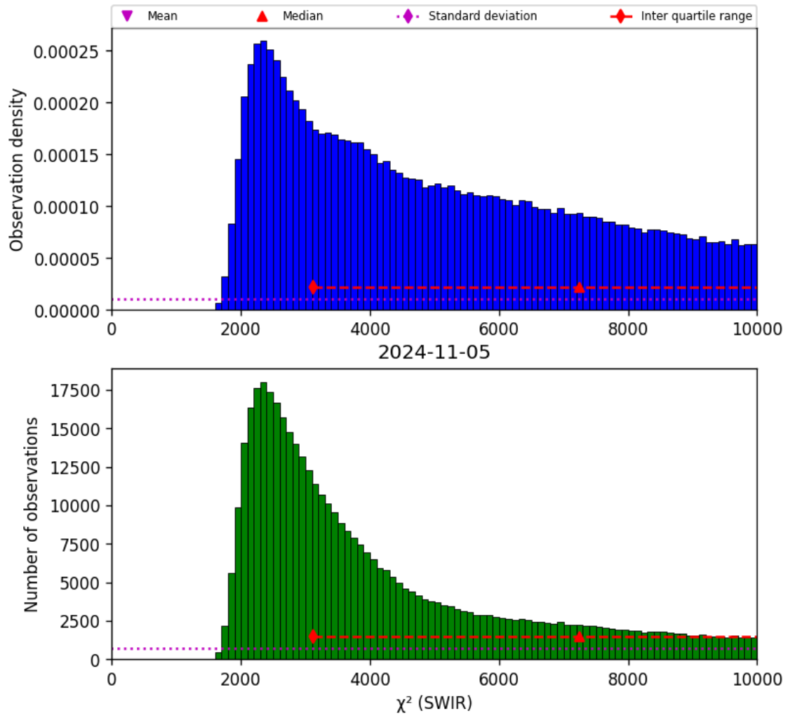
Figure 28: Histogram of “ \chi^2 (SWIR)” for 2024-11-04 to 2024-11-06
