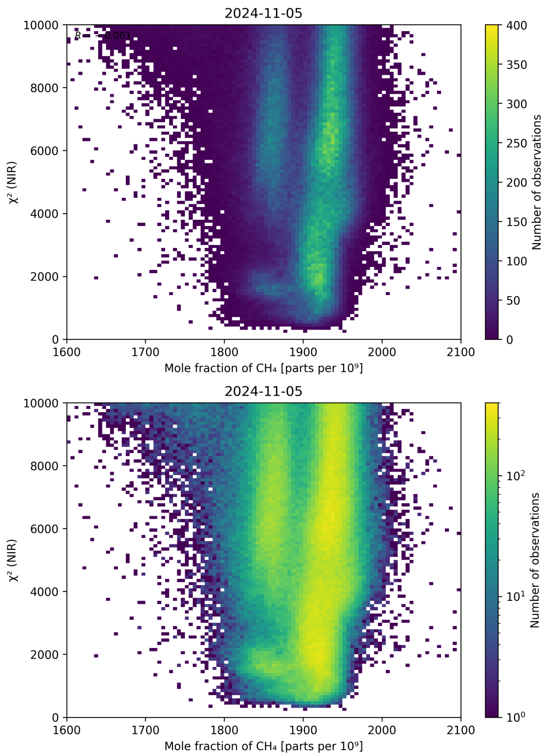
Figure 70: Scatter density plot of “Mole fraction of \text{CH}_4 ” against “ \chi^2 (NIR)” for 2024-11-04 to 2024-11-06.
