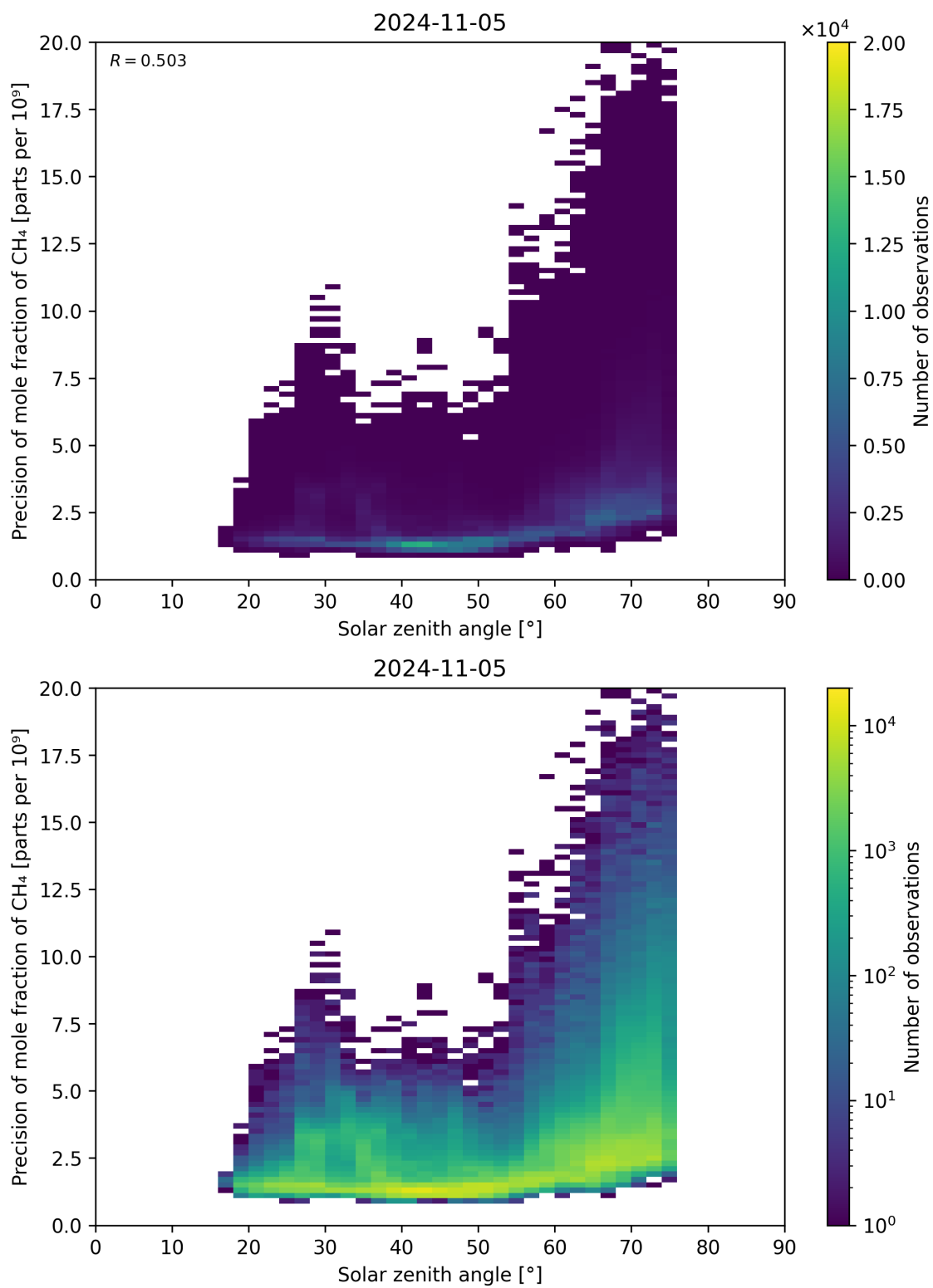
Figure 101: Scatter density plot of “Solar zenith angle” against “Precision of mole fraction of \text{CH}_4 ” for 2024-11-04 to 2024-11-06.
