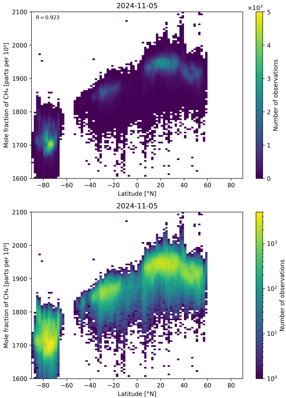
Figure 57: Scatter density plot of “Latitude” against “Mole fraction of CH 4 ” for 2024-11-04 to 2024-11-06.
