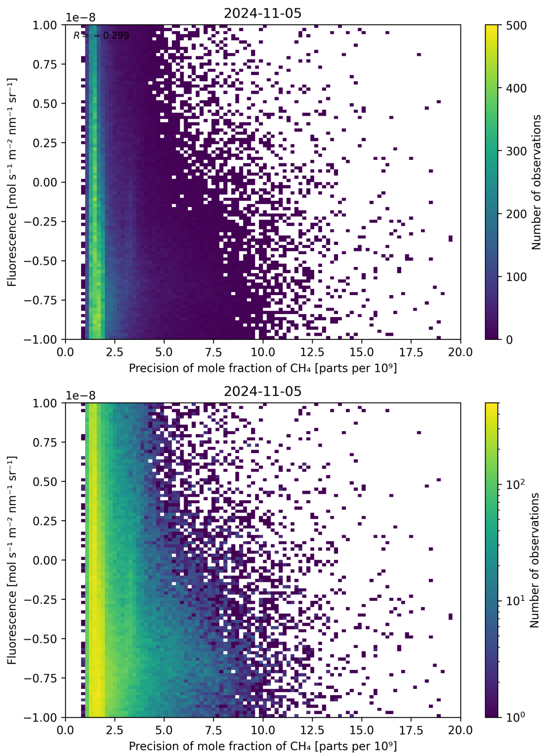
Figure 81: Scatter density plot of “Precision of mole fraction of \text{CH}_4 ” against “Fluorescence” for 2024-11-04 to 2024-11-06.
