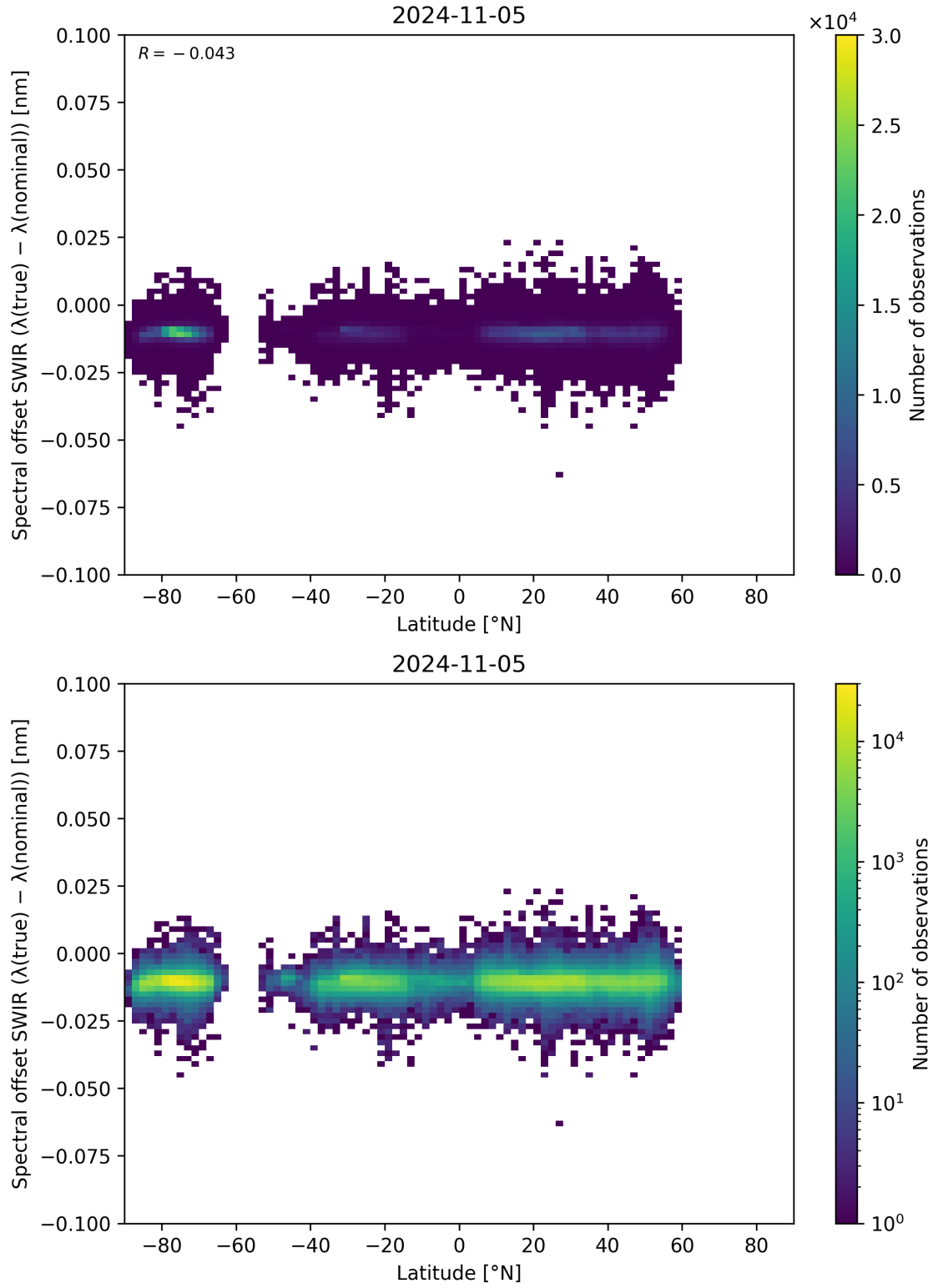
Figure 62: Scatter density plot of “Latitude” against “Spectral offset SWIR ( \lambda_{\text{true}} - \lambda_{\text{nominal}} )” for 2024-11-04 to 2024-11-06.
