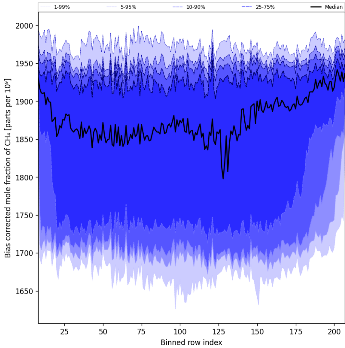
Figure 36: Along track statistics of “Bias corrected mole fraction of CH 4 ” for 2024-11-04 to 2024-11-06
