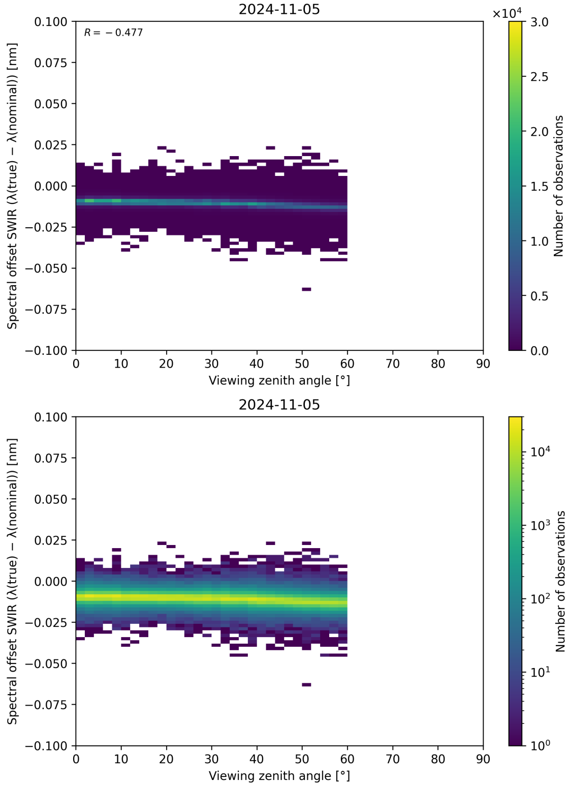
Figure 116: Scatter density plot of “Viewing zenith angle” against “Spectral offset SWIR ( \lambda_{\text{true}} - \lambda_{\text{nominal}} )” for 2024-11-04 to 2024-11-06.
