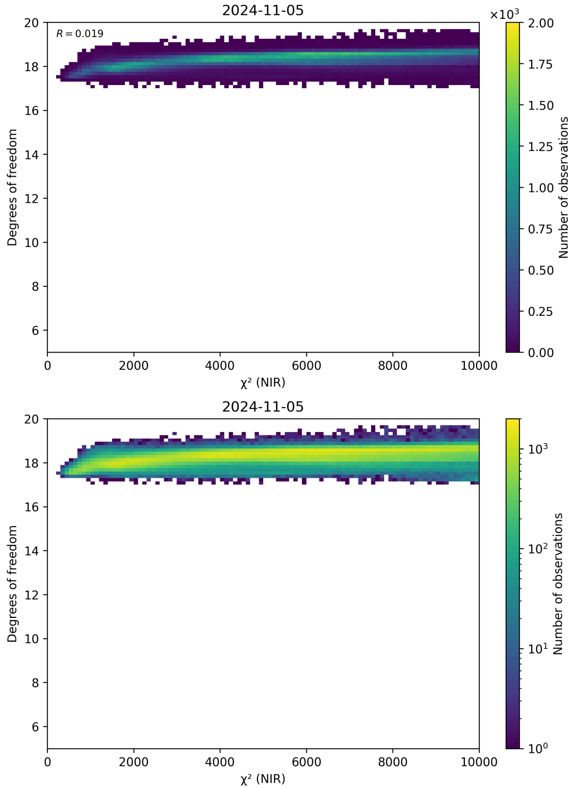
Figure 44: Scatter density plot of “ \chi^2 (NIR)” against “Degrees of freedom” for 2024-11-04 to 2024-11-06.
