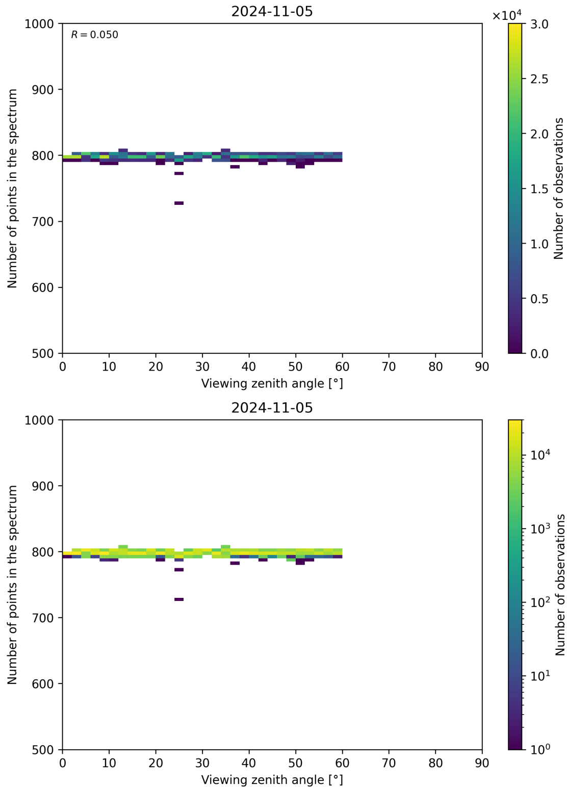
Figure 114: Scatter density plot of “Viewing zenith angle” against “Number of points in the spectrum” for 2024-11-04 to 2024-11-06.
