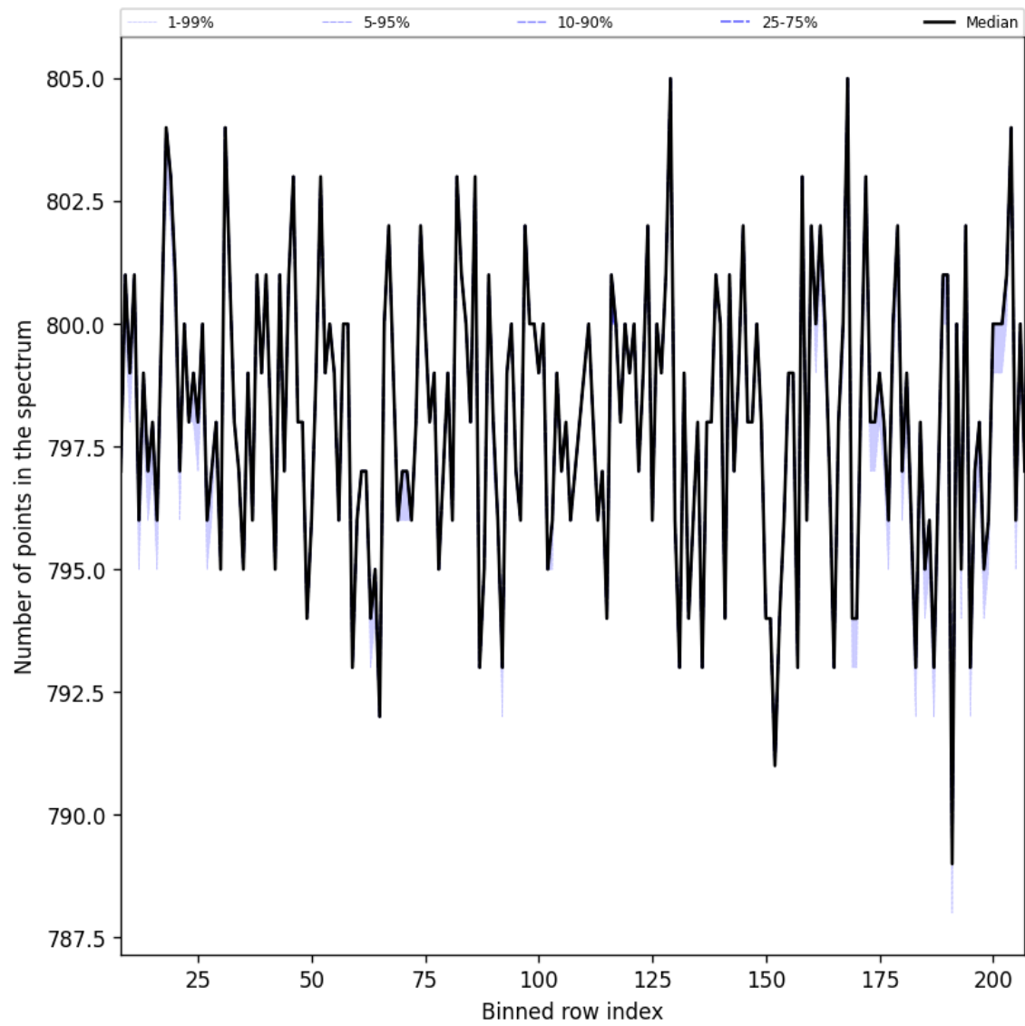
Figure 37: Along track statistics of “Number of points in the spectrum” for 2024-11-04 to 2024-11-06
