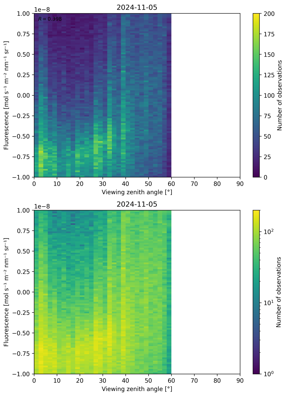
Figure 108: Scatter density plot of “Viewing zenith angle” against “Fluorescence” for 2024-11-04 to 2024-11-06.
