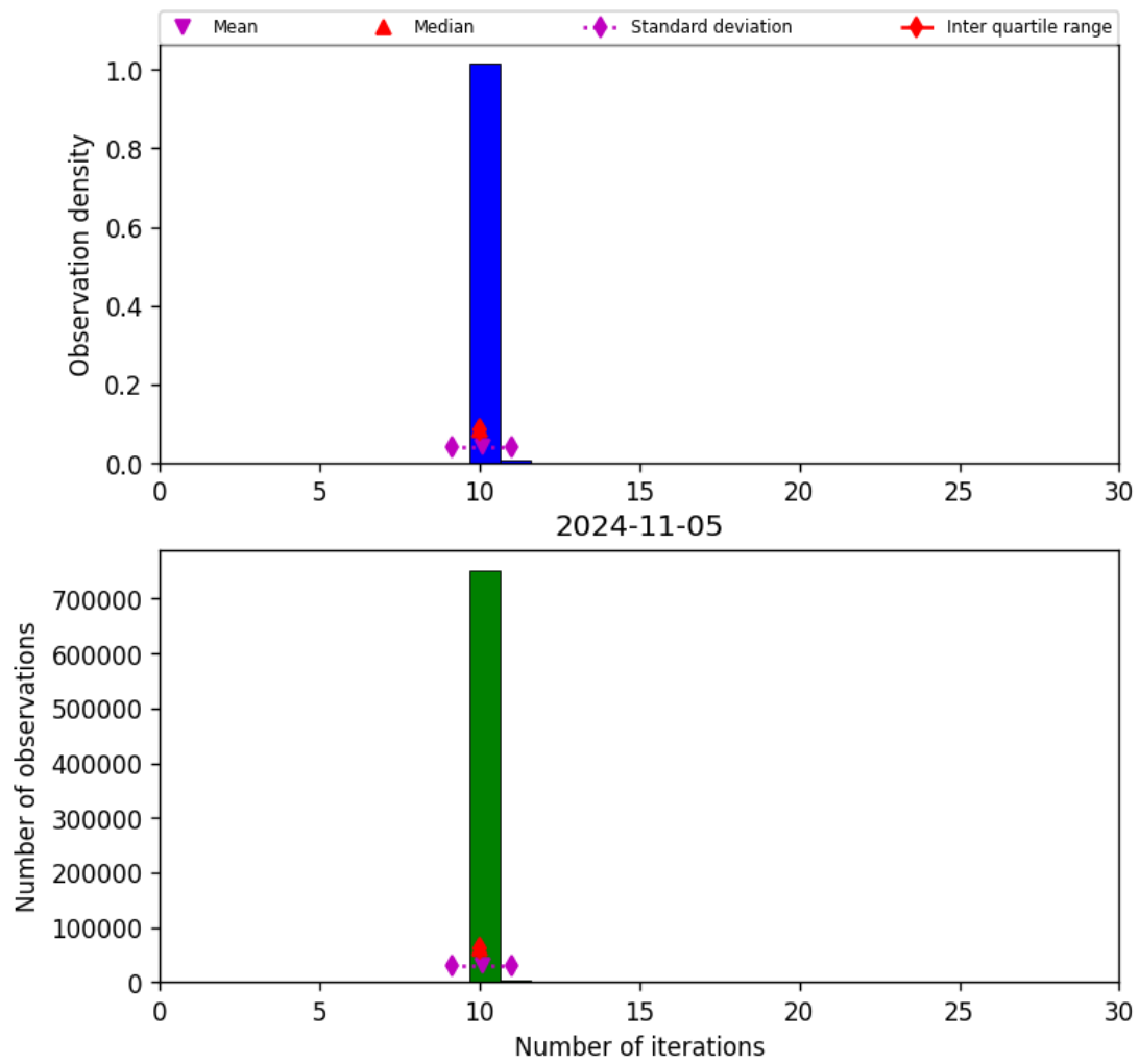
Figure 31: Histogram of “Number of iterations” for 2024-11-04 to 2024-11-06
