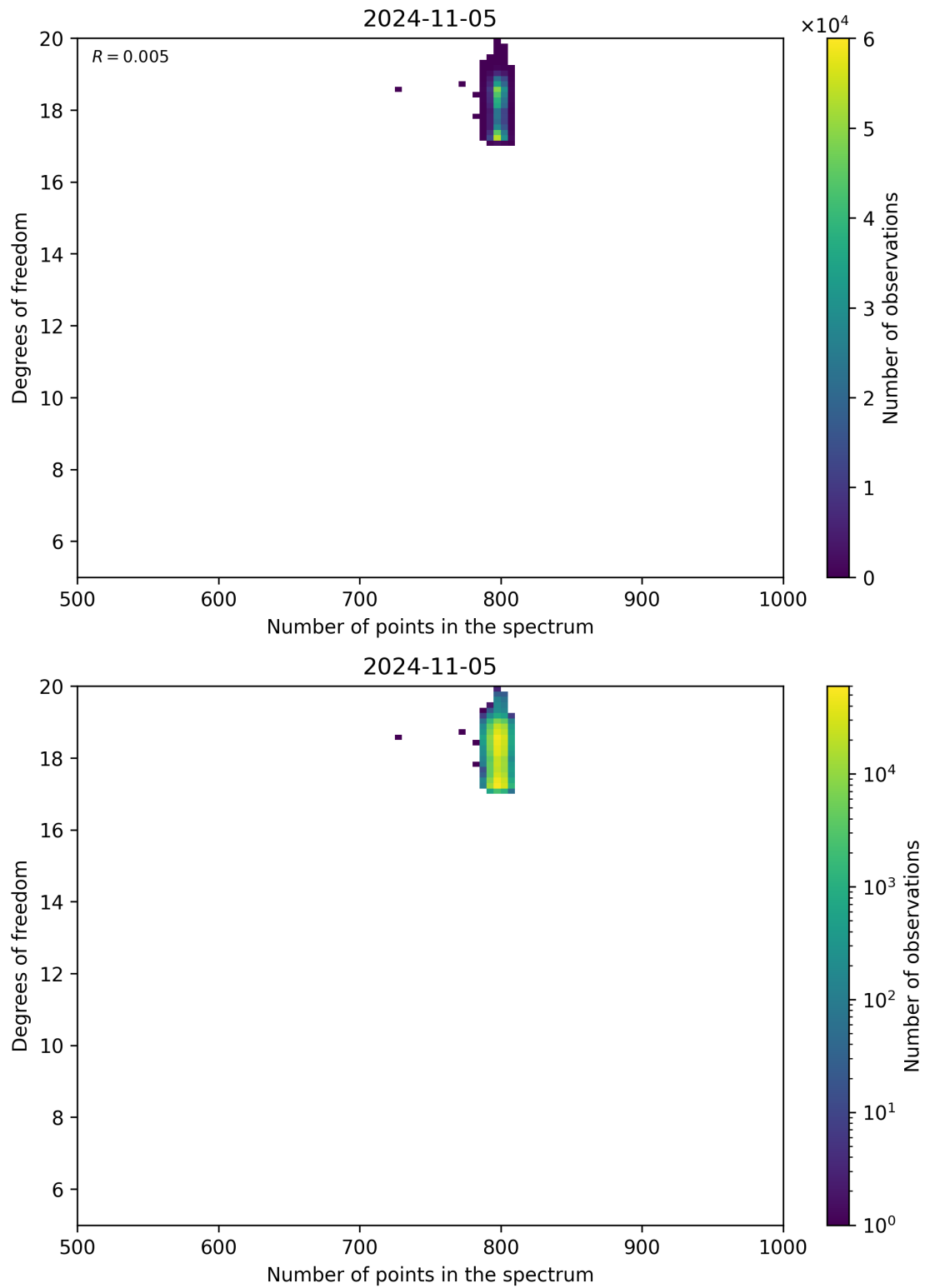
Figure 90: Scatter density plot of “Number of points in the spectrum” against “Degrees of freedom” for 2024-11-04 to 2024-11-06.
