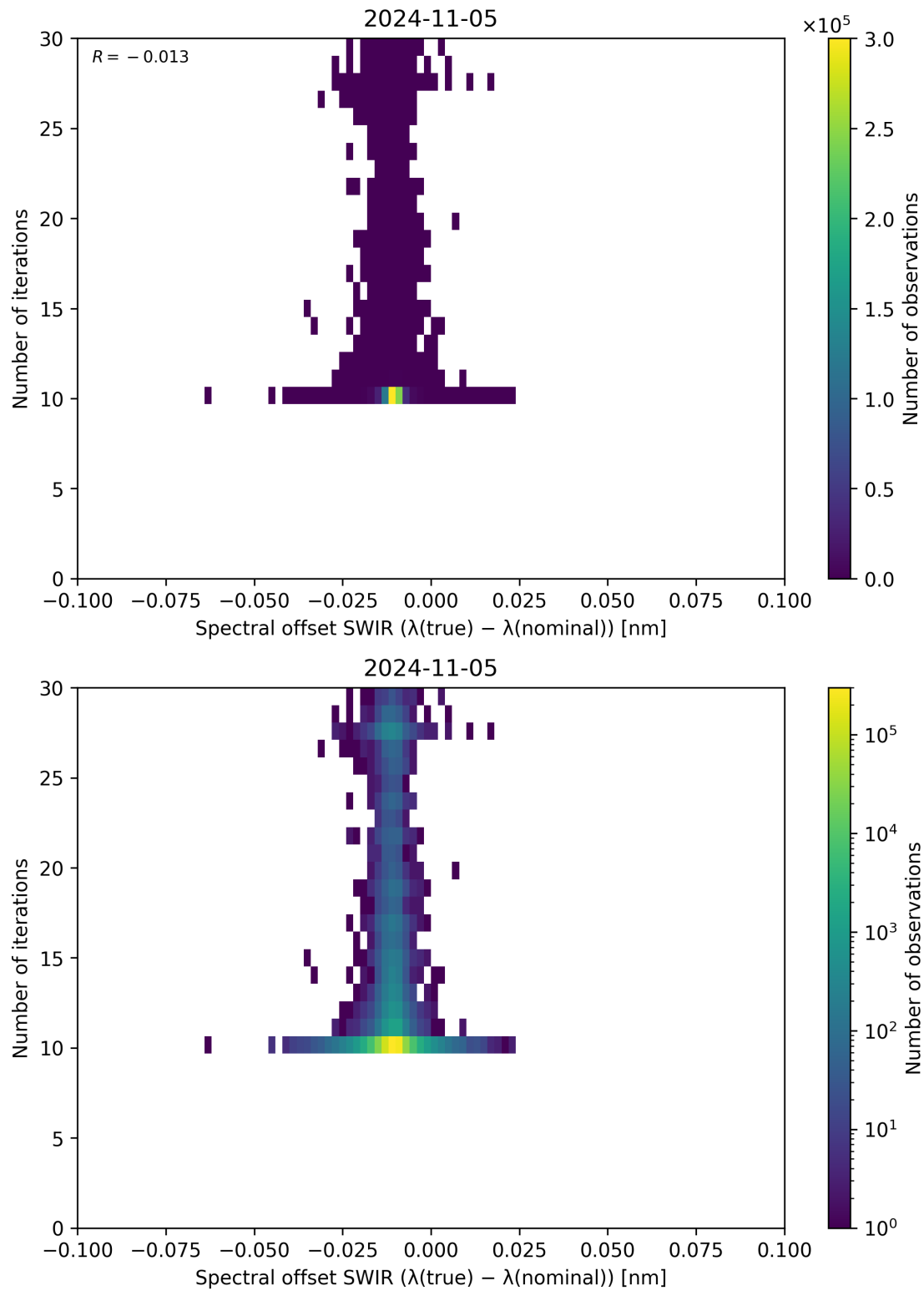
Figure 121: Scatter density plot of “Spectral offset SWIR ( \lambda_{\text{true}} - \lambda_{\text{nominal}} )” against “Number of iterations” for 2024-11-04 to 2024-11-06.
