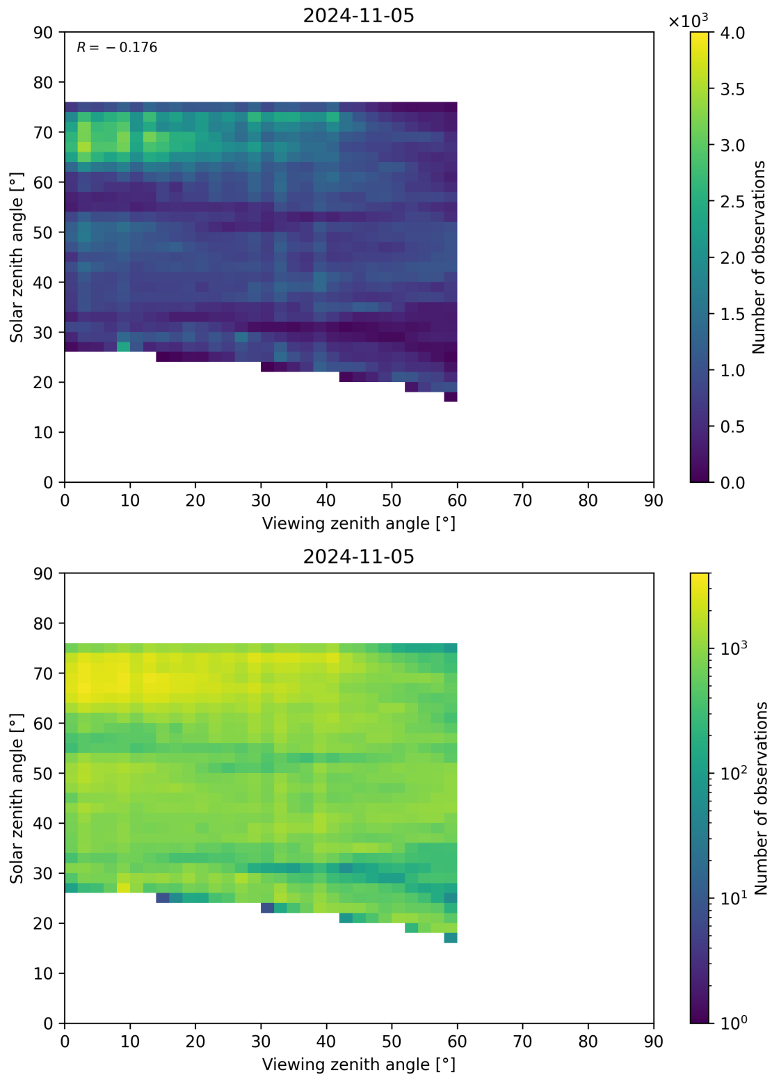
Figure 115: Scatter density plot of “Viewing zenith angle” against “Solar zenith angle” for 2024-11-04 to 2024-11-06.
