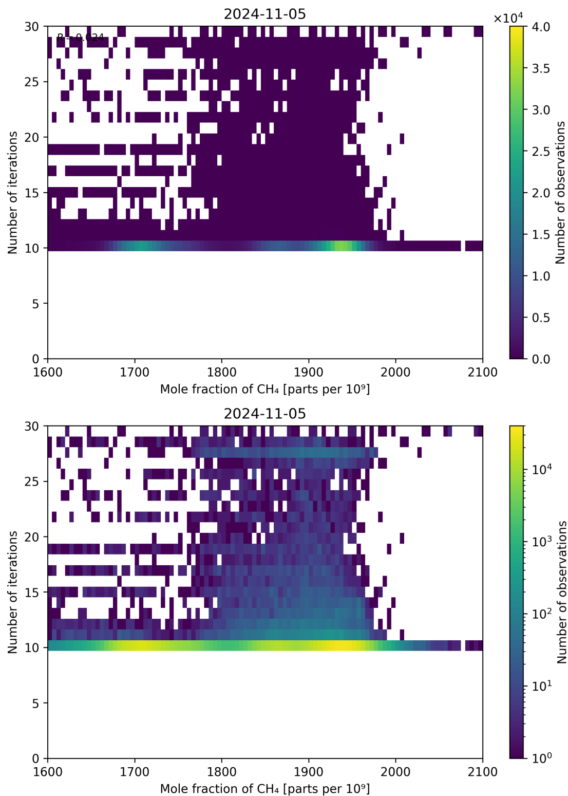
Figure 76: Scatter density plot of “Mole fraction of CH 4 ” against “Number of iterations” for 2024-11-04 to 2024-11-06.
