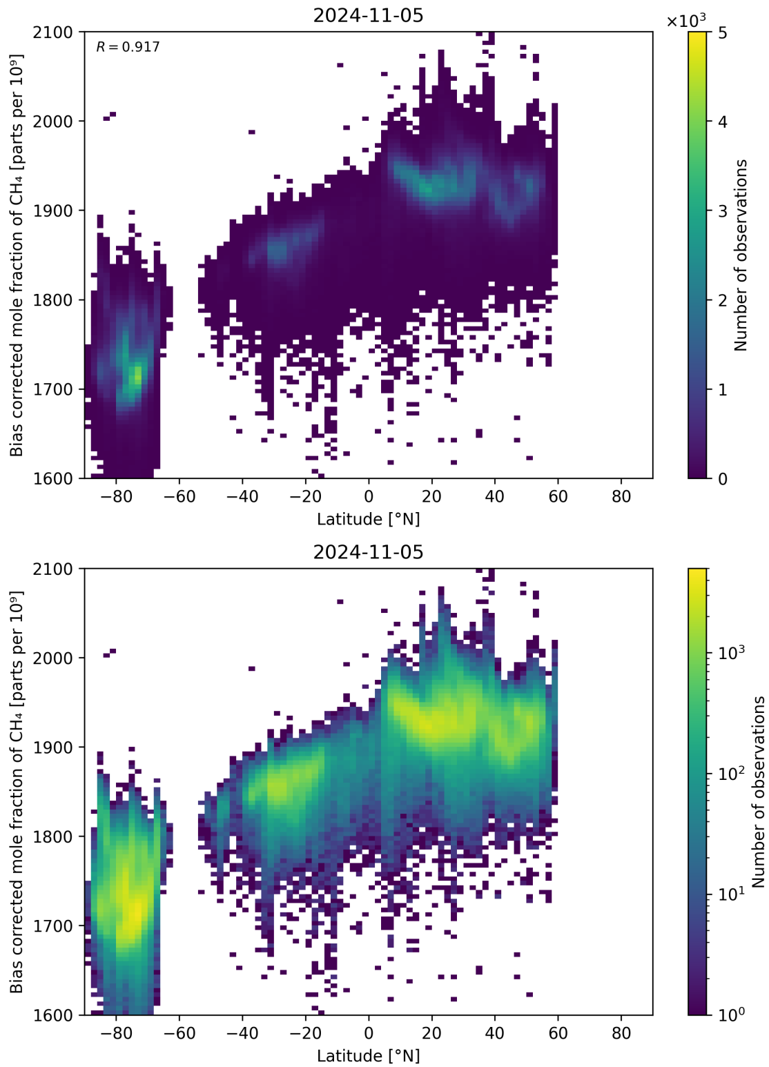
Figure 58: Scatter density plot of “Latitude” against “Bias corrected mole fraction of \text{CH}_4 ” for 2024-11-04 to 2024-11-06.
