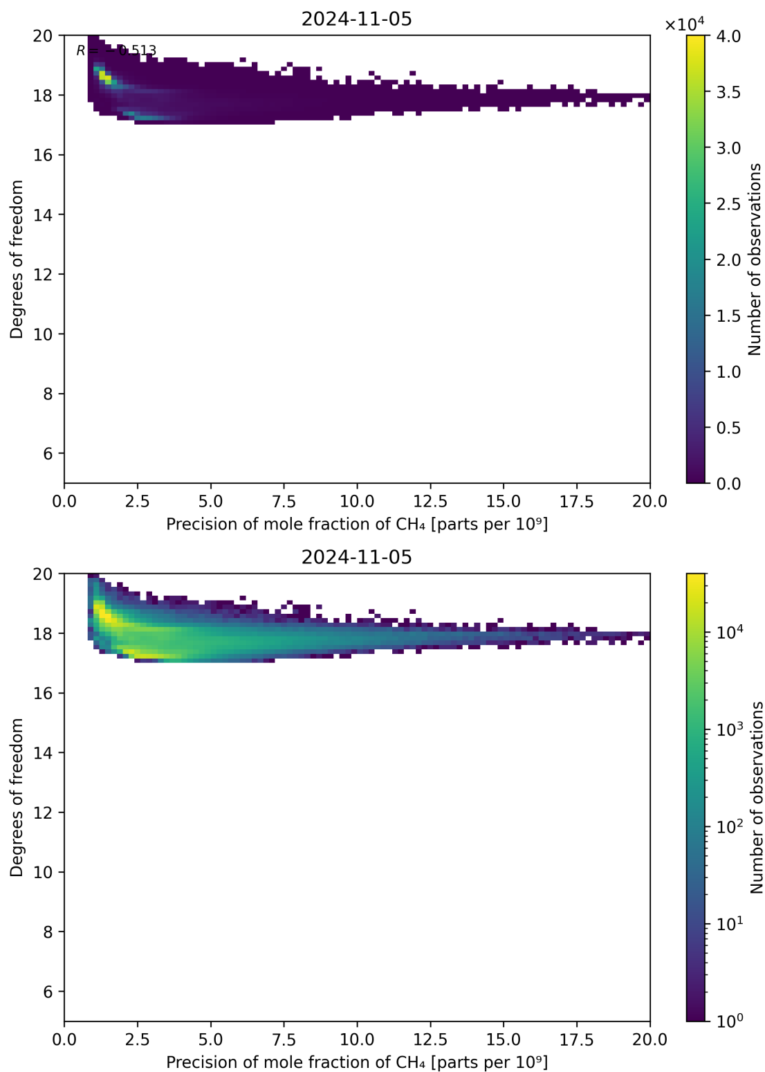
Figure 80: Scatter density plot of “Precision of mole fraction of CH 4 ” against “Degrees of freedom” for 2024-11-04 to 2024-11-06.
