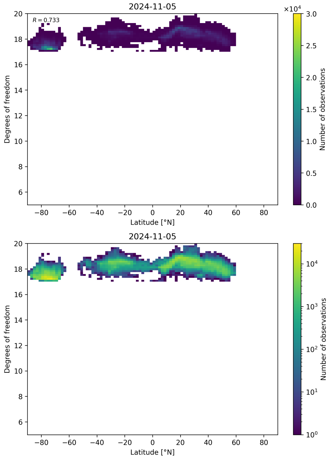
Figure 55: Scatter density plot of “Latitude” against “Degrees of freedom” for 2024-11-04 to 2024-11-06.
