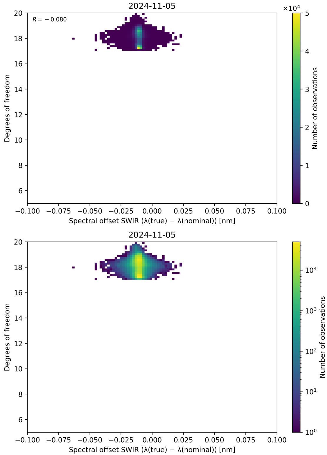
Figure 119: Scatter density plot of “Spectral offset SWIR ( \lambda_{\text{true}} - \lambda_{\text{nominal}} )” against “Degrees of freedom” for 2024-11-04 to 2024-11-06.
