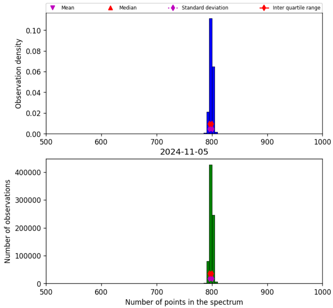
Figure 26: Histogram of “Number of points in the spectrum” for 2024-11-04 to 2024-11-06
