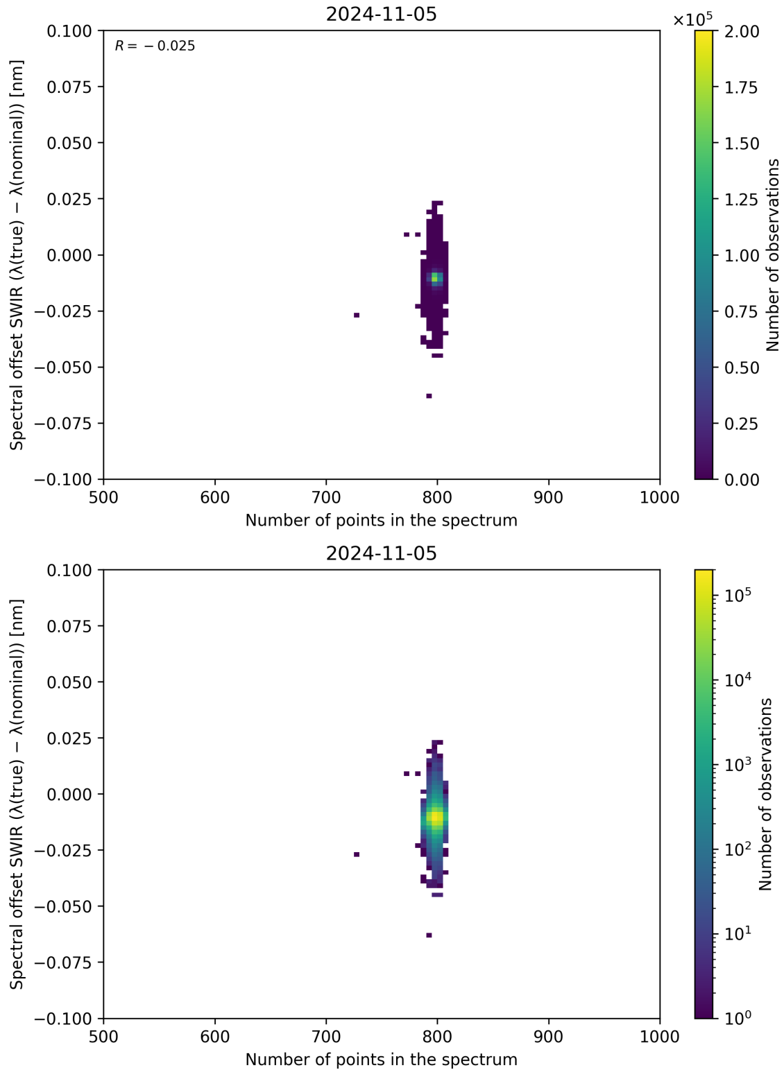
Figure 93: Scatter density plot of “Number of points in the spectrum” against “Spectral offset SWIR ( \lambda_{\text{true}} - \lambda_{\text{nominal}} )” for 2024-11-04 to 2024-11-06.
