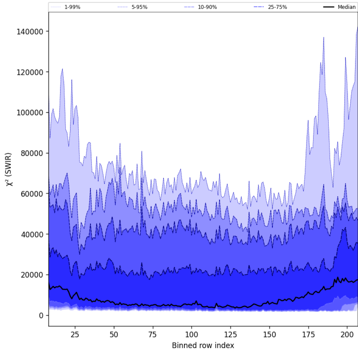
Figure 39: Along track statistics of “ \chi^2 (SWIR)” for 2024-11-04 to 2024-11-06
