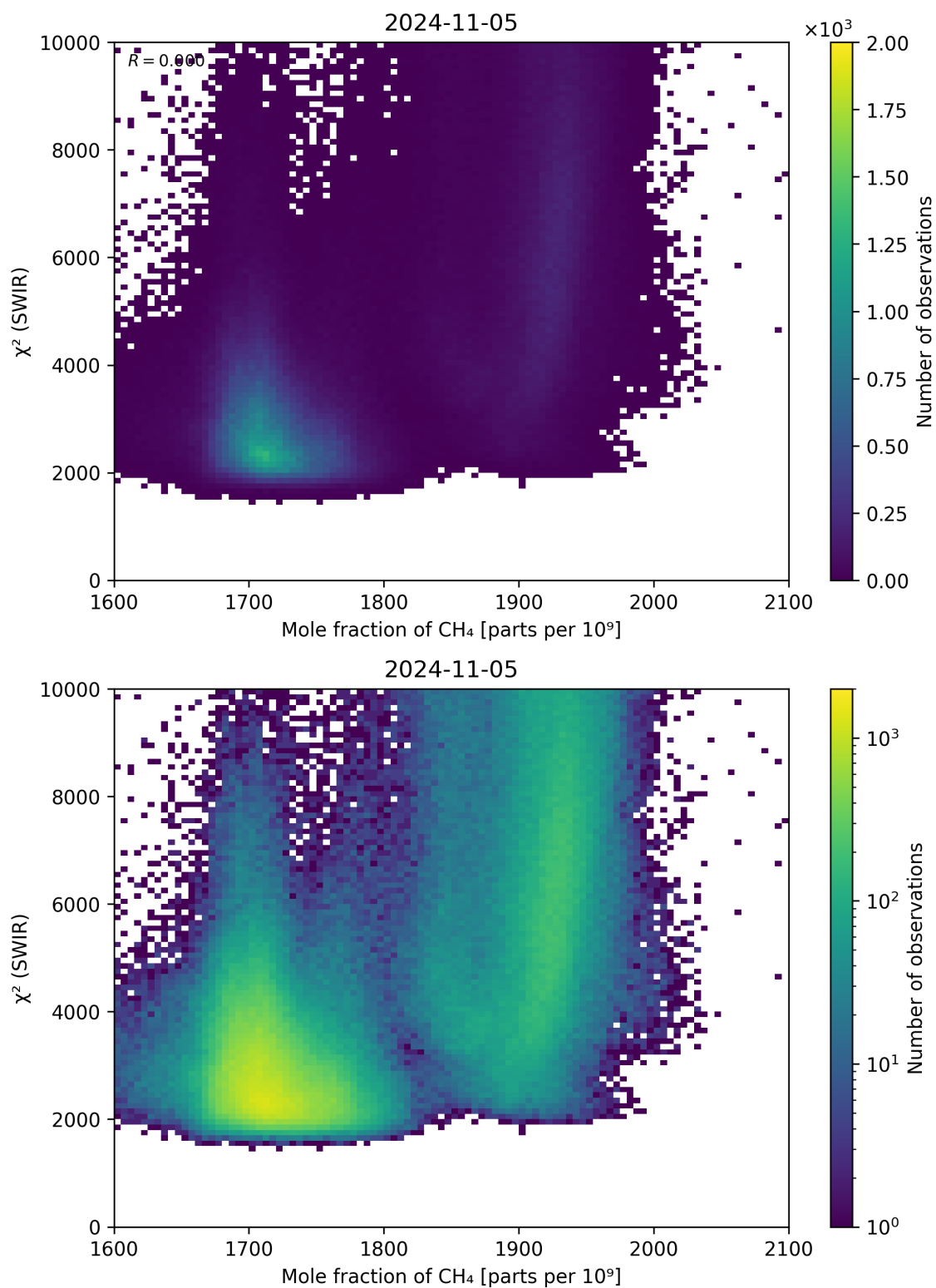
Figure 71: Scatter density plot of “Mole fraction of \text{CH}_4 ” against “ \chi^2 (SWIR)” for 2024-11-04 to 2024-11-06.
