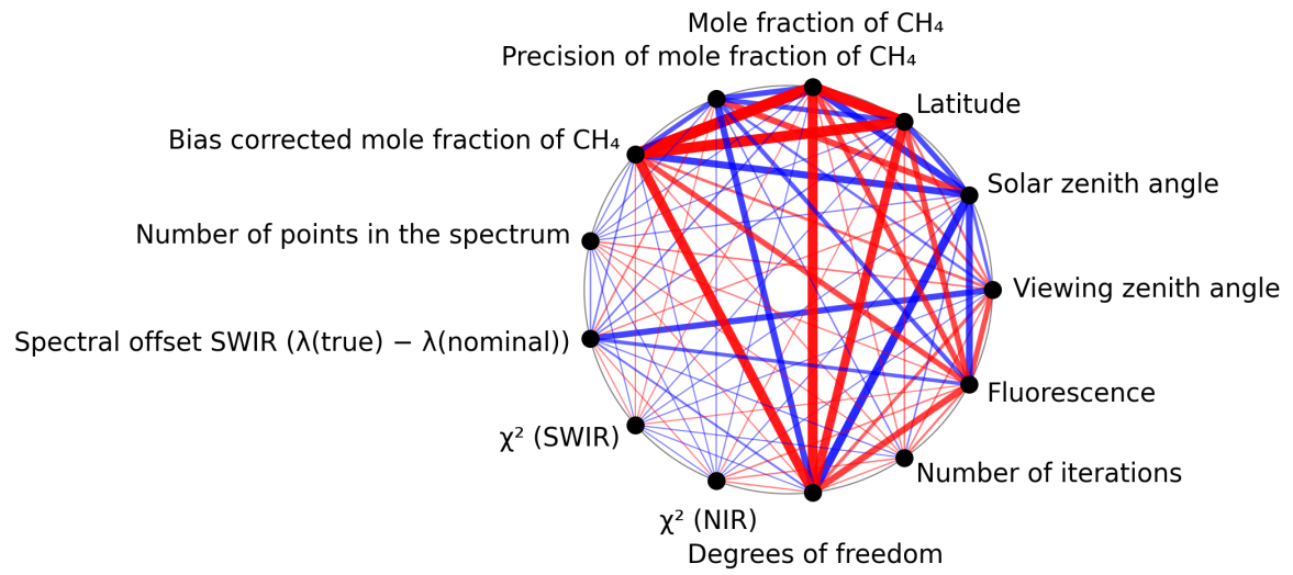
Figure 1: Map of correlation graph for 2024-11-04 to 2024-11-06.
