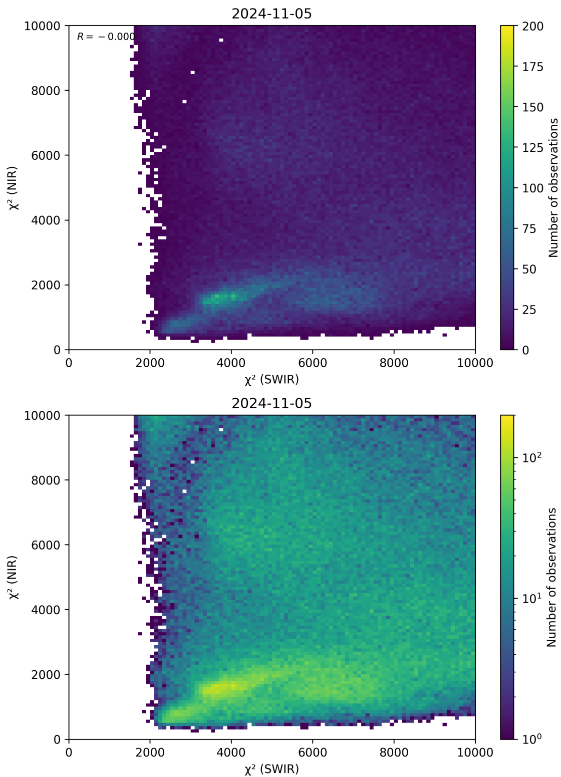
Figure 47: Scatter density plot of “ \chi^2 (SWIR)” against “ \chi^2 (NIR)” for 2024-11-04 to 2024-11-06.
