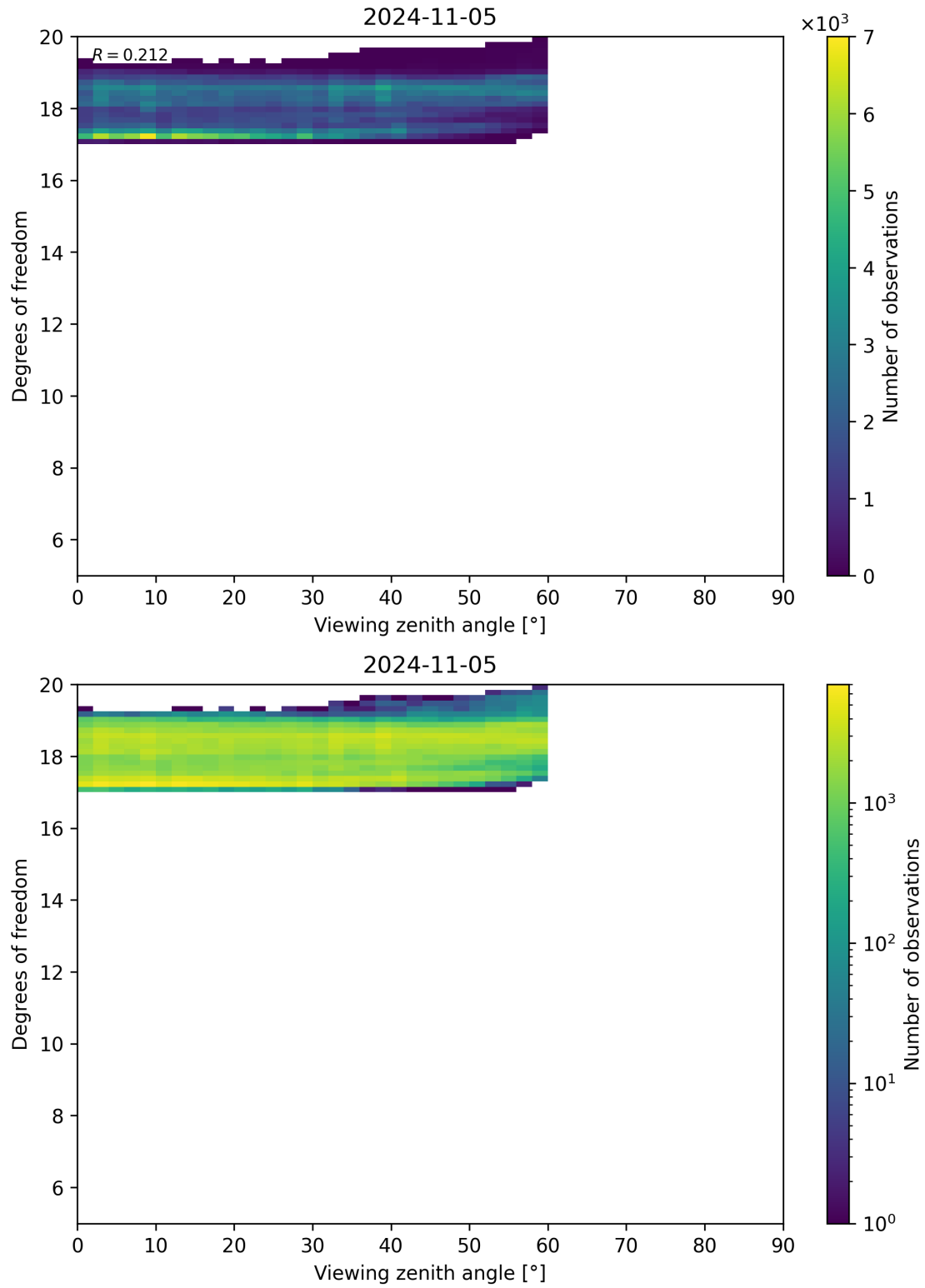
Figure 107: Scatter density plot of “Viewing zenith angle” against “Degrees of freedom” for 2024-11-04 to 2024-11-06.
