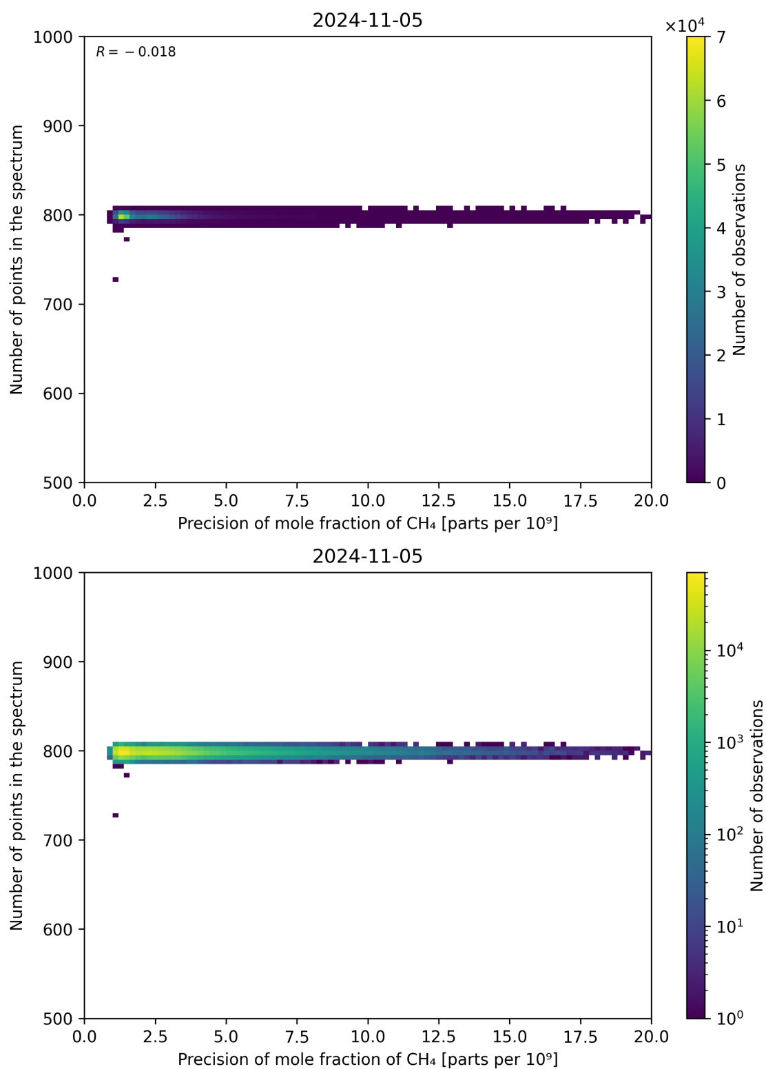
Figure 84: Scatter density plot of “Precision of mole fraction of CH 4 ” against “Number of points in the spectrum” for 2024-11-04 to 2024-11-06.
