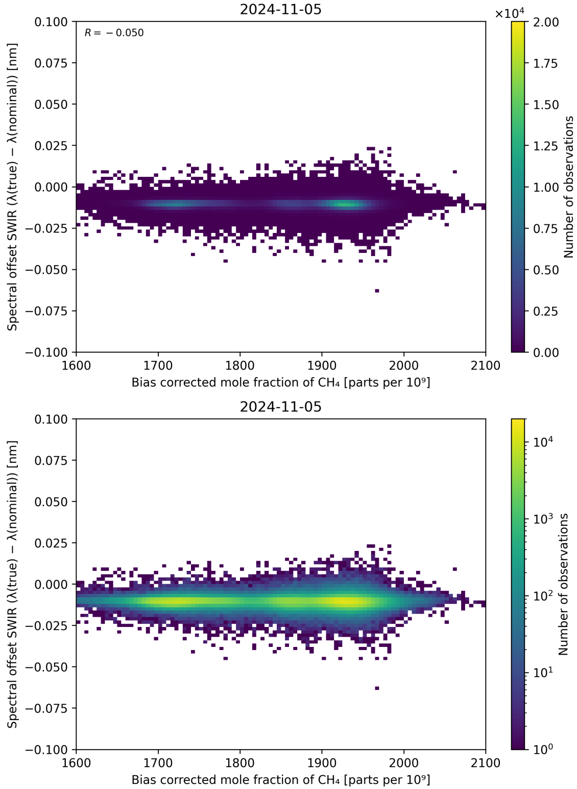
Figure 69: Scatter density plot of “Bias corrected mole fraction of \text{CH}_4 ” against “Spectral offset SWIR ( \lambda_{\text{true}} - \lambda_{\text{nominal}} )” for 2024-11-04 to 2024-11-06.
