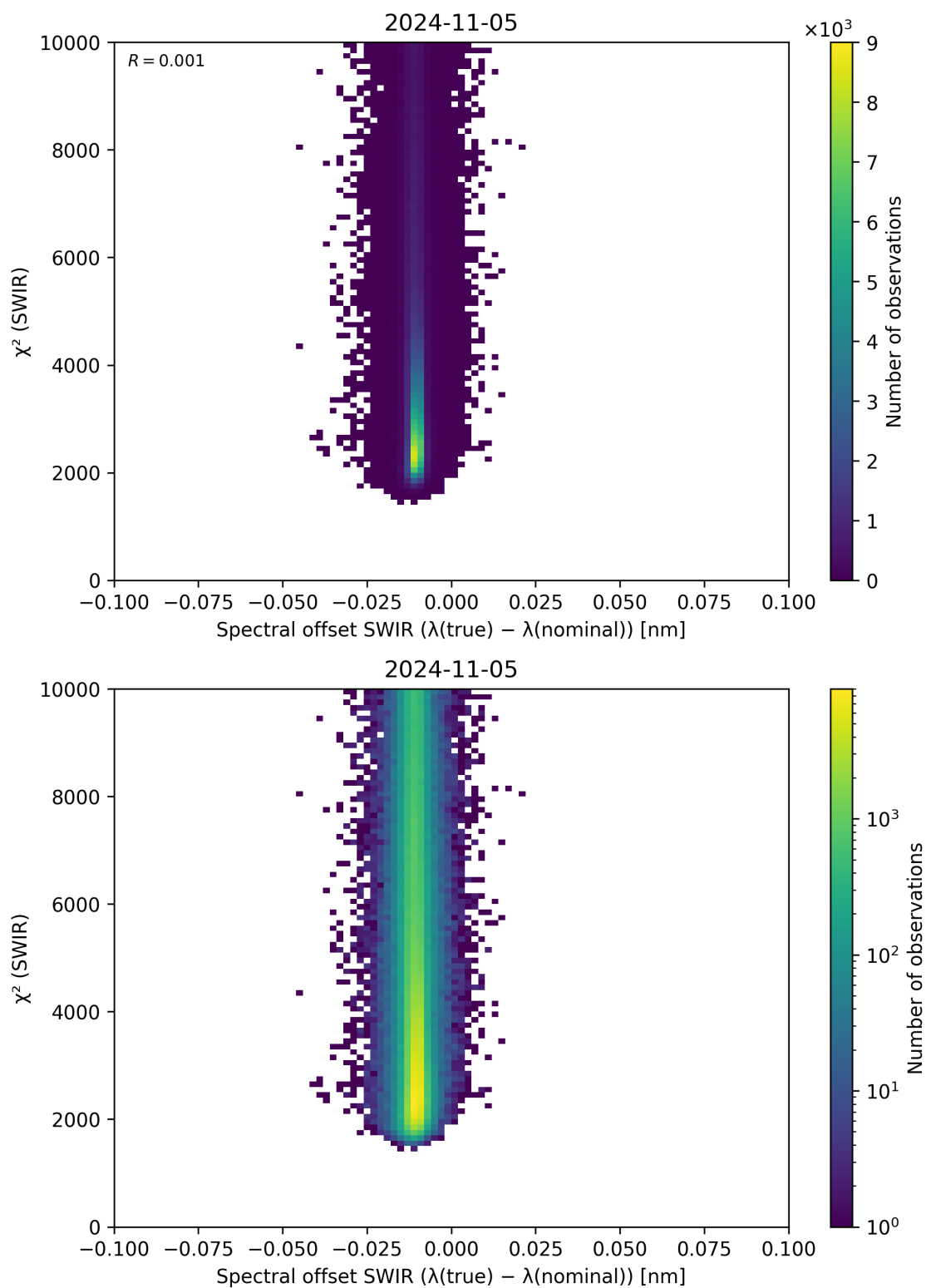
Figure 118: Scatter density plot of “Spectral offset SWIR ( \lambda_{\text{true}} - \lambda_{\text{nominal}} )” against “ \chi^2 (SWIR)” for 2024-11-04 to 2024-11-06.
