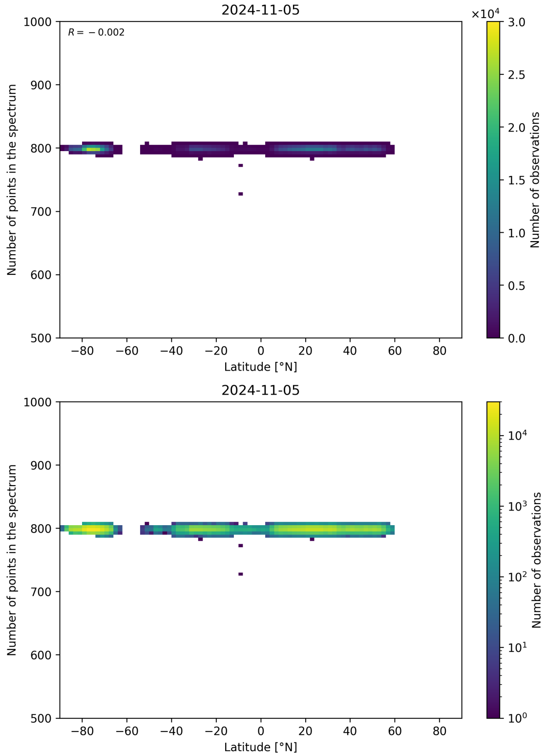
Figure 61: Scatter density plot of “Latitude” against “Number of points in the spectrum” for 2024-11-04 to 2024-11-06.
