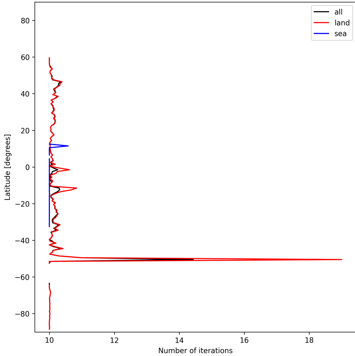
Figure 20: Zonal average of “Number of iterations” for 2024-11-04 to 2024-11-06.
