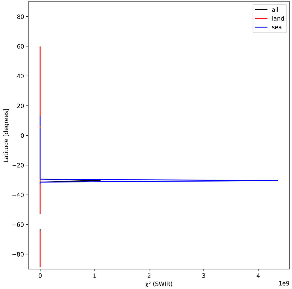
Figure 17: Zonal average of “ \chi^2 (SWIR)” for 2024-11-04 to 2024-11-06.
