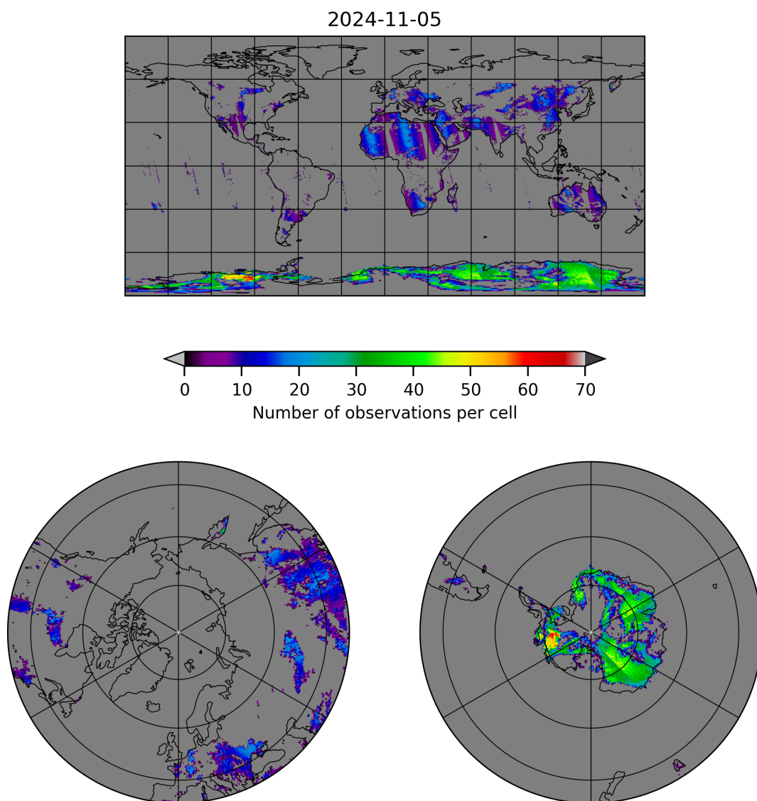
Figure 10: Map of the number of observations for 2024-11-04 to 2024-11-06
