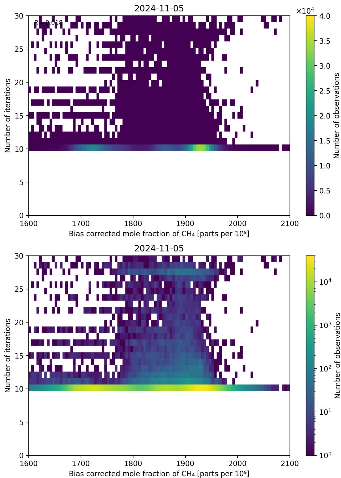
Figure 67: Scatter density plot of “Bias corrected mole fraction of \text{CH}_4 ” against “Number of iterations” for 2024-11-04 to 2024-11-06.
