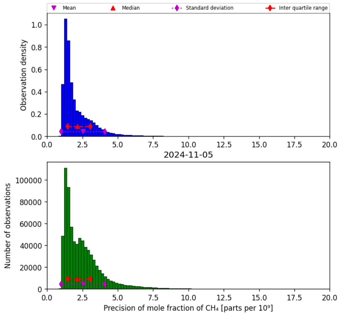
Figure 24: Histogram of “Precision of mole fraction of CH 4 ” for 2024-11-04 to 2024-11-06
