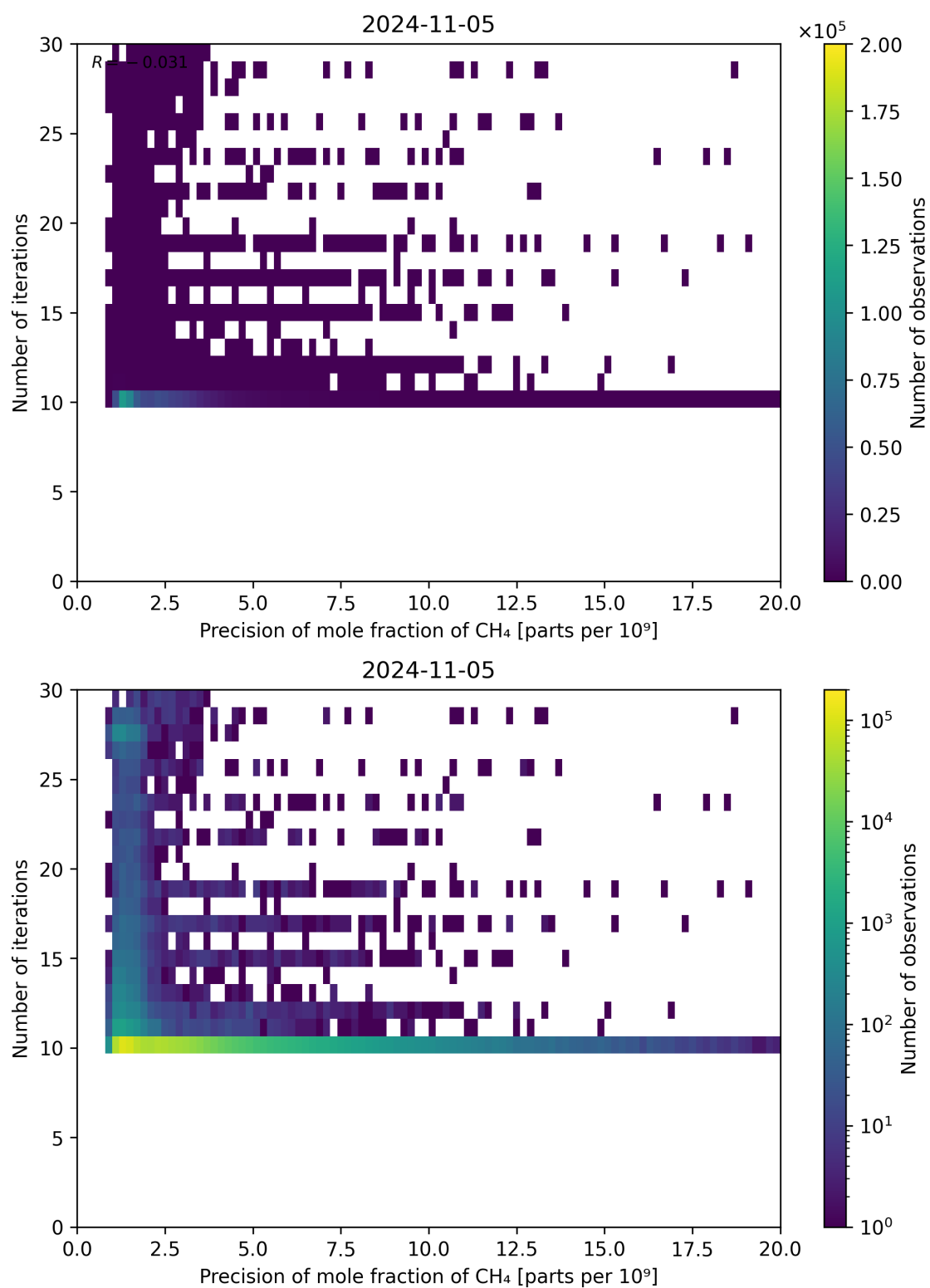
Figure 83: Scatter density plot of “Precision of mole fraction of CH 4 ” against “Number of iterations” for 2024-11-04 to 2024-11-06.
