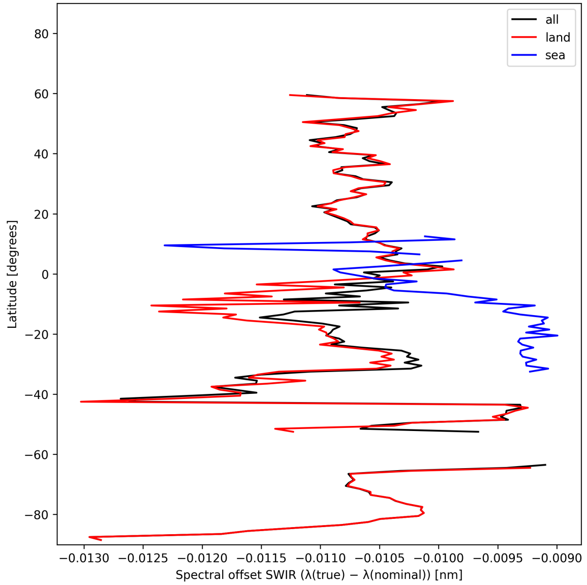
Figure 16: Zonal average of “Spectral offset SWIR ( \lambda_{\text{true}} - \lambda_{\text{nominal}} )” for 2024-11-04 to 2024-11-06.
