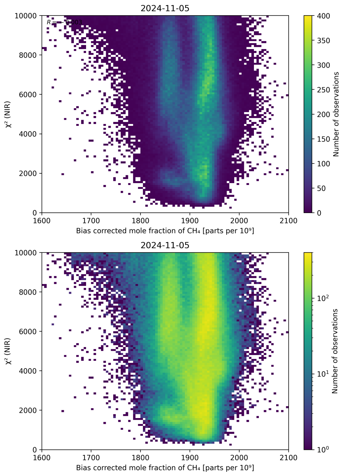
Figure 63: Scatter density plot of “Bias corrected mole fraction of CH 4 ” against “ \chi^2 (NIR)” for 2024-11-04 to 2024-11-06.
