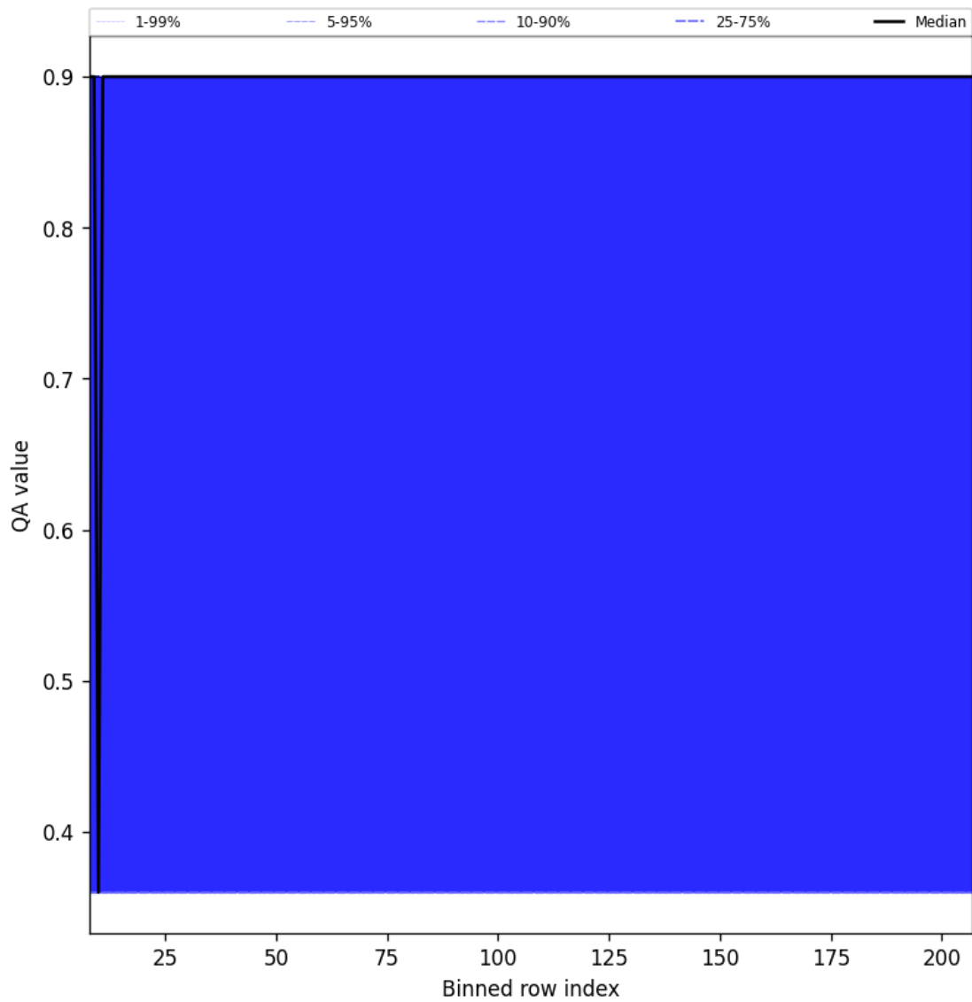
Figure 33: Along track statistics of "QA value" for 2024-11-04 to 2024-11-06
