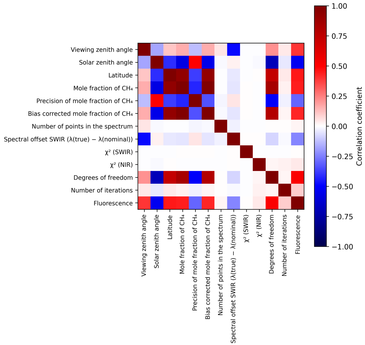
Figure 2: Map of correlation matrix for 2024-11-04 to 2024-11-06.
