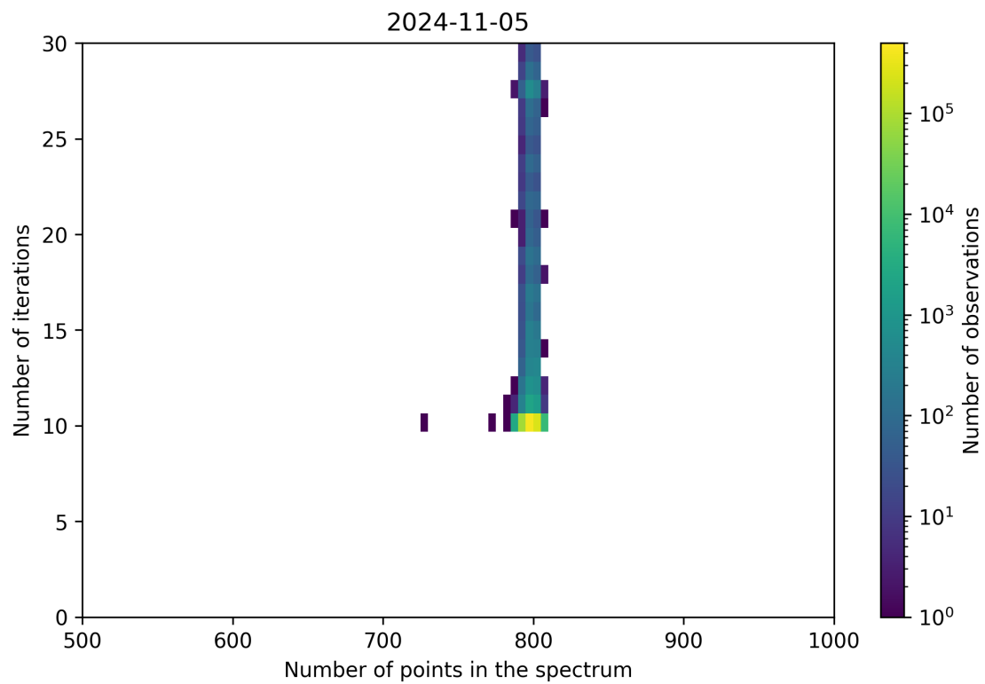
Figure 92: Scatter density plot of “Number of points in the spectrum” against “Number of iterations” for 2024-11-04 to 2024-11-06.
