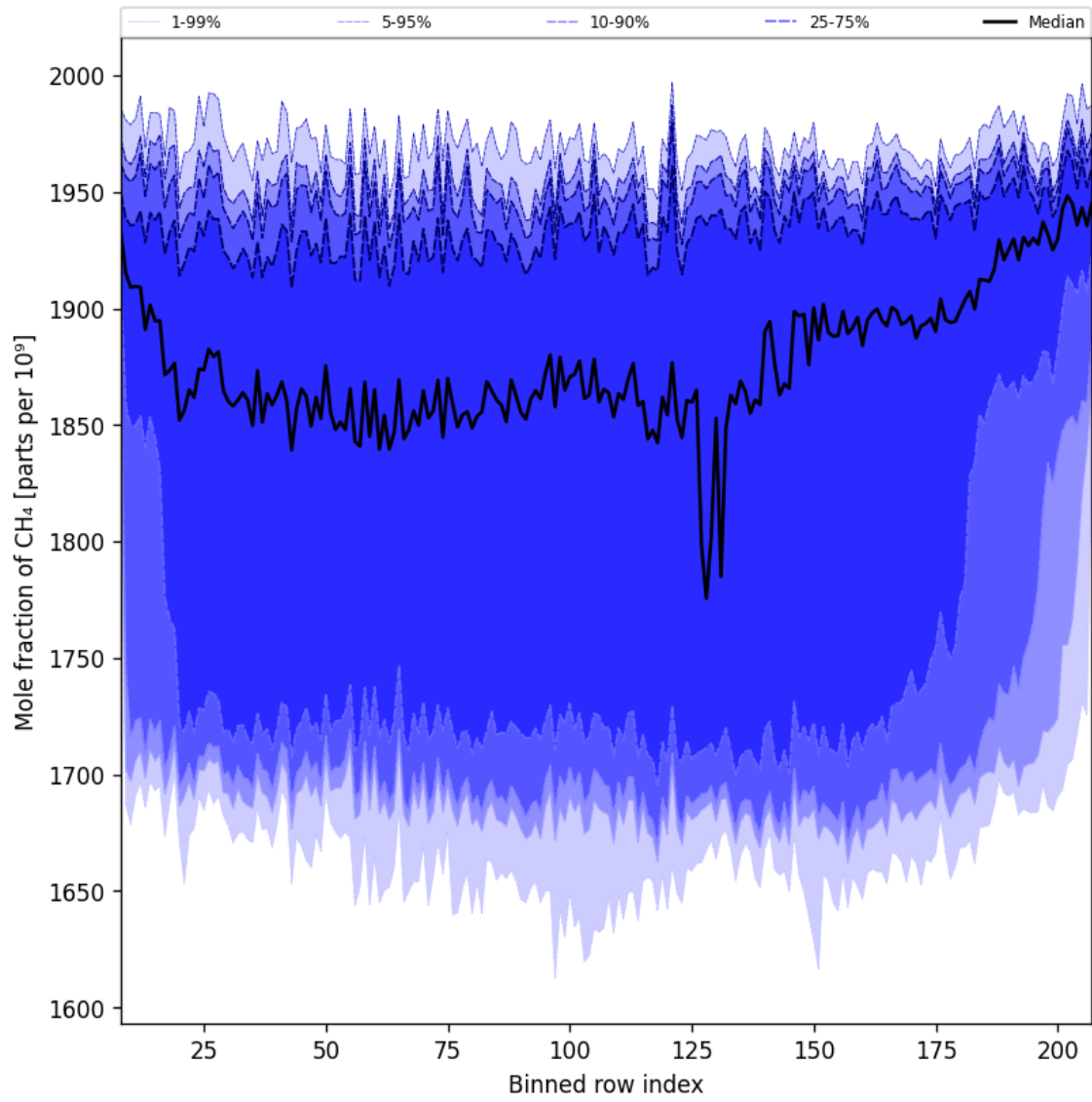
Figure 34: Along track statistics of “Mole fraction of CH 4 ” for 2024-11-04 to 2024-11-06
