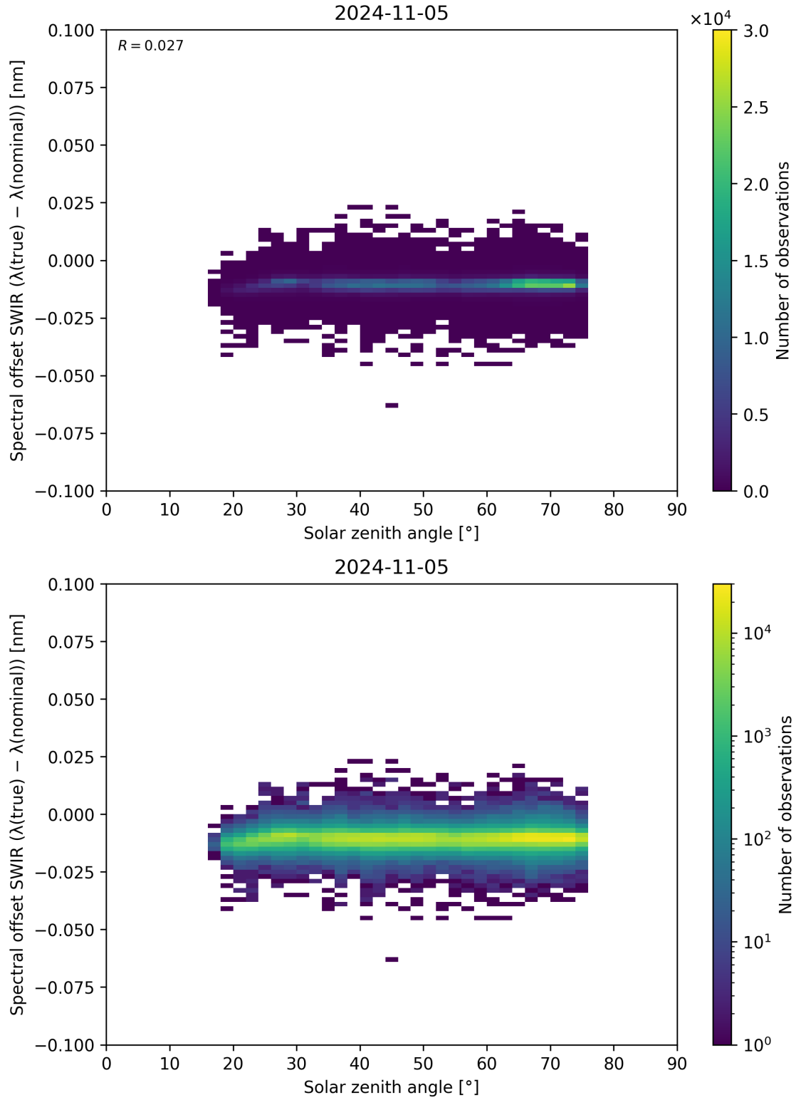
Figure 104: Scatter density plot of “Solar zenith angle” against “Spectral offset SWIR ( \lambda_{\text{true}} - \lambda_{\text{nominal}} )” for 2024-11-04 to 2024-11-06.
