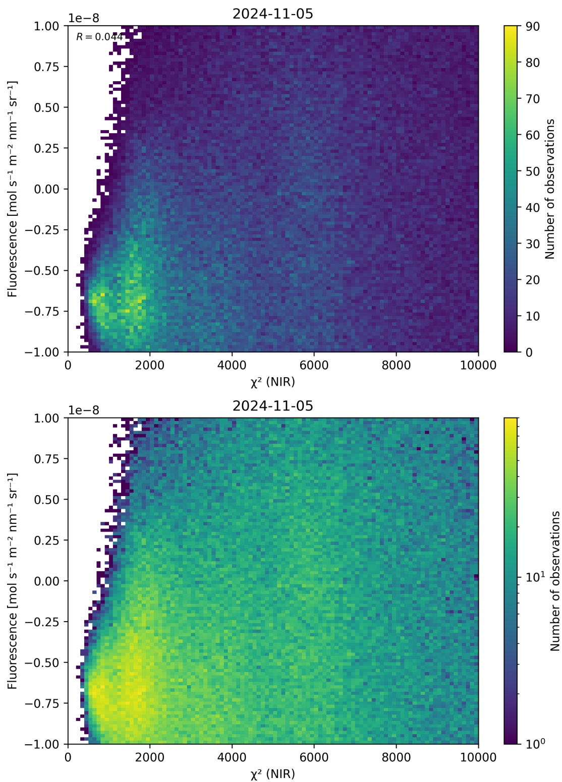
Figure 45: Scatter density plot of “ \chi^2 (NIR)” against “Fluorescence” for 2024-11-04 to 2024-11-06.
