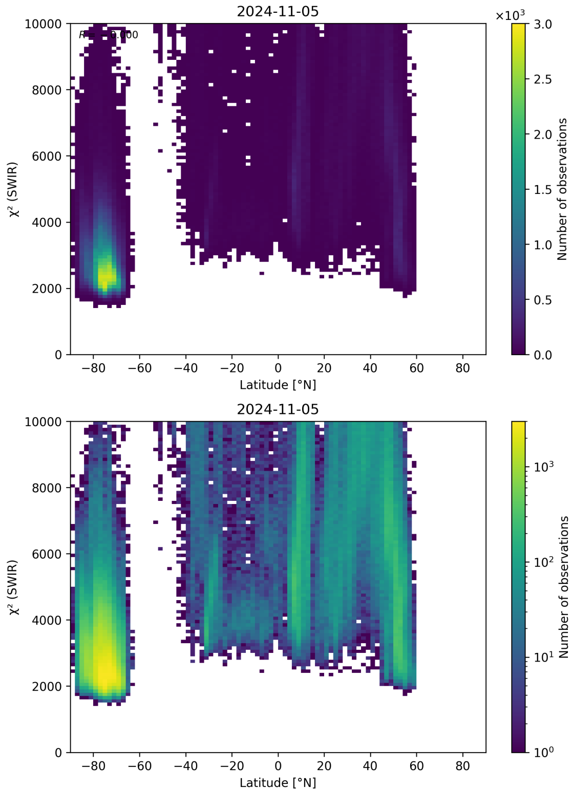
Figure 54: Scatter density plot of “Latitude” against “ \chi^2 (SWIR)” for 2024-11-04 to 2024-11-06.
