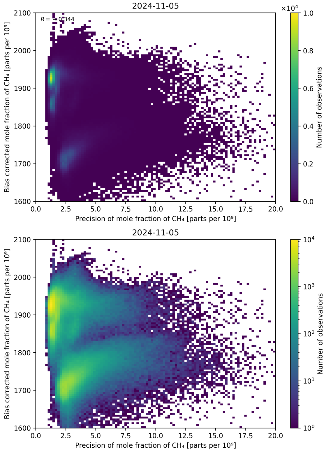
Figure 82: Scatter density plot of “Precision of mole fraction of CH 4 ” against “Bias corrected mole fraction of CH 4 ” for 2024-11-04 to 2024-11-06.
