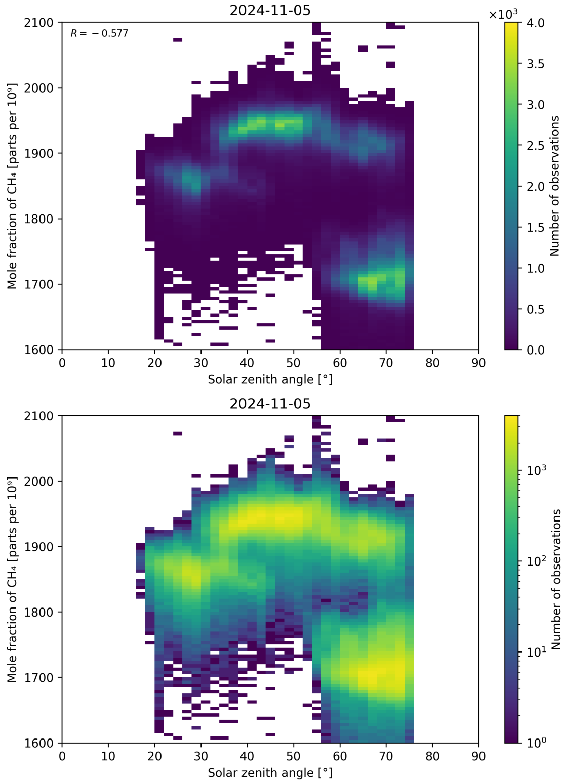
Figure 99: Scatter density plot of “Solar zenith angle” against “Mole fraction of CH 4 ” for 2024-11-04 to 2024-11-06.
