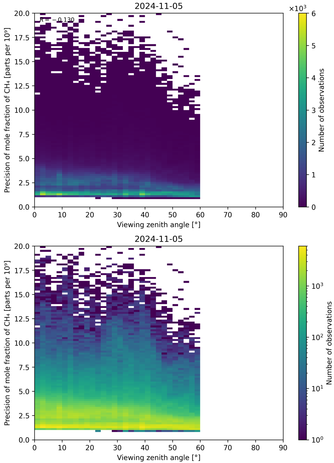
Figure 112: Scatter density plot of “Viewing zenith angle” against “Precision of mole fraction of CH 4 ” for 2024-11-04 to 2024-11-06.
