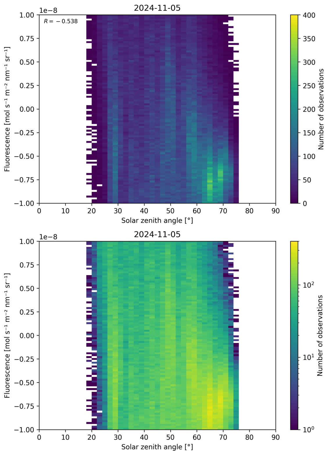
Figure 97: Scatter density plot of “Solar zenith angle” against “Fluorescence” for 2024-11-04 to 2024-11-06.
