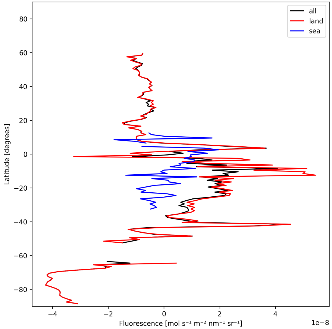
Figure 21: Zonal average of “Fluorescence” for 2024-11-04 to 2024-11-06.
