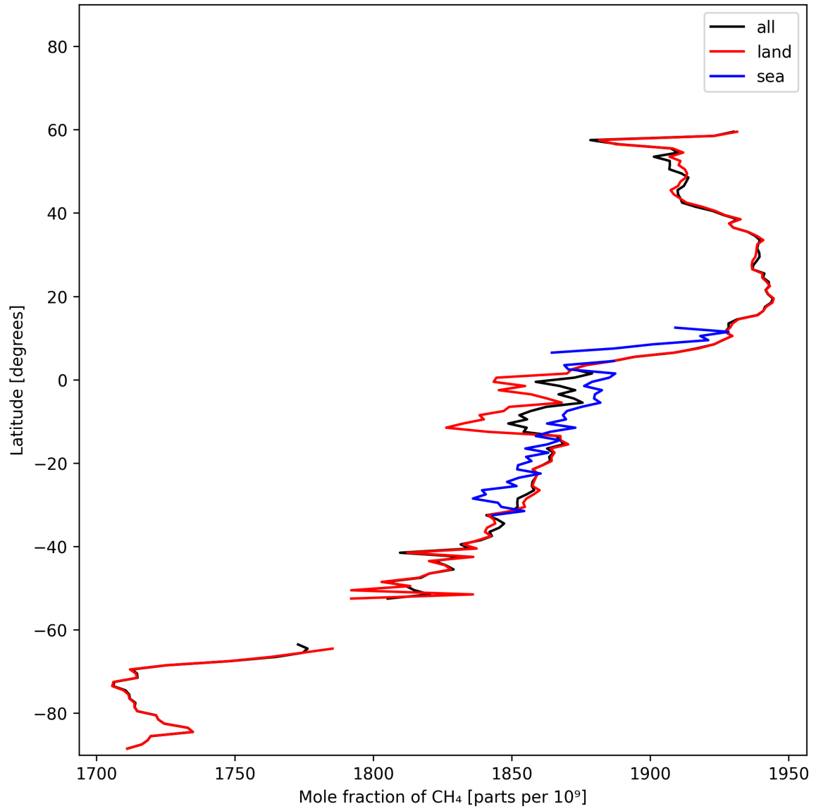
Figure 12: Zonal average of “Mole fraction of \text{CH}_4 ” for 2024-11-04 to 2024-11-06.
