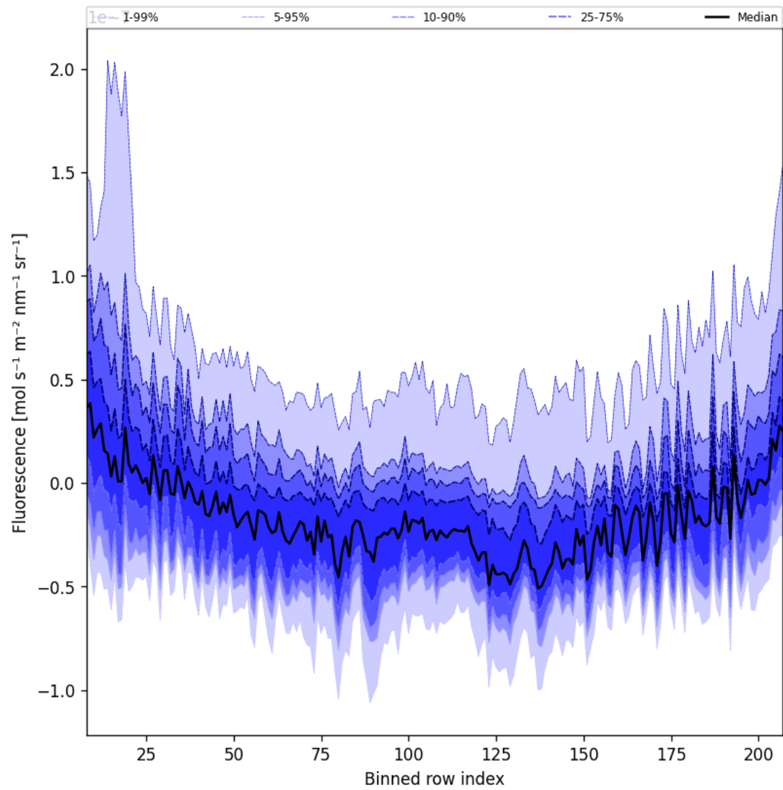
Figure 43: Along track statistics of “Fluorescence” for 2024-11-04 to 2024-11-06
