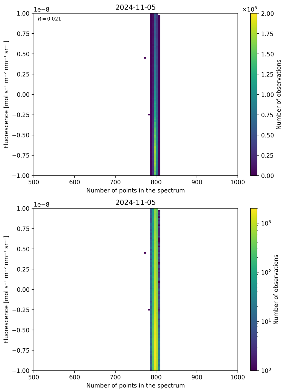
Figure 91: Scatter density plot of “Number of points in the spectrum” against “Fluorescence” for 2024-11-04 to 2024-11-06.
