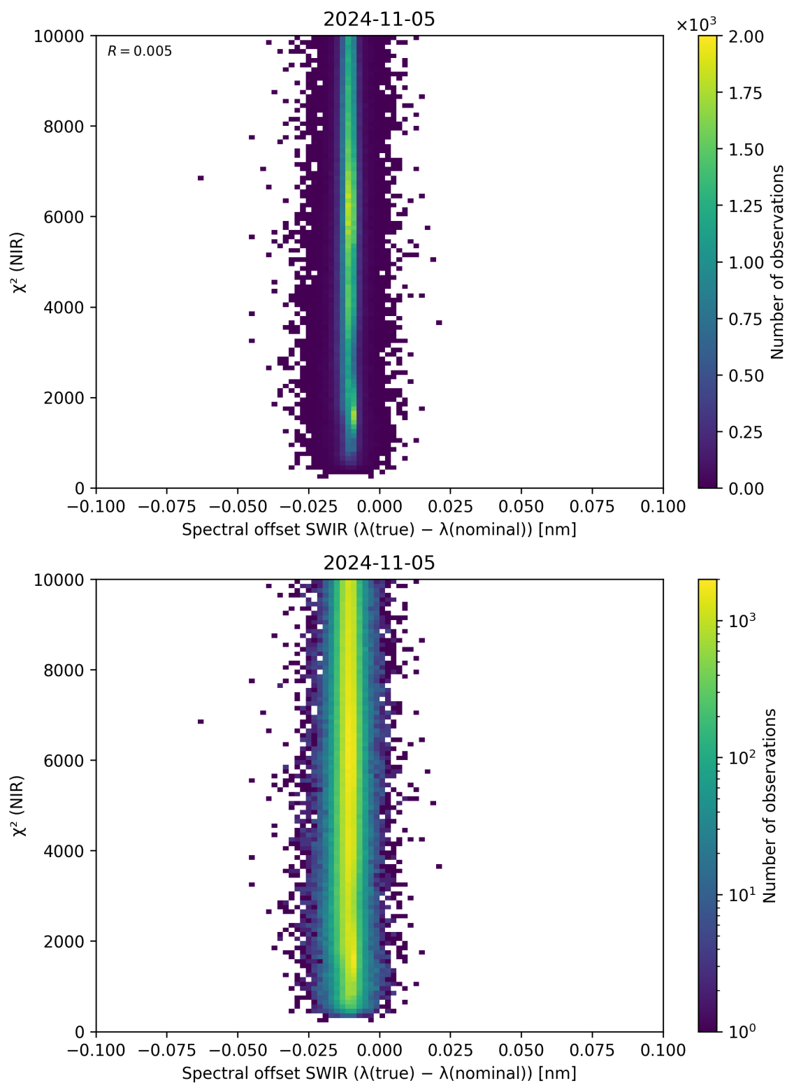
Figure 117: Scatter density plot of “Spectral offset SWIR ( \lambda_{\text{true}} - \lambda_{\text{nominal}} )” against “ \chi^2 (NIR)” for 2024-11-04 to 2024-11-06.
