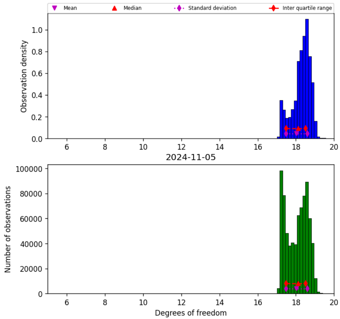
Figure 30: Histogram of “Degrees of freedom” for 2024-11-04 to 2024-11-06
