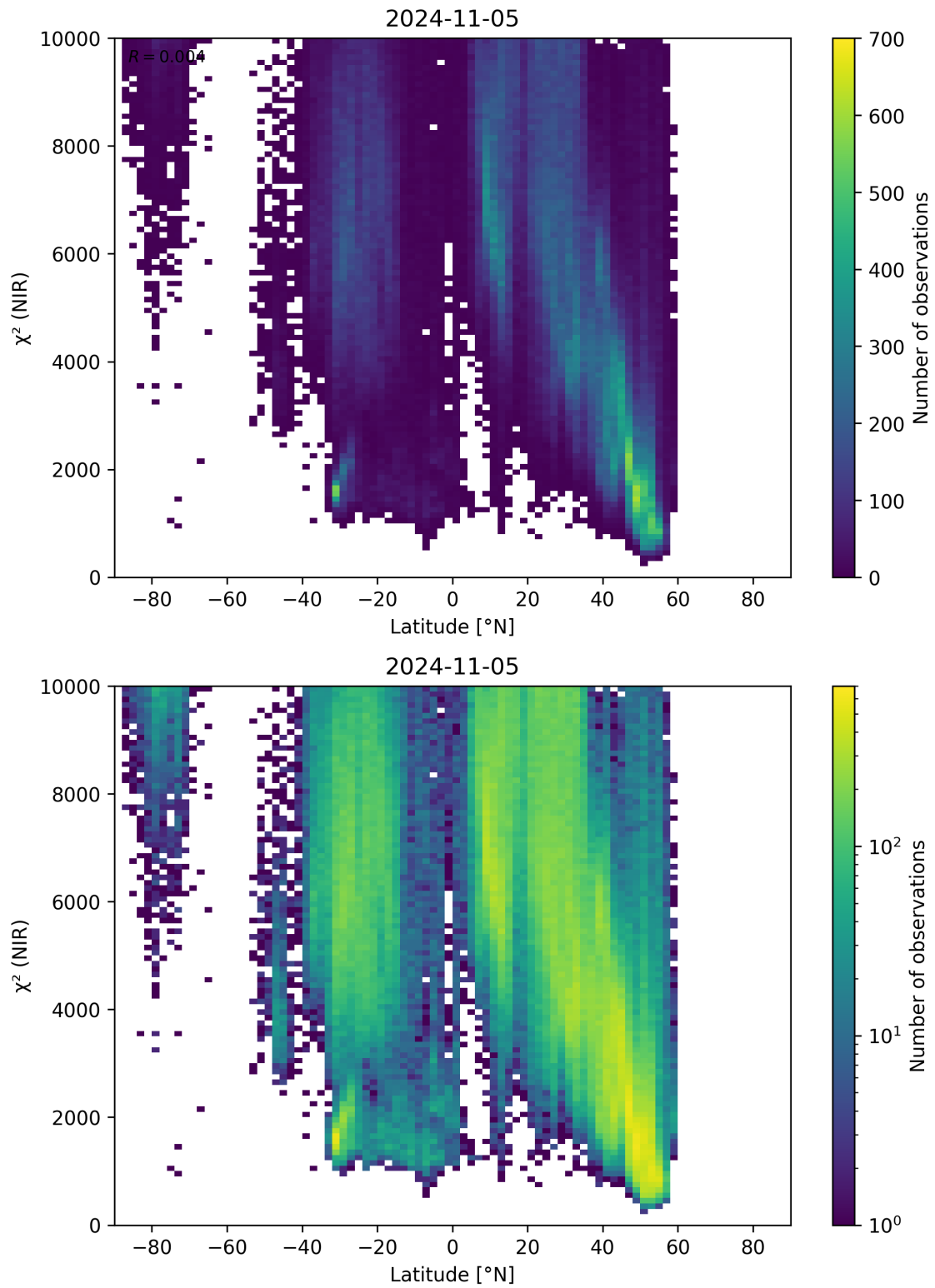
Figure 53: Scatter density plot of “Latitude” against “ \chi^2 (NIR)” for 2024-11-04 to 2024-11-06.
