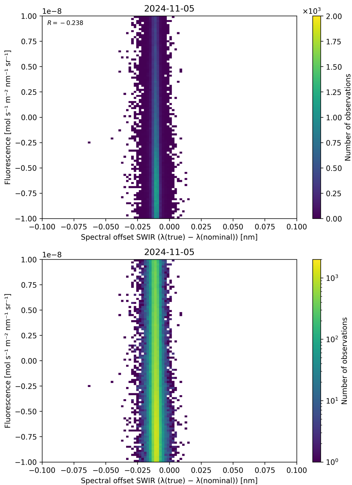
Figure 120: Scatter density plot of “Spectral offset SWIR ( \lambda_{\text{true}} - \lambda_{\text{nominal}} )” against “Fluorescence” for 2024-11-04 to 2024-11-06.
