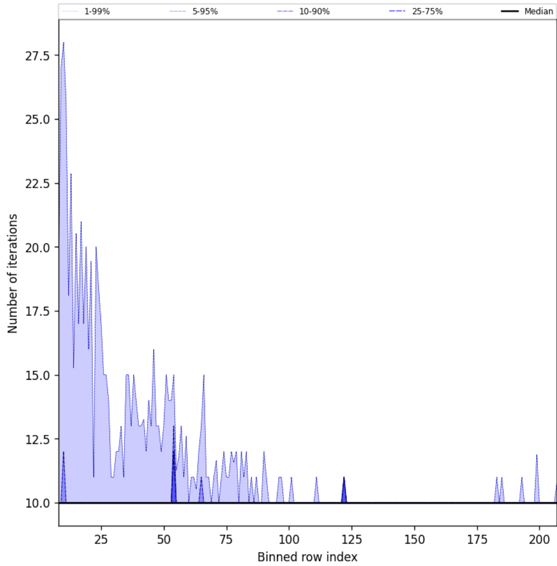
Figure 42: Along track statistics of “Number of iterations” for 2024-11-04 to 2024-11-06
