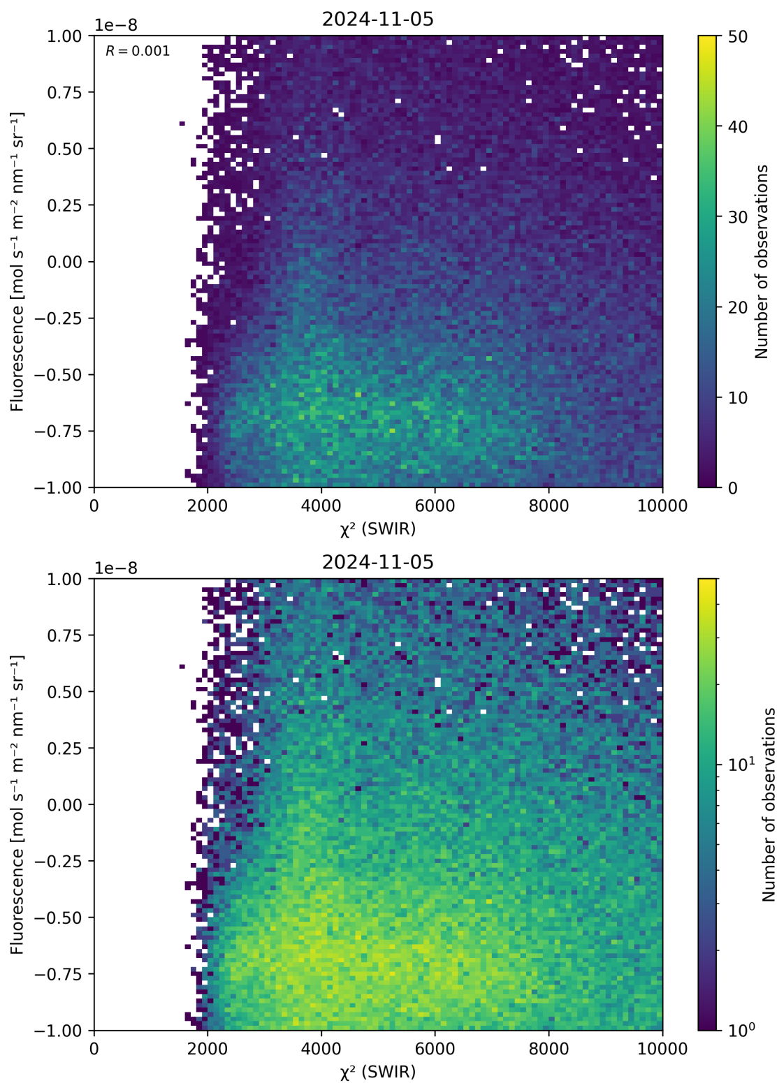
Figure 49: Scatter density plot of “ \chi^2 (SWIR)” against “Fluorescence” for 2024-11-04 to 2024-11-06.
