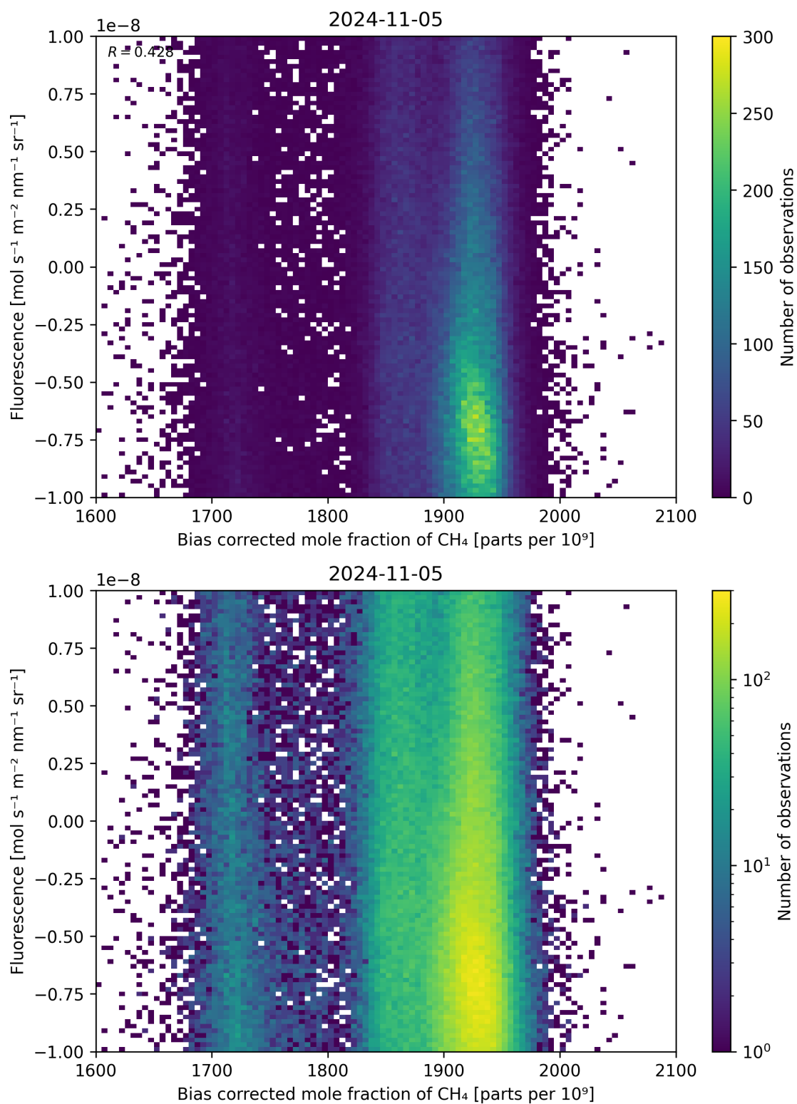
Figure 66: Scatter density plot of “Bias corrected mole fraction of \text{CH}_4 ” against “Fluorescence” for 2024-11-04 to 2024-11-06.
