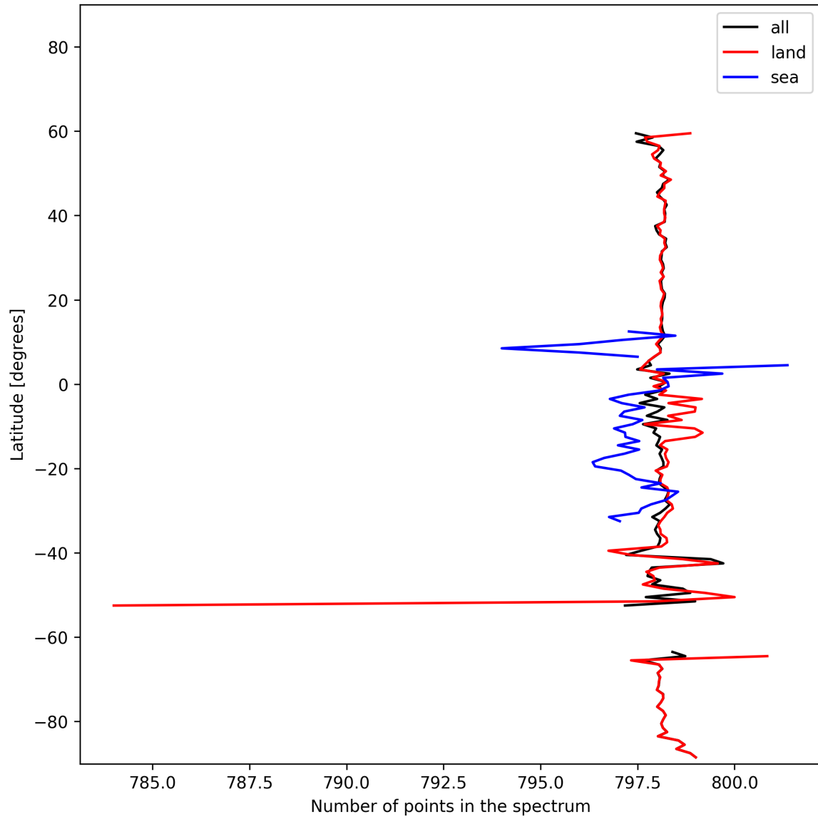
Figure 15: Zonal average of “Number of points in the spectrum” for 2024-11-04 to 2024-11-06.
