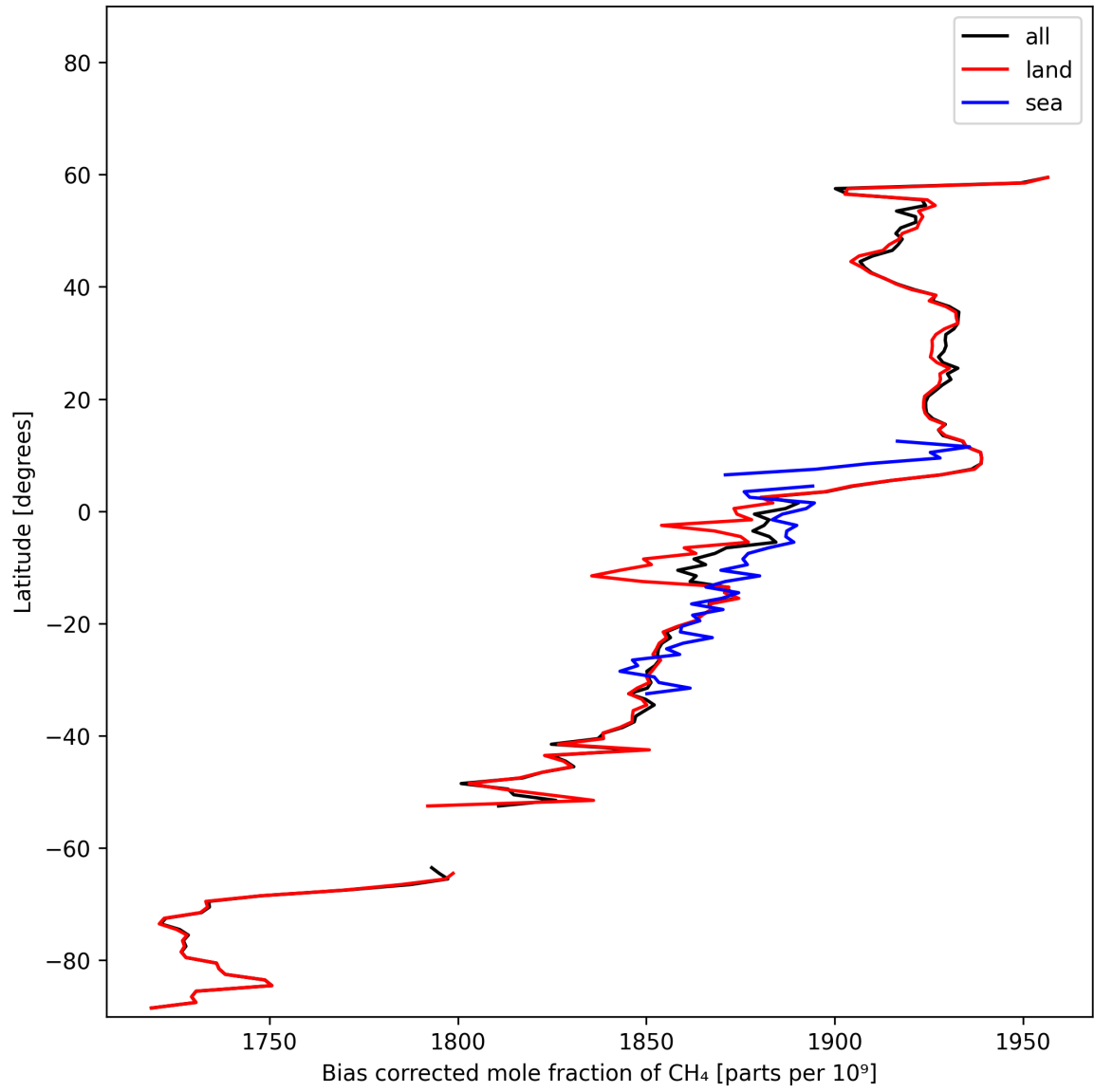
Figure 14: Zonal average of “Bias corrected mole fraction of CH 4 ” for 2024-11-04 to 2024-11-06.
