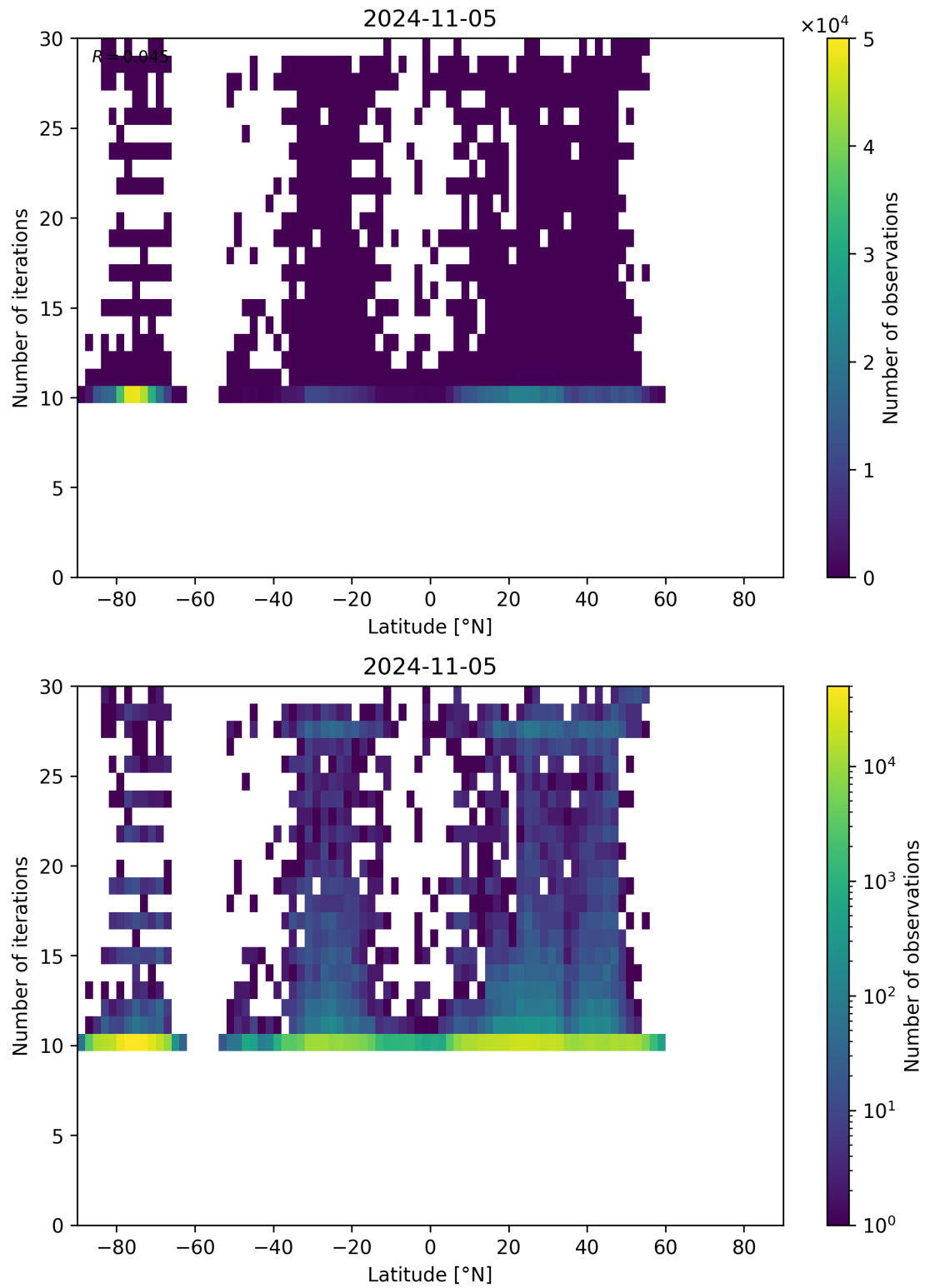
Figure 60: Scatter density plot of “Latitude” against “Number of iterations” for 2024-11-04 to 2024-11-06.
