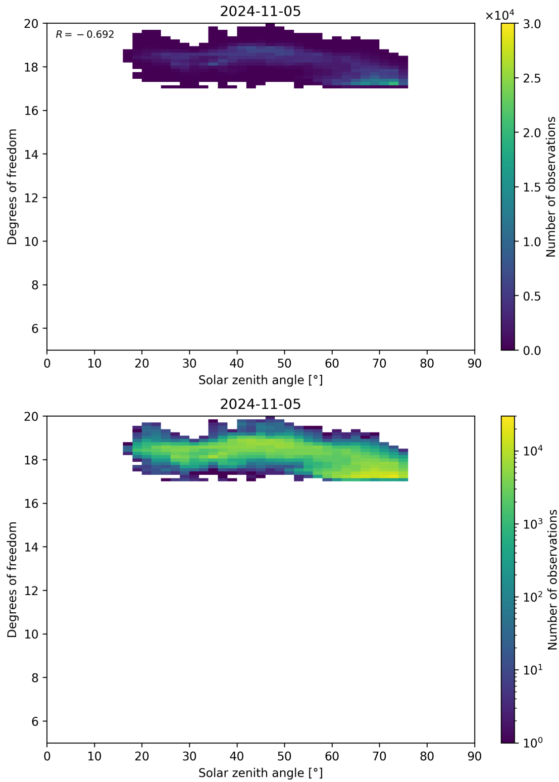
Figure 96: Scatter density plot of “Solar zenith angle” against “Degrees of freedom” for 2024-11-04 to 2024-11-06.
