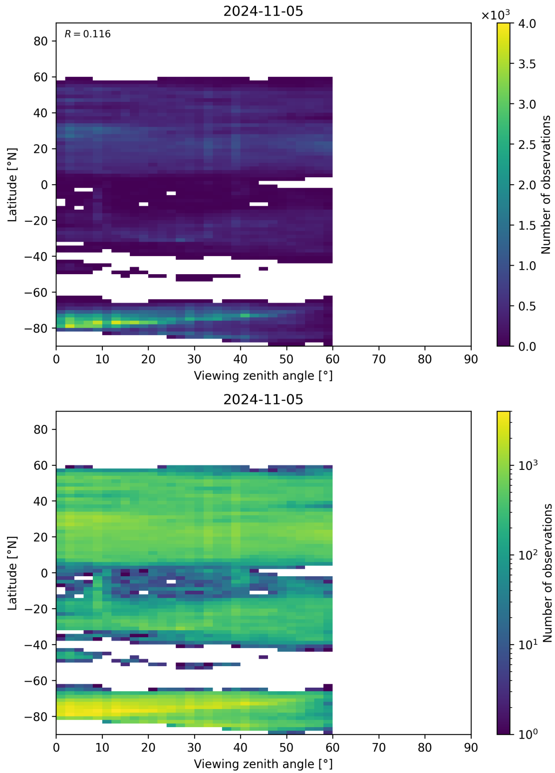
Figure 109: Scatter density plot of “Viewing zenith angle” against “Latitude” for 2024-11-04 to 2024-11-06.
