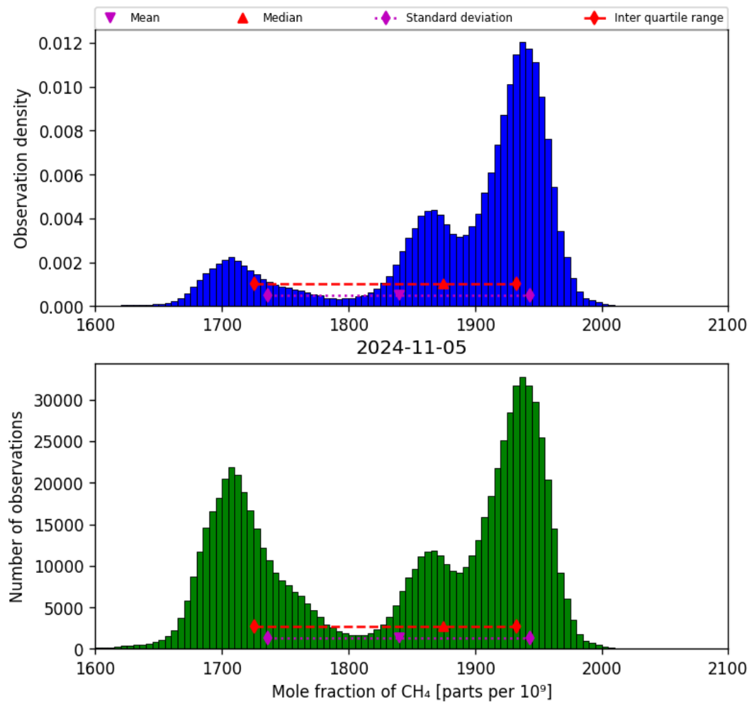
Figure 23: Histogram of “Mole fraction of CH 4 ” for 2024-11-04 to 2024-11-06
