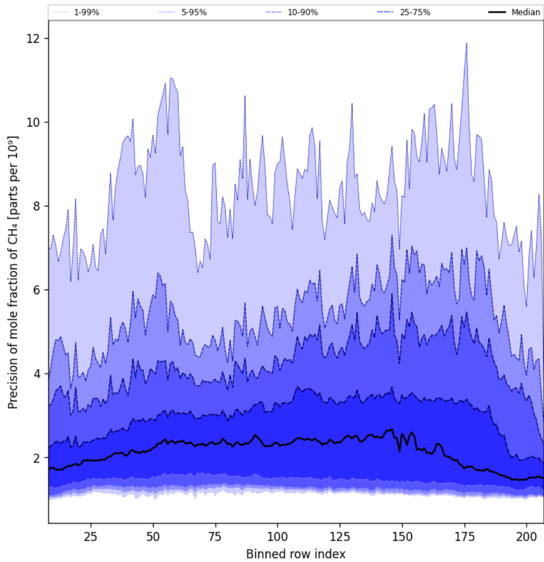
Figure 35: Along track statistics of “Precision of mole fraction of CH 4 ” for 2024-11-04 to 2024-11-06
