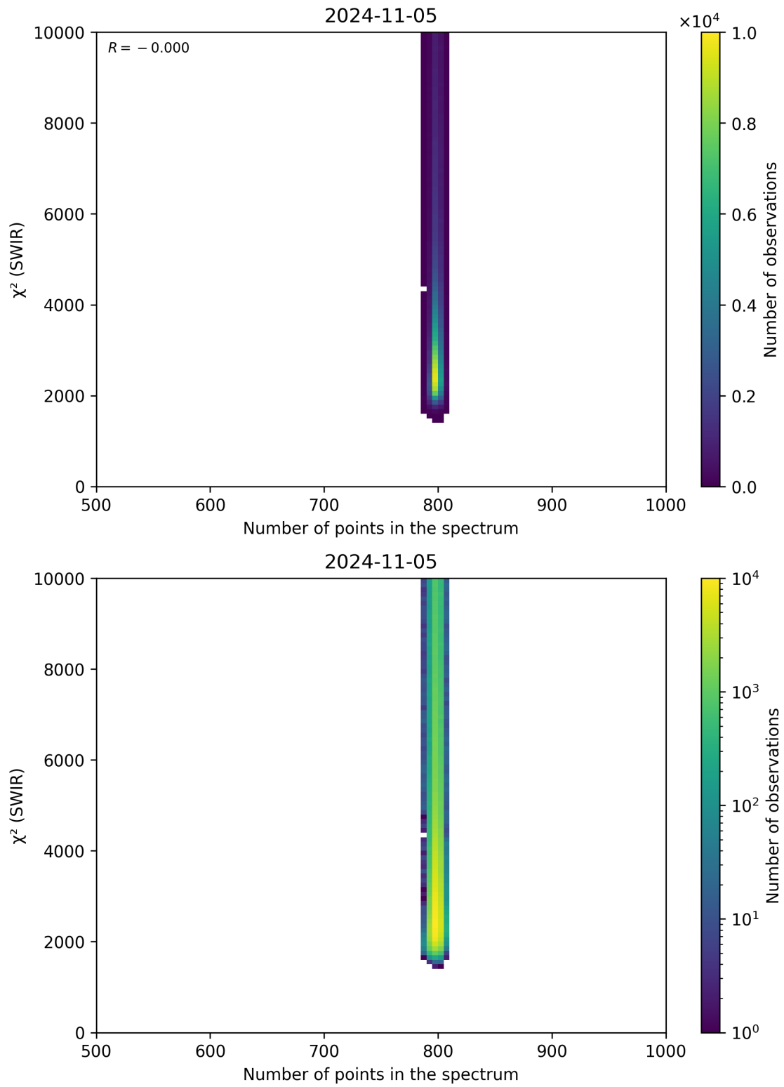
Figure 89: Scatter density plot of “Number of points in the spectrum” against “ \chi^2 (SWIR)” for 2024-11-04 to 2024-11-06.
