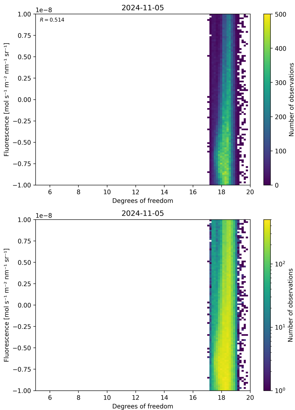
Figure 51: Scatter density plot of “Degrees of freedom” against “Fluorescence” for 2024-11-04 to 2024-11-06.
