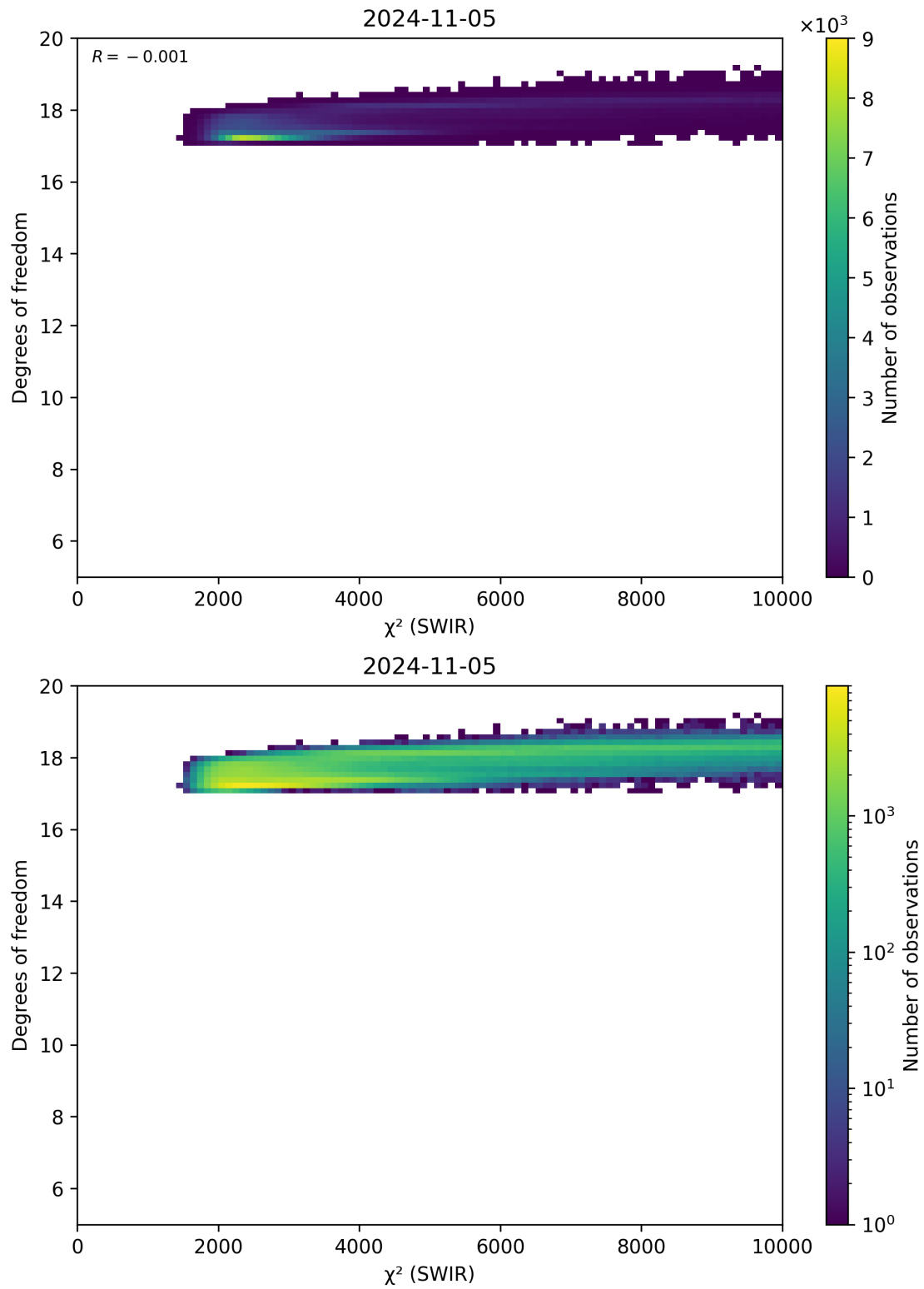
Figure 48: Scatter density plot of “ \chi^2 (SWIR)” against “Degrees of freedom” for 2024-11-04 to 2024-11-06.
