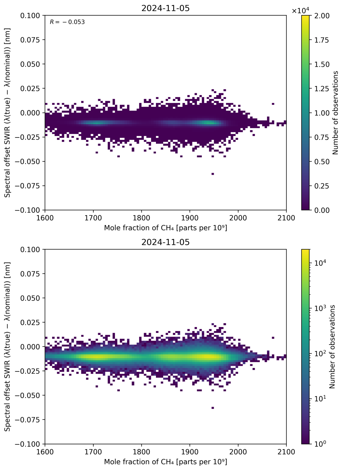
Figure 86: Scatter density plot of “Mole fraction of CH 4 ” against “Spectral offset SWIR ( \lambda_{\text{true}} - \lambda_{\text{nominal}} )” for 2024-11-04 to 2024-11-06.
