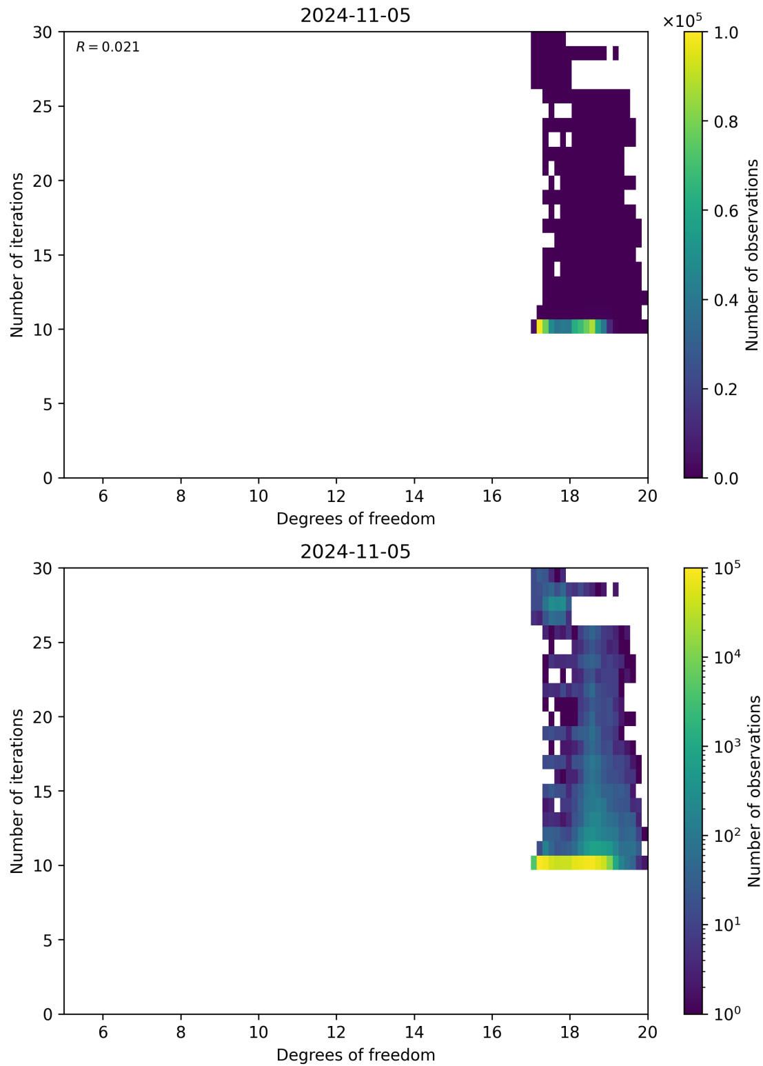
Figure 52: Scatter density plot of “Degrees of freedom” against “Number of iterations” for 2024-11-04 to 2024-11-06.
