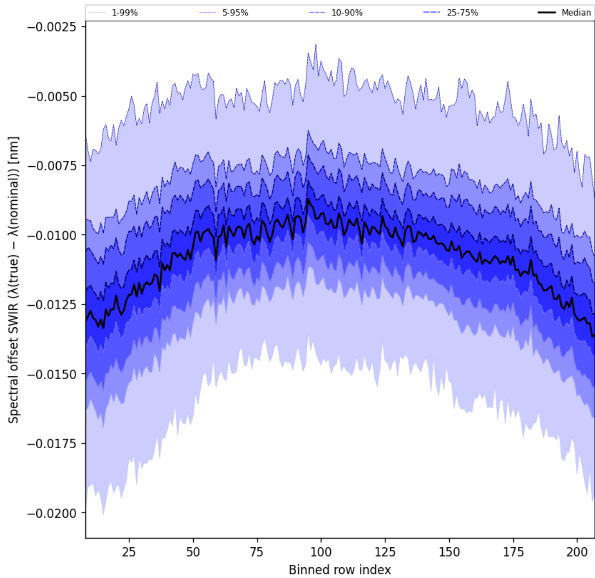
Figure 38: Along track statistics of “Spectral offset SWIR ( \lambda_{\text{true}} - \lambda_{\text{nominal}} )” for 2024-11-04 to 2024-11-06
