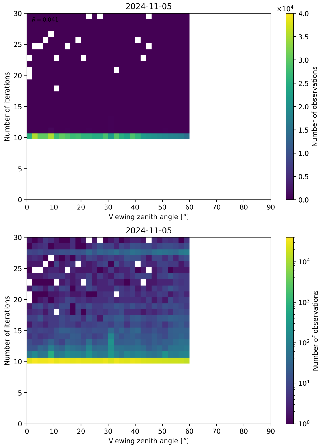
Figure 113: Scatter density plot of “Viewing zenith angle” against “Number of iterations” for 2024-11-04 to 2024-11-06.
