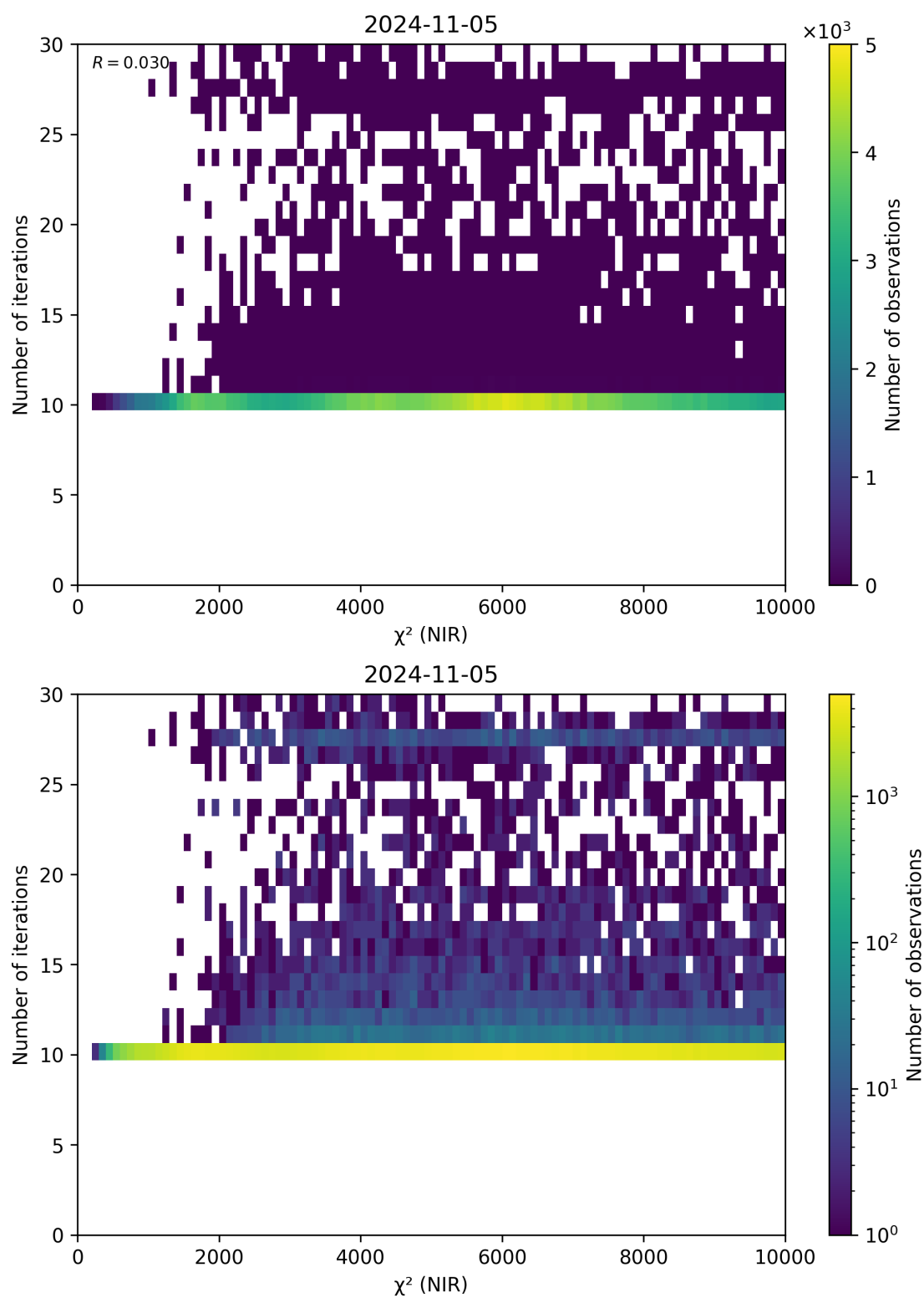
Figure 46: Scatter density plot of “ \chi^2 (NIR)” against “Number of iterations” for 2024-11-04 to 2024-11-06.
