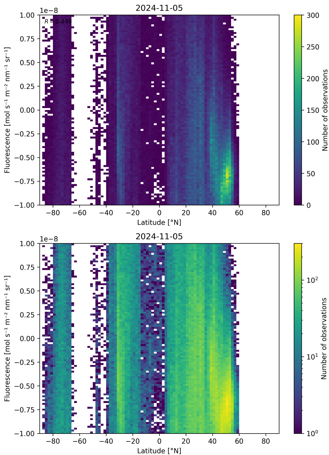
Figure 56: Scatter density plot of “Latitude” against “Fluorescence” for 2024-11-04 to 2024-11-06.
