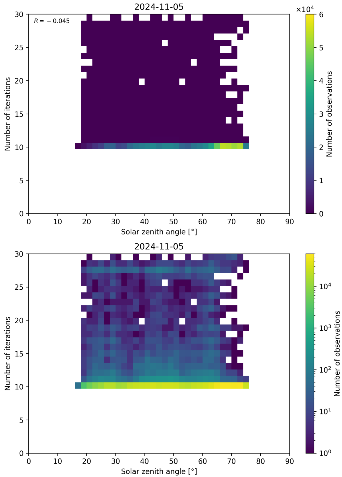
Figure 102: Scatter density plot of “Solar zenith angle” against “Number of iterations” for 2024-11-04 to 2024-11-06.
