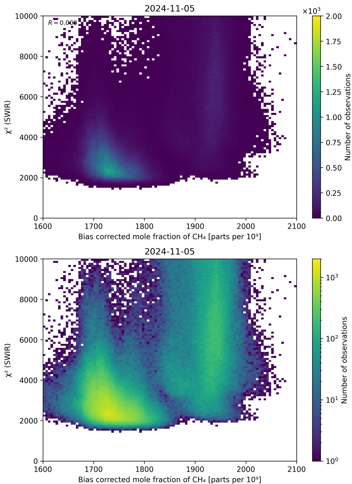
Figure 64: Scatter density plot of “Bias corrected mole fraction of \text{CH}_4 ” against “ \chi^2 (SWIR)” for 2024-11-04 to 2024-11-06.
