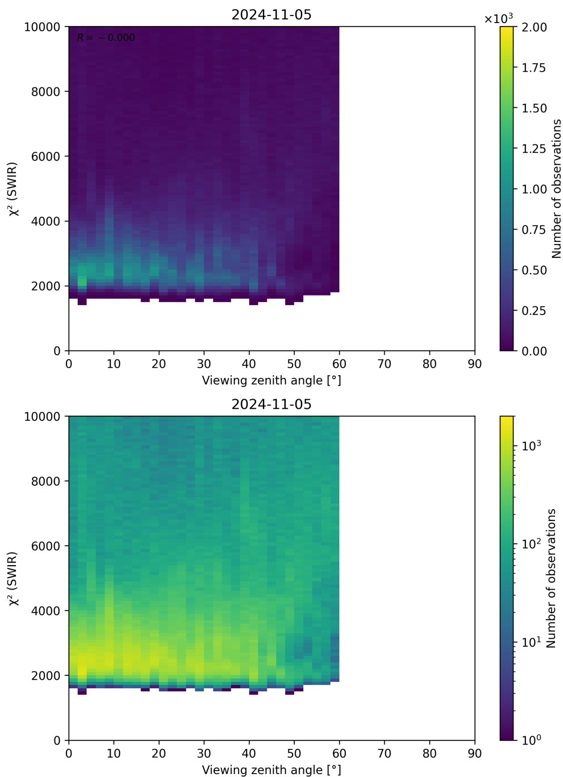
Figure 106: Scatter density plot of “Viewing zenith angle” against “ \chi^2 (SWIR)” for 2024-11-04 to 2024-11-06.
