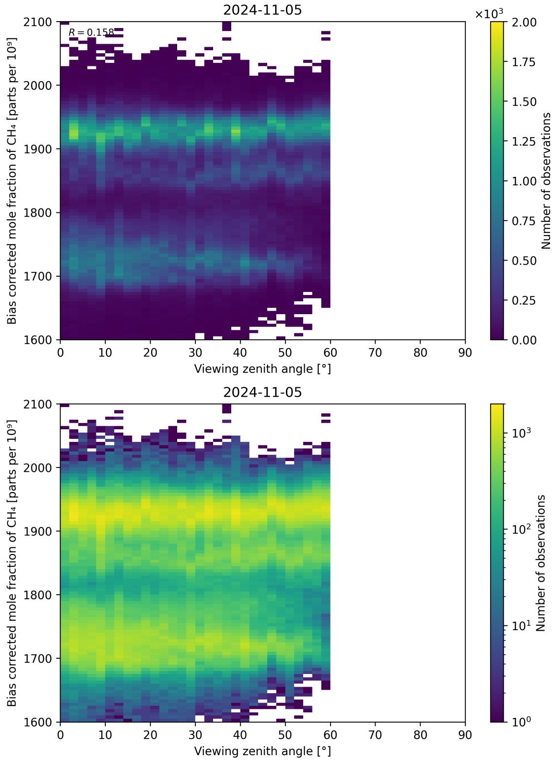
Figure 111: Scatter density plot of “Viewing zenith angle” against “Bias corrected mole fraction of CH 4 ” for 2024-11-04 to 2024-11-06.
