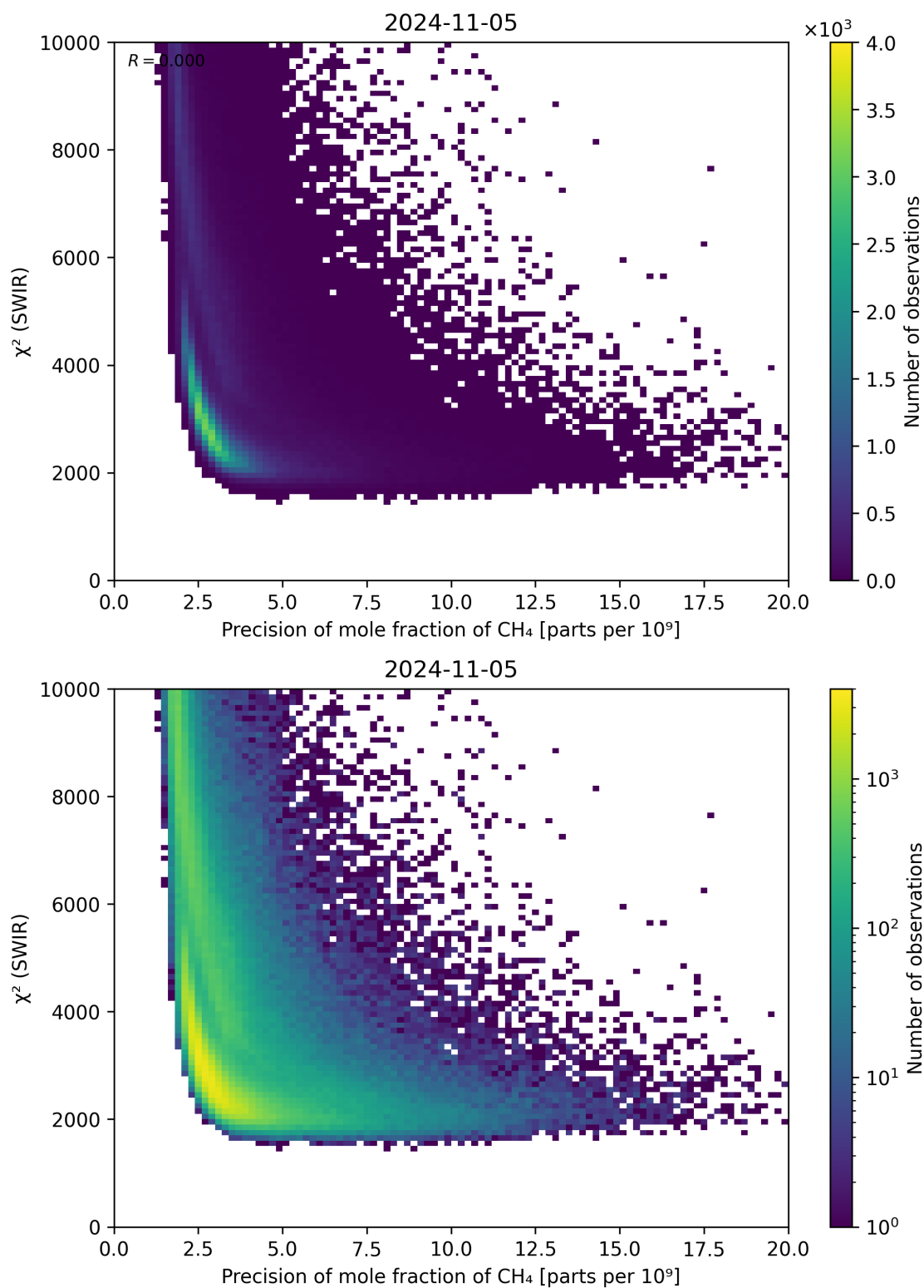
Figure 79: Scatter density plot of “Precision of mole fraction of CH 4 ” against “ \chi^2 (SWIR)” for 2024-11-04 to 2024-11-06.
