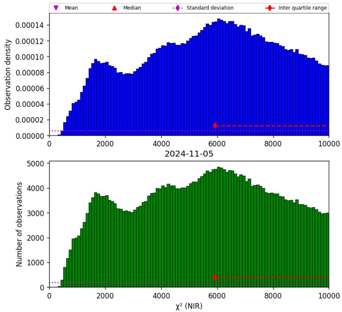
Figure 29: Histogram of “ \chi^2 (NIR)” for 2024-11-04 to 2024-11-06
