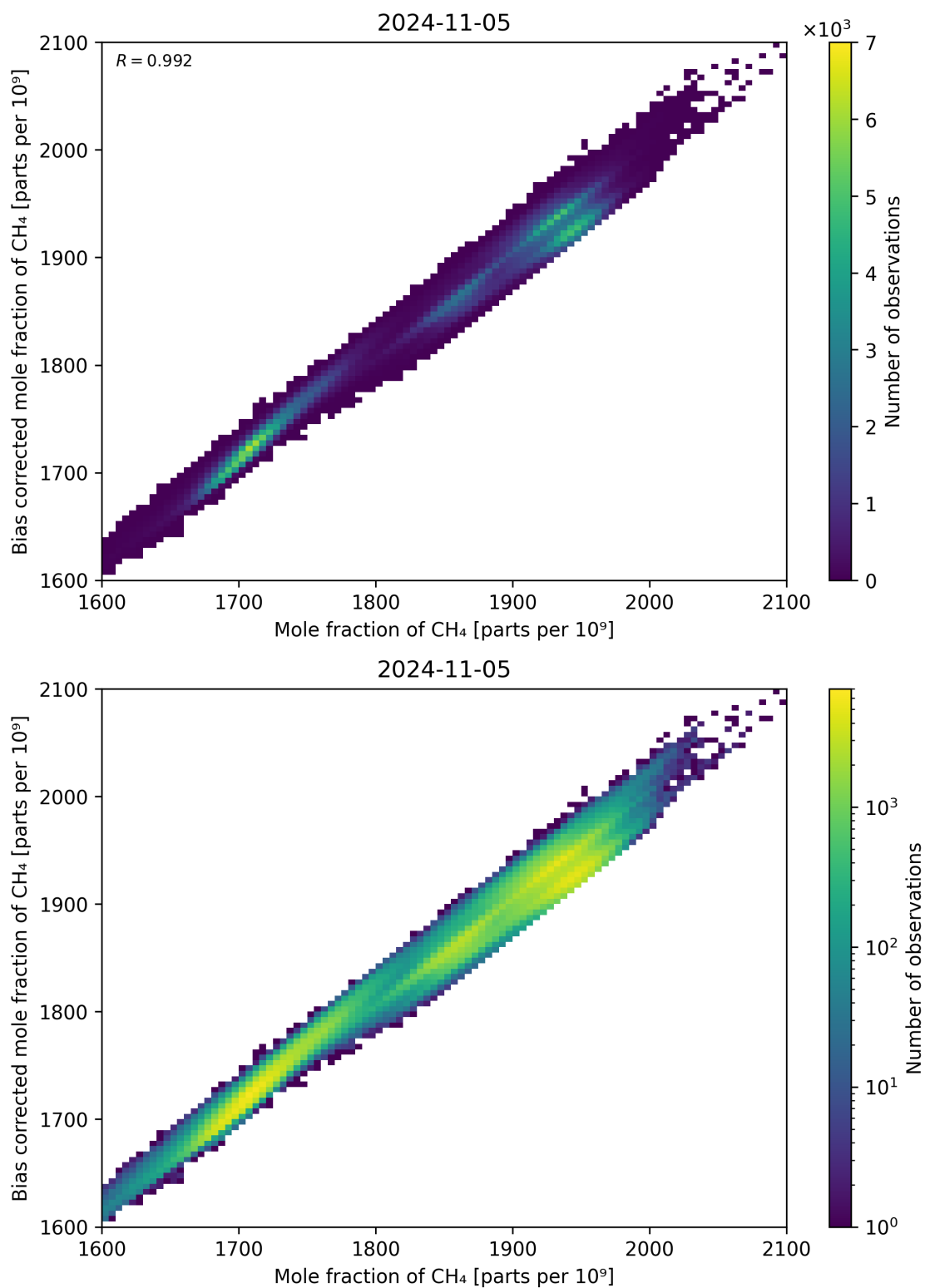
Figure 74: Scatter density plot of “Mole fraction of CH 4 ” against “Bias corrected mole fraction of CH 4 ” for 2024-11-04 to 2024-11-06.
