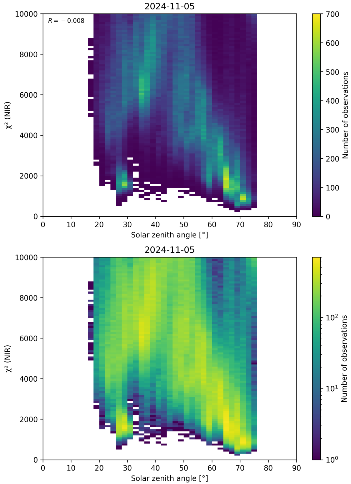
Figure 94: Scatter density plot of “Solar zenith angle” against “ \chi^2 (NIR)” for 2024-11-04 to 2024-11-06.
