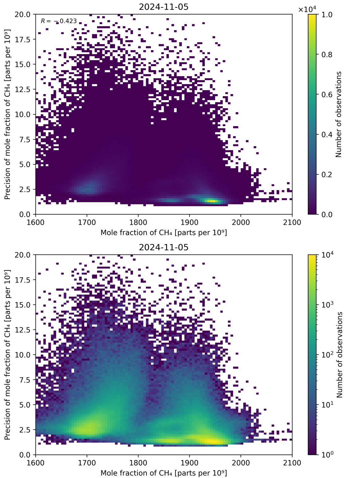
Figure 75: Scatter density plot of “Mole fraction of CH 4 ” against “Precision of mole fraction of CH 4 ” for 2024-11-04 to 2024-11-06.
