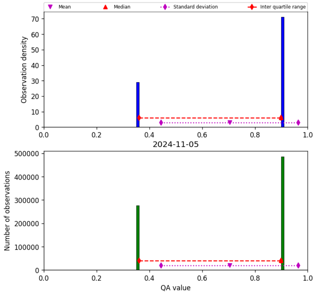
Figure 22: Histogram of “QA value” for 2024-11-04 to 2024-11-06
