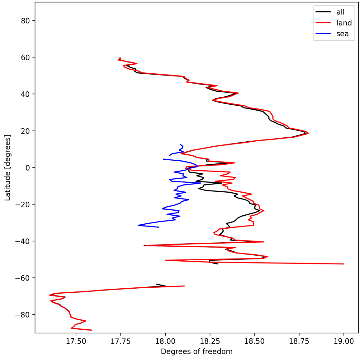
Figure 19: Zonal average of “Degrees of freedom” for 2024-11-04 to 2024-11-06.
