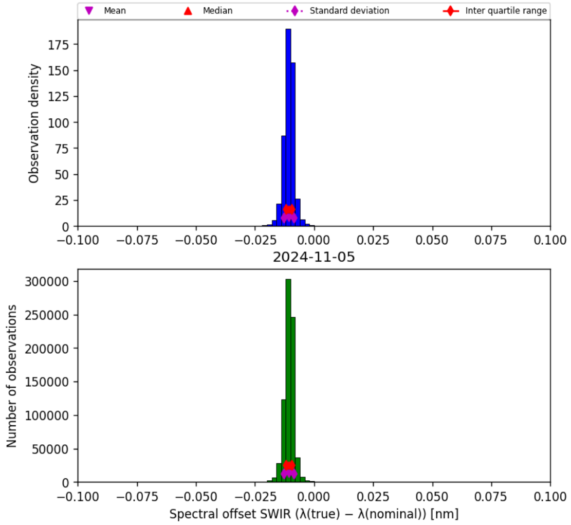
Figure 27: Histogram of “Spectral offset SWIR ( \lambda_{\text{true}} - \lambda_{\text{nominal}} )” for 2024-11-04 to 2024-11-06
