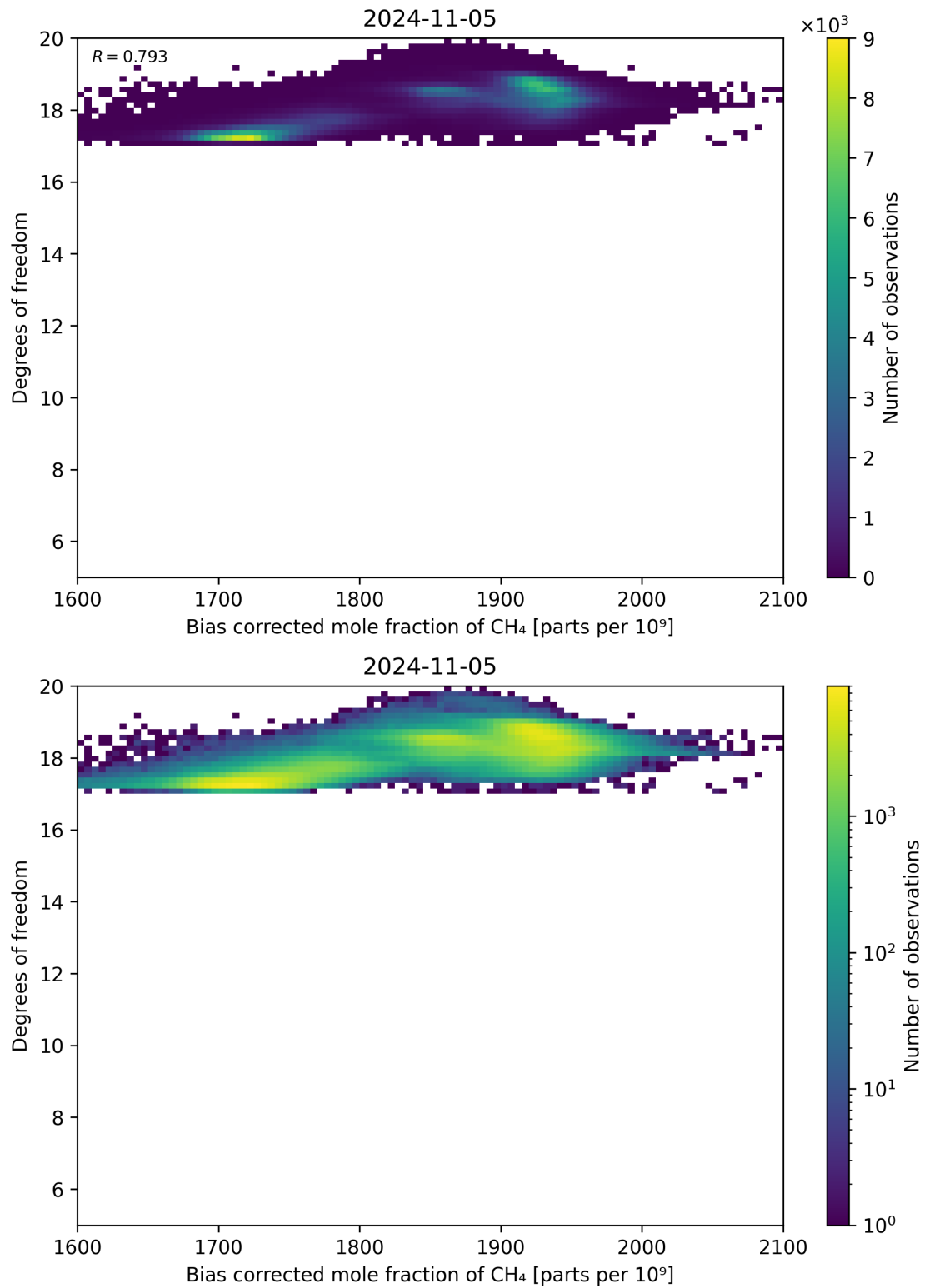
Figure 65: Scatter density plot of “Bias corrected mole fraction of CH 4 ” against “Degrees of freedom” for 2024-11-04 to 2024-11-06.
