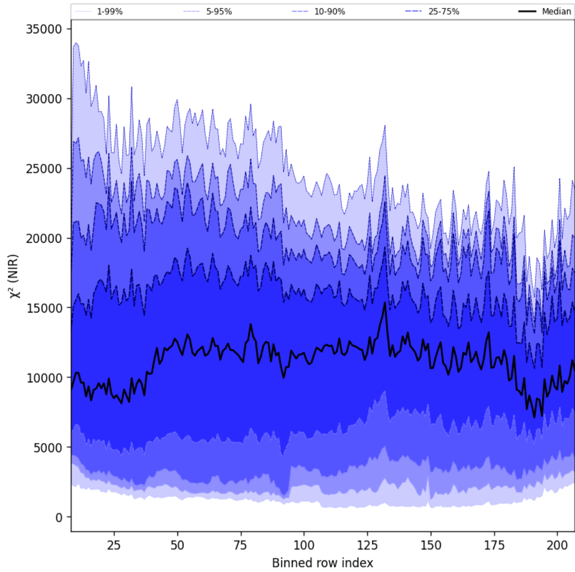
Figure 40: Along track statistics of “ \chi^2 (NIR)” for 2024-11-04 to 2024-11-06
