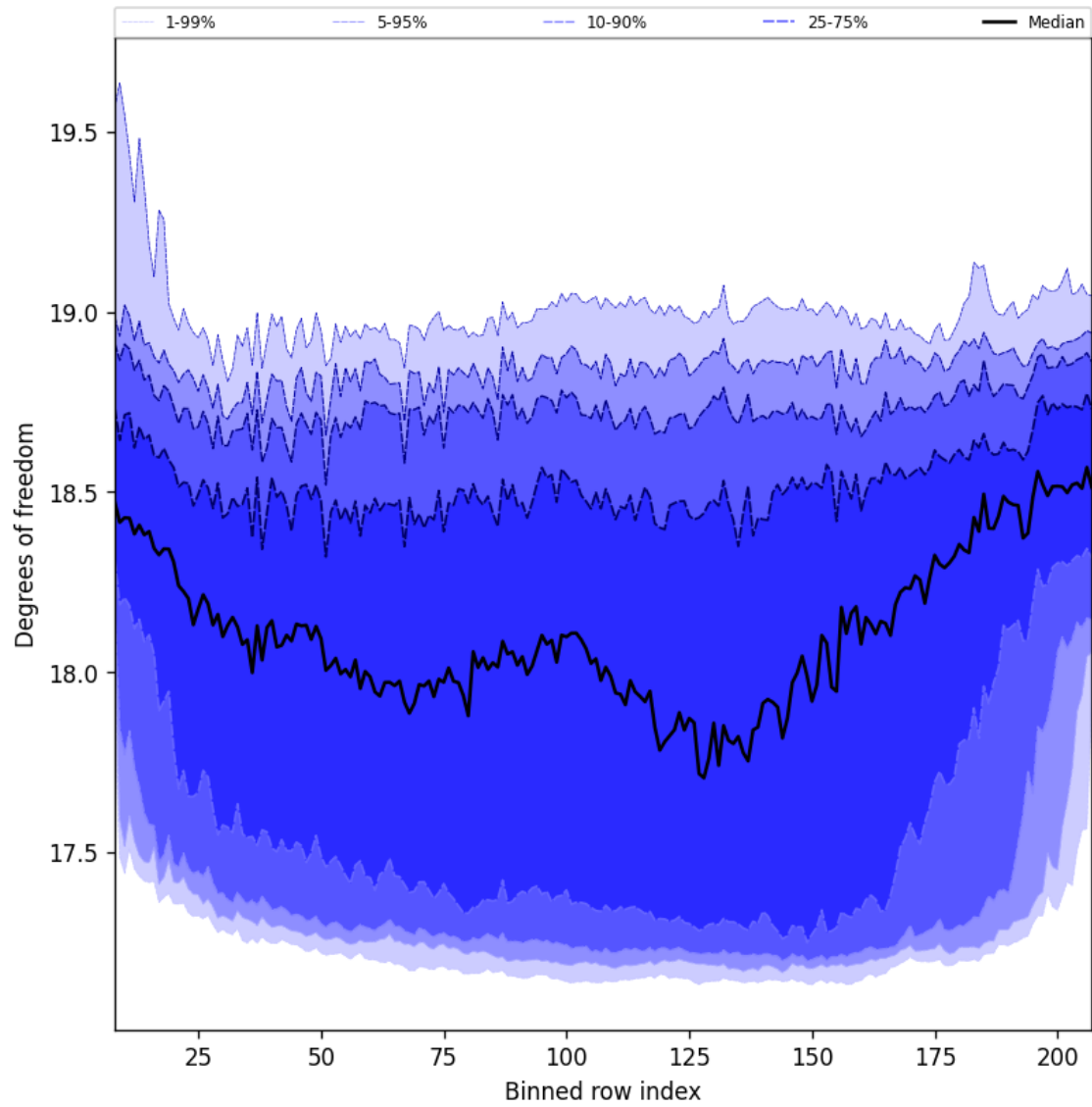
Figure 41: Along track statistics of “Degrees of freedom” for 2024-11-04 to 2024-11-06
