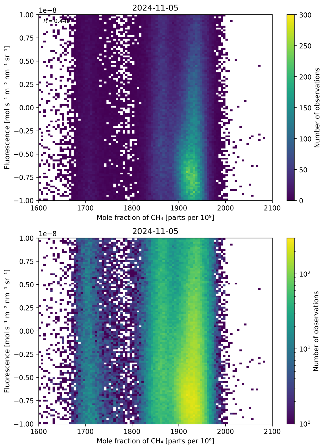
Figure 73: Scatter density plot of “Mole fraction of \text{CH}_4 ” against “Fluorescence” for 2024-11-04 to 2024-11-06.
