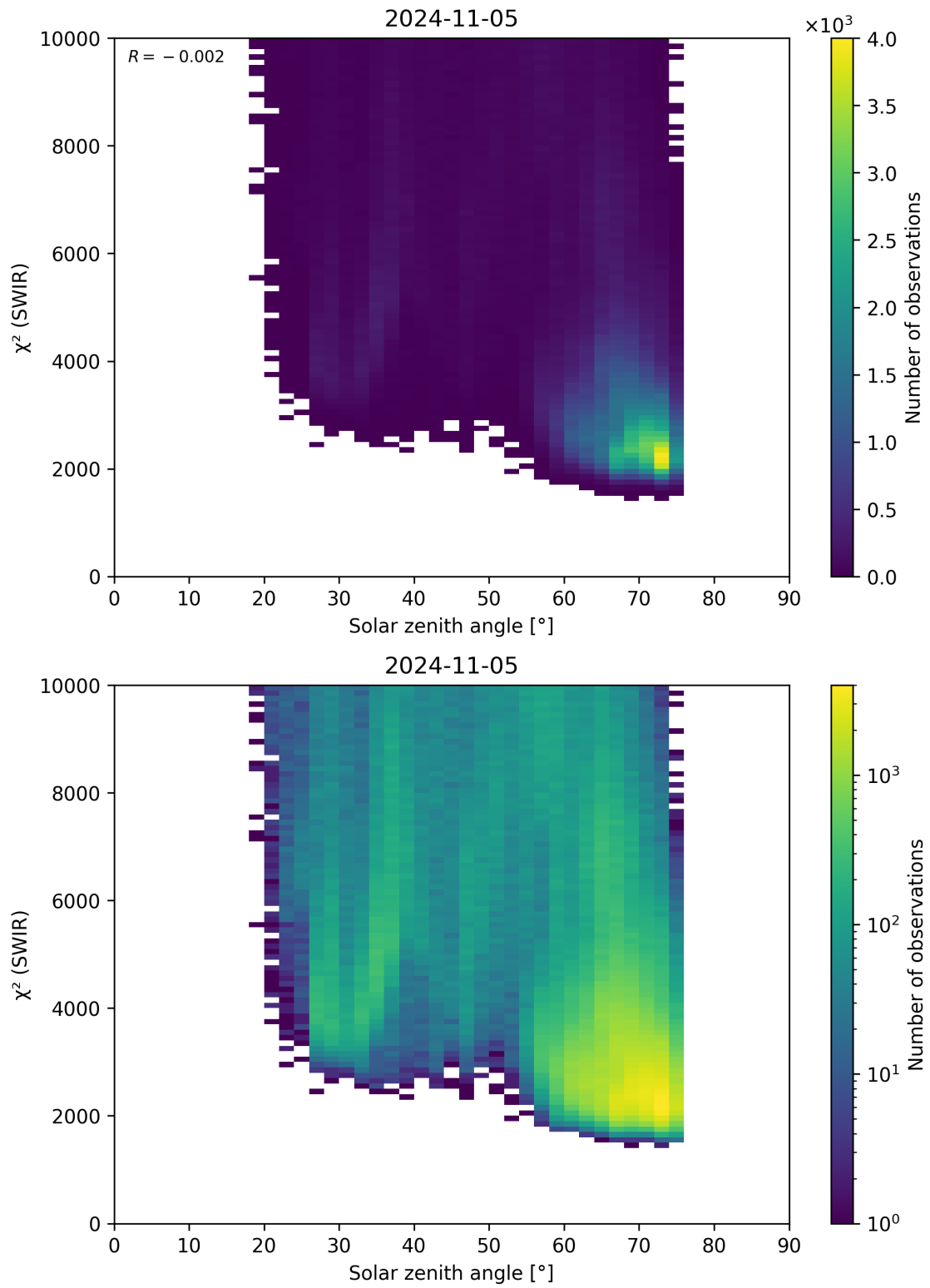
Figure 95: Scatter density plot of “Solar zenith angle” against “ \chi^2 (SWIR)” for 2024-11-04 to 2024-11-06.
