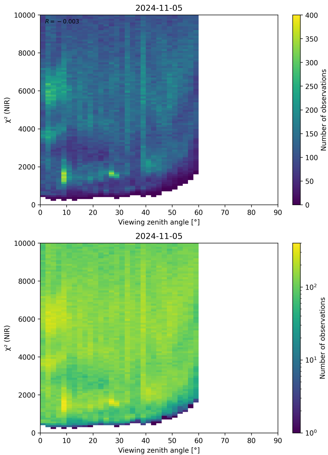
Figure 105: Scatter density plot of “Viewing zenith angle” against “ \chi^2 (NIR)” for 2024-11-04 to 2024-11-06.
