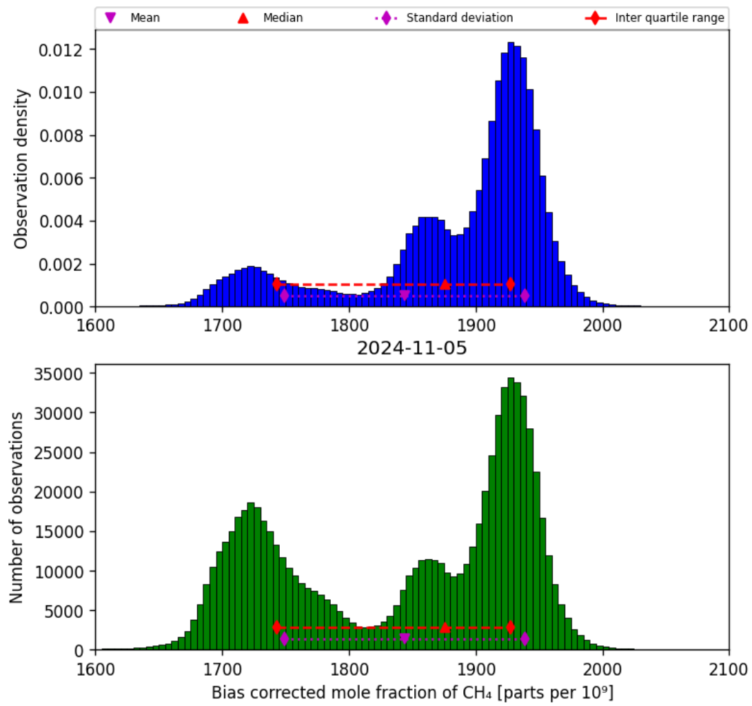
Figure 25: Histogram of “Bias corrected mole fraction of CH 4 ” for 2024-11-04 to 2024-11-06
