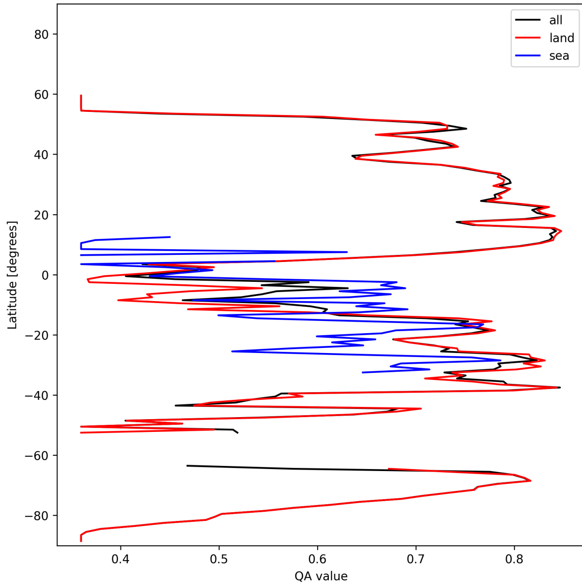
Figure 11: Zonal average of “QA value” for 2024-11-04 to 2024-11-06.
