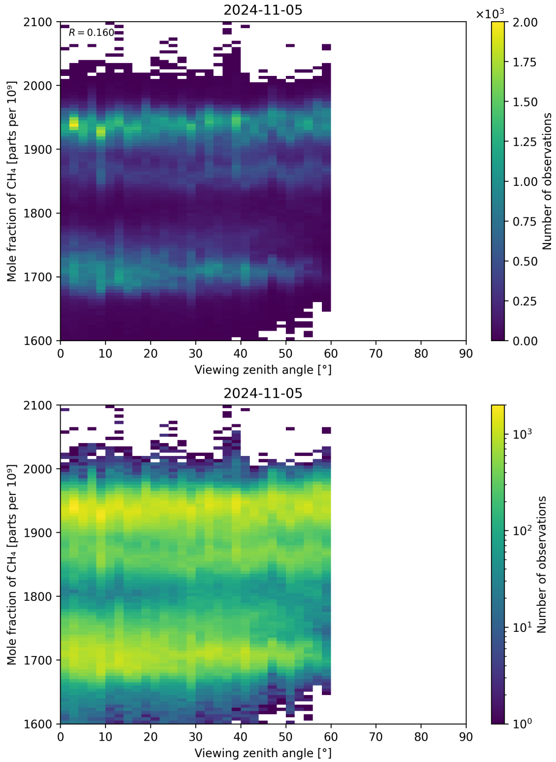
Figure 110: Scatter density plot of “Viewing zenith angle” against “Mole fraction of CH 4 ” for 2024-11-04 to 2024-11-06.
