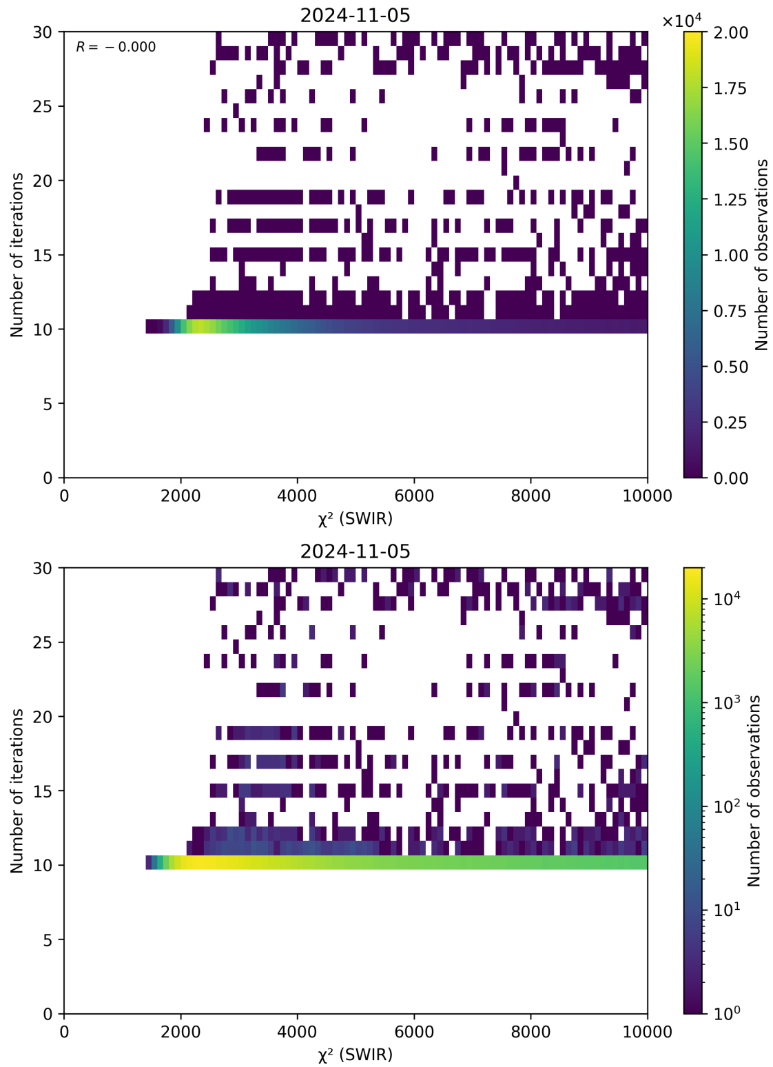
Figure 50: Scatter density plot of “ \chi^2 (SWIR)” against “Number of iterations” for 2024-11-04 to 2024-11-06.
