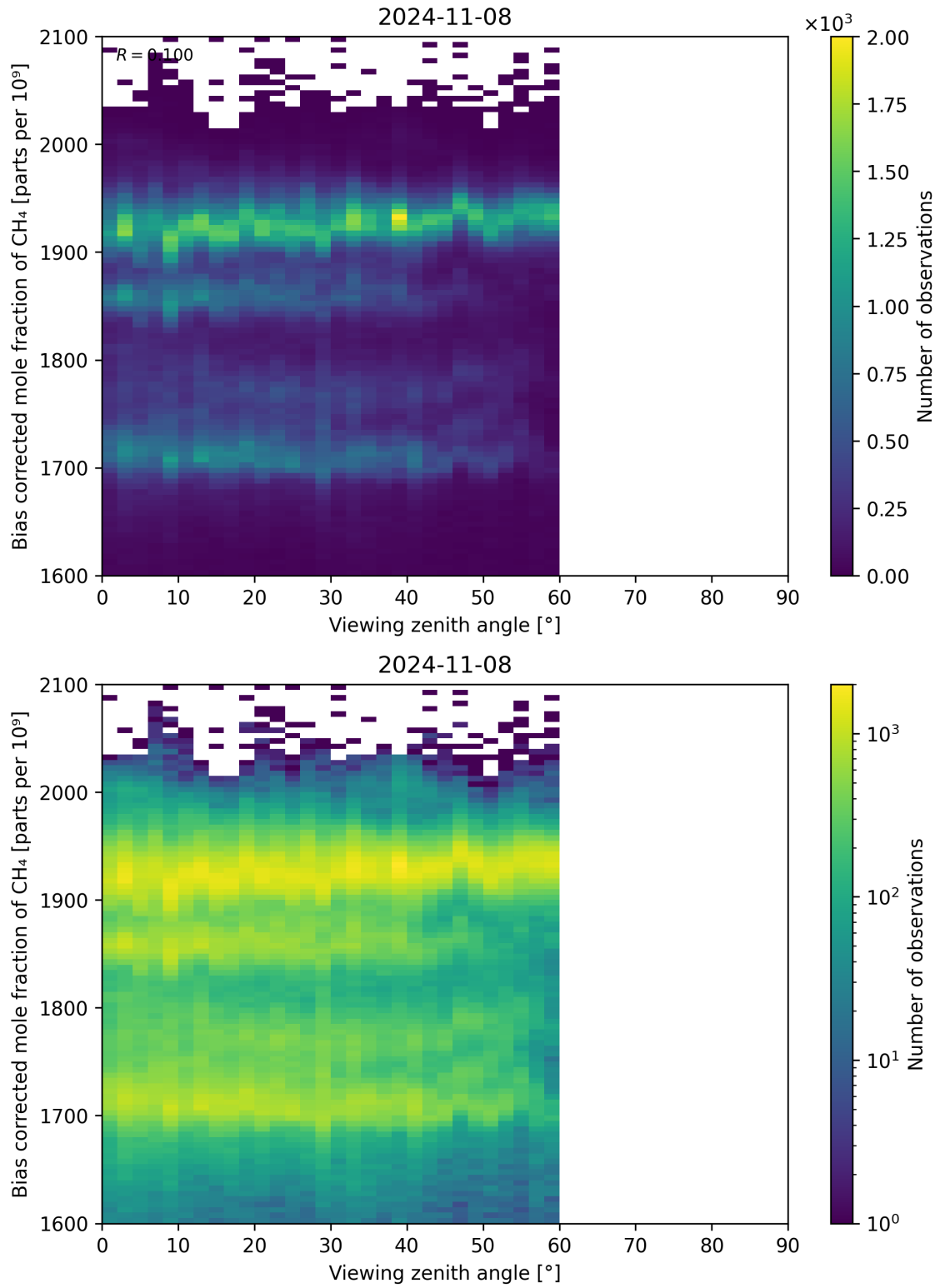
Figure 111: Scatter density plot of “Viewing zenith angle” against “Bias corrected mole fraction of CH 4 ” for 2024-11-07 to 2024-11-09.
