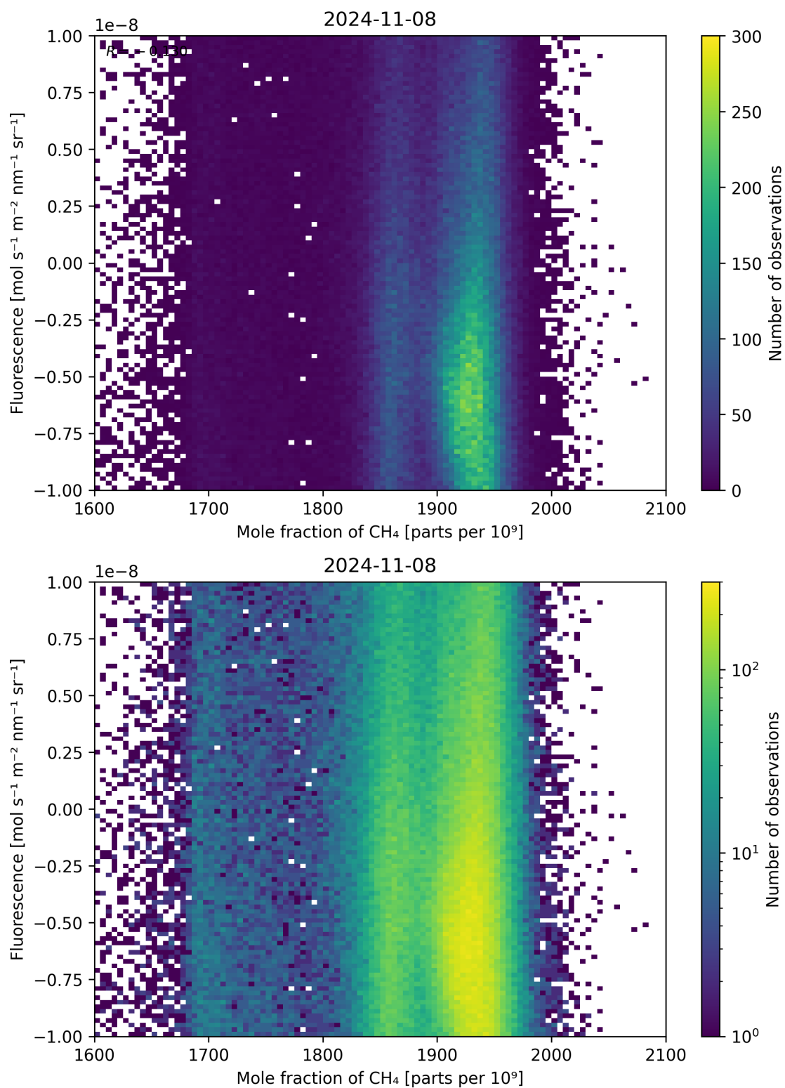
Figure 73: Scatter density plot of “Mole fraction of \text{CH}_4 ” against “Fluorescence” for 2024-11-07 to 2024-11-09.
