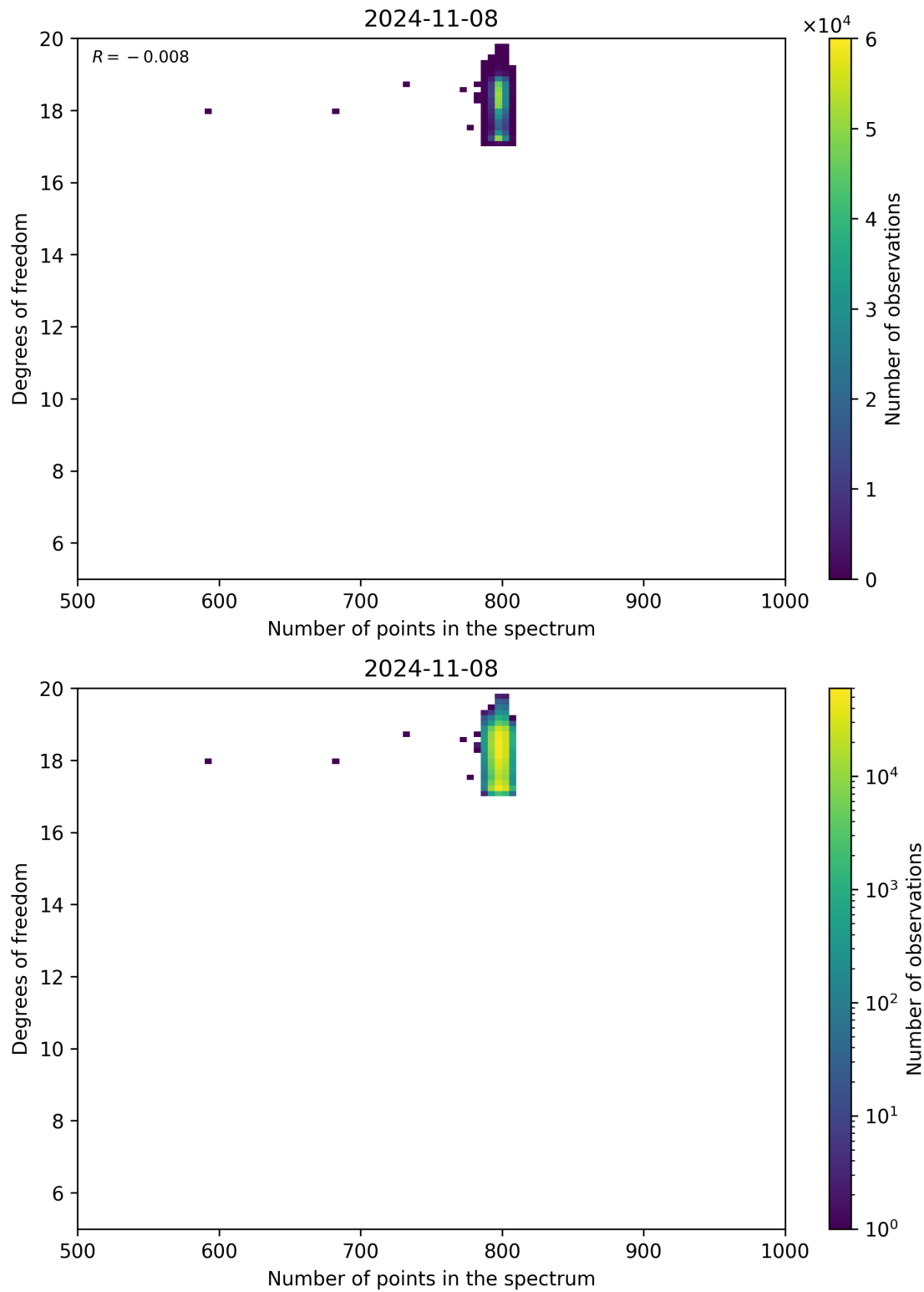
Figure 90: Scatter density plot of “Number of points in the spectrum” against “Degrees of freedom” for 2024-11-07 to 2024-11-09.
