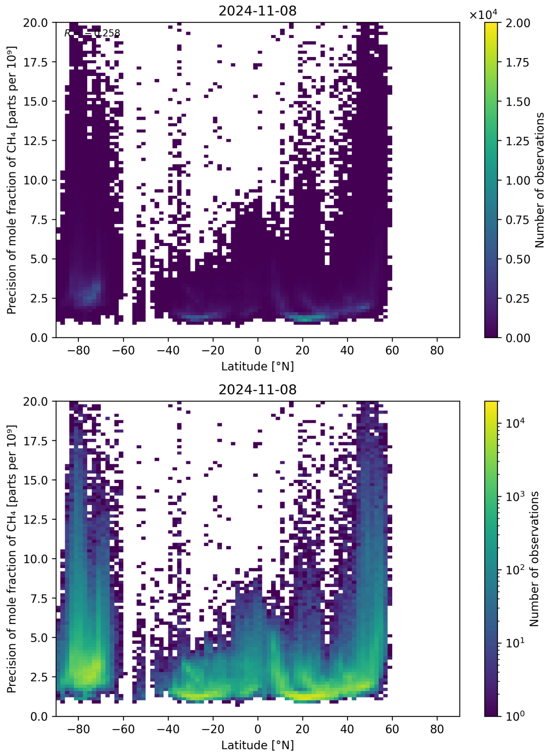
Figure 59: Scatter density plot of “Latitude” against “Precision of mole fraction of CH 4 ” for 2024-11-07 to 2024-11-09.
