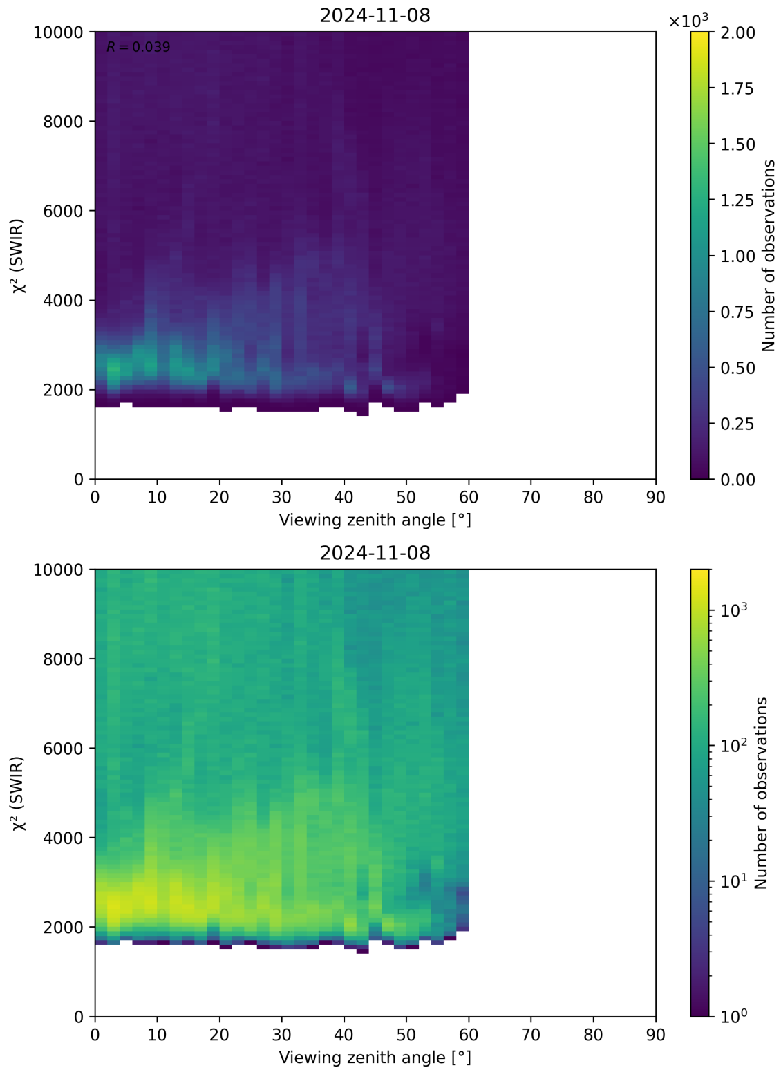
Figure 106: Scatter density plot of “Viewing zenith angle” against “ \chi^2 (SWIR)” for 2024-11-07 to 2024-11-09.
