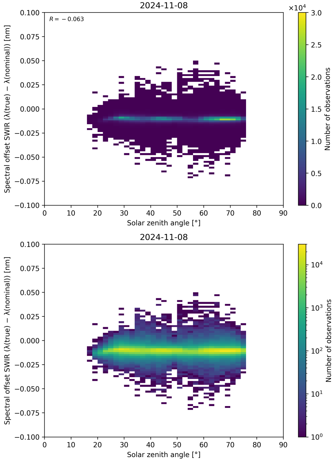
Figure 104: Scatter density plot of “Solar zenith angle” against “Spectral offset SWIR ( \lambda_{\text{true}} - \lambda_{\text{nominal}} )” for 2024-11-07 to 2024-11-09.
