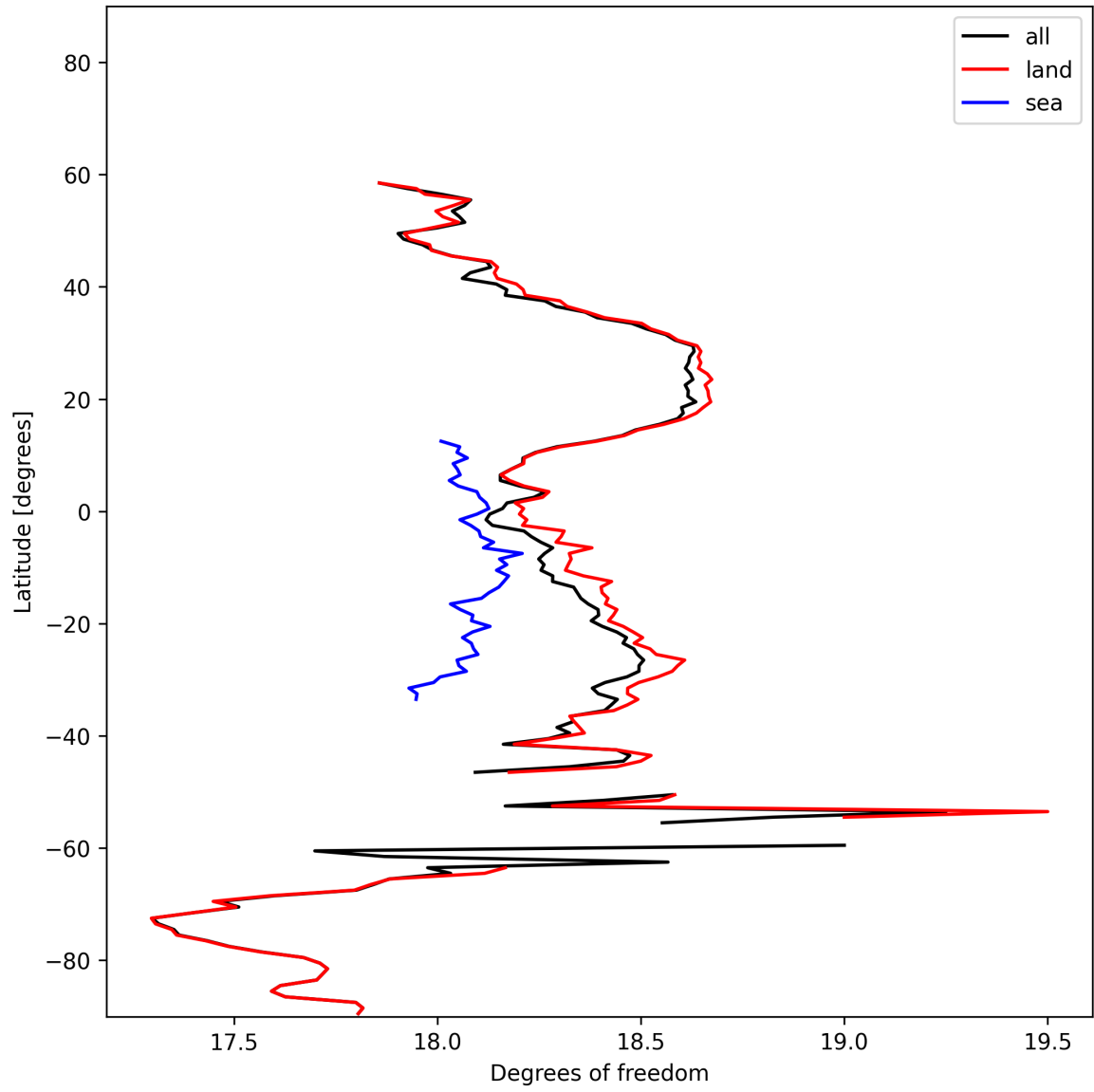
Figure 19: Zonal average of “Degrees of freedom” for 2024-11-07 to 2024-11-09.
