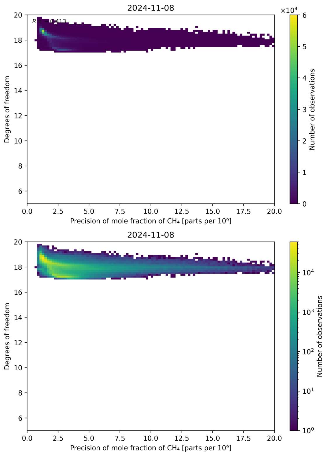
Figure 80: Scatter density plot of “Precision of mole fraction of CH 4 ” against “Degrees of freedom” for 2024-11-07 to 2024-11-09.
