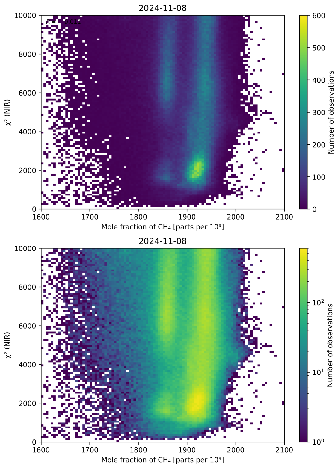
Figure 70: Scatter density plot of “Mole fraction of \text{CH}_4 ” against “ \chi^2 (NIR)” for 2024-11-07 to 2024-11-09.
