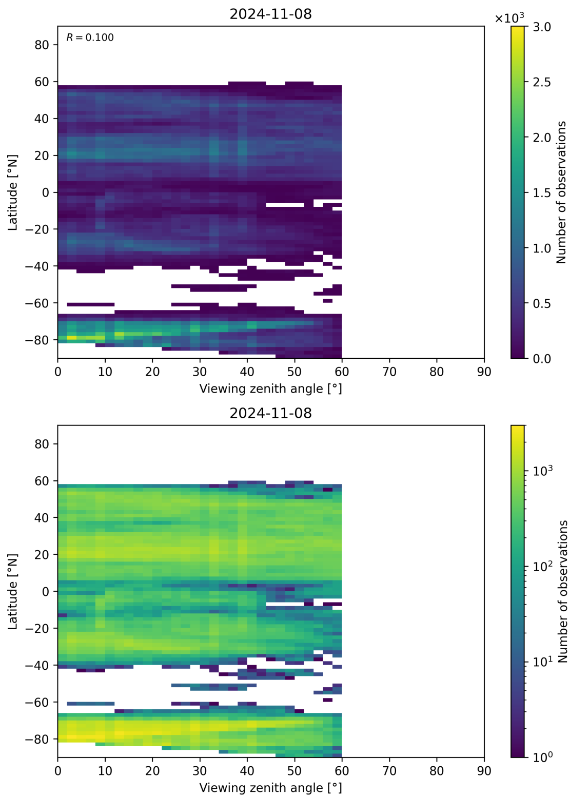
Figure 109: Scatter density plot of “Viewing zenith angle” against “Latitude” for 2024-11-07 to 2024-11-09.
