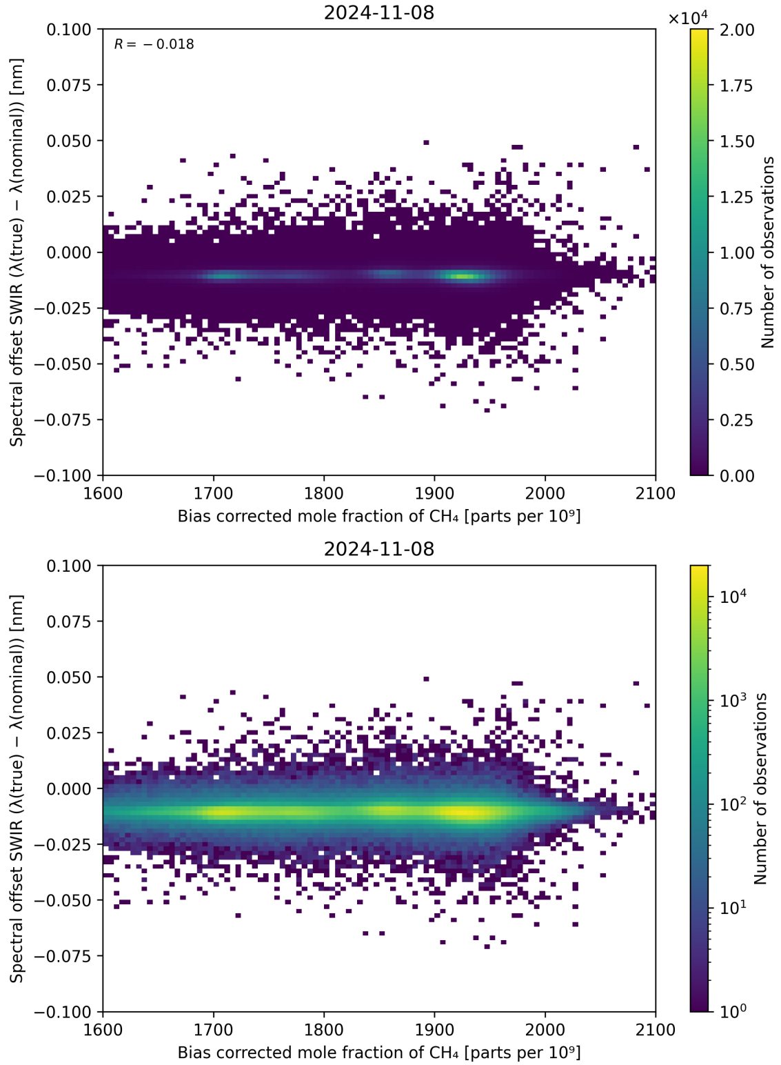
Figure 69: Scatter density plot of “Bias corrected mole fraction of CH 4 ” against “Spectral offset SWIR ( \lambda_{\text{true}} - \lambda_{\text{nominal}} )” for 2024-11-07 to 2024-11-09.
