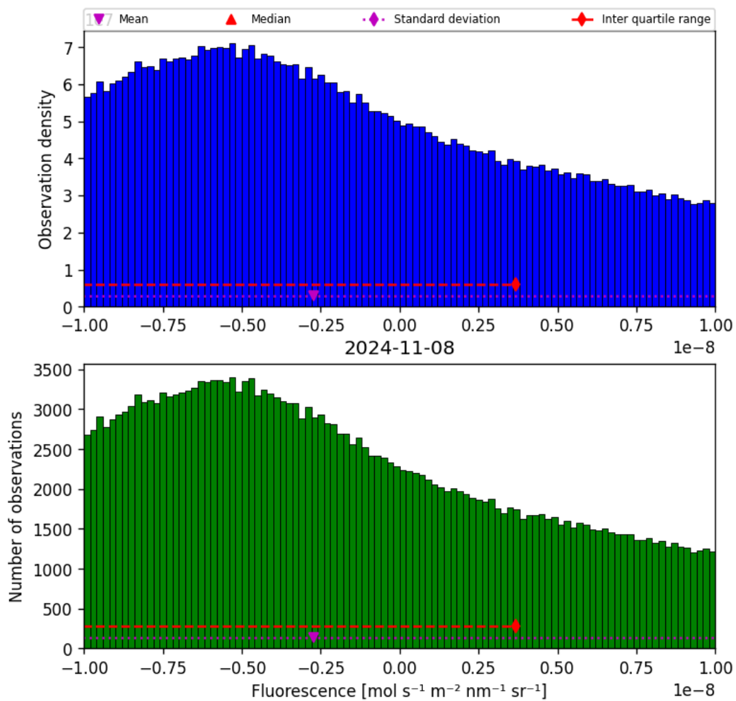
Figure 32: Histogram of “Fluorescence” for 2024-11-07 to 2024-11-09
