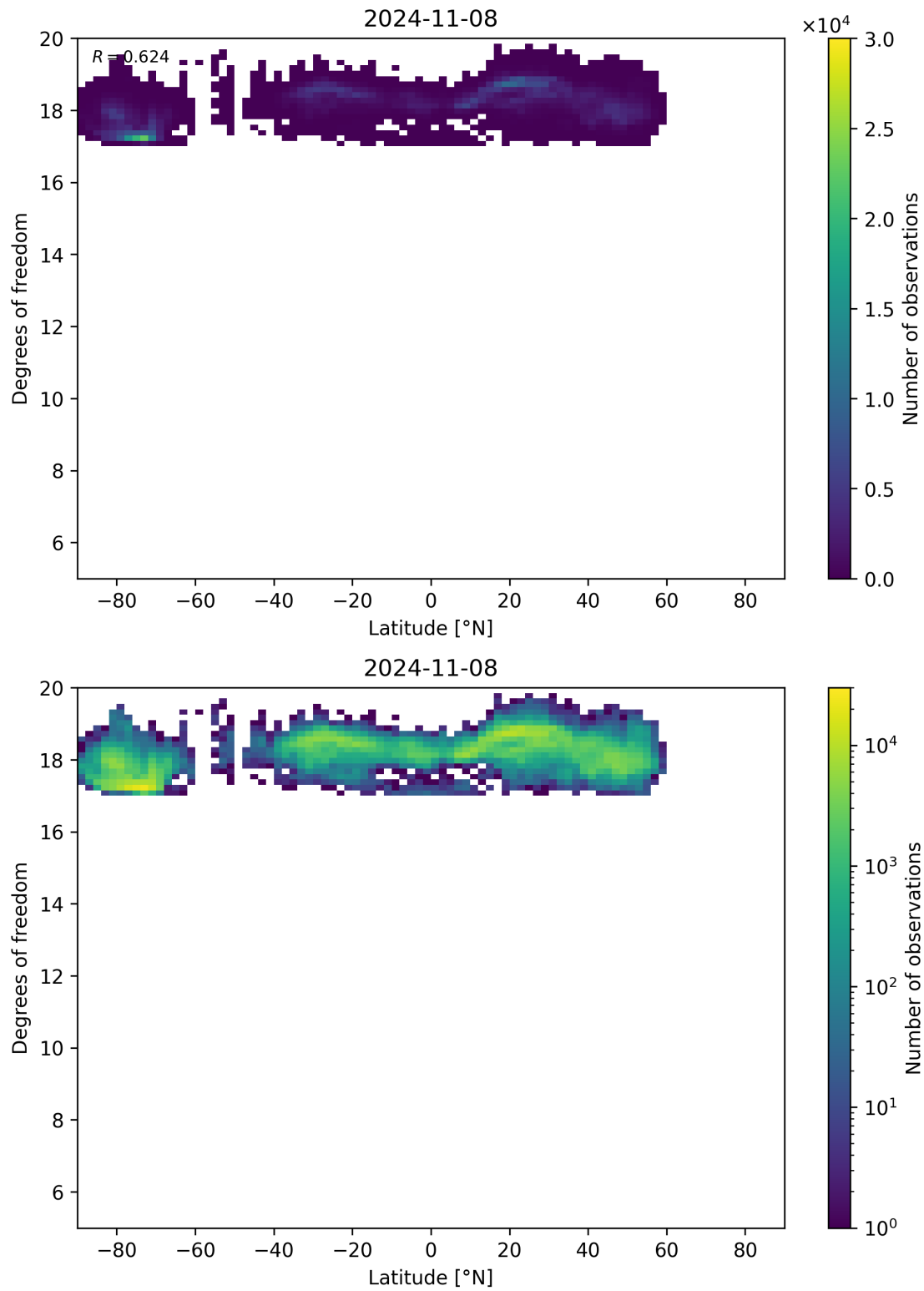
Figure 55: Scatter density plot of “Latitude” against “Degrees of freedom” for 2024-11-07 to 2024-11-09.
