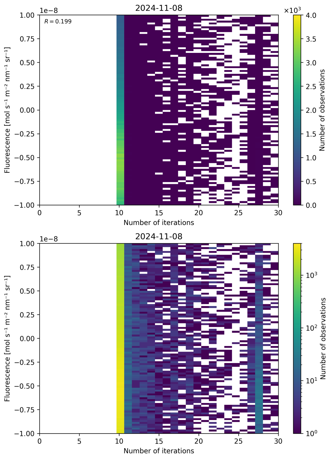
Figure 87: Scatter density plot of “Number of iterations” against “Fluorescence” for 2024-11-07 to 2024-11-09.
