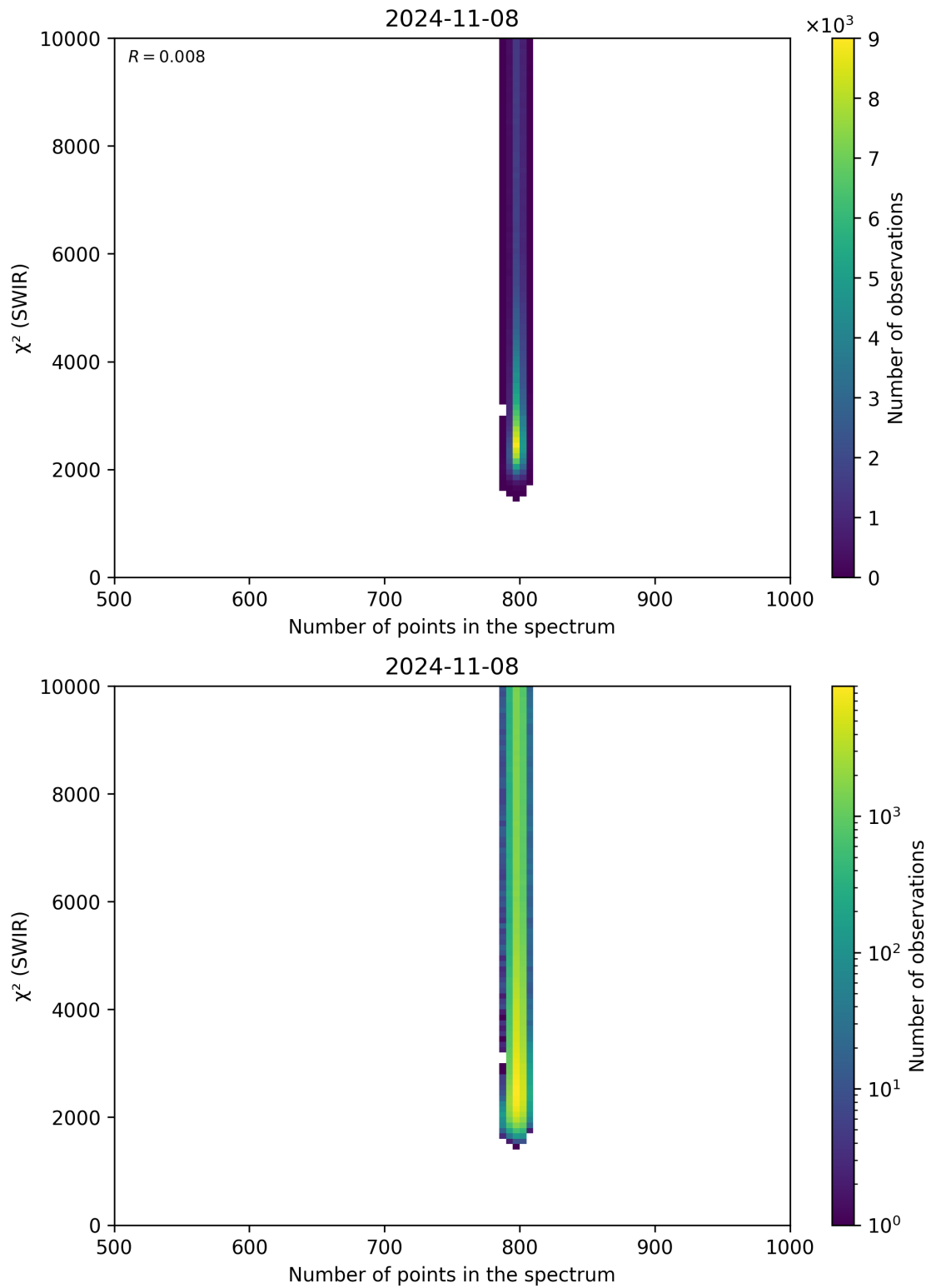
Figure 89: Scatter density plot of “Number of points in the spectrum” against “ \chi^2 (SWIR)” for 2024-11-07 to 2024-11-09.
