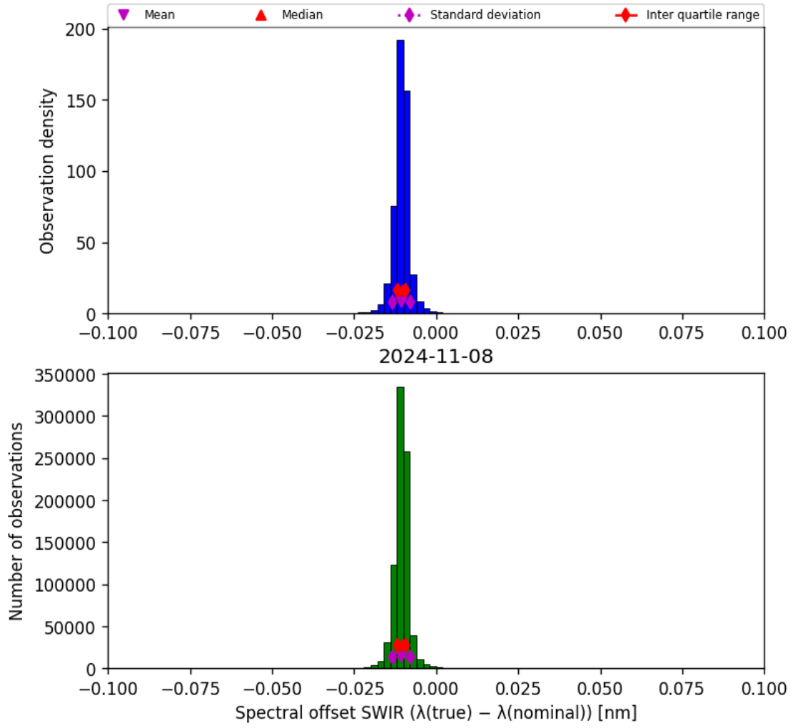
Figure 27: Histogram of “Spectral offset SWIR ( \lambda_{\text{true}} - \lambda_{\text{nominal}} )” for 2024-11-07 to 2024-11-09
