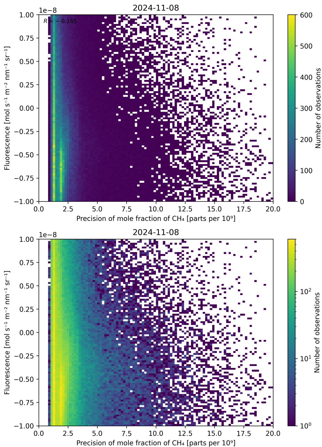
Figure 81: Scatter density plot of “Precision of mole fraction of \text{CH}_4 ” against “Fluorescence” for 2024-11-07 to 2024-11-09.
