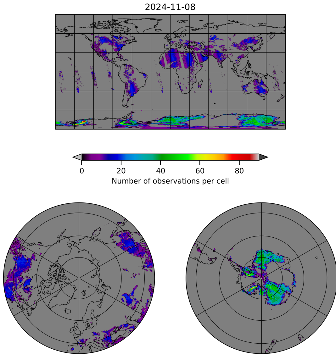
Figure 10: Map of the number of observations for 2024-11-07 to 2024-11-09
