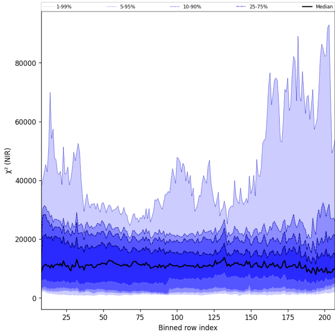
Figure 40: Along track statistics of “ \chi^2 (NIR)” for 2024-11-07 to 2024-11-09
