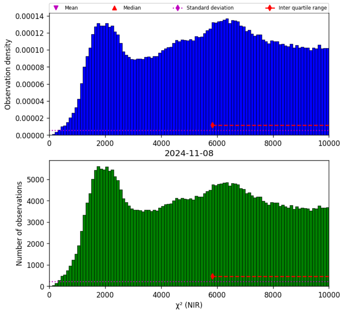
Figure 29: Histogram of “ \chi^2 (NIR)” for 2024-11-07 to 2024-11-09
