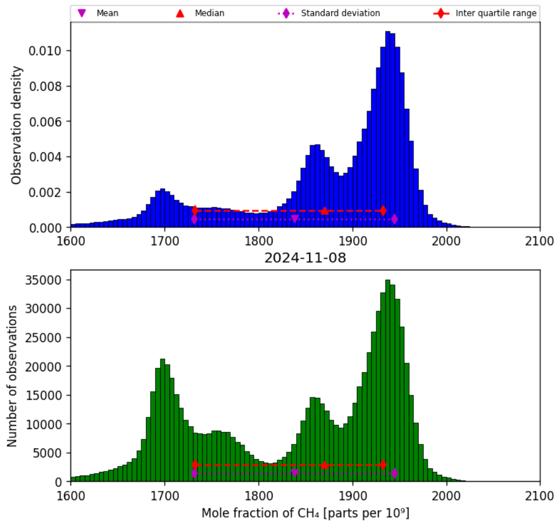
Figure 23: Histogram of “Mole fraction of CH 4 ” for 2024-11-07 to 2024-11-09
