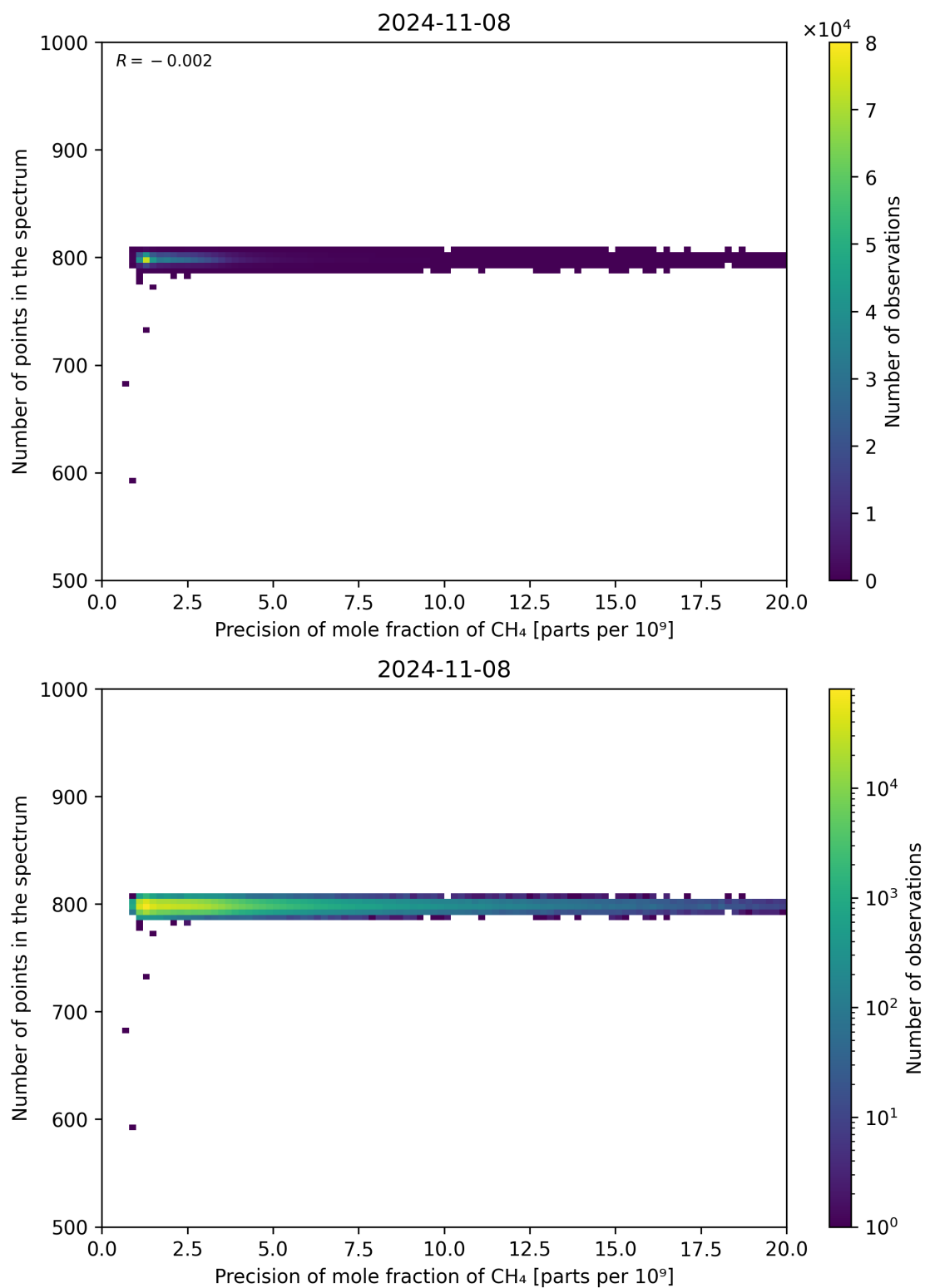
Figure 84: Scatter density plot of “Precision of mole fraction of CH 4 ” against “Number of points in the spectrum” for 2024-11-07 to 2024-11-09.
