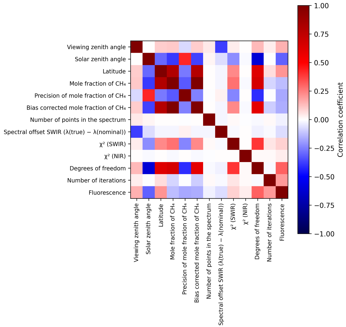
Figure 2: Map of correlation matrix for 2024-11-07 to 2024-11-09.
