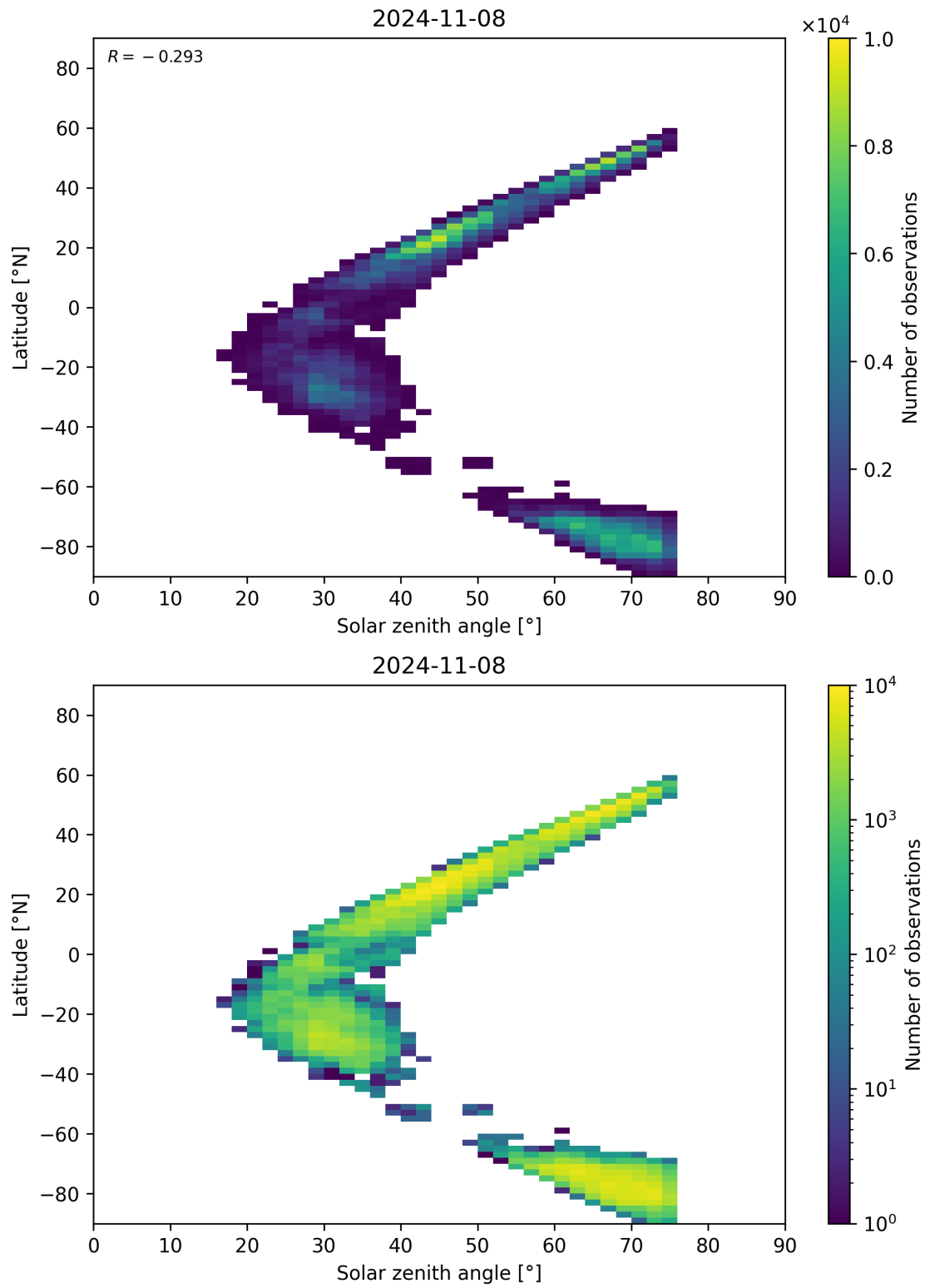
Figure 98: Scatter density plot of “Solar zenith angle” against “Latitude” for 2024-11-07 to 2024-11-09.
