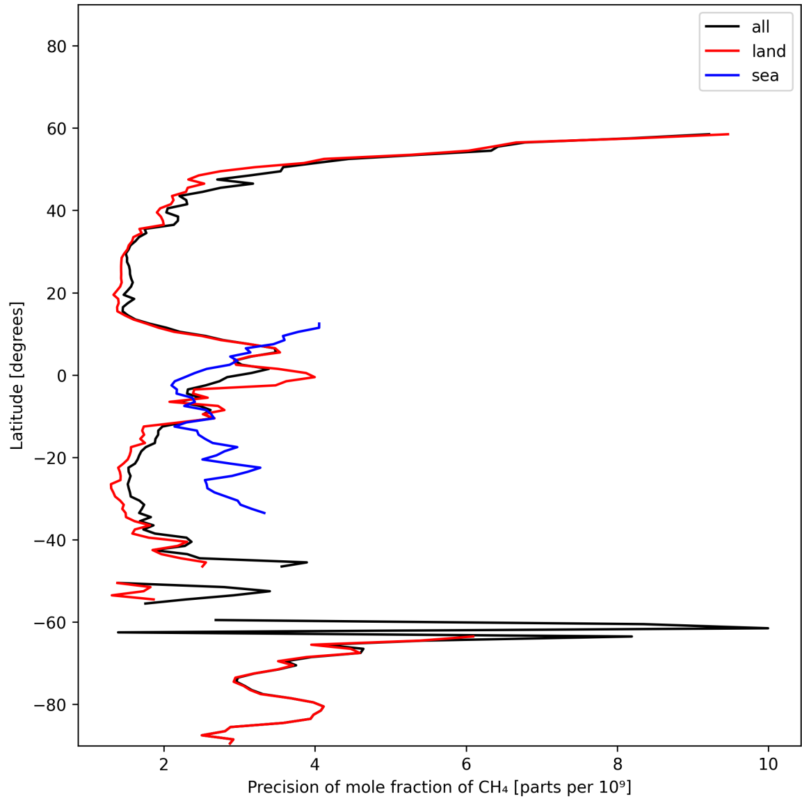
Figure 13: Zonal average of “Precision of mole fraction of CH 4 ” for 2024-11-07 to 2024-11-09.
