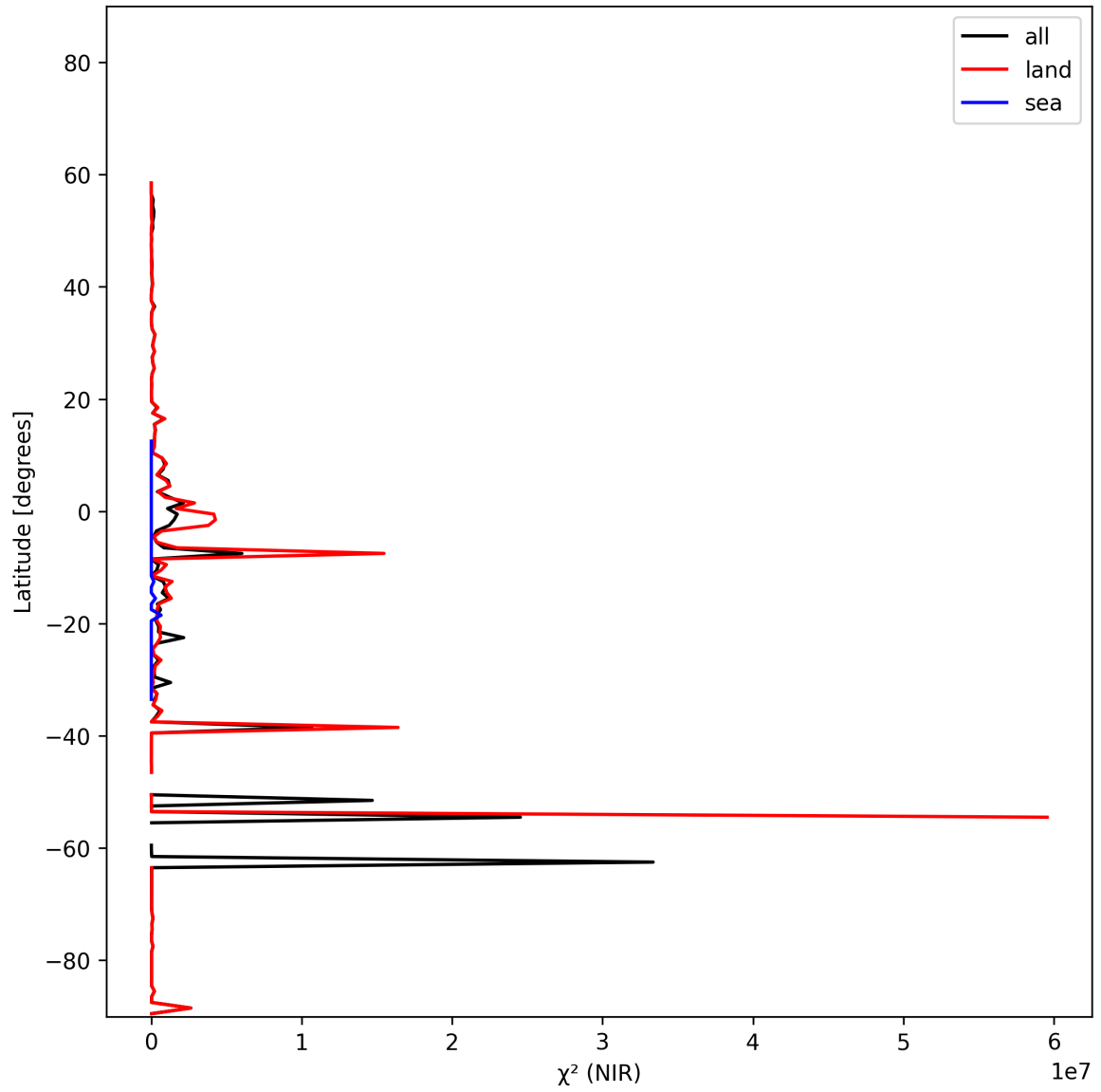
Figure 18: Zonal average of “ \chi^2 (NIR)” for 2024-11-07 to 2024-11-09.
