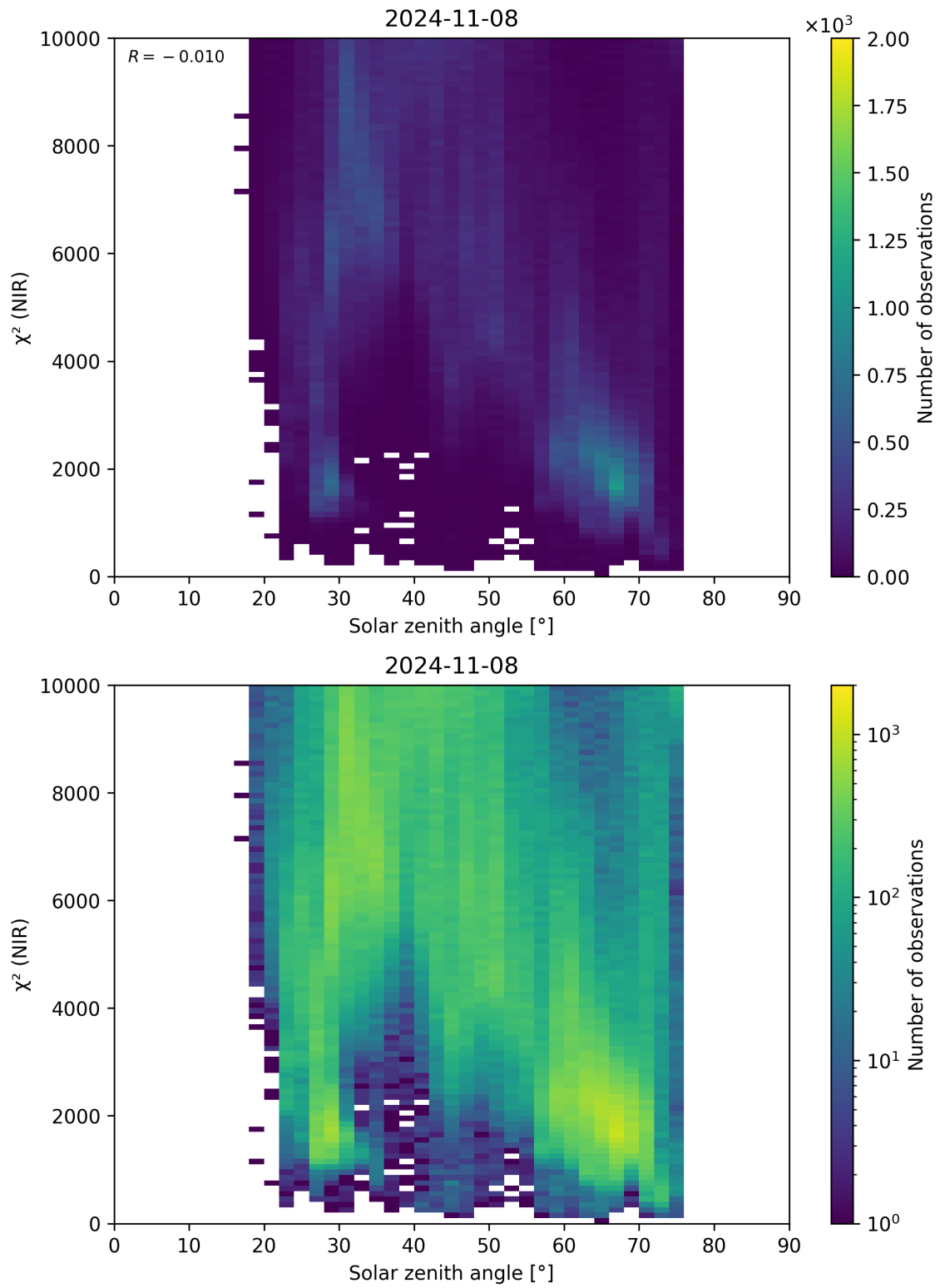
Figure 94: Scatter density plot of “Solar zenith angle” against “ \chi^2 (NIR)” for 2024-11-07 to 2024-11-09.
