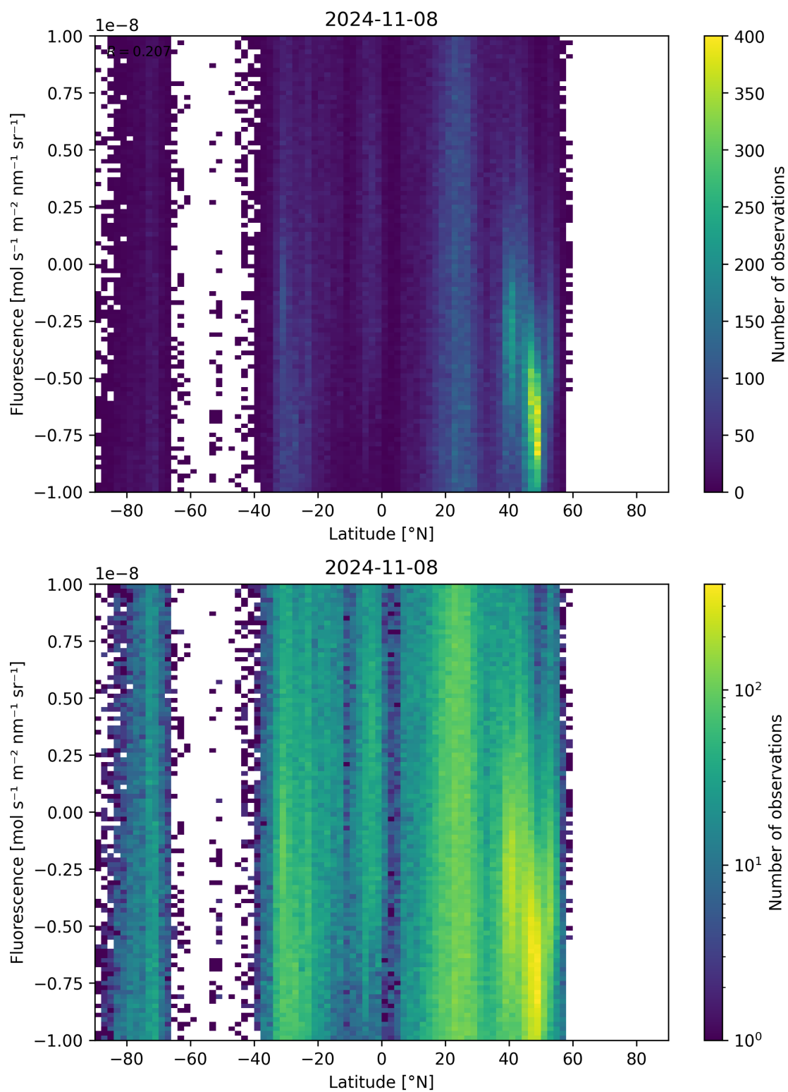
Figure 56: Scatter density plot of “Latitude” against “Fluorescence” for 2024-11-07 to 2024-11-09.
