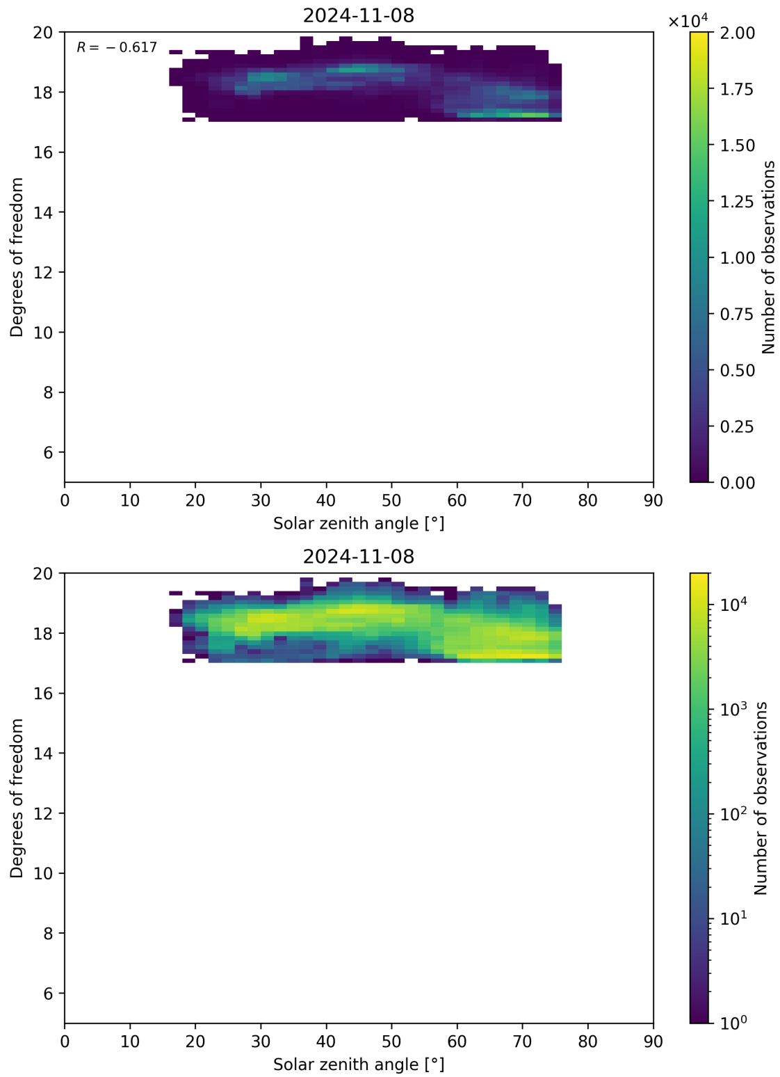
Figure 96: Scatter density plot of “Solar zenith angle” against “Degrees of freedom” for 2024-11-07 to 2024-11-09.
