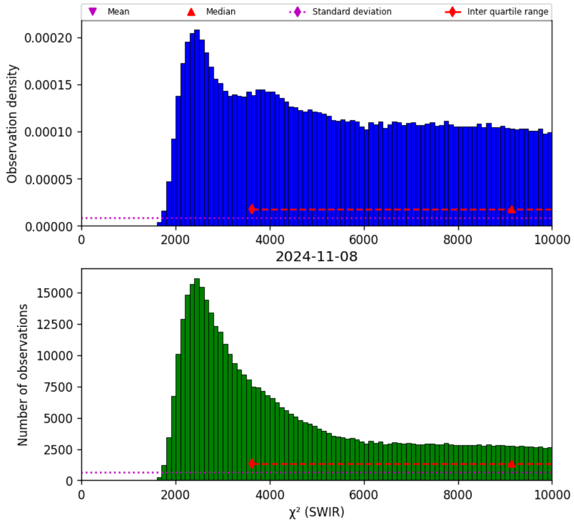
Figure 28: Histogram of “ \chi^2 (SWIR)” for 2024-11-07 to 2024-11-09
