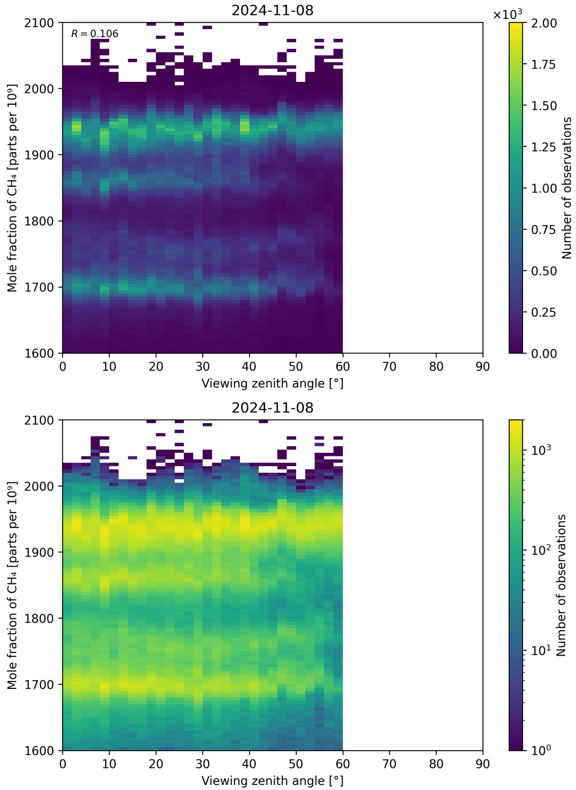
Figure 110: Scatter density plot of “Viewing zenith angle” against “Mole fraction of CH 4 ” for 2024-11-07 to 2024-11-09.
