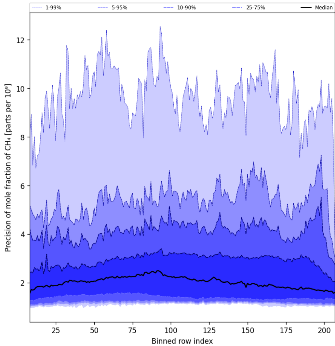
Figure 35: Along track statistics of “Precision of mole fraction of CH 4 ” for 2024-11-07 to 2024-11-09
