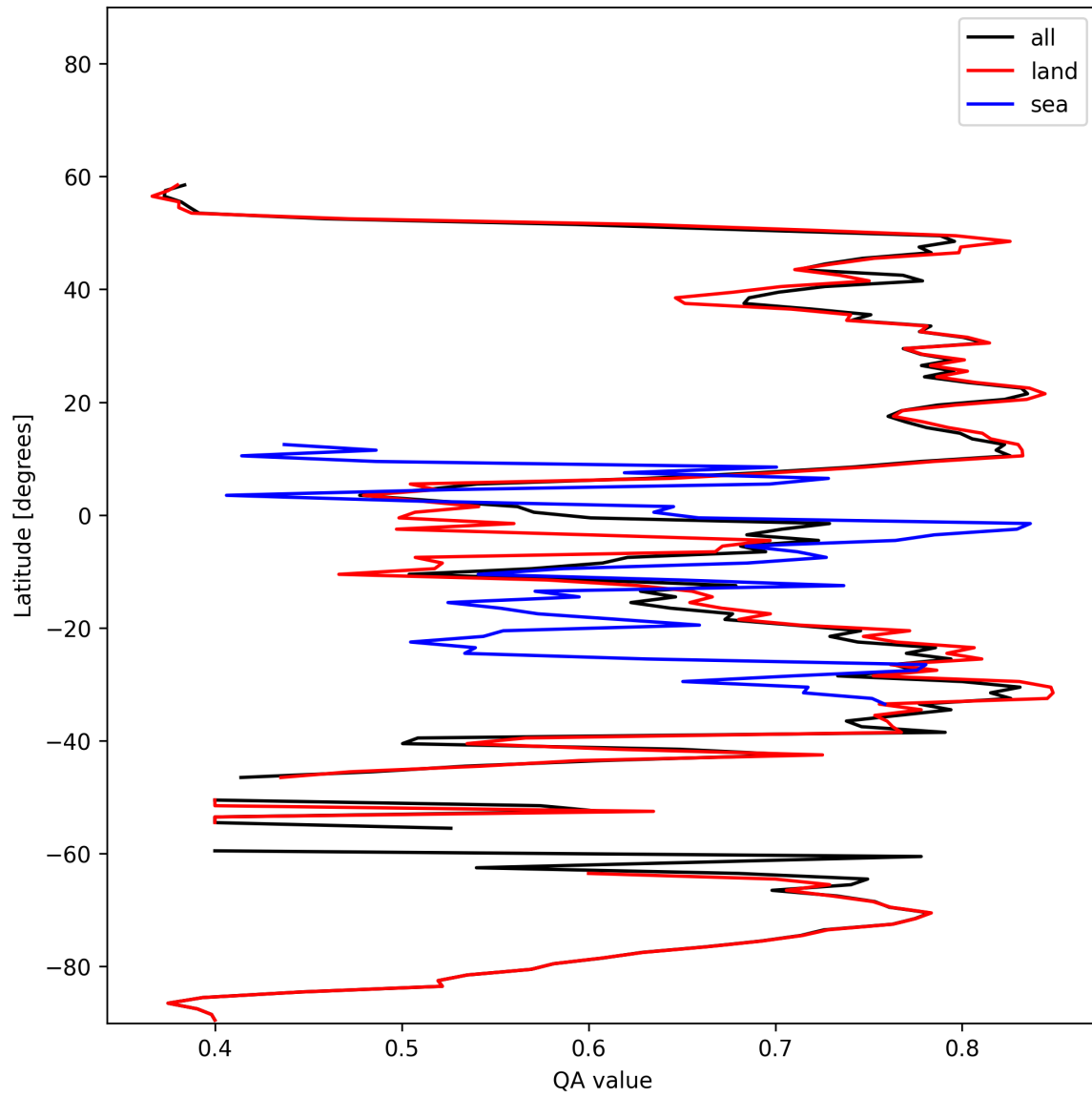
Figure 11: Zonal average of “QA value” for 2024-11-07 to 2024-11-09.
