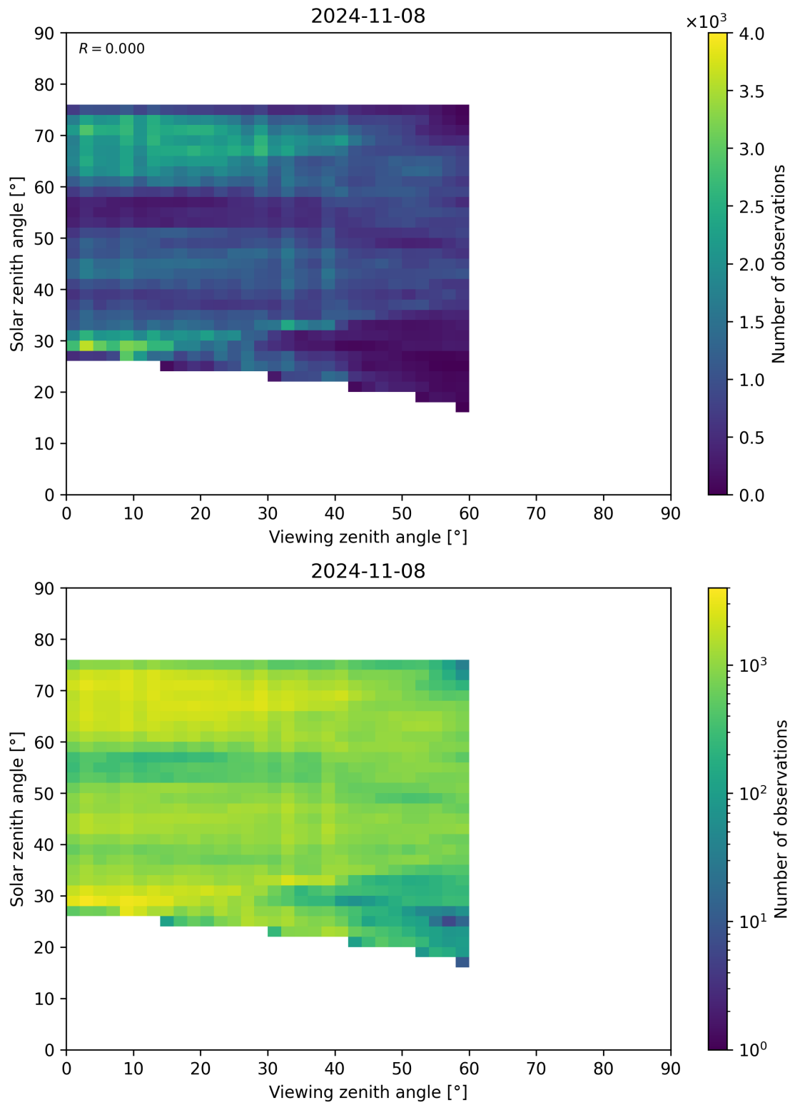
Figure 115: Scatter density plot of “Viewing zenith angle” against “Solar zenith angle” for 2024-11-07 to 2024-11-09.
