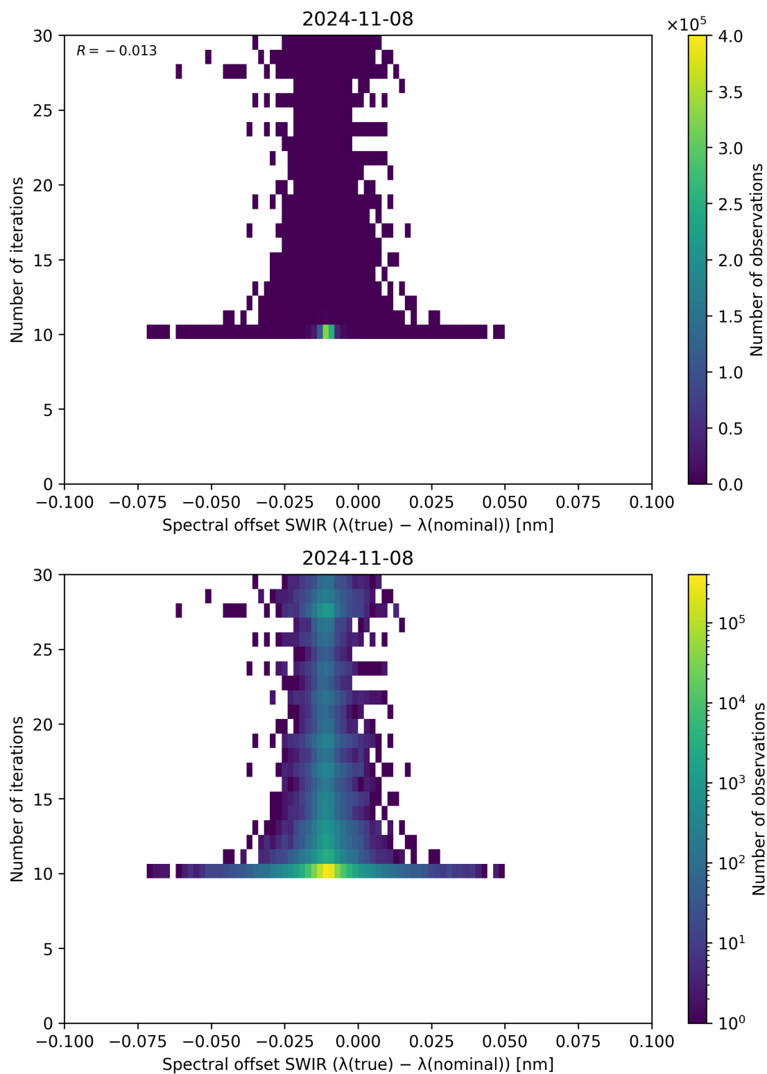
Figure 121: Scatter density plot of “Spectral offset SWIR ( \lambda_{\text{true}} - \lambda_{\text{nominal}} )” against “Number of iterations” for 2024-11-07 to 2024-11-09.
