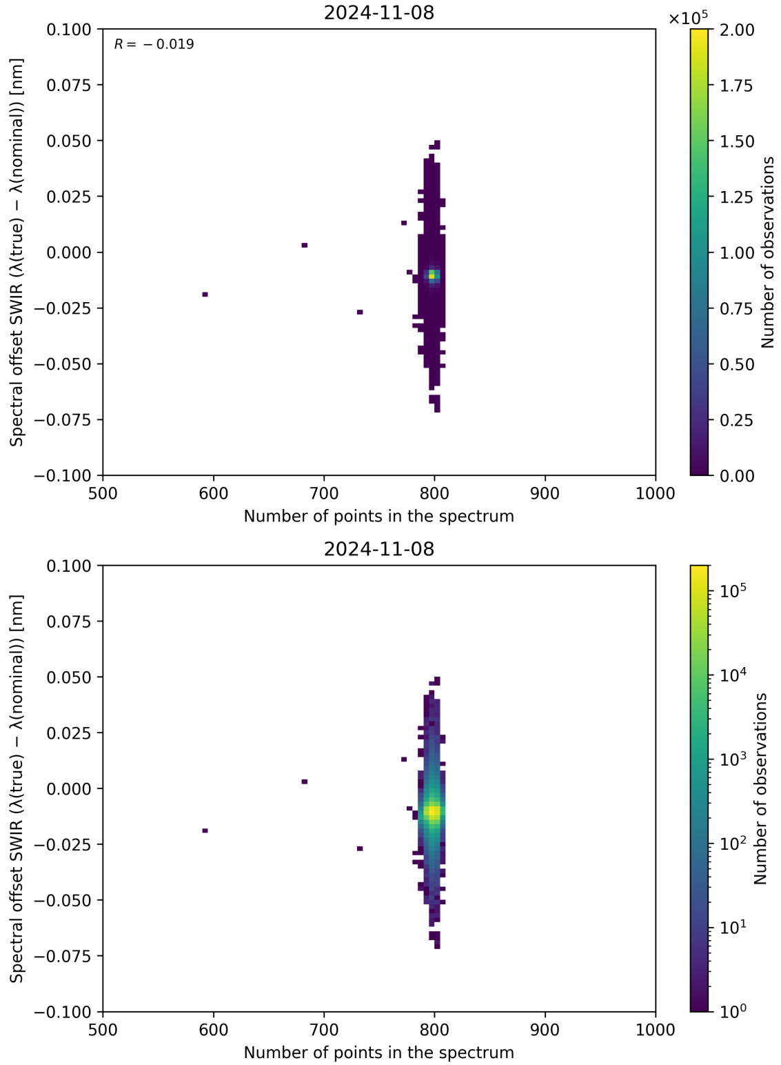
Figure 93: Scatter density plot of “Number of points in the spectrum” against “Spectral offset SWIR ( \lambda_{\text{true}} - \lambda_{\text{nominal}} )” for 2024-11-07 to 2024-11-09.
