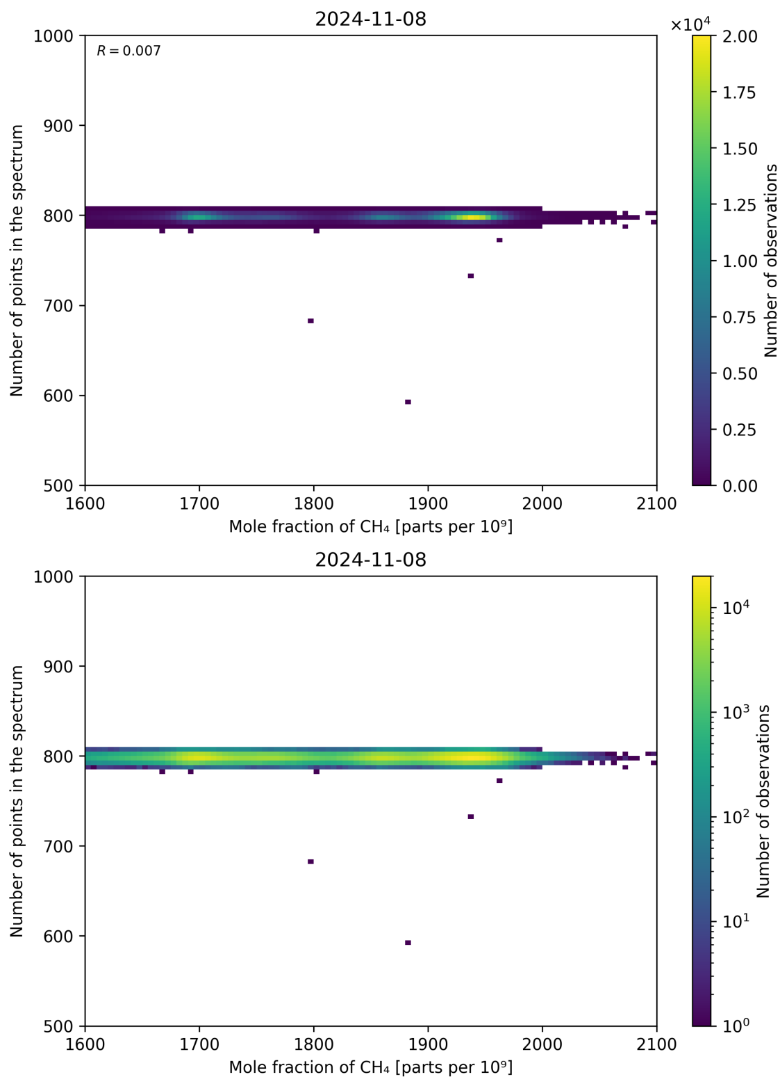
Figure 77: Scatter density plot of “Mole fraction of CH 4 ” against “Number of points in the spectrum” for 2024-11-07 to 2024-11-09.
