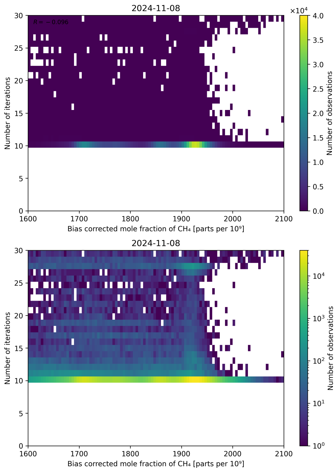
Figure 67: Scatter density plot of “Bias corrected mole fraction of \text{CH}_4 ” against “Number of iterations” for 2024-11-07 to 2024-11-09.
