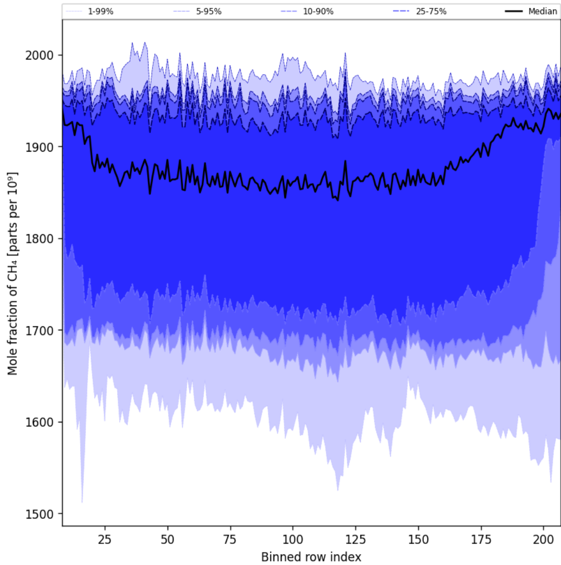
Figure 34: Along track statistics of “Mole fraction of CH 4 ” for 2024-11-07 to 2024-11-09
