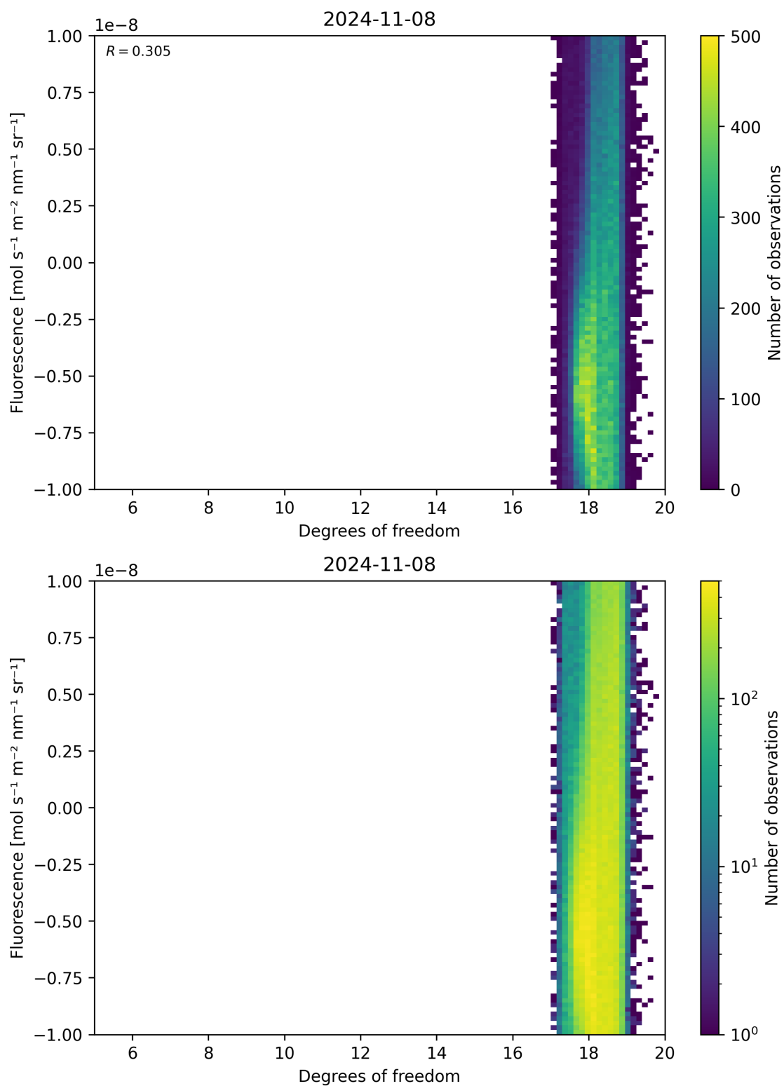
Figure 51: Scatter density plot of “Degrees of freedom” against “Fluorescence” for 2024-11-07 to 2024-11-09.
