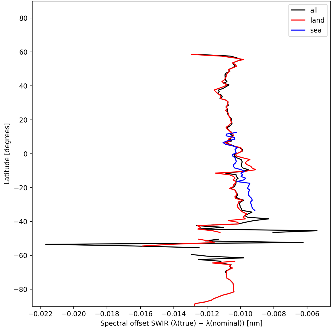
Figure 16: Zonal average of “Spectral offset SWIR ( \lambda_{\text{true}} - \lambda_{\text{nominal}} )” for 2024-11-07 to 2024-11-09.
