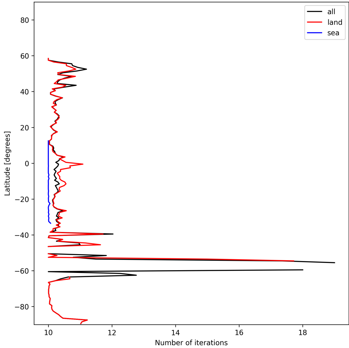
Figure 20: Zonal average of “Number of iterations” for 2024-11-07 to 2024-11-09.
