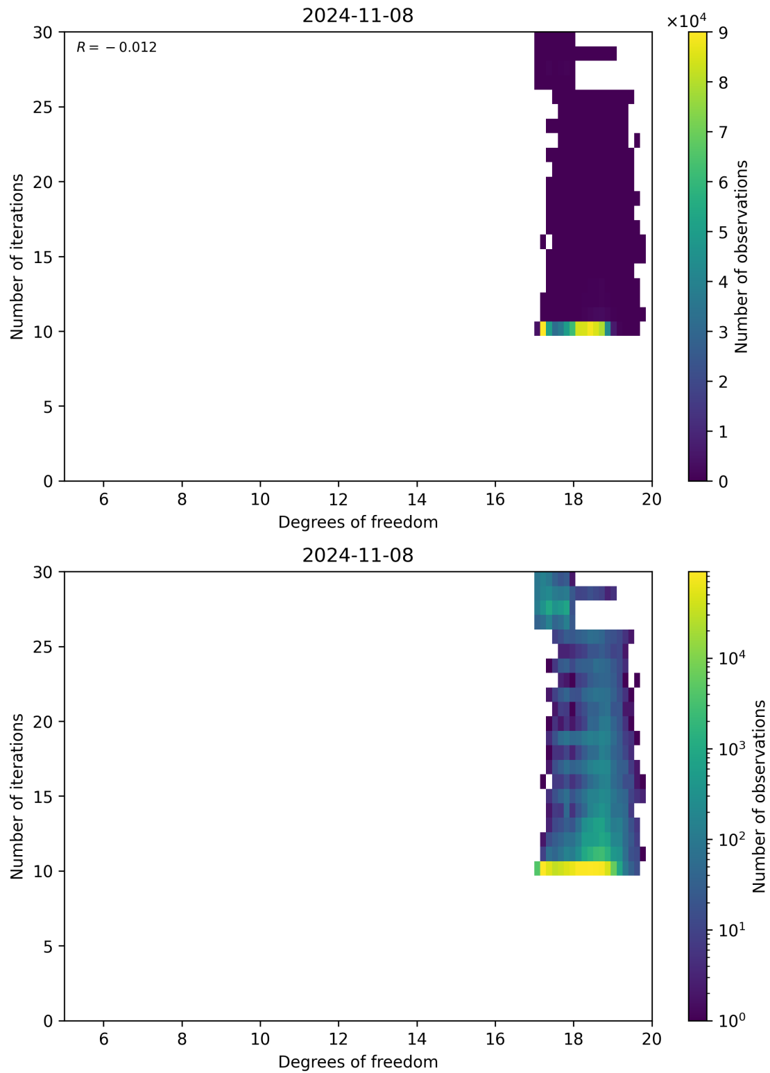
Figure 52: Scatter density plot of “Degrees of freedom” against “Number of iterations” for 2024-11-07 to 2024-11-09.
