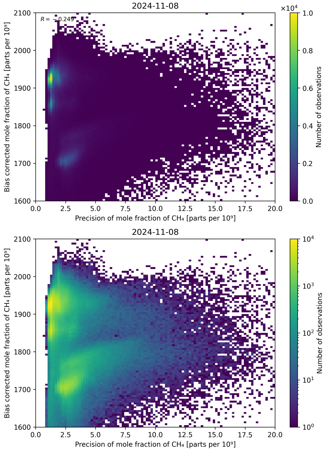
Figure 82: Scatter density plot of “Precision of mole fraction of CH 4 ” against “Bias corrected mole fraction of CH 4 ” for 2024-11-07 to 2024-11-09.
