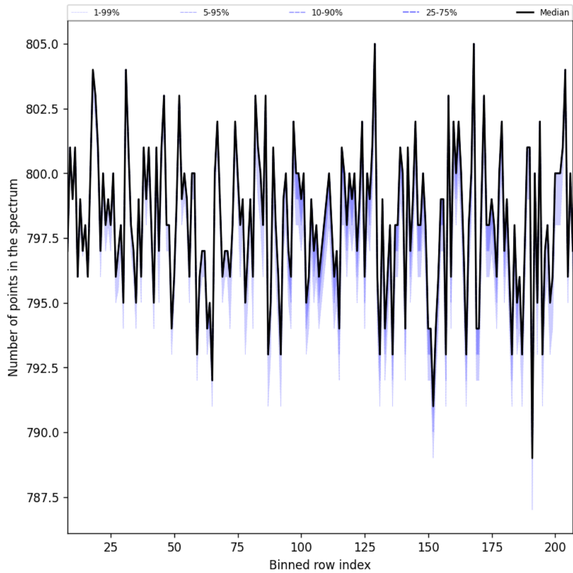
Figure 37: Along track statistics of “Number of points in the spectrum” for 2024-11-07 to 2024-11-09
