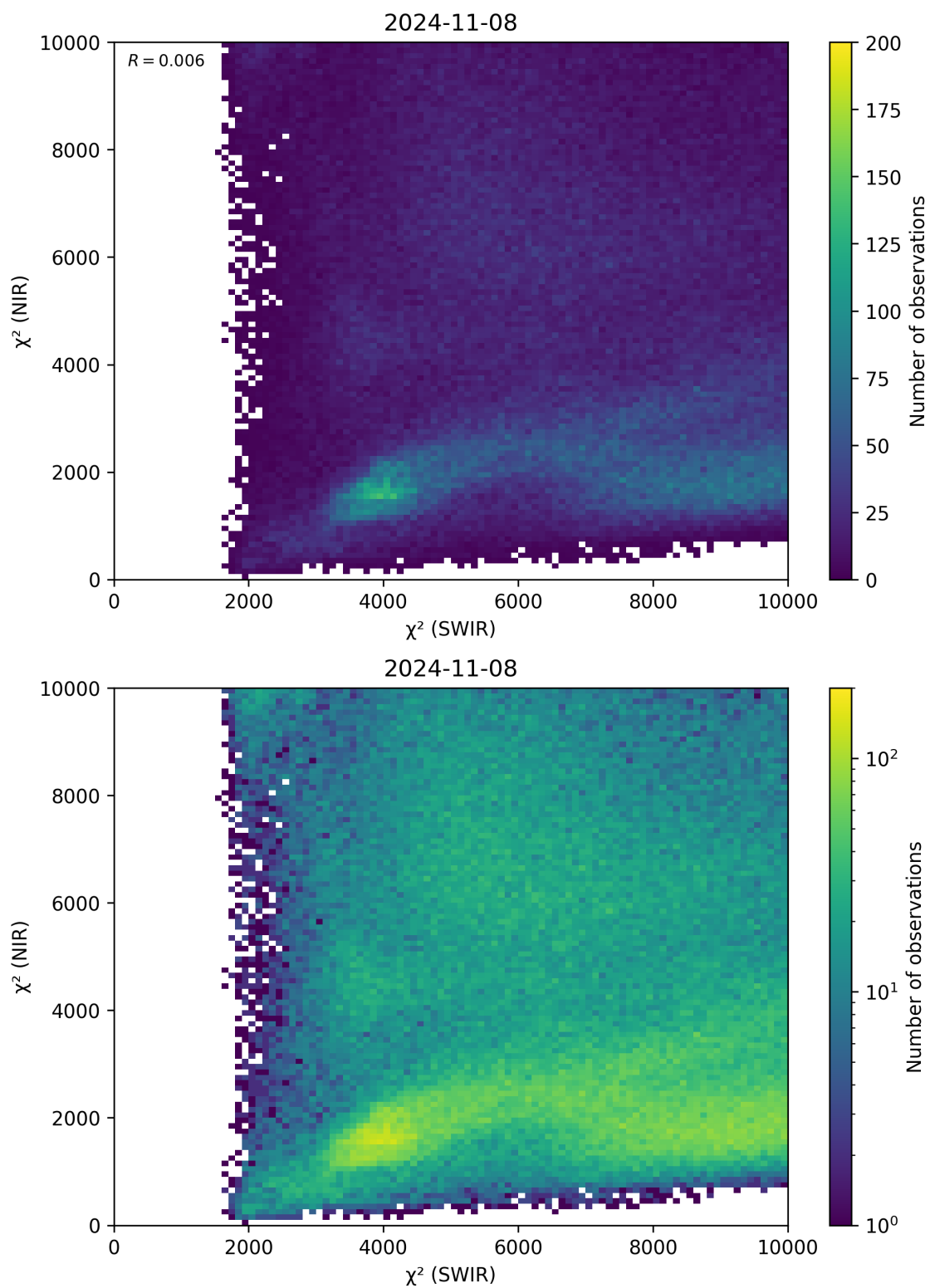
Figure 47: Scatter density plot of “ \chi^2 (SWIR)” against “ \chi^2 (NIR)” for 2024-11-07 to 2024-11-09.
