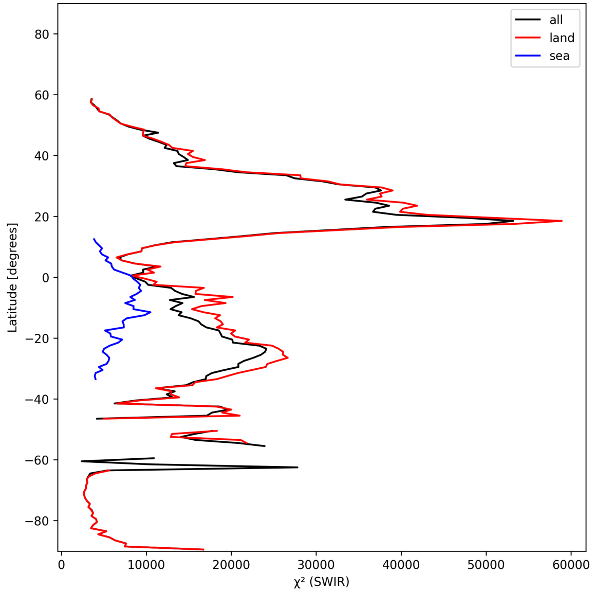
Figure 17: Zonal average of “ \chi^2 (SWIR)” for 2024-11-07 to 2024-11-09.
