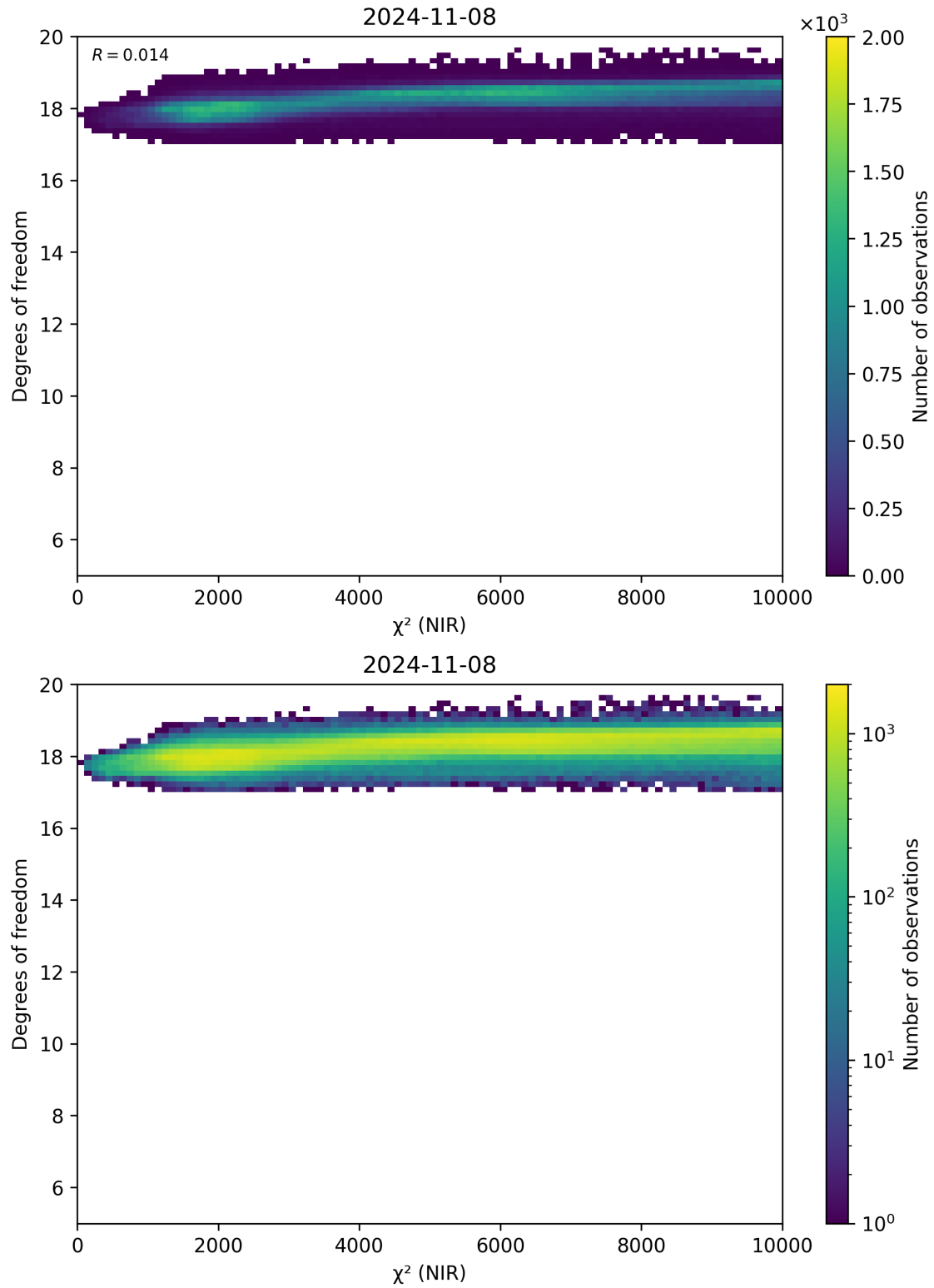
Figure 44: Scatter density plot of “ \chi^2 (NIR)” against “Degrees of freedom” for 2024-11-07 to 2024-11-09.
