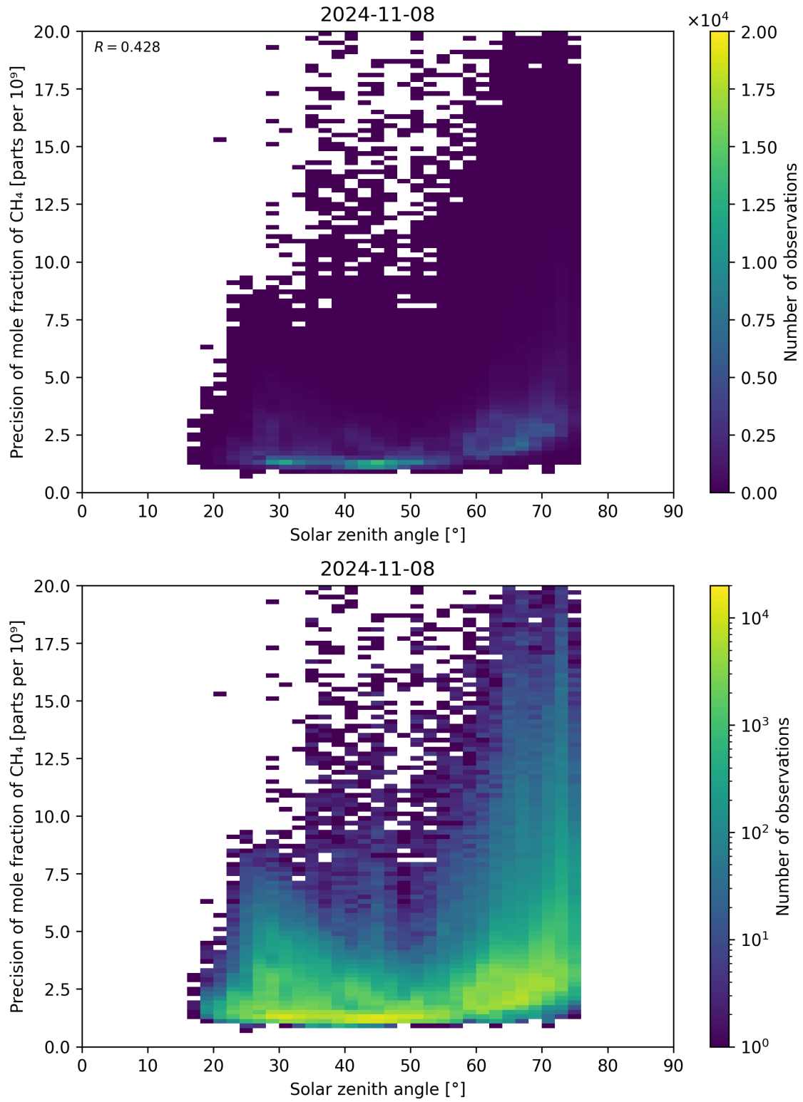
Figure 101: Scatter density plot of “Solar zenith angle” against “Precision of mole fraction of \text{CH}_4 ” for 2024-11-07 to 2024-11-09.
