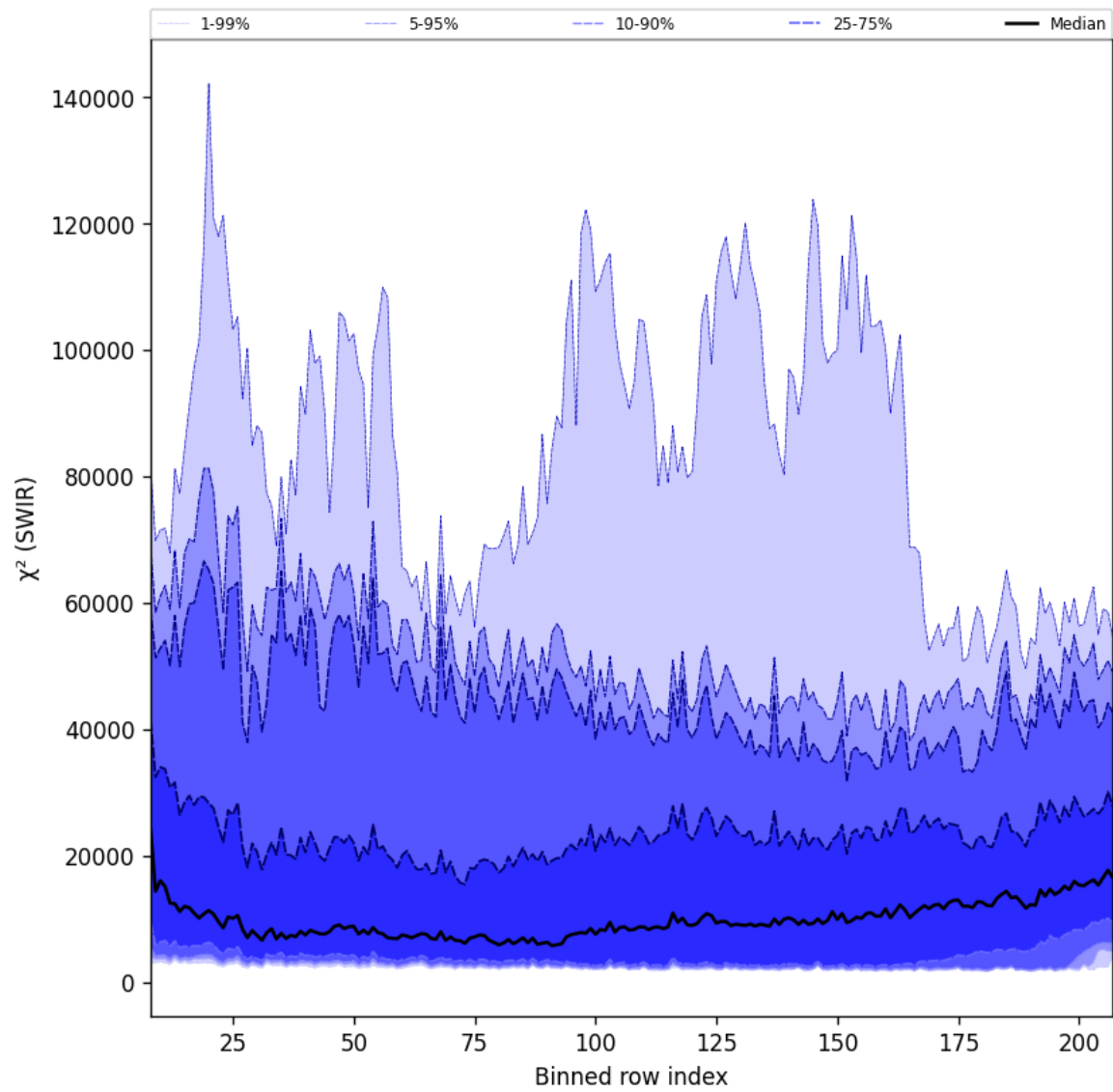
Figure 39: Along track statistics of “ \chi^2 (SWIR)” for 2024-11-07 to 2024-11-09
