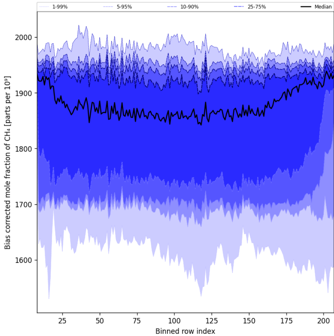
Figure 36: Along track statistics of “Bias corrected mole fraction of CH 4 ” for 2024-11-07 to 2024-11-09
