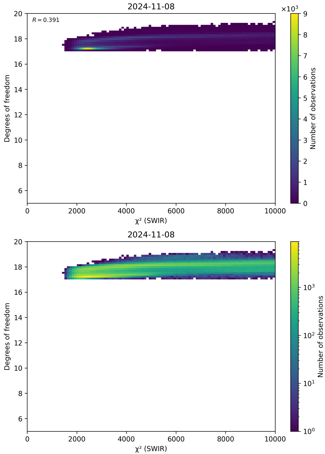
Figure 48: Scatter density plot of “ \chi^2 (SWIR)” against “Degrees of freedom” for 2024-11-07 to 2024-11-09.
