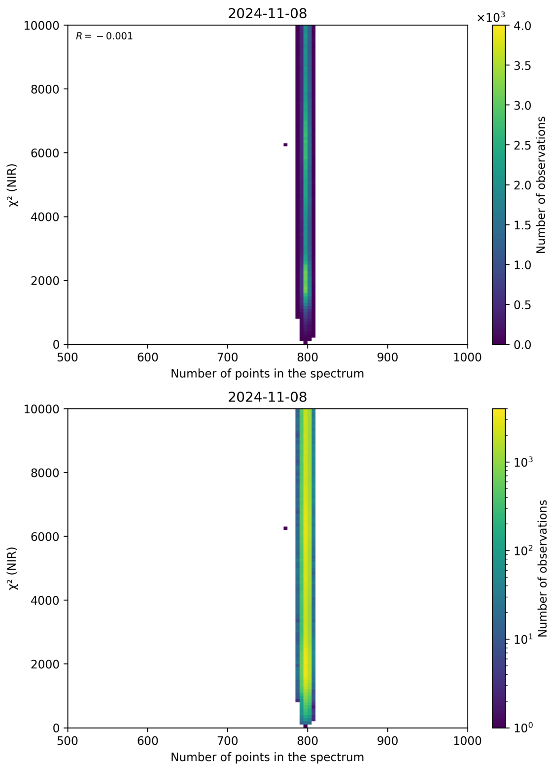
Figure 88: Scatter density plot of “Number of points in the spectrum” against “ \chi^2 (NIR)” for 2024-11-07 to 2024-11-09.
