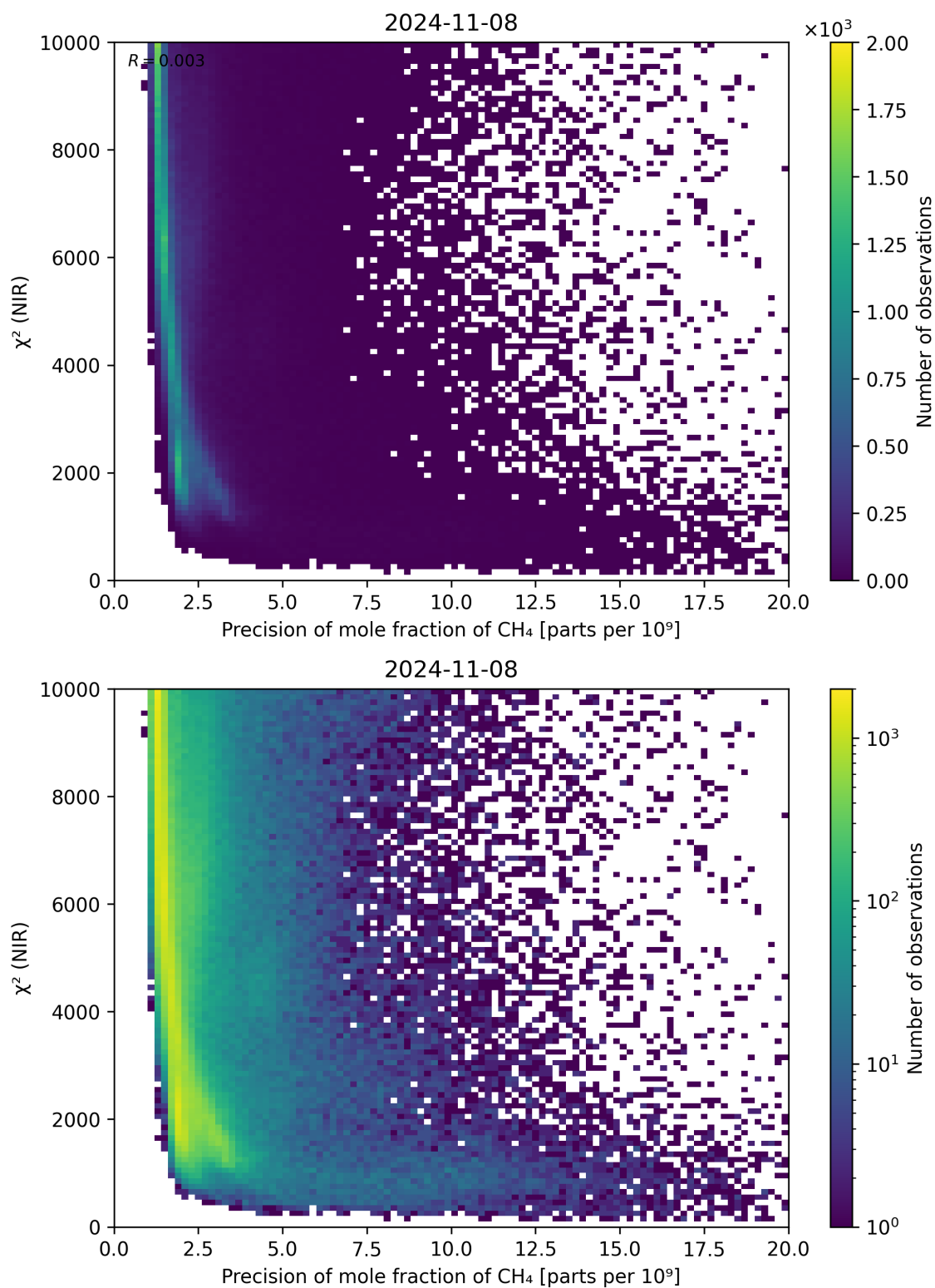
Figure 78: Scatter density plot of “Precision of mole fraction of CH 4 ” against “ \chi^2 (NIR)” for 2024-11-07 to 2024-11-09.
