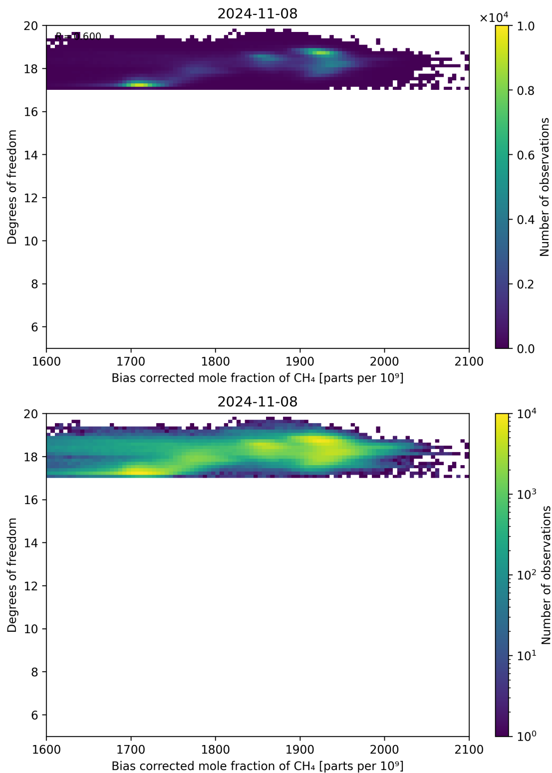
Figure 65: Scatter density plot of “Bias corrected mole fraction of CH 4 ” against “Degrees of freedom” for 2024-11-07 to 2024-11-09.
