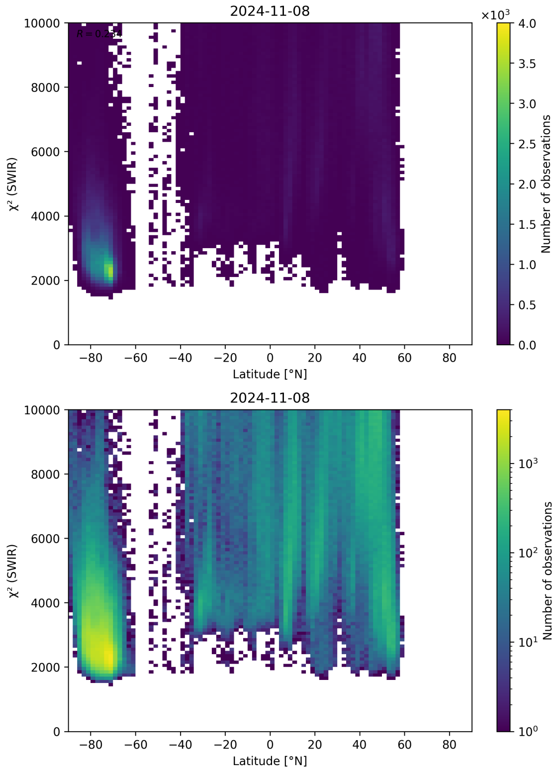
Figure 54: Scatter density plot of “Latitude” against “ \chi^2 (SWIR)” for 2024-11-07 to 2024-11-09.
