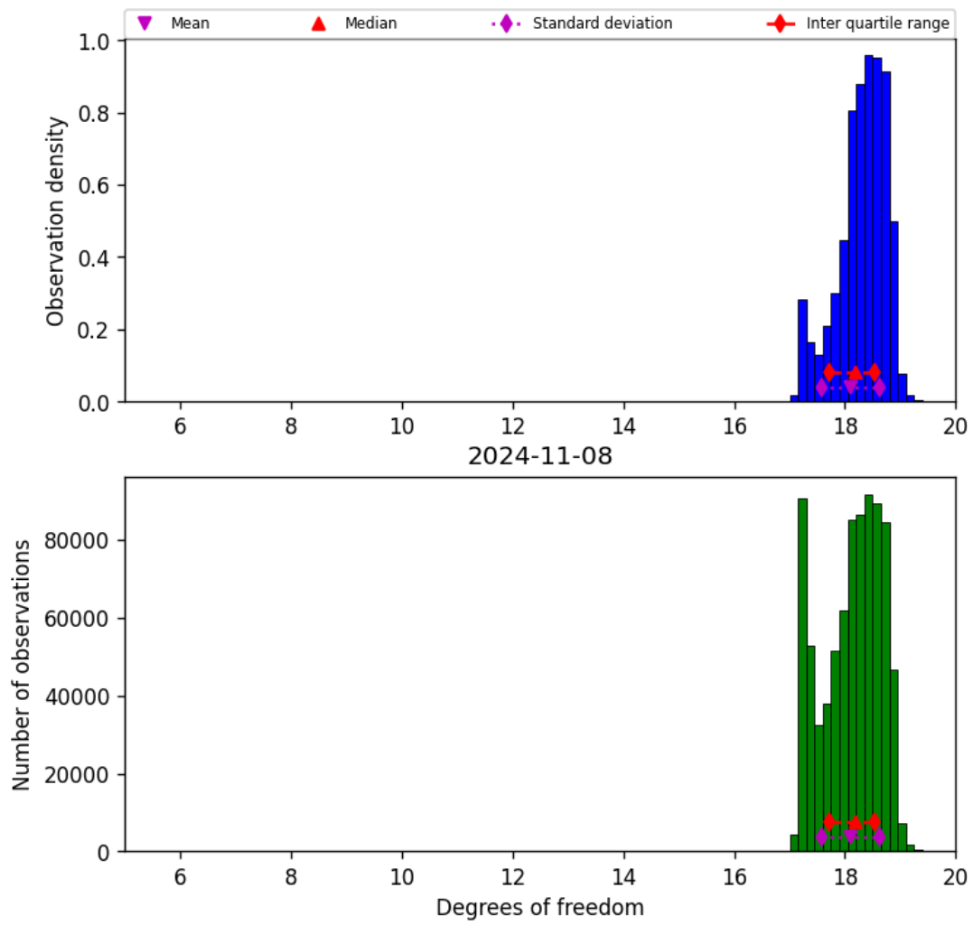
Figure 30: Histogram of “Degrees of freedom” for 2024-11-07 to 2024-11-09
