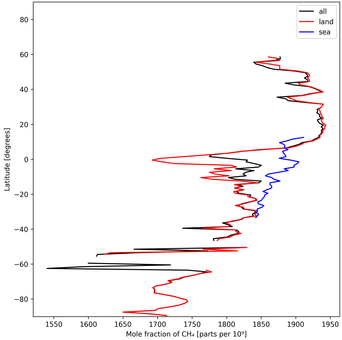
Figure 12: Zonal average of “Mole fraction of \text{CH}_4 ” for 2024-11-07 to 2024-11-09.
