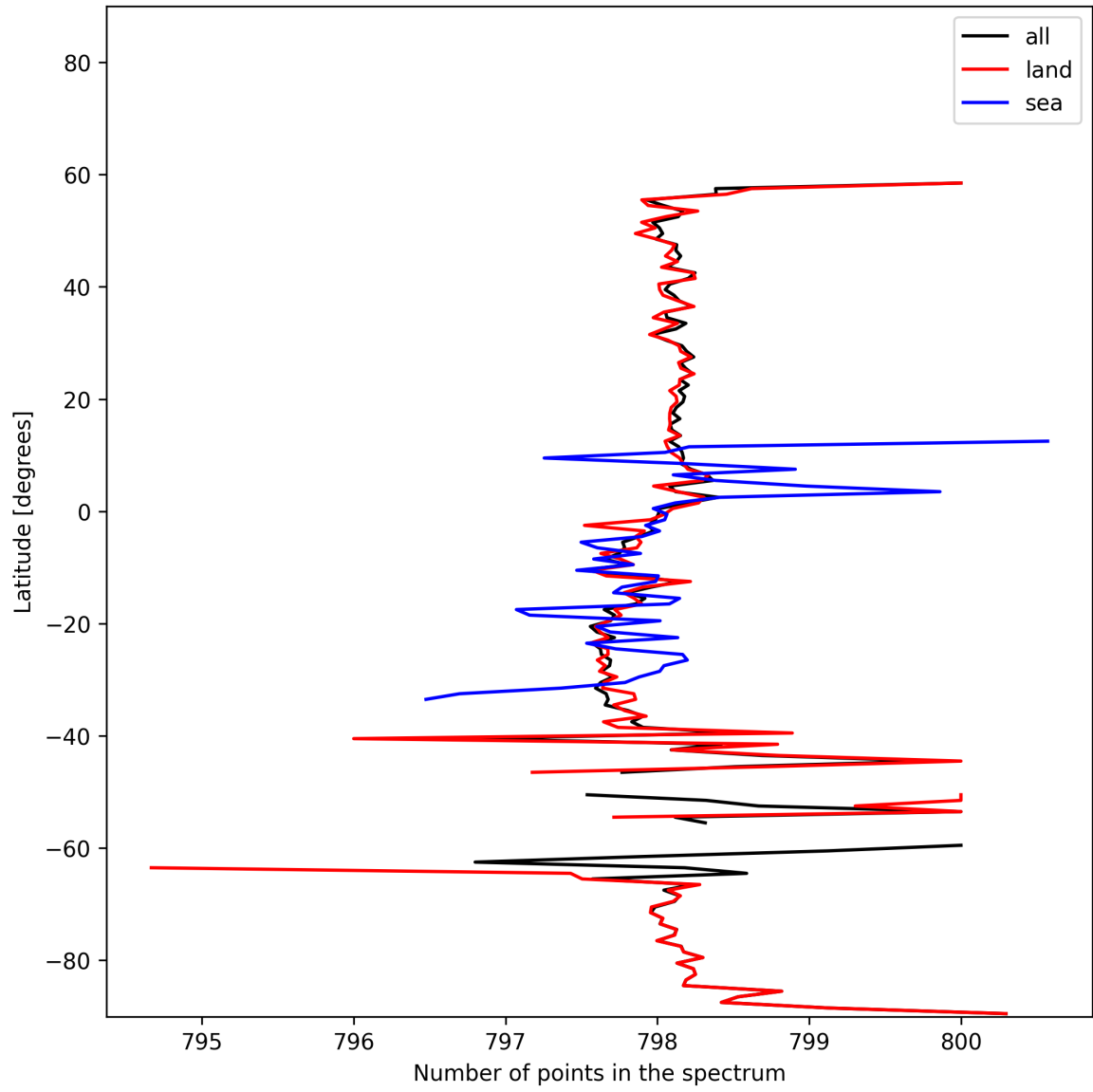
Figure 15: Zonal average of “Number of points in the spectrum” for 2024-11-07 to 2024-11-09.
