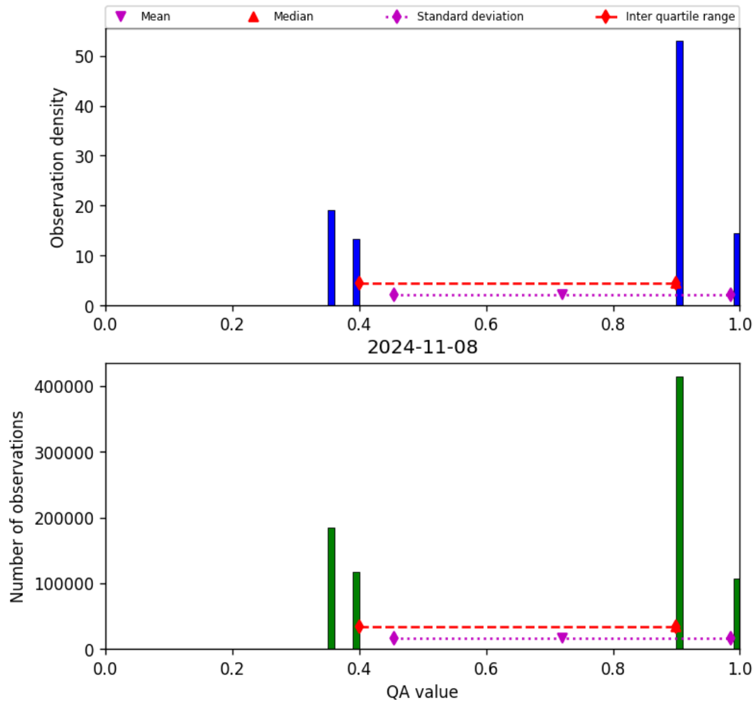
Figure 22: Histogram of “QA value” for 2024-11-07 to 2024-11-09
