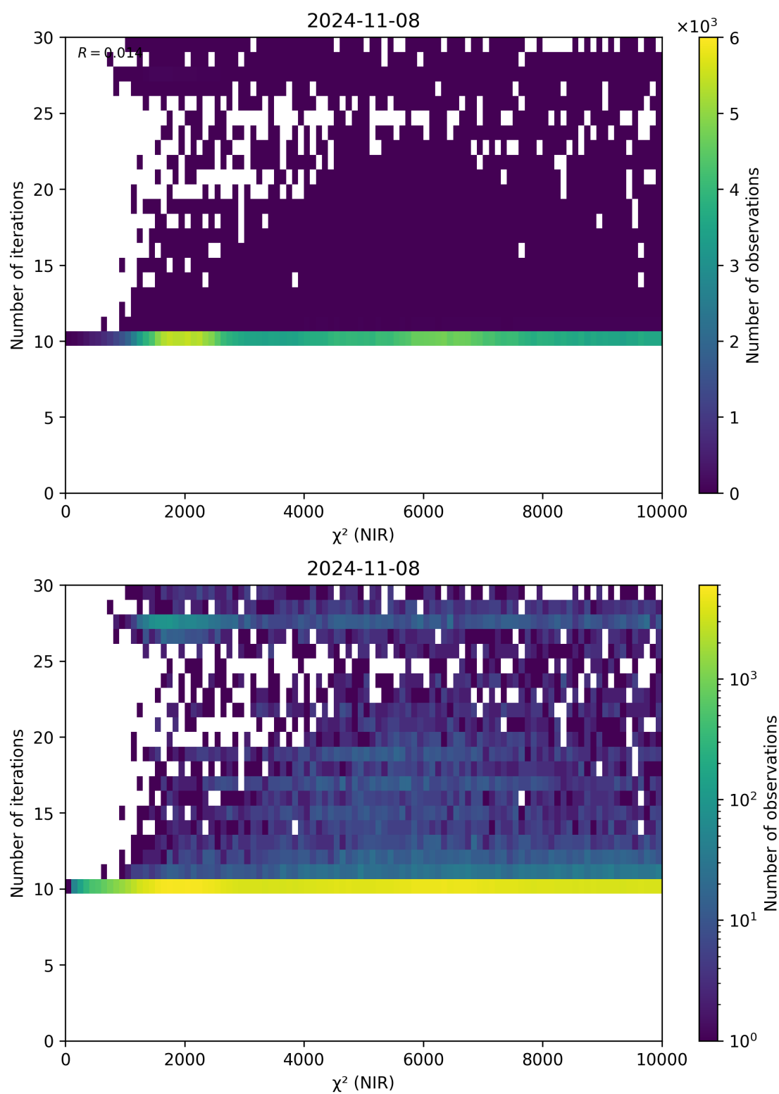
Figure 46: Scatter density plot of “ \chi^2 (NIR)” against “Number of iterations” for 2024-11-07 to 2024-11-09.
