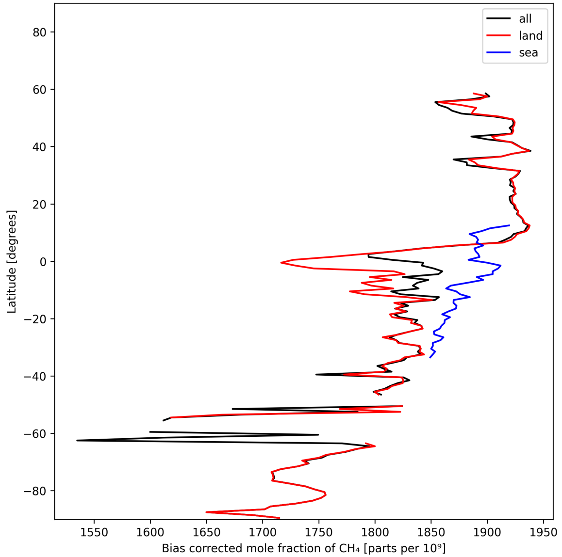
Figure 14: Zonal average of “Bias corrected mole fraction of \text{CH}_4 ” for 2024-11-07 to 2024-11-09.
