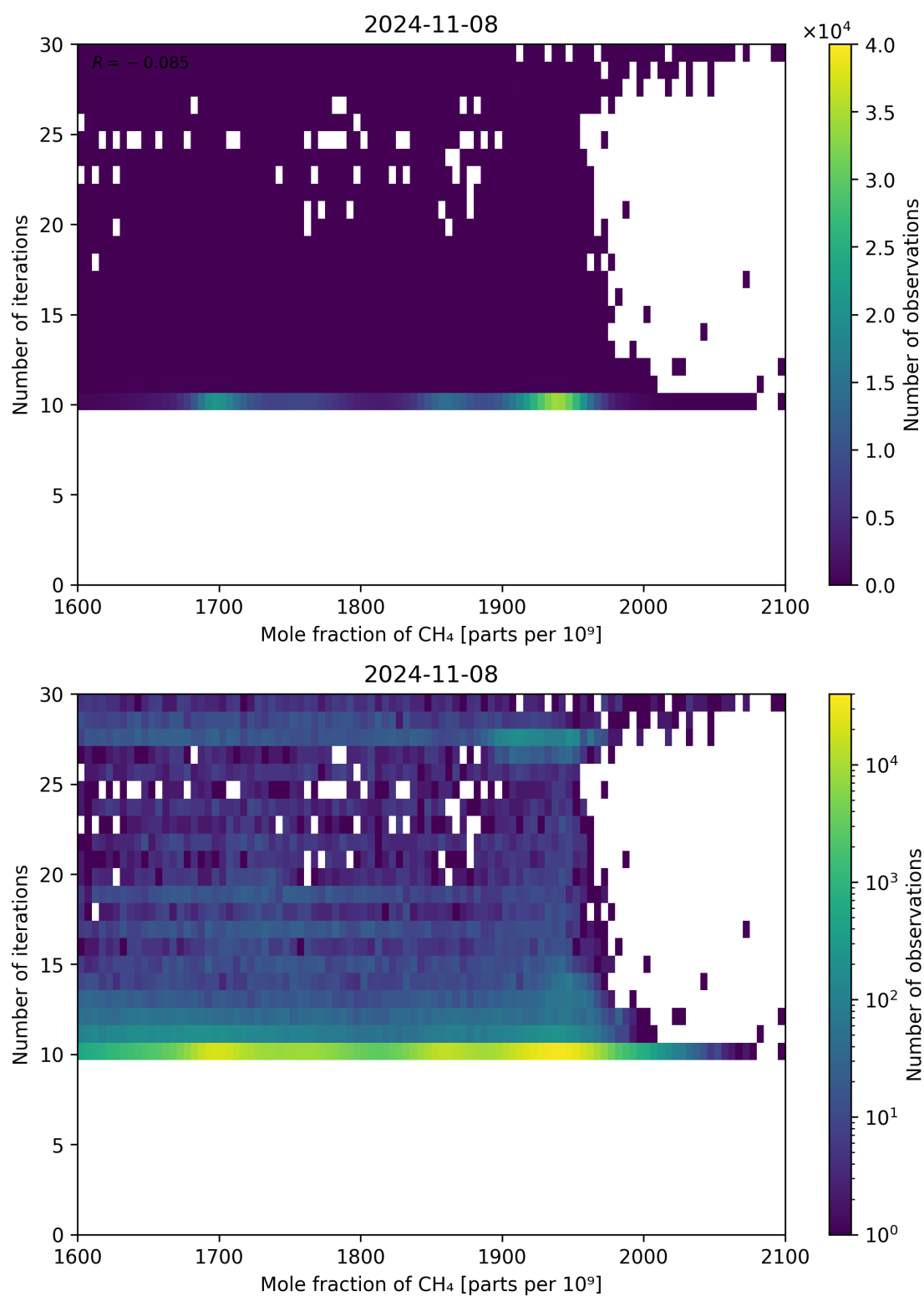
Figure 76: Scatter density plot of “Mole fraction of CH 4 ” against “Number of iterations” for 2024-11-07 to 2024-11-09.
