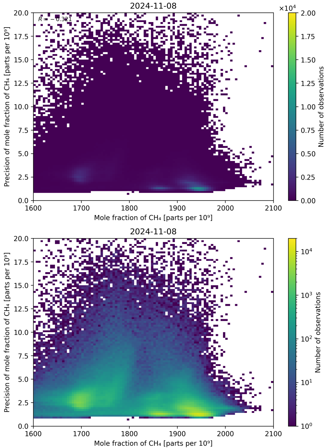
Figure 75: Scatter density plot of “Mole fraction of CH 4 ” against “Precision of mole fraction of CH 4 ” for 2024-11-07 to 2024-11-09.
