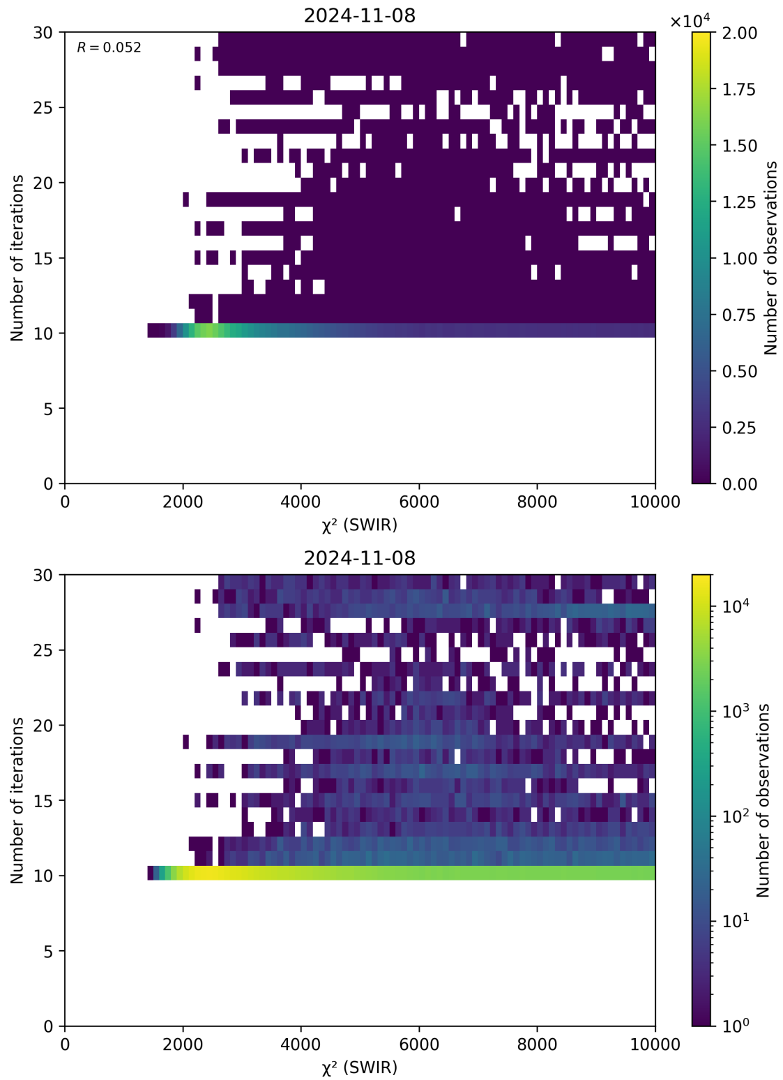
Figure 50: Scatter density plot of “ \chi^2 (SWIR)” against “Number of iterations” for 2024-11-07 to 2024-11-09.
