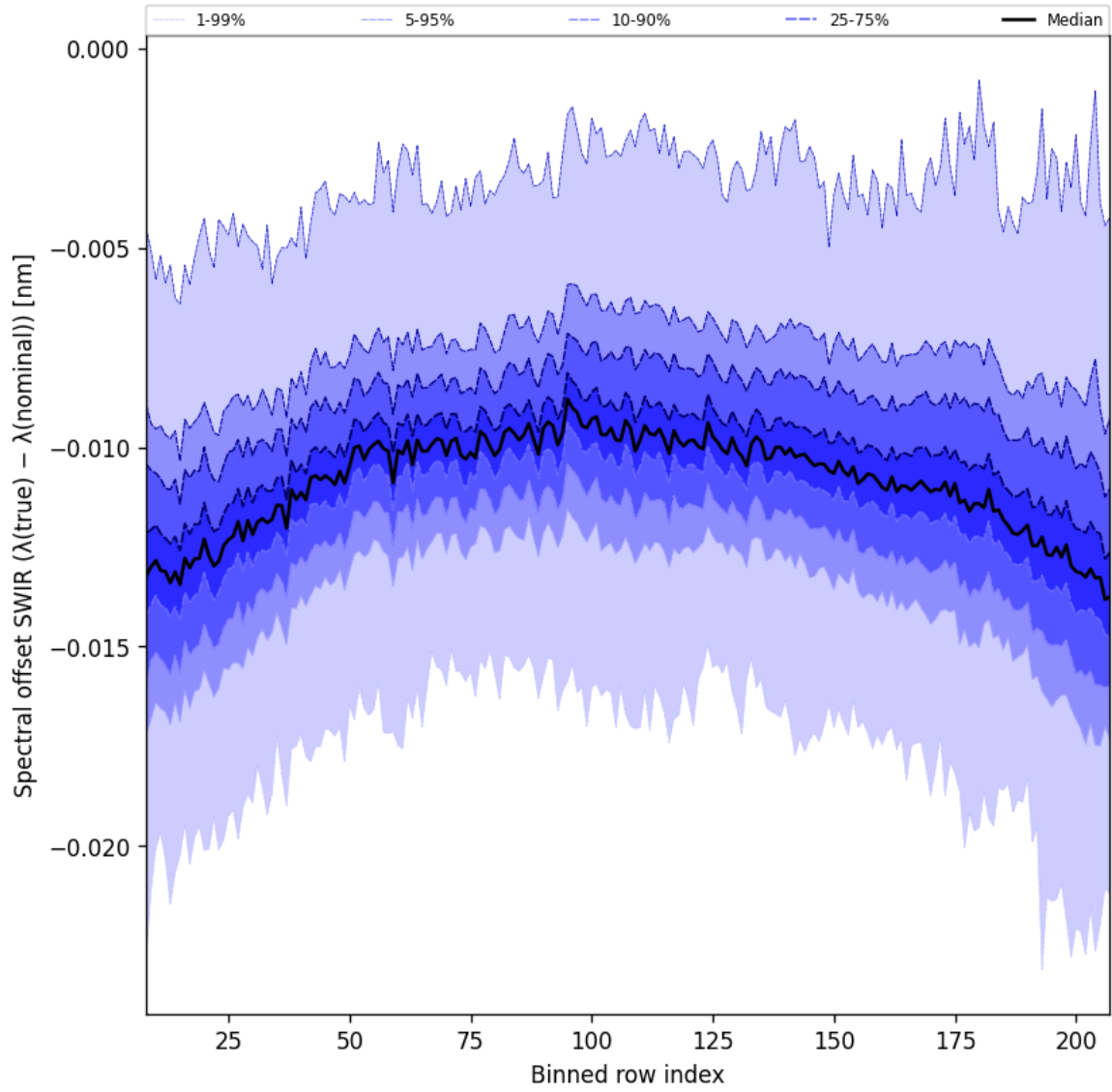
Figure 38: Along track statistics of “Spectral offset SWIR ( \lambda_{\text{true}} - \lambda_{\text{nominal}} )” for 2024-11-07 to 2024-11-09
