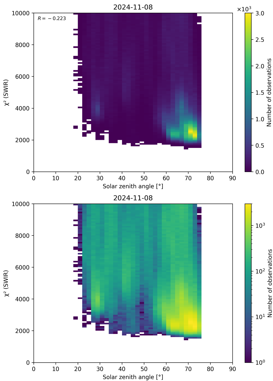
Figure 95: Scatter density plot of “Solar zenith angle” against “ \chi^2 (SWIR)” for 2024-11-07 to 2024-11-09.
