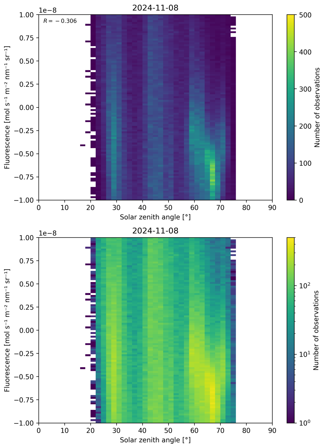
Figure 97: Scatter density plot of “Solar zenith angle” against “Fluorescence” for 2024-11-07 to 2024-11-09.
