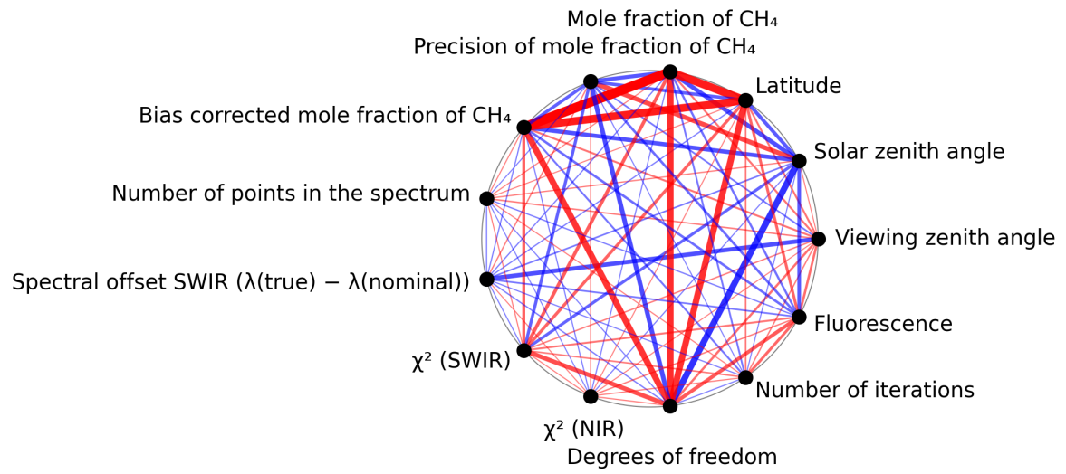
Figure 1: Map of correlation graph for 2024-11-07 to 2024-11-09.
