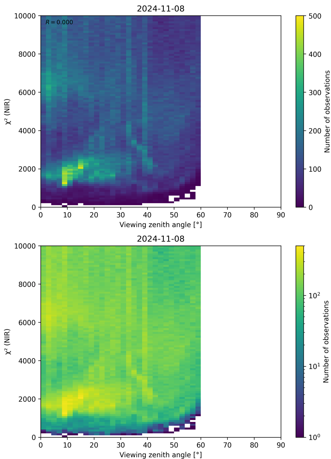
Figure 105: Scatter density plot of “Viewing zenith angle” against “ \chi^2 (NIR)” for 2024-11-07 to 2024-11-09.
