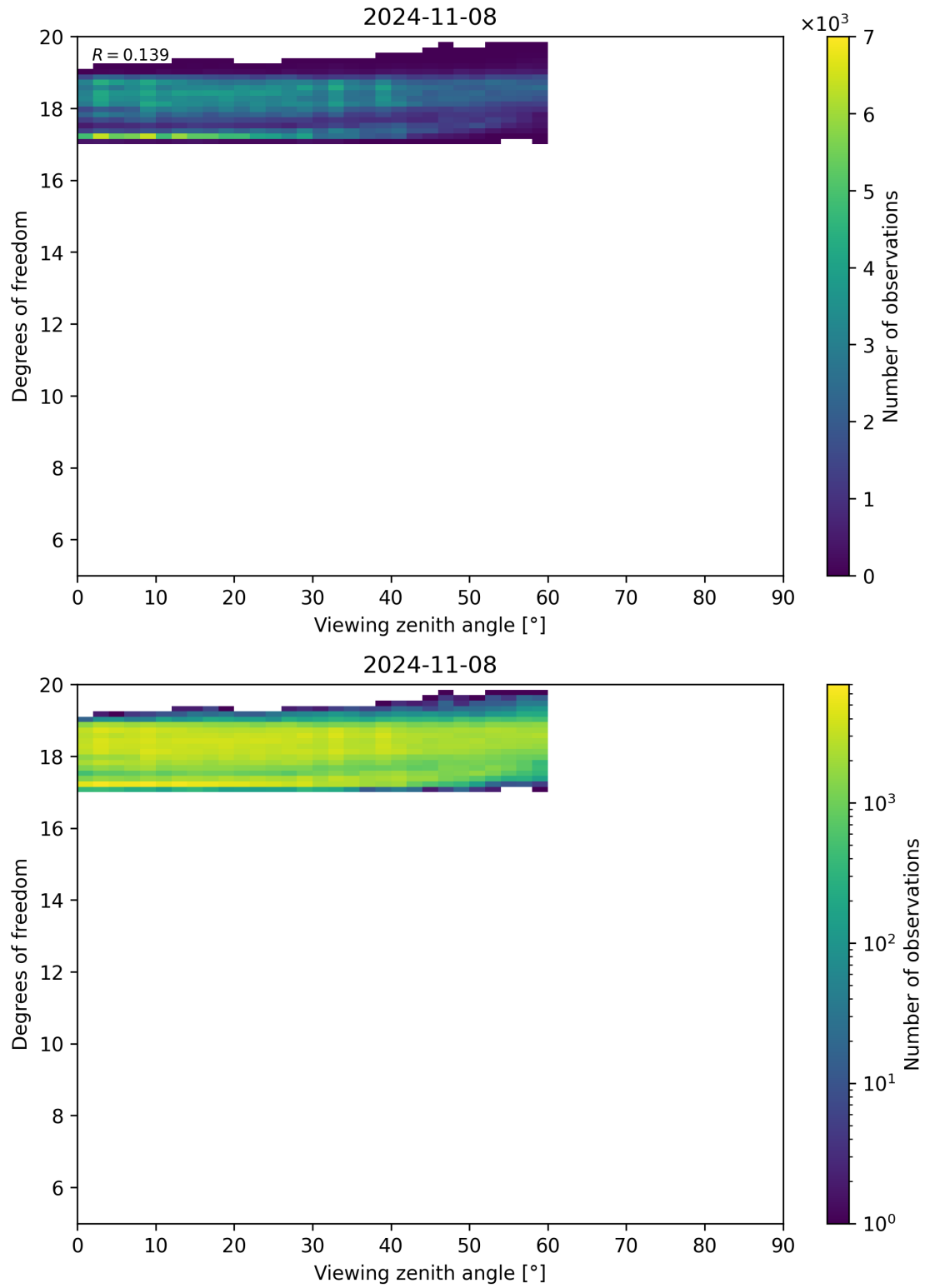
Figure 107: Scatter density plot of “Viewing zenith angle” against “Degrees of freedom” for 2024-11-07 to 2024-11-09.
