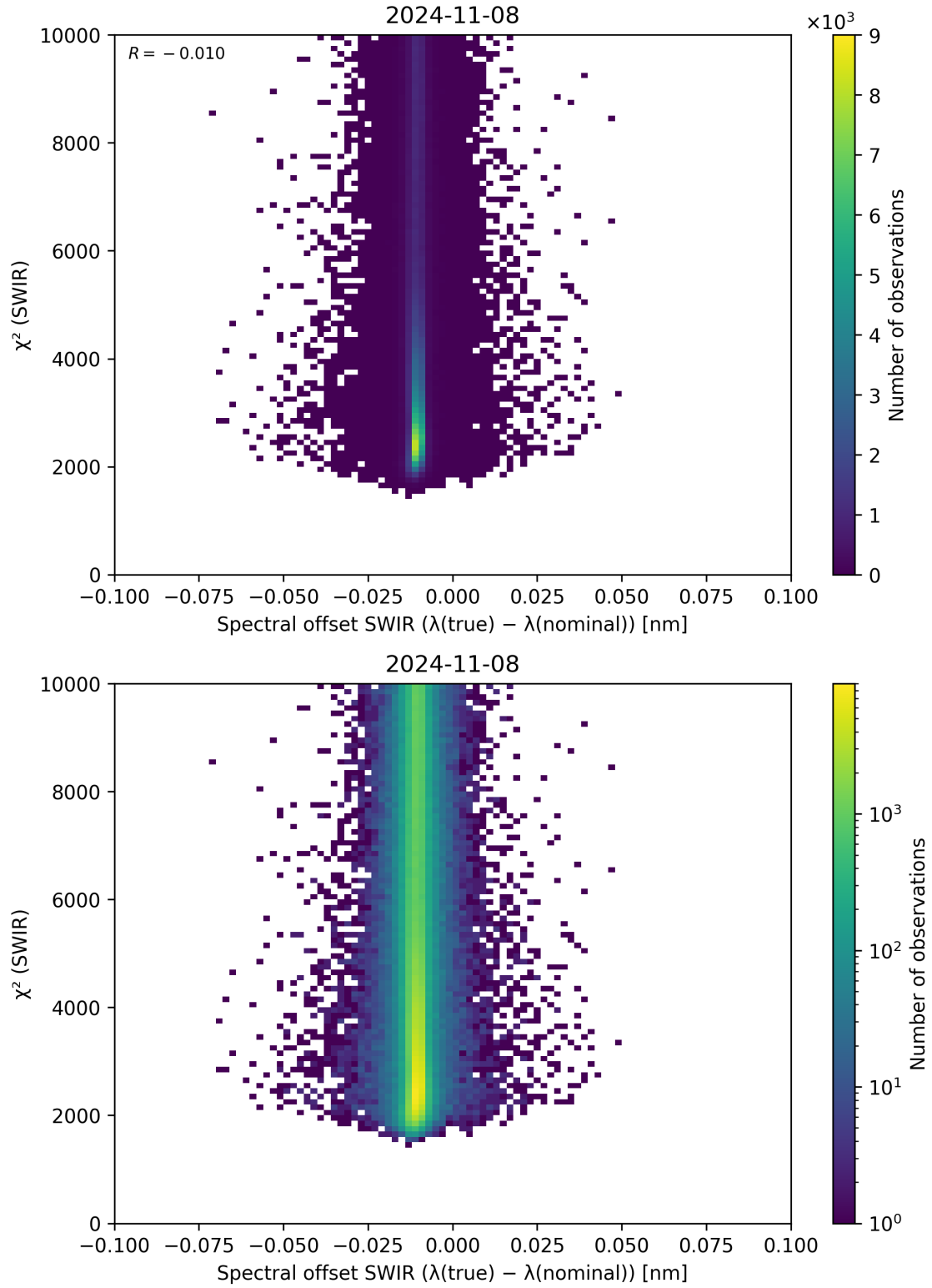
Figure 118: Scatter density plot of “Spectral offset SWIR ( \lambda_{\text{true}} - \lambda_{\text{nominal}} )” against “ \chi^2 (SWIR)” for 2024-11-07 to 2024-11-09.
