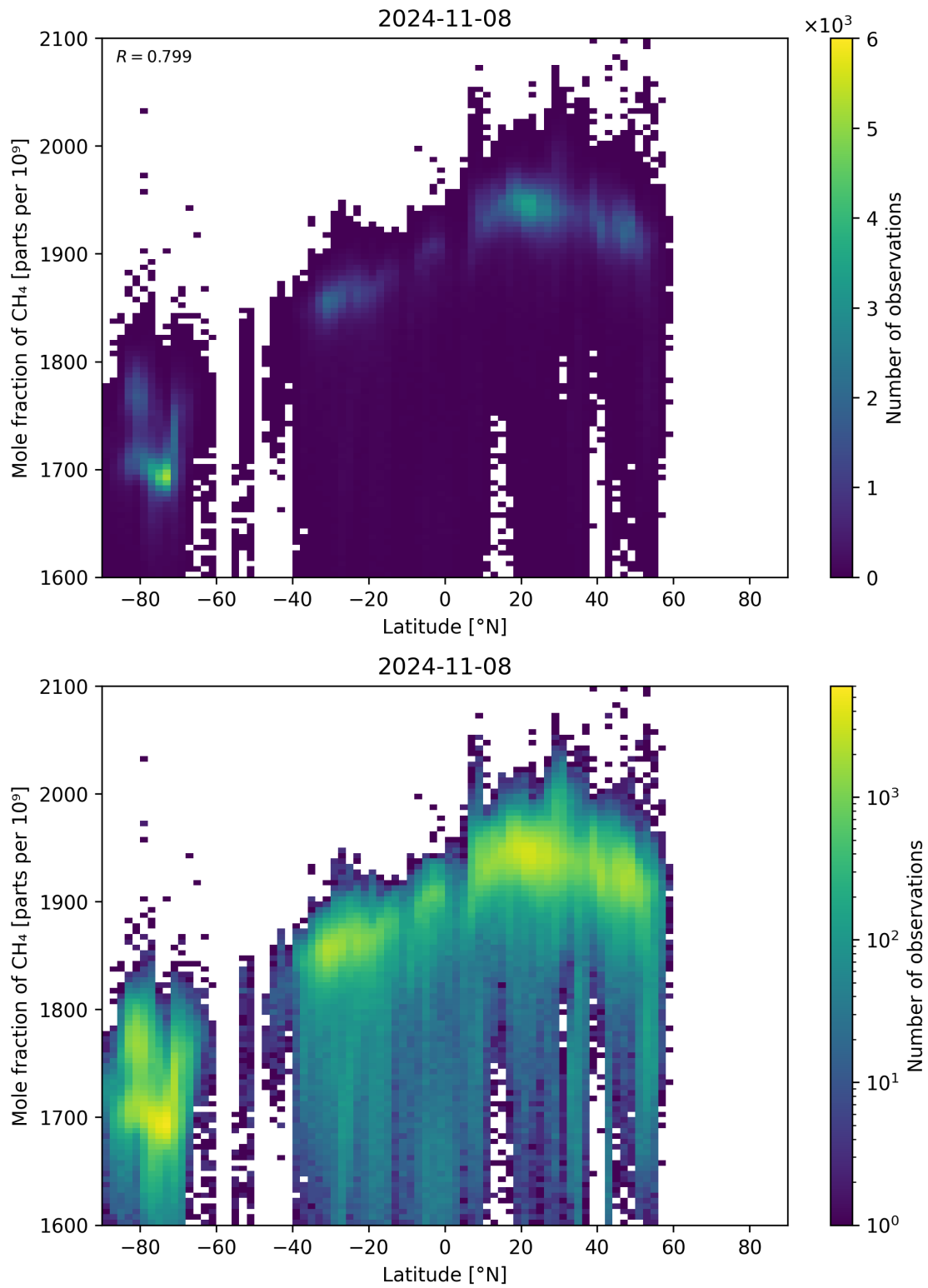
Figure 57: Scatter density plot of “Latitude” against “Mole fraction of CH 4 ” for 2024-11-07 to 2024-11-09.
