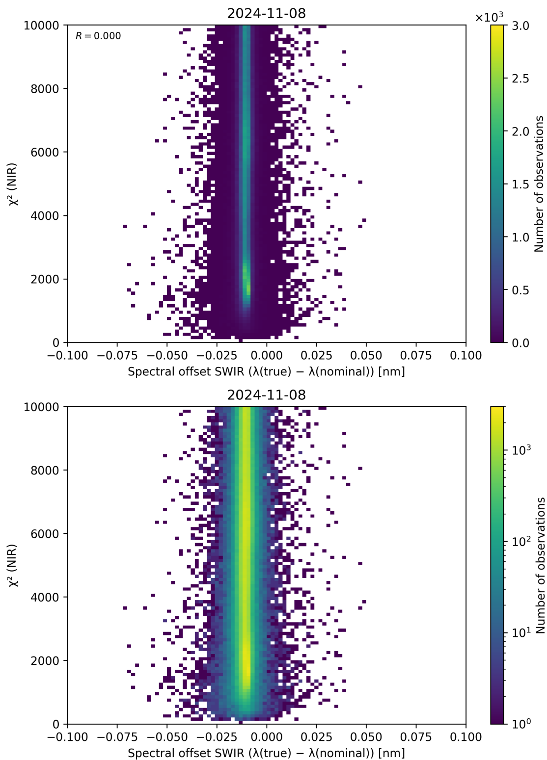
Figure 117: Scatter density plot of “Spectral offset SWIR ( \lambda_{\text{true}} - \lambda_{\text{nominal}} )” against “ \chi^2 (NIR)” for 2024-11-07 to 2024-11-09.
