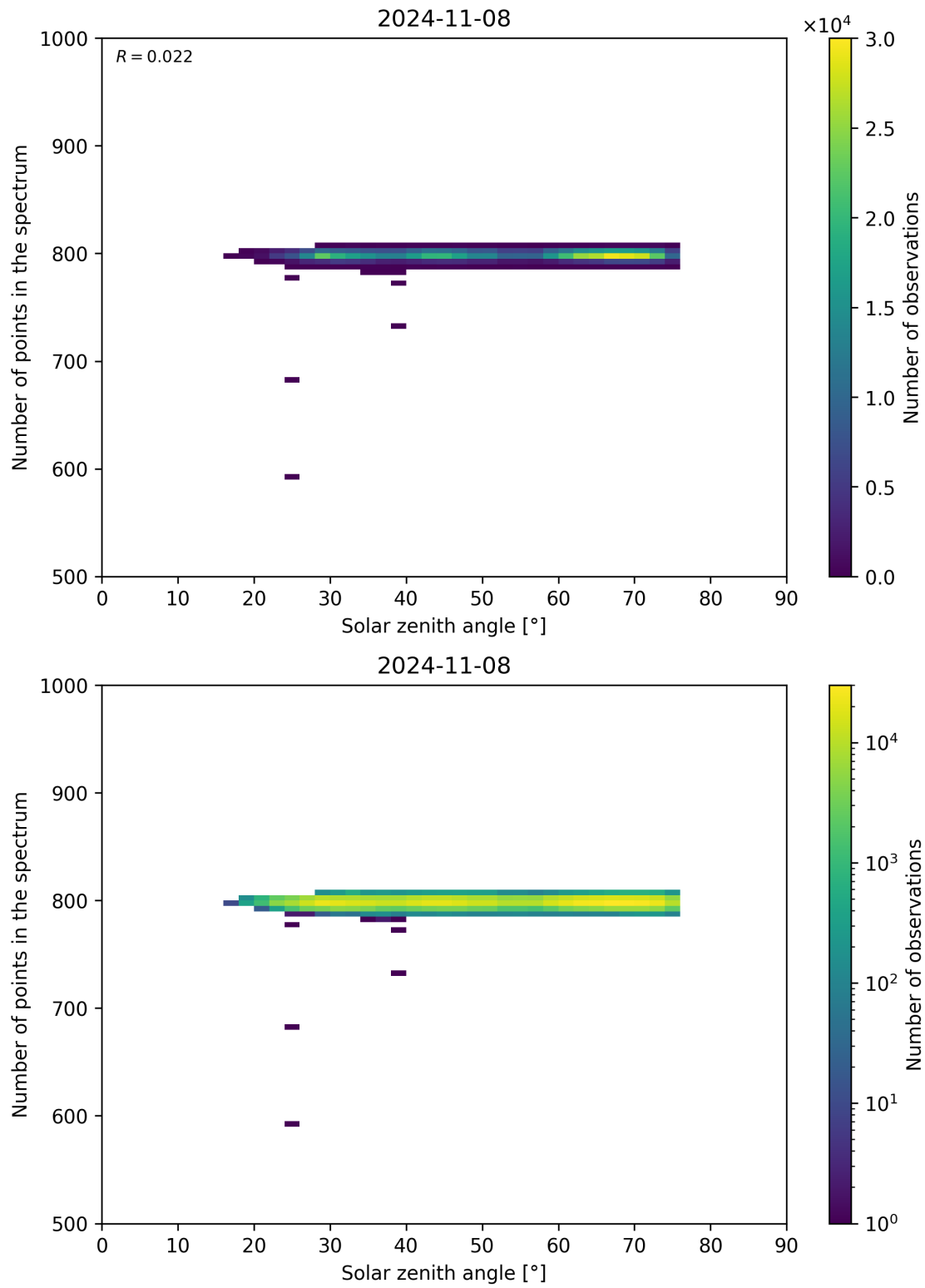
Figure 103: Scatter density plot of “Solar zenith angle” against “Number of points in the spectrum” for 2024-11-07 to 2024-11-09.
