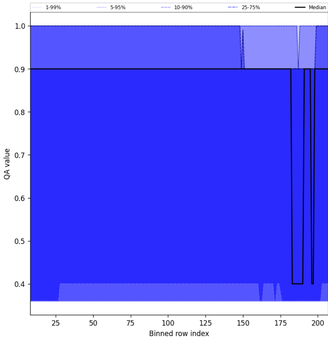
Figure 33: Along track statistics of “QA value” for 2024-11-07 to 2024-11-09
