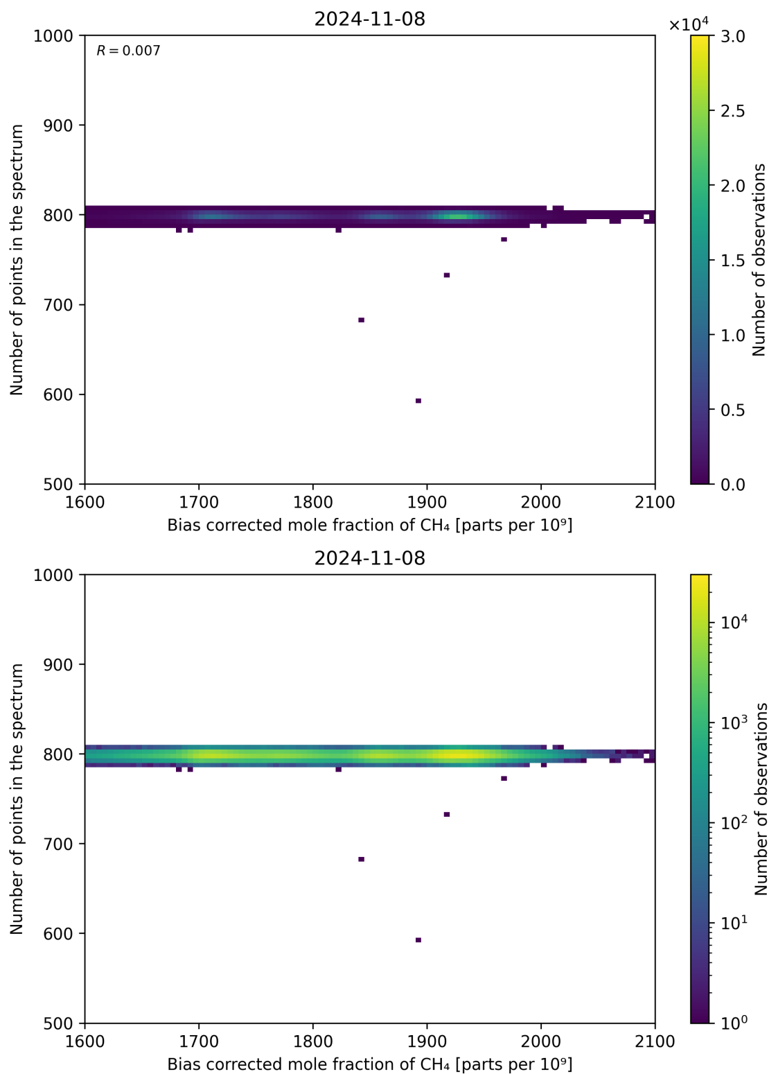
Figure 68: Scatter density plot of “Bias corrected mole fraction of CH 4 ” against “Number of points in the spectrum” for 2024-11-07 to 2024-11-09.
