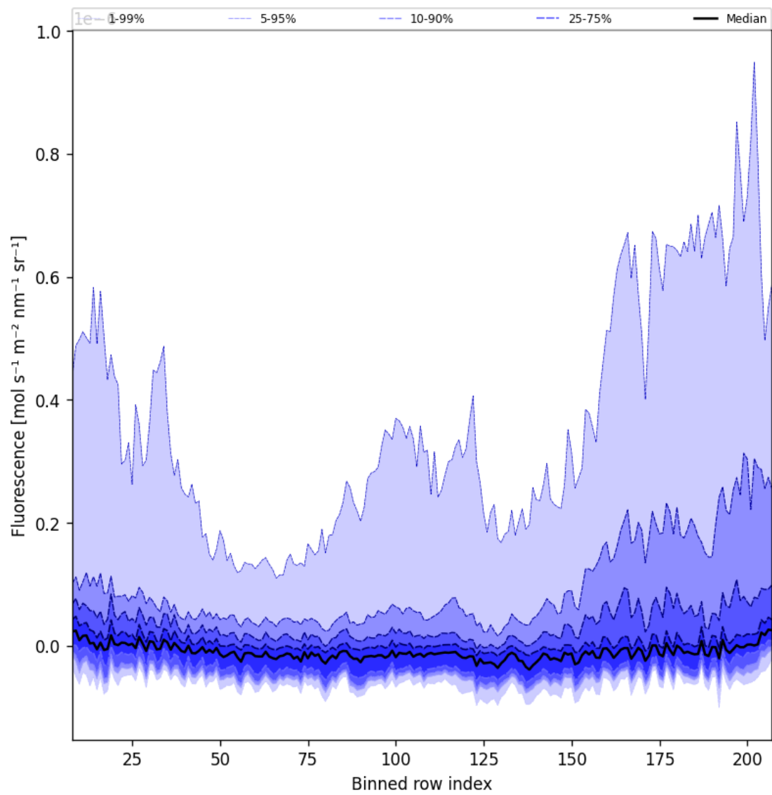
Figure 43: Along track statistics of “Fluorescence” for 2024-11-07 to 2024-11-09
