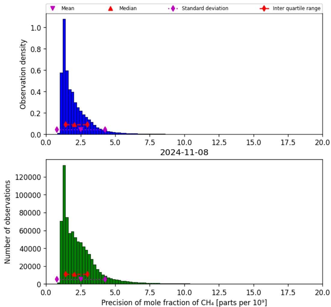
Figure 24: Histogram of “Precision of mole fraction of CH 4 ” for 2024-11-07 to 2024-11-09
