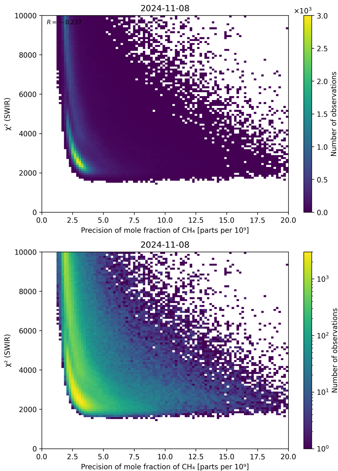
Figure 79: Scatter density plot of “Precision of mole fraction of CH 4 ” against “ \chi^2 (SWIR)” for 2024-11-07 to 2024-11-09.
