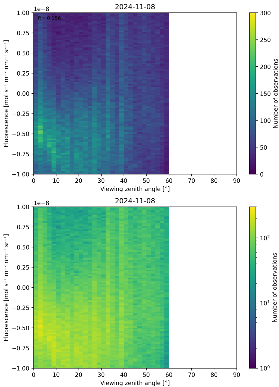
Figure 108: Scatter density plot of “Viewing zenith angle” against “Fluorescence” for 2024-11-07 to 2024-11-09.
