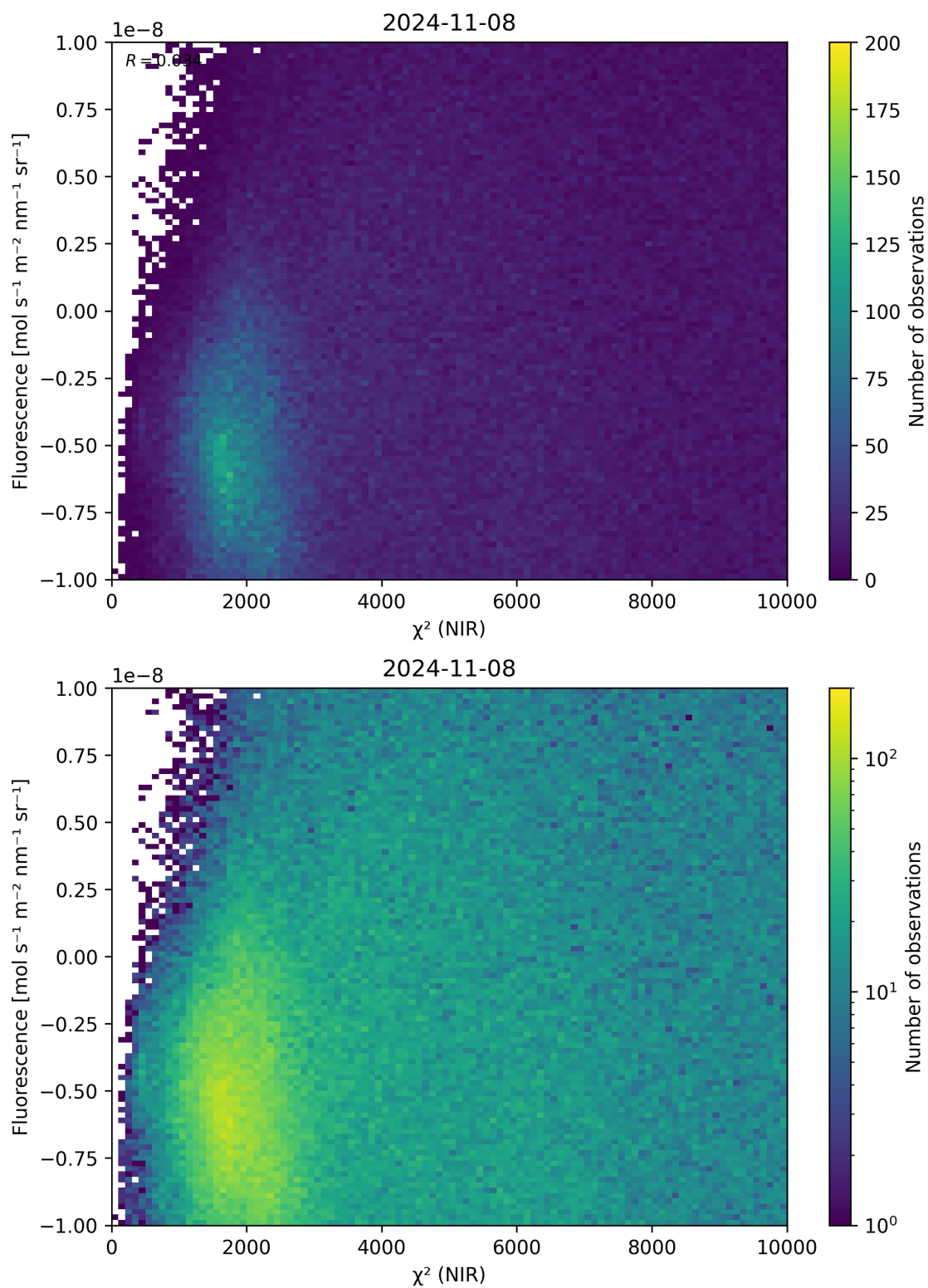
Figure 45: Scatter density plot of “ \chi^2 (NIR)” against “Fluorescence” for 2024-11-07 to 2024-11-09.
