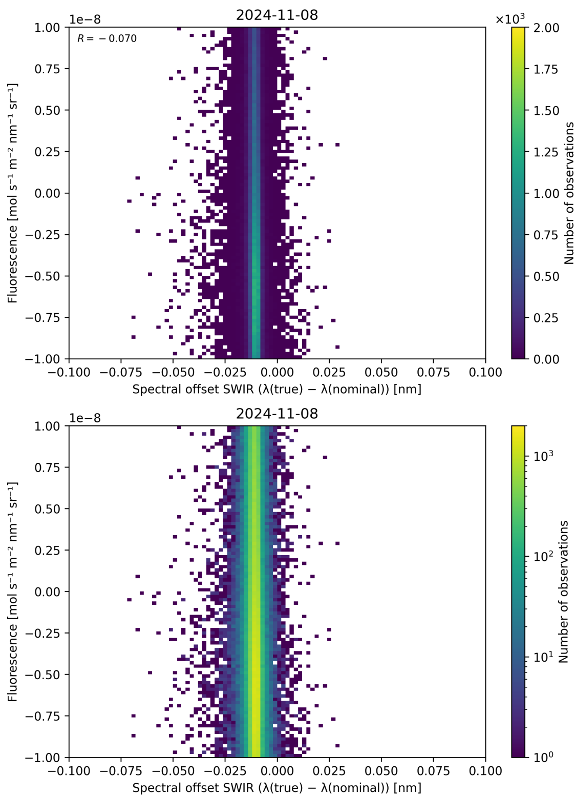
Figure 120: Scatter density plot of “Spectral offset SWIR ( \lambda_{\text{true}} - \lambda_{\text{nominal}} )” against “Fluorescence” for 2024-11-07 to 2024-11-09.
