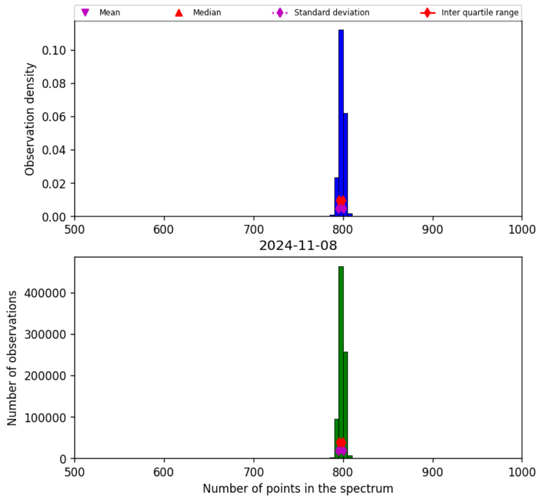
Figure 26: Histogram of “Number of points in the spectrum” for 2024-11-07 to 2024-11-09
