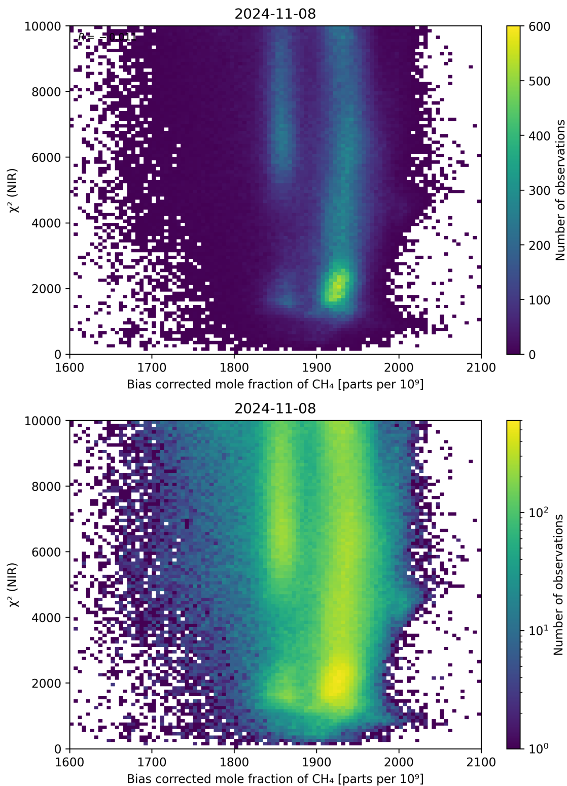
Figure 63: Scatter density plot of “Bias corrected mole fraction of CH 4 ” against “ \chi^2 (NIR)” for 2024-11-07 to 2024-11-09.
