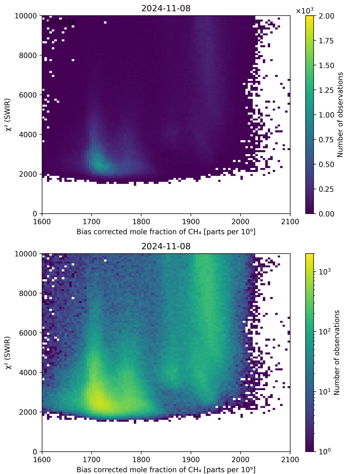
Figure 64: Scatter density plot of “Bias corrected mole fraction of \text{CH}_4 ” against “ \chi^2 (SWIR)” for 2024-11-07 to 2024-11-09.
