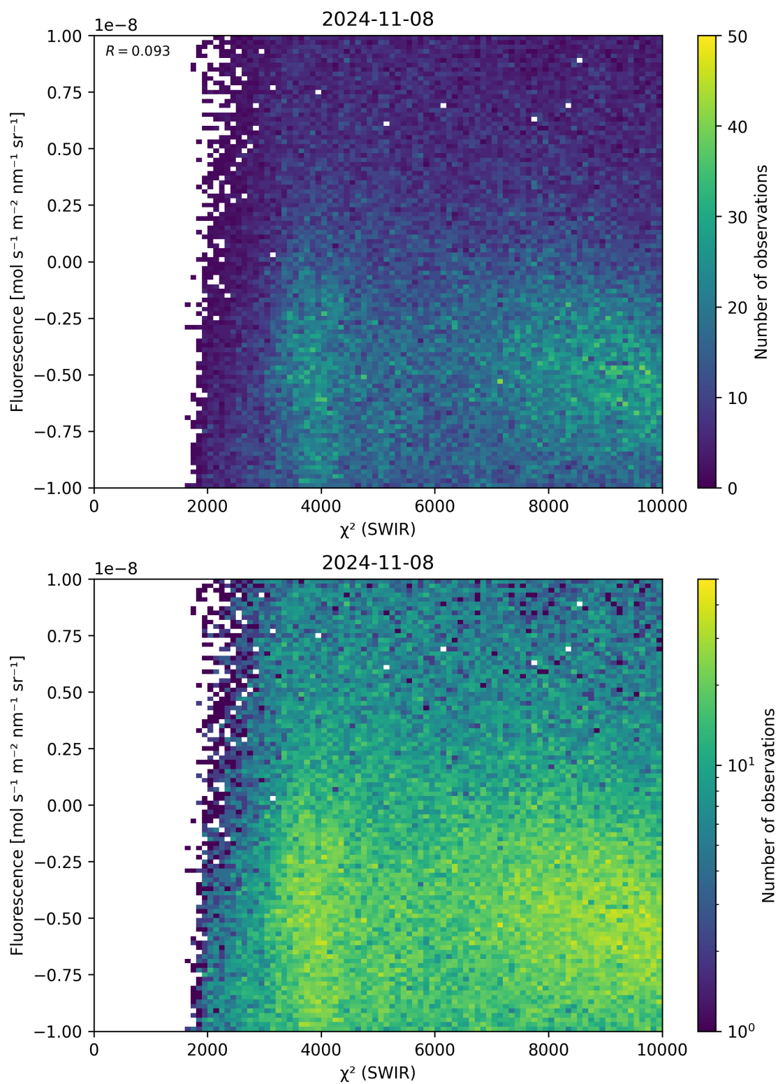
Figure 49: Scatter density plot of “ \chi^2 (SWIR)” against “Fluorescence” for 2024-11-07 to 2024-11-09.
