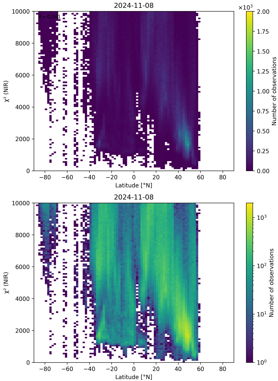
Figure 53: Scatter density plot of “Latitude” against “ \chi^2 (NIR)” for 2024-11-07 to 2024-11-09.
