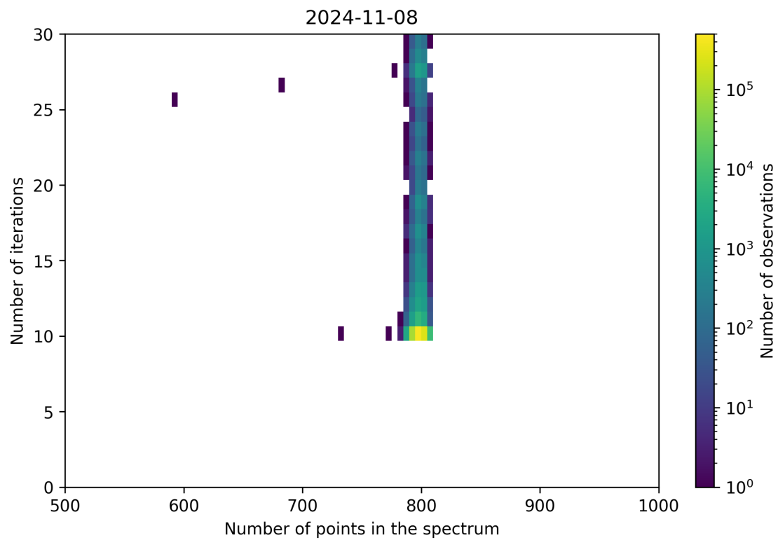
Figure 92: Scatter density plot of “Number of points in the spectrum” against “Number of iterations” for 2024-11-07 to 2024-11-09.
