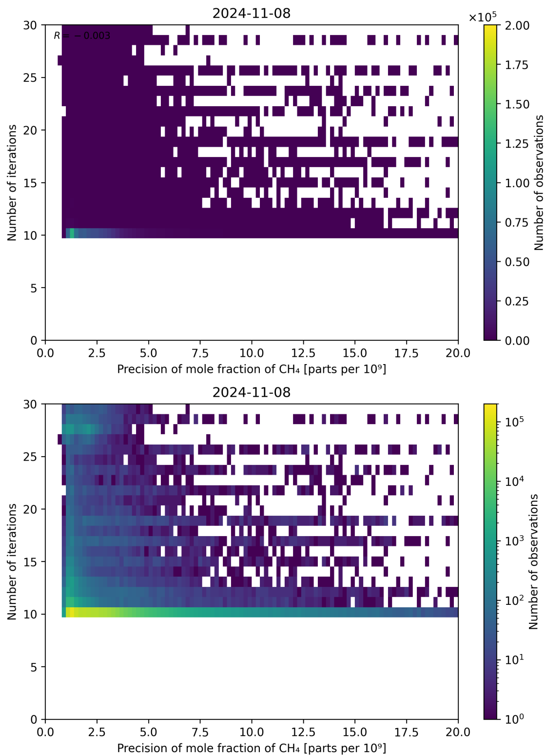
Figure 83: Scatter density plot of “Precision of mole fraction of CH 4 ” against “Number of iterations” for 2024-11-07 to 2024-11-09.
