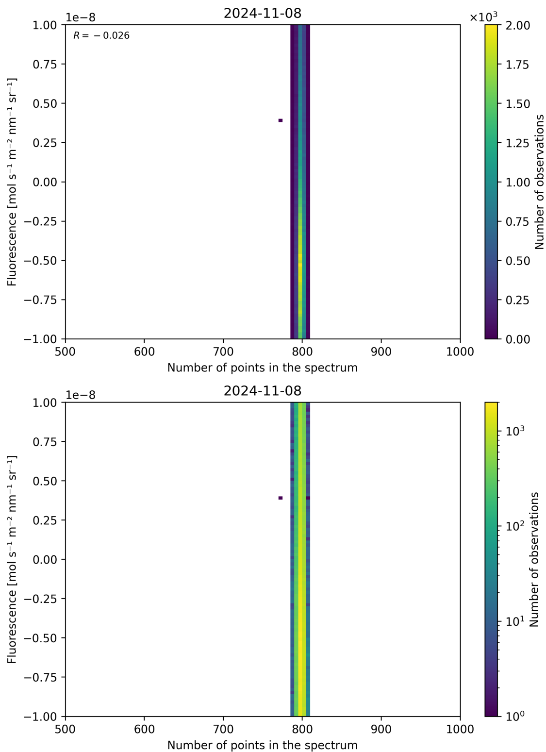
Figure 91: Scatter density plot of “Number of points in the spectrum” against “Fluorescence” for 2024-11-07 to 2024-11-09.
