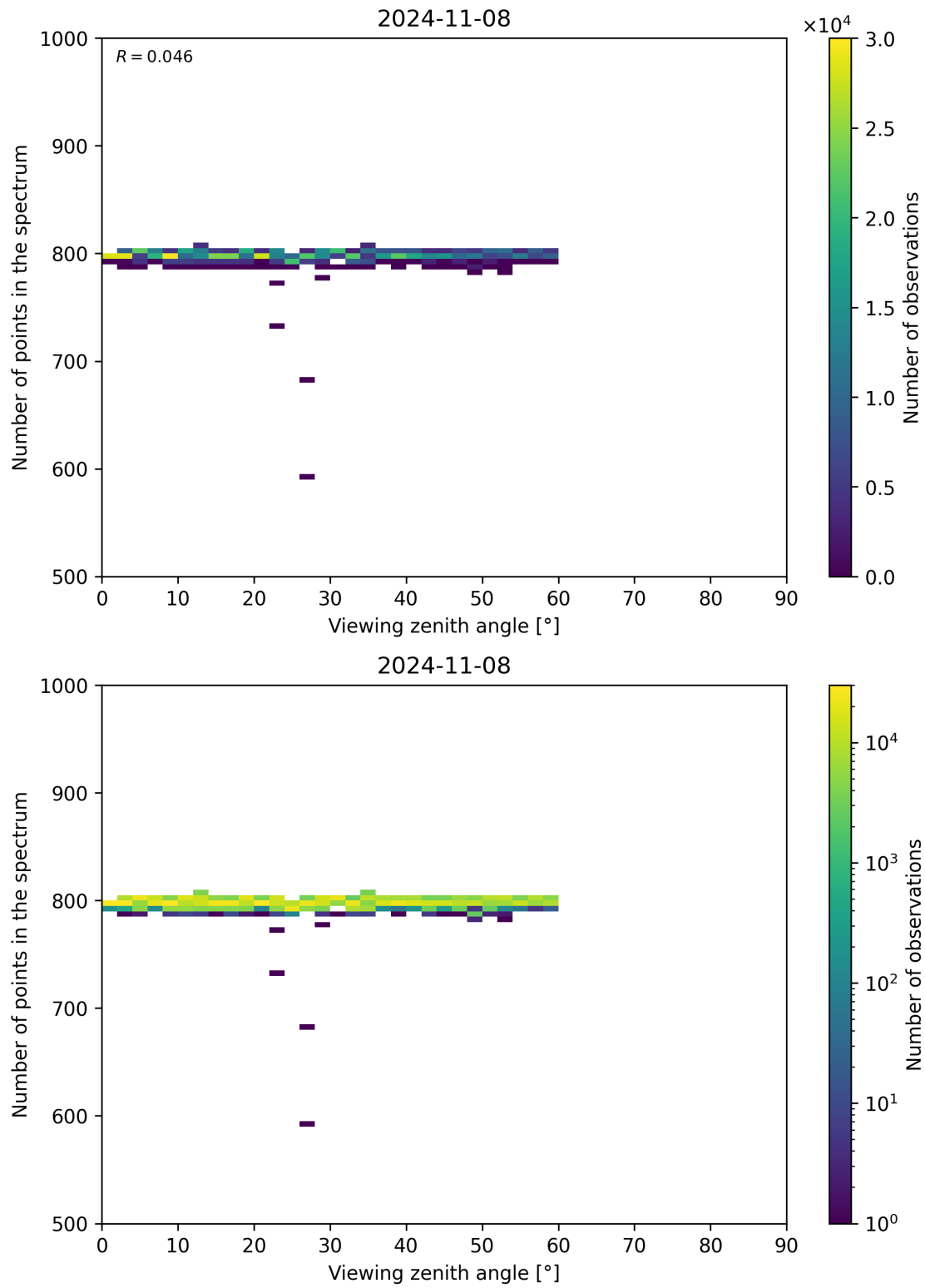
Figure 114: Scatter density plot of “Viewing zenith angle” against “Number of points in the spectrum” for 2024-11-07 to 2024-11-09.
