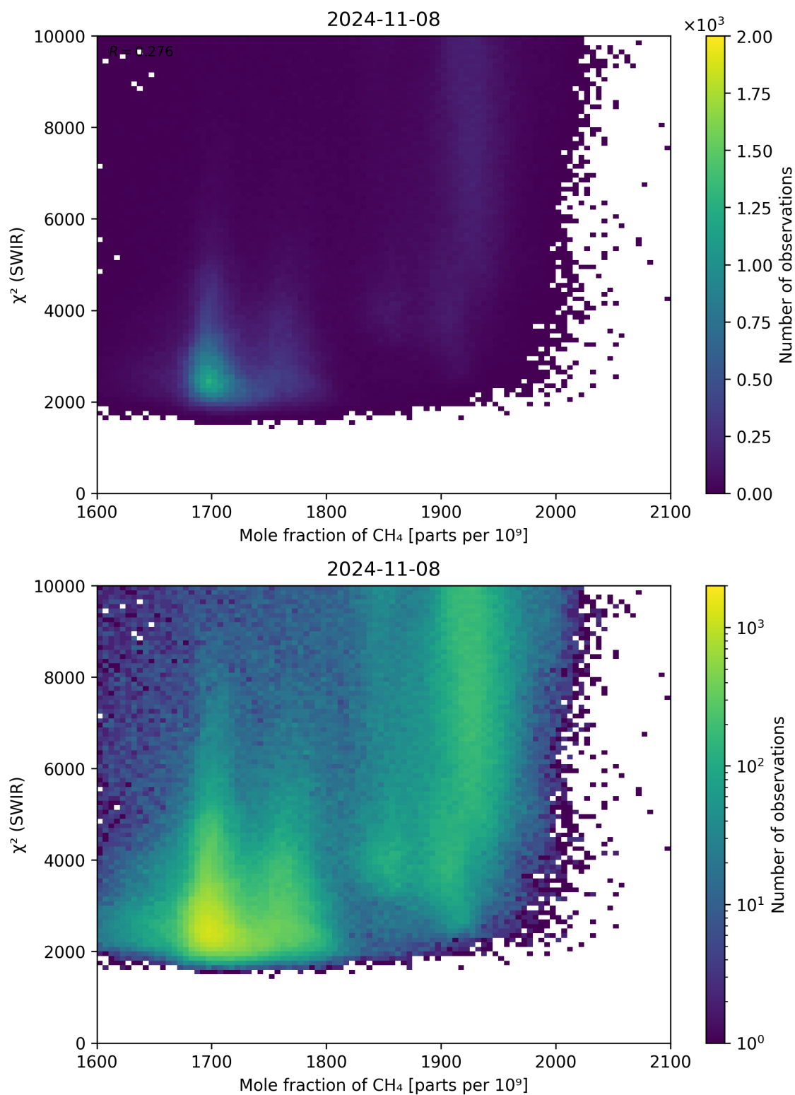
Figure 71: Scatter density plot of “Mole fraction of \text{CH}_4 ” against “ \chi^2 (SWIR)” for 2024-11-07 to 2024-11-09.
