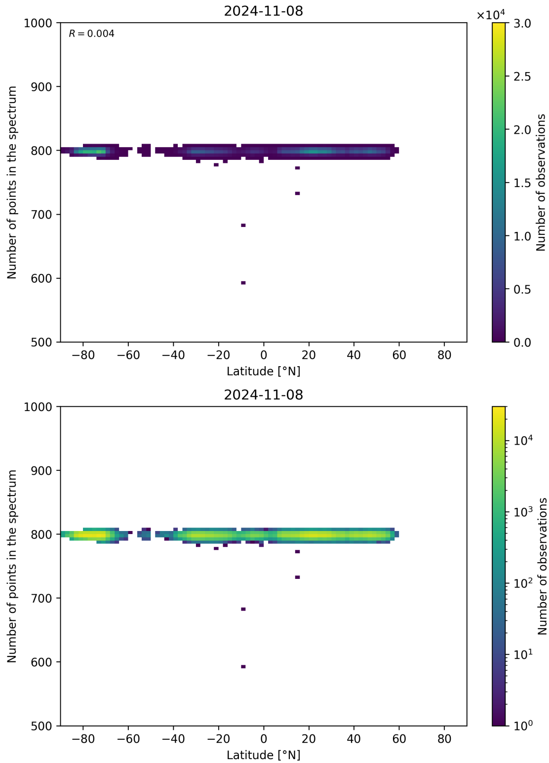
Figure 61: Scatter density plot of “Latitude” against “Number of points in the spectrum” for 2024-11-07 to 2024-11-09.
