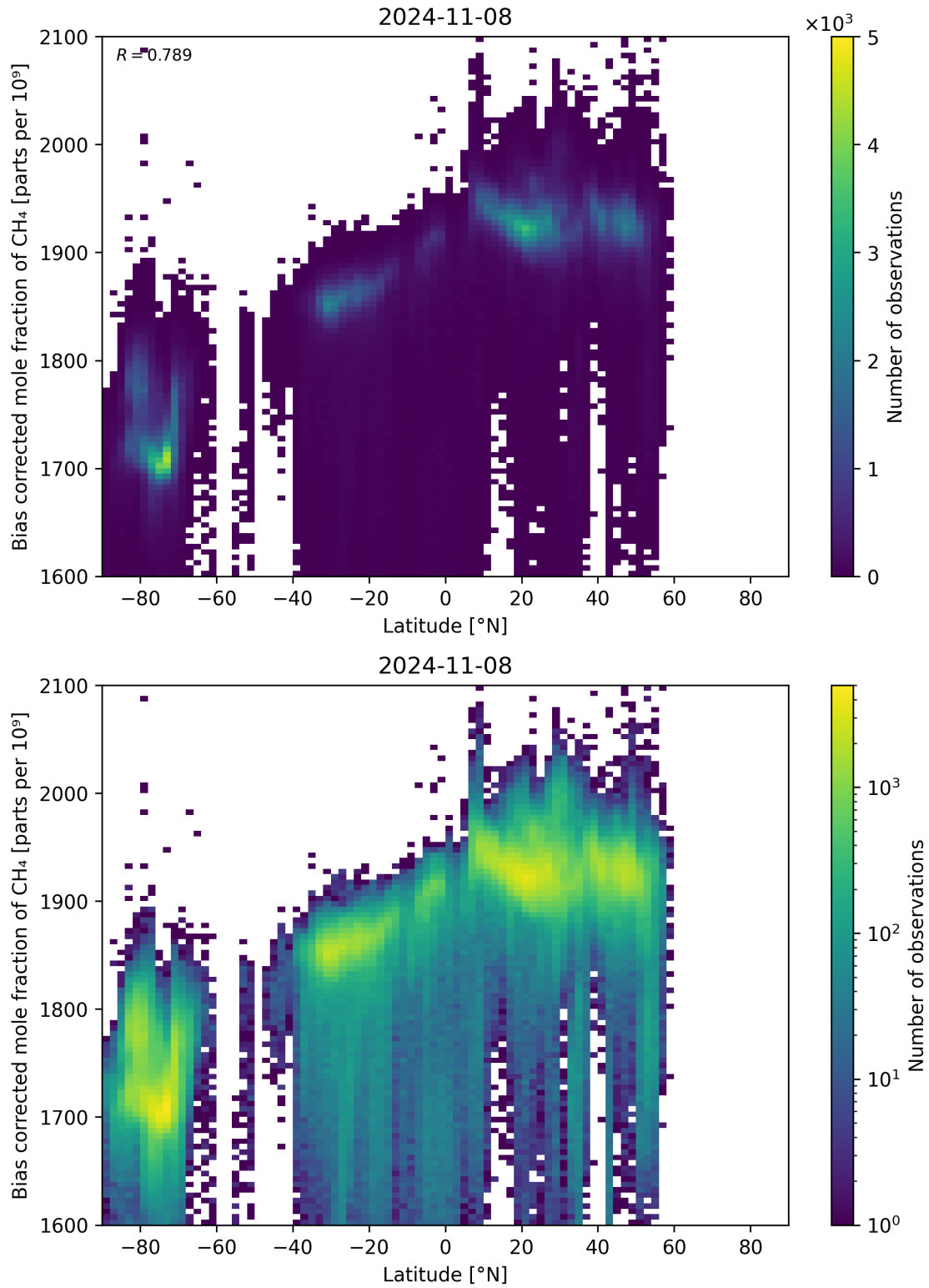
Figure 58: Scatter density plot of “Latitude” against “Bias corrected mole fraction of CH 4 ” for 2024-11-07 to 2024-11-09.
