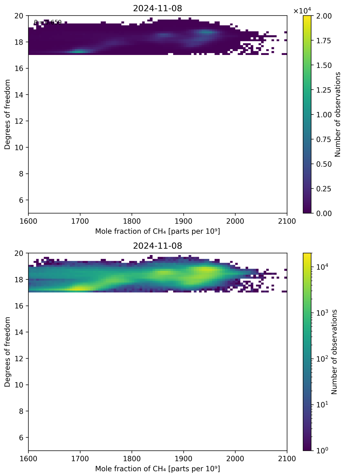
Figure 72: Scatter density plot of “Mole fraction of CH 4 ” against “Degrees of freedom” for 2024-11-07 to 2024-11-09.
