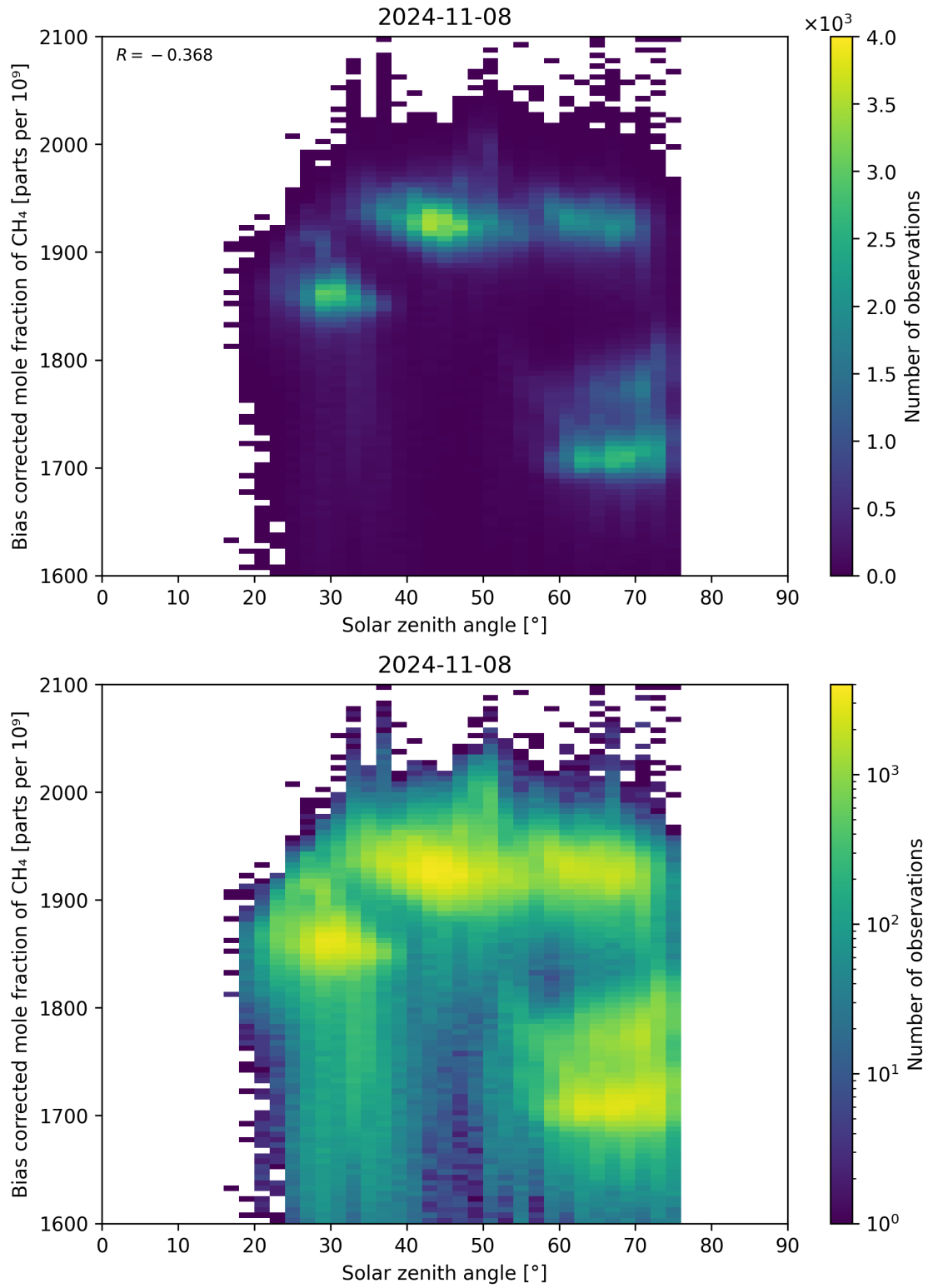
Figure 100: Scatter density plot of “Solar zenith angle” against “Bias corrected mole fraction of CH 4 ” for 2024-11-07 to 2024-11-09.
