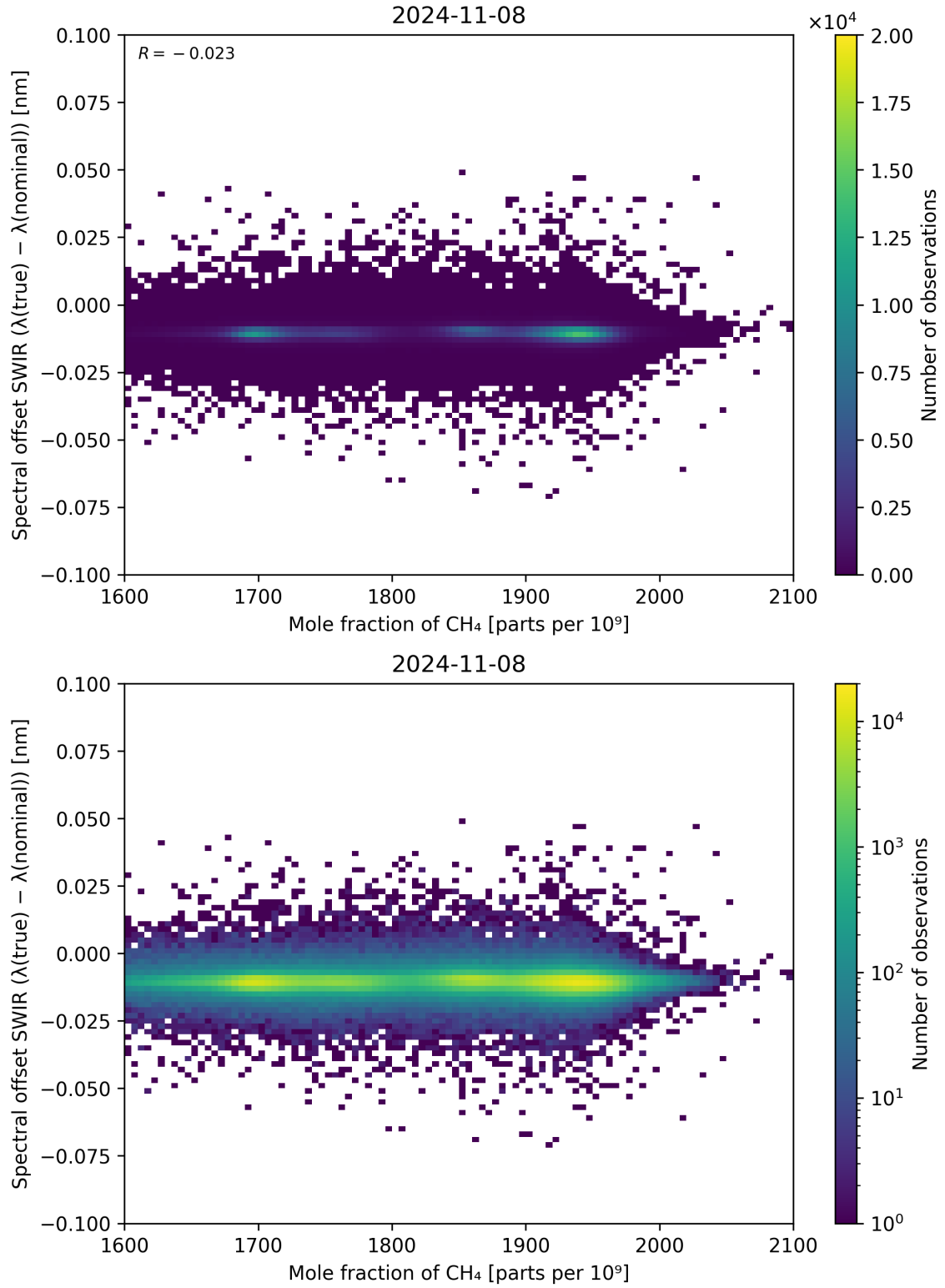
Figure 86: Scatter density plot of “Mole fraction of CH 4 ” against “Spectral offset SWIR ( \lambda_{\text{true}} - \lambda_{\text{nominal}} )” for 2024-11-07 to 2024-11-09.
