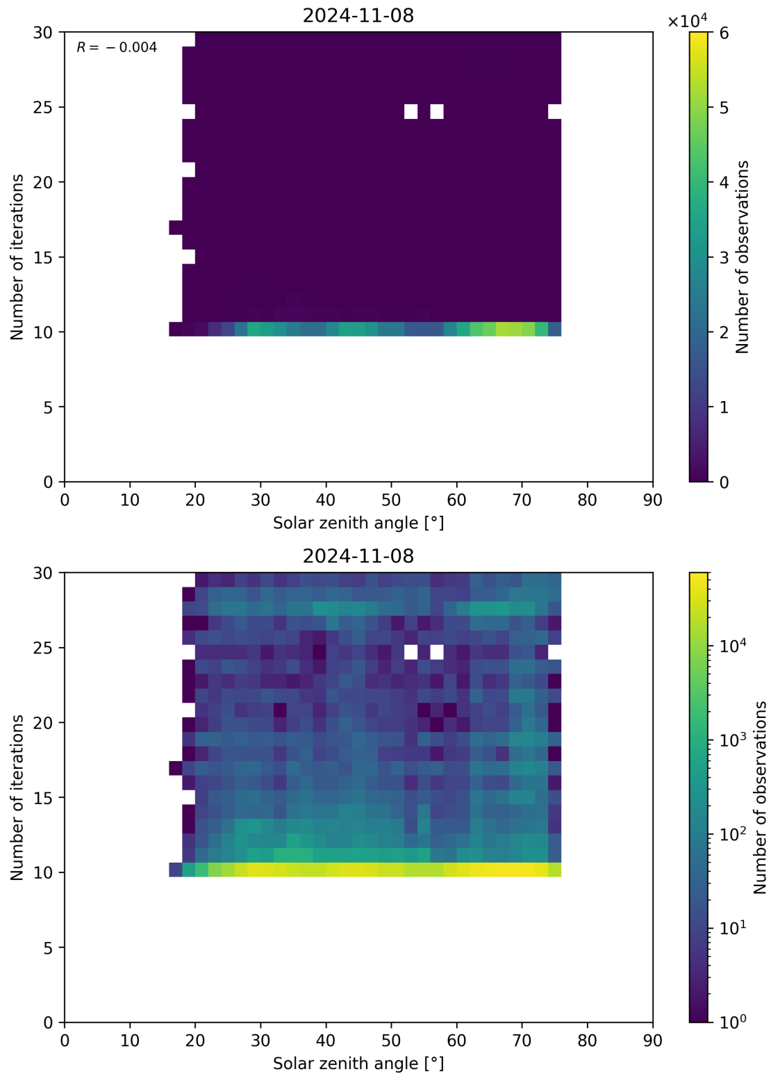
Figure 102: Scatter density plot of “Solar zenith angle” against “Number of iterations” for 2024-11-07 to 2024-11-09.
