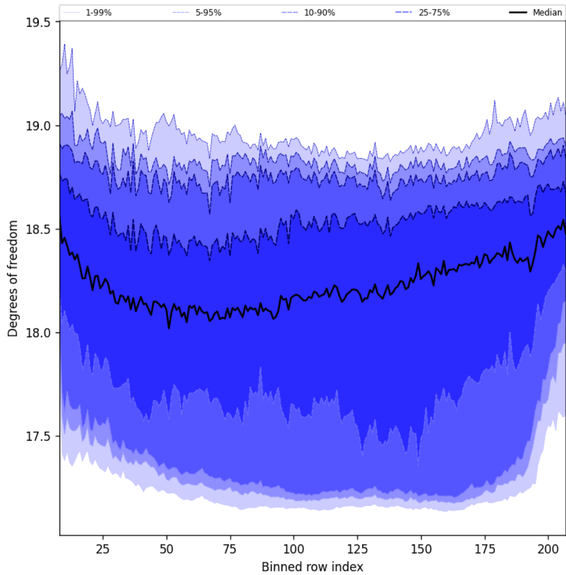
Figure 41: Along track statistics of “Degrees of freedom” for 2024-11-07 to 2024-11-09
