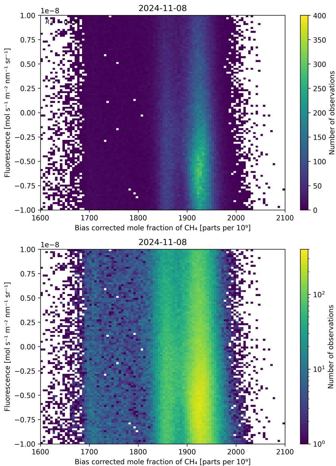
Figure 66: Scatter density plot of “Bias corrected mole fraction of CH 4 ” against “Fluorescence” for 2024-11-07 to 2024-11-09.
