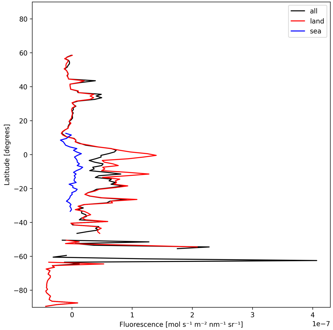
Figure 21: Zonal average of “Fluorescence” for 2024-11-07 to 2024-11-09.
