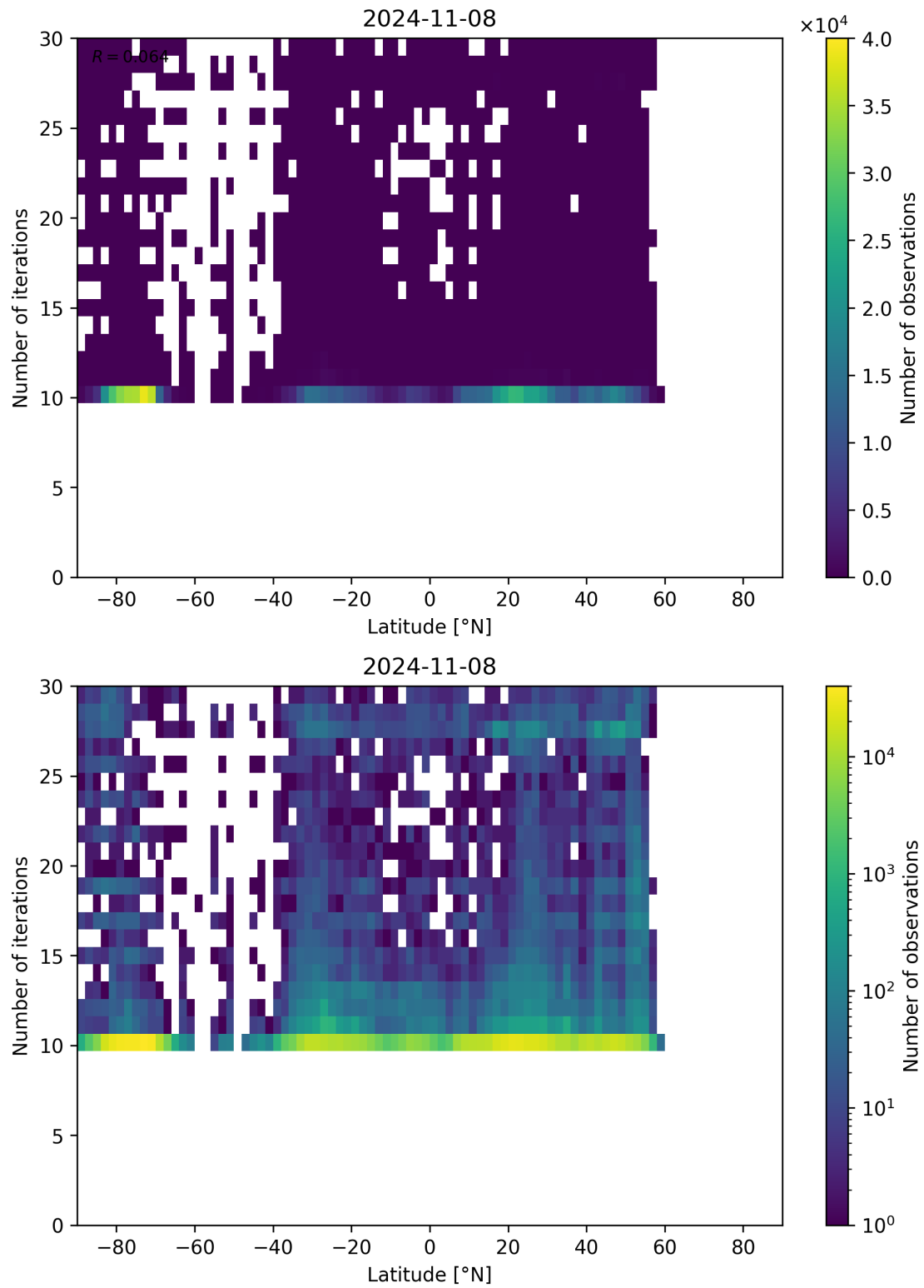
Figure 60: Scatter density plot of “Latitude” against “Number of iterations” for 2024-11-07 to 2024-11-09.
