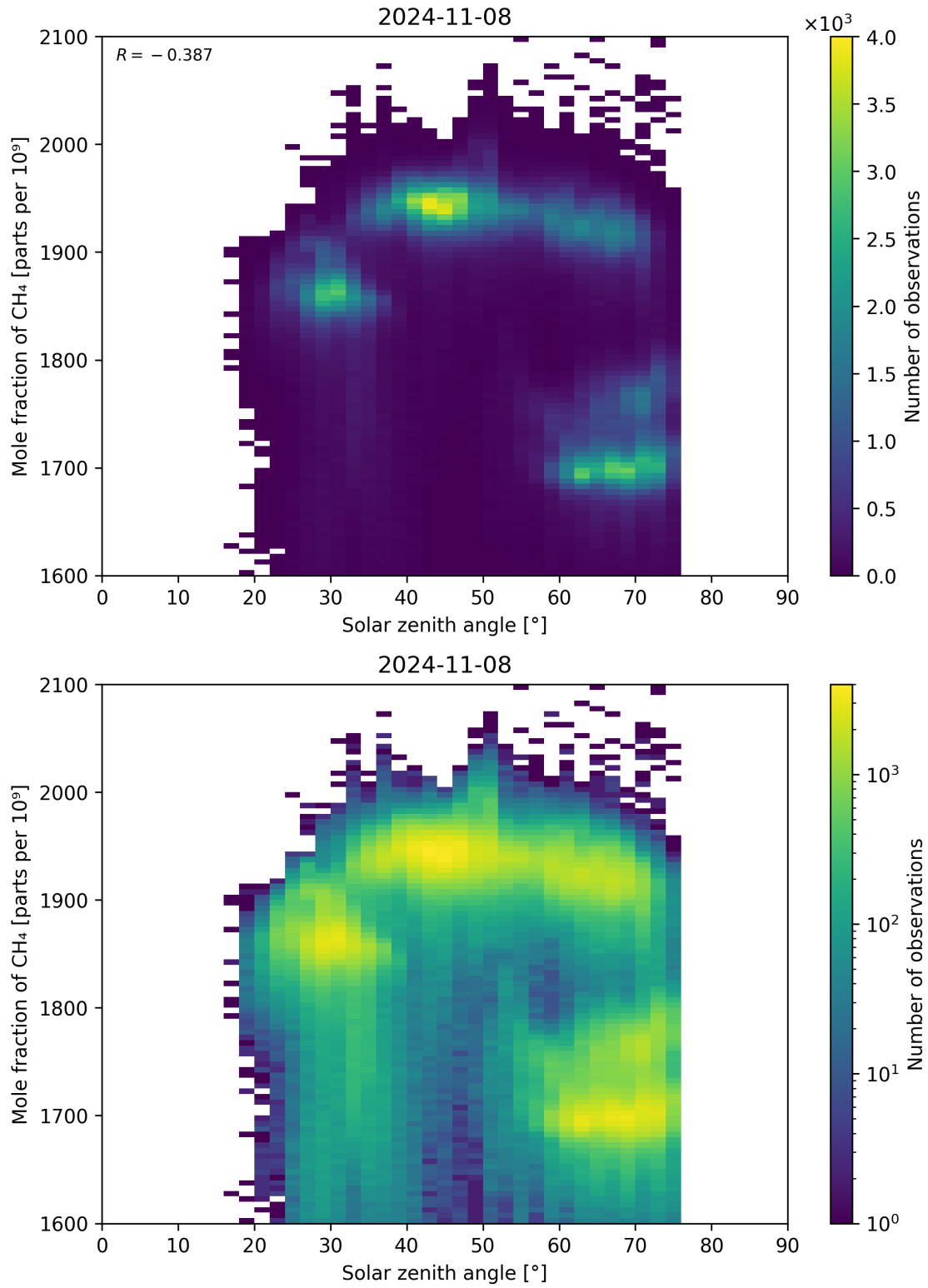
Figure 99: Scatter density plot of “Solar zenith angle” against “Mole fraction of CH 4 ” for 2024-11-07 to 2024-11-09.
