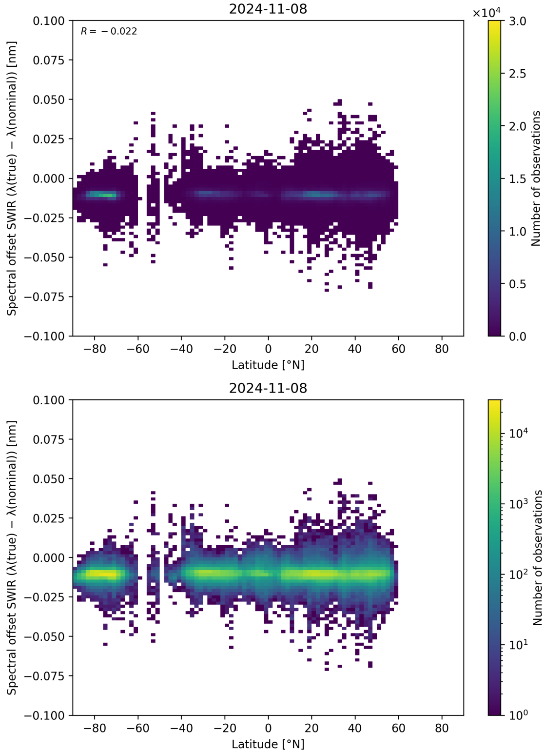
Figure 62: Scatter density plot of “Latitude” against “Spectral offset SWIR ( \lambda_{\text{true}} - \lambda_{\text{nominal}} )” for 2024-11-07 to 2024-11-09.
