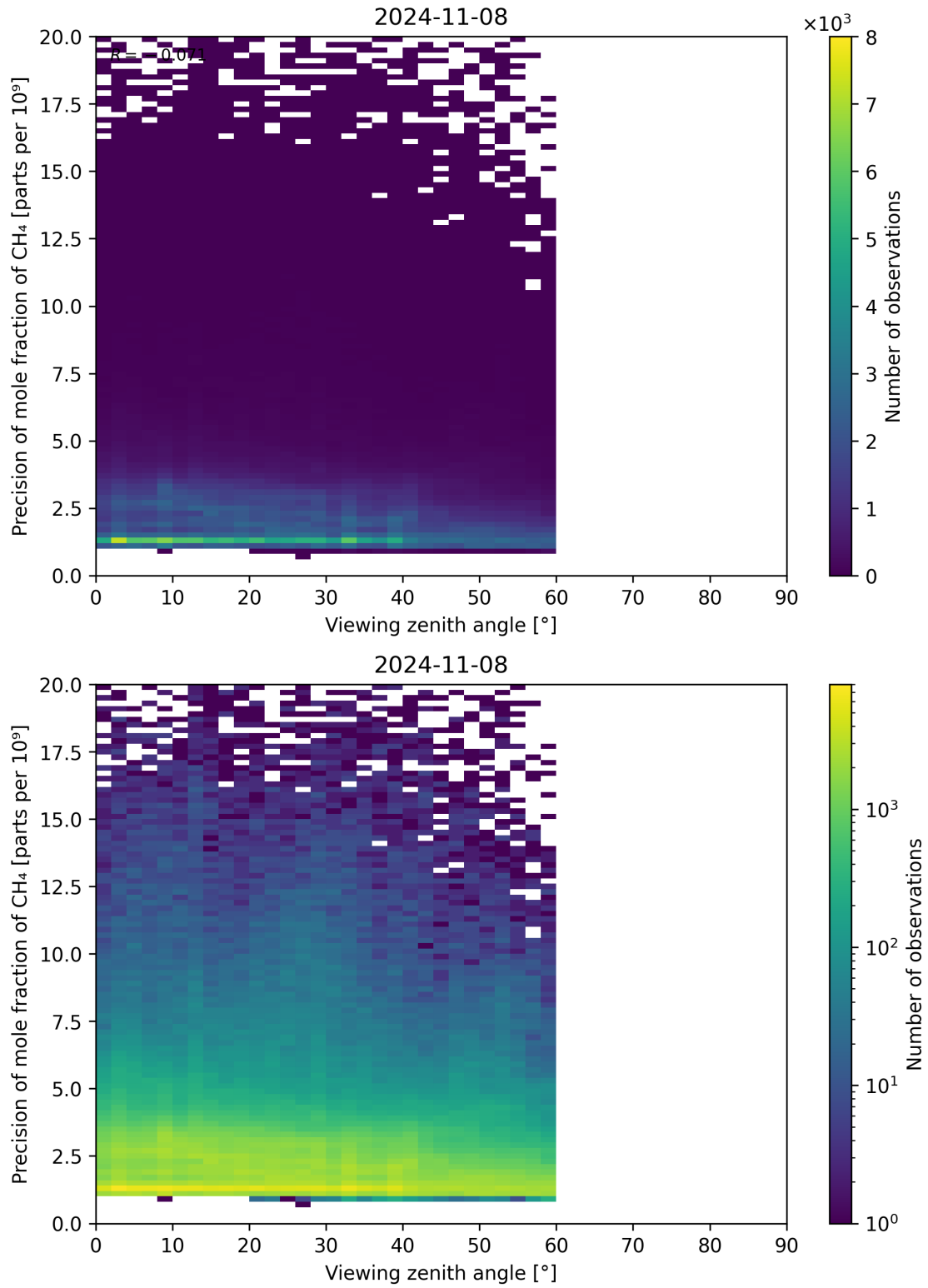
Figure 112: Scatter density plot of “Viewing zenith angle” against “Precision of mole fraction of CH 4 ” for 2024-11-07 to 2024-11-09.
