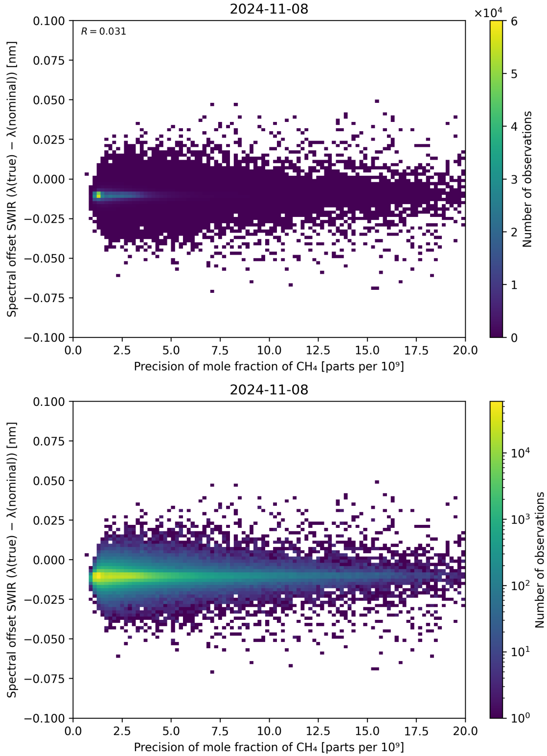
Figure 85: Scatter density plot of “Precision of mole fraction of \text{CH}_4 ” against “Spectral offset SWIR ( \lambda_{\text{true}} - \lambda_{\text{nominal}} )” for 2024-11-07 to 2024-11-09.
