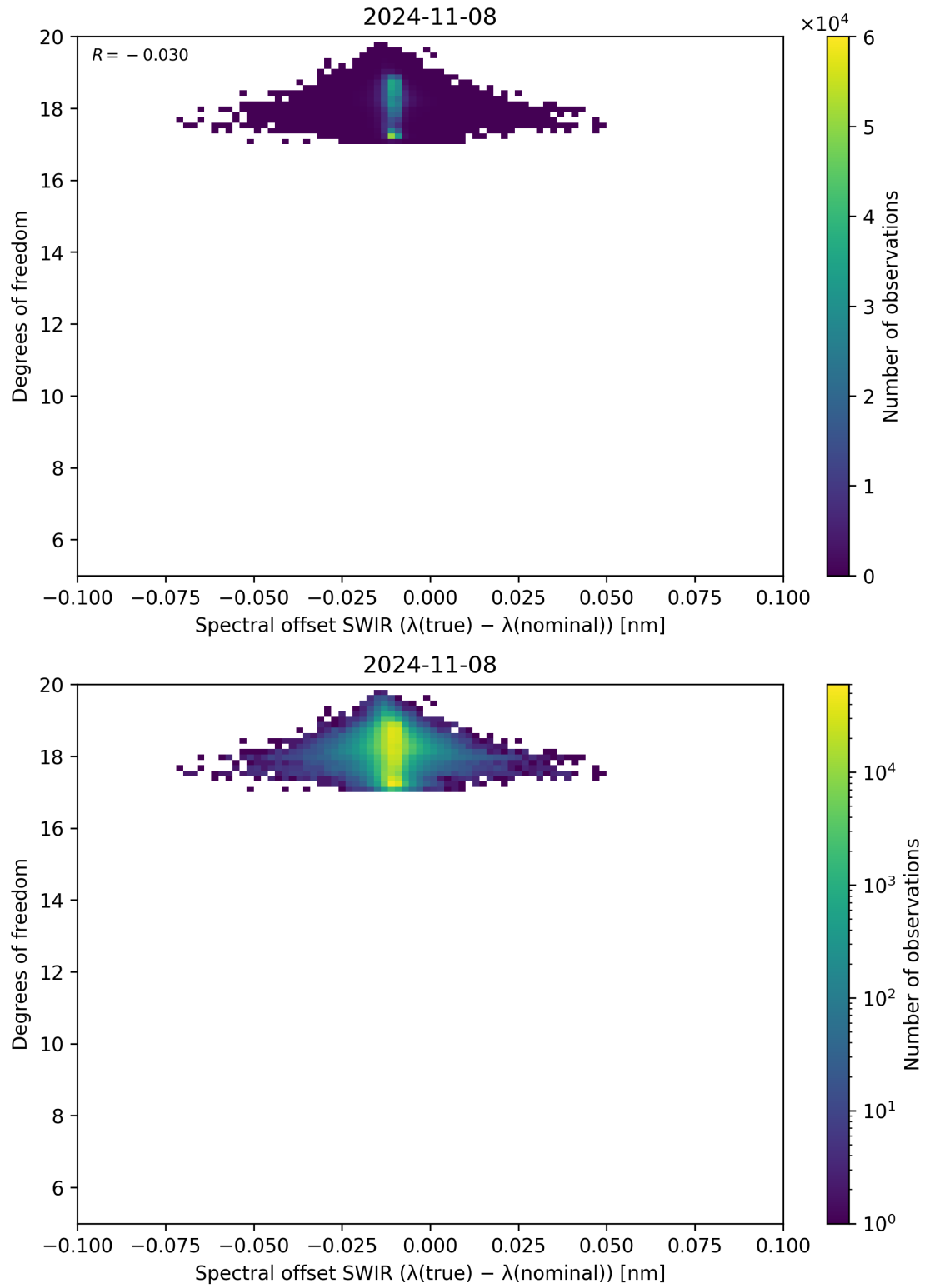
Figure 119: Scatter density plot of “Spectral offset SWIR ( \lambda_{\text{true}} - \lambda_{\text{nominal}} )” against “Degrees of freedom” for 2024-11-07 to 2024-11-09.
