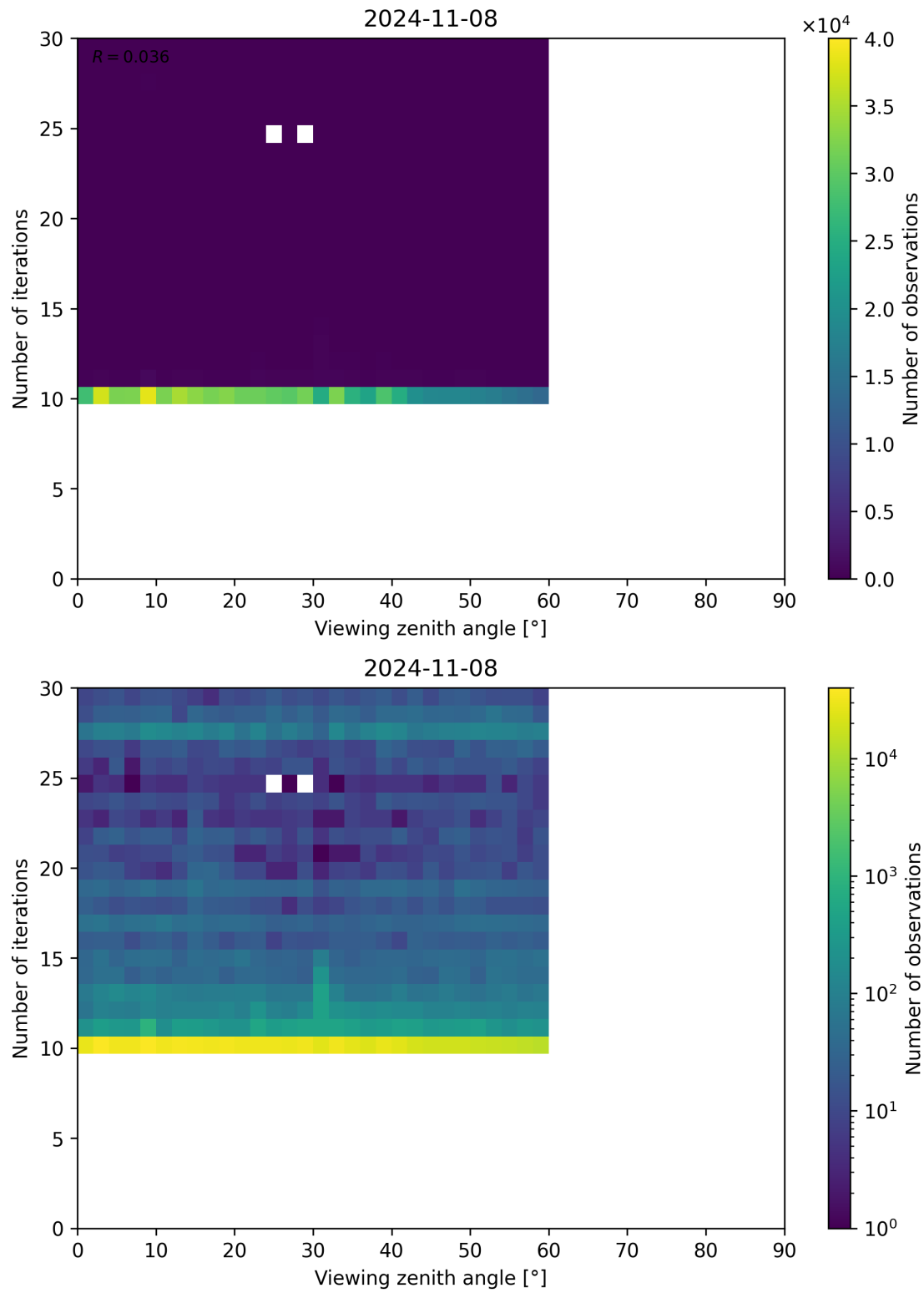
Figure 113: Scatter density plot of “Viewing zenith angle” against “Number of iterations” for 2024-11-07 to 2024-11-09.
