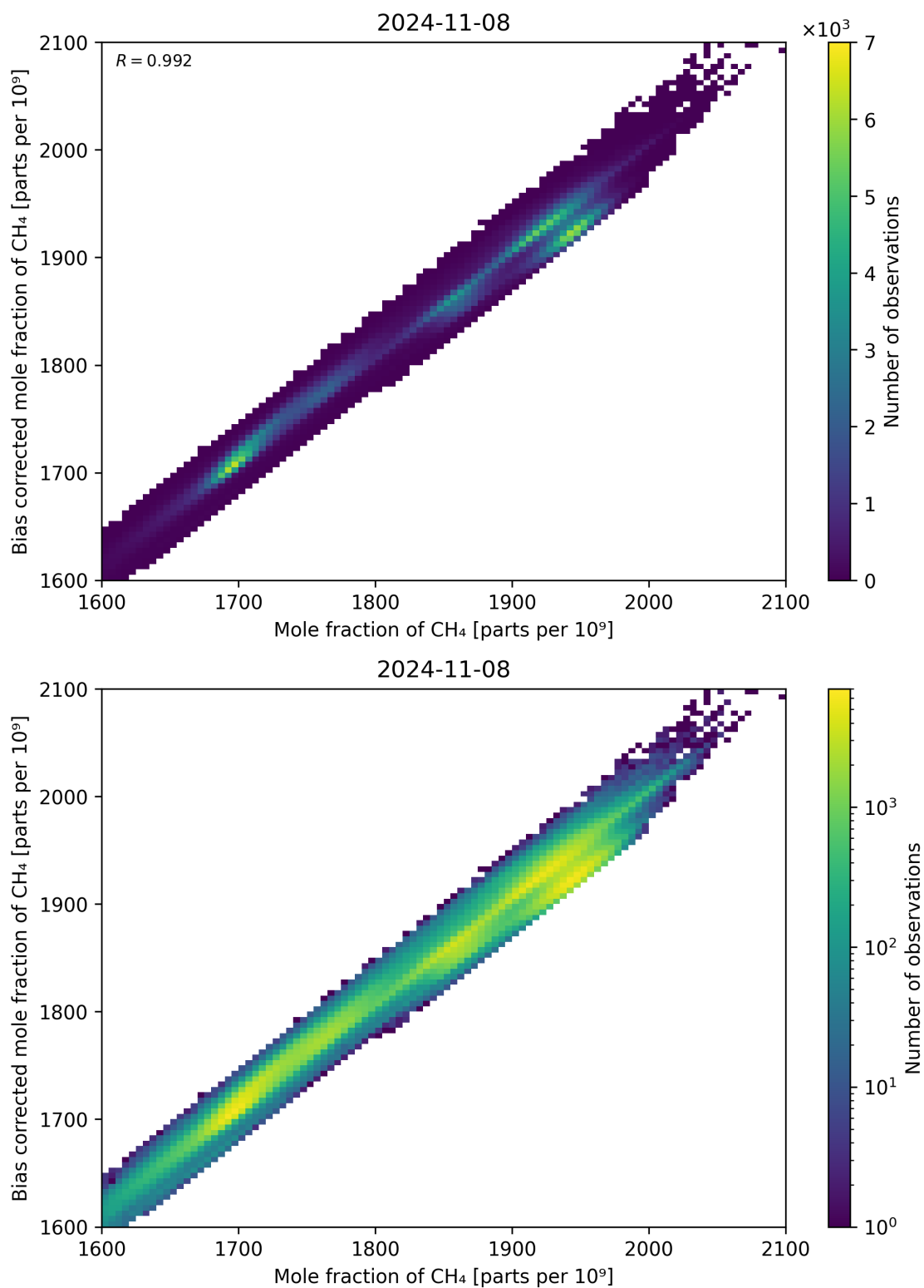
Figure 74: Scatter density plot of “Mole fraction of CH 4 ” against “Bias corrected mole fraction of CH 4 ” for 2024-11-07 to 2024-11-09.
