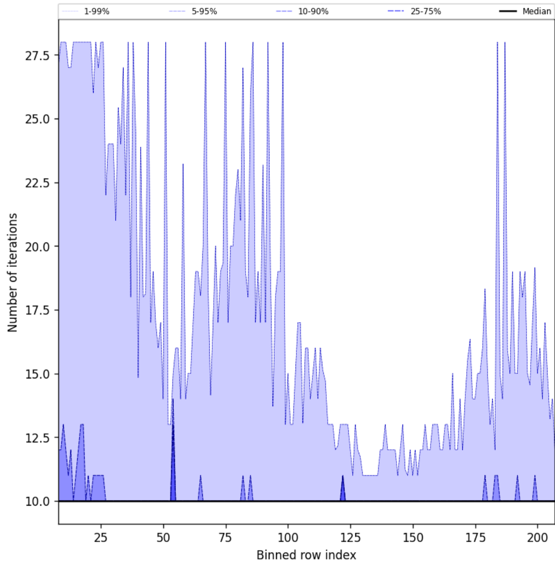
Figure 42: Along track statistics of “Number of iterations” for 2024-11-07 to 2024-11-09
