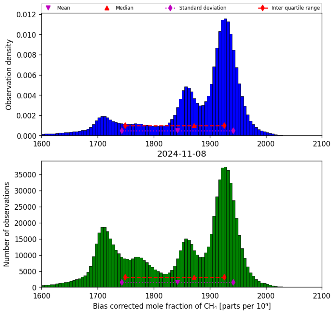
Figure 25: Histogram of “Bias corrected mole fraction of CH 4 ” for 2024-11-07 to 2024-11-09
