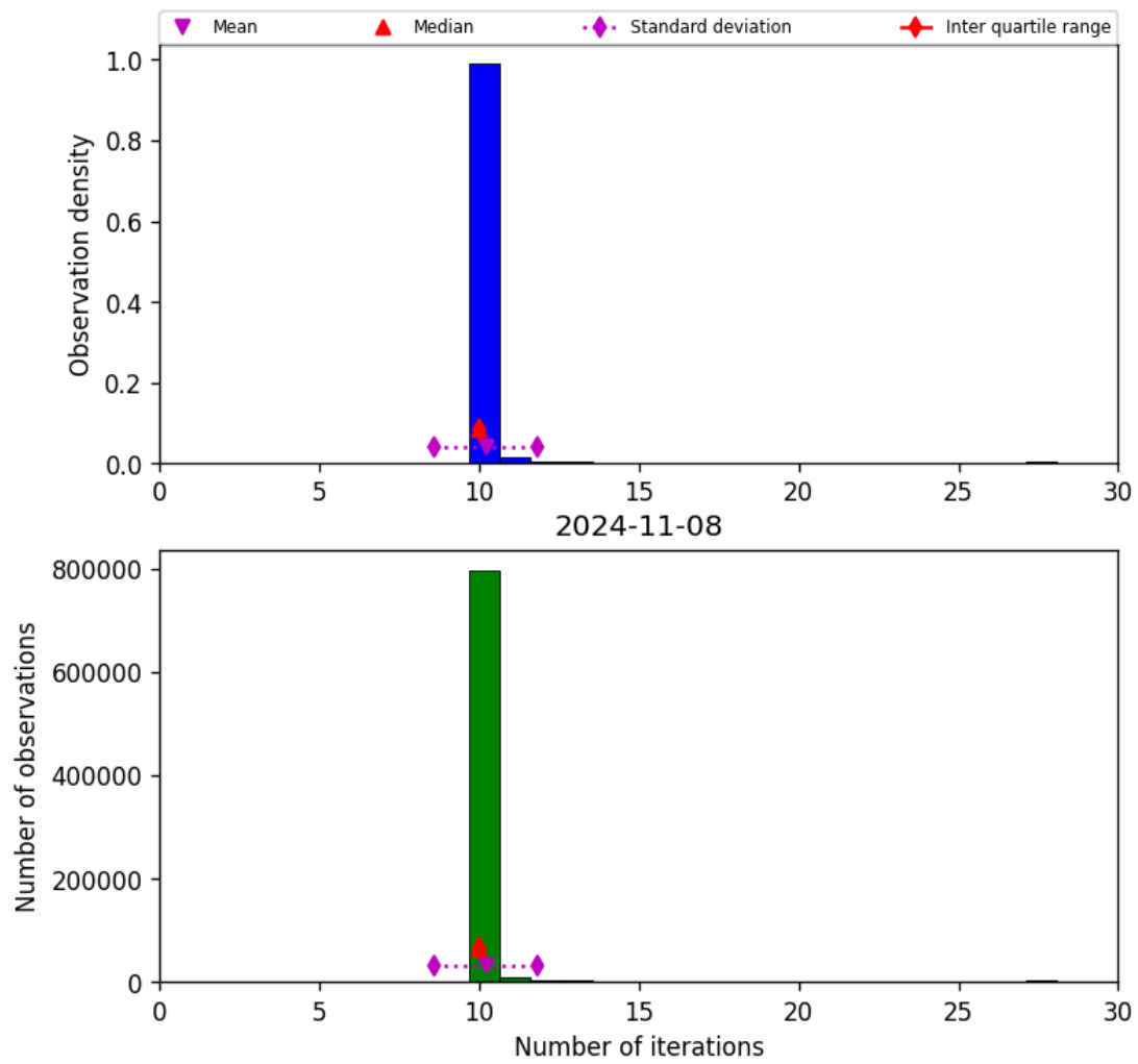
Figure 31: Histogram of “Number of iterations” for 2024-11-07 to 2024-11-09
