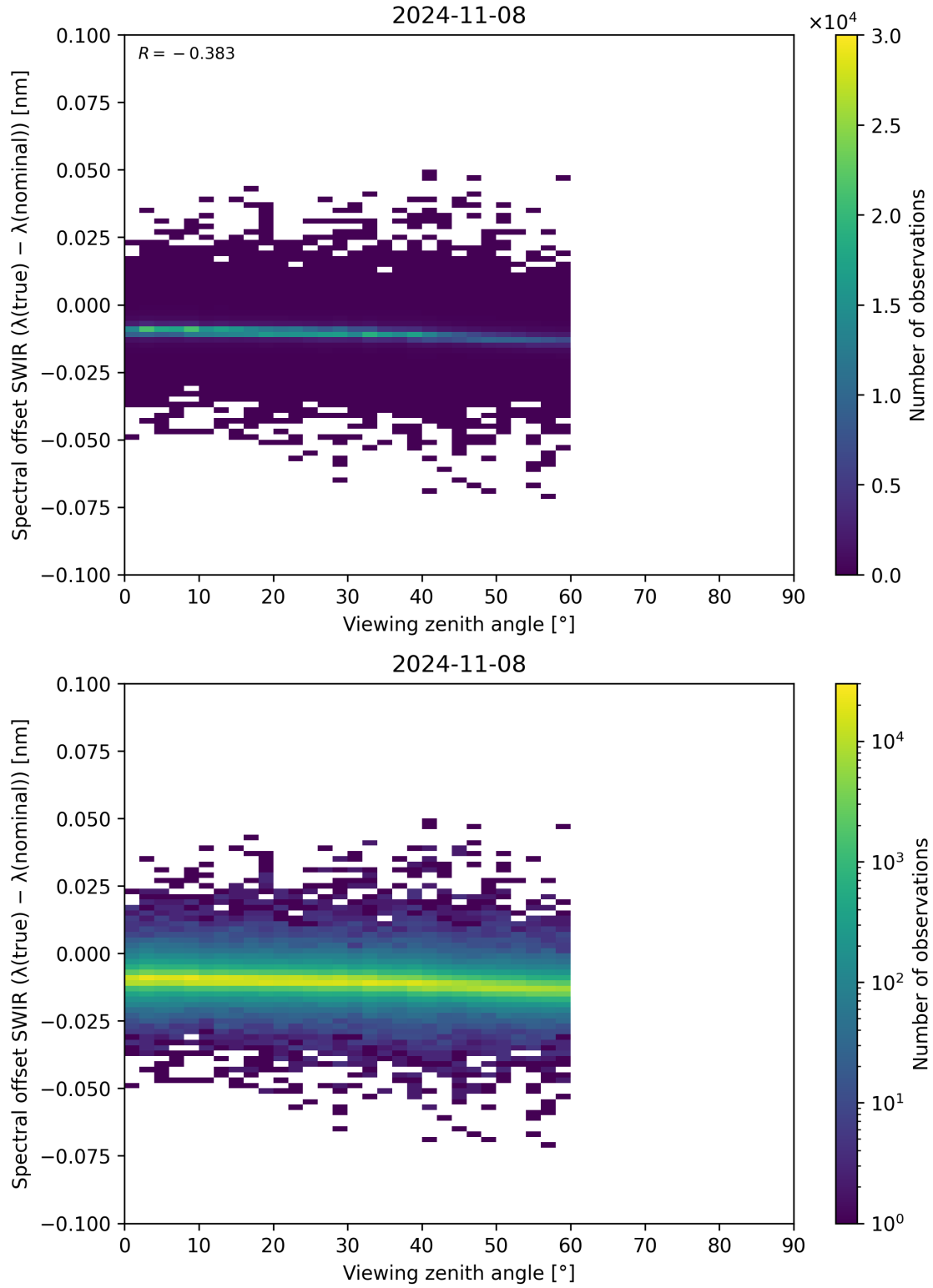
Figure 116: Scatter density plot of “Viewing zenith angle” against “Spectral offset SWIR ( \lambda_{\text{true}} - \lambda_{\text{nominal}} )” for 2024-11-07 to 2024-11-09.
