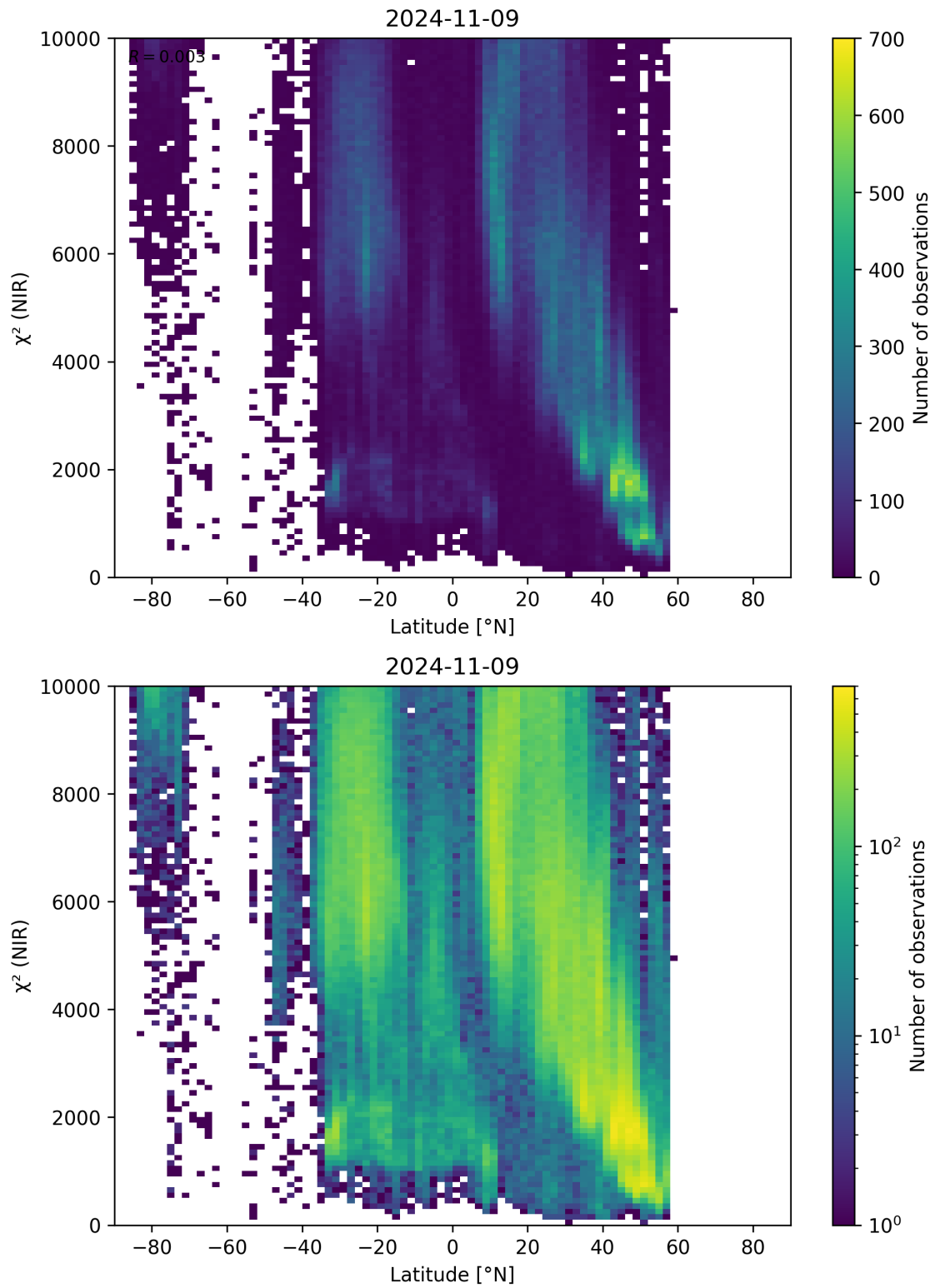
Figure 53: Scatter density plot of “Latitude” against “ \chi^2 (NIR)” for 2024-11-09 to 2024-11-10.
