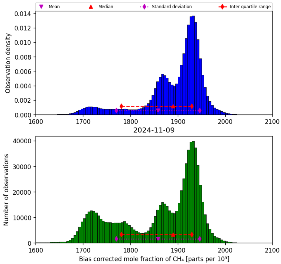
Figure 25: Histogram of “Bias corrected mole fraction of CH 4 ” for 2024-11-09 to 2024-11-10
