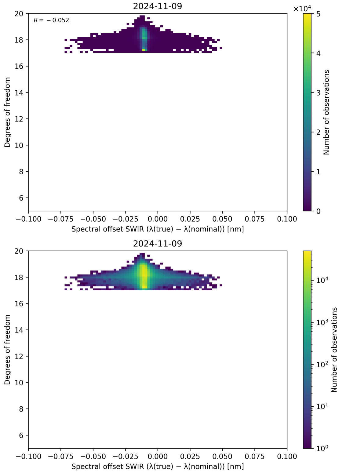
Figure 119: Scatter density plot of “Spectral offset SWIR ( \lambda_{\text{true}} - \lambda_{\text{nominal}} )” against “Degrees of freedom” for 2024-11-09 to 2024-11-10.
