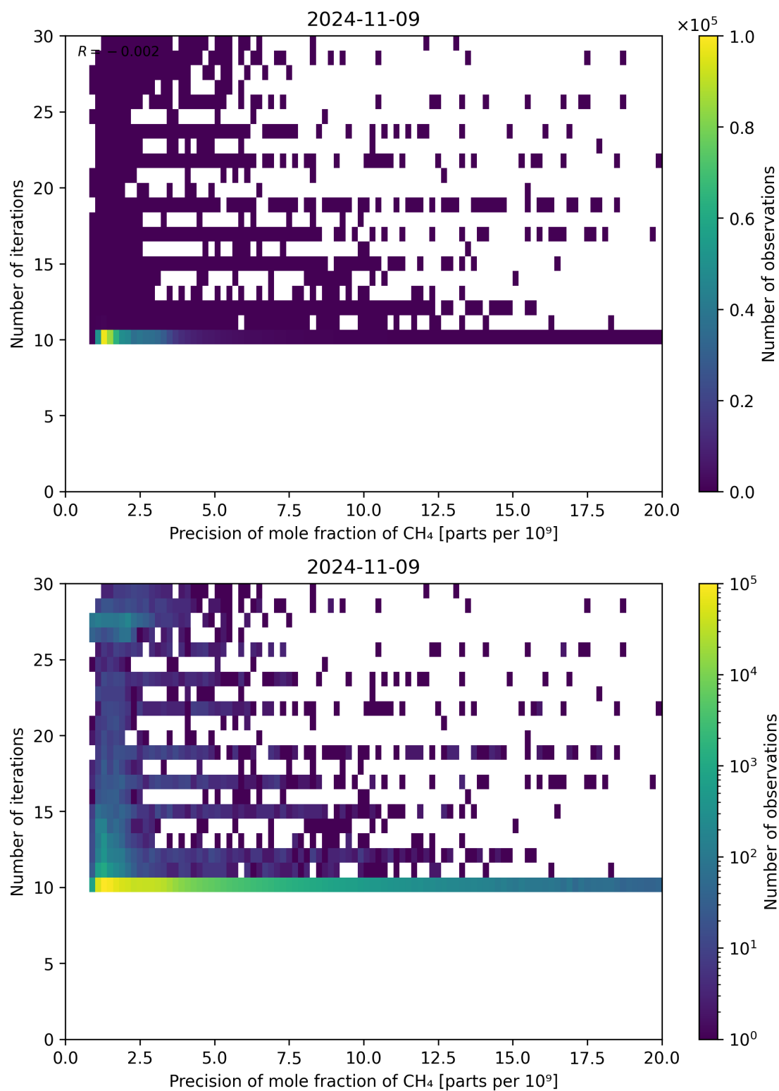
Figure 83: Scatter density plot of “Precision of mole fraction of CH 4 ” against “Number of iterations” for 2024-11-09 to 2024-11-10.
