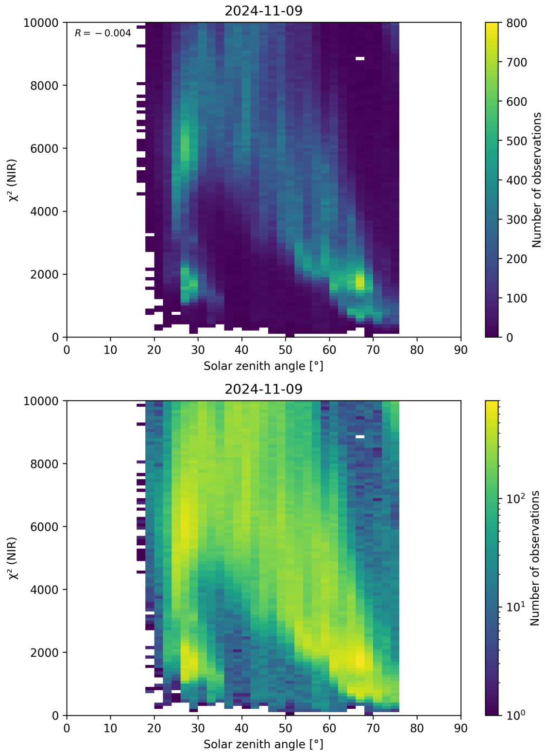
Figure 94: Scatter density plot of “Solar zenith angle” against “ \chi^2 (NIR)” for 2024-11-09 to 2024-11-10.
