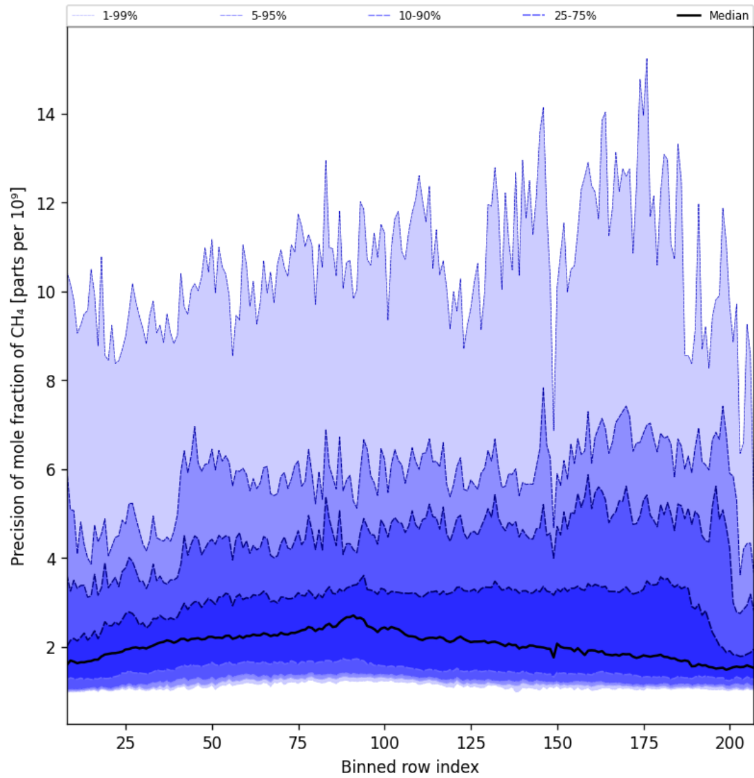
Figure 35: Along track statistics of “Precision of mole fraction of CH 4 ” for 2024-11-09 to 2024-11-10
