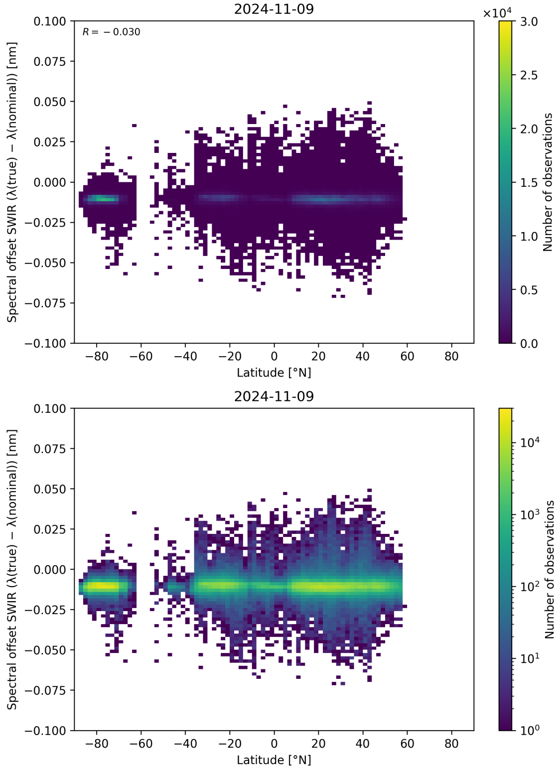
Figure 62: Scatter density plot of “Latitude” against “Spectral offset SWIR ( \lambda_{\text{true}} - \lambda_{\text{nominal}} )” for 2024-11-09 to 2024-11-10.
