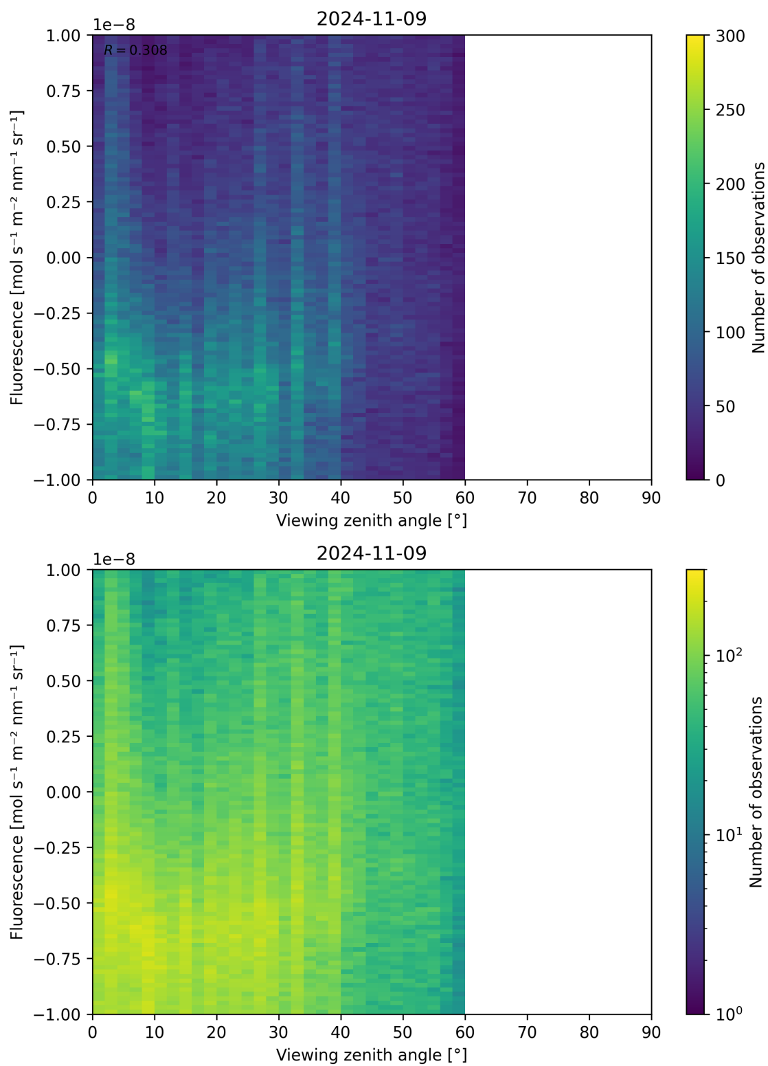
Figure 108: Scatter density plot of “Viewing zenith angle” against “Fluorescence” for 2024-11-09 to 2024-11-10.
