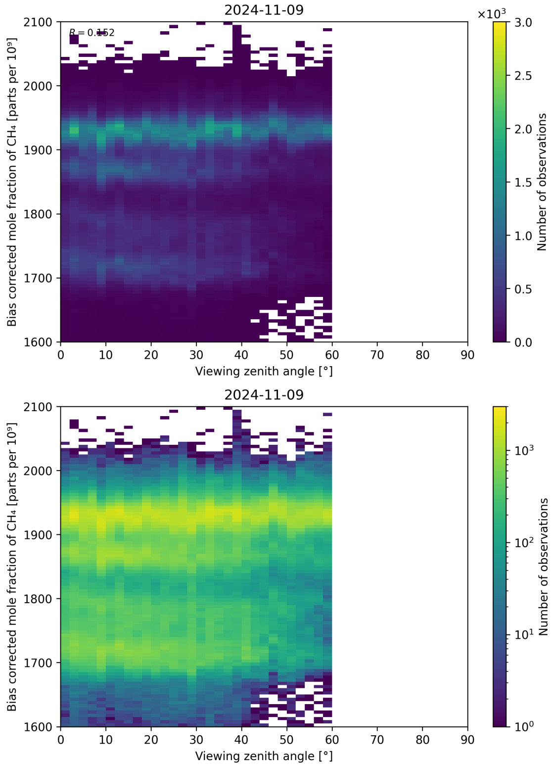
Figure 111: Scatter density plot of “Viewing zenith angle” against “Bias corrected mole fraction of CH 4 ” for 2024-11-09 to 2024-11-10.
