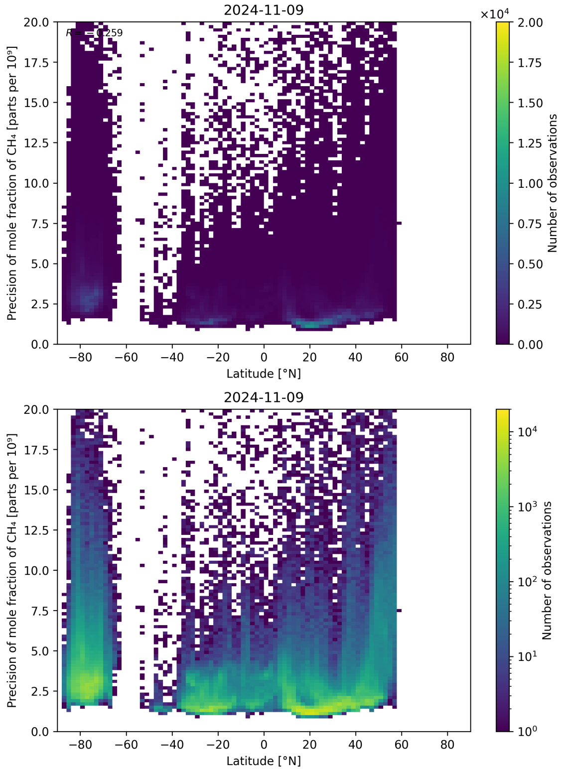
Figure 59: Scatter density plot of “Latitude” against “Precision of mole fraction of \text{CH}_4 ” for 2024-11-09 to 2024-11-10.
