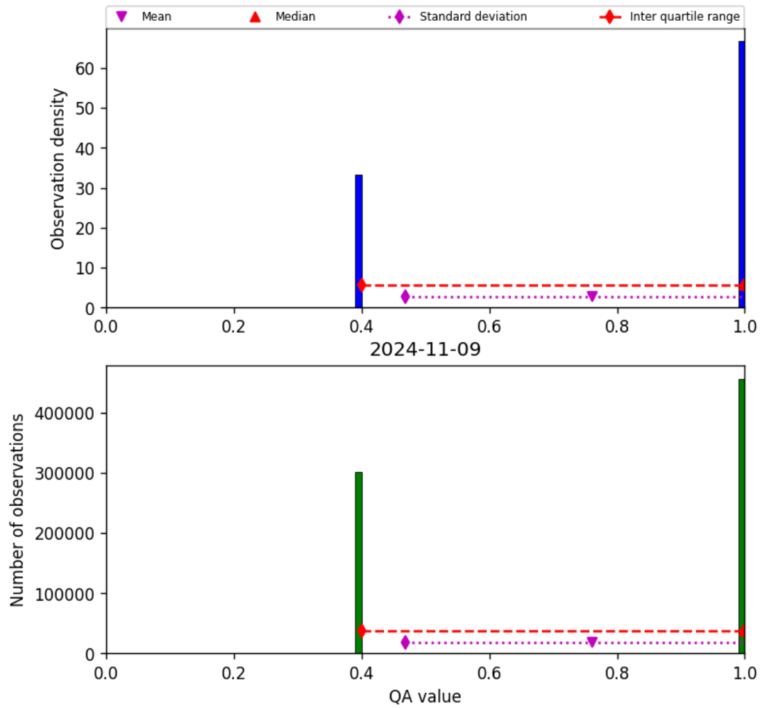
Figure 22: Histogram of “QA value” for 2024-11-09 to 2024-11-10
