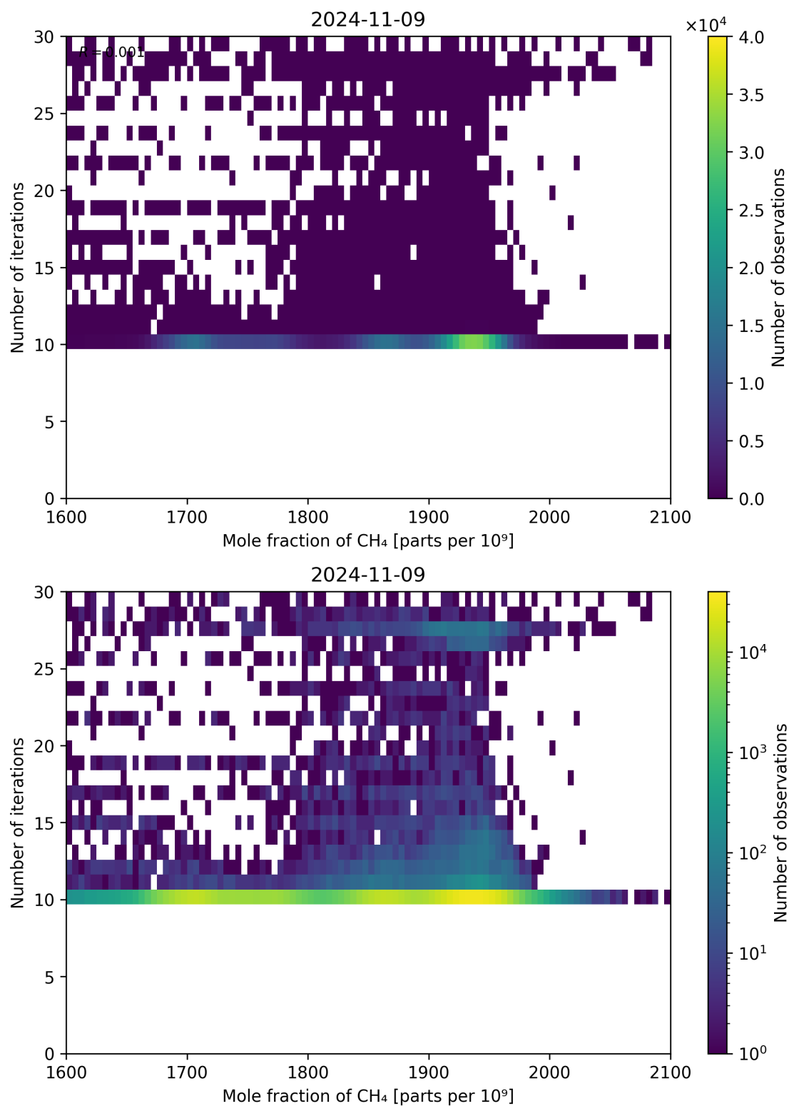
Figure 76: Scatter density plot of “Mole fraction of CH 4 ” against “Number of iterations” for 2024-11-09 to 2024-11-10.
