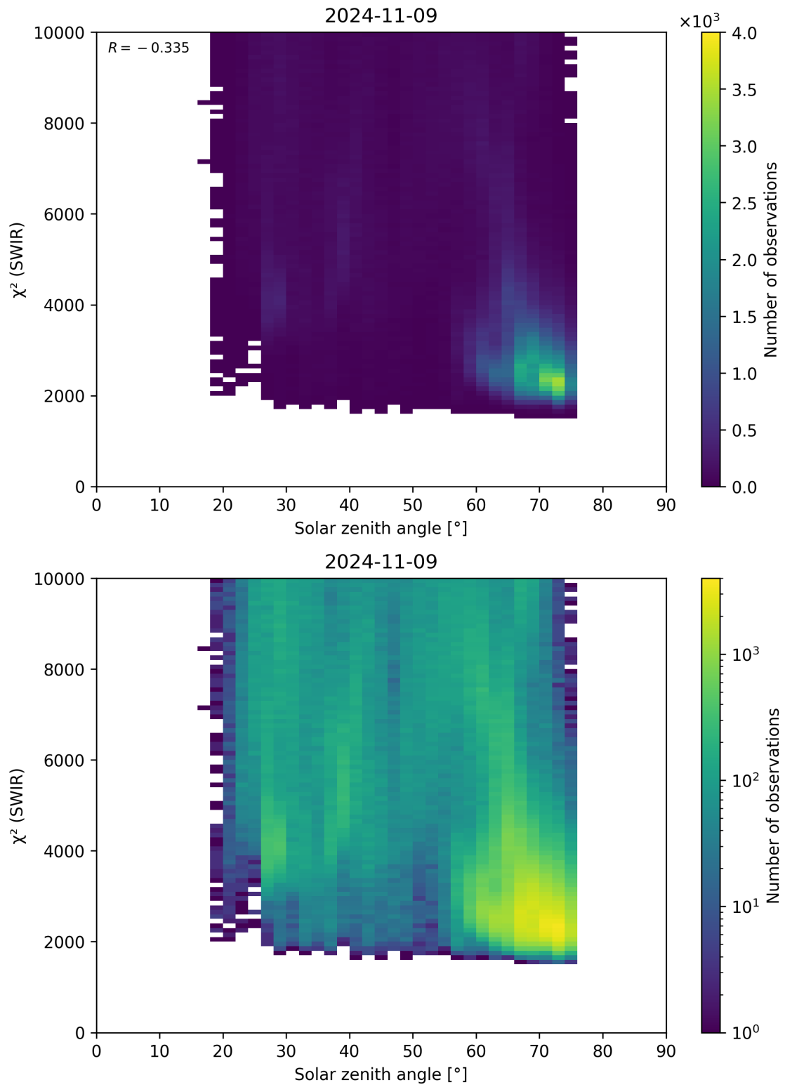
Figure 95: Scatter density plot of “Solar zenith angle” against “ \chi^2 (SWIR)” for 2024-11-09 to 2024-11-10.
