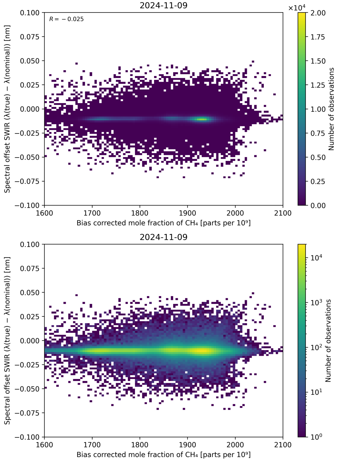
Figure 69: Scatter density plot of “Bias corrected mole fraction of \text{CH}_4 ” against “Spectral offset SWIR ( \lambda_{\text{true}} - \lambda_{\text{nominal}} )” for 2024-11-09 to 2024-11-10.
