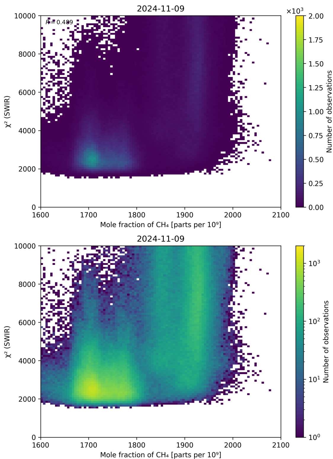
Figure 71: Scatter density plot of “Mole fraction of \text{CH}_4 ” against “ \chi^2 (SWIR)” for 2024-11-09 to 2024-11-10.
