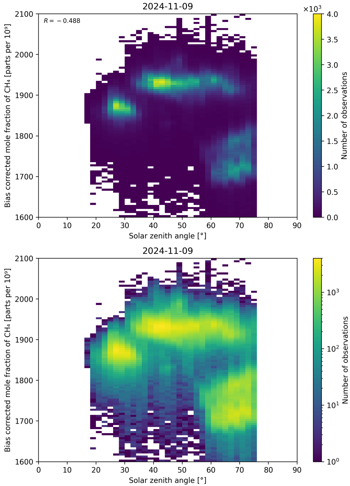
Figure 100: Scatter density plot of “Solar zenith angle” against “Bias corrected mole fraction of CH 4 ” for 2024-11-09 to 2024-11-10.
