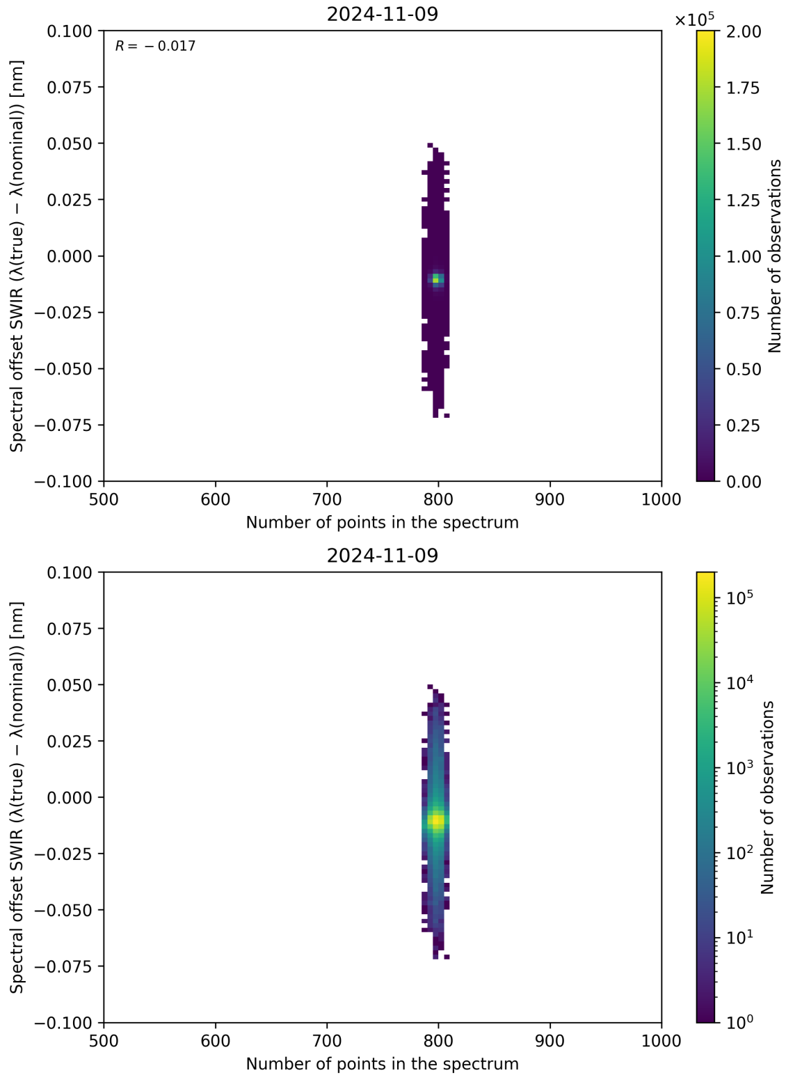
Figure 93: Scatter density plot of “Number of points in the spectrum” against “Spectral offset SWIR ( \lambda_{\text{true}} - \lambda_{\text{nominal}} )” for 2024-11-09 to 2024-11-10.
