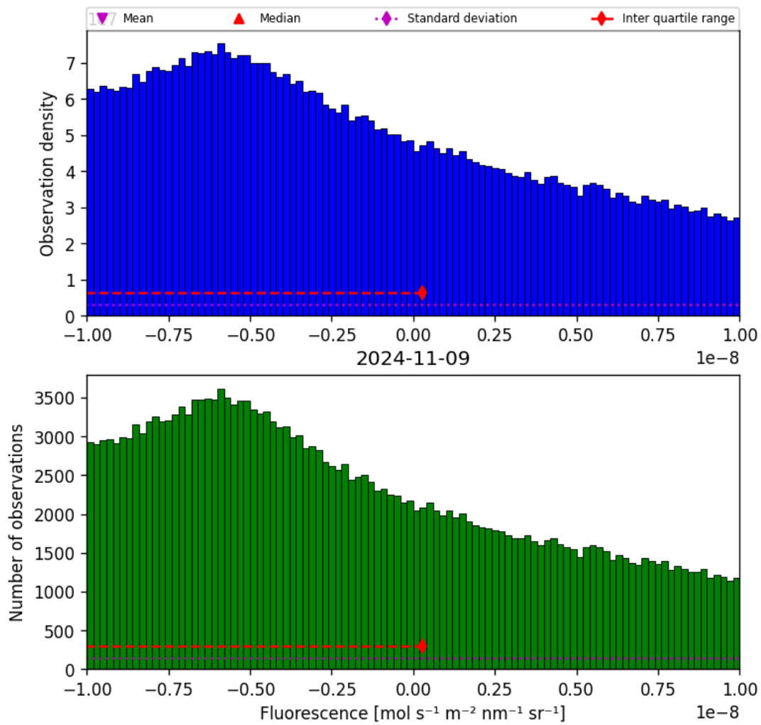
Figure 32: Histogram of “Fluorescence” for 2024-11-09 to 2024-11-10
