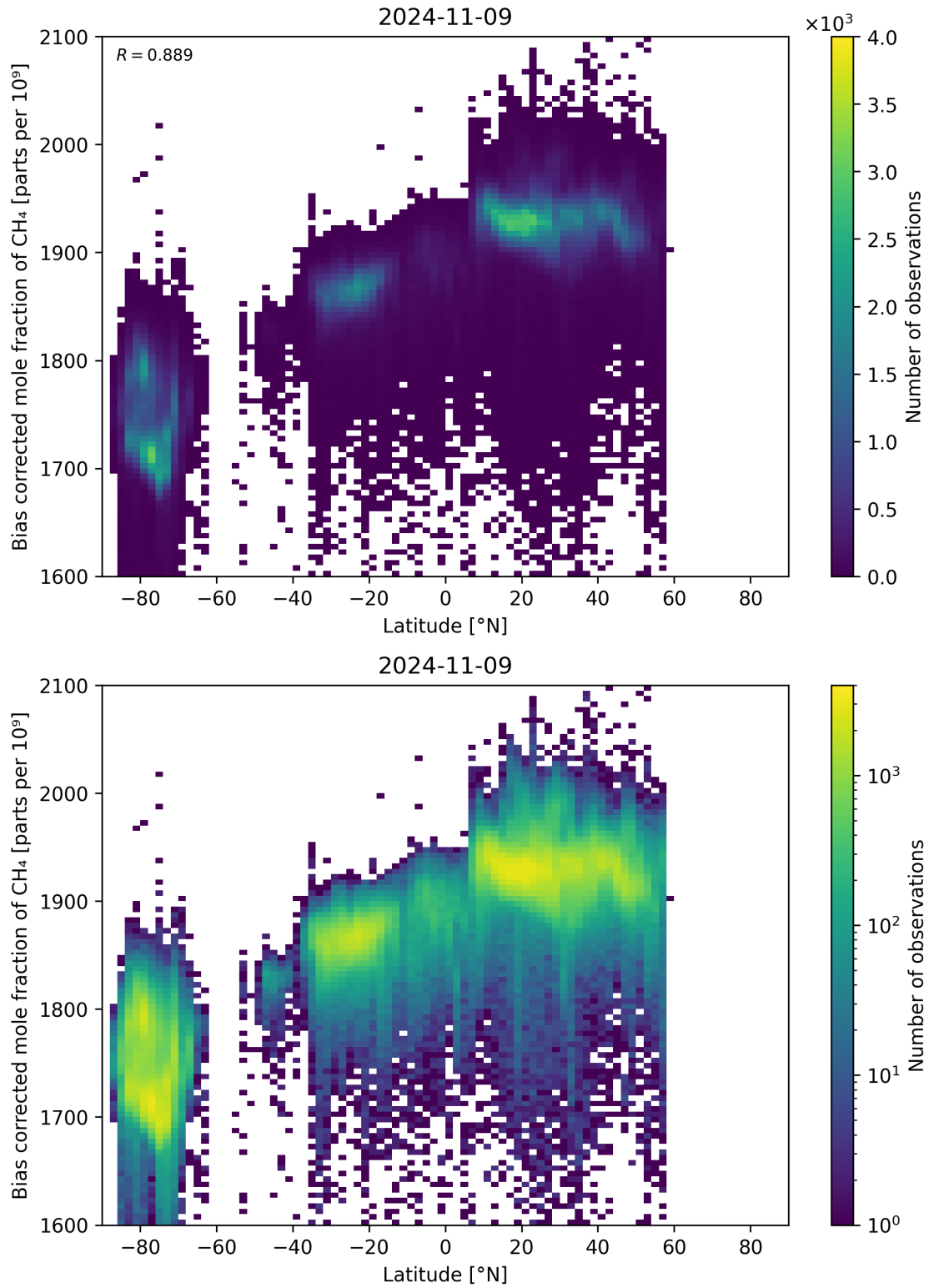
Figure 58: Scatter density plot of “Latitude” against “Bias corrected mole fraction of \text{CH}_4 ” for 2024-11-09 to 2024-11-10.
