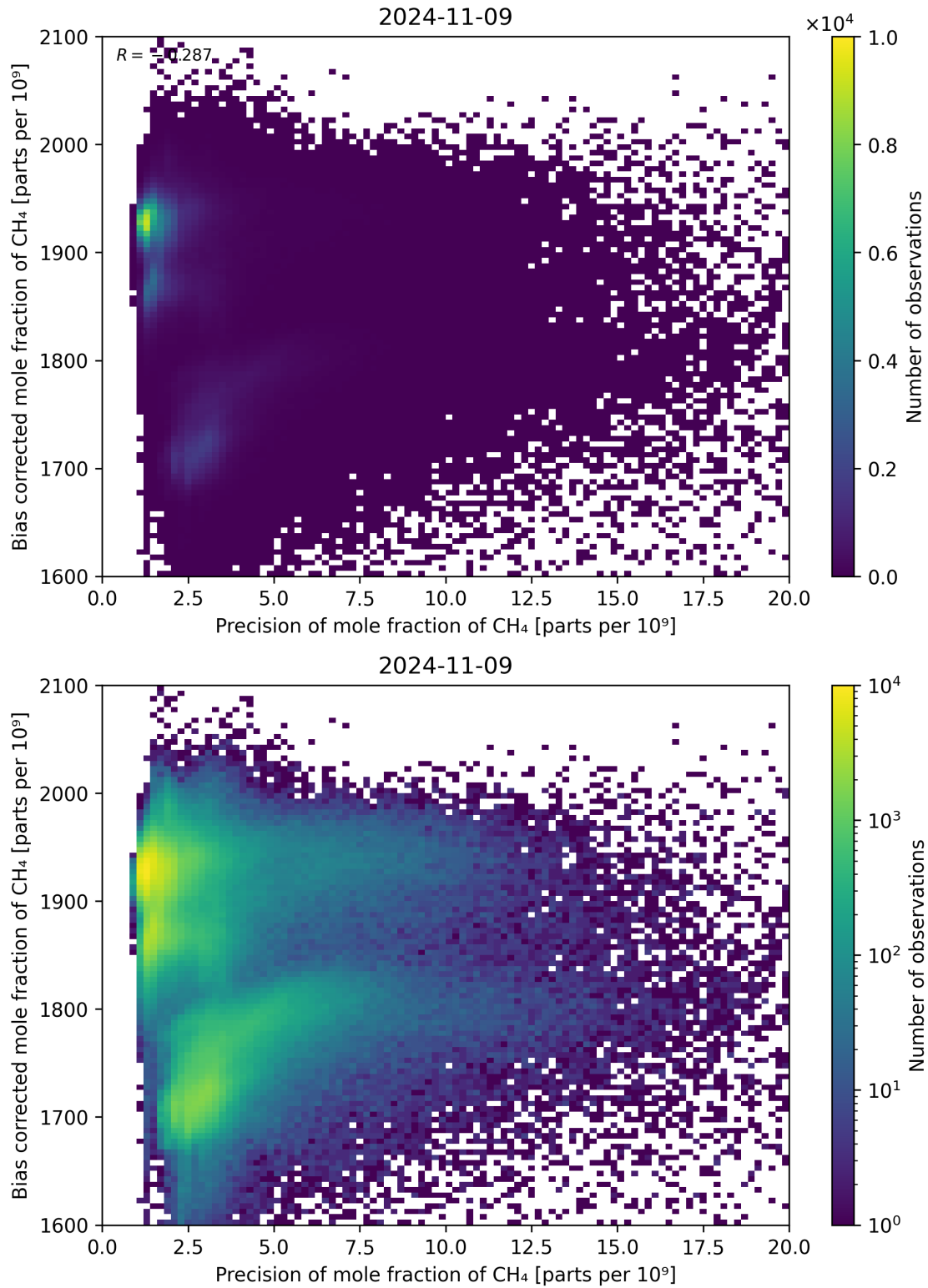
Figure 82: Scatter density plot of “Precision of mole fraction of CH 4 ” against “Bias corrected mole fraction of CH 4 ” for 2024-11-09 to 2024-11-10.
