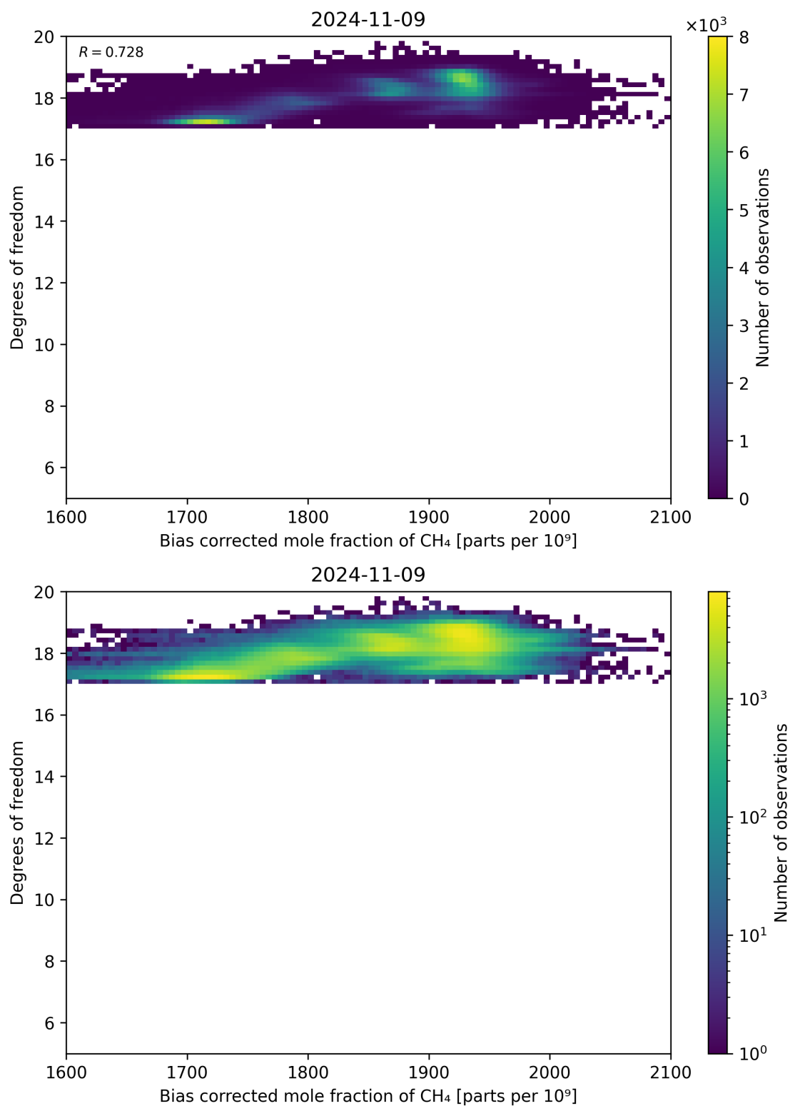
Figure 65: Scatter density plot of “Bias corrected mole fraction of CH 4 ” against “Degrees of freedom” for 2024-11-09 to 2024-11-10.
