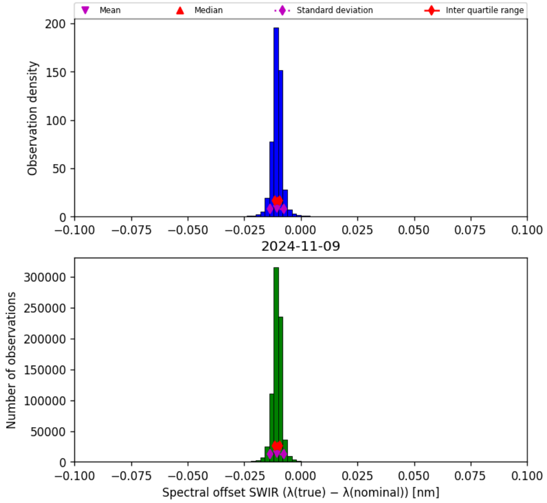
Figure 27: Histogram of “Spectral offset SWIR ( \lambda_{\text{true}} - \lambda_{\text{nominal}} )” for 2024-11-09 to 2024-11-10
