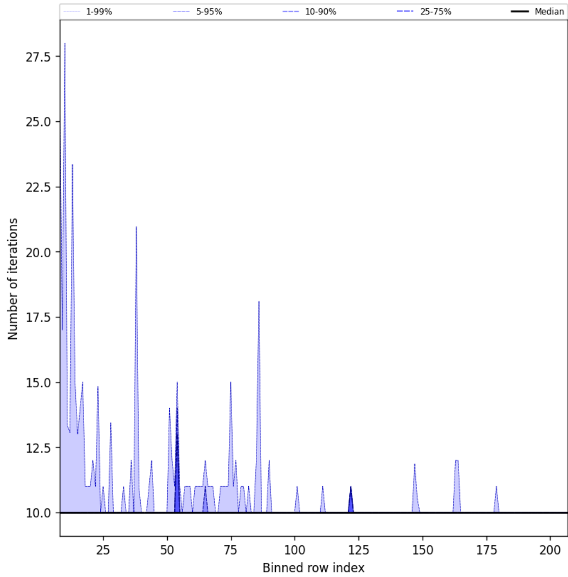
Figure 42: Along track statistics of “Number of iterations” for 2024-11-09 to 2024-11-10
