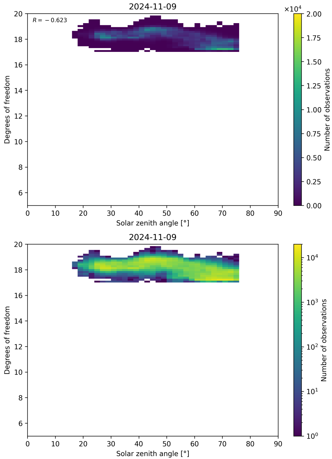
Figure 96: Scatter density plot of “Solar zenith angle” against “Degrees of freedom” for 2024-11-09 to 2024-11-10.
