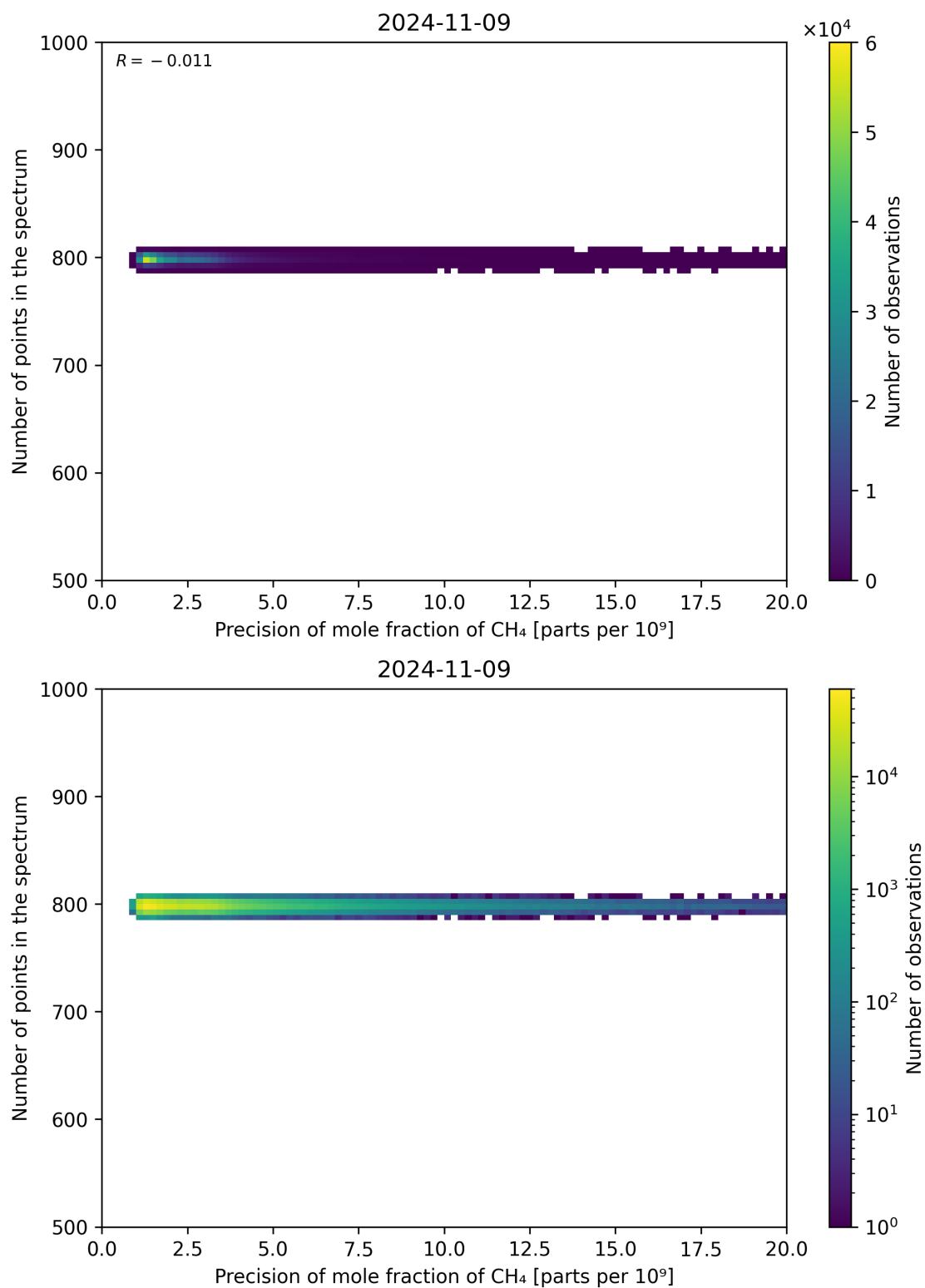
Figure 84: Scatter density plot of “Precision of mole fraction of CH 4 ” against “Number of points in the spectrum” for 2024-11-09 to 2024-11-10.
