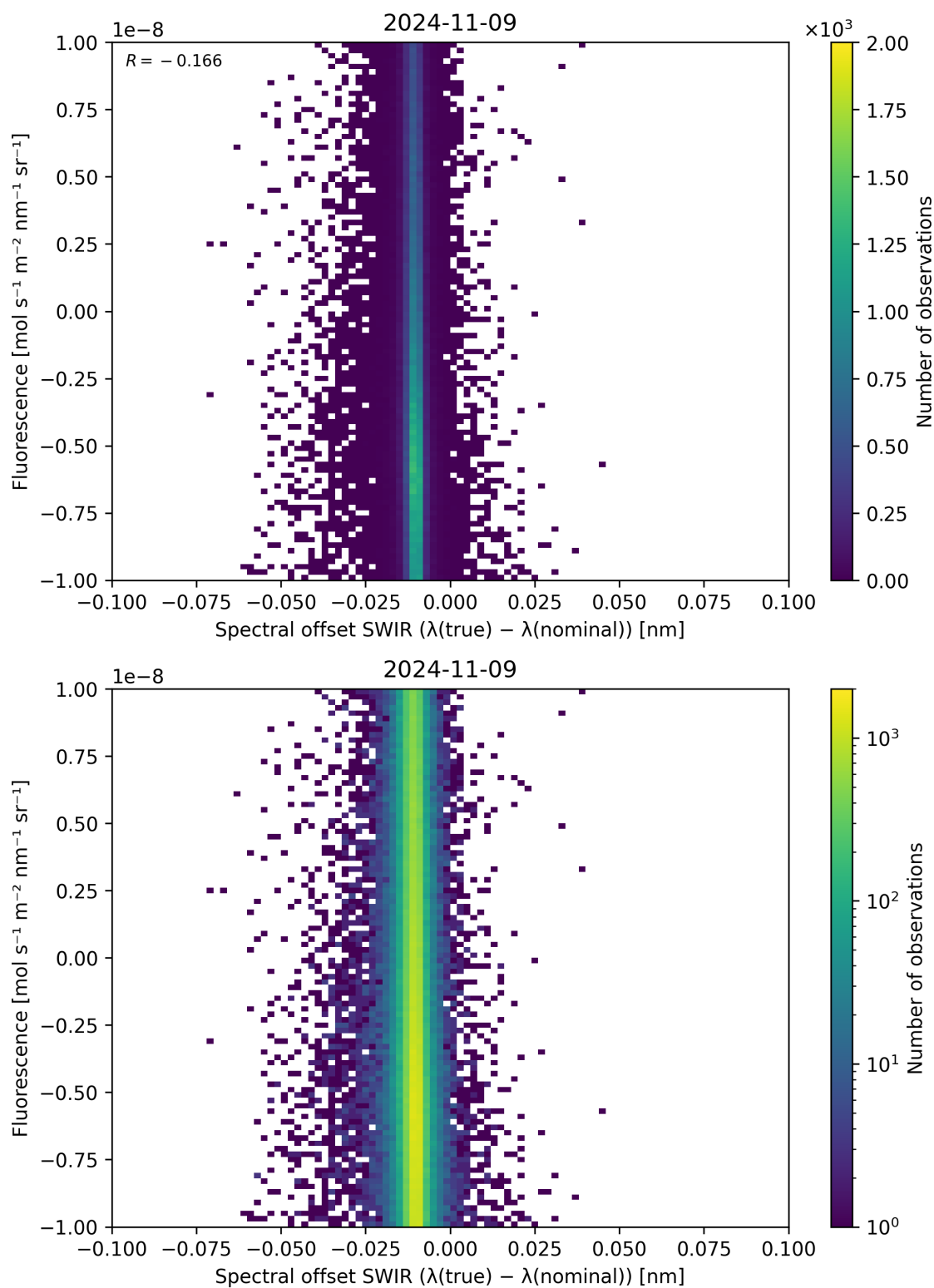
Figure 120: Scatter density plot of “Spectral offset SWIR ( \lambda_{\text{true}} - \lambda_{\text{nominal}} )” against “Fluorescence” for 2024-11-09 to 2024-11-10.
