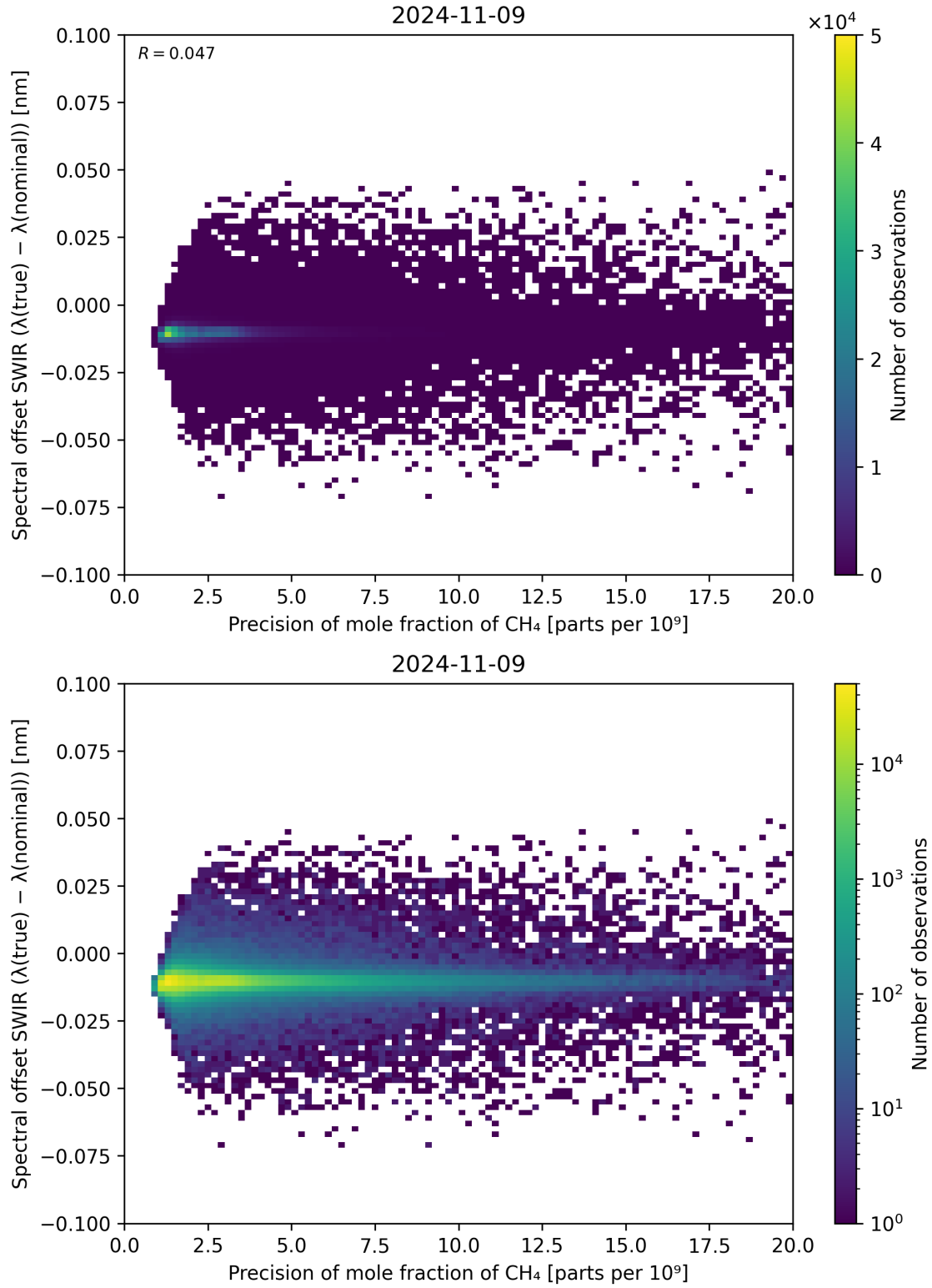
Figure 85: Scatter density plot of “Precision of mole fraction of \text{CH}_4 ” against “Spectral offset SWIR ( \lambda_{\text{true}} - \lambda_{\text{nominal}} )” for 2024-11-09 to 2024-11-10.
