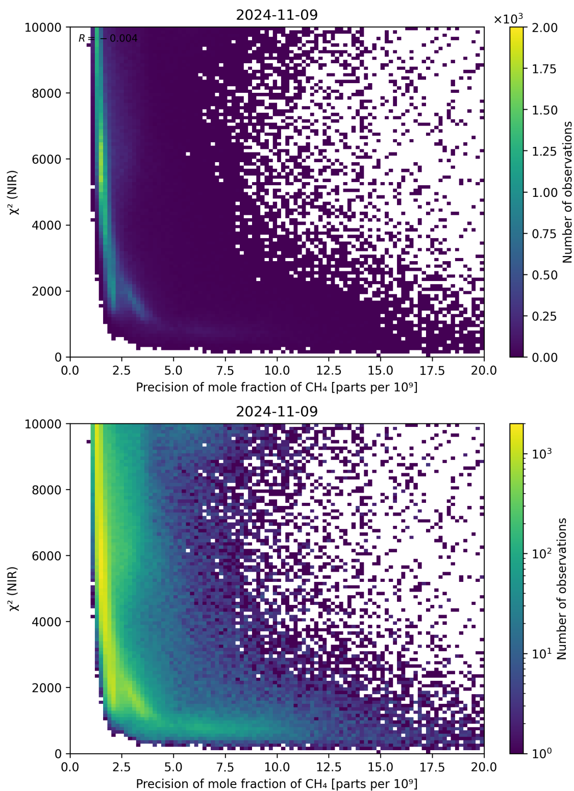
Figure 78: Scatter density plot of “Precision of mole fraction of CH 4 ” against “ \chi^2 (NIR)” for 2024-11-09 to 2024-11-10.
