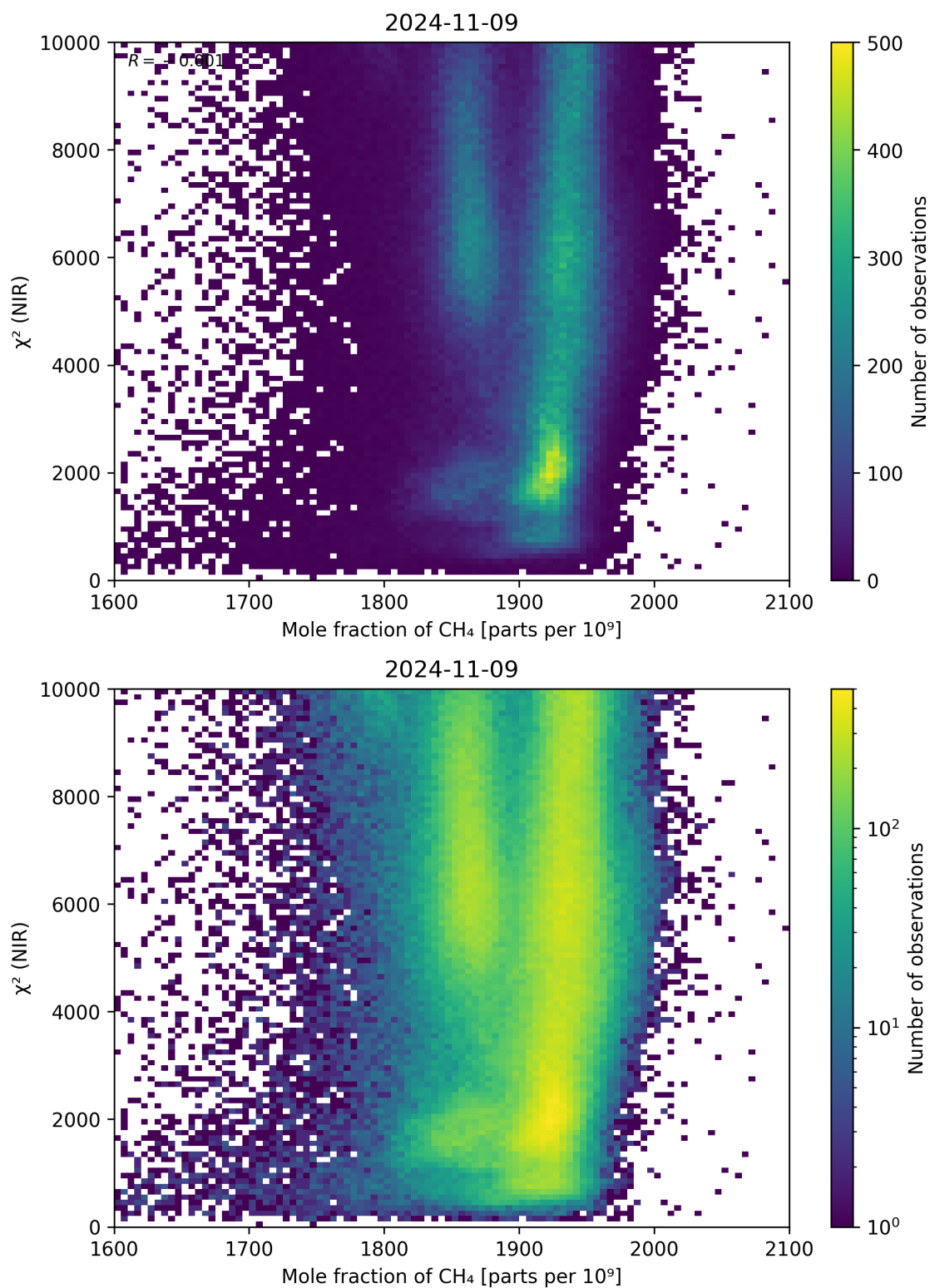
Figure 70: Scatter density plot of “Mole fraction of \text{CH}_4 ” against “ \chi^2 (NIR)” for 2024-11-09 to 2024-11-10.
