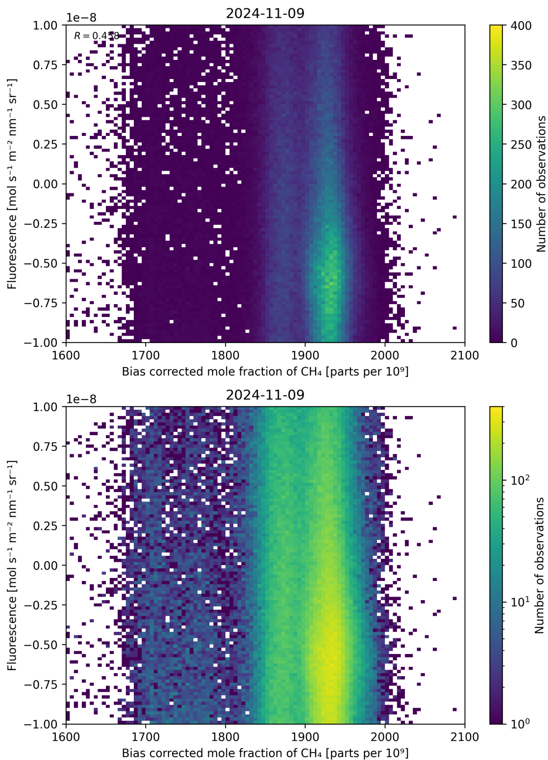
Figure 66: Scatter density plot of “Bias corrected mole fraction of \text{CH}_4 ” against “Fluorescence” for 2024-11-09 to 2024-11-10.
