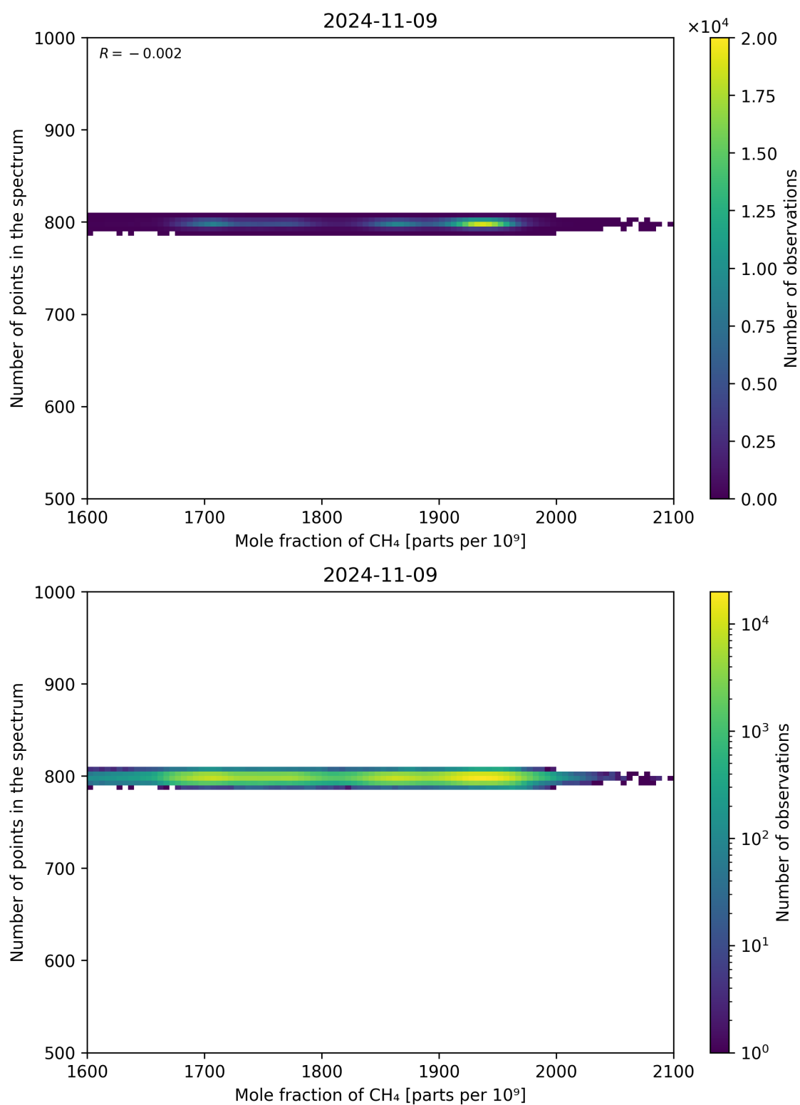
Figure 77: Scatter density plot of “Mole fraction of CH 4 ” against “Number of points in the spectrum” for 2024-11-09 to 2024-11-10.
