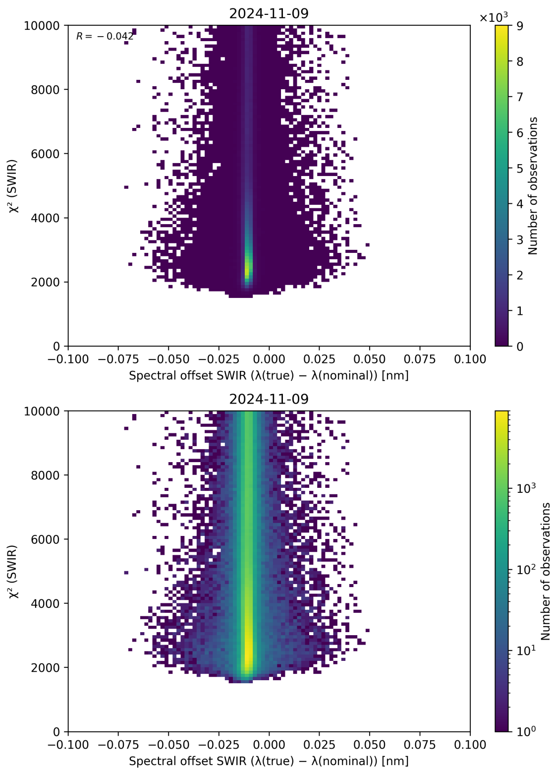
Figure 118: Scatter density plot of “Spectral offset SWIR ( \lambda_{\text{true}} - \lambda_{\text{nominal}} )” against “ \chi^2 (SWIR)” for 2024-11-09 to 2024-11-10.
