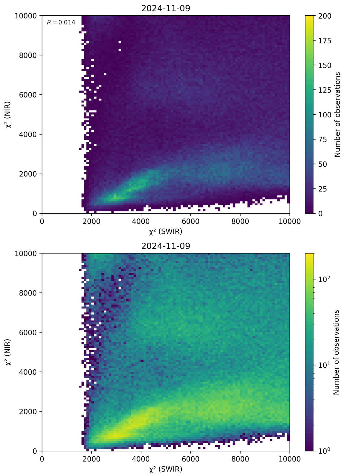
Figure 47: Scatter density plot of “ \chi^2 (SWIR)” against “ \chi^2 (NIR)” for 2024-11-09 to 2024-11-10.
