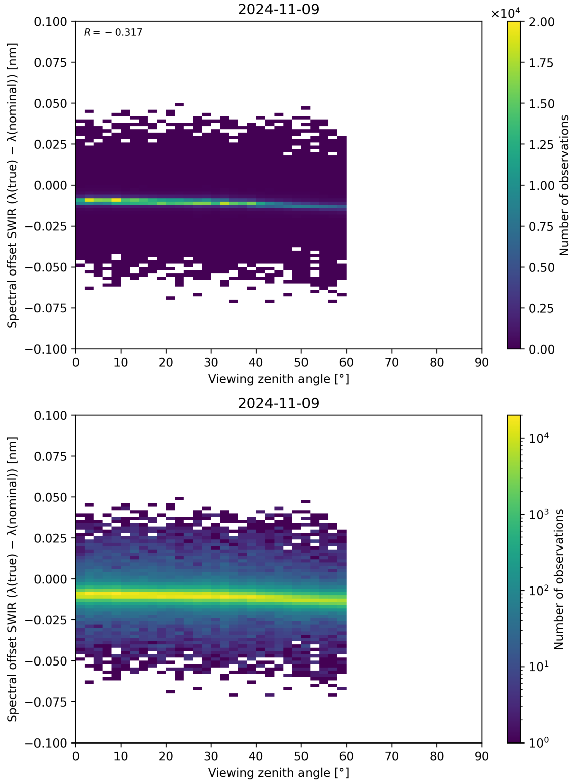
Figure 116: Scatter density plot of “Viewing zenith angle” against “Spectral offset SWIR ( \lambda_{\text{true}} - \lambda_{\text{nominal}} )” for 2024-11-09 to 2024-11-10.
