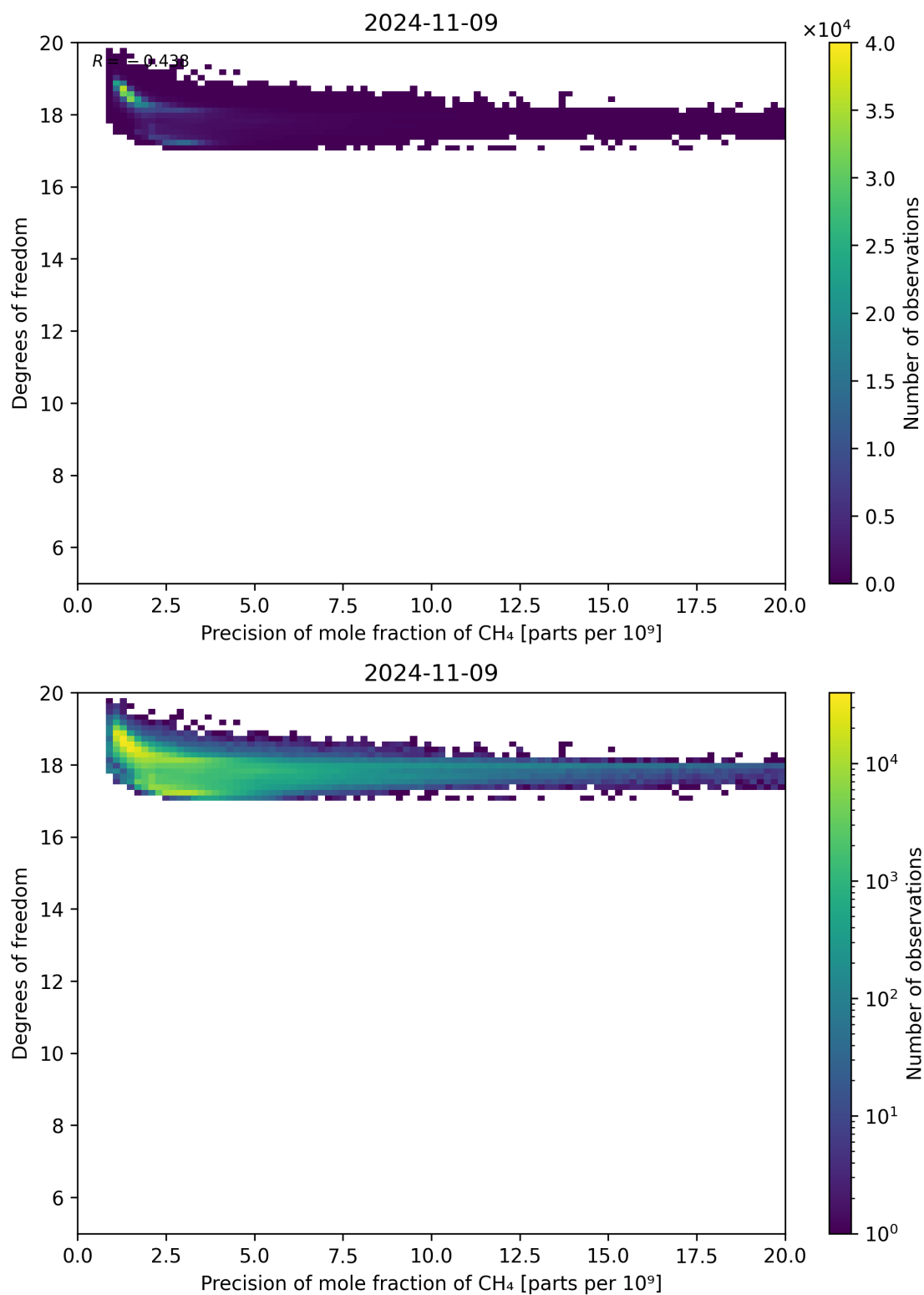
Figure 80: Scatter density plot of “Precision of mole fraction of CH 4 ” against “Degrees of freedom” for 2024-11-09 to 2024-11-10.
