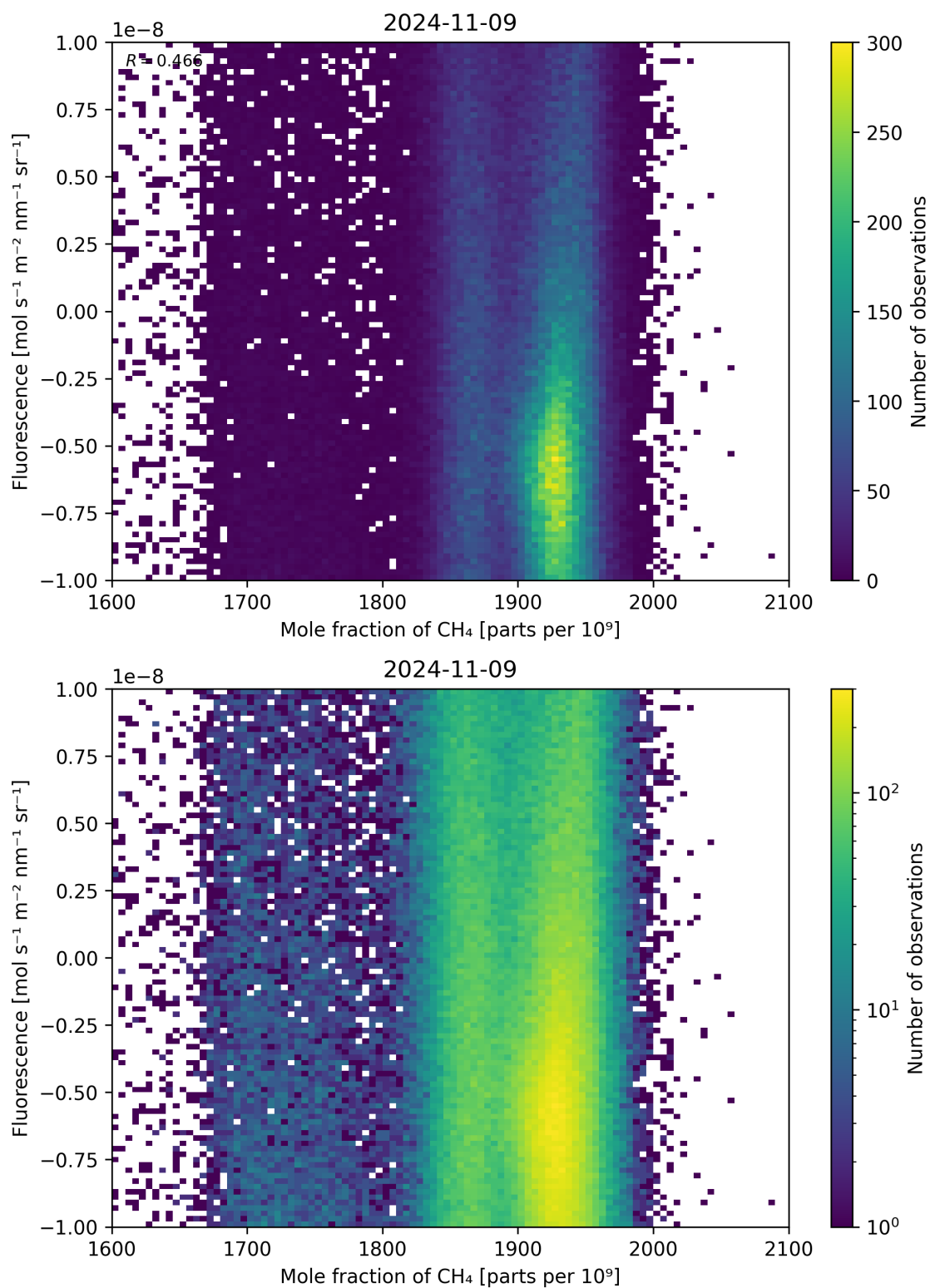
Figure 73: Scatter density plot of “Mole fraction of \text{CH}_4 ” against “Fluorescence” for 2024-11-09 to 2024-11-10.
