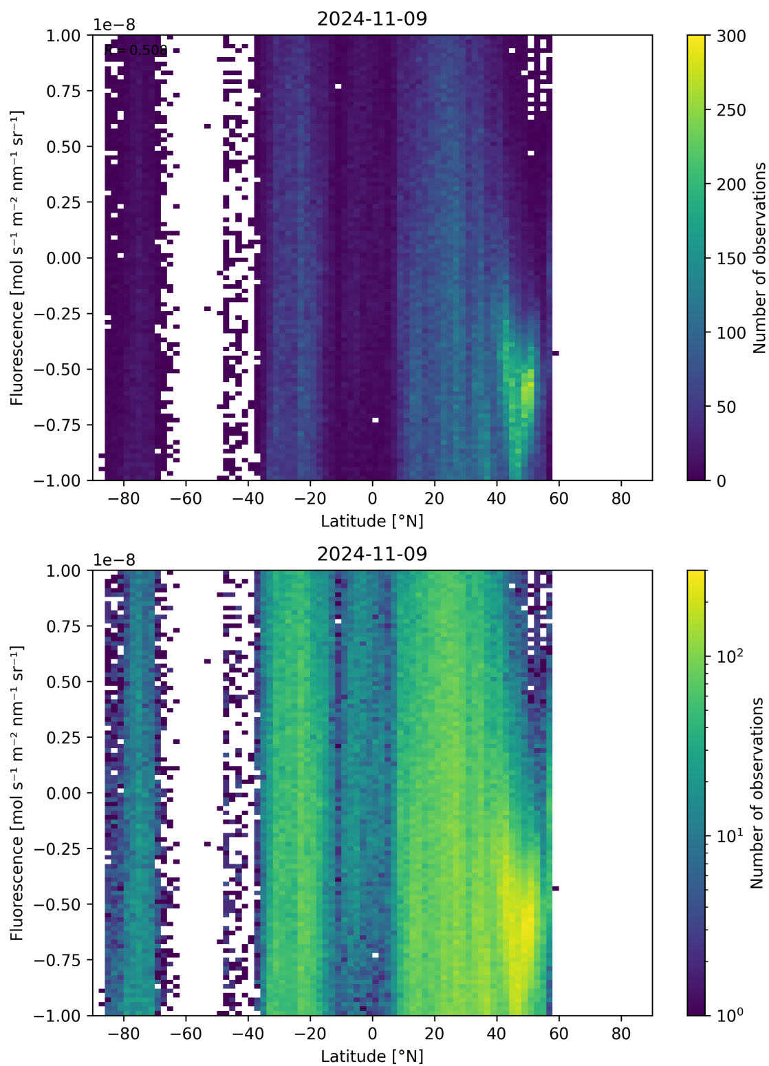
Figure 56: Scatter density plot of “Latitude” against “Fluorescence” for 2024-11-09 to 2024-11-10.
