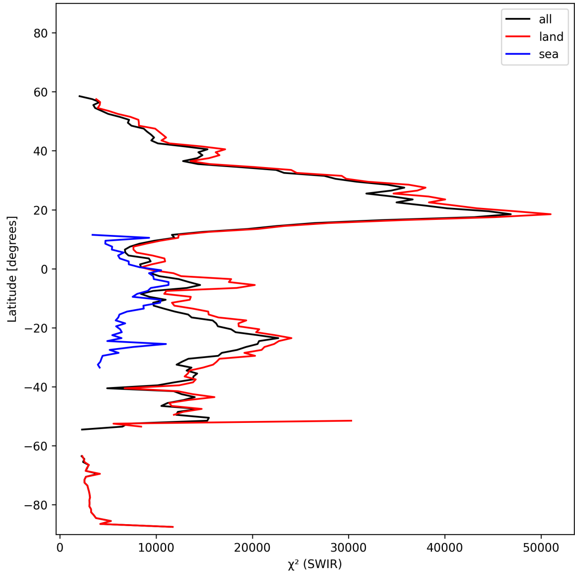
Figure 17: Zonal average of “ \chi^2 (SWIR)” for 2024-11-09 to 2024-11-10.
