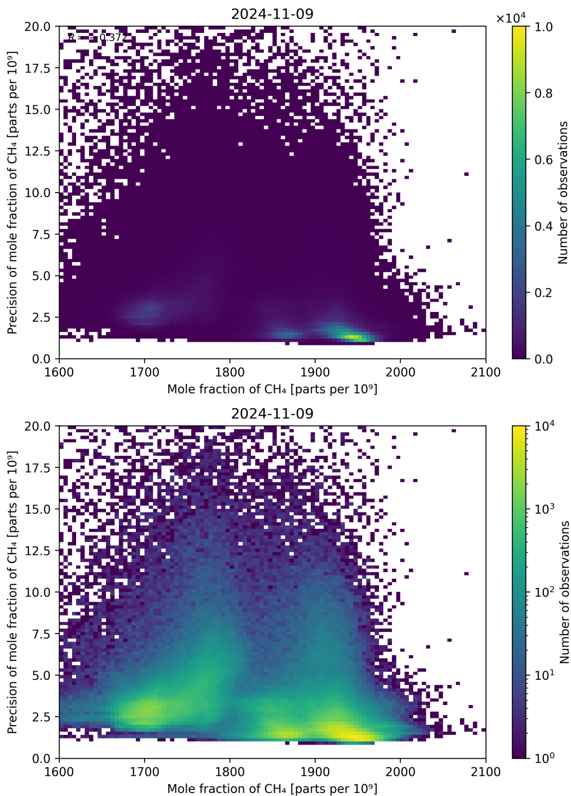
Figure 75: Scatter density plot of “Mole fraction of CH 4 ” against “Precision of mole fraction of CH 4 ” for 2024-11-09 to 2024-11-10.
