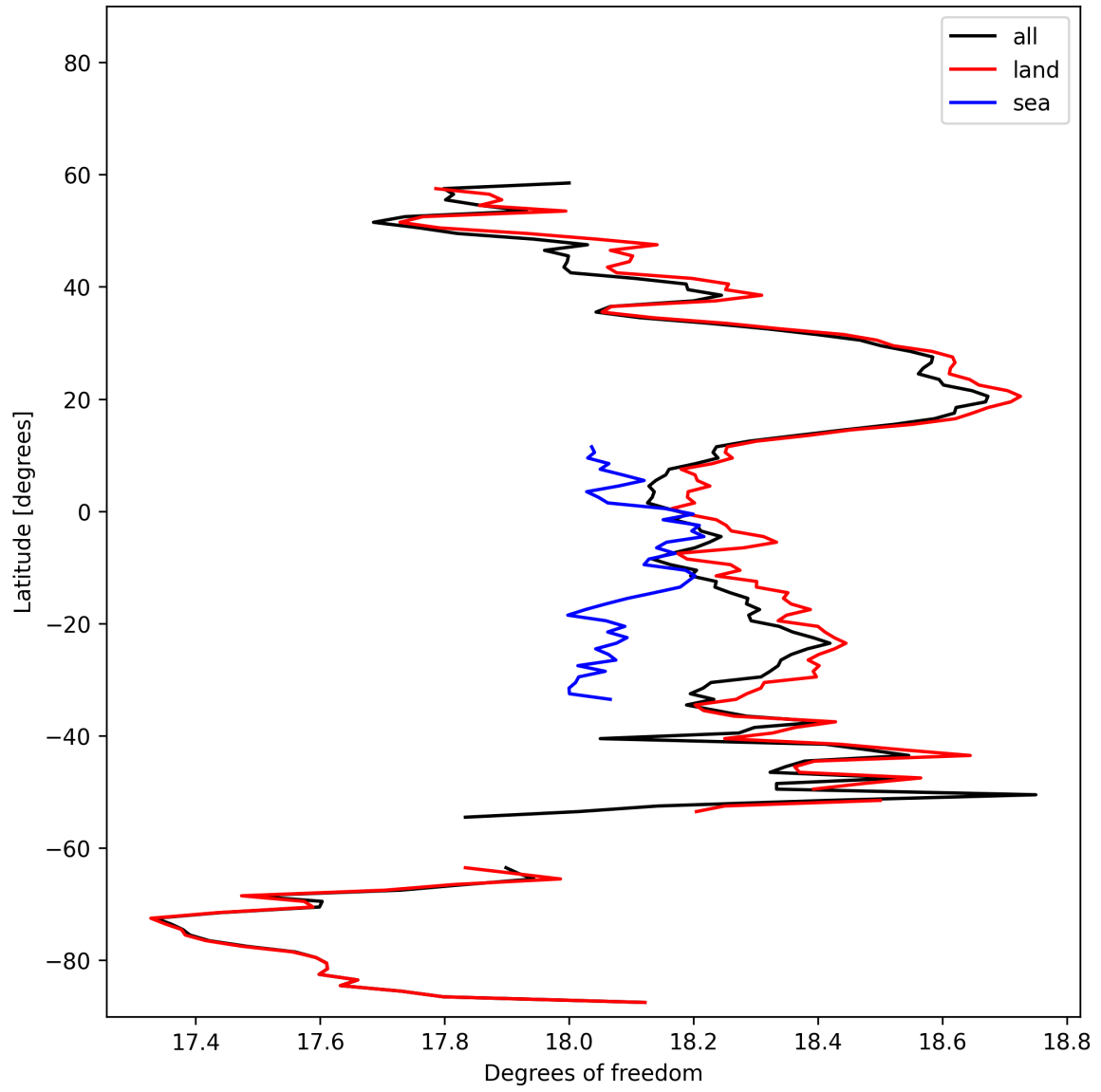
Figure 19: Zonal average of “Degrees of freedom” for 2024-11-09 to 2024-11-10.
