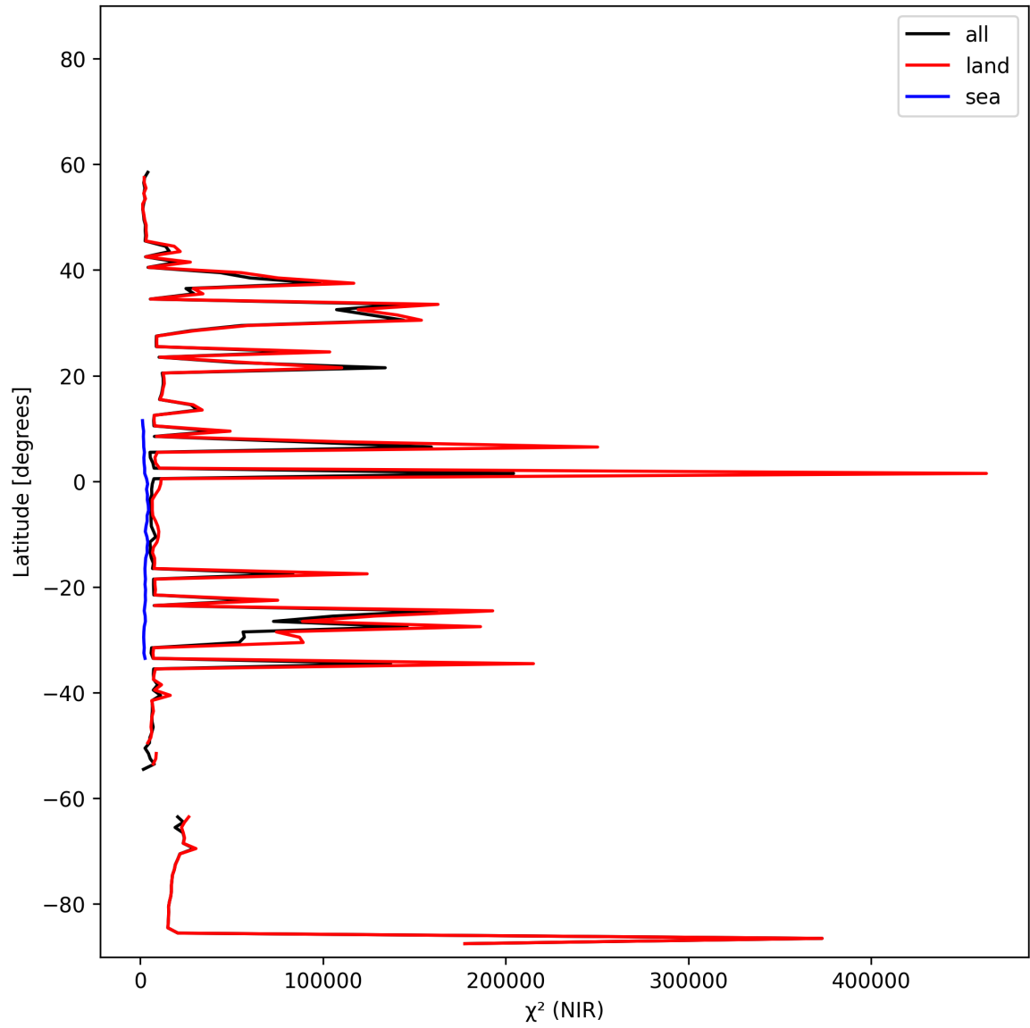
Figure 18: Zonal average of “ \chi^2 (NIR)” for 2024-11-09 to 2024-11-10.
