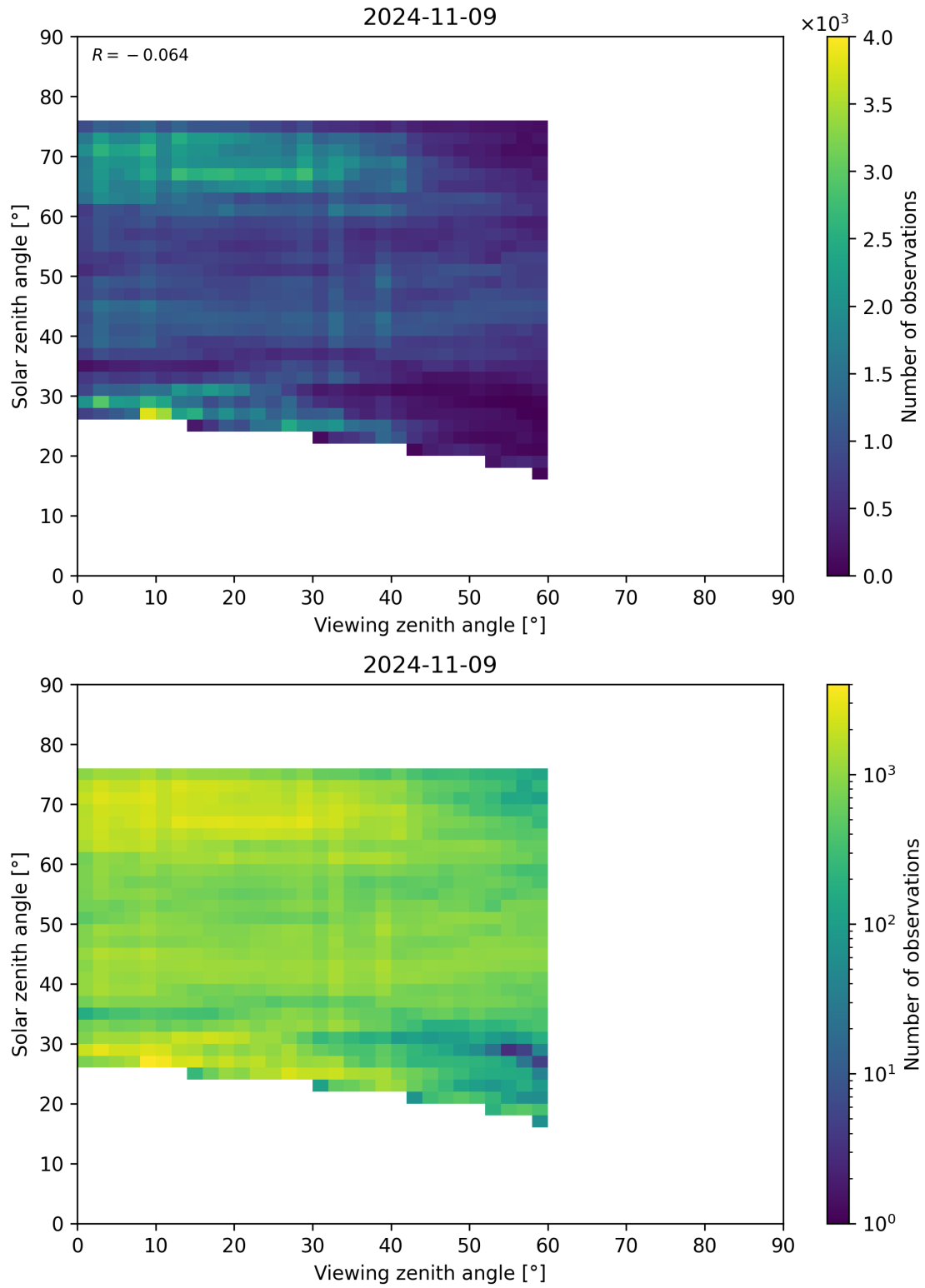
Figure 115: Scatter density plot of “Viewing zenith angle” against “Solar zenith angle” for 2024-11-09 to 2024-11-10.
