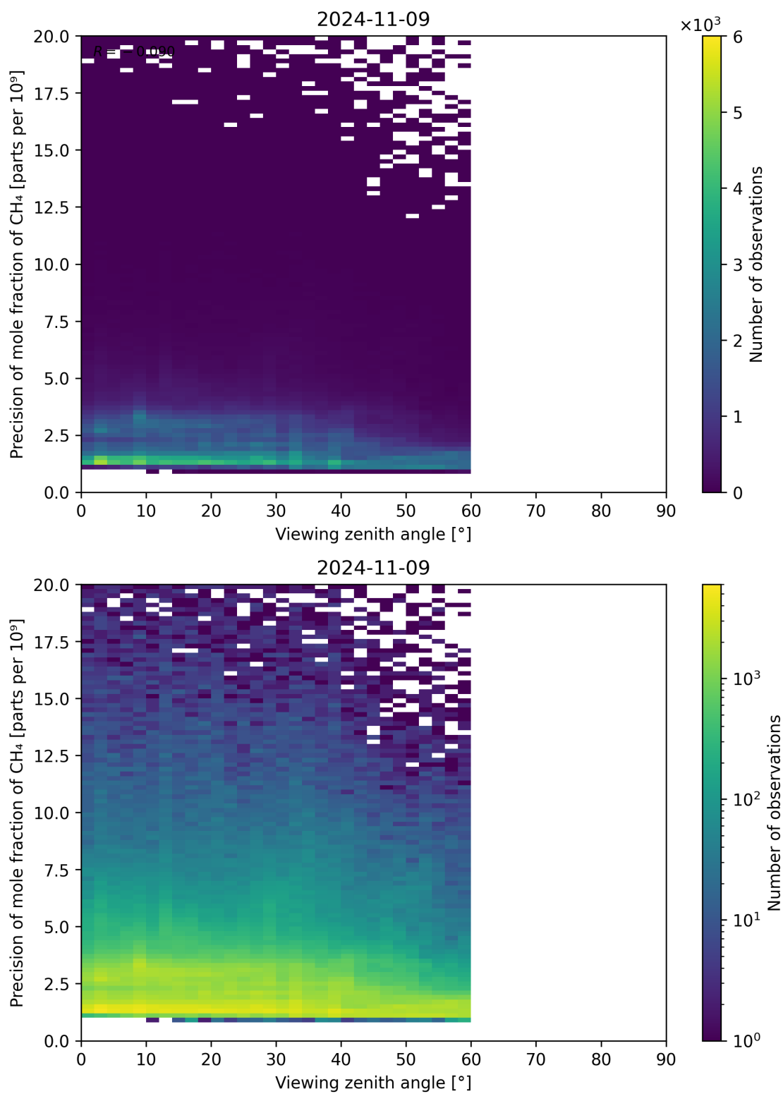
Figure 112: Scatter density plot of “Viewing zenith angle” against “Precision of mole fraction of CH 4 ” for 2024-11-09 to 2024-11-10.
