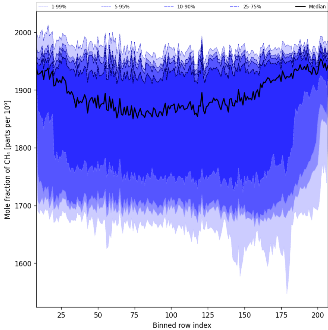
Figure 34: Along track statistics of “Mole fraction of CH 4 ” for 2024-11-09 to 2024-11-10
