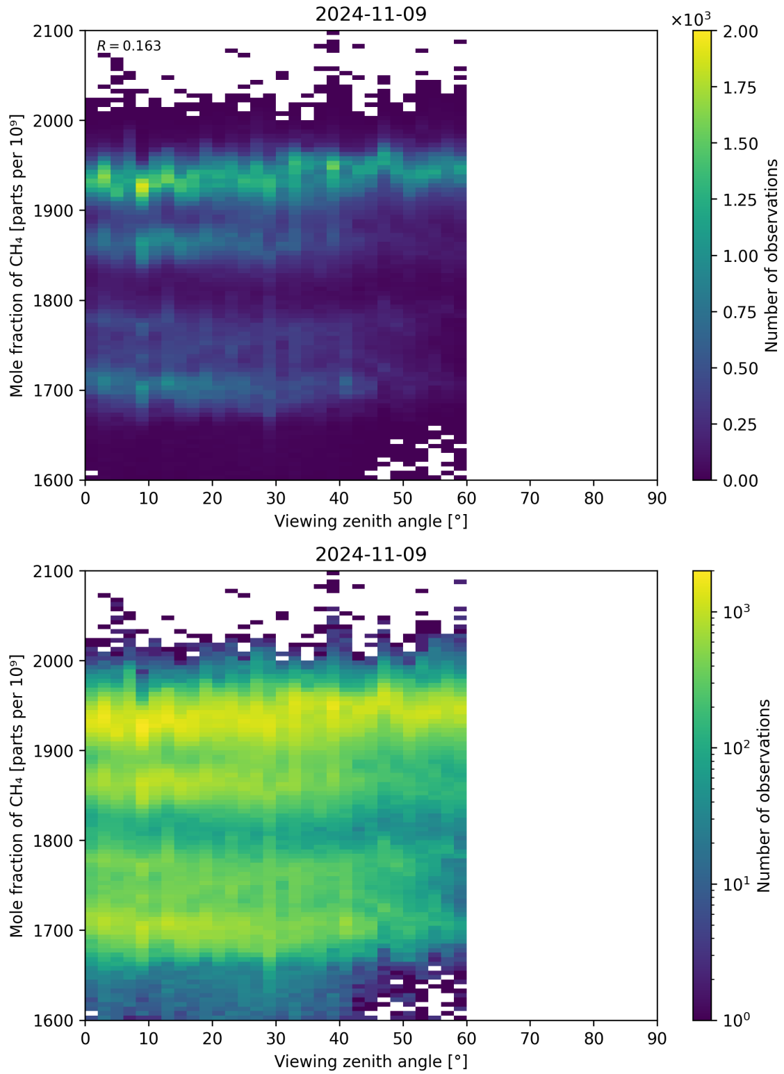
Figure 110: Scatter density plot of “Viewing zenith angle” against “Mole fraction of CH 4 ” for 2024-11-09 to 2024-11-10.
