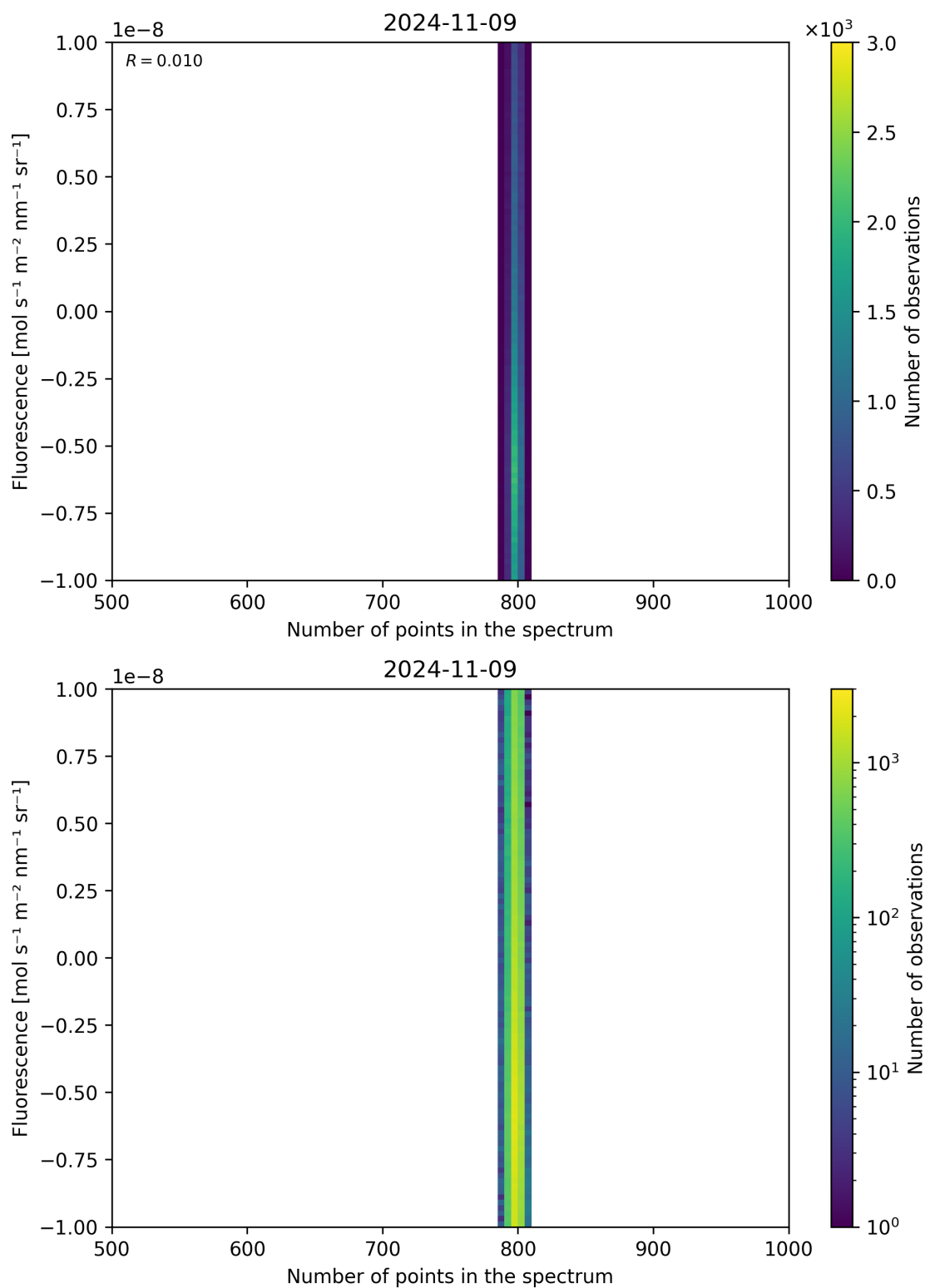
Figure 91: Scatter density plot of “Number of points in the spectrum” against “Fluorescence” for 2024-11-09 to 2024-11-10.
