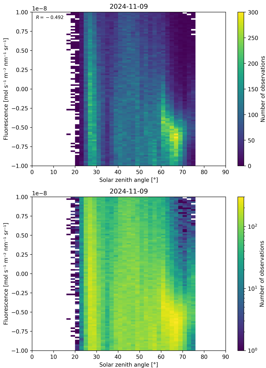
Figure 97: Scatter density plot of “Solar zenith angle” against “Fluorescence” for 2024-11-09 to 2024-11-10.
