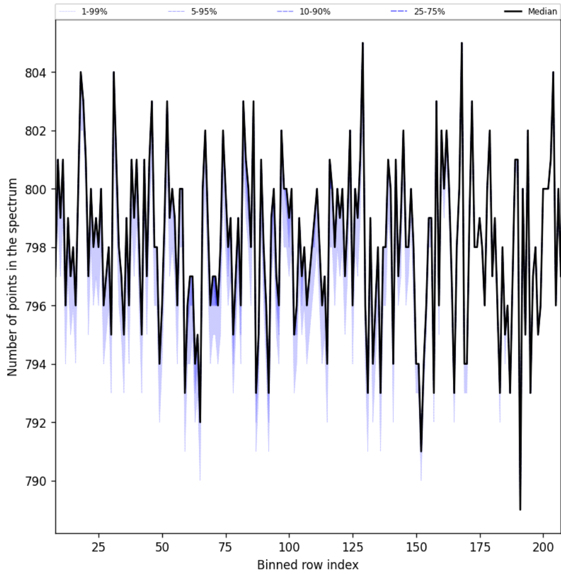
Figure 37: Along track statistics of “Number of points in the spectrum” for 2024-11-09 to 2024-11-10
