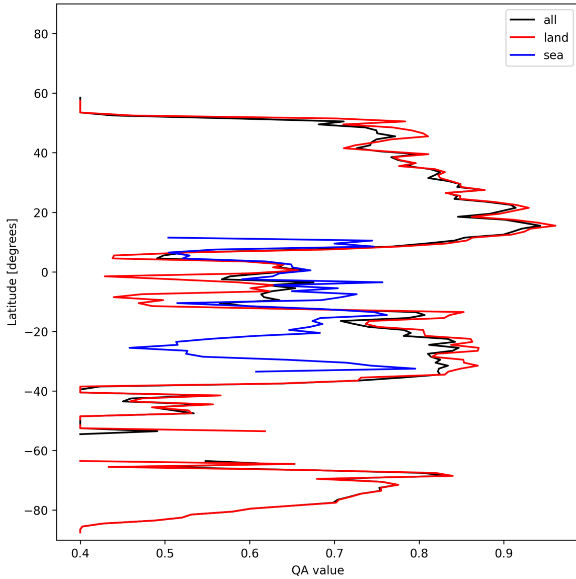
Figure 11: Zonal average of “QA value” for 2024-11-09 to 2024-11-10.
