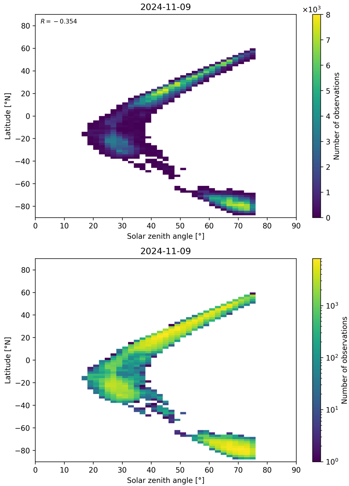
Figure 98: Scatter density plot of “Solar zenith angle” against “Latitude” for 2024-11-09 to 2024-11-10.
