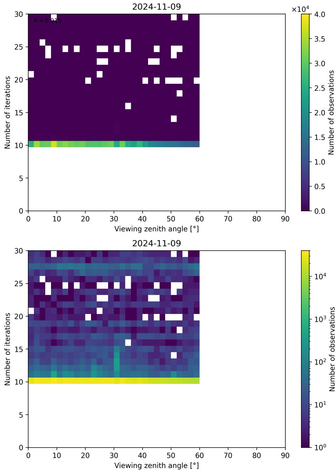
Figure 113: Scatter density plot of “Viewing zenith angle” against “Number of iterations” for 2024-11-09 to 2024-11-10.
