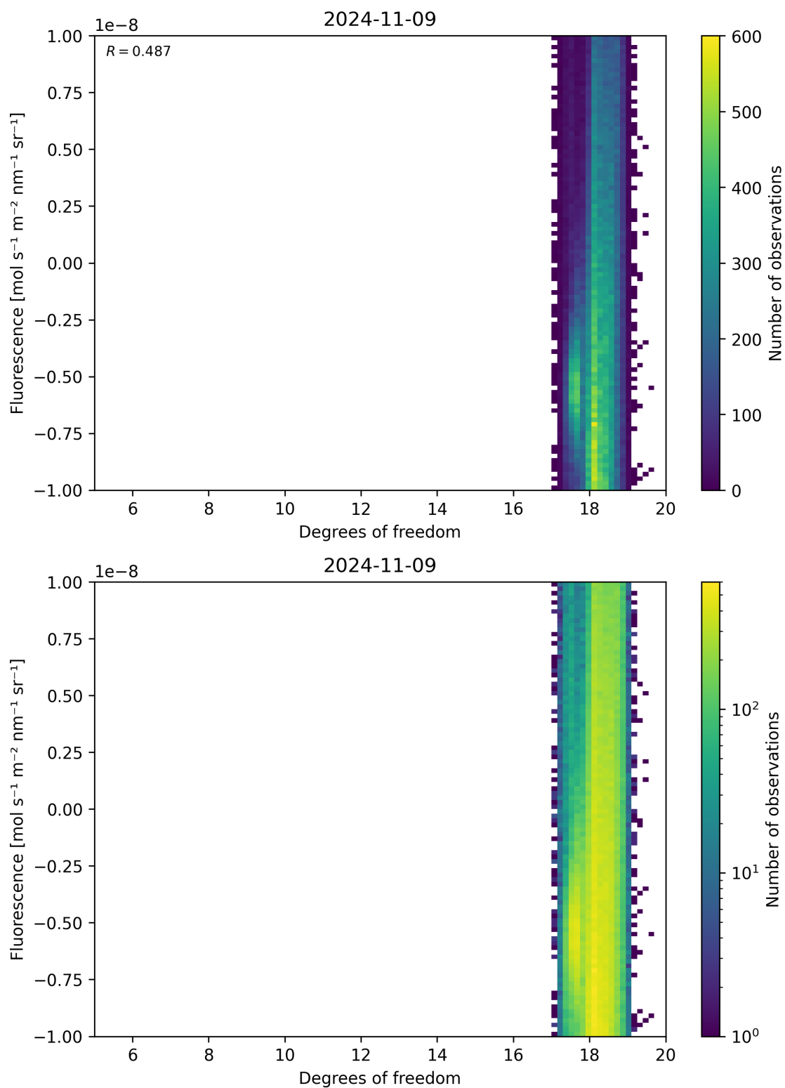
Figure 51: Scatter density plot of “Degrees of freedom” against “Fluorescence” for 2024-11-09 to 2024-11-10.
