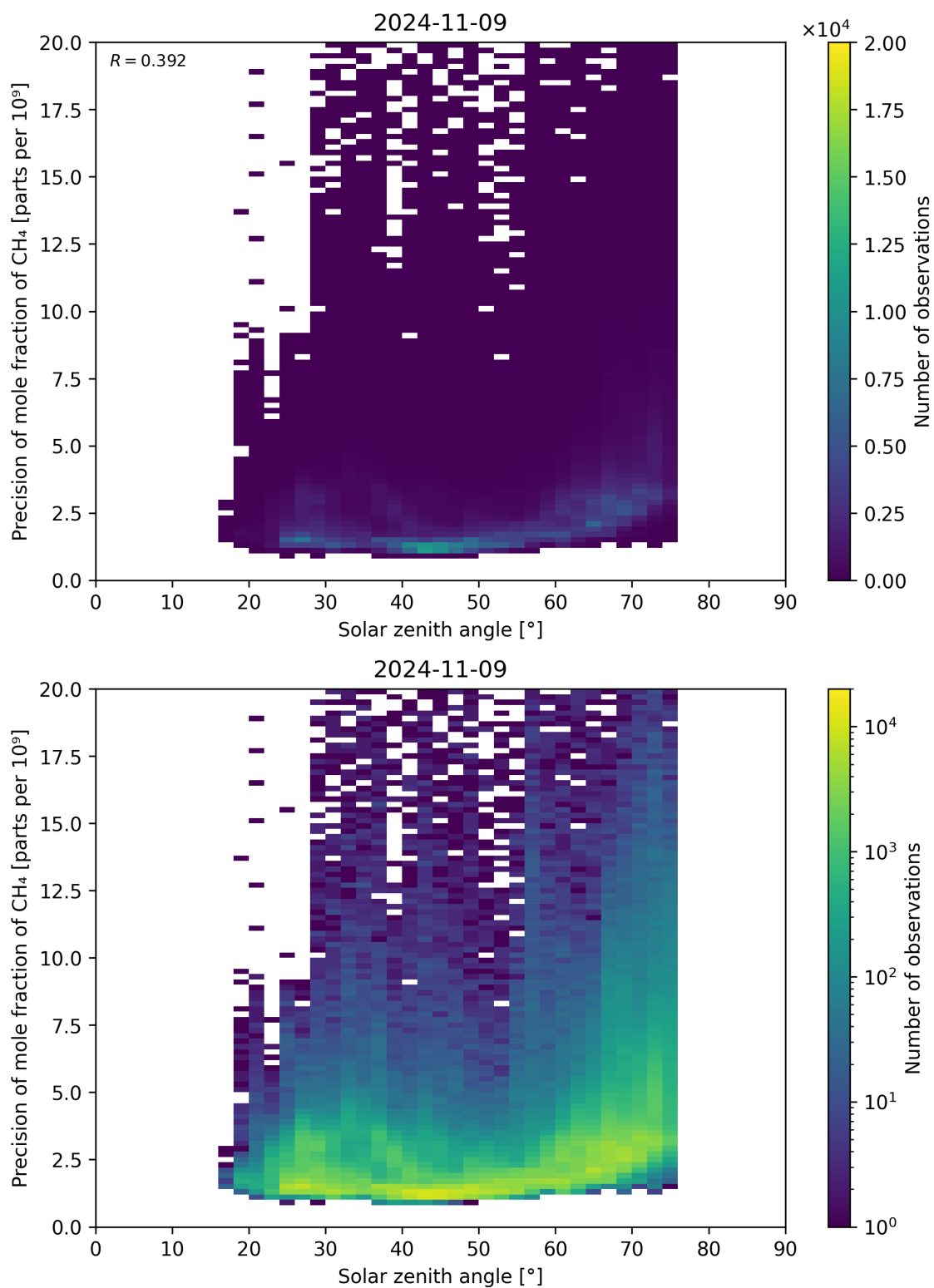
Figure 101: Scatter density plot of “Solar zenith angle” against “Precision of mole fraction of CH 4 ” for 2024-11-09 to 2024-11-10.
