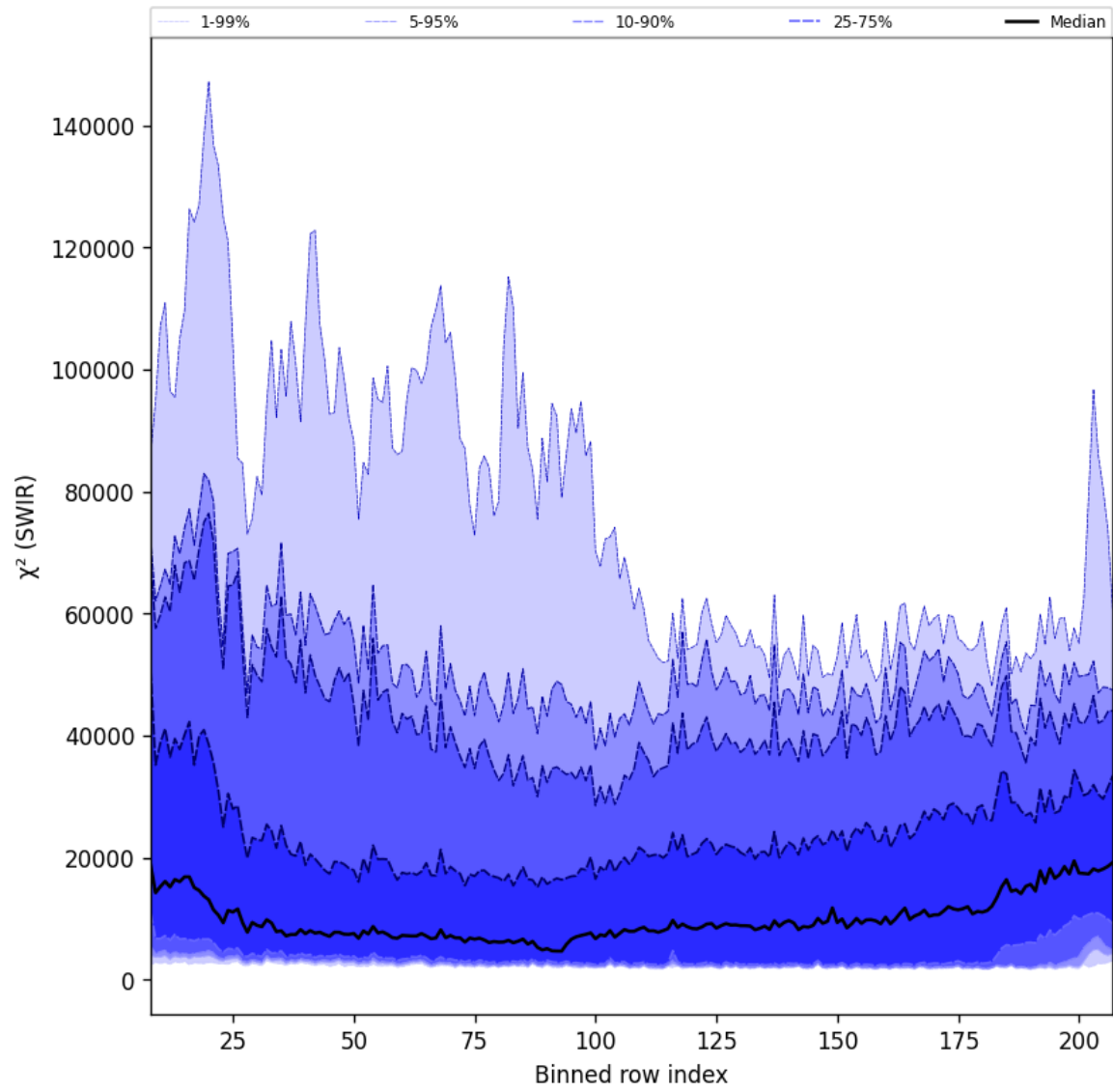
Figure 39: Along track statistics of “ \chi^2 (SWIR)” for 2024-11-09 to 2024-11-10
