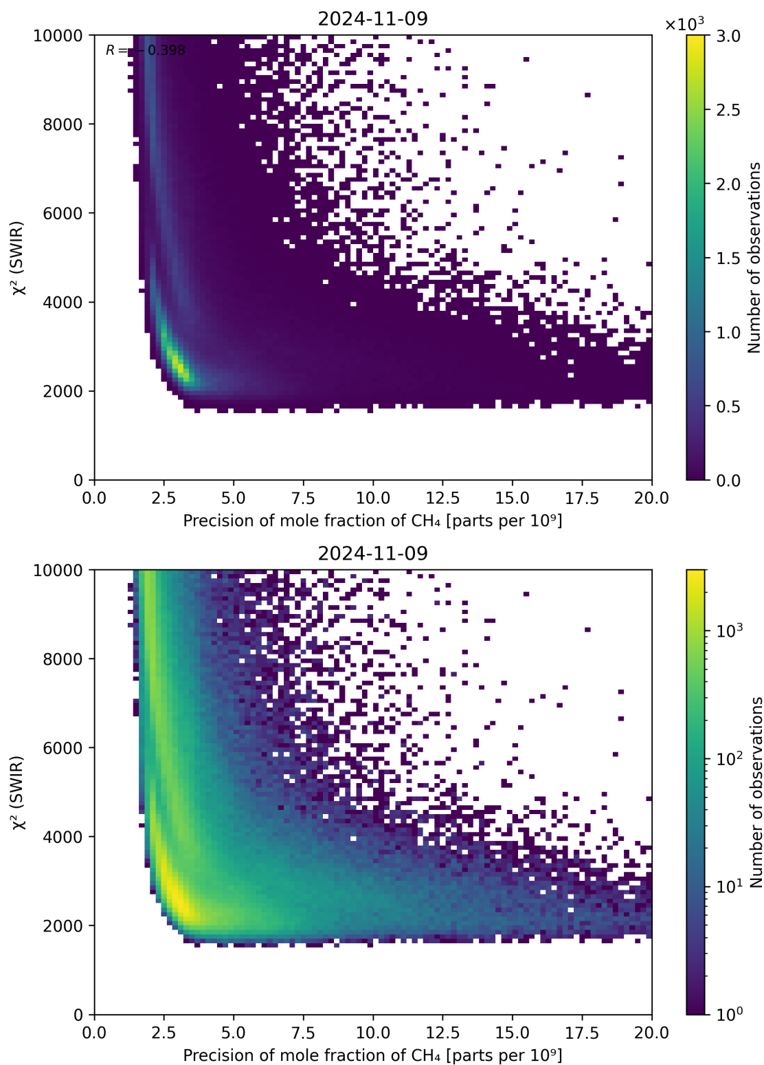
Figure 79: Scatter density plot of “Precision of mole fraction of CH 4 ” against “ \chi^2 (SWIR)” for 2024-11-09 to 2024-11-10.
