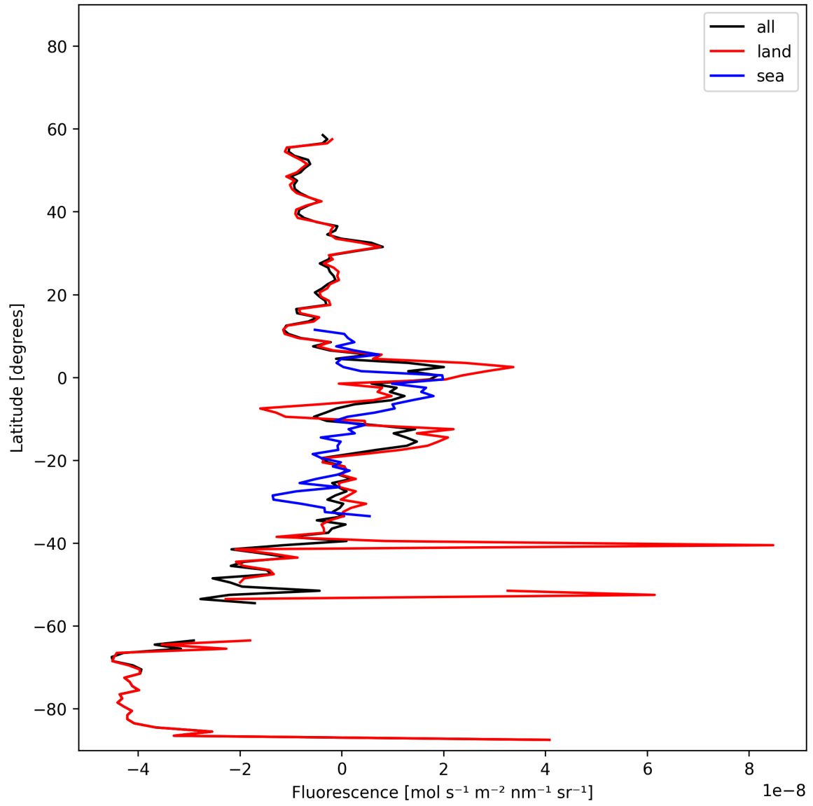
Figure 21: Zonal average of “Fluorescence” for 2024-11-09 to 2024-11-10.
