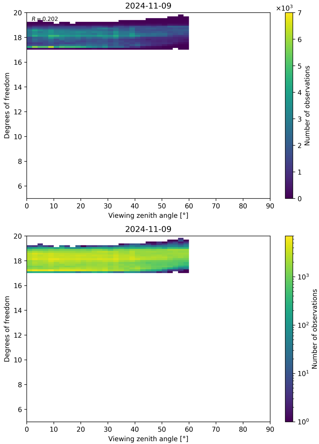
Figure 107: Scatter density plot of “Viewing zenith angle” against “Degrees of freedom” for 2024-11-09 to 2024-11-10.
