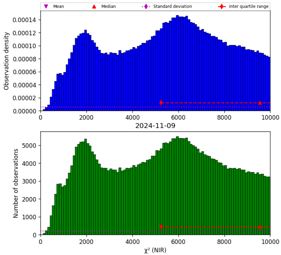
Figure 29: Histogram of “ \chi^2 (NIR)” for 2024-11-09 to 2024-11-10
