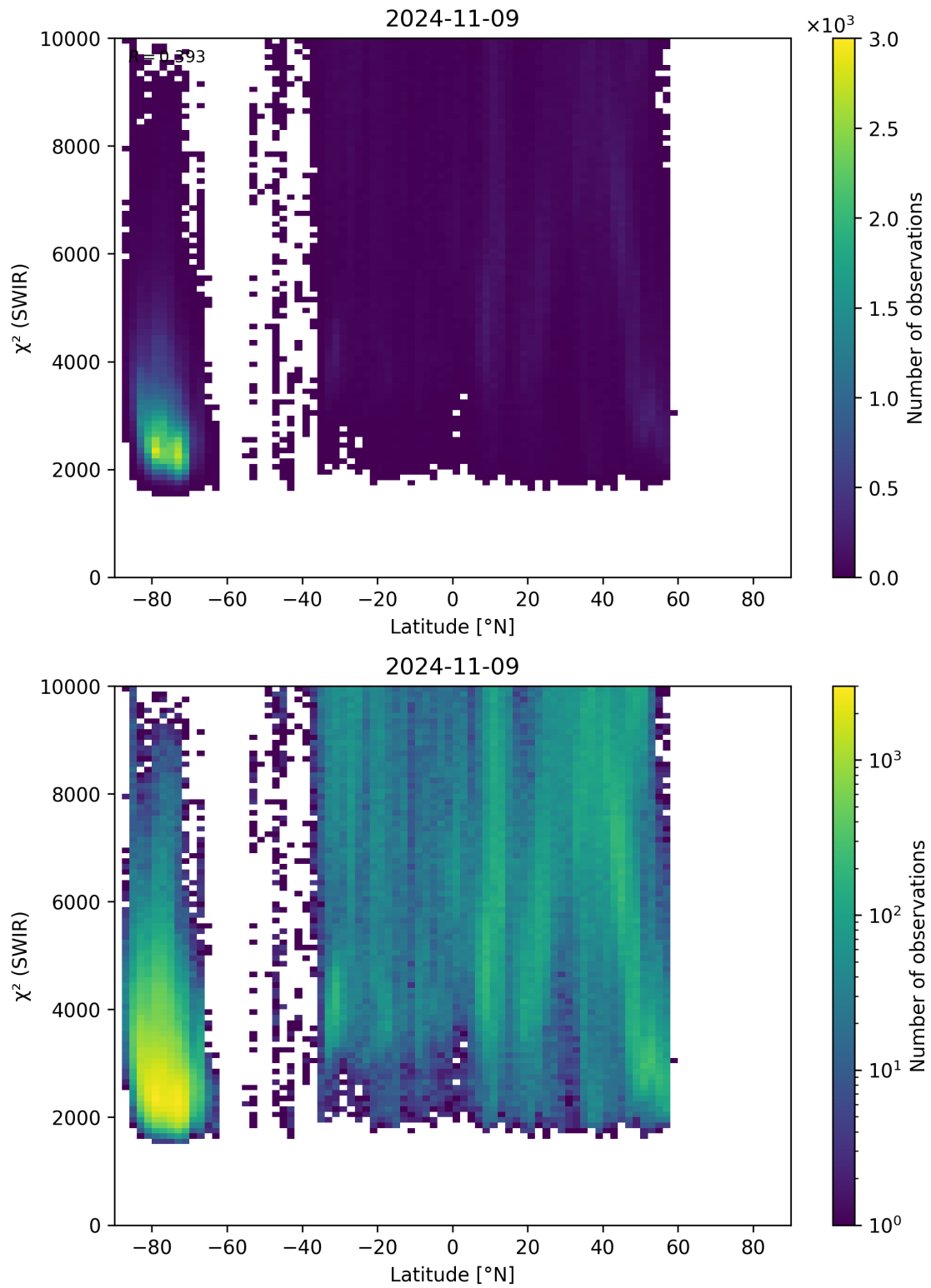
Figure 54: Scatter density plot of “Latitude” against “ \chi^2 (SWIR)” for 2024-11-09 to 2024-11-10.
