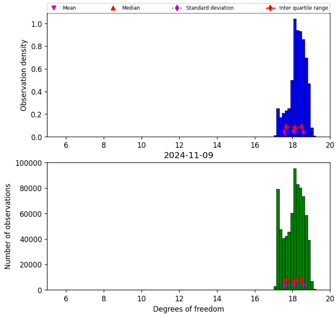
Figure 30: Histogram of “Degrees of freedom” for 2024-11-09 to 2024-11-10
