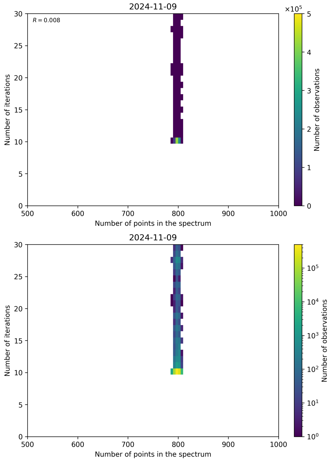
Figure 92: Scatter density plot of “Number of points in the spectrum” against “Number of iterations” for 2024-11-09 to 2024-11-10.
