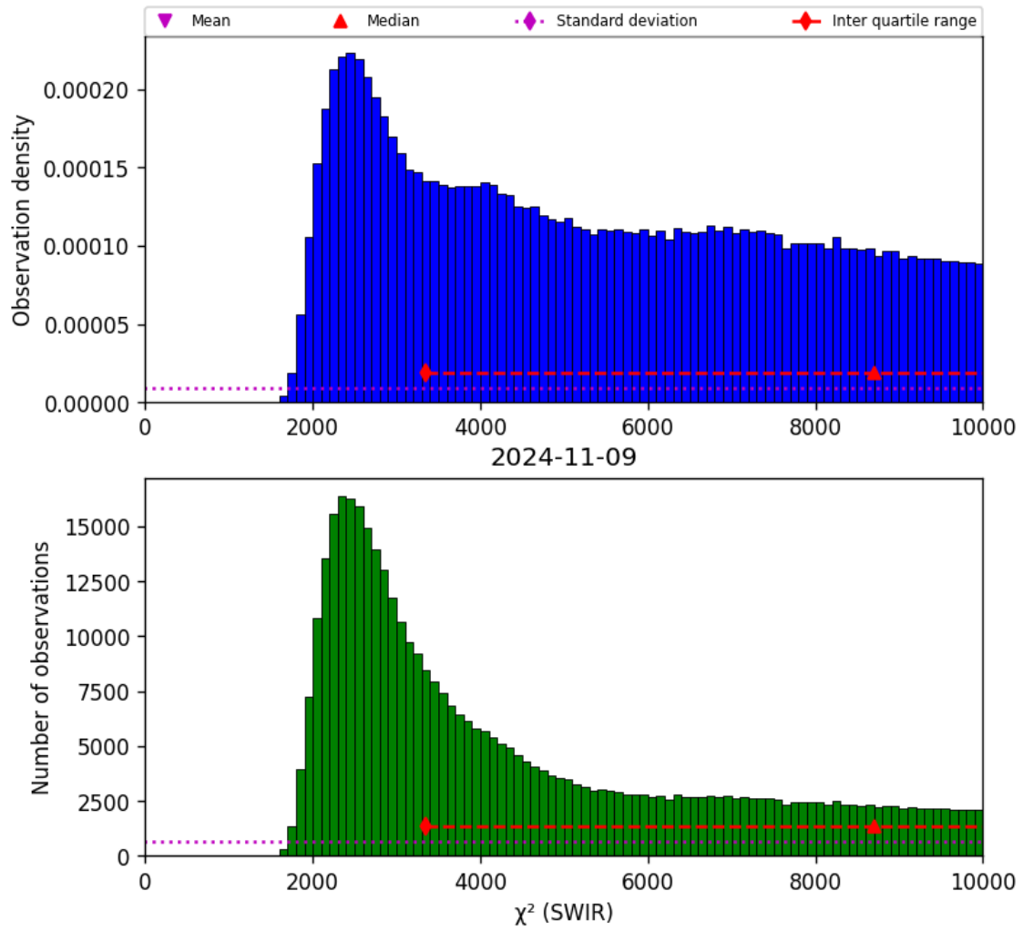
Figure 28: Histogram of “ \chi^2 (SWIR)” for 2024-11-09 to 2024-11-10
