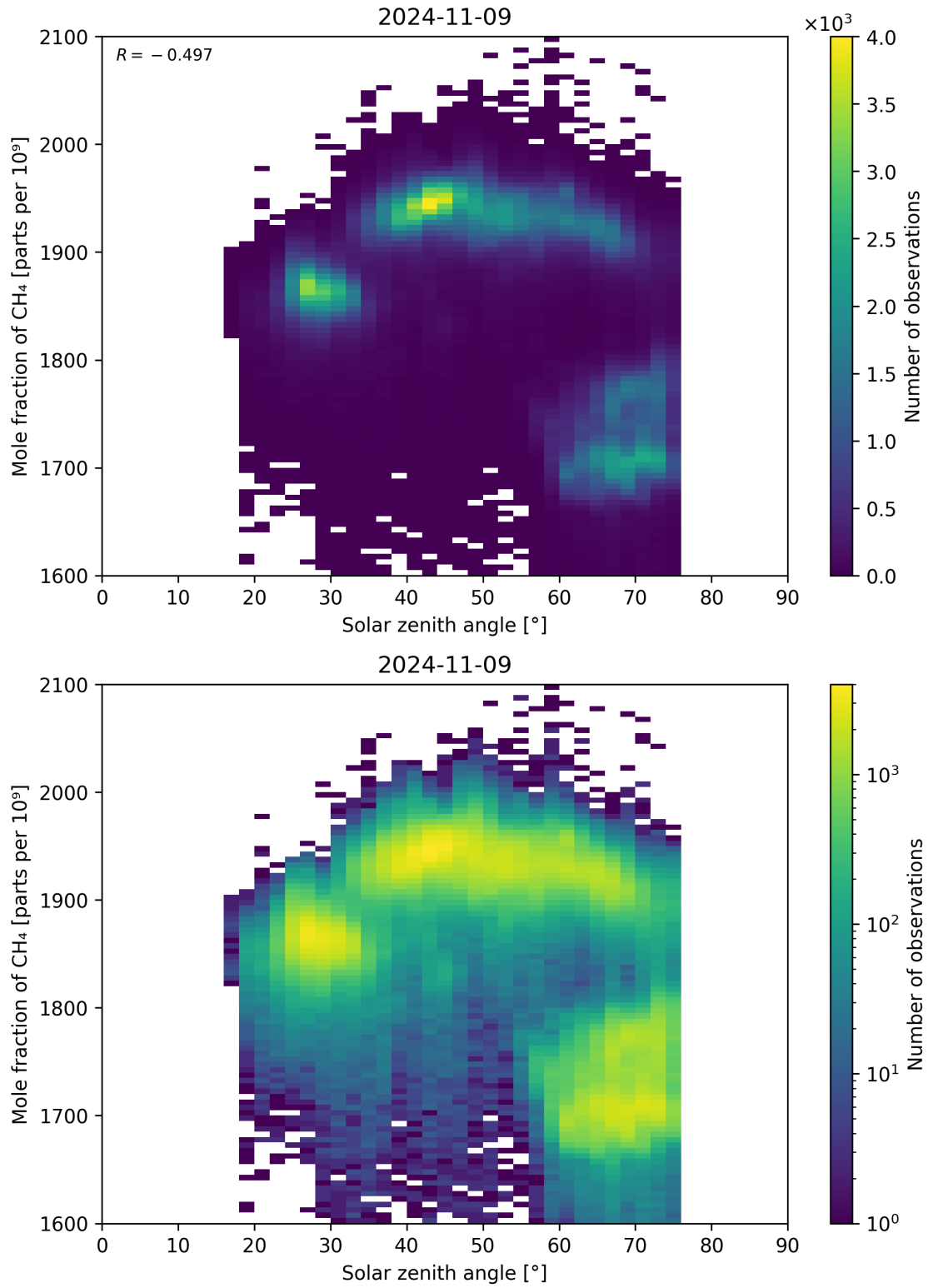
Figure 99: Scatter density plot of “Solar zenith angle” against “Mole fraction of CH 4 ” for 2024-11-09 to 2024-11-10.
