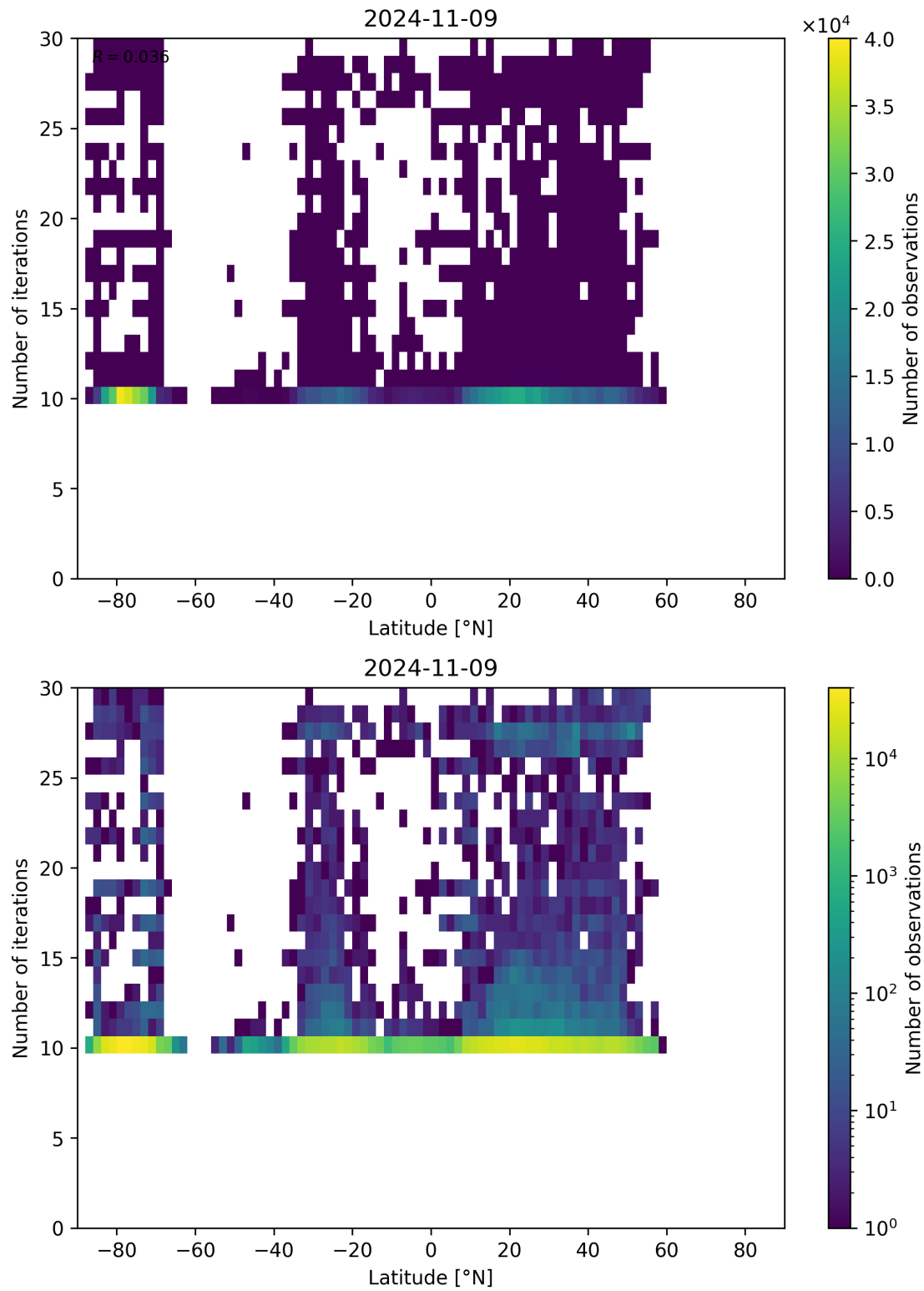
Figure 60: Scatter density plot of “Latitude” against “Number of iterations” for 2024-11-09 to 2024-11-10.
