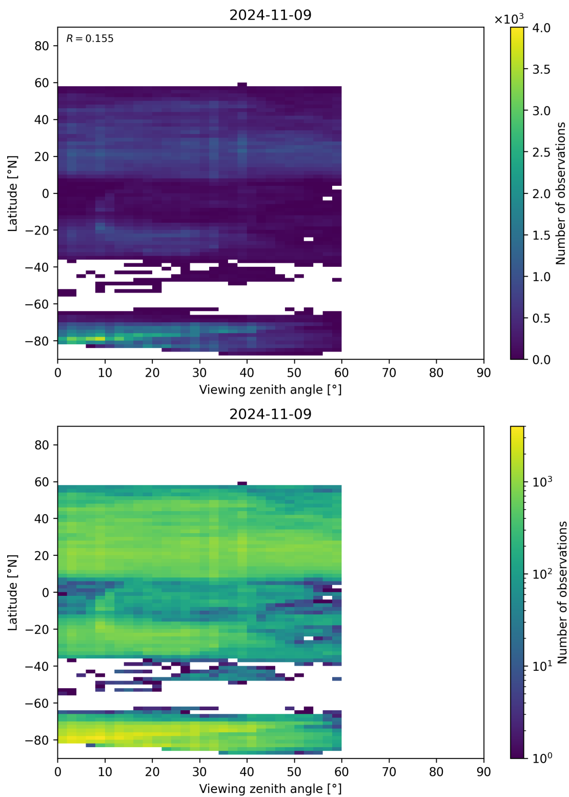
Figure 109: Scatter density plot of “Viewing zenith angle” against “Latitude” for 2024-11-09 to 2024-11-10.
