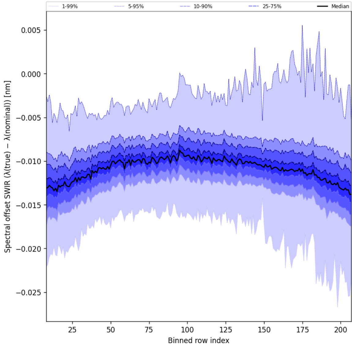
Figure 38: Along track statistics of “Spectral offset SWIR ( \lambda_{\text{true}} - \lambda_{\text{nominal}} )” for 2024-11-09 to 2024-11-10
