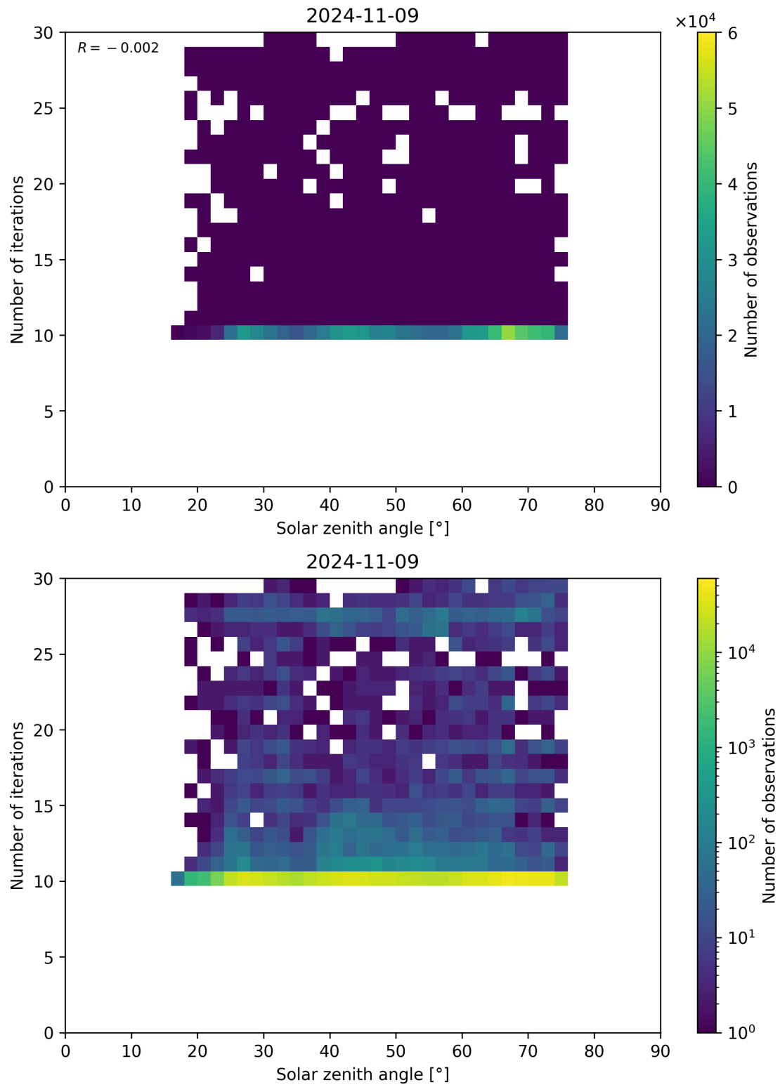
Figure 102: Scatter density plot of “Solar zenith angle” against “Number of iterations” for 2024-11-09 to 2024-11-10.
