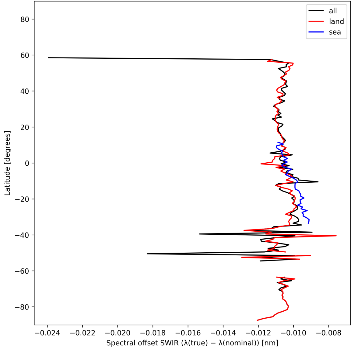
Figure 16: Zonal average of “Spectral offset SWIR ( \lambda_{\text{true}} - \lambda_{\text{nominal}} )” for 2024-11-09 to 2024-11-10.
