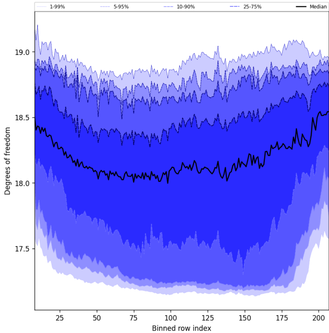
Figure 41: Along track statistics of “Degrees of freedom” for 2024-11-09 to 2024-11-10
