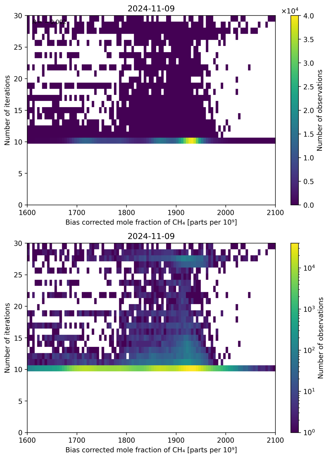
Figure 67: Scatter density plot of “Bias corrected mole fraction of CH 4 ” against “Number of iterations” for 2024-11-09 to 2024-11-10.
