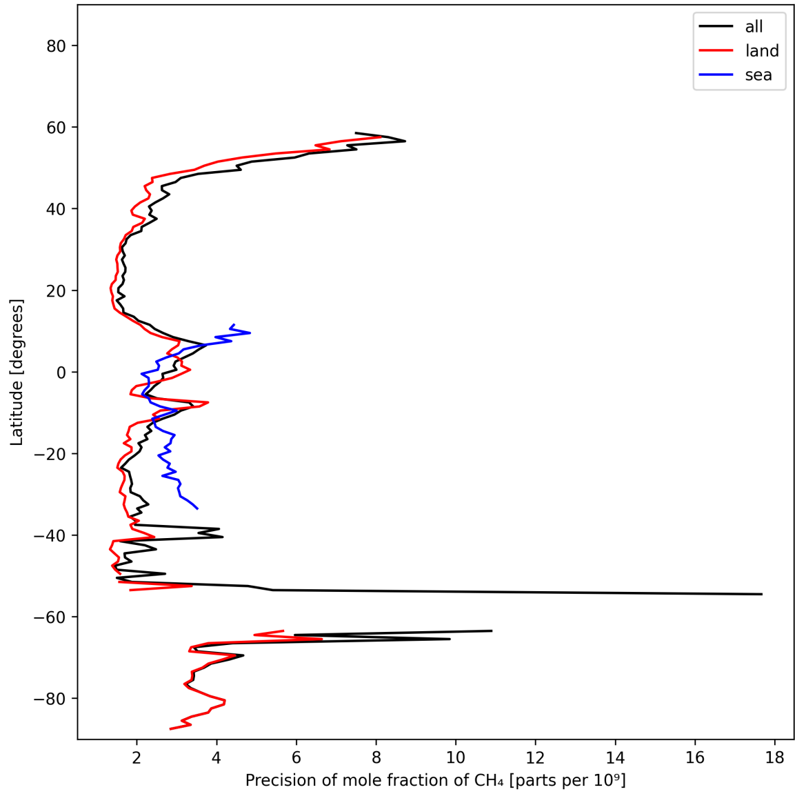
Figure 13: Zonal average of “Precision of mole fraction of CH 4 ” for 2024-11-09 to 2024-11-10.
