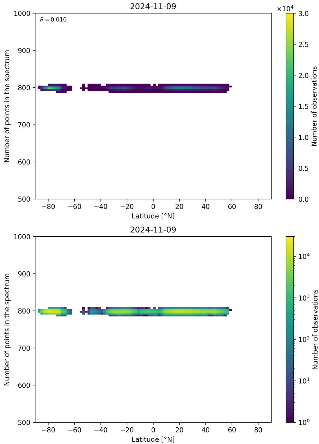
Figure 61: Scatter density plot of “Latitude” against “Number of points in the spectrum” for 2024-11-09 to 2024-11-10.
