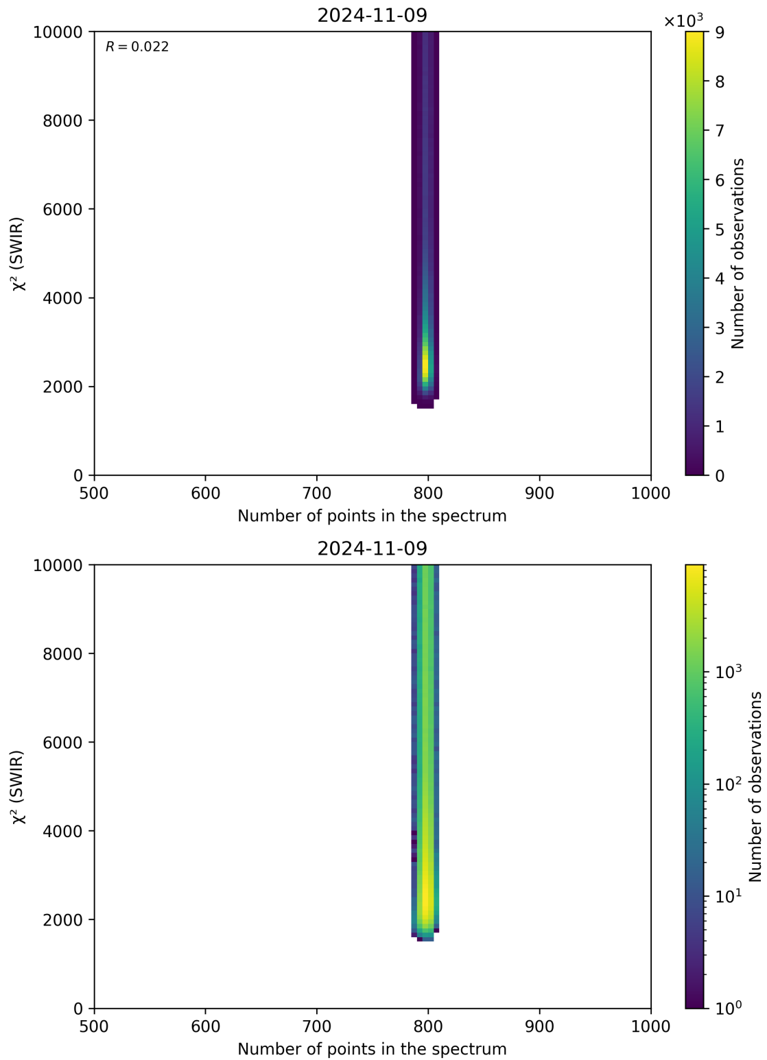
Figure 89: Scatter density plot of “Number of points in the spectrum” against “ \chi^2 (SWIR)” for 2024-11-09 to 2024-11-10.
