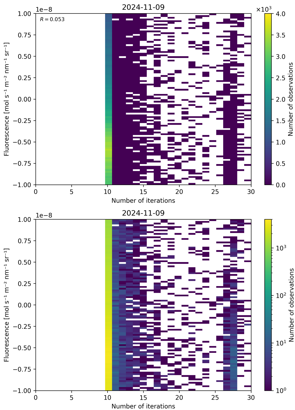
Figure 87: Scatter density plot of “Number of iterations” against “Fluorescence” for 2024-11-09 to 2024-11-10.
