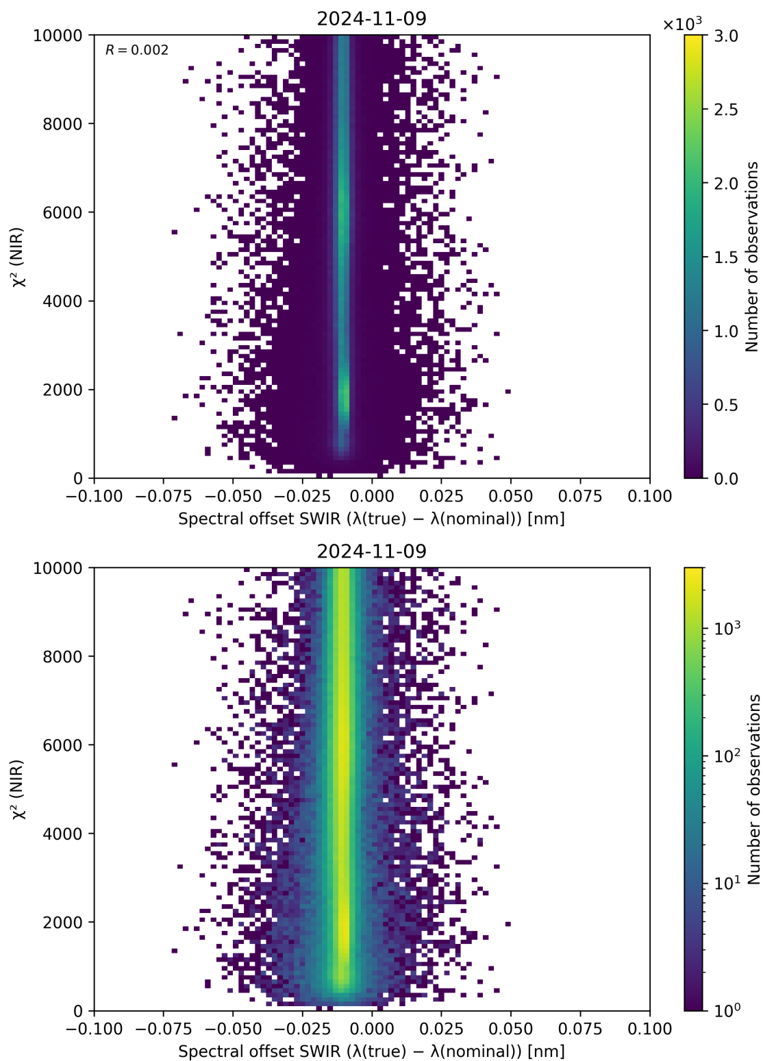
Figure 117: Scatter density plot of “Spectral offset SWIR ( \lambda_{\text{true}} - \lambda_{\text{nominal}} )” against “ \chi^2 (NIR)” for 2024-11-09 to 2024-11-10.
