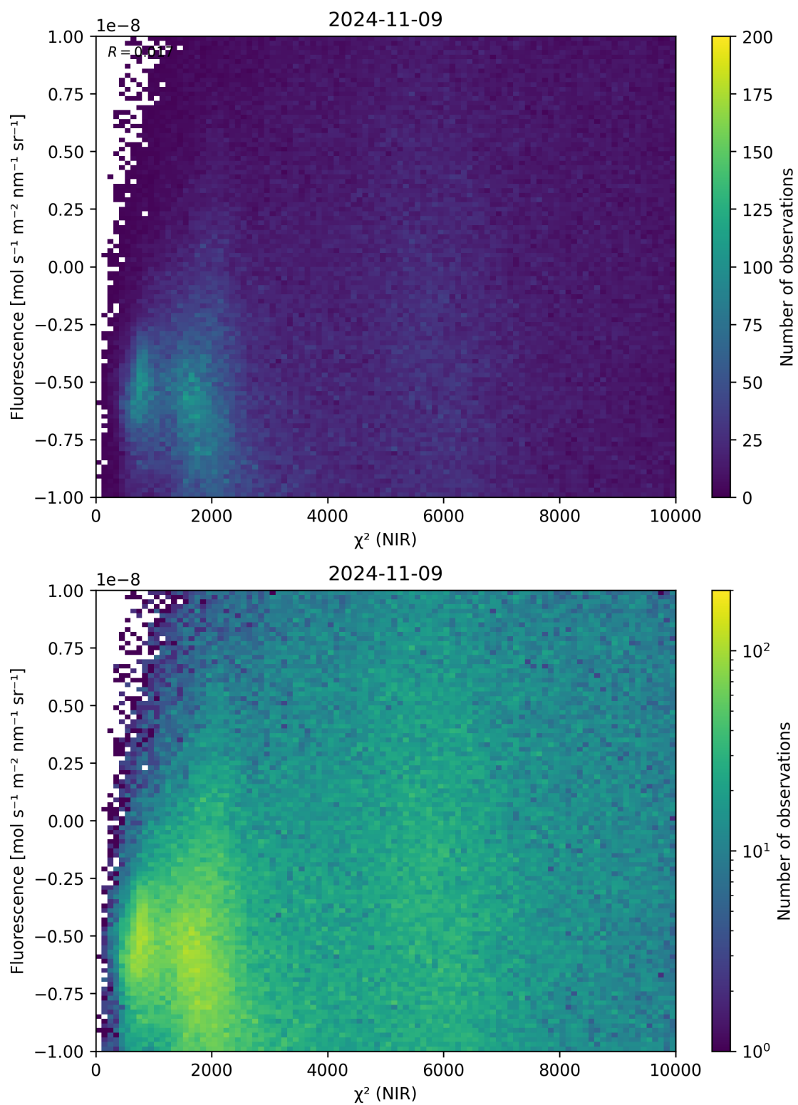
Figure 45: Scatter density plot of “ \chi^2 (NIR)” against “Fluorescence” for 2024-11-09 to 2024-11-10.
