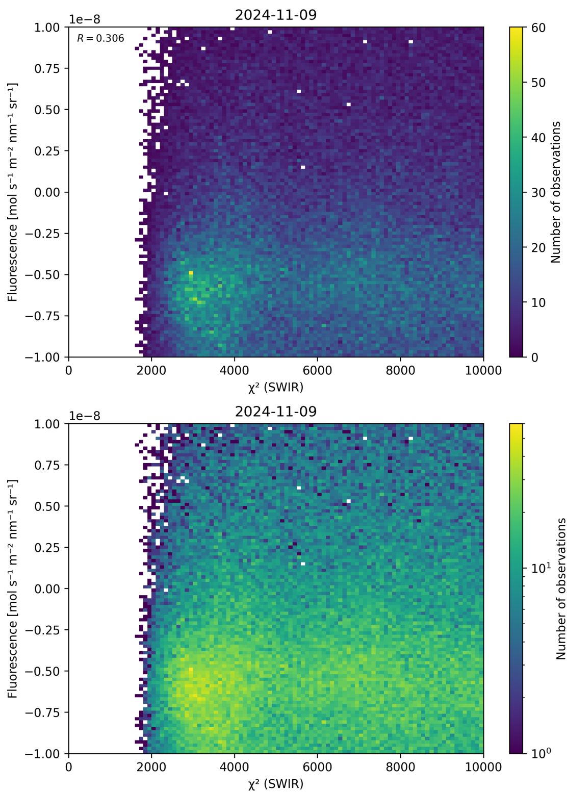
Figure 49: Scatter density plot of “ \chi^2 (SWIR)” against “Fluorescence” for 2024-11-09 to 2024-11-10.
