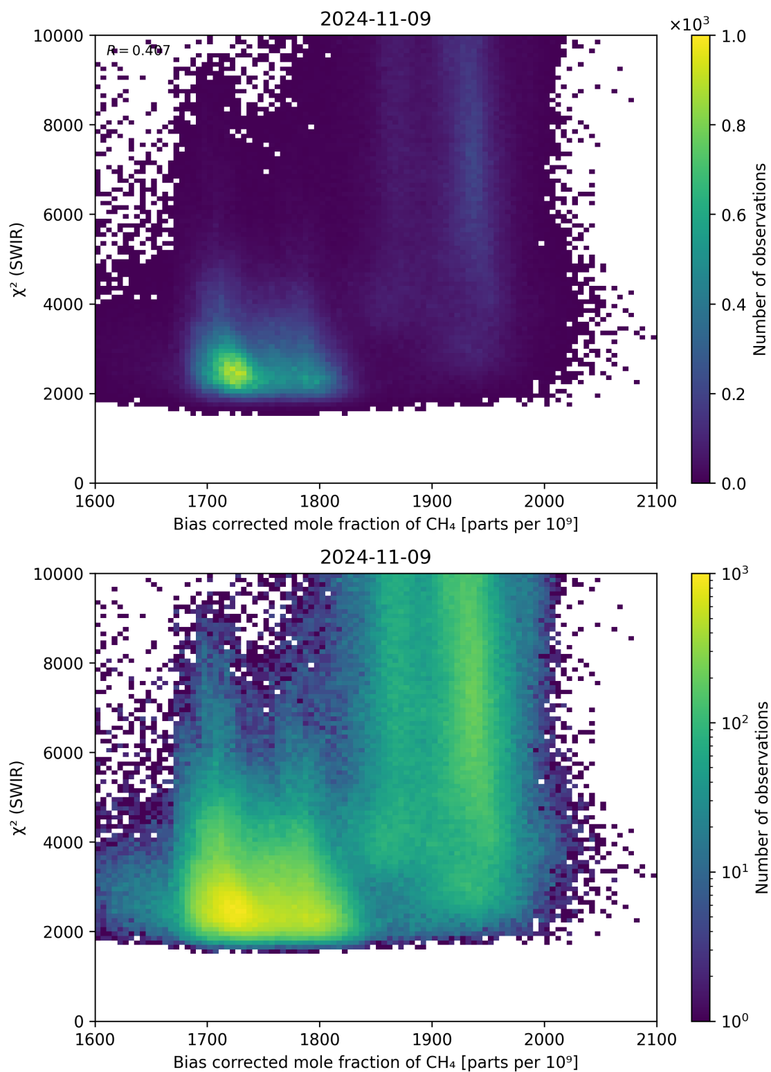
Figure 64: Scatter density plot of “Bias corrected mole fraction of \text{CH}_4 ” against “ \chi^2 (SWIR)” for 2024-11-09 to 2024-11-10.
