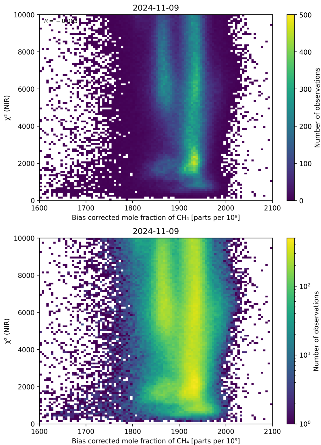
Figure 63: Scatter density plot of “Bias corrected mole fraction of CH 4 ” against “ \chi^2 (NIR)” for 2024-11-09 to 2024-11-10.
