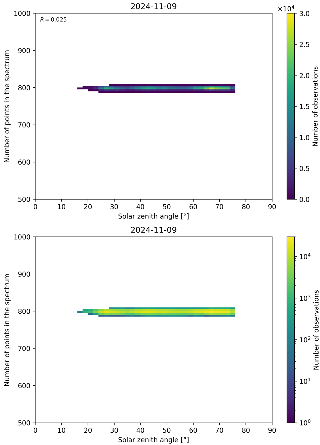
Figure 103: Scatter density plot of “Solar zenith angle” against “Number of points in the spectrum” for 2024-11-09 to 2024-11-10.
