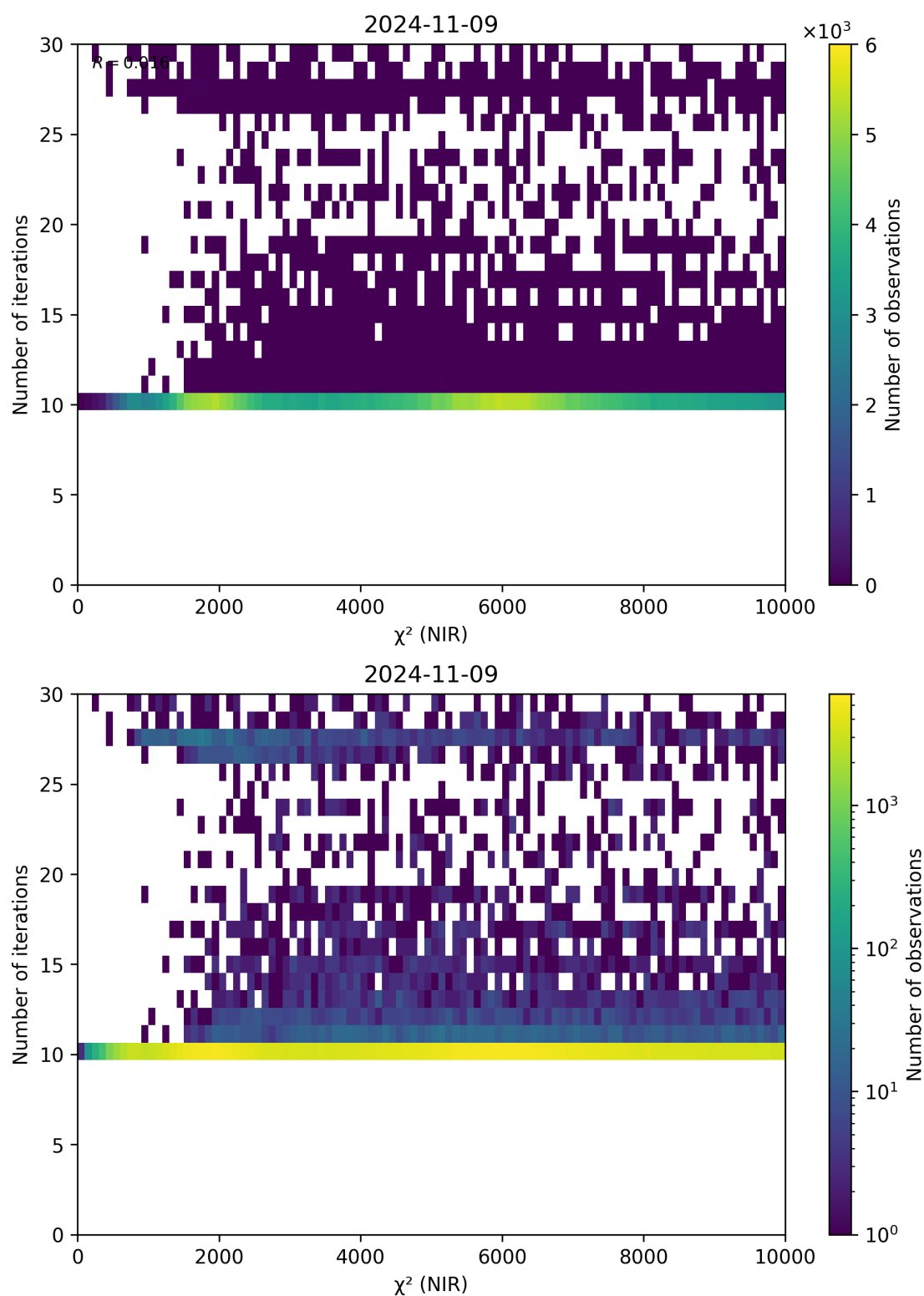
Figure 46: Scatter density plot of “ \chi^2 (NIR)” against “Number of iterations” for 2024-11-09 to 2024-11-10.
