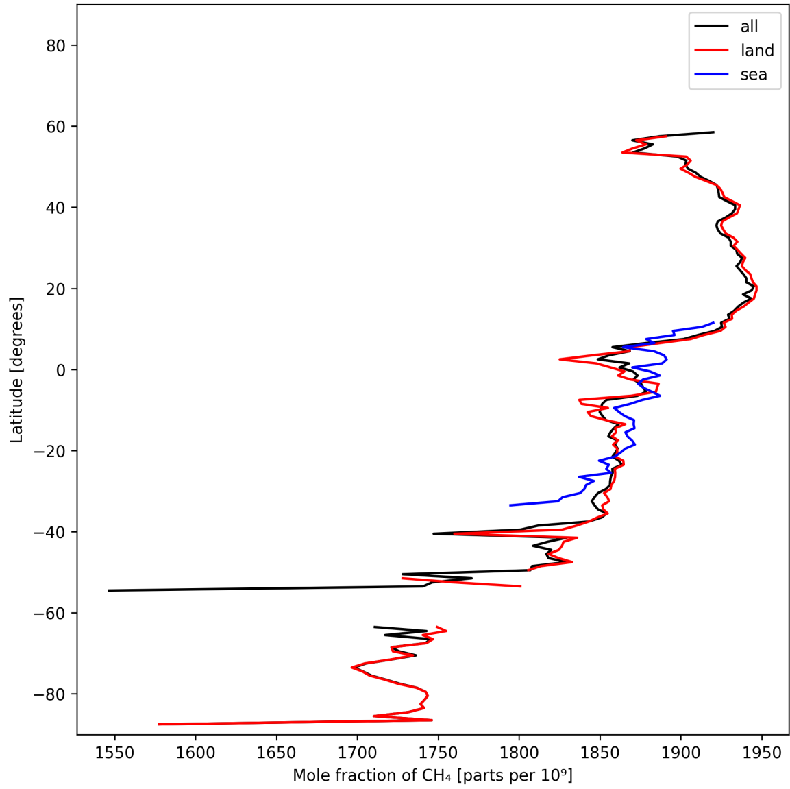
Figure 12: Zonal average of “Mole fraction of \text{CH}_4 ” for 2024-11-09 to 2024-11-10.
