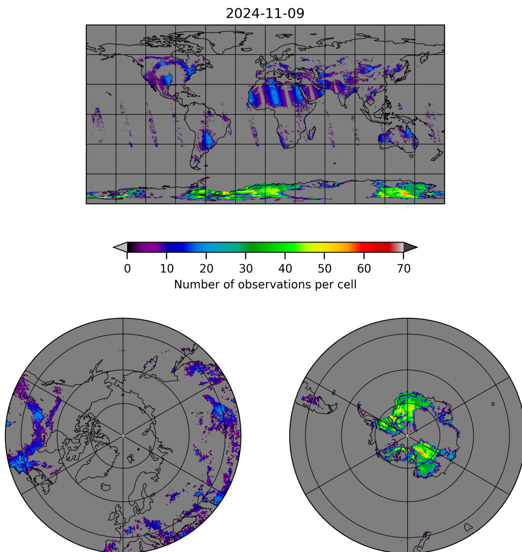
Figure 10: Map of the number of observations for 2024-11-09 to 2024-11-10
