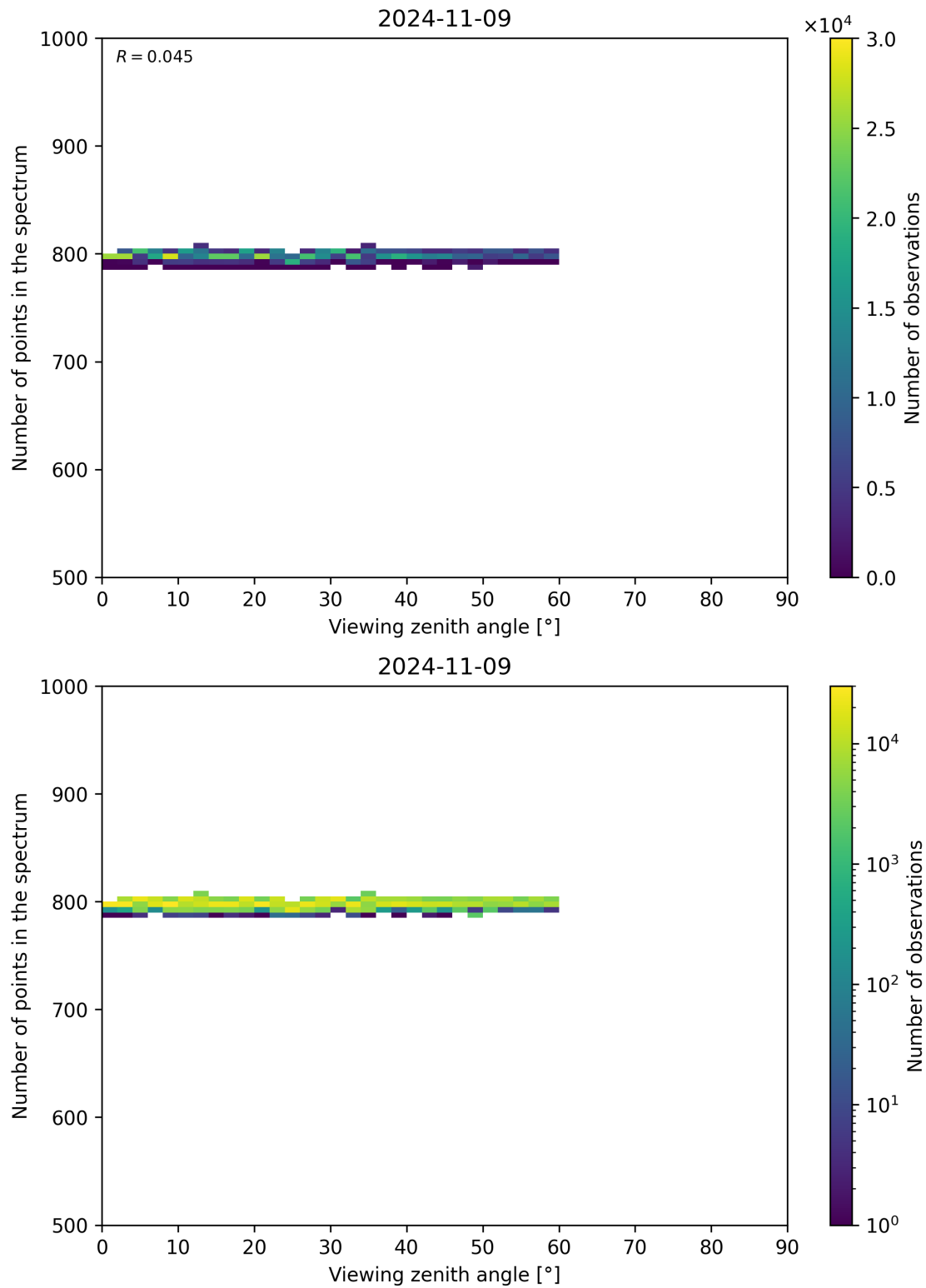
Figure 114: Scatter density plot of “Viewing zenith angle” against “Number of points in the spectrum” for 2024-11-09 to 2024-11-10.
