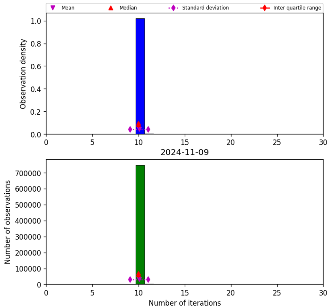
Figure 31: Histogram of “Number of iterations” for 2024-11-09 to 2024-11-10
