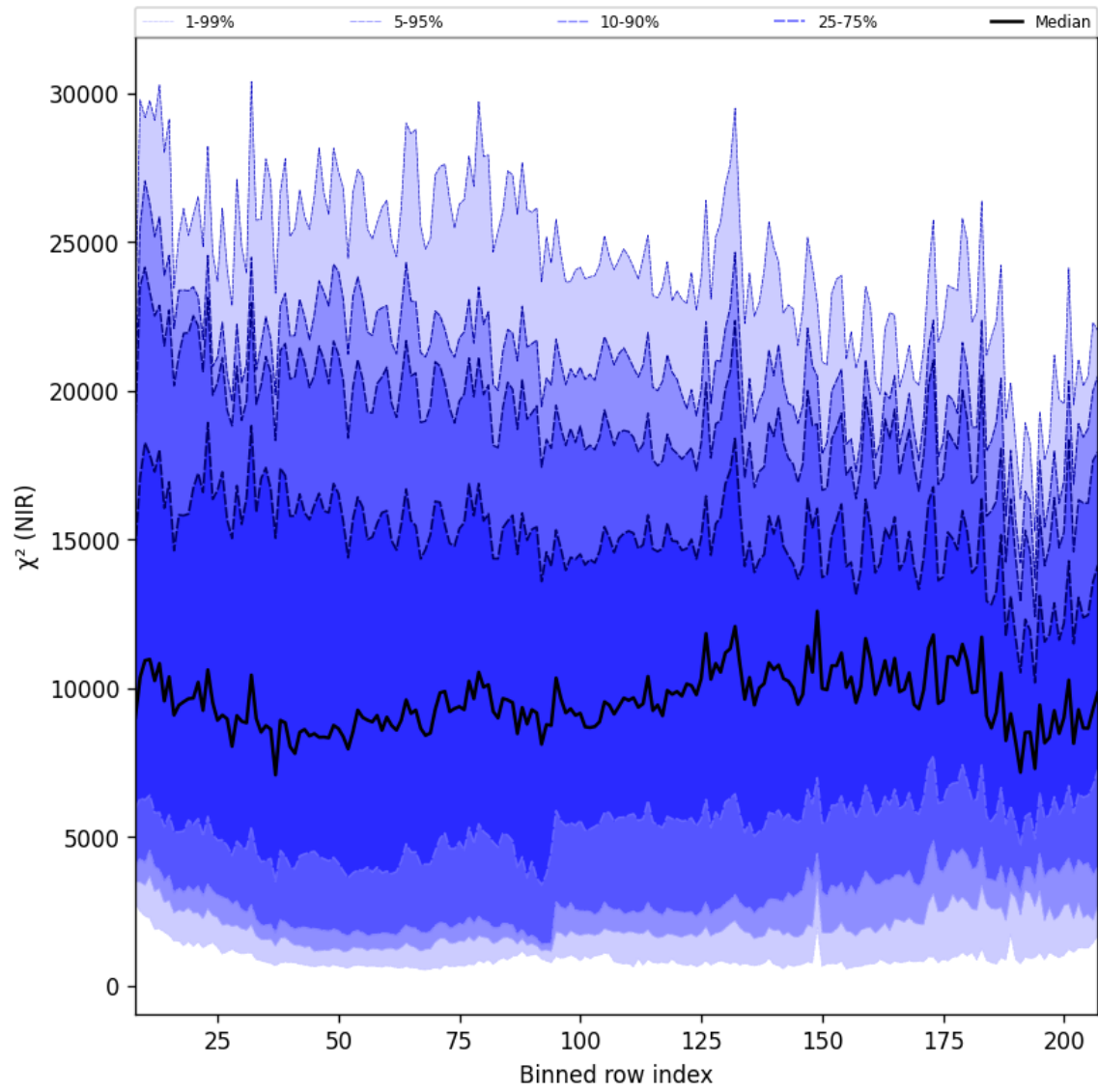
Figure 40: Along track statistics of " \chi^2 (NIR)" for 2024-11-09 to 2024-11-10
