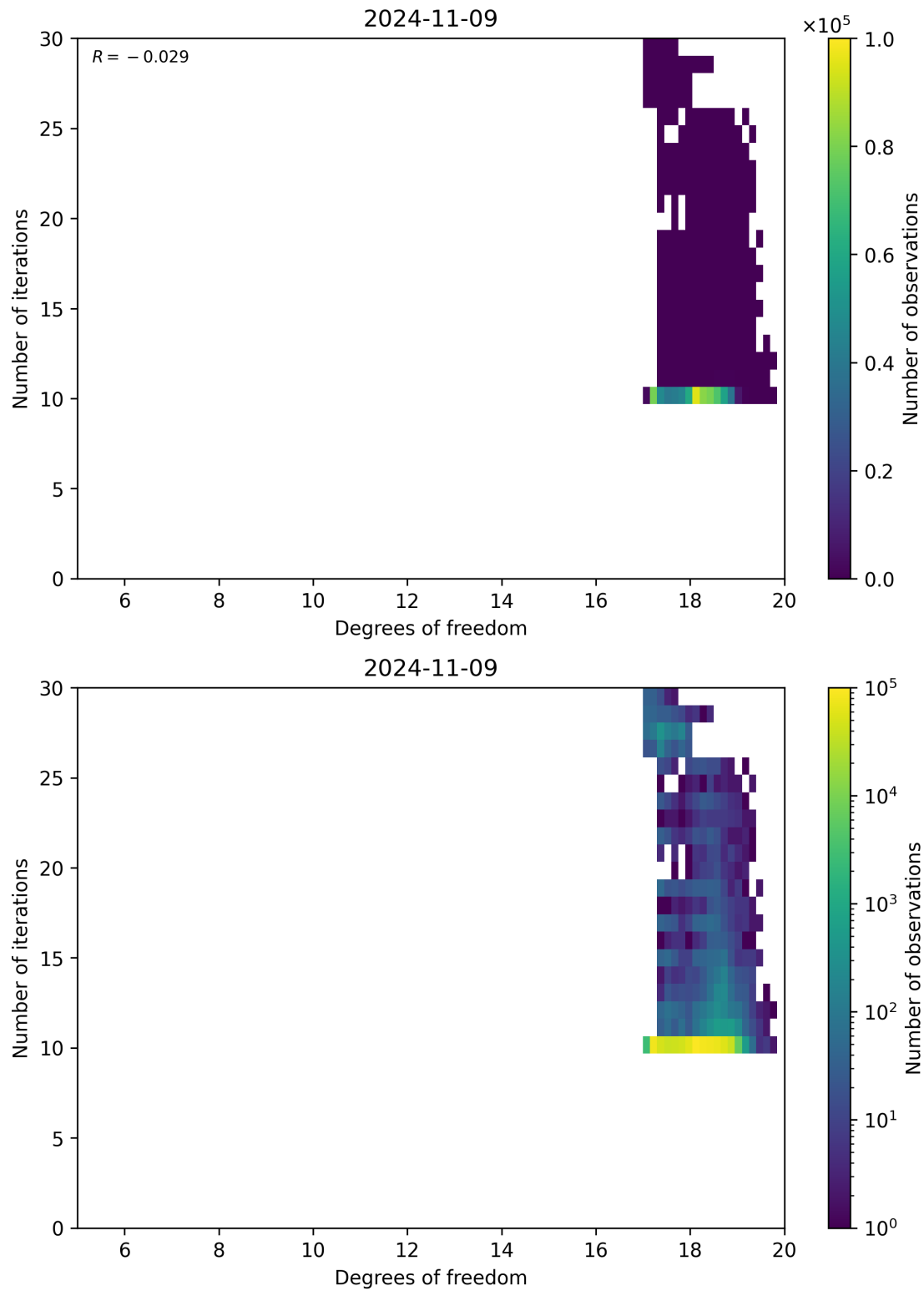
Figure 52: Scatter density plot of “Degrees of freedom” against “Number of iterations” for 2024-11-09 to 2024-11-10.
