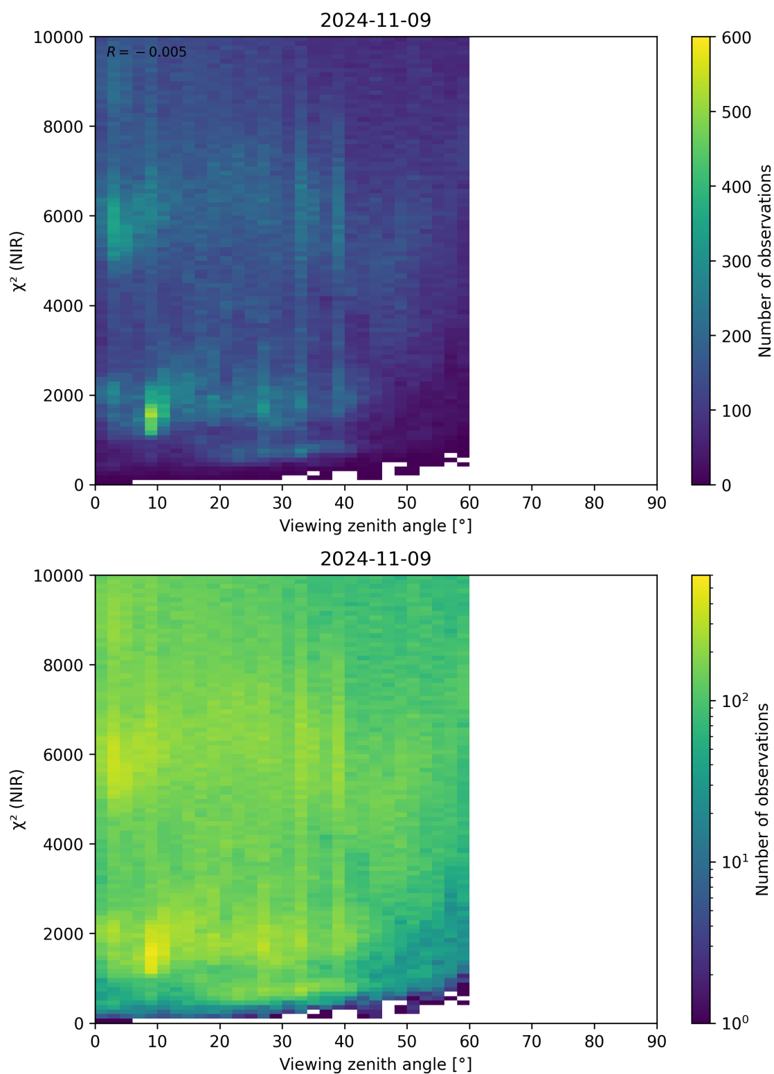
Figure 105: Scatter density plot of “Viewing zenith angle” against “ \chi^2 (NIR)” for 2024-11-09 to 2024-11-10.
