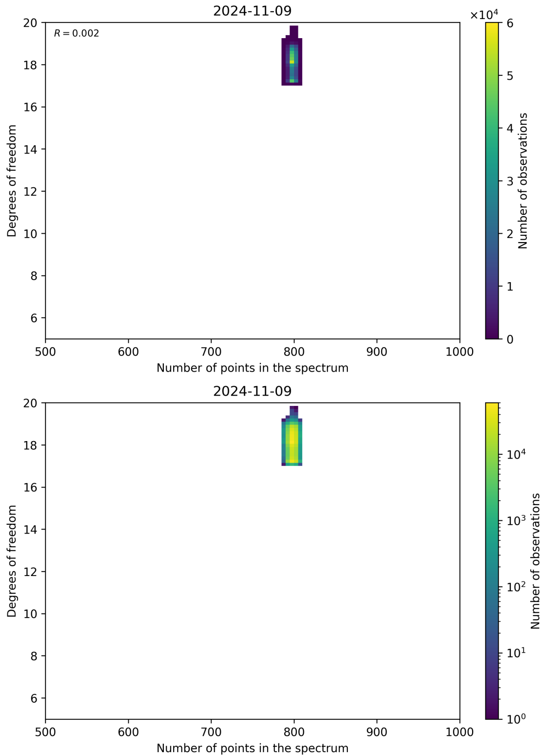
Figure 90: Scatter density plot of “Number of points in the spectrum” against “Degrees of freedom” for 2024-11-09 to 2024-11-10.
