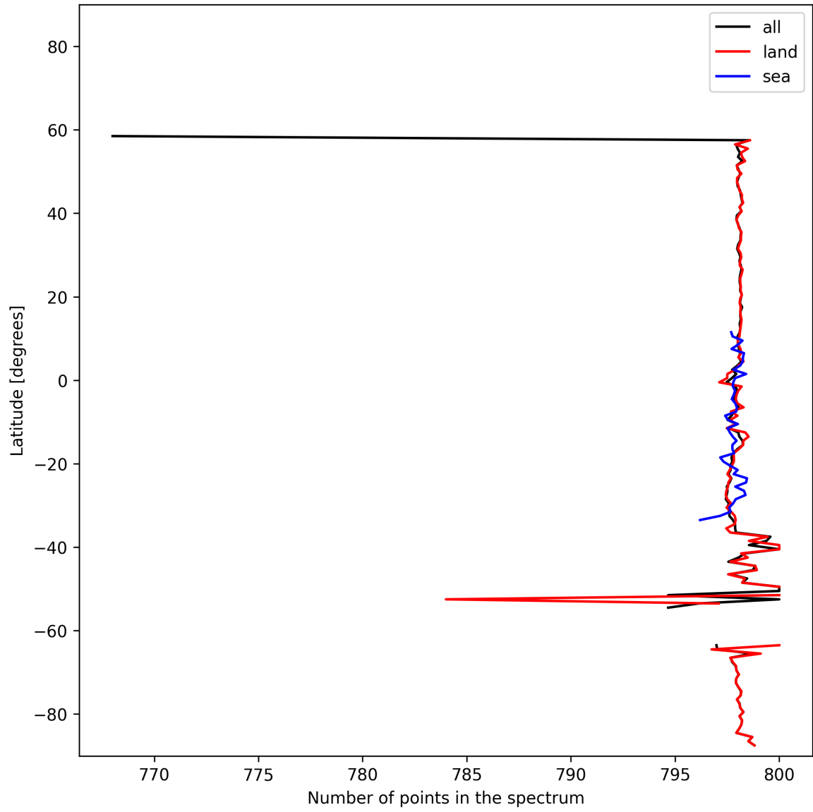
Figure 15: Zonal average of “Number of points in the spectrum” for 2024-11-09 to 2024-11-10.
