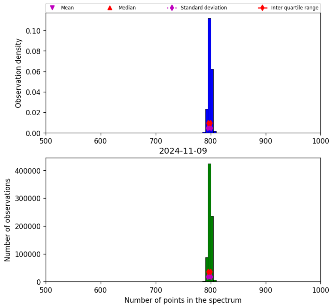
Figure 26: Histogram of “Number of points in the spectrum” for 2024-11-09 to 2024-11-10
