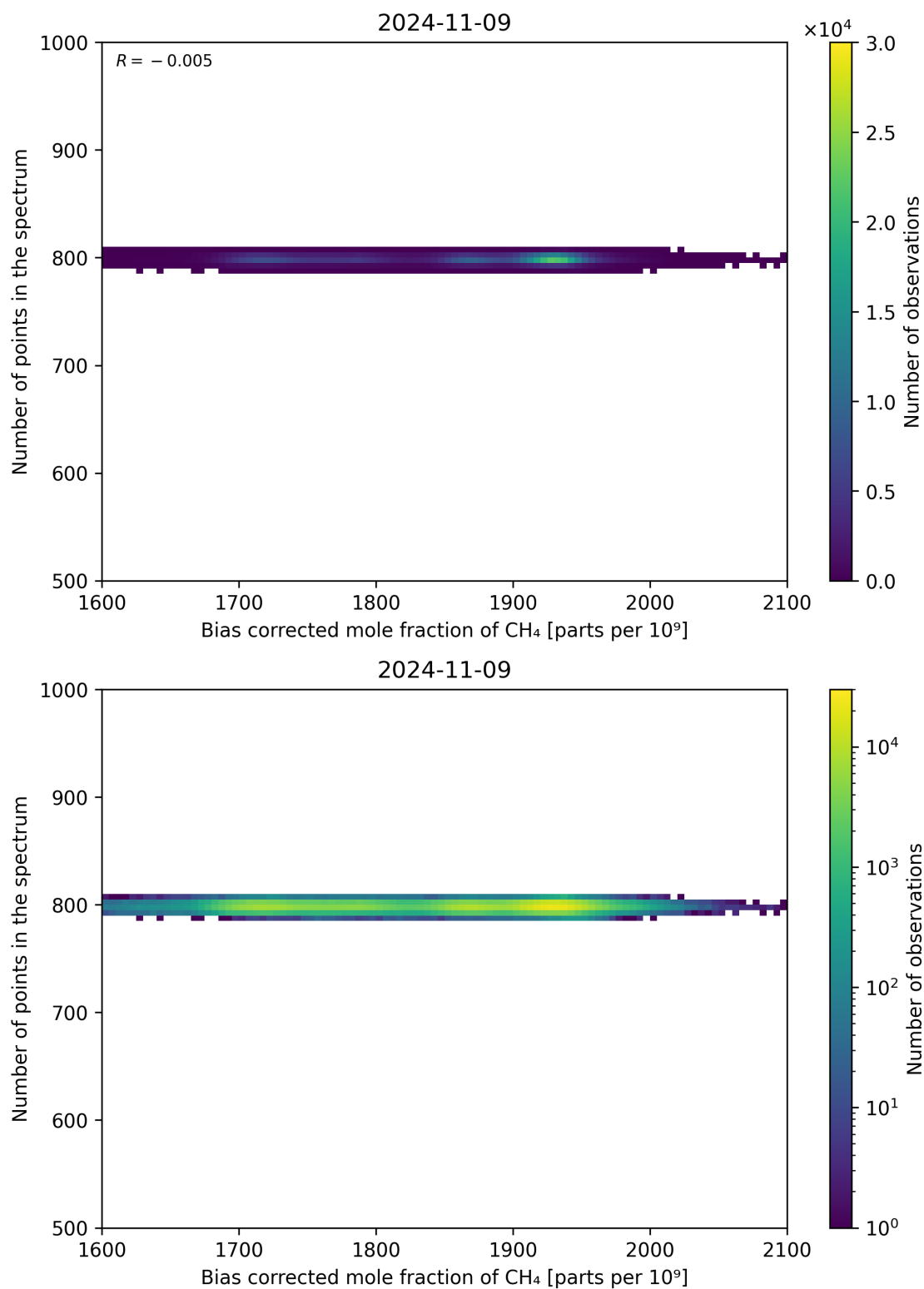
Figure 68: Scatter density plot of “Bias corrected mole fraction of CH 4 ” against “Number of points in the spectrum” for 2024-11-09 to 2024-11-10.
