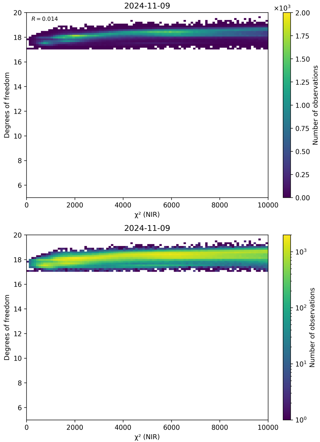
Figure 44: Scatter density plot of “ \chi^2 (NIR)” against “Degrees of freedom” for 2024-11-09 to 2024-11-10.
