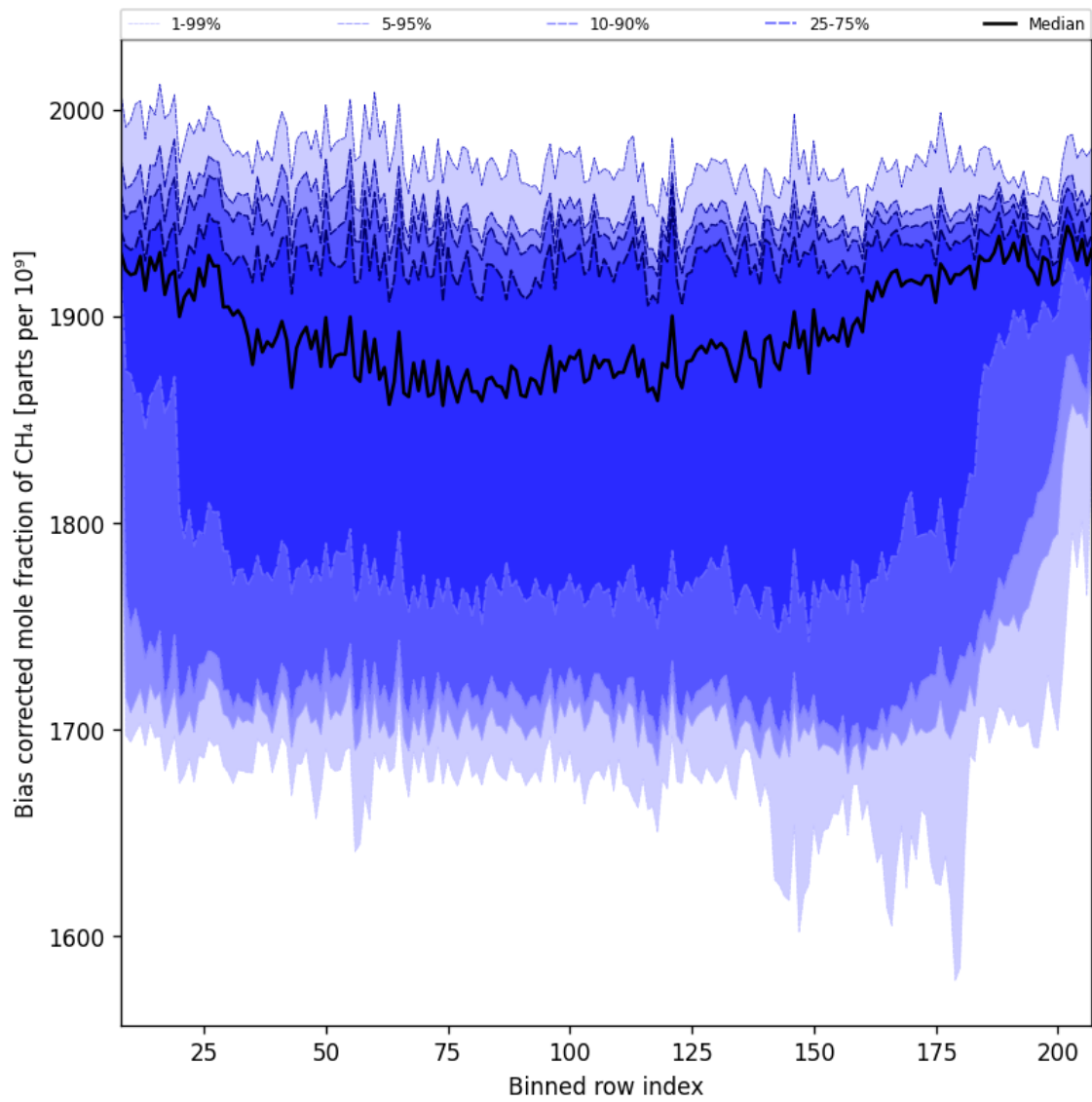
Figure 36: Along track statistics of “Bias corrected mole fraction of CH 4 ” for 2024-11-09 to 2024-11-10
