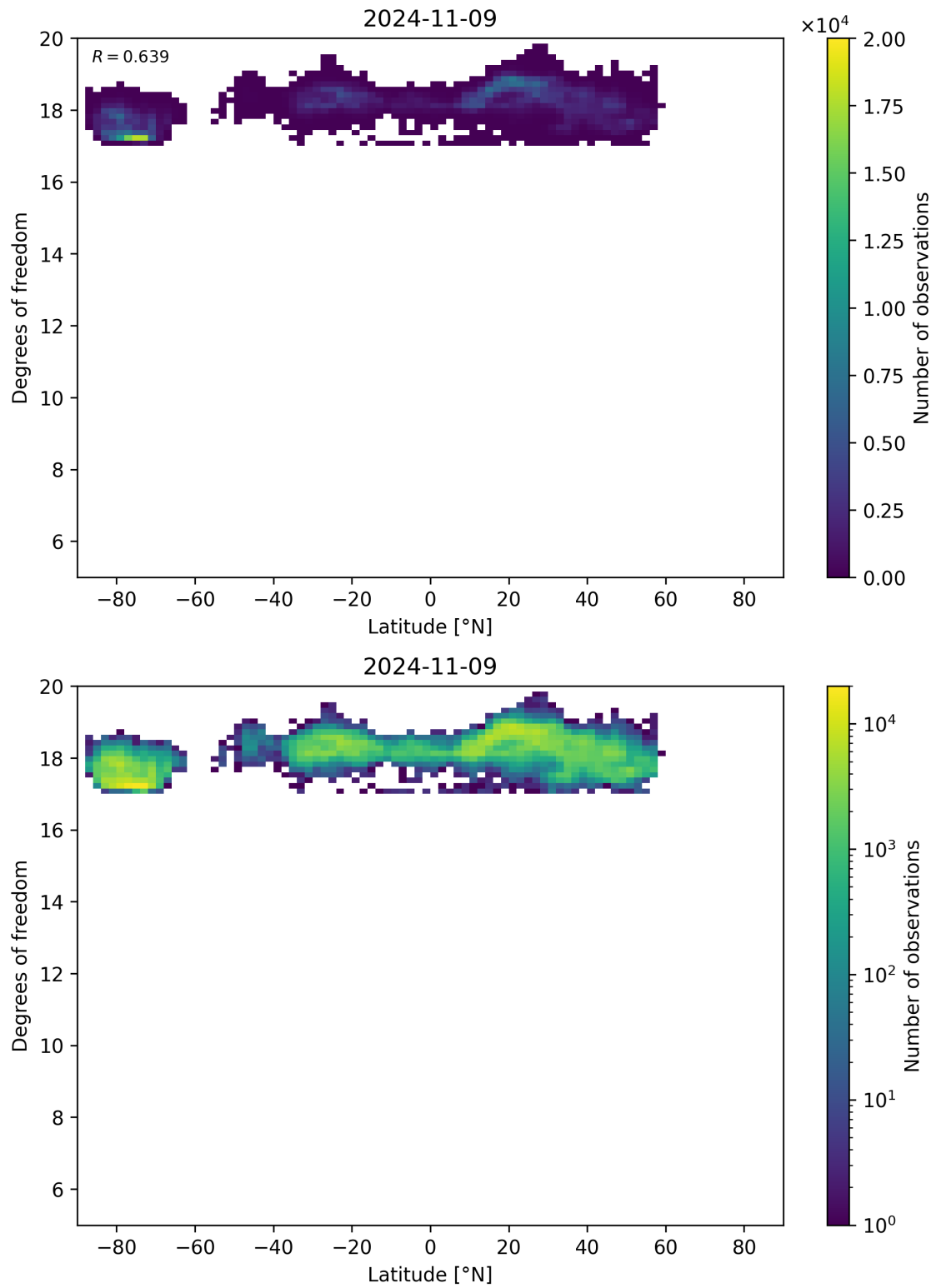
Figure 55: Scatter density plot of “Latitude” against “Degrees of freedom” for 2024-11-09 to 2024-11-10.
