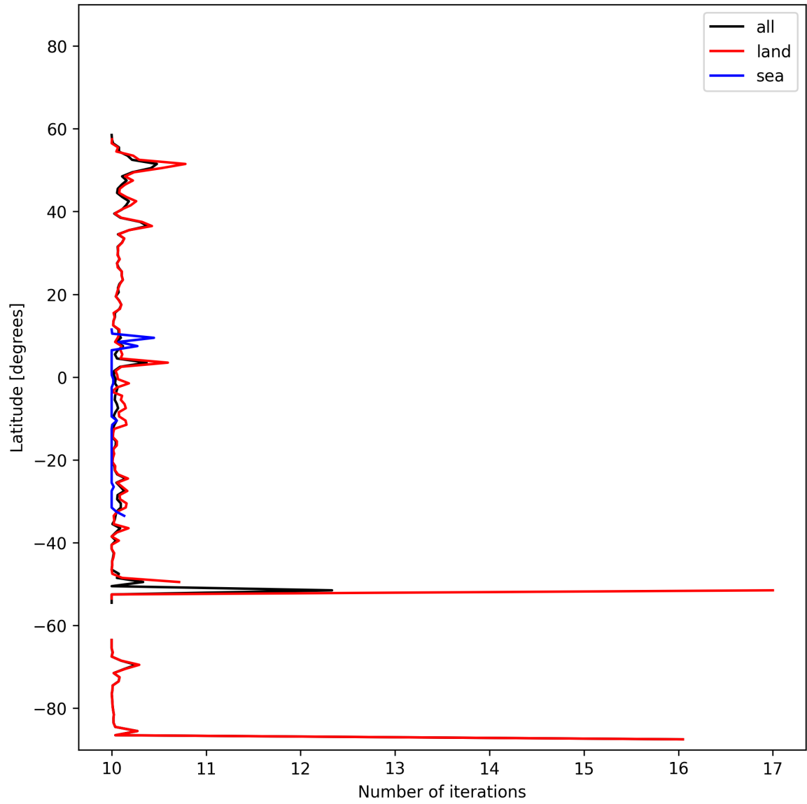
Figure 20: Zonal average of “Number of iterations” for 2024-11-09 to 2024-11-10.
