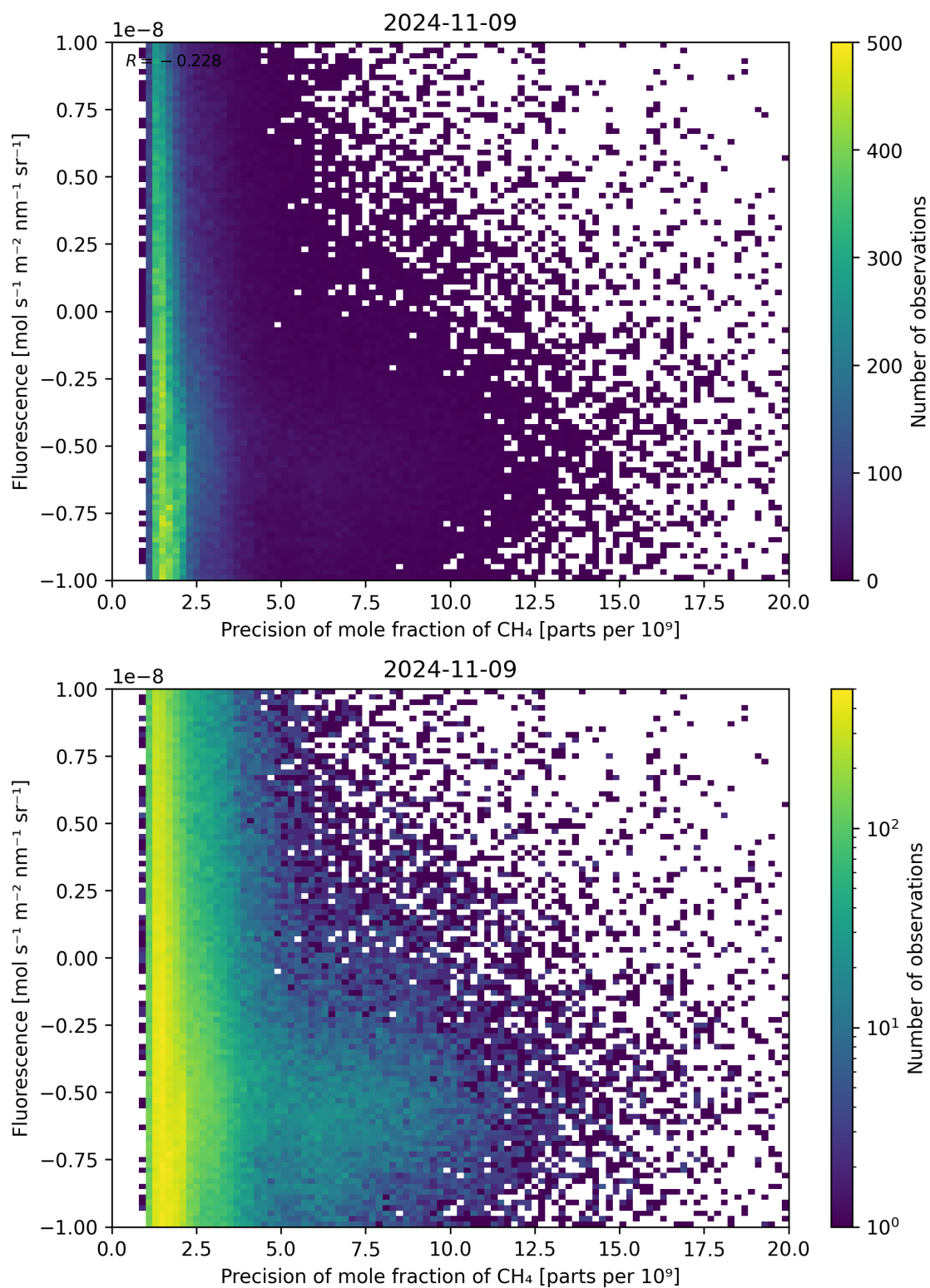
Figure 81: Scatter density plot of “Precision of mole fraction of \text{CH}_4 ” against “Fluorescence” for 2024-11-09 to 2024-11-10.
