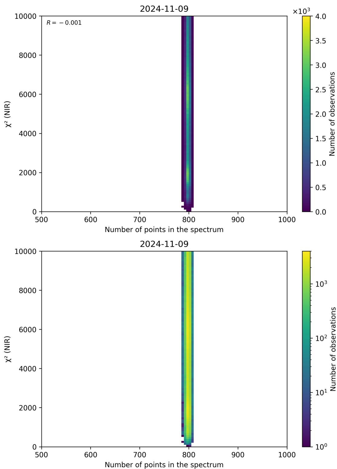
Figure 88: Scatter density plot of “Number of points in the spectrum” against “ \chi^2 (NIR)” for 2024-11-09 to 2024-11-10.
