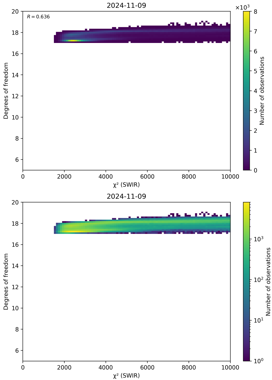
Figure 48: Scatter density plot of “ \chi^2 (SWIR)” against “Degrees of freedom” for 2024-11-09 to 2024-11-10.
