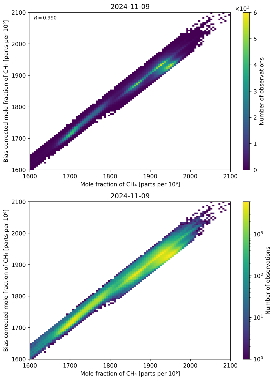
Figure 74: Scatter density plot of “Mole fraction of CH 4 ” against “Bias corrected mole fraction of CH 4 ” for 2024-11-09 to 2024-11-10.
