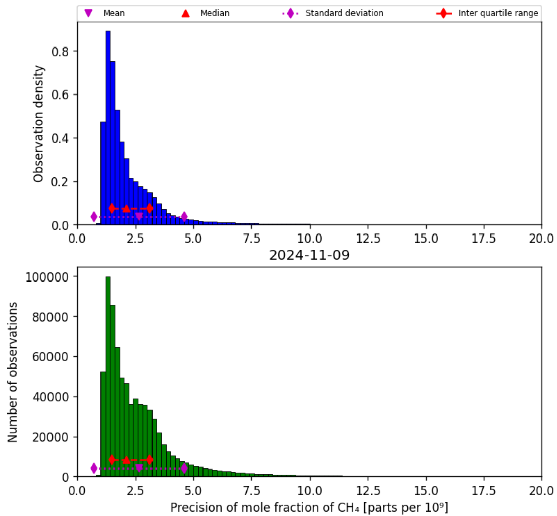
Figure 24: Histogram of “Precision of mole fraction of CH 4 ” for 2024-11-09 to 2024-11-10
