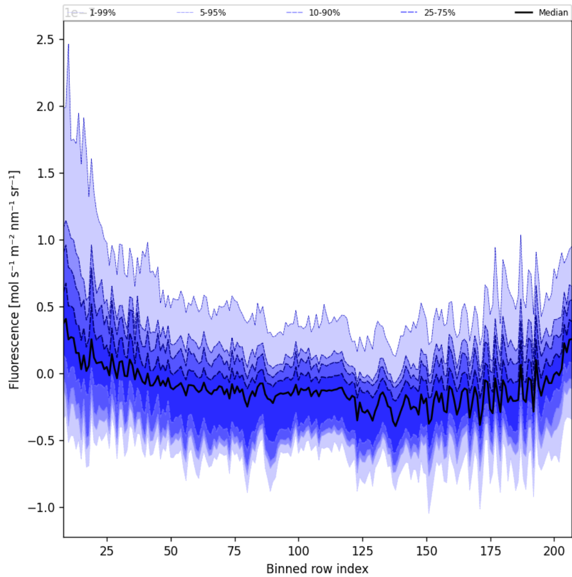
Figure 43: Along track statistics of “Fluorescence” for 2024-11-09 to 2024-11-10
