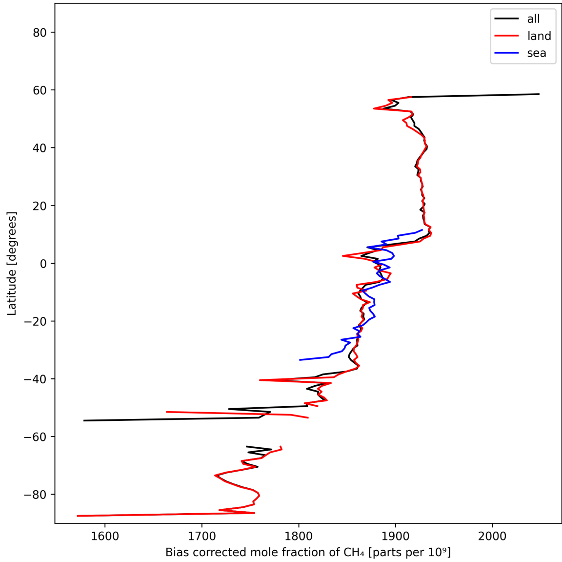
Figure 14: Zonal average of “Bias corrected mole fraction of CH 4 ” for 2024-11-09 to 2024-11-10.
