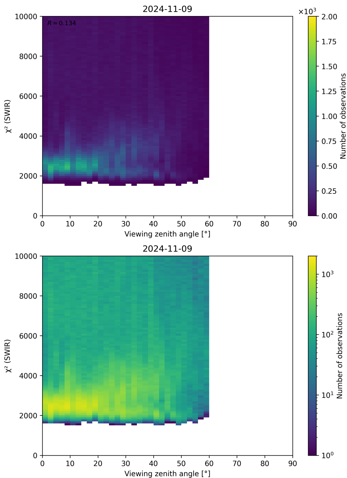
Figure 106: Scatter density plot of “Viewing zenith angle” against “ \chi^2 (SWIR)” for 2024-11-09 to 2024-11-10.
