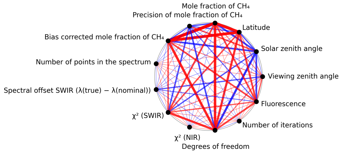
Figure 1: Map of correlation graph for 2024-11-09 to 2024-11-10.
