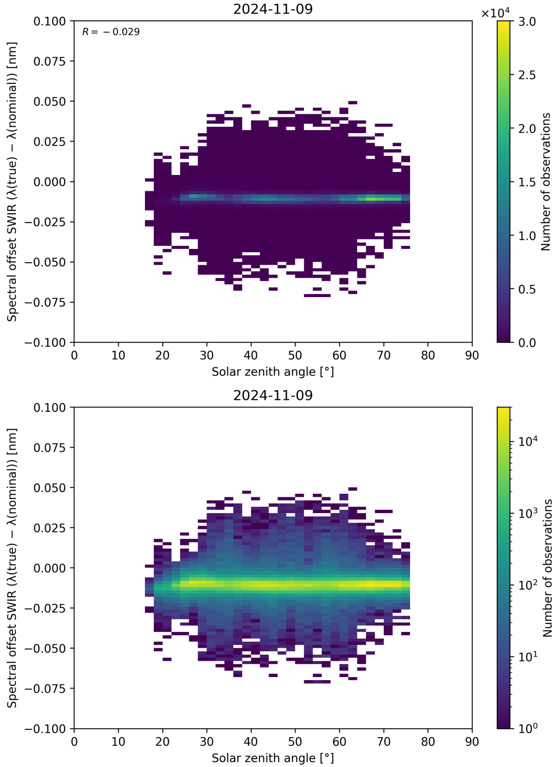
Figure 104: Scatter density plot of “Solar zenith angle” against “Spectral offset SWIR ( \lambda_{\text{true}} - \lambda_{\text{nominal}} )” for 2024-11-09 to 2024-11-10.
