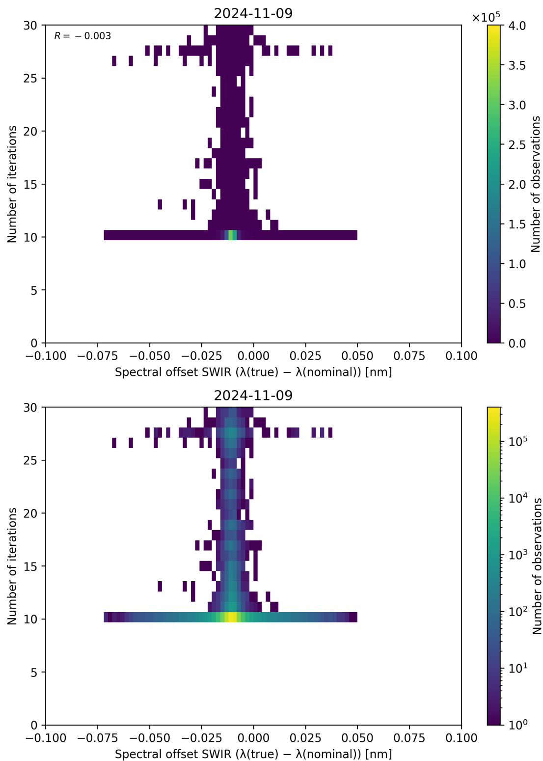
Figure 121: Scatter density plot of “Spectral offset SWIR ( \lambda_{\text{true}} - \lambda_{\text{nominal}} )” against “Number of iterations” for 2024-11-09 to 2024-11-10.
