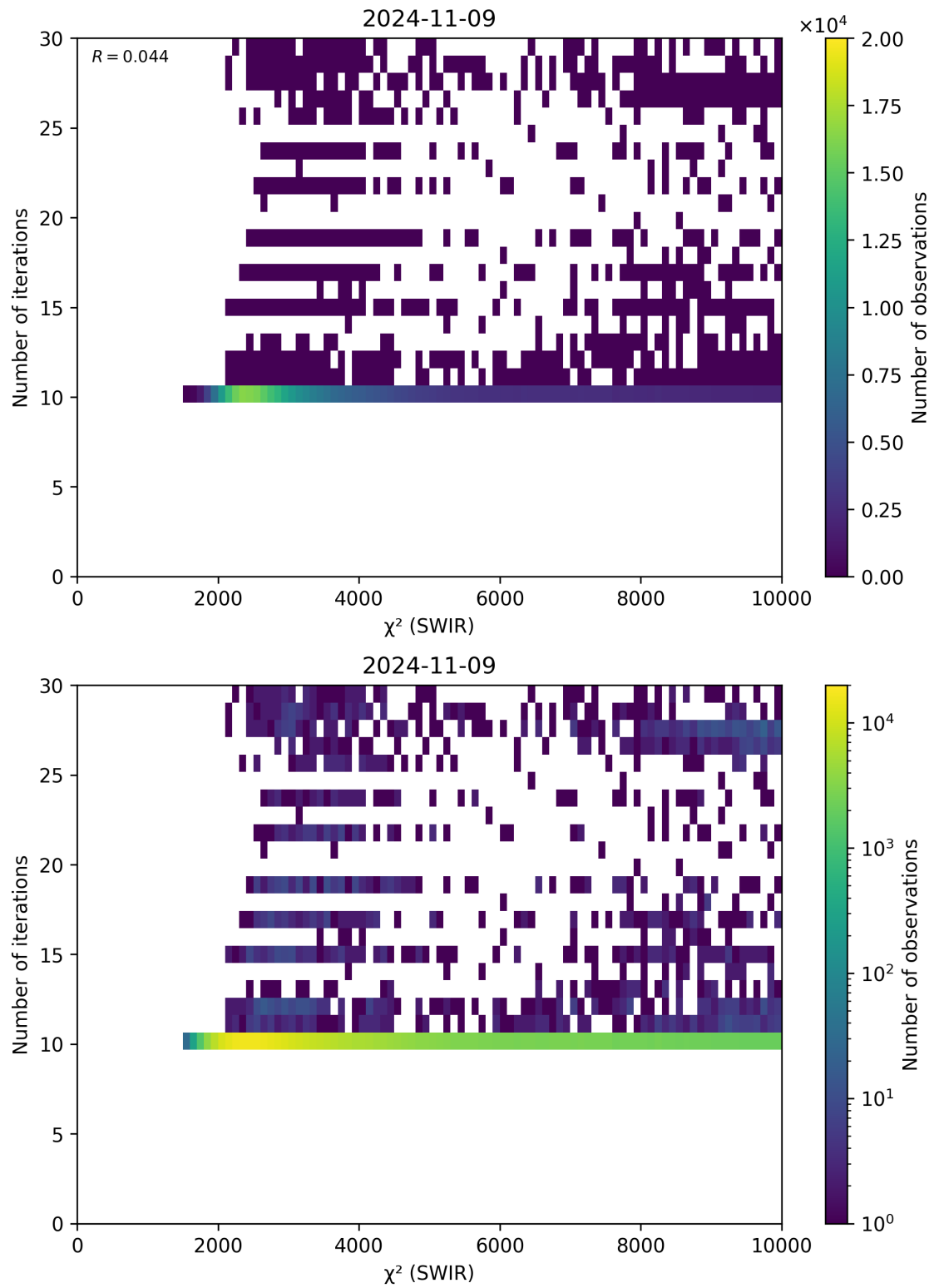
Figure 50: Scatter density plot of “ \chi^2 (SWIR)” against “Number of iterations” for 2024-11-09 to 2024-11-10.
