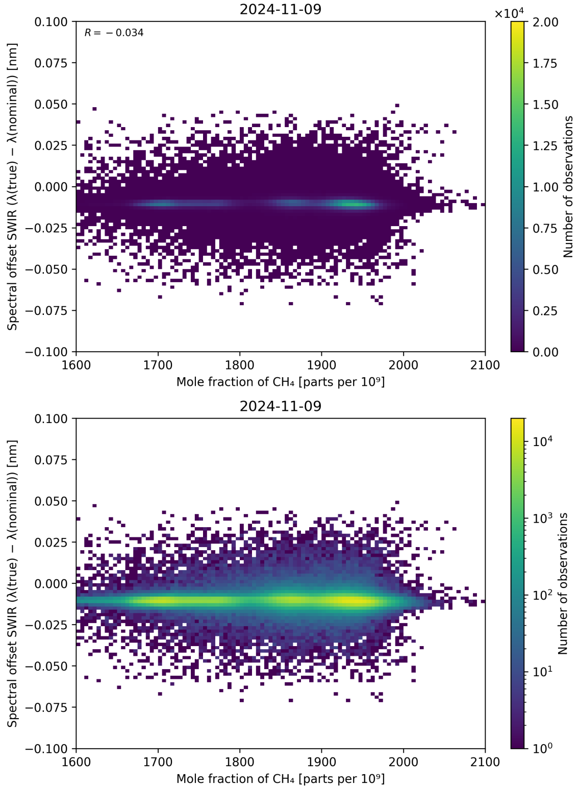
Figure 86: Scatter density plot of “Mole fraction of \text{CH}_4 ” against “Spectral offset SWIR ( \lambda_{\text{true}} - \lambda_{\text{nominal}} )” for 2024-11-09 to 2024-11-10.
