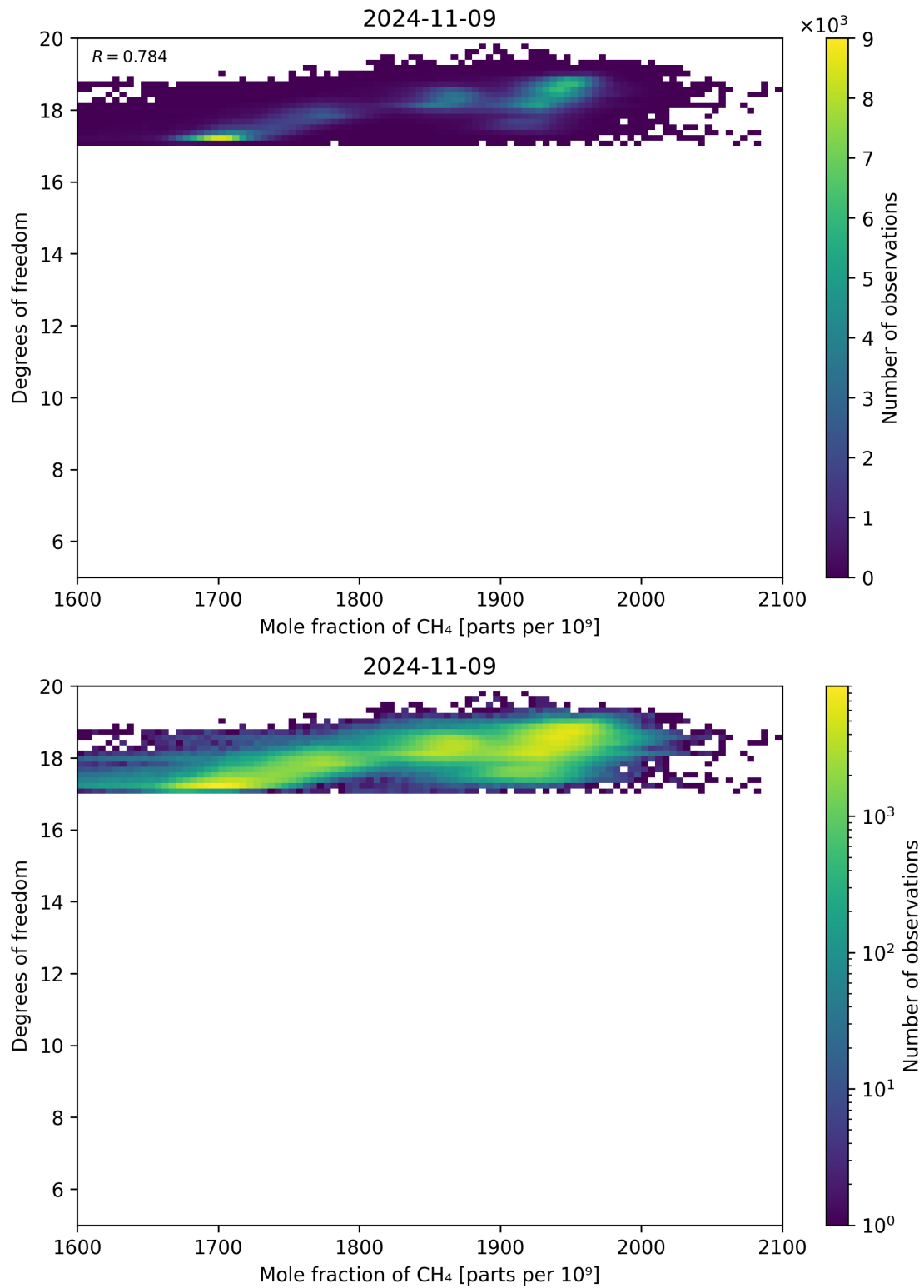
Figure 72: Scatter density plot of “Mole fraction of CH 4 ” against “Degrees of freedom” for 2024-11-09 to 2024-11-10.
