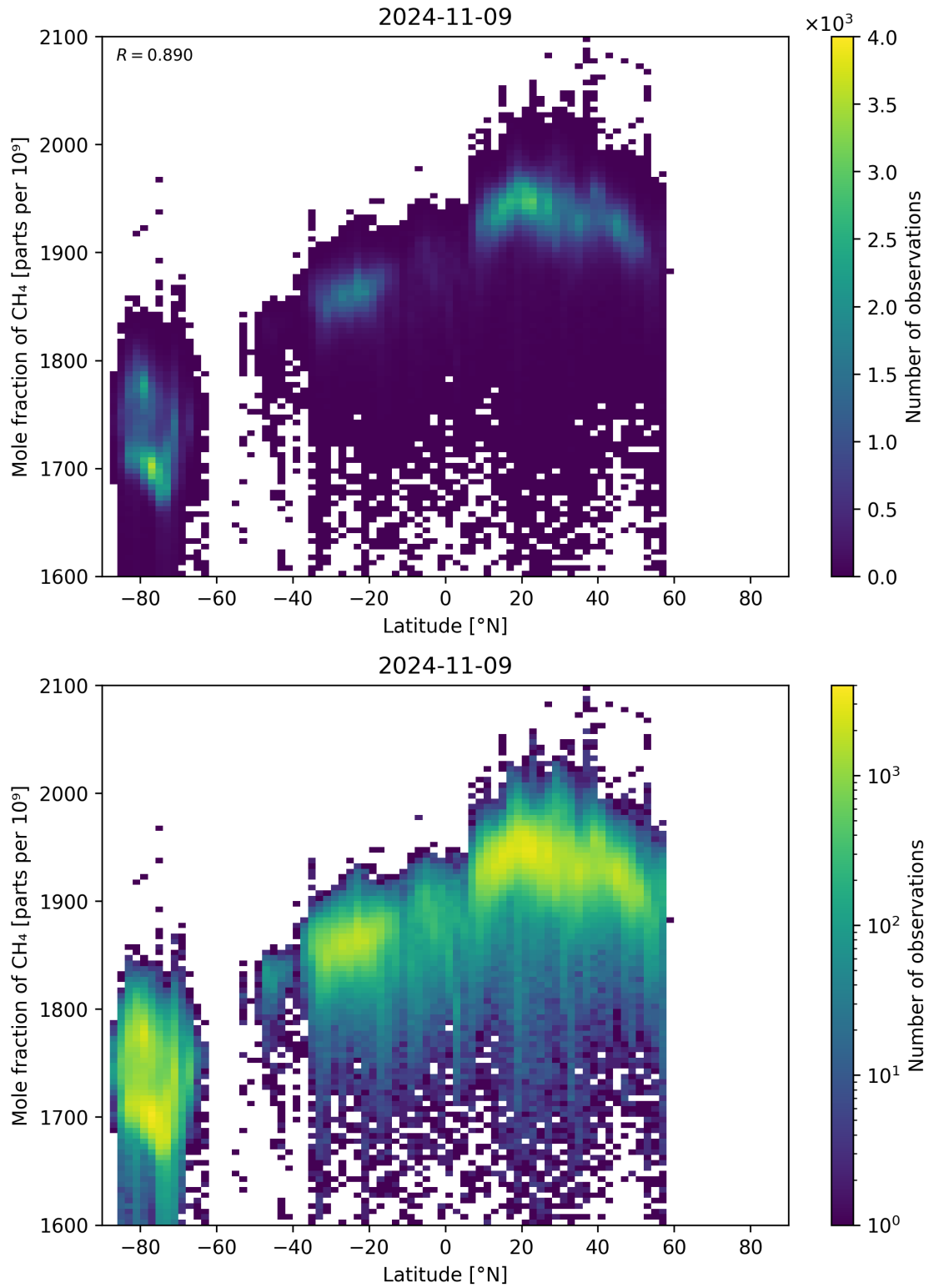
Figure 57: Scatter density plot of “Latitude” against “Mole fraction of CH 4 ” for 2024-11-09 to 2024-11-10.
