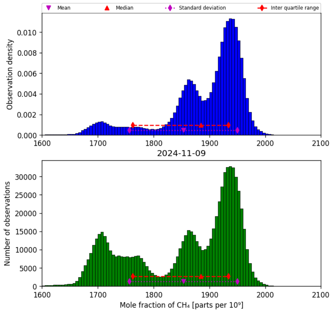
Figure 23: Histogram of “Mole fraction of CH 4 ” for 2024-11-09 to 2024-11-10
