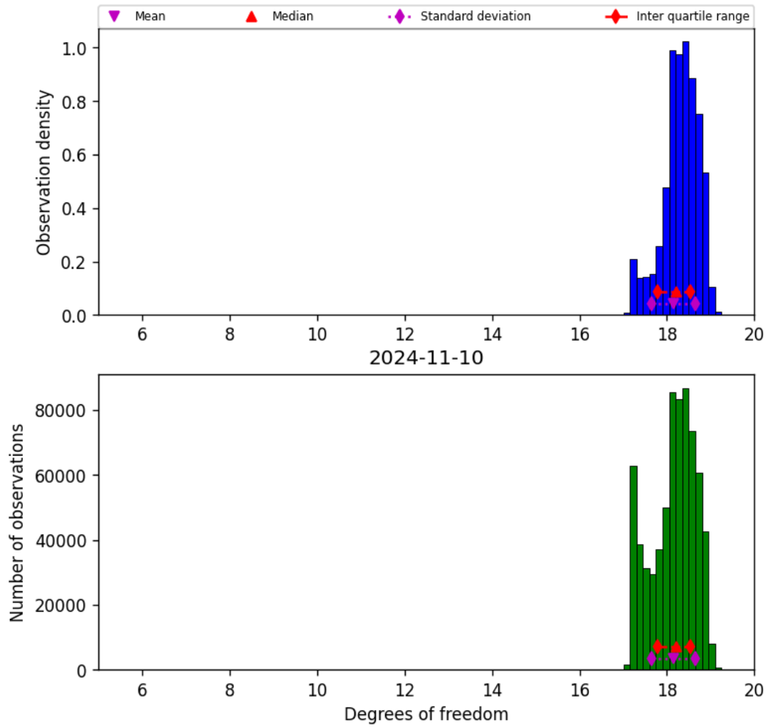
Figure 30: Histogram of “Degrees of freedom” for 2024-11-09 to 2024-11-11
