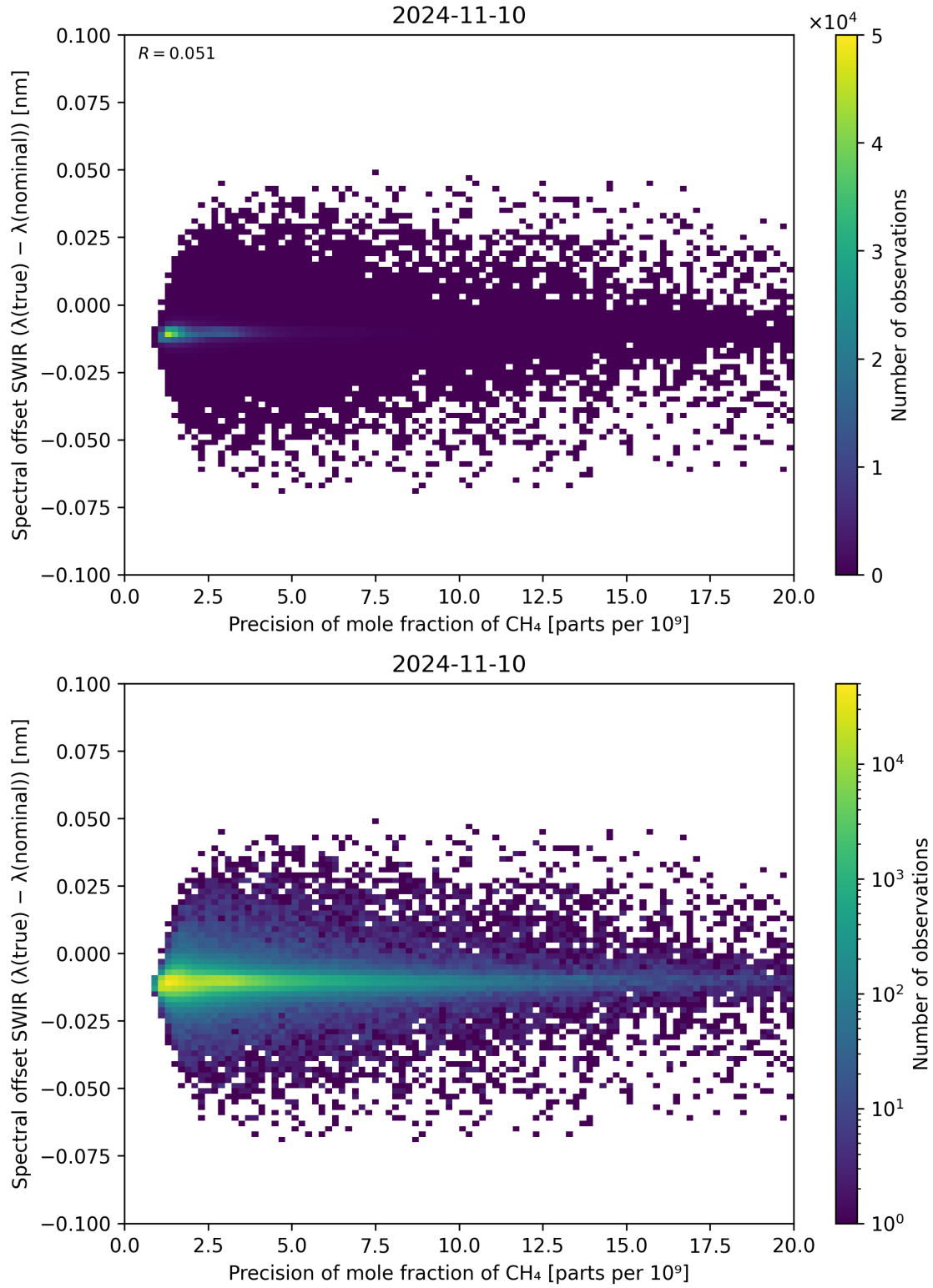
Figure 85: Scatter density plot of “Precision of mole fraction of \text{CH}_4 ” against “Spectral offset SWIR ( \lambda_{\text{true}} - \lambda_{\text{nominal}} )” for 2024-11-09 to 2024-11-11.
