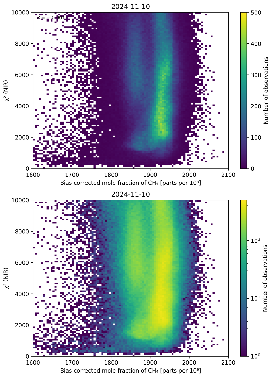
Figure 63: Scatter density plot of “Bias corrected mole fraction of CH 4 ” against “ \chi^2 (NIR)” for 2024-11-09 to 2024-11-11.
