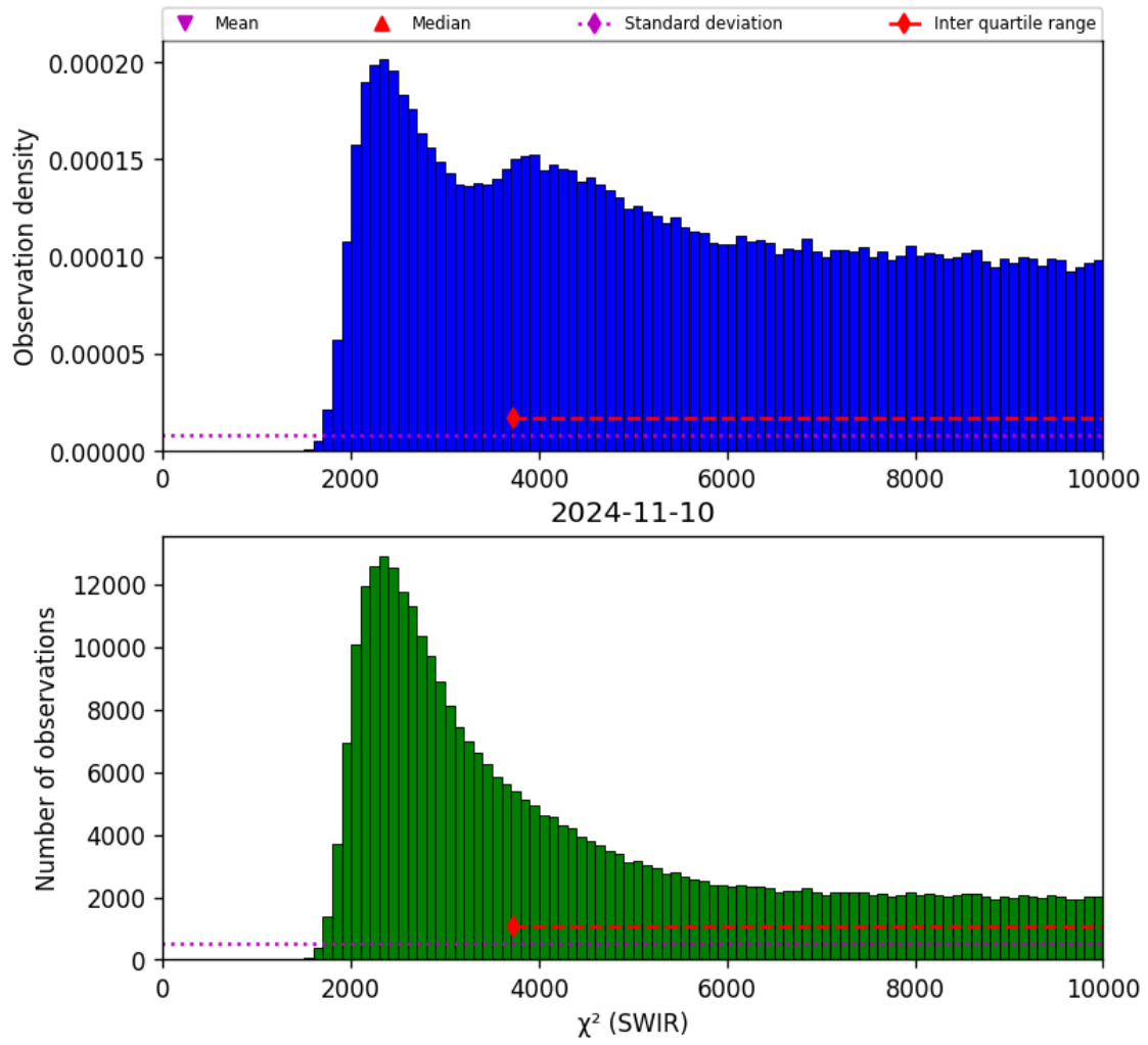
Figure 28: Histogram of “ \chi^2 (SWIR)” for 2024-11-09 to 2024-11-11
