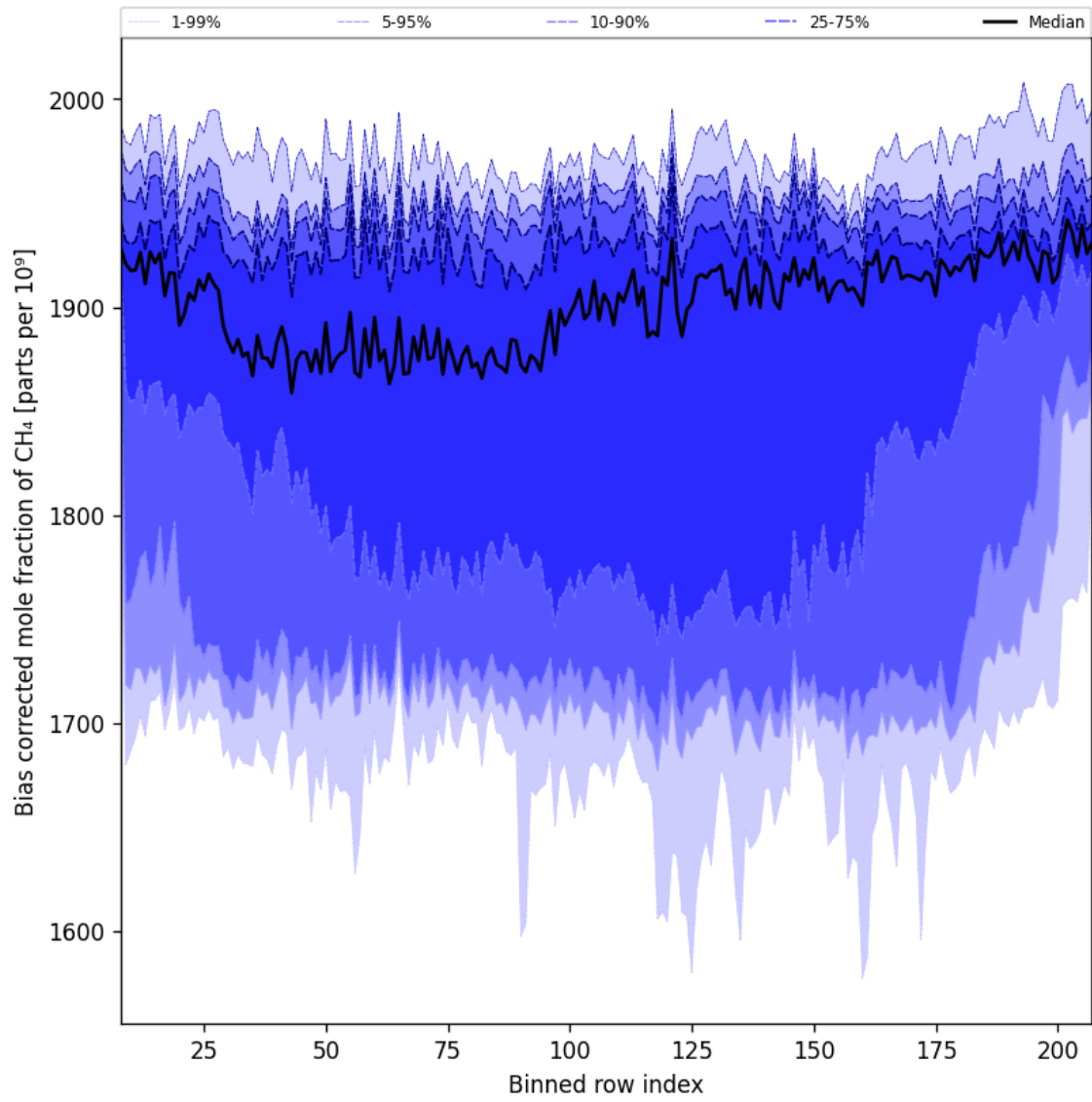
Figure 36: Along track statistics of “Bias corrected mole fraction of CH 4 ” for 2024-11-09 to 2024-11-11
