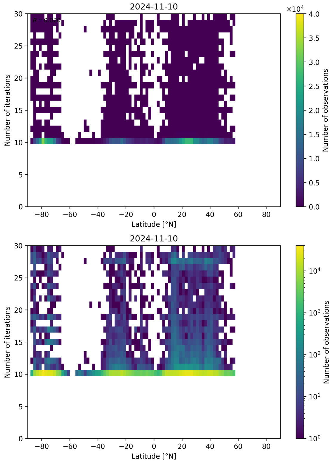
Figure 60: Scatter density plot of “Latitude” against “Number of iterations” for 2024-11-09 to 2024-11-11.
