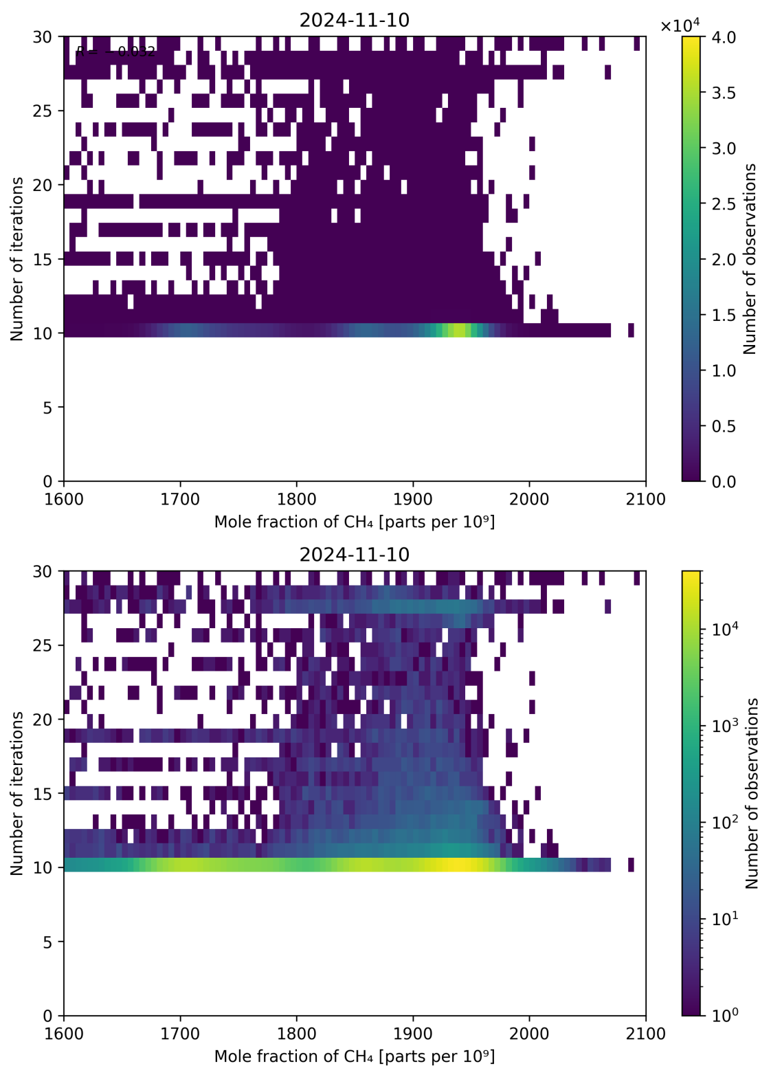
Figure 76: Scatter density plot of “Mole fraction of CH 4 ” against “Number of iterations” for 2024-11-09 to 2024-11-11.
