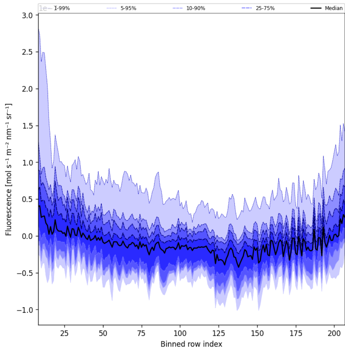
Figure 43: Along track statistics of “Fluorescence” for 2024-11-09 to 2024-11-11
