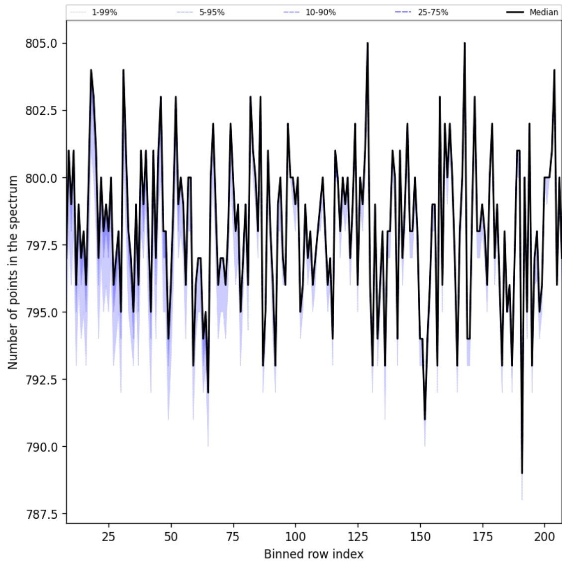
Figure 37: Along track statistics of “Number of points in the spectrum” for 2024-11-09 to 2024-11-11
