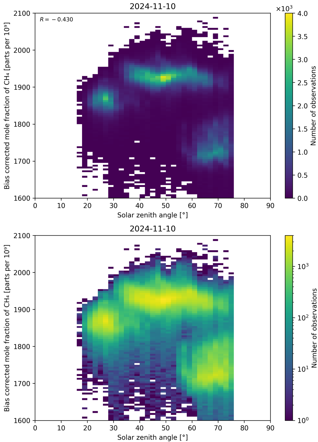
Figure 100: Scatter density plot of “Solar zenith angle” against “Bias corrected mole fraction of \text{CH}_4 ” for 2024-11-09 to 2024-11-11.
