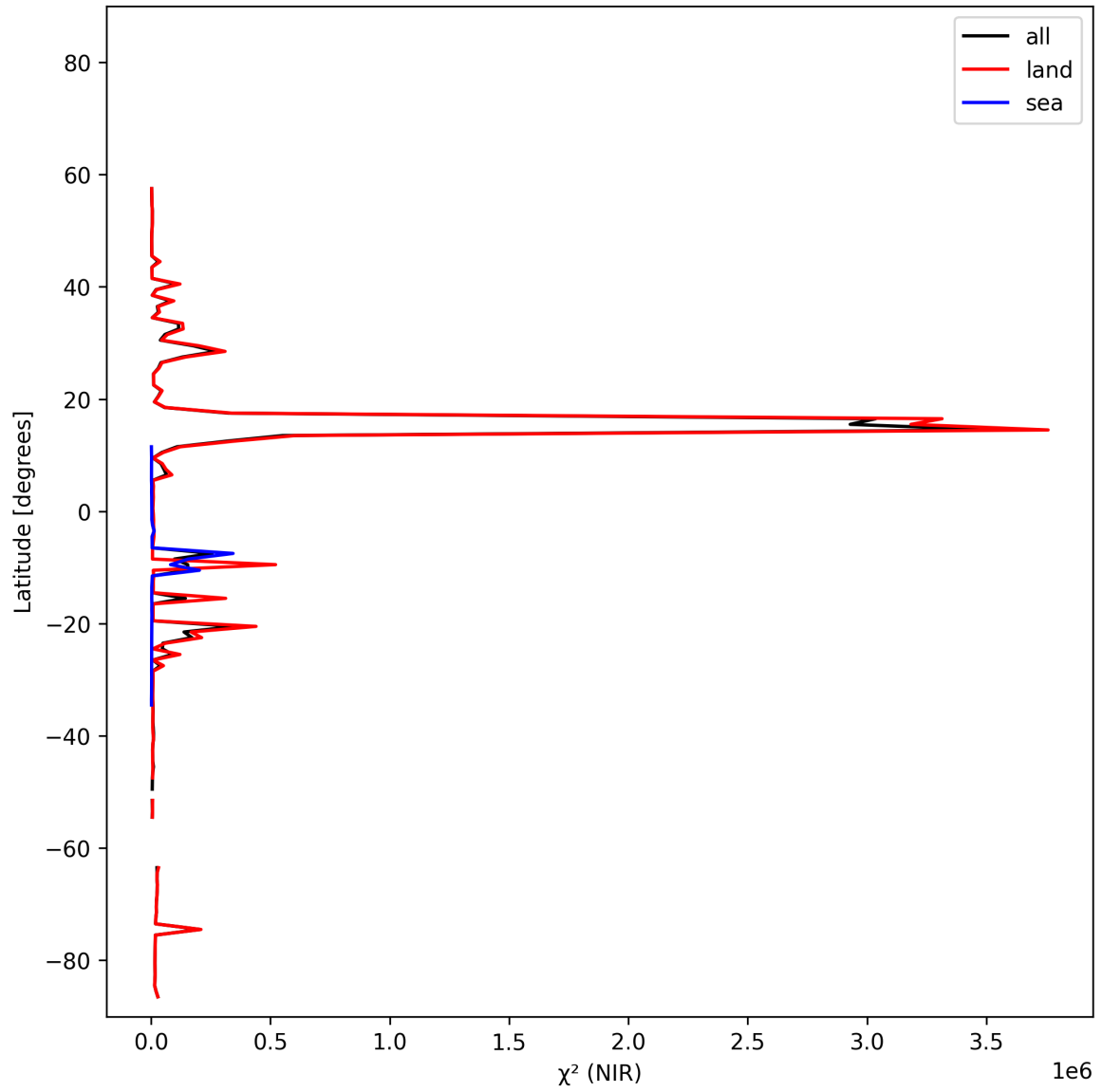
Figure 18: Zonal average of “ \chi^2 (NIR)” for 2024-11-09 to 2024-11-11.
