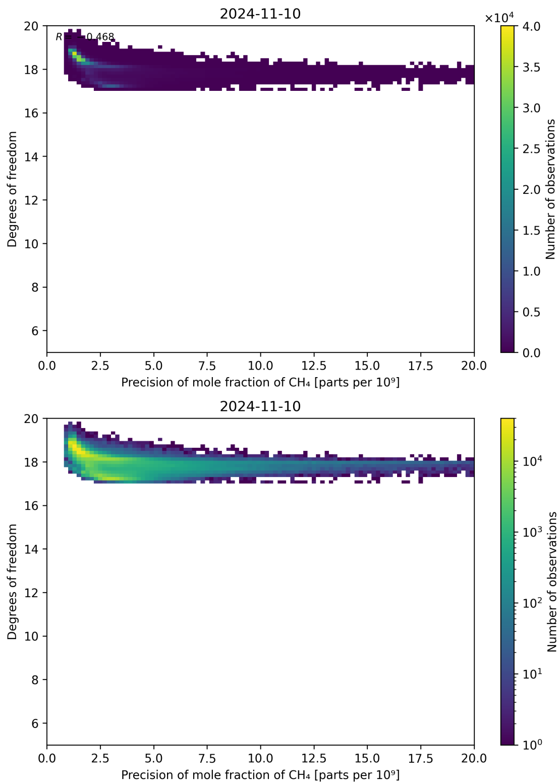
Figure 80: Scatter density plot of “Precision of mole fraction of CH 4 ” against “Degrees of freedom” for 2024-11-09 to 2024-11-11.
