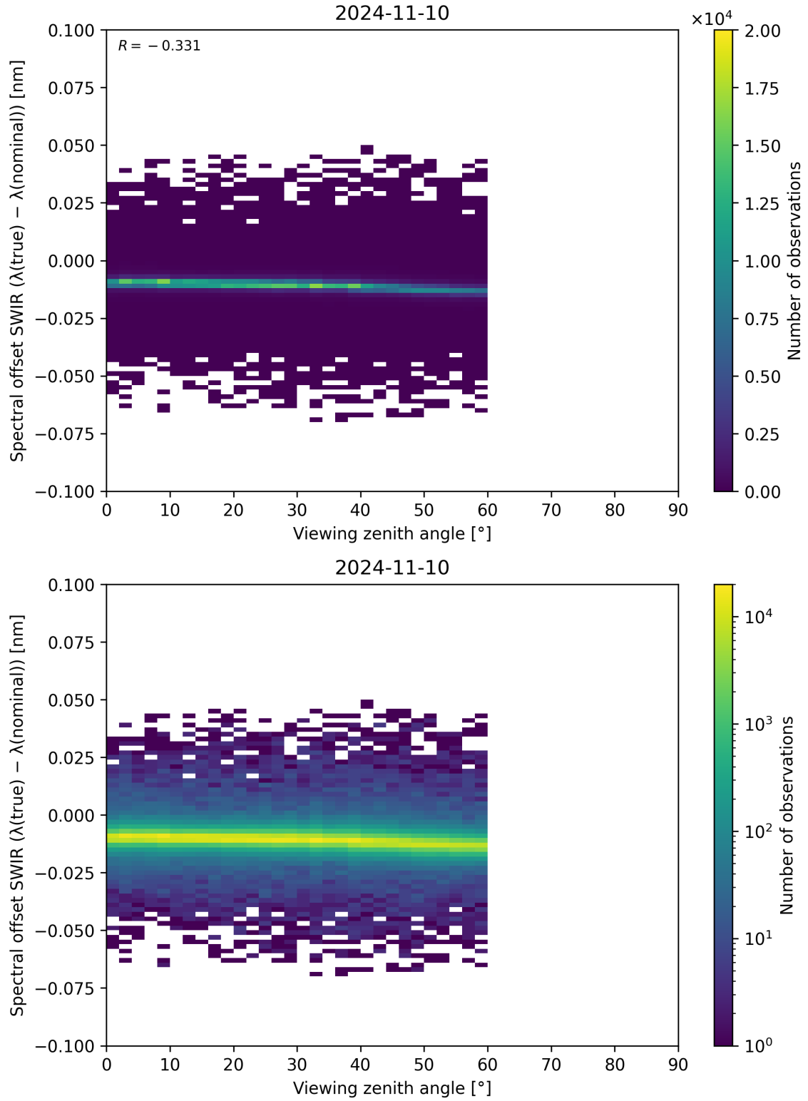
Figure 116: Scatter density plot of “Viewing zenith angle” against “Spectral offset SWIR ( \lambda_{\text{true}} - \lambda_{\text{nominal}} )” for 2024-11-09 to 2024-11-11.
