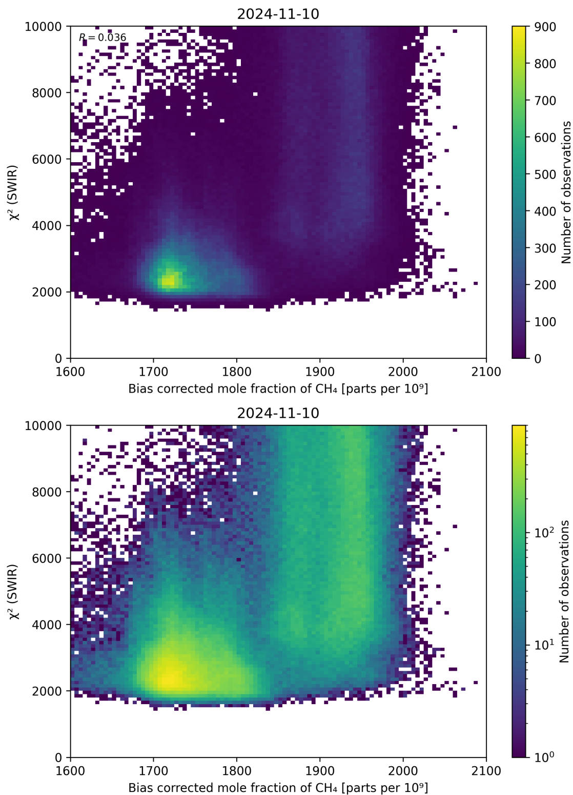
Figure 64: Scatter density plot of “Bias corrected mole fraction of \text{CH}_4 ” against “ \chi^2 (SWIR)” for 2024-11-09 to 2024-11-11.
