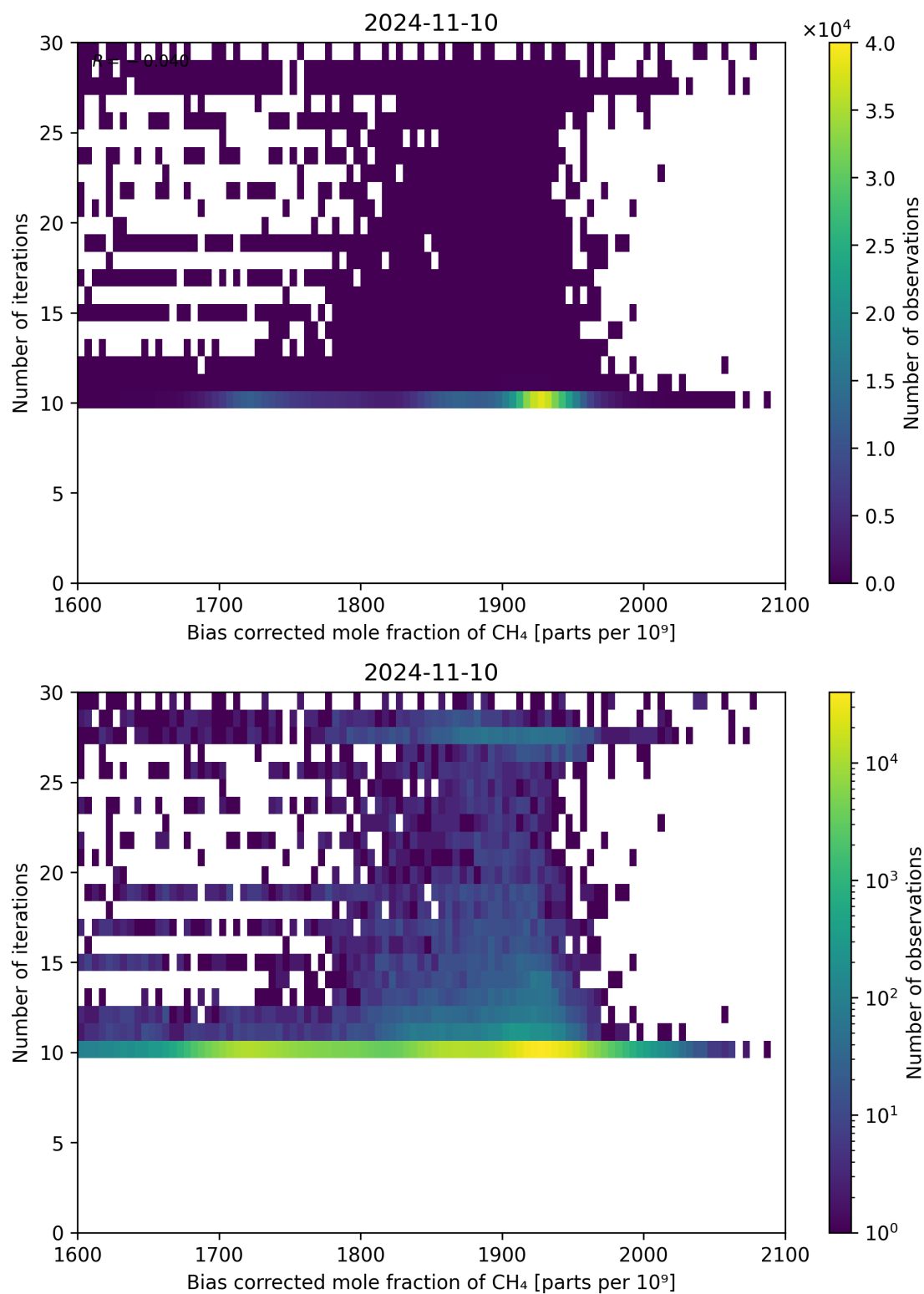
Figure 67: Scatter density plot of “Bias corrected mole fraction of CH 4 ” against “Number of iterations” for 2024-11-09 to 2024-11-11.
