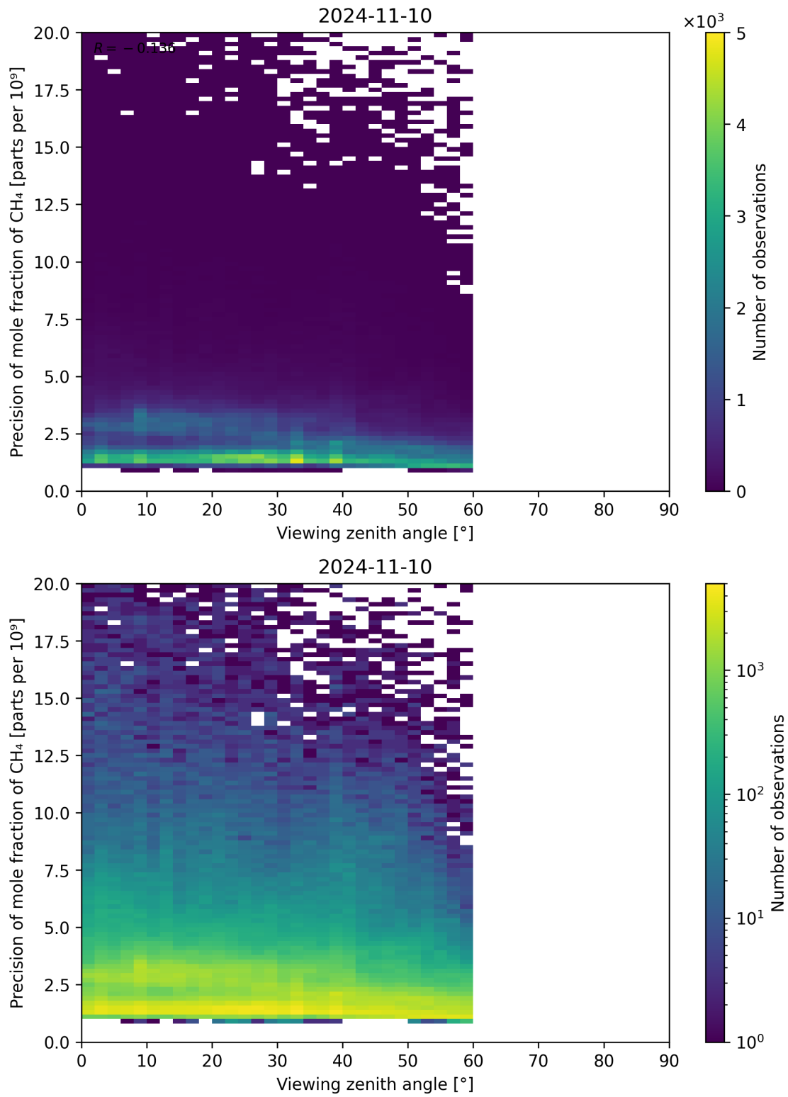
Figure 112: Scatter density plot of “Viewing zenith angle” against “Precision of mole fraction of CH 4 ” for 2024-11-09 to 2024-11-11.
