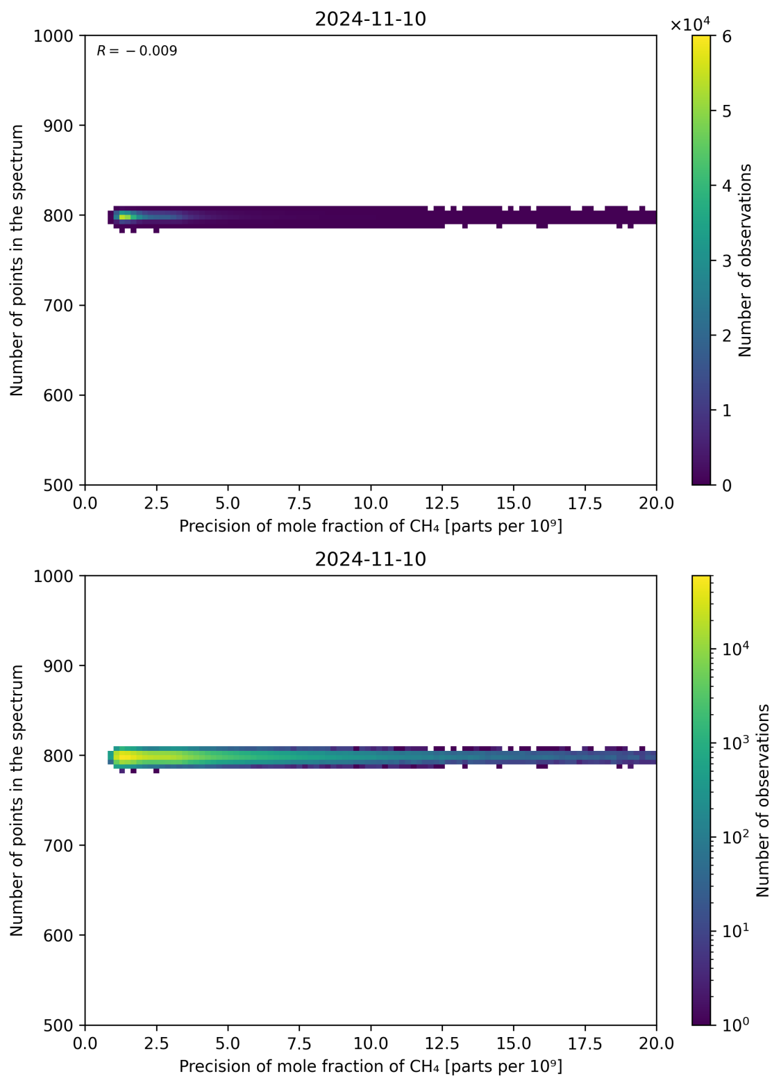
Figure 84: Scatter density plot of “Precision of mole fraction of CH 4 ” against “Number of points in the spectrum” for 2024-11-09 to 2024-11-11.
