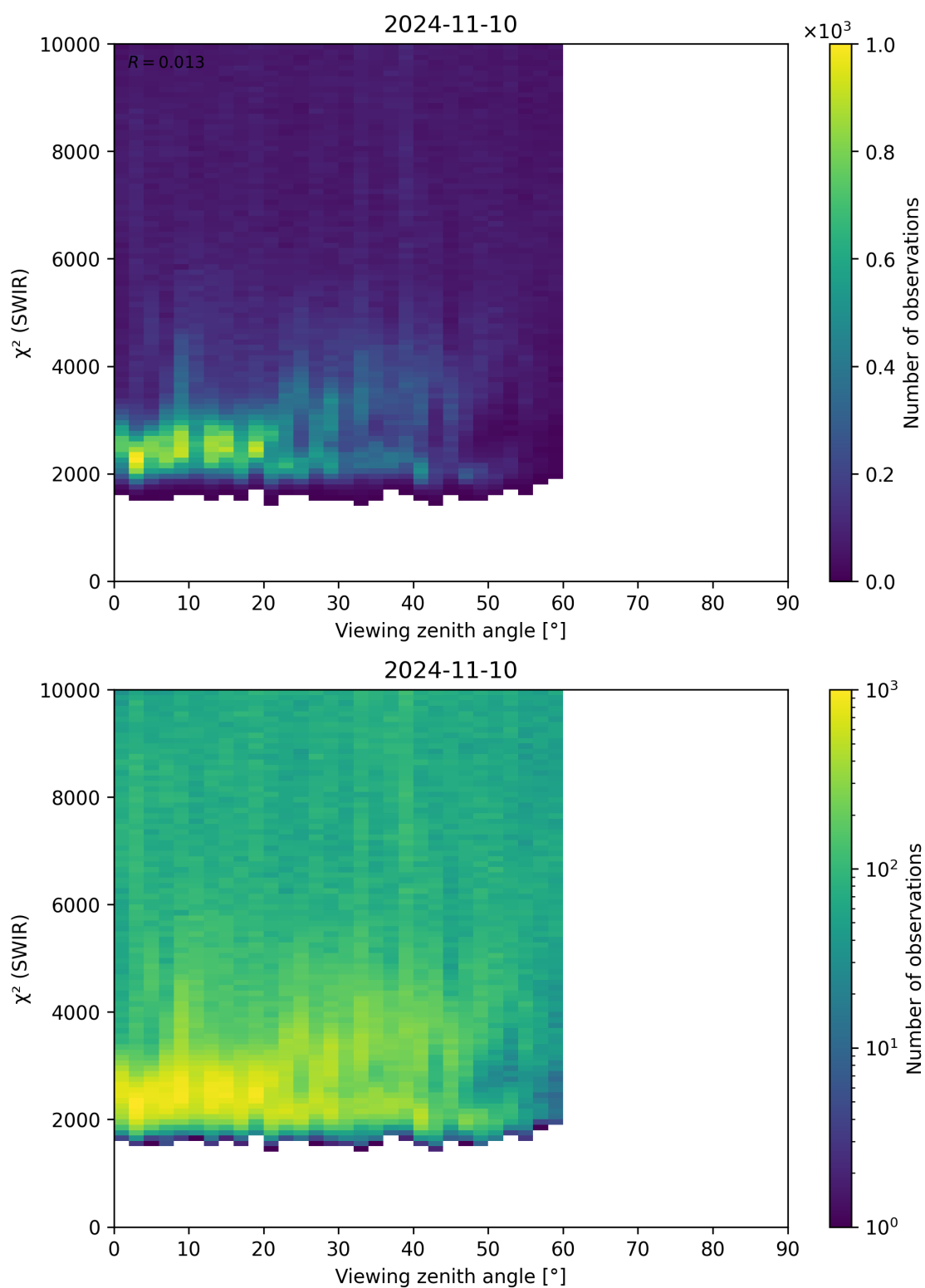
Figure 106: Scatter density plot of “Viewing zenith angle” against “ \chi^2 (SWIR)” for 2024-11-09 to 2024-11-11.
