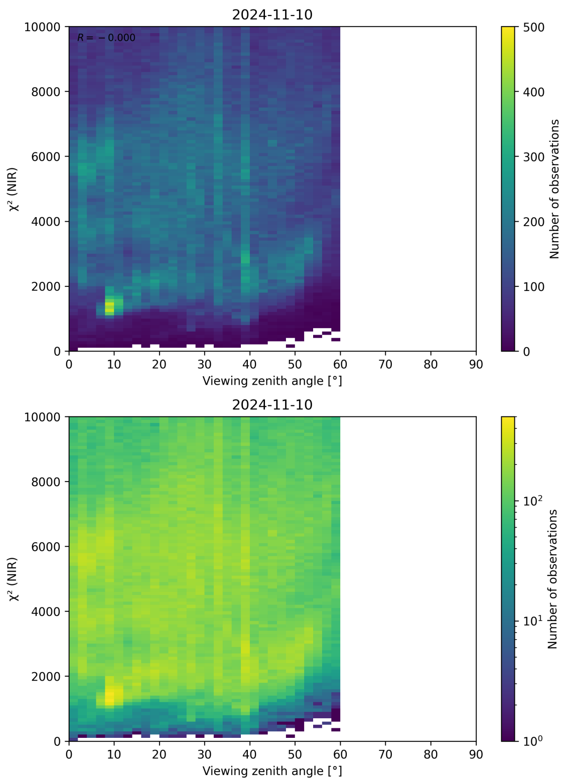
Figure 105: Scatter density plot of “Viewing zenith angle” against “ \chi^2 (NIR)” for 2024-11-09 to 2024-11-11.
