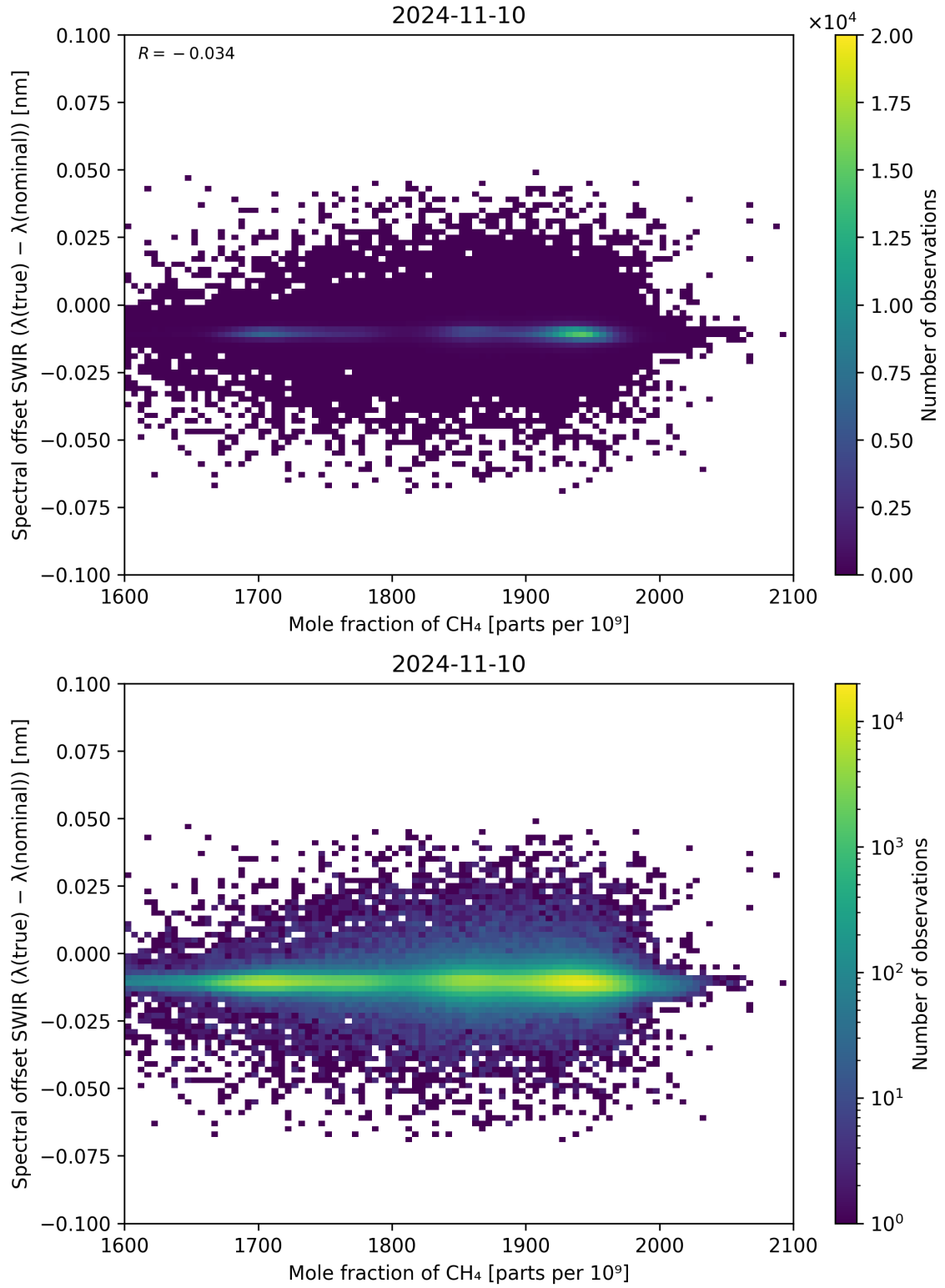
Figure 86: Scatter density plot of “Mole fraction of \text{CH}_4 ” against “Spectral offset SWIR ( \lambda_{\text{true}} - \lambda_{\text{nominal}} )” for 2024-11-09 to 2024-11-11.
