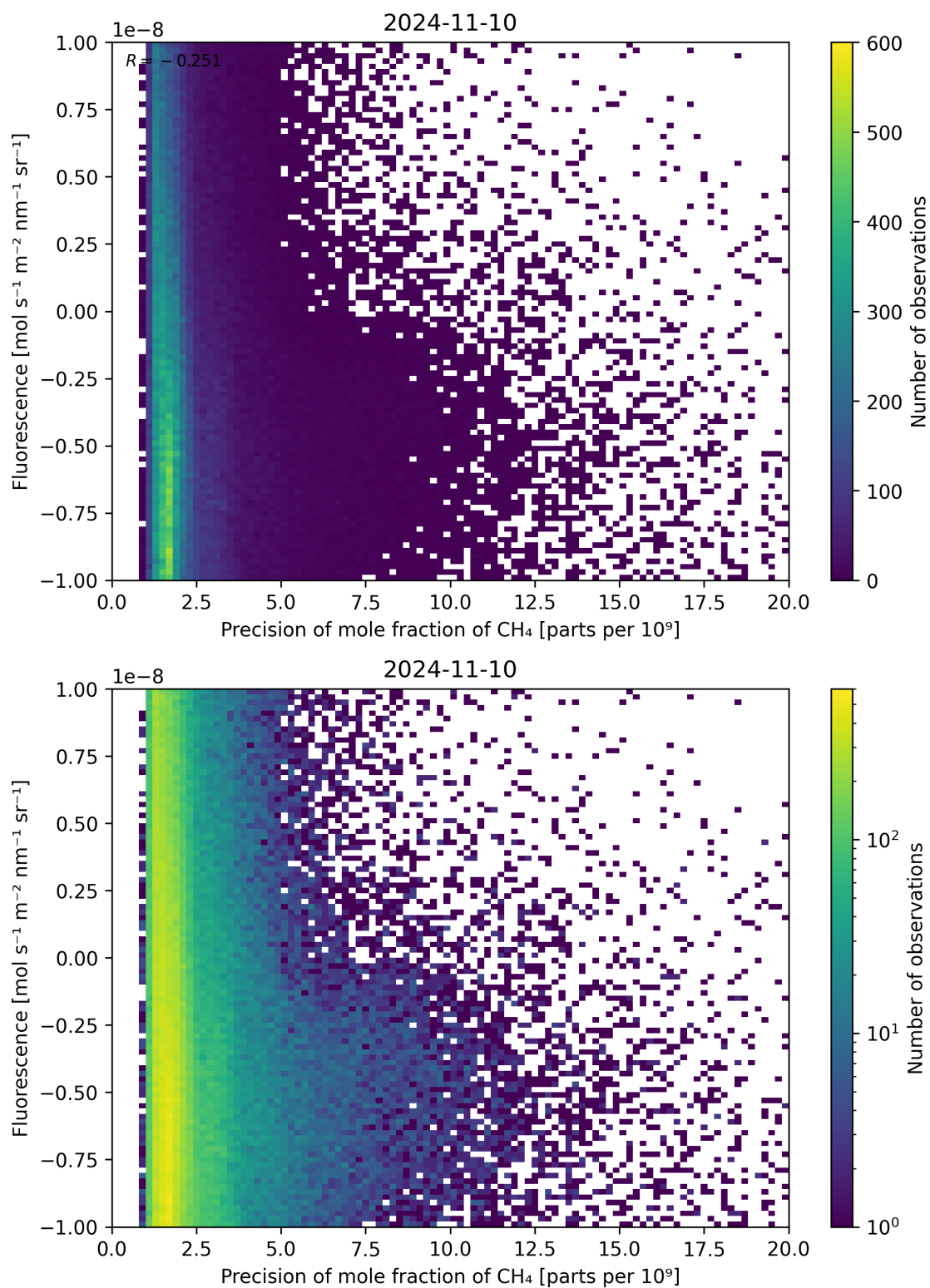
Figure 81: Scatter density plot of “Precision of mole fraction of \text{CH}_4 ” against “Fluorescence” for 2024-11-09 to 2024-11-11.
