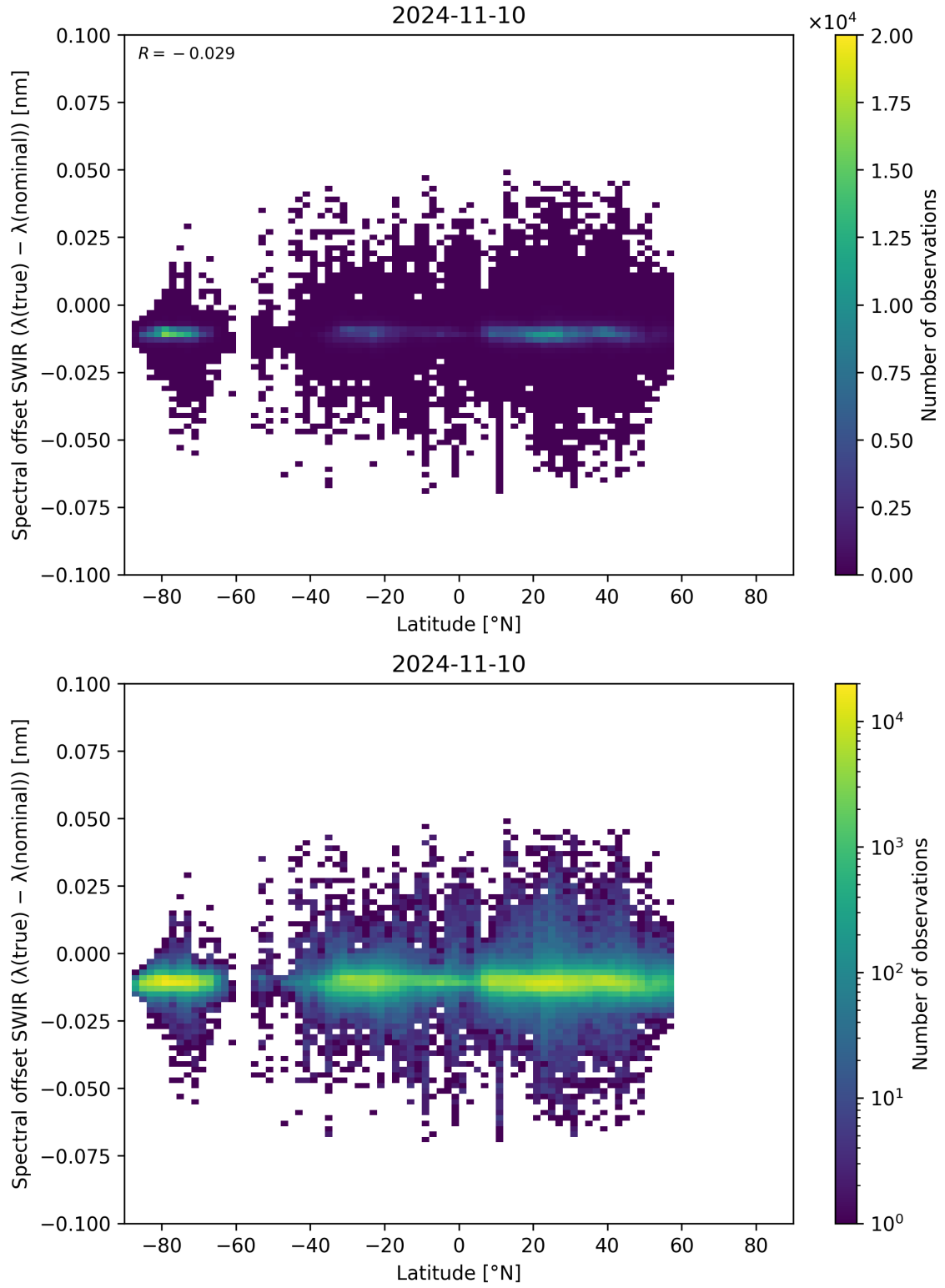
Figure 62: Scatter density plot of “Latitude” against “Spectral offset SWIR ( \lambda_{\text{true}} - \lambda_{\text{nominal}} )” for 2024-11-09 to 2024-11-11.
