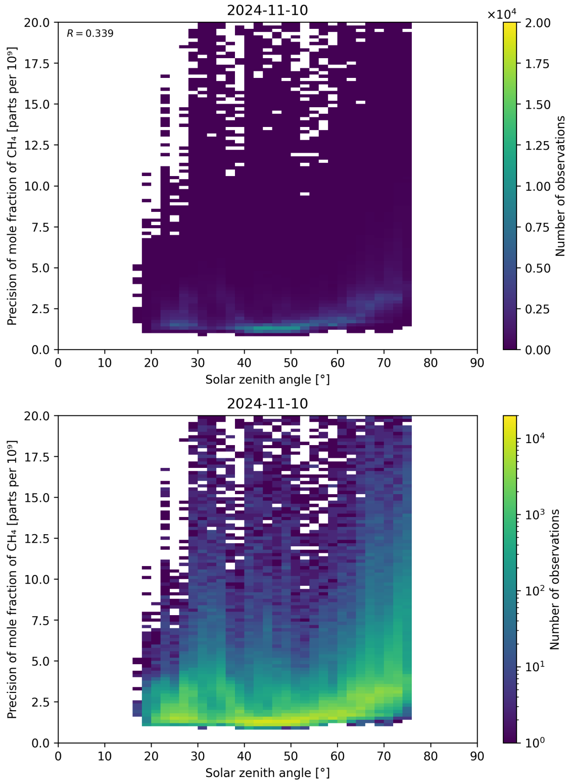
Figure 101: Scatter density plot of “Solar zenith angle” against “Precision of mole fraction of \text{CH}_4 ” for 2024-11-09 to 2024-11-11.
