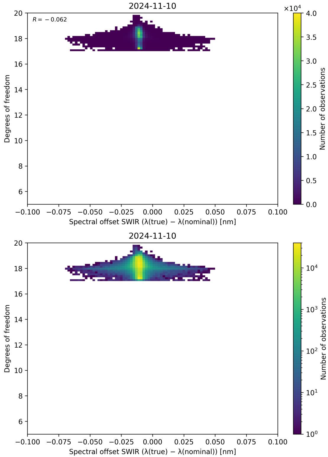
Figure 119: Scatter density plot of “Spectral offset SWIR ( \lambda_{\text{true}} - \lambda_{\text{nominal}} )” against “Degrees of freedom” for 2024-11-09 to 2024-11-11.
