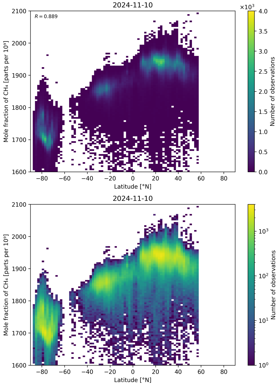
Figure 57: Scatter density plot of “Latitude” against “Mole fraction of CH 4 ” for 2024-11-09 to 2024-11-11.
