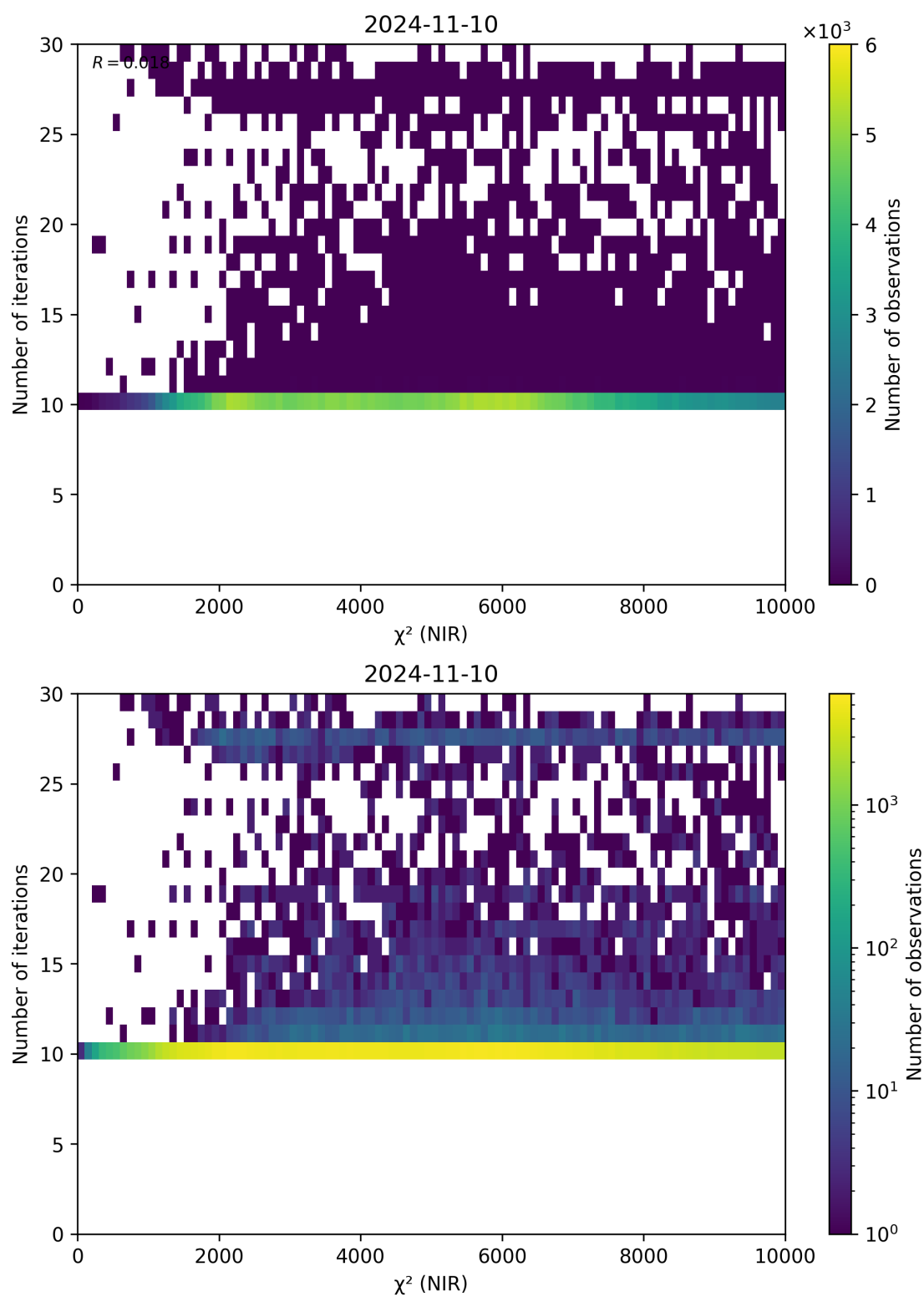
Figure 46: Scatter density plot of “ \chi^2 (NIR)” against “Number of iterations” for 2024-11-09 to 2024-11-11.
