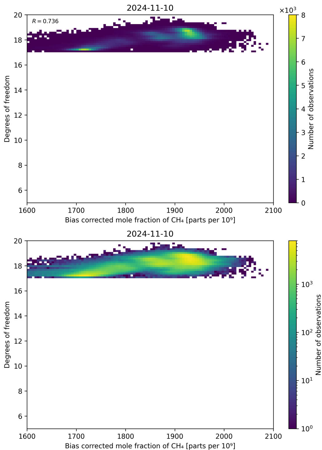
Figure 65: Scatter density plot of “Bias corrected mole fraction of CH 4 ” against “Degrees of freedom” for 2024-11-09 to 2024-11-11.
