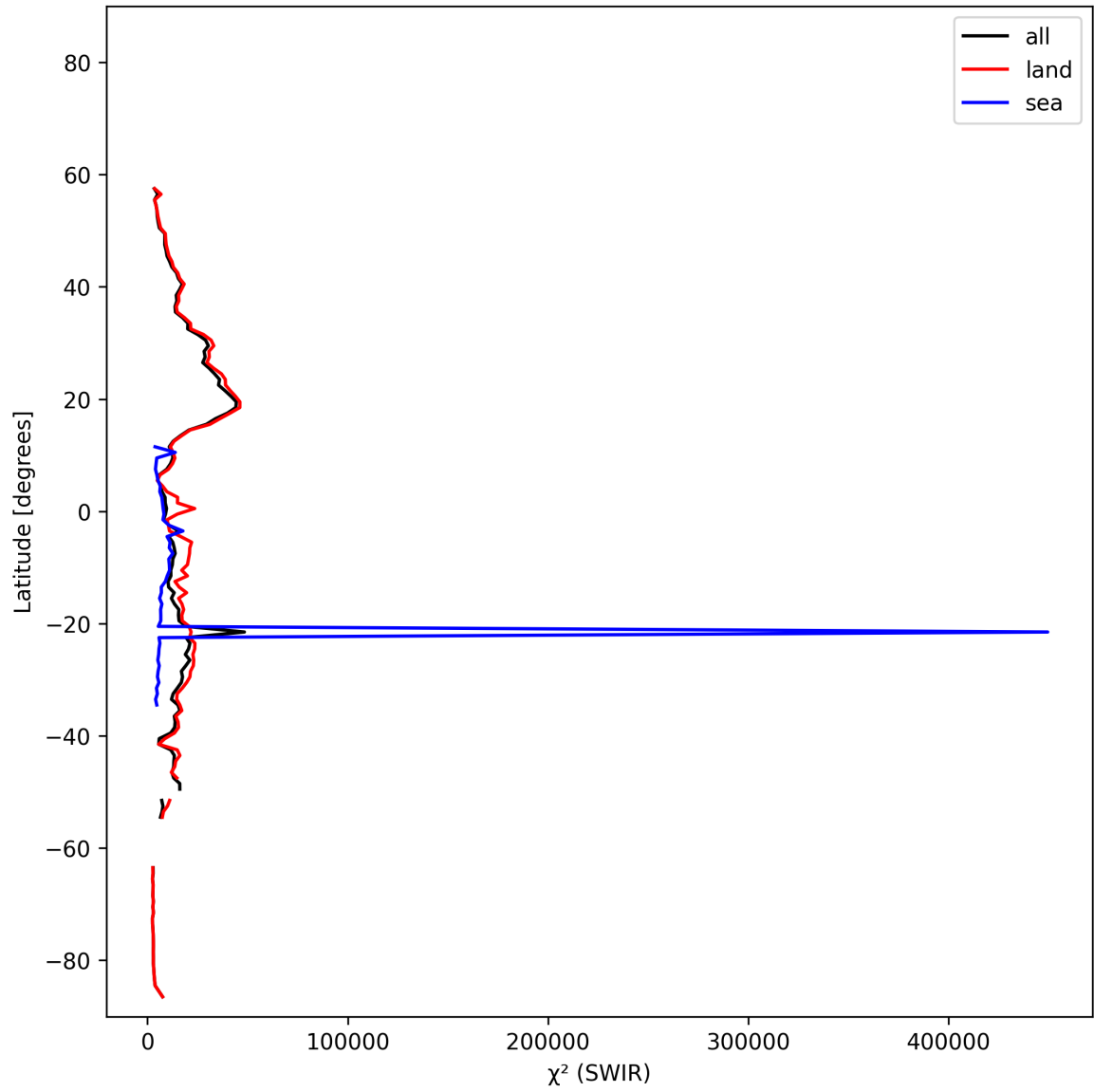
Figure 17: Zonal average of “ \chi^2 (SWIR)” for 2024-11-09 to 2024-11-11.
