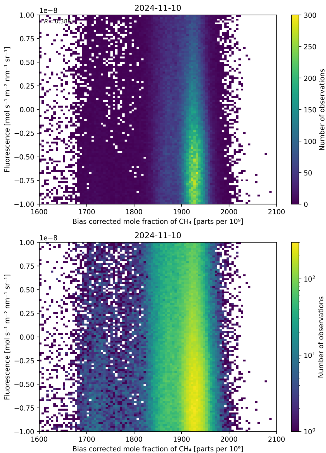
Figure 66: Scatter density plot of “Bias corrected mole fraction of \text{CH}_4 ” against “Fluorescence” for 2024-11-09 to 2024-11-11.
