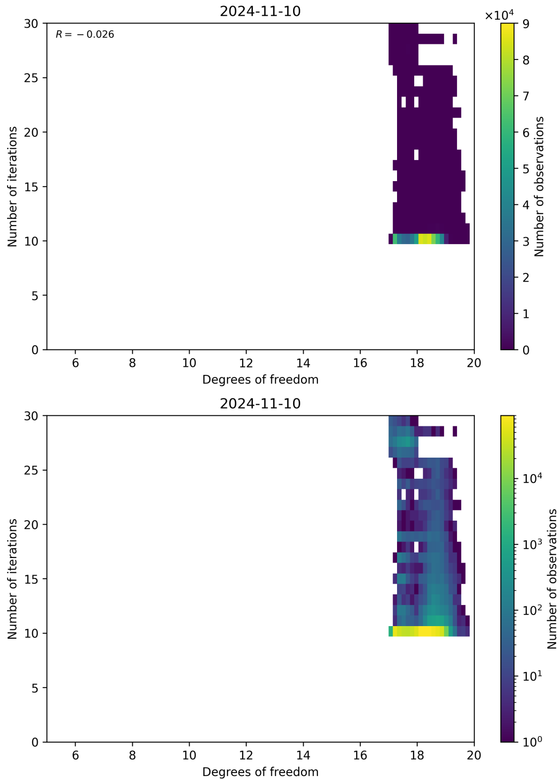
Figure 52: Scatter density plot of “Degrees of freedom” against “Number of iterations” for 2024-11-09 to 2024-11-11.
