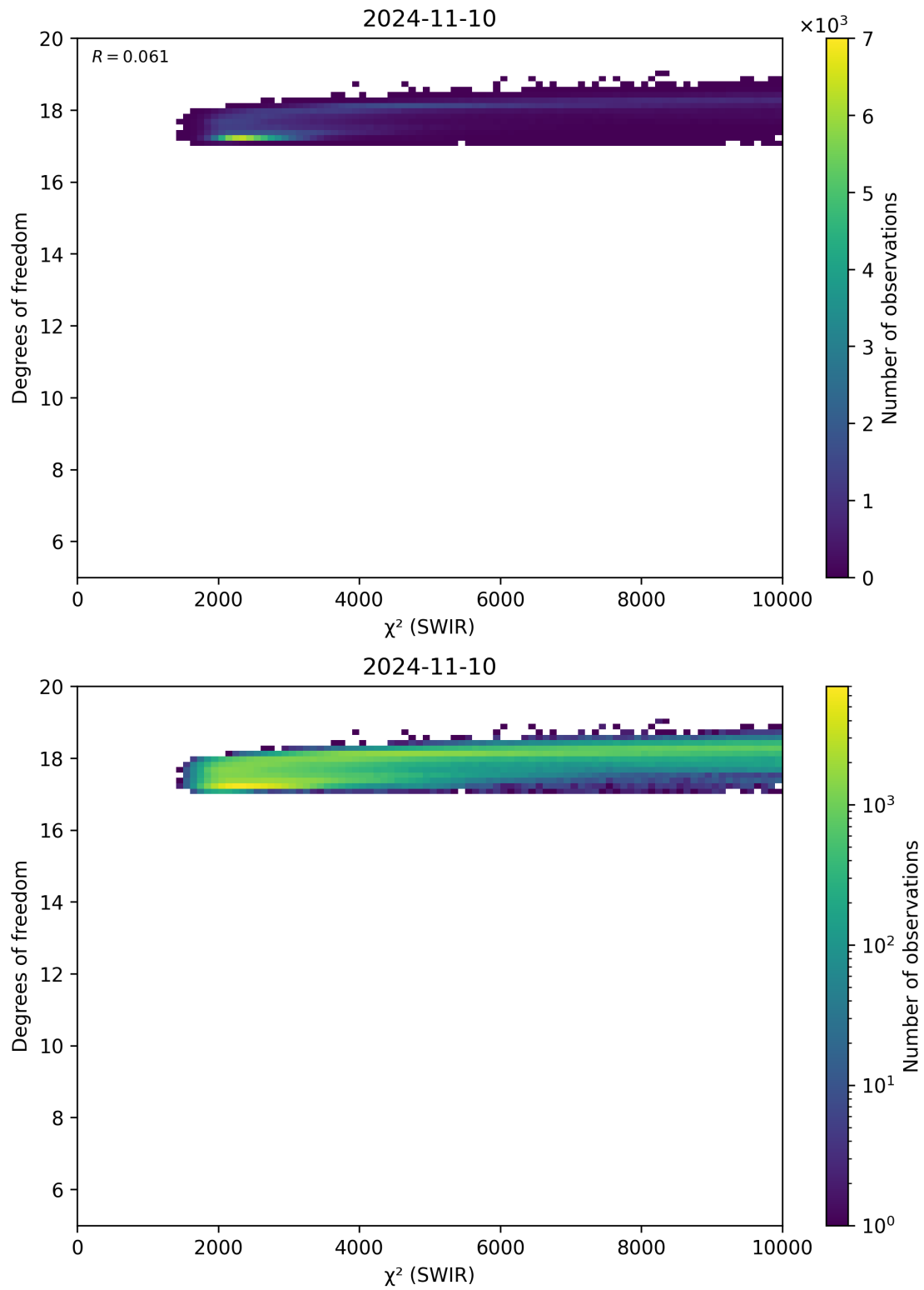
Figure 48: Scatter density plot of “ \chi^2 (SWIR)” against “Degrees of freedom” for 2024-11-09 to 2024-11-11.
