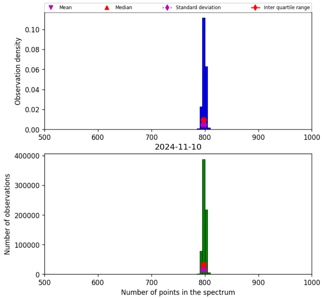
Figure 26: Histogram of “Number of points in the spectrum” for 2024-11-09 to 2024-11-11
