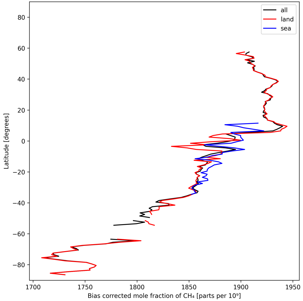
Figure 14: Zonal average of “Bias corrected mole fraction of CH 4 ” for 2024-11-09 to 2024-11-11.
