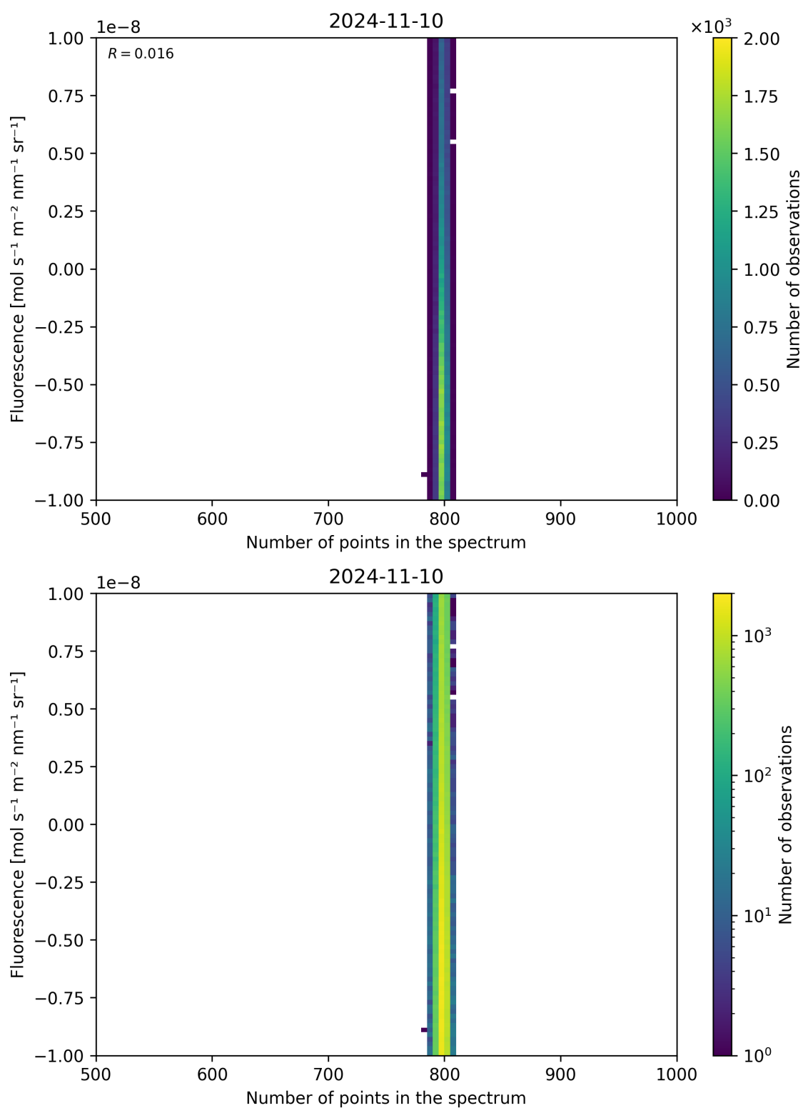
Figure 91: Scatter density plot of “Number of points in the spectrum” against “Fluorescence” for 2024-11-09 to 2024-11-11.
