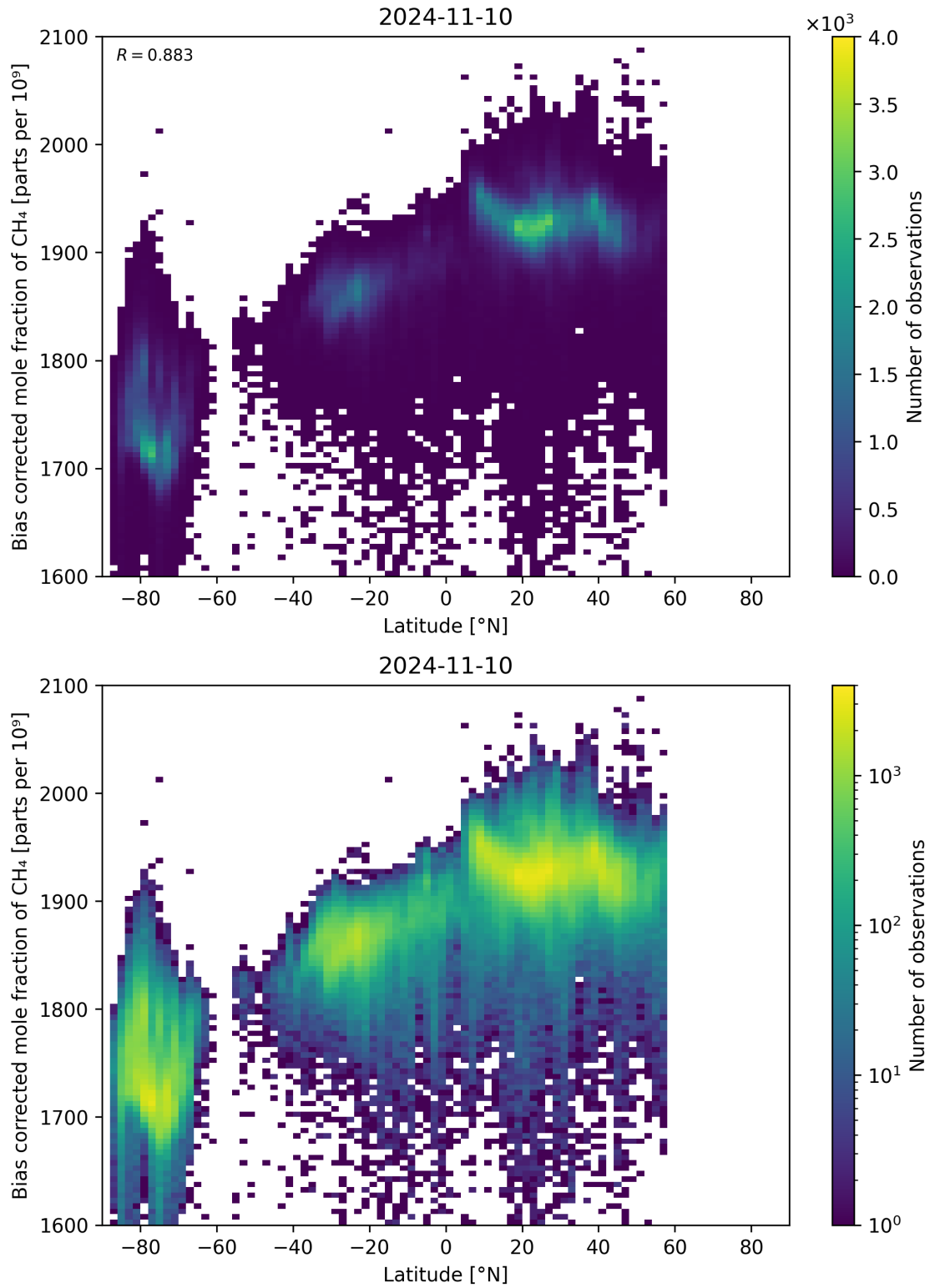
Figure 58: Scatter density plot of “Latitude” against “Bias corrected mole fraction of CH 4 ” for 2024-11-09 to 2024-11-11.
