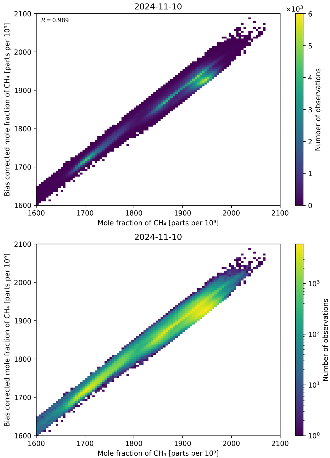
Figure 74: Scatter density plot of “Mole fraction of CH 4 ” against “Bias corrected mole fraction of CH 4 ” for 2024-11-09 to 2024-11-11.
