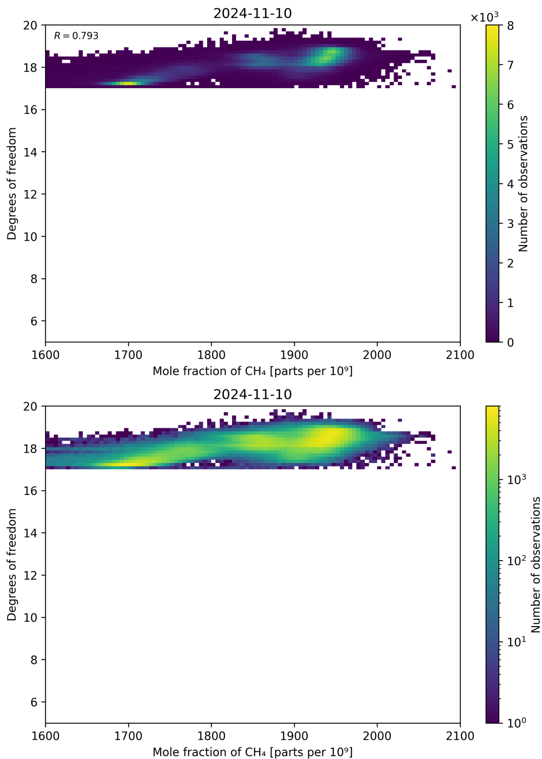
Figure 72: Scatter density plot of “Mole fraction of CH 4 ” against “Degrees of freedom” for 2024-11-09 to 2024-11-11.
