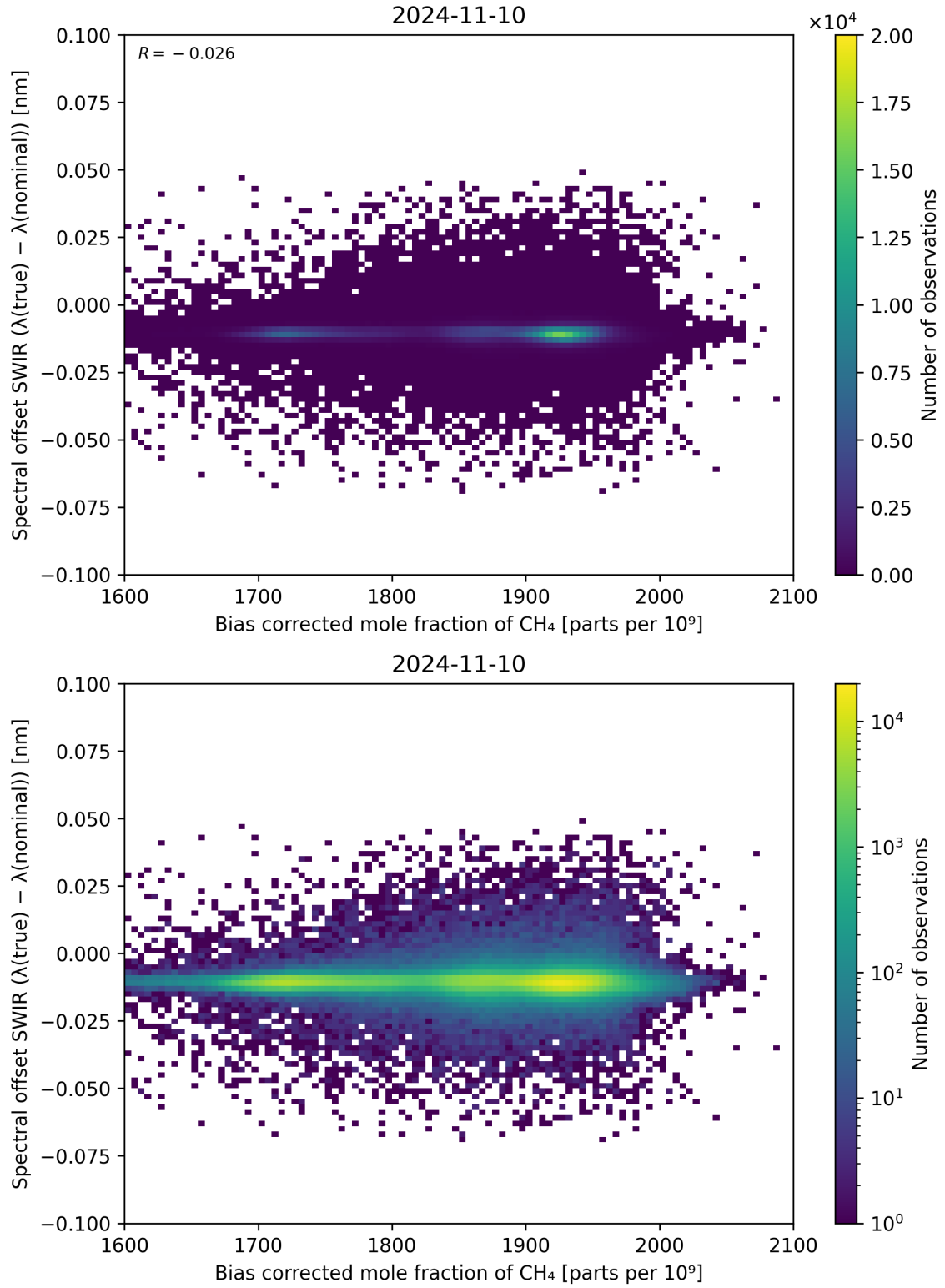
Figure 69: Scatter density plot of “Bias corrected mole fraction of \text{CH}_4 ” against “Spectral offset SWIR ( \lambda_{\text{true}} - \lambda_{\text{nominal}} )” for 2024-11-09 to 2024-11-11.
