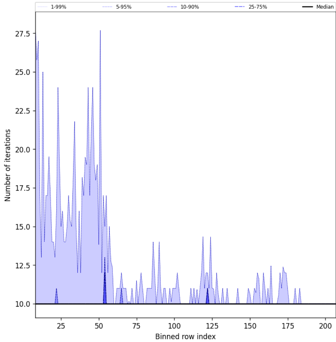
Figure 42: Along track statistics of “Number of iterations” for 2024-11-09 to 2024-11-11
