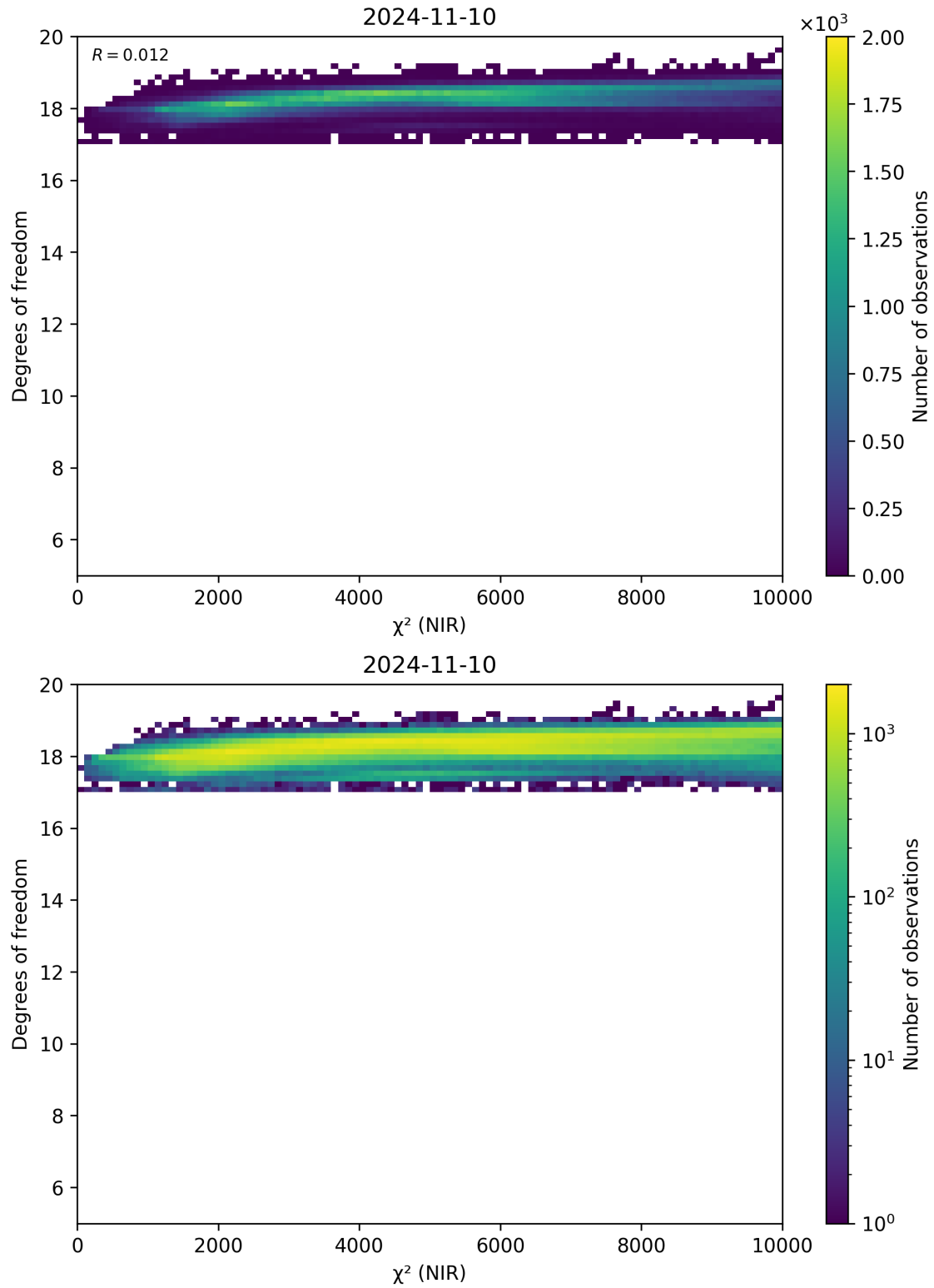
Figure 44: Scatter density plot of “ \chi^2 (NIR)” against “Degrees of freedom” for 2024-11-09 to 2024-11-11.
