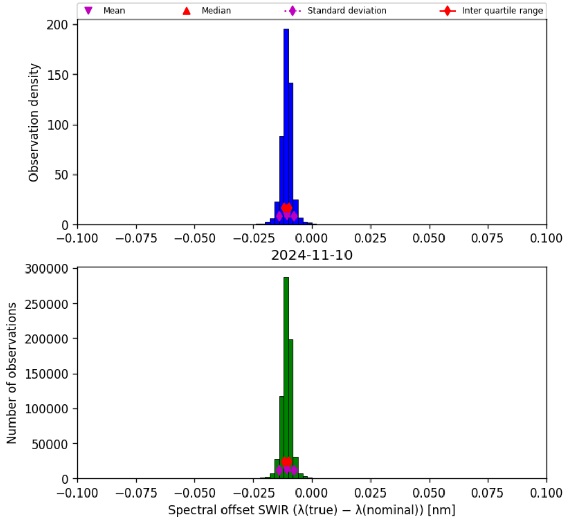
Figure 27: Histogram of “Spectral offset SWIR ( \lambda_{\text{true}} - \lambda_{\text{nominal}} )” for 2024-11-09 to 2024-11-11
