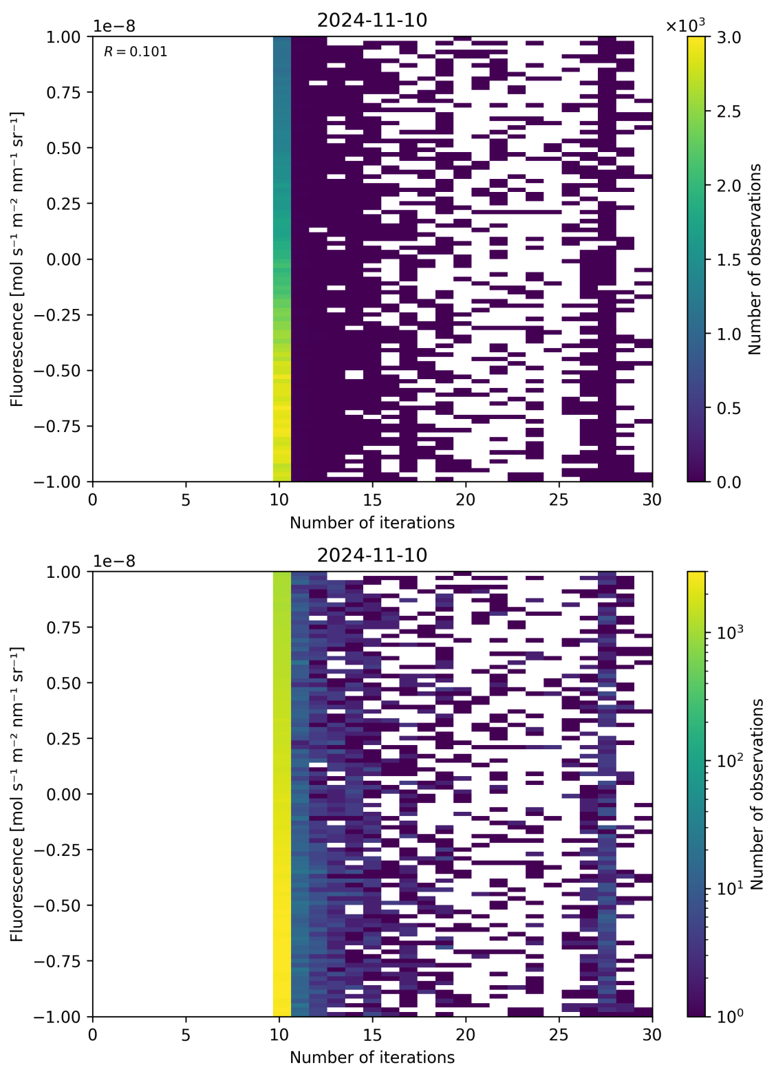
Figure 87: Scatter density plot of “Number of iterations” against “Fluorescence” for 2024-11-09 to 2024-11-11.
