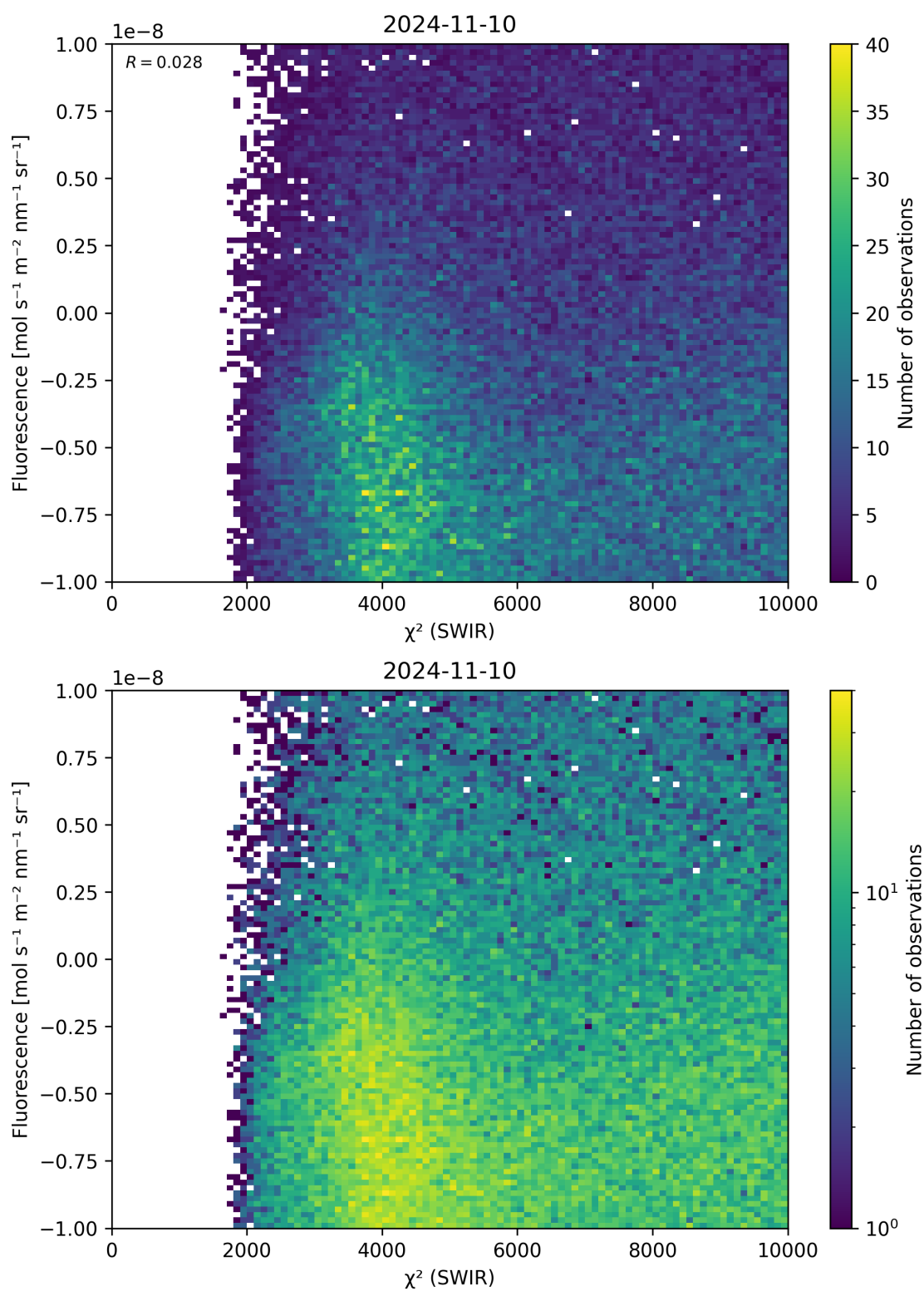
Figure 49: Scatter density plot of “ \chi^2 (SWIR)” against “Fluorescence” for 2024-11-09 to 2024-11-11.
