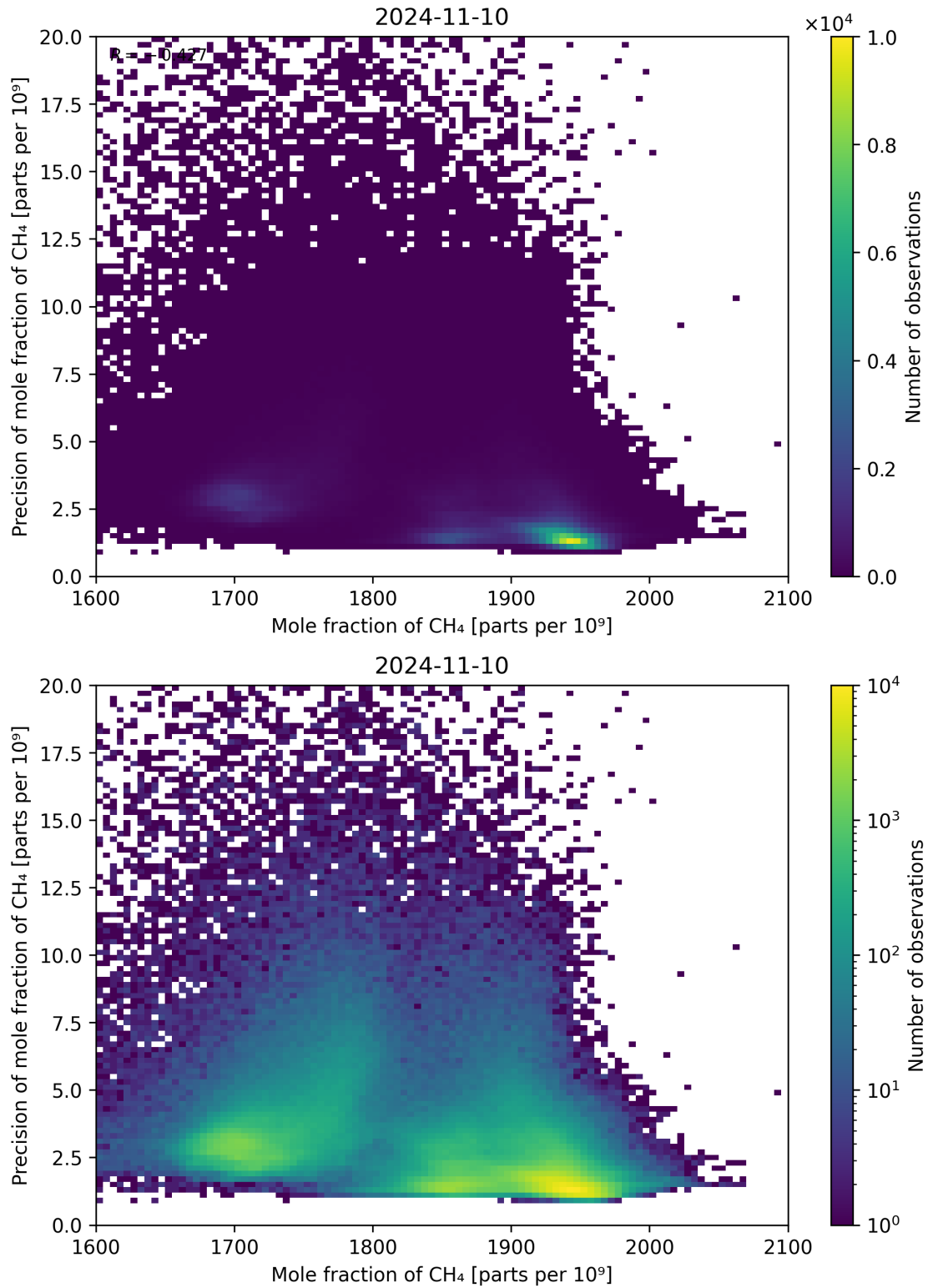
Figure 75: Scatter density plot of “Mole fraction of CH 4 ” against “Precision of mole fraction of CH 4 ” for 2024-11-09 to 2024-11-11.
