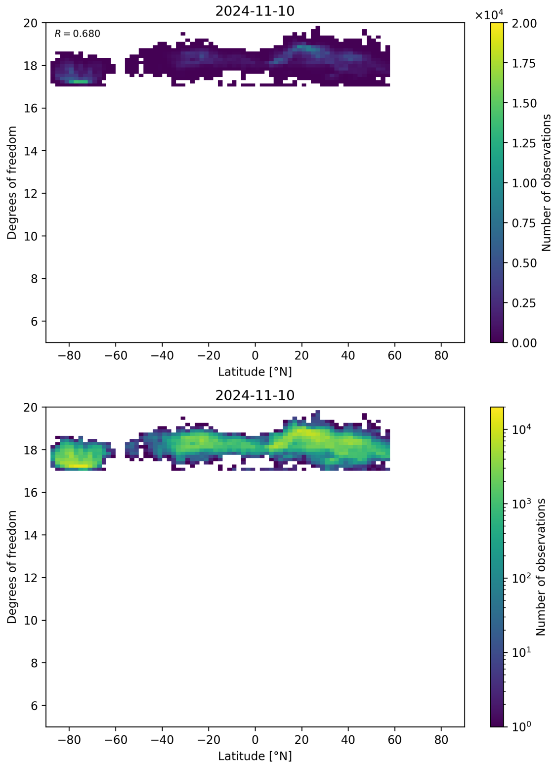
Figure 55: Scatter density plot of “Latitude” against “Degrees of freedom” for 2024-11-09 to 2024-11-11.
