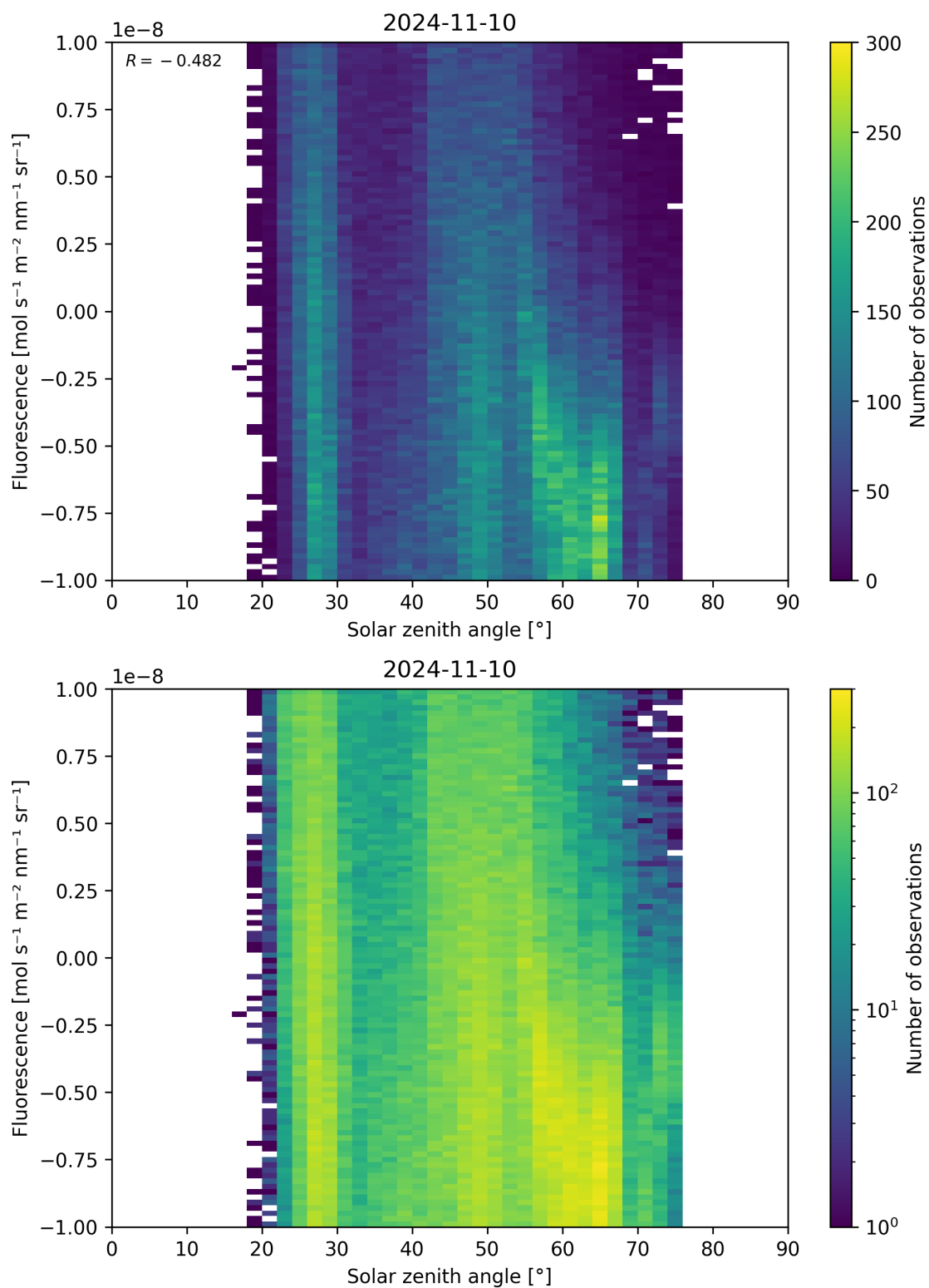
Figure 97: Scatter density plot of “Solar zenith angle” against “Fluorescence” for 2024-11-09 to 2024-11-11.
