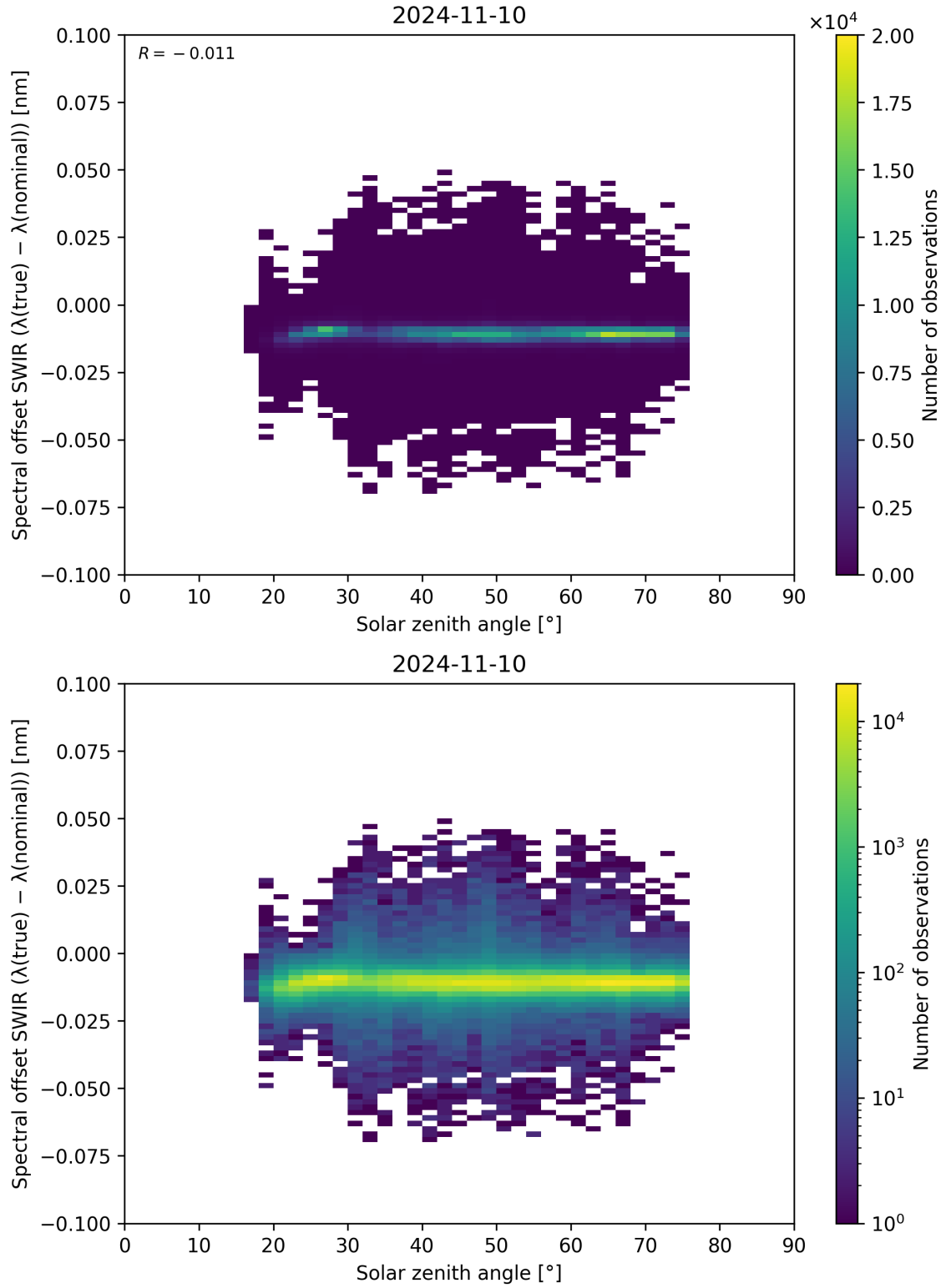
Figure 104: Scatter density plot of “Solar zenith angle” against “Spectral offset SWIR ( \lambda_{\text{true}} - \lambda_{\text{nominal}} )” for 2024-11-09 to 2024-11-11.
