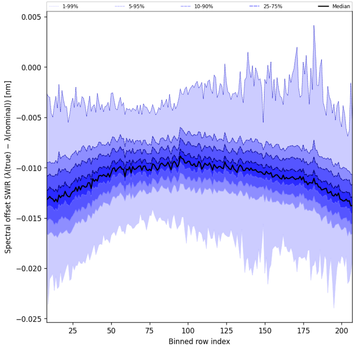
Figure 38: Along track statistics of “Spectral offset SWIR ( \lambda_{\text{true}} - \lambda_{\text{nominal}} )” for 2024-11-09 to 2024-11-11
