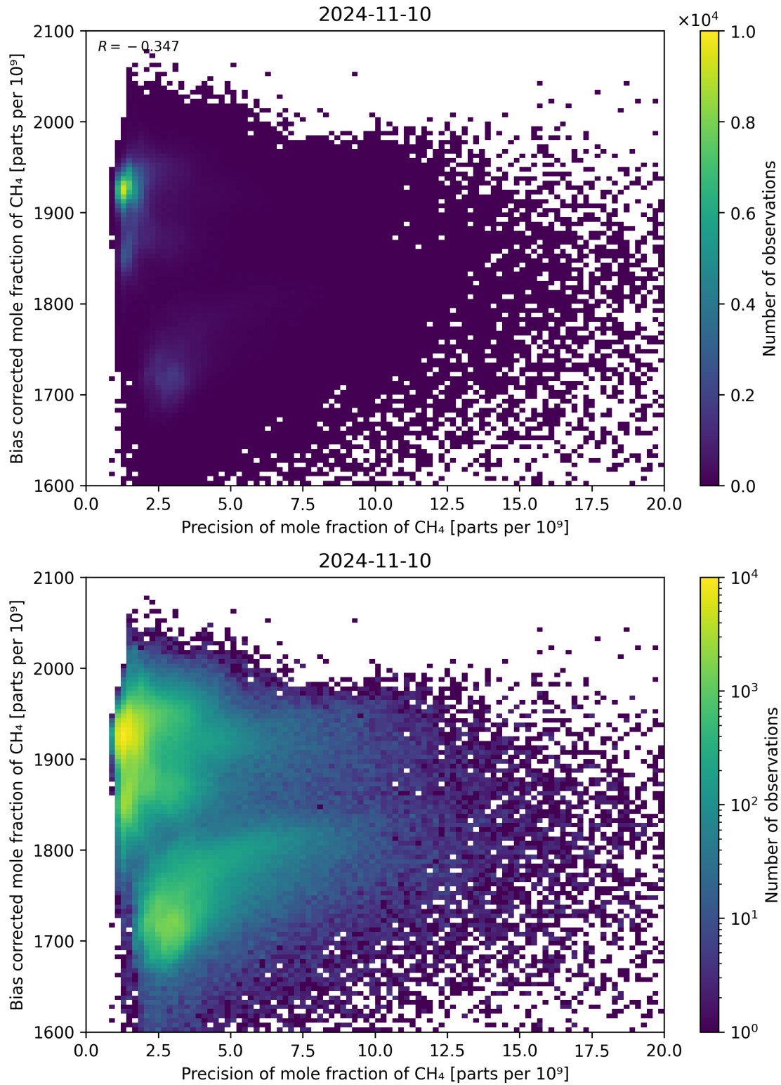
Figure 82: Scatter density plot of “Precision of mole fraction of CH 4 ” against “Bias corrected mole fraction of CH 4 ” for 2024-11-09 to 2024-11-11.
