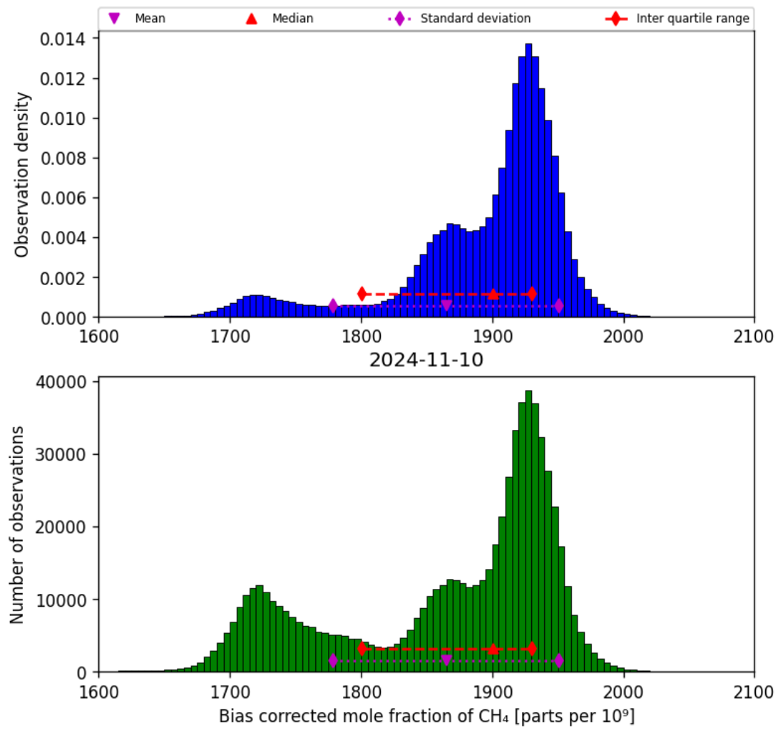
Figure 25: Histogram of “Bias corrected mole fraction of CH 4 ” for 2024-11-09 to 2024-11-11
