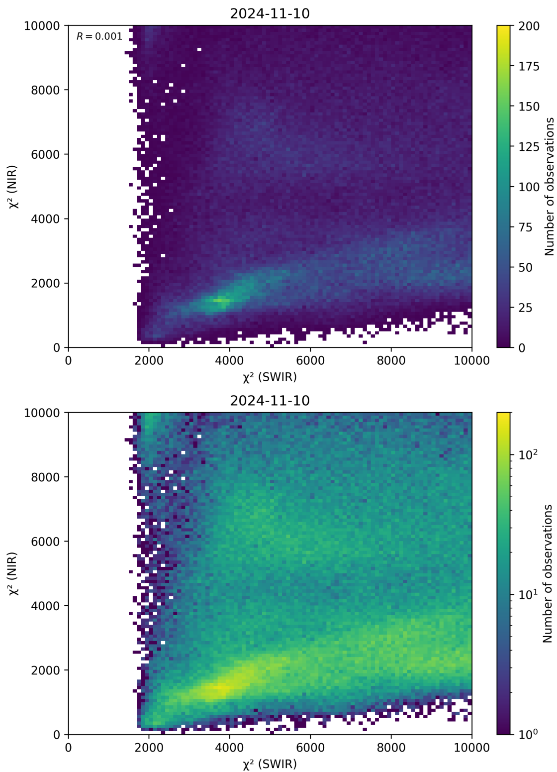
Figure 47: Scatter density plot of " \chi^2 (SWIR)" against " \chi^2 (NIR)" for 2024-11-09 to 2024-11-11.
