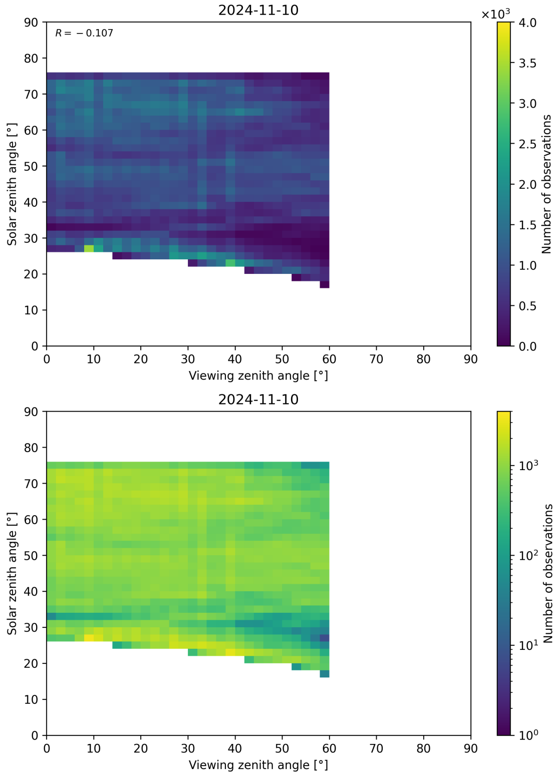
Figure 115: Scatter density plot of “Viewing zenith angle” against “Solar zenith angle” for 2024-11-09 to 2024-11-11.
