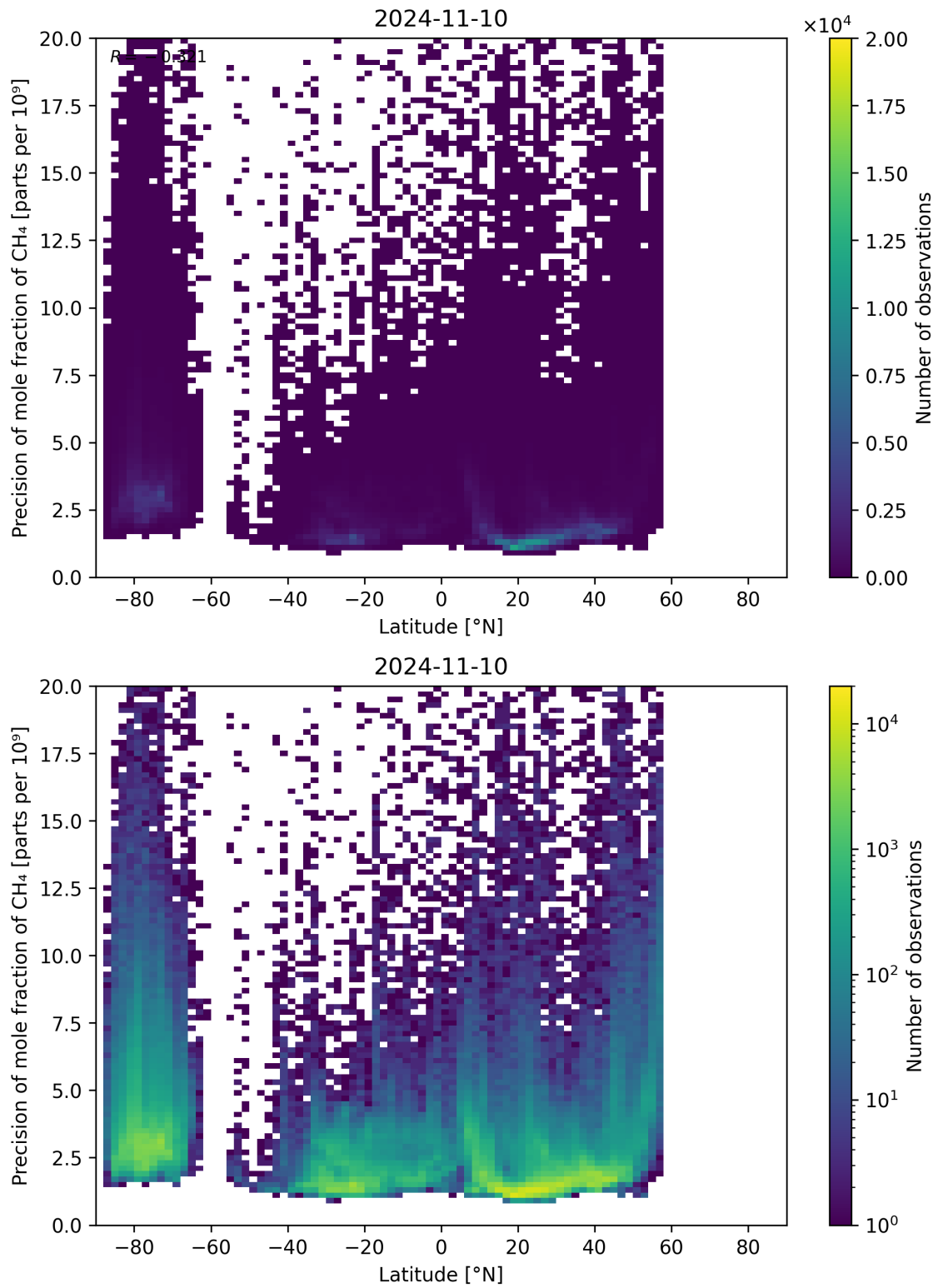
Figure 59: Scatter density plot of “Latitude” against “Precision of mole fraction of CH 4 ” for 2024-11-09 to 2024-11-11.
