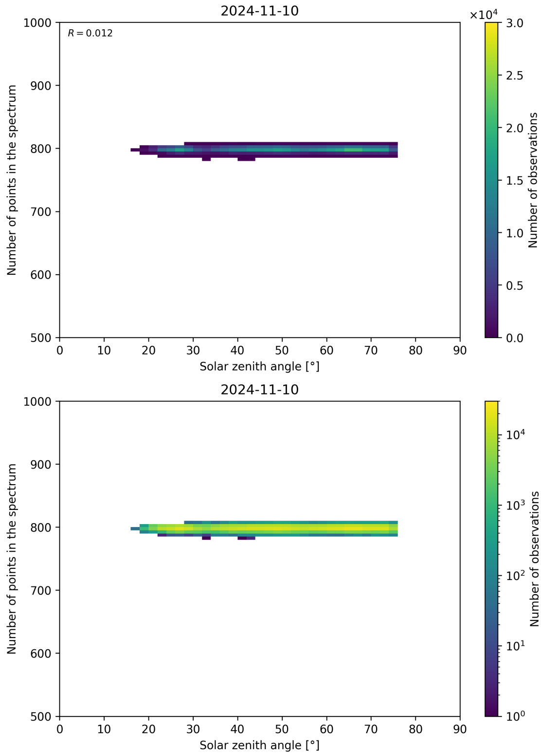
Figure 103: Scatter density plot of “Solar zenith angle” against “Number of points in the spectrum” for 2024-11-09 to 2024-11-11.
