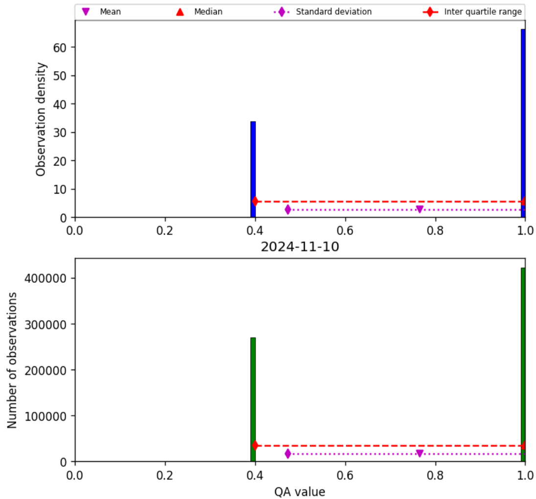
Figure 22: Histogram of “QA value” for 2024-11-09 to 2024-11-11
