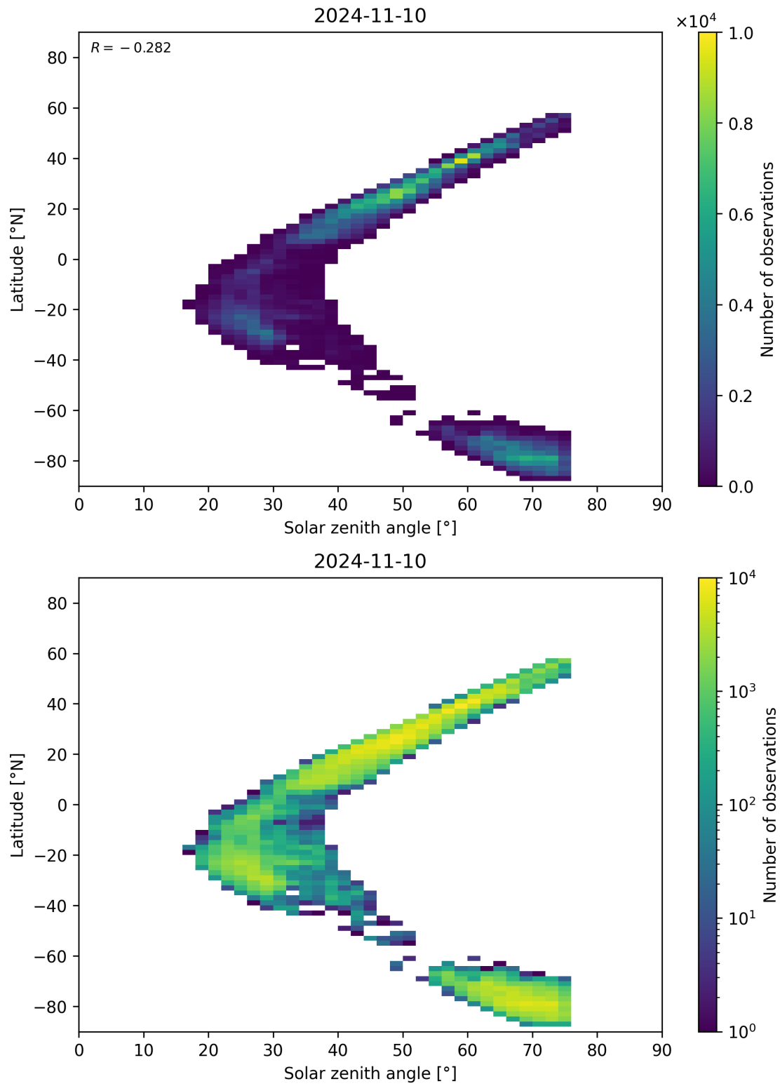
Figure 98: Scatter density plot of “Solar zenith angle” against “Latitude” for 2024-11-09 to 2024-11-11.
