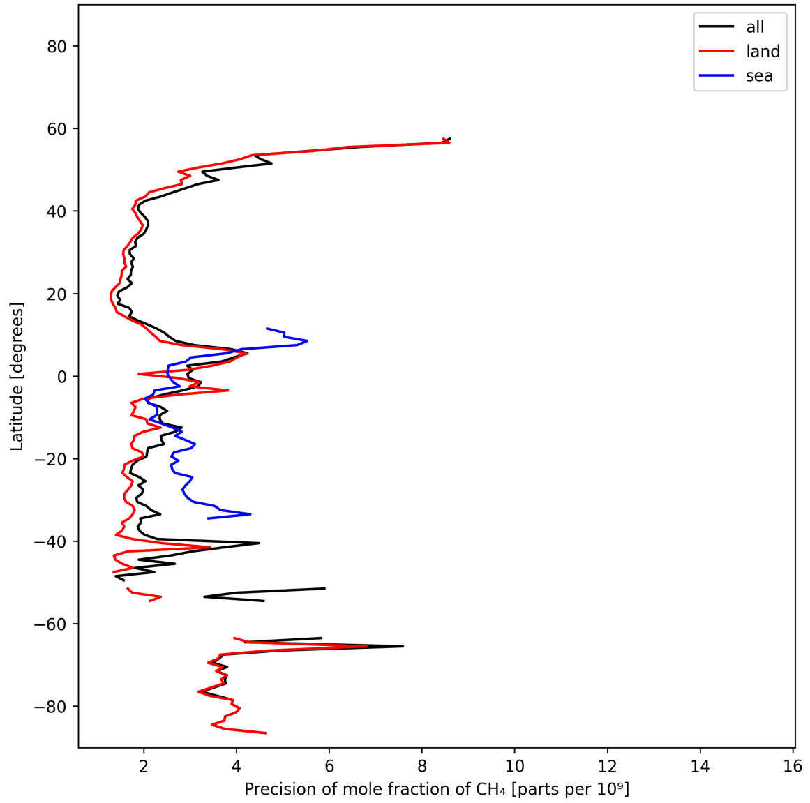
Figure 13: Zonal average of “Precision of mole fraction of CH 4 ” for 2024-11-09 to 2024-11-11.
