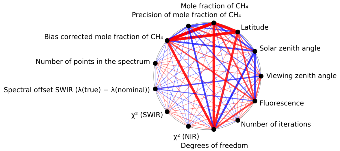
Figure 1: Map of correlation graph for 2024-11-09 to 2024-11-11.
