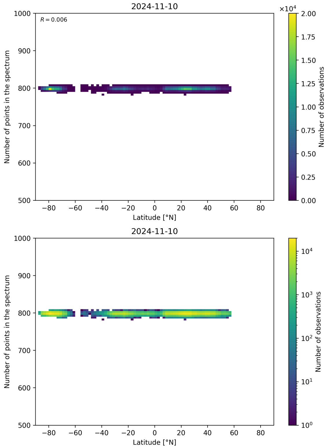
Figure 61: Scatter density plot of “Latitude” against “Number of points in the spectrum” for 2024-11-09 to 2024-11-11.
