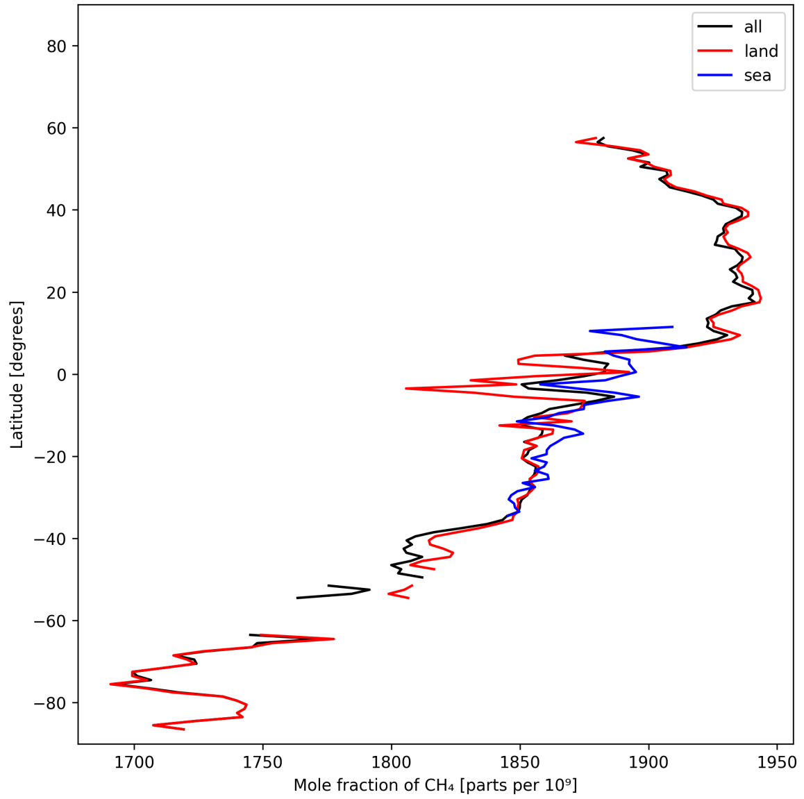
Figure 12: Zonal average of “Mole fraction of \text{CH}_4 ” for 2024-11-09 to 2024-11-11.
