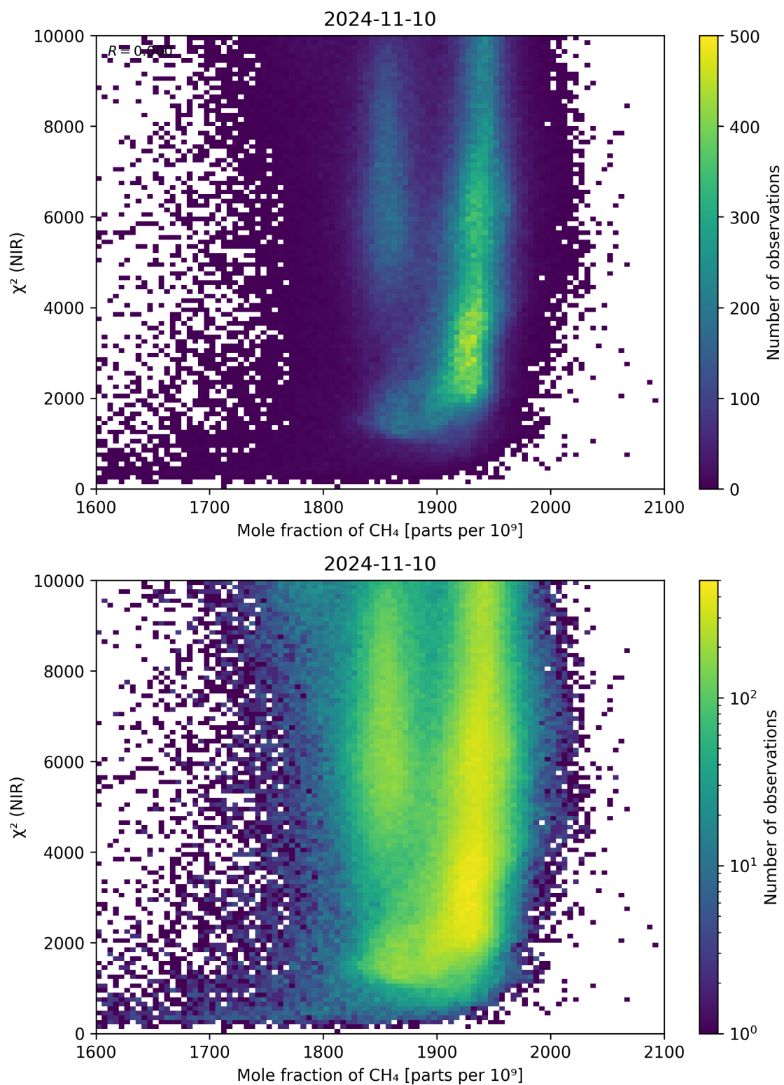
Figure 70: Scatter density plot of “Mole fraction of CH 4 ” against “ \chi^2 (NIR)” for 2024-11-09 to 2024-11-11.
