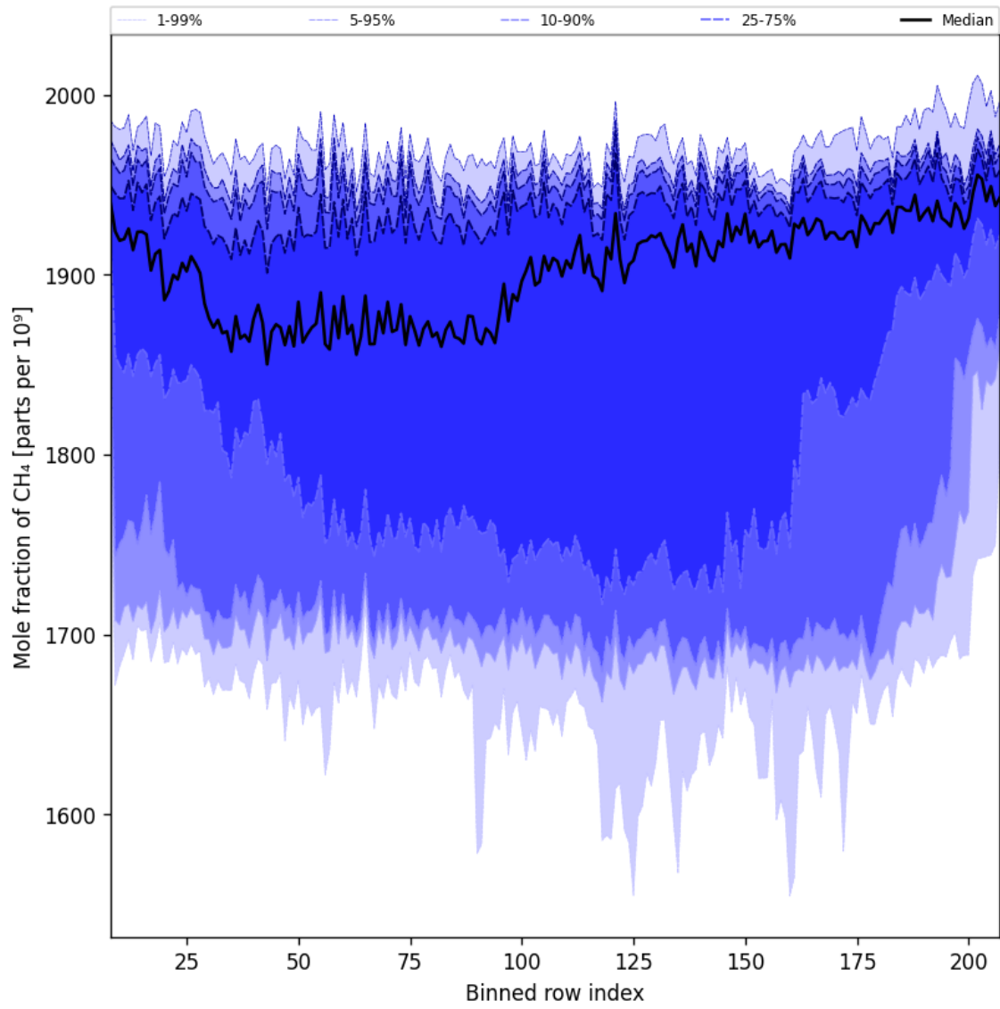
Figure 34: Along track statistics of “Mole fraction of CH 4 ” for 2024-11-09 to 2024-11-11
