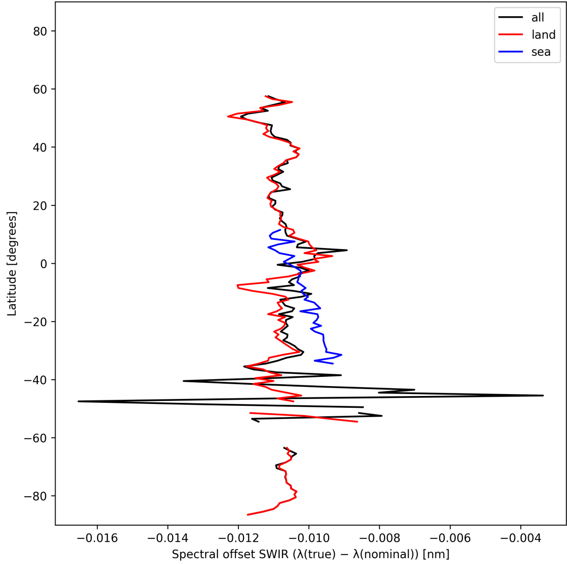
Figure 16: Zonal average of “Spectral offset SWIR ( \lambda_{\text{true}} - \lambda_{\text{nominal}} )” for 2024-11-09 to 2024-11-11.
