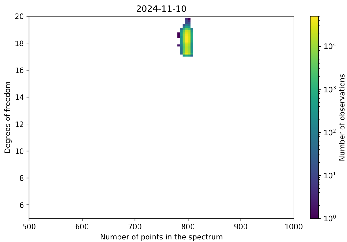
Figure 90: Scatter density plot of “Number of points in the spectrum” against “Degrees of freedom” for 2024-11-09 to 2024-11-11.
