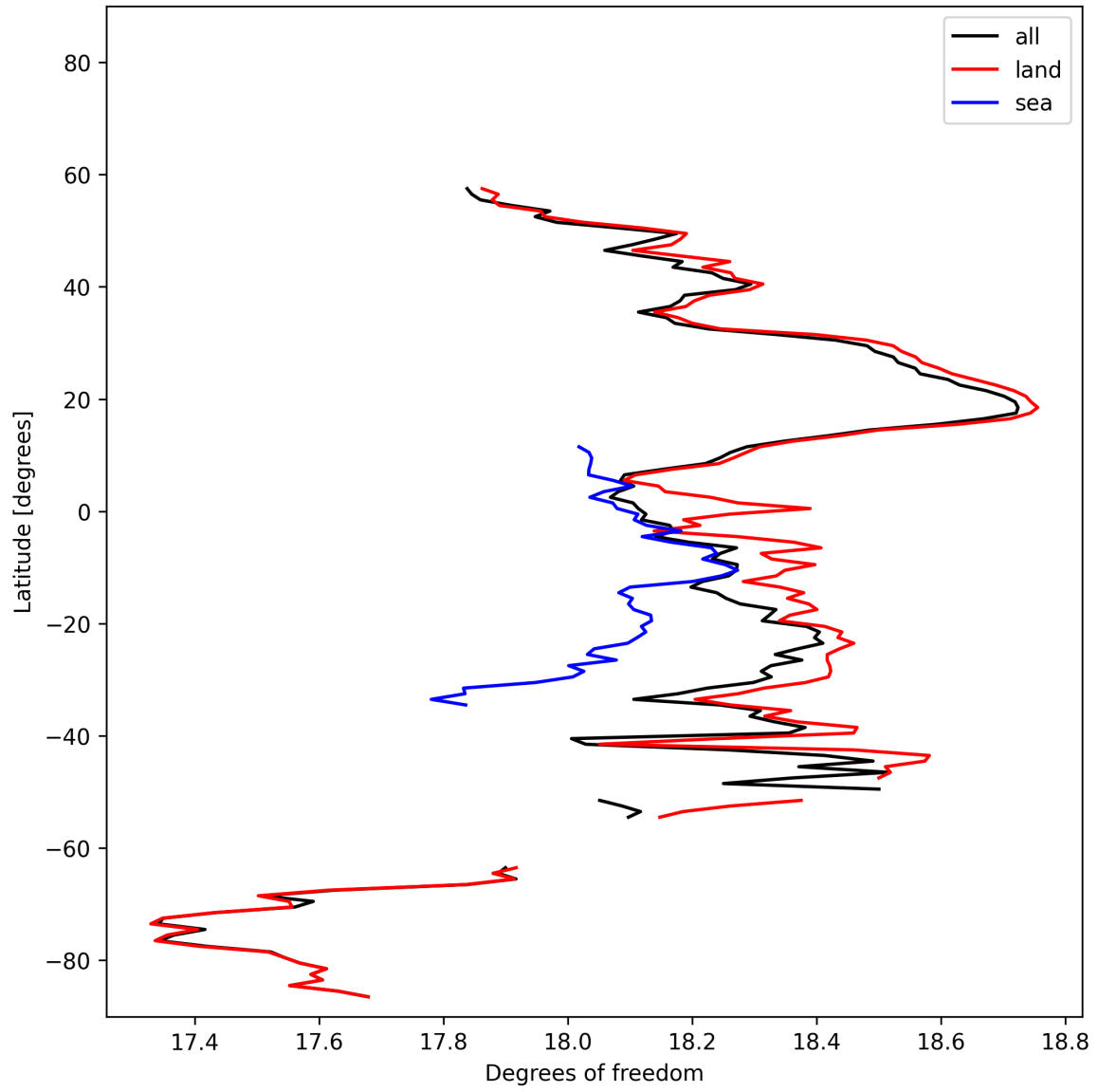
Figure 19: Zonal average of “Degrees of freedom” for 2024-11-09 to 2024-11-11.
