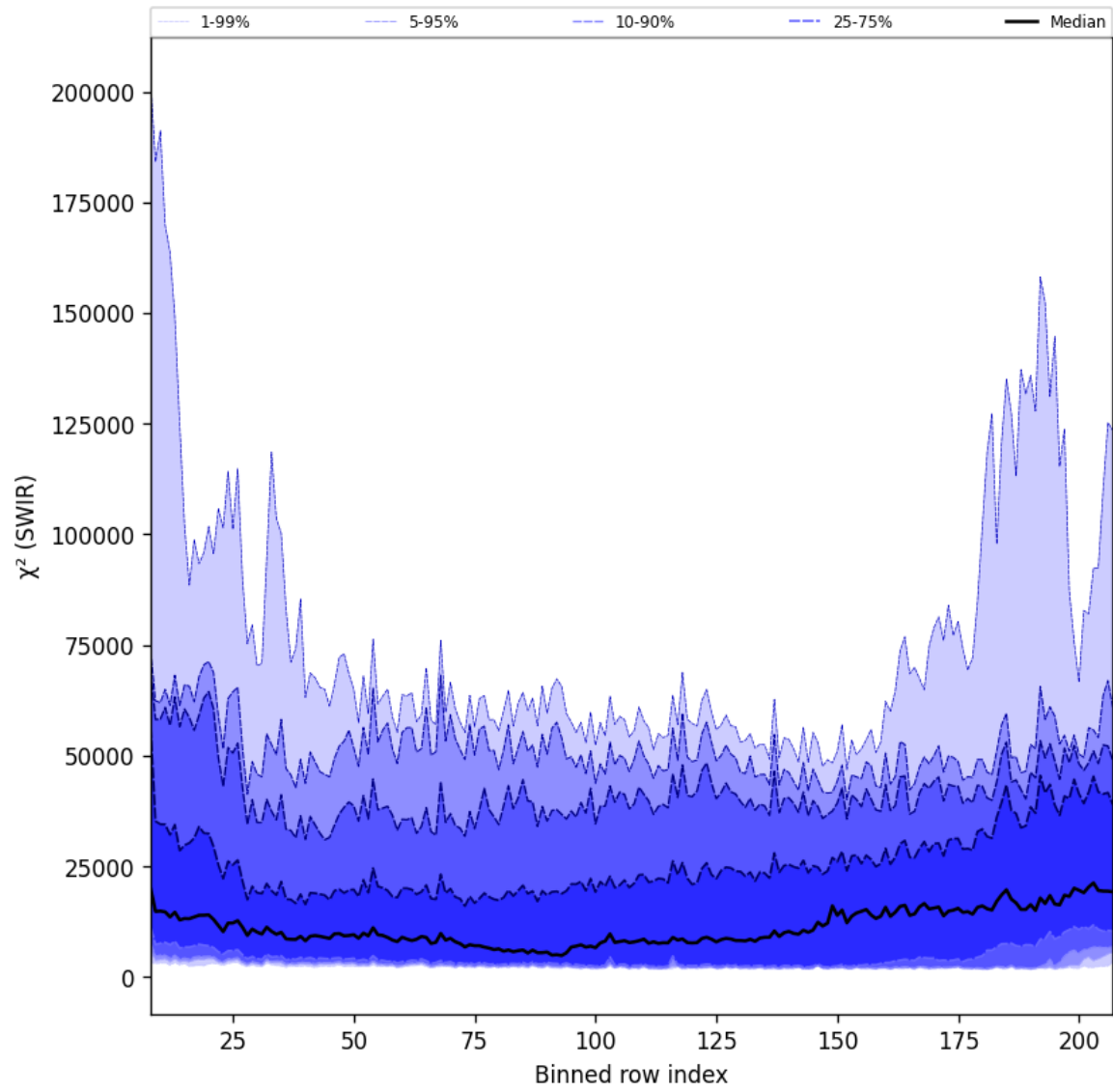
Figure 39: Along track statistics of " \chi^2 (SWIR)" for 2024-11-09 to 2024-11-11
