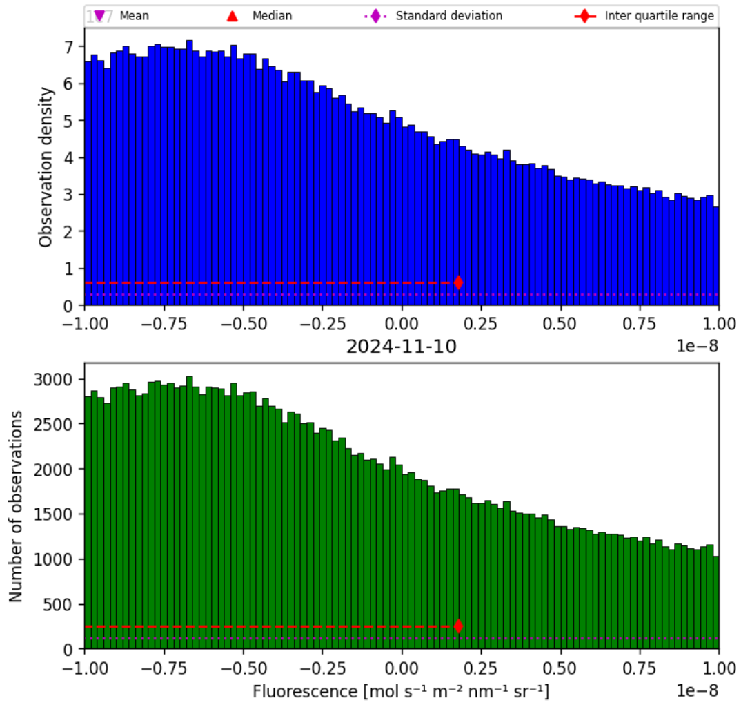
Figure 32: Histogram of “Fluorescence” for 2024-11-09 to 2024-11-11
