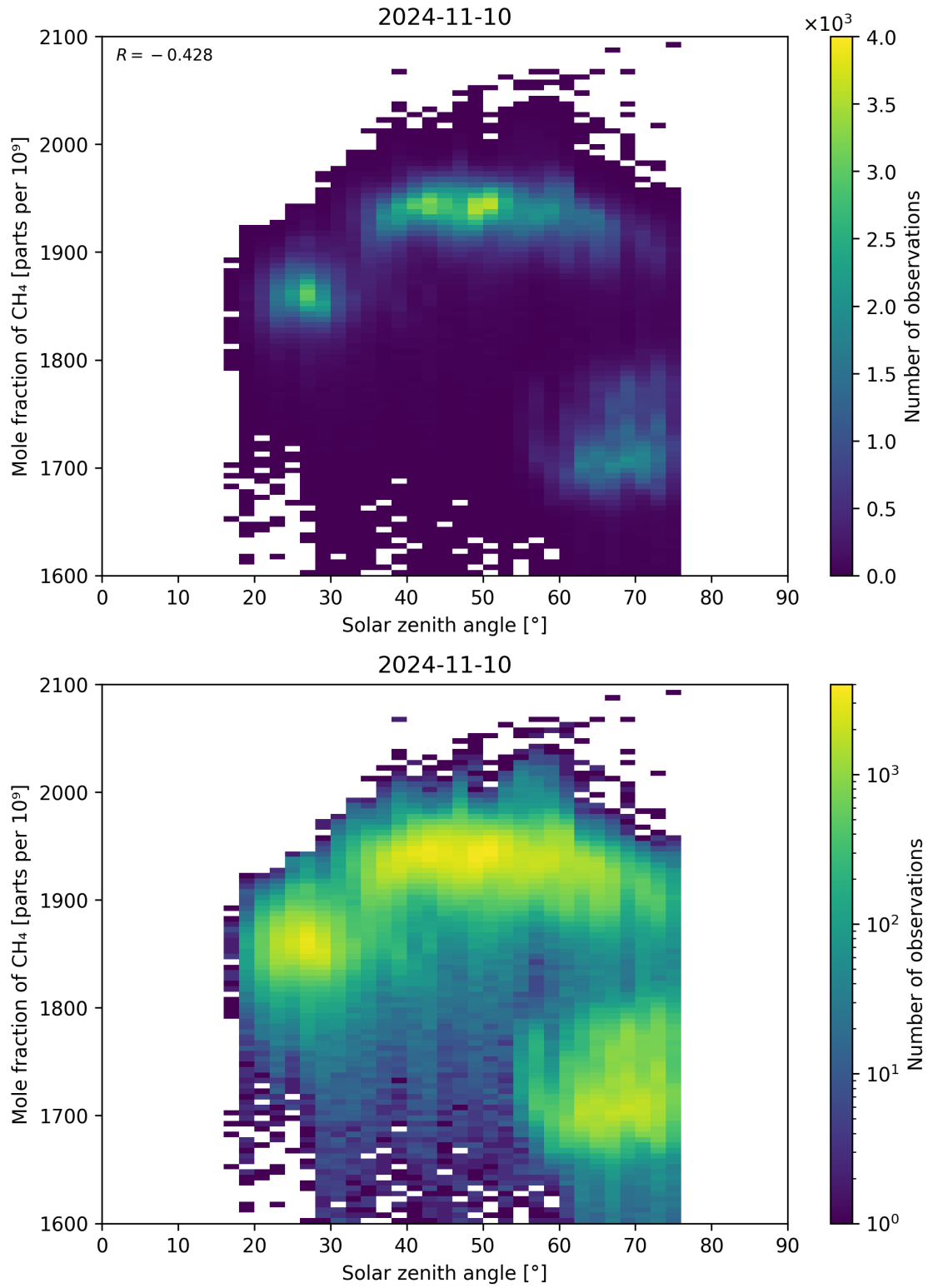
Figure 99: Scatter density plot of “Solar zenith angle” against “Mole fraction of CH 4 ” for 2024-11-09 to 2024-11-11.
