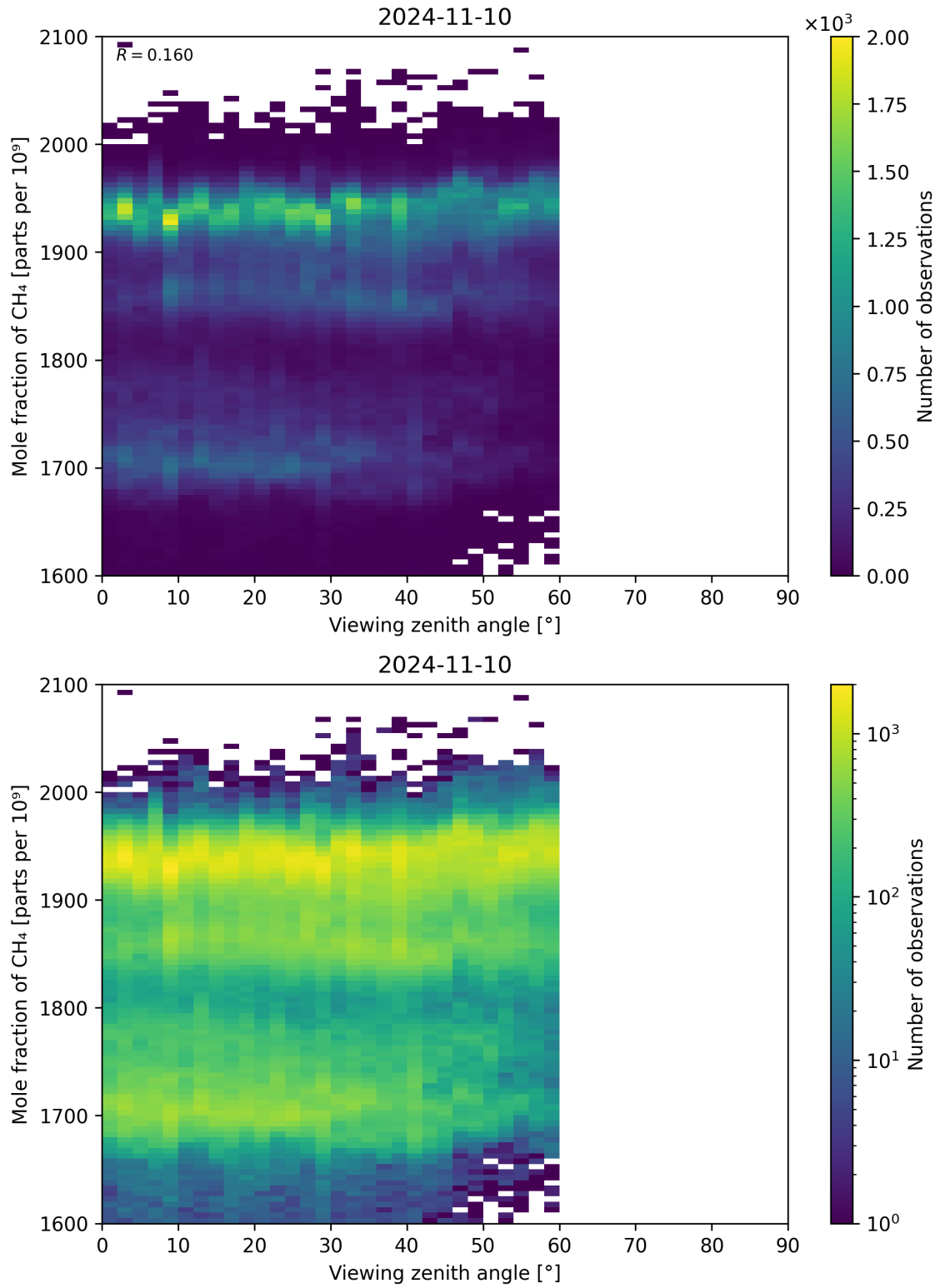
Figure 110: Scatter density plot of “Viewing zenith angle” against “Mole fraction of CH 4 ” for 2024-11-09 to 2024-11-11.
