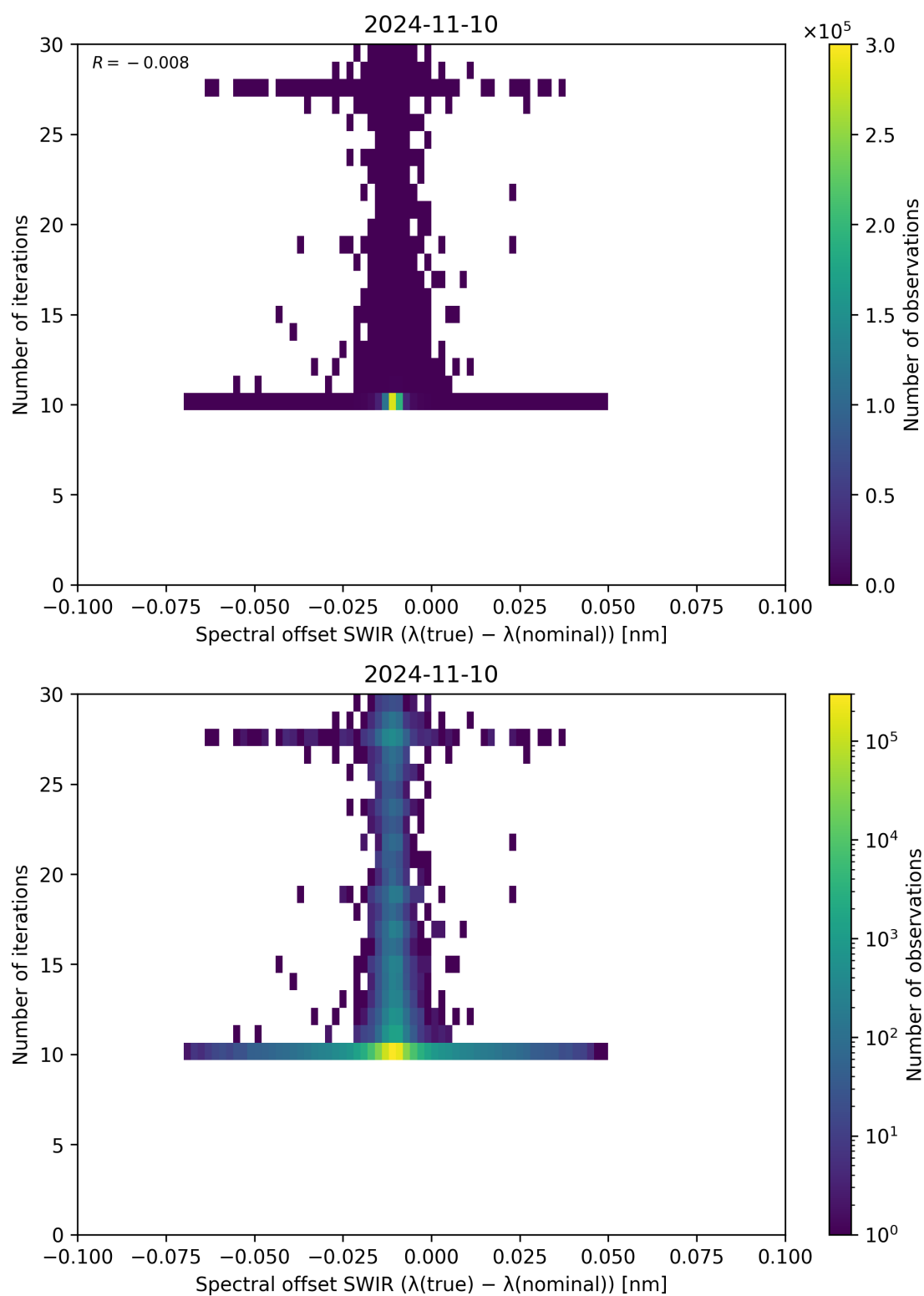
Figure 121: Scatter density plot of “Spectral offset SWIR ( \lambda_{\text{true}} - \lambda_{\text{nominal}} )” against “Number of iterations” for 2024-11-09 to 2024-11-11.
