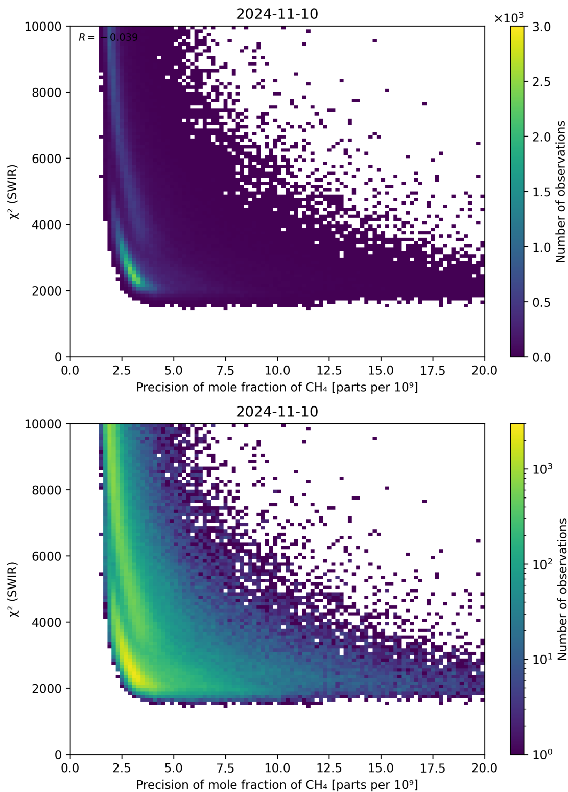
Figure 79: Scatter density plot of “Precision of mole fraction of \text{CH}_4 ” against “ \chi^2 (SWIR)” for 2024-11-09 to 2024-11-11.
