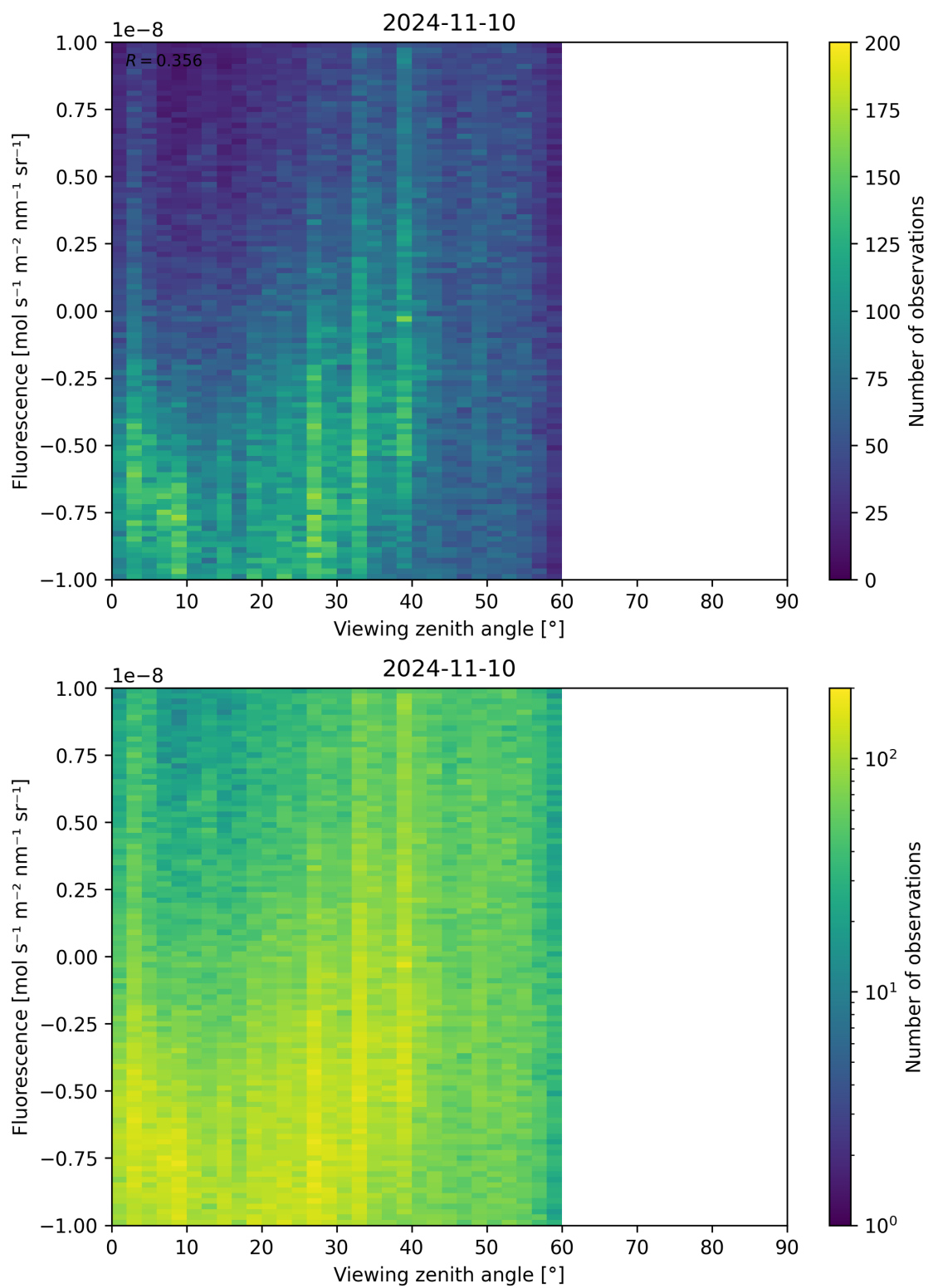
Figure 108: Scatter density plot of “Viewing zenith angle” against “Fluorescence” for 2024-11-09 to 2024-11-11.
