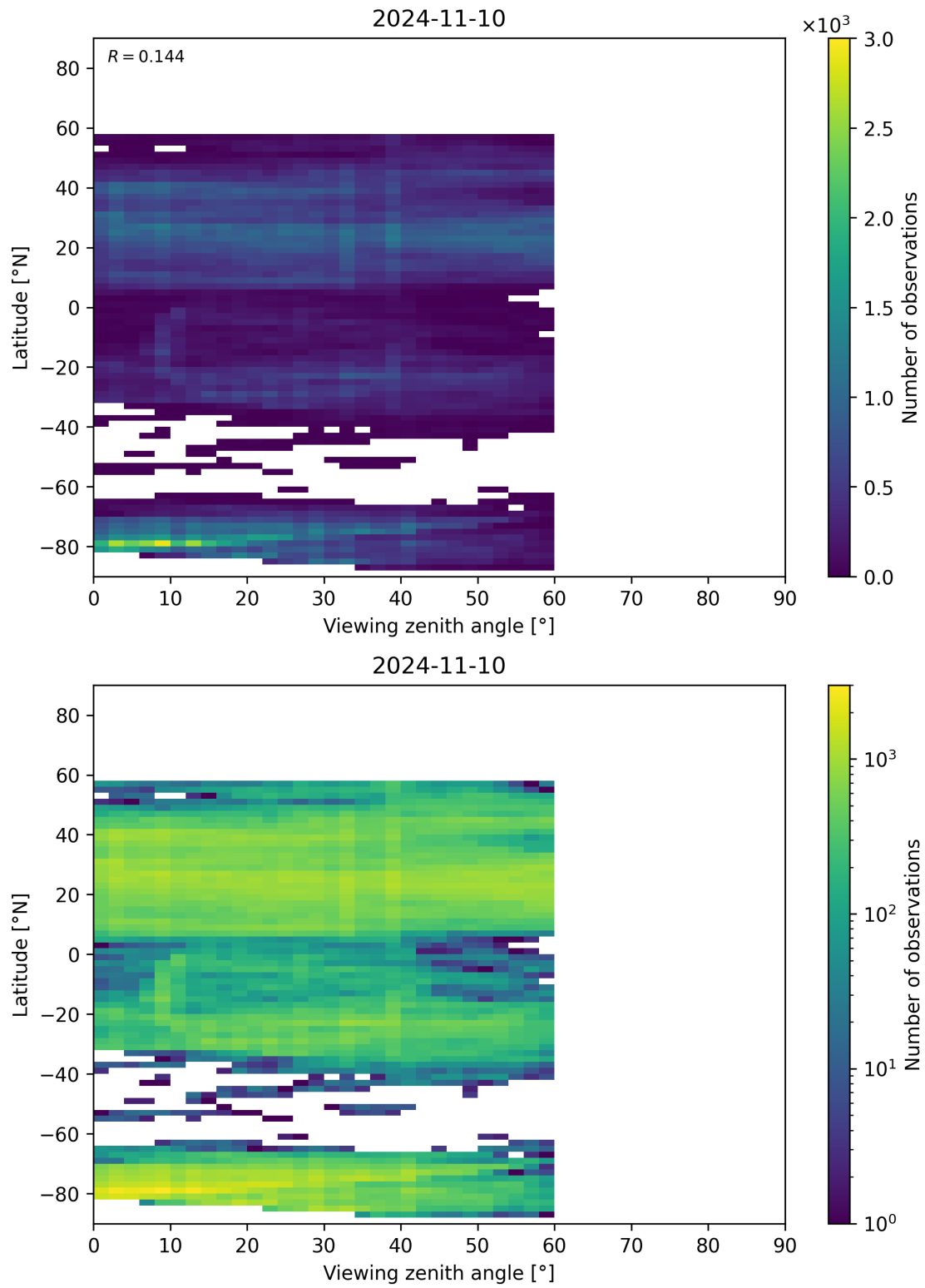
Figure 109: Scatter density plot of “Viewing zenith angle” against “Latitude” for 2024-11-09 to 2024-11-11.
