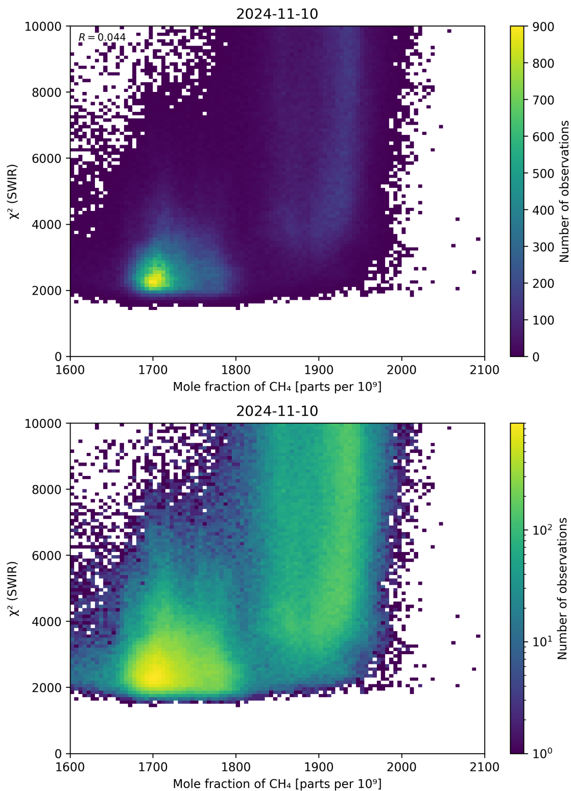
Figure 71: Scatter density plot of “Mole fraction of CH 4 ” against “ \chi^2 (SWIR)” for 2024-11-09 to 2024-11-11.
