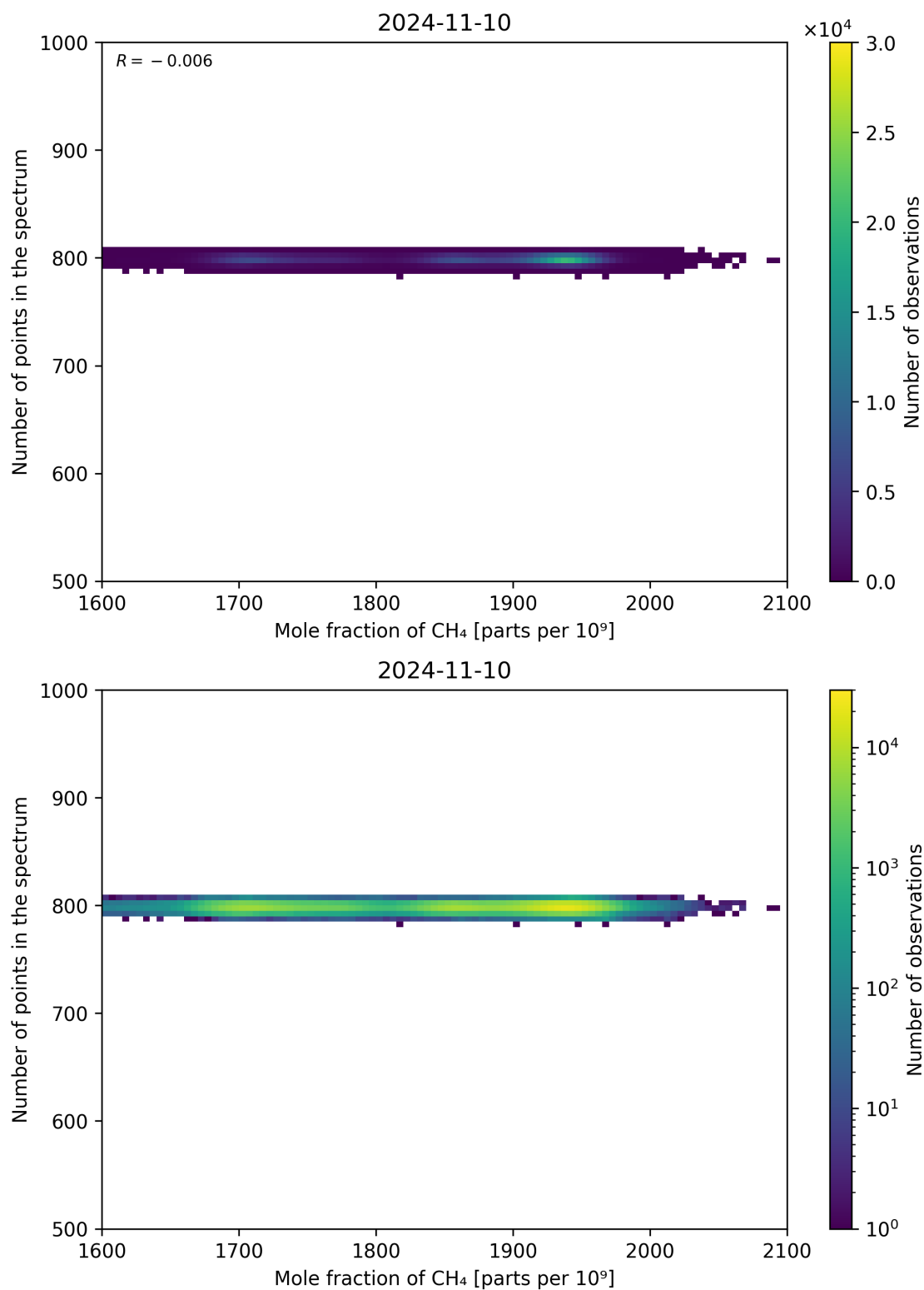
Figure 77: Scatter density plot of “Mole fraction of CH 4 ” against “Number of points in the spectrum” for 2024-11-09 to 2024-11-11.
