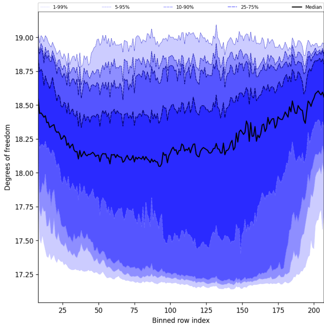
Figure 41: Along track statistics of “Degrees of freedom” for 2024-11-09 to 2024-11-11
