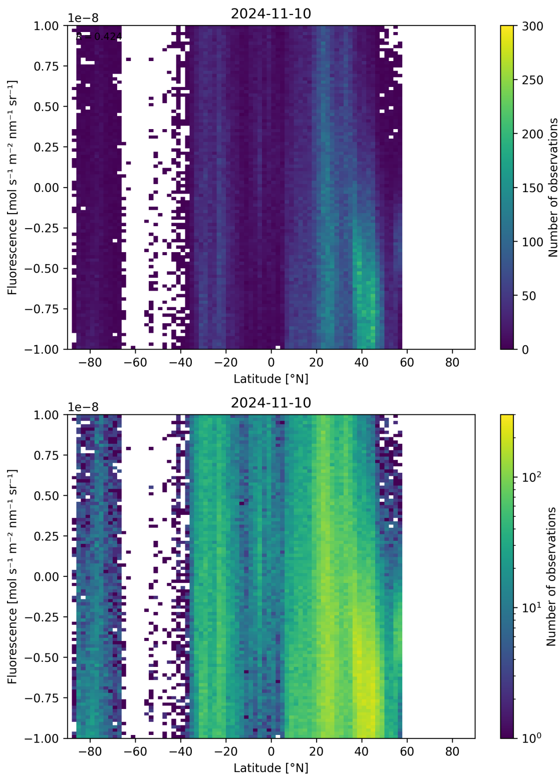
Figure 56: Scatter density plot of “Latitude” against “Fluorescence” for 2024-11-09 to 2024-11-11.
