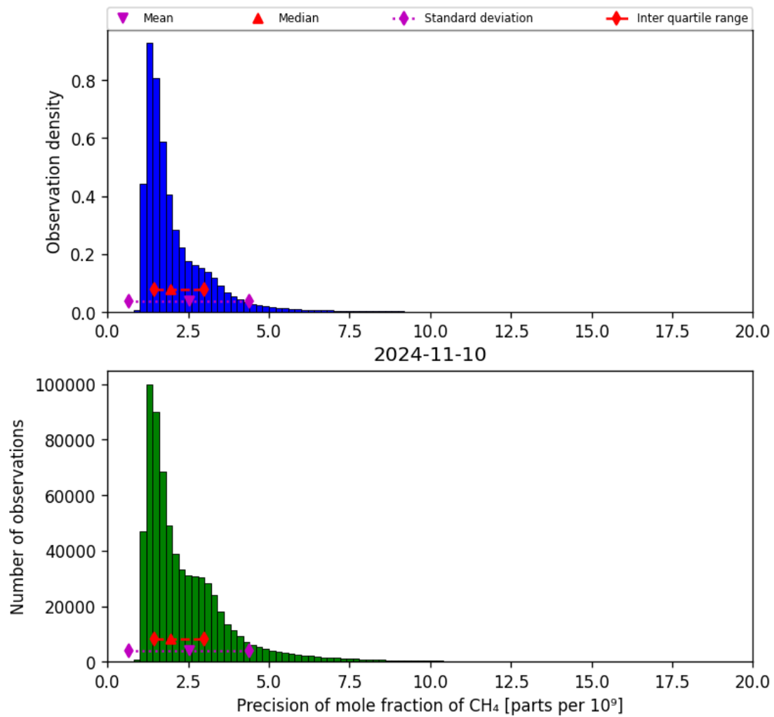
Figure 24: Histogram of “Precision of mole fraction of CH 4 ” for 2024-11-09 to 2024-11-11
