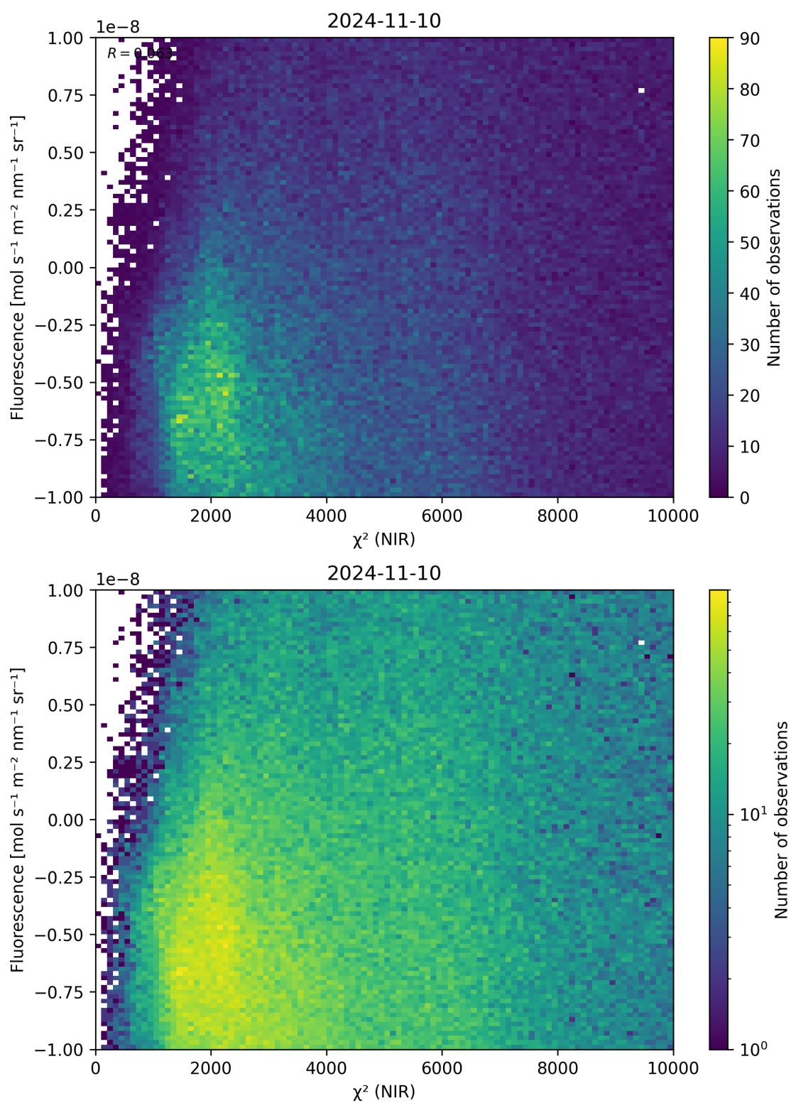
Figure 45: Scatter density plot of “ \chi^2 (NIR)” against “Fluorescence” for 2024-11-09 to 2024-11-11.
