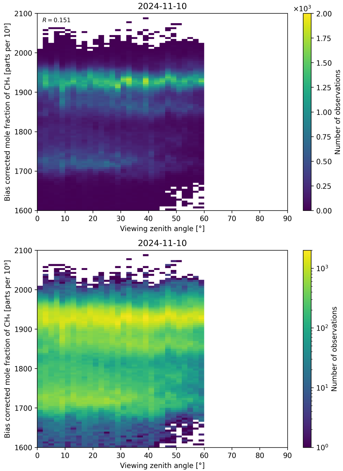
Figure 111: Scatter density plot of “Viewing zenith angle” against “Bias corrected mole fraction of CH 4 ” for 2024-11-09 to 2024-11-11.
