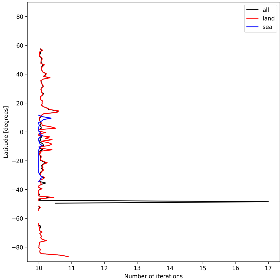
Figure 20: Zonal average of “Number of iterations” for 2024-11-09 to 2024-11-11.
