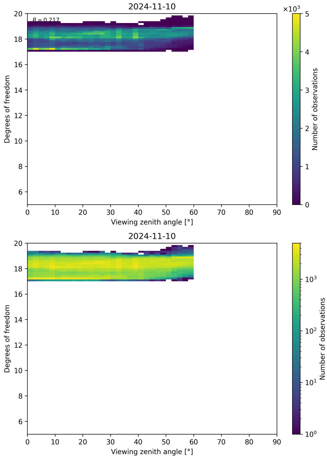
Figure 107: Scatter density plot of “Viewing zenith angle” against “Degrees of freedom” for 2024-11-09 to 2024-11-11.
