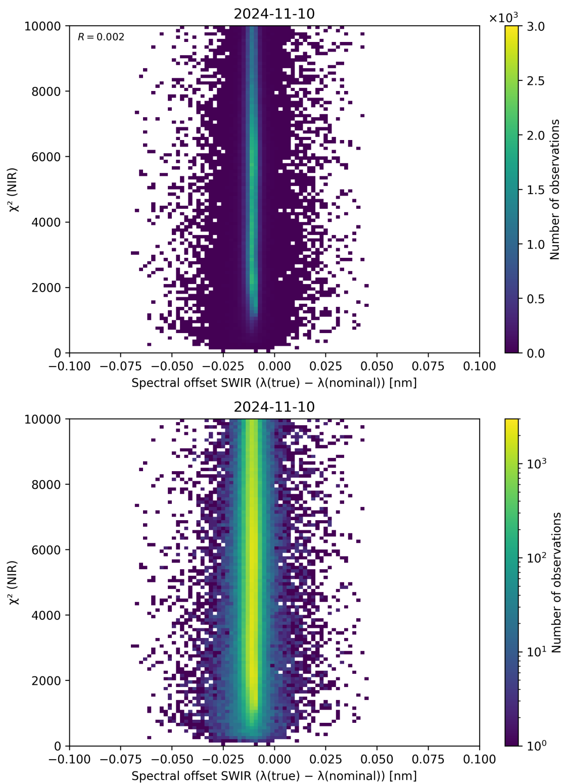
Figure 117: Scatter density plot of “Spectral offset SWIR ( \lambda_{\text{true}} - \lambda_{\text{nominal}} )” against “ \chi^2 (NIR)” for 2024-11-09 to 2024-11-11.
