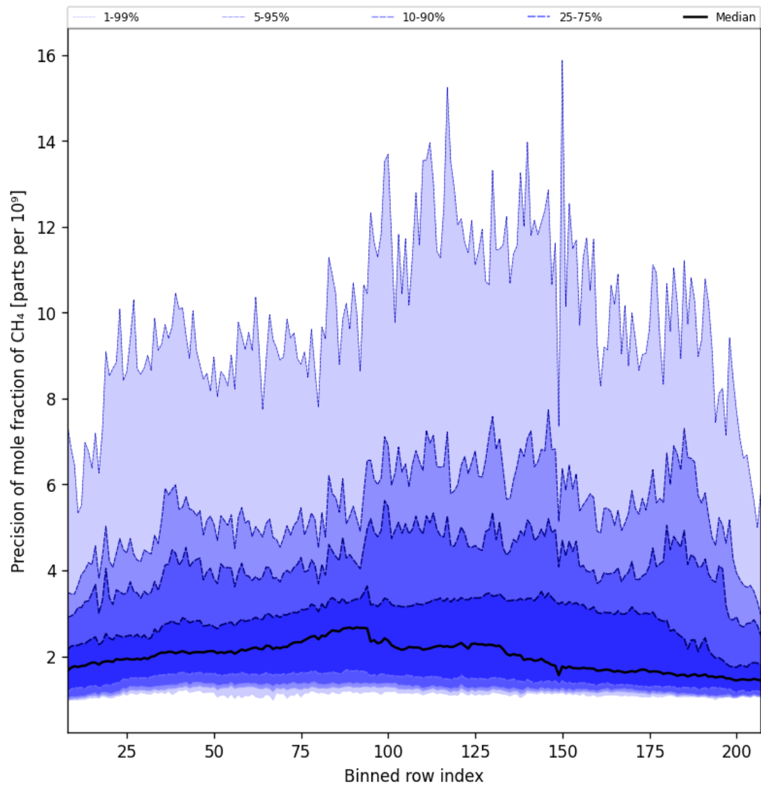
Figure 35: Along track statistics of “Precision of mole fraction of CH 4 ” for 2024-11-09 to 2024-11-11
