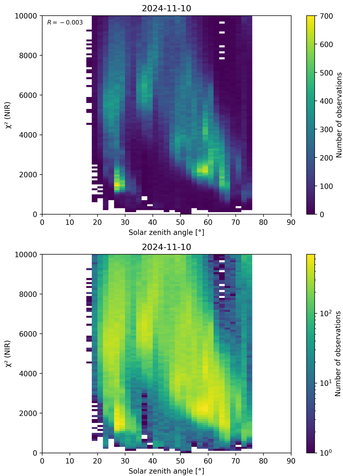
Figure 94: Scatter density plot of “Solar zenith angle” against “ \chi^2 (NIR)” for 2024-11-09 to 2024-11-11.
