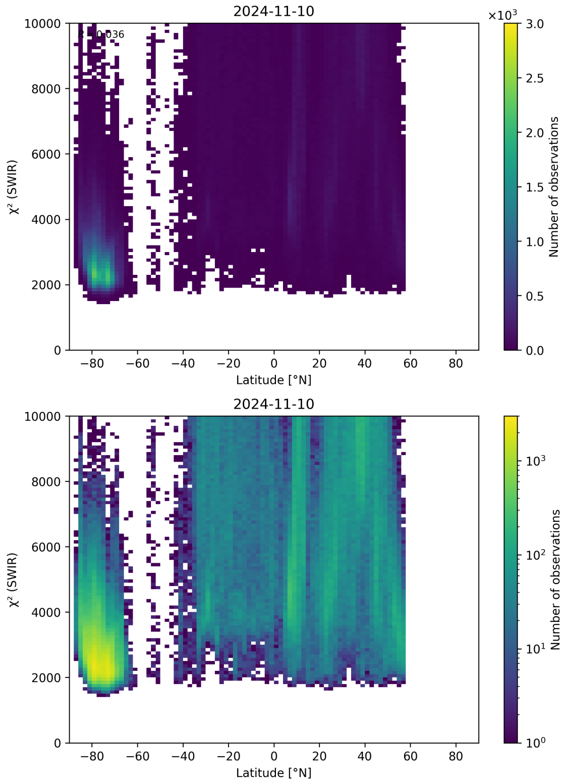
Figure 54: Scatter density plot of “Latitude” against “ \chi^2 (SWIR)” for 2024-11-09 to 2024-11-11.
