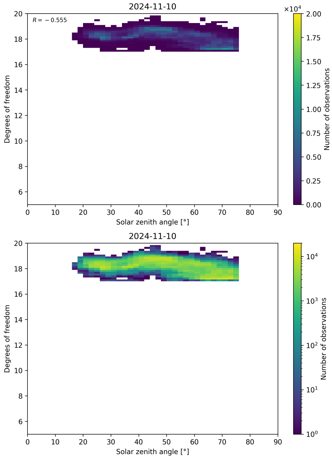
Figure 96: Scatter density plot of “Solar zenith angle” against “Degrees of freedom” for 2024-11-09 to 2024-11-11.
