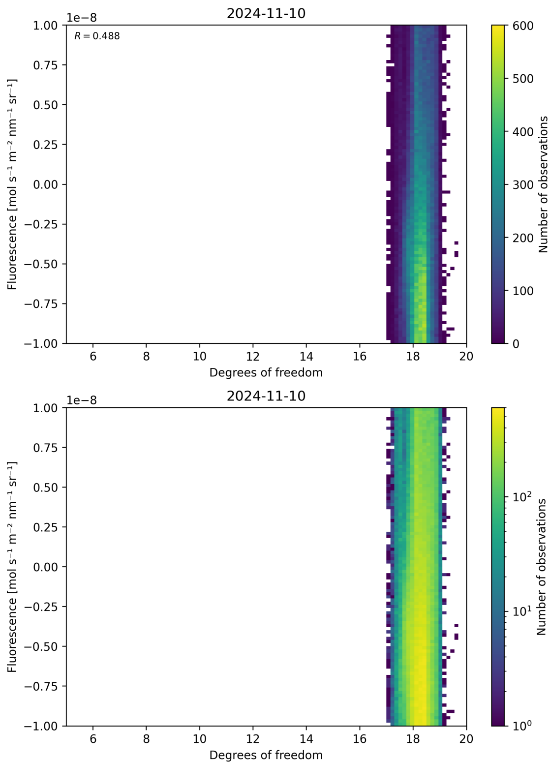
Figure 51: Scatter density plot of “Degrees of freedom” against “Fluorescence” for 2024-11-09 to 2024-11-11.
