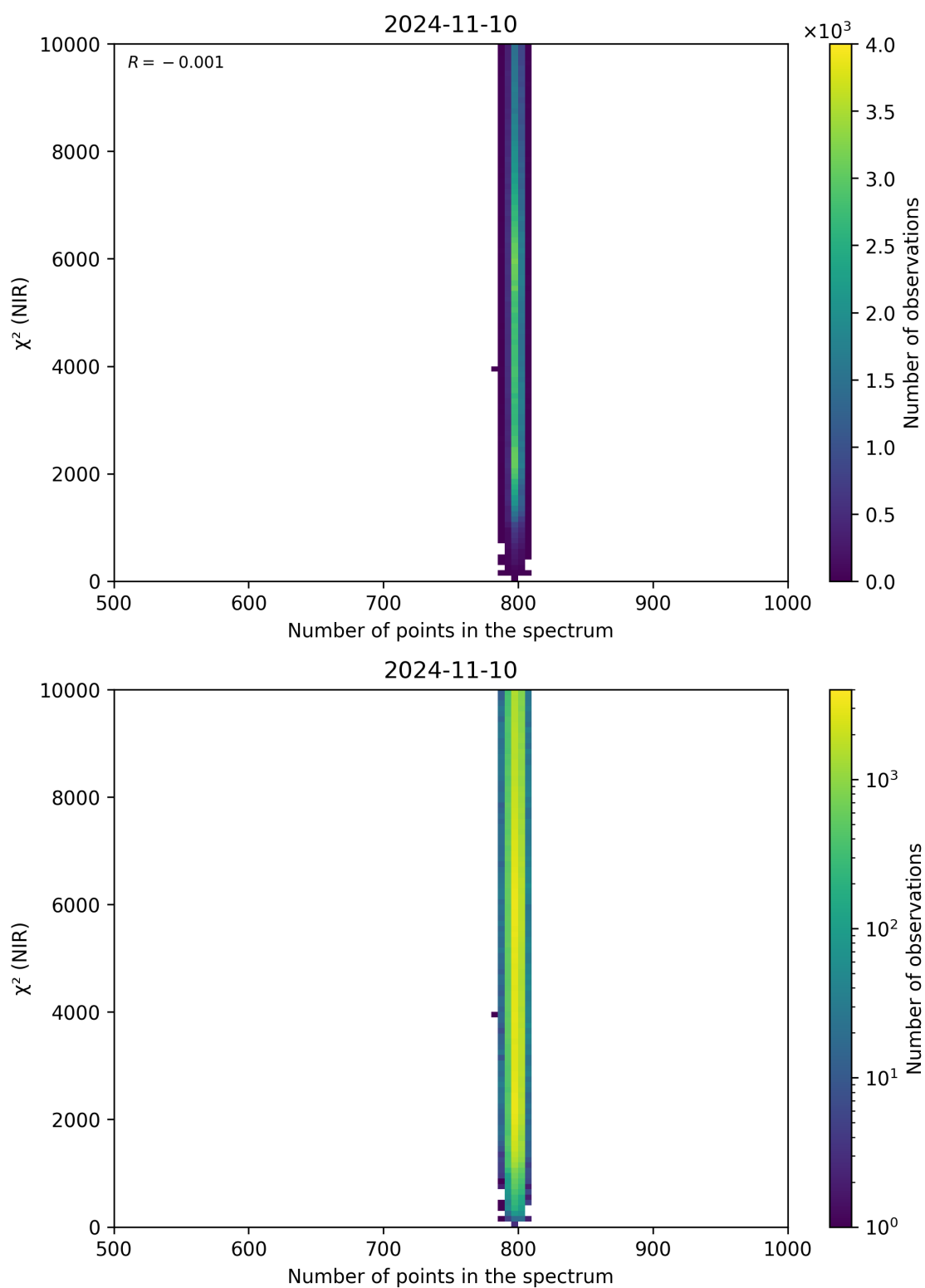
Figure 88: Scatter density plot of “Number of points in the spectrum” against “ \chi^2 (NIR)” for 2024-11-09 to 2024-11-11.
