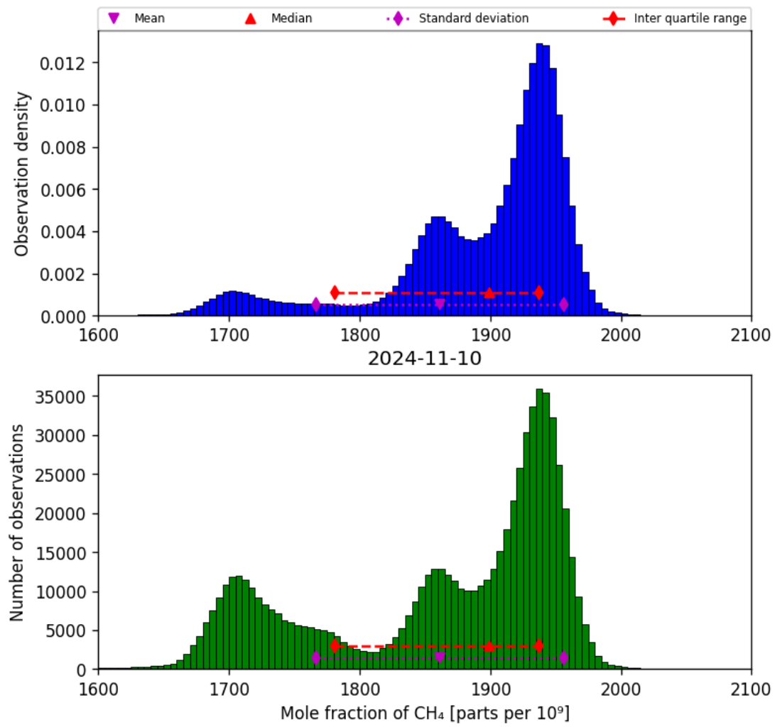
Figure 23: Histogram of “Mole fraction of CH 4 ” for 2024-11-09 to 2024-11-11
