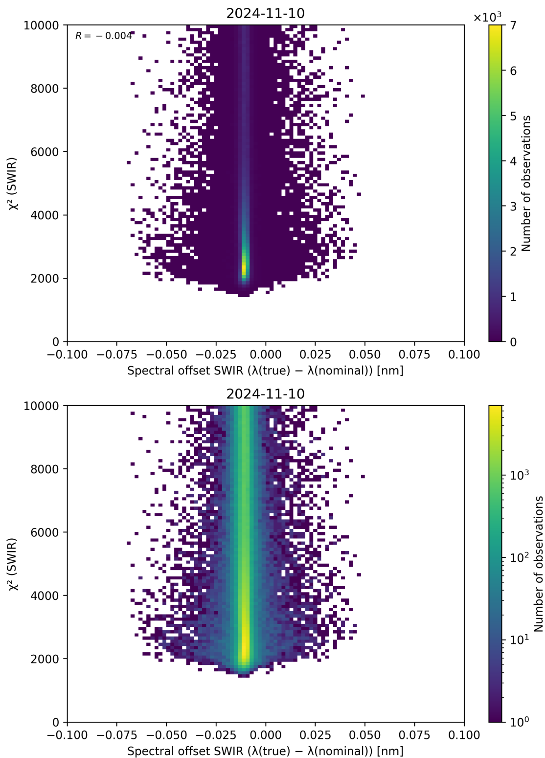
Figure 118: Scatter density plot of “Spectral offset SWIR ( \lambda_{\text{true}} - \lambda_{\text{nominal}} )” against “ \chi^2 (SWIR)” for 2024-11-09 to 2024-11-11.
