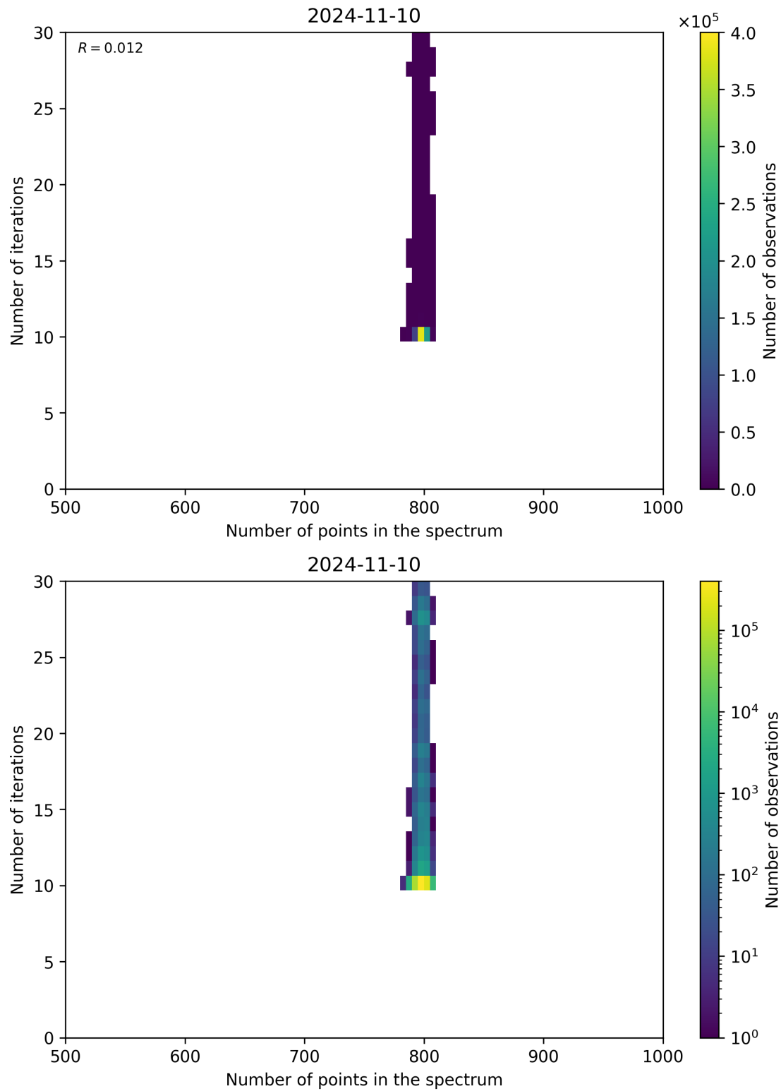
Figure 92: Scatter density plot of “Number of points in the spectrum” against “Number of iterations” for 2024-11-09 to 2024-11-11.
