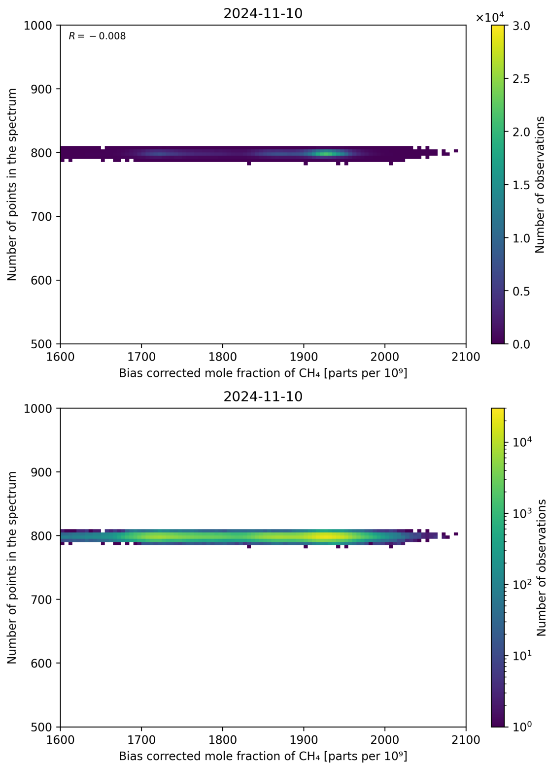
Figure 68: Scatter density plot of “Bias corrected mole fraction of CH 4 ” against “Number of points in the spectrum” for 2024-11-09 to 2024-11-11.
