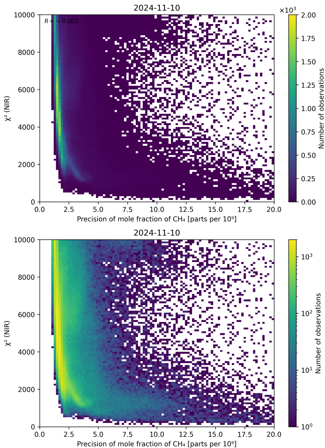
Figure 78: Scatter density plot of “Precision of mole fraction of CH 4 ” against “ \chi^2 (NIR)” for 2024-11-09 to 2024-11-11.
