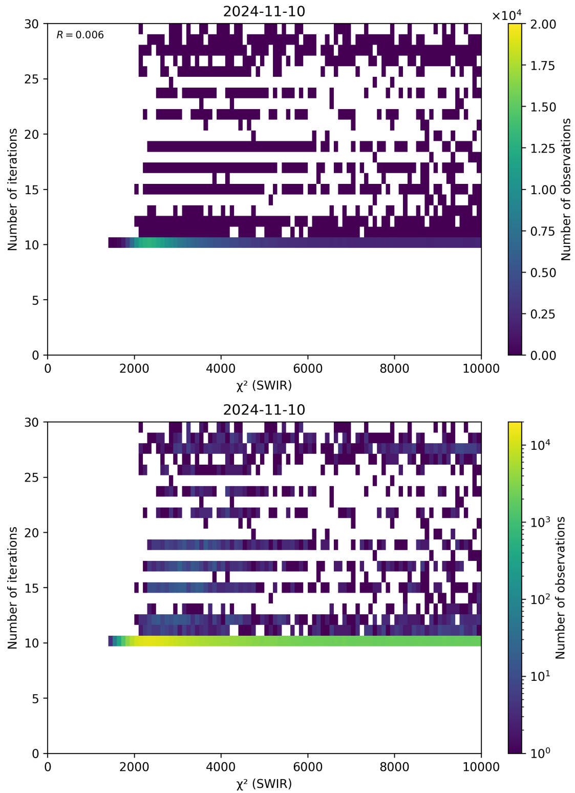
Figure 50: Scatter density plot of “ \chi^2 (SWIR)” against “Number of iterations” for 2024-11-09 to 2024-11-11.
