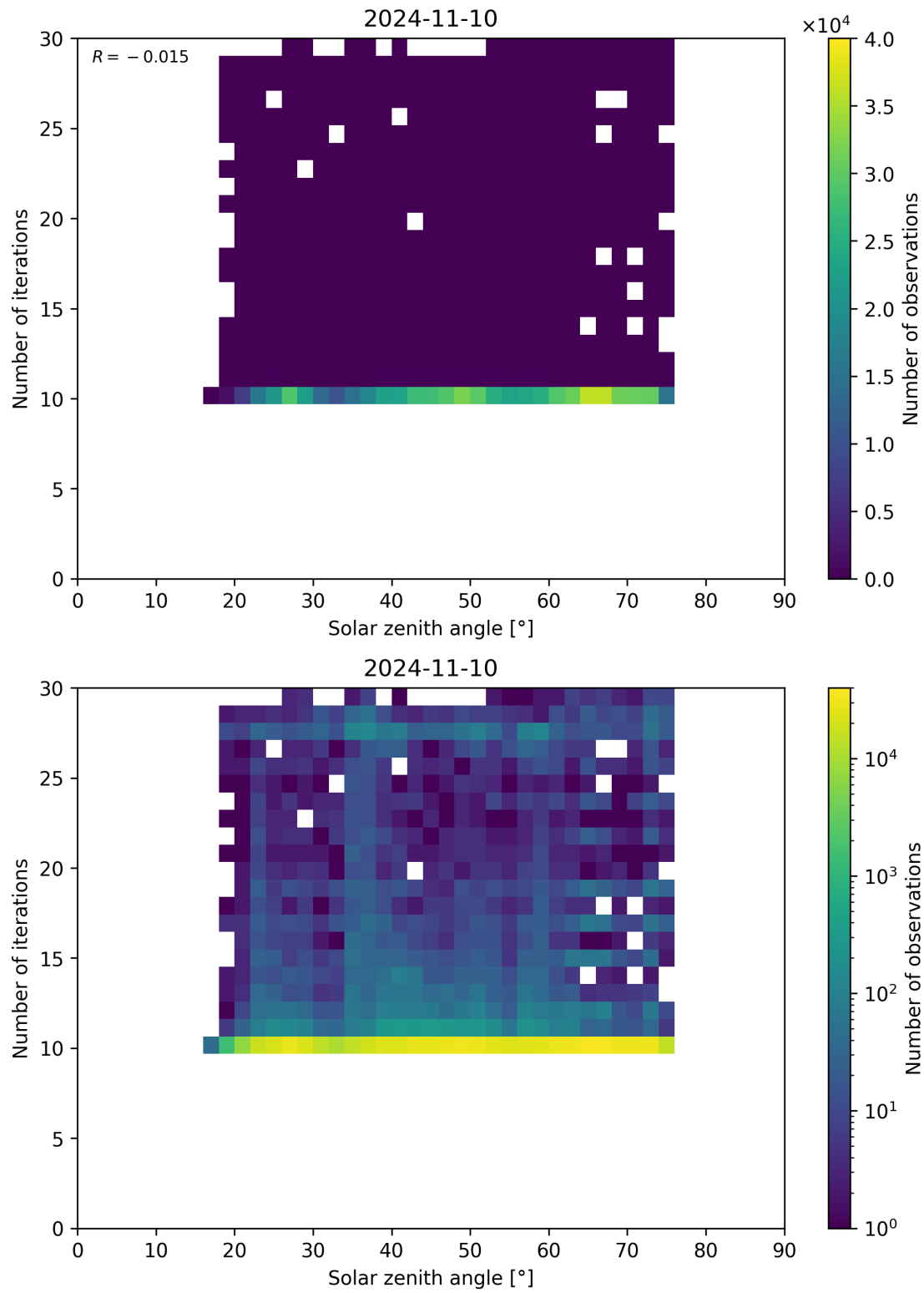
Figure 102: Scatter density plot of “Solar zenith angle” against “Number of iterations” for 2024-11-09 to 2024-11-11.
