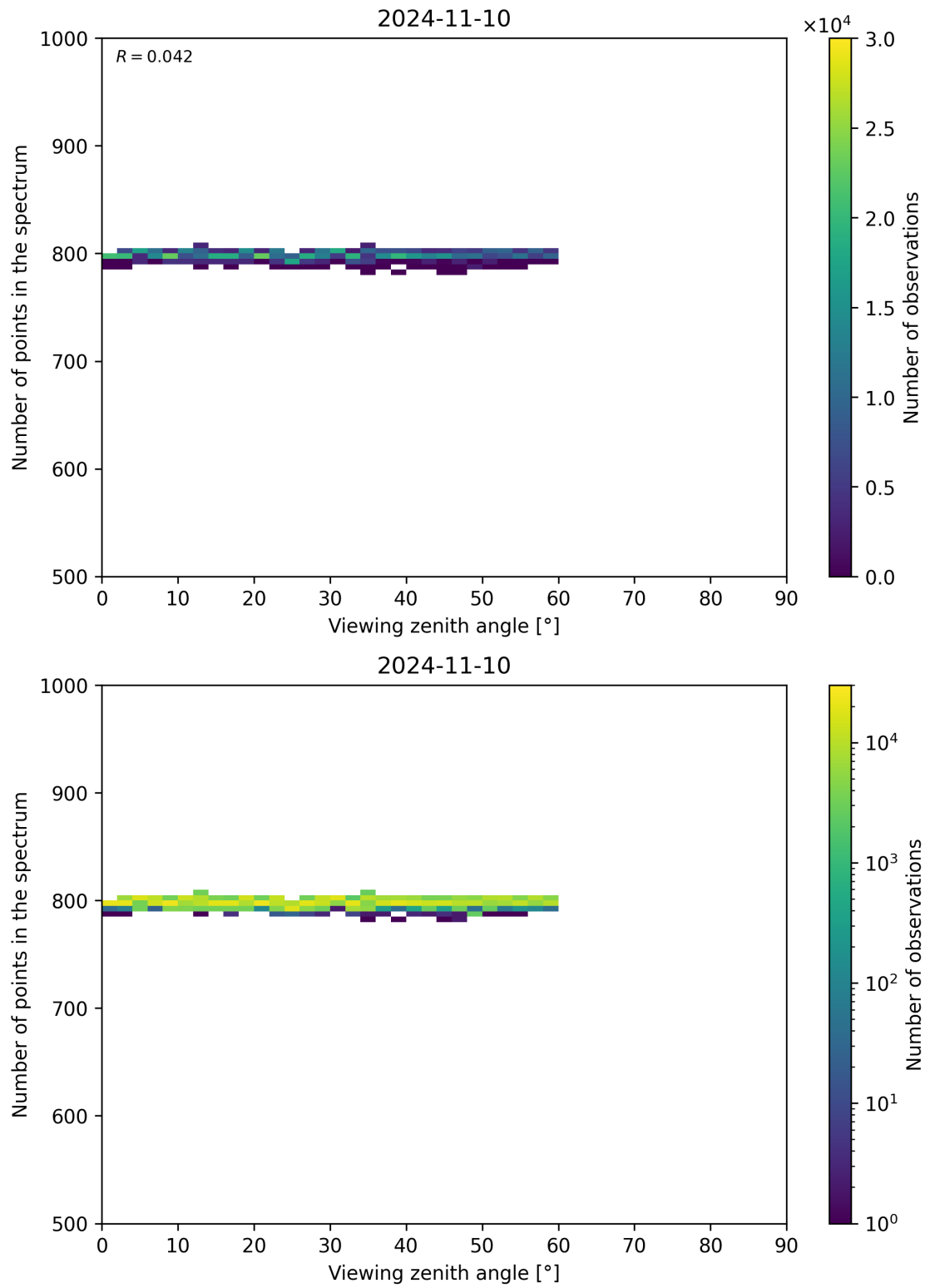
Figure 114: Scatter density plot of “Viewing zenith angle” against “Number of points in the spectrum” for 2024-11-09 to 2024-11-11.
