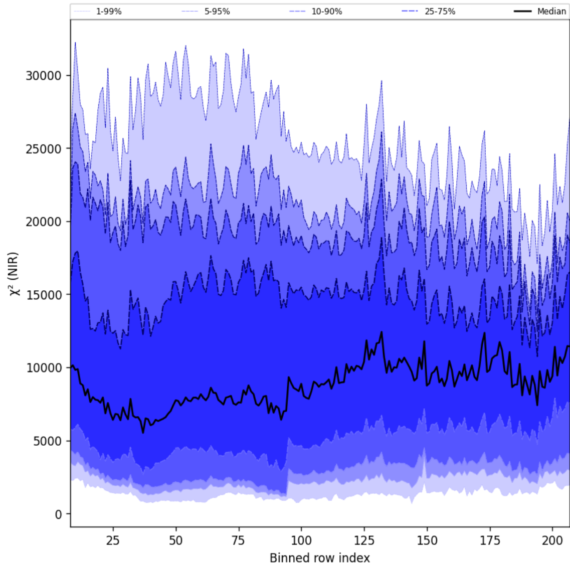
Figure 40: Along track statistics of “ \chi^2 (NIR)” for 2024-11-09 to 2024-11-11
