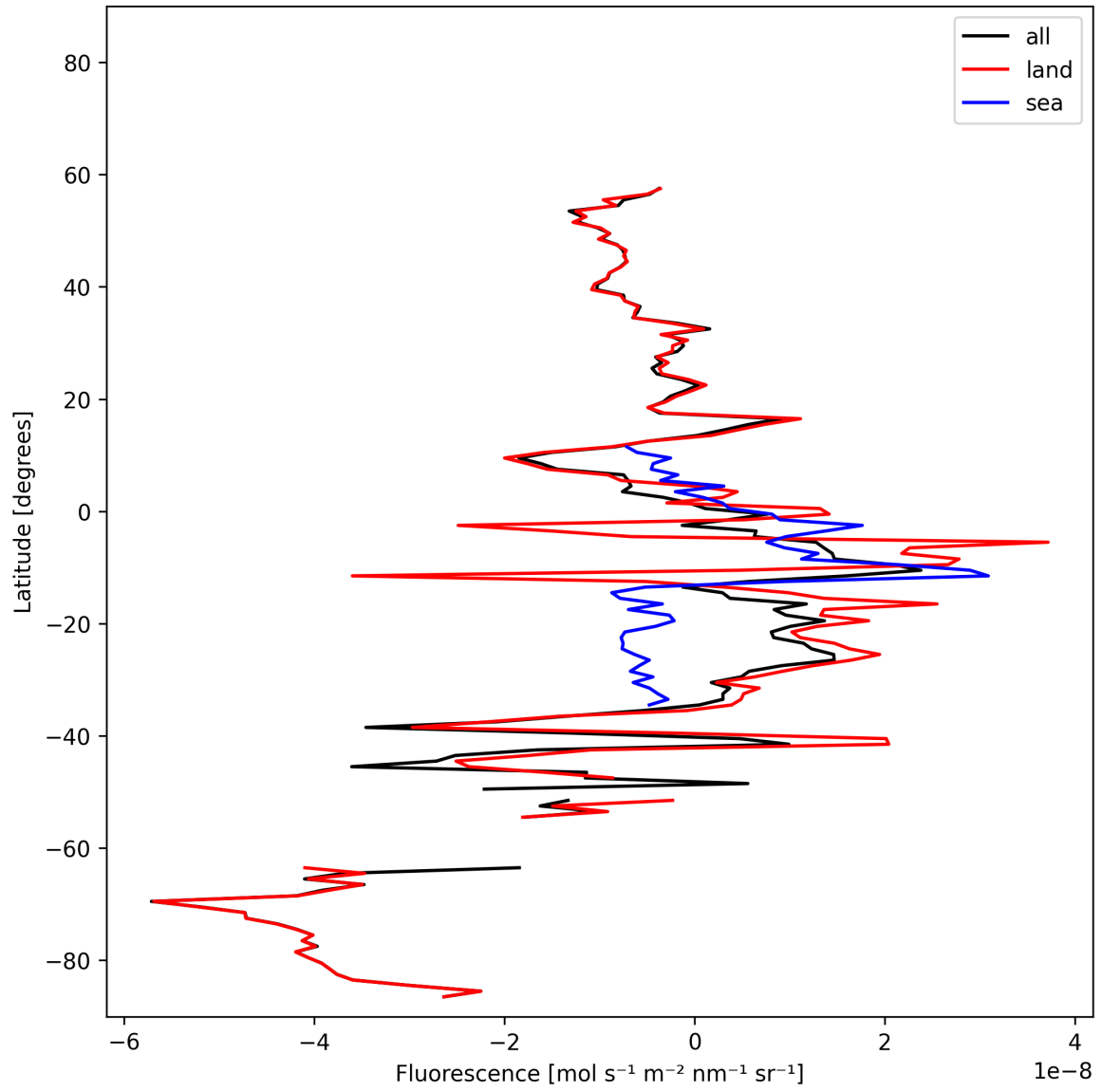
Figure 21: Zonal average of “Fluorescence” for 2024-11-09 to 2024-11-11.
