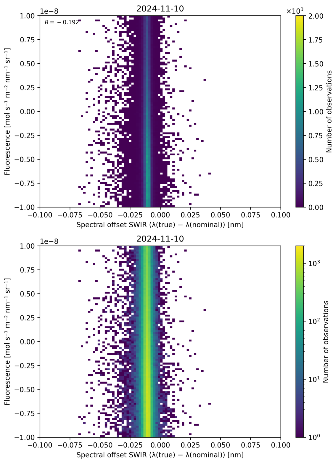
Figure 120: Scatter density plot of “Spectral offset SWIR ( \lambda_{\text{true}} - \lambda_{\text{nominal}} )” against “Fluorescence” for 2024-11-09 to 2024-11-11.
