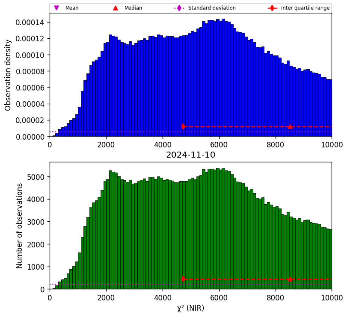
Figure 29: Histogram of “ \chi^2 (NIR)” for 2024-11-09 to 2024-11-11
