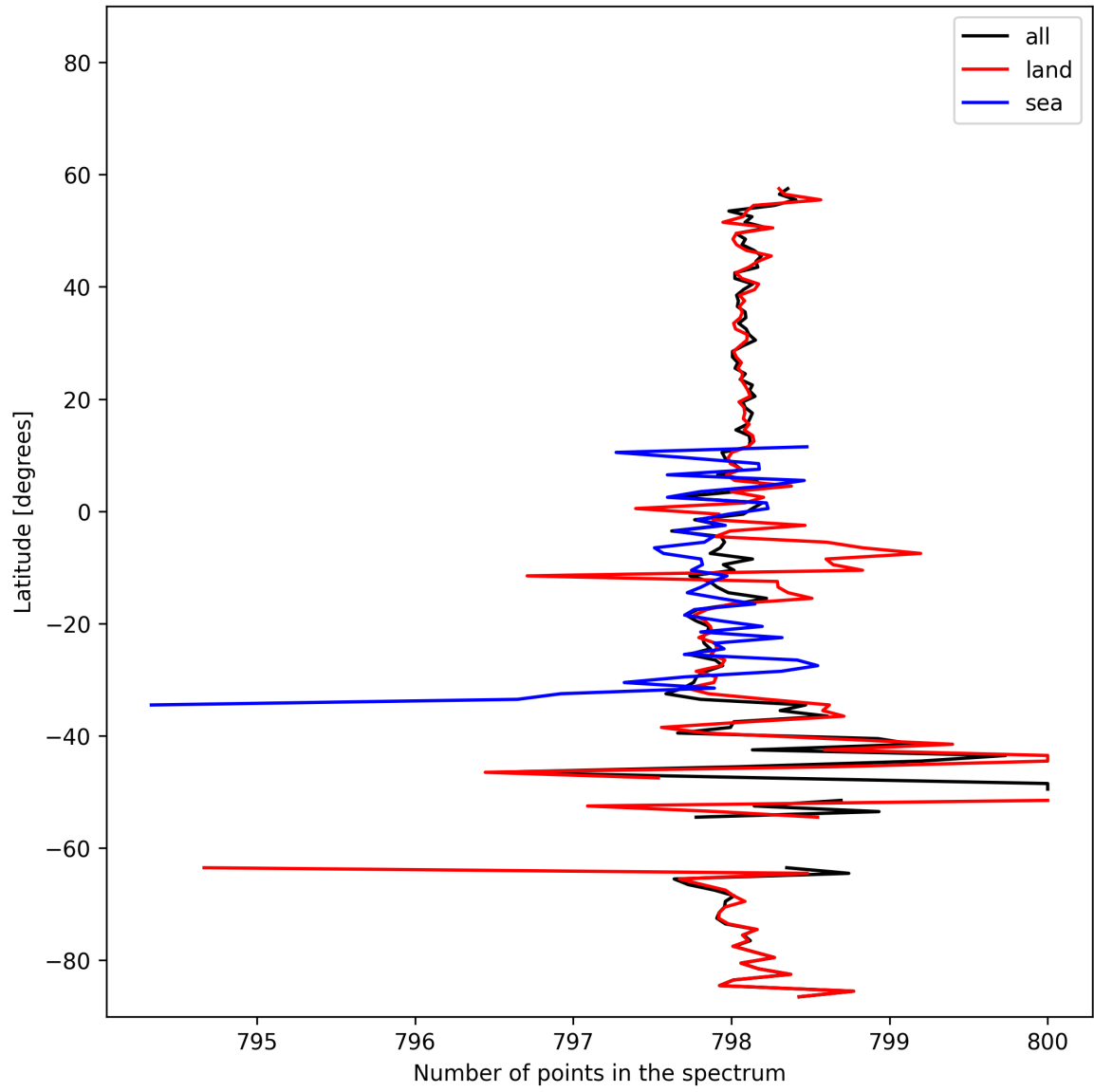
Figure 15: Zonal average of “Number of points in the spectrum” for 2024-11-09 to 2024-11-11.
