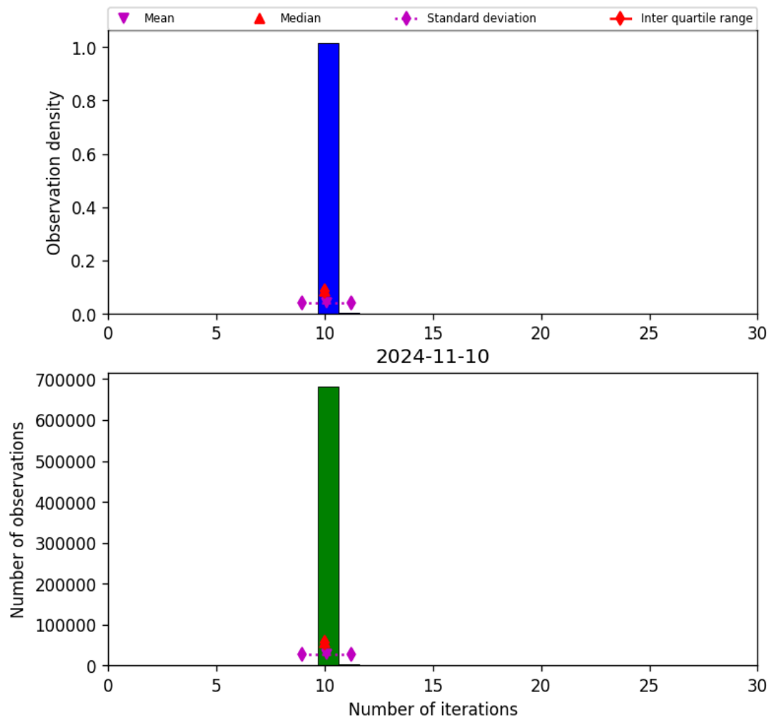
Figure 31: Histogram of “Number of iterations” for 2024-11-09 to 2024-11-11
