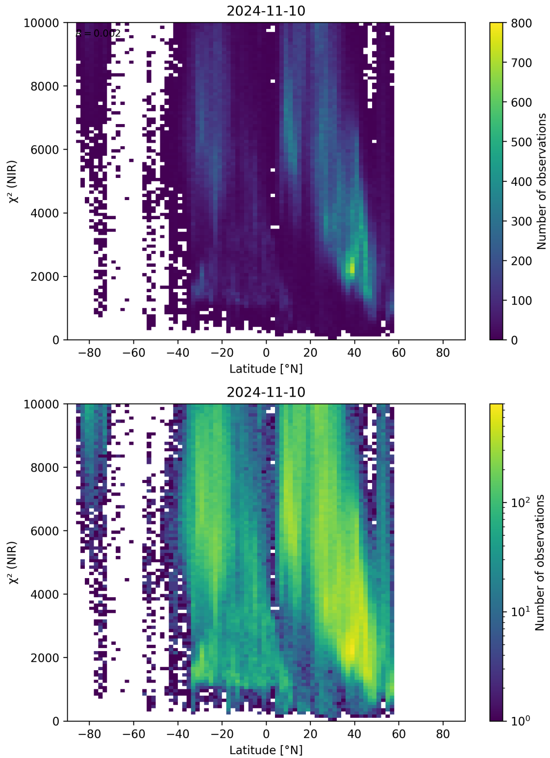
Figure 53: Scatter density plot of “Latitude” against “ \chi^2 (NIR)” for 2024-11-09 to 2024-11-11.
