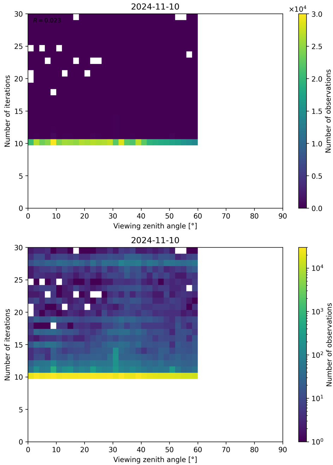
Figure 113: Scatter density plot of “Viewing zenith angle” against “Number of iterations” for 2024-11-09 to 2024-11-11.
