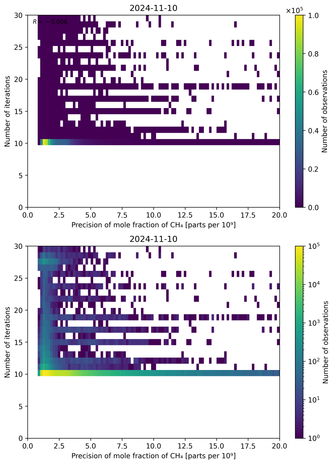
Figure 83: Scatter density plot of “Precision of mole fraction of CH 4 ” against “Number of iterations” for 2024-11-09 to 2024-11-11.
