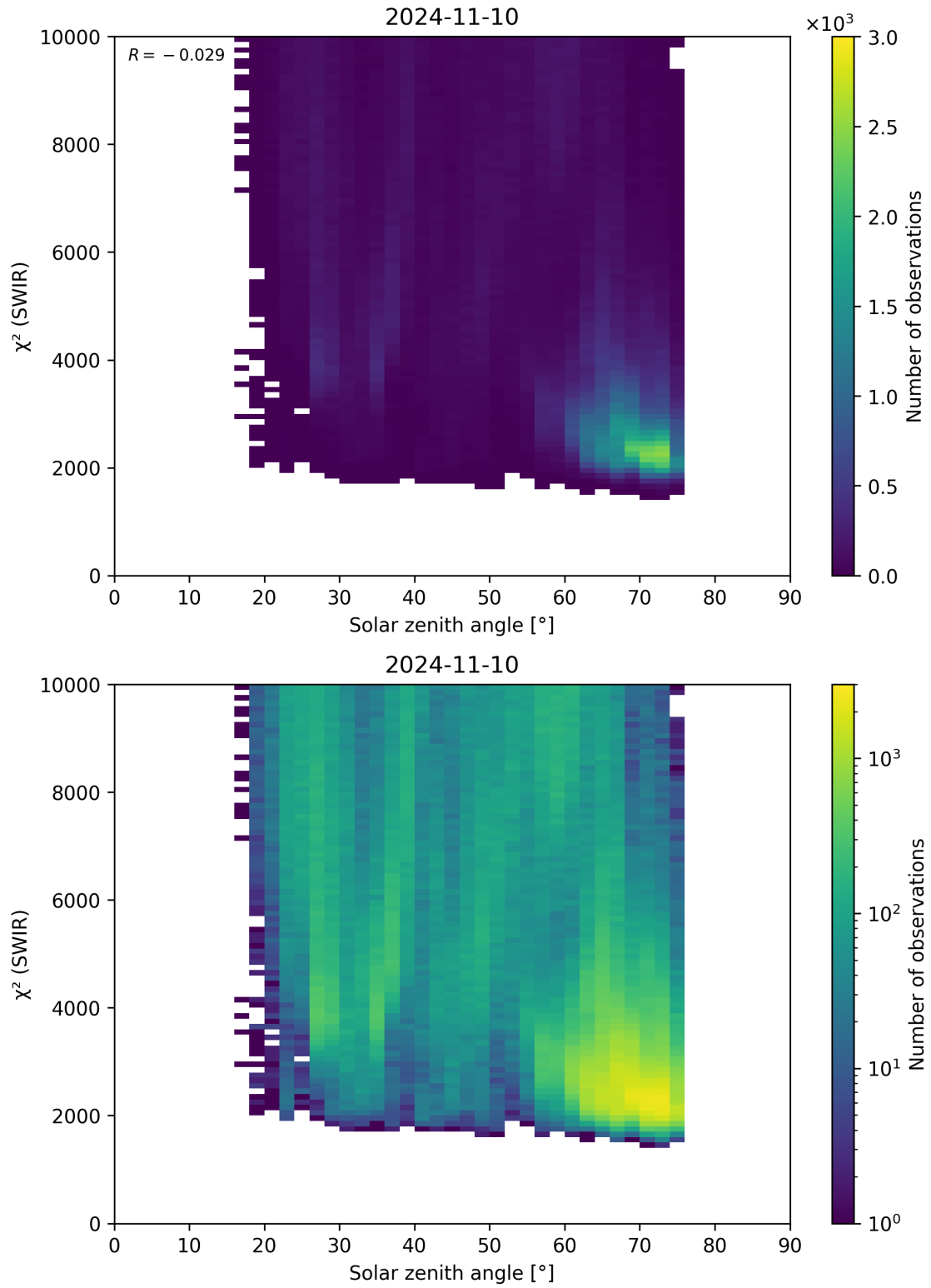
Figure 95: Scatter density plot of “Solar zenith angle” against “ \chi^2 (SWIR)” for 2024-11-09 to 2024-11-11.
