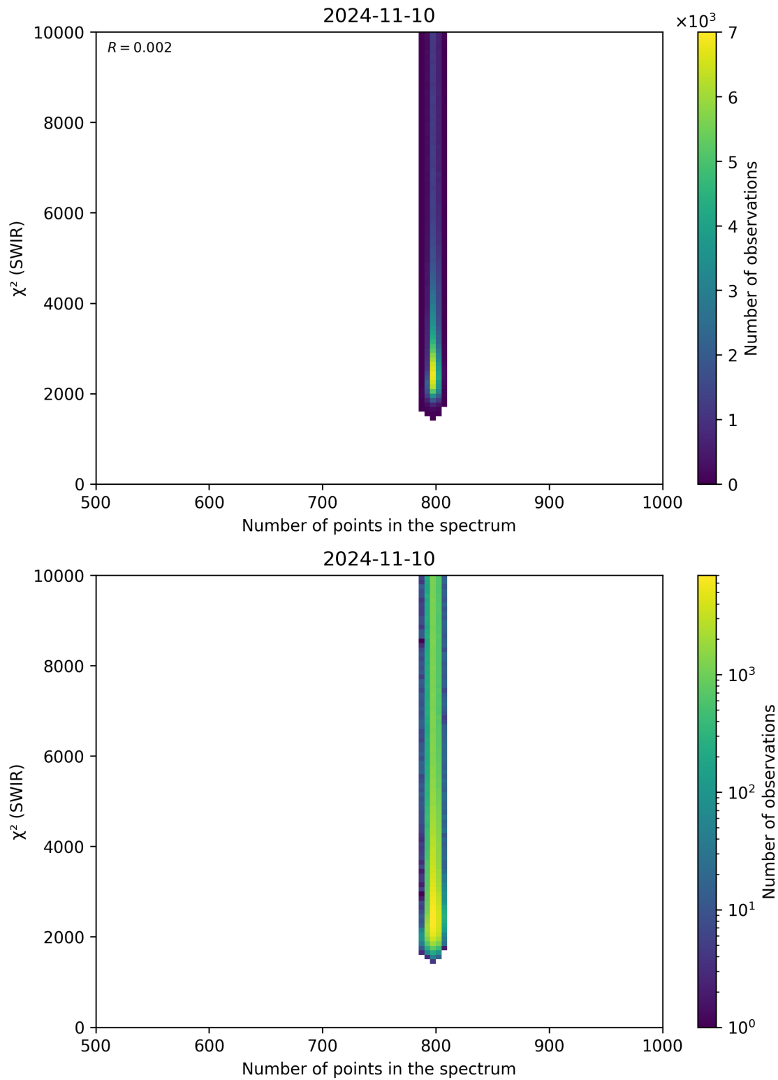
Figure 89: Scatter density plot of “Number of points in the spectrum” against “ \chi^2 (SWIR)” for 2024-11-09 to 2024-11-11.
