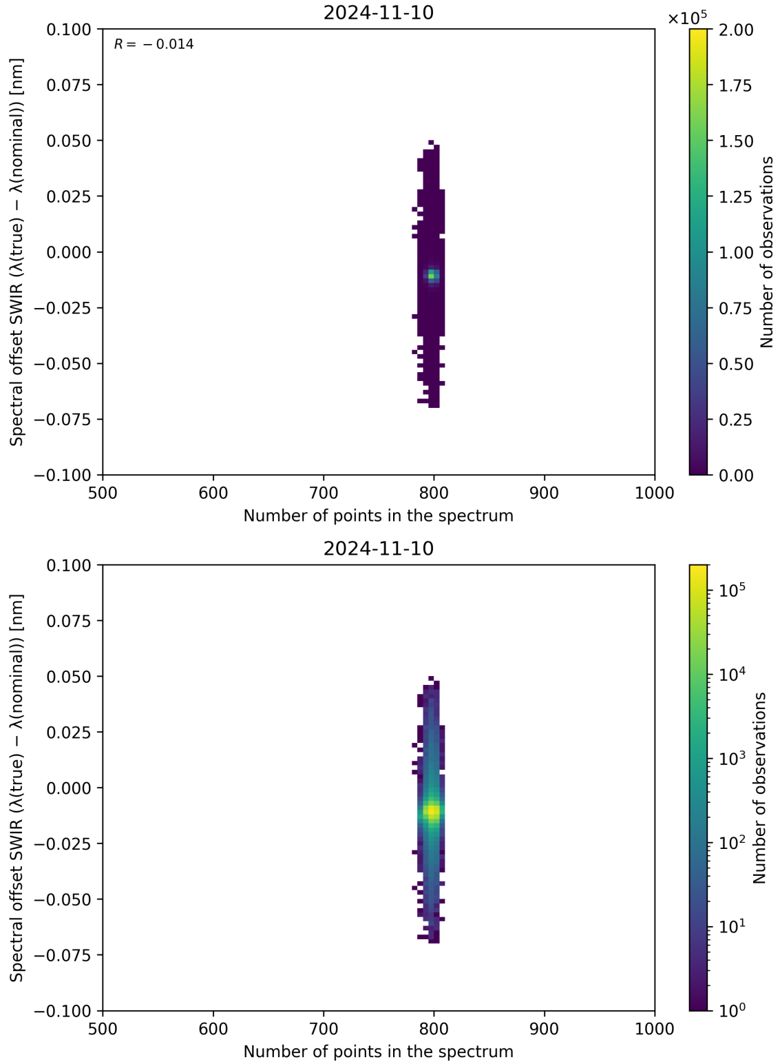
Figure 93: Scatter density plot of “Number of points in the spectrum” against “Spectral offset SWIR ( \lambda_{\text{true}} - \lambda_{\text{nominal}} )” for 2024-11-09 to 2024-11-11.
