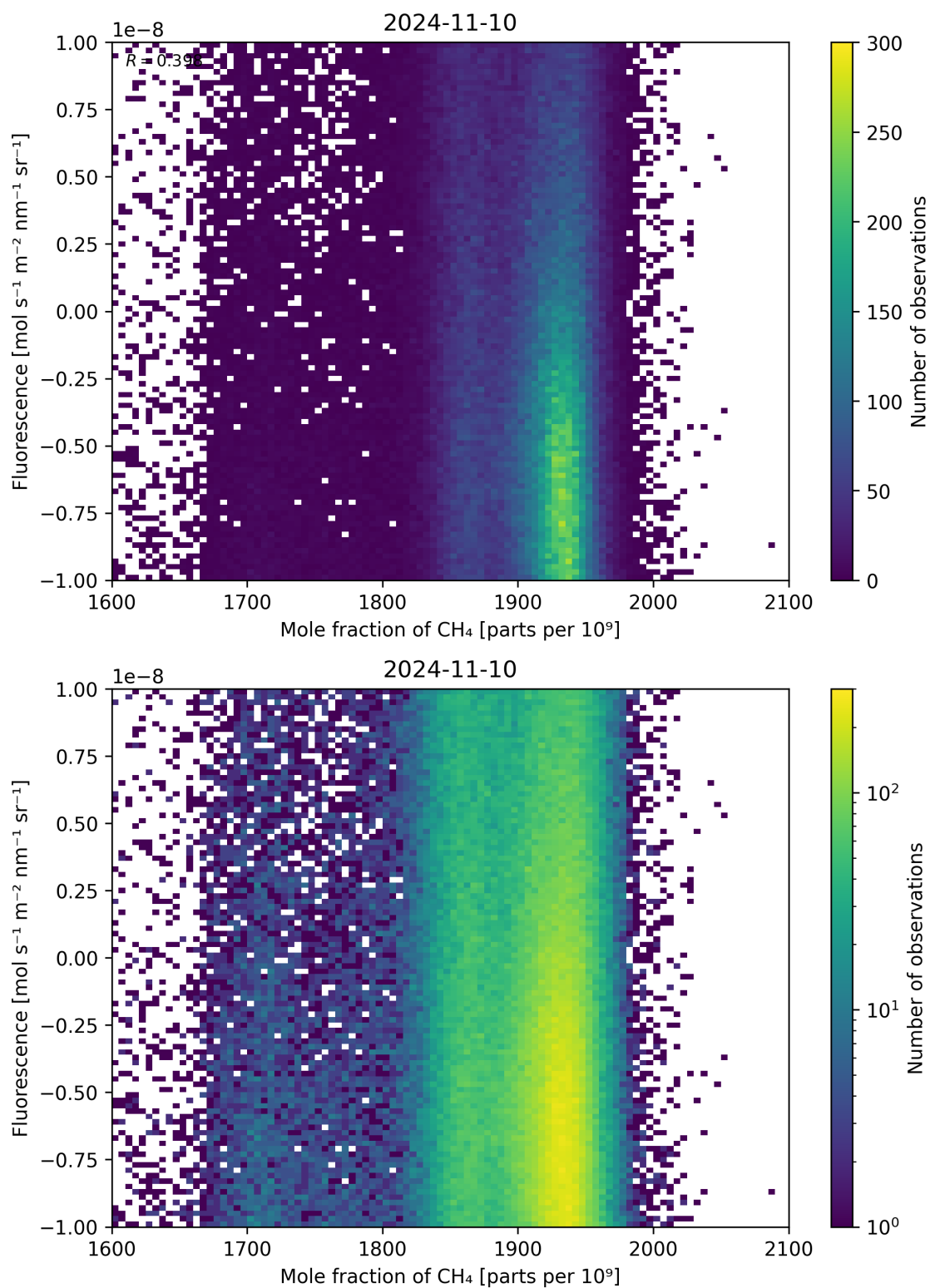
Figure 73: Scatter density plot of “Mole fraction of \text{CH}_4 ” against “Fluorescence” for 2024-11-09 to 2024-11-11.
