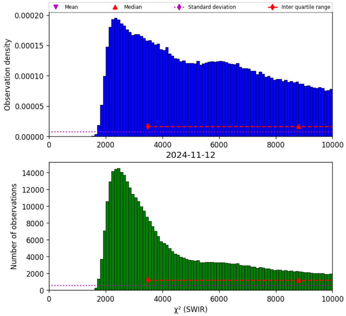
Figure 28: Histogram of “ \chi^2 (SWIR)” for 2024-11-11 to 2024-11-13
