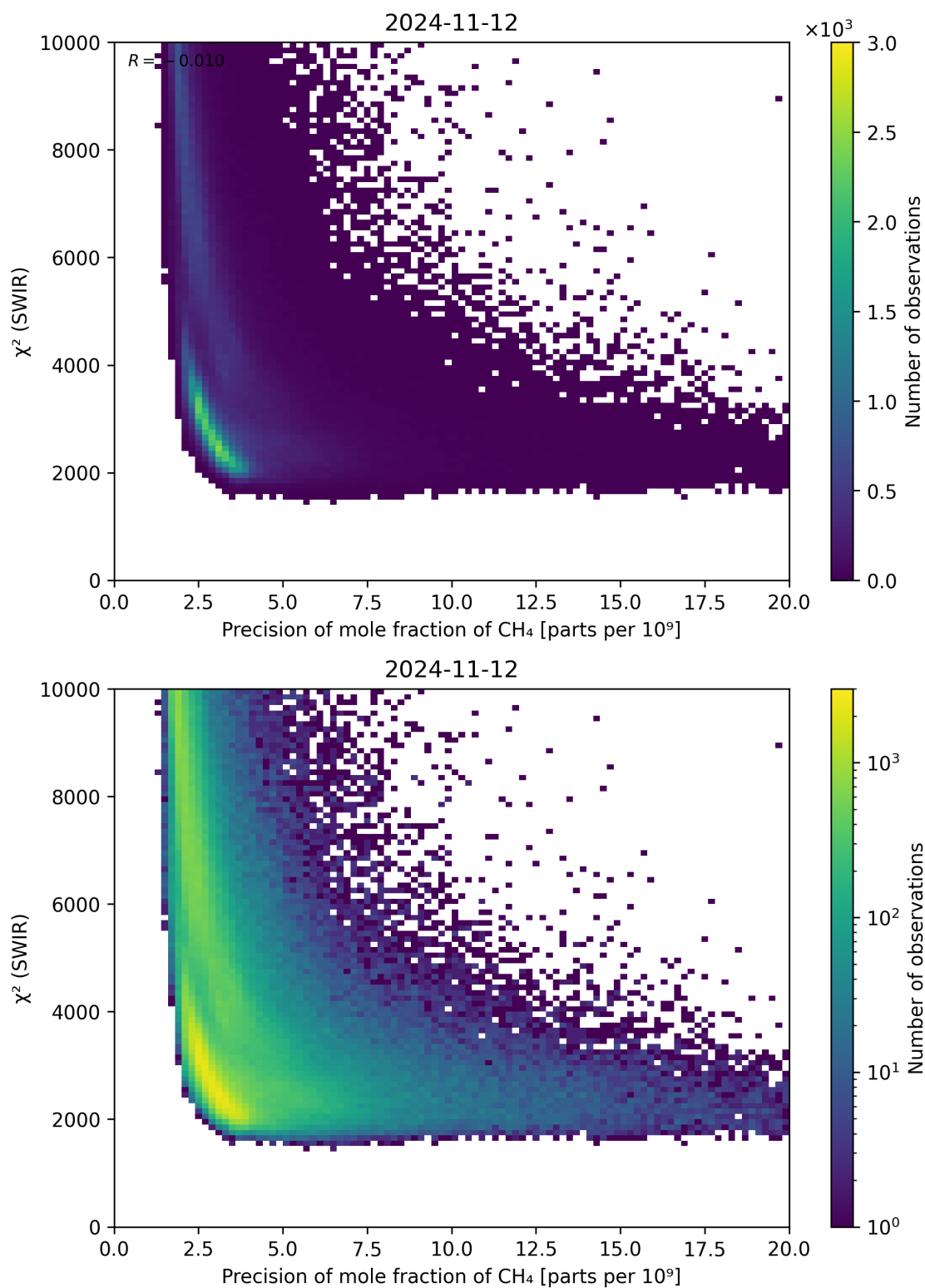
Figure 79: Scatter density plot of “Precision of mole fraction of \text{CH}_4 ” against “ \chi^2 (SWIR)” for 2024-11-11 to 2024-11-13.
