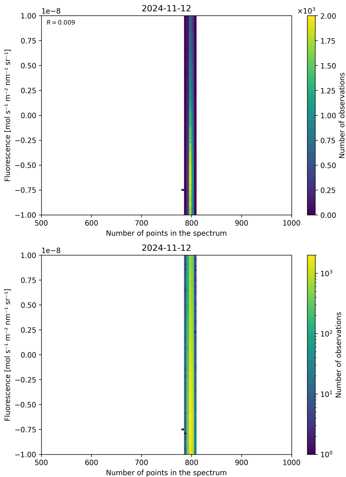
Figure 91: Scatter density plot of “Number of points in the spectrum” against “Fluorescence” for 2024-11-11 to 2024-11-13.
