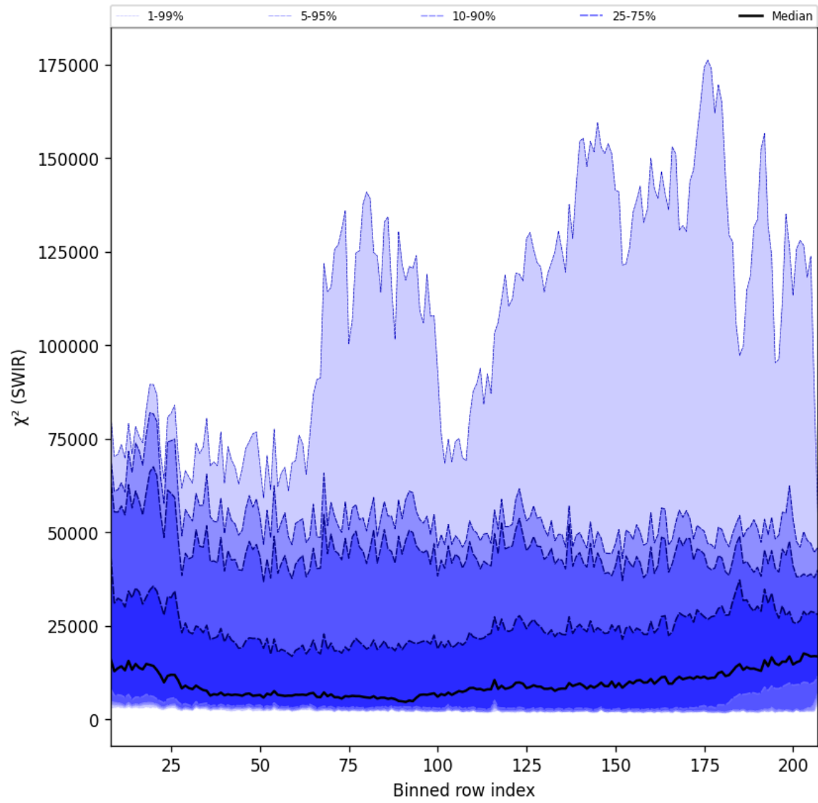
Figure 39: Along track statistics of “ \chi^2 (SWIR)” for 2024-11-11 to 2024-11-13
