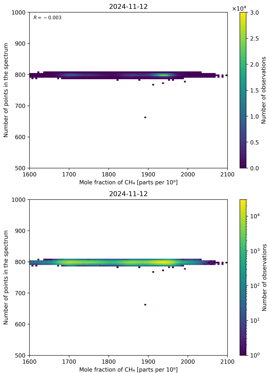
Figure 77: Scatter density plot of “Mole fraction of CH 4 ” against “Number of points in the spectrum” for 2024-11-11 to 2024-11-13.
