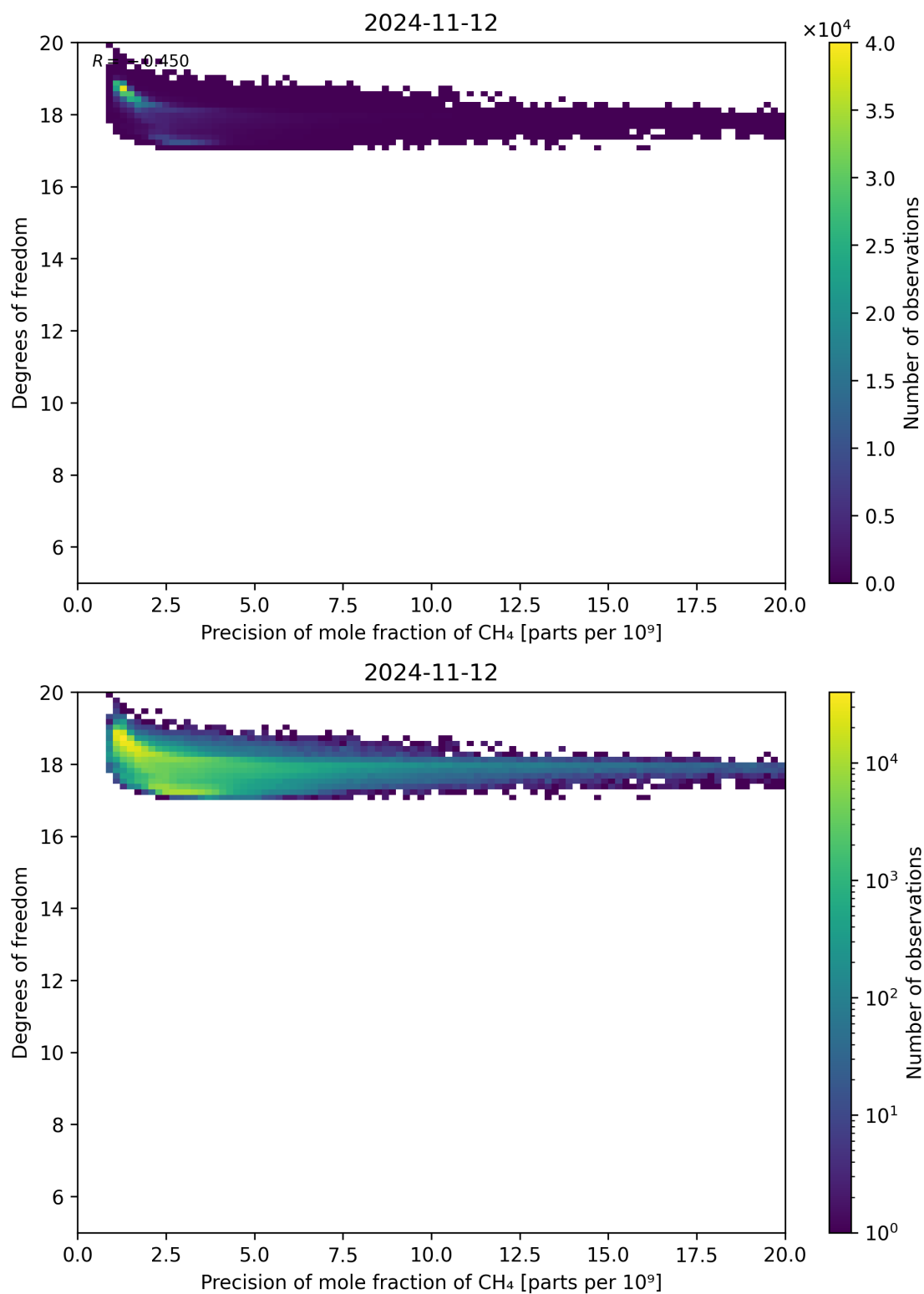
Figure 80: Scatter density plot of “Precision of mole fraction of CH 4 ” against “Degrees of freedom” for 2024-11-11 to 2024-11-13.
