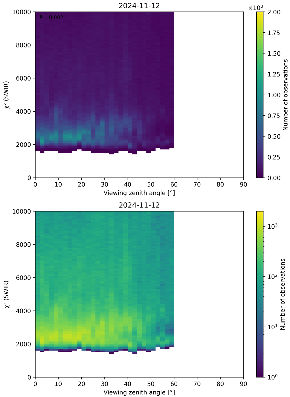
Figure 106: Scatter density plot of “Viewing zenith angle” against “ \chi^2 (SWIR)” for 2024-11-11 to 2024-11-13.
