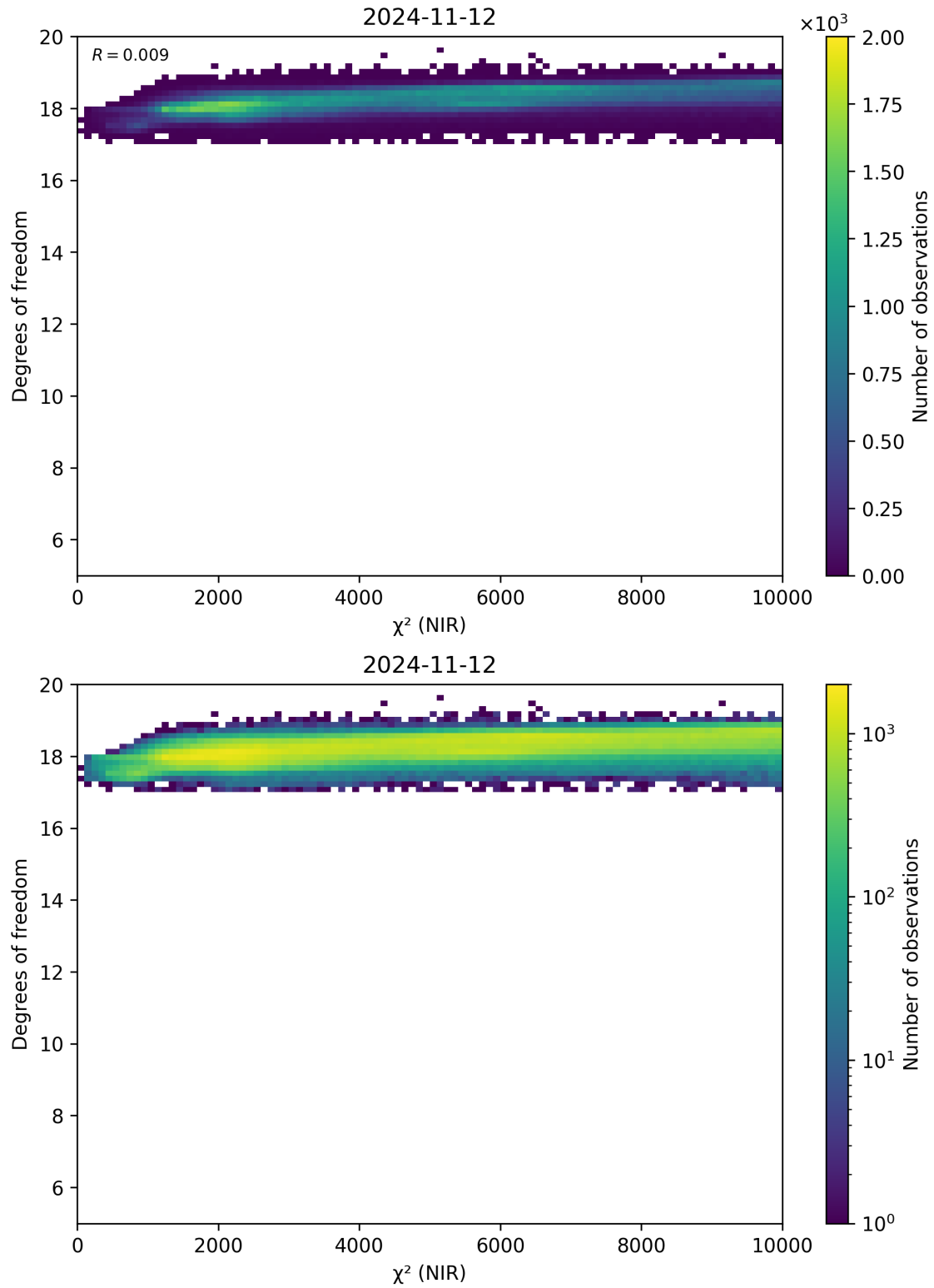
Figure 44: Scatter density plot of “ \chi^2 (NIR)” against “Degrees of freedom” for 2024-11-11 to 2024-11-13.
