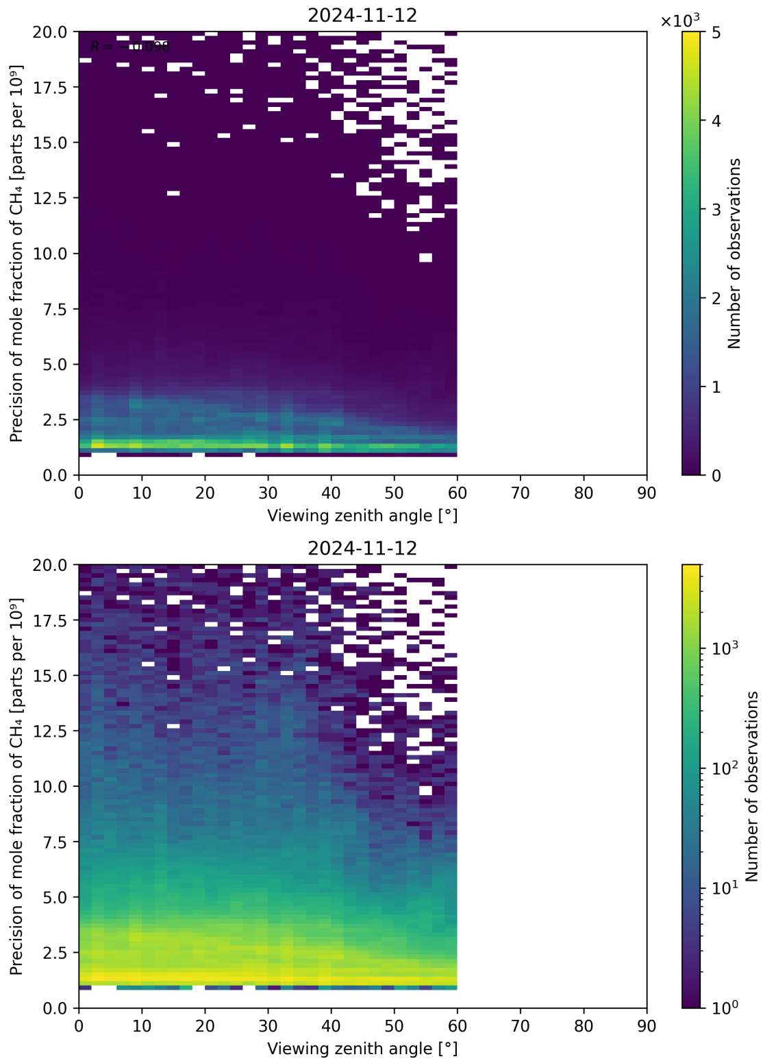
Figure 112: Scatter density plot of “Viewing zenith angle” against “Precision of mole fraction of CH 4 ” for 2024-11-11 to 2024-11-13.
