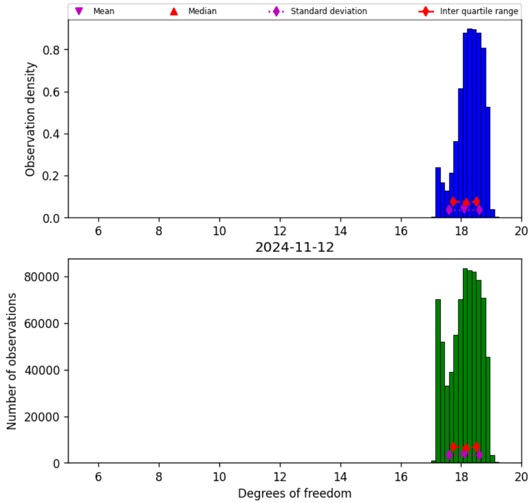
Figure 30: Histogram of “Degrees of freedom” for 2024-11-11 to 2024-11-13
