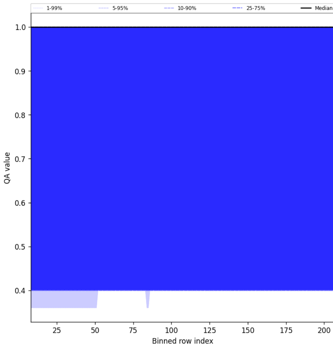
Figure 33: Along track statistics of “QA value” for 2024-11-11 to 2024-11-13
