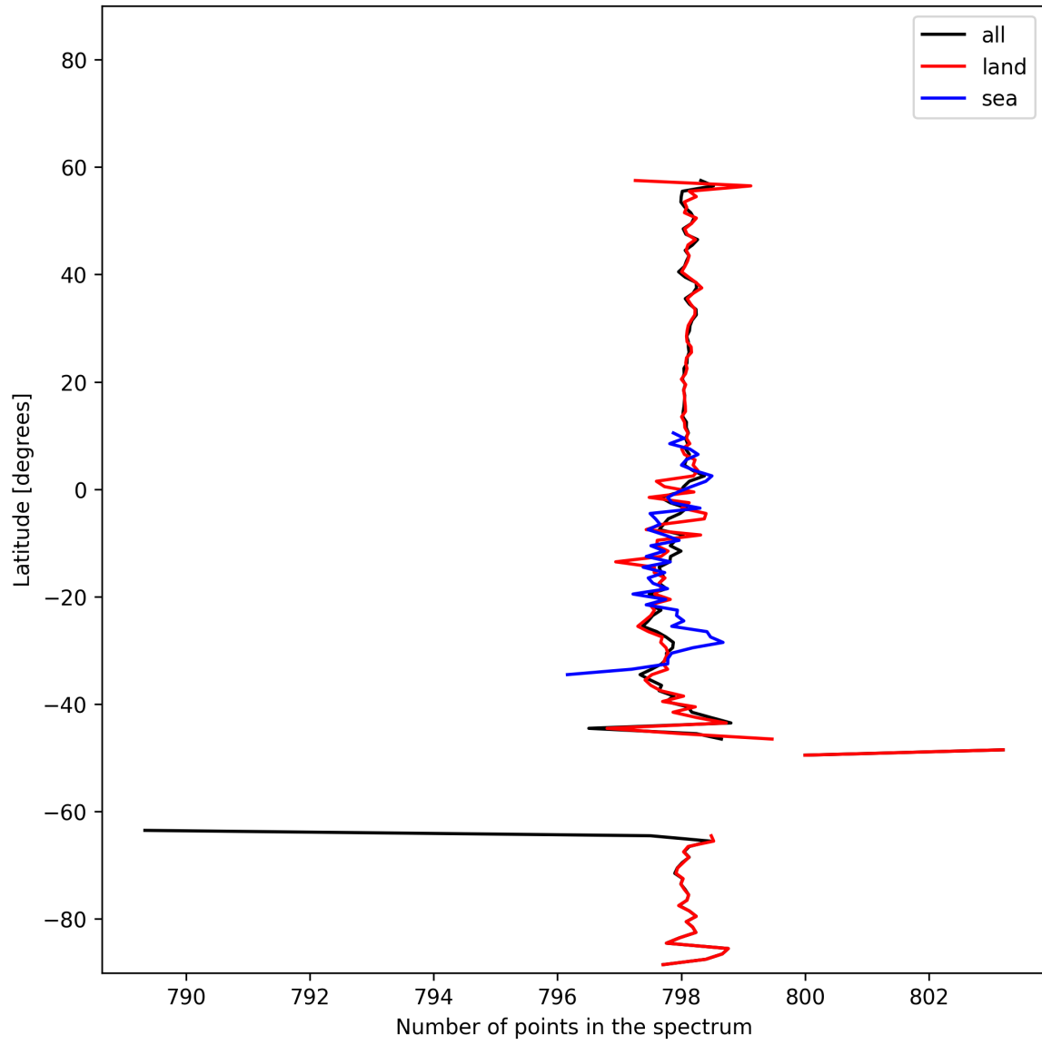
Figure 15: Zonal average of “Number of points in the spectrum” for 2024-11-11 to 2024-11-13.
