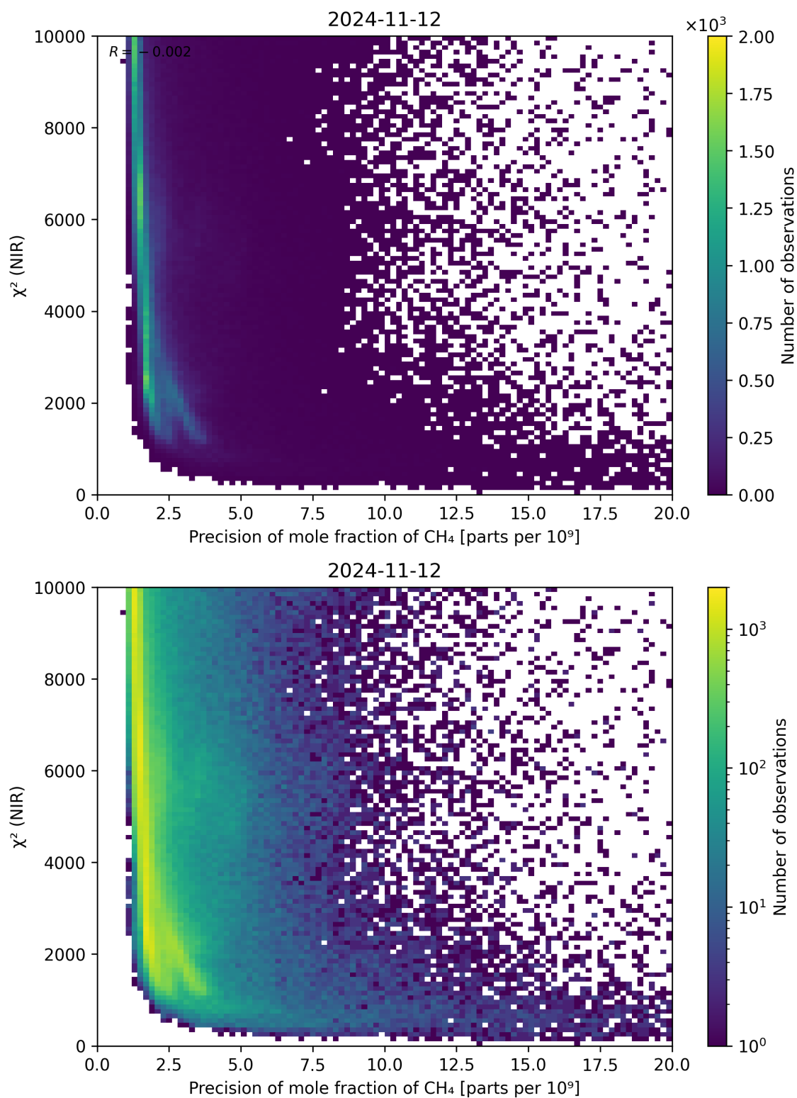
Figure 78: Scatter density plot of “Precision of mole fraction of CH 4 ” against “ \chi^2 (NIR)” for 2024-11-11 to 2024-11-13.
