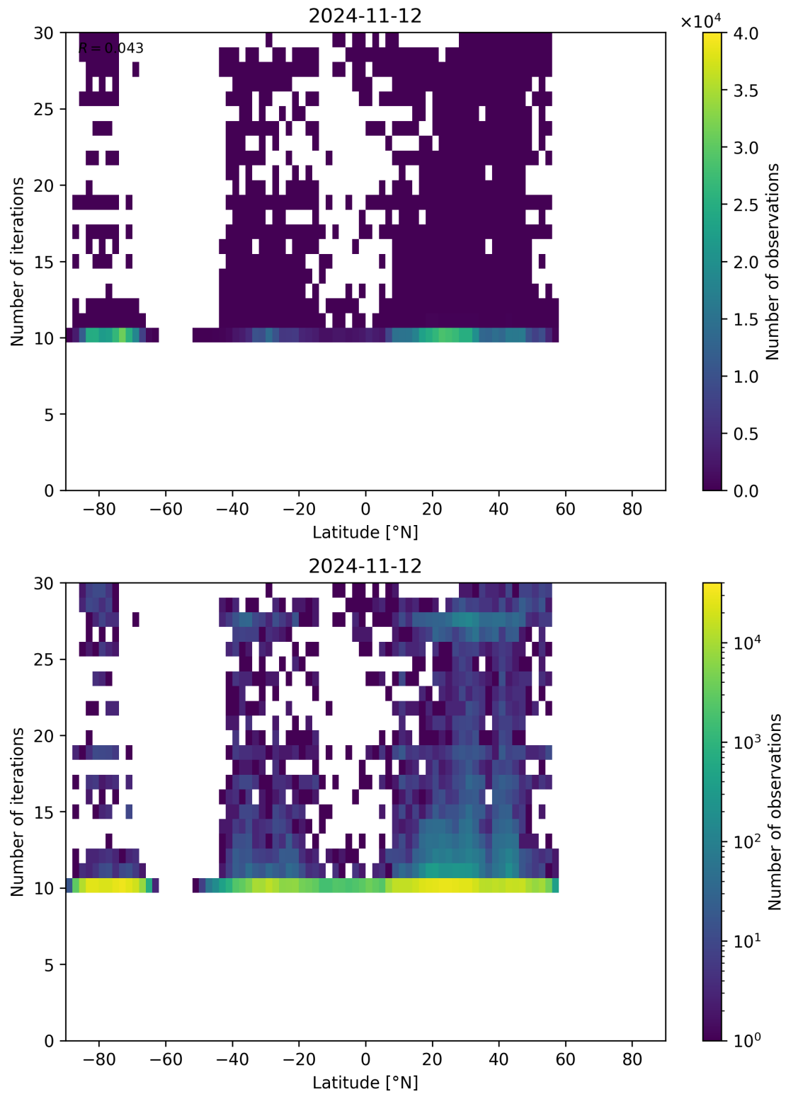
Figure 60: Scatter density plot of “Latitude” against “Number of iterations” for 2024-11-11 to 2024-11-13.
