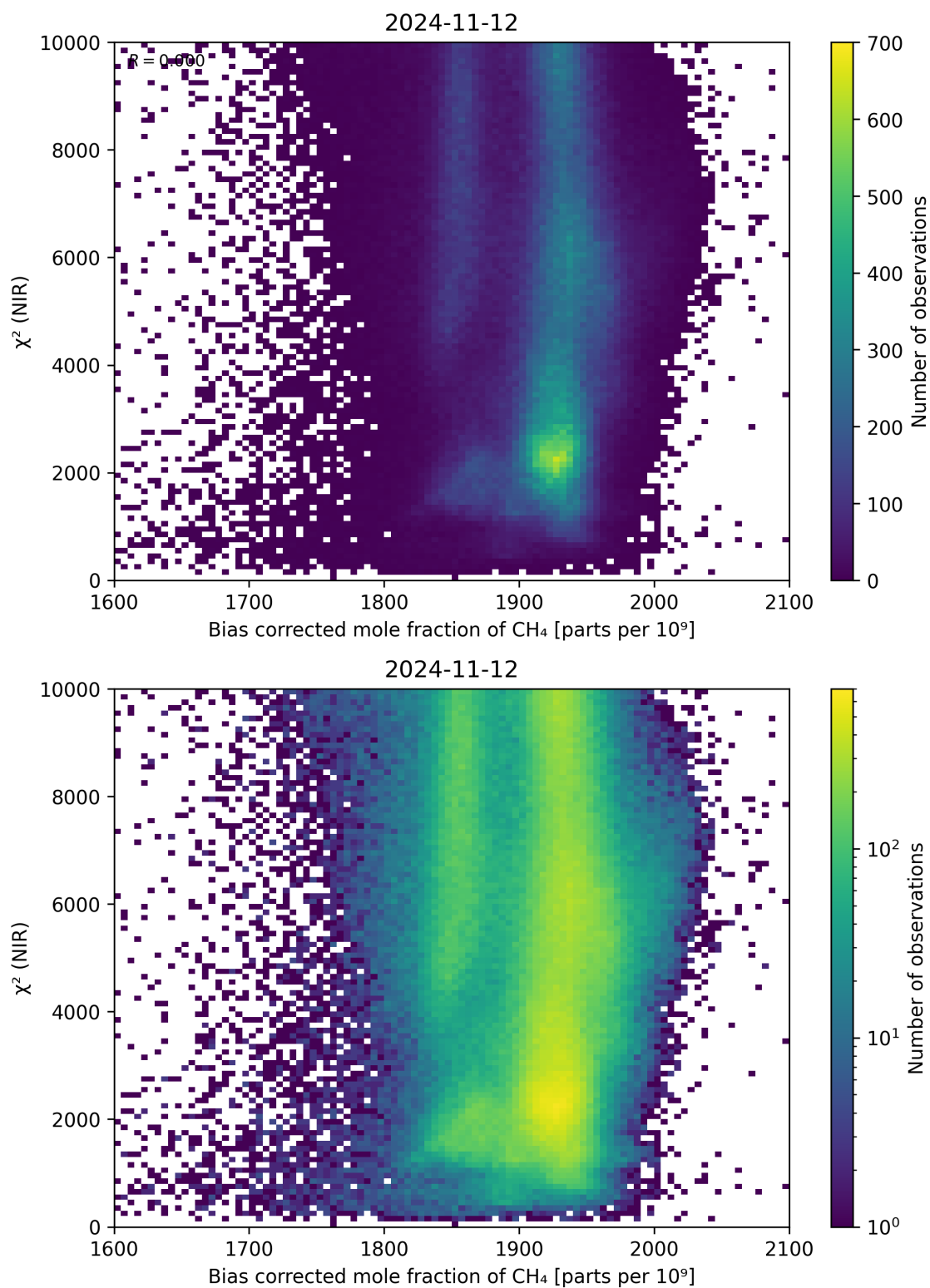
Figure 63: Scatter density plot of “Bias corrected mole fraction of CH 4 ” against “ \chi^2 (NIR)” for 2024-11-11 to 2024-11-13.
