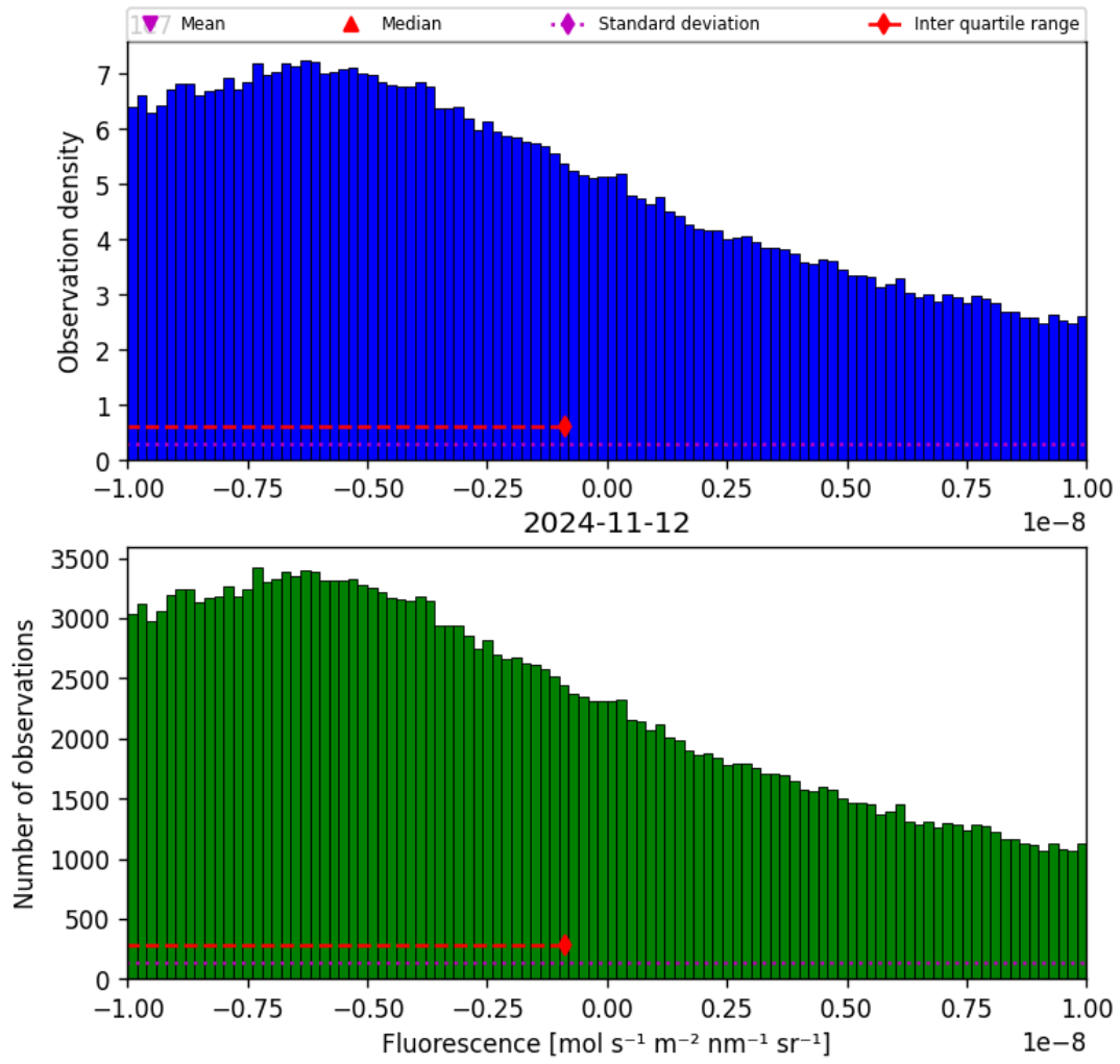
Figure 32: Histogram of “Fluorescence” for 2024-11-11 to 2024-11-13
