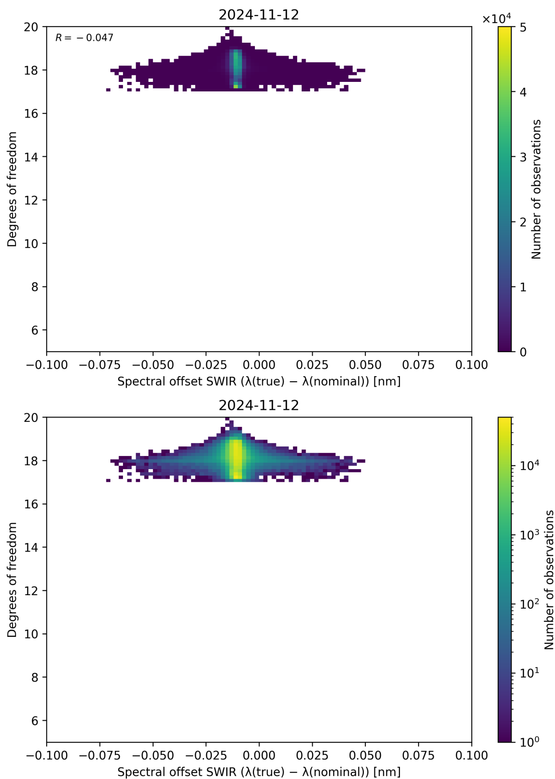
Figure 119: Scatter density plot of “Spectral offset SWIR ( \lambda_{\text{true}} - \lambda_{\text{nominal}} )” against “Degrees of freedom” for 2024-11-11 to 2024-11-13.
