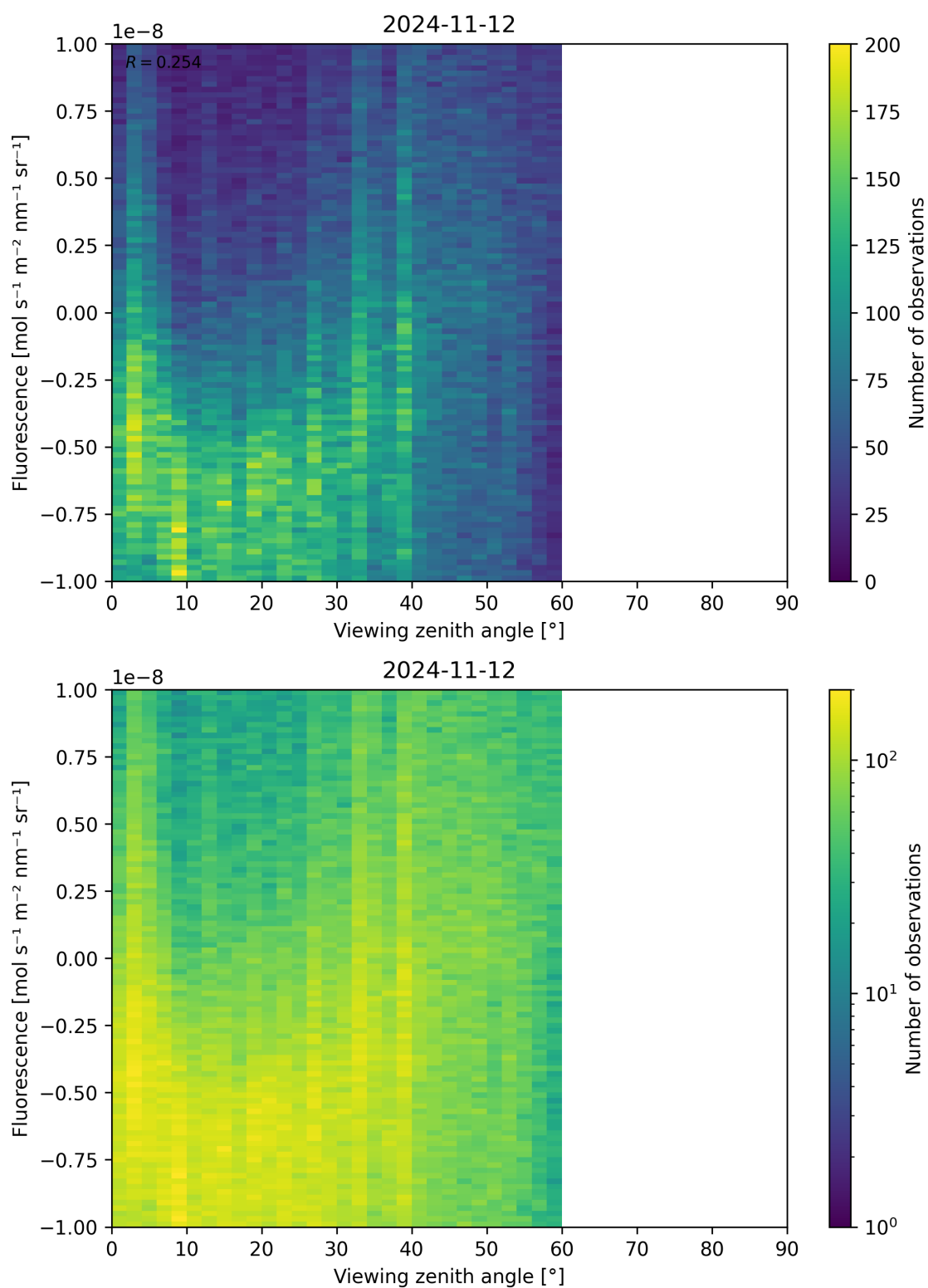
Figure 108: Scatter density plot of “Viewing zenith angle” against “Fluorescence” for 2024-11-11 to 2024-11-13.
