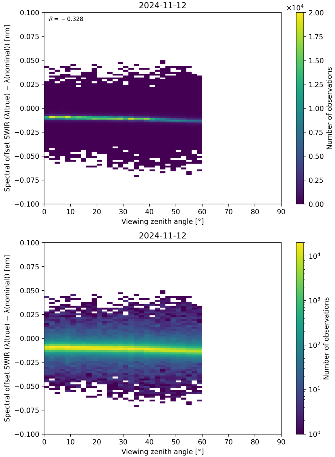
Figure 116: Scatter density plot of “Viewing zenith angle” against “Spectral offset SWIR ( \lambda_{\text{true}} - \lambda_{\text{nominal}} )” for 2024-11-11 to 2024-11-13.
