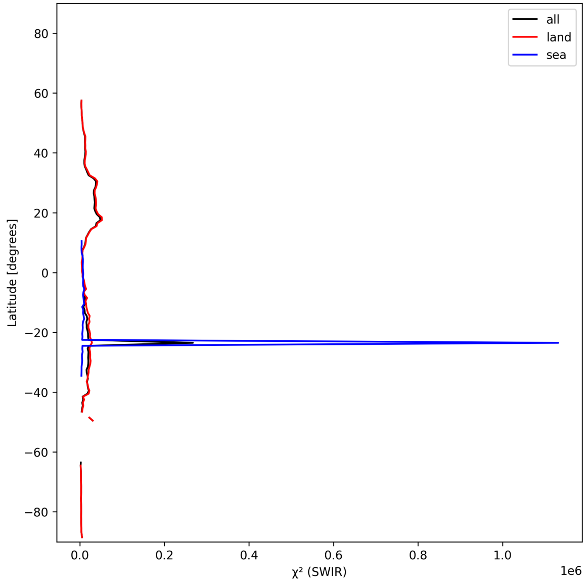
Figure 17: Zonal average of “ \chi^2 (SWIR)” for 2024-11-11 to 2024-11-13.
