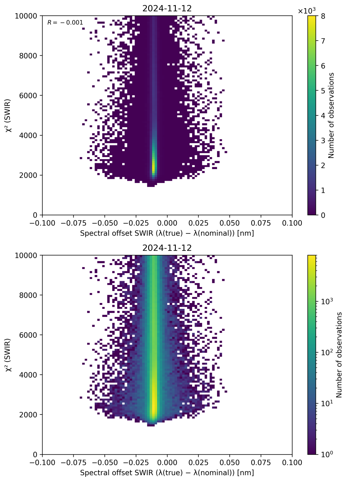
Figure 118: Scatter density plot of “Spectral offset SWIR ( \lambda_{\text{true}} - \lambda_{\text{nominal}} )” against “ \chi^2 (SWIR)” for 2024-11-11 to 2024-11-13.
