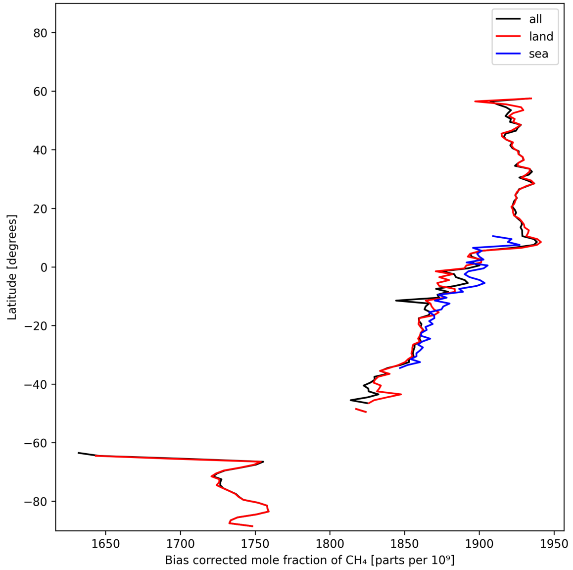
Figure 14: Zonal average of “Bias corrected mole fraction of CH 4 ” for 2024-11-11 to 2024-11-13.
