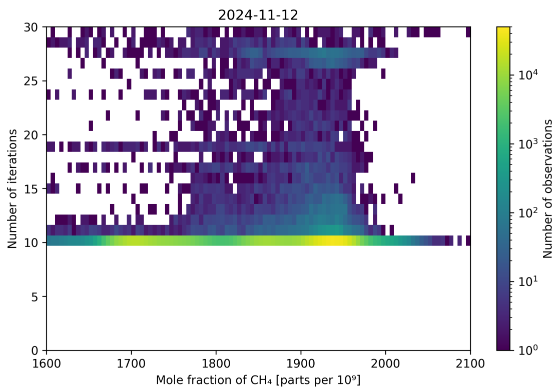
Figure 76: Scatter density plot of “Mole fraction of CH 4 ” against “Number of iterations” for 2024-11-11 to 2024-11-13.
