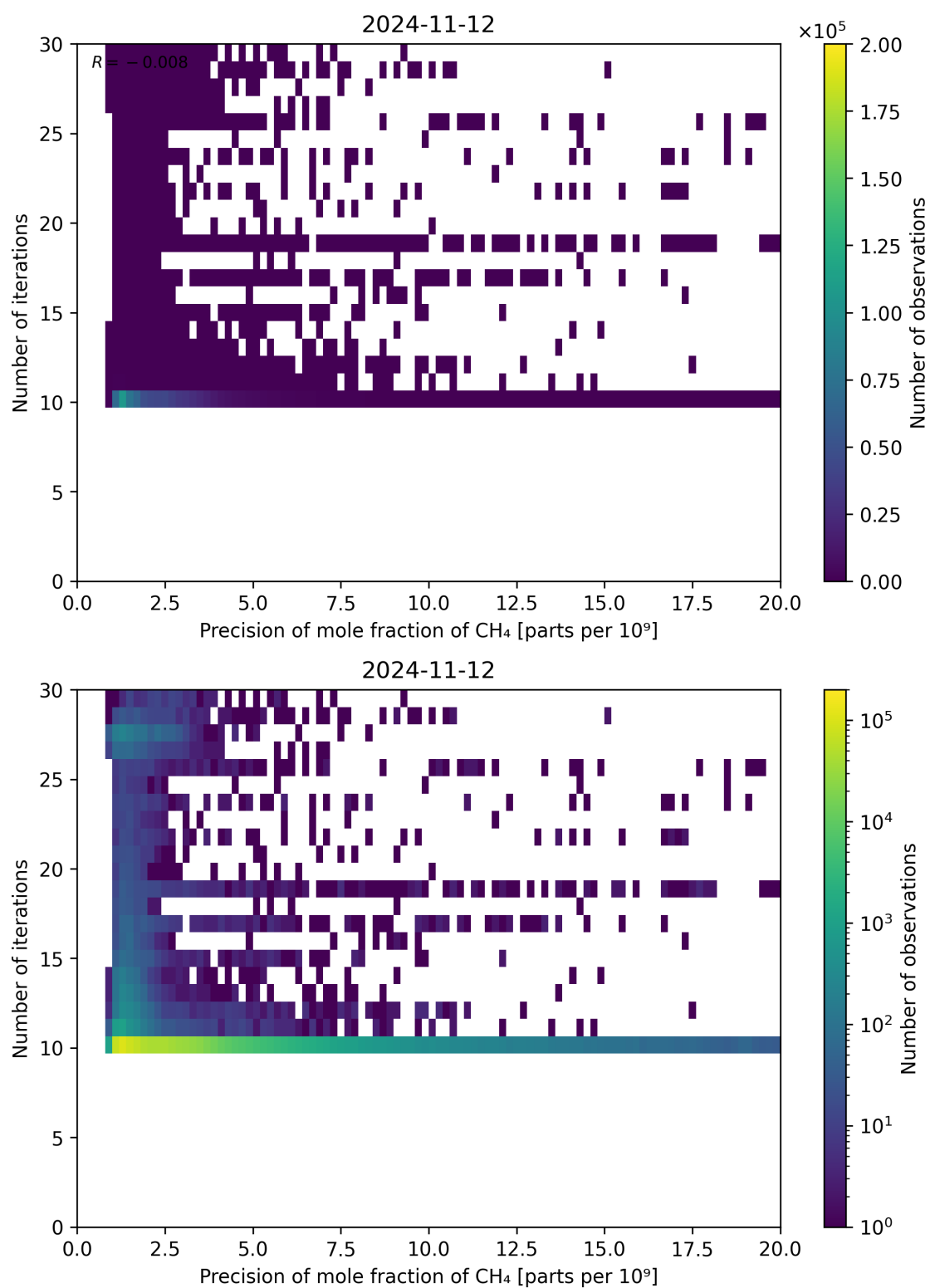
Figure 83: Scatter density plot of “Precision of mole fraction of CH 4 ” against “Number of iterations” for 2024-11-11 to 2024-11-13.
