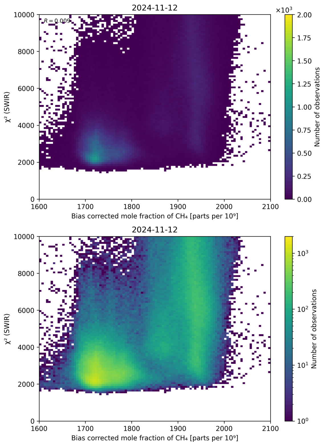
Figure 64: Scatter density plot of “Bias corrected mole fraction of \text{CH}_4 ” against “ \chi^2 (SWIR)” for 2024-11-11 to 2024-11-13.
