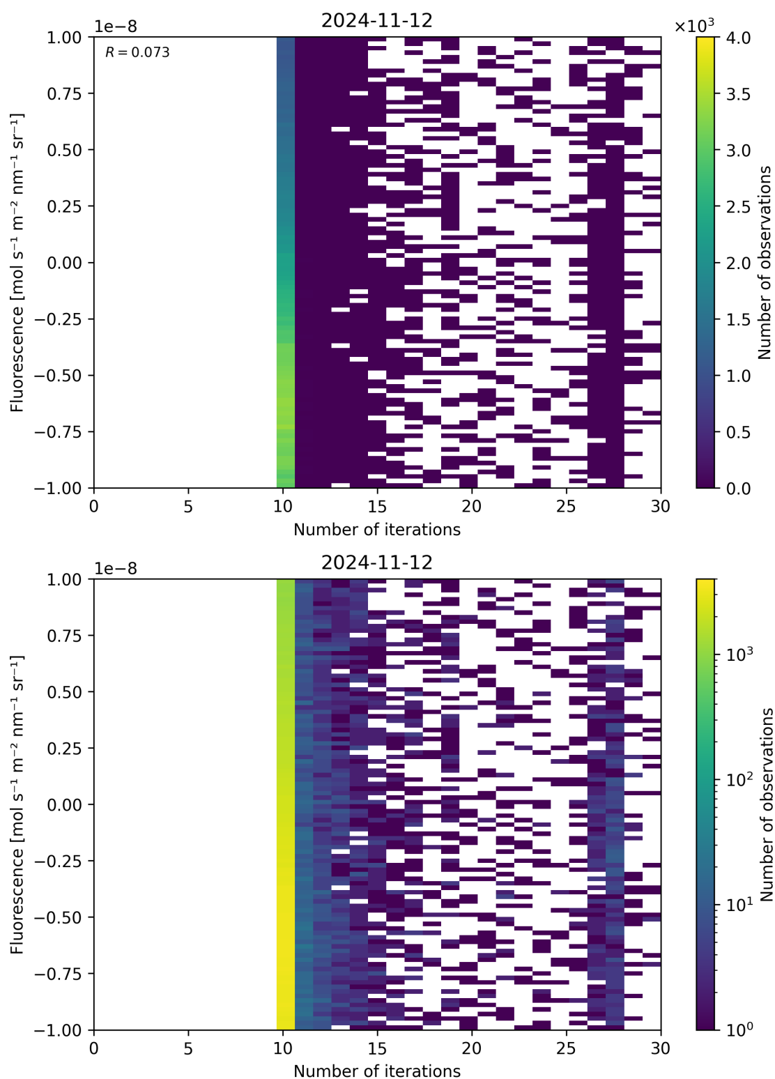
Figure 87: Scatter density plot of “Number of iterations” against “Fluorescence” for 2024-11-11 to 2024-11-13.
