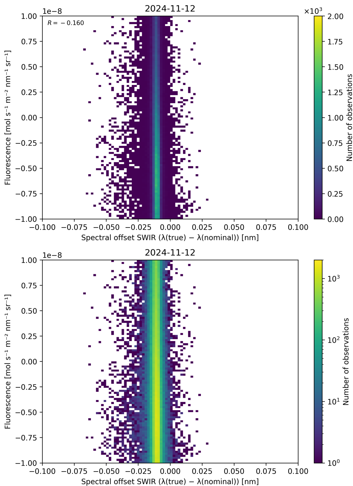
Figure 120: Scatter density plot of “Spectral offset SWIR ( \lambda_{\text{true}} - \lambda_{\text{nominal}} )” against “Fluorescence” for 2024-11-11 to 2024-11-13.
