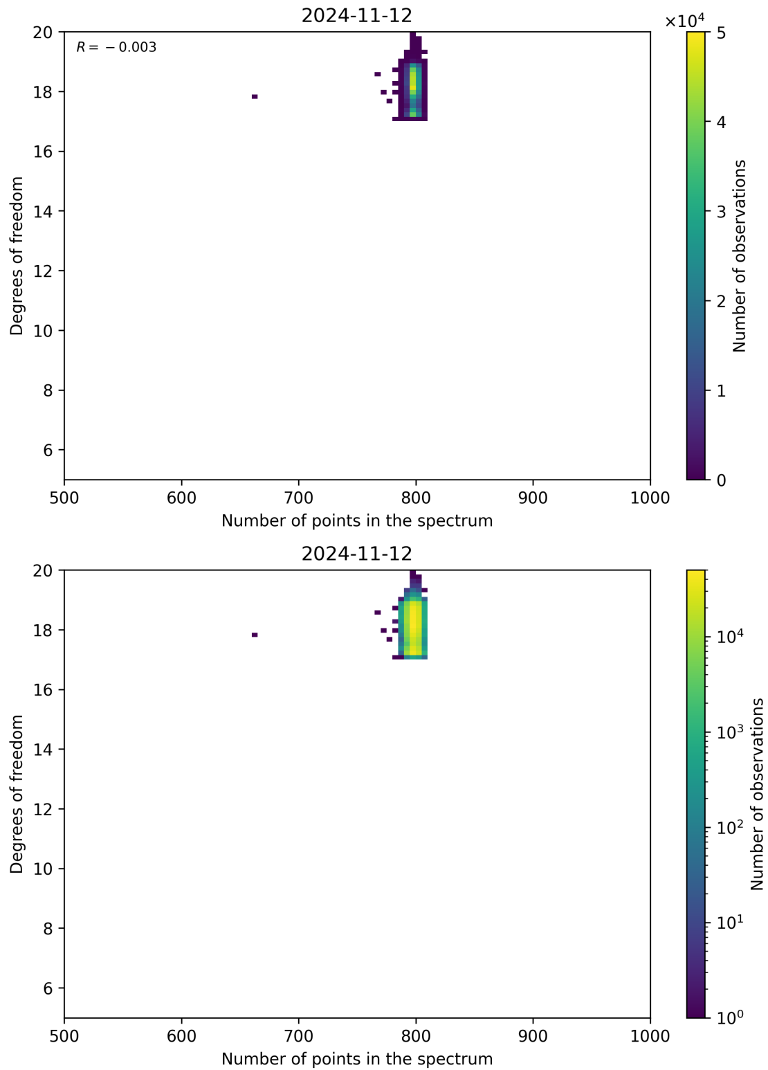
Figure 90: Scatter density plot of “Number of points in the spectrum” against “Degrees of freedom” for 2024-11-11 to 2024-11-13.
