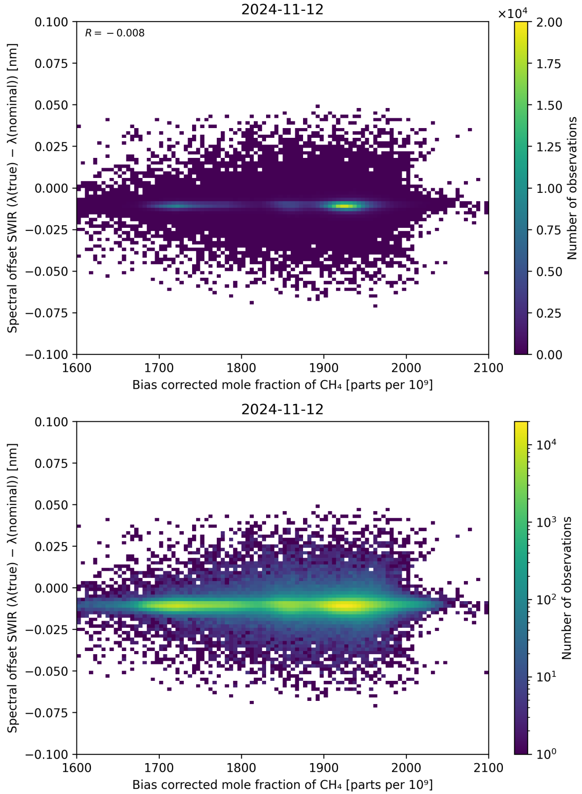
Figure 69: Scatter density plot of “Bias corrected mole fraction of \text{CH}_4 ” against “Spectral offset SWIR ( \lambda_{\text{true}} - \lambda_{\text{nominal}} )” for 2024-11-11 to 2024-11-13.
