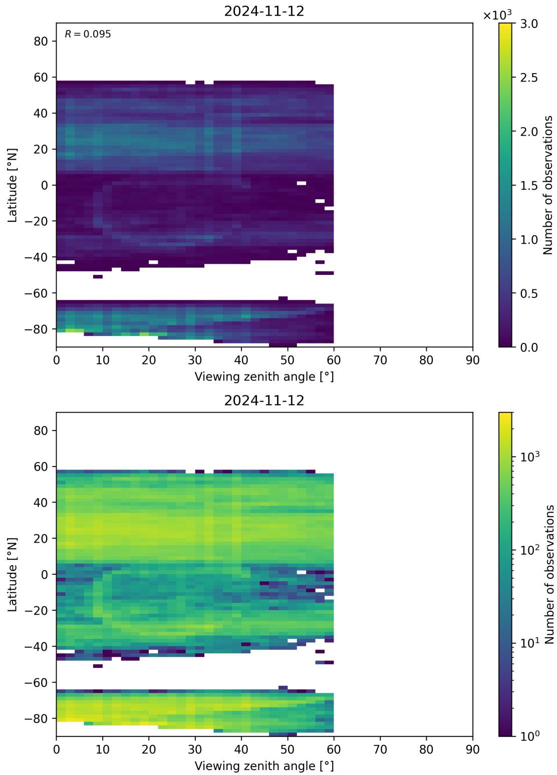
Figure 109: Scatter density plot of “Viewing zenith angle” against “Latitude” for 2024-11-11 to 2024-11-13.
