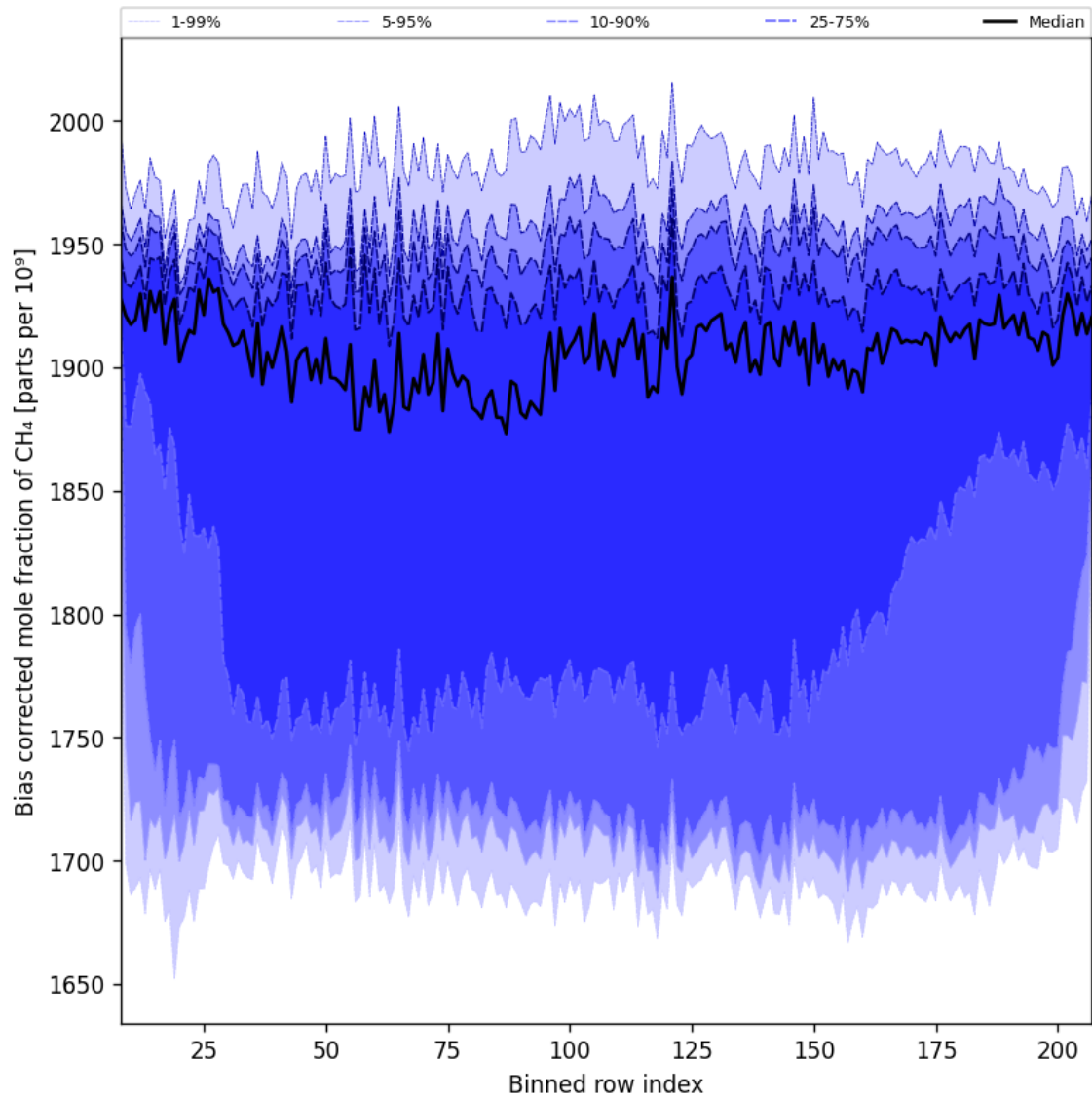
Figure 36: Along track statistics of “Bias corrected mole fraction of CH 4 ” for 2024-11-11 to 2024-11-13
