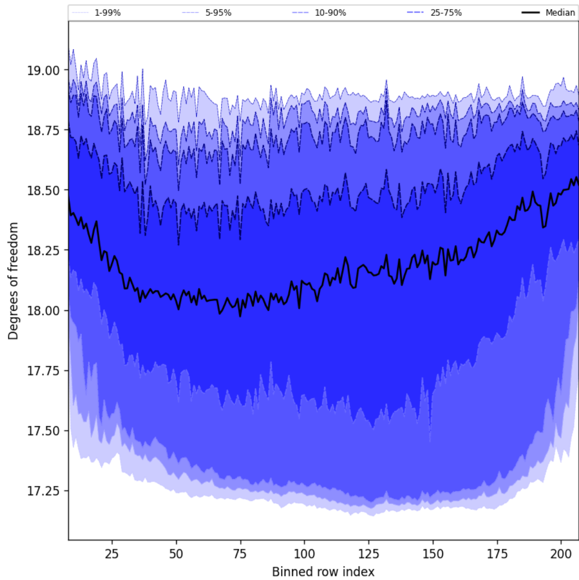
Figure 41: Along track statistics of “Degrees of freedom” for 2024-11-11 to 2024-11-13
