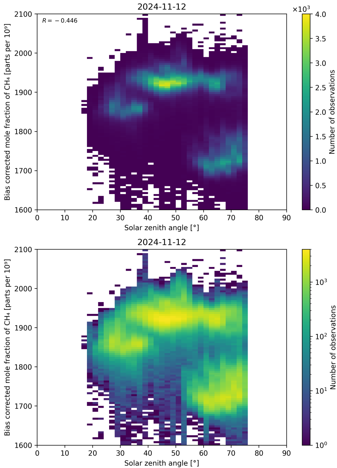
Figure 100: Scatter density plot of “Solar zenith angle” against “Bias corrected mole fraction of CH 4 ” for 2024-11-11 to 2024-11-13.
