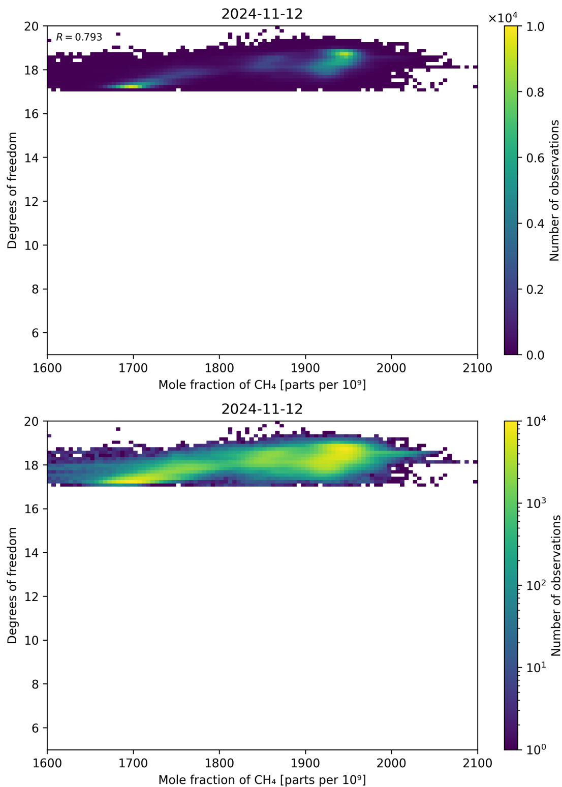
Figure 72: Scatter density plot of “Mole fraction of CH 4 ” against “Degrees of freedom” for 2024-11-11 to 2024-11-13.
