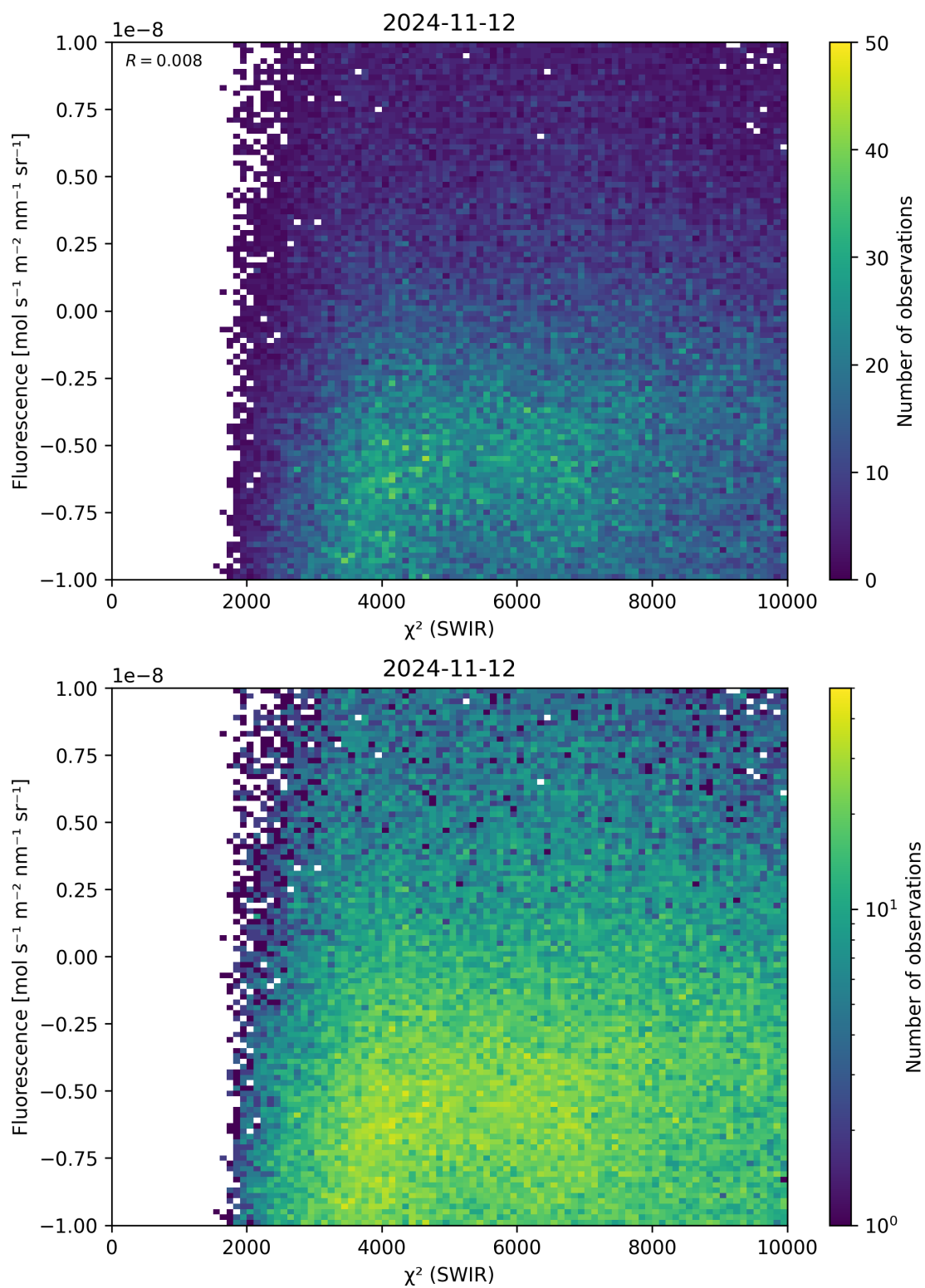
Figure 49: Scatter density plot of “ \chi^2 (SWIR)” against “Fluorescence” for 2024-11-11 to 2024-11-13.
