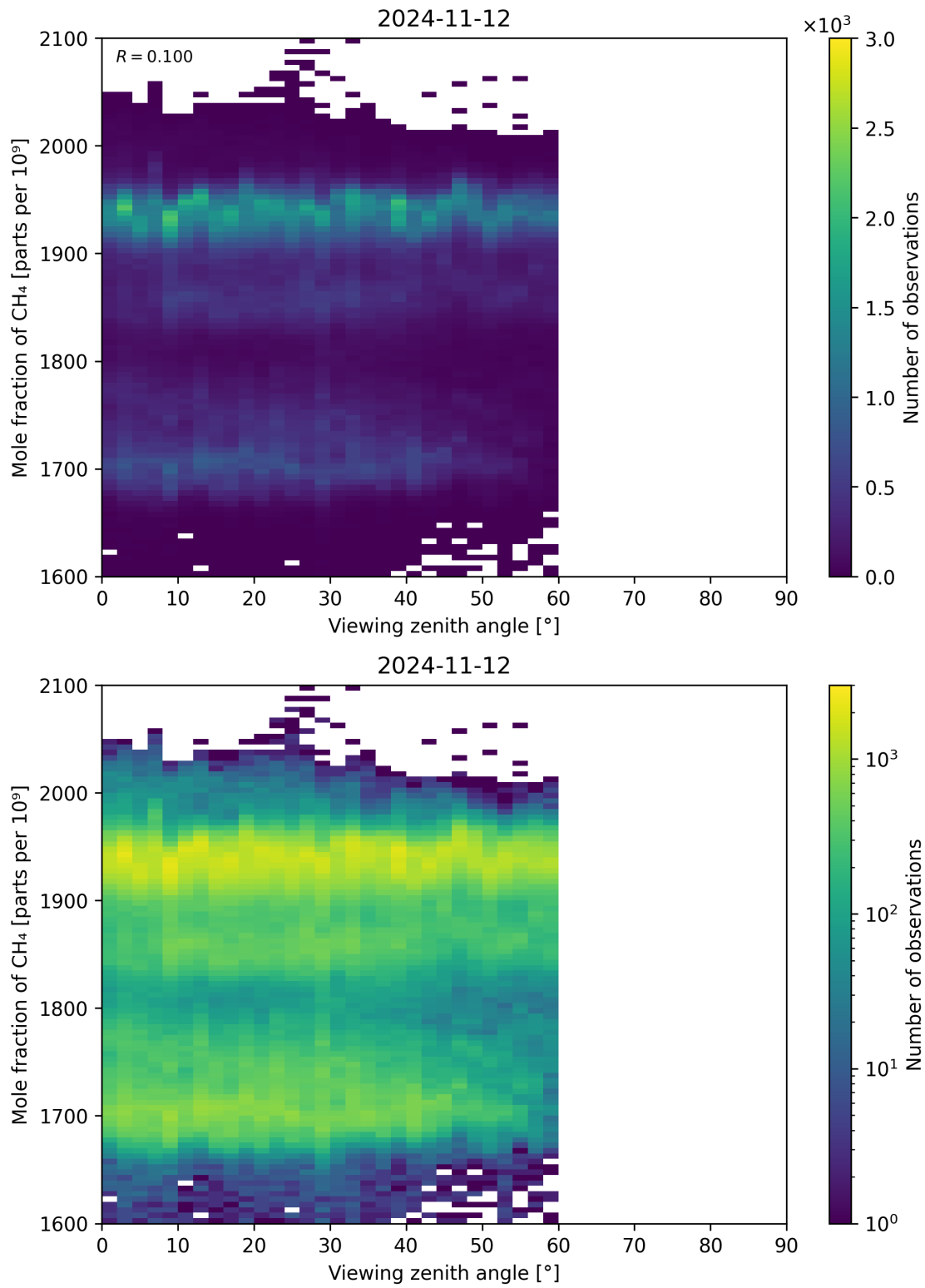
Figure 110: Scatter density plot of “Viewing zenith angle” against “Mole fraction of CH 4 ” for 2024-11-11 to 2024-11-13.
