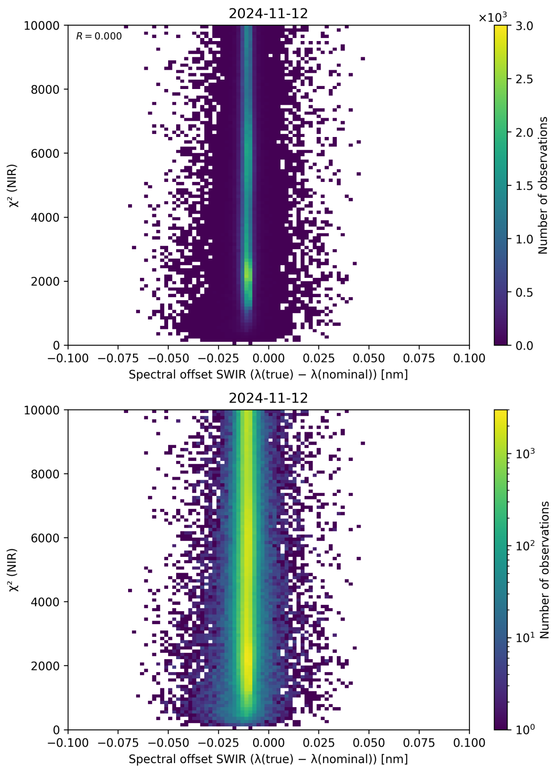
Figure 117: Scatter density plot of “Spectral offset SWIR ( \lambda_{\text{true}} - \lambda_{\text{nominal}} )” against “ \chi^2 (NIR)” for 2024-11-11 to 2024-11-13.
