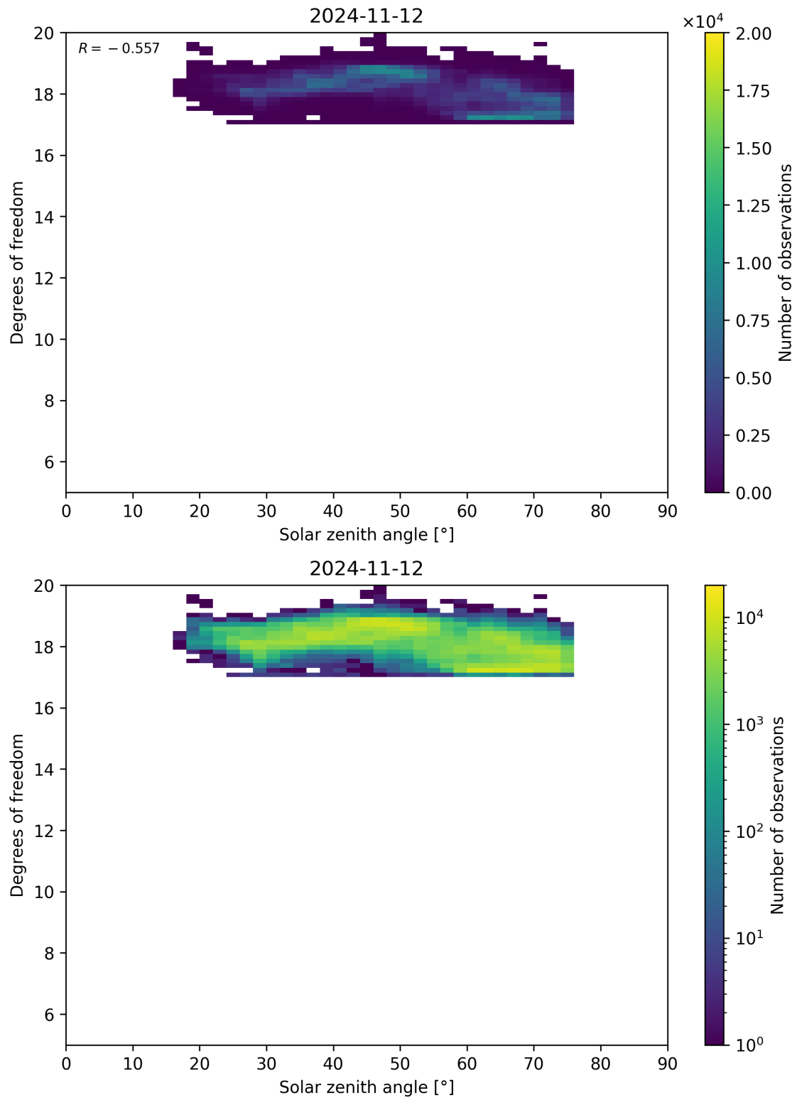
Figure 96: Scatter density plot of “Solar zenith angle” against “Degrees of freedom” for 2024-11-11 to 2024-11-13.
