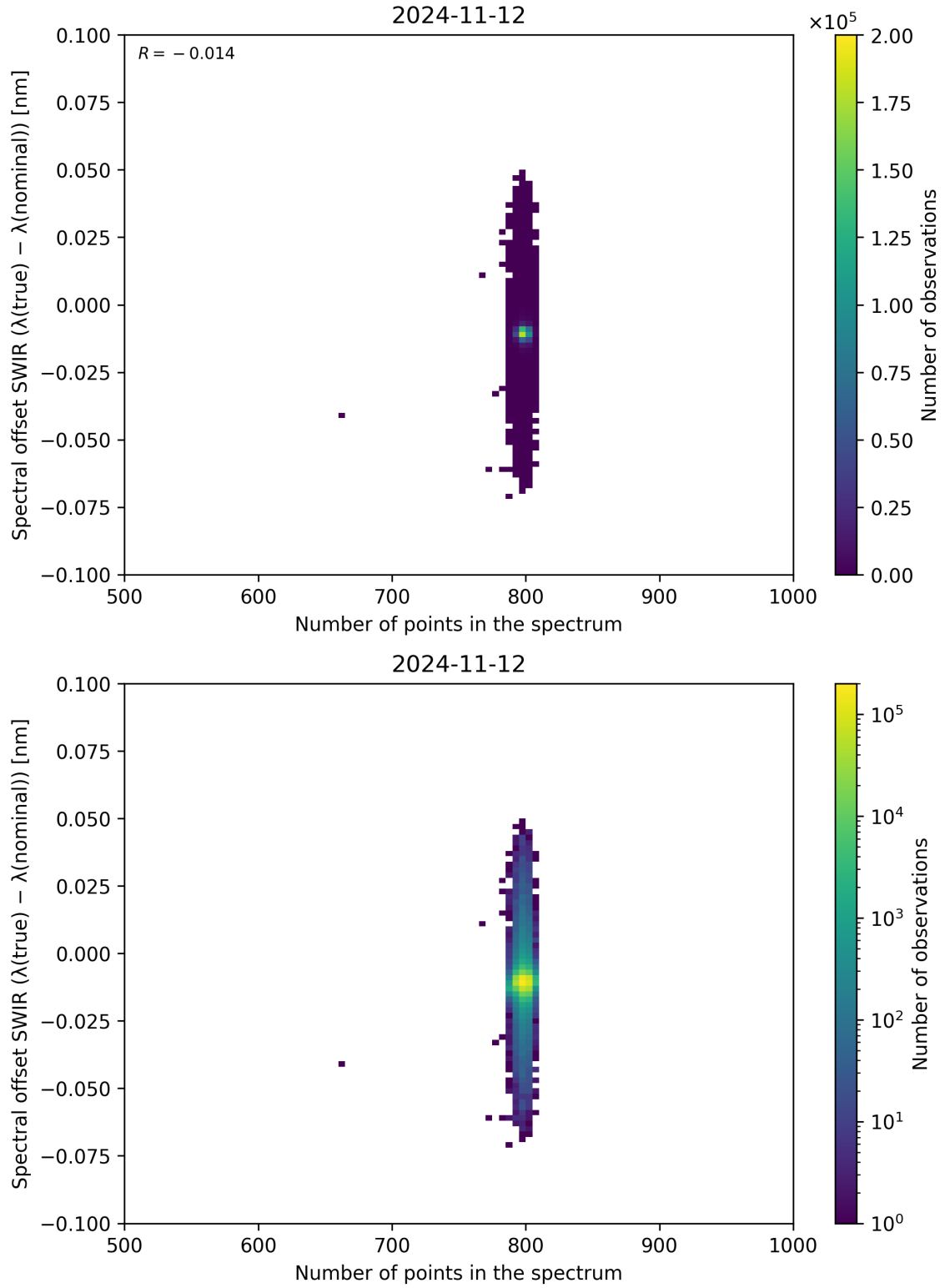
Figure 93: Scatter density plot of “Number of points in the spectrum” against “Spectral offset SWIR ( \lambda_{\text{true}} - \lambda_{\text{nominal}} )” for 2024-11-11 to 2024-11-13.
