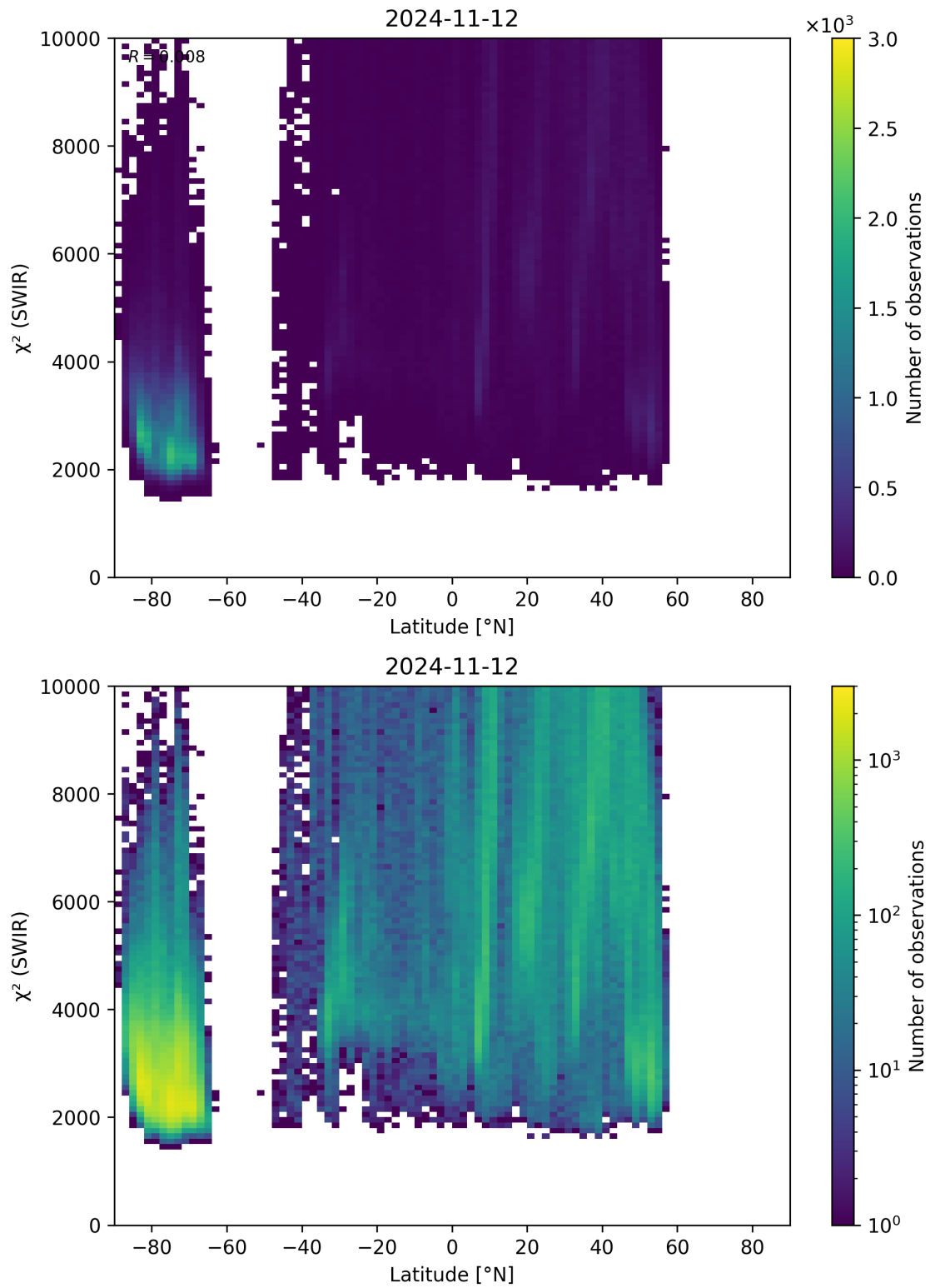
Figure 54: Scatter density plot of “Latitude” against “ \chi^2 (SWIR)” for 2024-11-11 to 2024-11-13.
