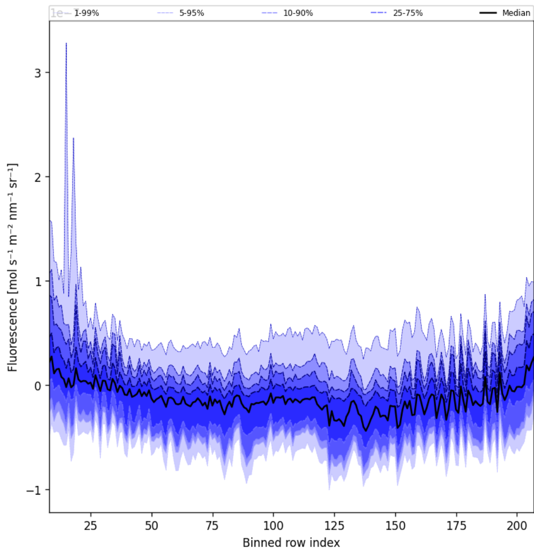
Figure 43: Along track statistics of “Fluorescence” for 2024-11-11 to 2024-11-13
