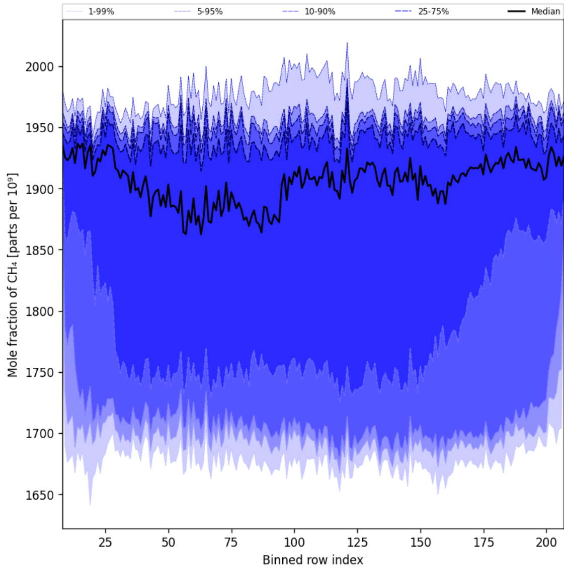
Figure 34: Along track statistics of “Mole fraction of CH 4 ” for 2024-11-11 to 2024-11-13
