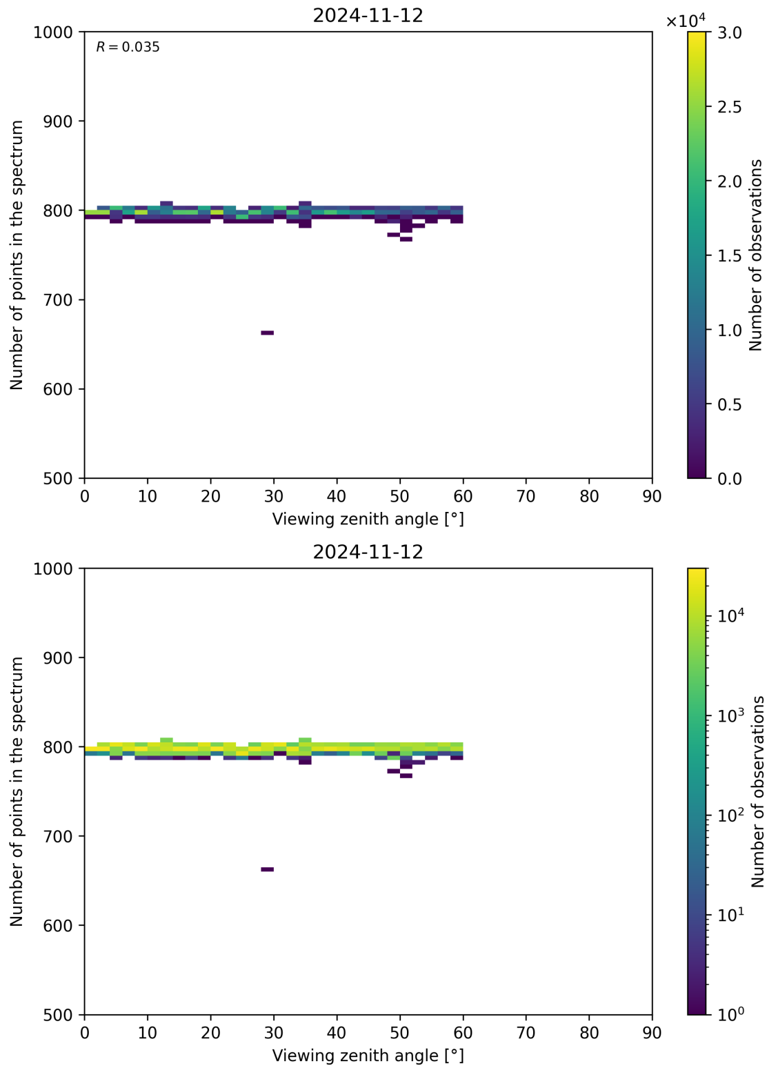
Figure 114: Scatter density plot of “Viewing zenith angle” against “Number of points in the spectrum” for 2024-11-11 to 2024-11-13.
