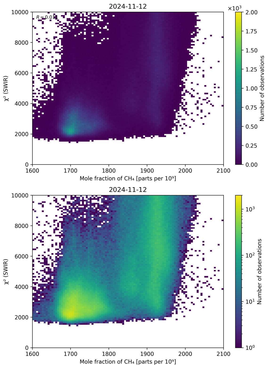
Figure 71: Scatter density plot of “Mole fraction of CH 4 ” against “ \chi^2 (SWIR)” for 2024-11-11 to 2024-11-13.
