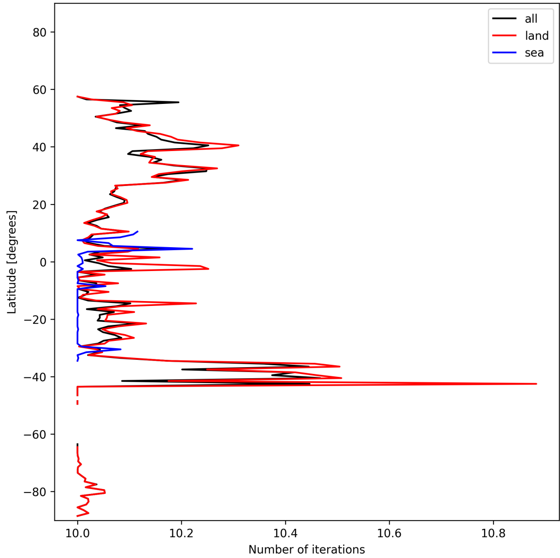
Figure 20: Zonal average of “Number of iterations” for 2024-11-11 to 2024-11-13.
