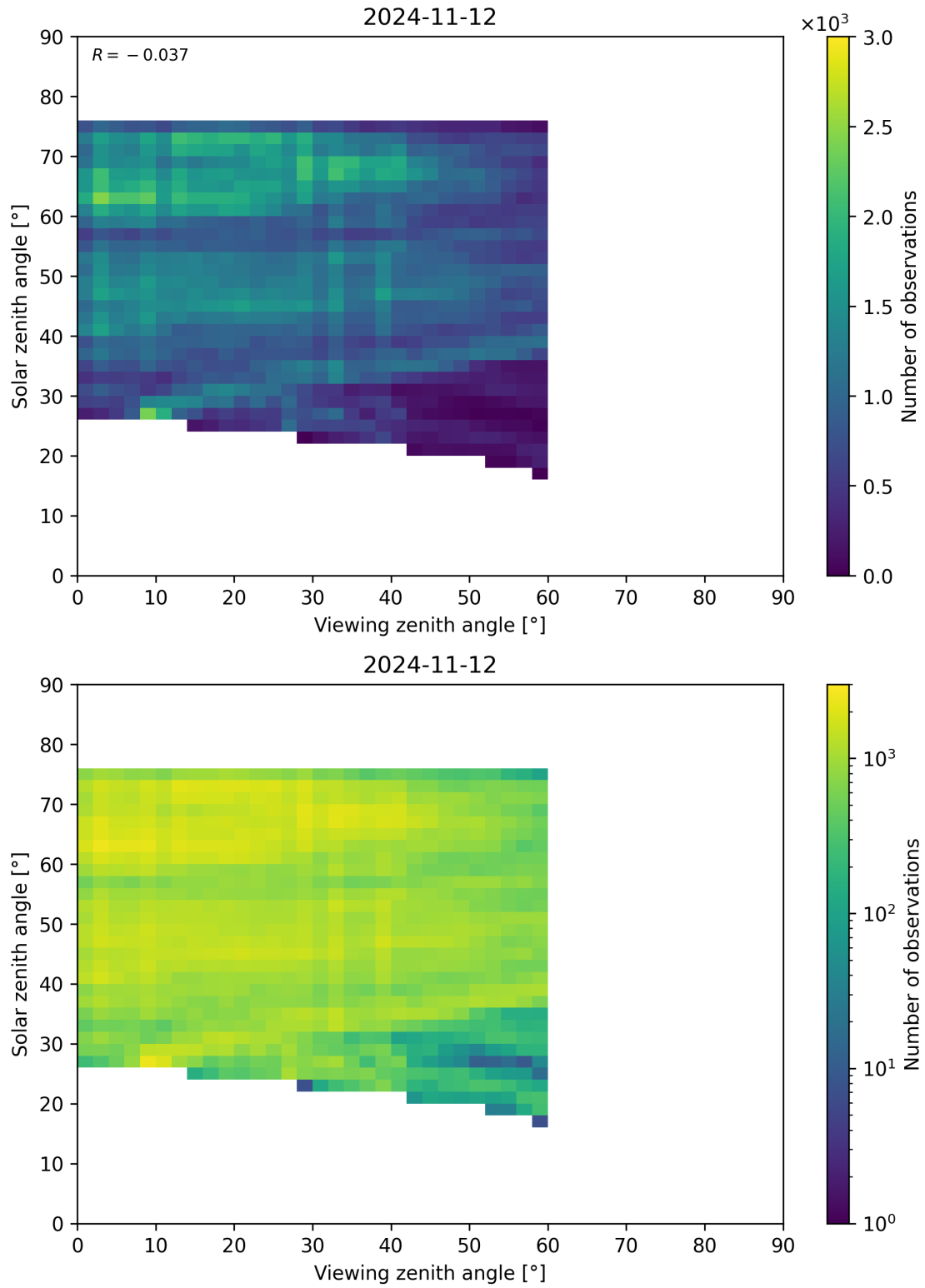
Figure 115: Scatter density plot of “Viewing zenith angle” against “Solar zenith angle” for 2024-11-11 to 2024-11-13.
