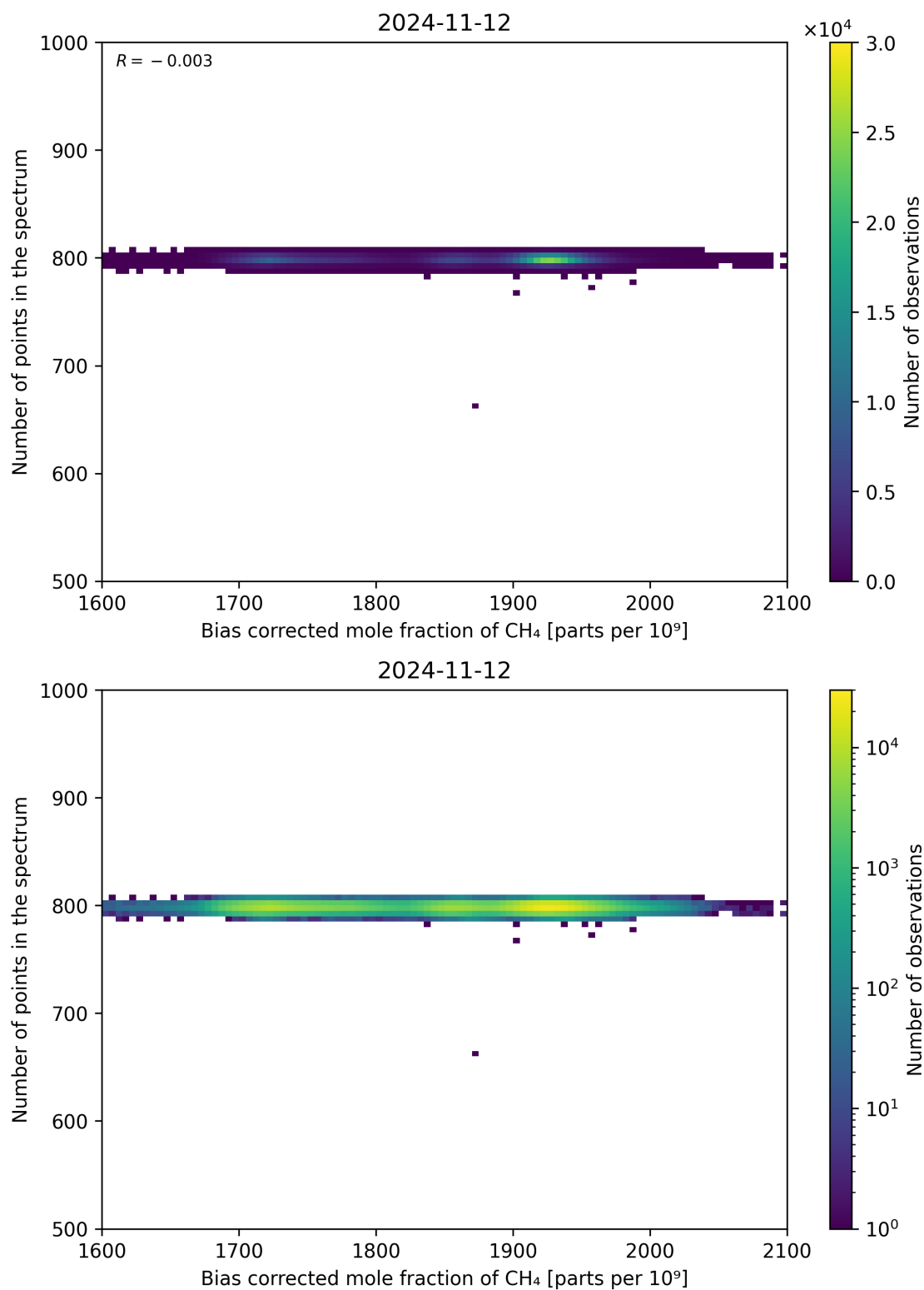
Figure 68: Scatter density plot of “Bias corrected mole fraction of \text{CH}_4 ” against “Number of points in the spectrum” for 2024-11-11 to 2024-11-13.
