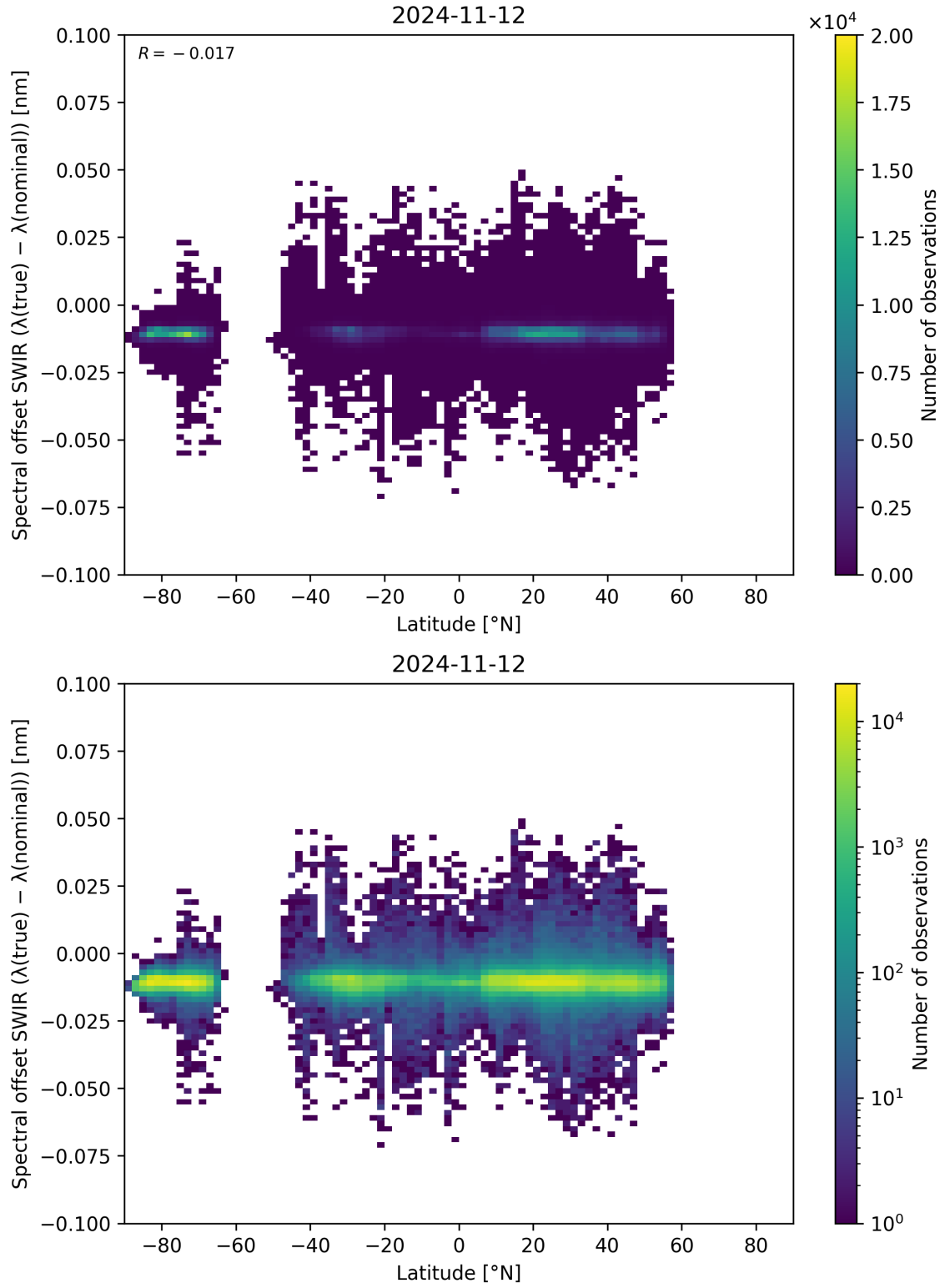
Figure 62: Scatter density plot of “Latitude” against “Spectral offset SWIR ( \lambda_{\text{true}} - \lambda_{\text{nominal}} )” for 2024-11-11 to 2024-11-13.
