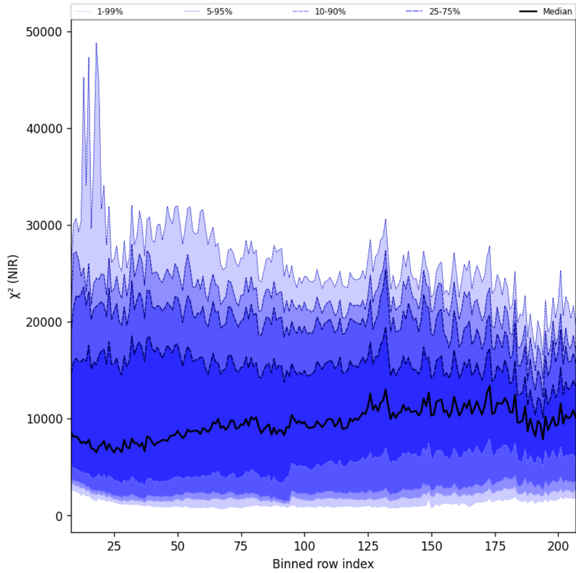
Figure 40: Along track statistics of “ \chi^2 (NIR)” for 2024-11-11 to 2024-11-13
