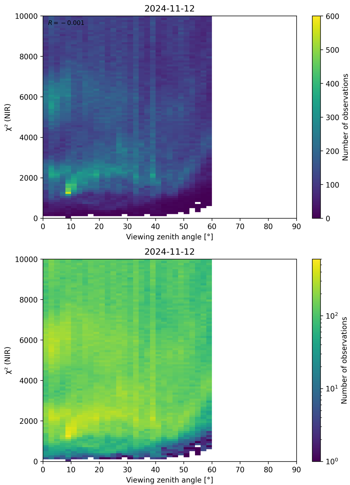
Figure 105: Scatter density plot of “Viewing zenith angle” against “ \chi^2 (NIR)” for 2024-11-11 to 2024-11-13.
