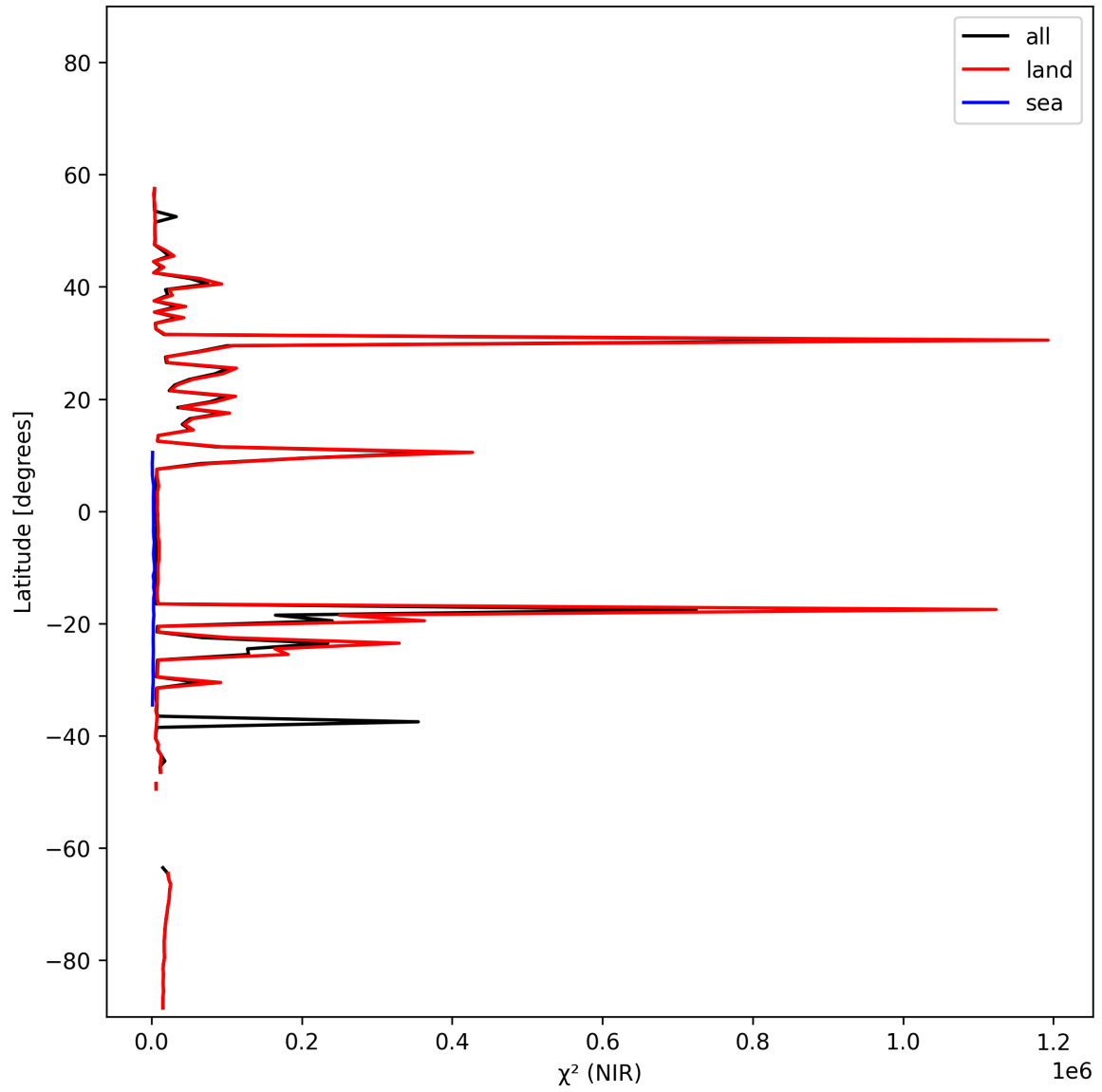
Figure 18: Zonal average of “ \chi^2 (NIR)” for 2024-11-11 to 2024-11-13.
