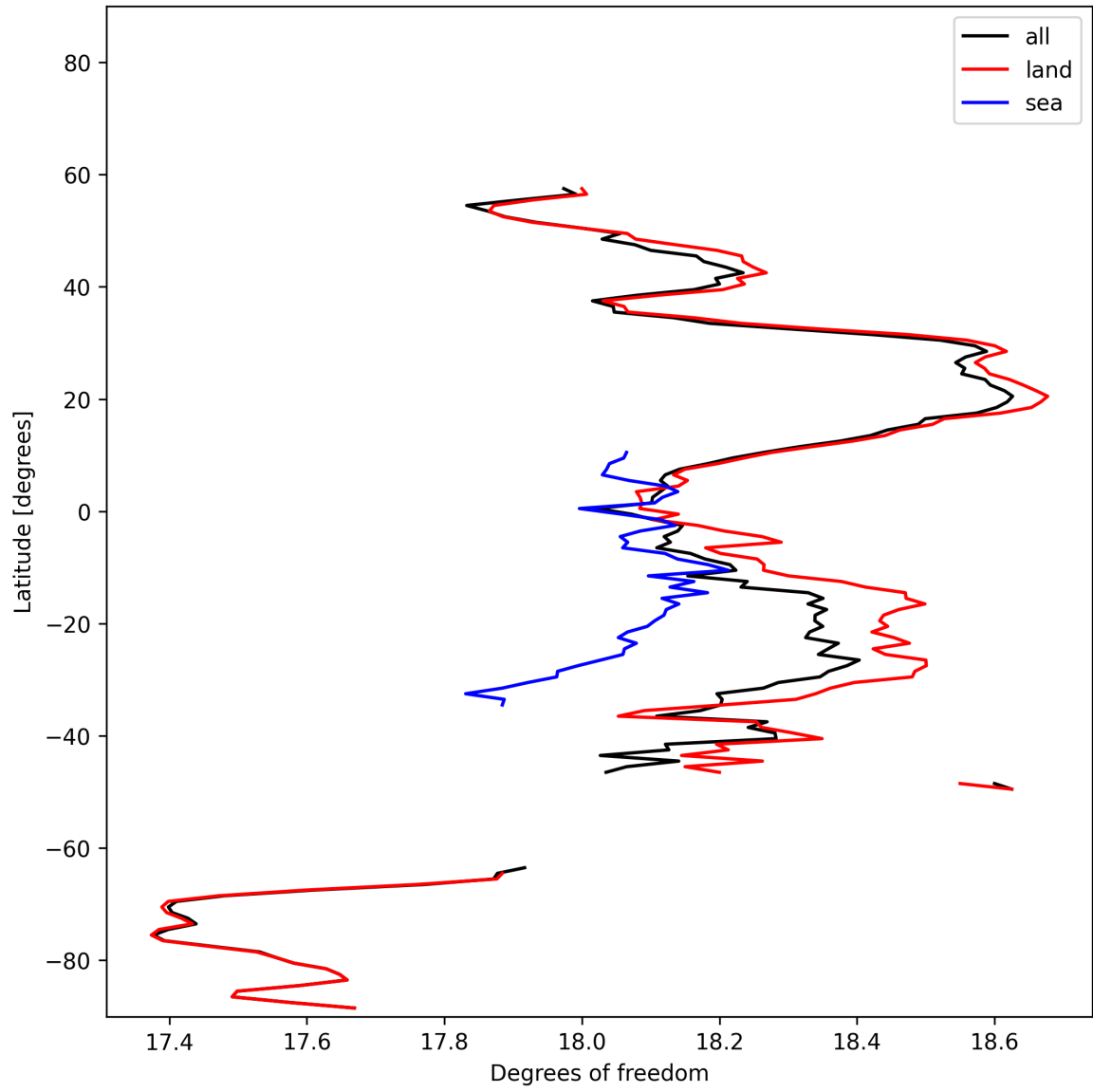
Figure 19: Zonal average of “Degrees of freedom” for 2024-11-11 to 2024-11-13.
