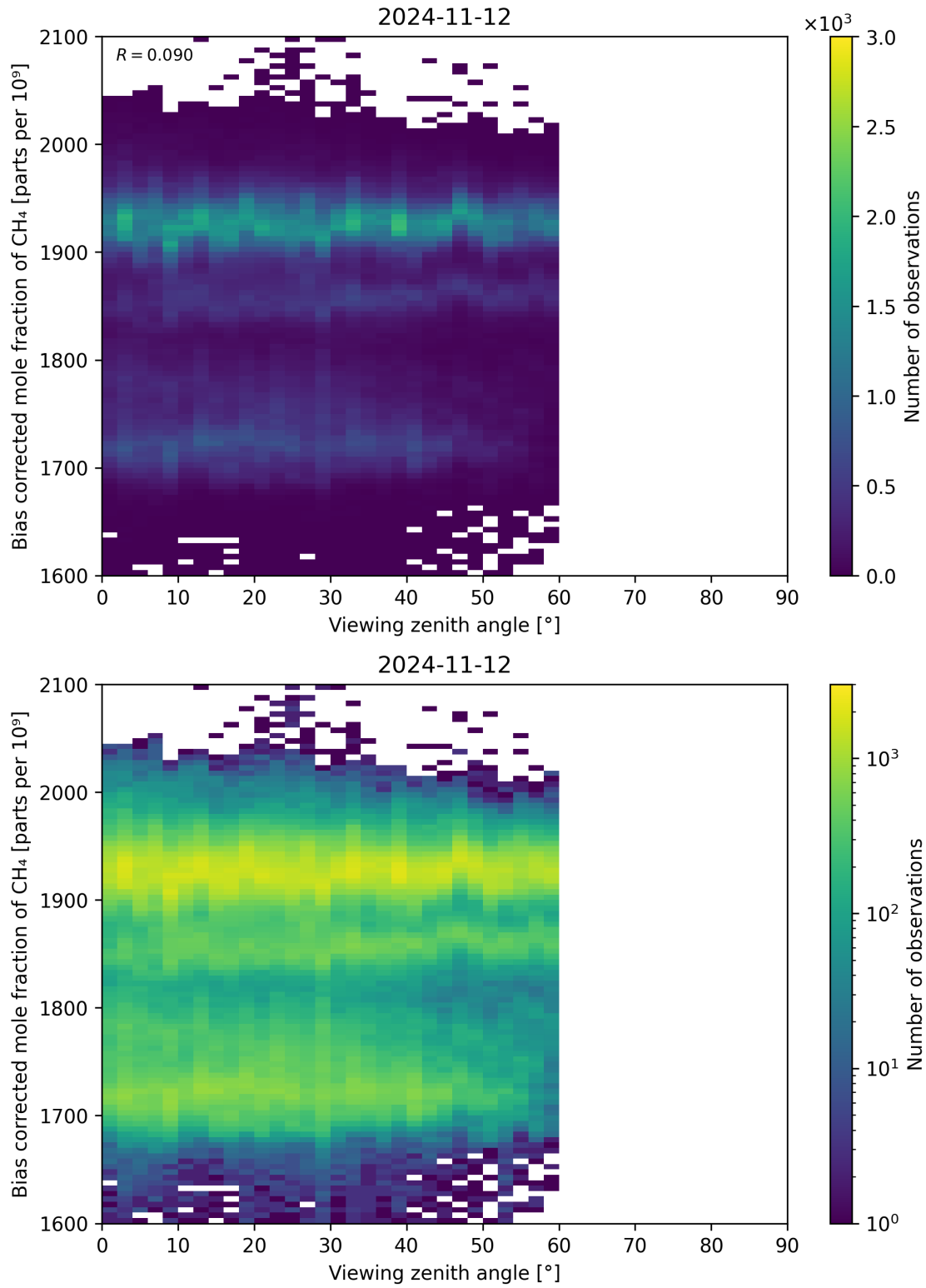
Figure 111: Scatter density plot of “Viewing zenith angle” against “Bias corrected mole fraction of CH 4 ” for 2024-11-11 to 2024-11-13.
