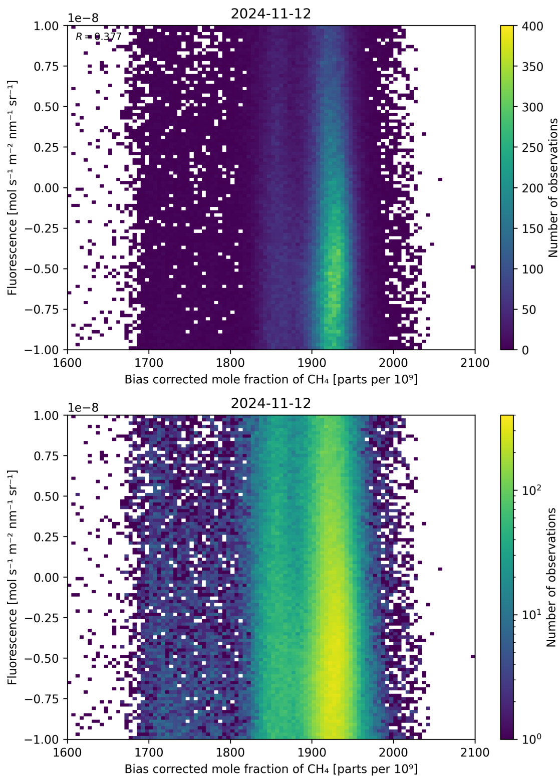
Figure 66: Scatter density plot of “Bias corrected mole fraction of \text{CH}_4 ” against “Fluorescence” for 2024-11-11 to 2024-11-13.
