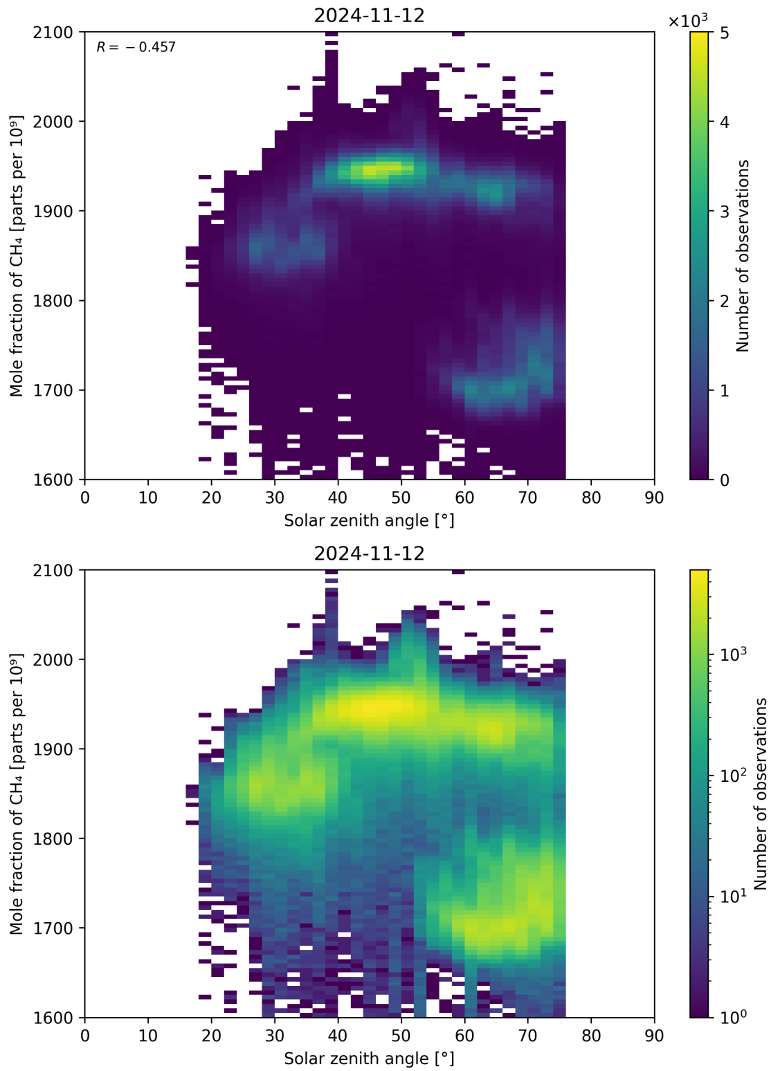
Figure 99: Scatter density plot of “Solar zenith angle” against “Mole fraction of \text{CH}_4 ” for 2024-11-11 to 2024-11-13.
