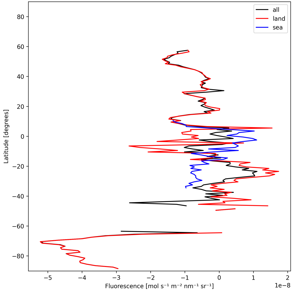
Figure 21: Zonal average of “Fluorescence” for 2024-11-11 to 2024-11-13.
