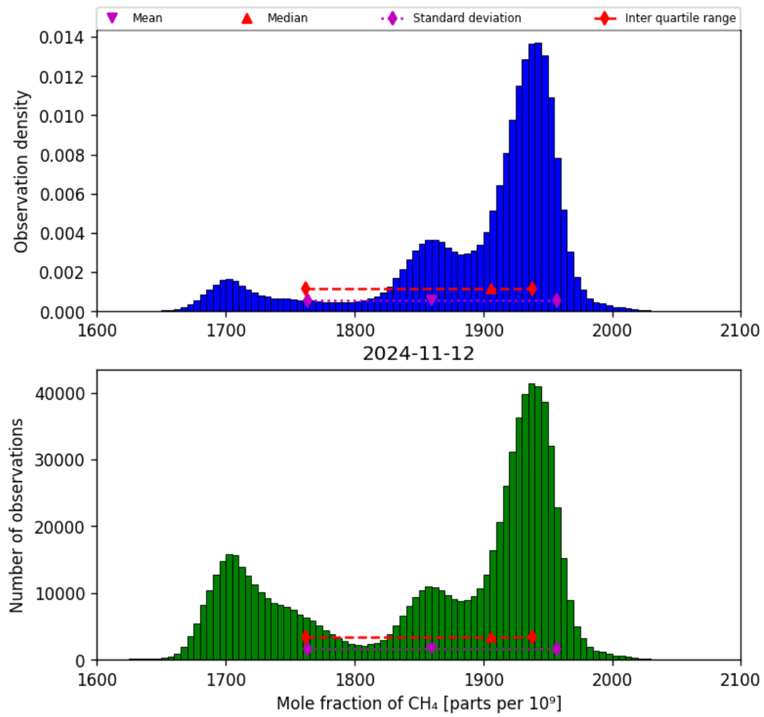
Figure 23: Histogram of “Mole fraction of CH 4 ” for 2024-11-11 to 2024-11-13
