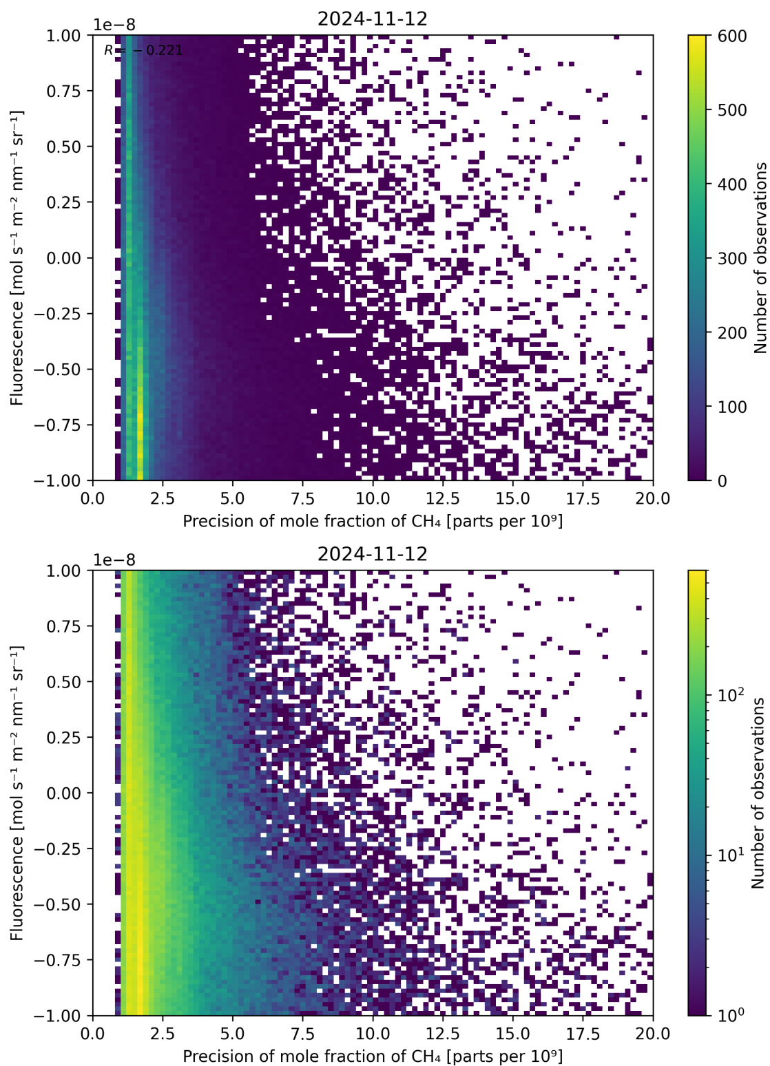
Figure 81: Scatter density plot of “Precision of mole fraction of CH 4 ” against “Fluorescence” for 2024-11-11 to 2024-11-13.
