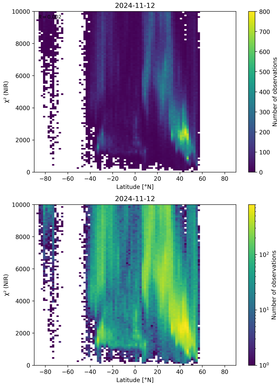
Figure 53: Scatter density plot of “Latitude” against “ \chi^2 (NIR)” for 2024-11-11 to 2024-11-13.
