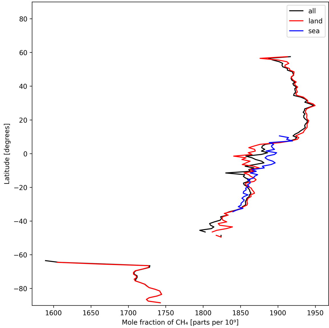
Figure 12: Zonal average of “Mole fraction of \text{CH}_4 ” for 2024-11-11 to 2024-11-13.
