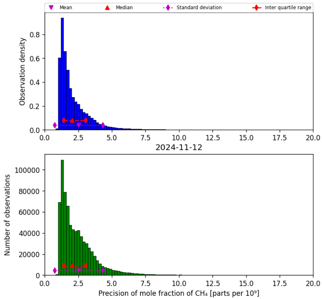
Figure 24: Histogram of “Precision of mole fraction of CH 4 ” for 2024-11-11 to 2024-11-13
