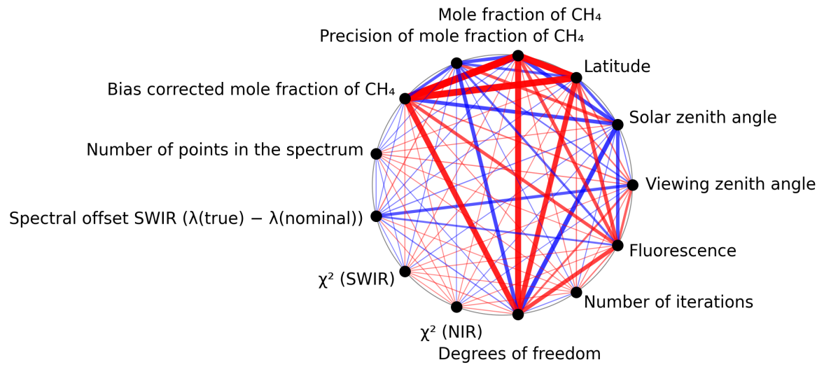
Figure 1: Map of correlation graph for 2024-11-11 to 2024-11-13.
