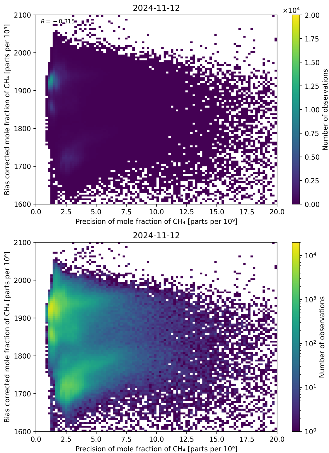
Figure 82: Scatter density plot of “Precision of mole fraction of CH 4 ” against “Bias corrected mole fraction of CH 4 ” for 2024-11-11 to 2024-11-13.
