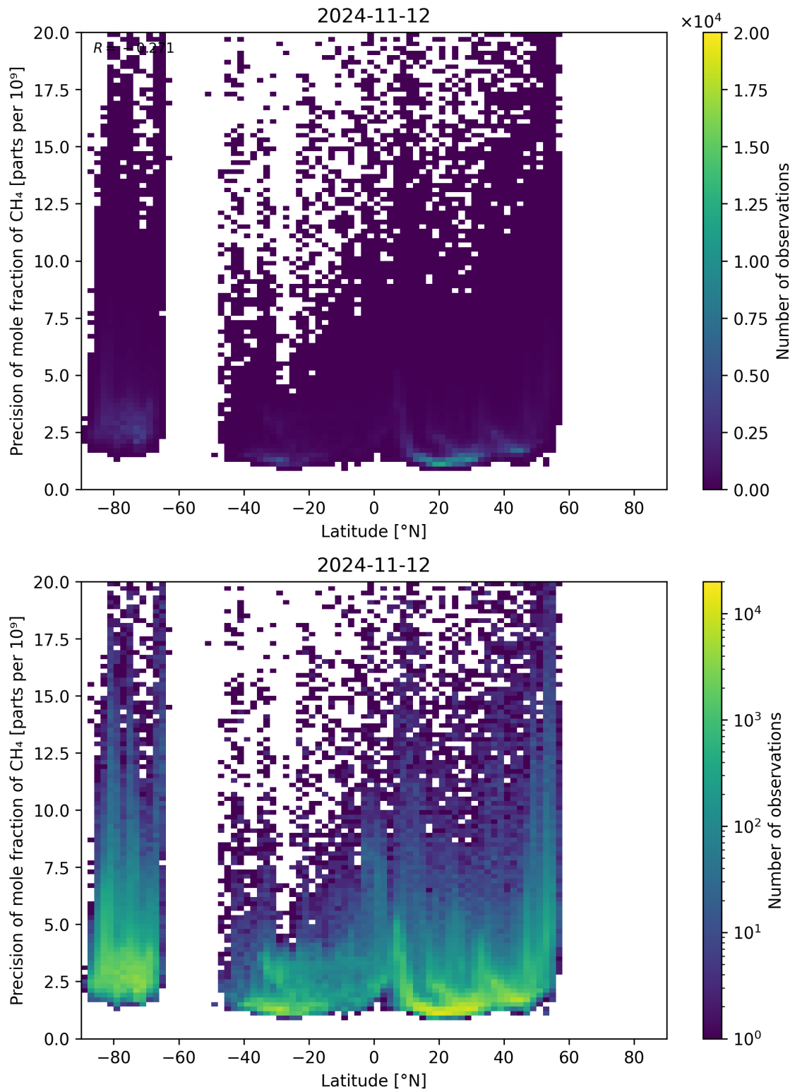
Figure 59: Scatter density plot of “Latitude” against “Precision of mole fraction of CH 4 ” for 2024-11-11 to 2024-11-13.
