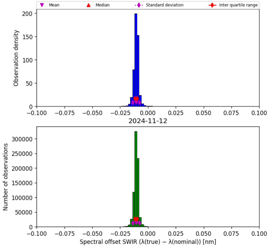
Figure 27: Histogram of “Spectral offset SWIR ( \lambda_{\text{true}} - \lambda_{\text{nominal}} )” for 2024-11-11 to 2024-11-13
