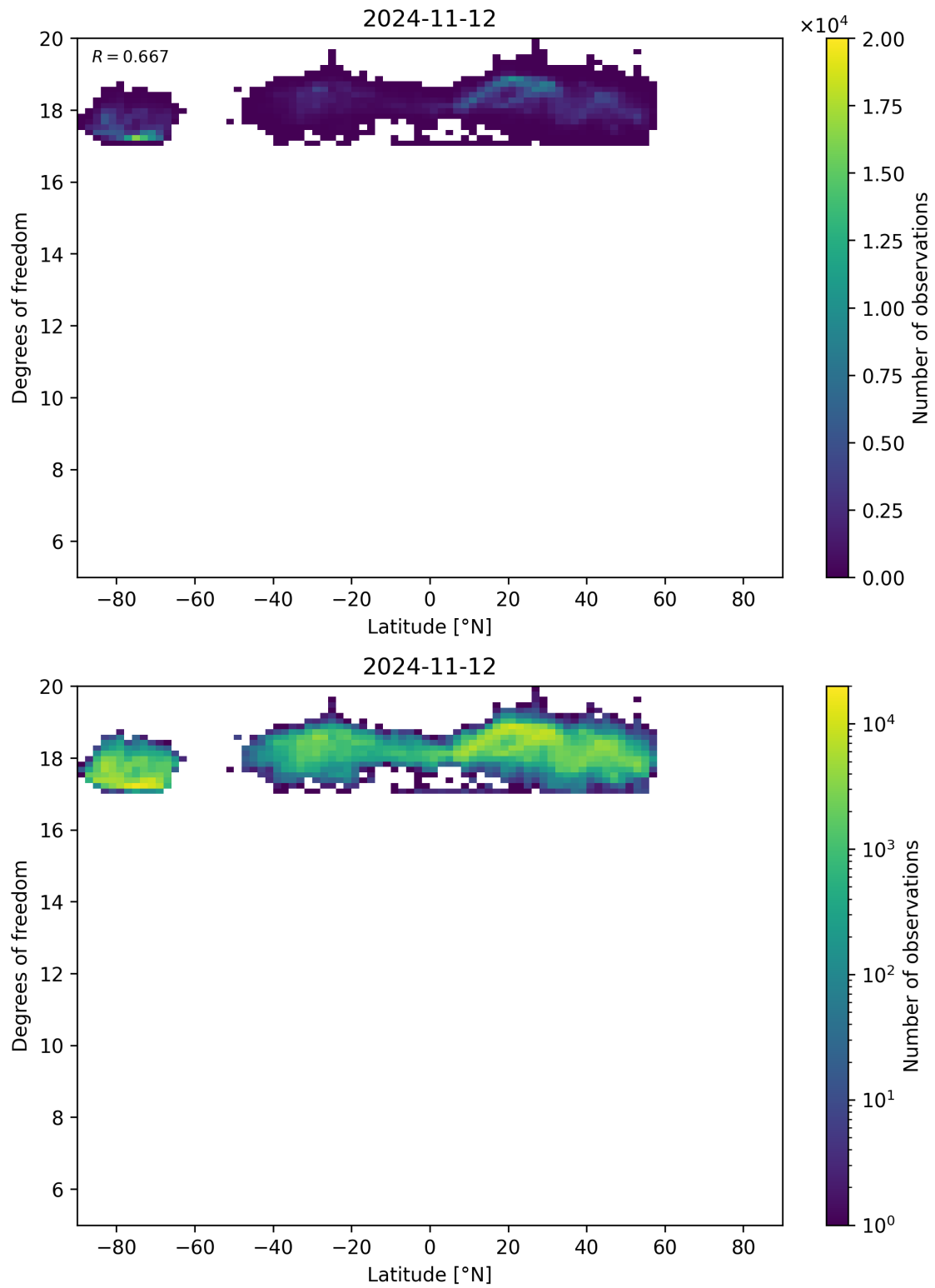
Figure 55: Scatter density plot of “Latitude” against “Degrees of freedom” for 2024-11-11 to 2024-11-13.
