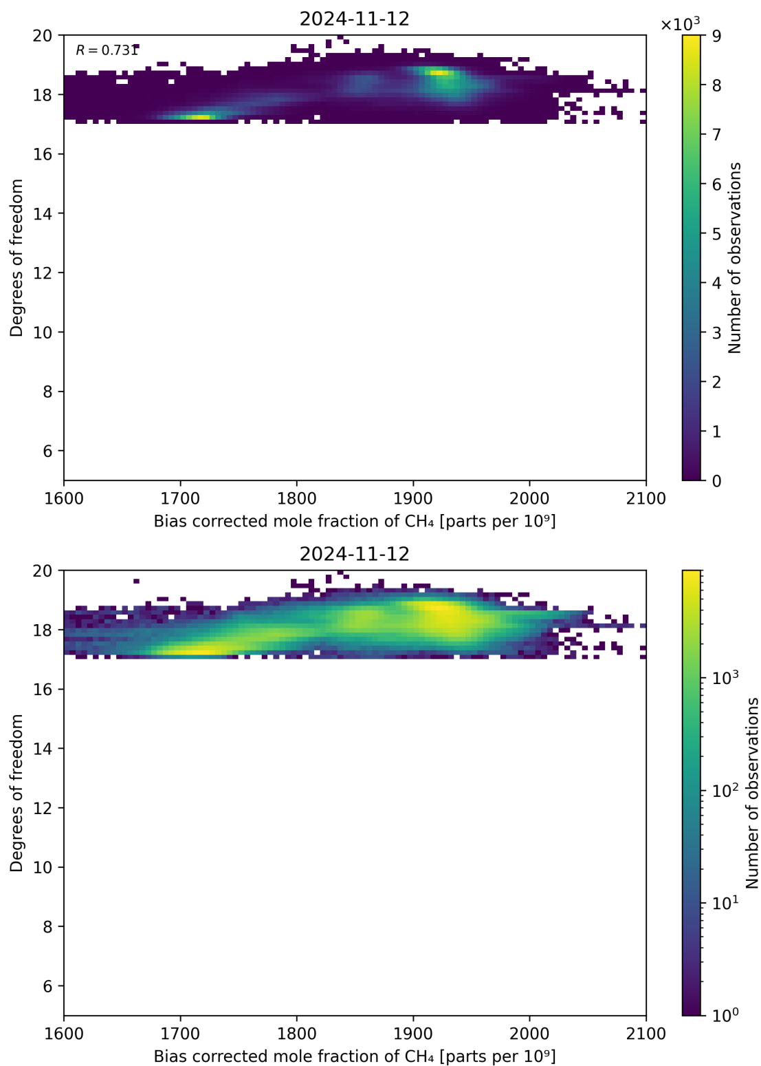
Figure 65: Scatter density plot of “Bias corrected mole fraction of CH 4 ” against “Degrees of freedom” for 2024-11-11 to 2024-11-13.
