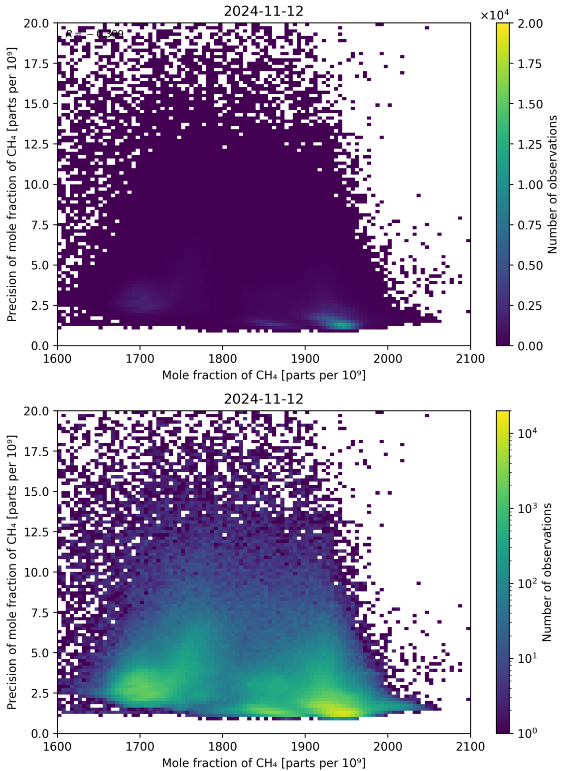
Figure 75: Scatter density plot of “Mole fraction of CH 4 ” against “Precision of mole fraction of CH 4 ” for 2024-11-11 to 2024-11-13.
