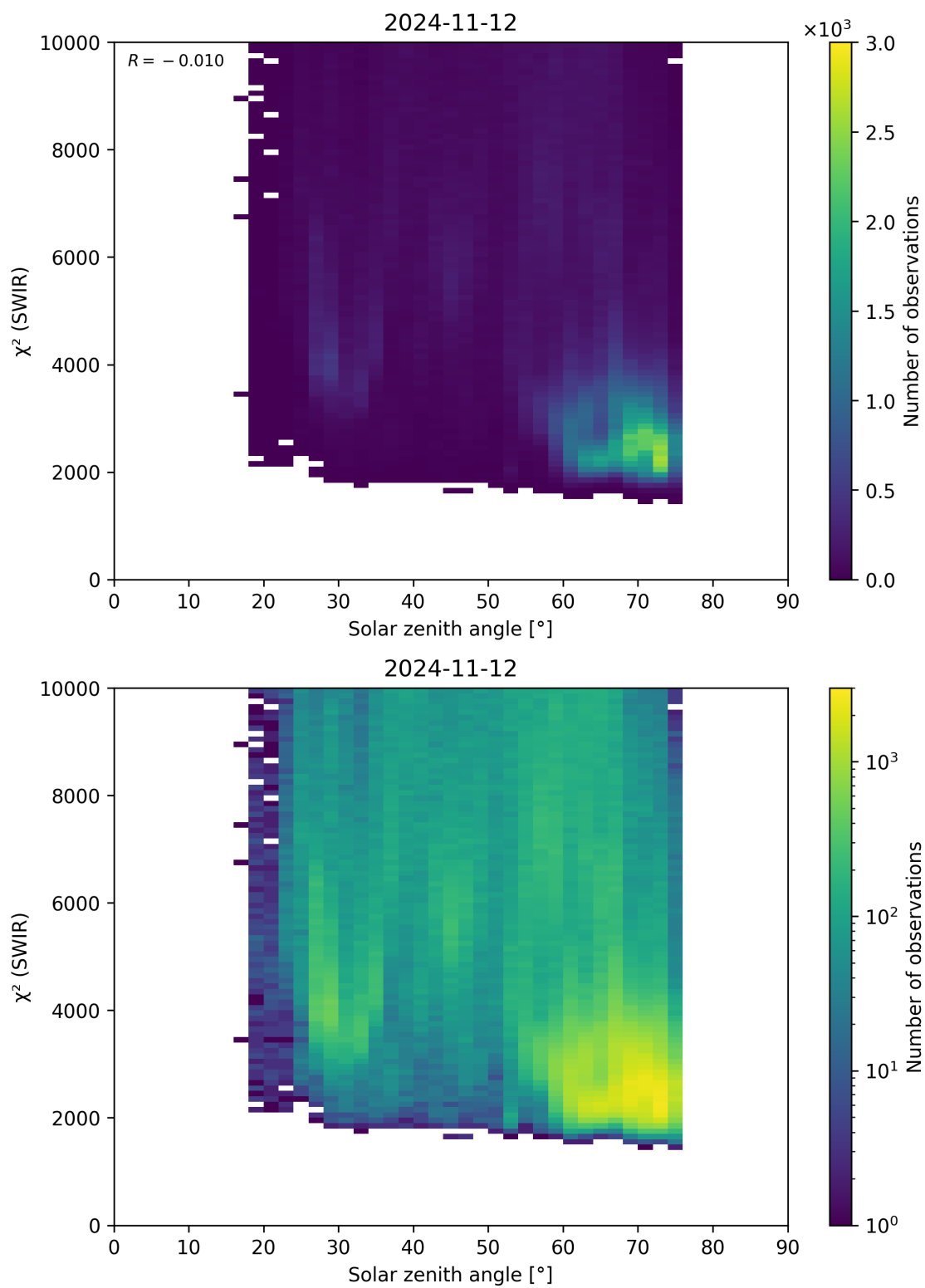
Figure 95: Scatter density plot of “Solar zenith angle” against “ \chi^2 (SWIR)” for 2024-11-11 to 2024-11-13.
