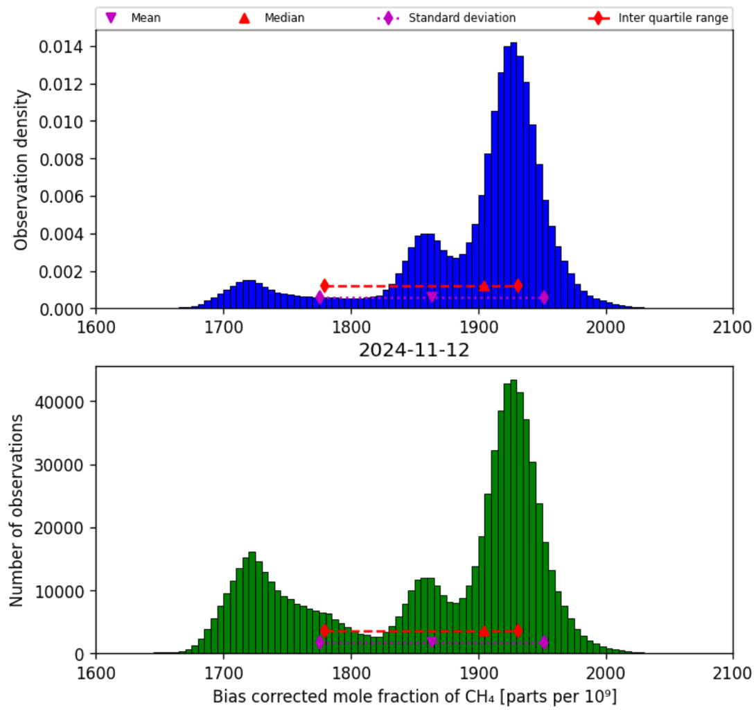
Figure 25: Histogram of “Bias corrected mole fraction of CH 4 ” for 2024-11-11 to 2024-11-13
