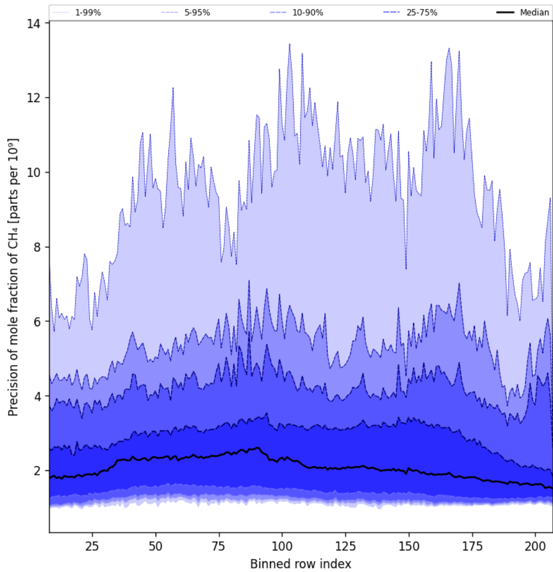
Figure 35: Along track statistics of “Precision of mole fraction of CH 4 ” for 2024-11-11 to 2024-11-13
