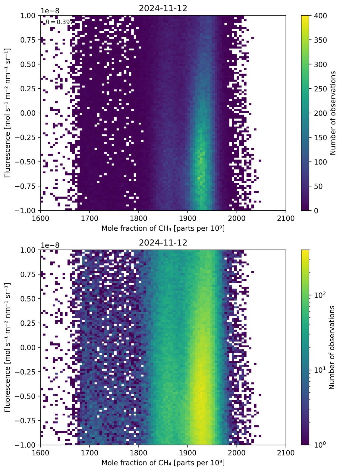
Figure 73: Scatter density plot of “Mole fraction of \text{CH}_4 ” against “Fluorescence” for 2024-11-11 to 2024-11-13.
