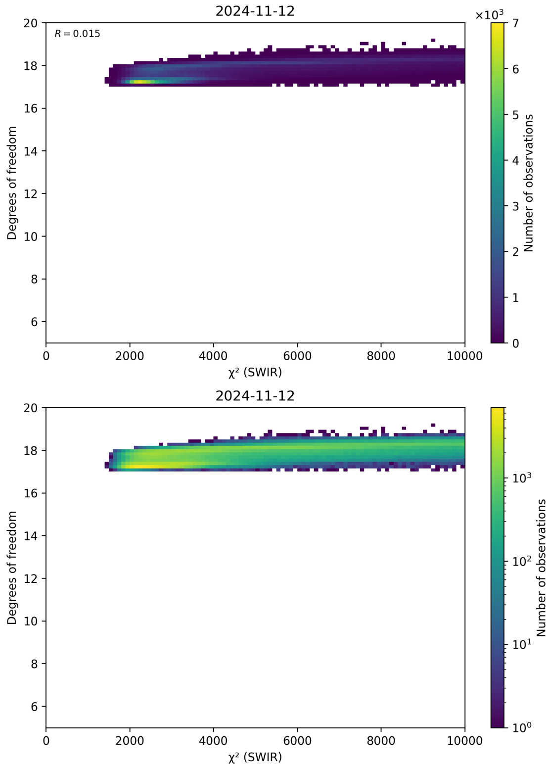
Figure 48: Scatter density plot of “ \chi^2 (SWIR)” against “Degrees of freedom” for 2024-11-11 to 2024-11-13.
