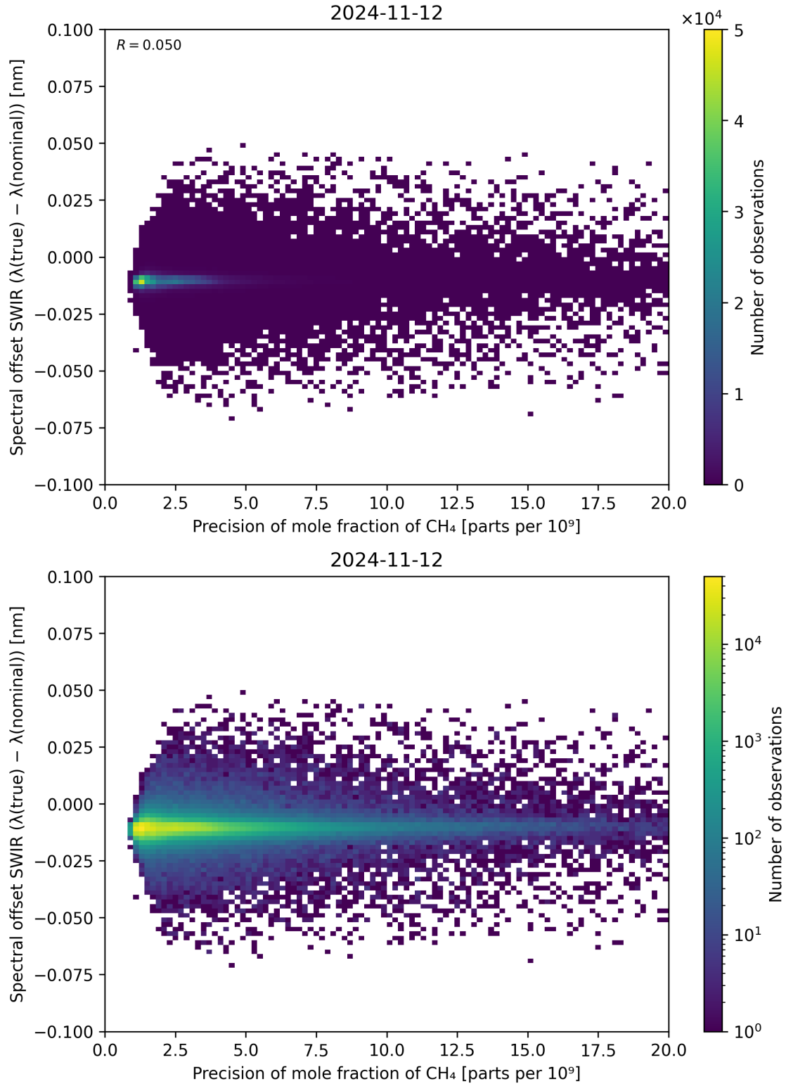
Figure 85: Scatter density plot of “Precision of mole fraction of \text{CH}_4 ” against “Spectral offset SWIR ( \lambda_{\text{true}} - \lambda_{\text{nominal}} )” for 2024-11-11 to 2024-11-13.
