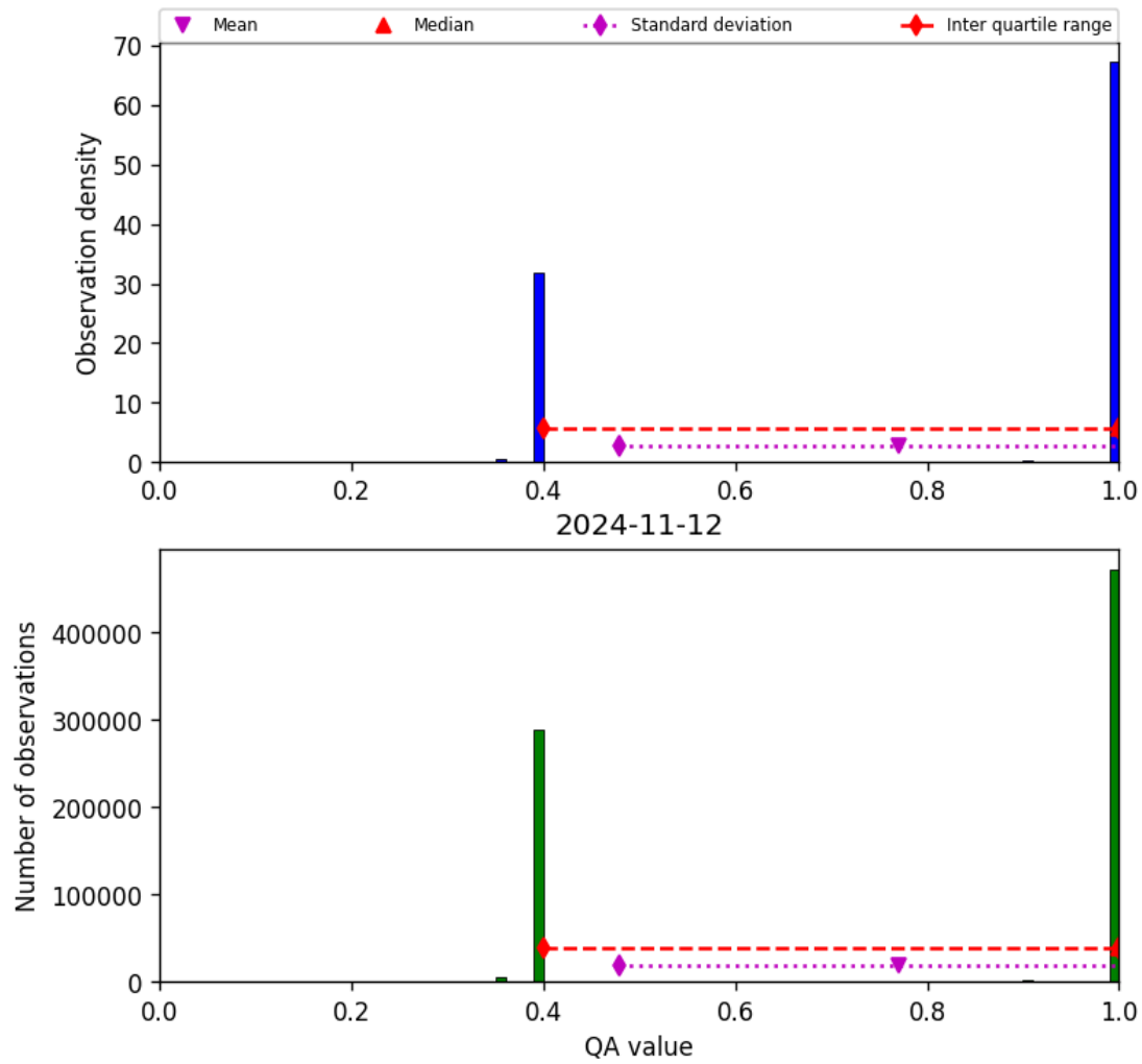
Figure 22: Histogram of “QA value” for 2024-11-11 to 2024-11-13
