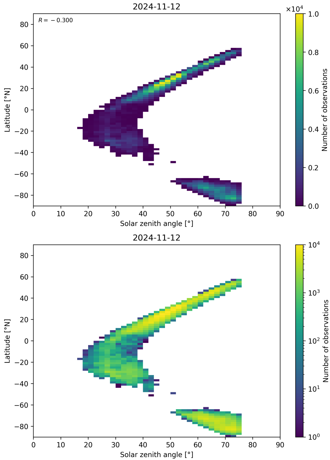
Figure 98: Scatter density plot of “Solar zenith angle” against “Latitude” for 2024-11-11 to 2024-11-13.
