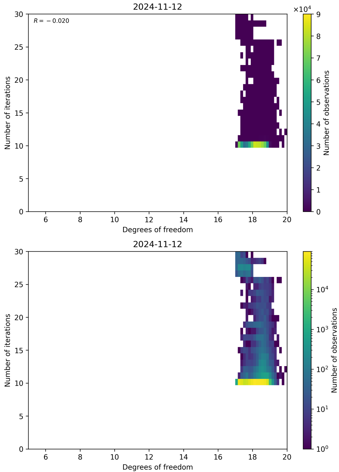
Figure 52: Scatter density plot of “Degrees of freedom” against “Number of iterations” for 2024-11-11 to 2024-11-13.
