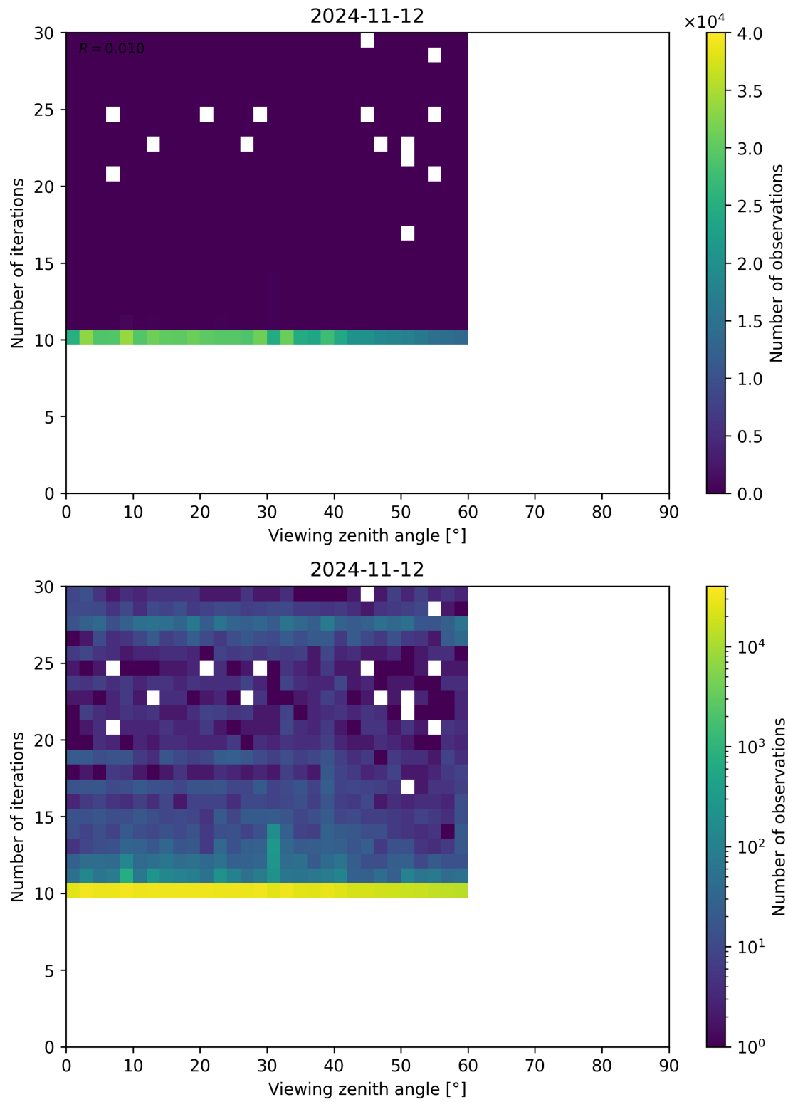
Figure 113: Scatter density plot of “Viewing zenith angle” against “Number of iterations” for 2024-11-11 to 2024-11-13.
