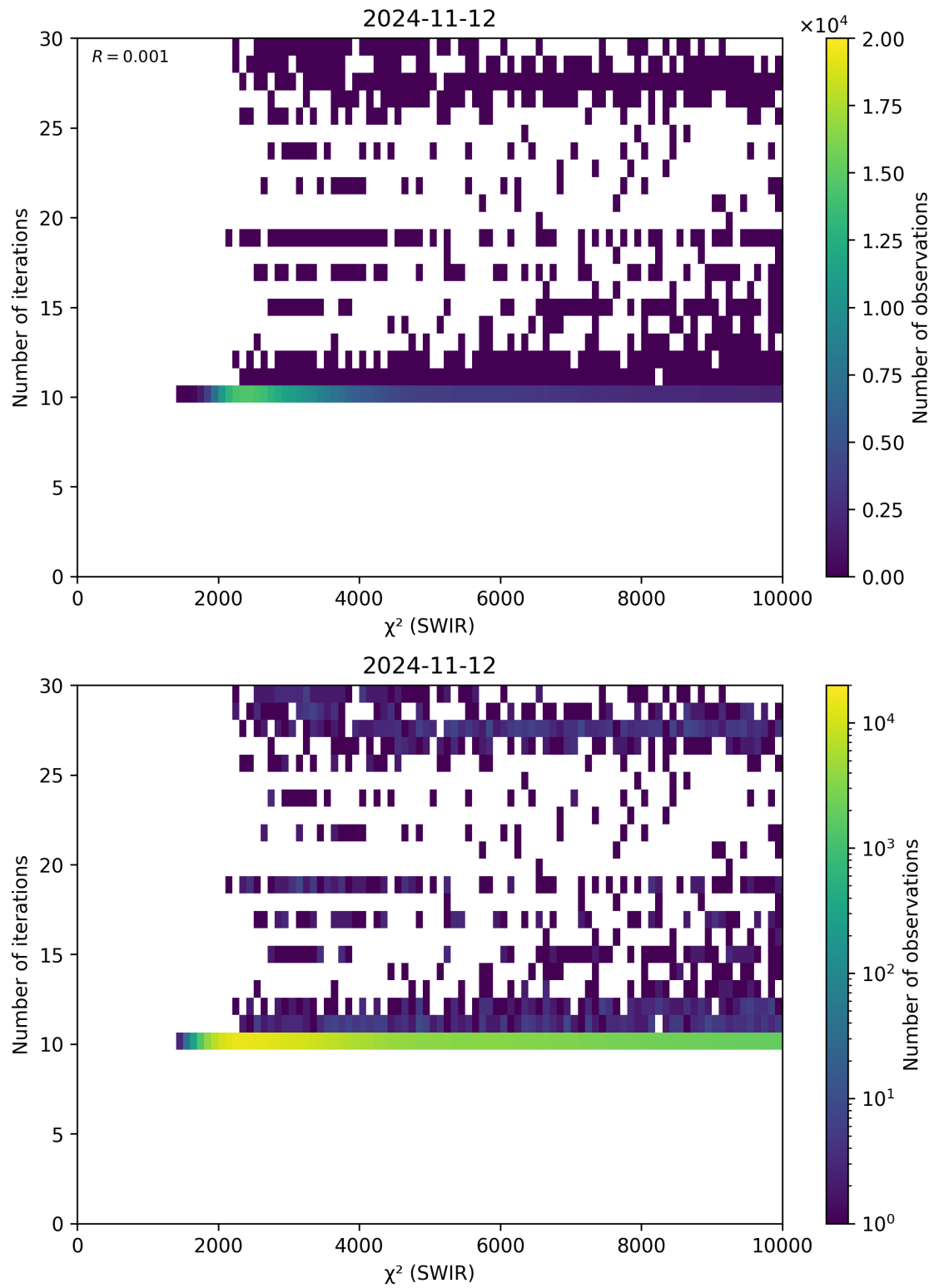
Figure 50: Scatter density plot of “ \chi^2 (SWIR)” against “Number of iterations” for 2024-11-11 to 2024-11-13.
