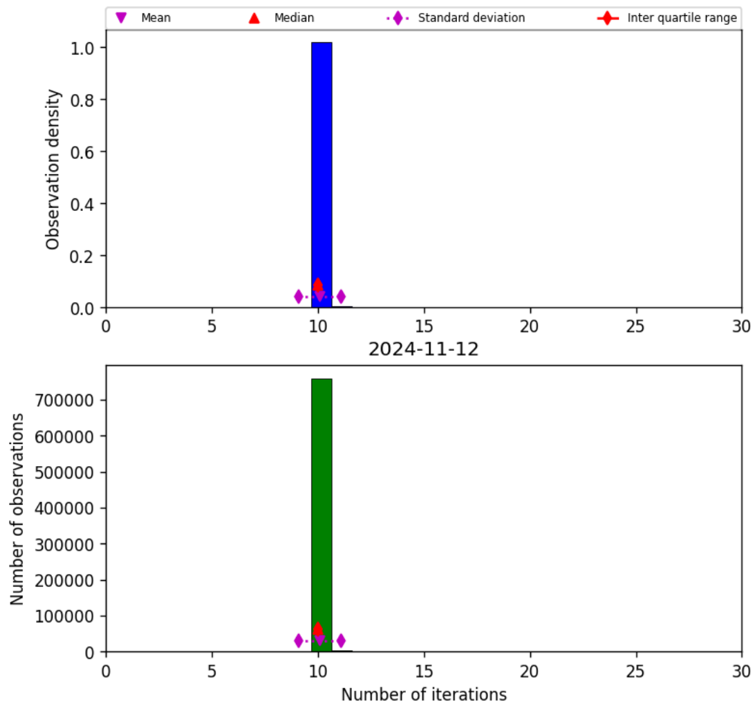
Figure 31: Histogram of “Number of iterations” for 2024-11-11 to 2024-11-13
