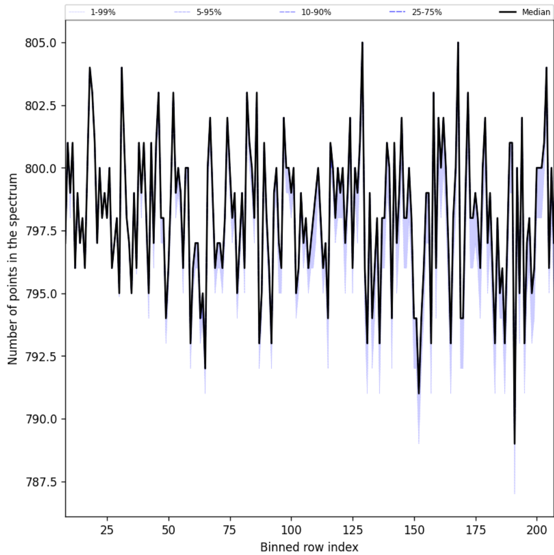
Figure 37: Along track statistics of “Number of points in the spectrum” for 2024-11-11 to 2024-11-13
