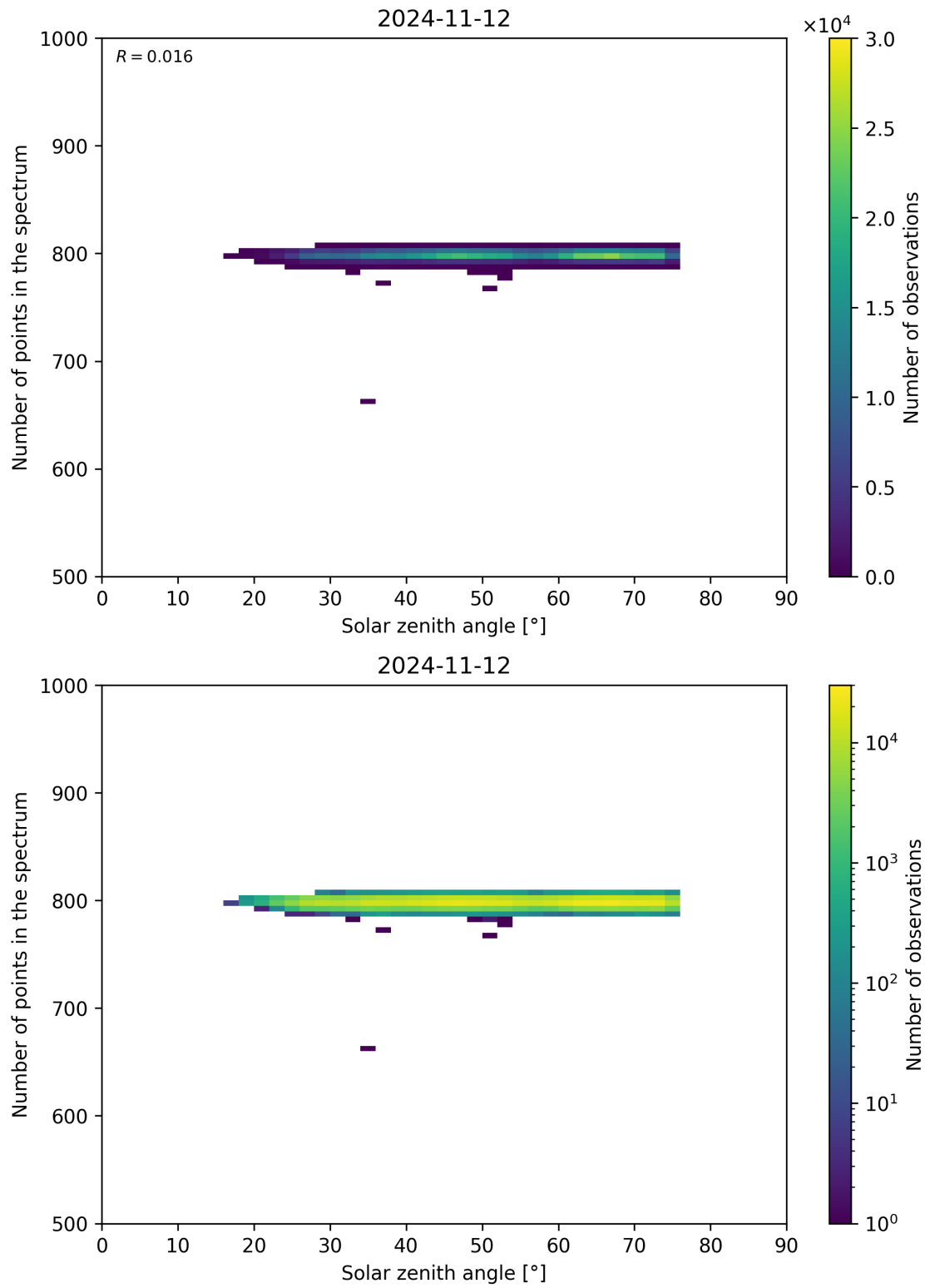
Figure 103: Scatter density plot of “Solar zenith angle” against “Number of points in the spectrum” for 2024-11-11 to 2024-11-13.
