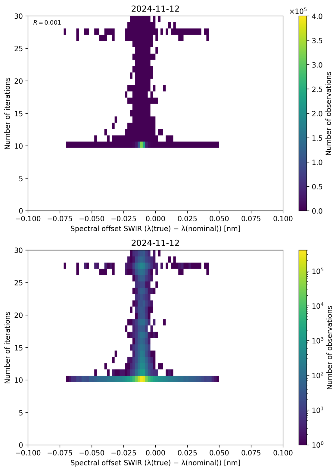
Figure 121: Scatter density plot of “Spectral offset SWIR ( \lambda_{\text{true}} - \lambda_{\text{nominal}} )” against “Number of iterations” for 2024-11-11 to 2024-11-13.
