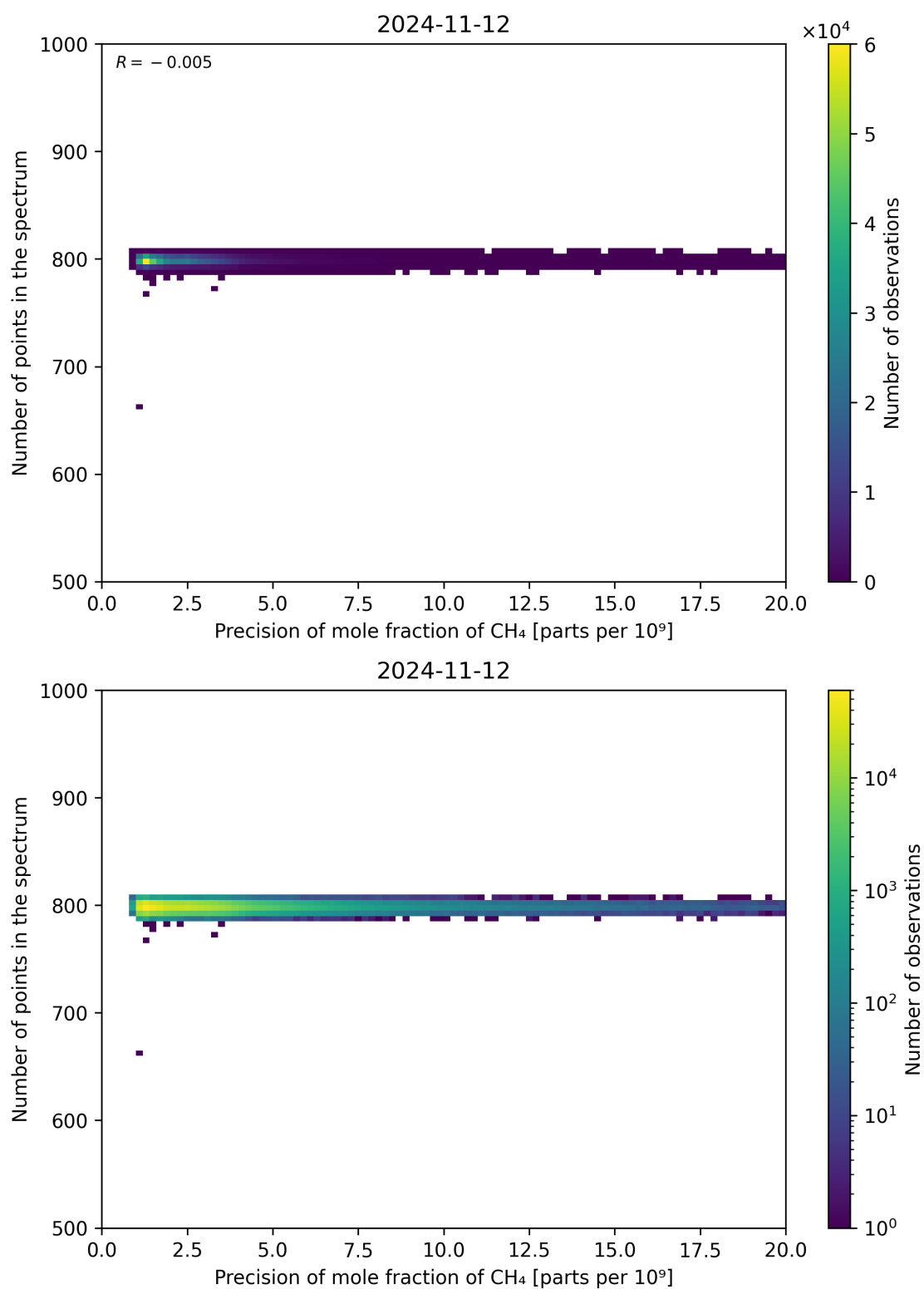
Figure 84: Scatter density plot of “Precision of mole fraction of CH 4 ” against “Number of points in the spectrum” for 2024-11-11 to 2024-11-13.
