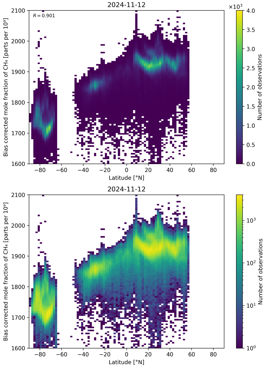
Figure 58: Scatter density plot of “Latitude” against “Bias corrected mole fraction of CH 4 ” for 2024-11-11 to 2024-11-13.
