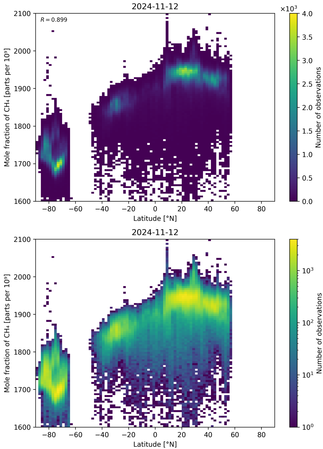
Figure 57: Scatter density plot of “Latitude” against “Mole fraction of CH 4 ” for 2024-11-11 to 2024-11-13.
