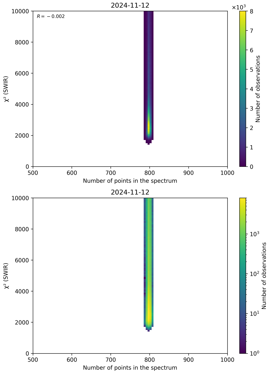
Figure 89: Scatter density plot of “Number of points in the spectrum” against “ \chi^2 (SWIR)” for 2024-11-11 to 2024-11-13.
