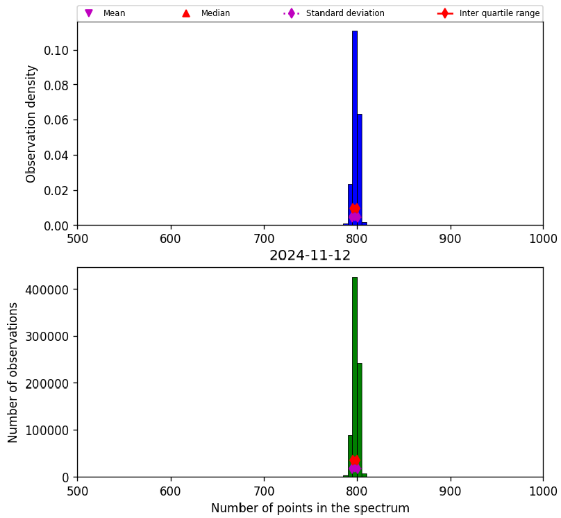
Figure 26: Histogram of “Number of points in the spectrum” for 2024-11-11 to 2024-11-13
