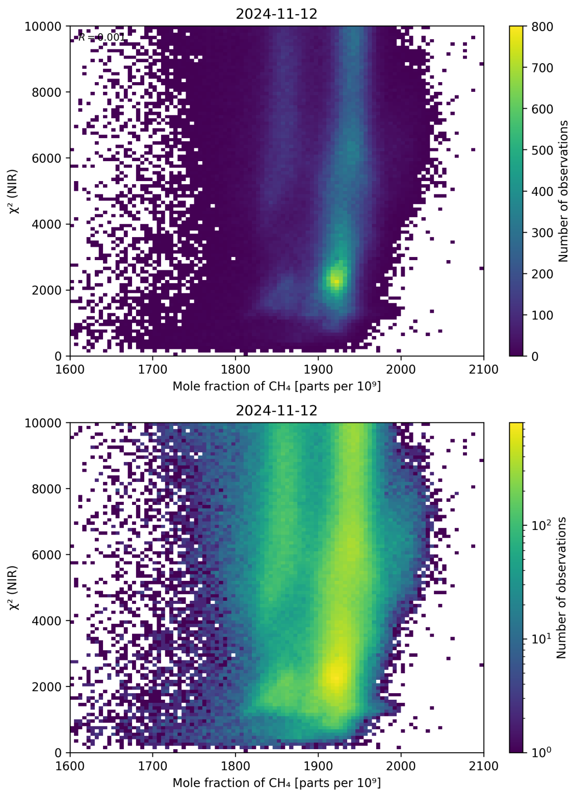
Figure 70: Scatter density plot of “Mole fraction of \text{CH}_4 ” against “ \chi^2 (NIR)” for 2024-11-11 to 2024-11-13.
