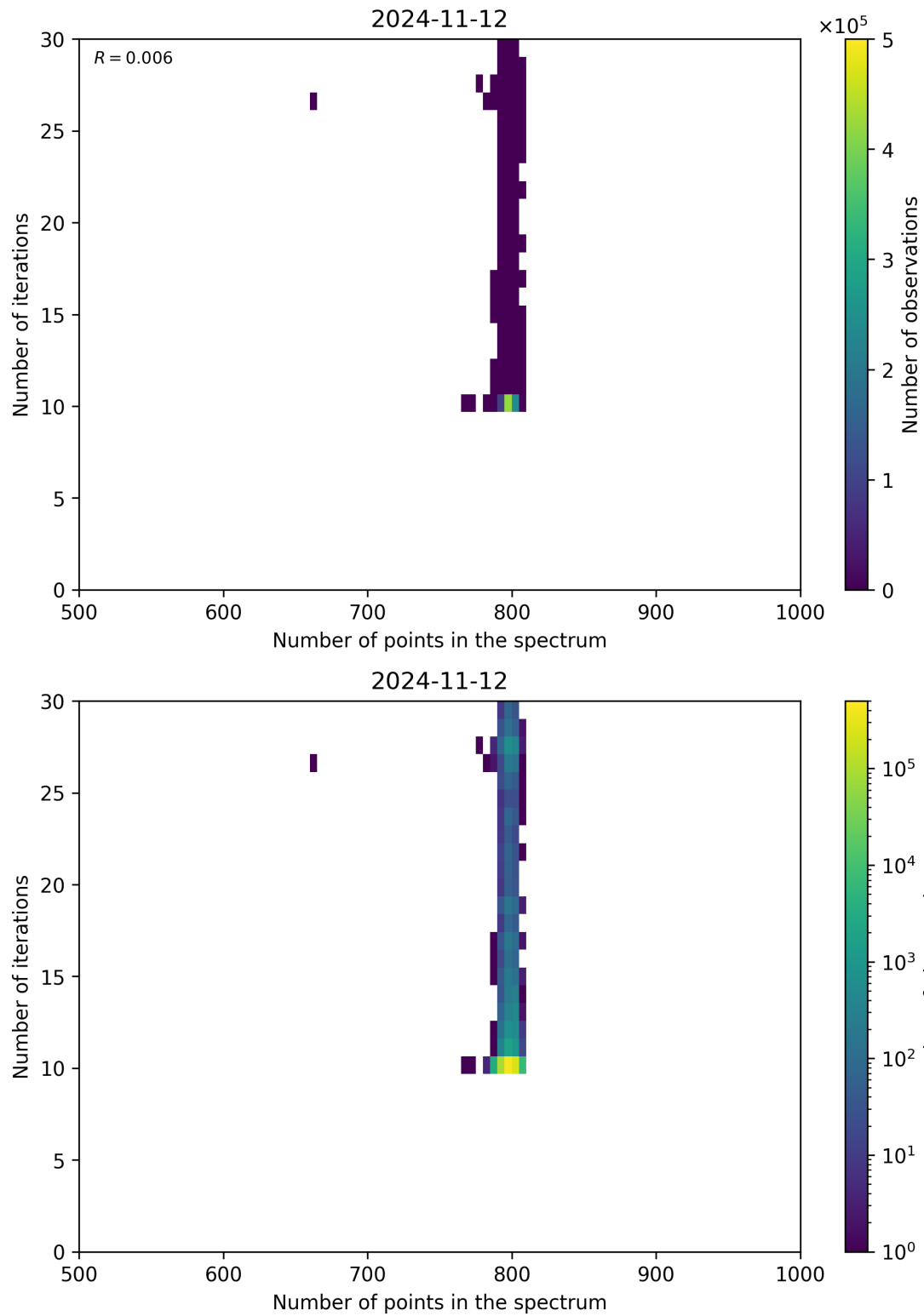
Figure 92: Scatter density plot of “Number of points in the spectrum” against “Number of iterations” for 2024-11-11 to 2024-11-13.
