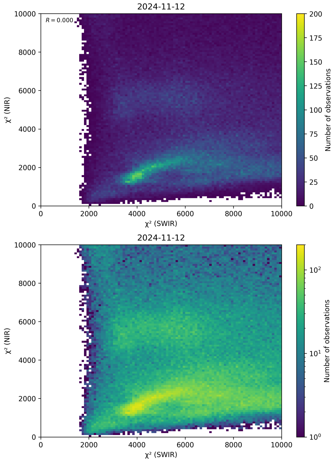
Figure 47: Scatter density plot of “ \chi^2 (SWIR)” against “ \chi^2 (NIR)” for 2024-11-11 to 2024-11-13.
