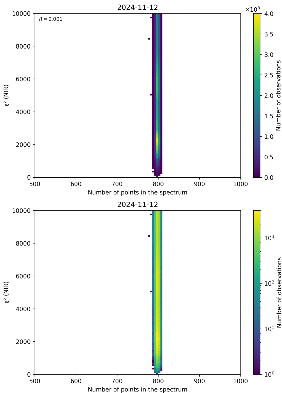
Figure 88: Scatter density plot of “Number of points in the spectrum” against “ \chi^2 (NIR)” for 2024-11-11 to 2024-11-13.
