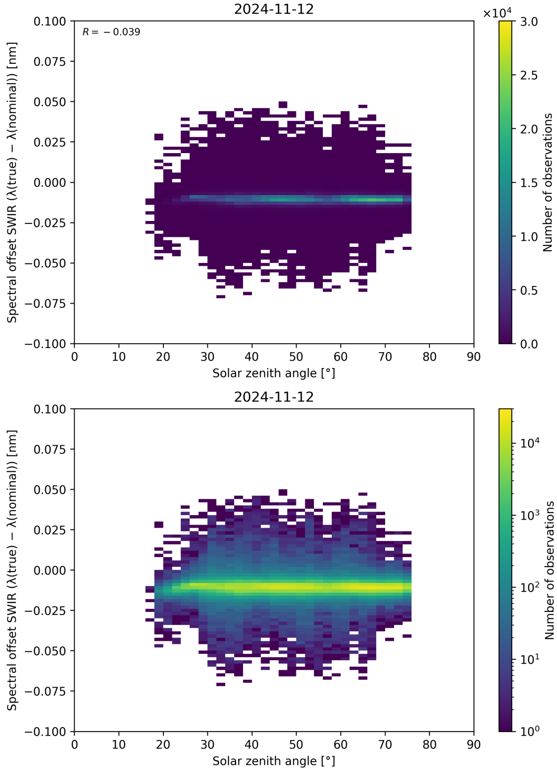
Figure 104: Scatter density plot of “Solar zenith angle” against “Spectral offset SWIR ( \lambda_{\text{true}} - \lambda_{\text{nominal}} )” for 2024-11-11 to 2024-11-13.
