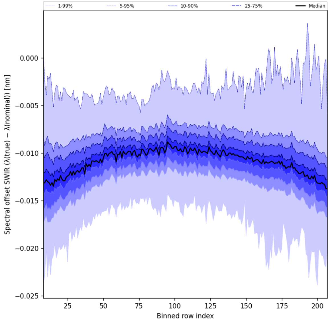
Figure 38: Along track statistics of “Spectral offset SWIR ( \lambda_{\text{true}} - \lambda_{\text{nominal}} )” for 2024-11-11 to 2024-11-13
