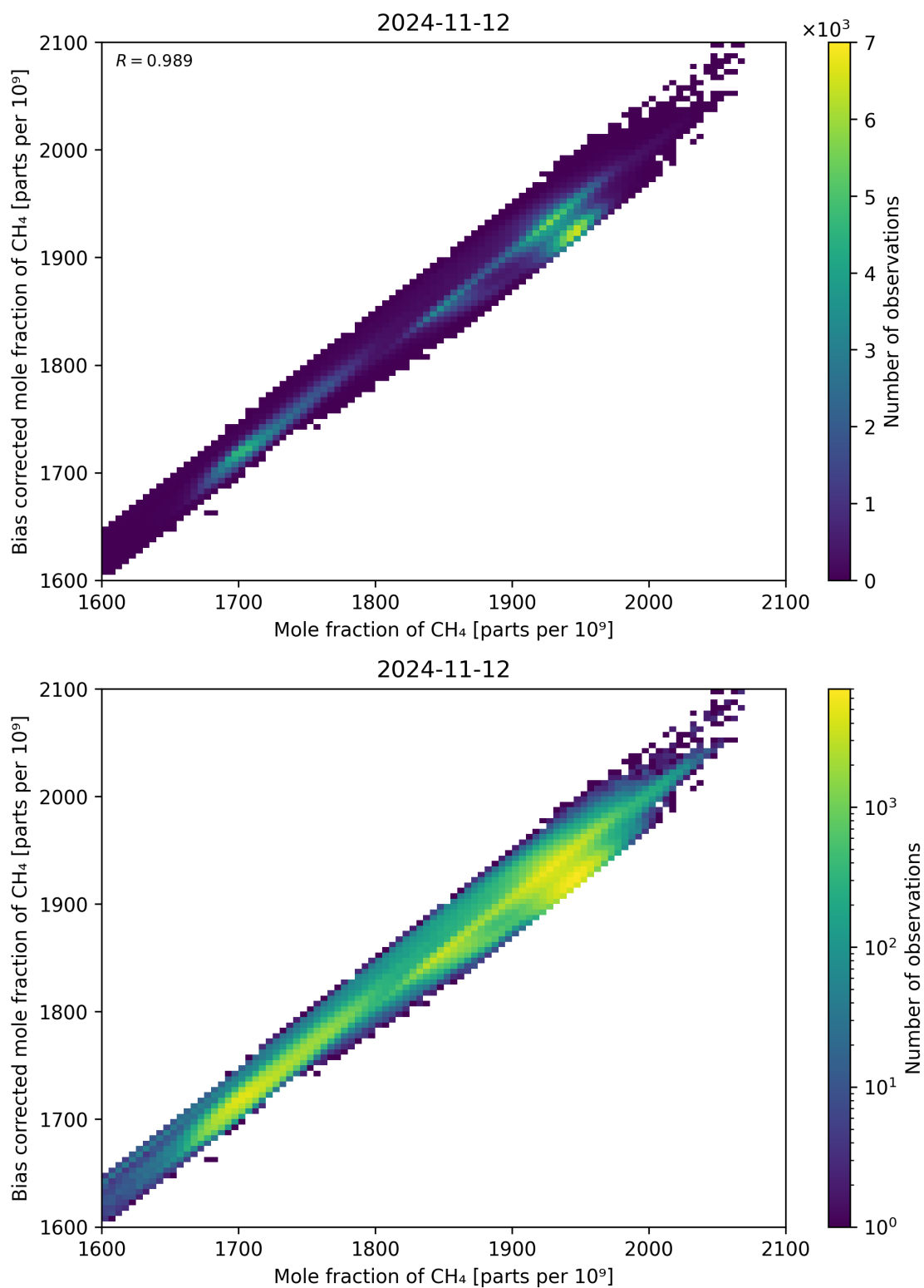
Figure 74: Scatter density plot of “Mole fraction of CH 4 ” against “Bias corrected mole fraction of CH 4 ” for 2024-11-11 to 2024-11-13.
