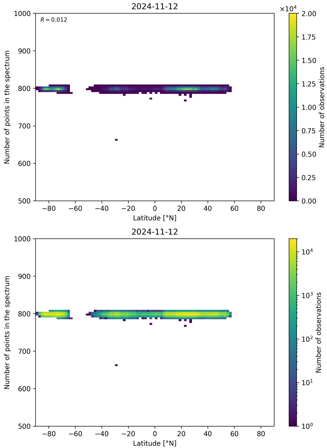
Figure 61: Scatter density plot of “Latitude” against “Number of points in the spectrum” for 2024-11-11 to 2024-11-13.
