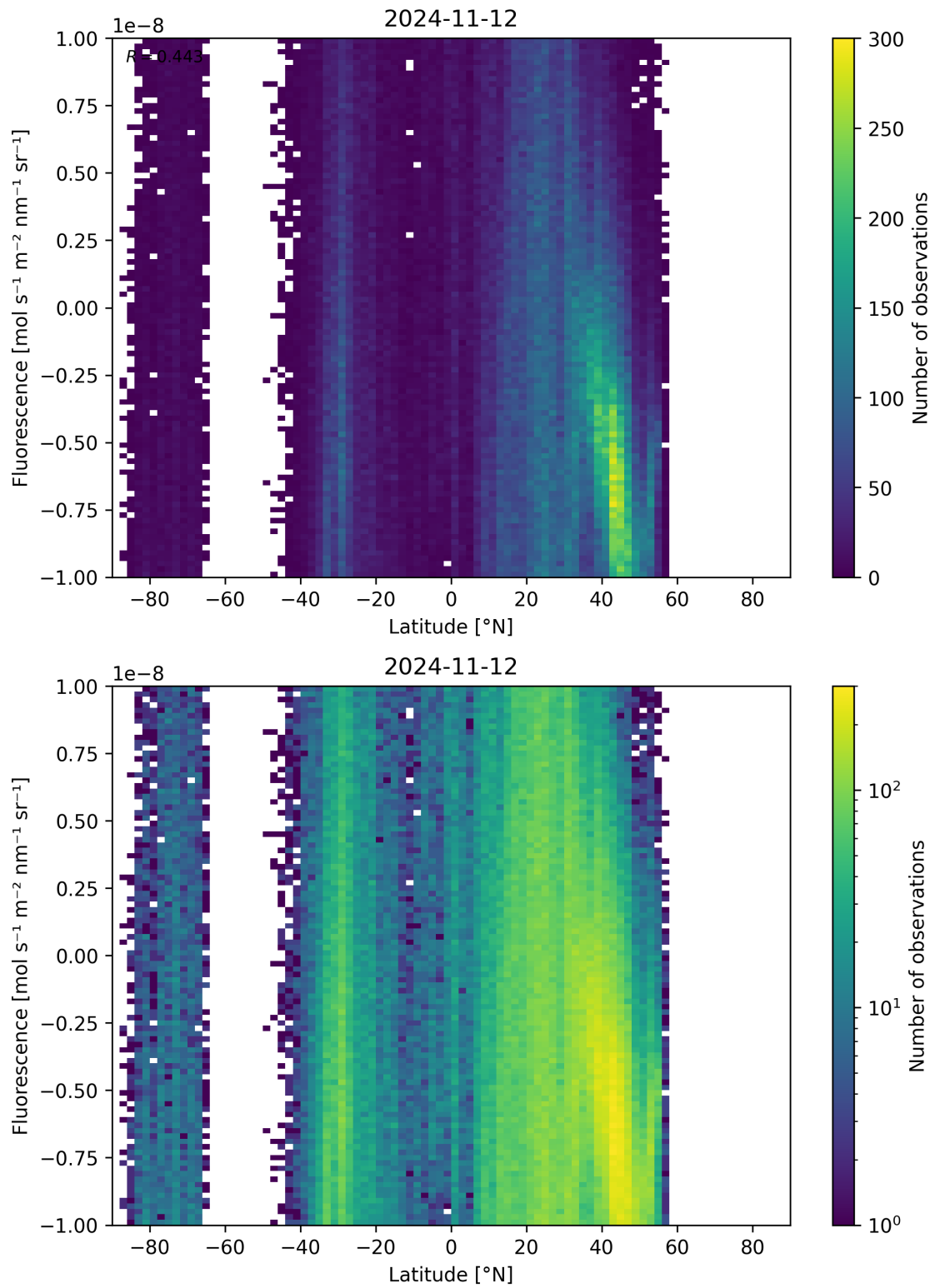
Figure 56: Scatter density plot of “Latitude” against “Fluorescence” for 2024-11-11 to 2024-11-13.
