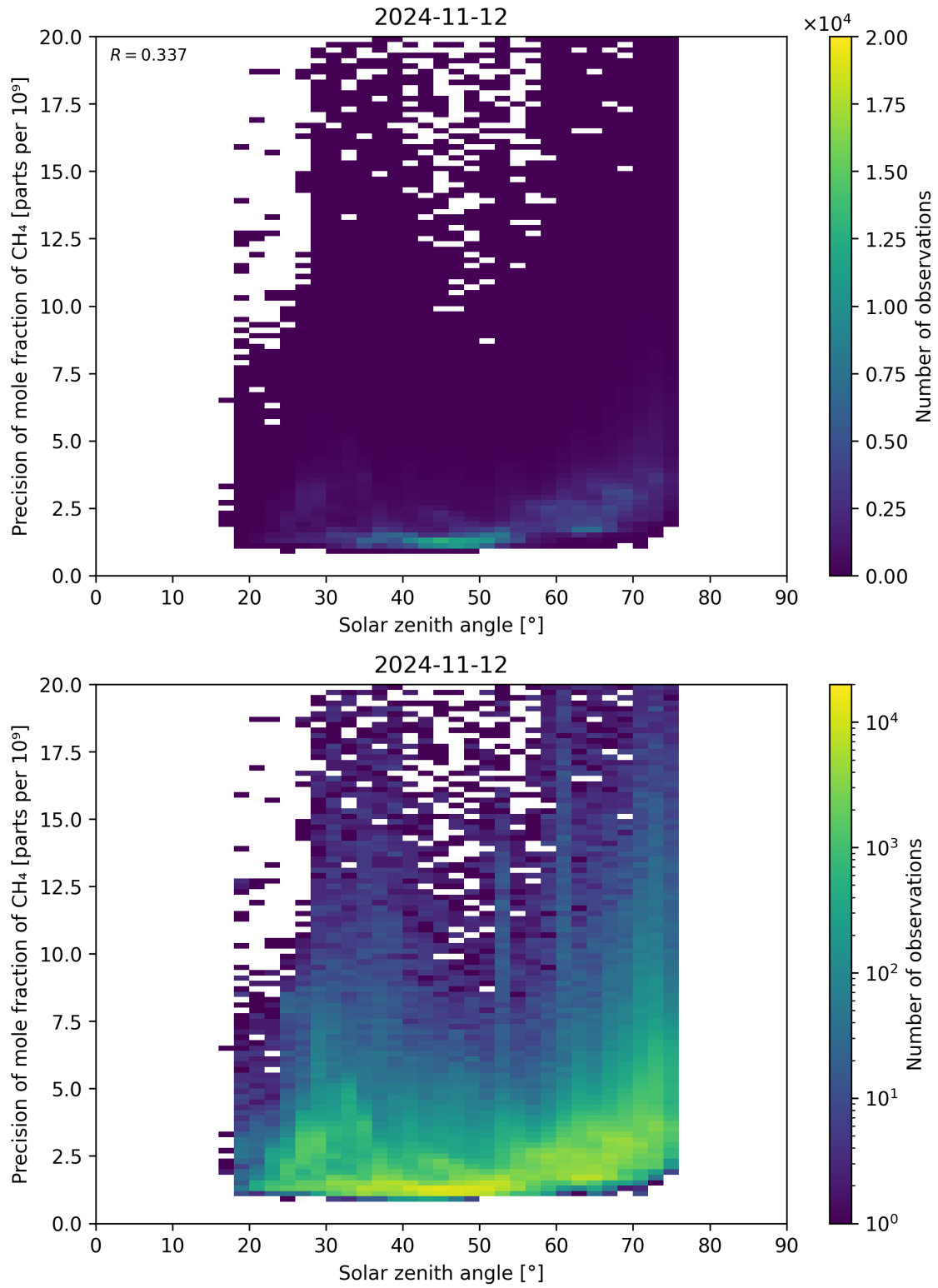
Figure 101: Scatter density plot of “Solar zenith angle” against “Precision of mole fraction of \text{CH}_4 ” for 2024-11-11 to 2024-11-13.
