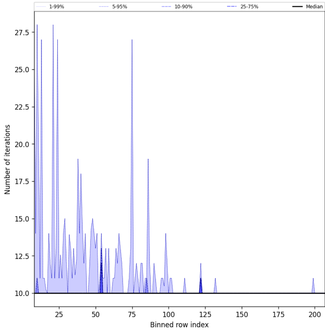
Figure 42: Along track statistics of “Number of iterations” for 2024-11-11 to 2024-11-13
