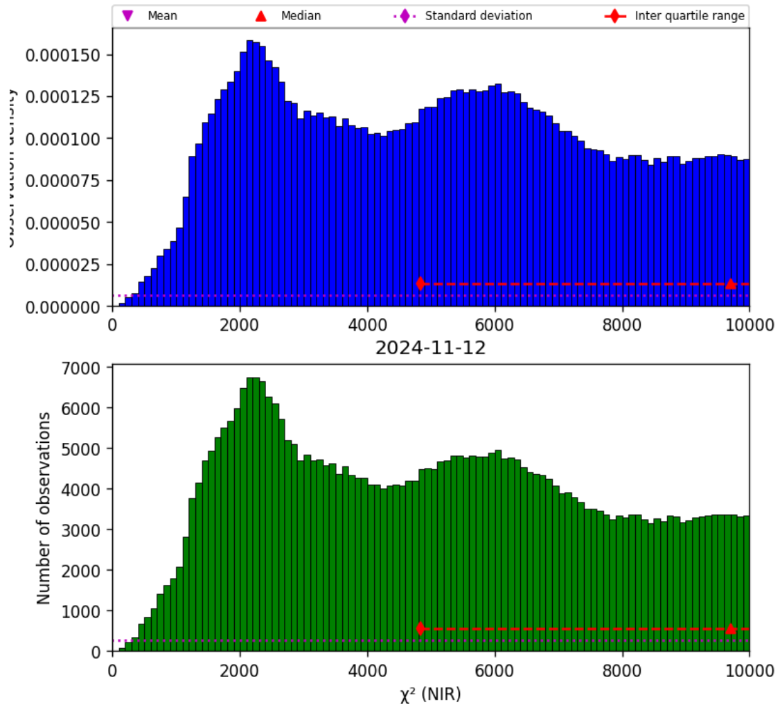
Figure 29: Histogram of “ \chi^2 (NIR)” for 2024-11-11 to 2024-11-13
