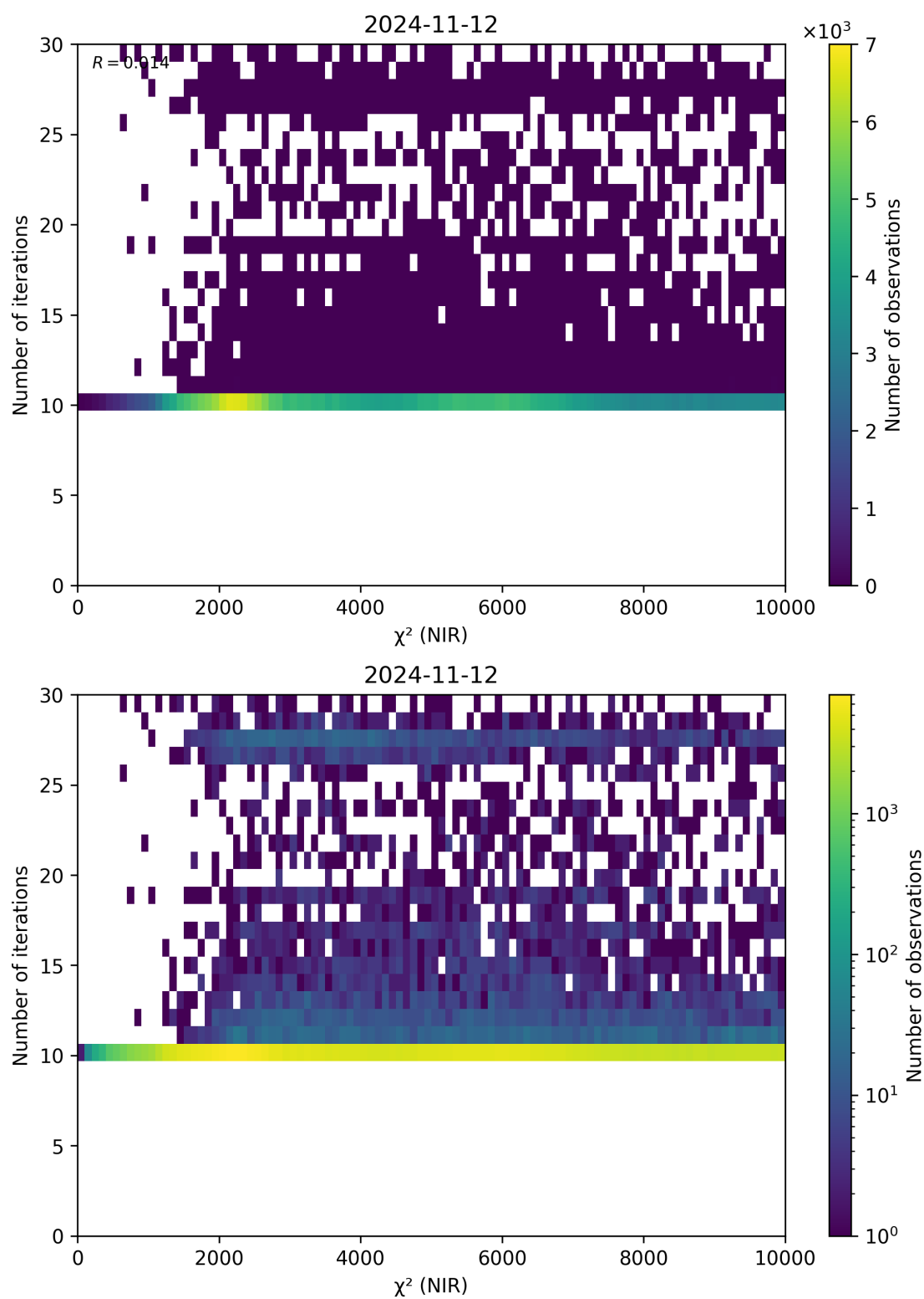
Figure 46: Scatter density plot of “ \chi^2 (NIR)” against “Number of iterations” for 2024-11-11 to 2024-11-13.
