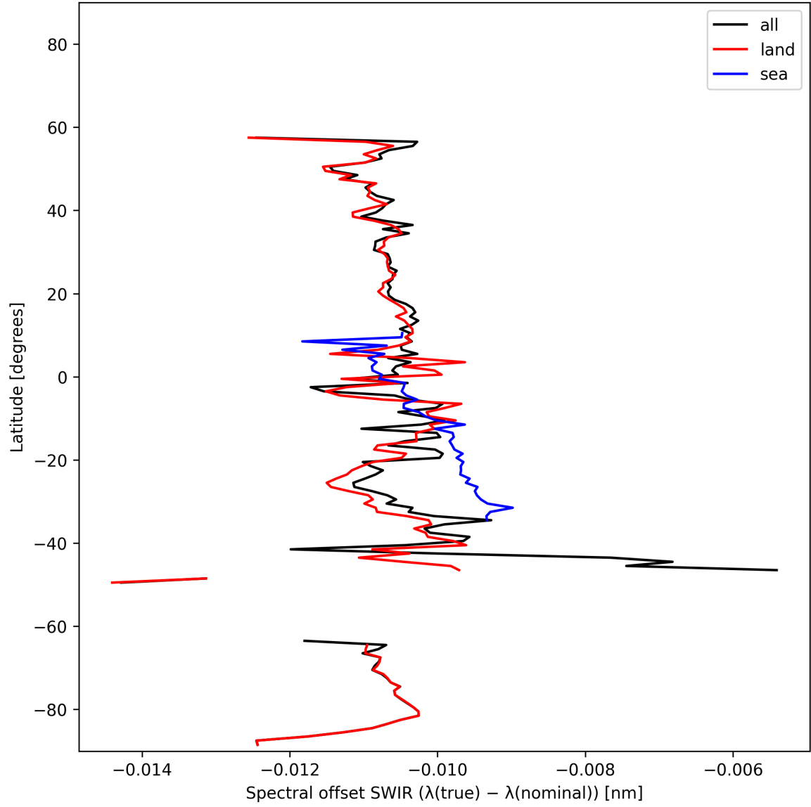
Figure 16: Zonal average of “Spectral offset SWIR ( \lambda_{\text{true}} - \lambda_{\text{nominal}} )” for 2024-11-11 to 2024-11-13.
