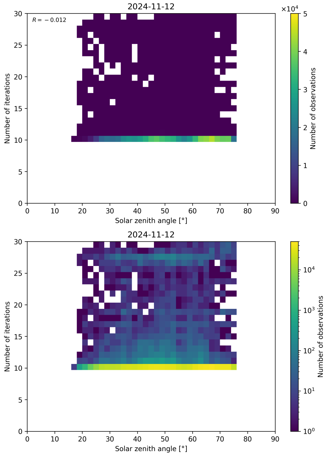
Figure 102: Scatter density plot of “Solar zenith angle” against “Number of iterations” for 2024-11-11 to 2024-11-13.
