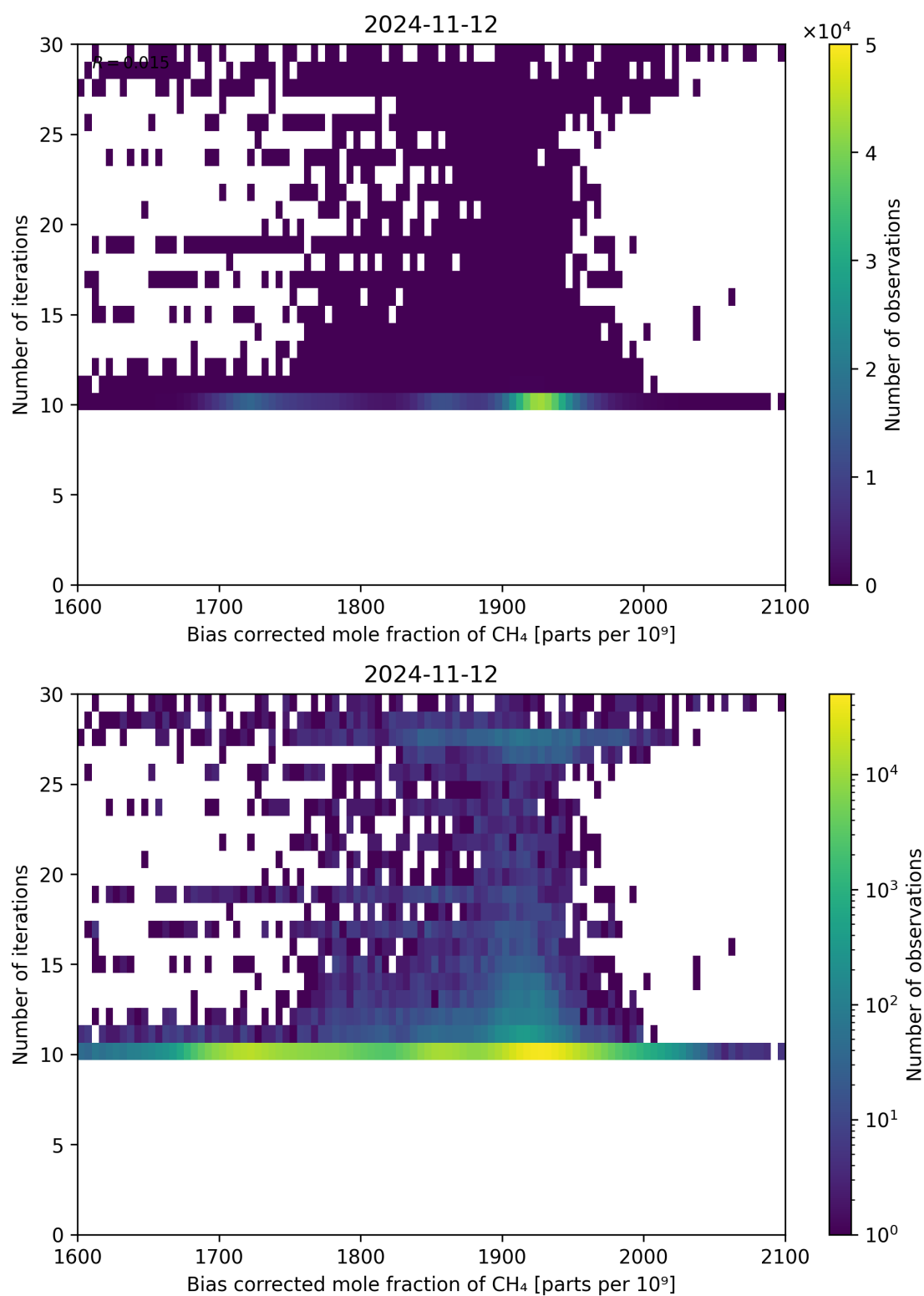
Figure 67: Scatter density plot of “Bias corrected mole fraction of CH 4 ” against “Number of iterations” for 2024-11-11 to 2024-11-13.
