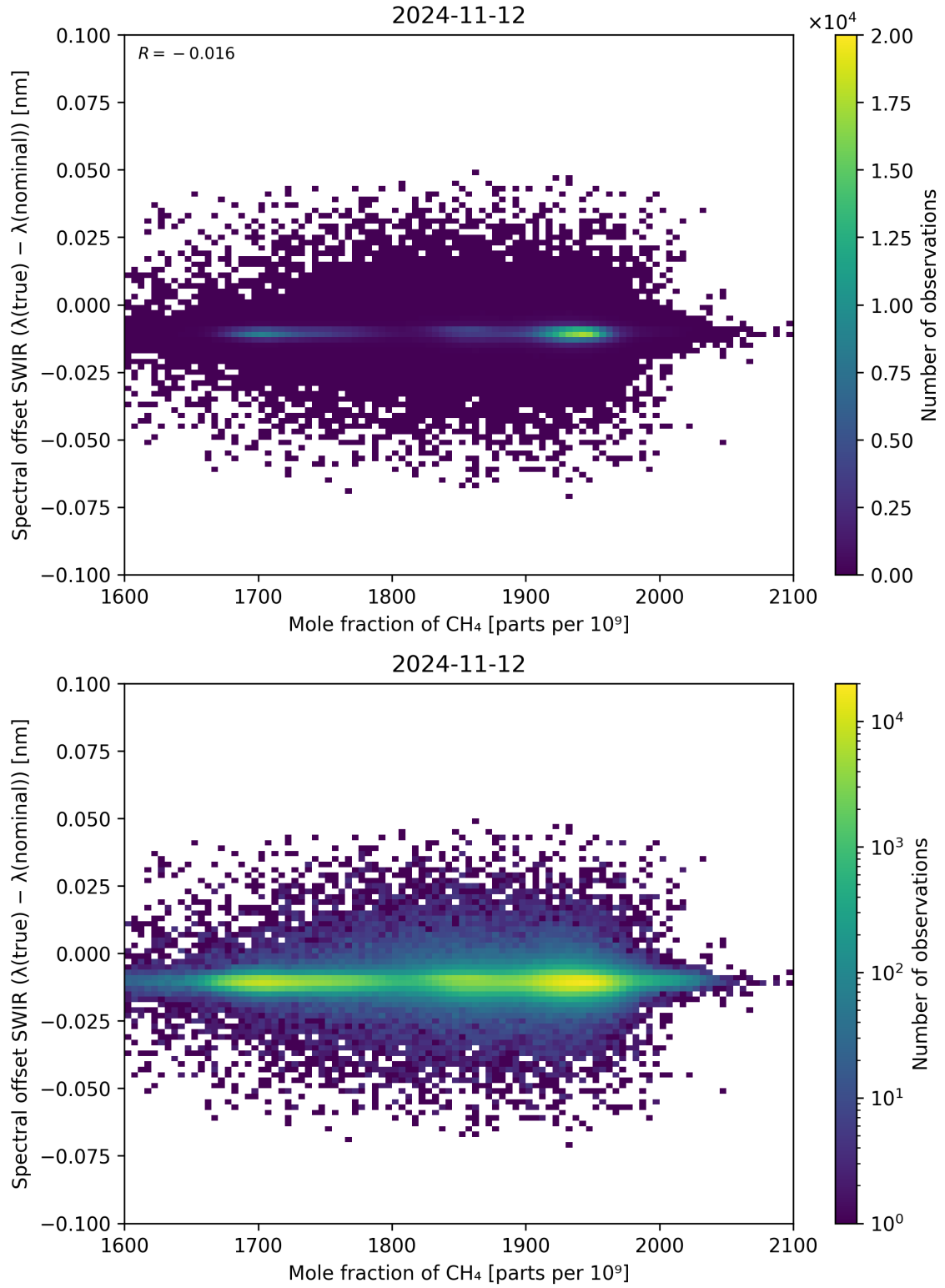
Figure 86: Scatter density plot of “Mole fraction of CH 4 ” against “Spectral offset SWIR ( \lambda_{\text{true}} - \lambda_{\text{nominal}} )” for 2024-11-11 to 2024-11-13.
