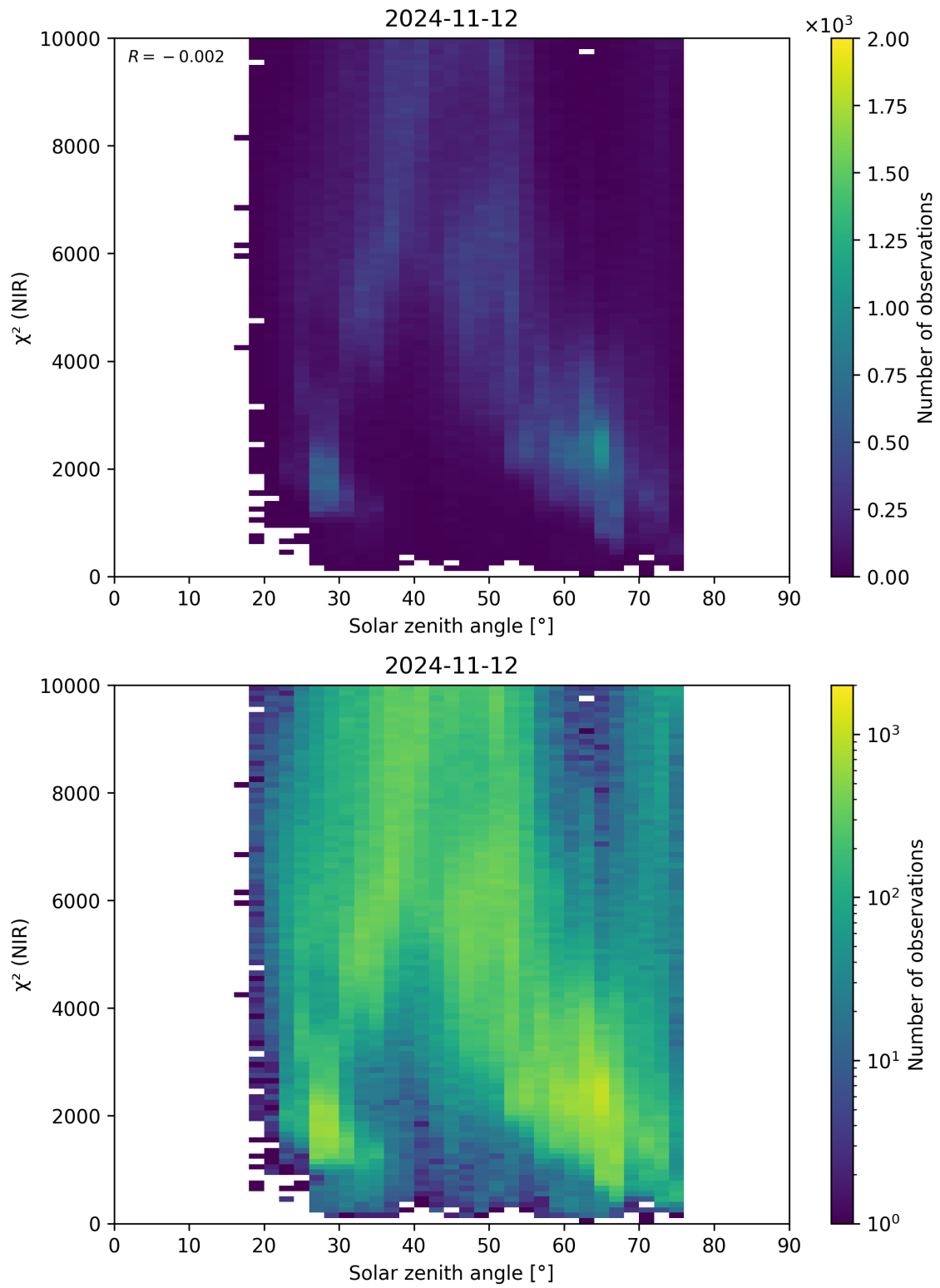
Figure 94: Scatter density plot of “Solar zenith angle” against “ \chi^2 (NIR)” for 2024-11-11 to 2024-11-13.
