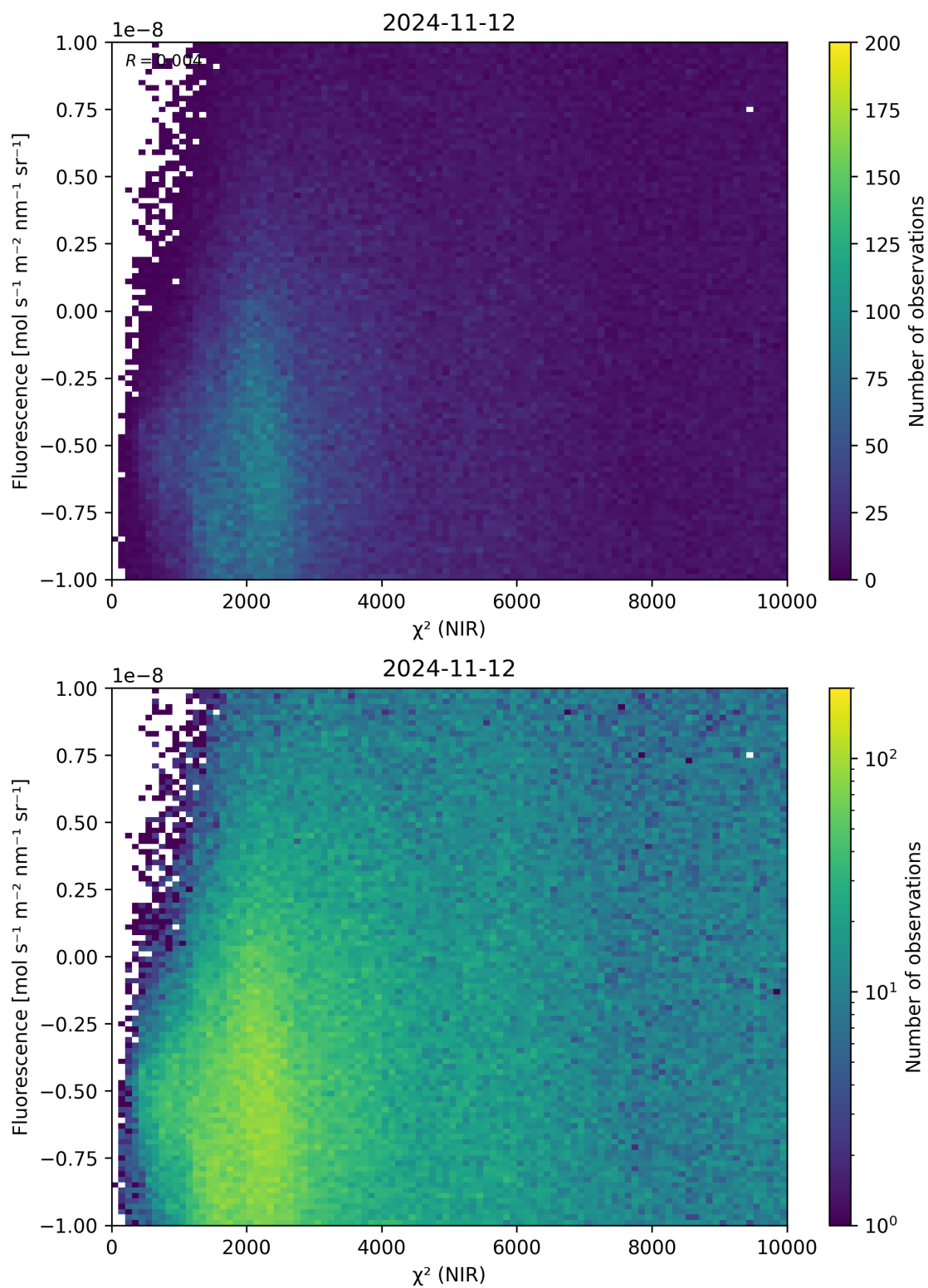
Figure 45: Scatter density plot of “ \chi^2 (NIR)” against “Fluorescence” for 2024-11-11 to 2024-11-13.
