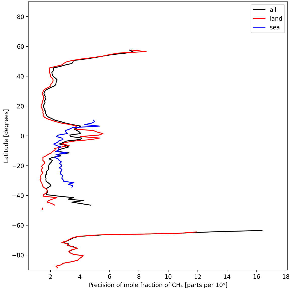
Figure 13: Zonal average of “Precision of mole fraction of CH 4 ” for 2024-11-11 to 2024-11-13.
