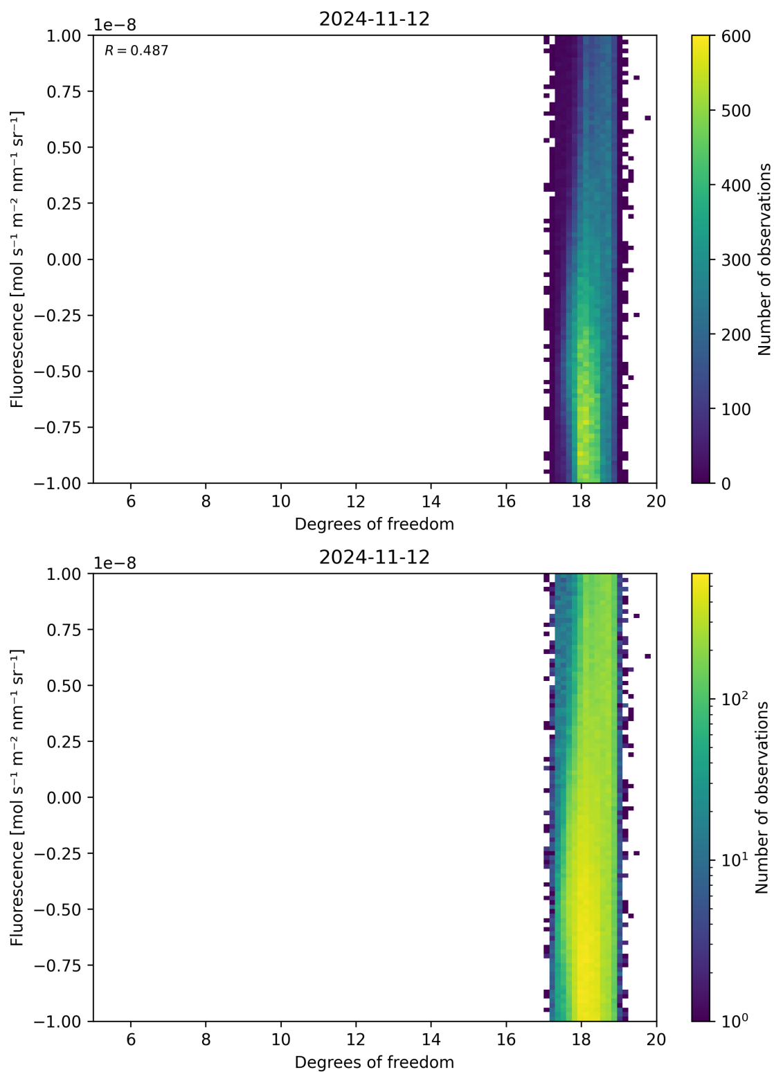
Figure 51: Scatter density plot of “Degrees of freedom” against “Fluorescence” for 2024-11-11 to 2024-11-13.
