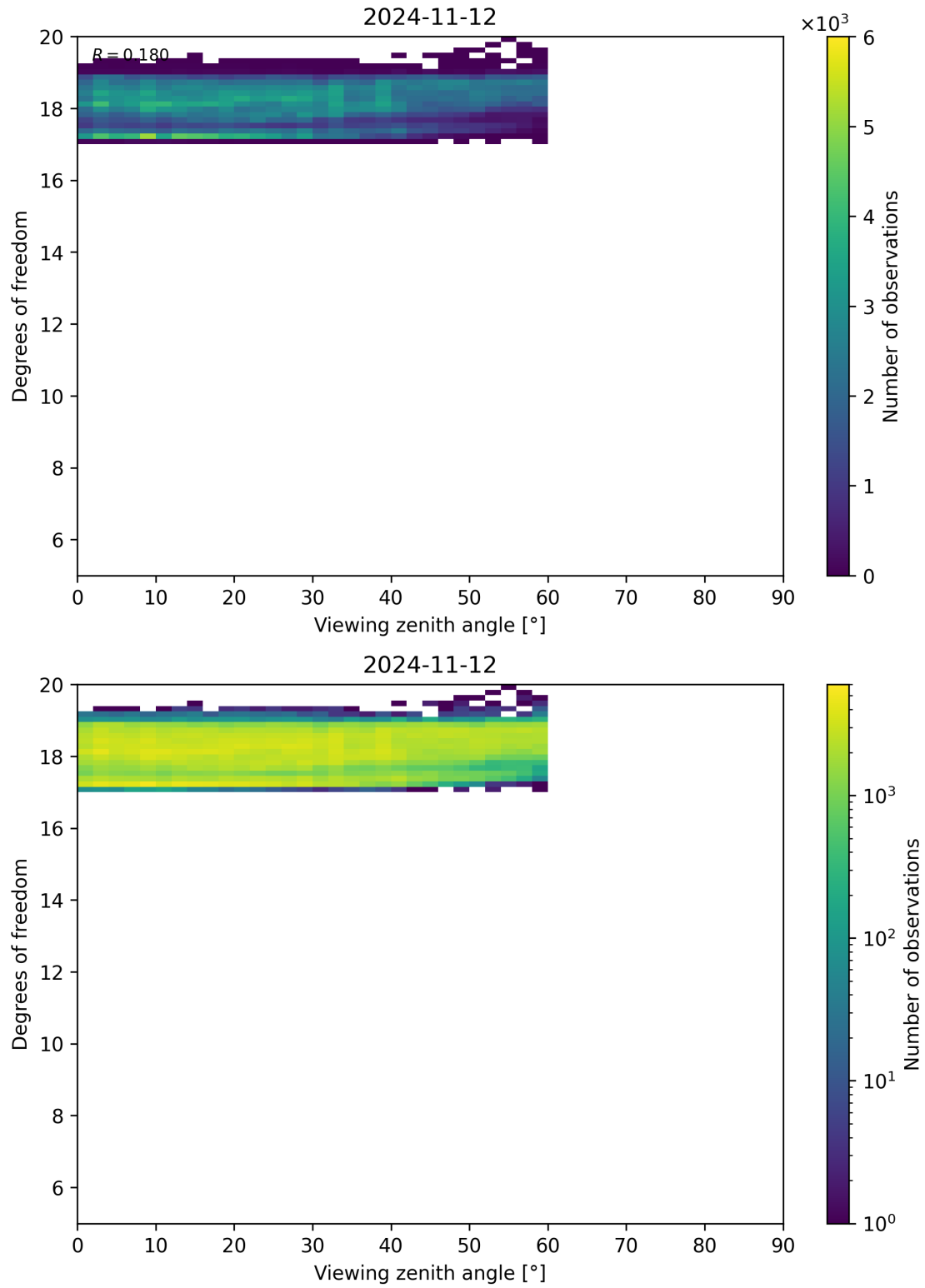
Figure 107: Scatter density plot of “Viewing zenith angle” against “Degrees of freedom” for 2024-11-11 to 2024-11-13.
