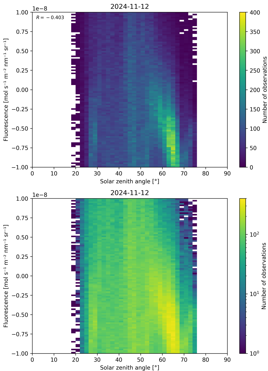
Figure 97: Scatter density plot of “Solar zenith angle” against “Fluorescence” for 2024-11-11 to 2024-11-13.
