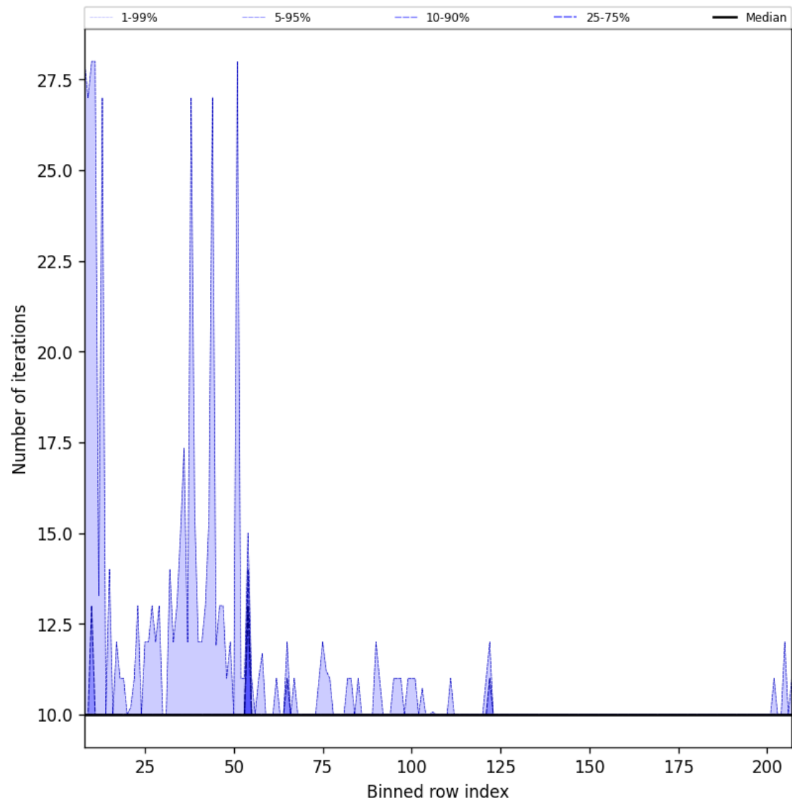
Figure 42: Along track statistics of “Number of iterations” for 2024-11-12 to 2024-11-14
