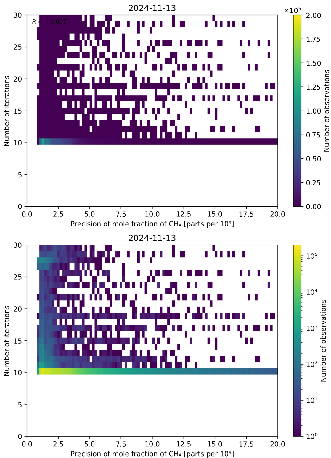
Figure 83: Scatter density plot of “Precision of mole fraction of CH 4 ” against “Number of iterations” for 2024-11-12 to 2024-11-14.
