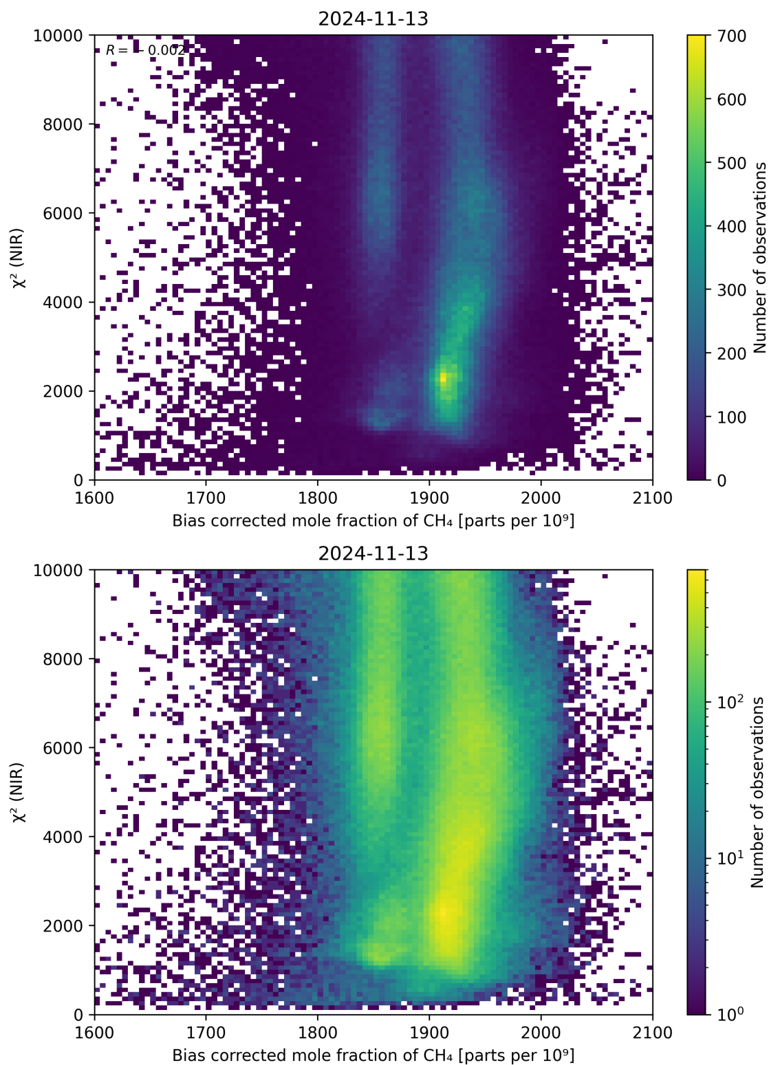
Figure 63: Scatter density plot of “Bias corrected mole fraction of \text{CH}_4 ” against “ \chi^2 (NIR)” for 2024-11-12 to 2024-11-14.
