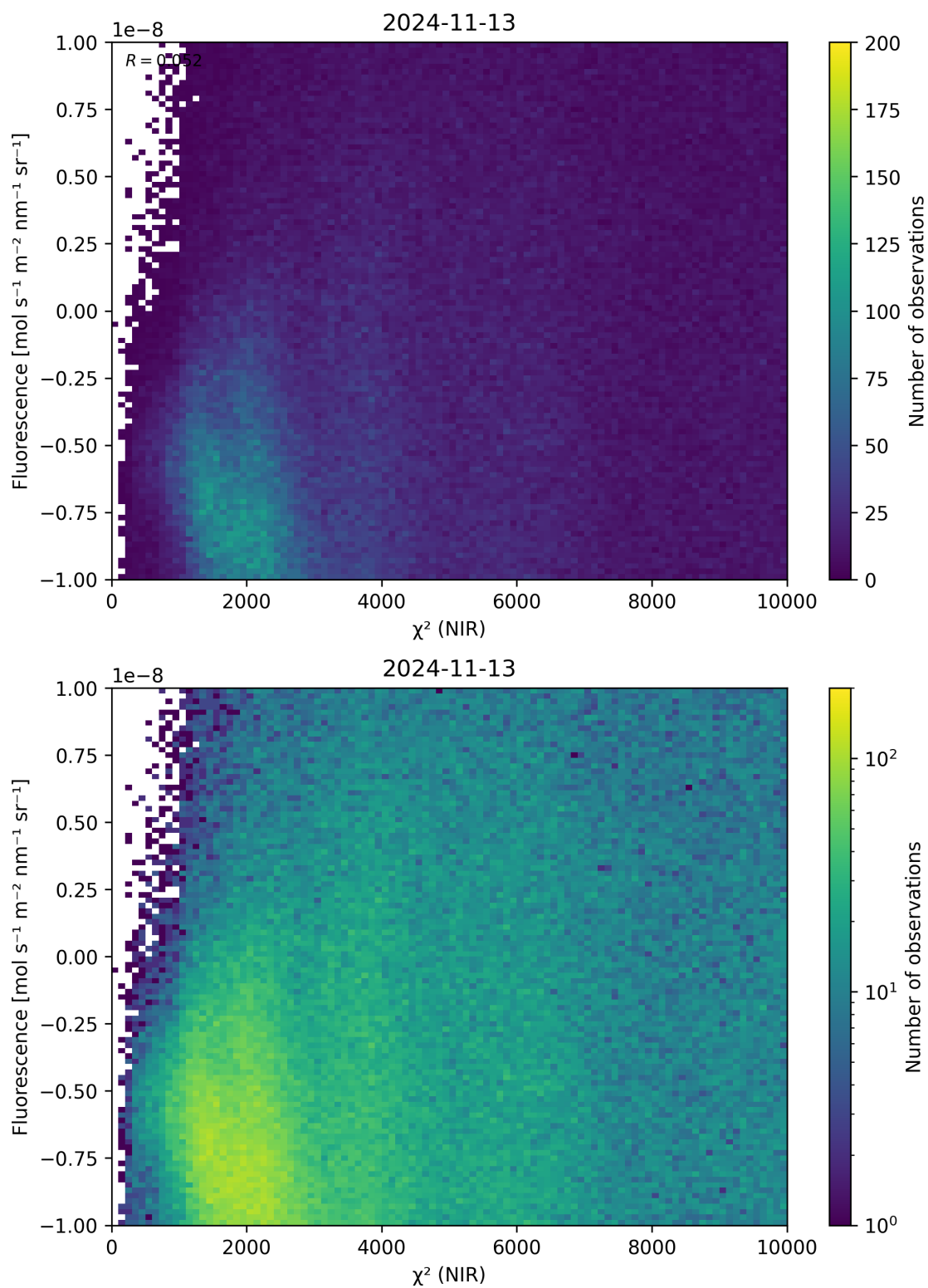
Figure 45: Scatter density plot of “ \chi^2 (NIR)” against “Fluorescence” for 2024-11-12 to 2024-11-14.
