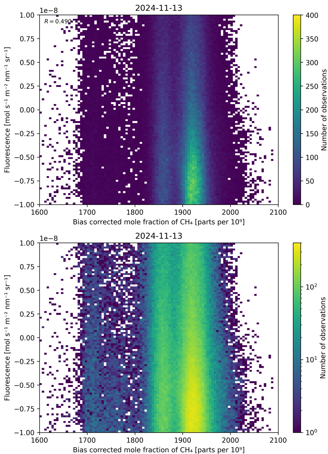
Figure 66: Scatter density plot of “Bias corrected mole fraction of \text{CH}_4 ” against “Fluorescence” for 2024-11-12 to 2024-11-14.
