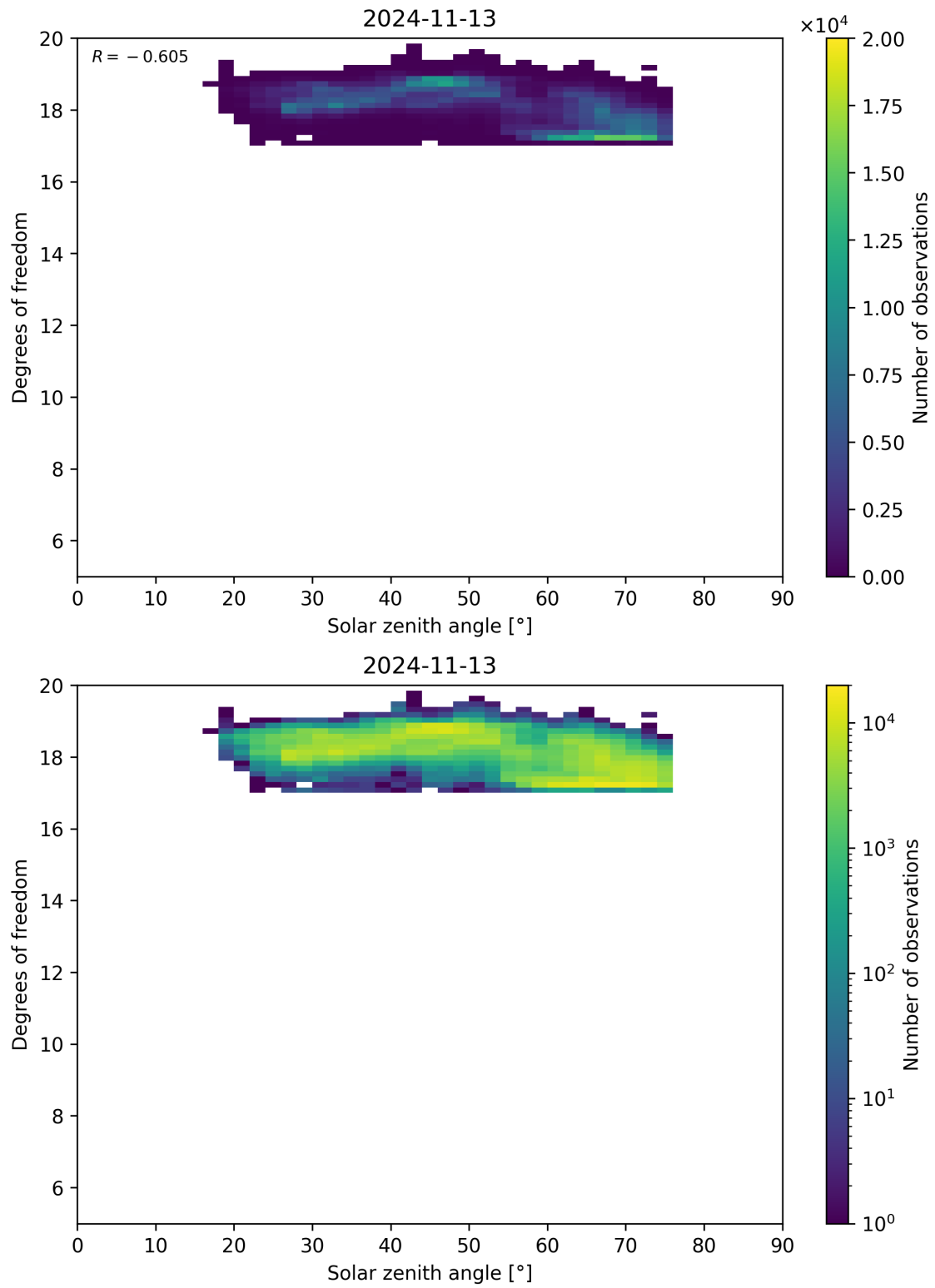
Figure 96: Scatter density plot of “Solar zenith angle” against “Degrees of freedom” for 2024-11-12 to 2024-11-14.
