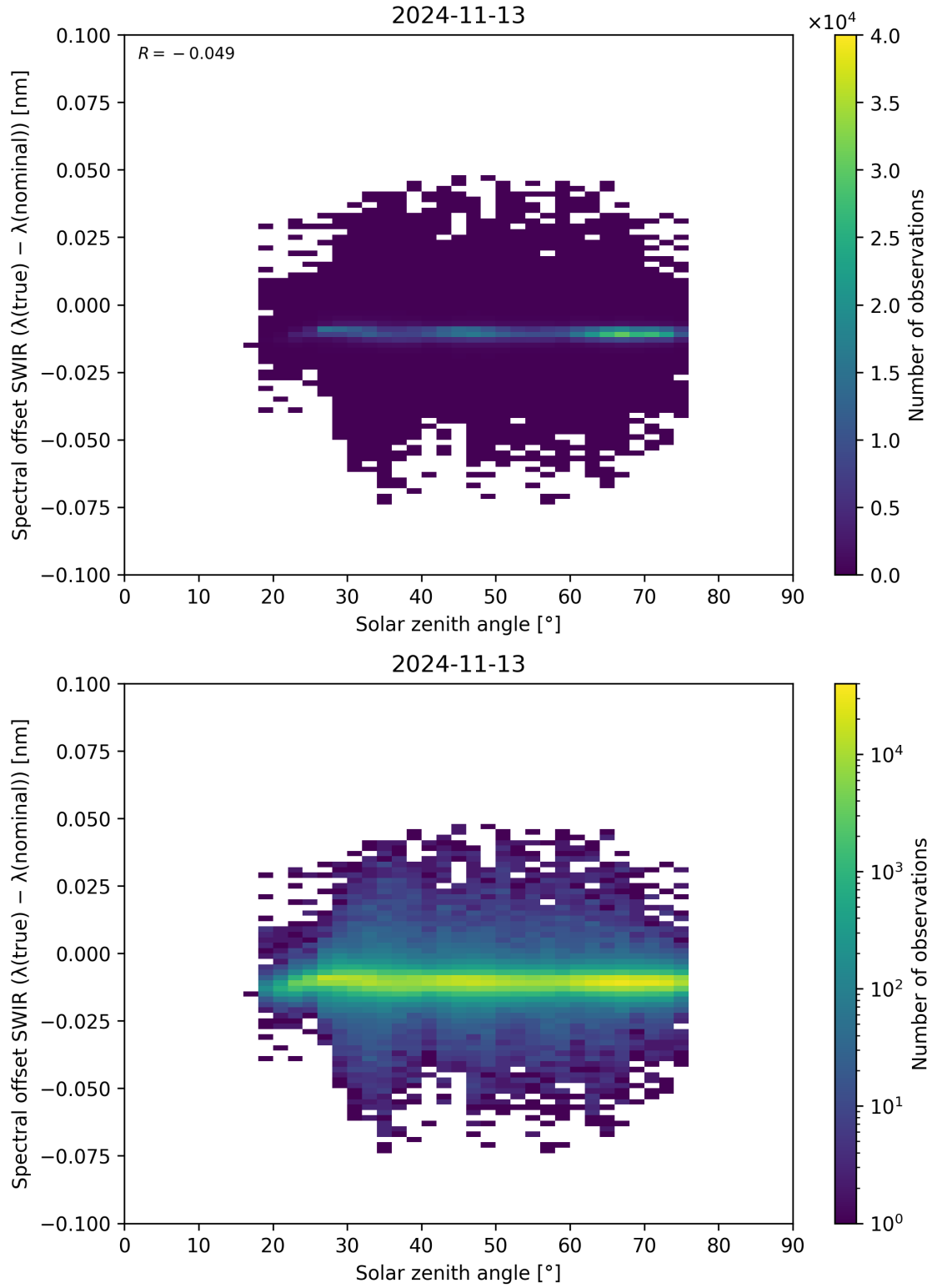
Figure 104: Scatter density plot of “Solar zenith angle” against “Spectral offset SWIR ( \lambda_{\text{true}} - \lambda_{\text{nominal}} )” for 2024-11-12 to 2024-11-14.
