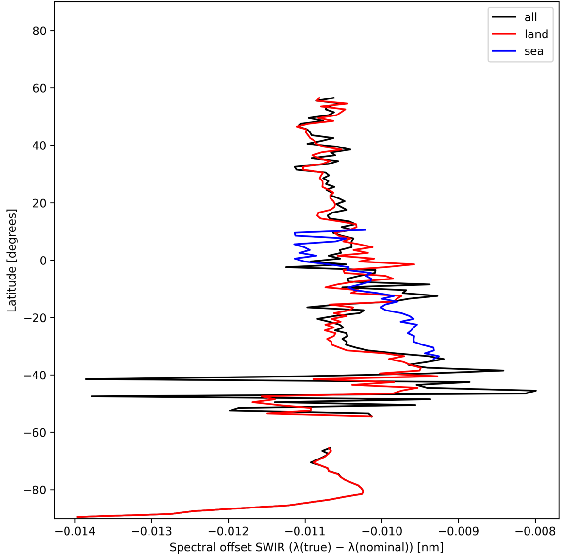
Figure 16: Zonal average of “Spectral offset SWIR ( \lambda_{\text{true}} - \lambda_{\text{nominal}} )” for 2024-11-12 to 2024-11-14.
