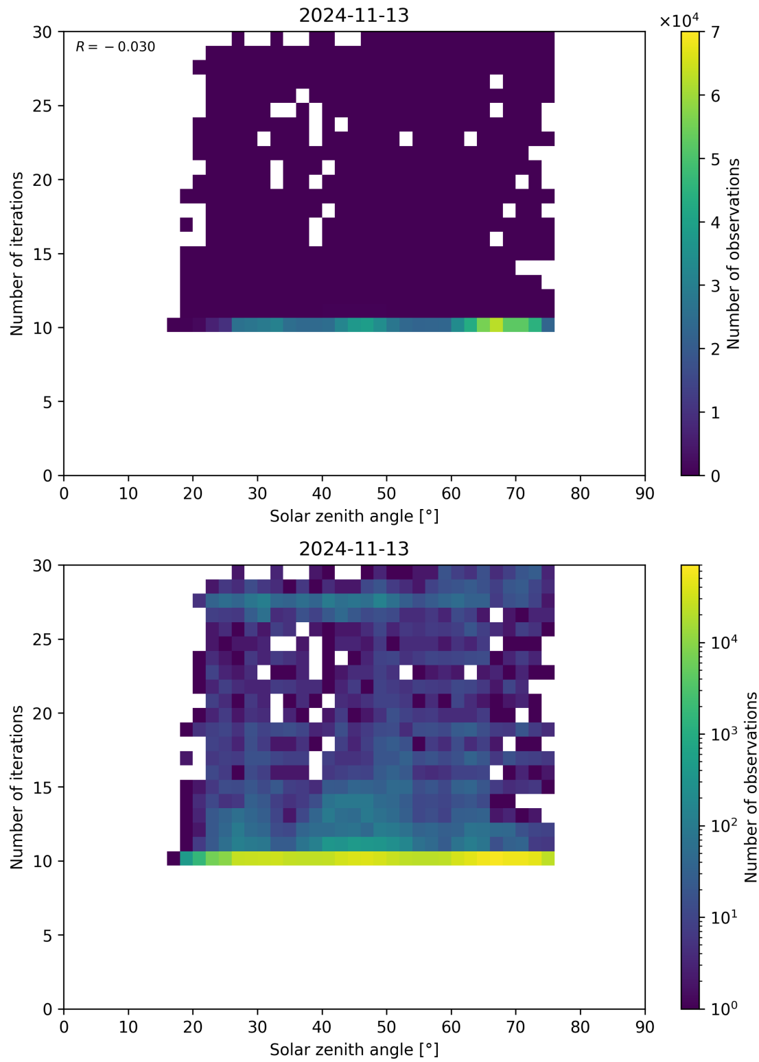
Figure 102: Scatter density plot of “Solar zenith angle” against “Number of iterations” for 2024-11-12 to 2024-11-14.
