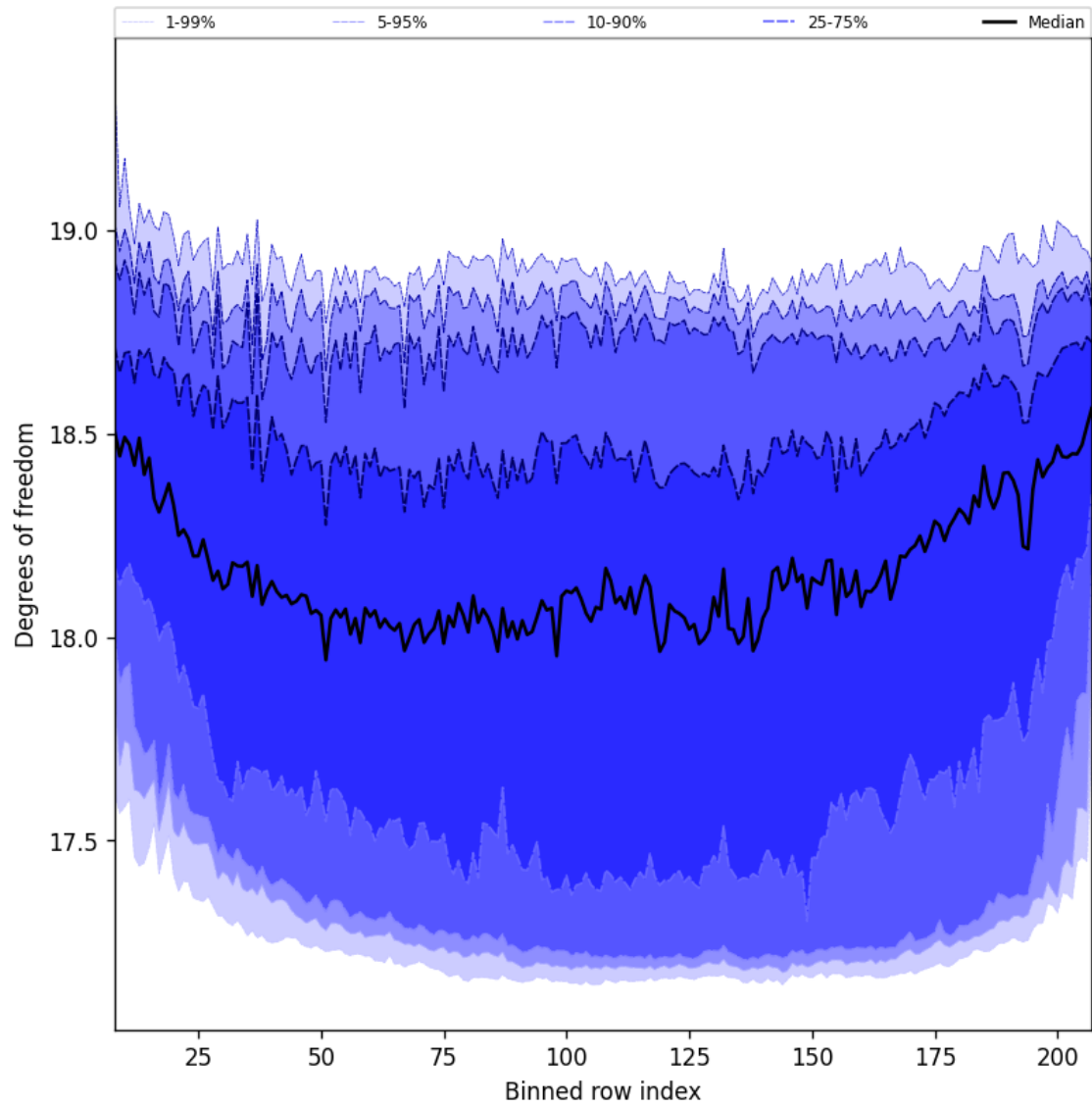
Figure 41: Along track statistics of “Degrees of freedom” for 2024-11-12 to 2024-11-14
