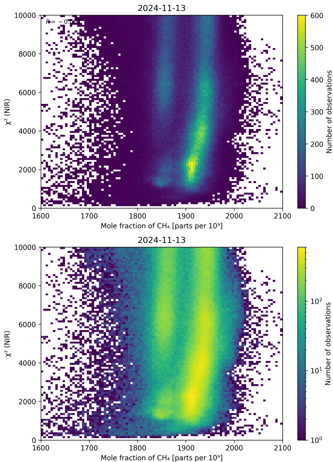
Figure 70: Scatter density plot of “Mole fraction of \text{CH}_4 ” against “ \chi^2 (NIR)” for 2024-11-12 to 2024-11-14.
