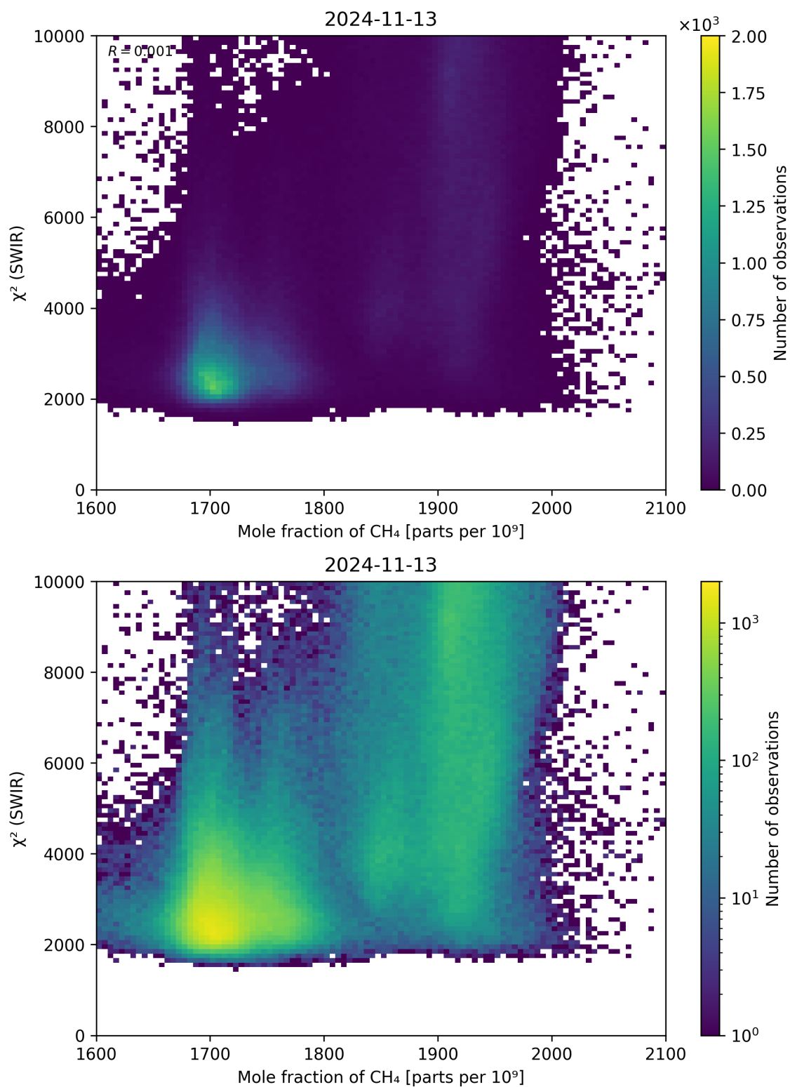
Figure 71: Scatter density plot of “Mole fraction of CH 4 ” against “ \chi^2 (SWIR)” for 2024-11-12 to 2024-11-14.
