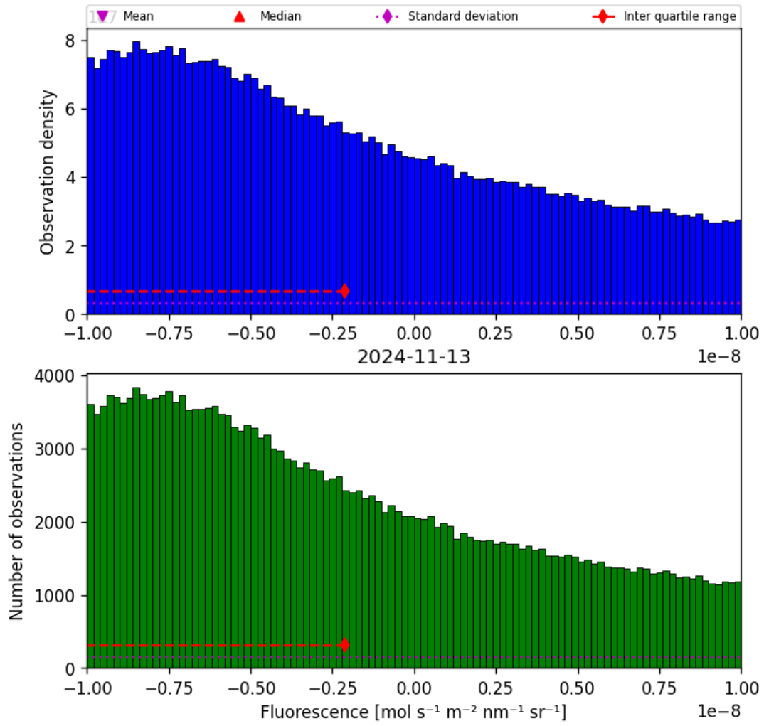
Figure 32: Histogram of “Fluorescence” for 2024-11-12 to 2024-11-14
