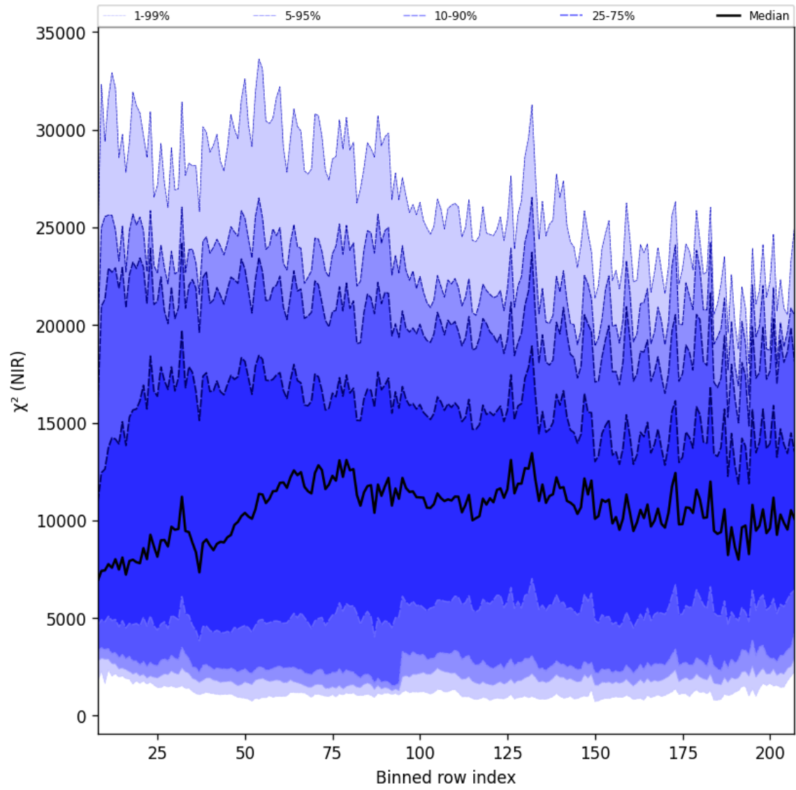
Figure 40: Along track statistics of “ \chi^2 (NIR)” for 2024-11-12 to 2024-11-14
