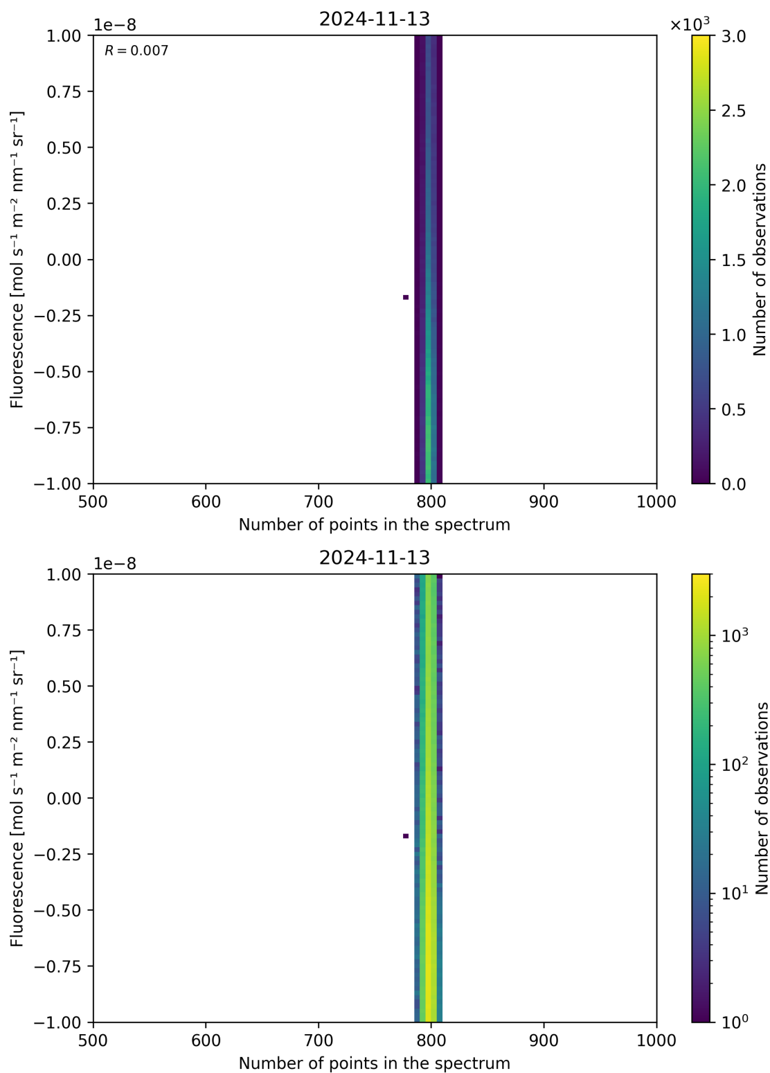
Figure 91: Scatter density plot of “Number of points in the spectrum” against “Fluorescence” for 2024-11-12 to 2024-11-14.
