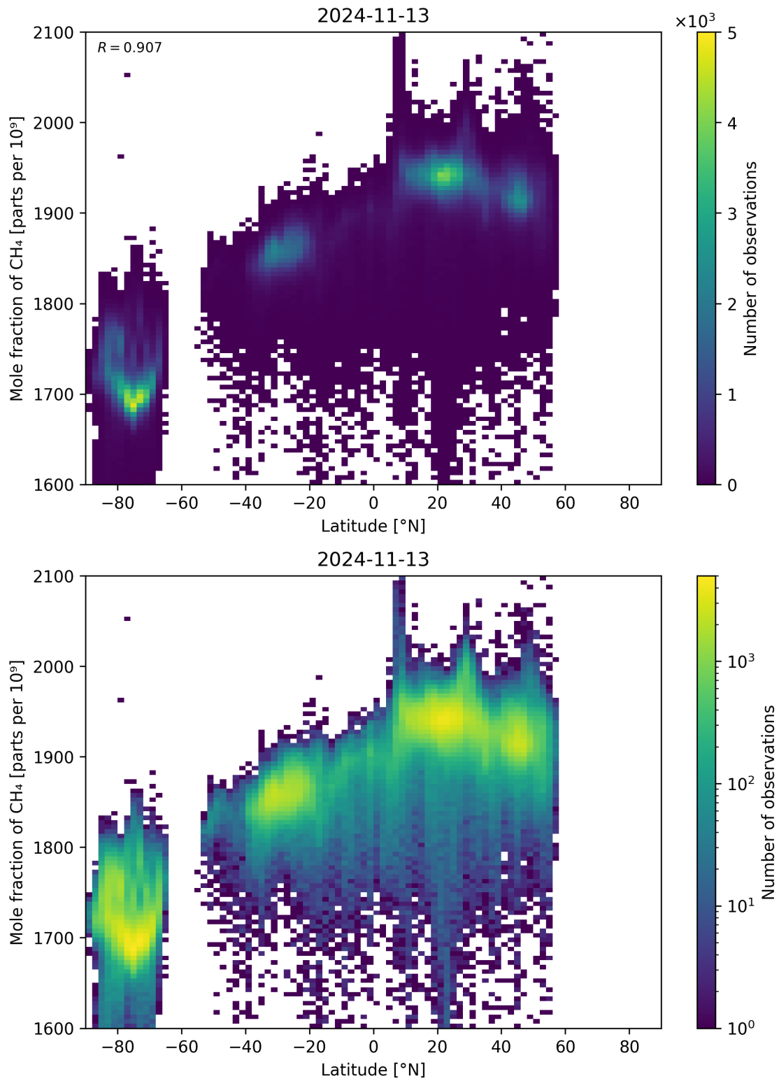
Figure 57: Scatter density plot of “Latitude” against “Mole fraction of \text{CH}_4 ” for 2024-11-12 to 2024-11-14.
