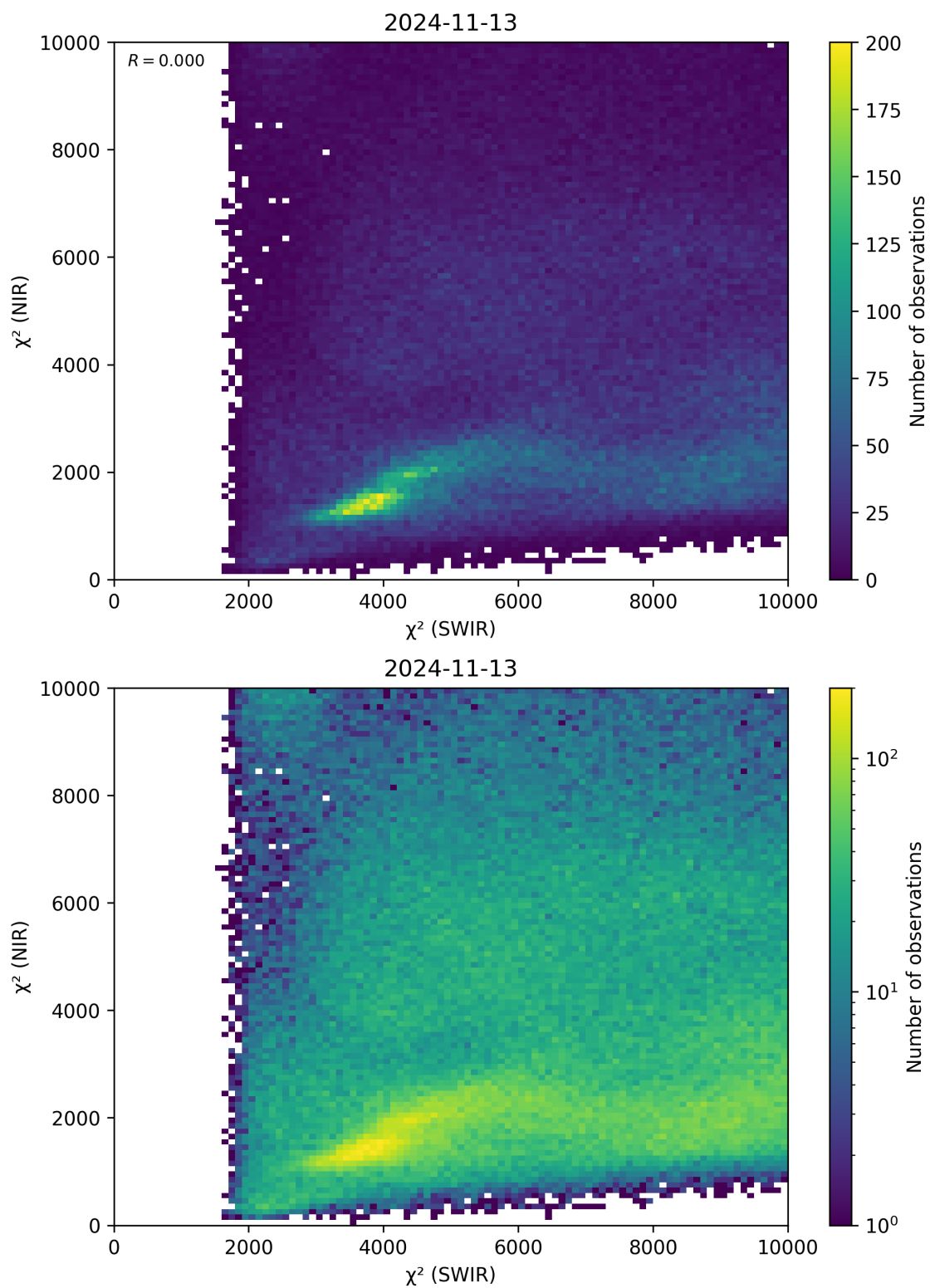
Figure 47: Scatter density plot of “ \chi^2 (SWIR)” against “ \chi^2 (NIR)” for 2024-11-12 to 2024-11-14.
