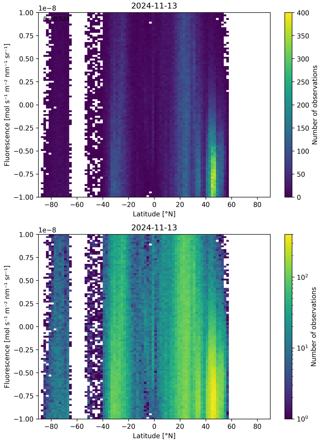
Figure 56: Scatter density plot of “Latitude” against “Fluorescence” for 2024-11-12 to 2024-11-14.
