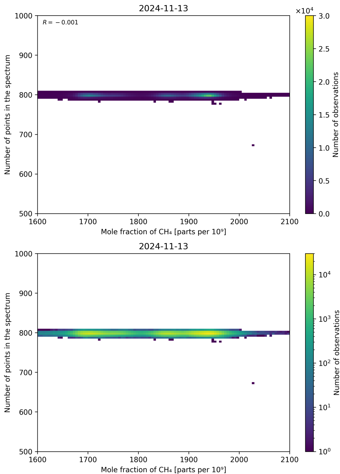
Figure 77: Scatter density plot of “Mole fraction of CH 4 ” against “Number of points in the spectrum” for 2024-11-12 to 2024-11-14.
