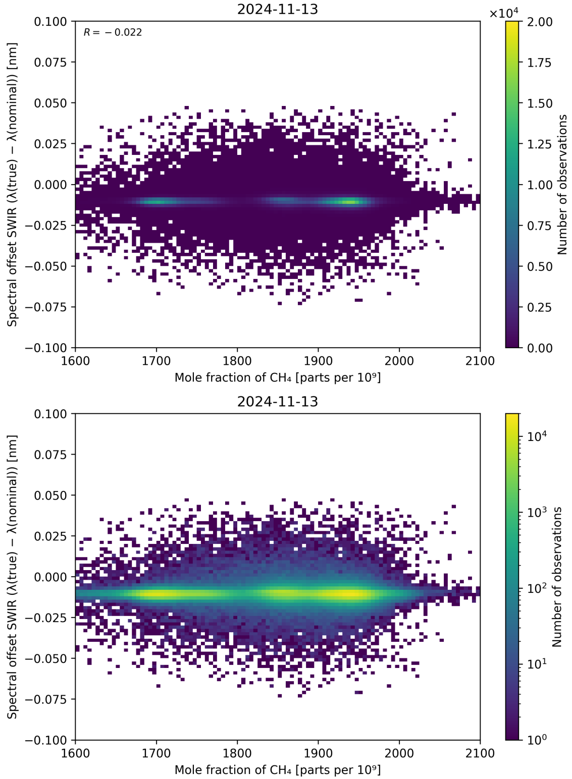
Figure 86: Scatter density plot of “Mole fraction of CH 4 ” against “Spectral offset SWIR ( \lambda_{\text{true}} - \lambda_{\text{nominal}} )” for 2024-11-12 to 2024-11-14.
