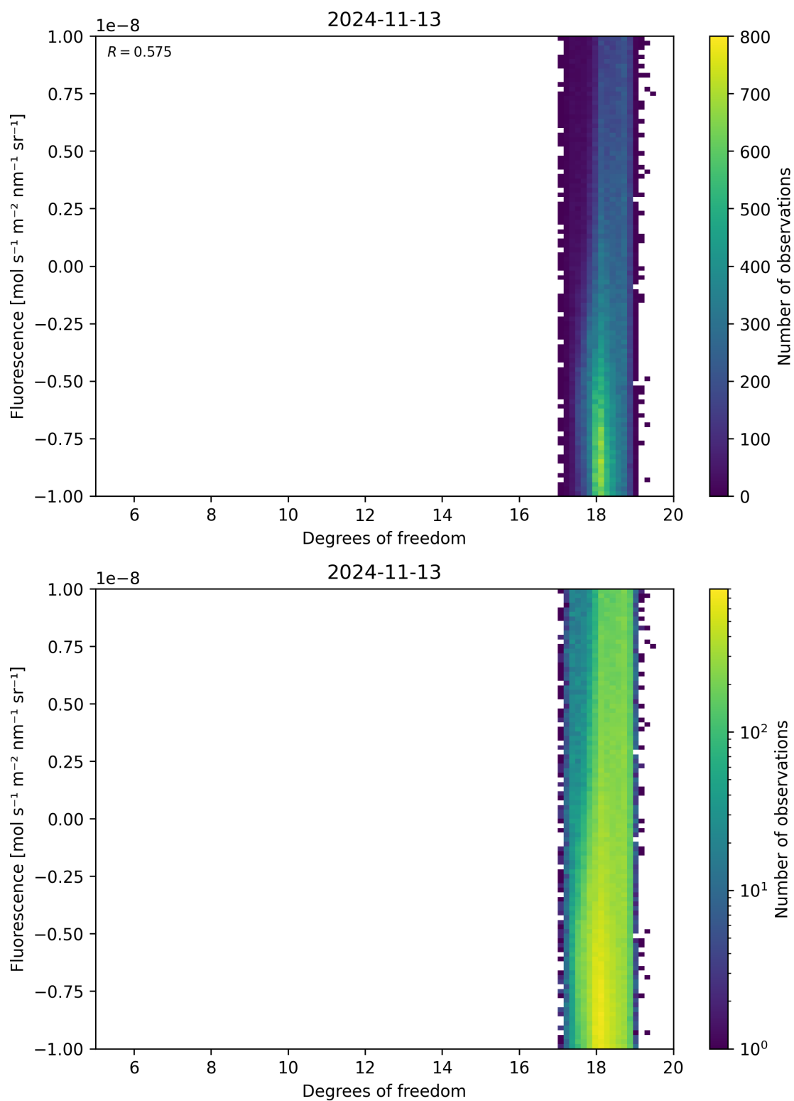
Figure 51: Scatter density plot of “Degrees of freedom” against “Fluorescence” for 2024-11-12 to 2024-11-14.
