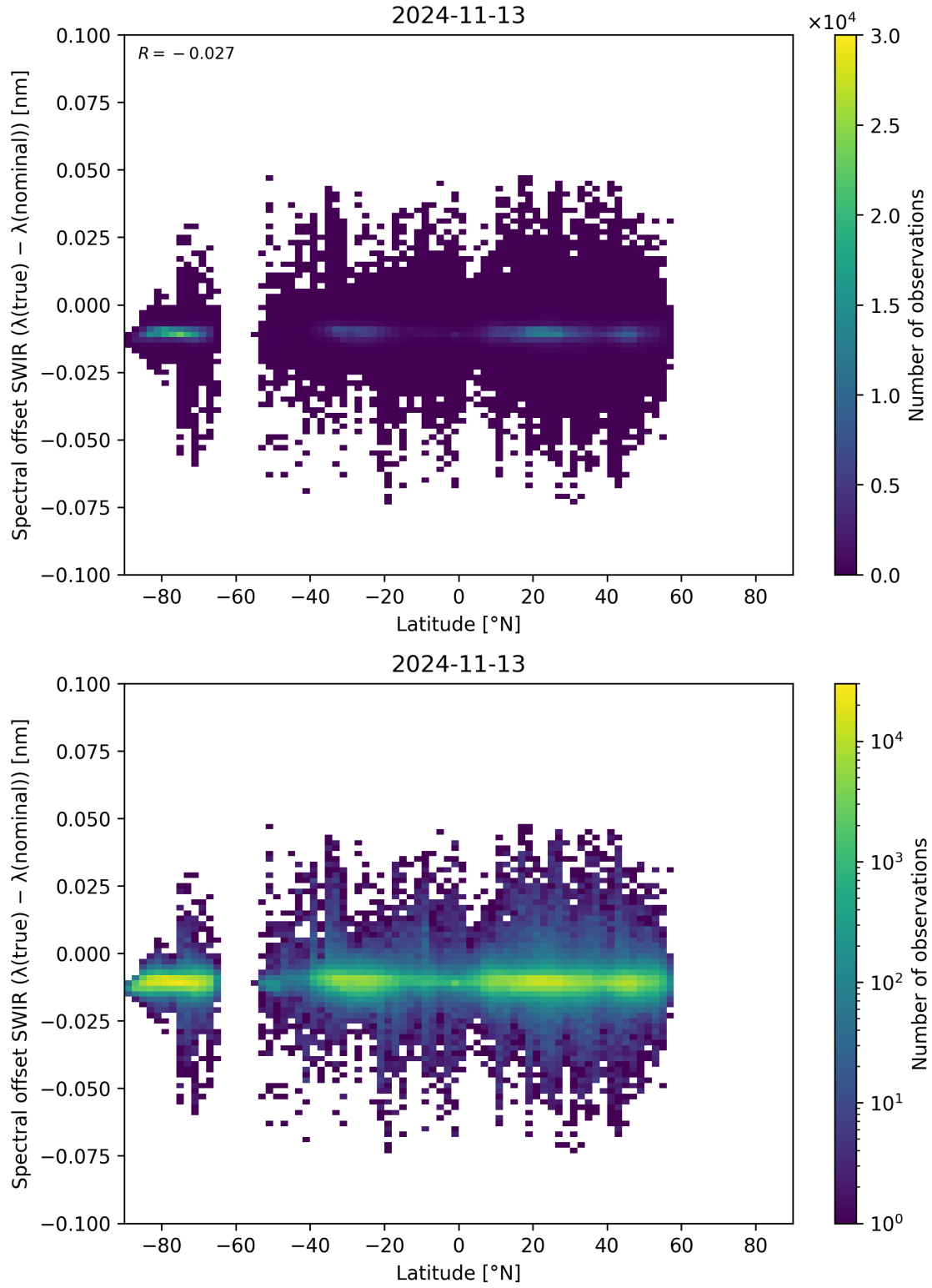
Figure 62: Scatter density plot of “Latitude” against “Spectral offset SWIR ( \lambda_{\text{true}} - \lambda_{\text{nominal}} )” for 2024-11-12 to 2024-11-14.
