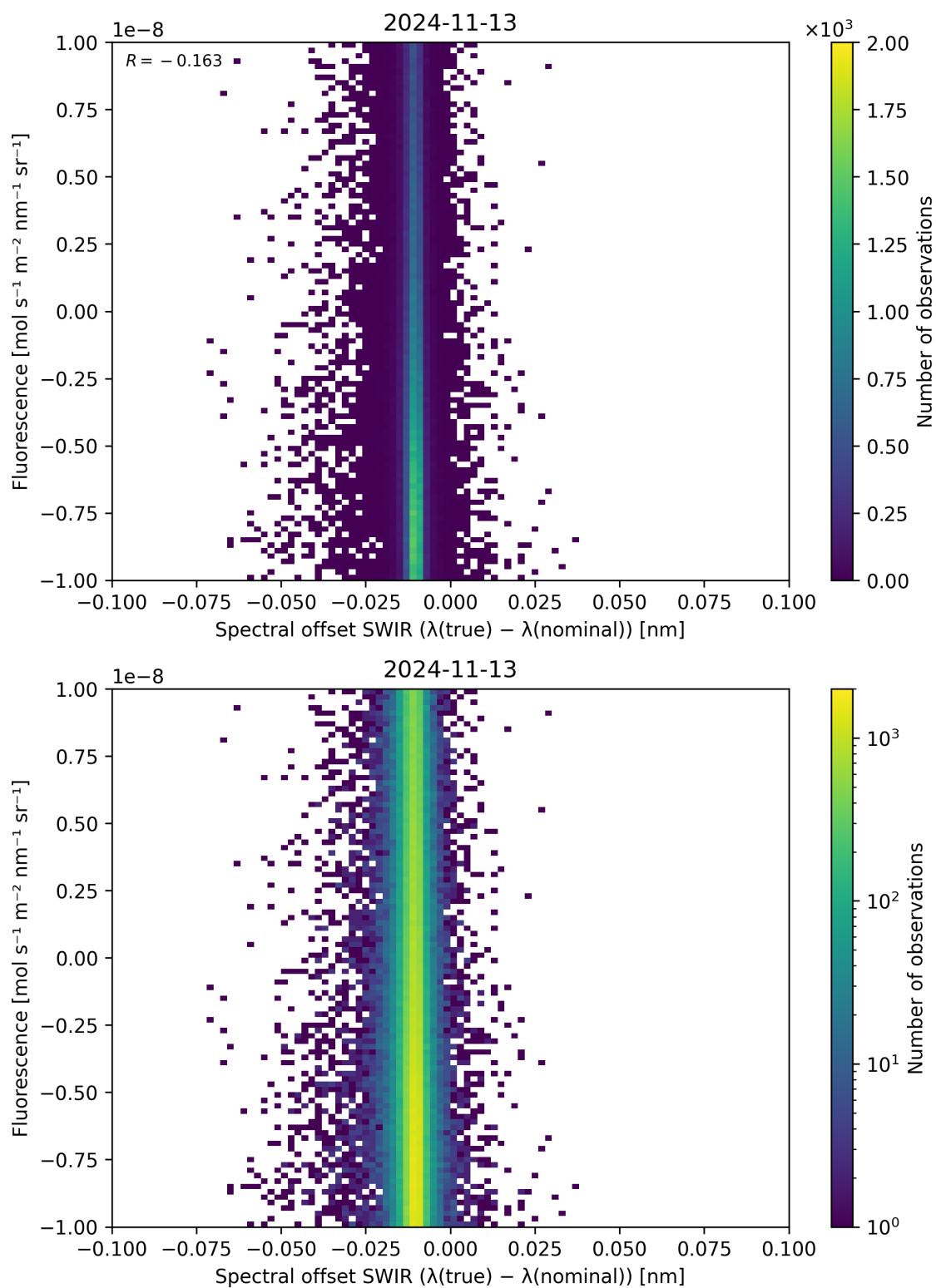
Figure 120: Scatter density plot of “Spectral offset SWIR ( \lambda_{\text{true}} - \lambda_{\text{nominal}} )” against “Fluorescence” for 2024-11-12 to 2024-11-14.
