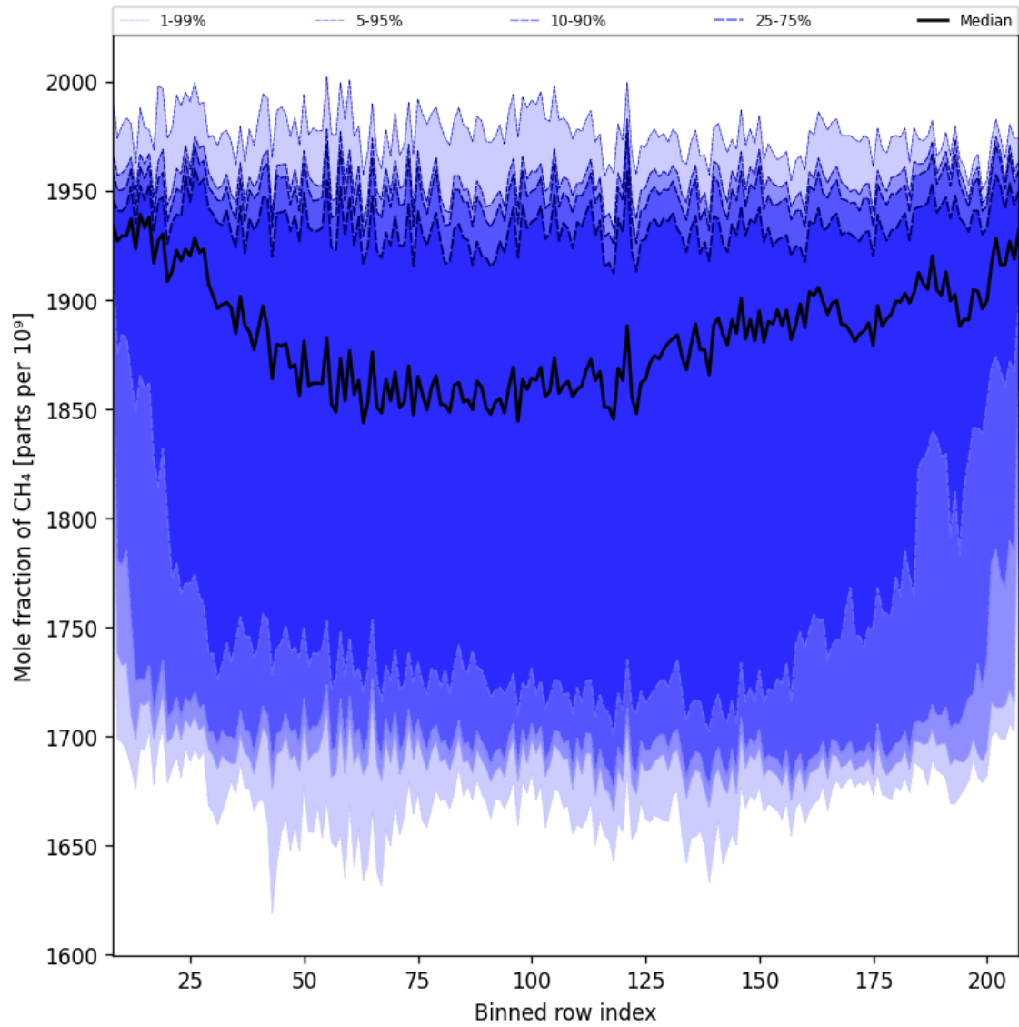
Figure 34: Along track statistics of “Mole fraction of CH 4 ” for 2024-11-12 to 2024-11-14
