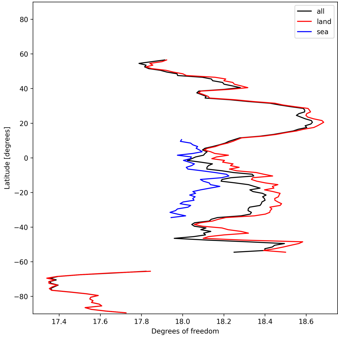
Figure 19: Zonal average of “Degrees of freedom” for 2024-11-12 to 2024-11-14.
