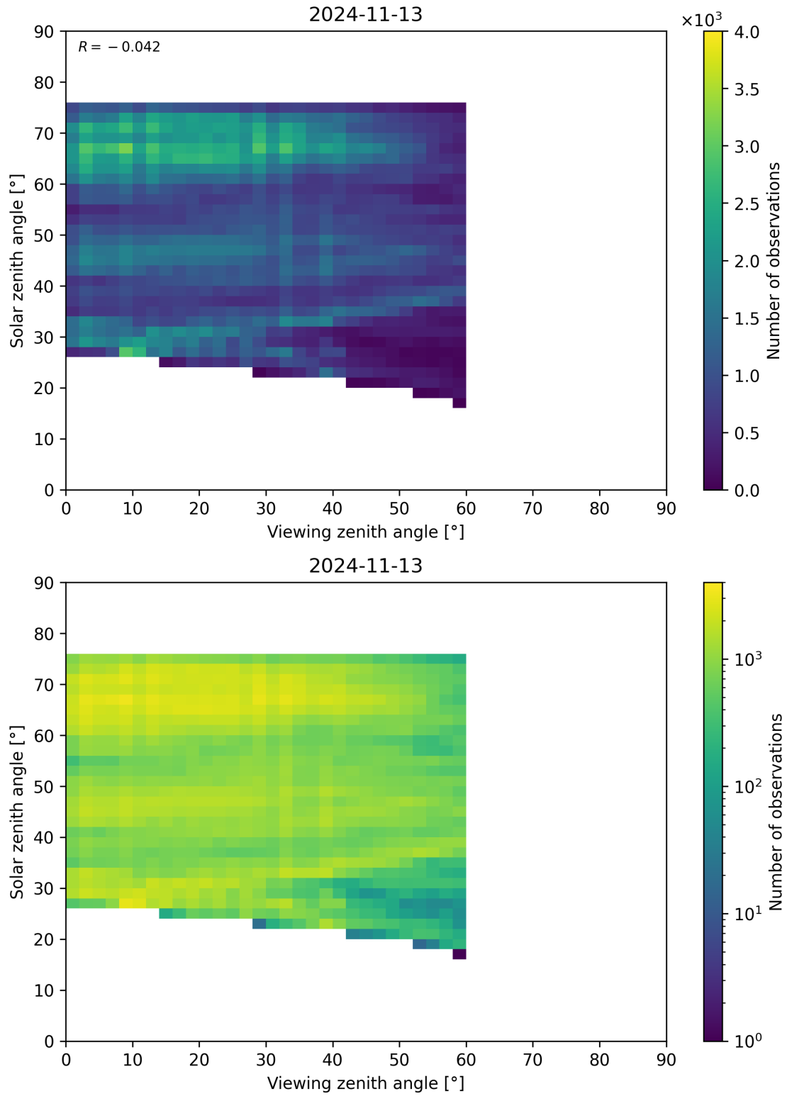
Figure 115: Scatter density plot of “Viewing zenith angle” against “Solar zenith angle” for 2024-11-12 to 2024-11-14.
