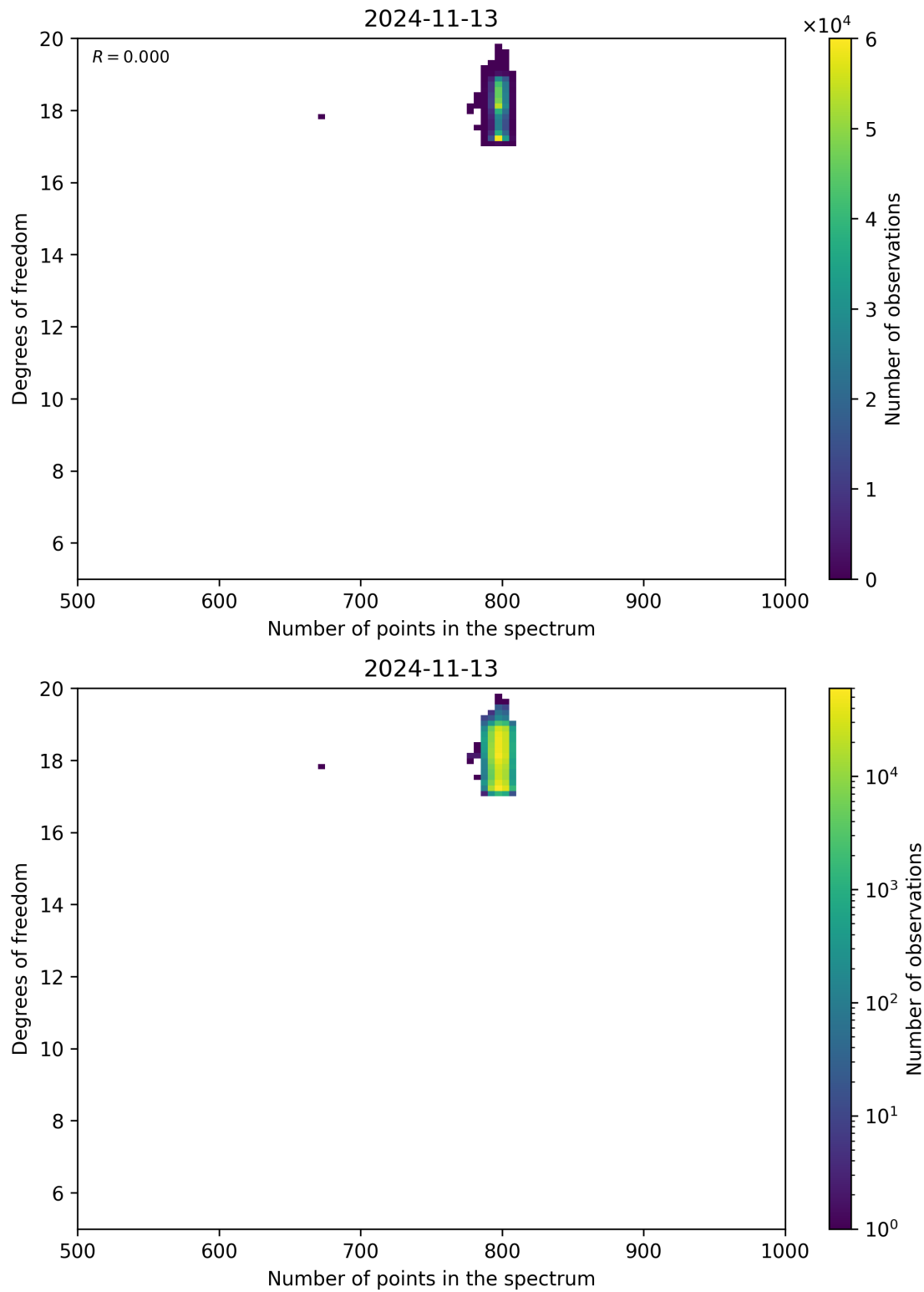
Figure 90: Scatter density plot of “Number of points in the spectrum” against “Degrees of freedom” for 2024-11-12 to 2024-11-14.
