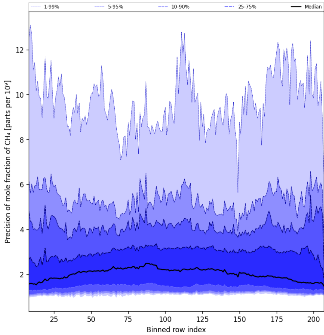
Figure 35: Along track statistics of “Precision of mole fraction of CH 4 ” for 2024-11-12 to 2024-11-14
