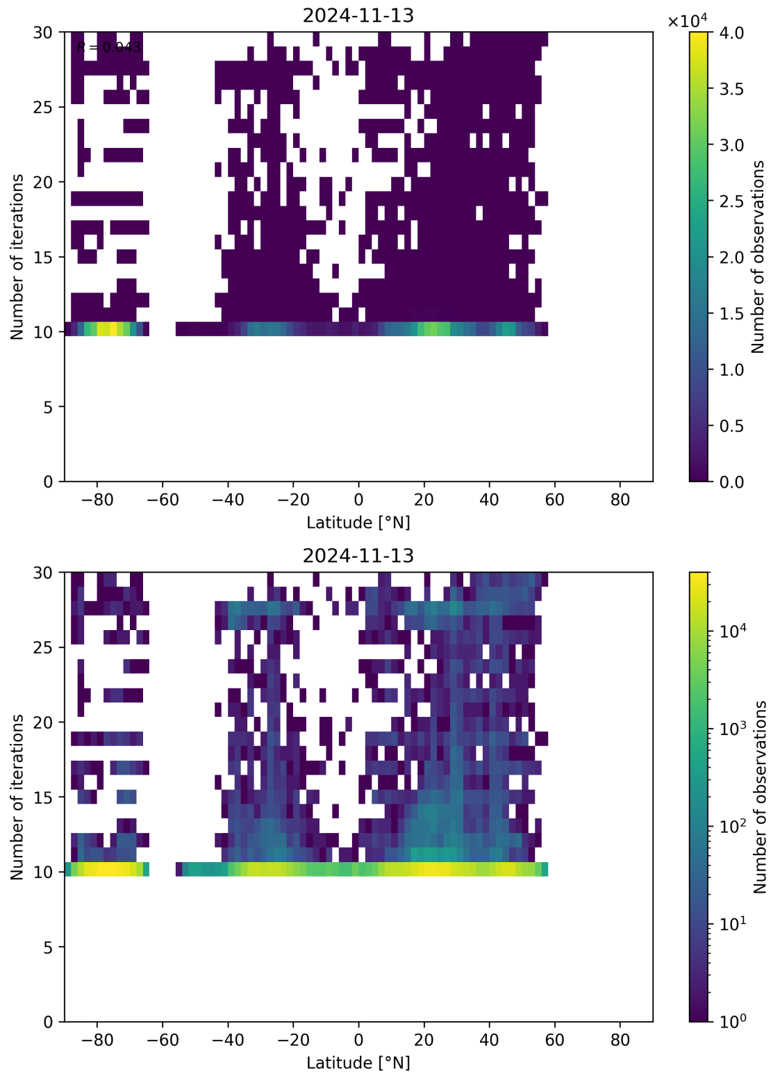
Figure 60: Scatter density plot of “Latitude” against “Number of iterations” for 2024-11-12 to 2024-11-14.
