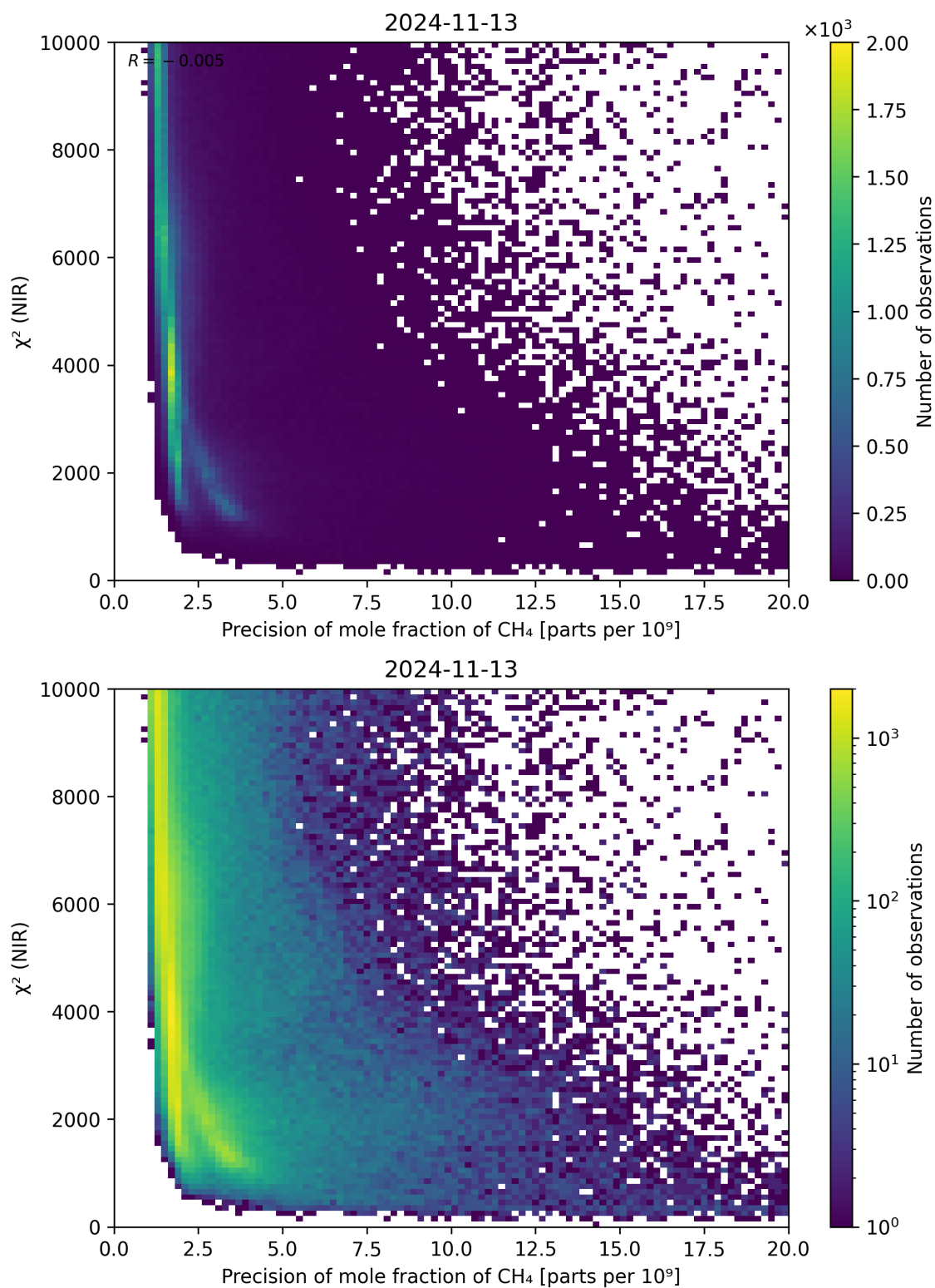
Figure 78: Scatter density plot of “Precision of mole fraction of CH 4 ” against “ \chi^2 (NIR)” for 2024-11-12 to 2024-11-14.
