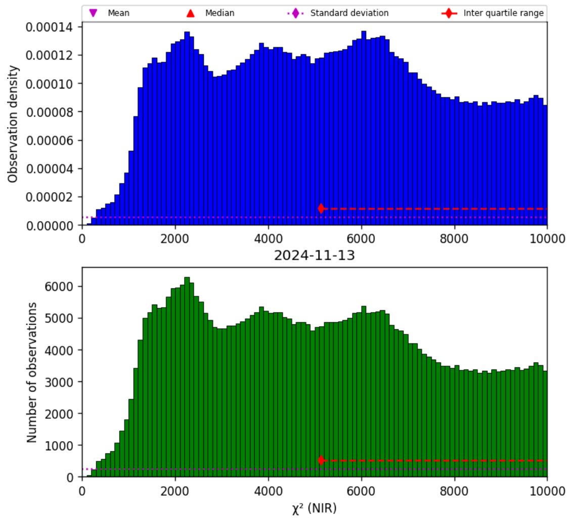
Figure 29: Histogram of “ \chi^2 (NIR)” for 2024-11-12 to 2024-11-14
