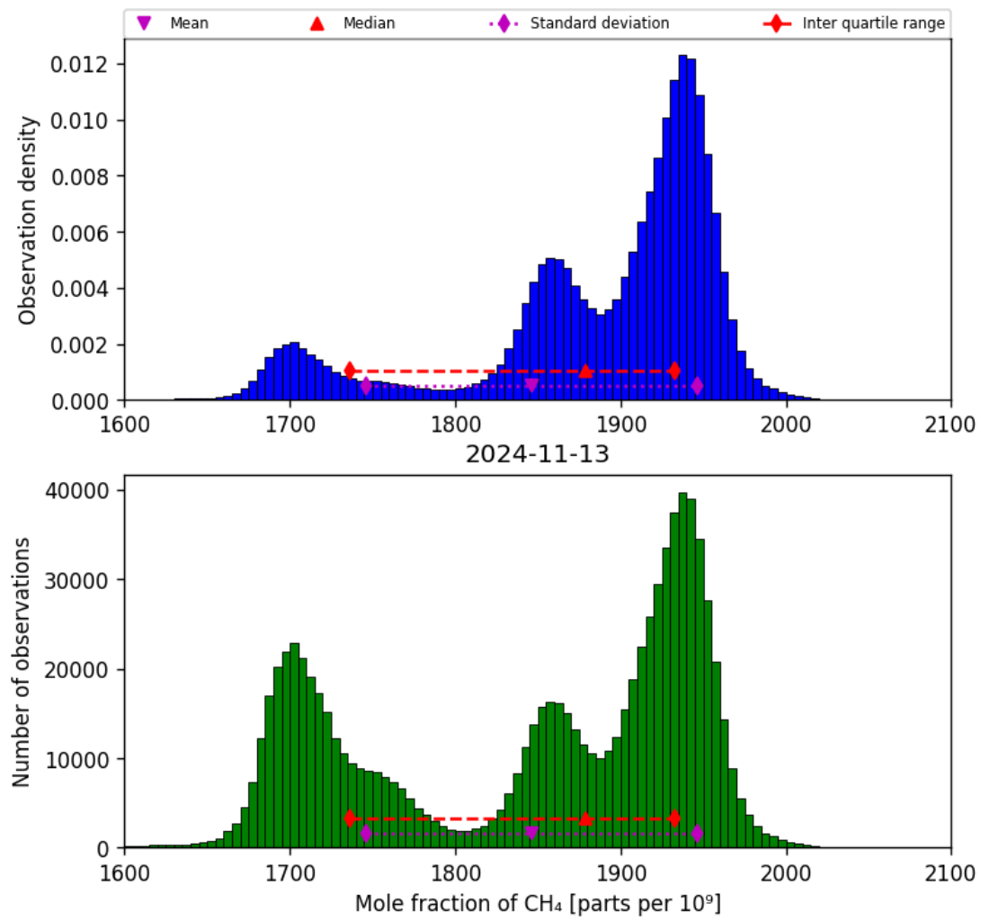
Figure 23: Histogram of “Mole fraction of CH 4 ” for 2024-11-12 to 2024-11-14
