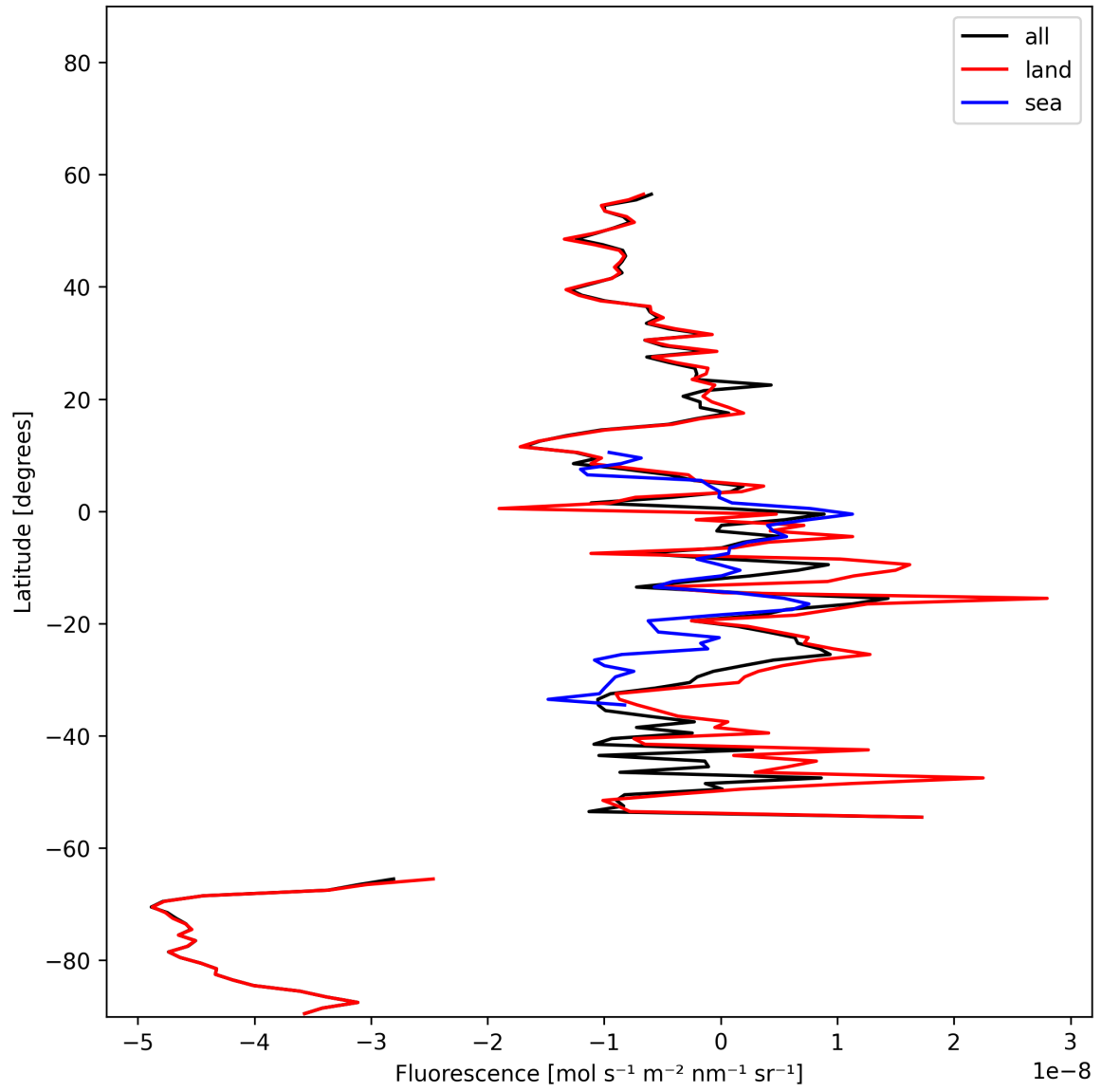
Figure 21: Zonal average of “Fluorescence” for 2024-11-12 to 2024-11-14.
