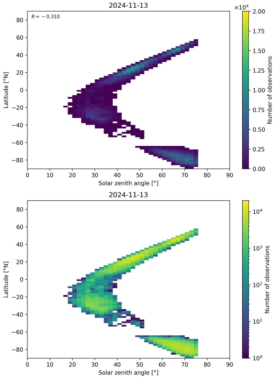
Figure 98: Scatter density plot of “Solar zenith angle” against “Latitude” for 2024-11-12 to 2024-11-14.
