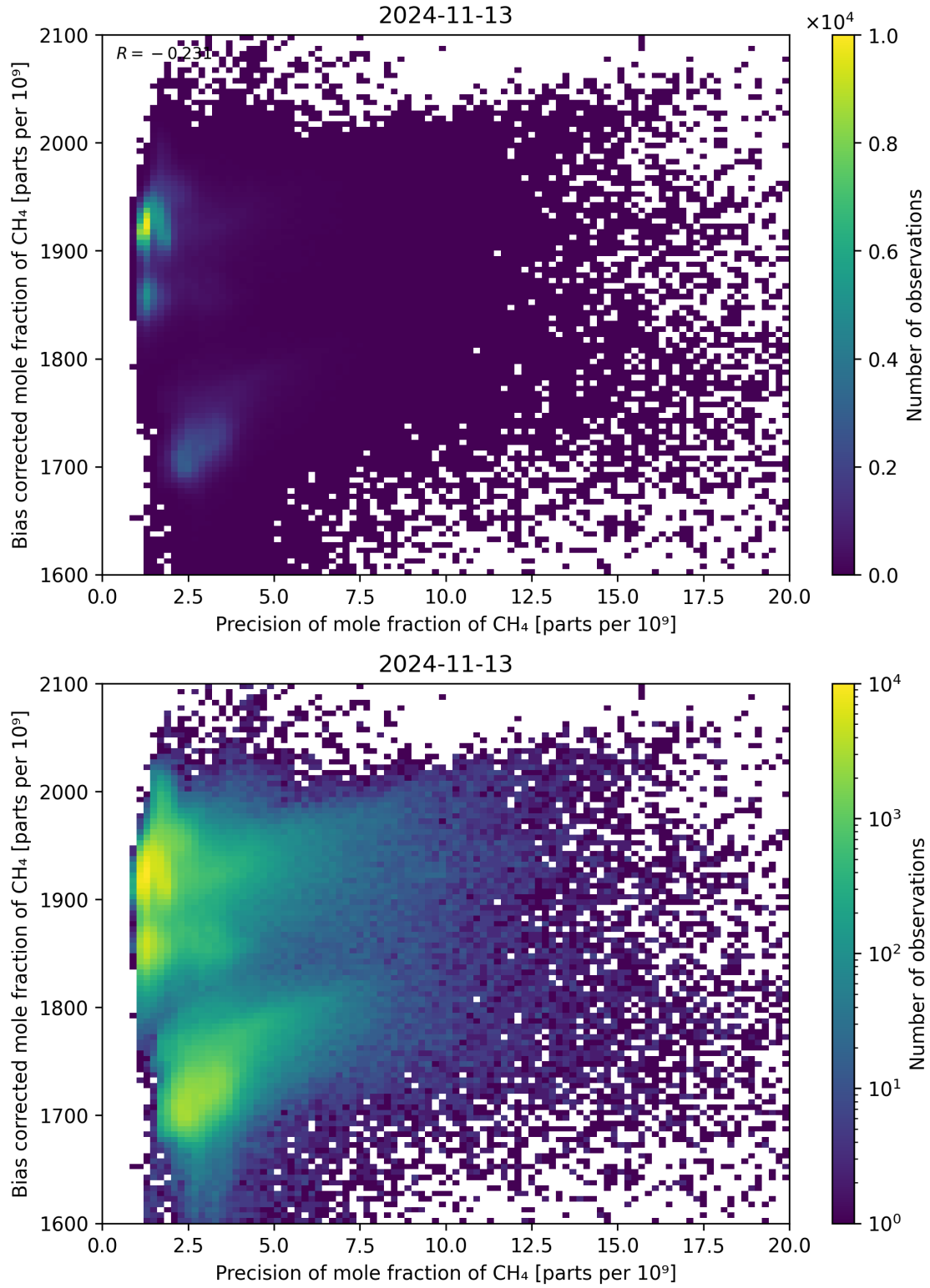
Figure 82: Scatter density plot of “Precision of mole fraction of CH 4 ” against “Bias corrected mole fraction of CH 4 ” for 2024-11-12 to 2024-11-14.
