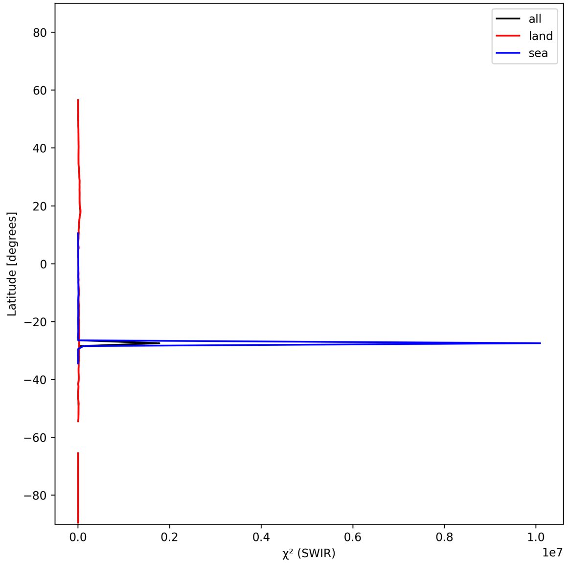
Figure 17: Zonal average of “ \chi^2 (SWIR)” for 2024-11-12 to 2024-11-14.
