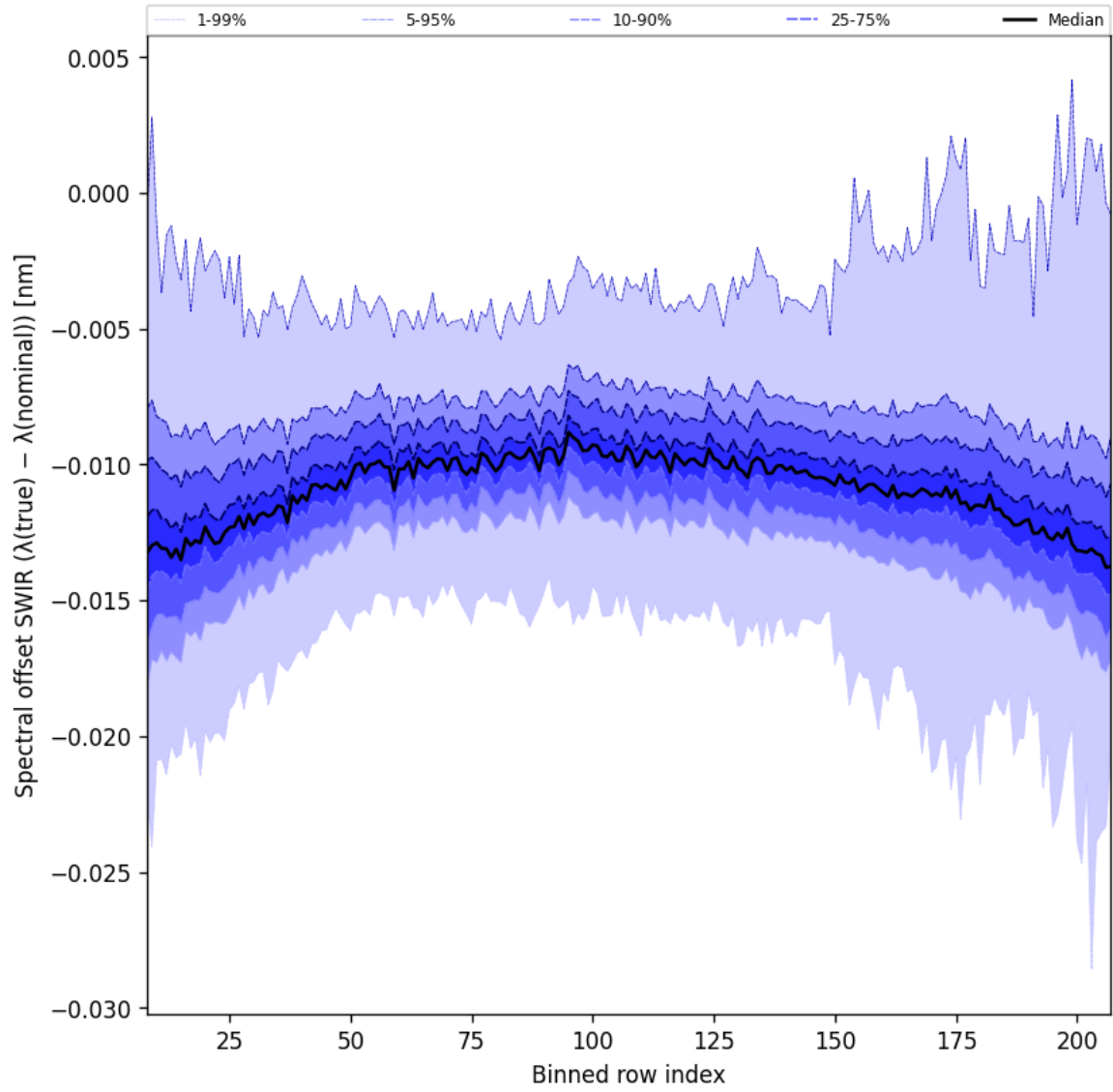
Figure 38: Along track statistics of “Spectral offset SWIR ( \lambda_{\text{true}} - \lambda_{\text{nominal}} )” for 2024-11-12 to 2024-11-14
