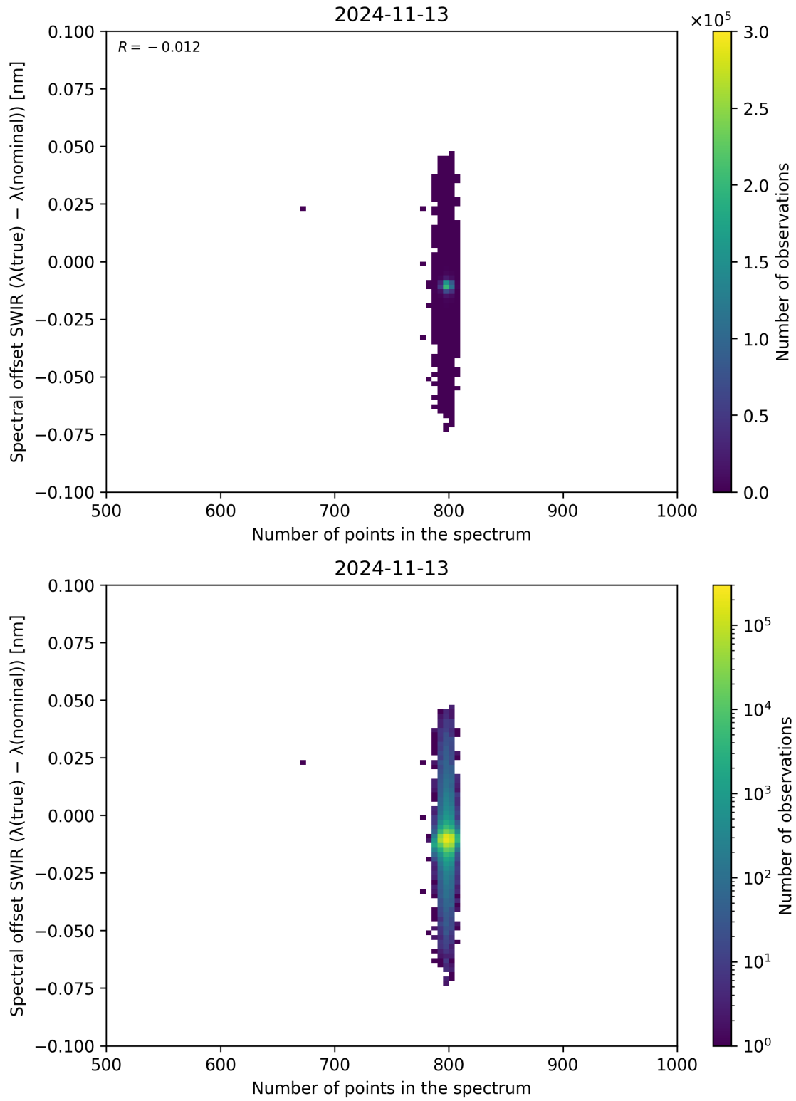
Figure 93: Scatter density plot of “Number of points in the spectrum” against “Spectral offset SWIR ( \lambda_{\text{true}} - \lambda_{\text{nominal}} )” for 2024-11-12 to 2024-11-14.
