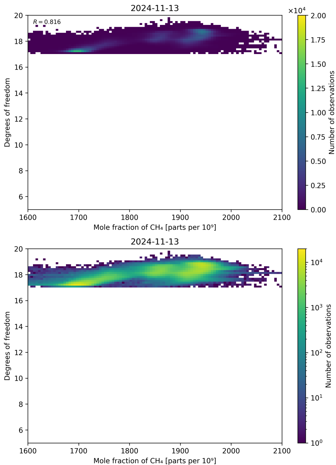
Figure 72: Scatter density plot of “Mole fraction of CH 4 ” against “Degrees of freedom” for 2024-11-12 to 2024-11-14.
