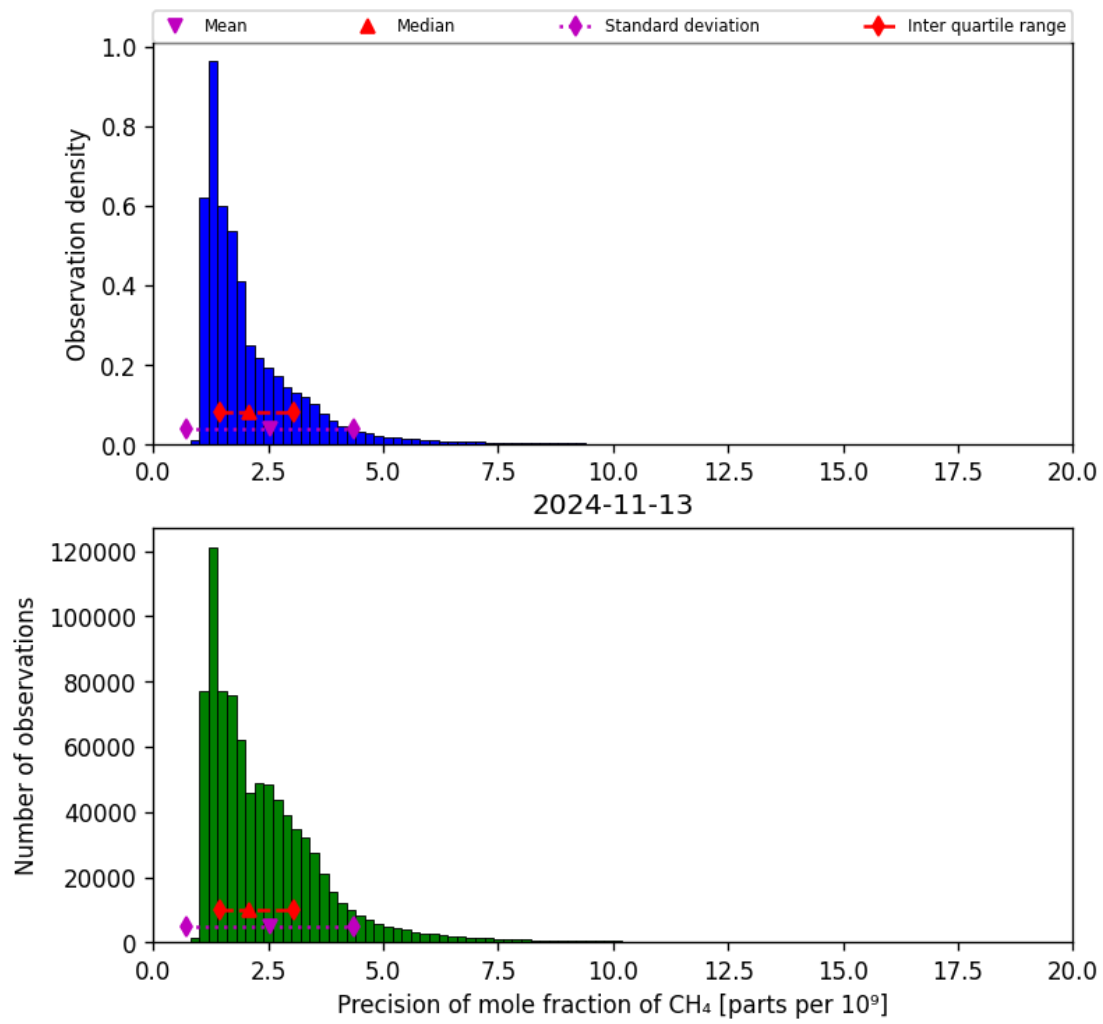
Figure 24: Histogram of “Precision of mole fraction of CH 4 ” for 2024-11-12 to 2024-11-14
