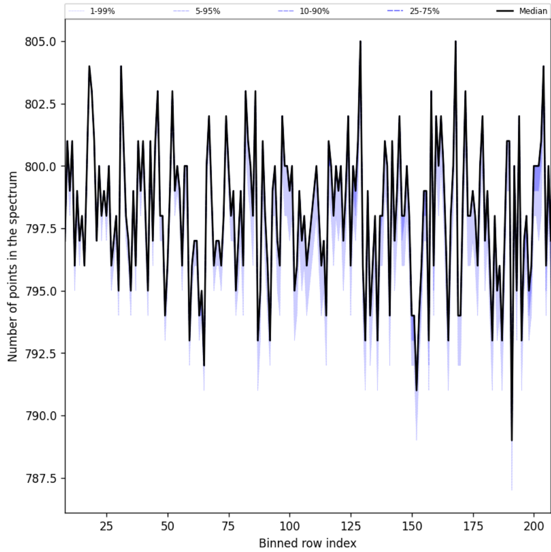
Figure 37: Along track statistics of “Number of points in the spectrum” for 2024-11-12 to 2024-11-14
