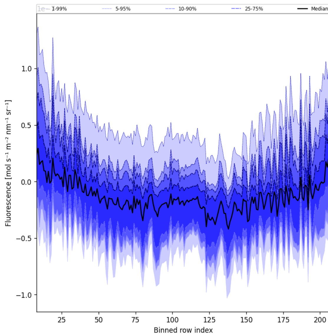
Figure 43: Along track statistics of “Fluorescence” for 2024-11-12 to 2024-11-14
