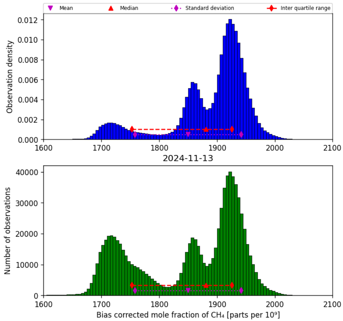
Figure 25: Histogram of “Bias corrected mole fraction of CH 4 ” for 2024-11-12 to 2024-11-14
