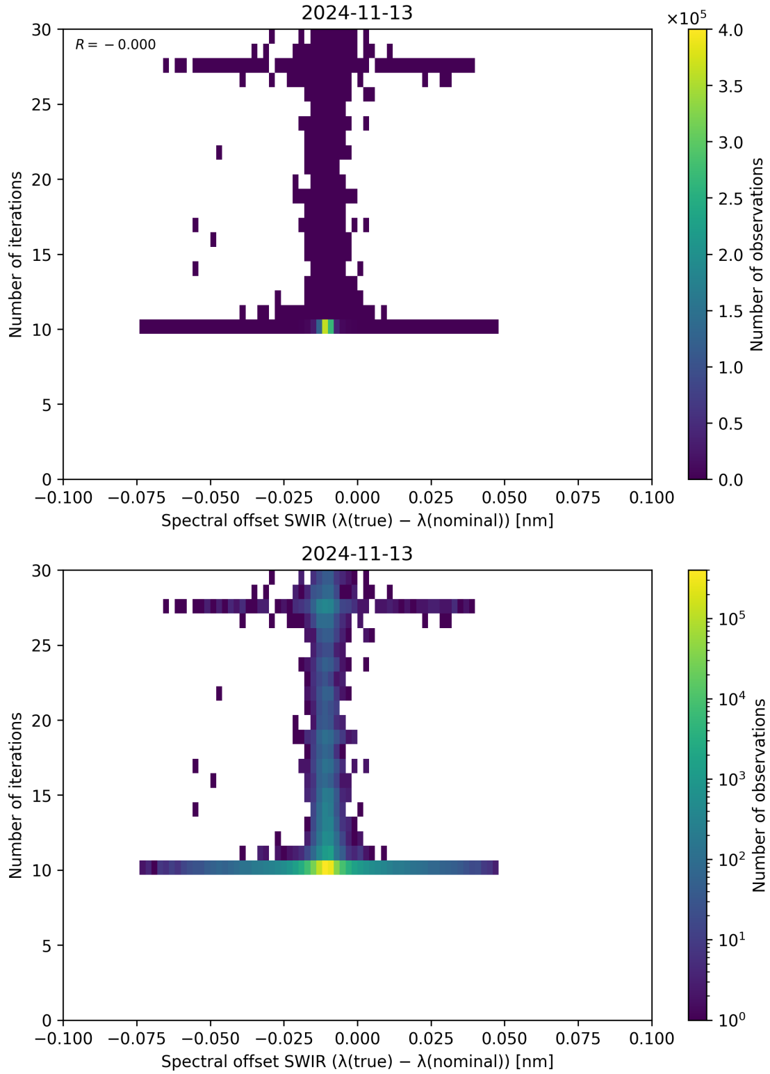
Figure 121: Scatter density plot of “Spectral offset SWIR ( \lambda_{\text{true}} - \lambda_{\text{nominal}} )” against “Number of iterations” for 2024-11-12 to 2024-11-14.
