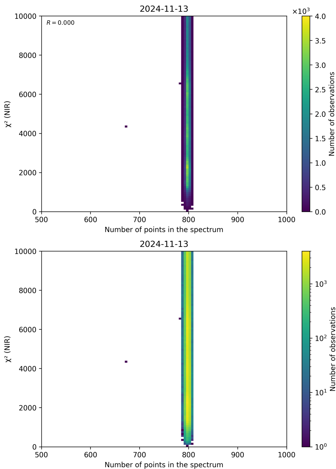
Figure 88: Scatter density plot of “Number of points in the spectrum” against “ \chi^2 (NIR)” for 2024-11-12 to 2024-11-14.
