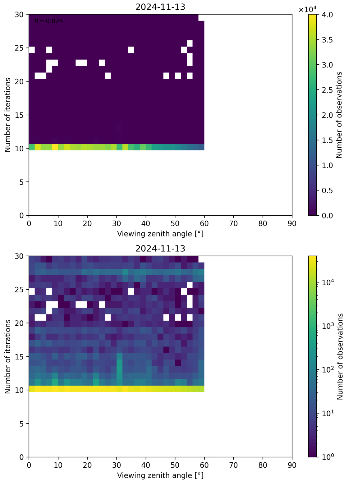
Figure 113: Scatter density plot of “Viewing zenith angle” against “Number of iterations” for 2024-11-12 to 2024-11-14.
