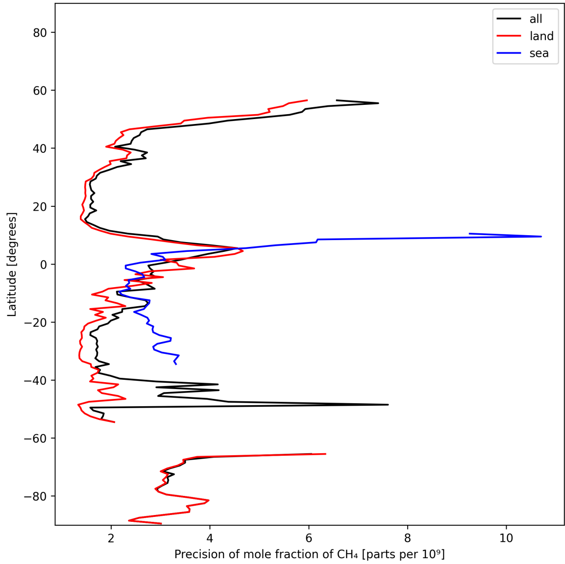
Figure 13: Zonal average of “Precision of mole fraction of CH 4 ” for 2024-11-12 to 2024-11-14.
