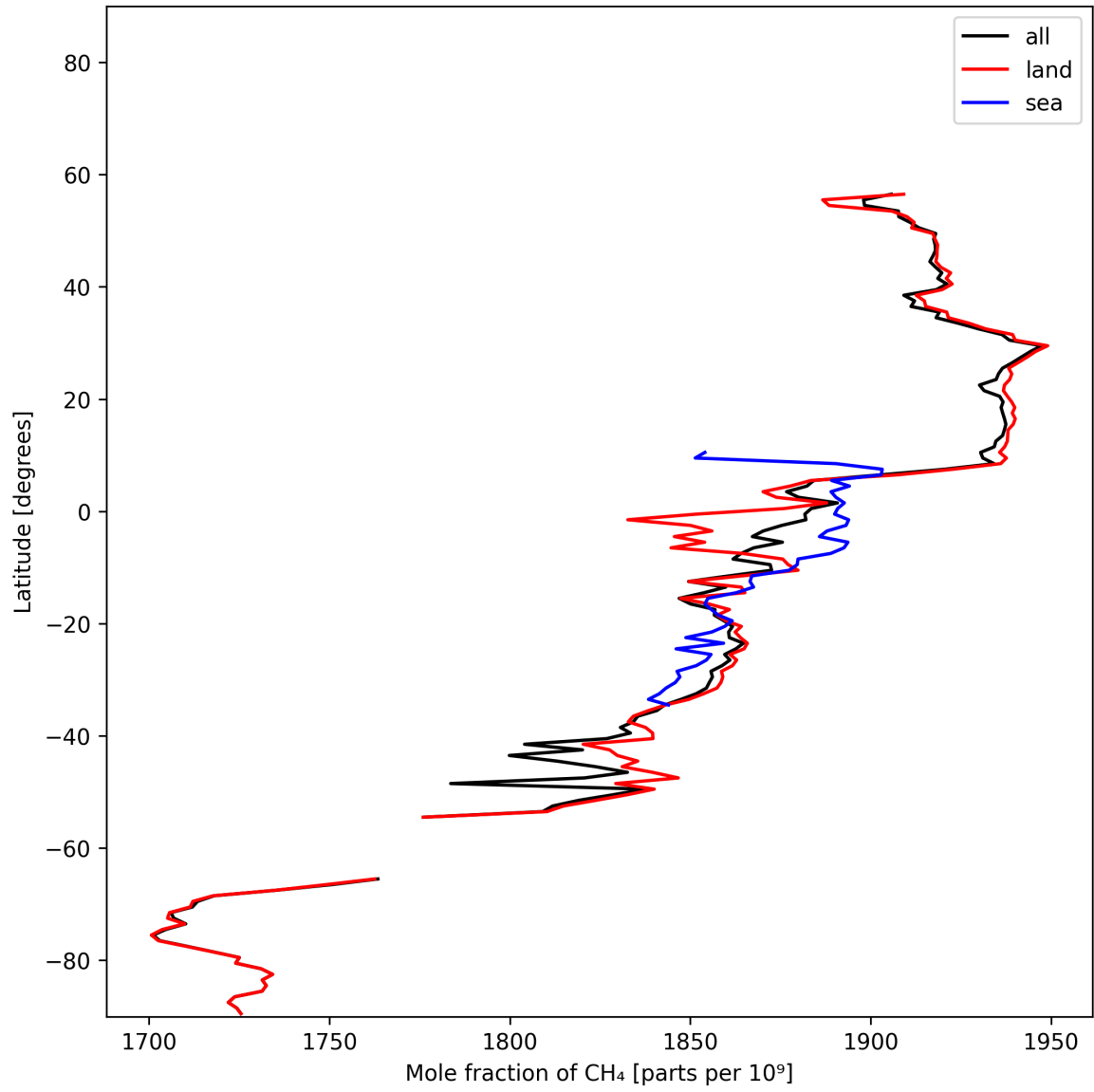
Figure 12: Zonal average of “Mole fraction of \text{CH}_4 ” for 2024-11-12 to 2024-11-14.
