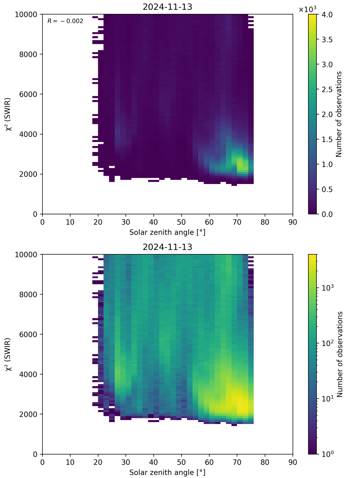
Figure 95: Scatter density plot of “Solar zenith angle” against “ \chi^2 (SWIR)” for 2024-11-12 to 2024-11-14.
