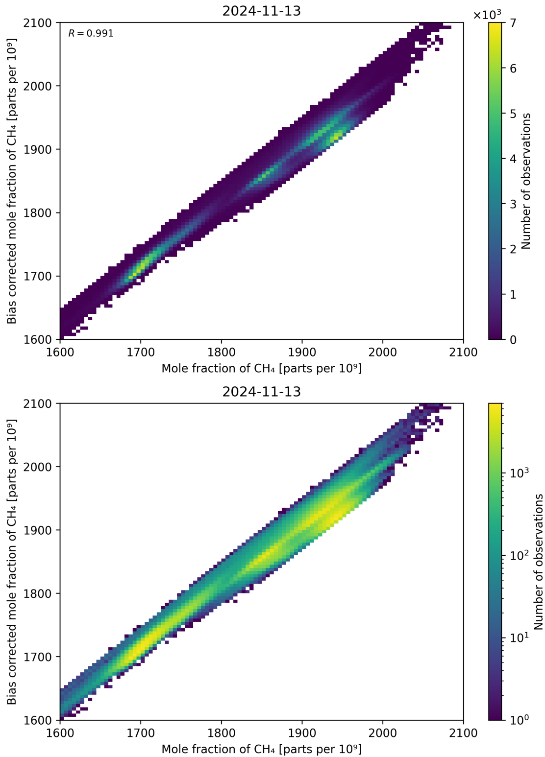
Figure 74: Scatter density plot of “Mole fraction of CH 4 ” against “Bias corrected mole fraction of CH 4 ” for 2024-11-12 to 2024-11-14.
