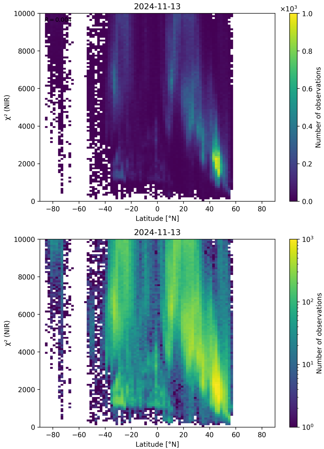
Figure 53: Scatter density plot of “Latitude” against “ \chi^2 (NIR)” for 2024-11-12 to 2024-11-14.
