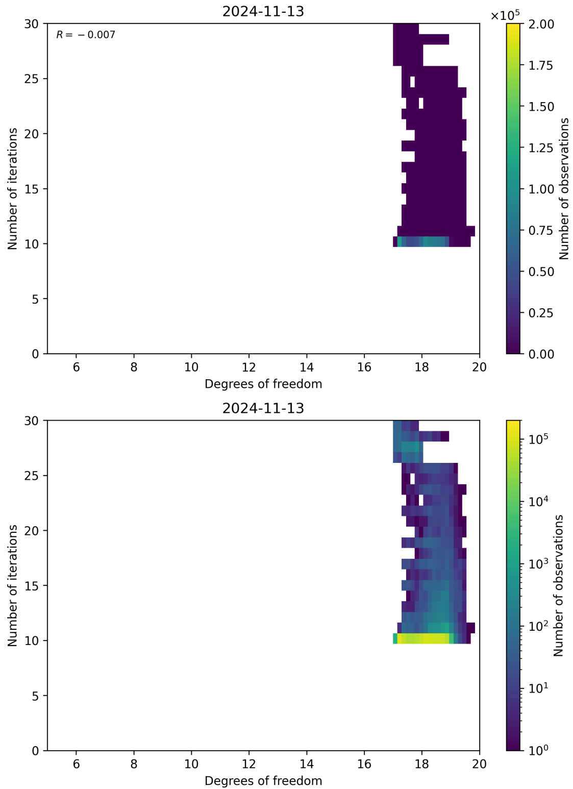
Figure 52: Scatter density plot of “Degrees of freedom” against “Number of iterations” for 2024-11-12 to 2024-11-14.
