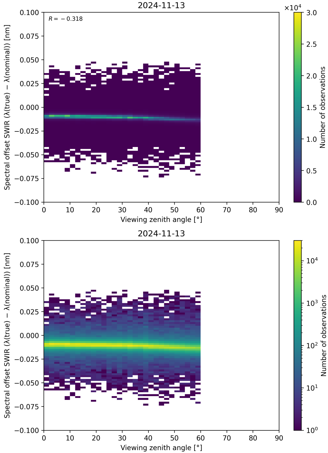
Figure 116: Scatter density plot of “Viewing zenith angle” against “Spectral offset SWIR ( \lambda_{\text{true}} - \lambda_{\text{nominal}} )” for 2024-11-12 to 2024-11-14.
