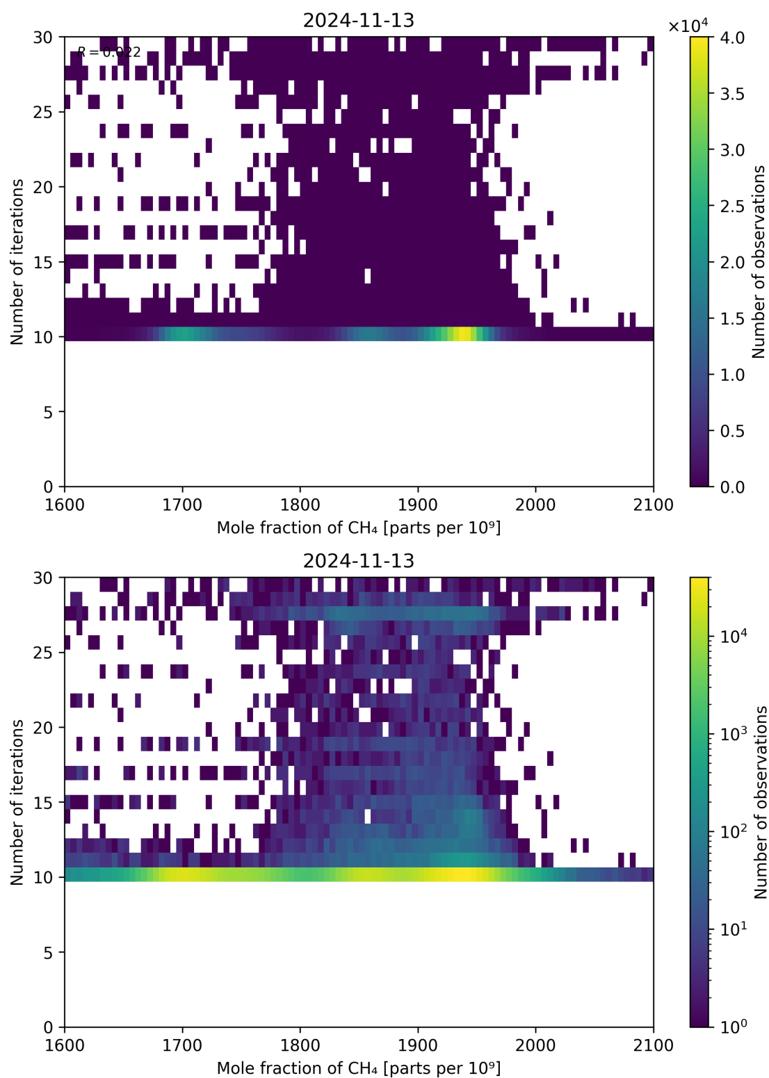
Figure 76: Scatter density plot of “Mole fraction of CH 4 ” against “Number of iterations” for 2024-11-12 to 2024-11-14.
