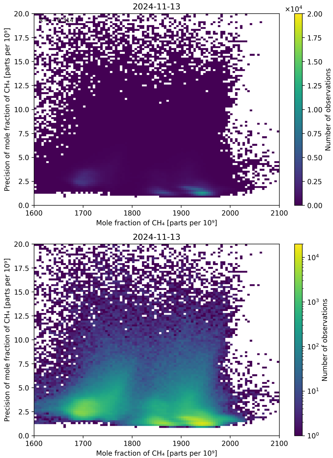
Figure 75: Scatter density plot of “Mole fraction of CH 4 ” against “Precision of mole fraction of CH 4 ” for 2024-11-12 to 2024-11-14.
