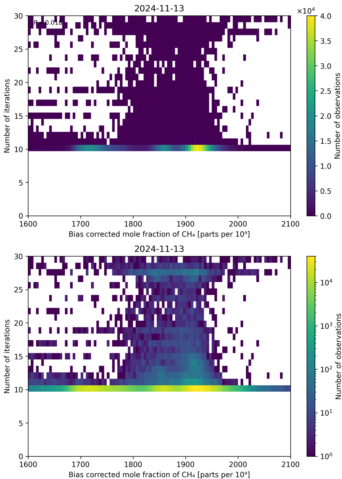
Figure 67: Scatter density plot of “Bias corrected mole fraction of \text{CH}_4 ” against “Number of iterations” for 2024-11-12 to 2024-11-14.
