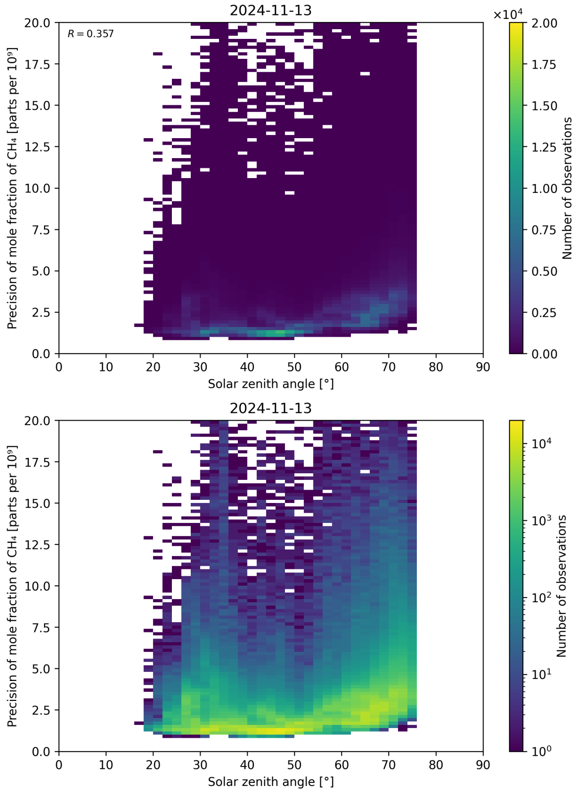
Figure 101: Scatter density plot of “Solar zenith angle” against “Precision of mole fraction of \text{CH}_4 ” for 2024-11-12 to 2024-11-14.
