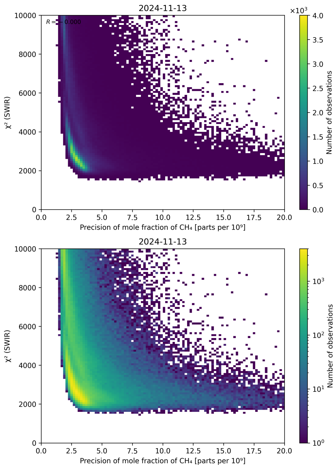
Figure 79: Scatter density plot of “Precision of mole fraction of CH 4 ” against “ \chi^2 (SWIR)” for 2024-11-12 to 2024-11-14.
