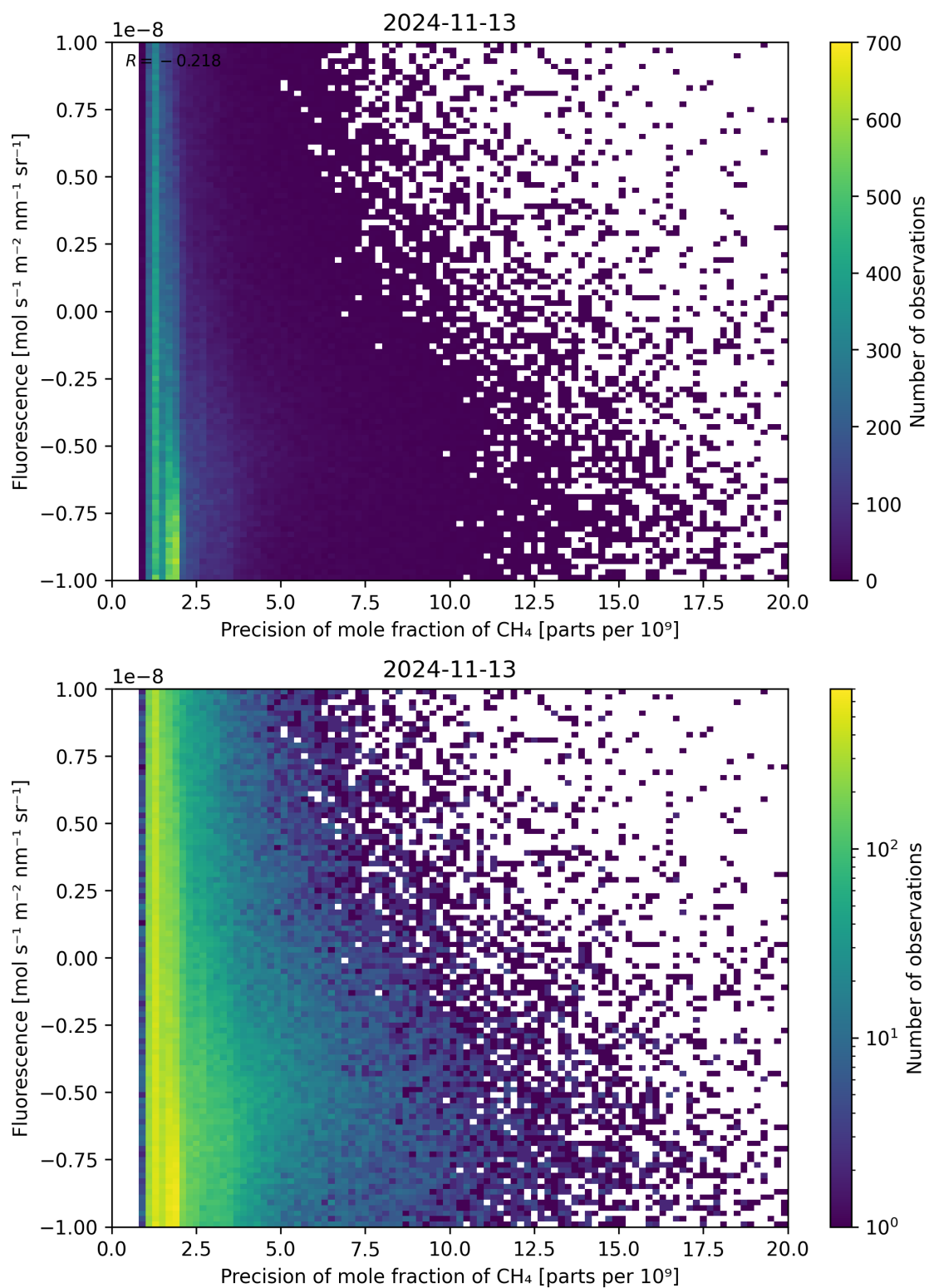
Figure 81: Scatter density plot of “Precision of mole fraction of \text{CH}_4 ” against “Fluorescence” for 2024-11-12 to 2024-11-14.
