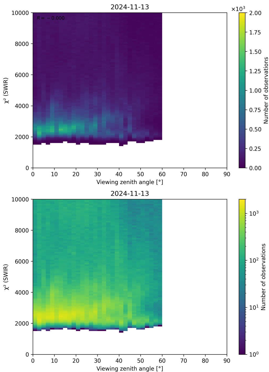
Figure 106: Scatter density plot of “Viewing zenith angle” against “ \chi^2 (SWIR)” for 2024-11-12 to 2024-11-14.
