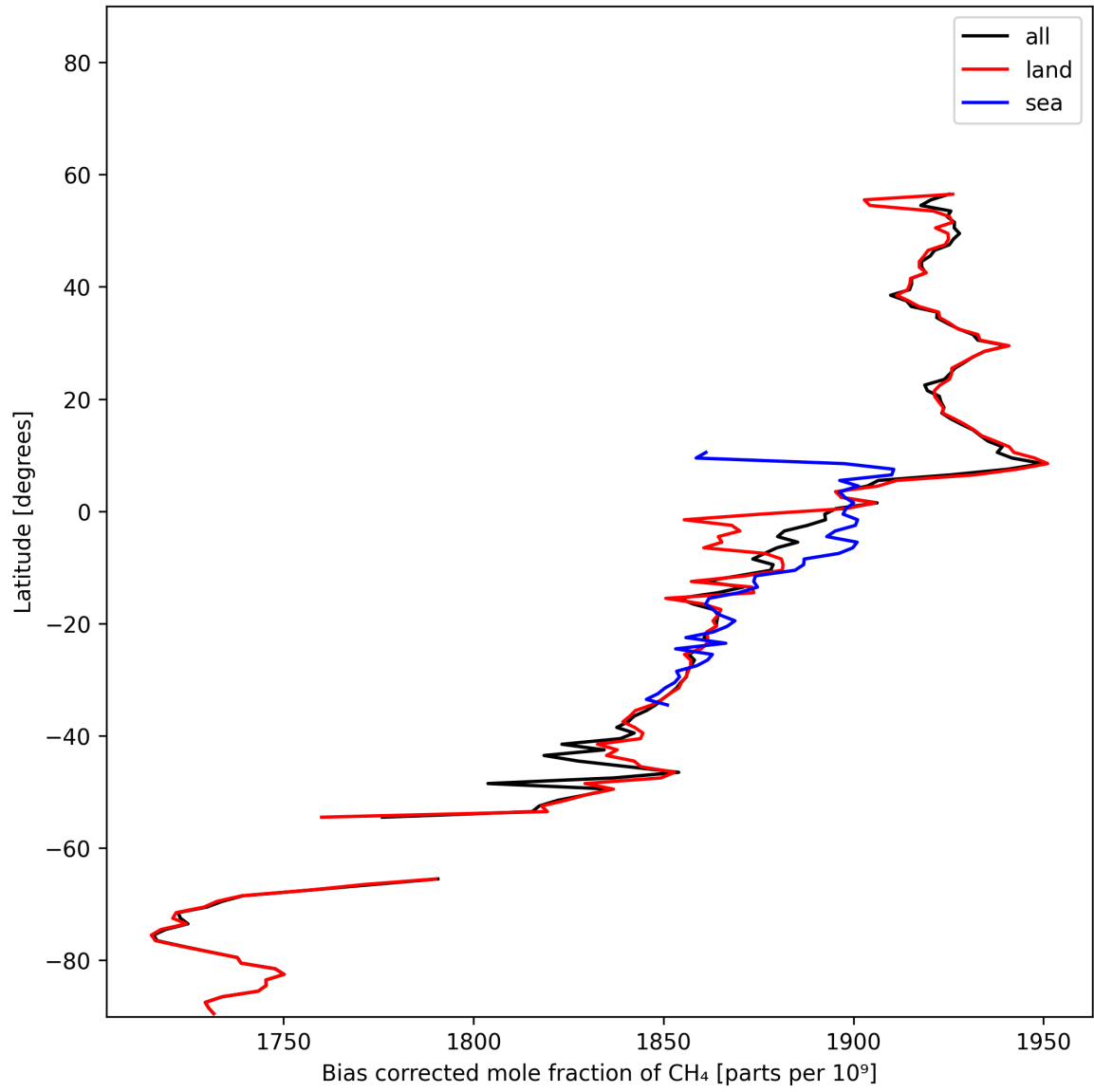
Figure 14: Zonal average of “Bias corrected mole fraction of CH 4 ” for 2024-11-12 to 2024-11-14.
