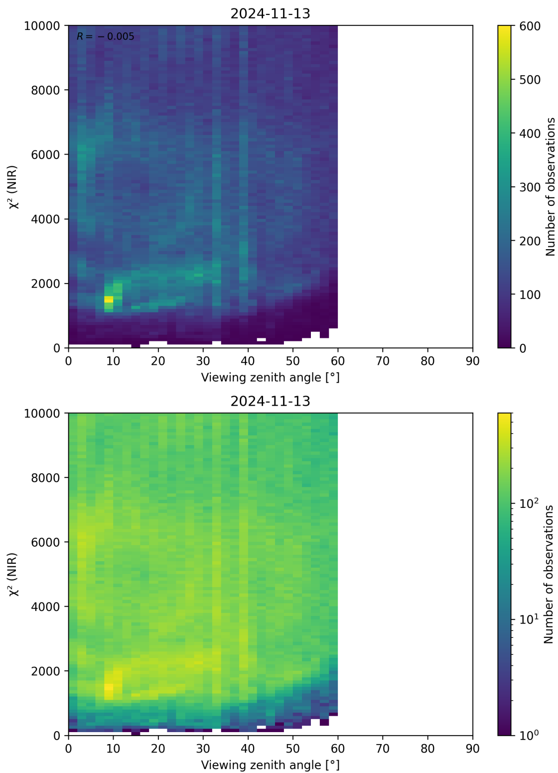
Figure 105: Scatter density plot of “Viewing zenith angle” against “ \chi^2 (NIR)” for 2024-11-12 to 2024-11-14.
