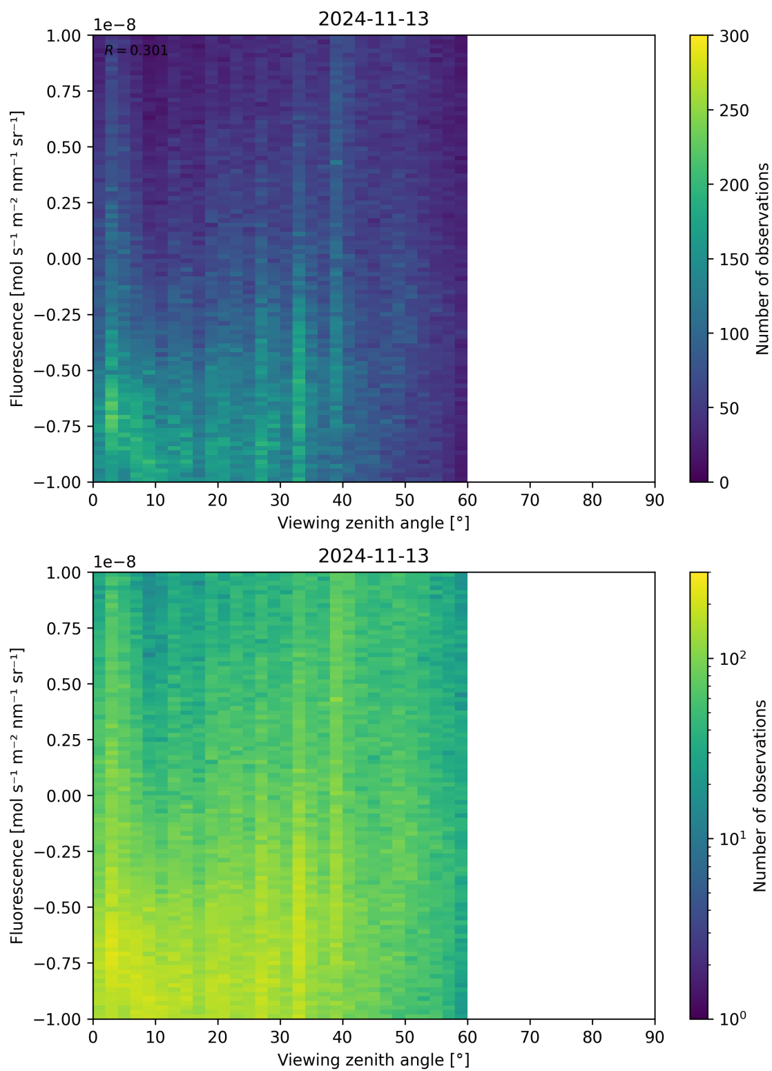
Figure 108: Scatter density plot of “Viewing zenith angle” against “Fluorescence” for 2024-11-12 to 2024-11-14.
