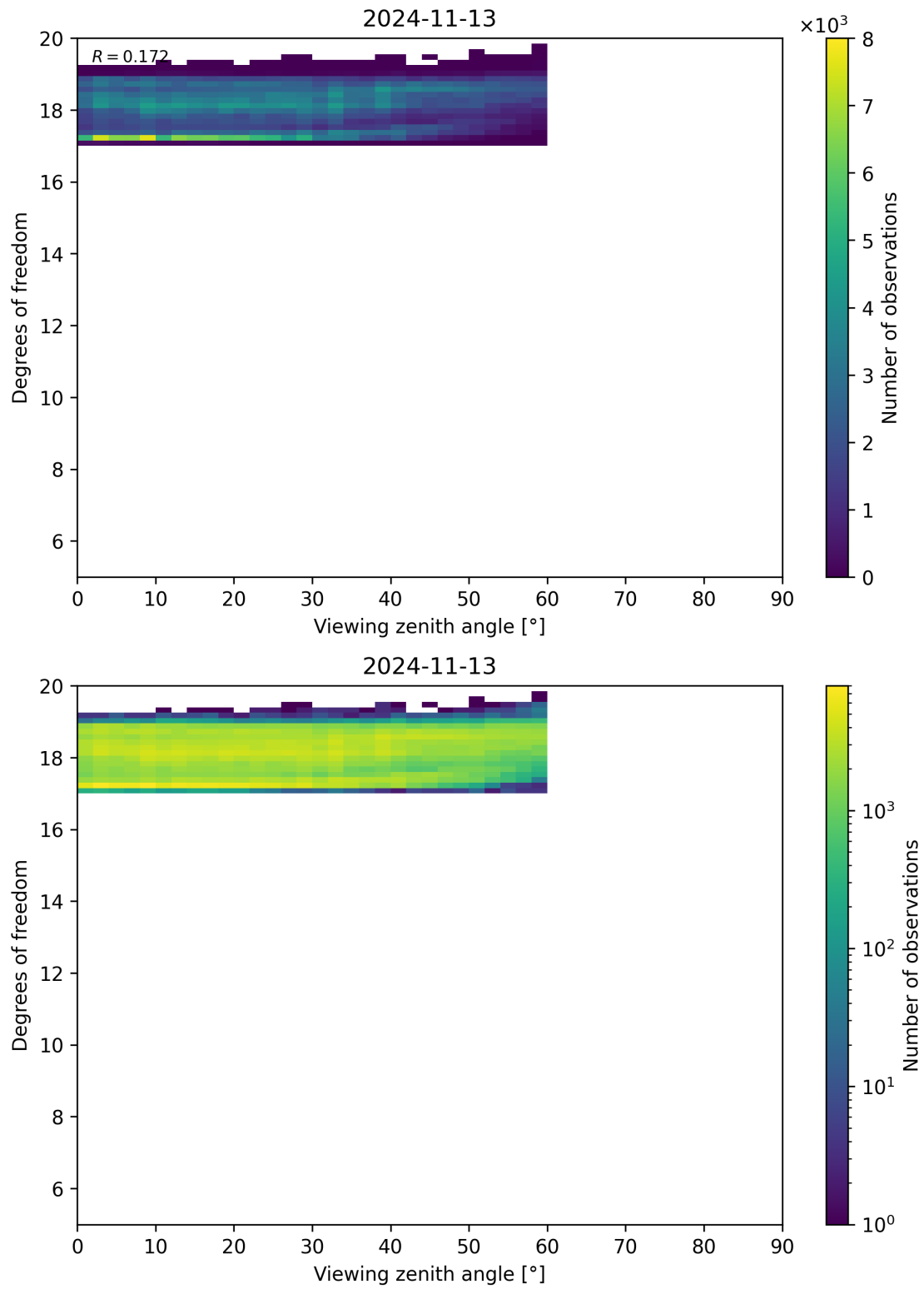
Figure 107: Scatter density plot of “Viewing zenith angle” against “Degrees of freedom” for 2024-11-12 to 2024-11-14.
