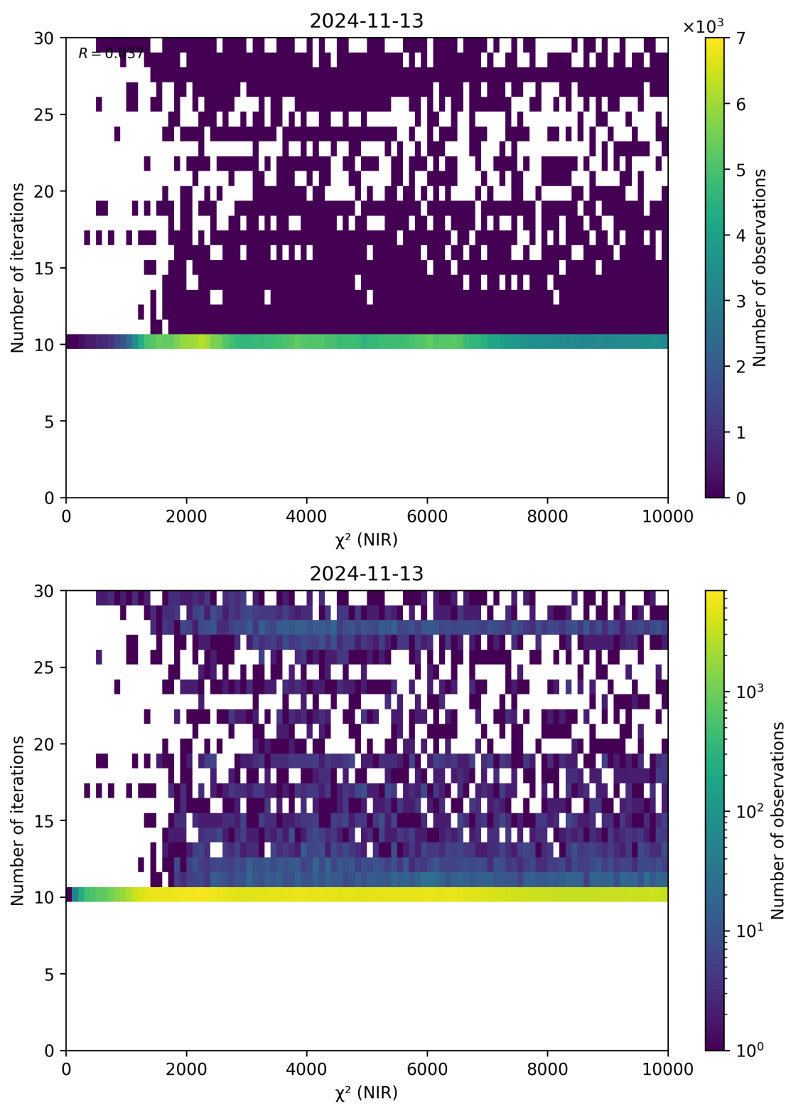
Figure 46: Scatter density plot of “ \chi^2 (NIR)” against “Number of iterations” for 2024-11-12 to 2024-11-14.
