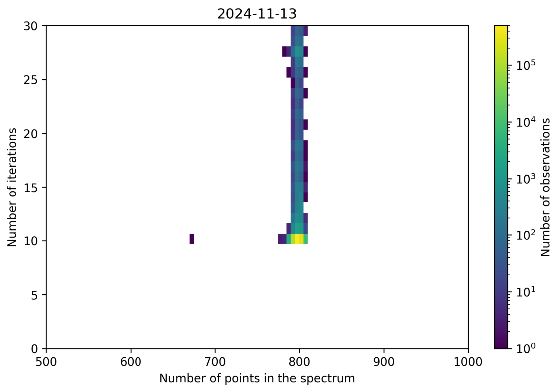
Figure 92: Scatter density plot of “Number of points in the spectrum” against “Number of iterations” for 2024-11-12 to 2024-11-14.
