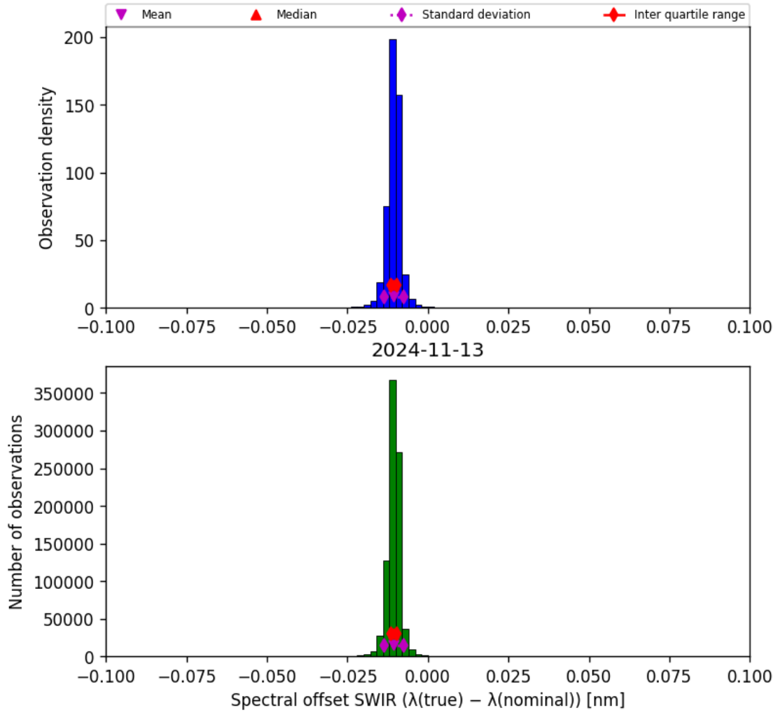
Figure 27: Histogram of “Spectral offset SWIR ( \lambda_{\text{true}} - \lambda_{\text{nominal}} )” for 2024-11-12 to 2024-11-14
