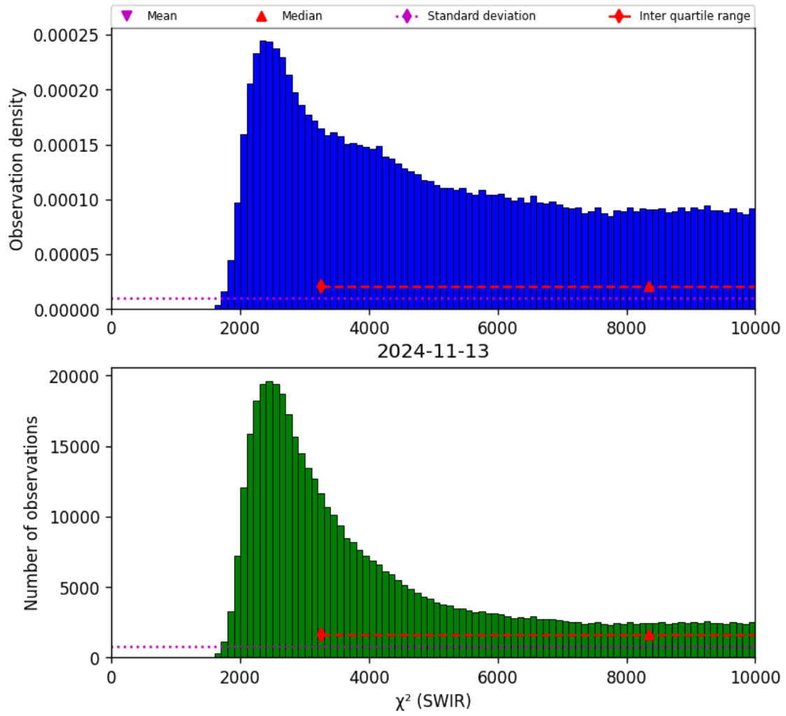
Figure 28: Histogram of " \chi^2 (SWIR)" for 2024-11-12 to 2024-11-14
