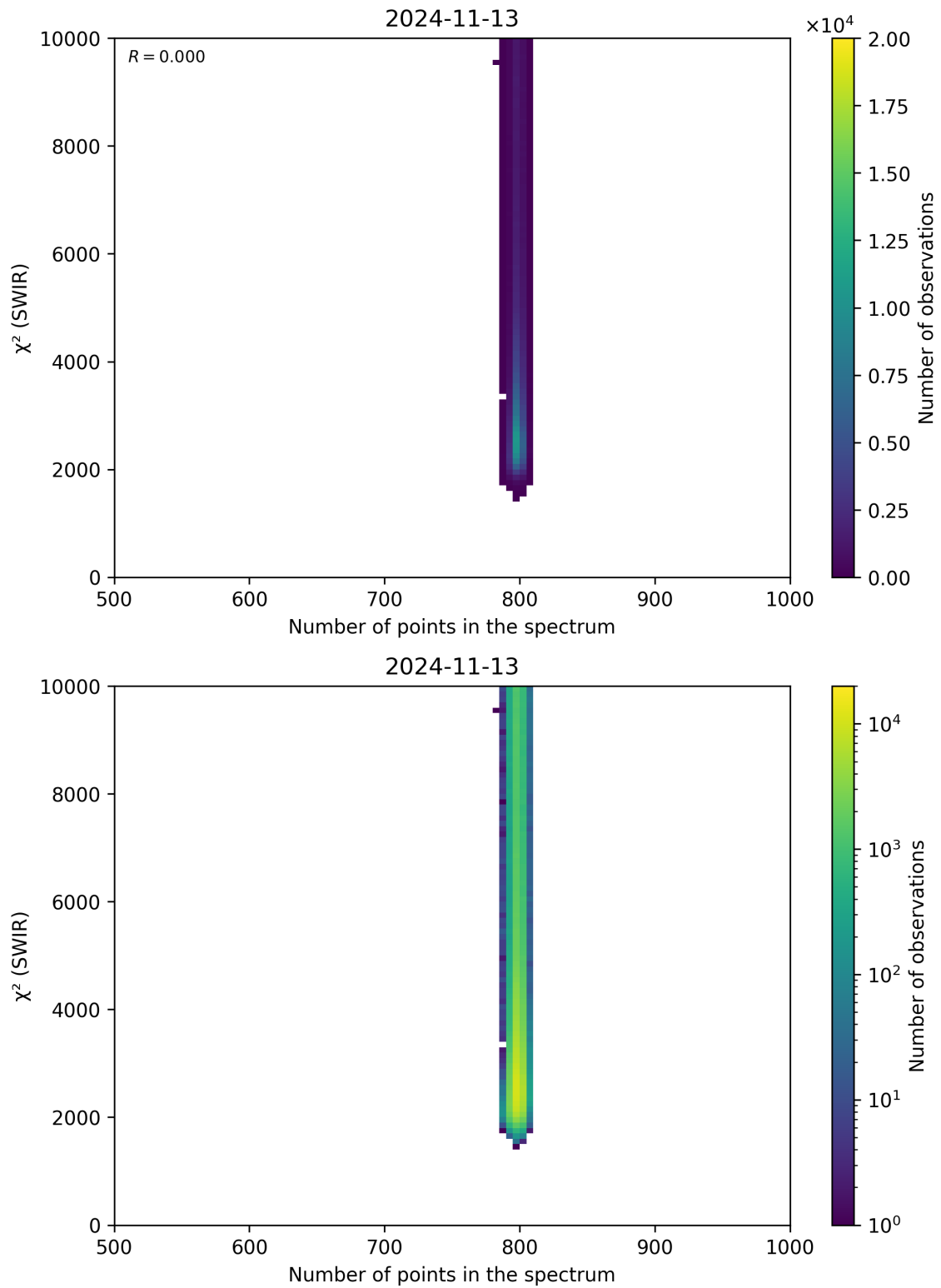
Figure 89: Scatter density plot of “Number of points in the spectrum” against “ \chi^2 (SWIR)” for 2024-11-12 to 2024-11-14.
