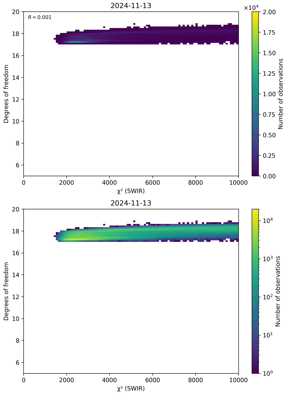
Figure 48: Scatter density plot of “ \chi^2 (SWIR)” against “Degrees of freedom” for 2024-11-12 to 2024-11-14.
