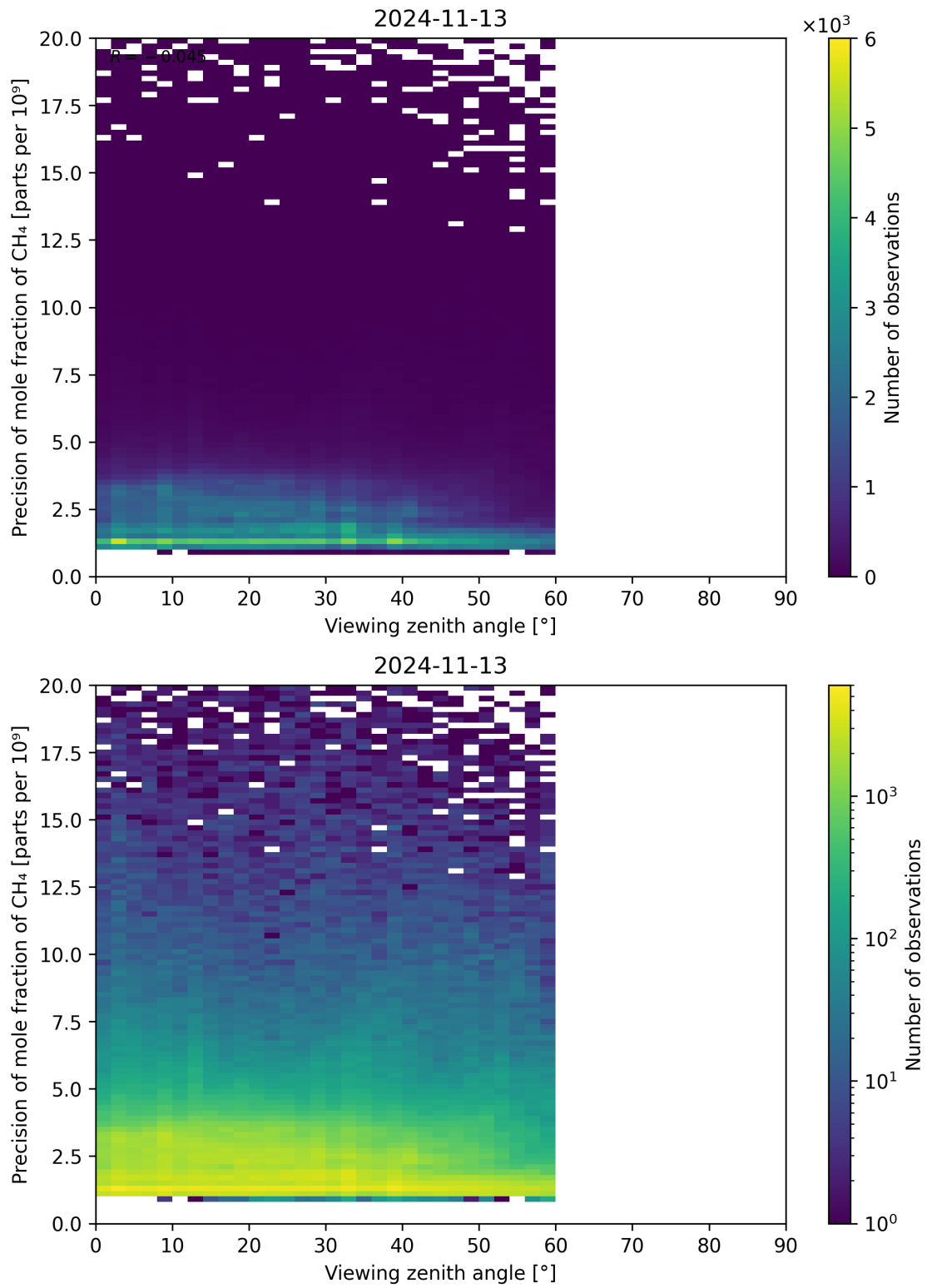
Figure 112: Scatter density plot of “Viewing zenith angle” against “Precision of mole fraction of CH 4 ” for 2024-11-12 to 2024-11-14.
