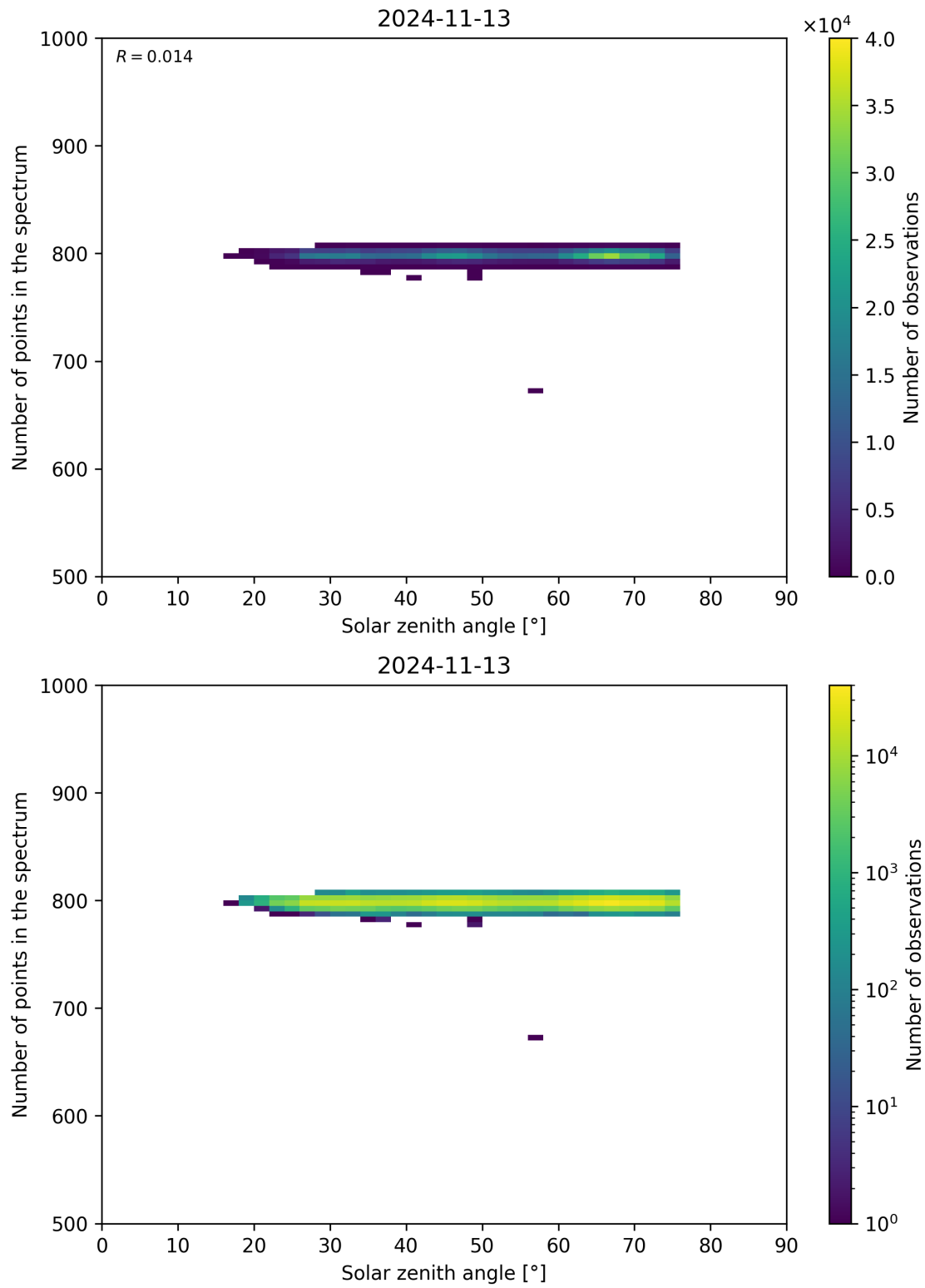
Figure 103: Scatter density plot of “Solar zenith angle” against “Number of points in the spectrum” for 2024-11-12 to 2024-11-14.
