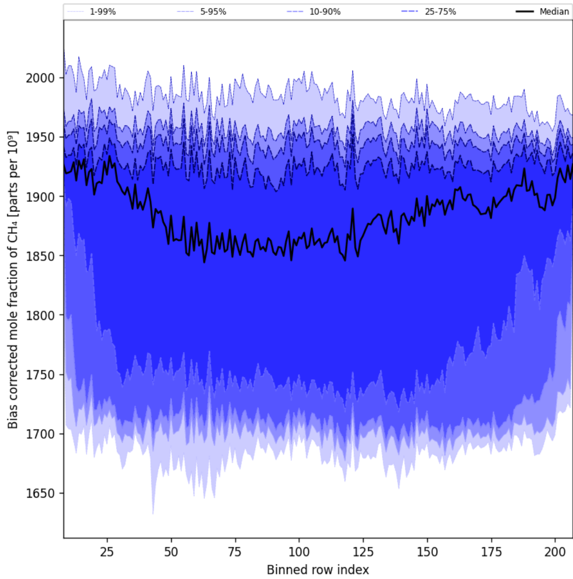
Figure 36: Along track statistics of “Bias corrected mole fraction of CH 4 ” for 2024-11-12 to 2024-11-14
