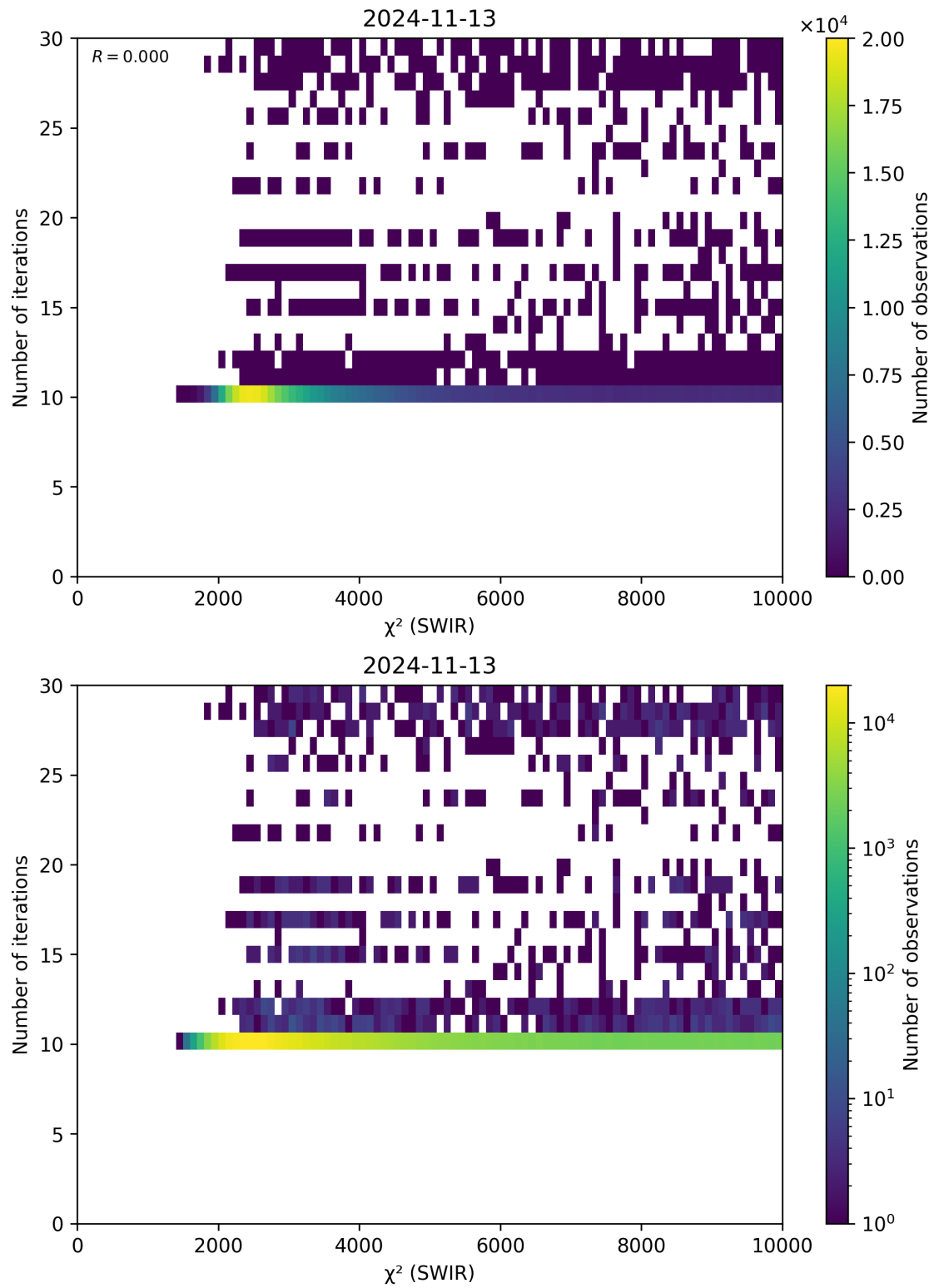
Figure 50: Scatter density plot of “ \chi^2 (SWIR)” against “Number of iterations” for 2024-11-12 to 2024-11-14.
