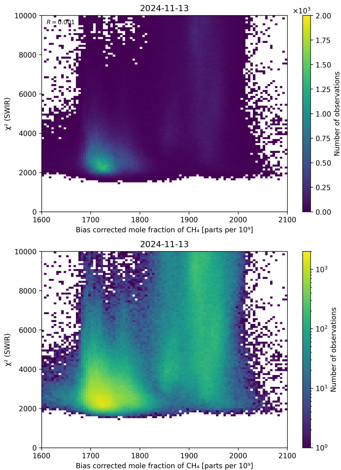
Figure 64: Scatter density plot of “Bias corrected mole fraction of CH 4 ” against “ \chi^2 (SWIR)” for 2024-11-12 to 2024-11-14.
