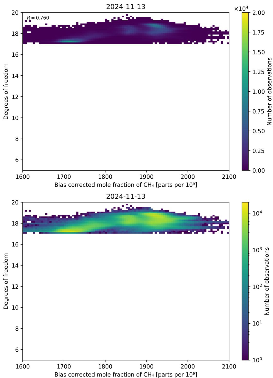
Figure 65: Scatter density plot of “Bias corrected mole fraction of CH 4 ” against “Degrees of freedom” for 2024-11-12 to 2024-11-14.
