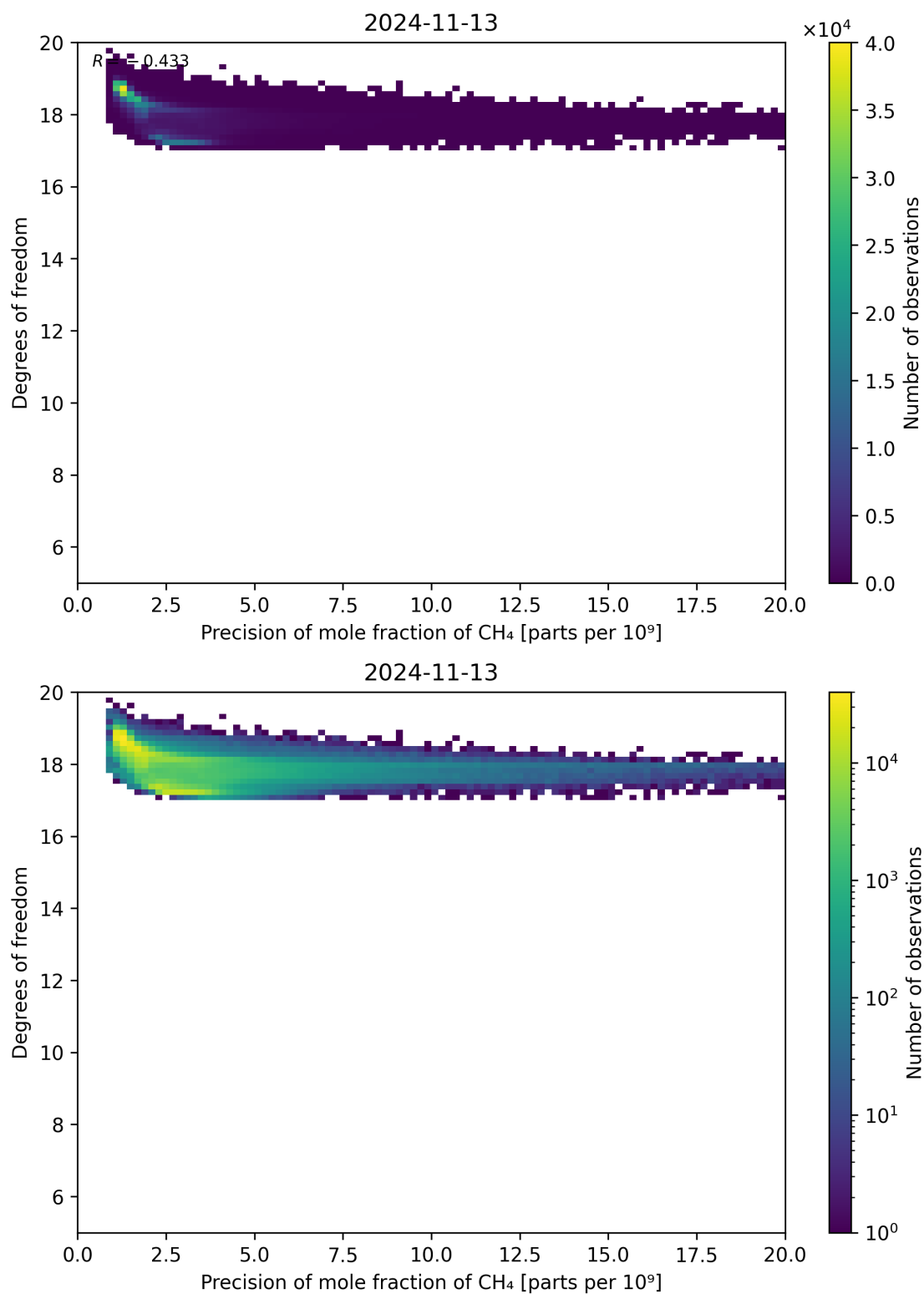
Figure 80: Scatter density plot of “Precision of mole fraction of CH 4 ” against “Degrees of freedom” for 2024-11-12 to 2024-11-14.
