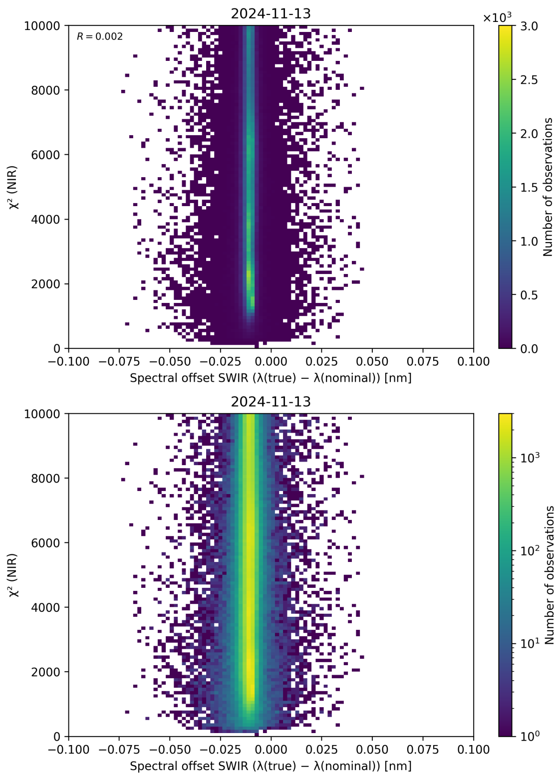
Figure 117: Scatter density plot of “Spectral offset SWIR ( \lambda_{\text{true}} - \lambda_{\text{nominal}} )” against “ \chi^2 (NIR)” for 2024-11-12 to 2024-11-14.
