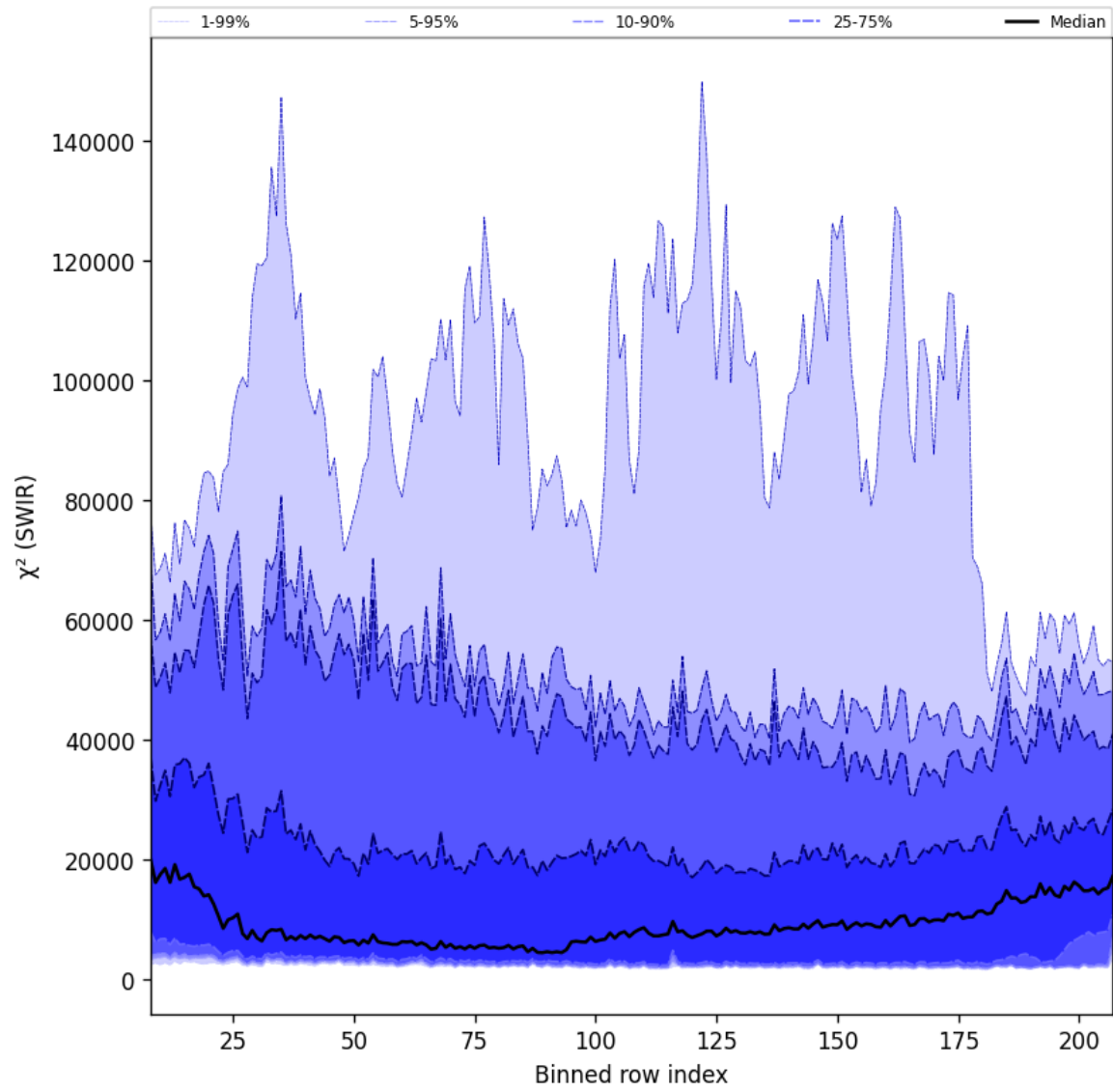
Figure 39: Along track statistics of “ \chi^2 (SWIR)” for 2024-11-12 to 2024-11-14
