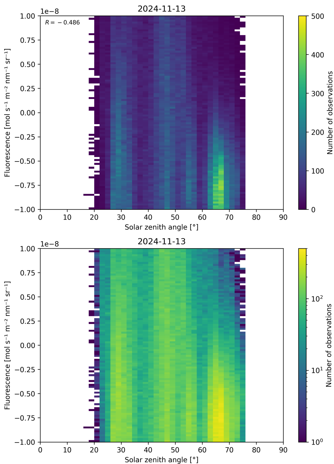
Figure 97: Scatter density plot of “Solar zenith angle” against “Fluorescence” for 2024-11-12 to 2024-11-14.
