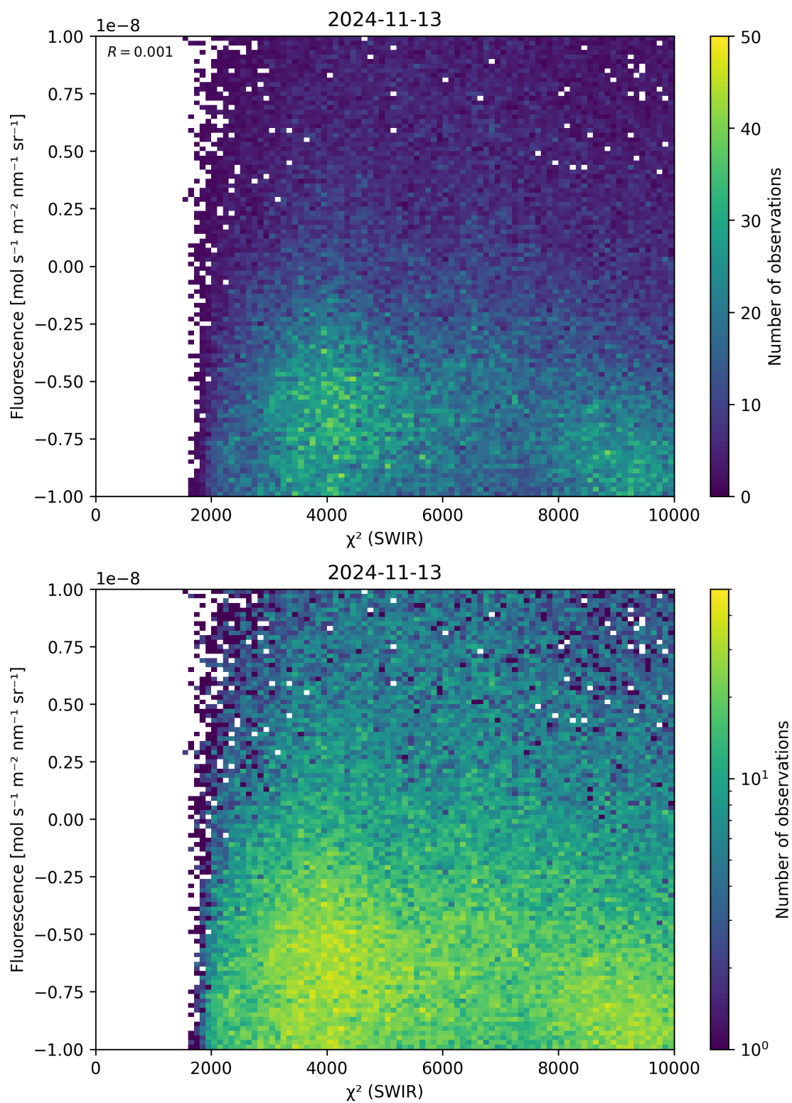
Figure 49: Scatter density plot of “ \chi^2 (SWIR)” against “Fluorescence” for 2024-11-12 to 2024-11-14.
