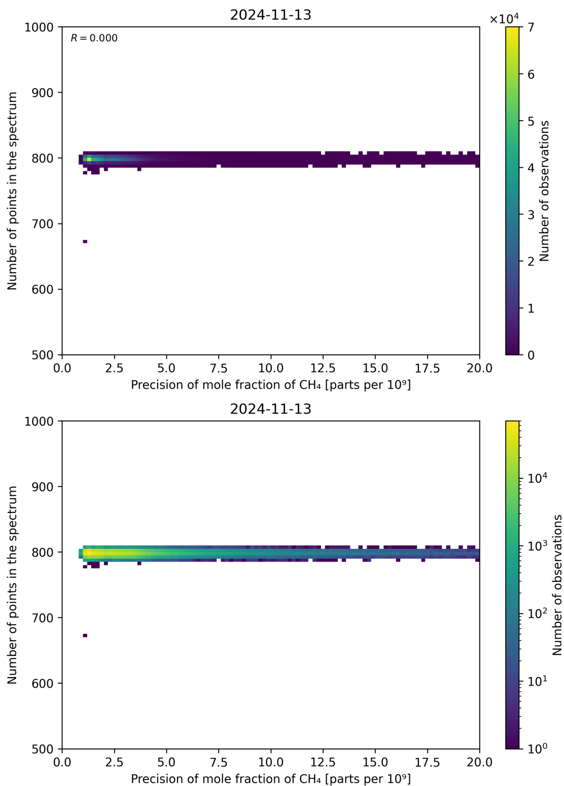
Figure 84: Scatter density plot of “Precision of mole fraction of CH 4 ” against “Number of points in the spectrum” for 2024-11-12 to 2024-11-14.
