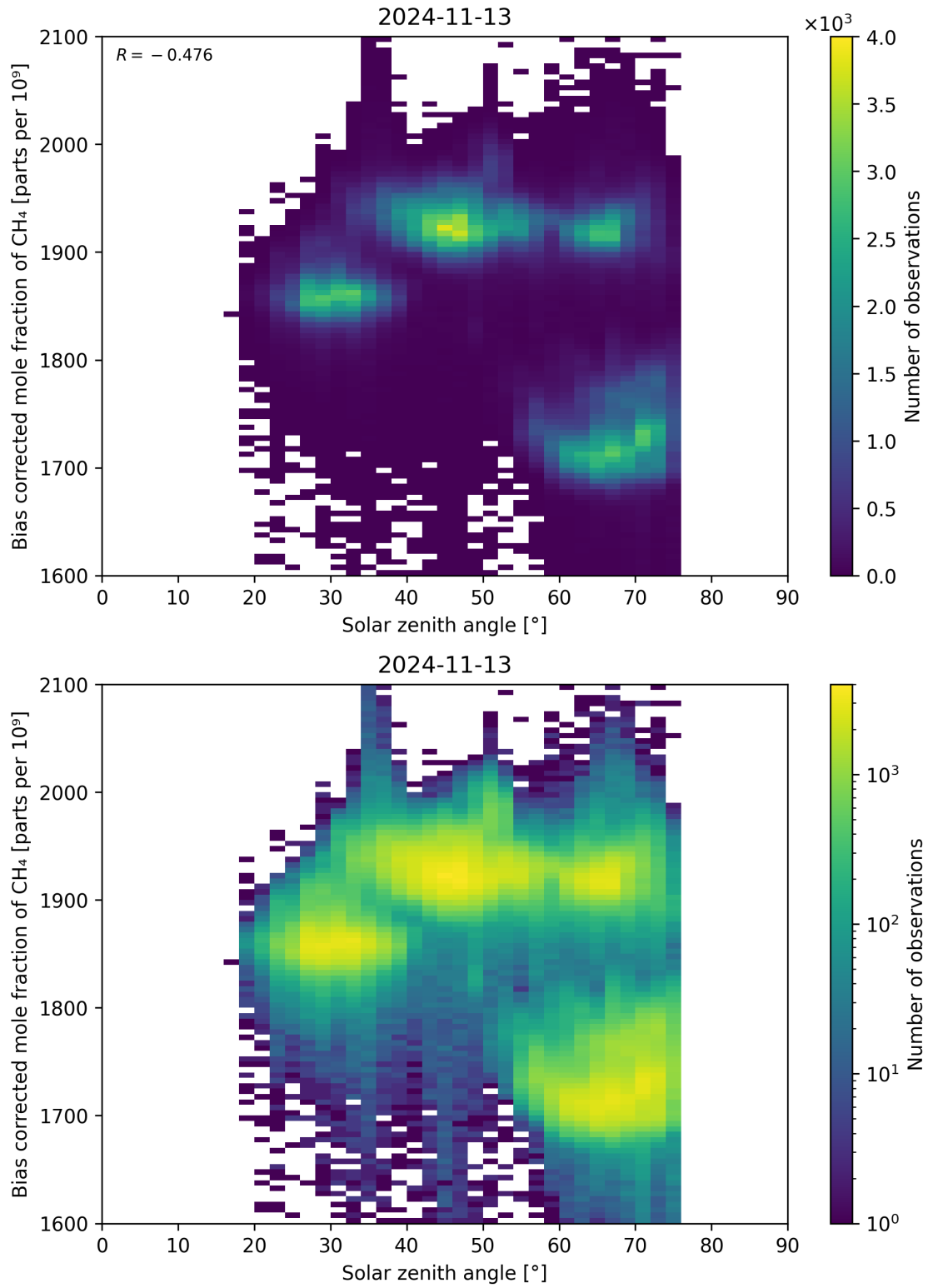
Figure 100: Scatter density plot of “Solar zenith angle” against “Bias corrected mole fraction of CH 4 ” for 2024-11-12 to 2024-11-14.
