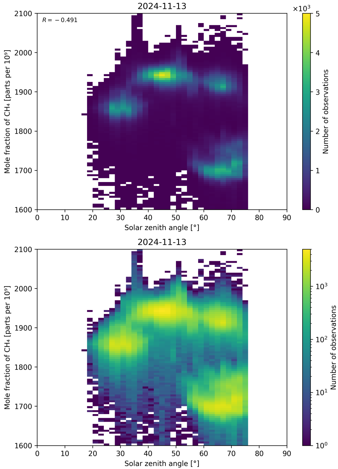
Figure 99: Scatter density plot of “Solar zenith angle” against “Mole fraction of CH 4 ” for 2024-11-12 to 2024-11-14.
