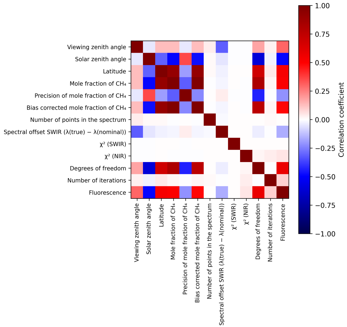
Figure 2: Map of correlation matrix for 2024-11-12 to 2024-11-14.
