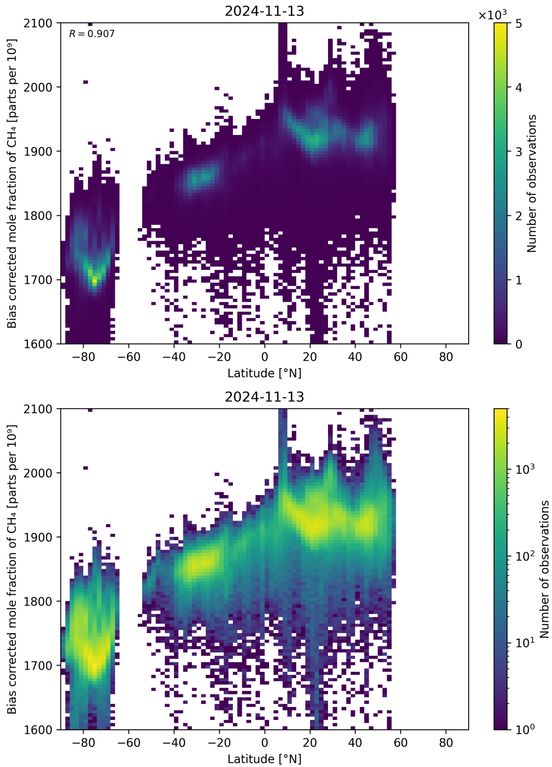
Figure 58: Scatter density plot of “Latitude” against “Bias corrected mole fraction of CH 4 ” for 2024-11-12 to 2024-11-14.
