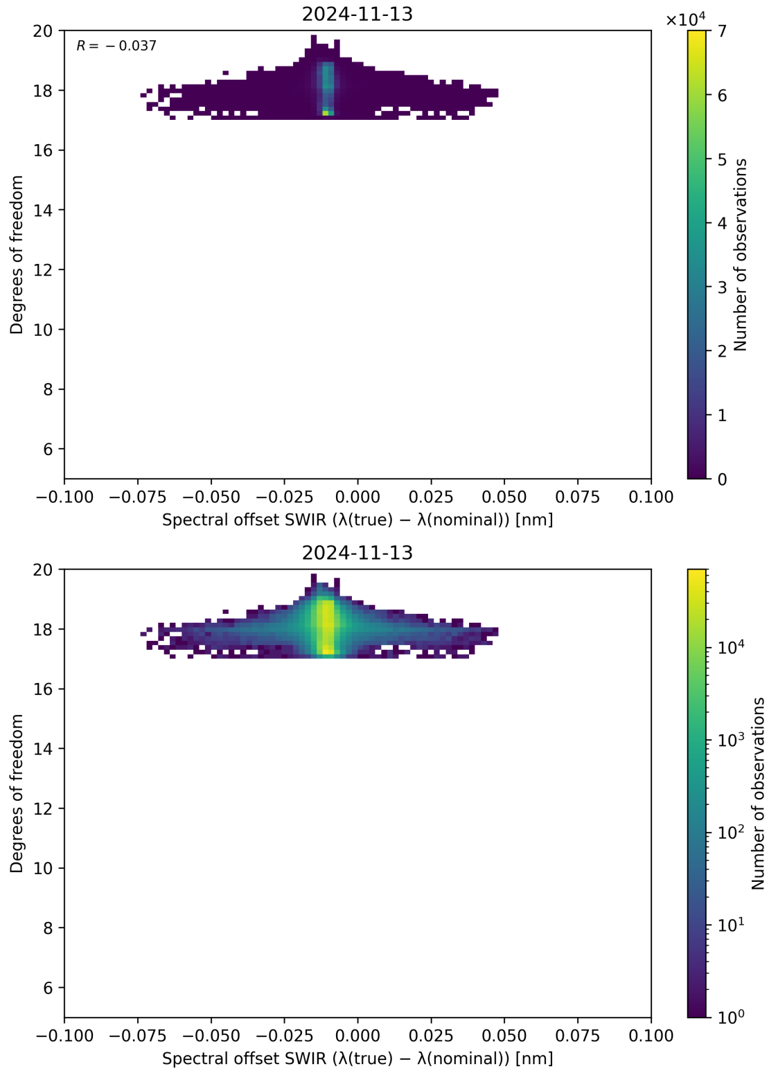
Figure 119: Scatter density plot of “Spectral offset SWIR ( \lambda_{\text{true}} - \lambda_{\text{nominal}} )” against “Degrees of freedom” for 2024-11-12 to 2024-11-14.
