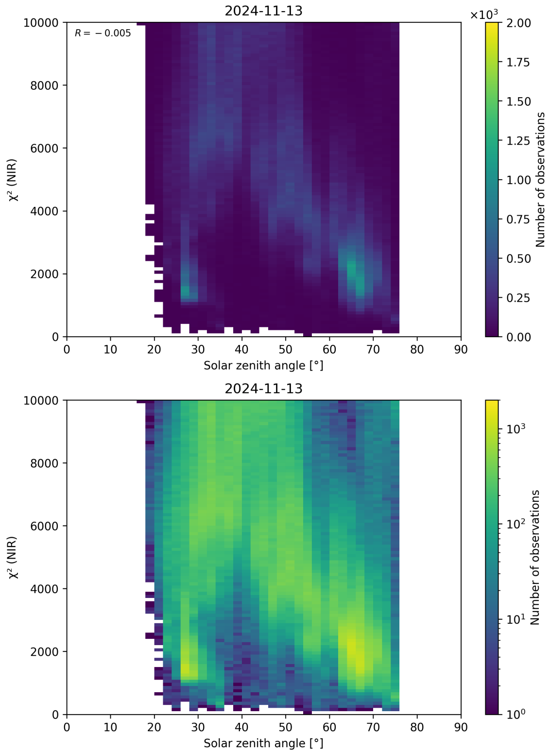
Figure 94: Scatter density plot of “Solar zenith angle” against “ \chi^2 (NIR)” for 2024-11-12 to 2024-11-14.
