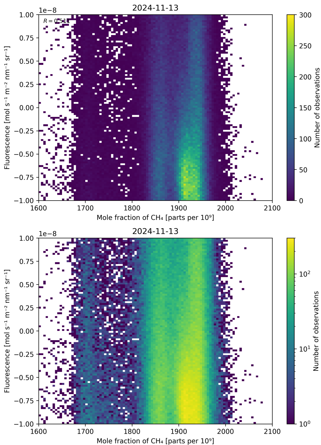
Figure 73: Scatter density plot of “Mole fraction of \text{CH}_4 ” against “Fluorescence” for 2024-11-12 to 2024-11-14.
