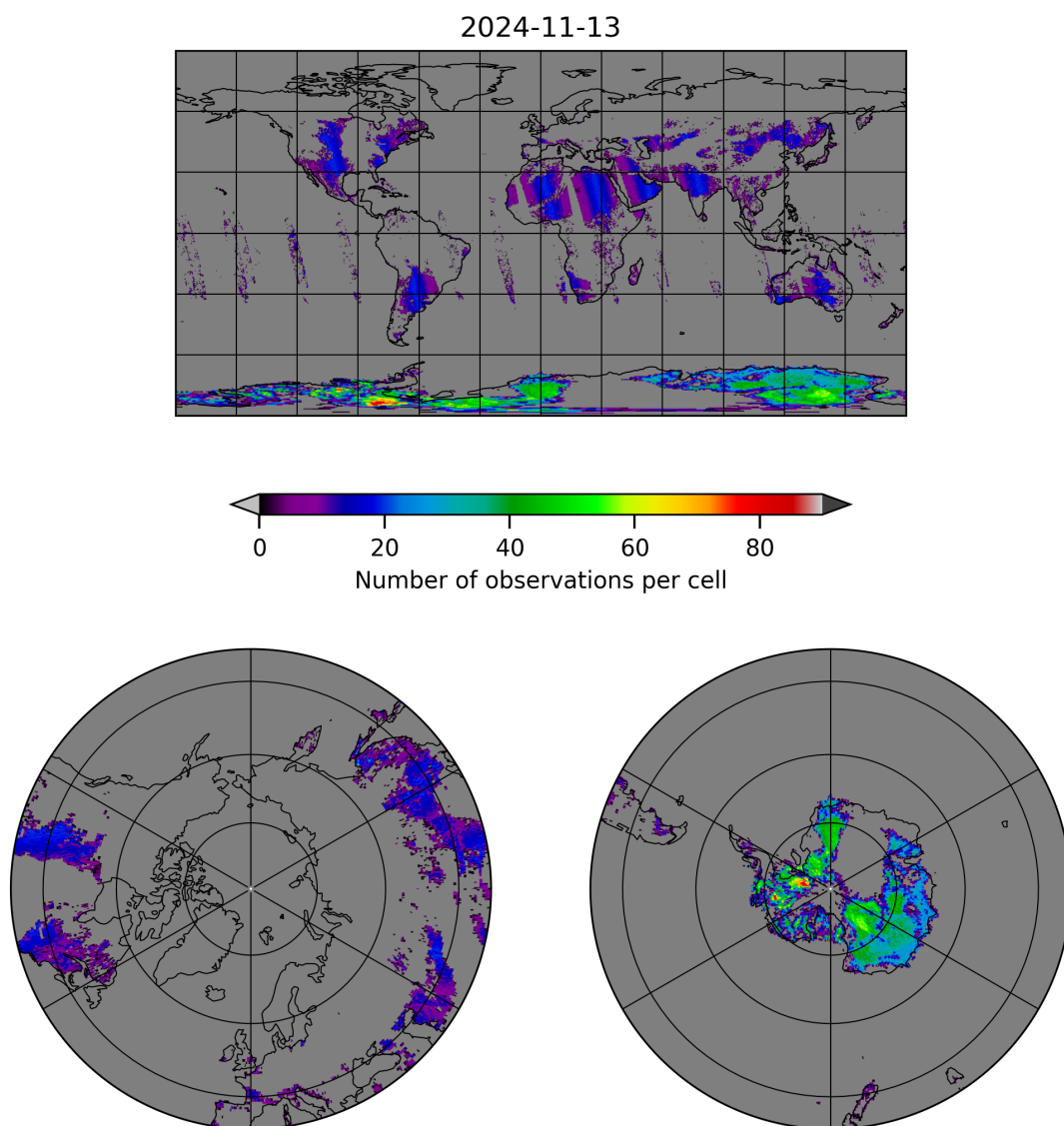
Figure 10: Map of the number of observations for 2024-11-12 to 2024-11-14
