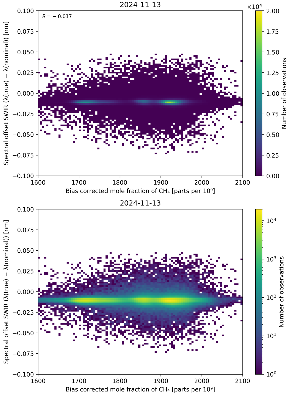
Figure 69: Scatter density plot of “Bias corrected mole fraction of CH 4 ” against “Spectral offset SWIR ( \lambda_{\text{true}} - \lambda_{\text{nominal}} )” for 2024-11-12 to 2024-11-14.
