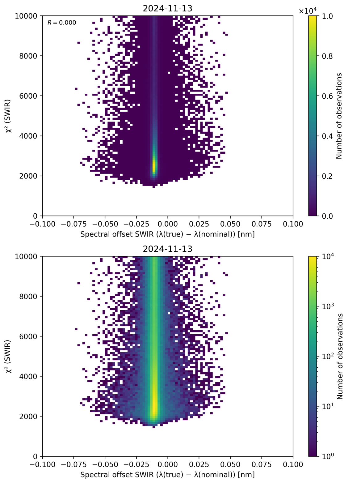
Figure 118: Scatter density plot of “Spectral offset SWIR ( \lambda_{\text{true}} - \lambda_{\text{nominal}} )” against “ \chi^2 (SWIR)” for 2024-11-12 to 2024-11-14.
