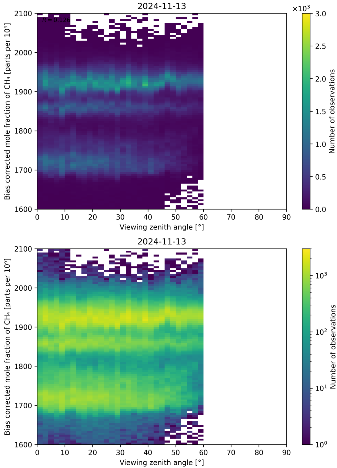
Figure 111: Scatter density plot of “Viewing zenith angle” against “Bias corrected mole fraction of CH 4 ” for 2024-11-12 to 2024-11-14.
