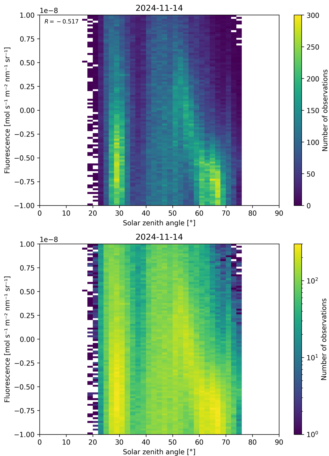
Figure 97: Scatter density plot of “Solar zenith angle” against “Fluorescence” for 2024-11-14 to 2024-11-15.
