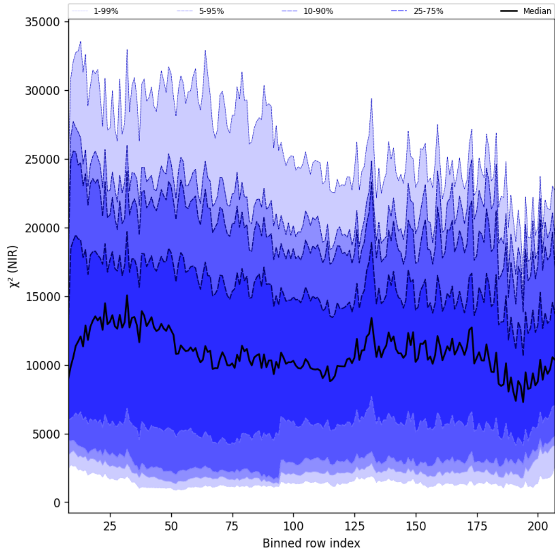
Figure 40: Along track statistics of “ \chi^2 (NIR)” for 2024-11-14 to 2024-11-15
