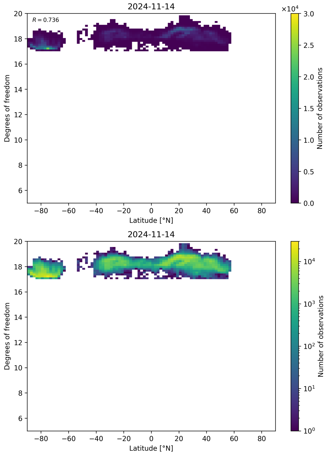
Figure 55: Scatter density plot of “Latitude” against “Degrees of freedom” for 2024-11-14 to 2024-11-15.
