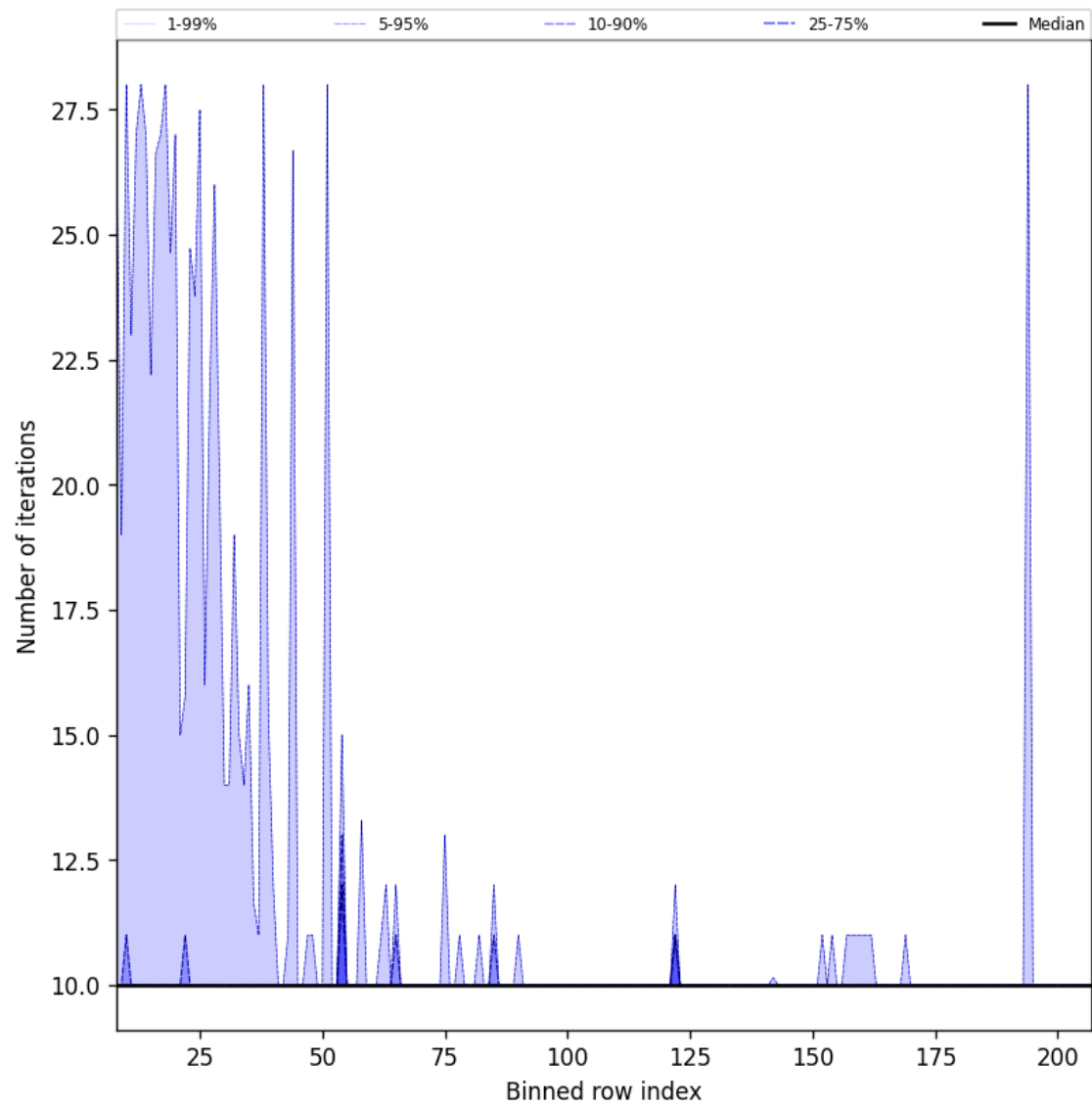
Figure 42: Along track statistics of “Number of iterations” for 2024-11-14 to 2024-11-15
