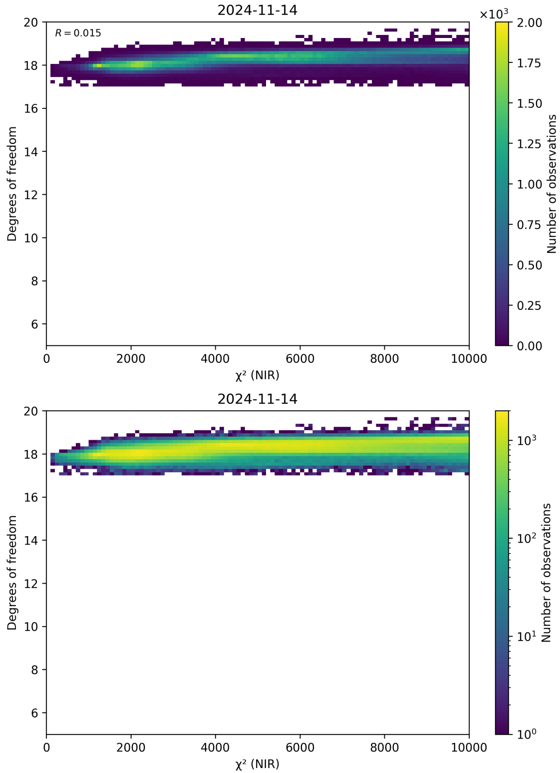
Figure 44: Scatter density plot of “ \chi^2 (NIR)” against “Degrees of freedom” for 2024-11-14 to 2024-11-15.
