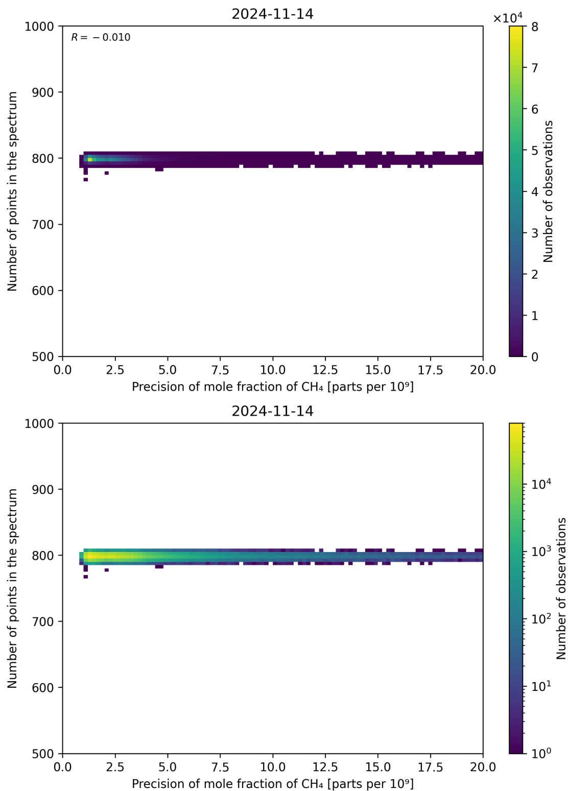
Figure 84: Scatter density plot of “Precision of mole fraction of CH 4 ” against “Number of points in the spectrum” for 2024-11-14 to 2024-11-15.
