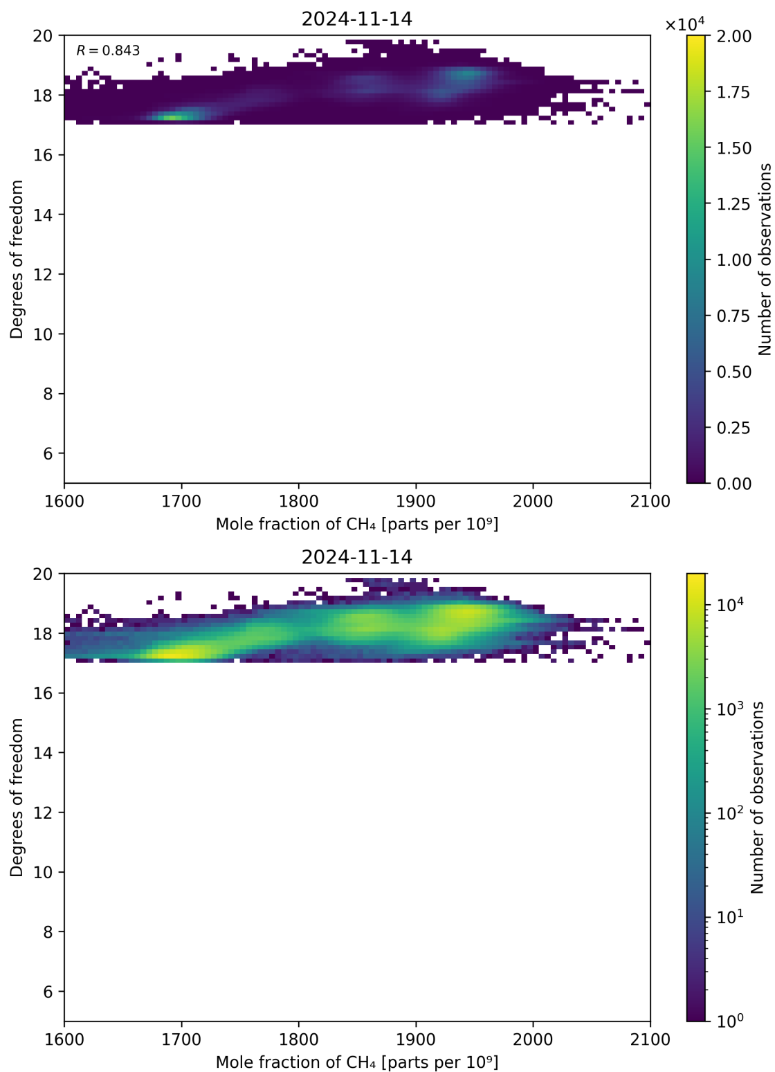
Figure 72: Scatter density plot of “Mole fraction of CH 4 ” against “Degrees of freedom” for 2024-11-14 to 2024-11-15.
