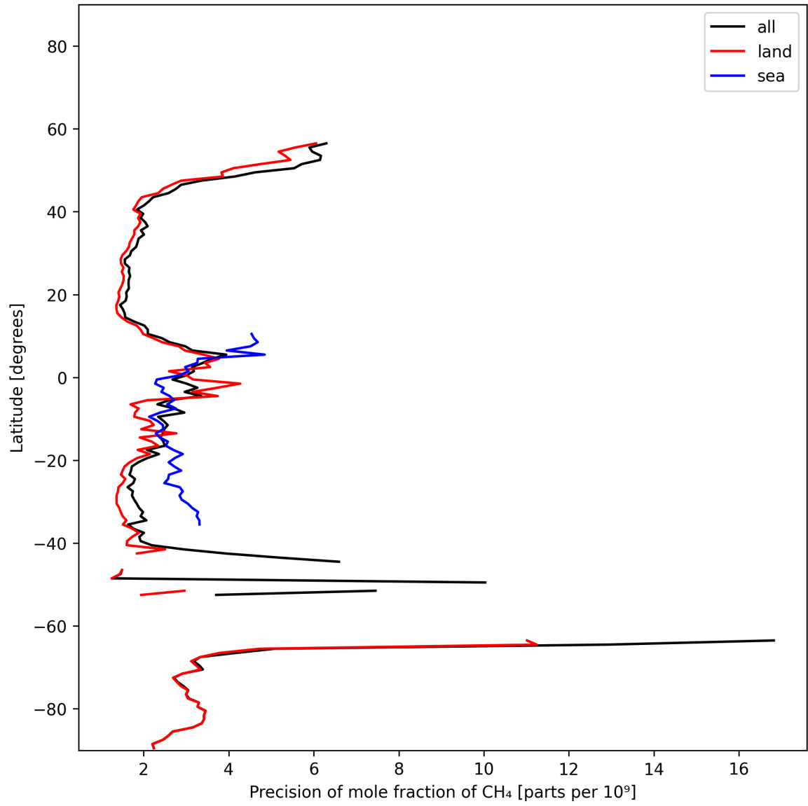
Figure 13: Zonal average of “Precision of mole fraction of CH 4 ” for 2024-11-14 to 2024-11-15.
