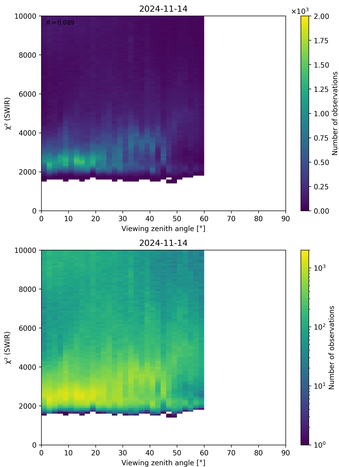
Figure 106: Scatter density plot of “Viewing zenith angle” against “ \chi^2 (SWIR)” for 2024-11-14 to 2024-11-15.
