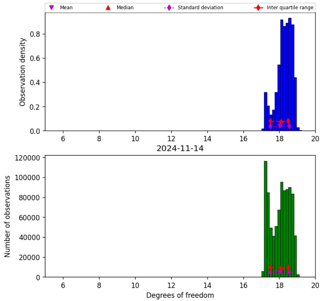
Figure 30: Histogram of “Degrees of freedom” for 2024-11-14 to 2024-11-15
