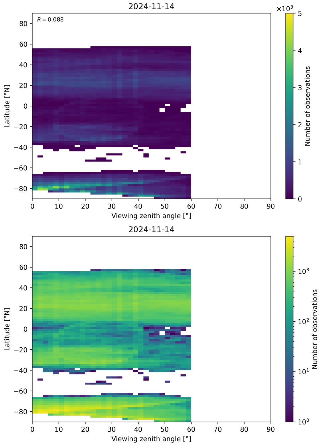
Figure 109: Scatter density plot of “Viewing zenith angle” against “Latitude” for 2024-11-14 to 2024-11-15.
