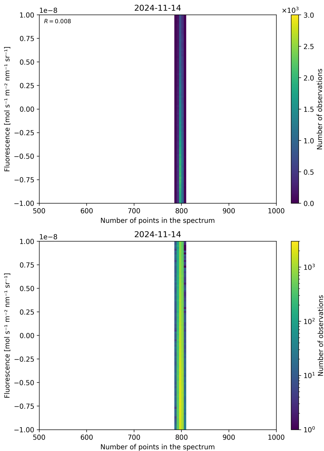
Figure 91: Scatter density plot of “Number of points in the spectrum” against “Fluorescence” for 2024-11-14 to 2024-11-15.
