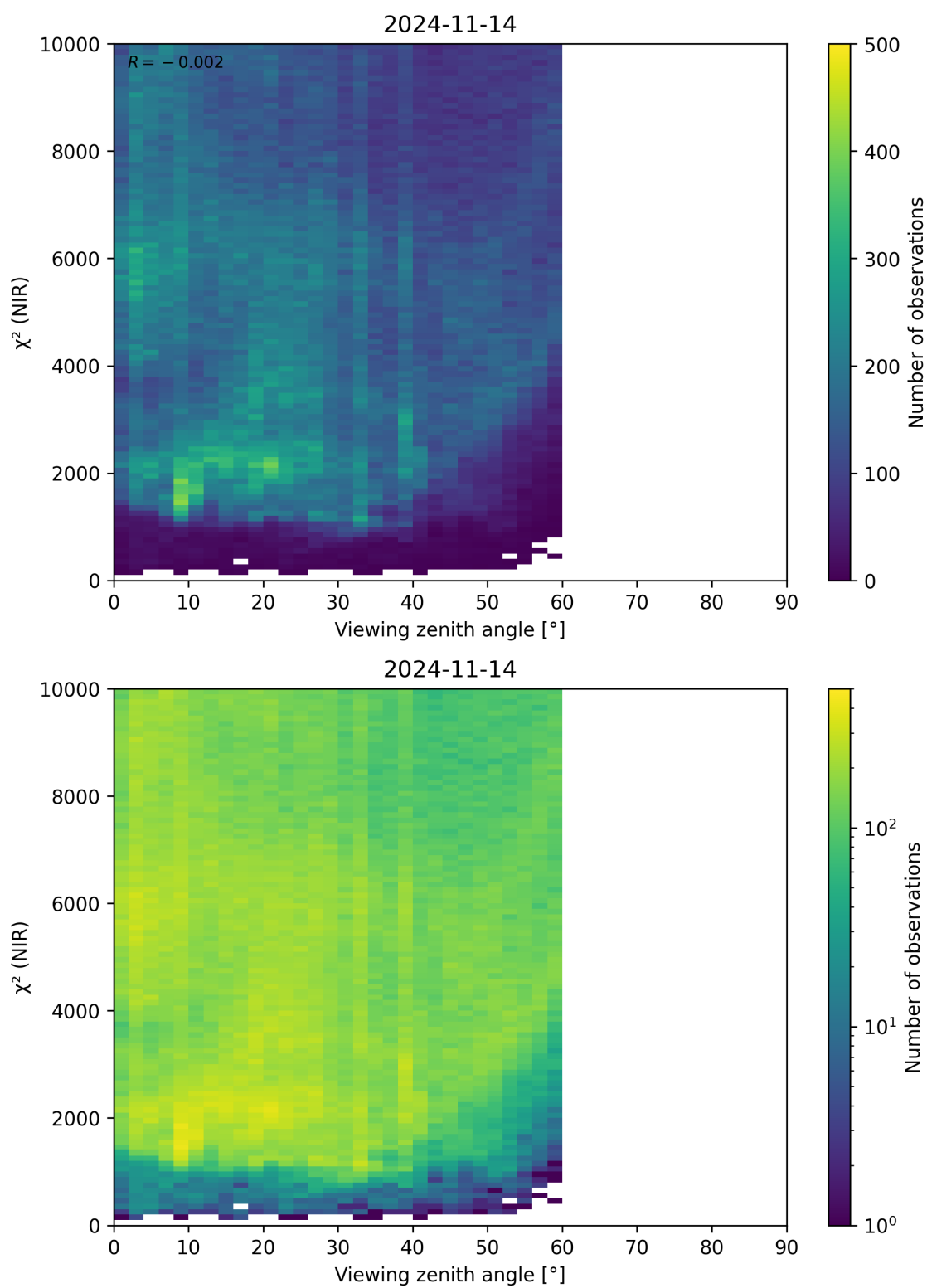
Figure 105: Scatter density plot of “Viewing zenith angle” against “ \chi^2 (NIR)” for 2024-11-14 to 2024-11-15.
