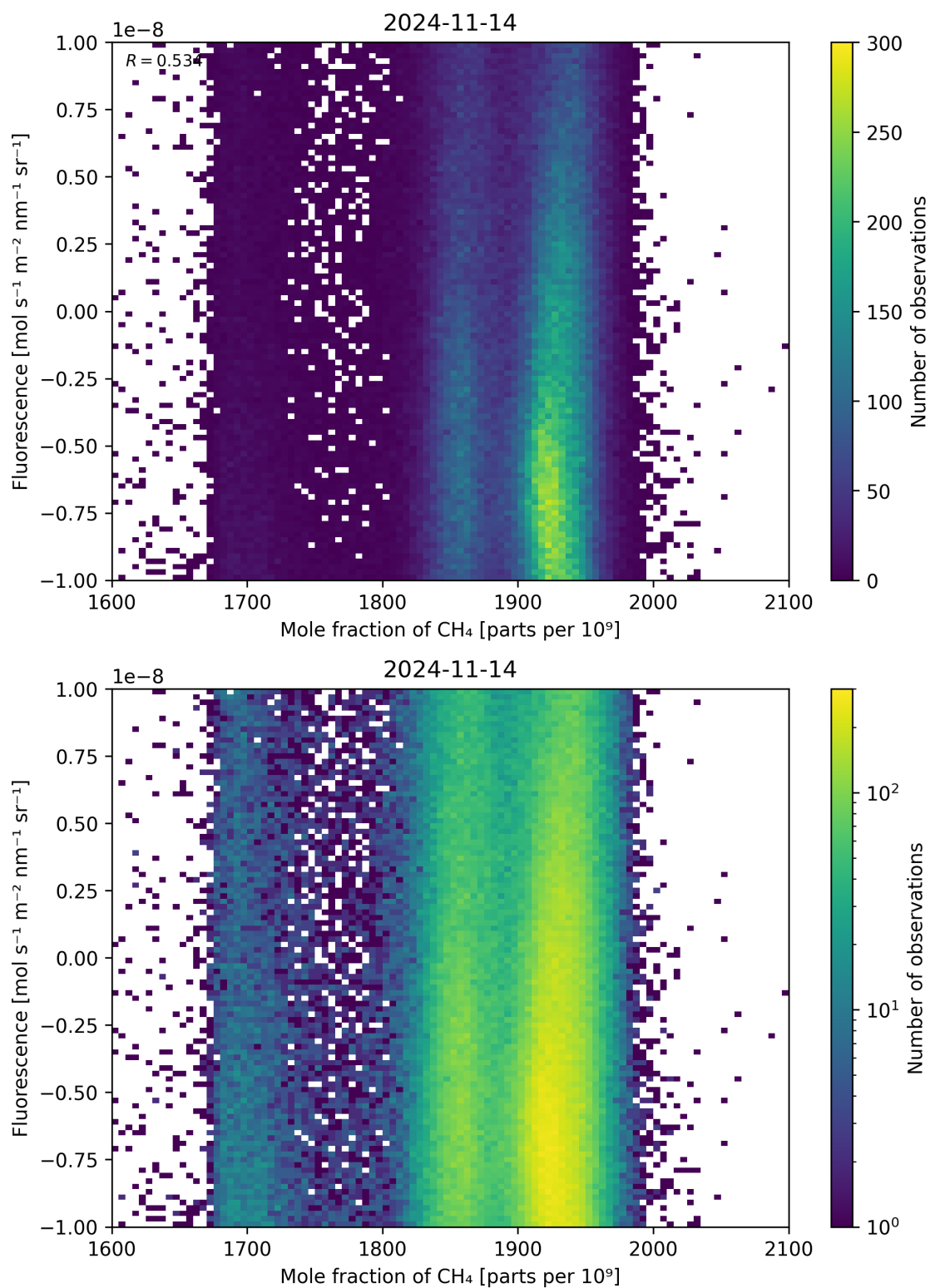
Figure 73: Scatter density plot of “Mole fraction of \text{CH}_4 ” against “Fluorescence” for 2024-11-14 to 2024-11-15.
