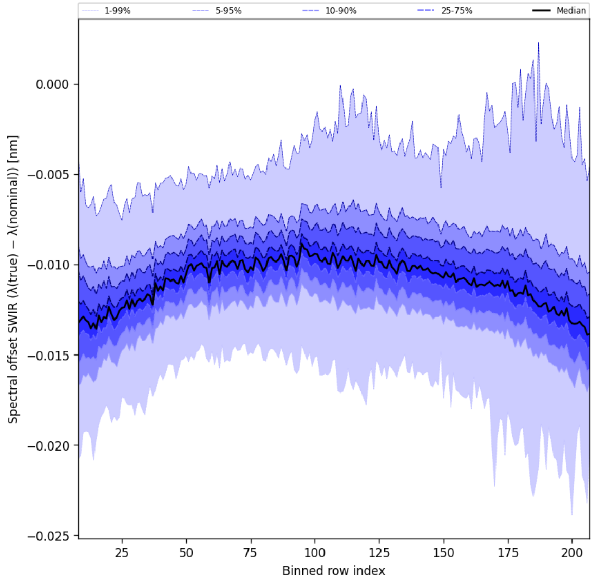
Figure 38: Along track statistics of “Spectral offset SWIR ( \lambda_{\text{true}} - \lambda_{\text{nominal}} )” for 2024-11-14 to 2024-11-15
