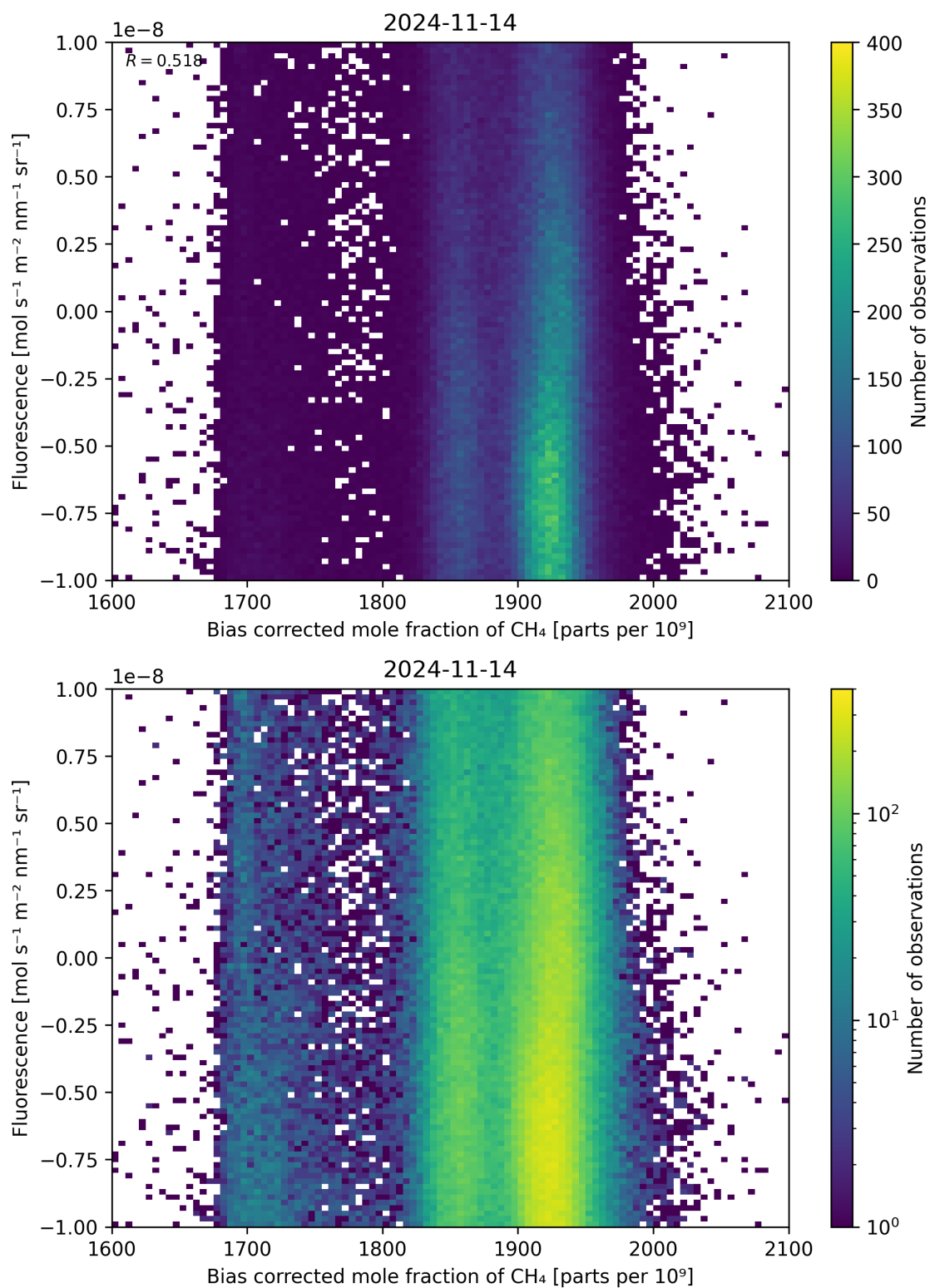
Figure 66: Scatter density plot of “Bias corrected mole fraction of \text{CH}_4 ” against “Fluorescence” for 2024-11-14 to 2024-11-15.
