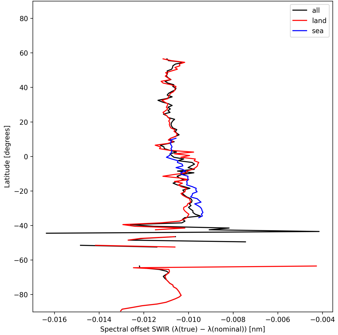
Figure 16: Zonal average of “Spectral offset SWIR ( \lambda_{\text{true}} - \lambda_{\text{nominal}} )” for 2024-11-14 to 2024-11-15.
