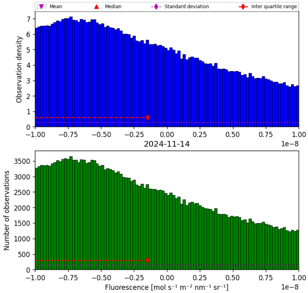
Figure 32: Histogram of “Fluorescence” for 2024-11-14 to 2024-11-15
