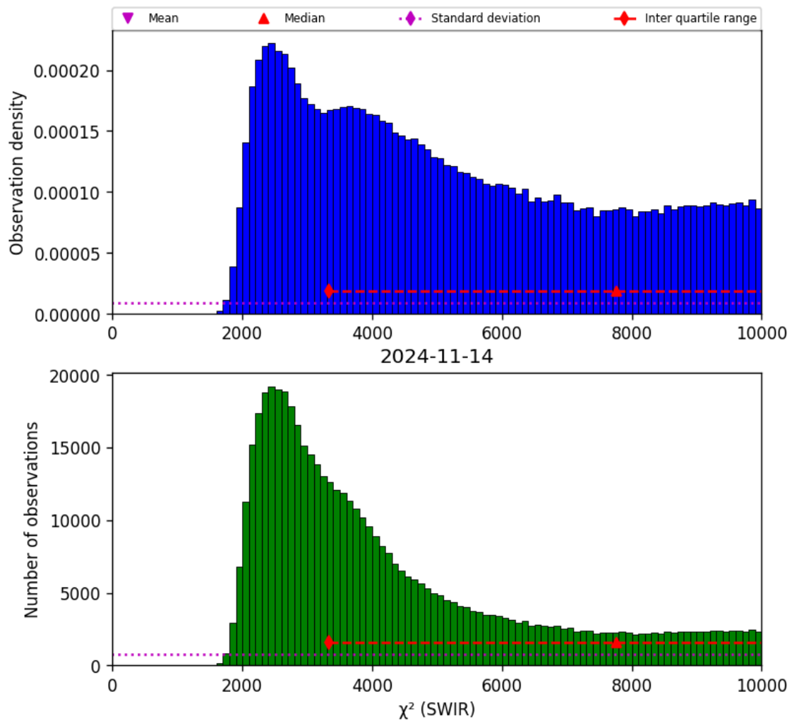
Figure 28: Histogram of “ \chi^2 (SWIR)” for 2024-11-14 to 2024-11-15
