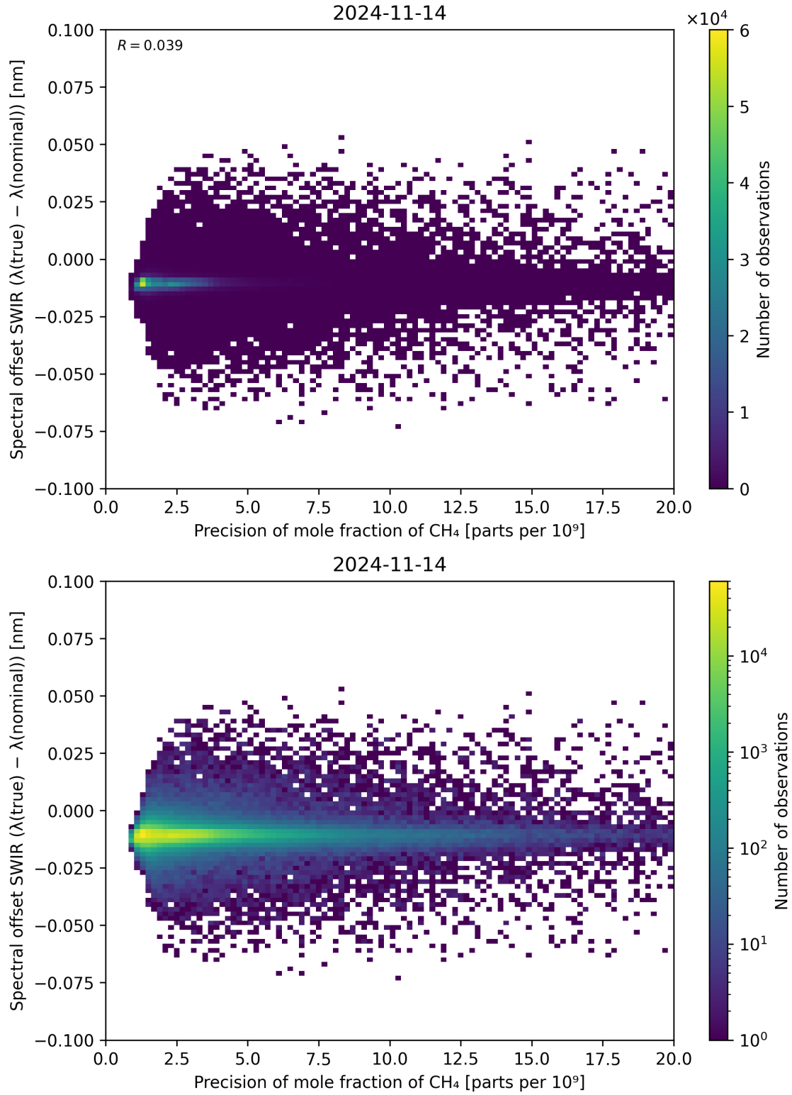
Figure 85: Scatter density plot of “Precision of mole fraction of CH 4 ” against “Spectral offset SWIR ( \lambda_{\text{true}} - \lambda_{\text{nominal}} )” for 2024-11-14 to 2024-11-15.
