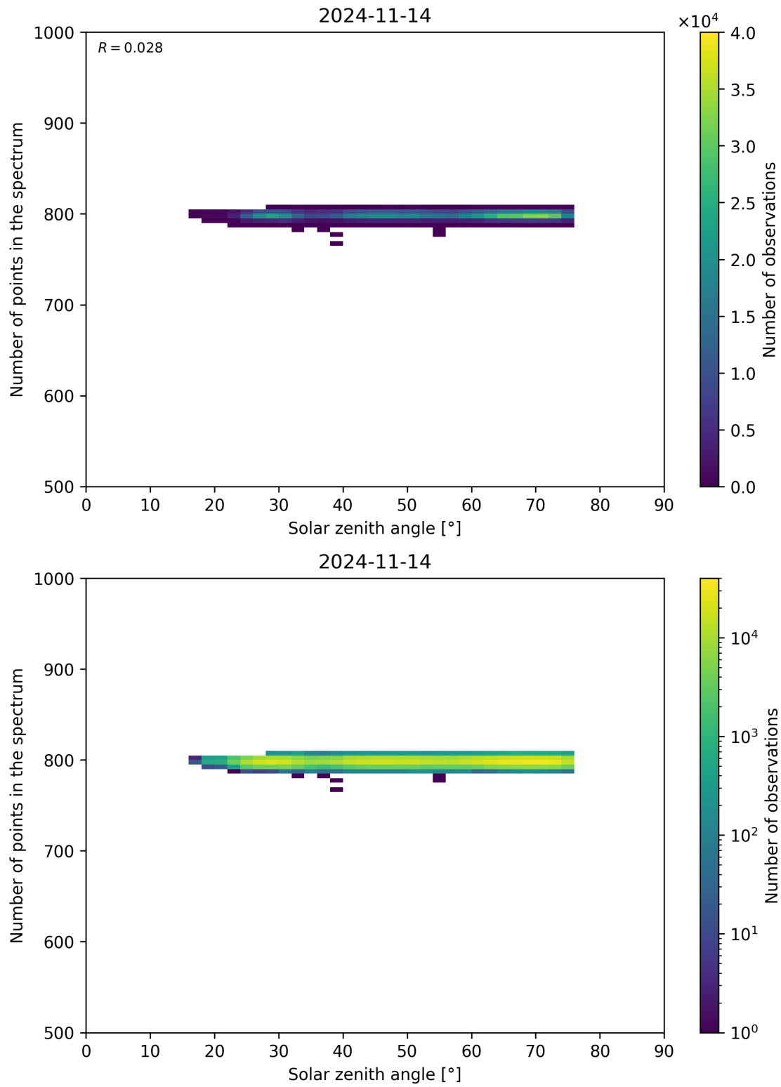
Figure 103: Scatter density plot of “Solar zenith angle” against “Number of points in the spectrum” for 2024-11-14 to 2024-11-15.
