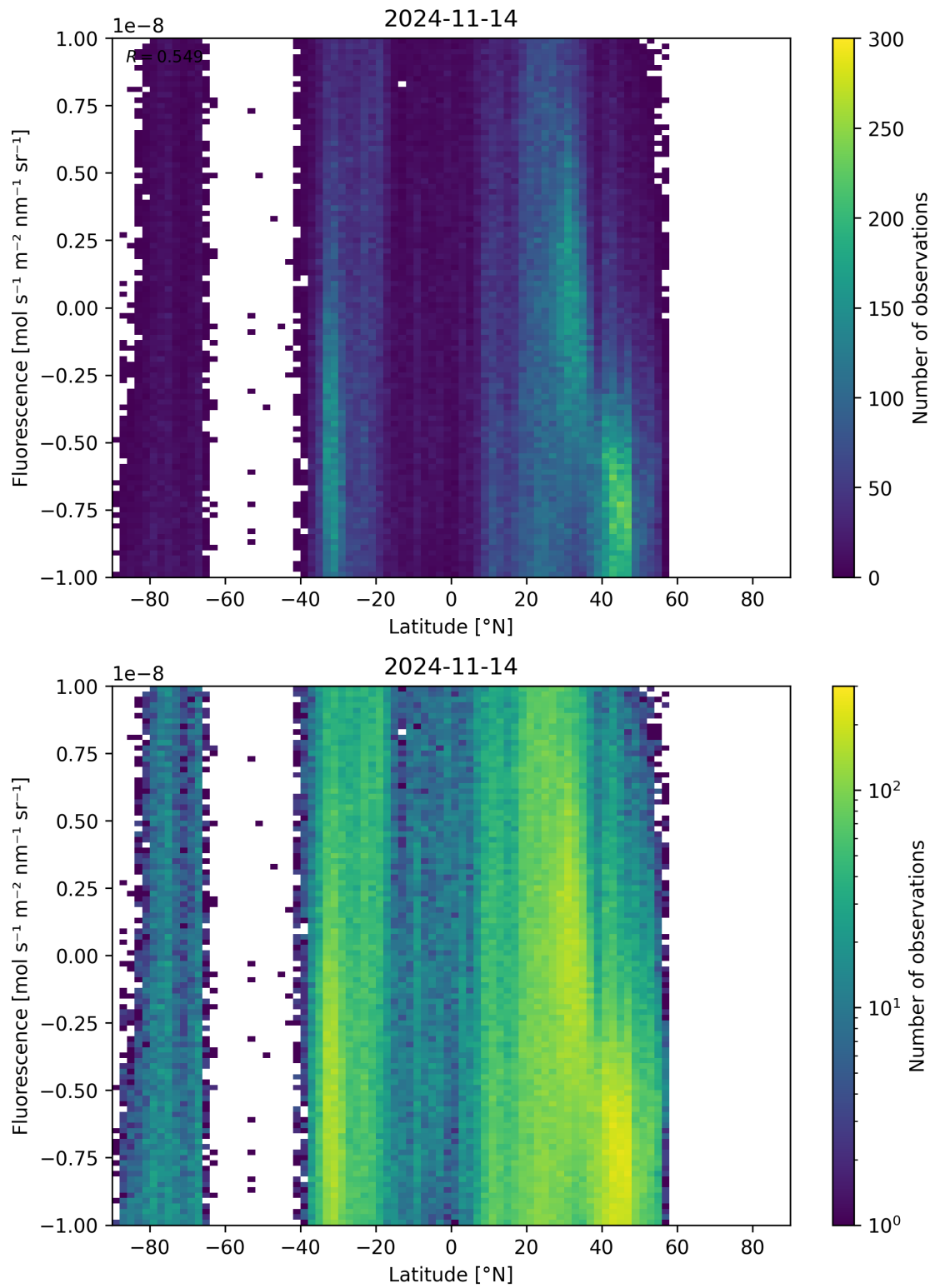
Figure 56: Scatter density plot of “Latitude” against “Fluorescence” for 2024-11-14 to 2024-11-15.
