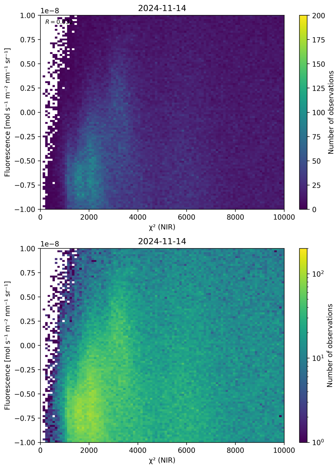
Figure 45: Scatter density plot of “ \chi^2 (NIR)” against “Fluorescence” for 2024-11-14 to 2024-11-15.
