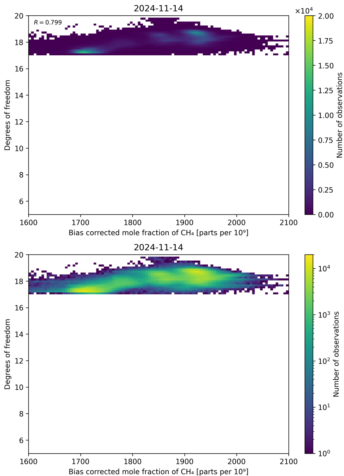
Figure 65: Scatter density plot of “Bias corrected mole fraction of CH 4 ” against “Degrees of freedom” for 2024-11-14 to 2024-11-15.
