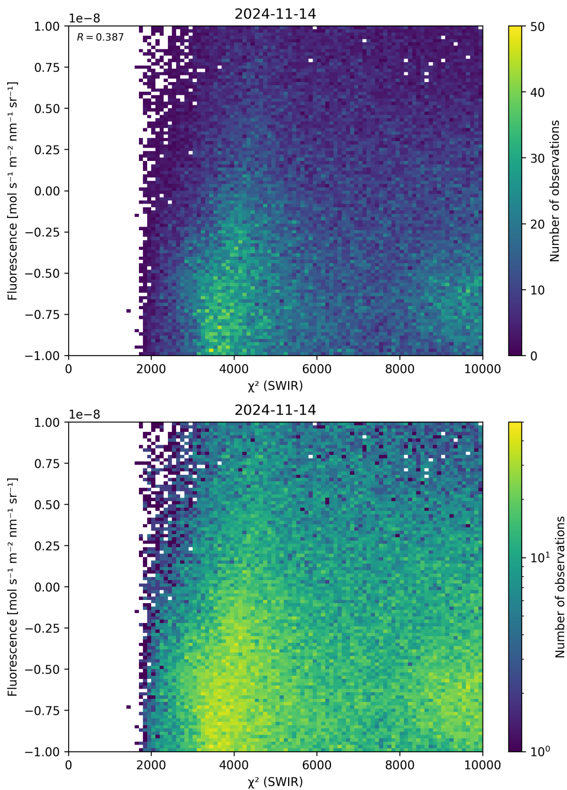
Figure 49: Scatter density plot of “ \chi^2 (SWIR)” against “Fluorescence” for 2024-11-14 to 2024-11-15.
