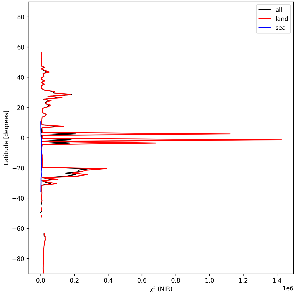
Figure 18: Zonal average of “ \chi^2 (NIR)” for 2024-11-14 to 2024-11-15.
