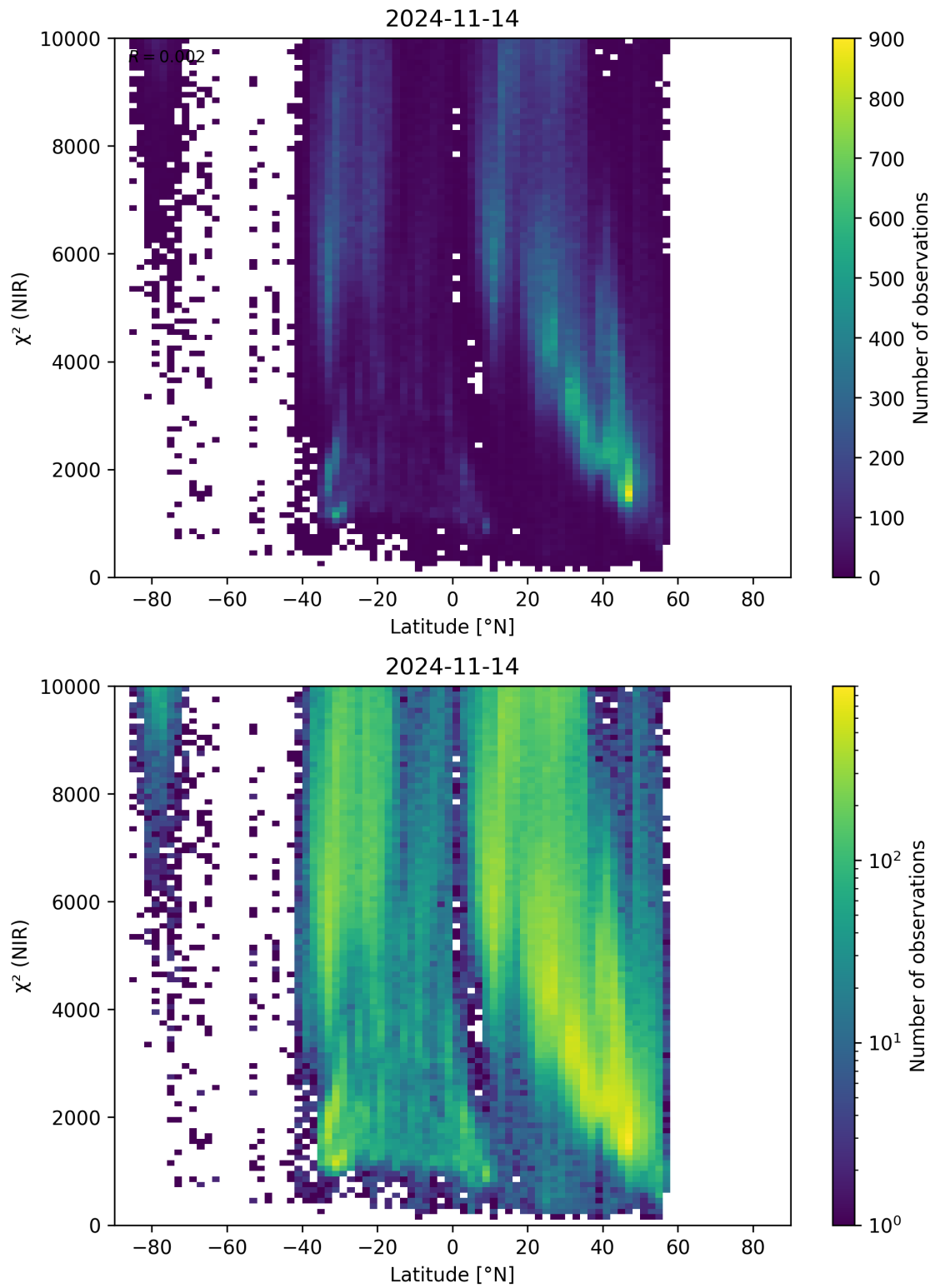
Figure 53: Scatter density plot of “Latitude” against “ \chi^2 (NIR)” for 2024-11-14 to 2024-11-15.
