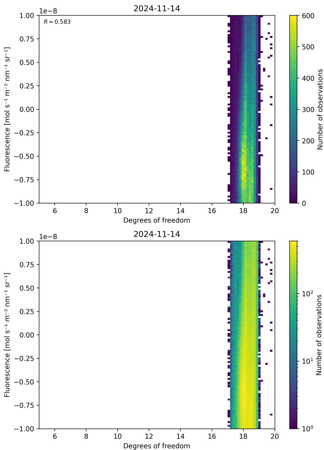
Figure 51: Scatter density plot of “Degrees of freedom” against “Fluorescence” for 2024-11-14 to 2024-11-15.
