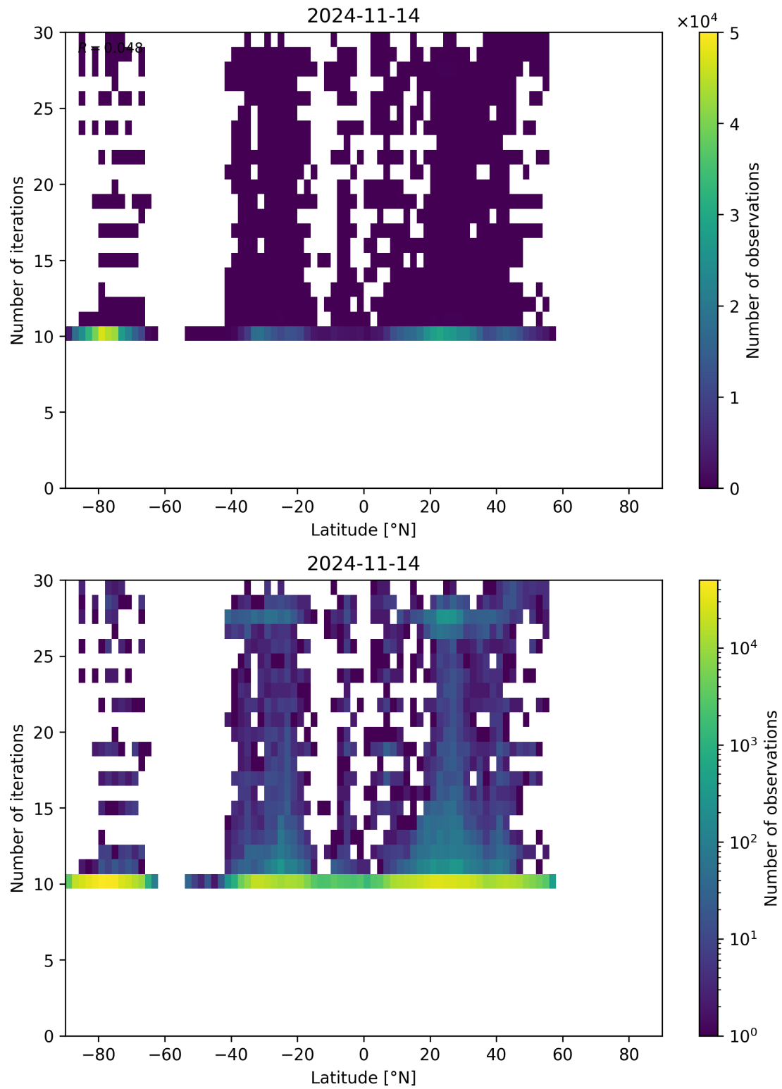
Figure 60: Scatter density plot of “Latitude” against “Number of iterations” for 2024-11-14 to 2024-11-15.
