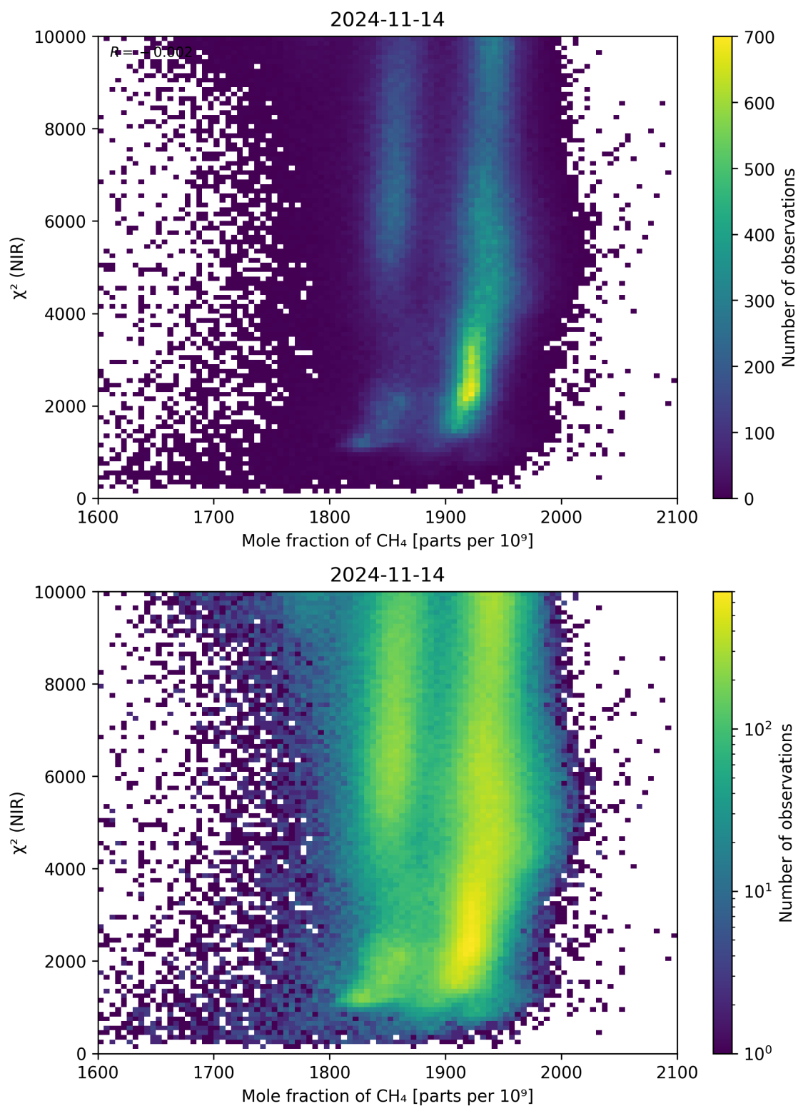
Figure 70: Scatter density plot of “Mole fraction of \text{CH}_4 ” against “ \chi^2 (NIR)” for 2024-11-14 to 2024-11-15.
