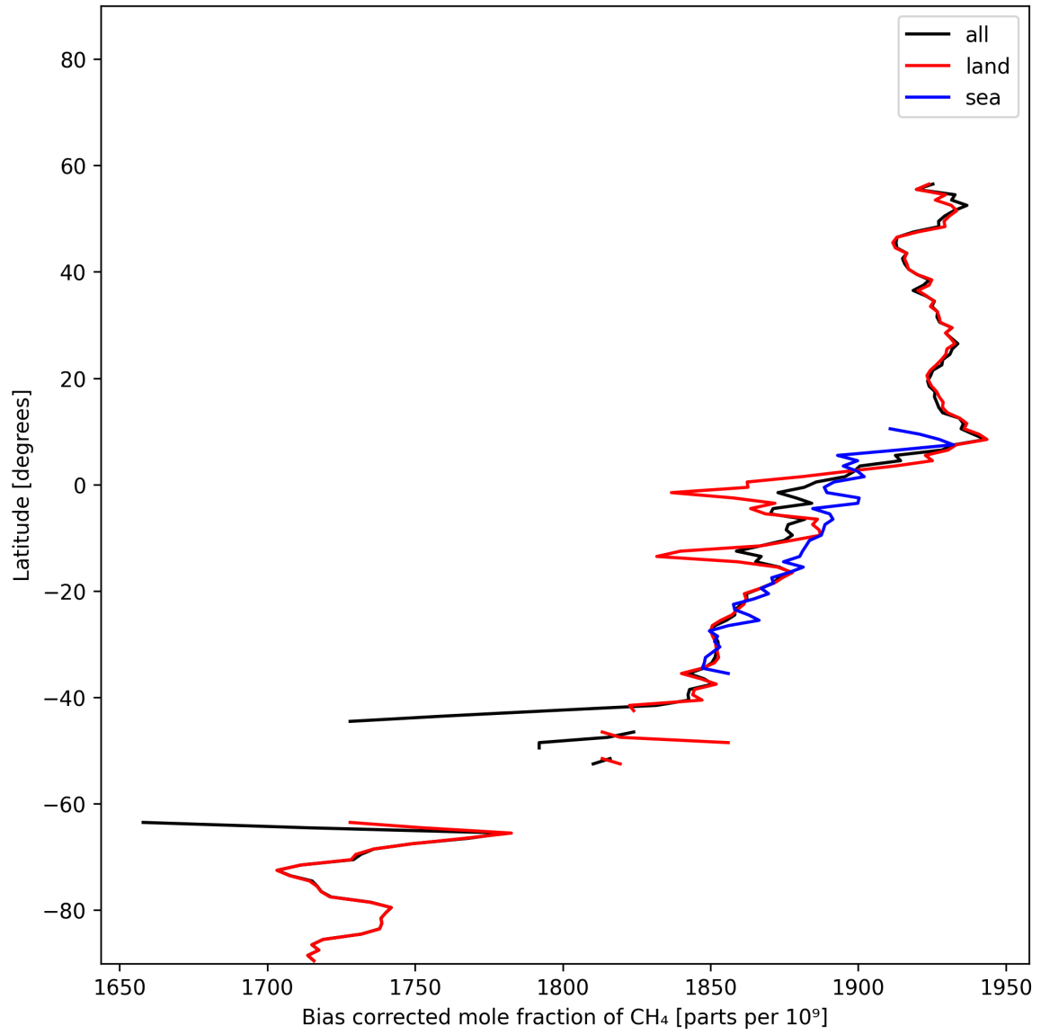
Figure 14: Zonal average of “Bias corrected mole fraction of CH 4 ” for 2024-11-14 to 2024-11-15.
