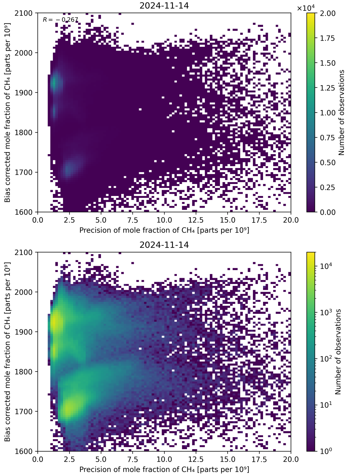
Figure 82: Scatter density plot of “Precision of mole fraction of CH 4 ” against “Bias corrected mole fraction of CH 4 ” for 2024-11-14 to 2024-11-15.
