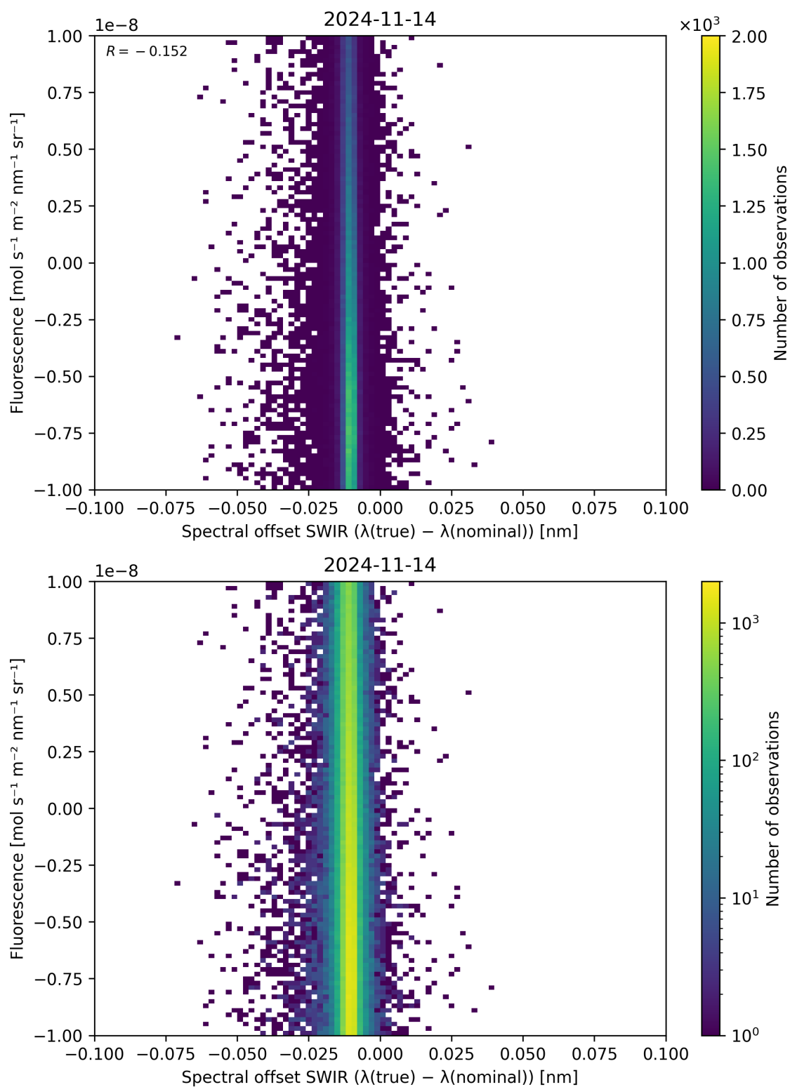
Figure 120: Scatter density plot of “Spectral offset SWIR ( \lambda_{\text{true}} - \lambda_{\text{nominal}} )” against “Fluorescence” for 2024-11-14 to 2024-11-15.
