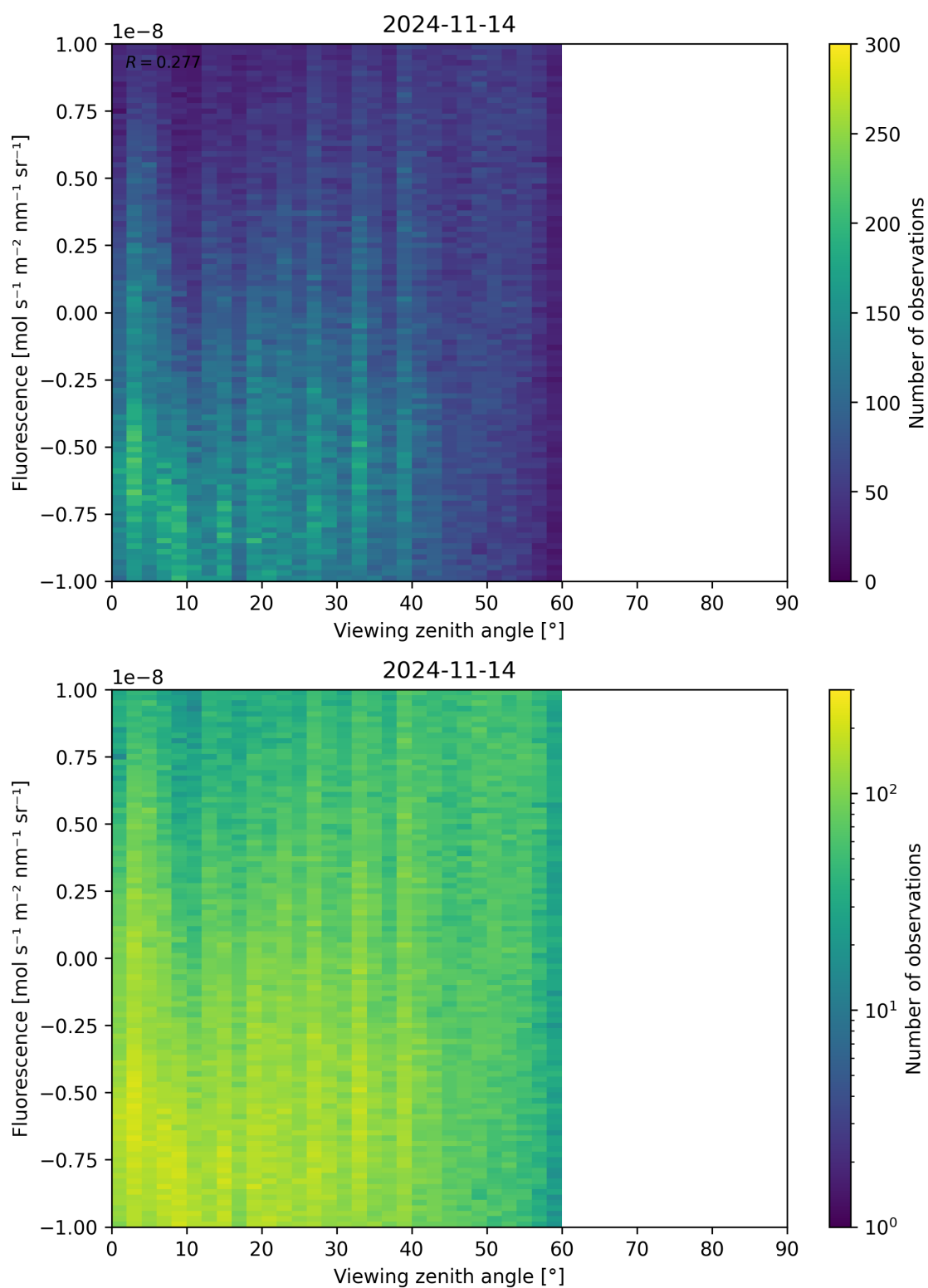
Figure 108: Scatter density plot of “Viewing zenith angle” against “Fluorescence” for 2024-11-14 to 2024-11-15.
