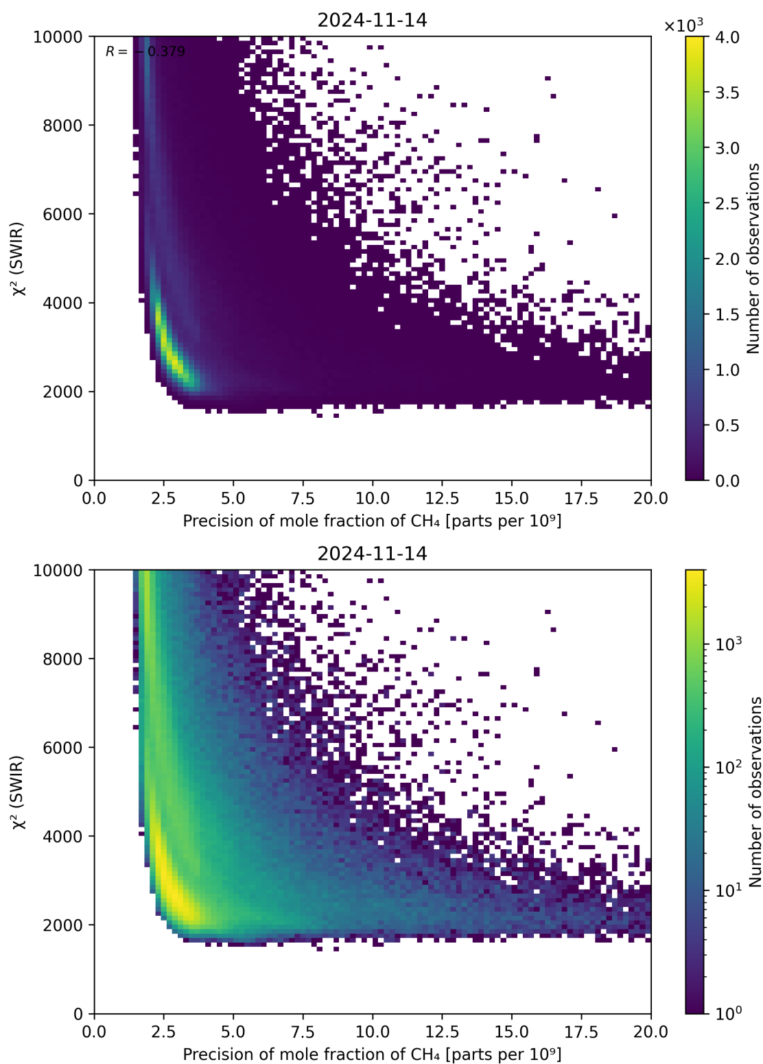
Figure 79: Scatter density plot of “Precision of mole fraction of \text{CH}_4 ” against “ \chi^2 (SWIR)” for 2024-11-14 to 2024-11-15.
