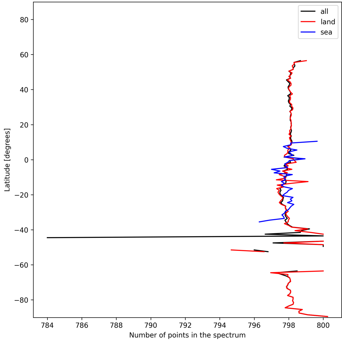
Figure 15: Zonal average of “Number of points in the spectrum” for 2024-11-14 to 2024-11-15.
