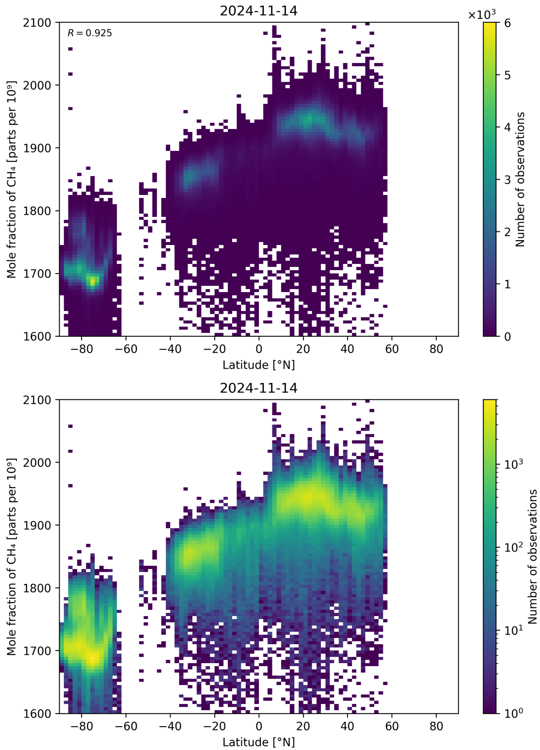
Figure 57: Scatter density plot of “Latitude” against “Mole fraction of CH 4 ” for 2024-11-14 to 2024-11-15.
