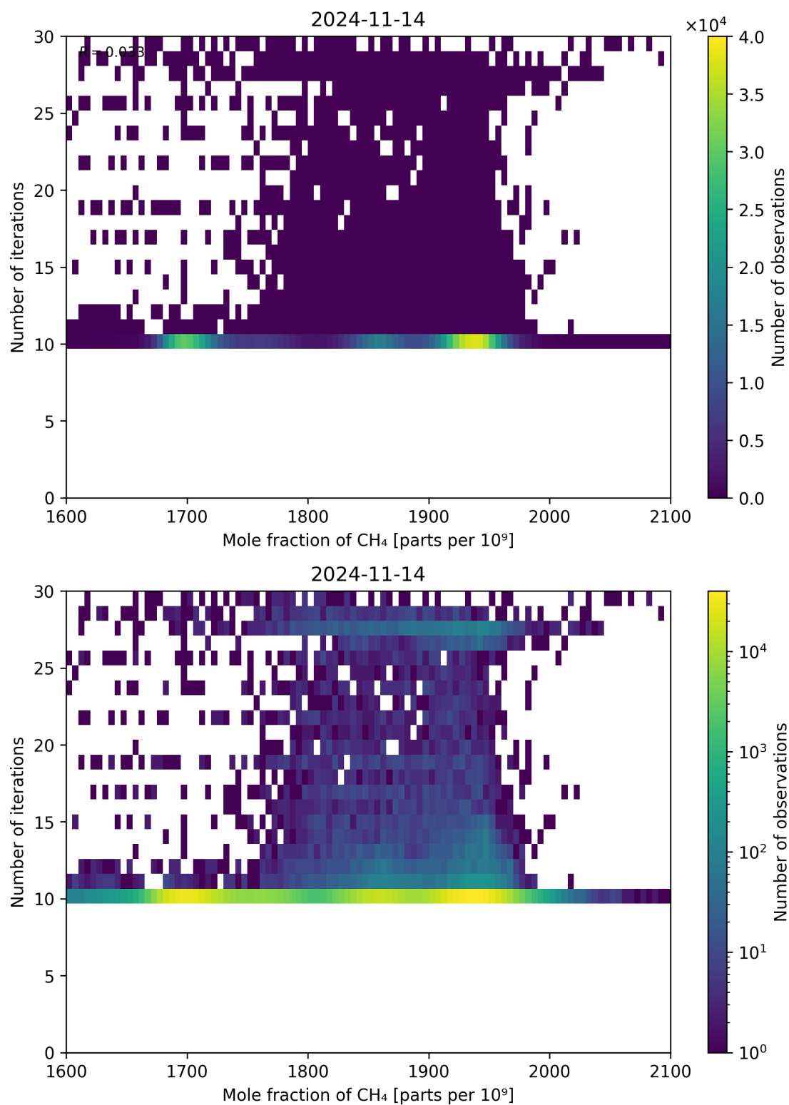
Figure 76: Scatter density plot of “Mole fraction of CH 4 ” against “Number of iterations” for 2024-11-14 to 2024-11-15.
