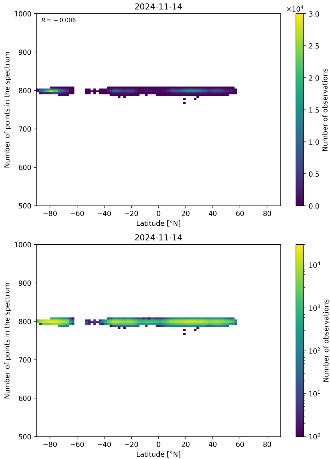
Figure 61: Scatter density plot of “Latitude” against “Number of points in the spectrum” for 2024-11-14 to 2024-11-15.
