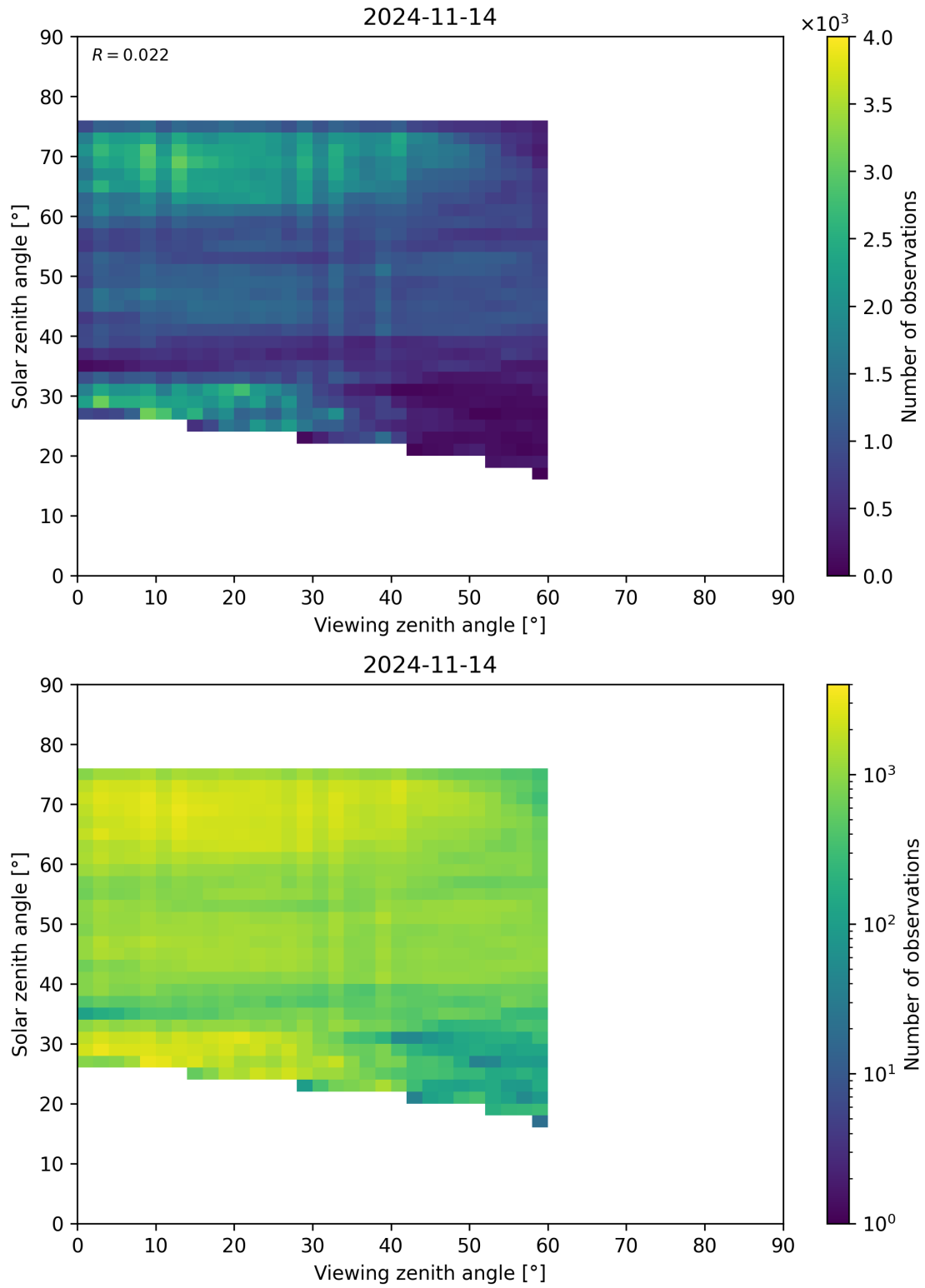
Figure 115: Scatter density plot of “Viewing zenith angle” against “Solar zenith angle” for 2024-11-14 to 2024-11-15.
