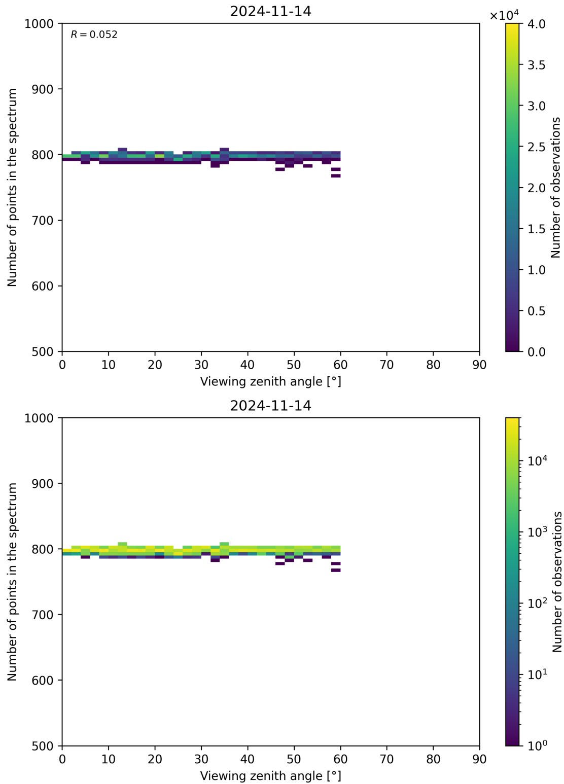
Figure 114: Scatter density plot of “Viewing zenith angle” against “Number of points in the spectrum” for 2024-11-14 to 2024-11-15.
