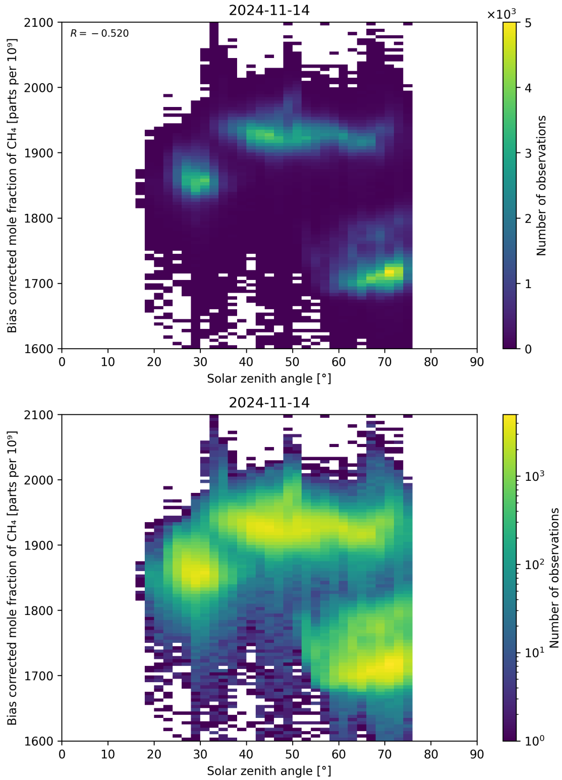
Figure 100: Scatter density plot of “Solar zenith angle” against “Bias corrected mole fraction of CH 4 ” for 2024-11-14 to 2024-11-15.
