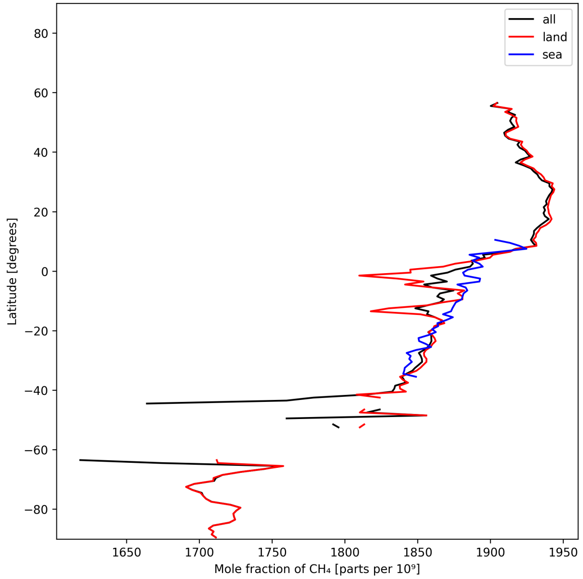
Figure 12: Zonal average of “Mole fraction of \text{CH}_4 ” for 2024-11-14 to 2024-11-15.
