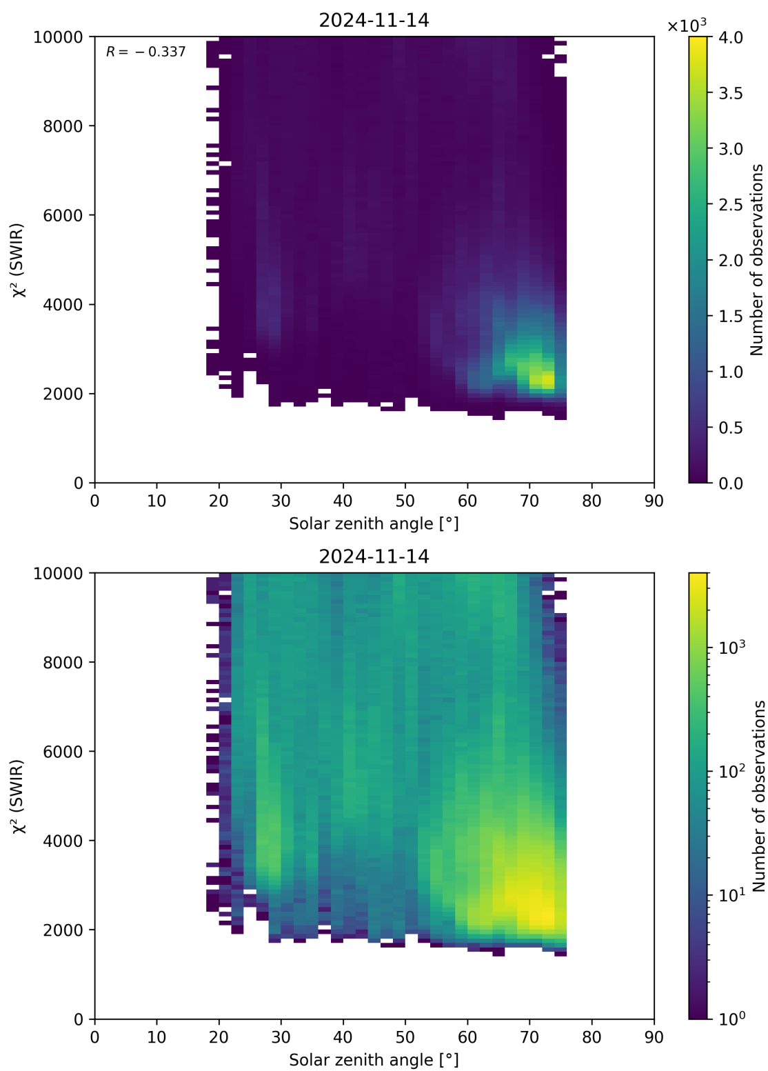
Figure 95: Scatter density plot of “Solar zenith angle” against “ \chi^2 (SWIR)” for 2024-11-14 to 2024-11-15.
