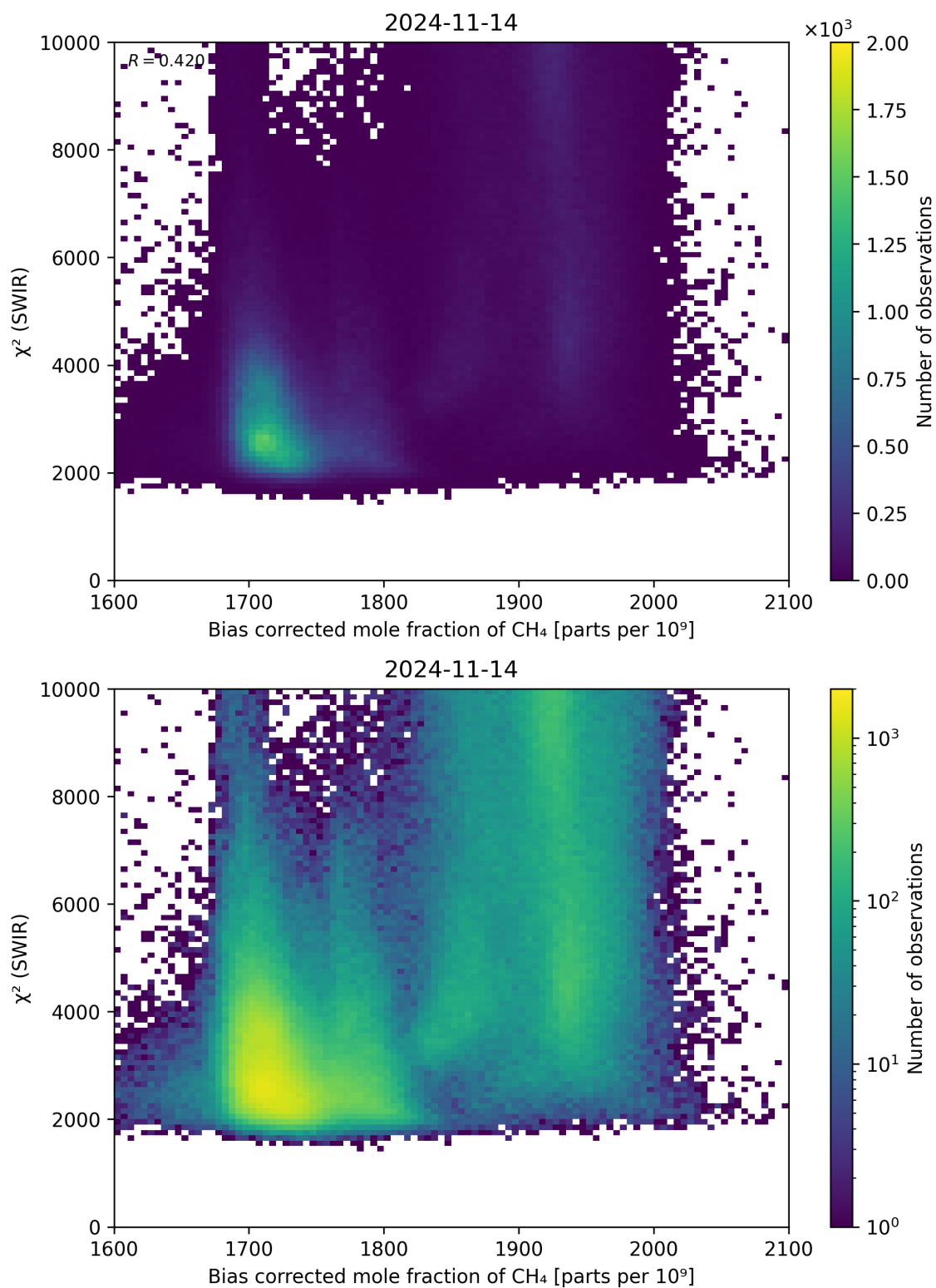
Figure 64: Scatter density plot of “Bias corrected mole fraction of \text{CH}_4 ” against “ \chi^2 (SWIR)” for 2024-11-14 to 2024-11-15.
