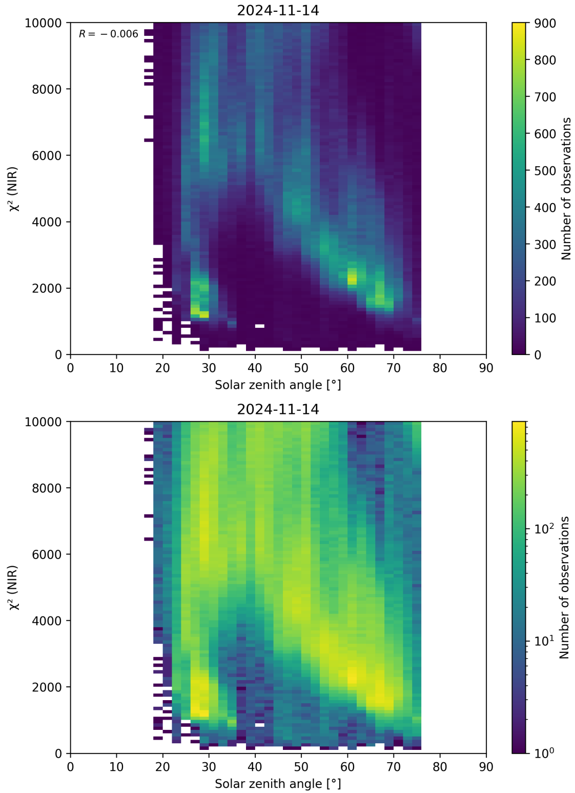
Figure 94: Scatter density plot of “Solar zenith angle” against “ \chi^2 (NIR)” for 2024-11-14 to 2024-11-15.
