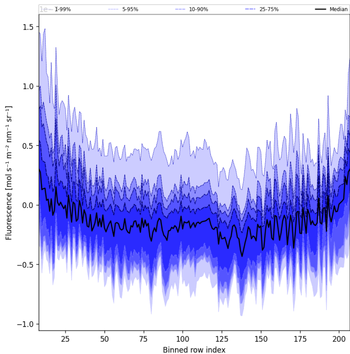
Figure 43: Along track statistics of “Fluorescence” for 2024-11-14 to 2024-11-15
