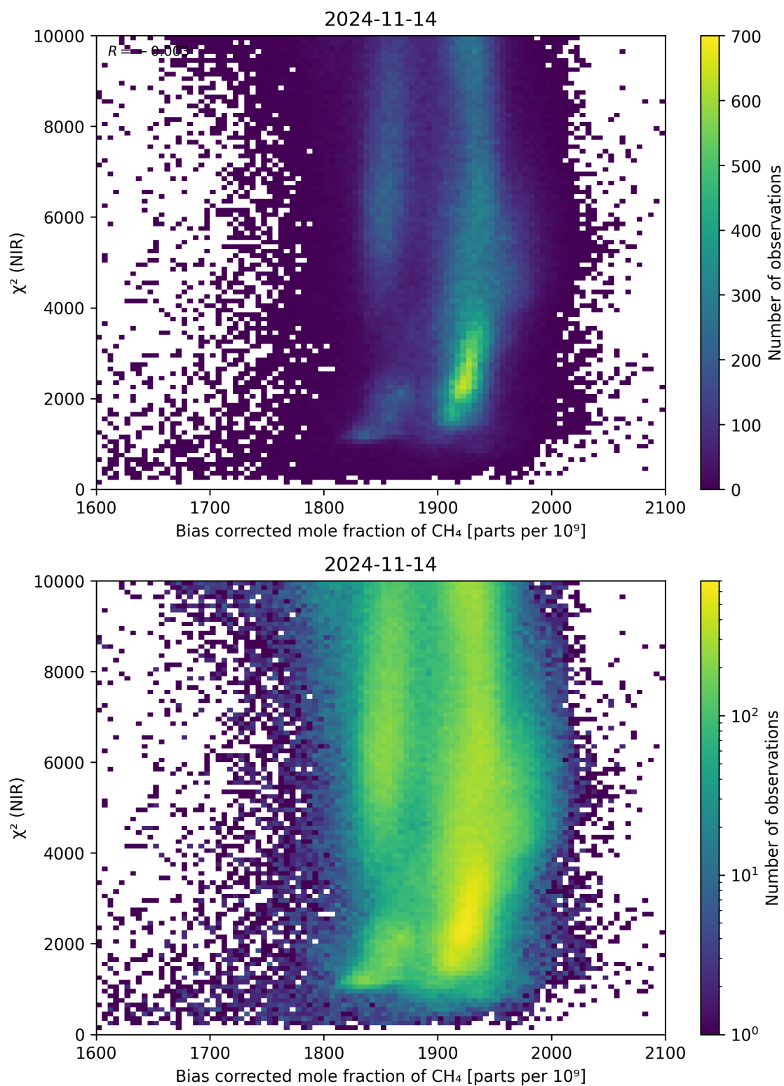
Figure 63: Scatter density plot of “Bias corrected mole fraction of \text{CH}_4 ” against “ \chi^2 (NIR)” for 2024-11-14 to 2024-11-15.
