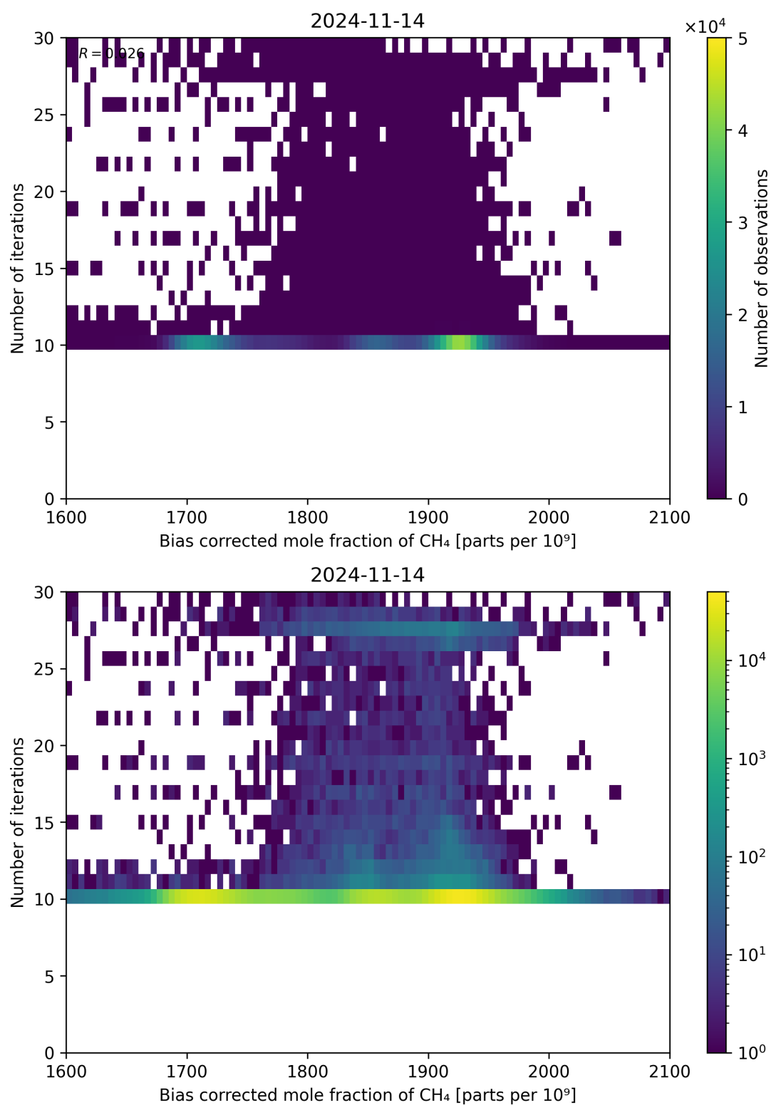
Figure 67: Scatter density plot of “Bias corrected mole fraction of \text{CH}_4 ” against “Number of iterations” for 2024-11-14 to 2024-11-15.
