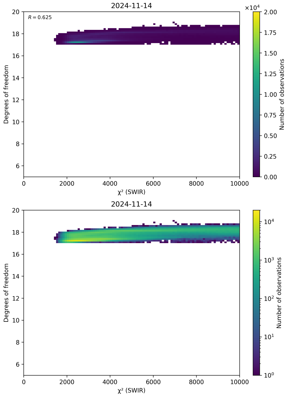
Figure 48: Scatter density plot of “ \chi^2 (SWIR)” against “Degrees of freedom” for 2024-11-14 to 2024-11-15.
