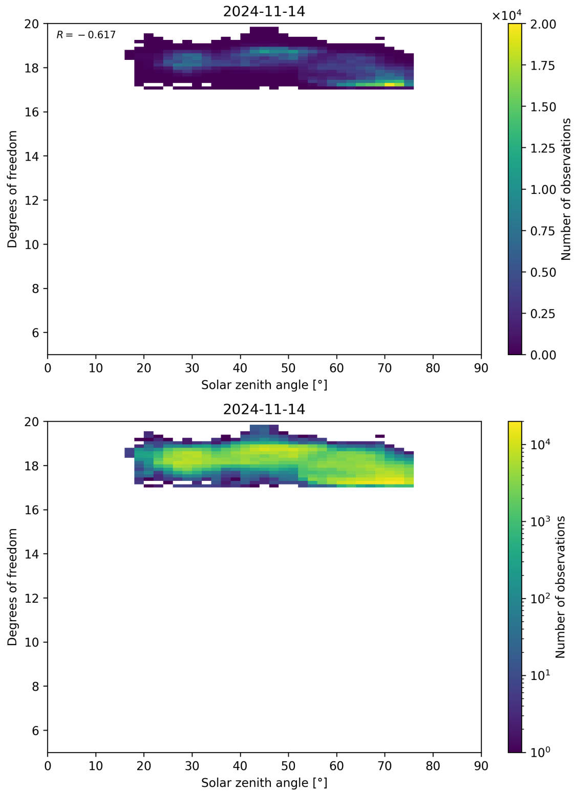
Figure 96: Scatter density plot of “Solar zenith angle” against “Degrees of freedom” for 2024-11-14 to 2024-11-15.
