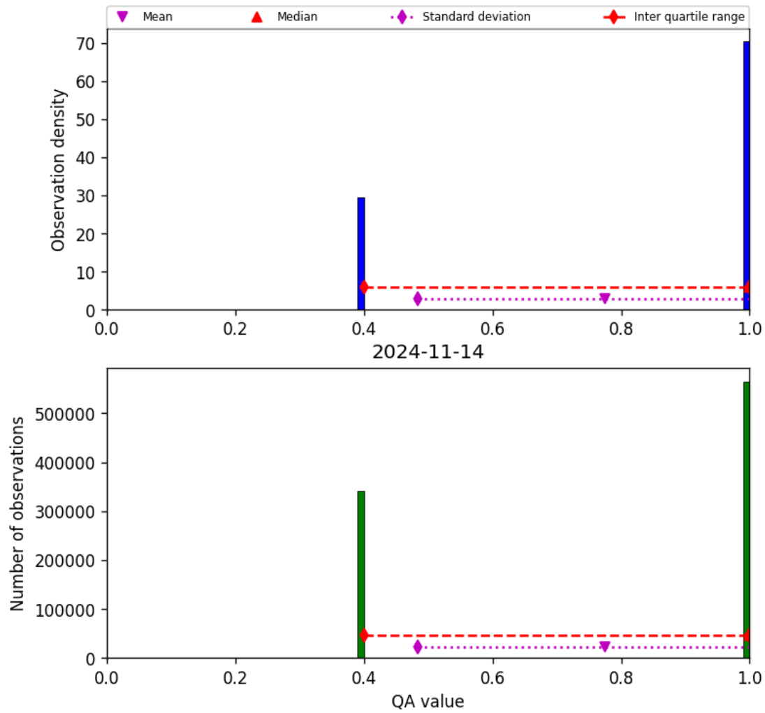
Figure 22: Histogram of “QA value” for 2024-11-14 to 2024-11-15
