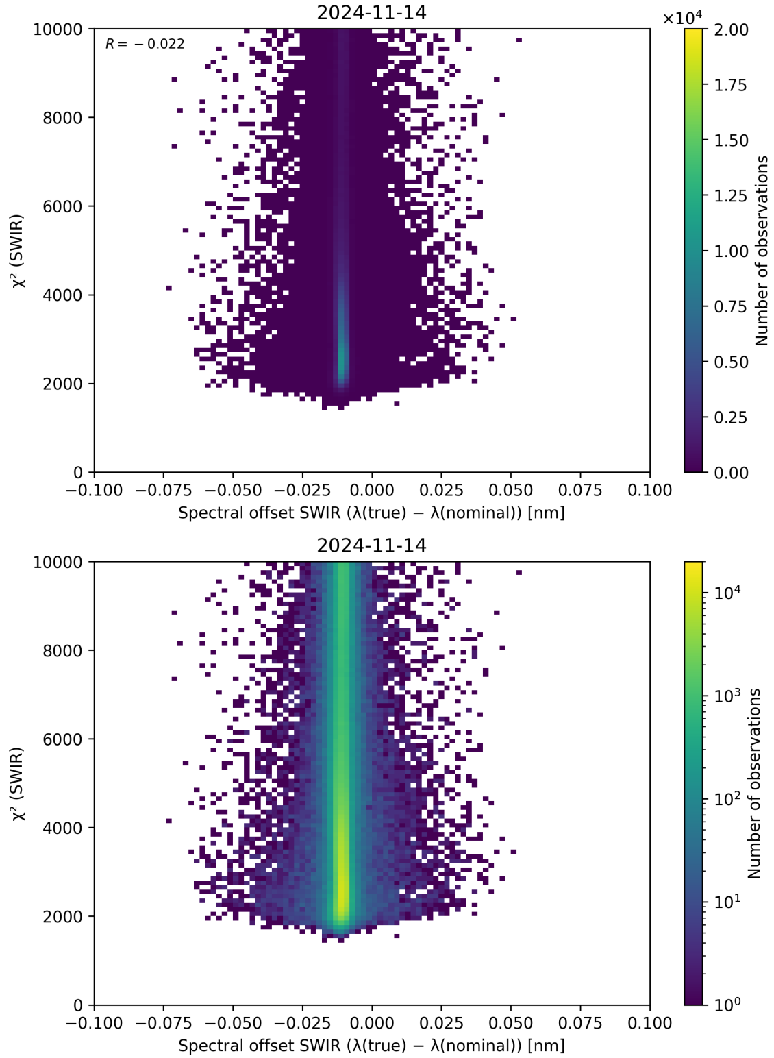
Figure 118: Scatter density plot of “Spectral offset SWIR ( \lambda_{\text{true}} - \lambda_{\text{nominal}} )” against “ \chi^2 (SWIR)” for 2024-11-14 to 2024-11-15.
