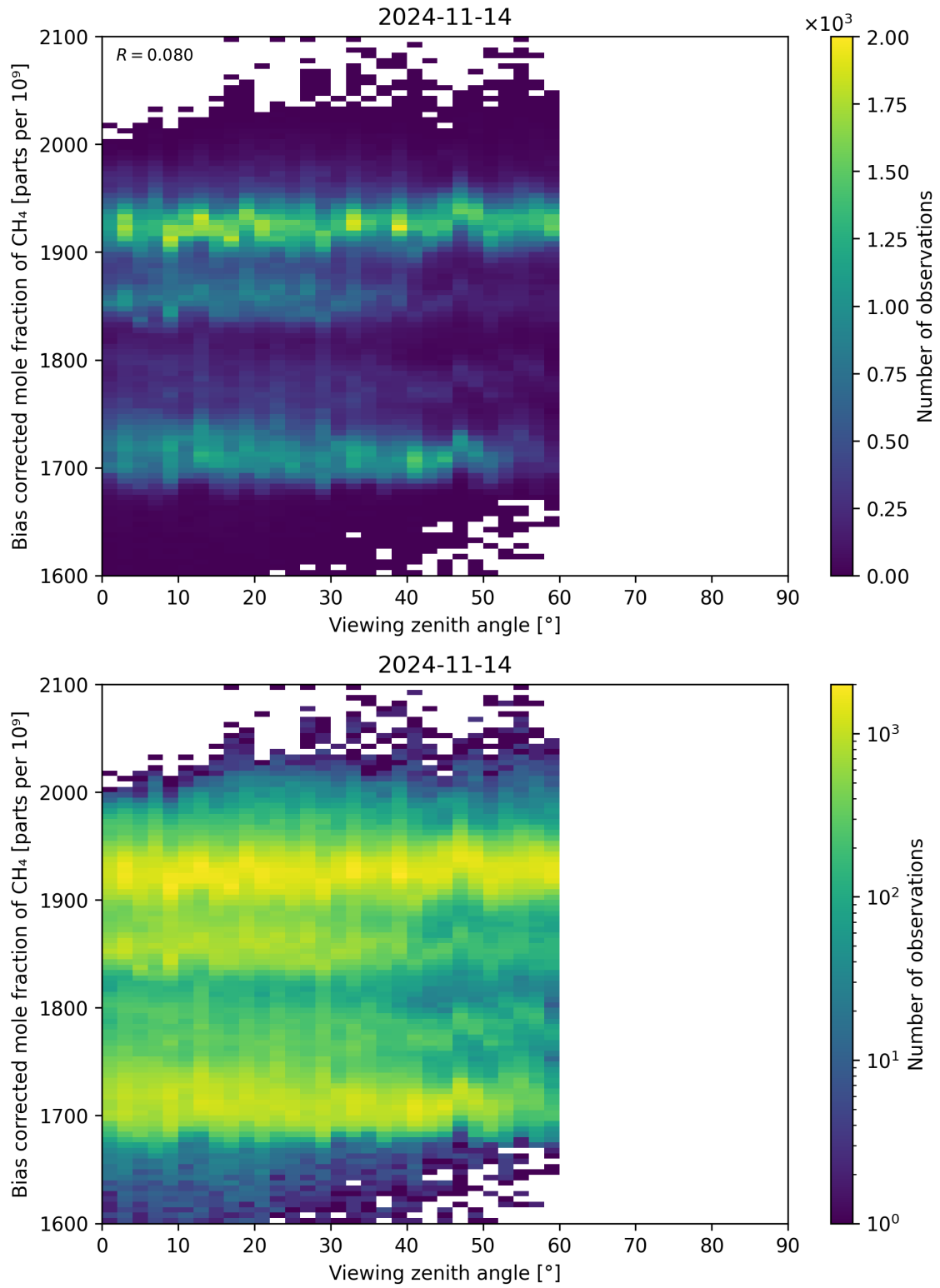
Figure 111: Scatter density plot of “Viewing zenith angle” against “Bias corrected mole fraction of CH 4 ” for 2024-11-14 to 2024-11-15.
