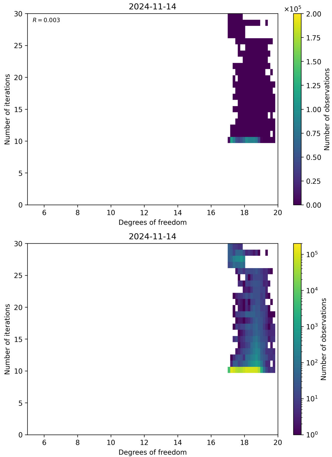
Figure 52: Scatter density plot of “Degrees of freedom” against “Number of iterations” for 2024-11-14 to 2024-11-15.
