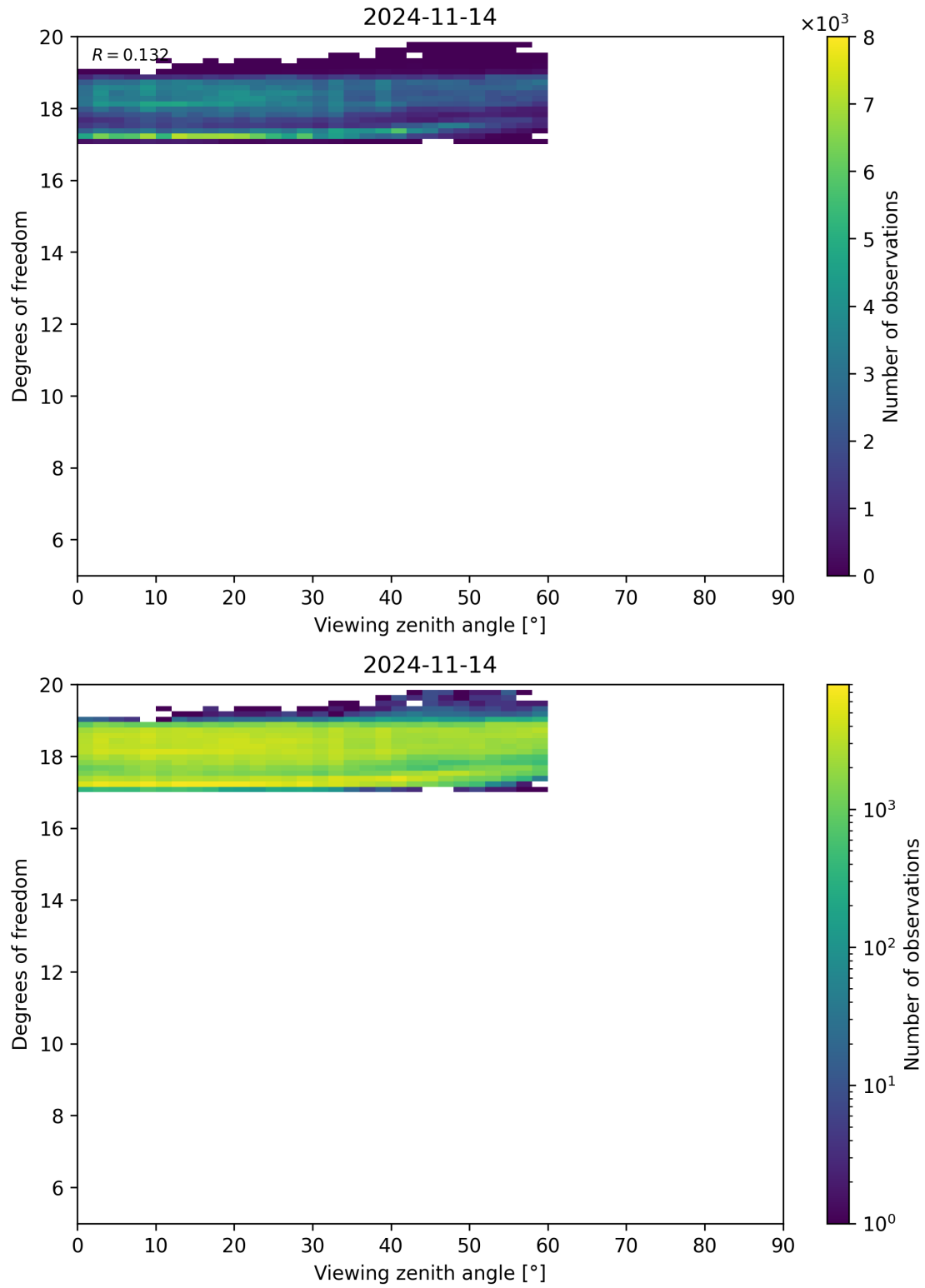
Figure 107: Scatter density plot of “Viewing zenith angle” against “Degrees of freedom” for 2024-11-14 to 2024-11-15.
