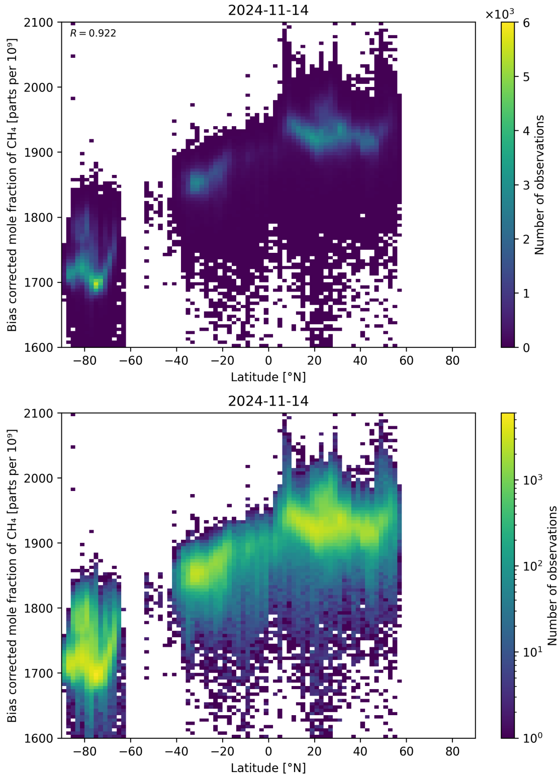
Figure 58: Scatter density plot of “Latitude” against “Bias corrected mole fraction of CH 4 ” for 2024-11-14 to 2024-11-15.
