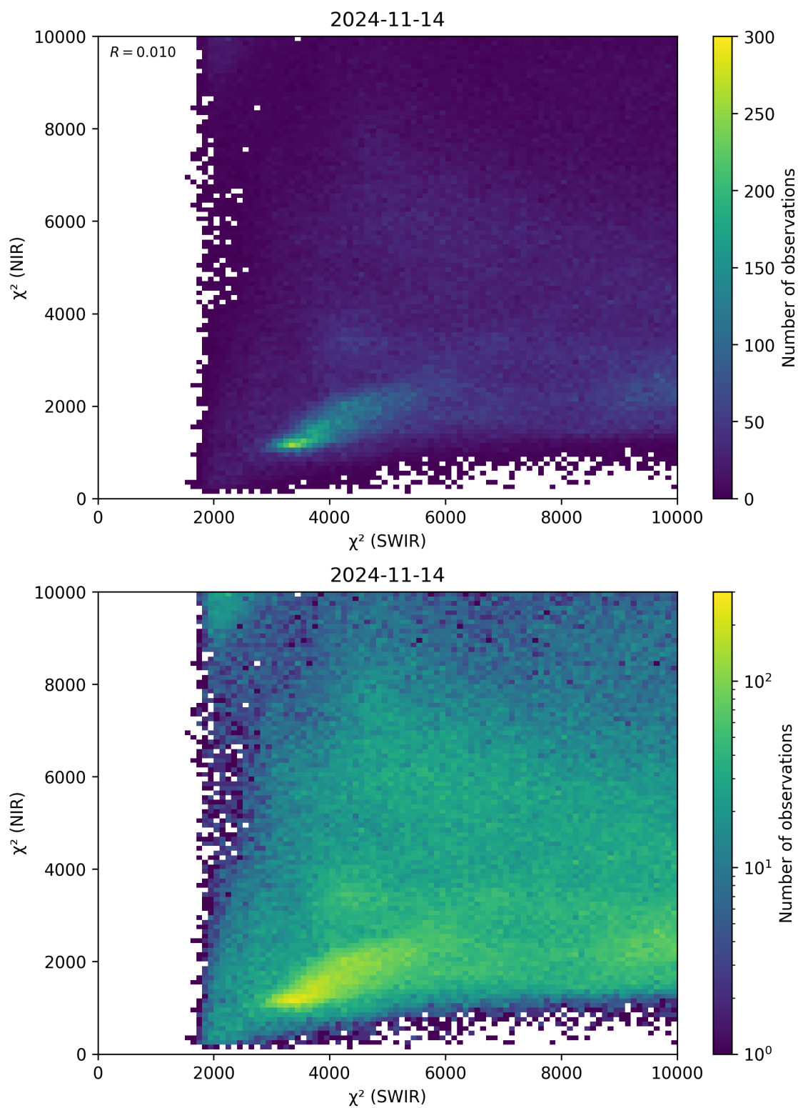
Figure 47: Scatter density plot of “ \chi^2 (SWIR)” against “ \chi^2 (NIR)” for 2024-11-14 to 2024-11-15.
