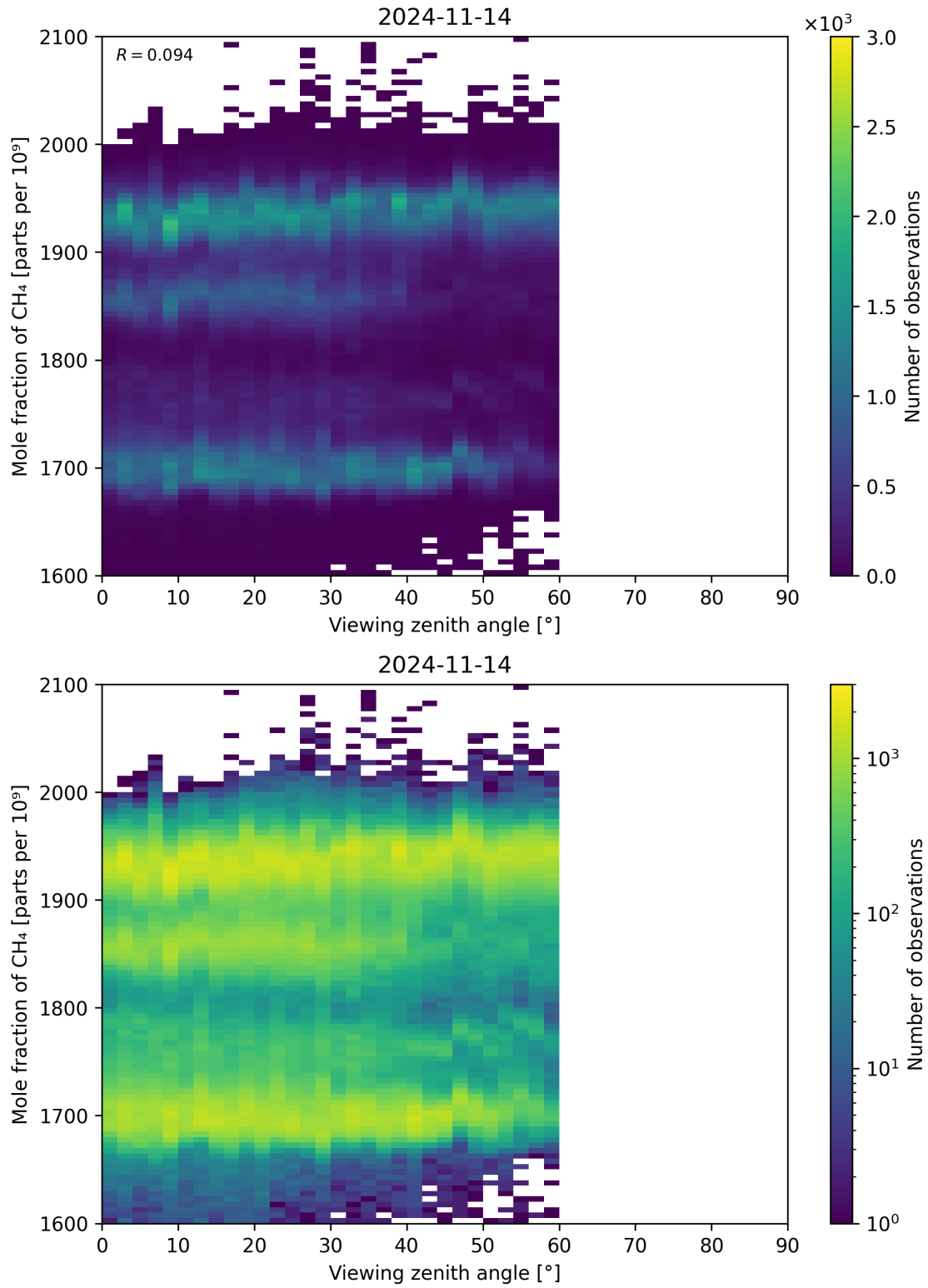
Figure 110: Scatter density plot of “Viewing zenith angle” against “Mole fraction of CH 4 ” for 2024-11-14 to 2024-11-15.
