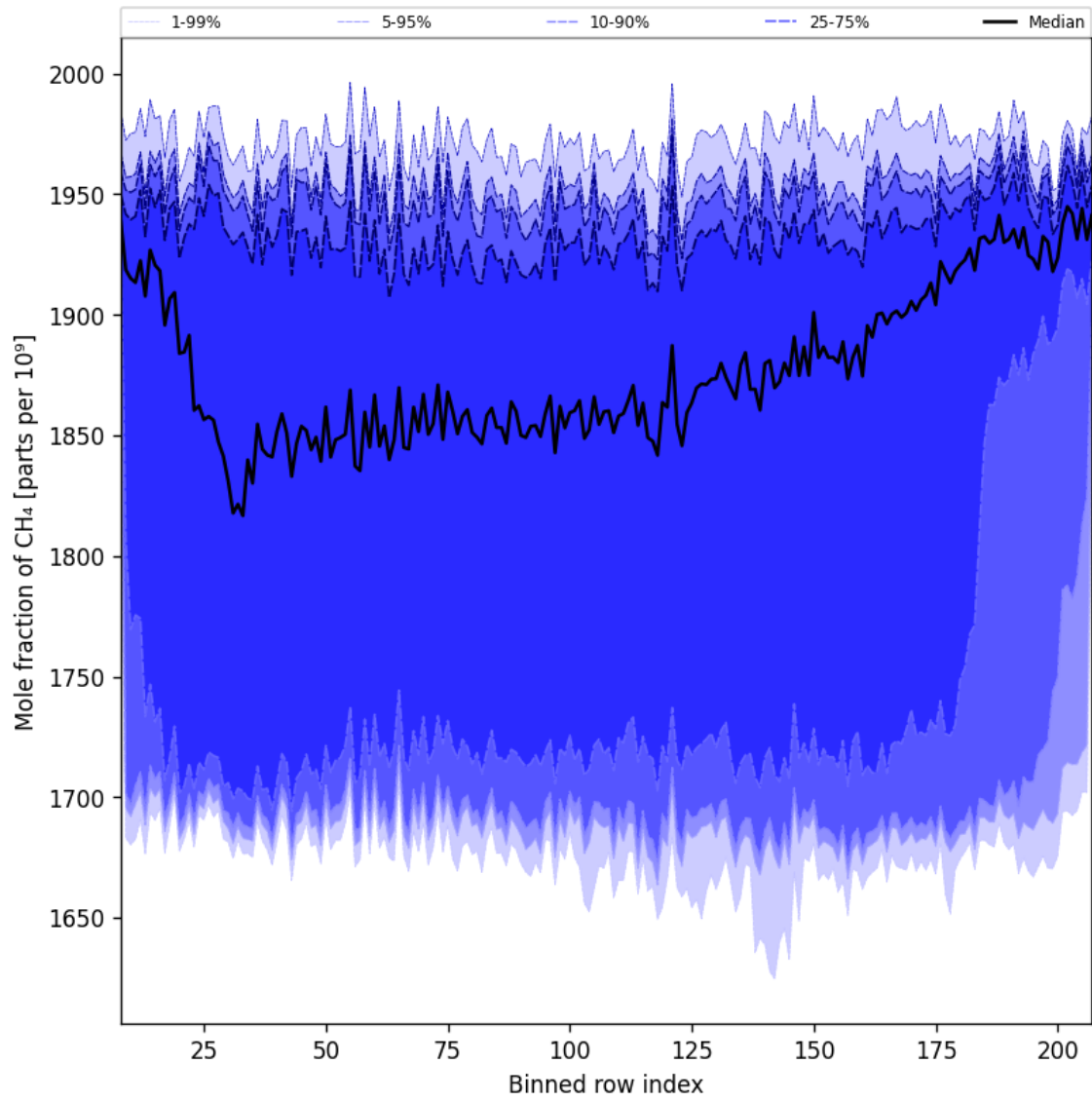
Figure 34: Along track statistics of “Mole fraction of CH 4 ” for 2024-11-14 to 2024-11-15
