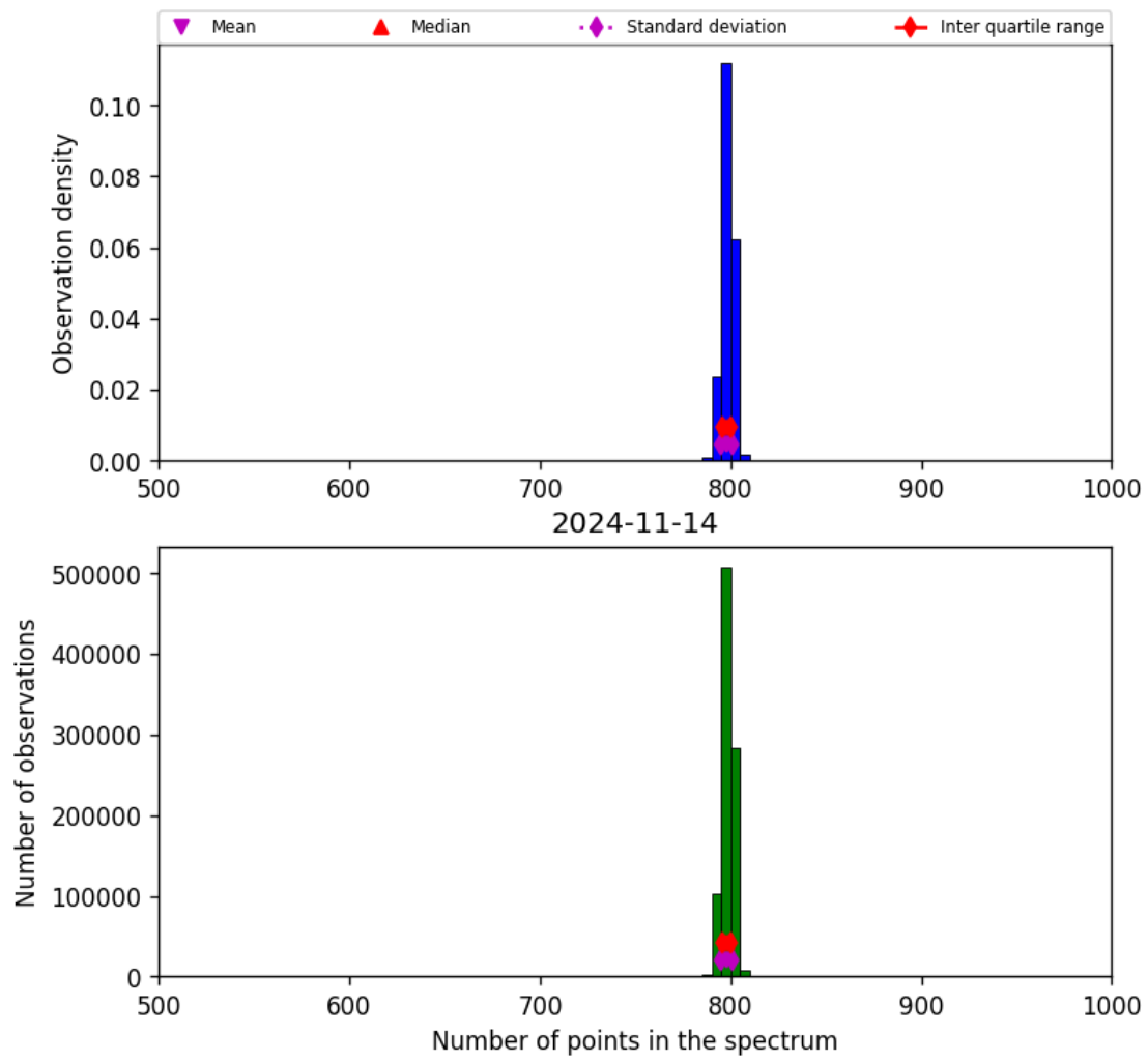
Figure 26: Histogram of “Number of points in the spectrum” for 2024-11-14 to 2024-11-15
