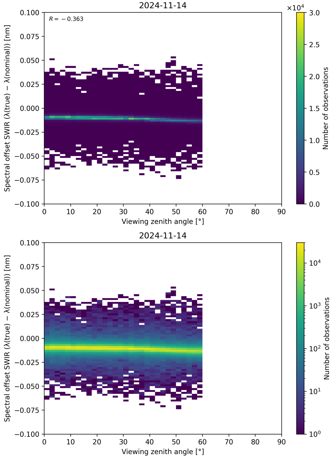
Figure 116: Scatter density plot of “Viewing zenith angle” against “Spectral offset SWIR ( \lambda_{\text{true}} - \lambda_{\text{nominal}} )” for 2024-11-14 to 2024-11-15.
