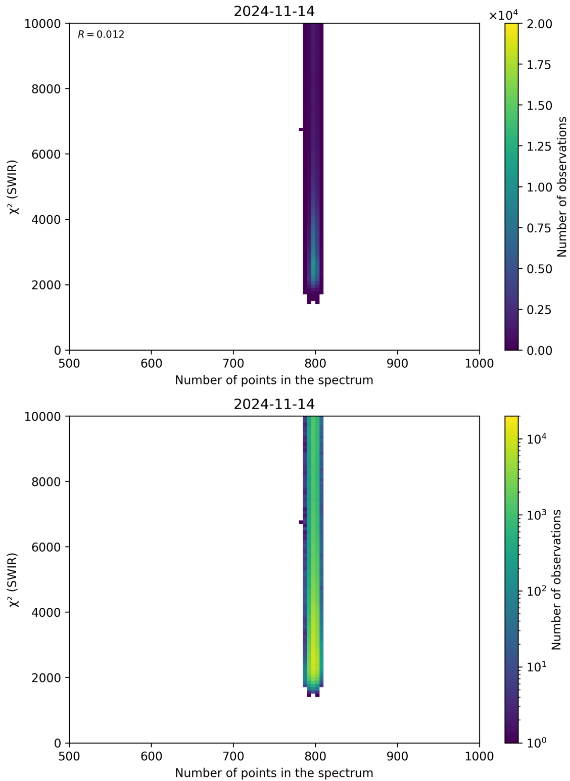
Figure 89: Scatter density plot of “Number of points in the spectrum” against “ \chi^2 (SWIR)” for 2024-11-14 to 2024-11-15.
