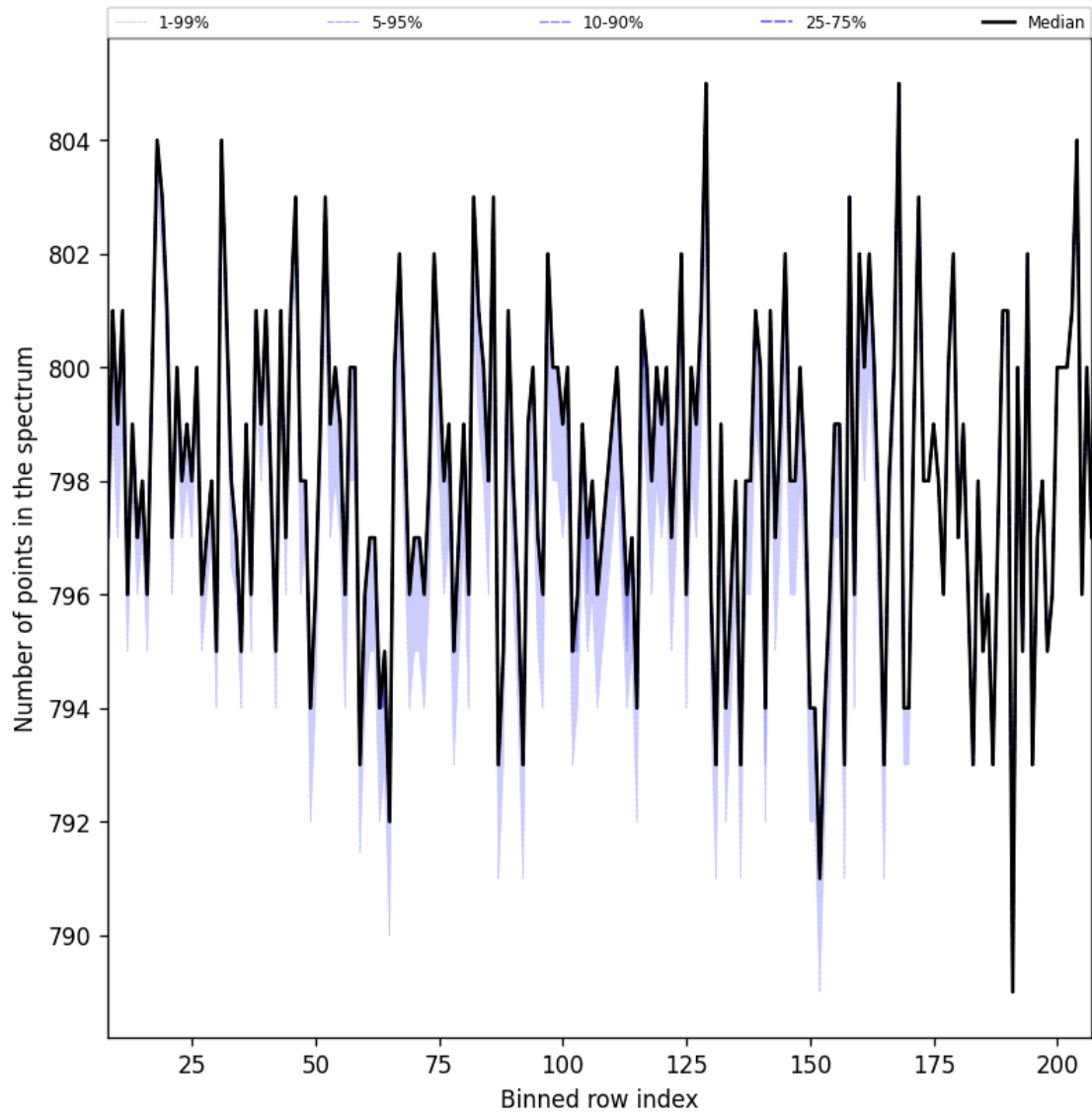
Figure 37: Along track statistics of “Number of points in the spectrum” for 2024-11-14 to 2024-11-15
