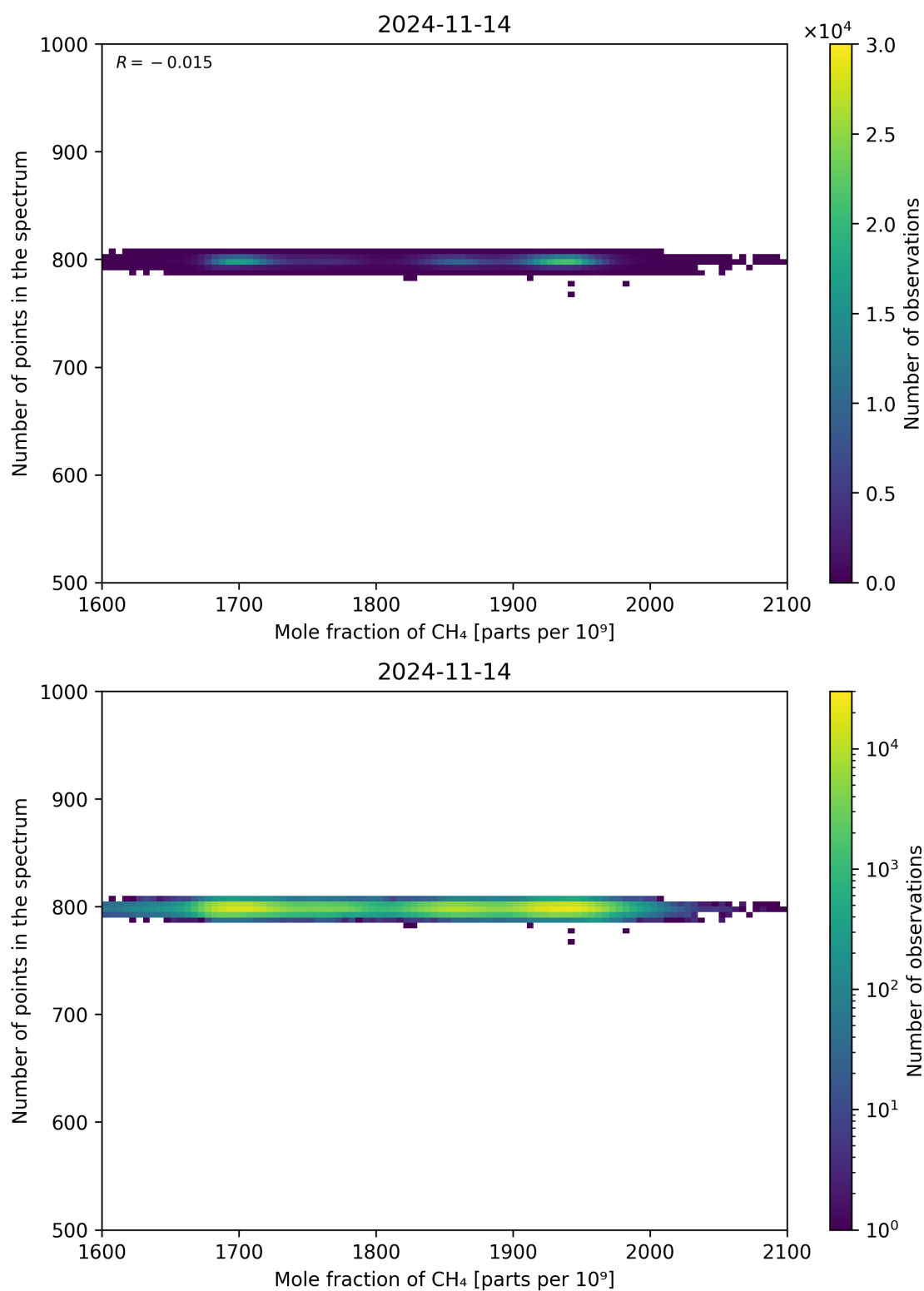
Figure 77: Scatter density plot of “Mole fraction of CH 4 ” against “Number of points in the spectrum” for 2024-11-14 to 2024-11-15.
