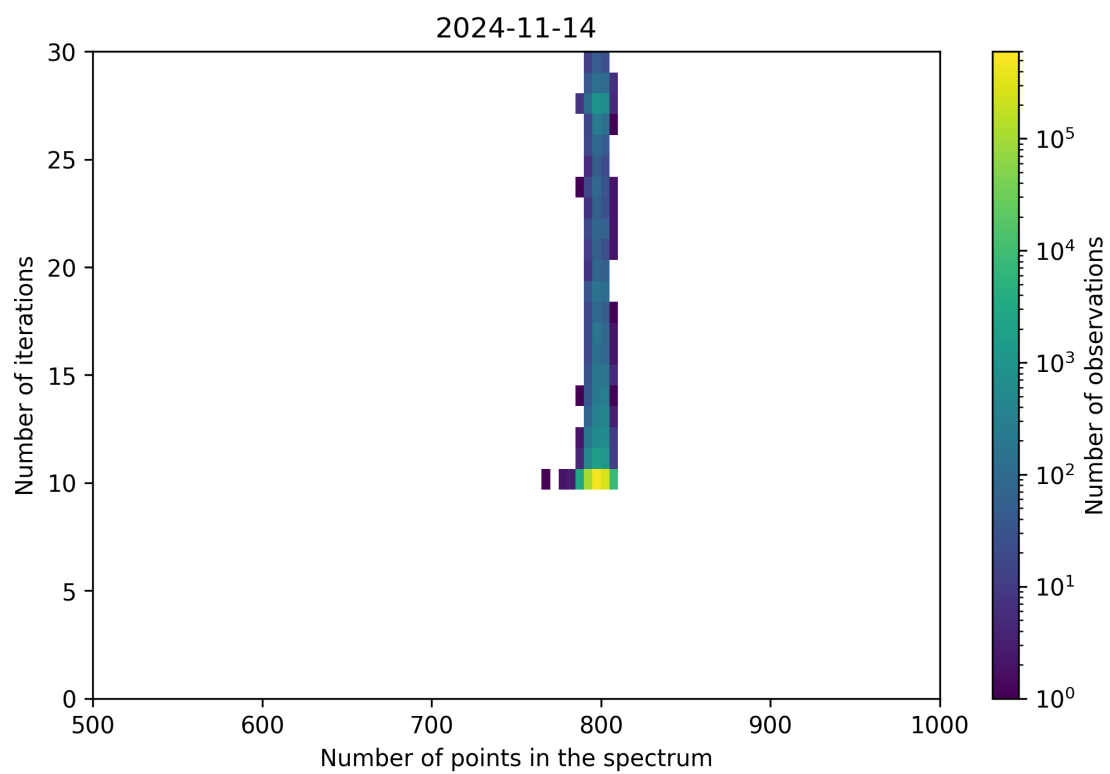
Figure 92: Scatter density plot of “Number of points in the spectrum” against “Number of iterations” for 2024-11-14 to 2024-11-15.
