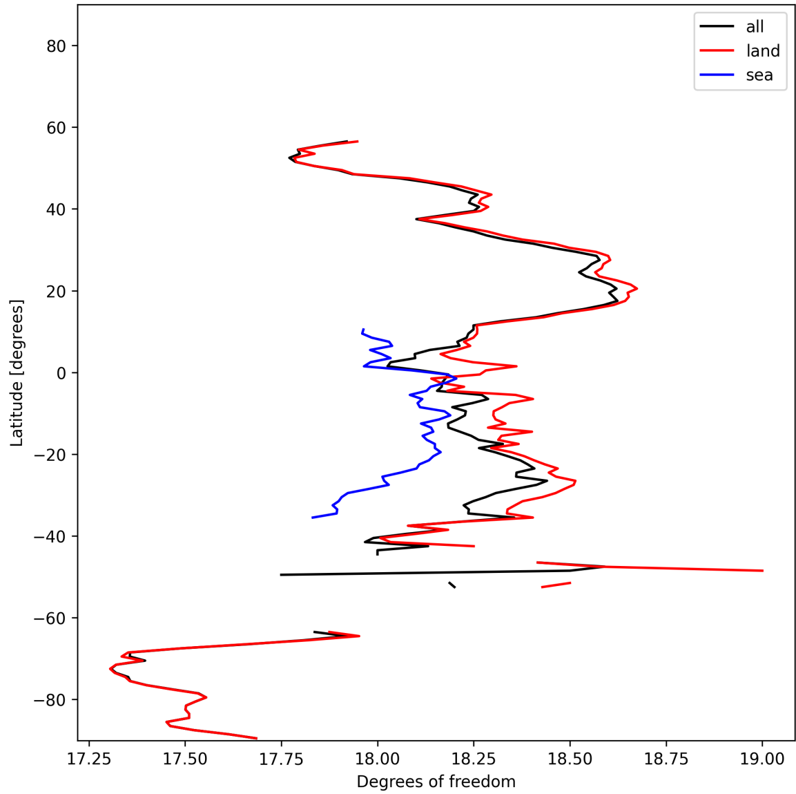
Figure 19: Zonal average of “Degrees of freedom” for 2024-11-14 to 2024-11-15.
