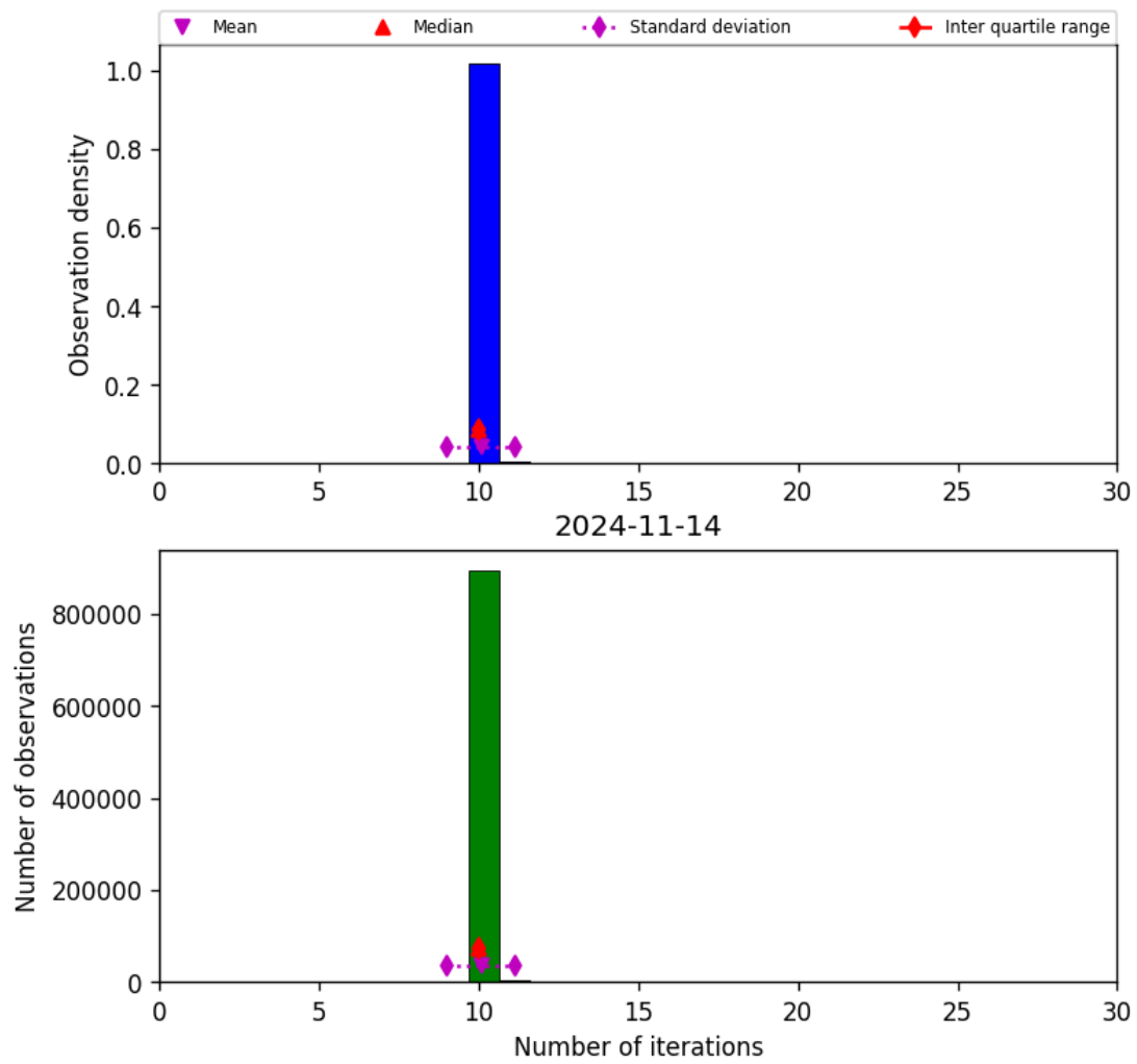
Figure 31: Histogram of “Number of iterations” for 2024-11-14 to 2024-11-15
