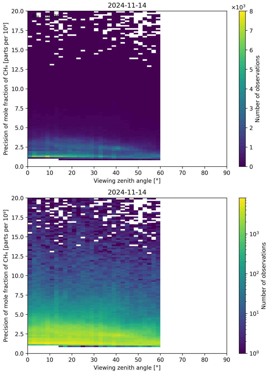
Figure 112: Scatter density plot of “Viewing zenith angle” against “Precision of mole fraction of CH 4 ” for 2024-11-14 to 2024-11-15.
