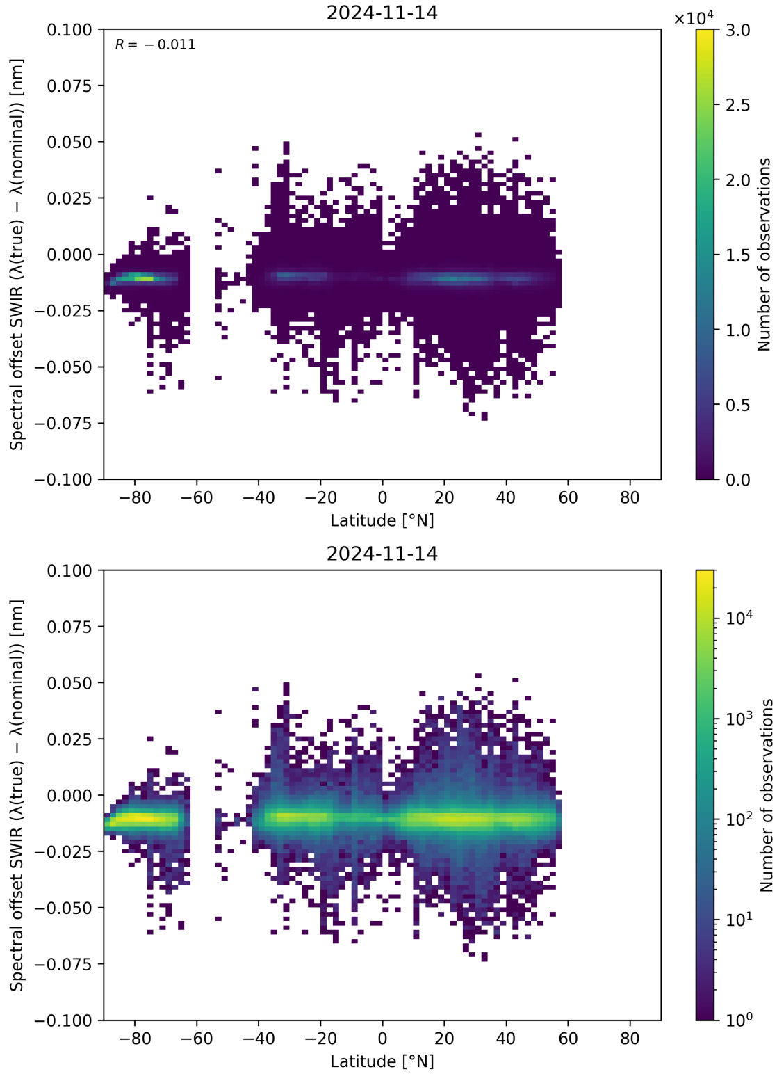
Figure 62: Scatter density plot of “Latitude” against “Spectral offset SWIR ( \lambda_{\text{true}} - \lambda_{\text{nominal}} )” for 2024-11-14 to 2024-11-15.
