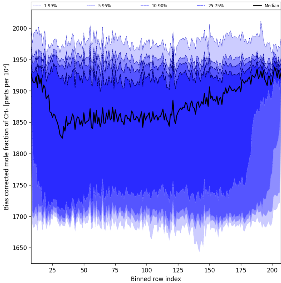
Figure 36: Along track statistics of “Bias corrected mole fraction of CH 4 ” for 2024-11-14 to 2024-11-15
