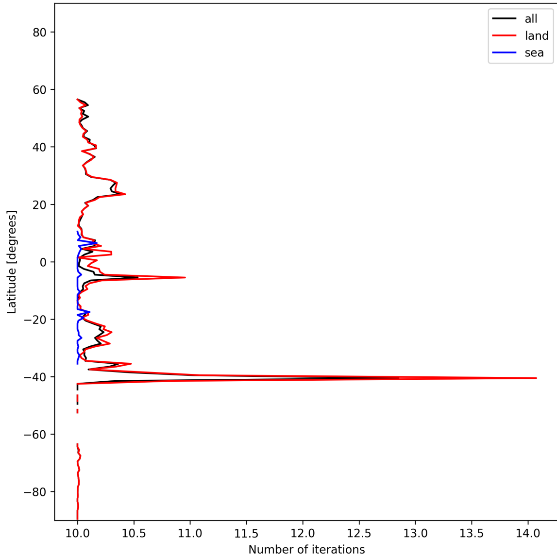
Figure 20: Zonal average of “Number of iterations” for 2024-11-14 to 2024-11-15.
