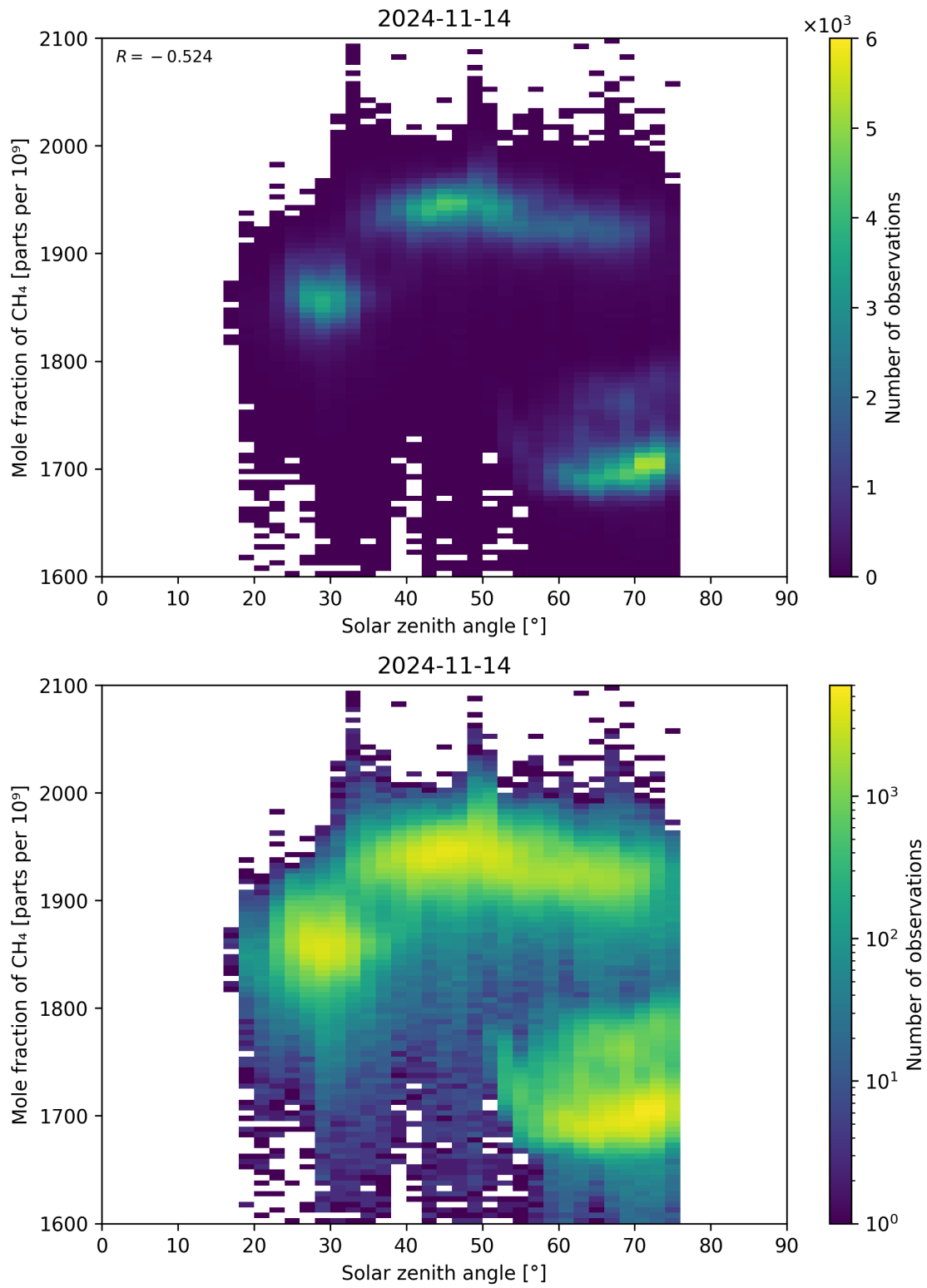
Figure 99: Scatter density plot of “Solar zenith angle” against “Mole fraction of CH 4 ” for 2024-11-14 to 2024-11-15.
