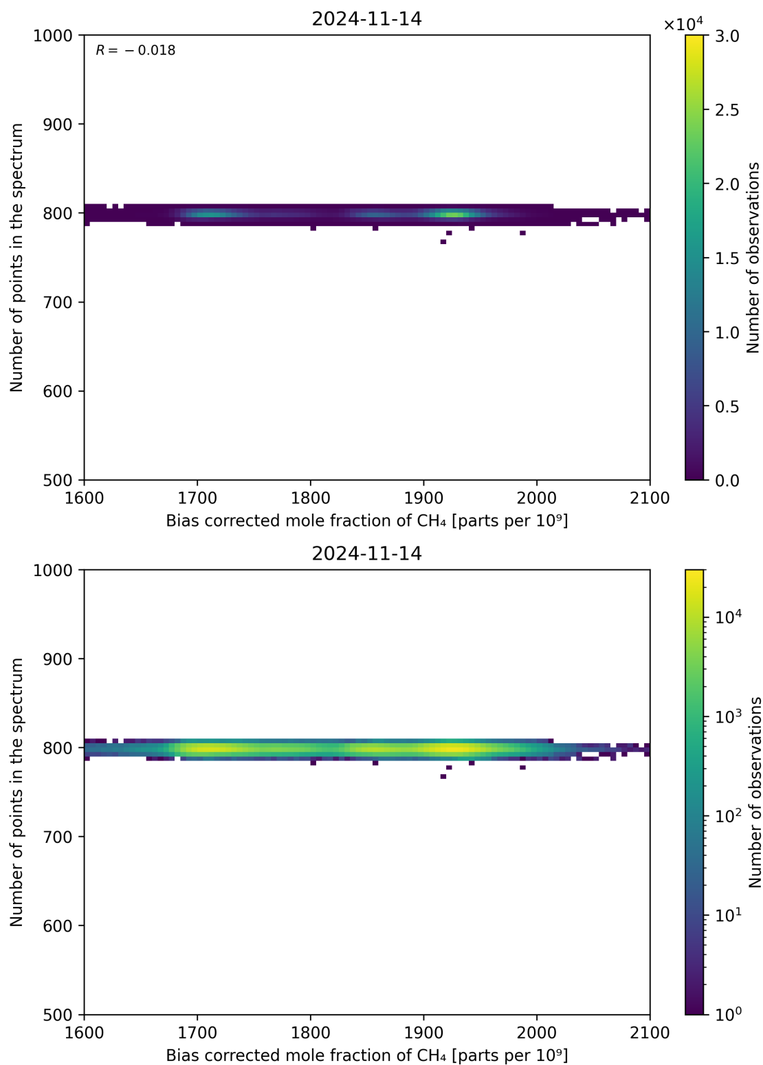
Figure 68: Scatter density plot of “Bias corrected mole fraction of CH 4 ” against “Number of points in the spectrum” for 2024-11-14 to 2024-11-15.
