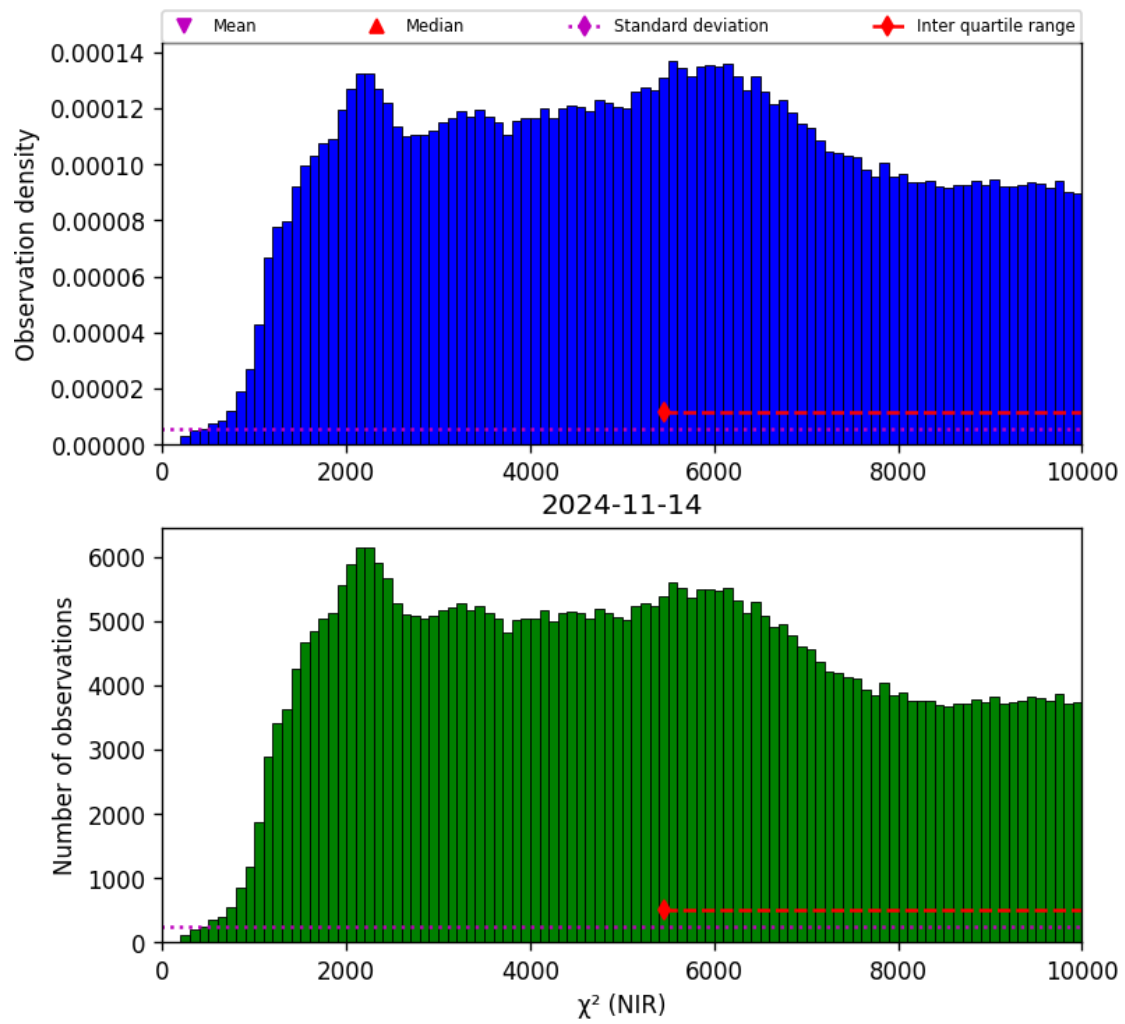
Figure 29: Histogram of “ \chi^2 (NIR)” for 2024-11-14 to 2024-11-15
