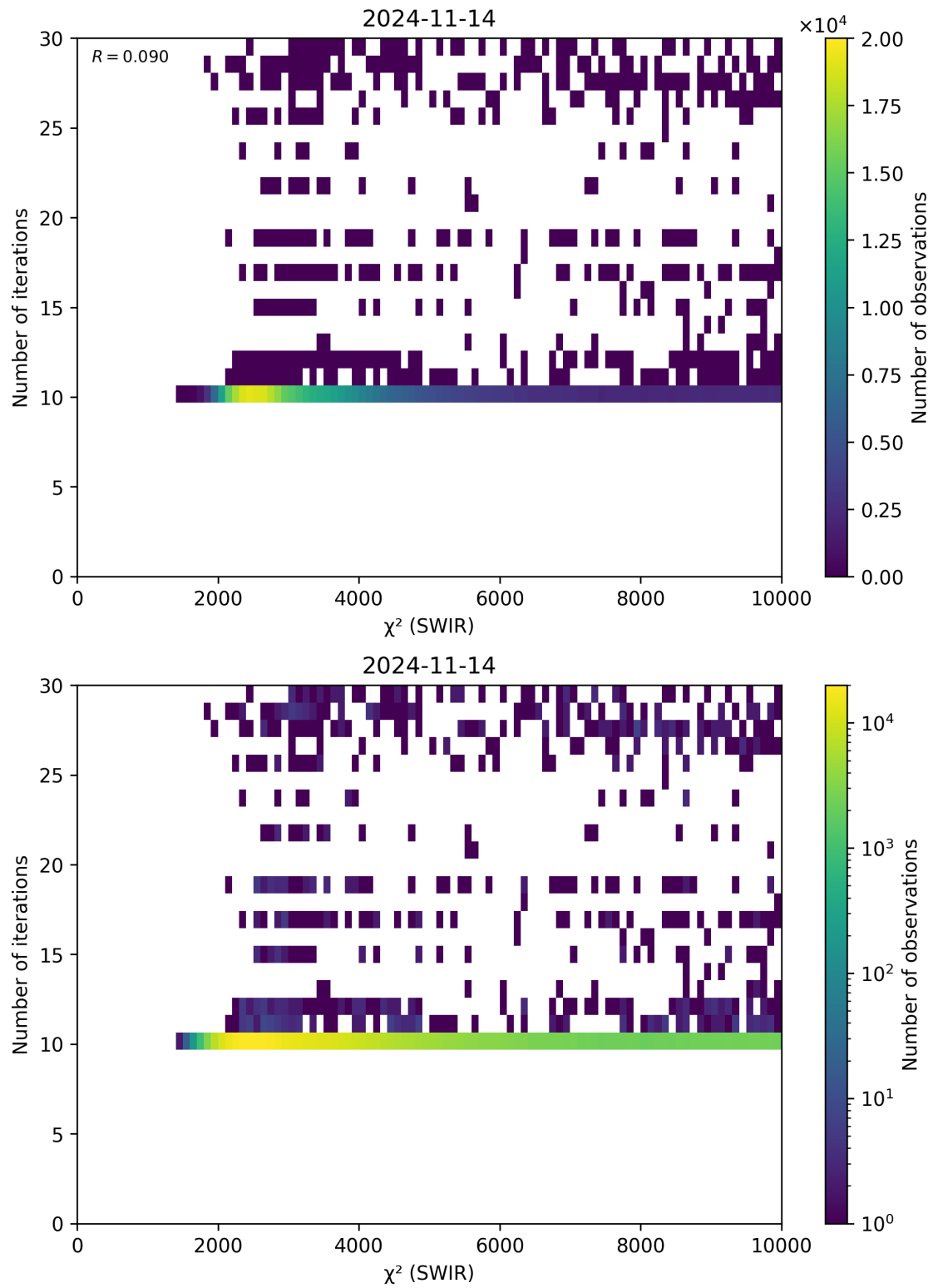
Figure 50: Scatter density plot of “ \chi^2 (SWIR)” against “Number of iterations” for 2024-11-14 to 2024-11-15.
