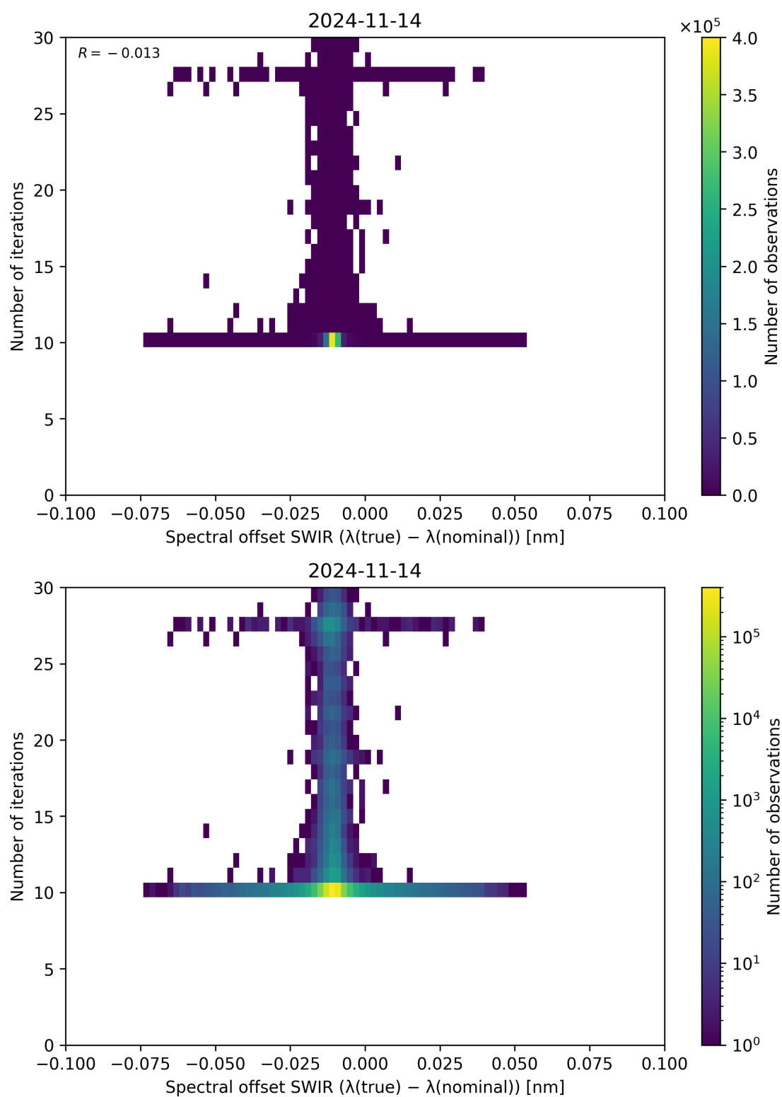
Figure 121: Scatter density plot of “Spectral offset SWIR ( \lambda_{\text{true}} - \lambda_{\text{nominal}} )” against “Number of iterations” for 2024-11-14 to 2024-11-15.
