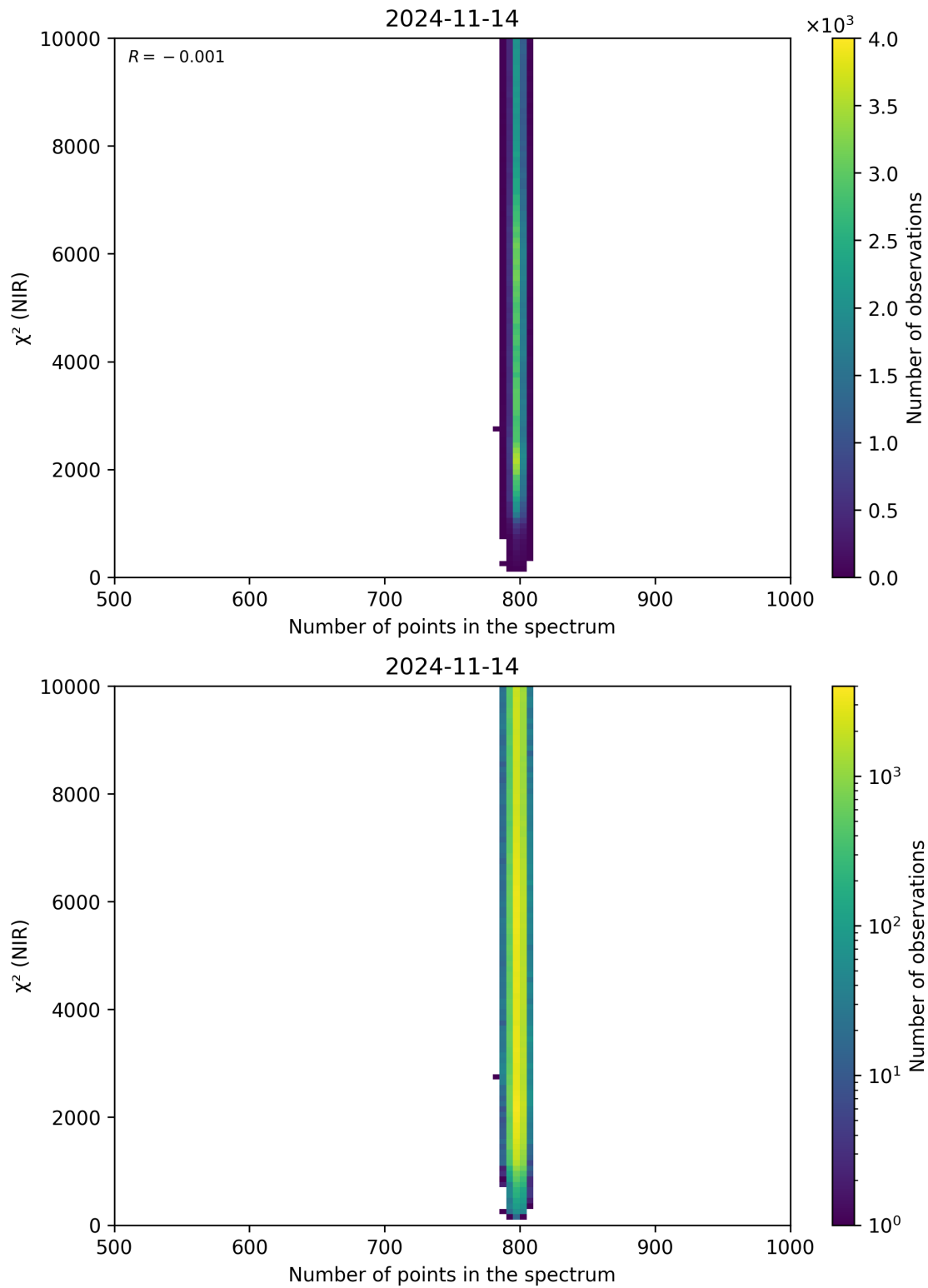
Figure 88: Scatter density plot of “Number of points in the spectrum” against “ \chi^2 (NIR)” for 2024-11-14 to 2024-11-15.
