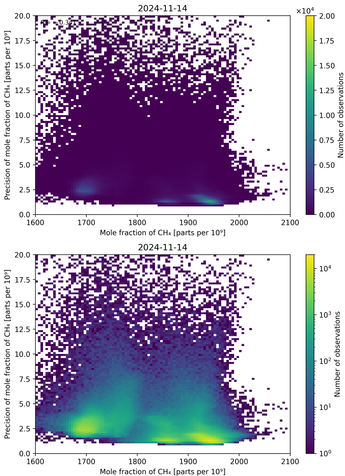
Figure 75: Scatter density plot of “Mole fraction of CH 4 ” against “Precision of mole fraction of CH 4 ” for 2024-11-14 to 2024-11-15.
