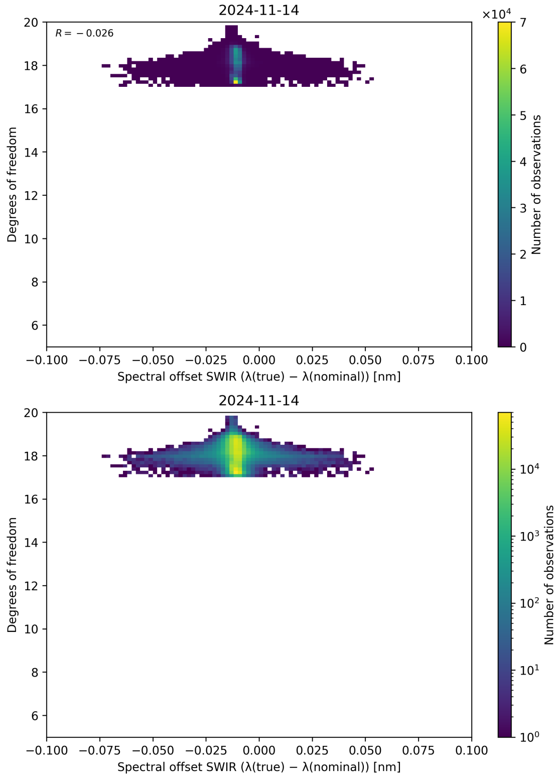
Figure 119: Scatter density plot of “Spectral offset SWIR ( \lambda_{\text{true}} - \lambda_{\text{nominal}} )” against “Degrees of freedom” for 2024-11-14 to 2024-11-15.
