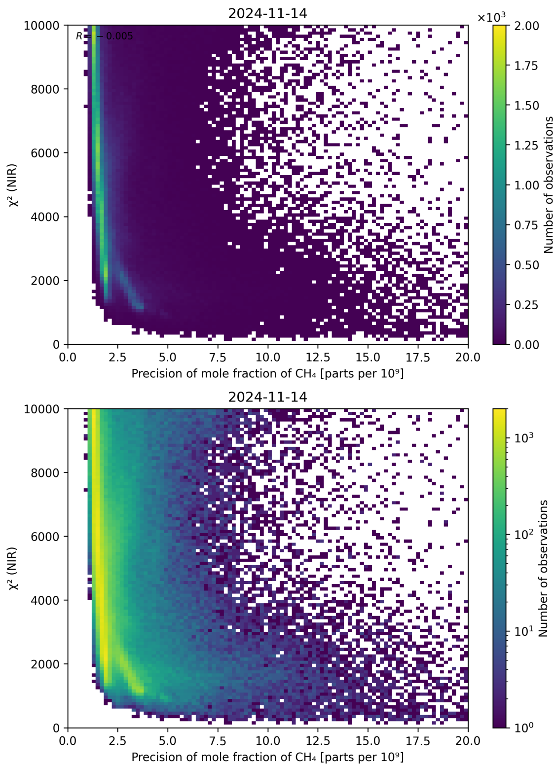
Figure 78: Scatter density plot of “Precision of mole fraction of CH 4 ” against “ \chi^2 (NIR)” for 2024-11-14 to 2024-11-15.
