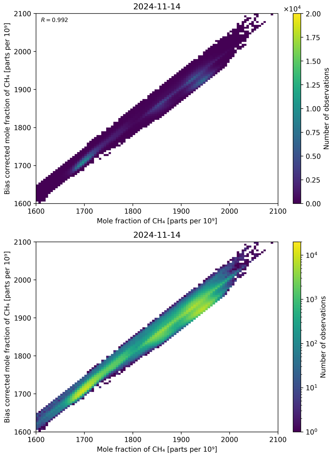
Figure 74: Scatter density plot of “Mole fraction of CH 4 ” against “Bias corrected mole fraction of CH 4 ” for 2024-11-14 to 2024-11-15.
