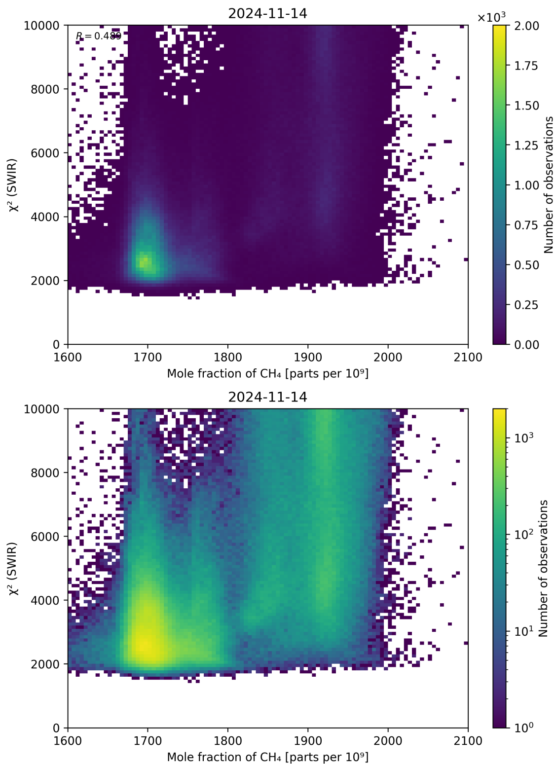
Figure 71: Scatter density plot of “Mole fraction of \text{CH}_4 ” against “ \chi^2 (SWIR)” for 2024-11-14 to 2024-11-15.
