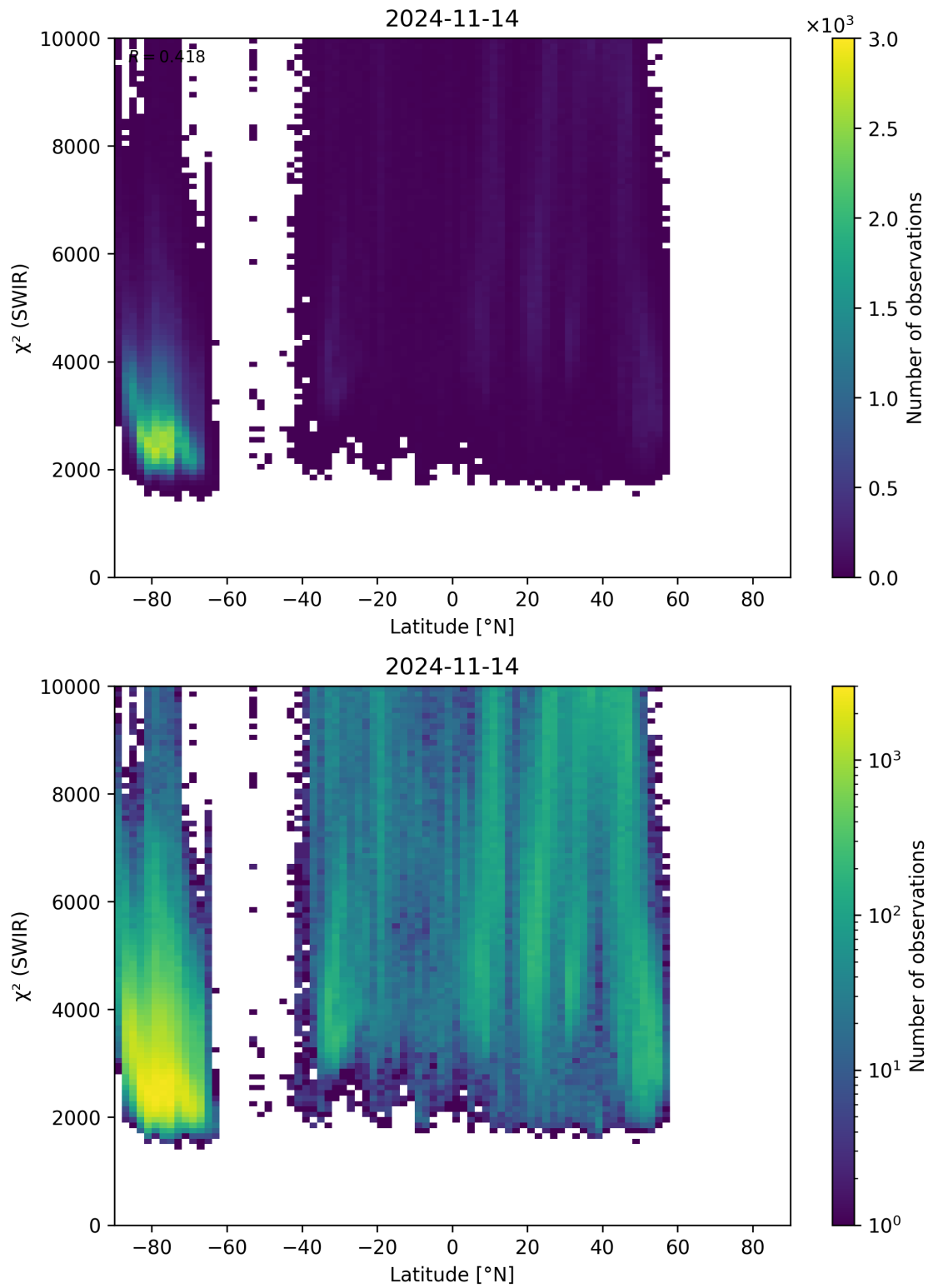
Figure 54: Scatter density plot of “Latitude” against “ \chi^2 (SWIR)” for 2024-11-14 to 2024-11-15.
