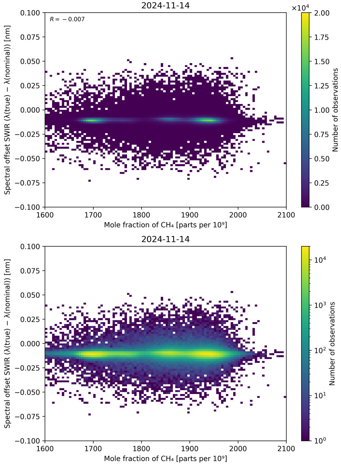
Figure 86: Scatter density plot of “Mole fraction of CH 4 ” against “Spectral offset SWIR ( \lambda_{\text{true}} - \lambda_{\text{nominal}} )” for 2024-11-14 to 2024-11-15.
