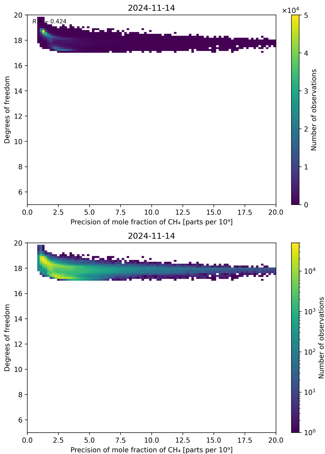
Figure 80: Scatter density plot of “Precision of mole fraction of CH 4 ” against “Degrees of freedom” for 2024-11-14 to 2024-11-15.
