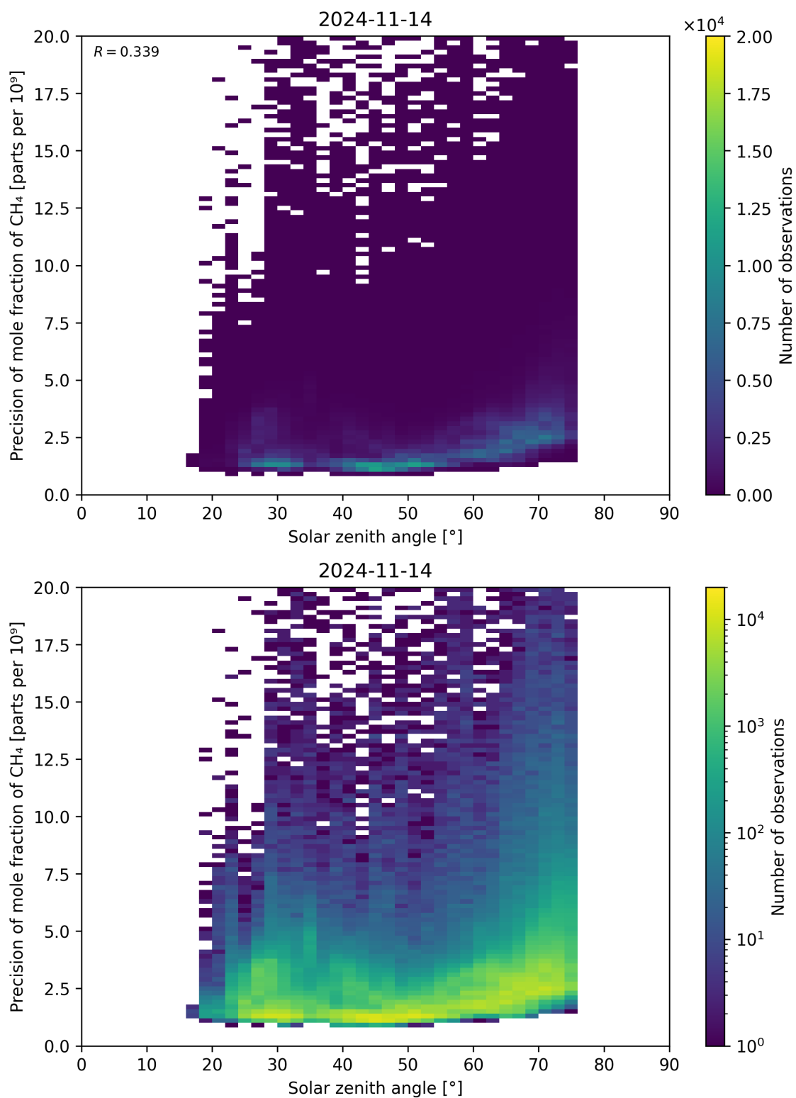
Figure 101: Scatter density plot of “Solar zenith angle” against “Precision of mole fraction of CH 4 ” for 2024-11-14 to 2024-11-15.
