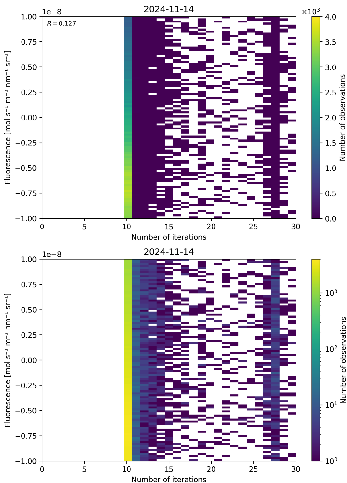
Figure 87: Scatter density plot of “Number of iterations” against “Fluorescence” for 2024-11-14 to 2024-11-15.
