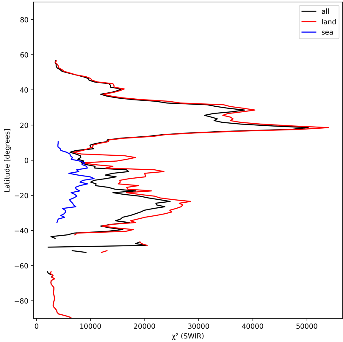
Figure 17: Zonal average of “ \chi^2 (SWIR)” for 2024-11-14 to 2024-11-15.
