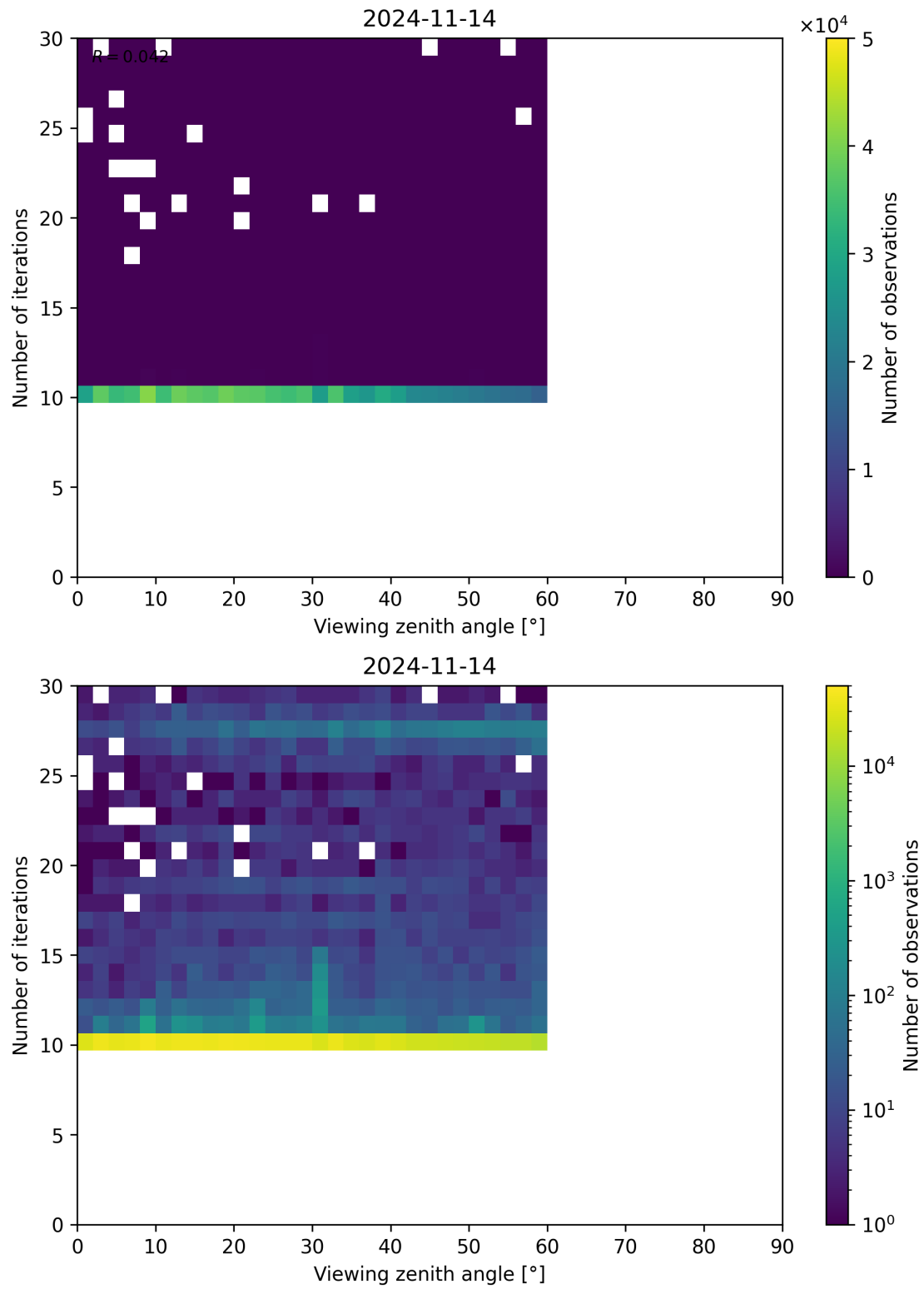
Figure 113: Scatter density plot of “Viewing zenith angle” against “Number of iterations” for 2024-11-14 to 2024-11-15.
