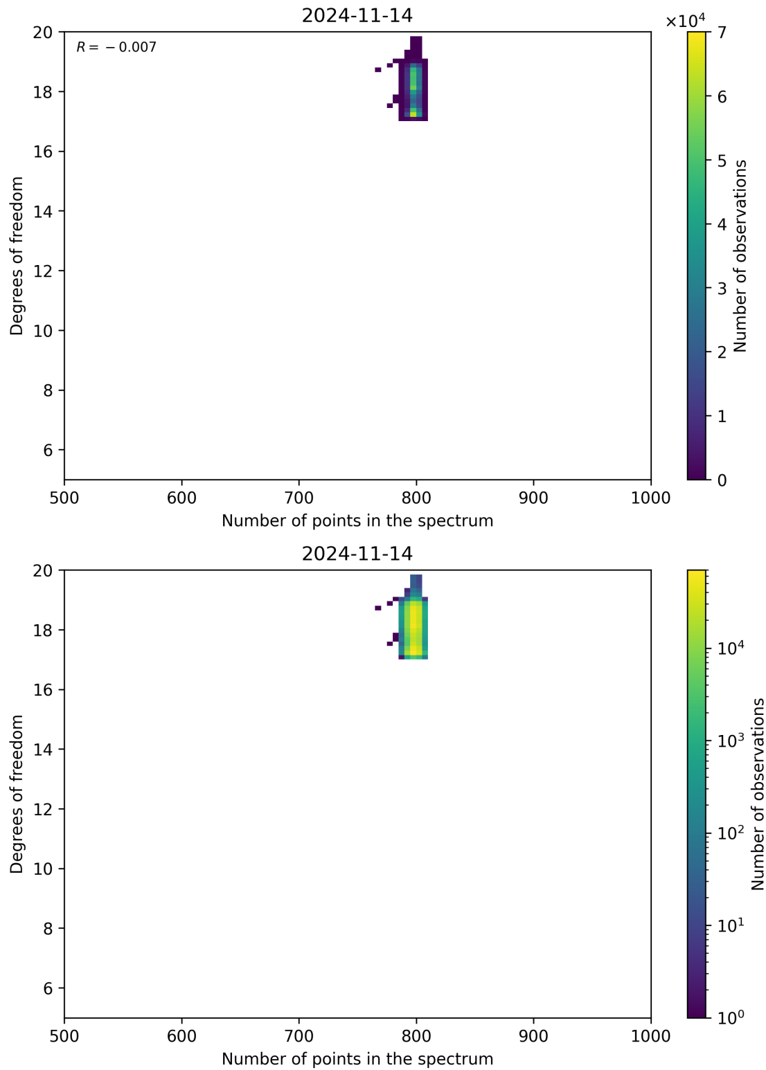
Figure 90: Scatter density plot of “Number of points in the spectrum” against “Degrees of freedom” for 2024-11-14 to 2024-11-15.
