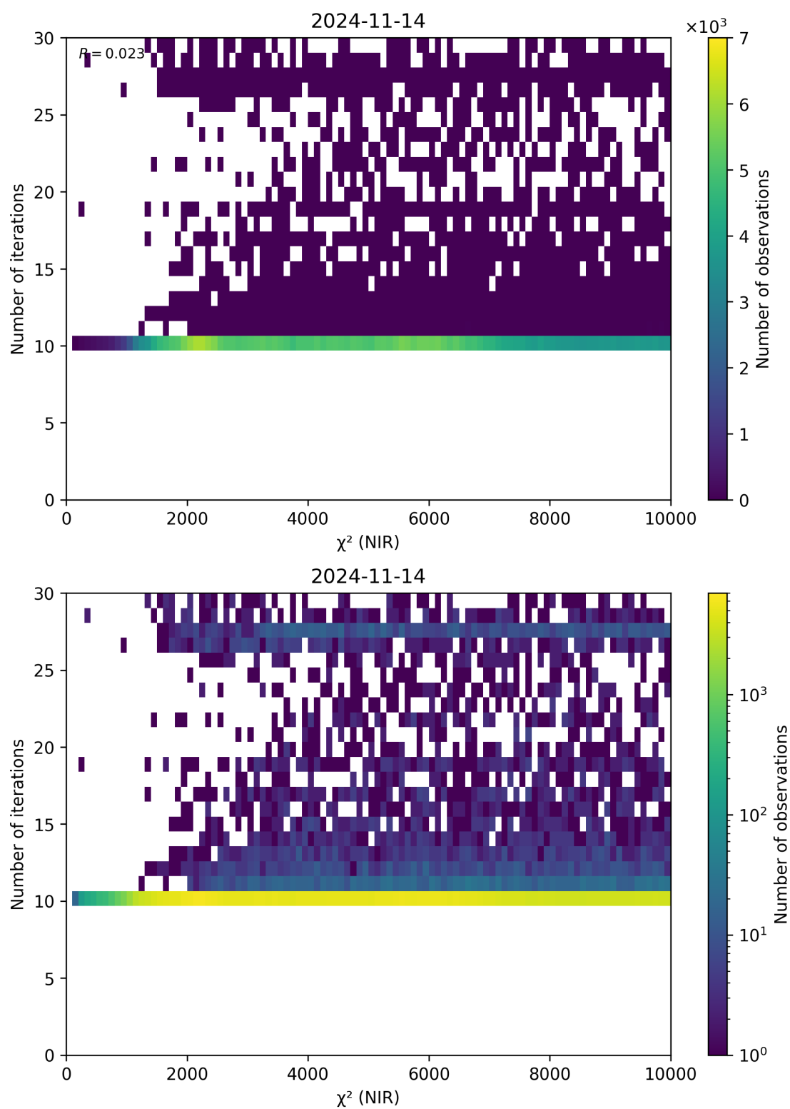
Figure 46: Scatter density plot of “ \chi^2 (NIR)” against “Number of iterations” for 2024-11-14 to 2024-11-15.
