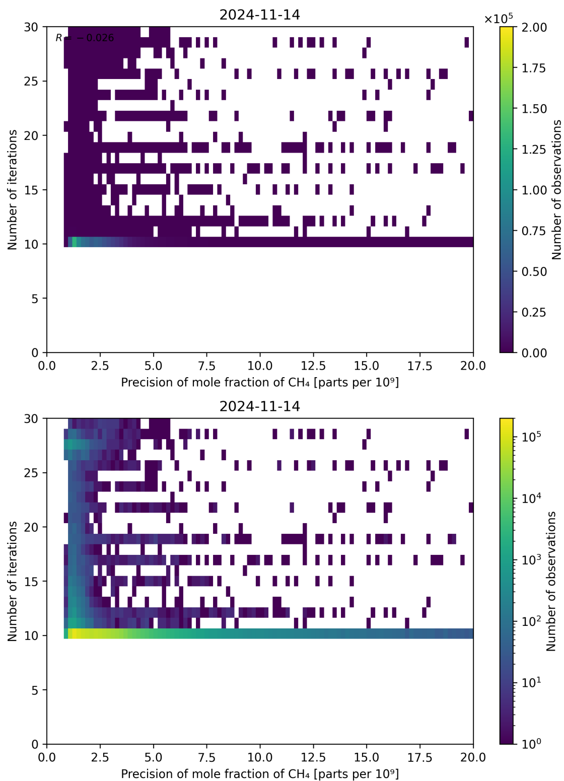
Figure 83: Scatter density plot of “Precision of mole fraction of CH 4 ” against “Number of iterations” for 2024-11-14 to 2024-11-15.
