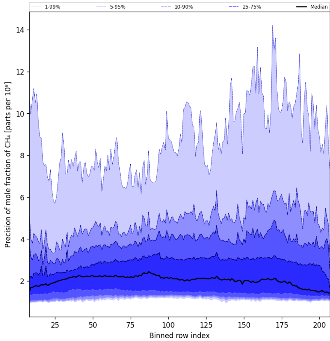
Figure 35: Along track statistics of “Precision of mole fraction of CH 4 ” for 2024-11-14 to 2024-11-15
