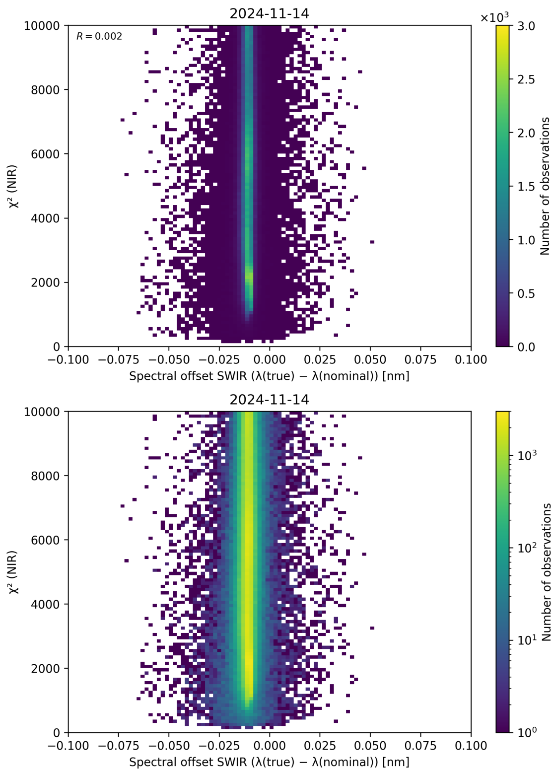
Figure 117: Scatter density plot of “Spectral offset SWIR ( \lambda_{\text{true}} - \lambda_{\text{nominal}} )” against “ \chi^2 (NIR)” for 2024-11-14 to 2024-11-15.
