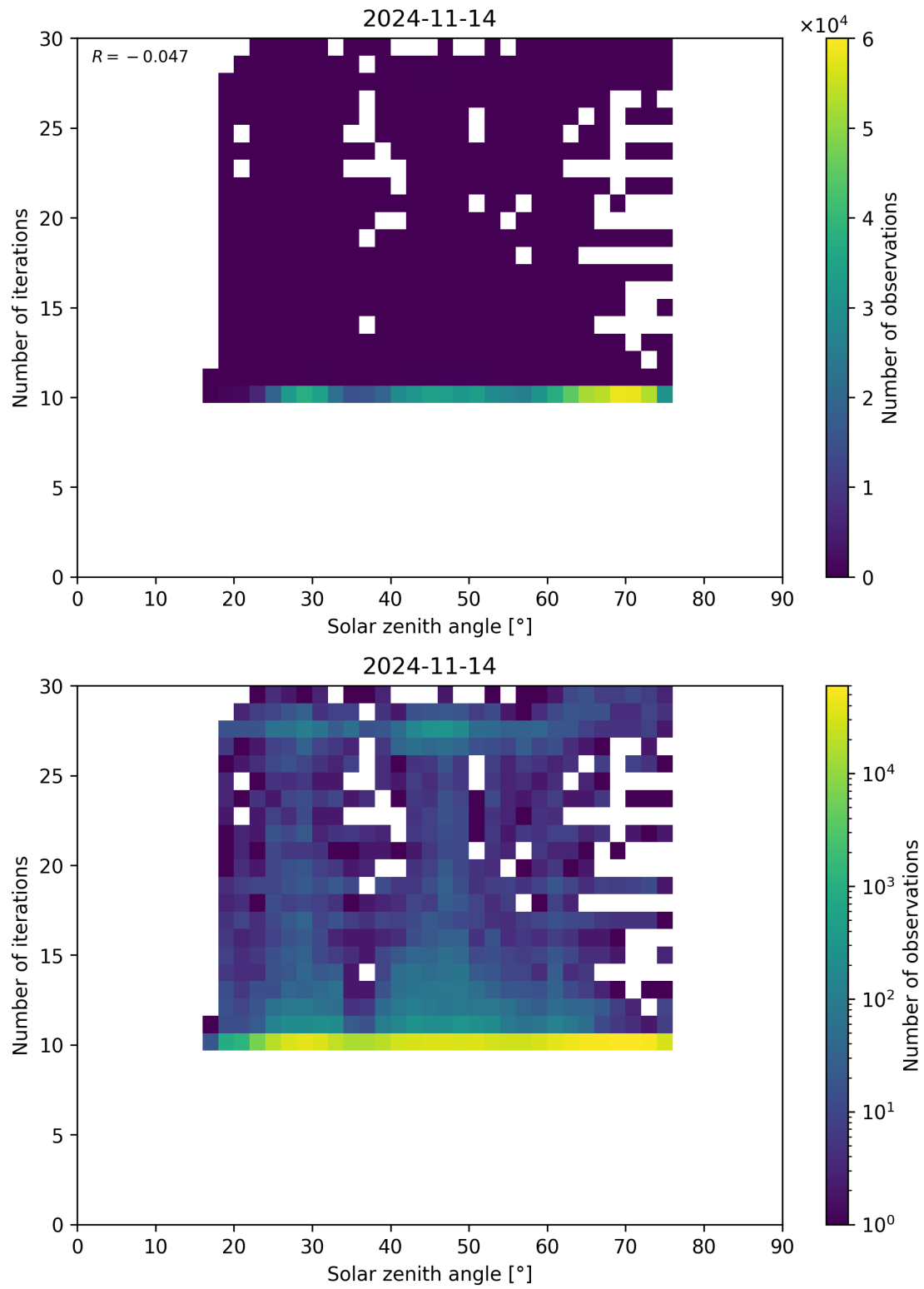
Figure 102: Scatter density plot of “Solar zenith angle” against “Number of iterations” for 2024-11-14 to 2024-11-15.
