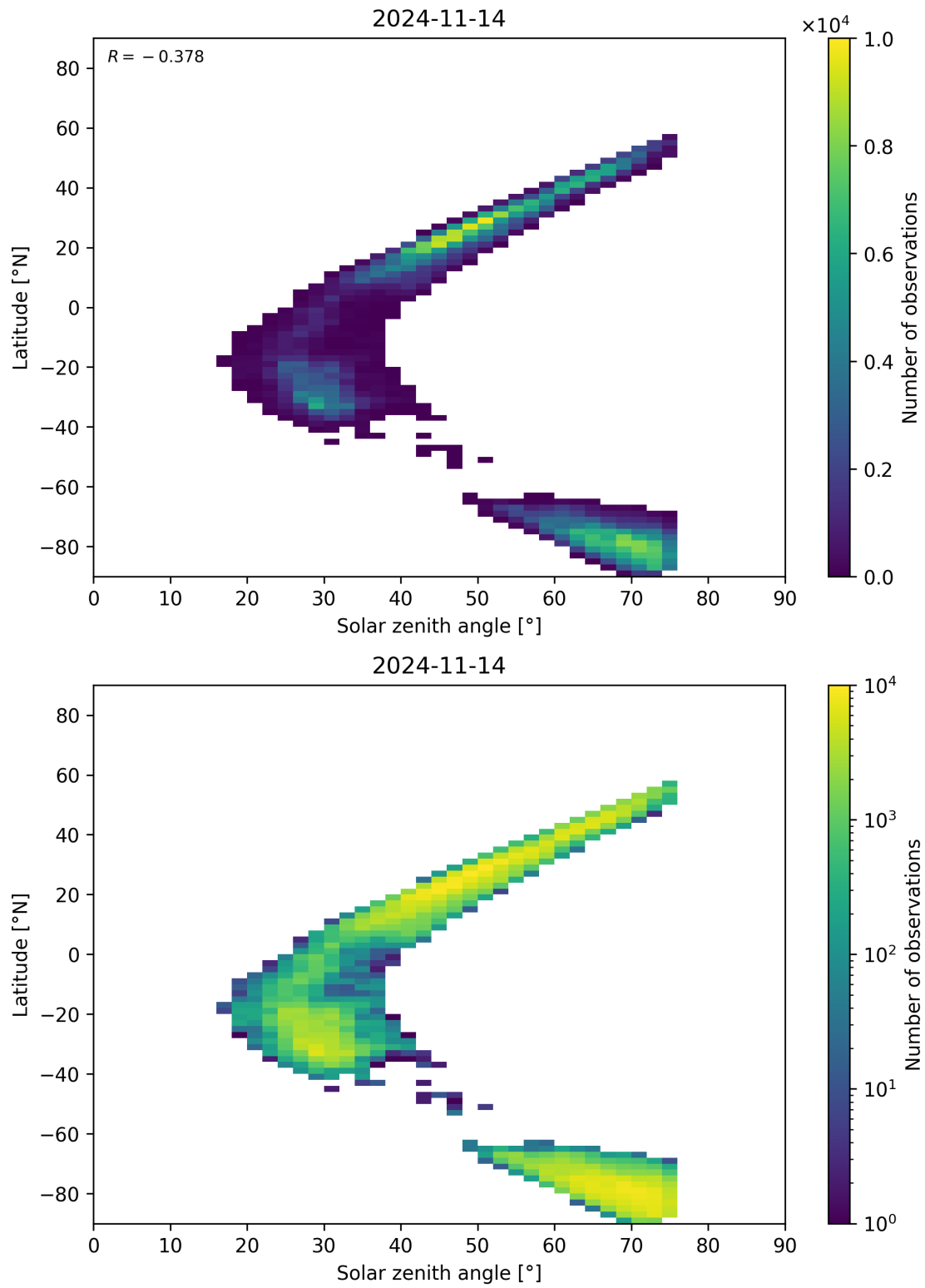
Figure 98: Scatter density plot of “Solar zenith angle” against “Latitude” for 2024-11-14 to 2024-11-15.
