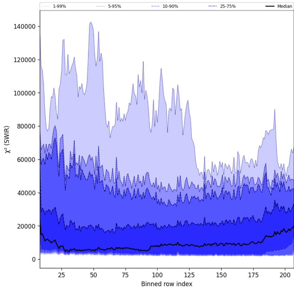
Figure 39: Along track statistics of “ \chi^2 (SWIR)” for 2024-11-14 to 2024-11-15
