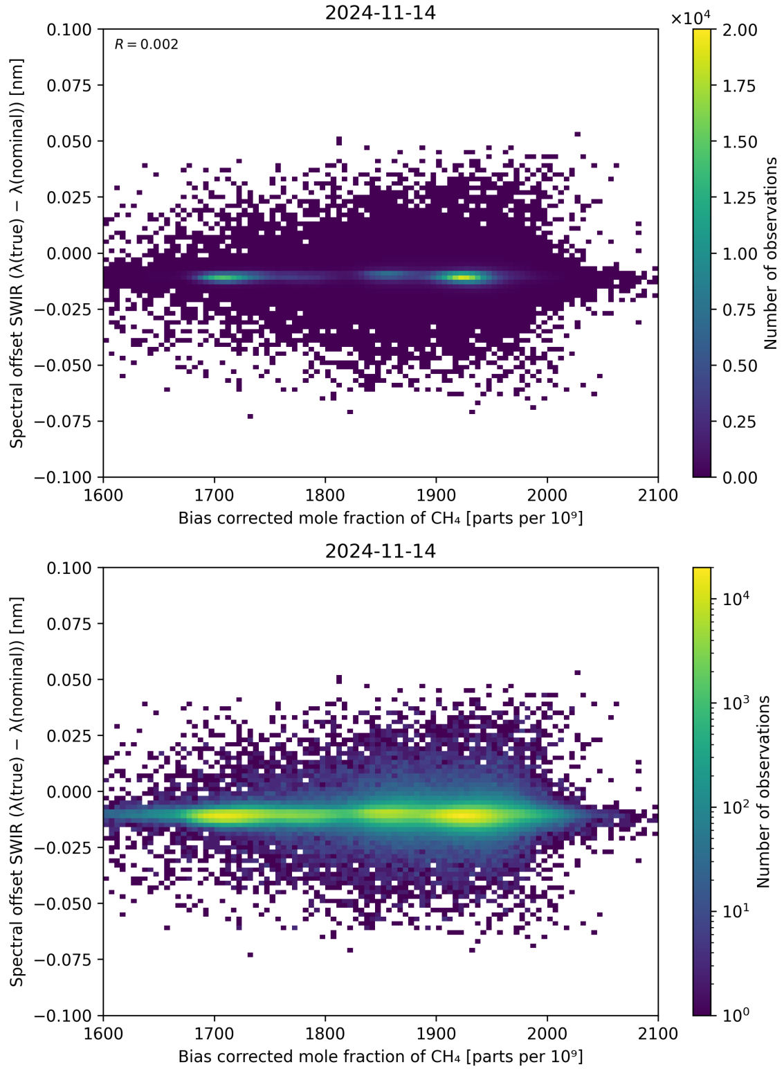
Figure 69: Scatter density plot of “Bias corrected mole fraction of CH 4 ” against “Spectral offset SWIR ( \lambda_{\text{true}} - \lambda_{\text{nominal}} )” for 2024-11-14 to 2024-11-15.
