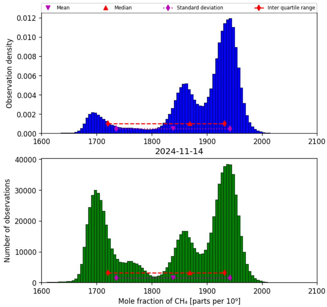
Figure 23: Histogram of “Mole fraction of CH 4 ” for 2024-11-14 to 2024-11-15
