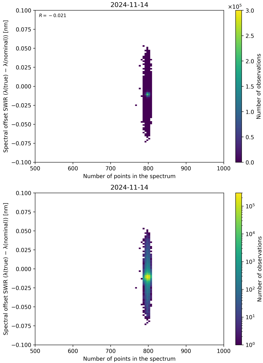
Figure 93: Scatter density plot of “Number of points in the spectrum” against “Spectral offset SWIR ( \lambda_{\text{true}} - \lambda_{\text{nominal}} )” for 2024-11-14 to 2024-11-15.
