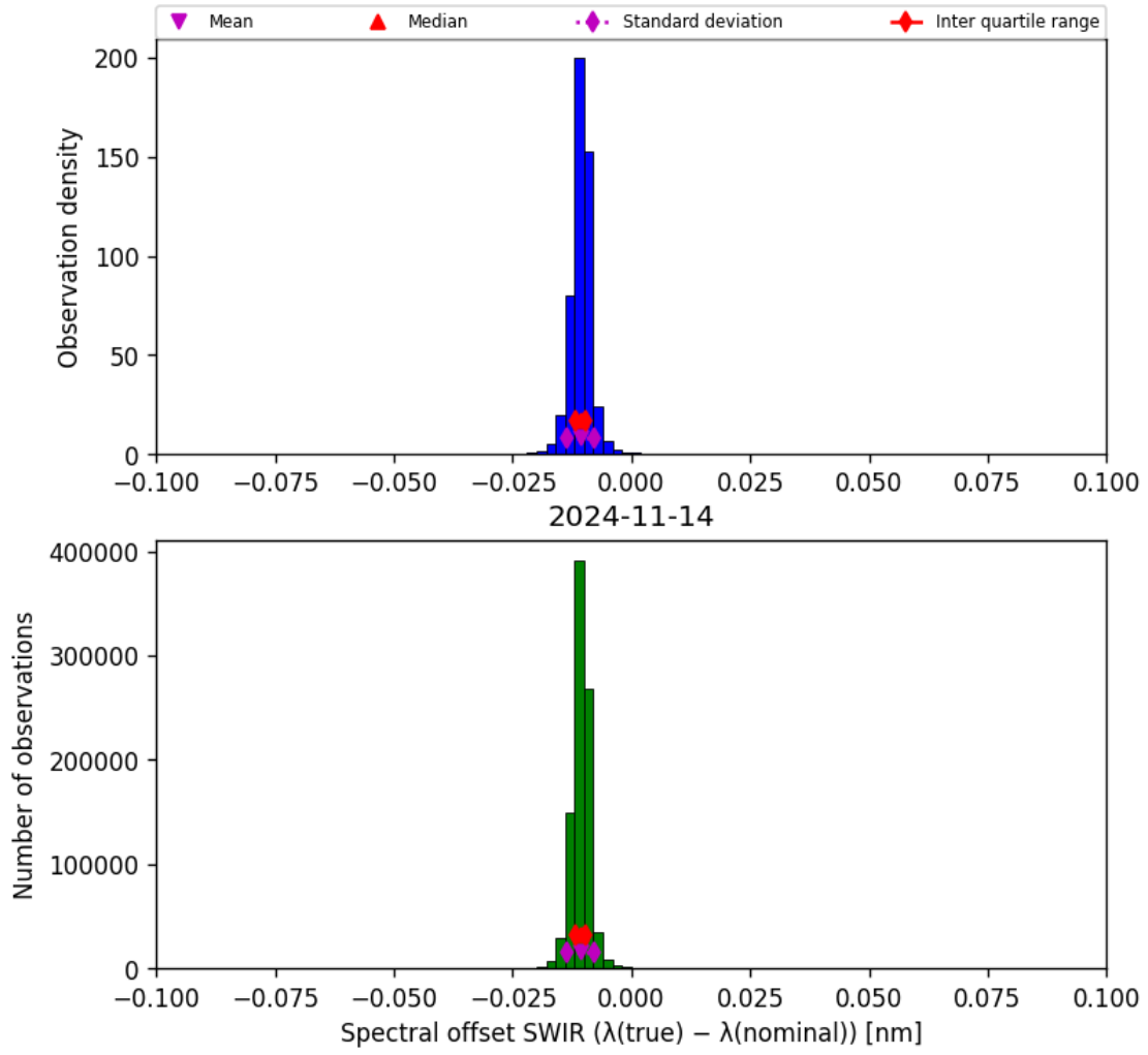
Figure 27: Histogram of “Spectral offset SWIR ( \lambda_{\text{true}} - \lambda_{\text{nominal}} )” for 2024-11-14 to 2024-11-15
