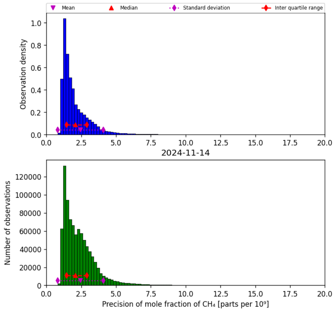
Figure 24: Histogram of “Precision of mole fraction of CH 4 ” for 2024-11-14 to 2024-11-15
