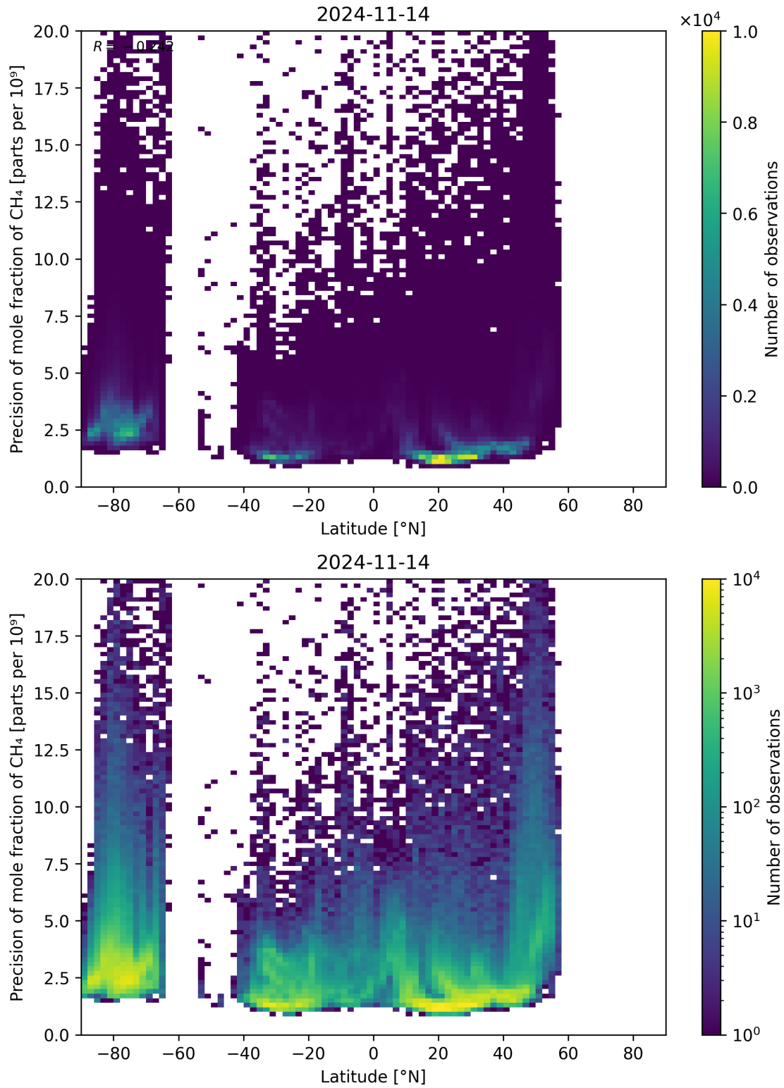
Figure 59: Scatter density plot of “Latitude” against “Precision of mole fraction of CH 4 ” for 2024-11-14 to 2024-11-15.
