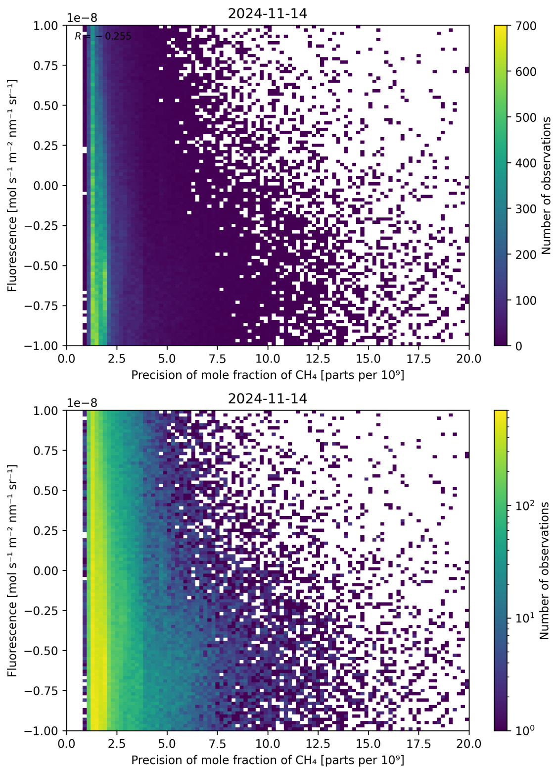
Figure 81: Scatter density plot of “Precision of mole fraction of CH 4 ” against “Fluorescence” for 2024-11-14 to 2024-11-15.
