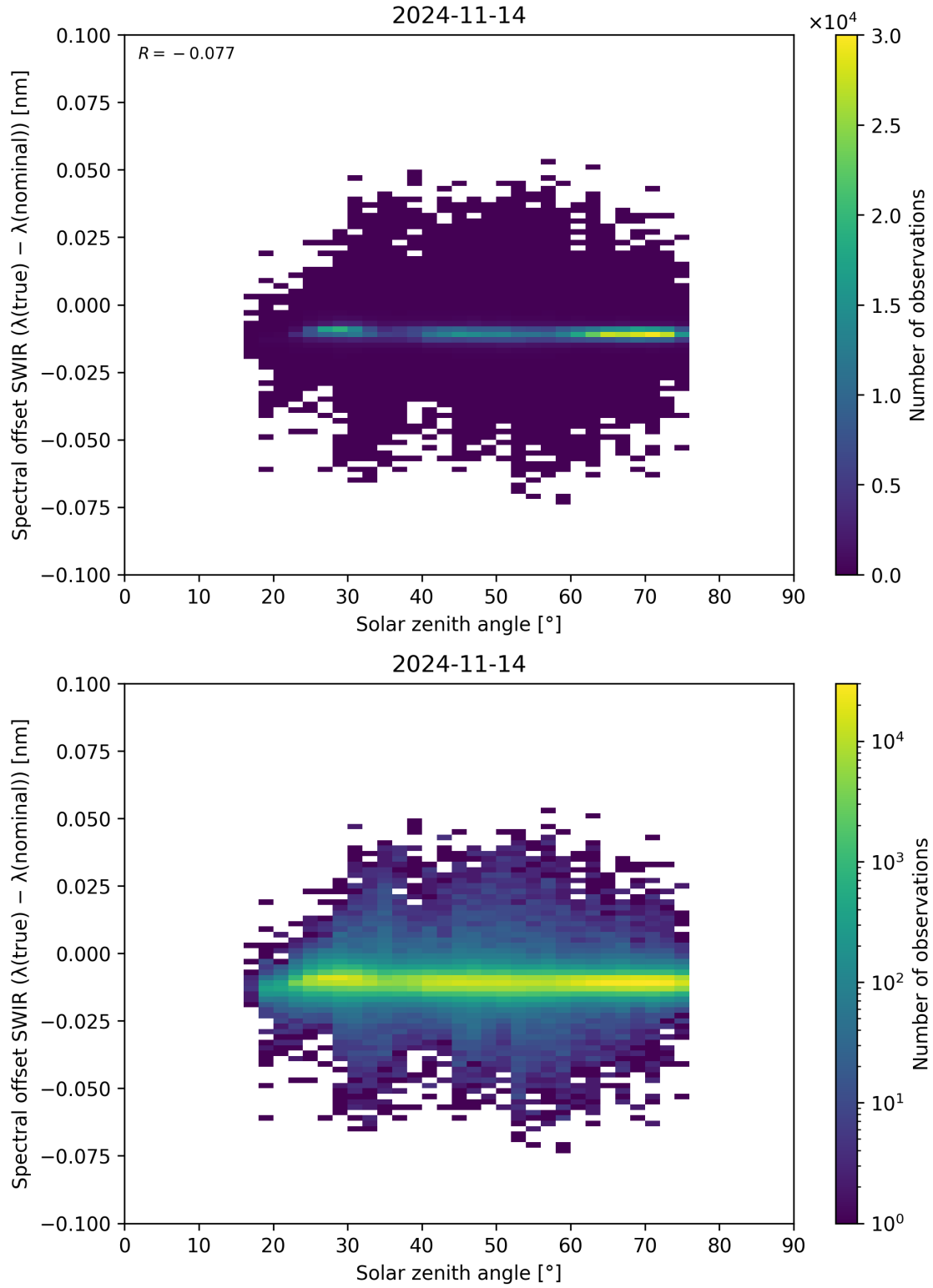
Figure 104: Scatter density plot of “Solar zenith angle” against “Spectral offset SWIR ( \lambda_{\text{true}} - \lambda_{\text{nominal}} )” for 2024-11-14 to 2024-11-15.
