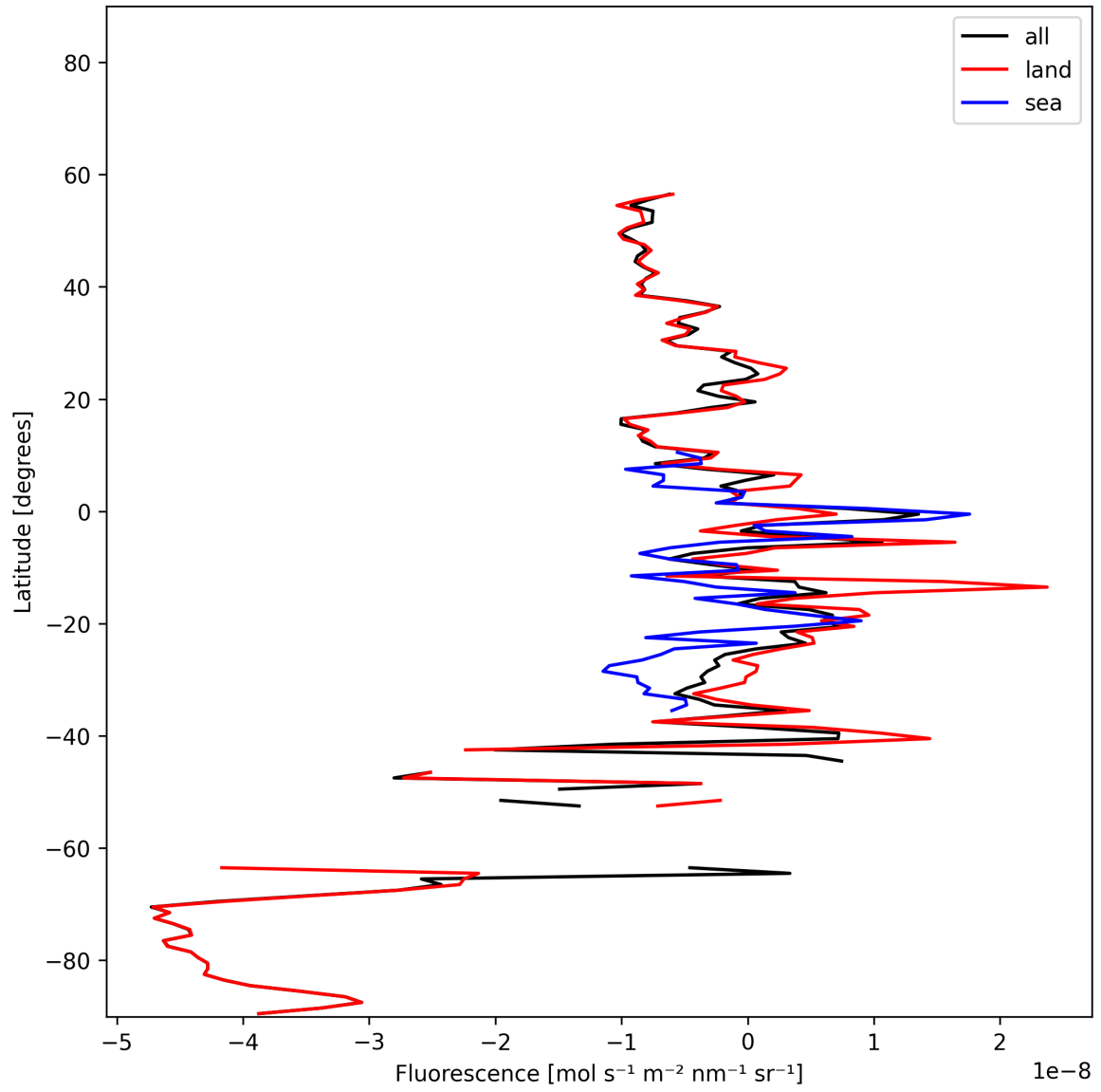
Figure 21: Zonal average of “Fluorescence” for 2024-11-14 to 2024-11-15.
