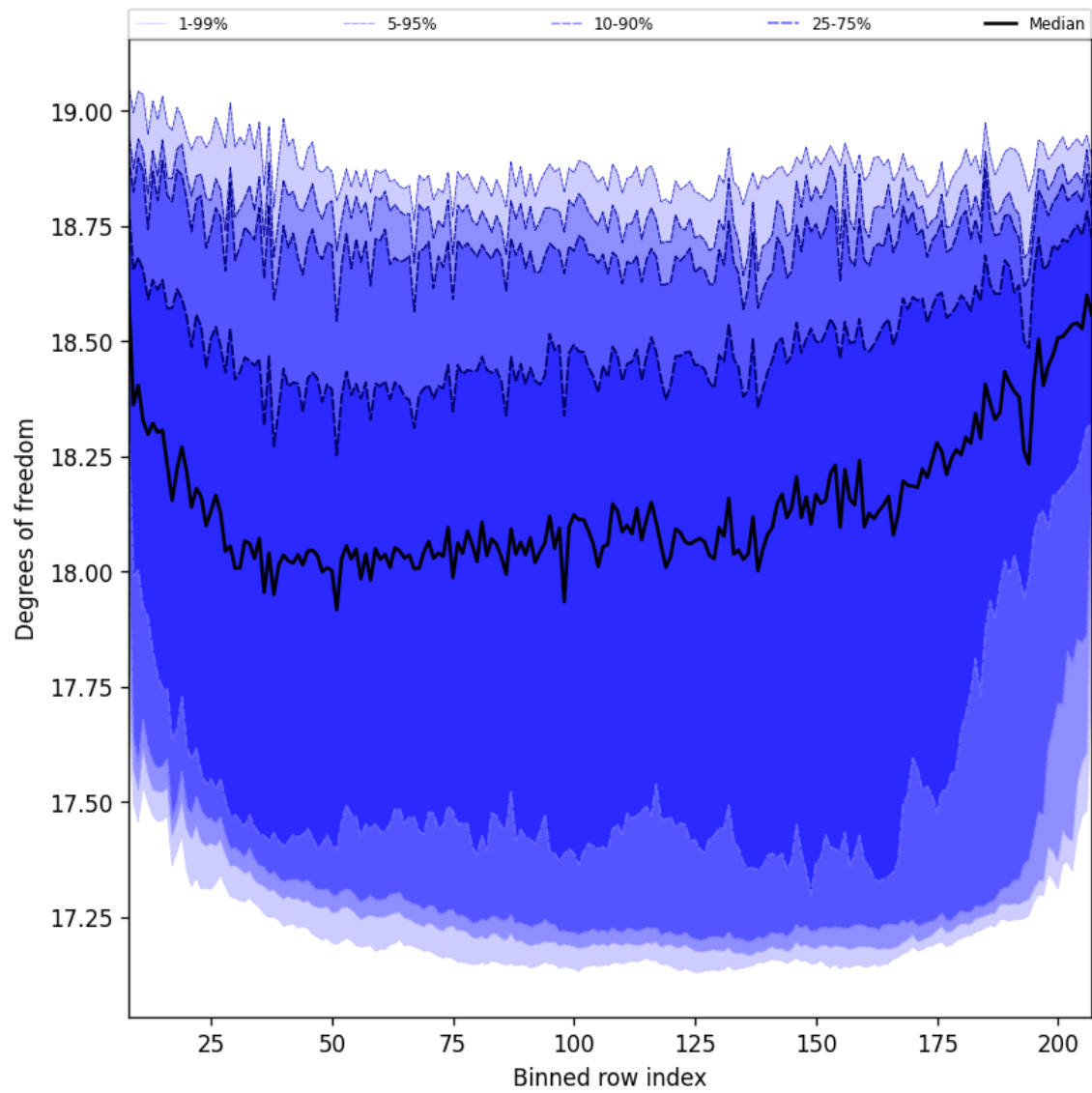
Figure 41: Along track statistics of “Degrees of freedom” for 2024-11-14 to 2024-11-15
