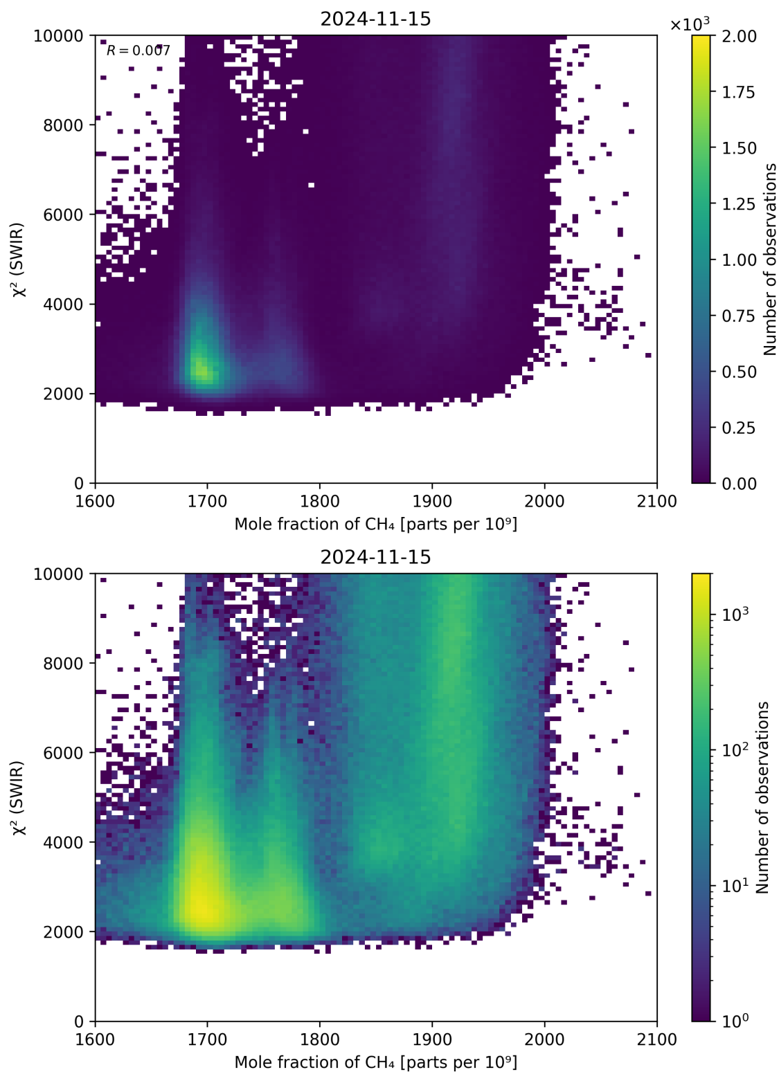
Figure 71: Scatter density plot of “Mole fraction of \text{CH}_4 ” against “ \chi^2 (SWIR)” for 2024-11-14 to 2024-11-16.
