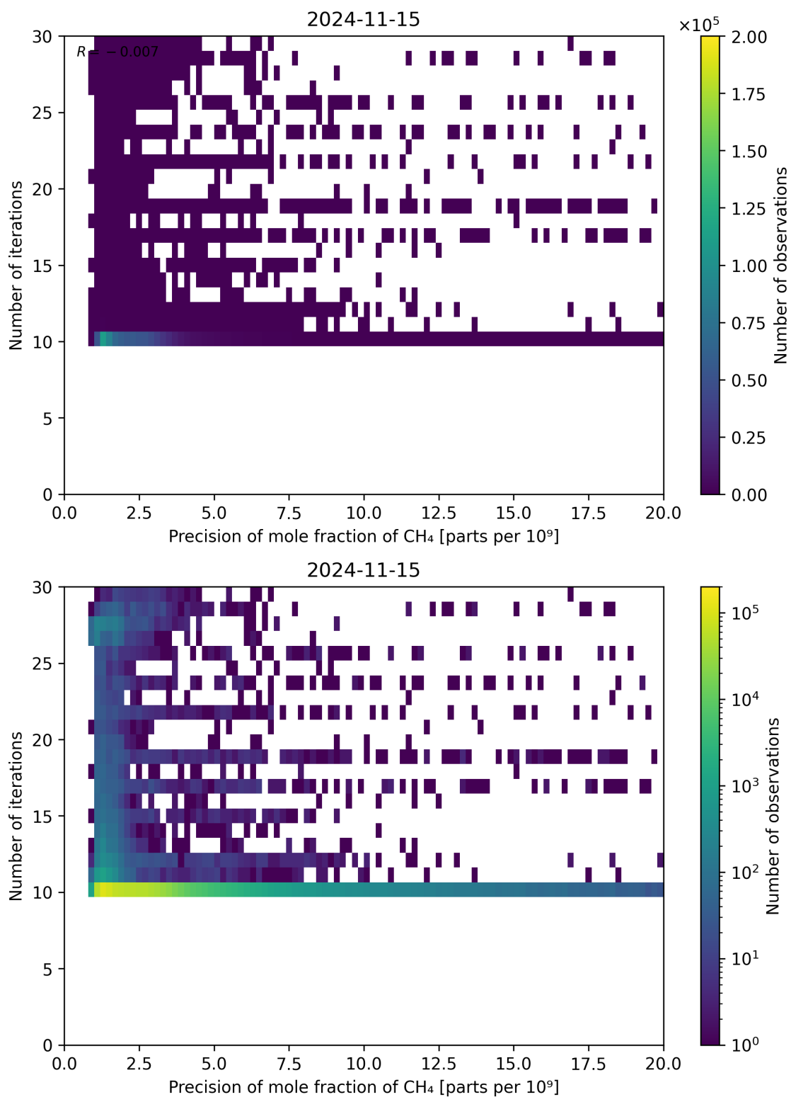
Figure 83: Scatter density plot of “Precision of mole fraction of CH 4 ” against “Number of iterations” for 2024-11-14 to 2024-11-16.
