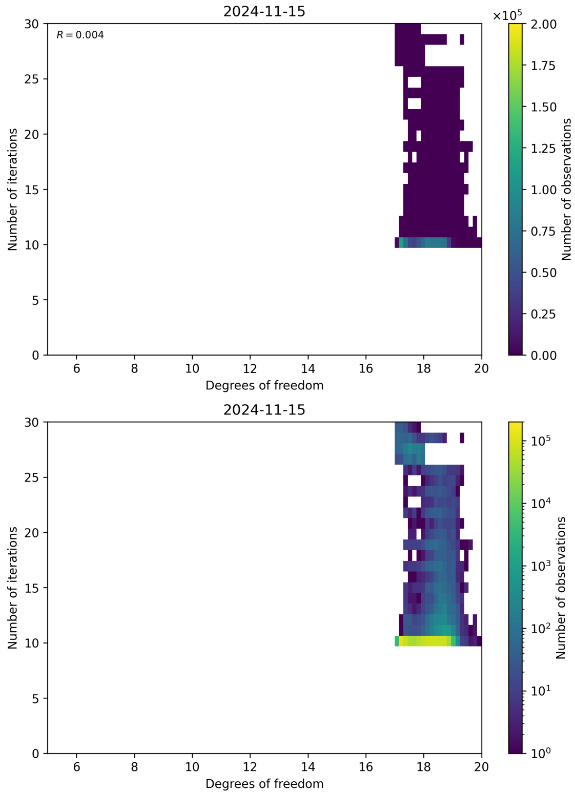
Figure 52: Scatter density plot of “Degrees of freedom” against “Number of iterations” for 2024-11-14 to 2024-11-16.
