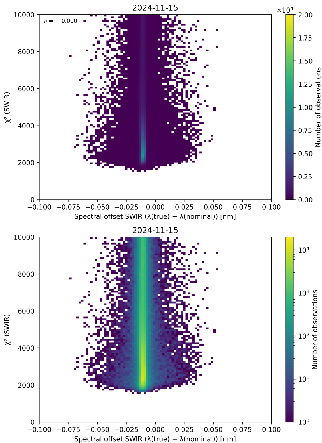
Figure 118: Scatter density plot of “Spectral offset SWIR ( \lambda_{\text{true}} - \lambda_{\text{nominal}} )” against “ \chi^2 (SWIR)” for 2024-11-14 to 2024-11-16.
