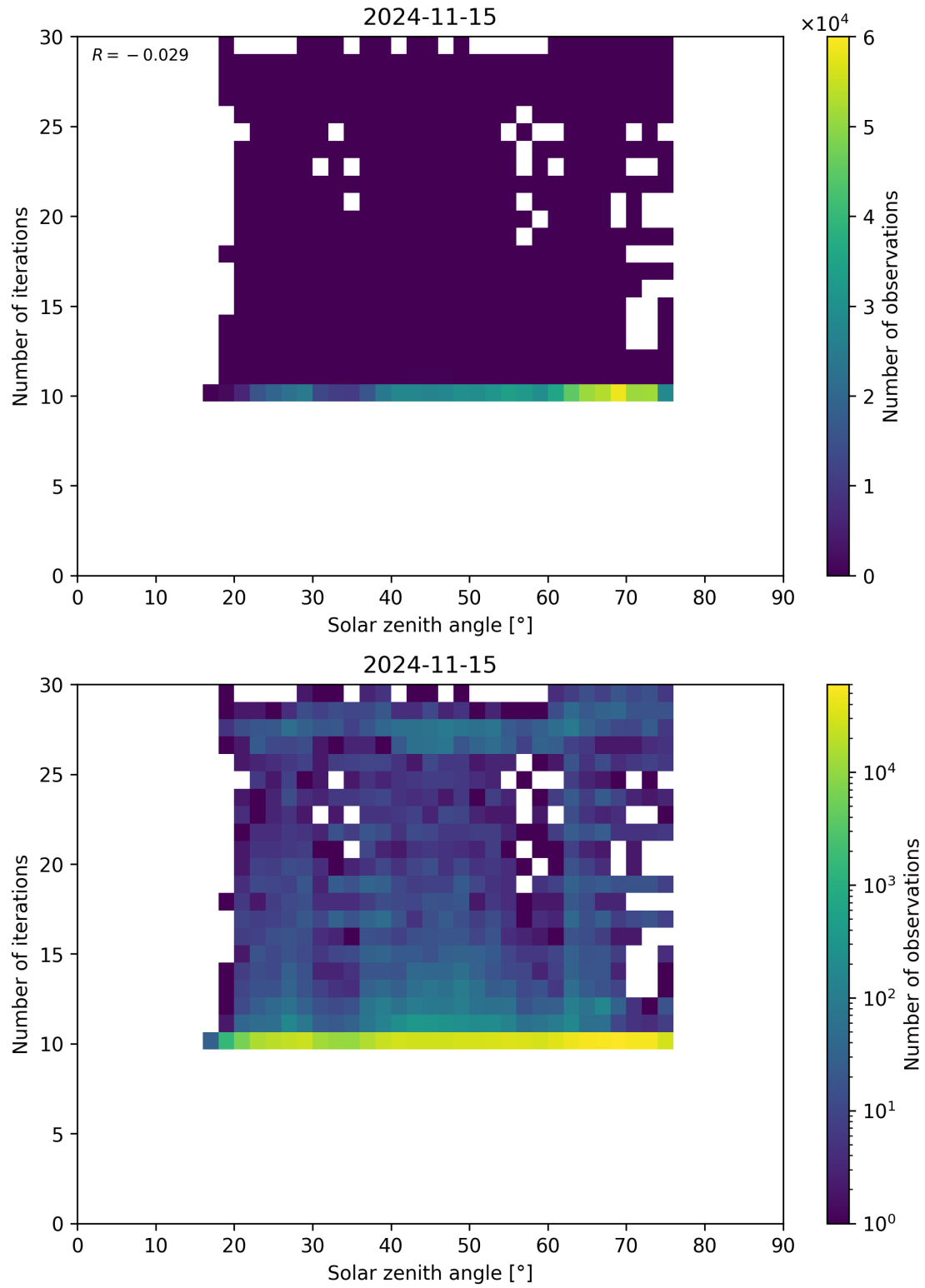
Figure 102: Scatter density plot of “Solar zenith angle” against “Number of iterations” for 2024-11-14 to 2024-11-16.
