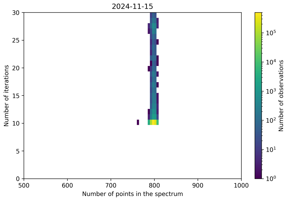
Figure 92: Scatter density plot of “Number of points in the spectrum” against “Number of iterations” for 2024-11-14 to 2024-11-16.
