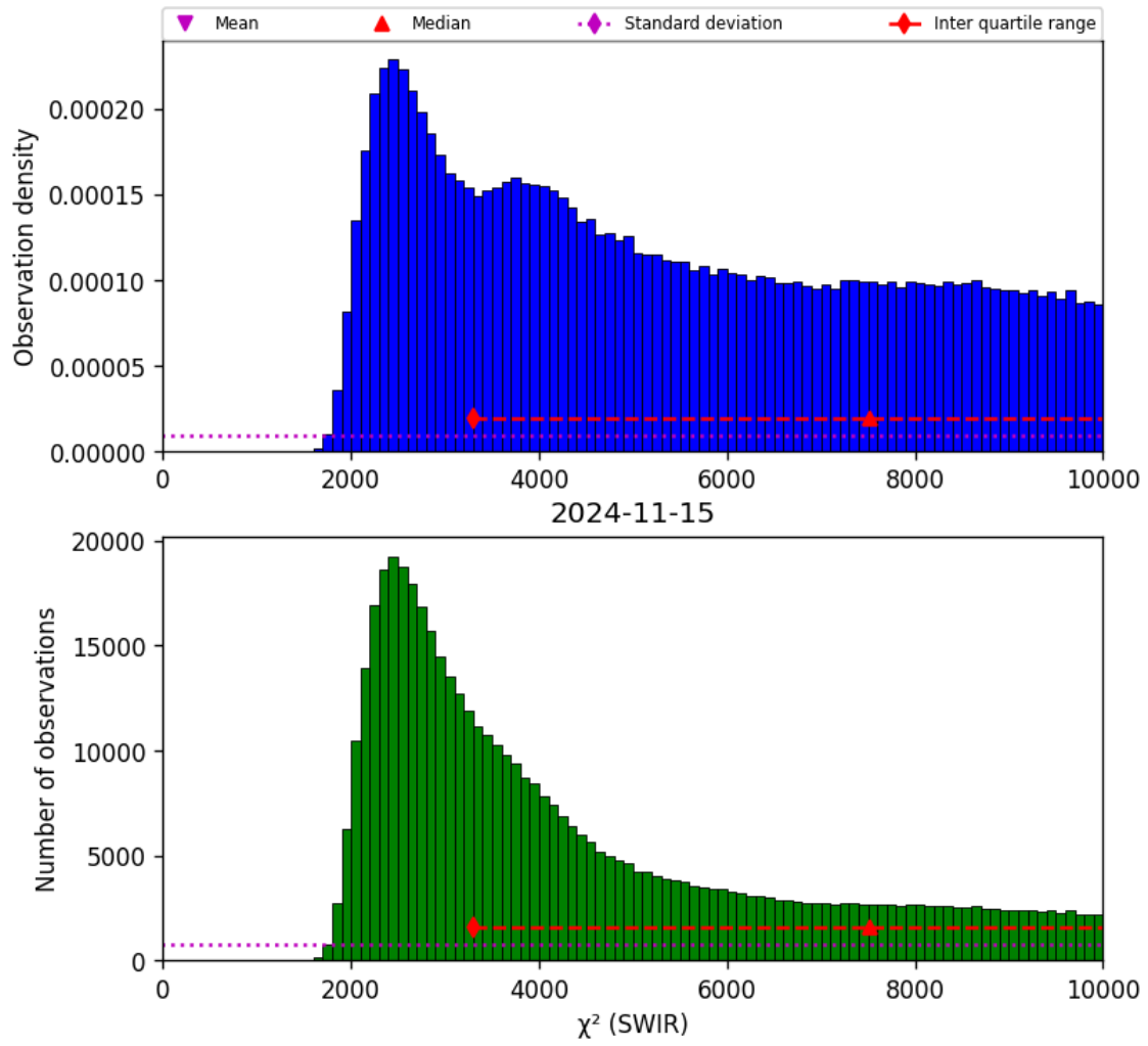
Figure 28: Histogram of “ \chi^2 (SWIR)” for 2024-11-14 to 2024-11-16
