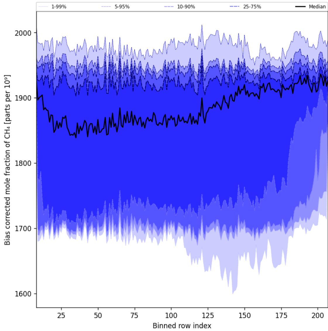
Figure 36: Along track statistics of “Bias corrected mole fraction of CH 4 ” for 2024-11-14 to 2024-11-16
