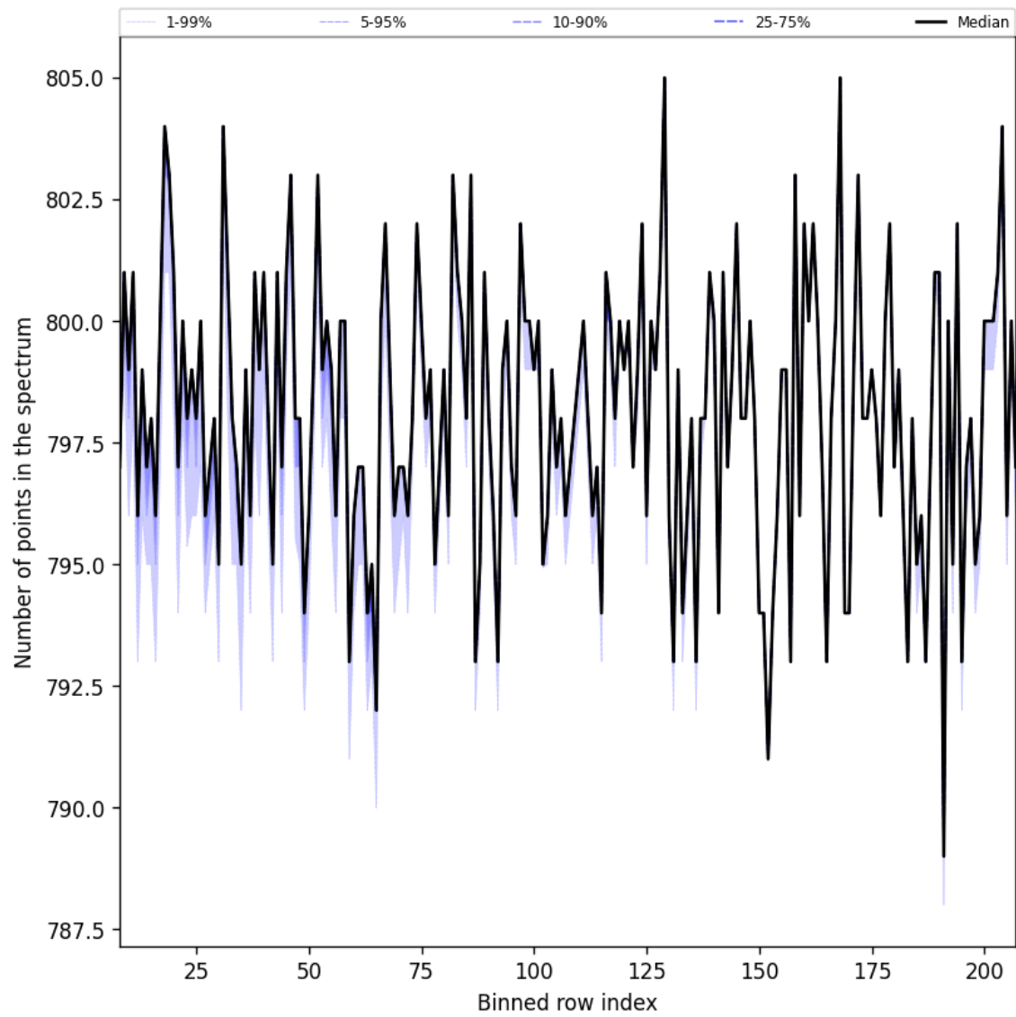
Figure 37: Along track statistics of “Number of points in the spectrum” for 2024-11-14 to 2024-11-16
