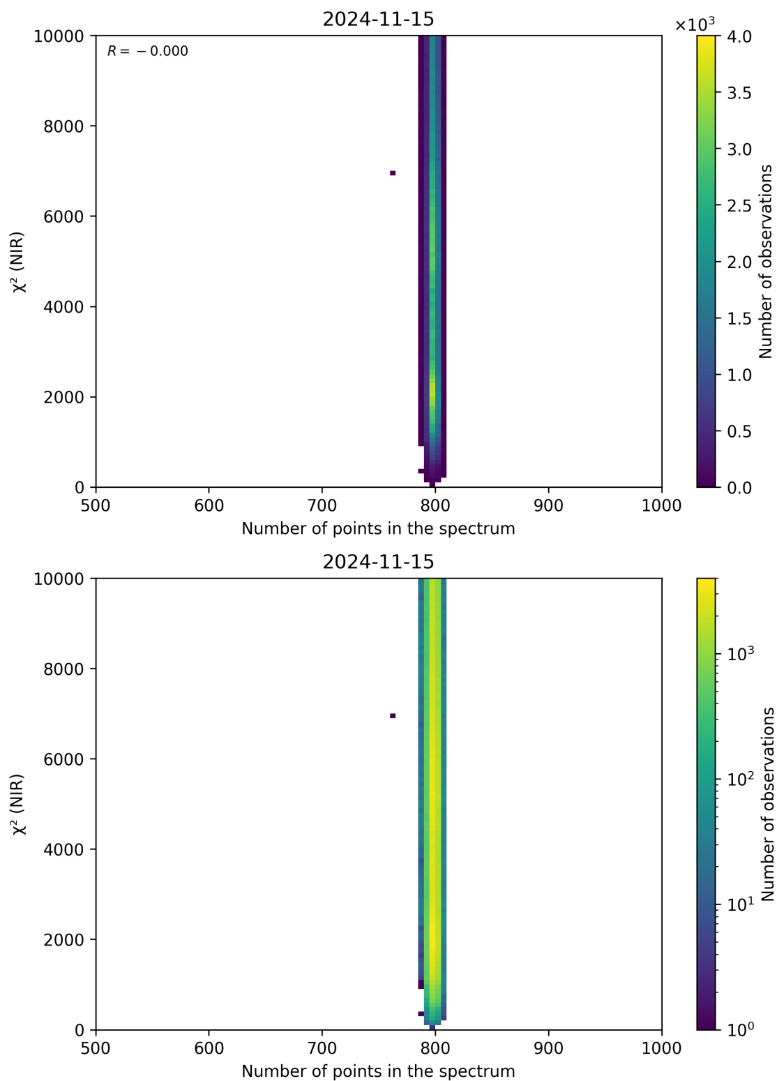
Figure 88: Scatter density plot of “Number of points in the spectrum” against “ \chi^2 (NIR)” for 2024-11-14 to 2024-11-16.
