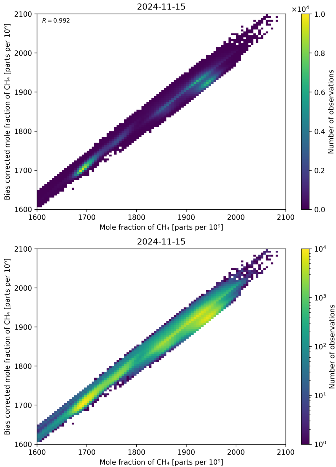
Figure 74: Scatter density plot of “Mole fraction of CH 4 ” against “Bias corrected mole fraction of CH 4 ” for 2024-11-14 to 2024-11-16.
