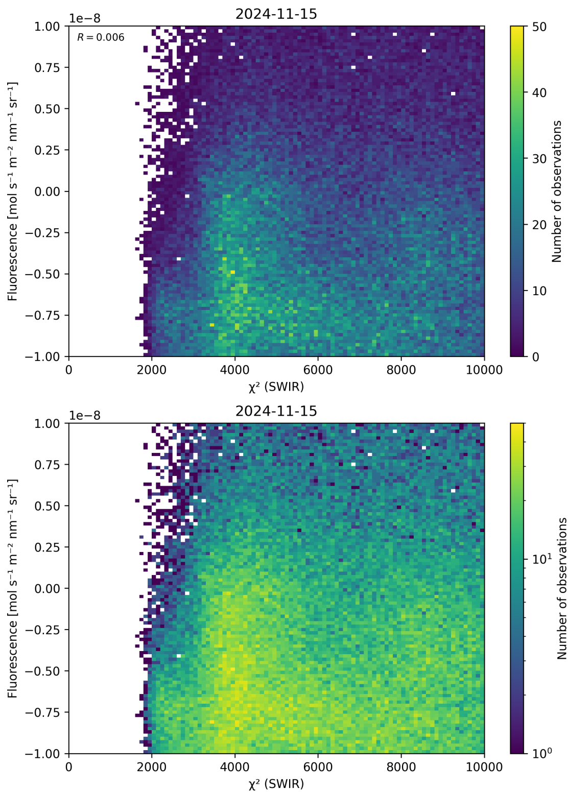
Figure 49: Scatter density plot of “ \chi^2 (SWIR)” against “Fluorescence” for 2024-11-14 to 2024-11-16.
