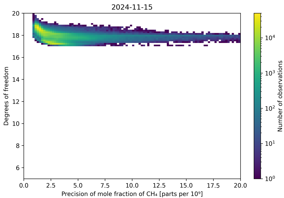
Figure 80: Scatter density plot of “Precision of mole fraction of CH 4 ” against “Degrees of freedom” for 2024-11-14 to 2024-11-16.
