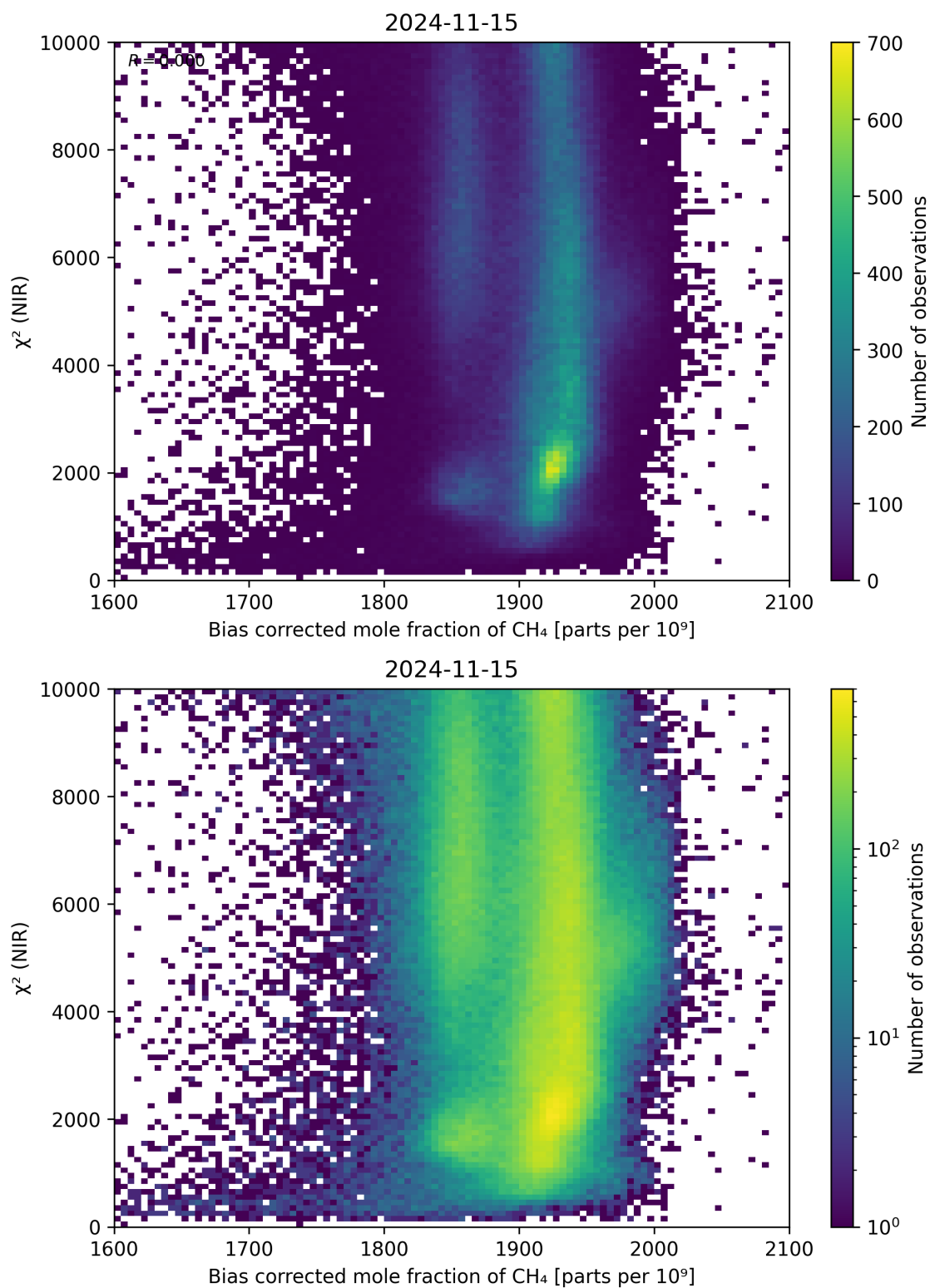
Figure 63: Scatter density plot of “Bias corrected mole fraction of \text{CH}_4 ” against “ \chi^2 (NIR)” for 2024-11-14 to 2024-11-16.
