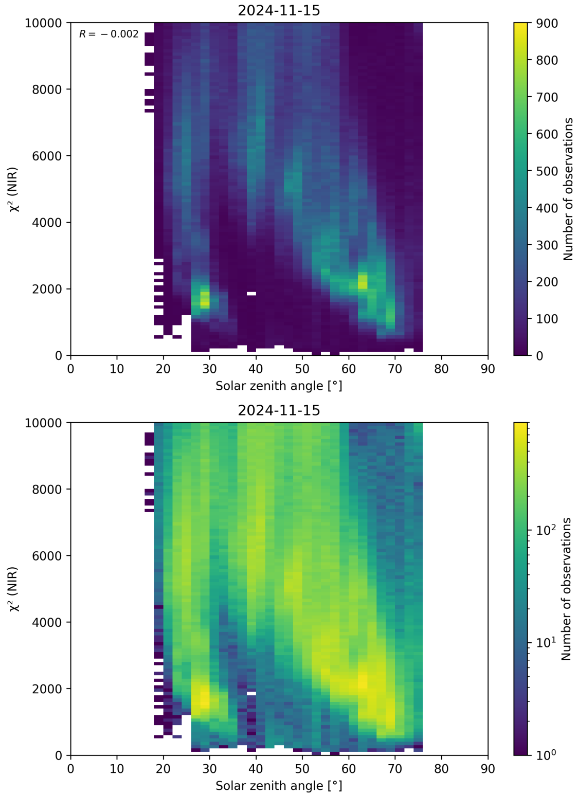
Figure 94: Scatter density plot of “Solar zenith angle” against “ \chi^2 (NIR)” for 2024-11-14 to 2024-11-16.
