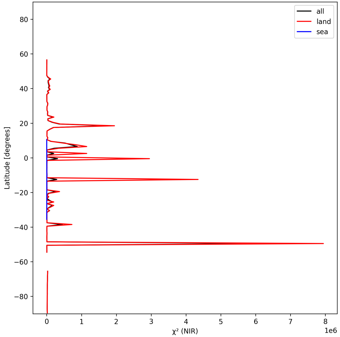
Figure 18: Zonal average of “ \chi^2 (NIR)” for 2024-11-14 to 2024-11-16.
