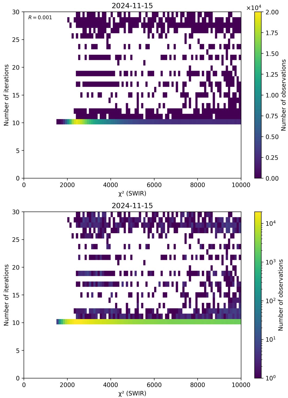
Figure 50: Scatter density plot of “ \chi^2 (SWIR)” against “Number of iterations” for 2024-11-14 to 2024-11-16.
