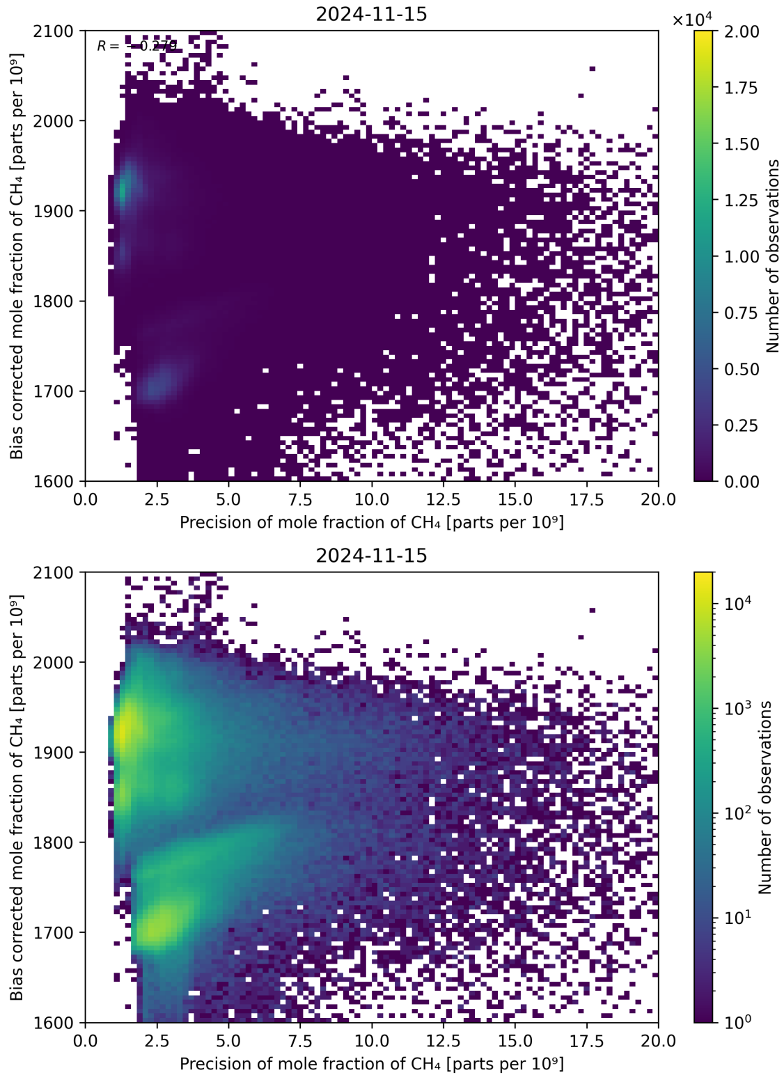
Figure 82: Scatter density plot of “Precision of mole fraction of \text{CH}_4 ” against “Bias corrected mole fraction of \text{CH}_4 ” for 2024-11-14 to 2024-11-16.
