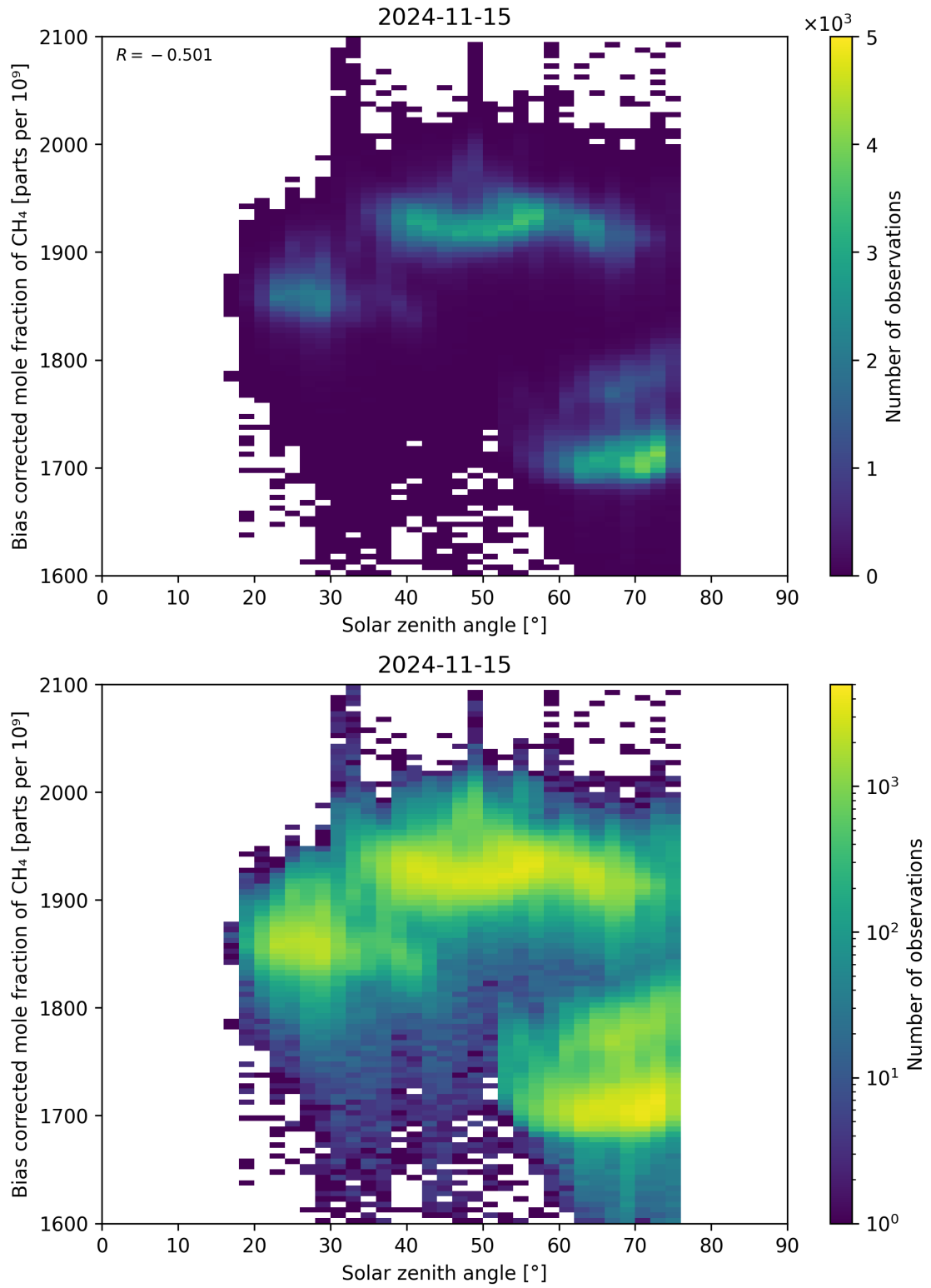
Figure 100: Scatter density plot of “Solar zenith angle” against “Bias corrected mole fraction of \text{CH}_4 ” for 2024-11-14 to 2024-11-16.
