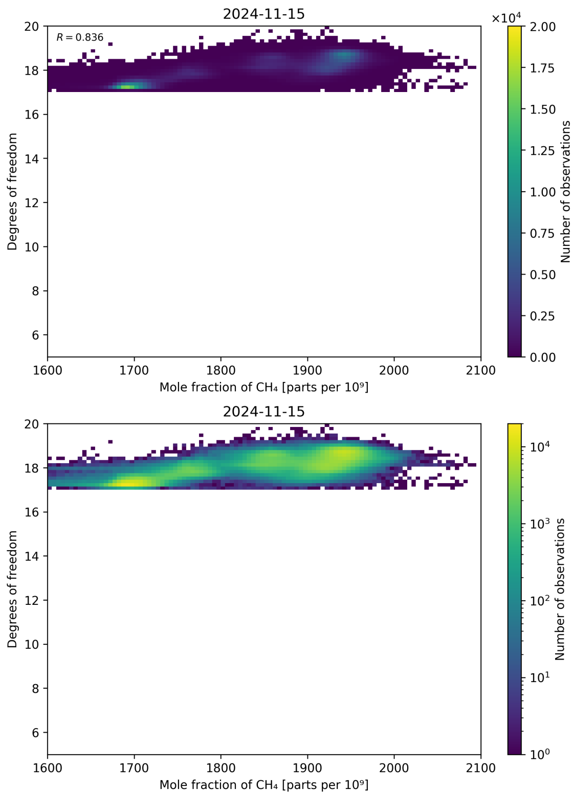
Figure 72: Scatter density plot of “Mole fraction of CH 4 ” against “Degrees of freedom” for 2024-11-14 to 2024-11-16.
