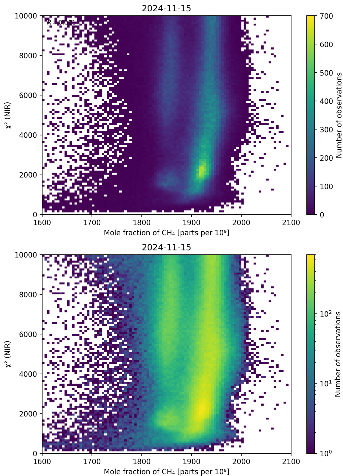
Figure 70: Scatter density plot of “Mole fraction of \text{CH}_4 ” against “ \chi^2 (NIR)” for 2024-11-14 to 2024-11-16.
