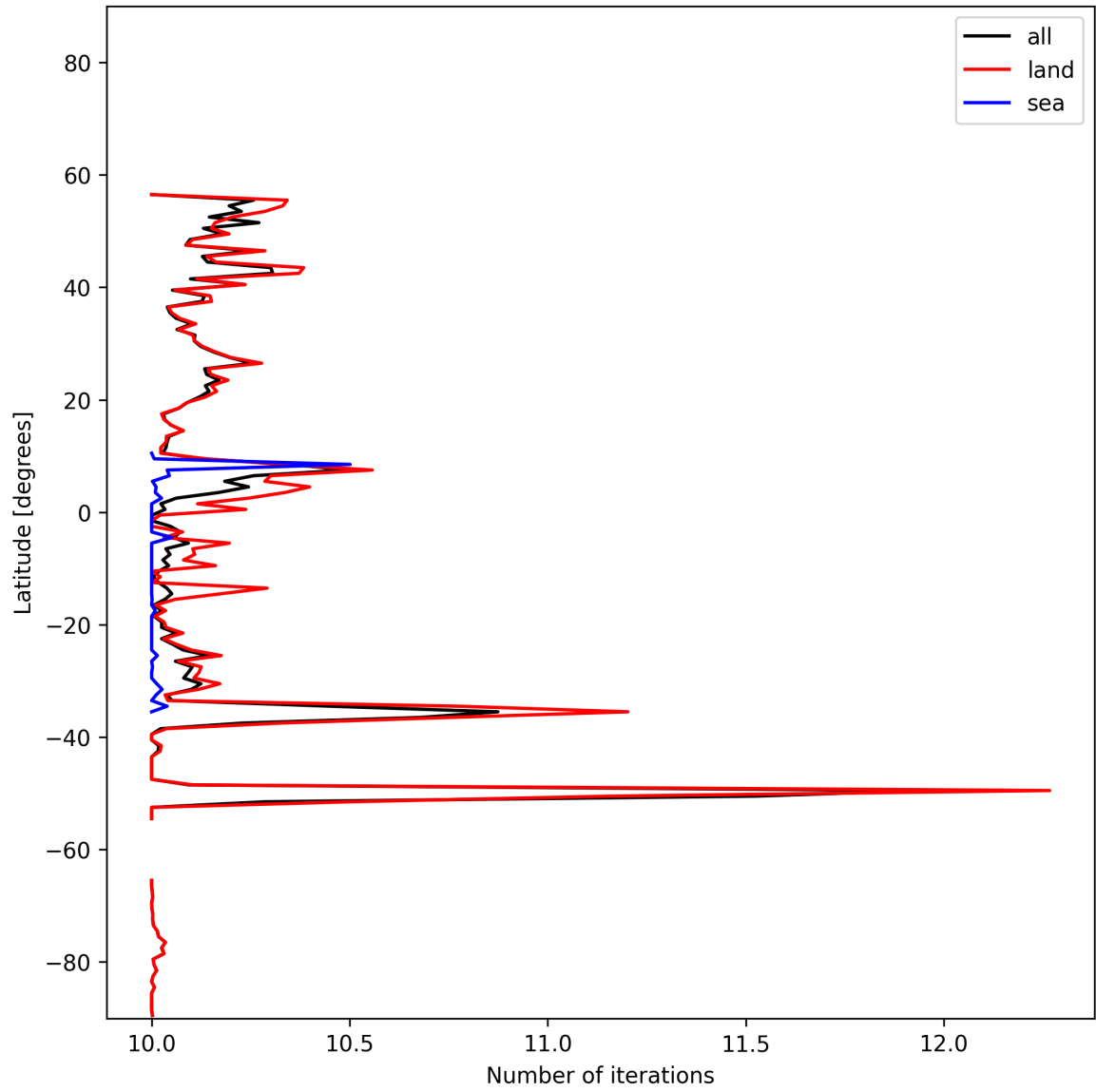
Figure 20: Zonal average of “Number of iterations” for 2024-11-14 to 2024-11-16.
