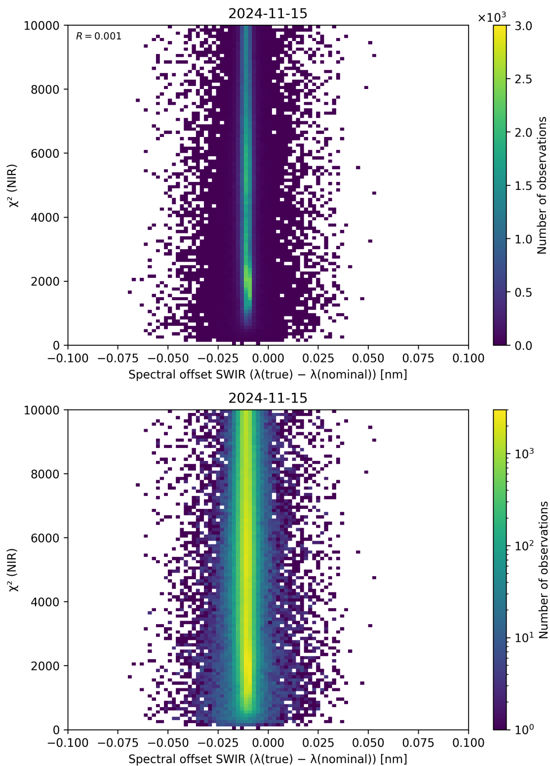
Figure 117: Scatter density plot of “Spectral offset SWIR ( \lambda_{\text{true}} - \lambda_{\text{nominal}} )” against “ \chi^2 (NIR)” for 2024-11-14 to 2024-11-16.
