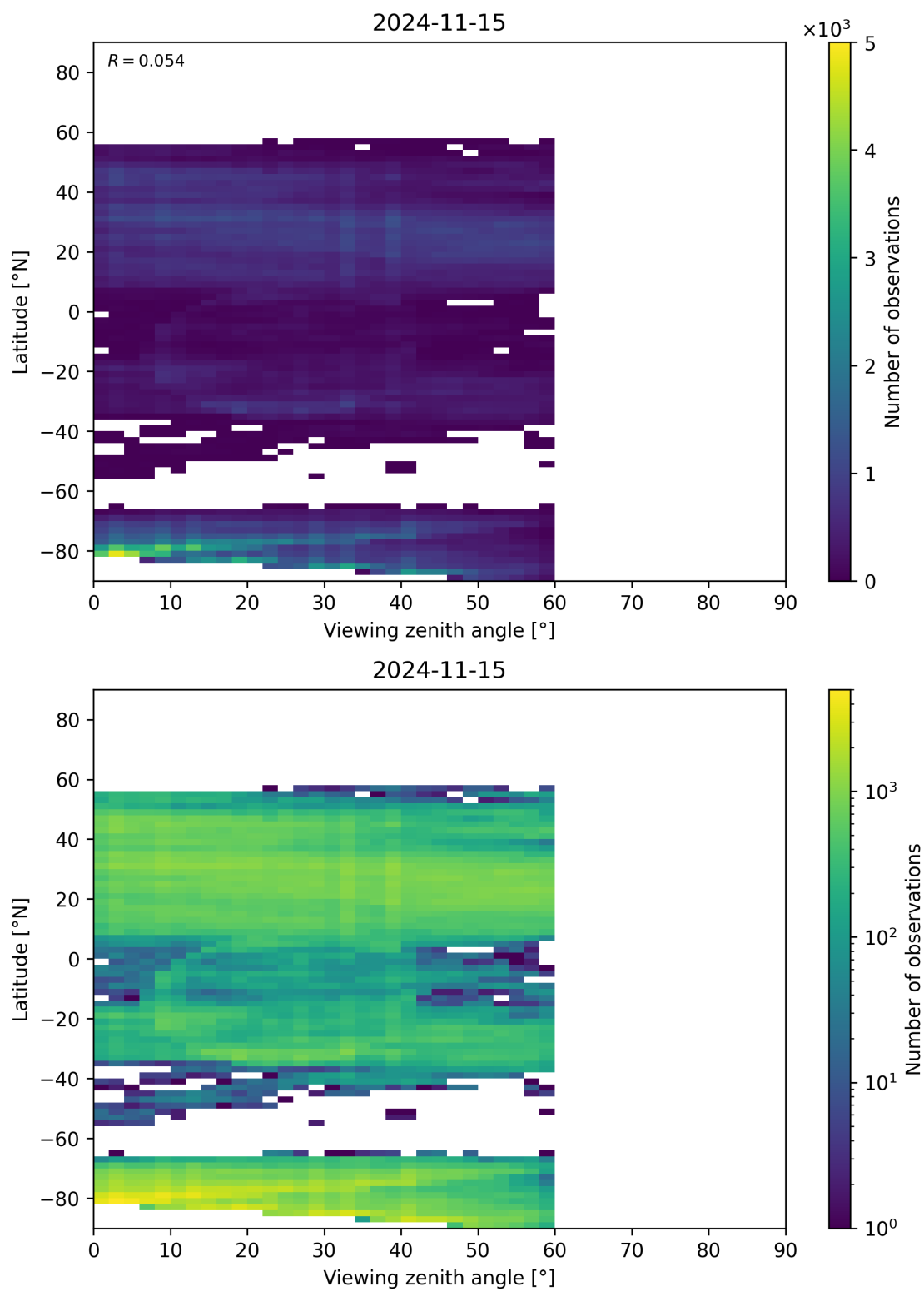
Figure 109: Scatter density plot of “Viewing zenith angle” against “Latitude” for 2024-11-14 to 2024-11-16.
