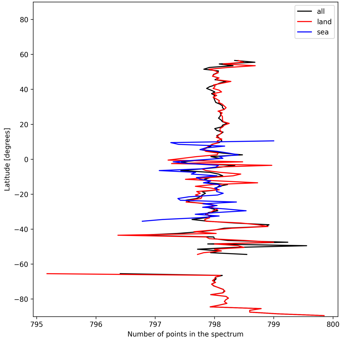
Figure 15: Zonal average of “Number of points in the spectrum” for 2024-11-14 to 2024-11-16.
