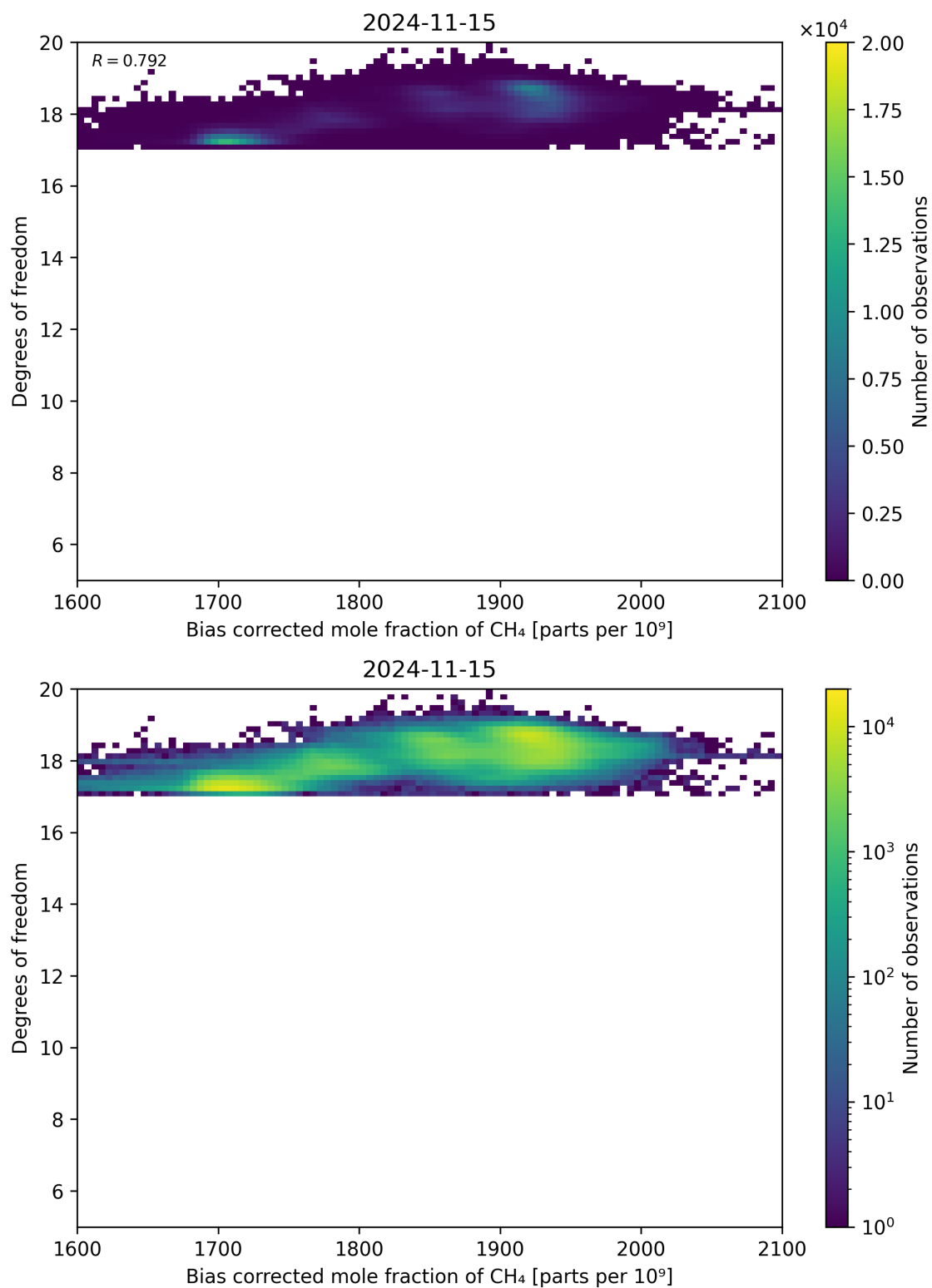
Figure 65: Scatter density plot of “Bias corrected mole fraction of CH 4 ” against “Degrees of freedom” for 2024-11-14 to 2024-11-16.
