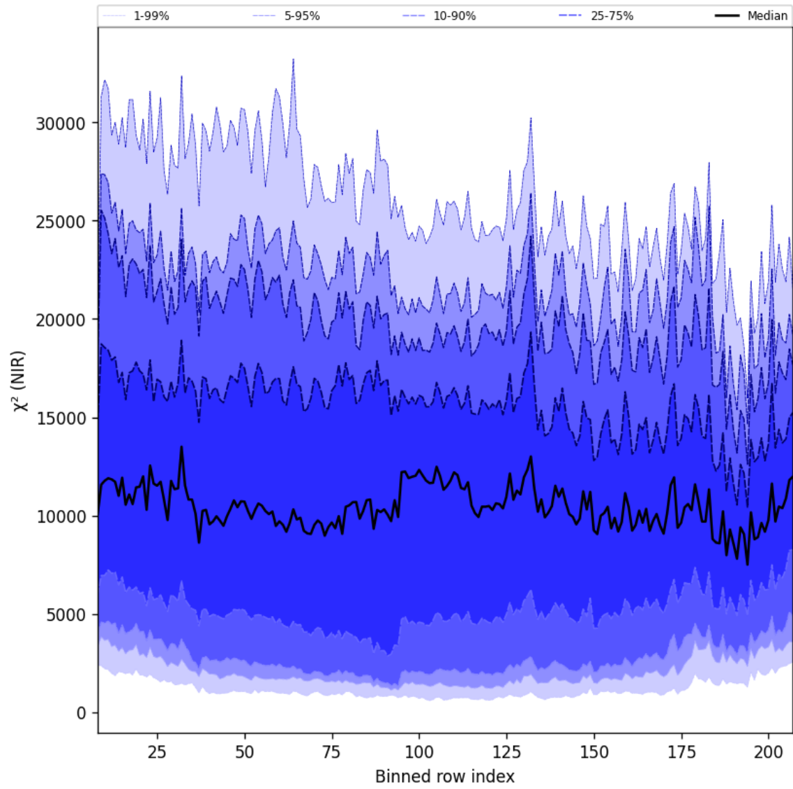
Figure 40: Along track statistics of " \chi^2 (NIR)" for 2024-11-14 to 2024-11-16
