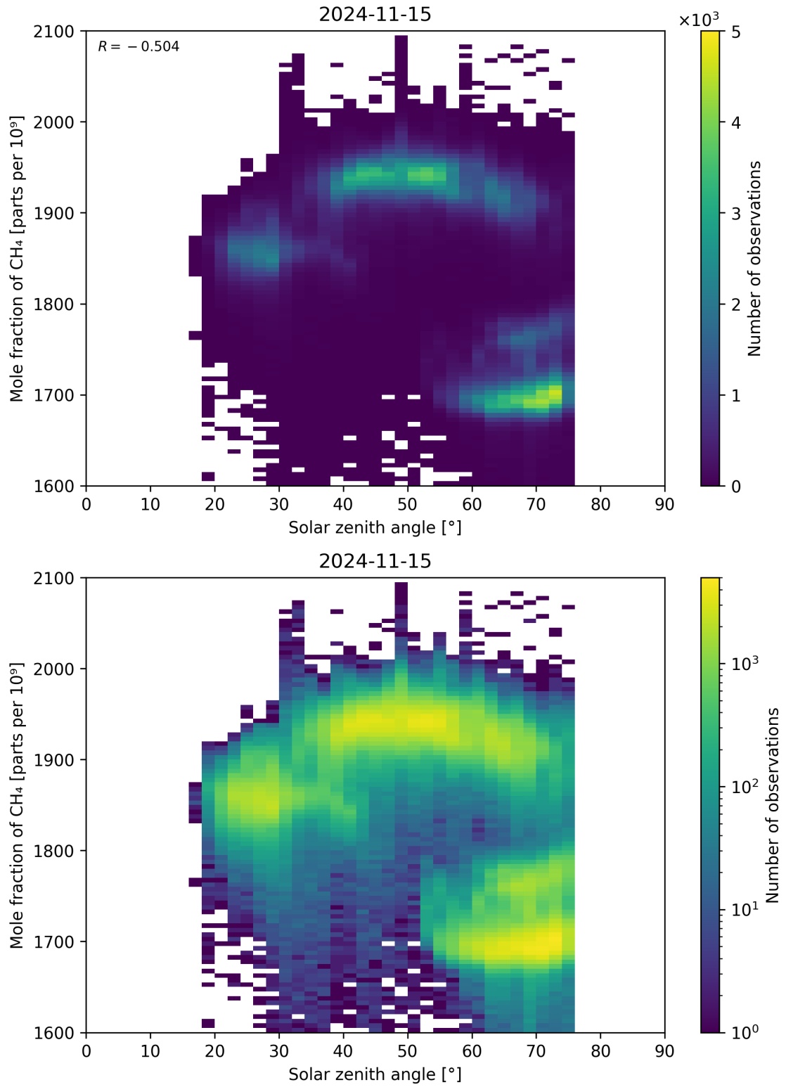
Figure 99: Scatter density plot of “Solar zenith angle” against “Mole fraction of \text{CH}_4 ” for 2024-11-14 to 2024-11-16.
