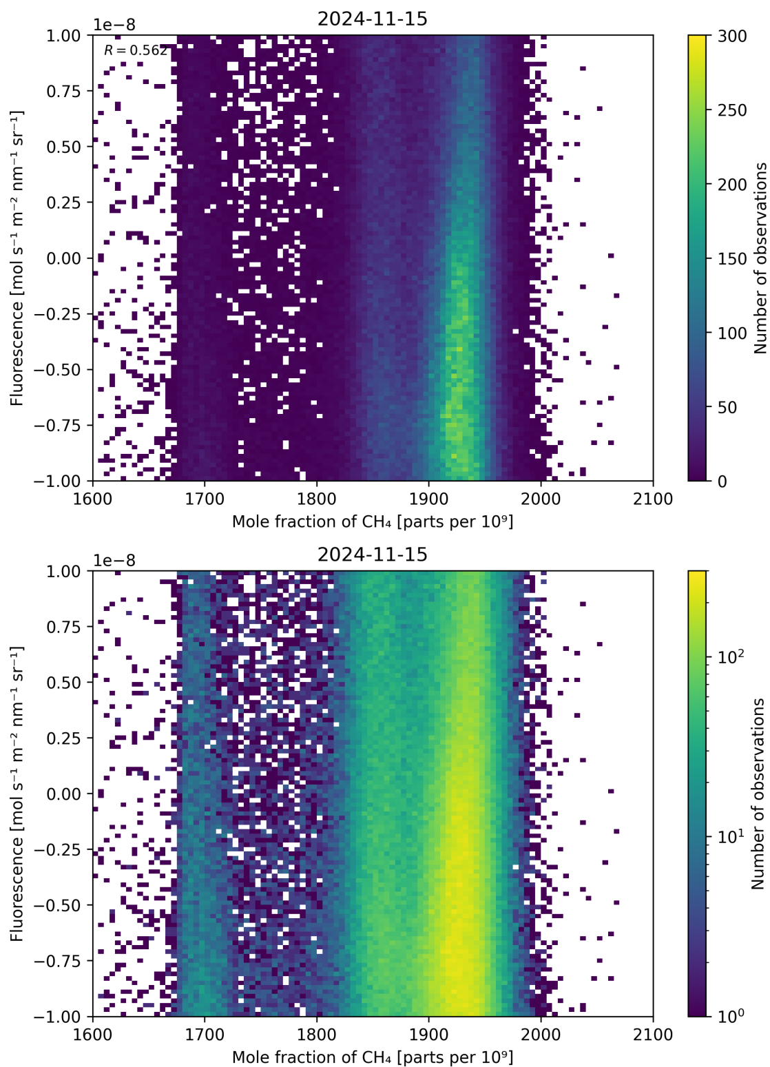
Figure 73: Scatter density plot of “Mole fraction of \text{CH}_4 ” against “Fluorescence” for 2024-11-14 to 2024-11-16.
