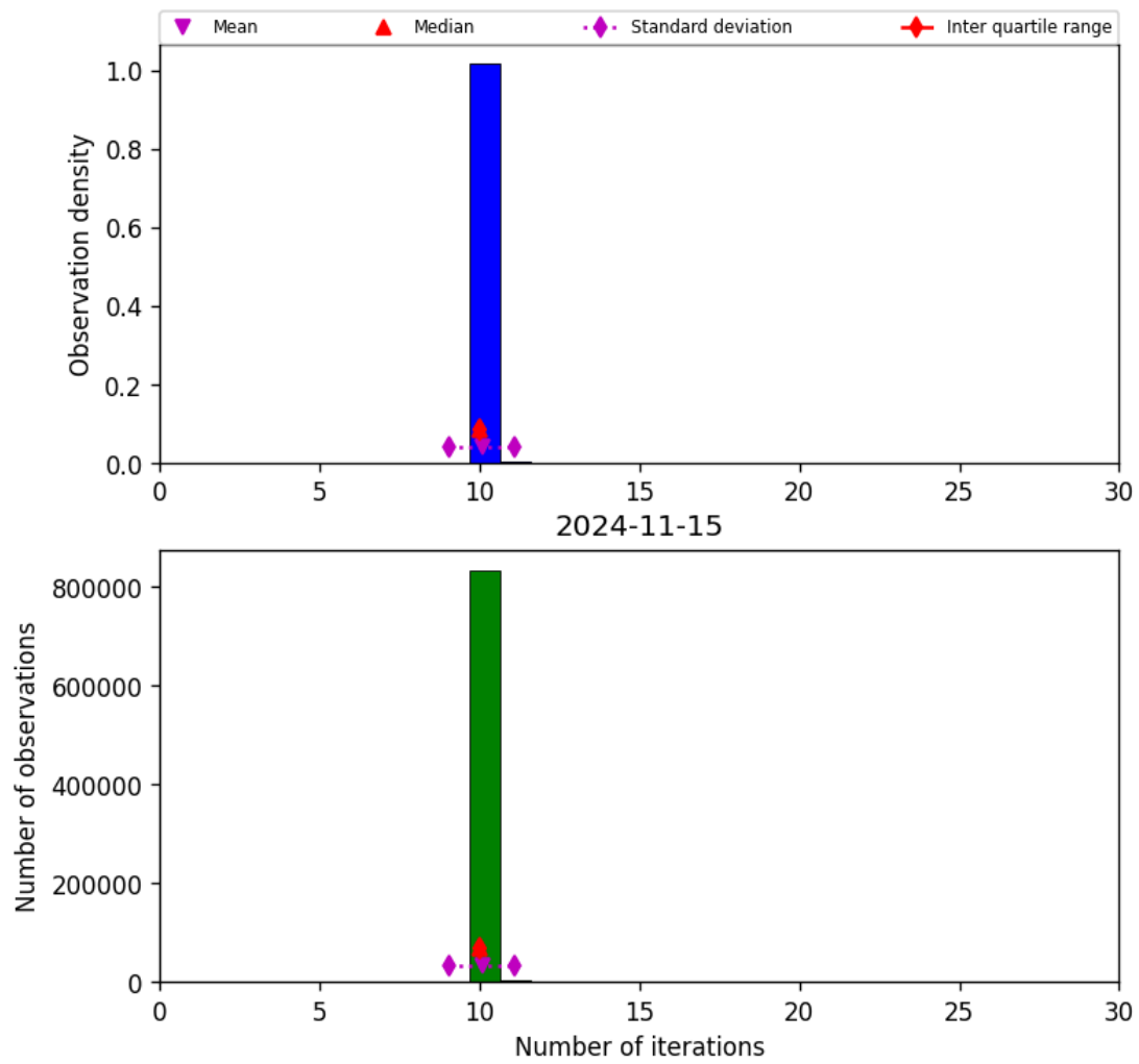
Figure 31: Histogram of “Number of iterations” for 2024-11-14 to 2024-11-16
