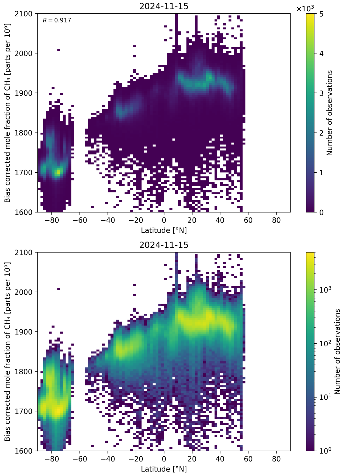
Figure 58: Scatter density plot of “Latitude” against “Bias corrected mole fraction of \text{CH}_4 ” for 2024-11-14 to 2024-11-16.
