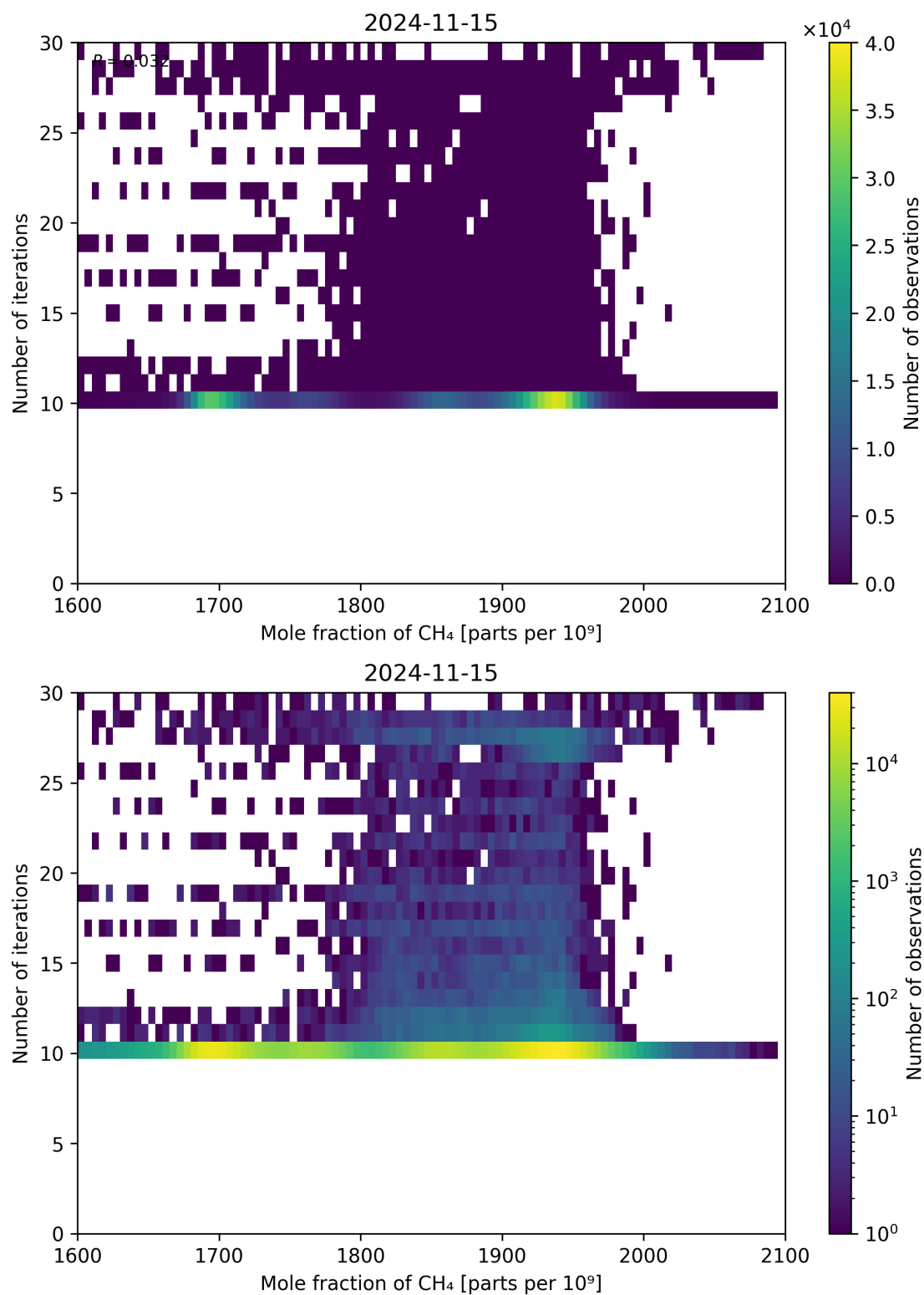
Figure 76: Scatter density plot of “Mole fraction of CH 4 ” against “Number of iterations” for 2024-11-14 to 2024-11-16.
