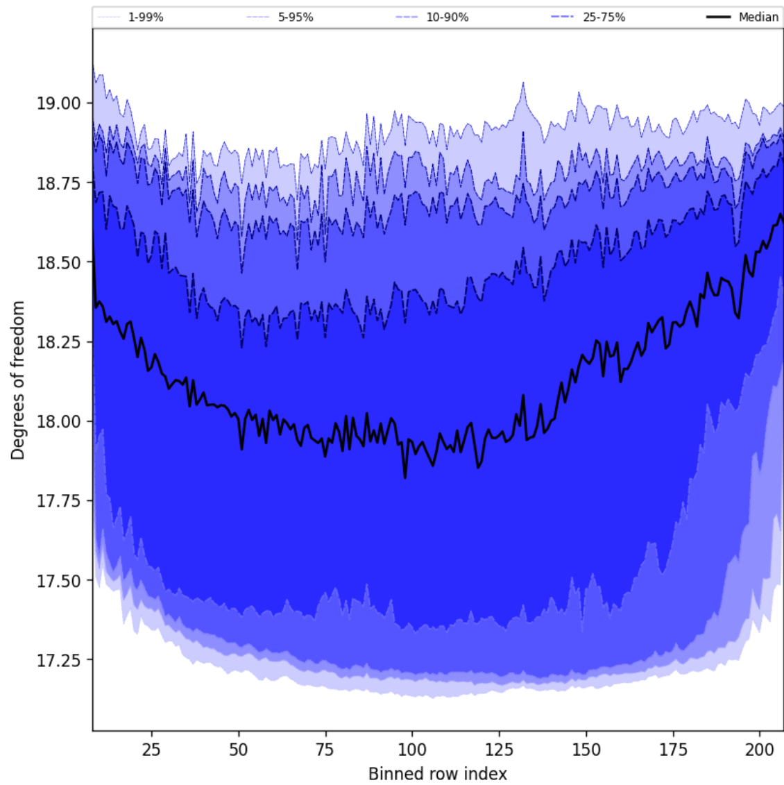
Figure 41: Along track statistics of “Degrees of freedom” for 2024-11-14 to 2024-11-16
