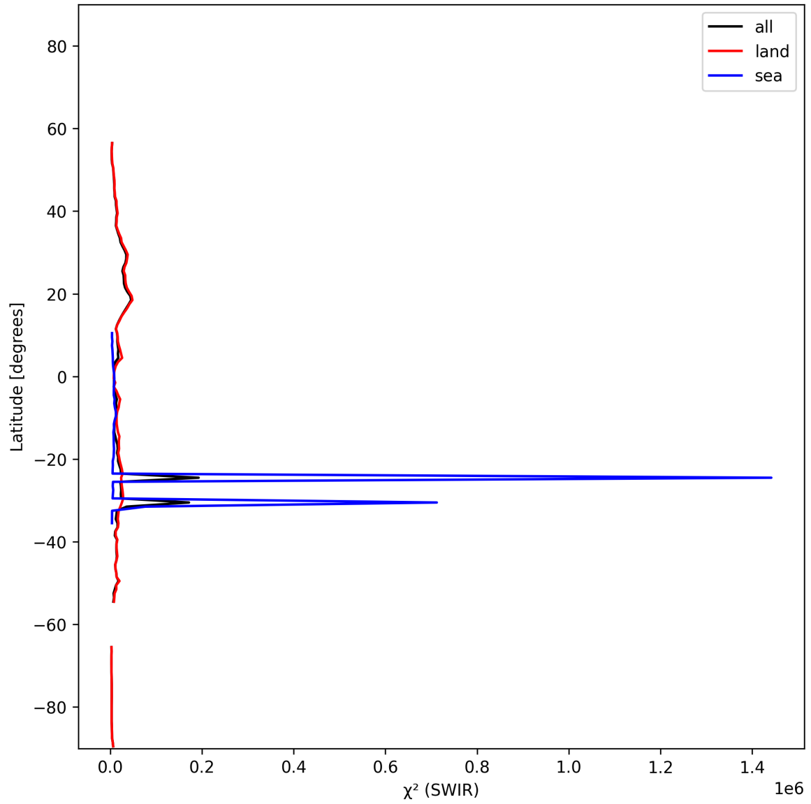
Figure 17: Zonal average of “ \chi^2 (SWIR)” for 2024-11-14 to 2024-11-16.
