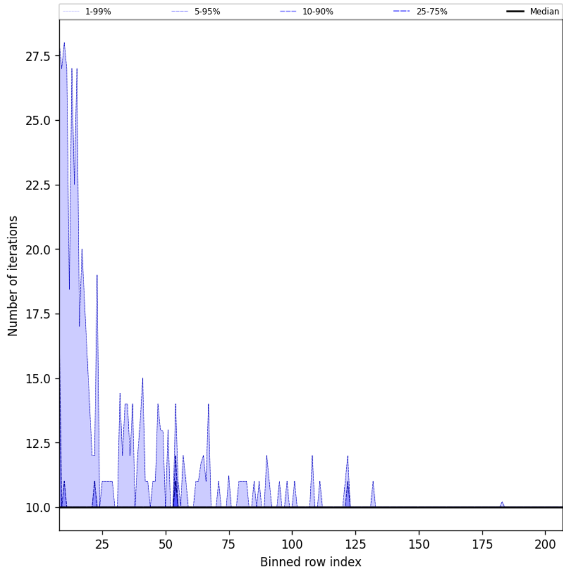
Figure 42: Along track statistics of “Number of iterations” for 2024-11-14 to 2024-11-16
