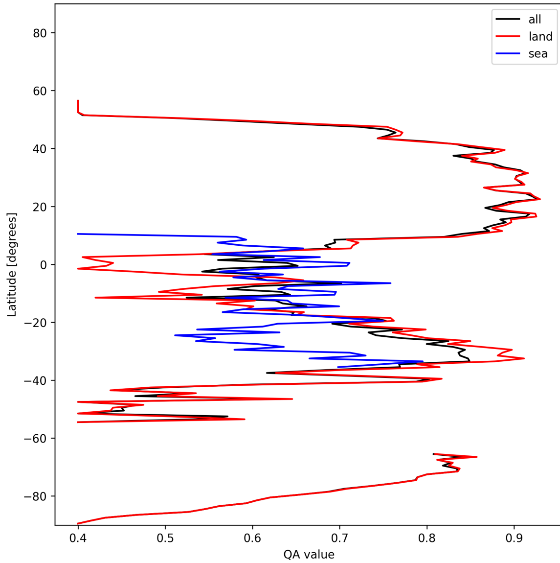
Figure 11: Zonal average of “QA value” for 2024-11-14 to 2024-11-16.
