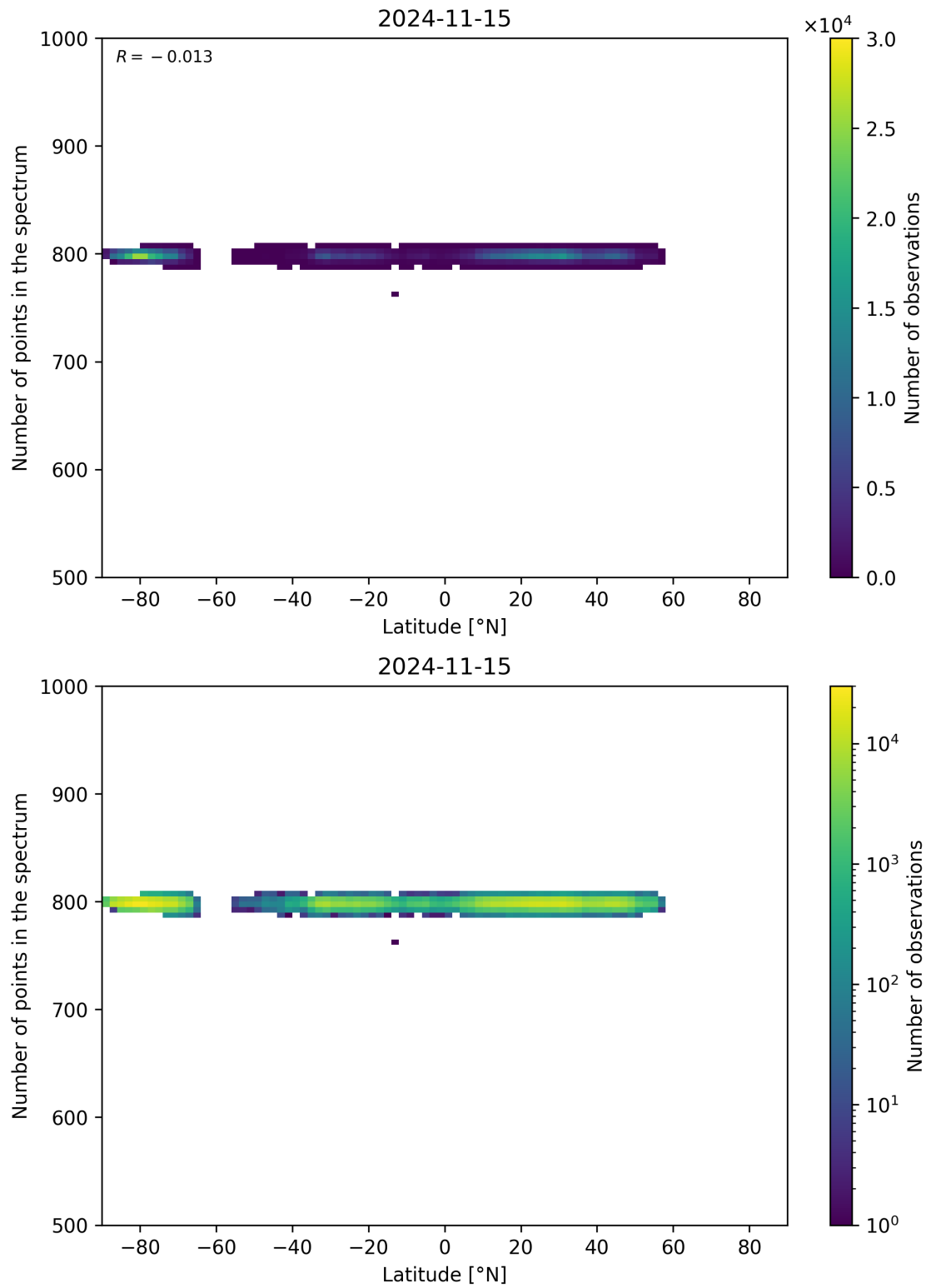
Figure 61: Scatter density plot of “Latitude” against “Number of points in the spectrum” for 2024-11-14 to 2024-11-16.
