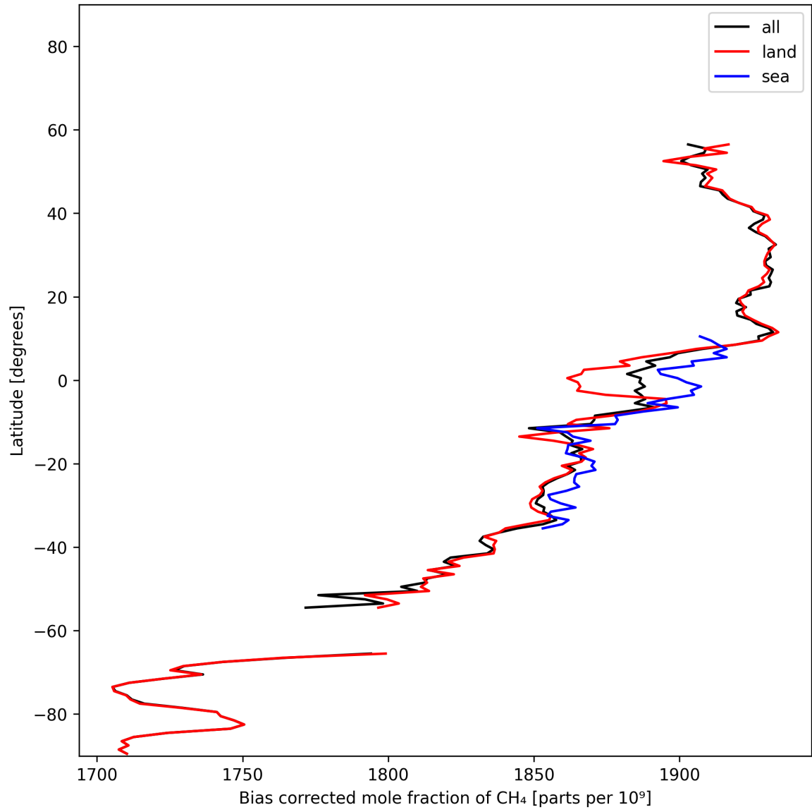
Figure 14: Zonal average of “Bias corrected mole fraction of CH 4 ” for 2024-11-14 to 2024-11-16.
