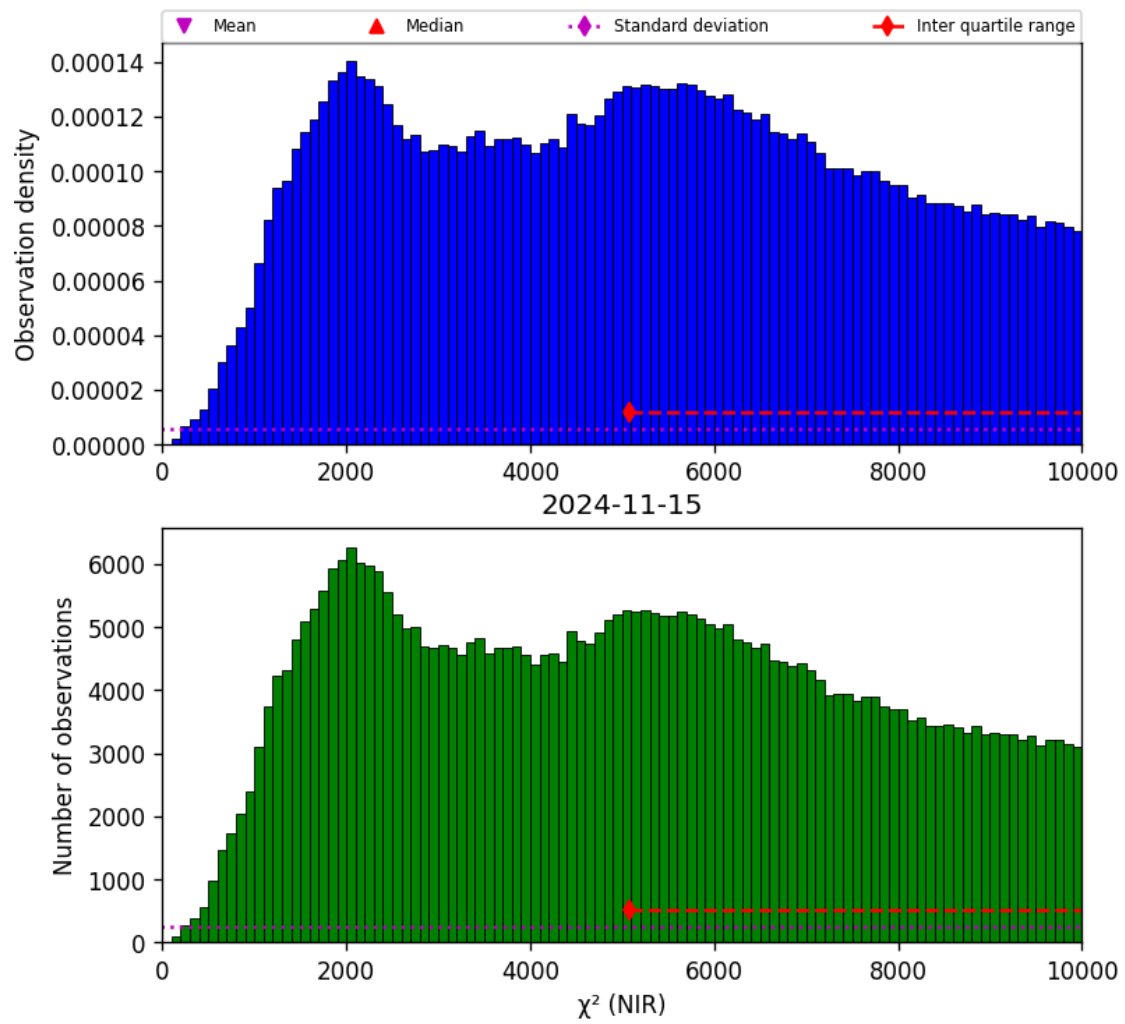
Figure 29: Histogram of “ \chi^2 (NIR)” for 2024-11-14 to 2024-11-16
