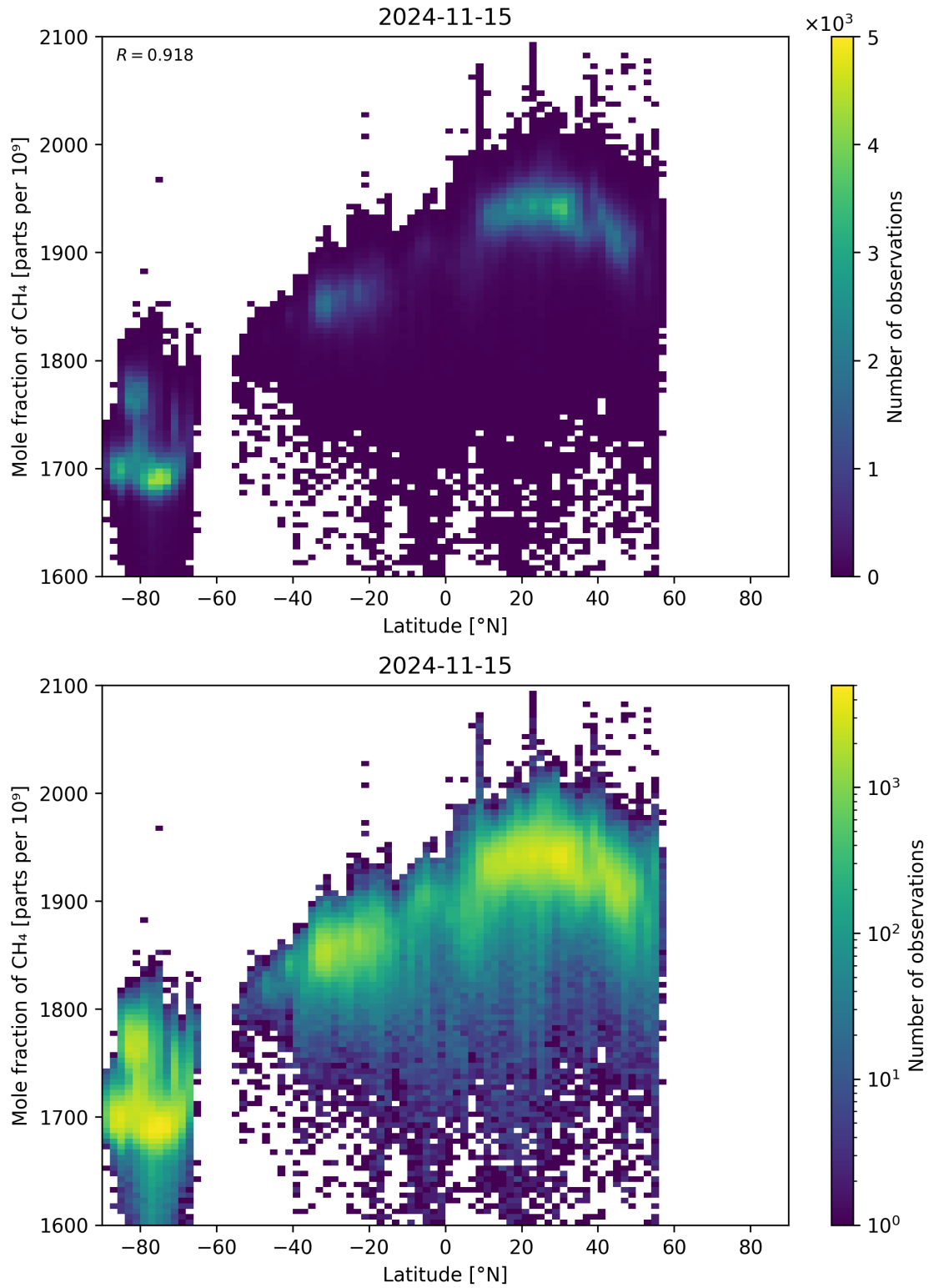
Figure 57: Scatter density plot of “Latitude” against “Mole fraction of CH 4 ” for 2024-11-14 to 2024-11-16.
