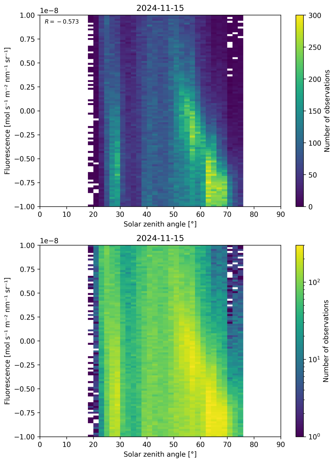
Figure 97: Scatter density plot of “Solar zenith angle” against “Fluorescence” for 2024-11-14 to 2024-11-16.
