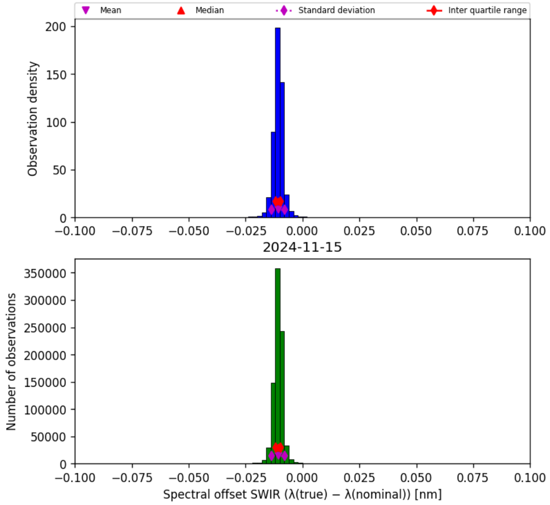
Figure 27: Histogram of “Spectral offset SWIR ( \lambda_{\text{true}} - \lambda_{\text{nominal}} )” for 2024-11-14 to 2024-11-16
