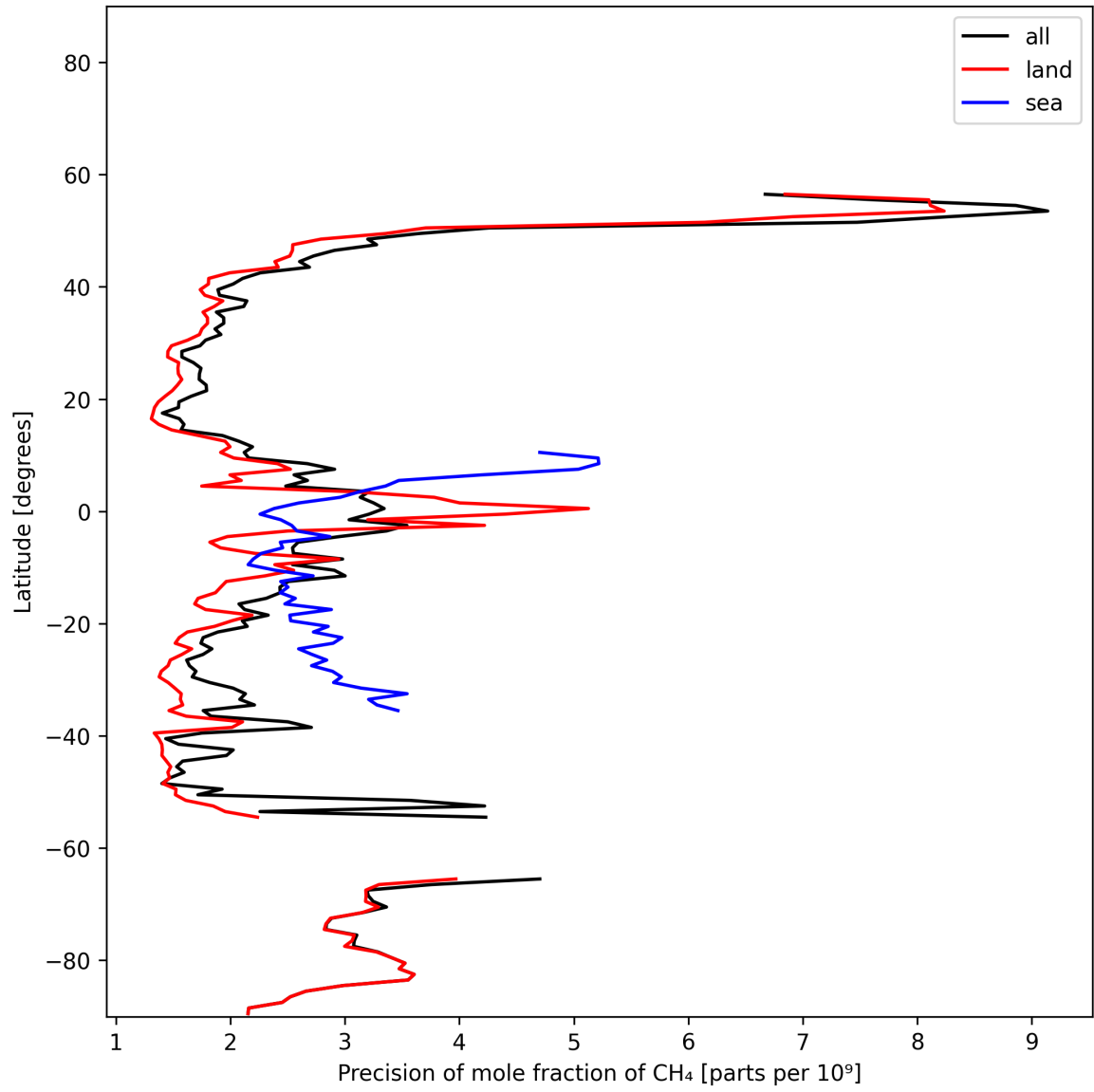
Figure 13: Zonal average of “Precision of mole fraction of CH 4 ” for 2024-11-14 to 2024-11-16.
