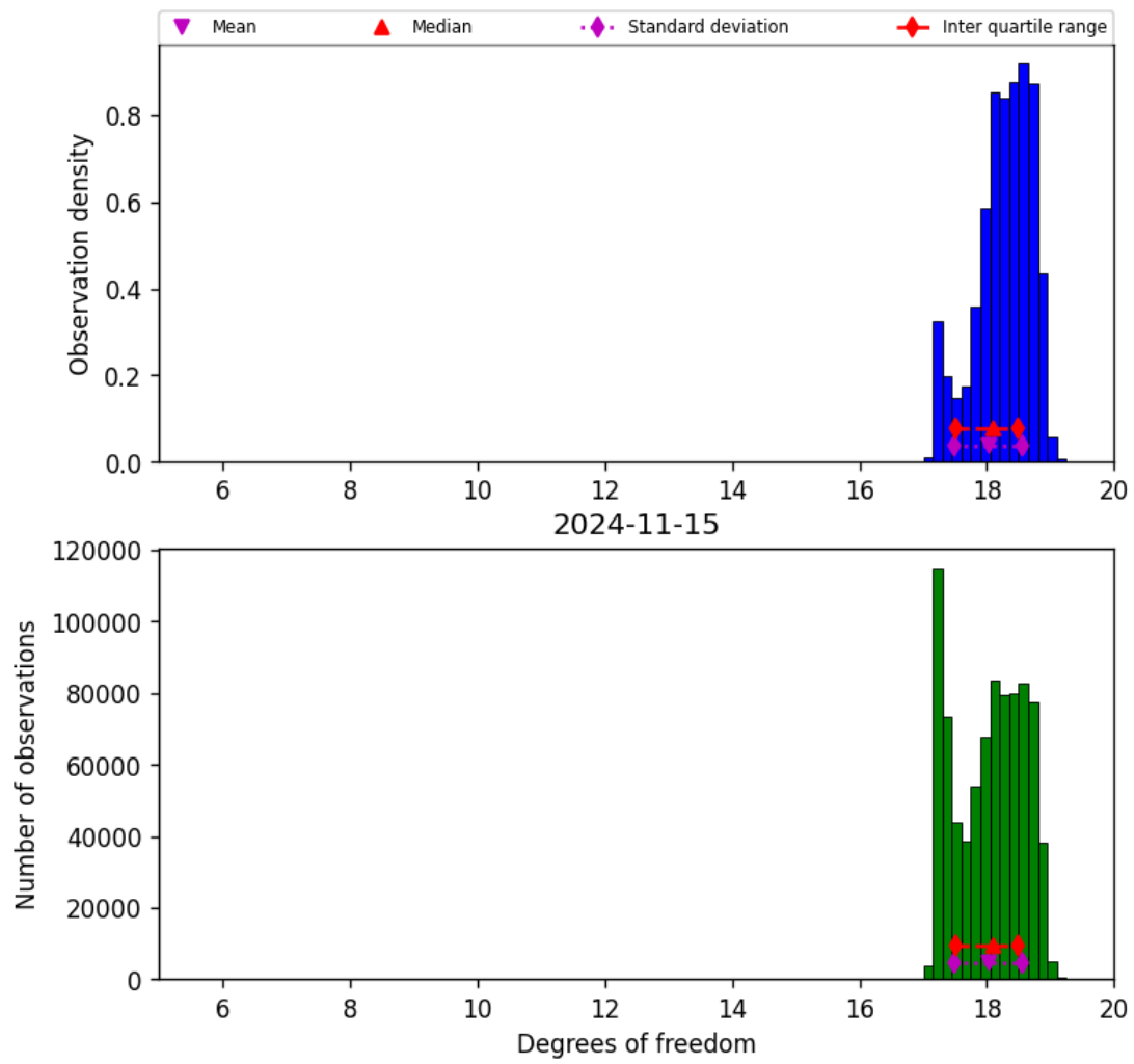
Figure 30: Histogram of “Degrees of freedom” for 2024-11-14 to 2024-11-16
