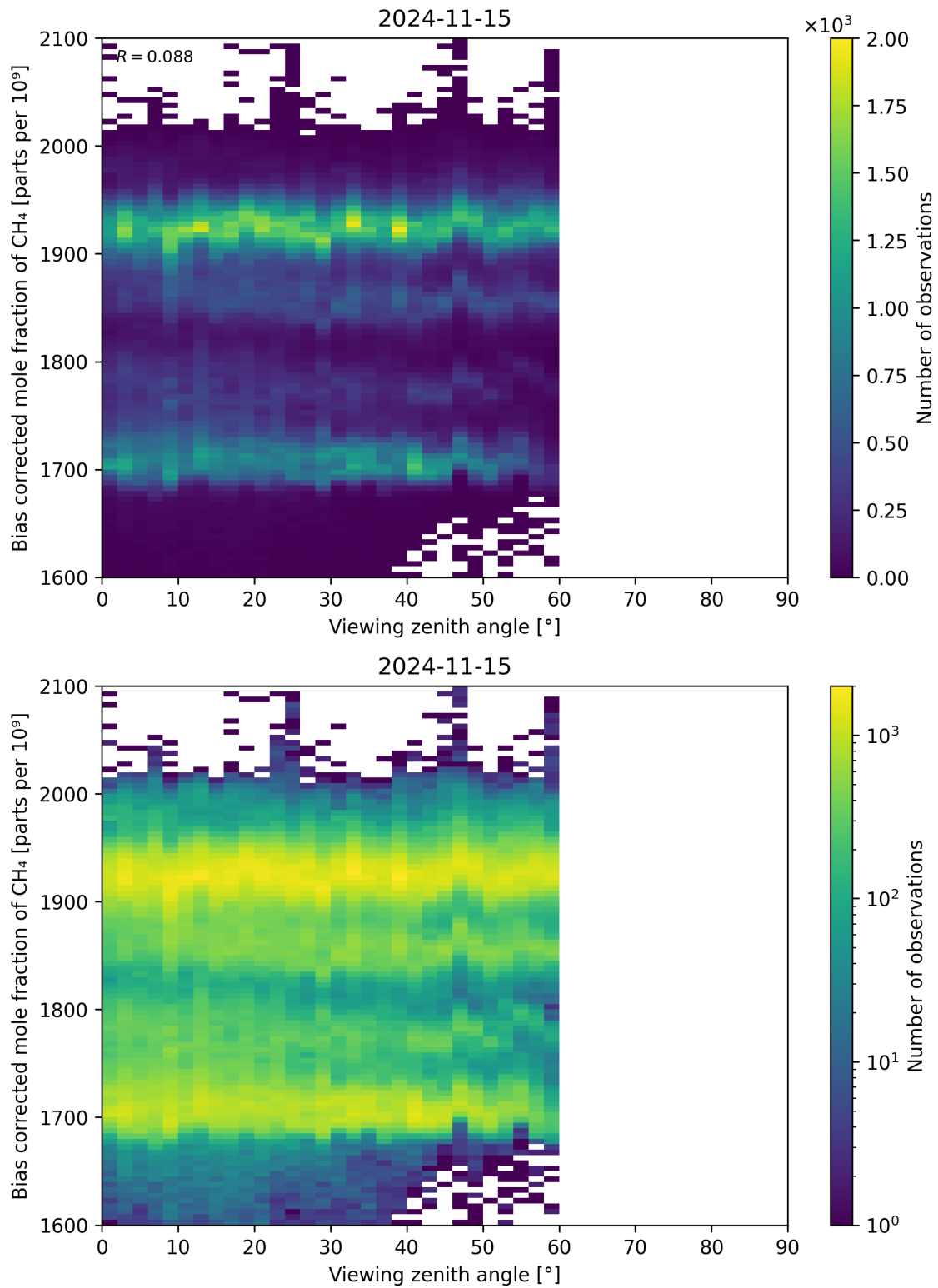
Figure 111: Scatter density plot of “Viewing zenith angle” against “Bias corrected mole fraction of CH 4 ” for 2024-11-14 to 2024-11-16.
