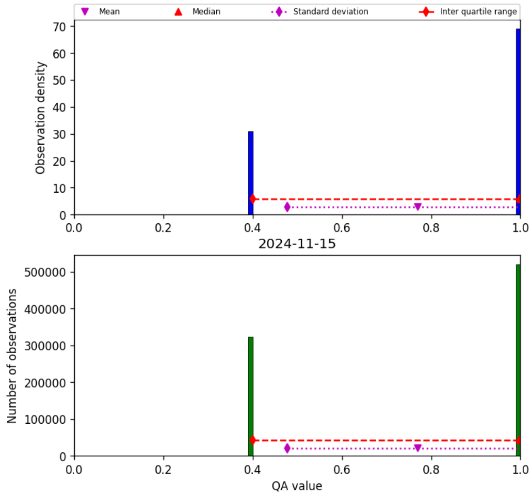
Figure 22: Histogram of “QA value” for 2024-11-14 to 2024-11-16
