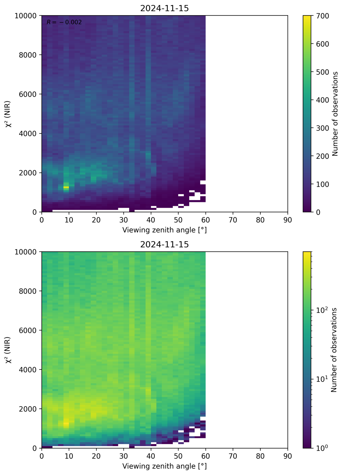
Figure 105: Scatter density plot of “Viewing zenith angle” against “ \chi^2 (NIR)” for 2024-11-14 to 2024-11-16.
