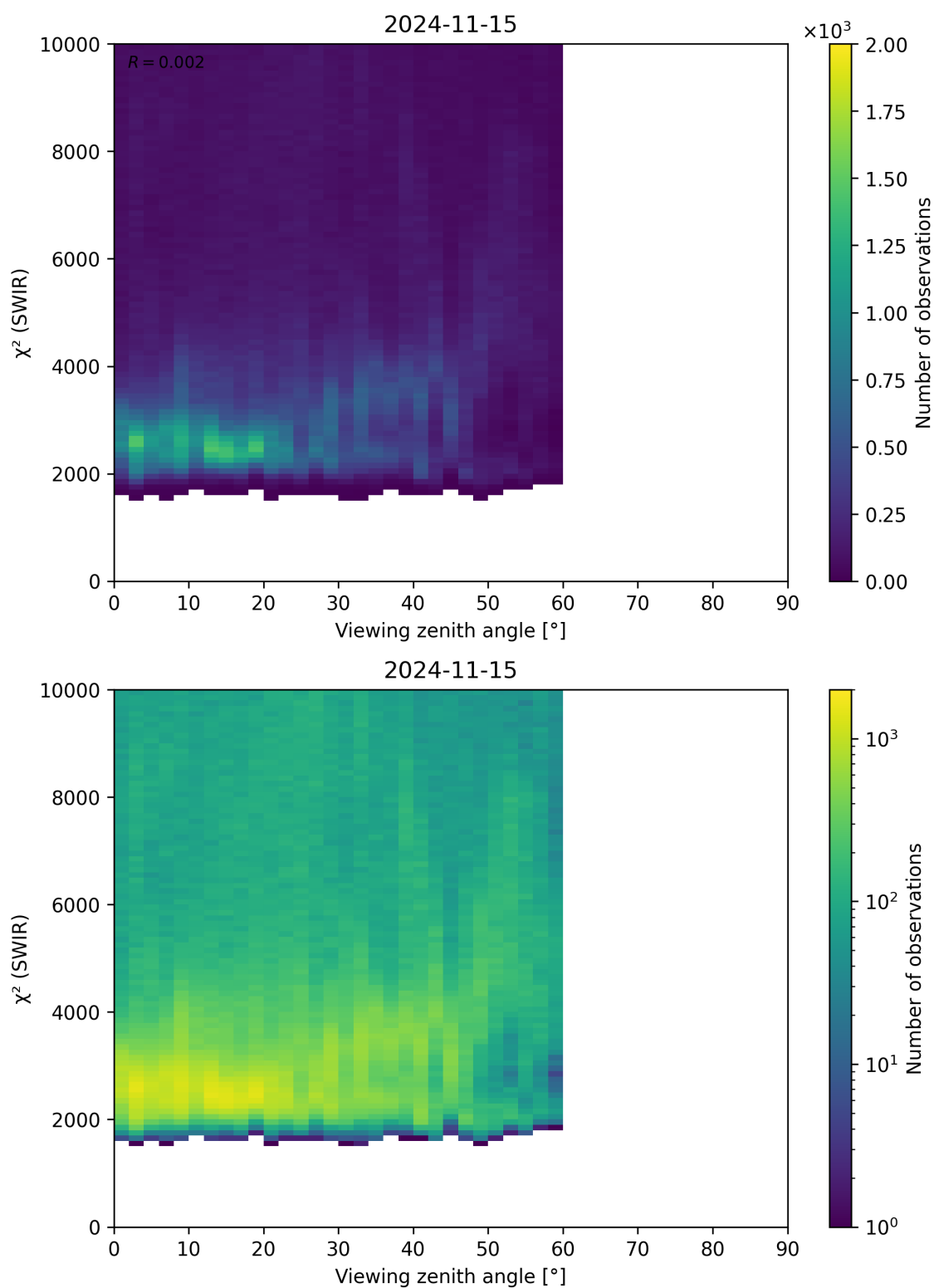
Figure 106: Scatter density plot of “Viewing zenith angle” against “ \chi^2 (SWIR)” for 2024-11-14 to 2024-11-16.
