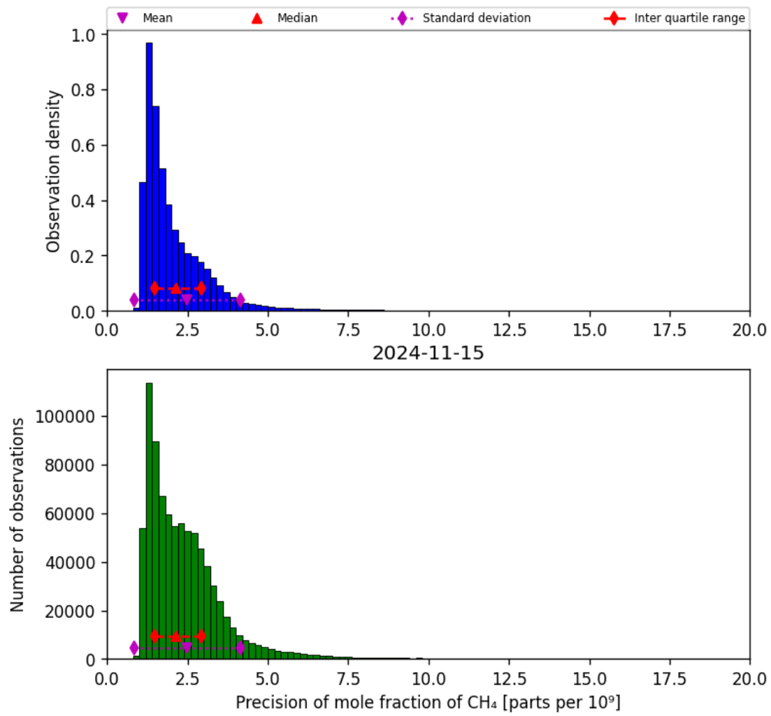
Figure 24: Histogram of “Precision of mole fraction of CH 4 ” for 2024-11-14 to 2024-11-16
