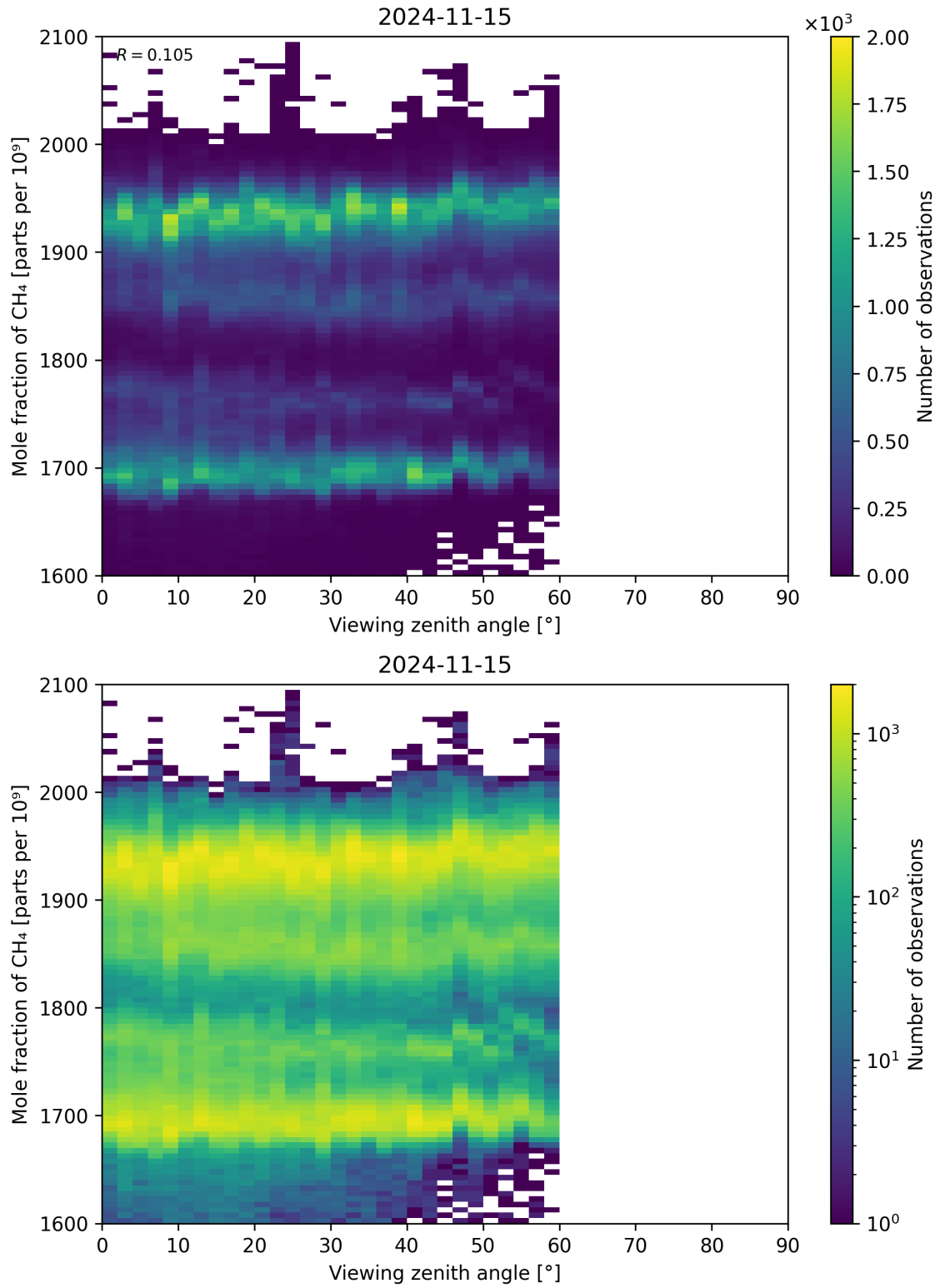
Figure 110: Scatter density plot of “Viewing zenith angle” against “Mole fraction of CH 4 ” for 2024-11-14 to 2024-11-16.
