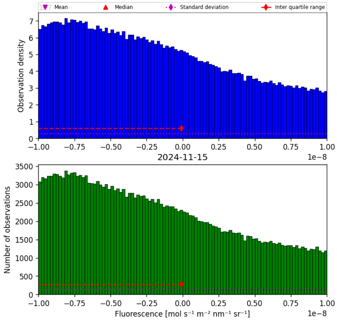
Figure 32: Histogram of “Fluorescence” for 2024-11-14 to 2024-11-16
