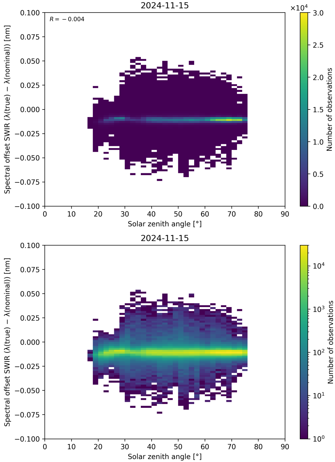
Figure 104: Scatter density plot of “Solar zenith angle” against “Spectral offset SWIR ( \lambda_{\text{true}} - \lambda_{\text{nominal}} )” for 2024-11-14 to 2024-11-16.
