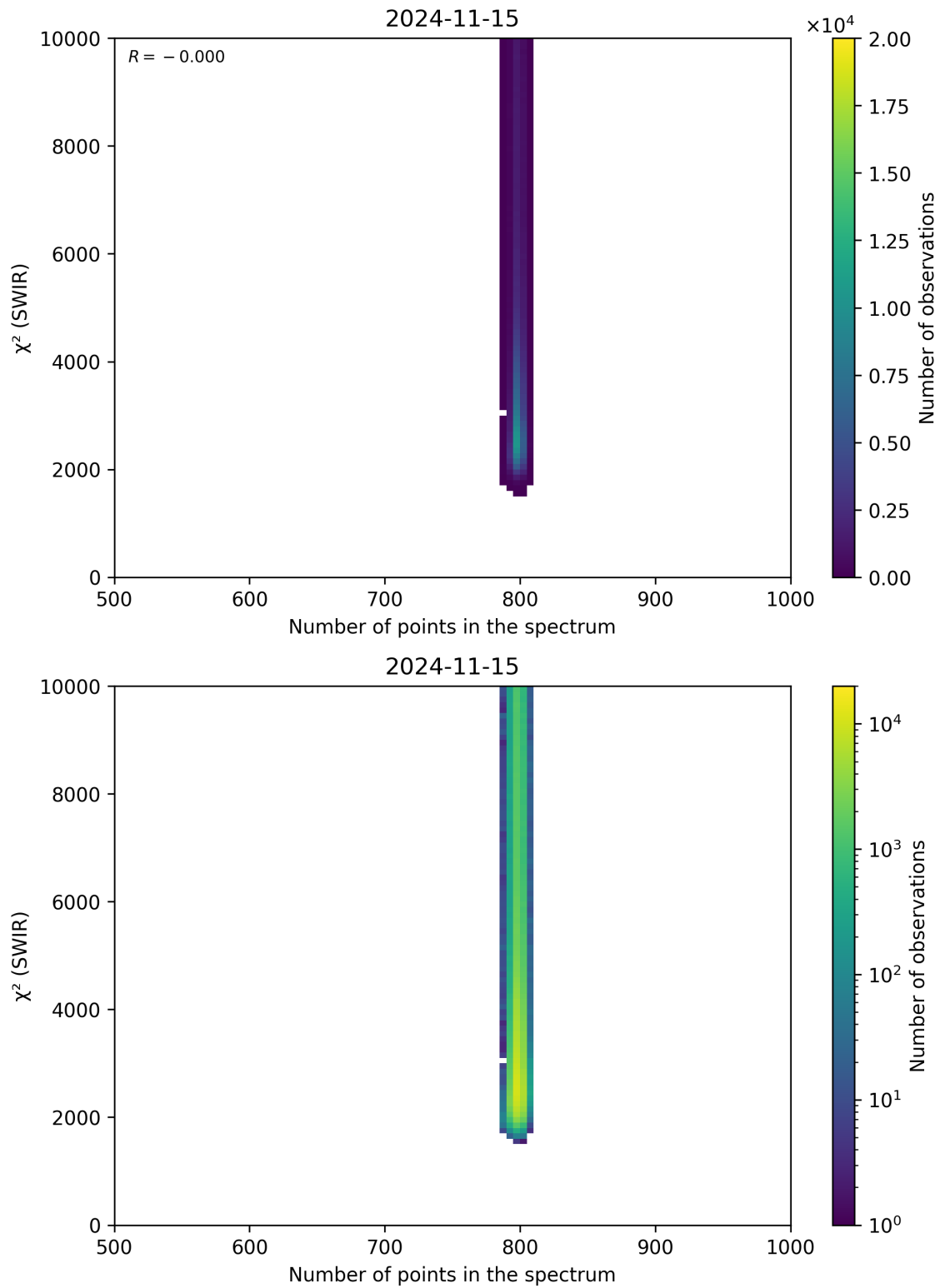
Figure 89: Scatter density plot of “Number of points in the spectrum” against “ \chi^2 (SWIR)” for 2024-11-14 to 2024-11-16.
