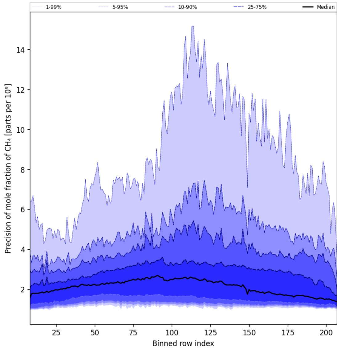
Figure 35: Along track statistics of “Precision of mole fraction of CH 4 ” for 2024-11-14 to 2024-11-16
