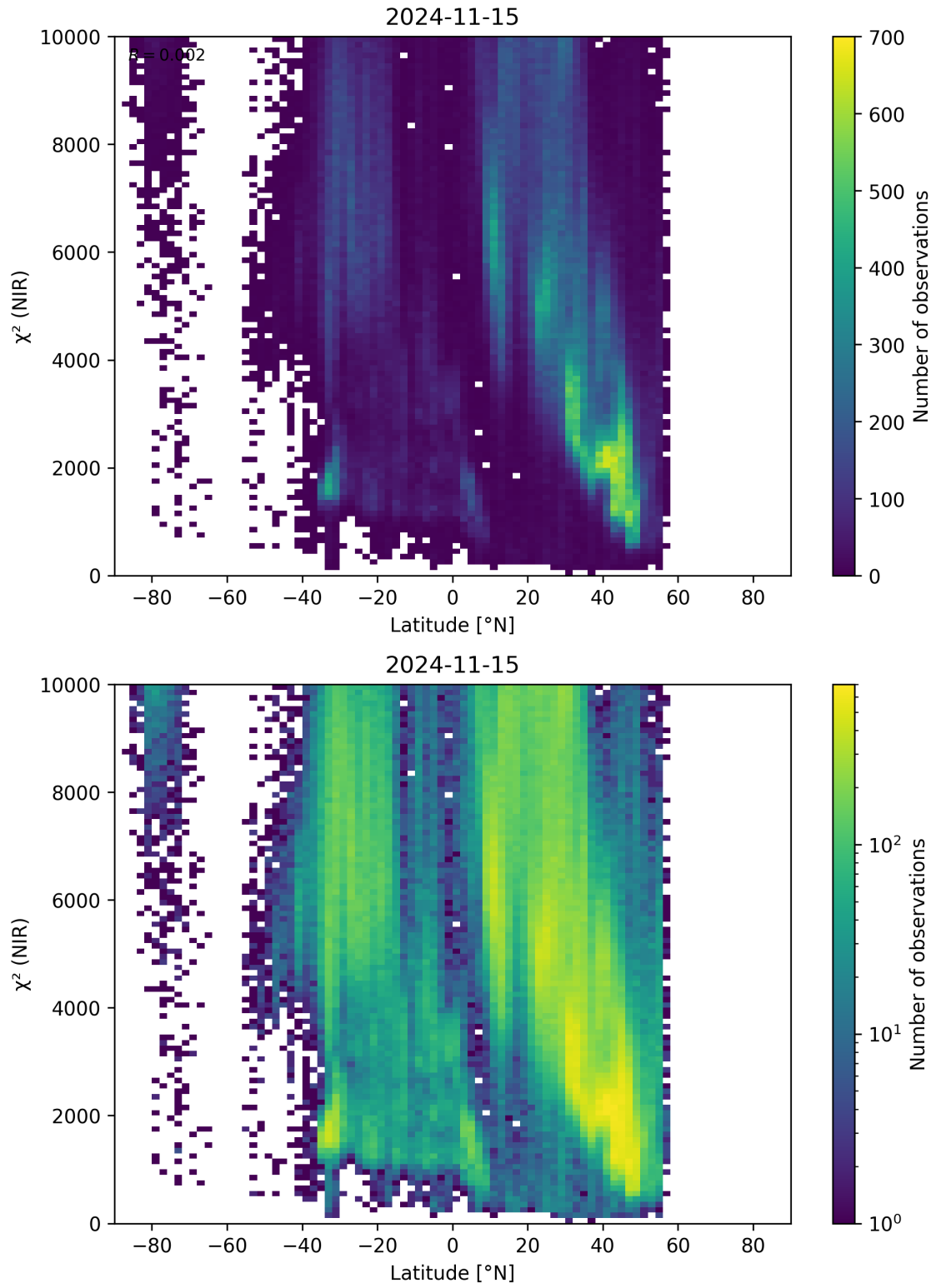
Figure 53: Scatter density plot of “Latitude” against “ \chi^2 (NIR)” for 2024-11-14 to 2024-11-16.
