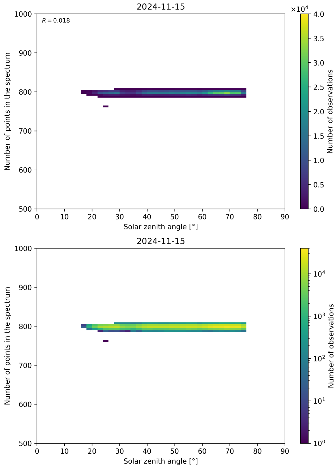
Figure 103: Scatter density plot of “Solar zenith angle” against “Number of points in the spectrum” for 2024-11-14 to 2024-11-16.
