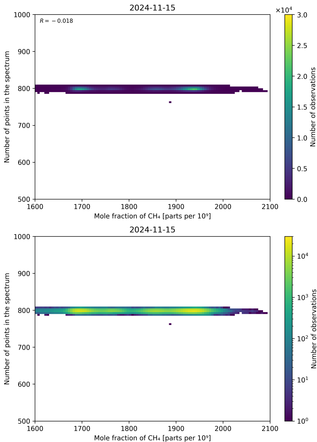
Figure 77: Scatter density plot of “Mole fraction of CH 4 ” against “Number of points in the spectrum” for 2024-11-14 to 2024-11-16.
