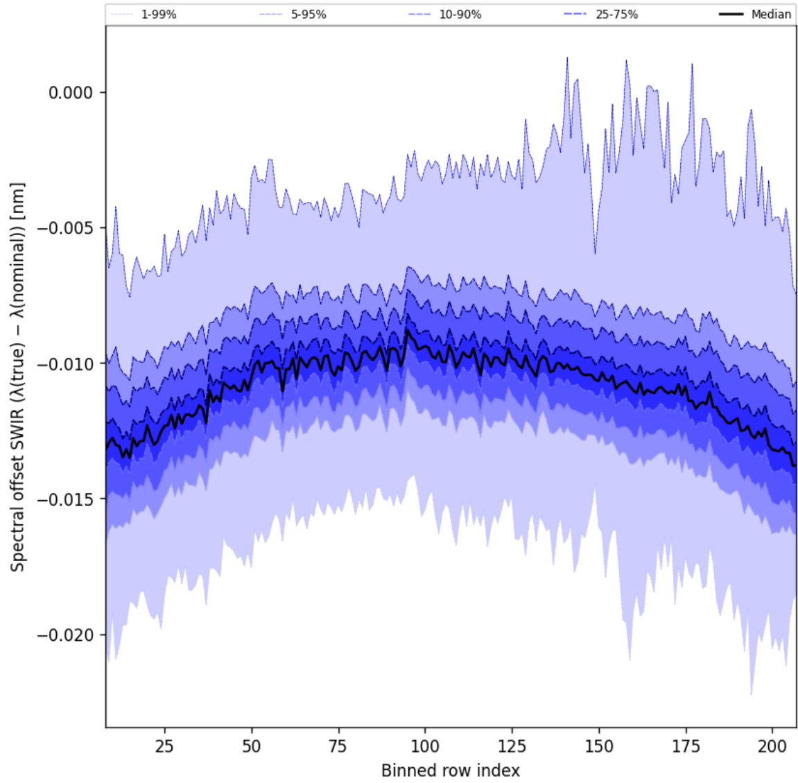
Figure 38: Along track statistics of “Spectral offset SWIR ( \lambda_{\text{true}} - \lambda_{\text{nominal}} )” for 2024-11-14 to 2024-11-16
