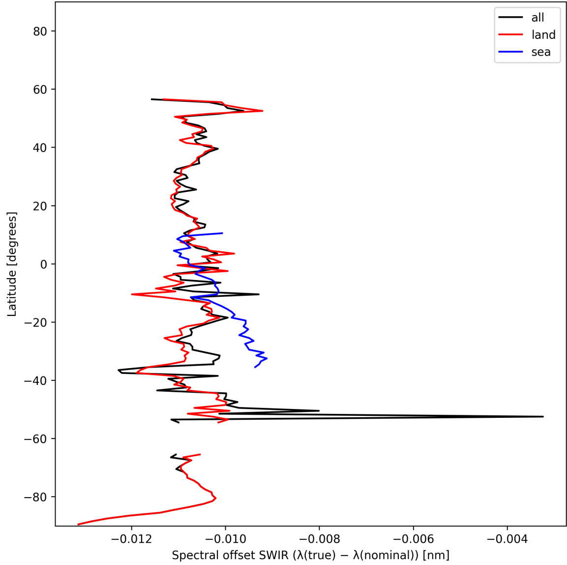
Figure 16: Zonal average of “Spectral offset SWIR ( \lambda_{\text{true}} - \lambda_{\text{nominal}} )” for 2024-11-14 to 2024-11-16.
