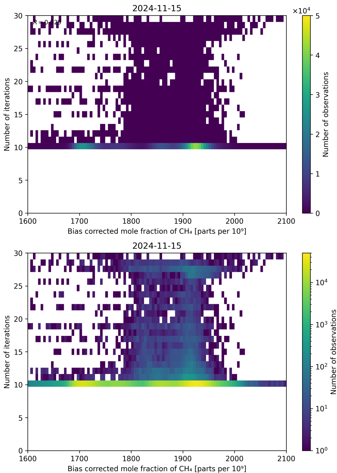
Figure 67: Scatter density plot of “Bias corrected mole fraction of \text{CH}_4 ” against “Number of iterations” for 2024-11-14 to 2024-11-16.
