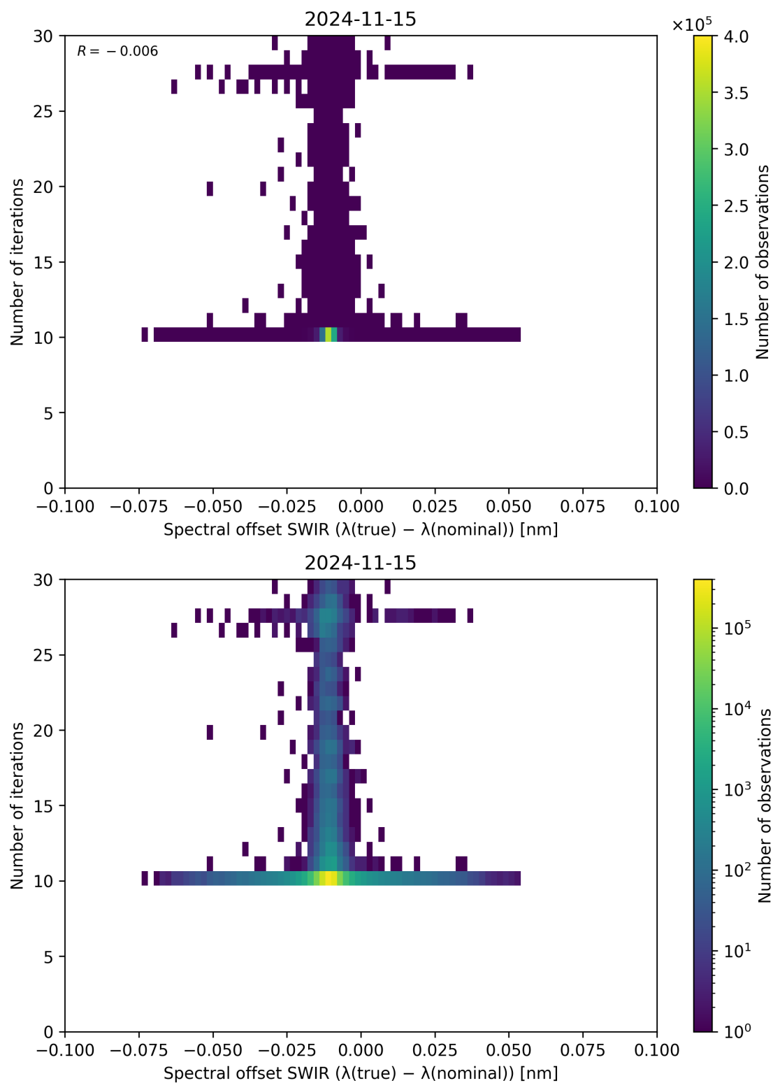
Figure 121: Scatter density plot of “Spectral offset SWIR ( \lambda_{\text{true}} - \lambda_{\text{nominal}} )” against “Number of iterations” for 2024-11-14 to 2024-11-16.
