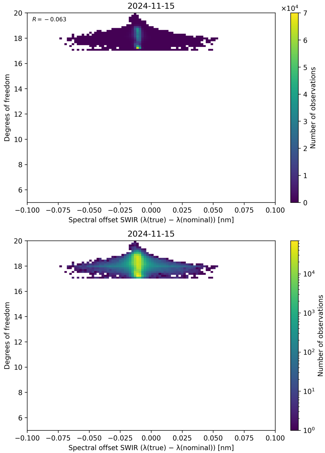
Figure 119: Scatter density plot of “Spectral offset SWIR ( \lambda_{\text{true}} - \lambda_{\text{nominal}} )” against “Degrees of freedom” for 2024-11-14 to 2024-11-16.
