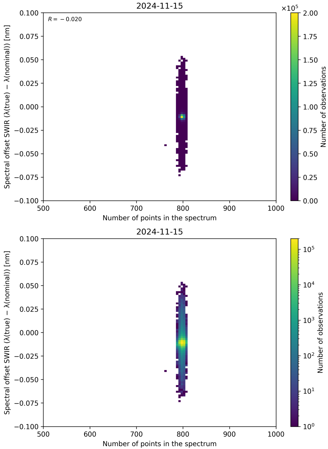
Figure 93: Scatter density plot of “Number of points in the spectrum” against “Spectral offset SWIR ( \lambda_{\text{true}} - \lambda_{\text{nominal}} )” for 2024-11-14 to 2024-11-16.
