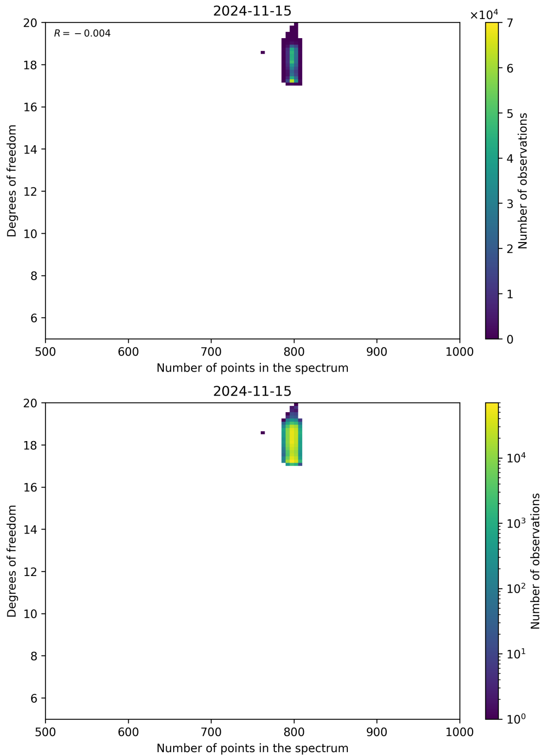
Figure 90: Scatter density plot of “Number of points in the spectrum” against “Degrees of freedom” for 2024-11-14 to 2024-11-16.
