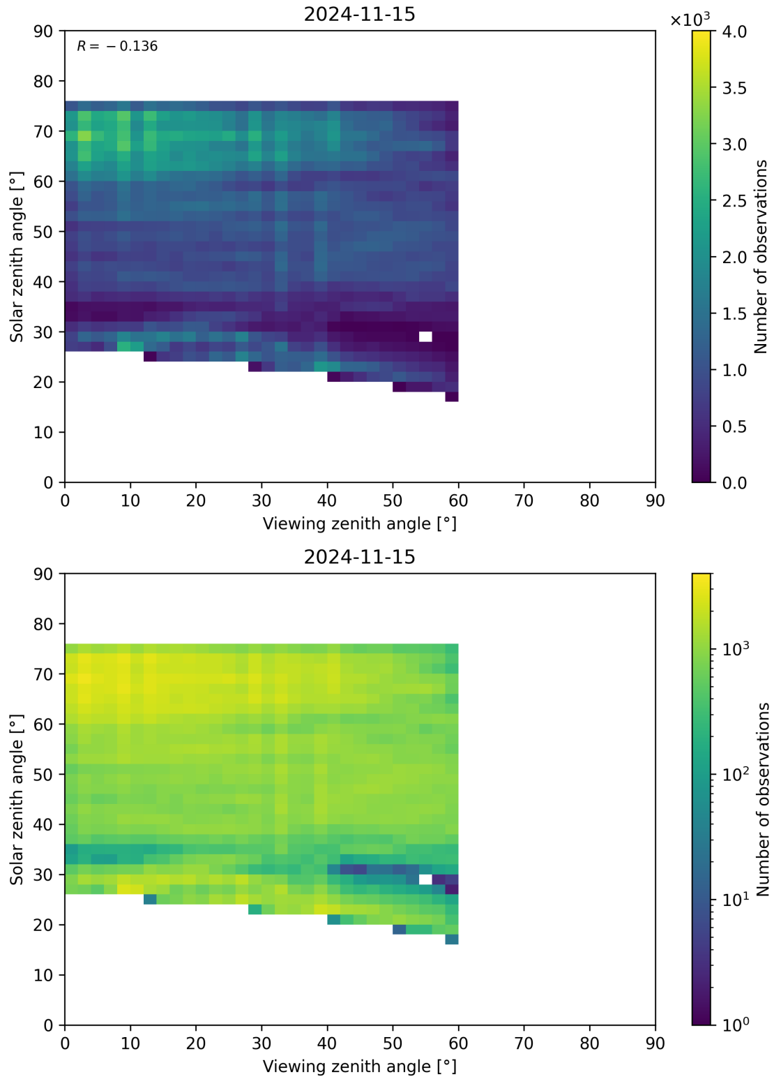
Figure 115: Scatter density plot of “Viewing zenith angle” against “Solar zenith angle” for 2024-11-14 to 2024-11-16.
