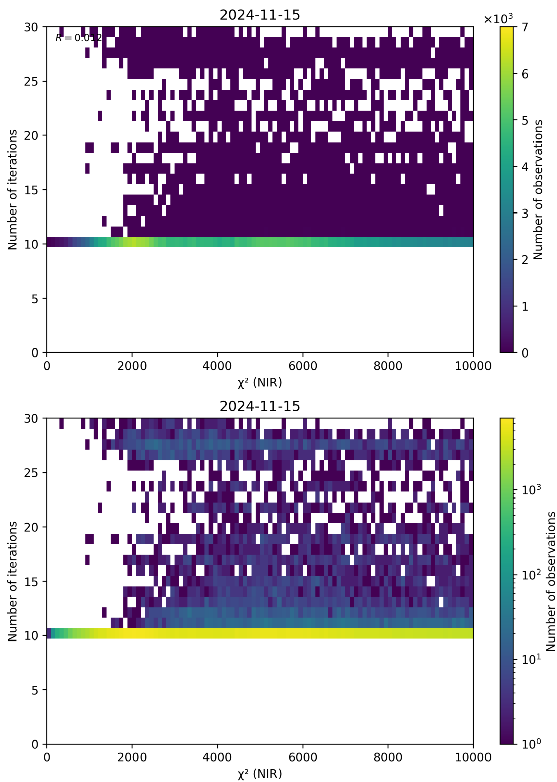
Figure 46: Scatter density plot of “ \chi^2 (NIR)” against “Number of iterations” for 2024-11-14 to 2024-11-16.
