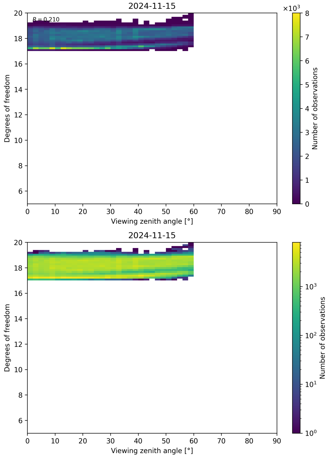
Figure 107: Scatter density plot of “Viewing zenith angle” against “Degrees of freedom” for 2024-11-14 to 2024-11-16.
