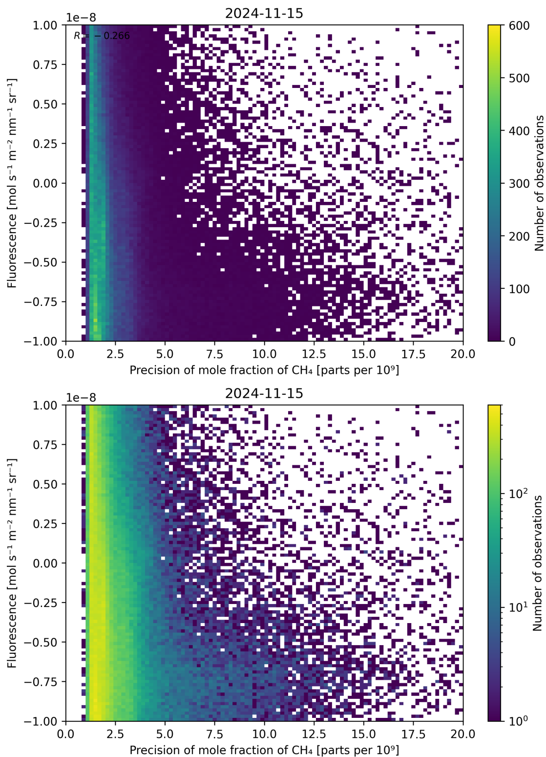
Figure 81: Scatter density plot of “Precision of mole fraction of \text{CH}_4 ” against “Fluorescence” for 2024-11-14 to 2024-11-16.
