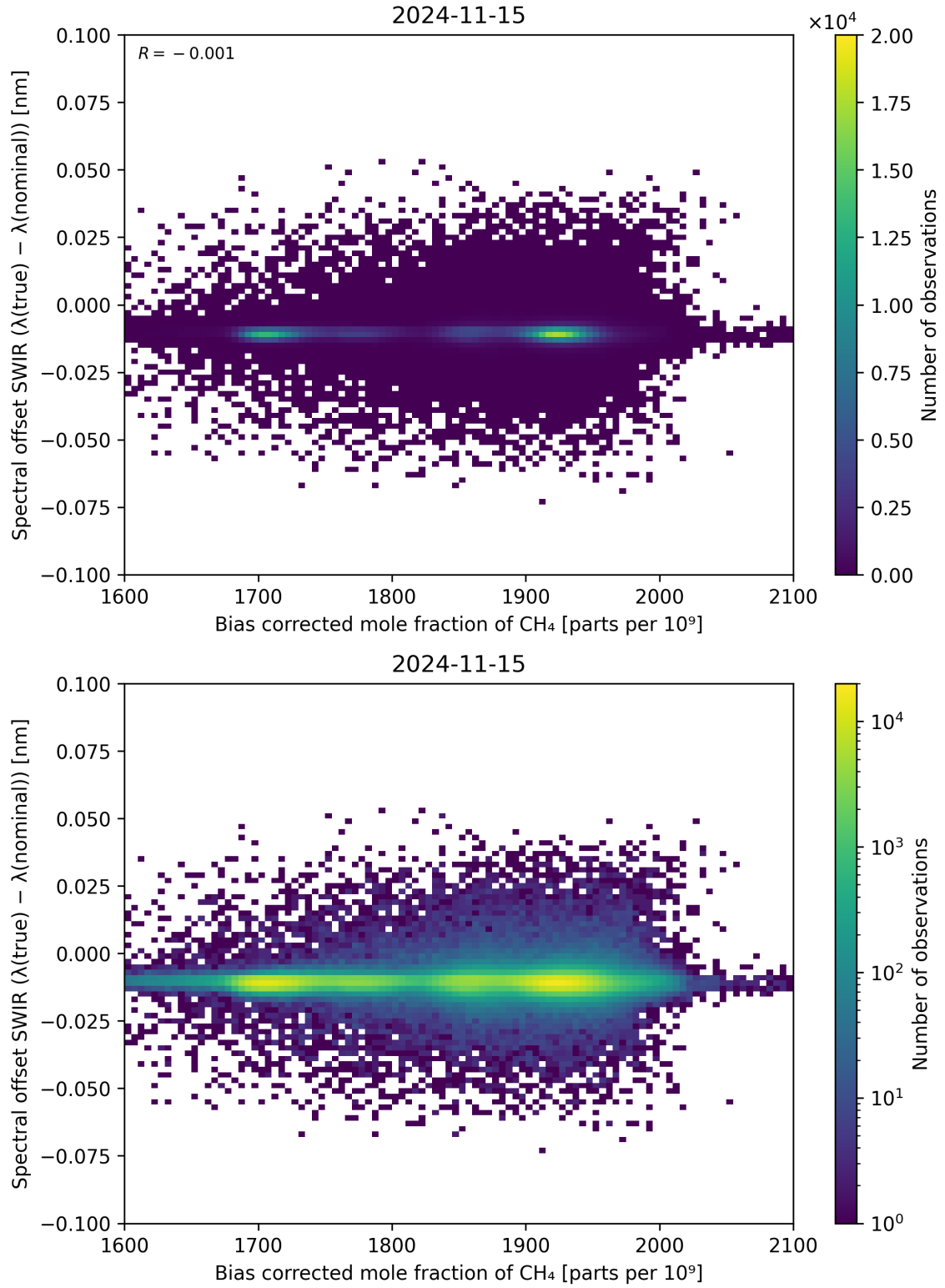
Figure 69: Scatter density plot of “Bias corrected mole fraction of \text{CH}_4 ” against “Spectral offset SWIR ( \lambda_{\text{true}} - \lambda_{\text{nominal}} )” for 2024-11-14 to 2024-11-16.
