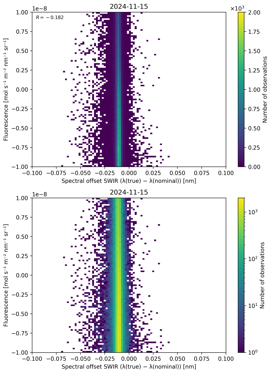
Figure 120: Scatter density plot of “Spectral offset SWIR ( \lambda_{\text{true}} - \lambda_{\text{nominal}} )” against “Fluorescence” for 2024-11-14 to 2024-11-16.
