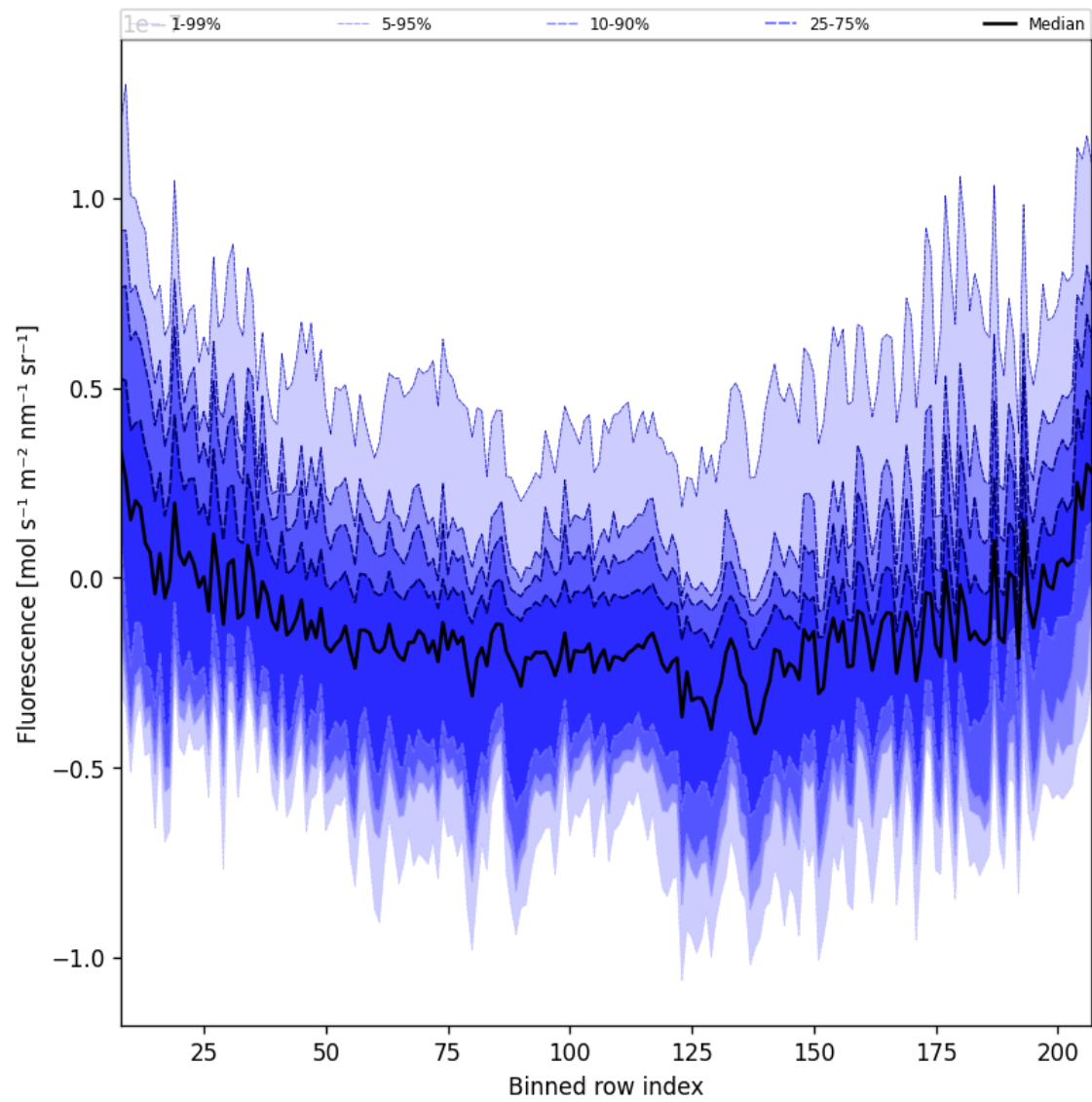
Figure 43: Along track statistics of “Fluorescence” for 2024-11-14 to 2024-11-16
