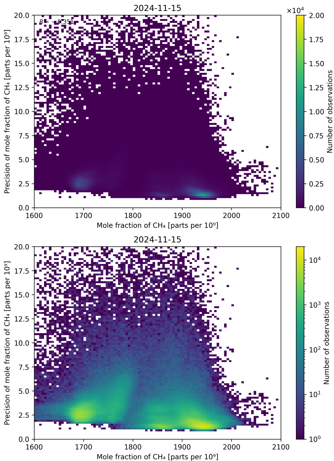
Figure 75: Scatter density plot of “Mole fraction of CH 4 ” against “Precision of mole fraction of CH 4 ” for 2024-11-14 to 2024-11-16.
