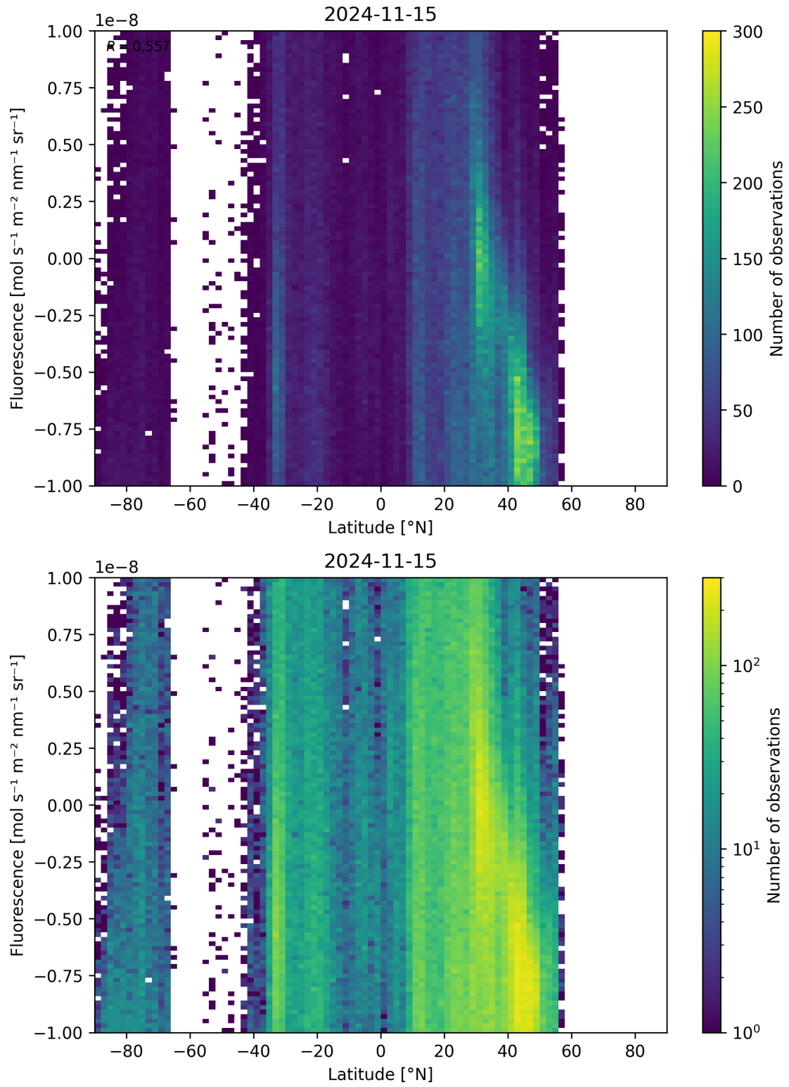
Figure 56: Scatter density plot of “Latitude” against “Fluorescence” for 2024-11-14 to 2024-11-16.
