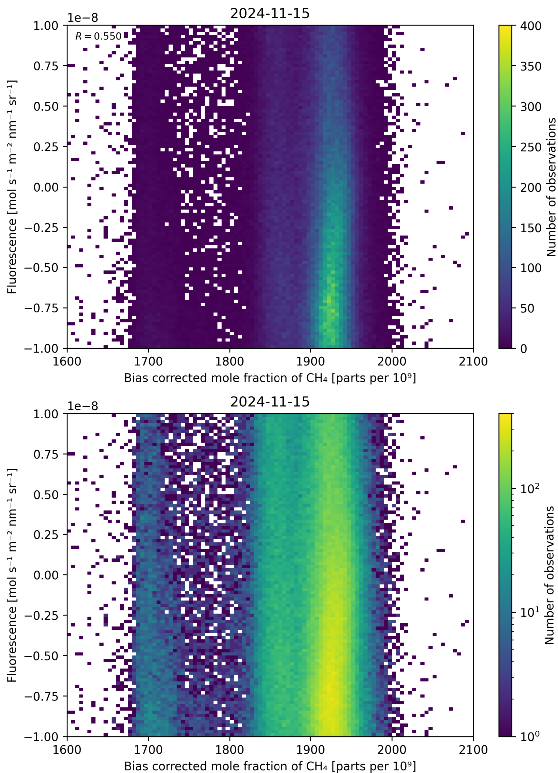
Figure 66: Scatter density plot of “Bias corrected mole fraction of \text{CH}_4 ” against “Fluorescence” for 2024-11-14 to 2024-11-16.
