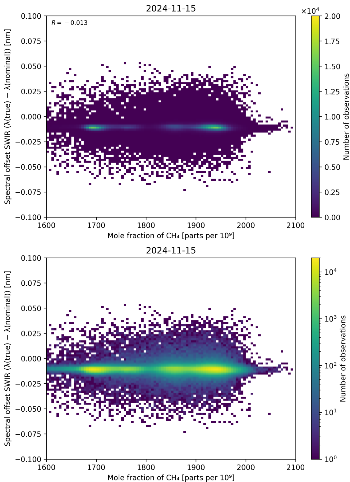
Figure 86: Scatter density plot of “Mole fraction of CH 4 ” against “Spectral offset SWIR ( \lambda_{\text{true}} - \lambda_{\text{nominal}} )” for 2024-11-14 to 2024-11-16.
