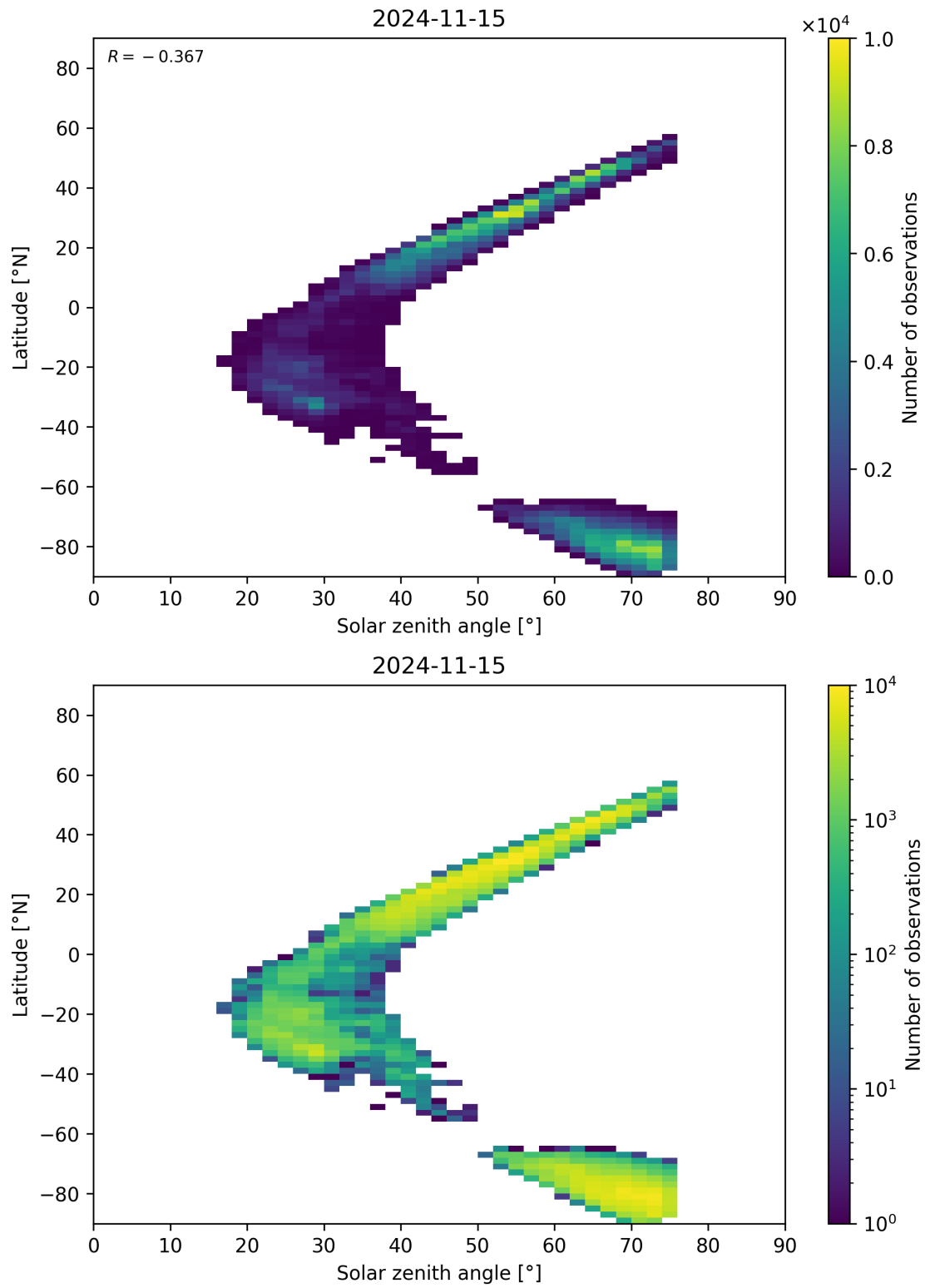
Figure 98: Scatter density plot of “Solar zenith angle” against “Latitude” for 2024-11-14 to 2024-11-16.
