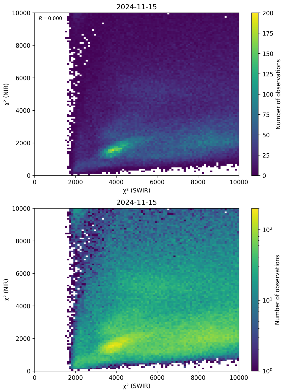
Figure 47: Scatter density plot of “ \chi^2 (SWIR)” against “ \chi^2 (NIR)” for 2024-11-14 to 2024-11-16.
