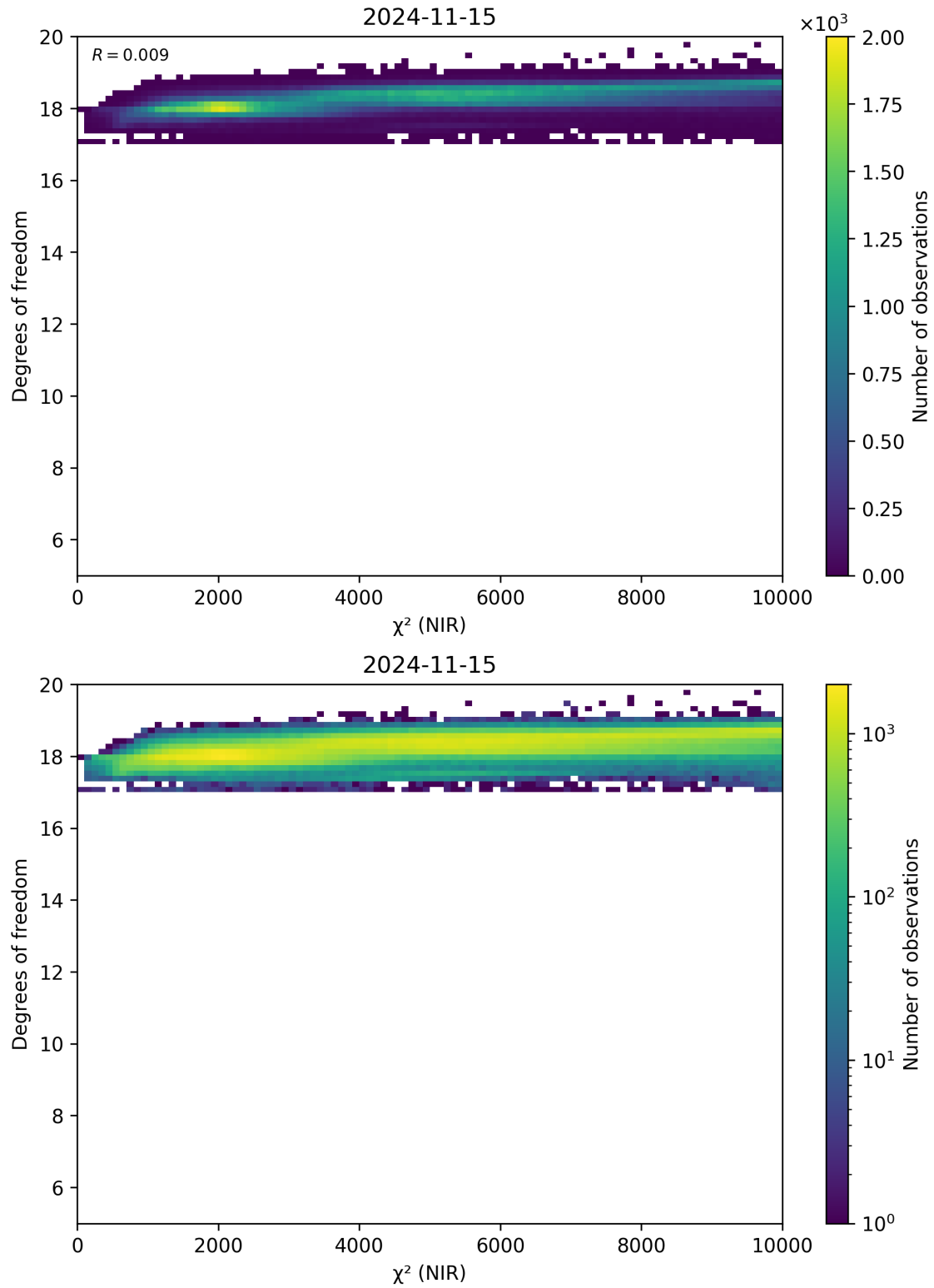
Figure 44: Scatter density plot of “ \chi^2 (NIR)” against “Degrees of freedom” for 2024-11-14 to 2024-11-16.
