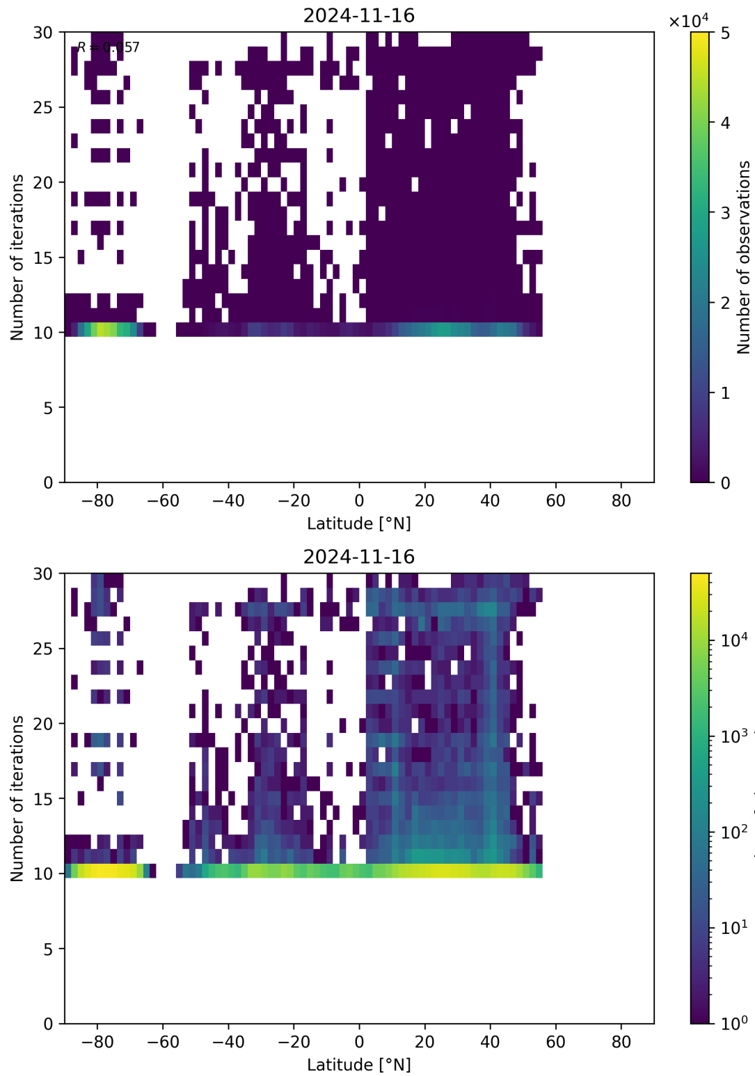
Figure 60: Scatter density plot of “Latitude” against “Number of iterations” for 2024-11-15 to 2024-11-17.
