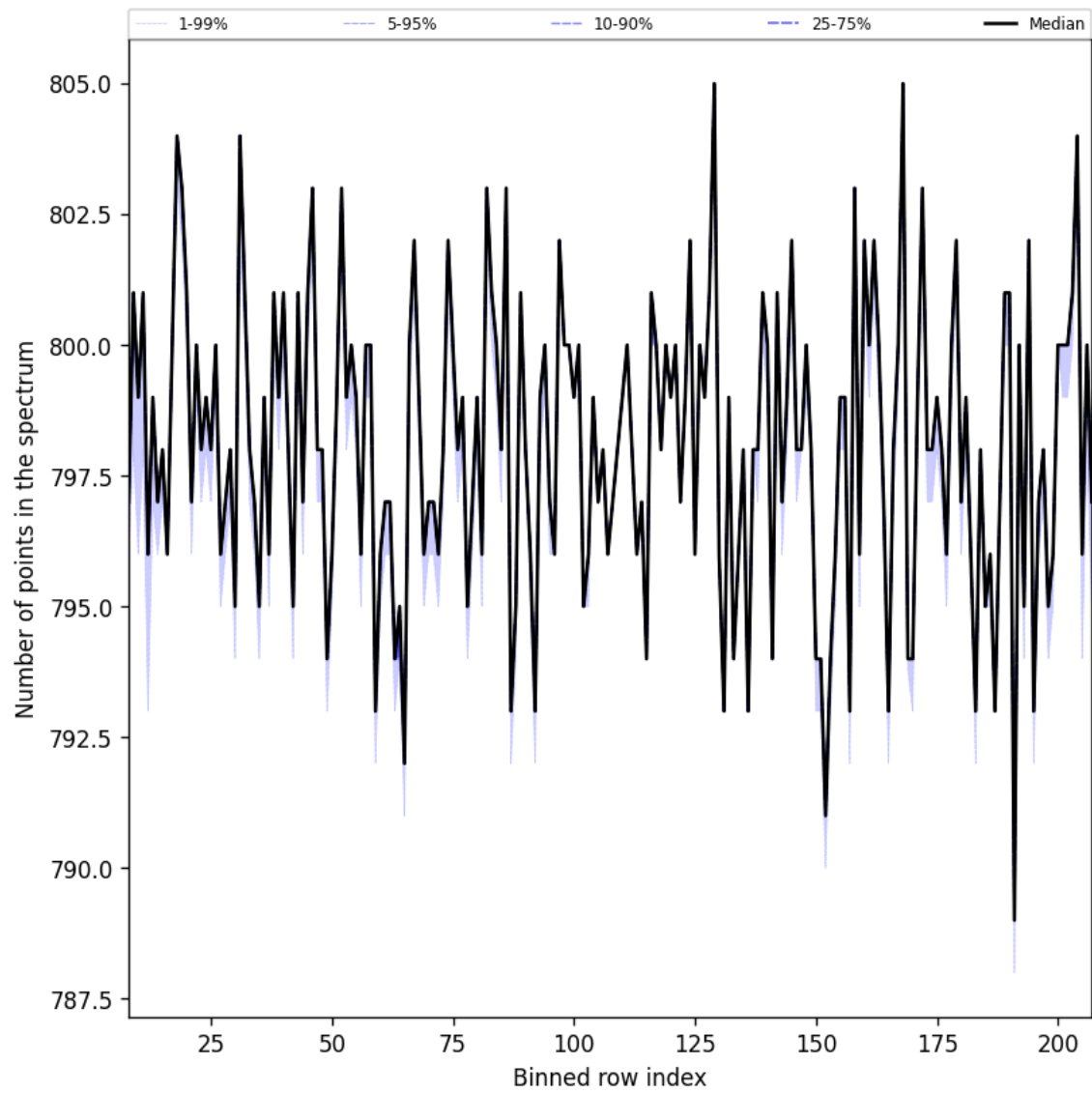
Figure 37: Along track statistics of “Number of points in the spectrum” for 2024-11-15 to 2024-11-17
