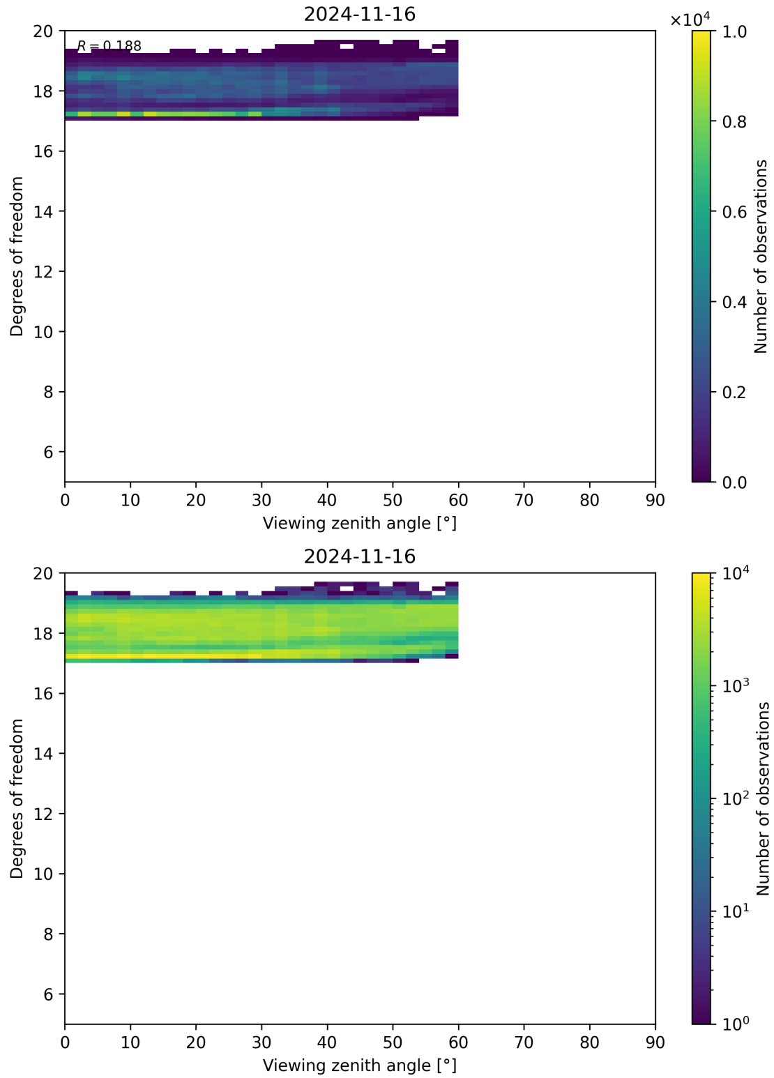
Figure 107: Scatter density plot of “Viewing zenith angle” against “Degrees of freedom” for 2024-11-15 to 2024-11-17.
