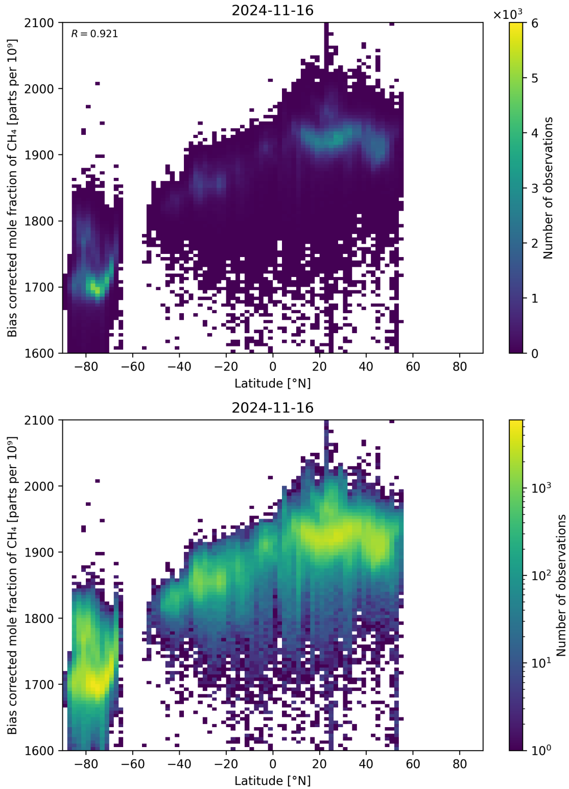
Figure 58: Scatter density plot of “Latitude” against “Bias corrected mole fraction of \text{CH}_4 ” for 2024-11-15 to 2024-11-17.
