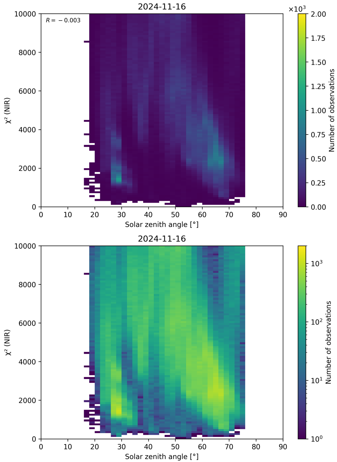
Figure 94: Scatter density plot of “Solar zenith angle” against “ \chi^2 (NIR)” for 2024-11-15 to 2024-11-17.
