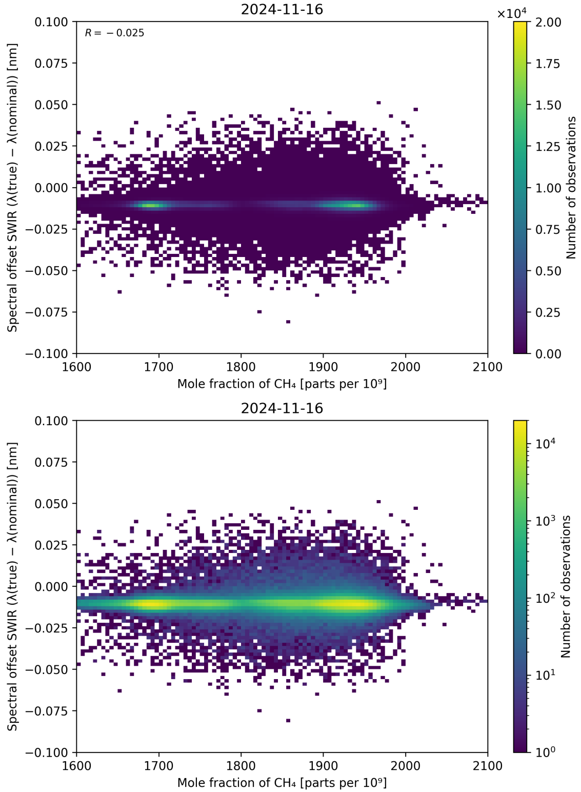
Figure 86: Scatter density plot of “Mole fraction of CH 4 ” against “Spectral offset SWIR ( \lambda_{\text{true}} - \lambda_{\text{nominal}} )” for 2024-11-15 to 2024-11-17.
