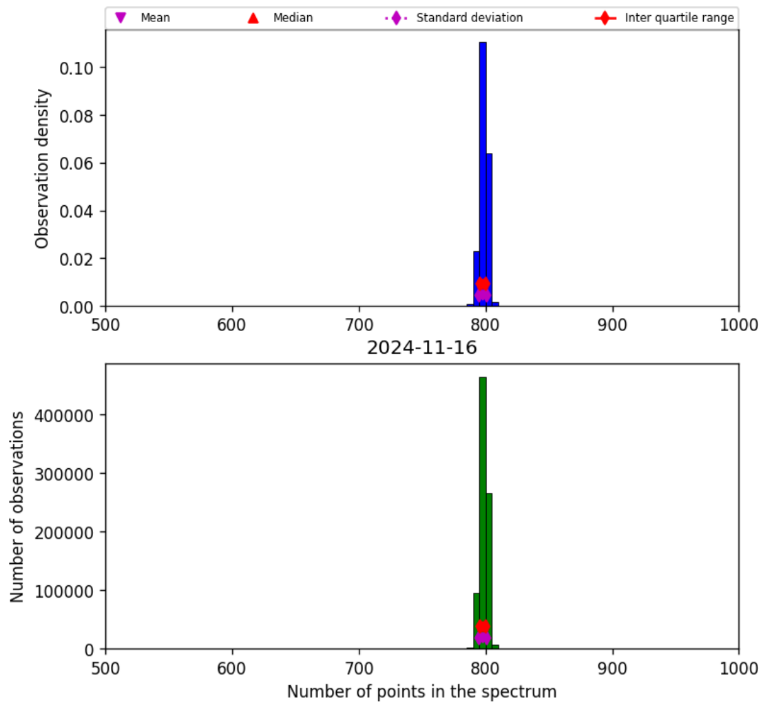
Figure 26: Histogram of “Number of points in the spectrum” for 2024-11-15 to 2024-11-17
