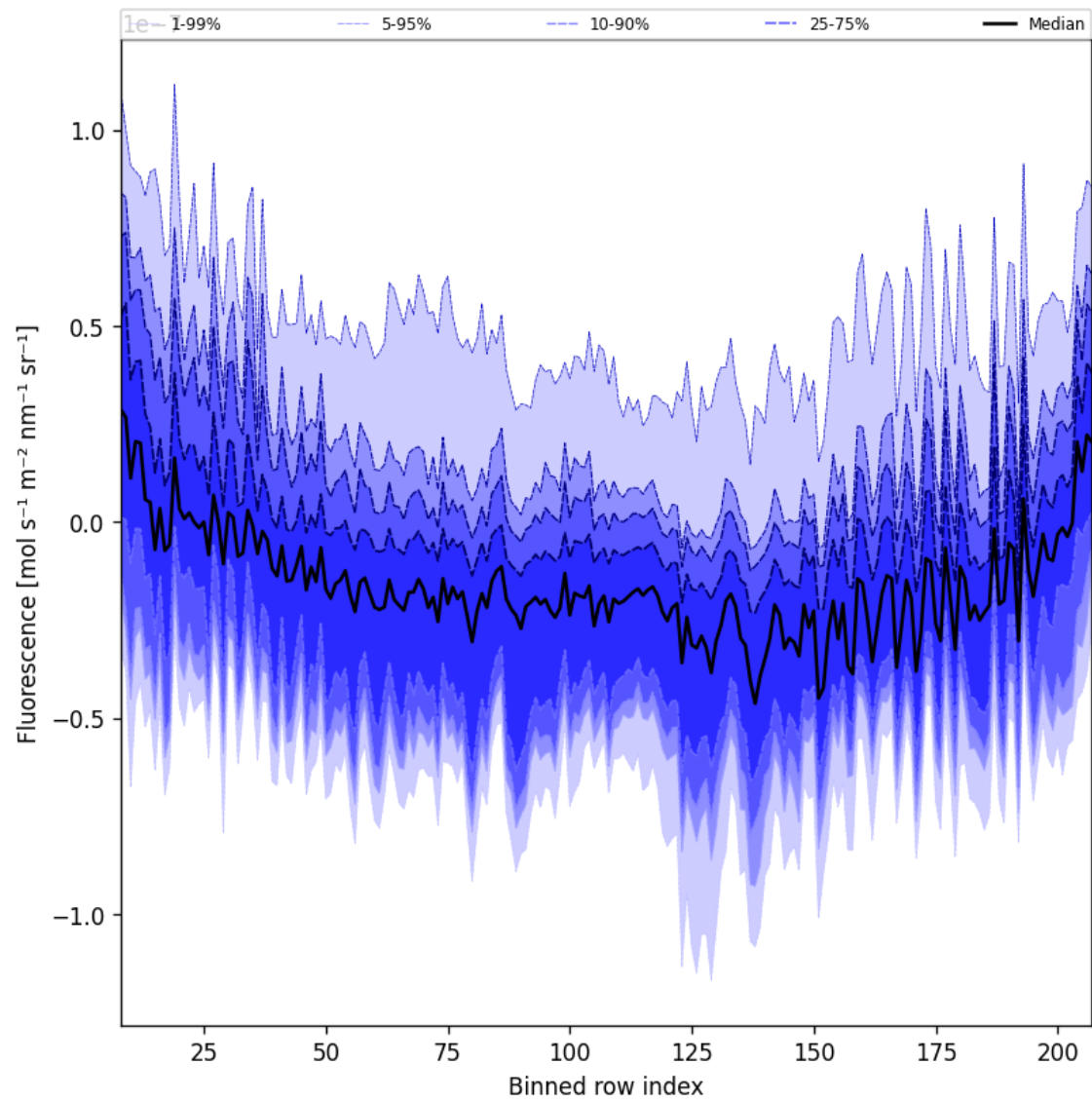
Figure 43: Along track statistics of “Fluorescence” for 2024-11-15 to 2024-11-17
