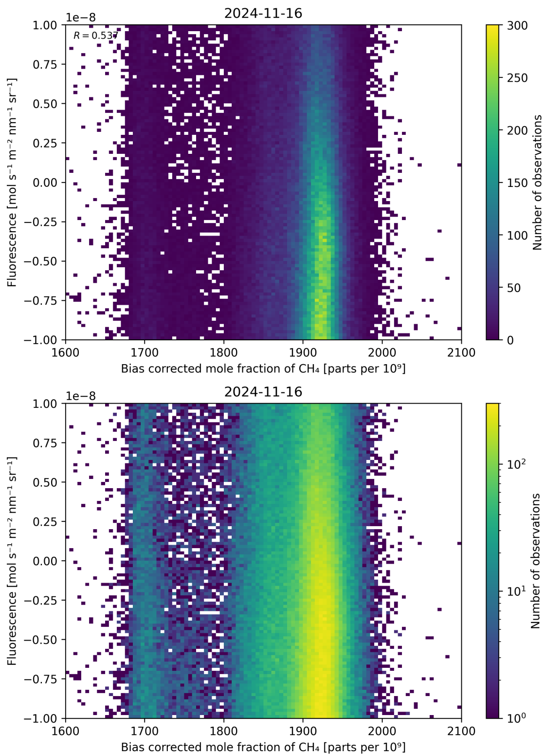
Figure 66: Scatter density plot of “Bias corrected mole fraction of \text{CH}_4 ” against “Fluorescence” for 2024-11-15 to 2024-11-17.
