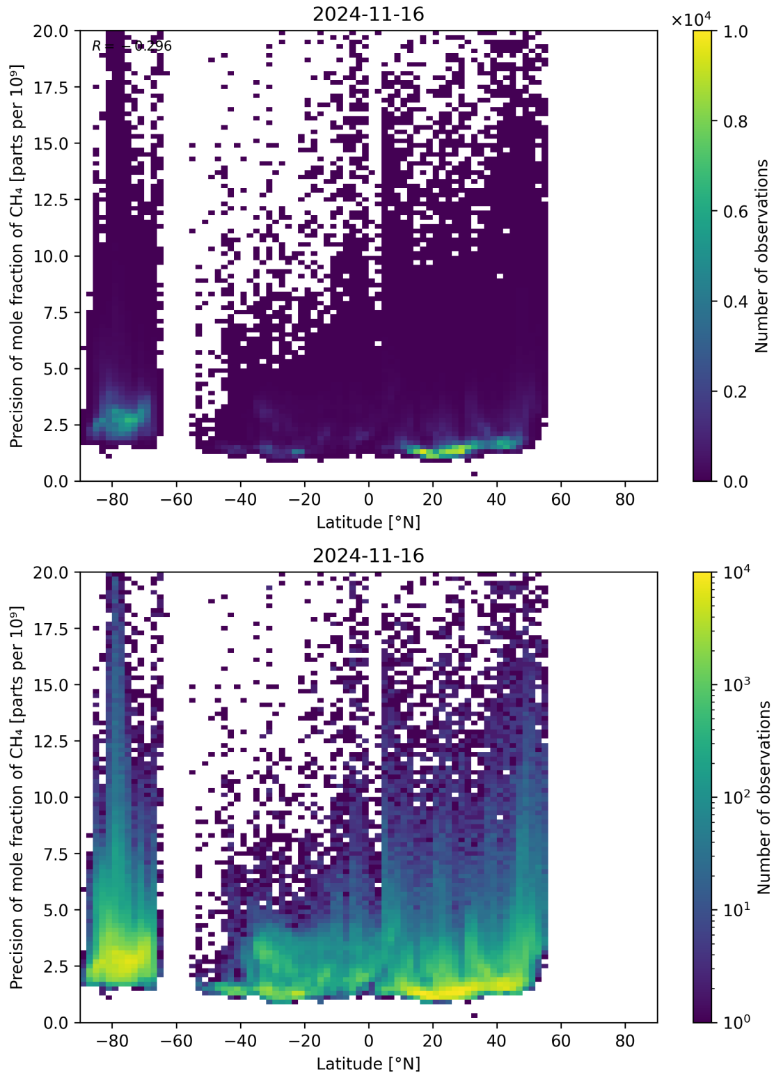
Figure 59: Scatter density plot of “Latitude” against “Precision of mole fraction of CH 4 ” for 2024-11-15 to 2024-11-17.
