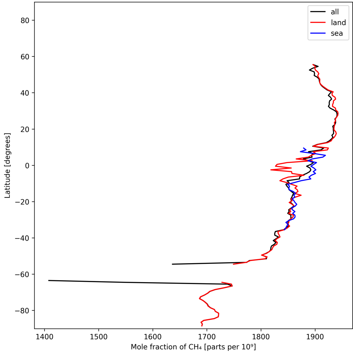
Figure 12: Zonal average of “Mole fraction of \text{CH}_4 ” for 2024-11-15 to 2024-11-17.
