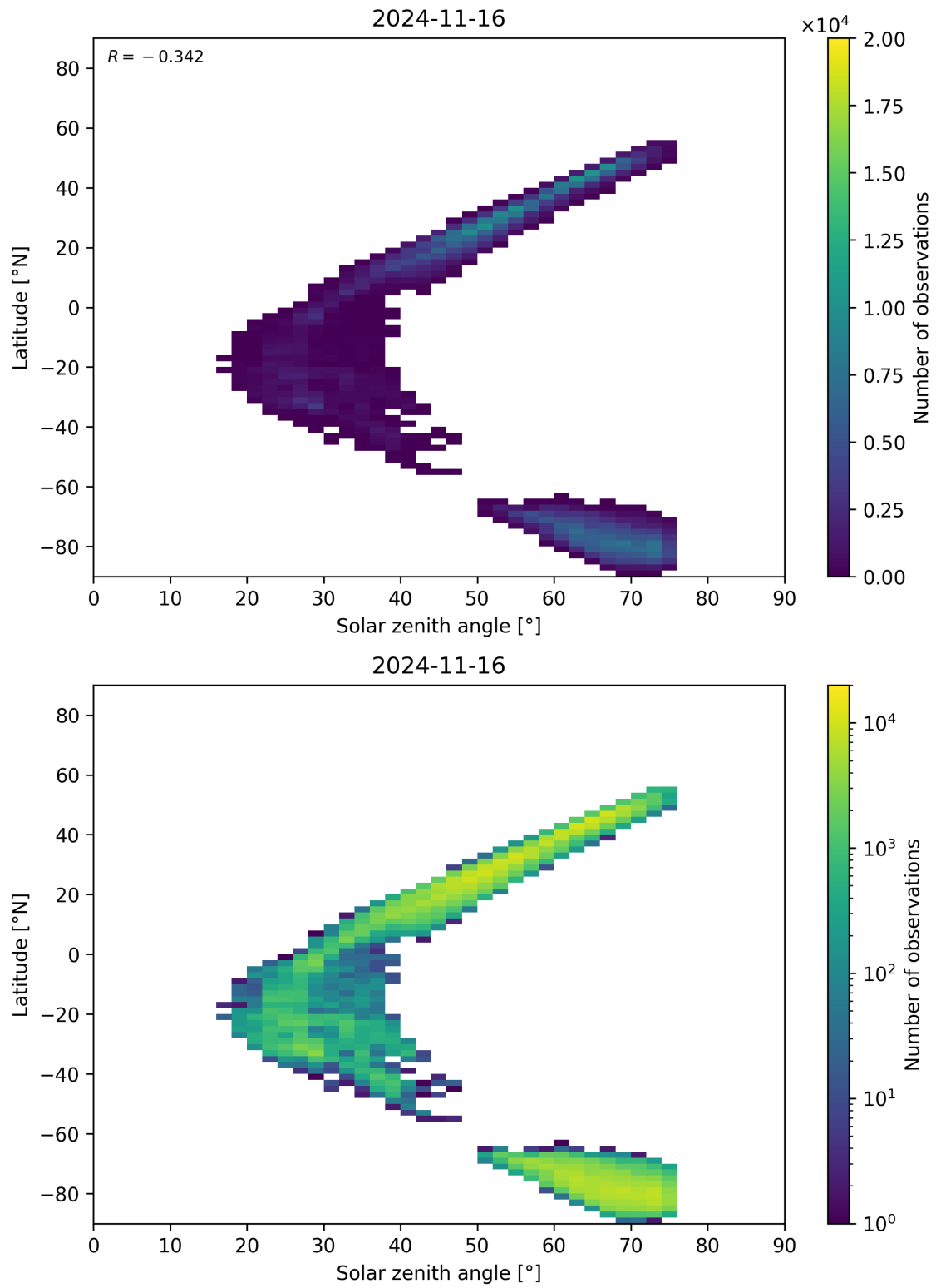
Figure 98: Scatter density plot of “Solar zenith angle” against “Latitude” for 2024-11-15 to 2024-11-17.
