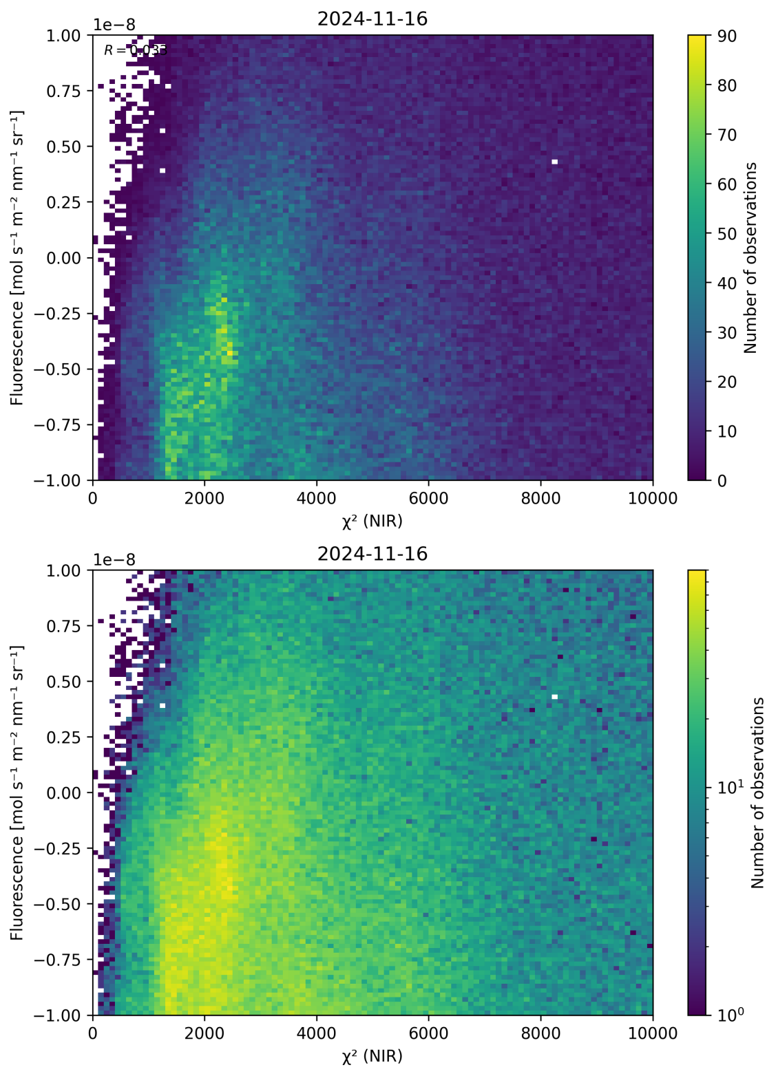
Figure 45: Scatter density plot of “ \chi^2 (NIR)” against “Fluorescence” for 2024-11-15 to 2024-11-17.
