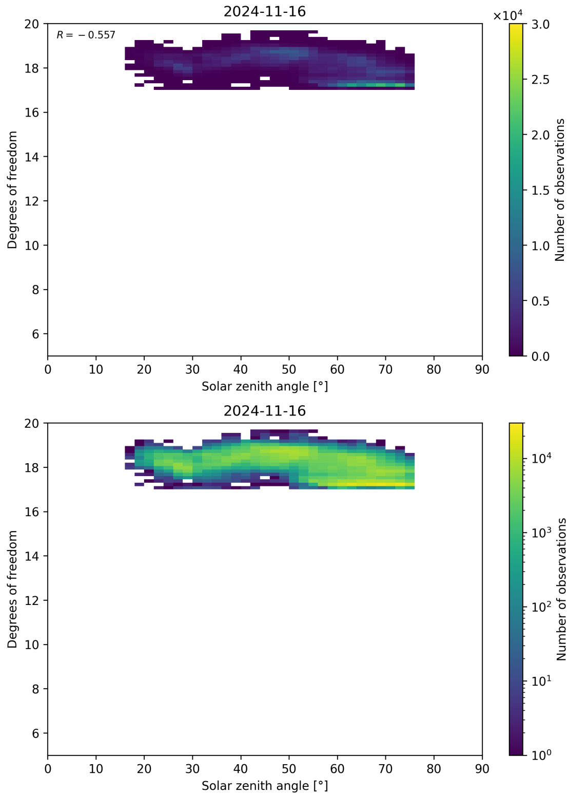
Figure 96: Scatter density plot of “Solar zenith angle” against “Degrees of freedom” for 2024-11-15 to 2024-11-17.
