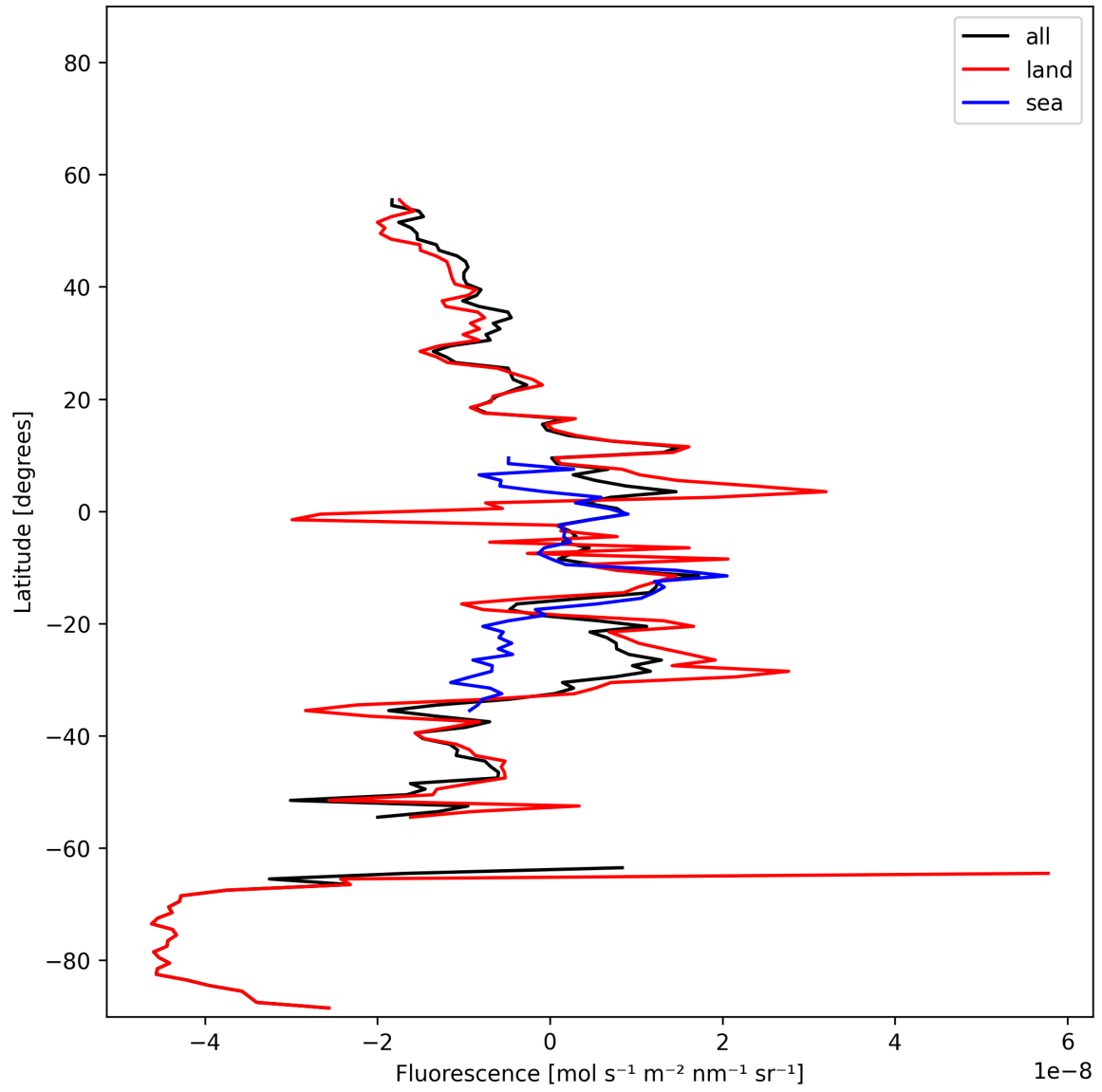
Figure 21: Zonal average of “Fluorescence” for 2024-11-15 to 2024-11-17.
