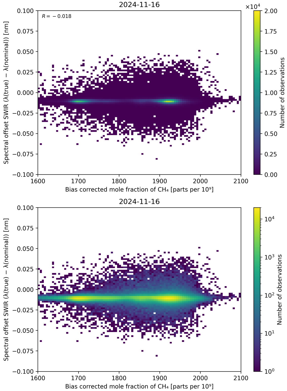
Figure 69: Scatter density plot of “Bias corrected mole fraction of \text{CH}_4 ” against “Spectral offset SWIR ( \lambda_{\text{true}} - \lambda_{\text{nominal}} )” for 2024-11-15 to 2024-11-17.
