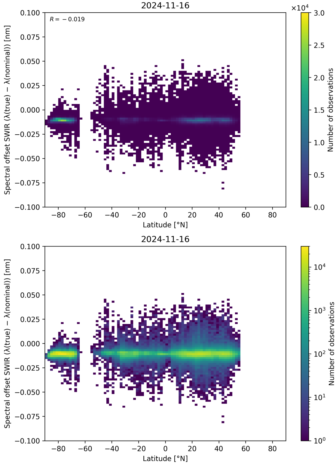
Figure 62: Scatter density plot of “Latitude” against “Spectral offset SWIR ( \lambda_{\text{true}} - \lambda_{\text{nominal}} )” for 2024-11-15 to 2024-11-17.
