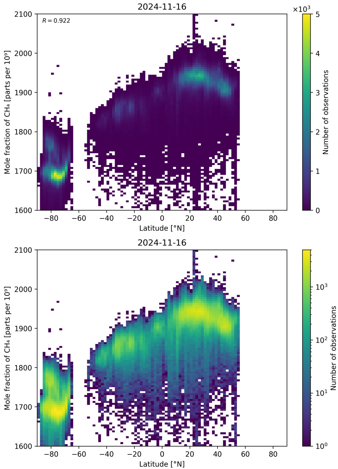
Figure 57: Scatter density plot of “Latitude” against “Mole fraction of \text{CH}_4 ” for 2024-11-15 to 2024-11-17.
