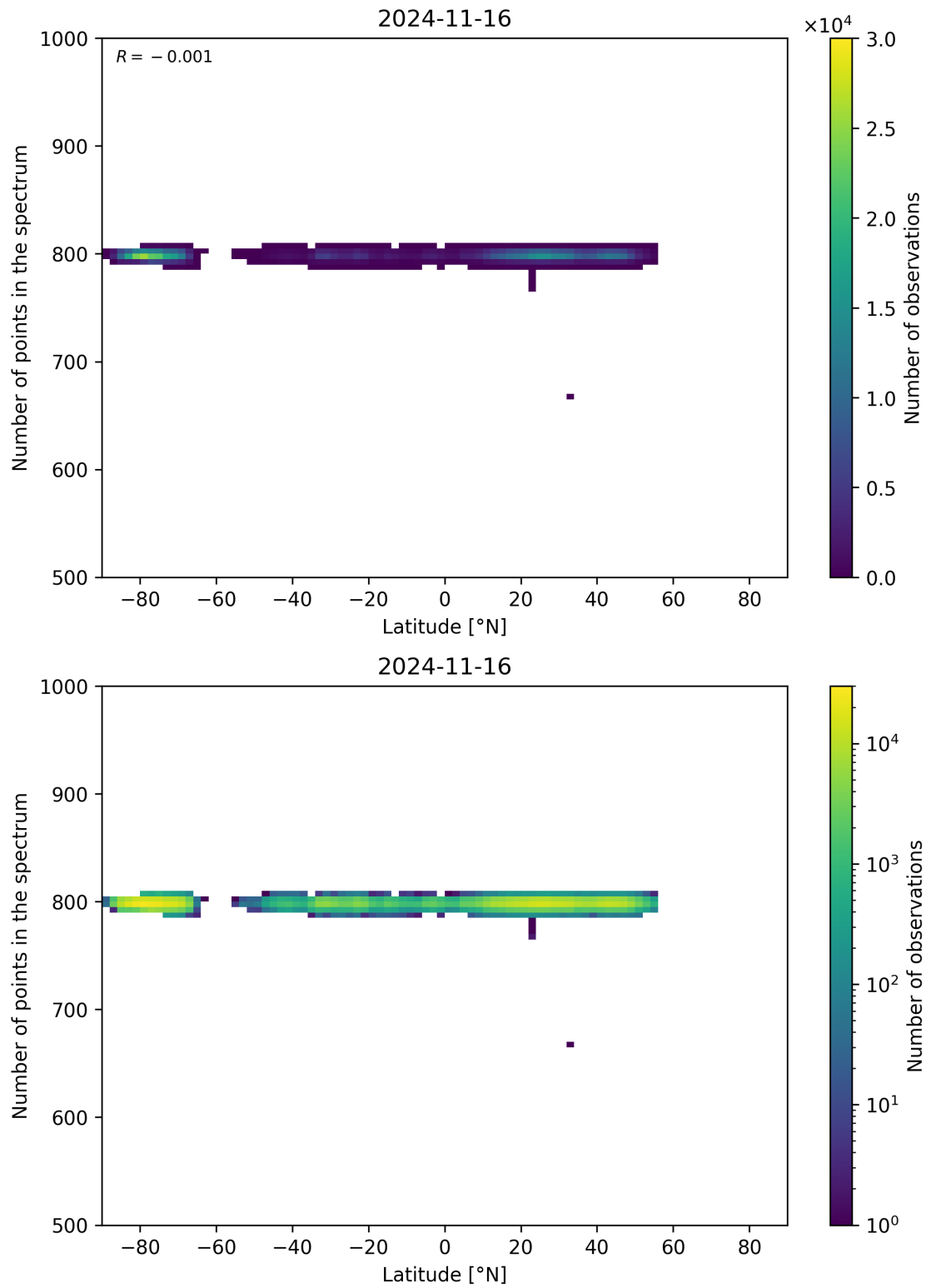
Figure 61: Scatter density plot of “Latitude” against “Number of points in the spectrum” for 2024-11-15 to 2024-11-17.
