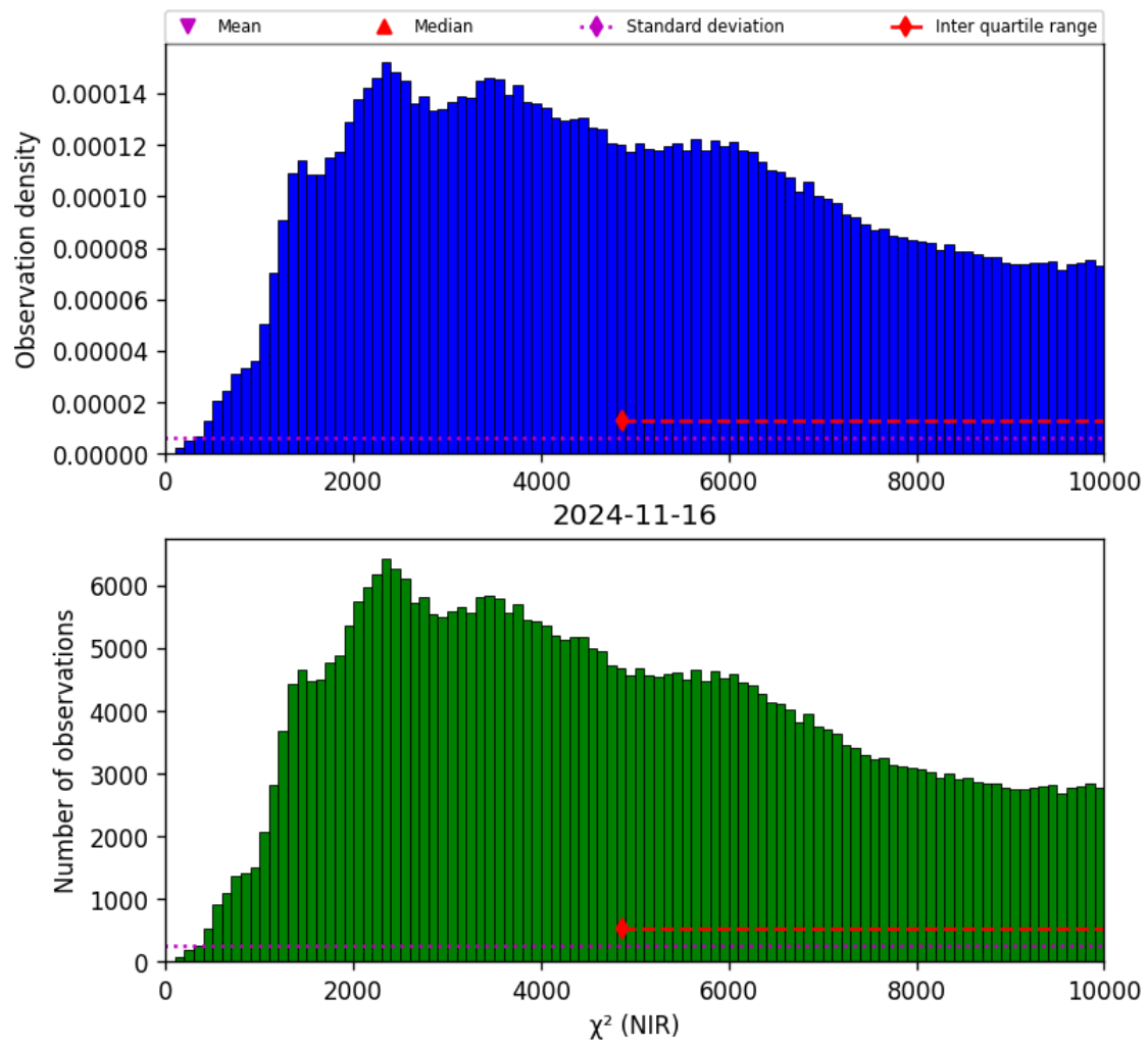
Figure 29: Histogram of " \chi^2 (NIR)" for 2024-11-15 to 2024-11-17
