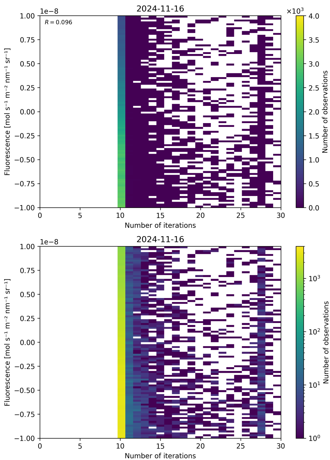
Figure 87: Scatter density plot of “Number of iterations” against “Fluorescence” for 2024-11-15 to 2024-11-17.
