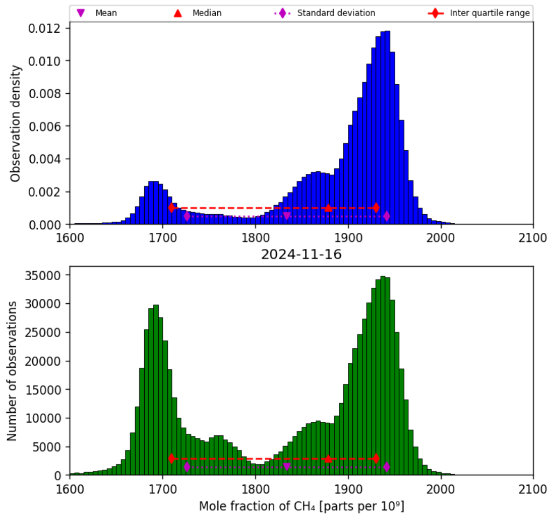
Figure 23: Histogram of “Mole fraction of CH 4 ” for 2024-11-15 to 2024-11-17
