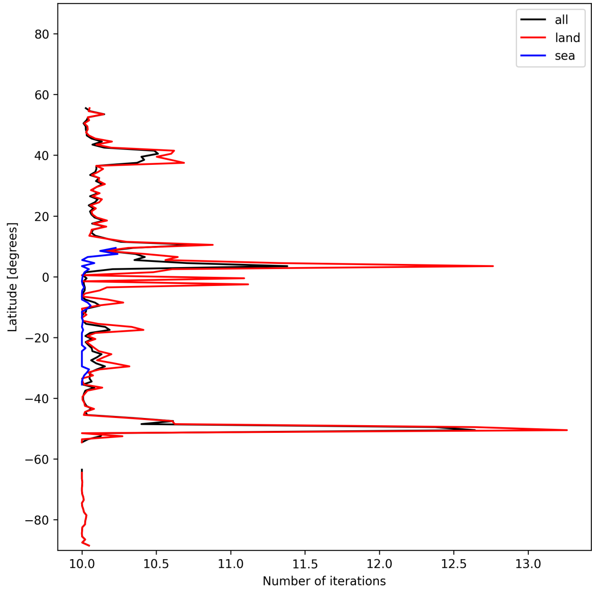
Figure 20: Zonal average of “Number of iterations” for 2024-11-15 to 2024-11-17.
