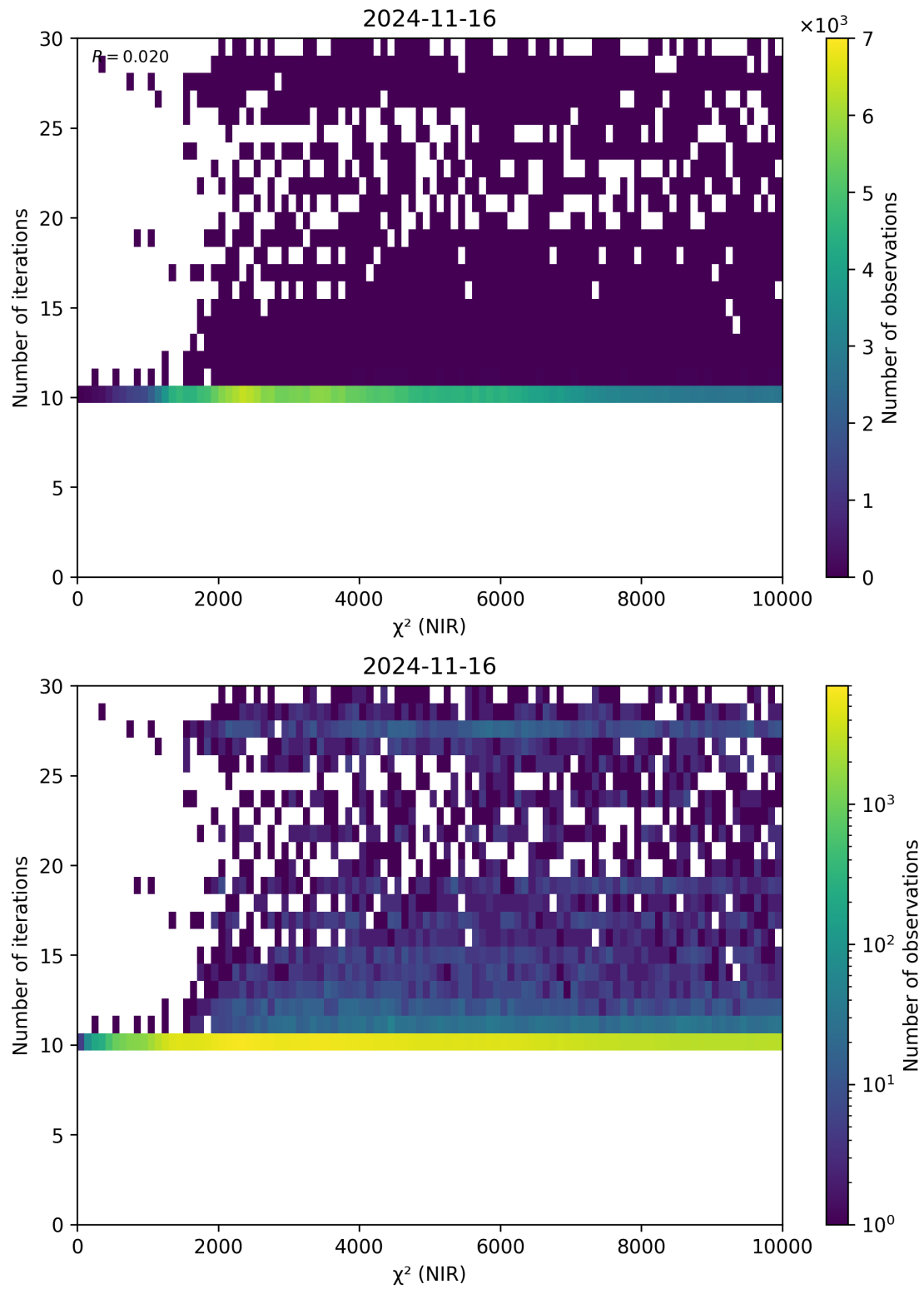
Figure 46: Scatter density plot of “ \chi^2 (NIR)” against “Number of iterations” for 2024-11-15 to 2024-11-17.
