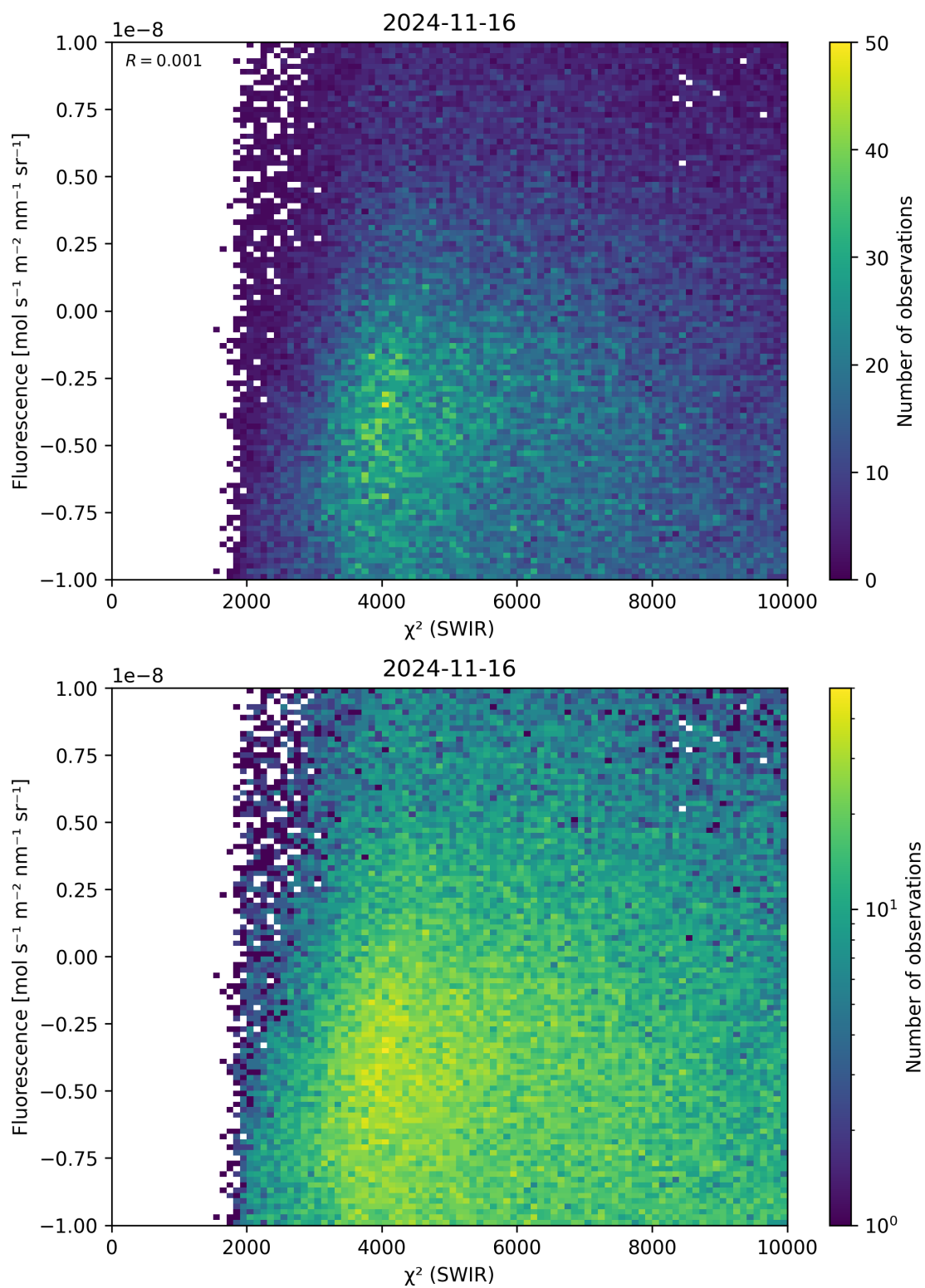
Figure 49: Scatter density plot of “ \chi^2 (SWIR)” against “Fluorescence” for 2024-11-15 to 2024-11-17.
