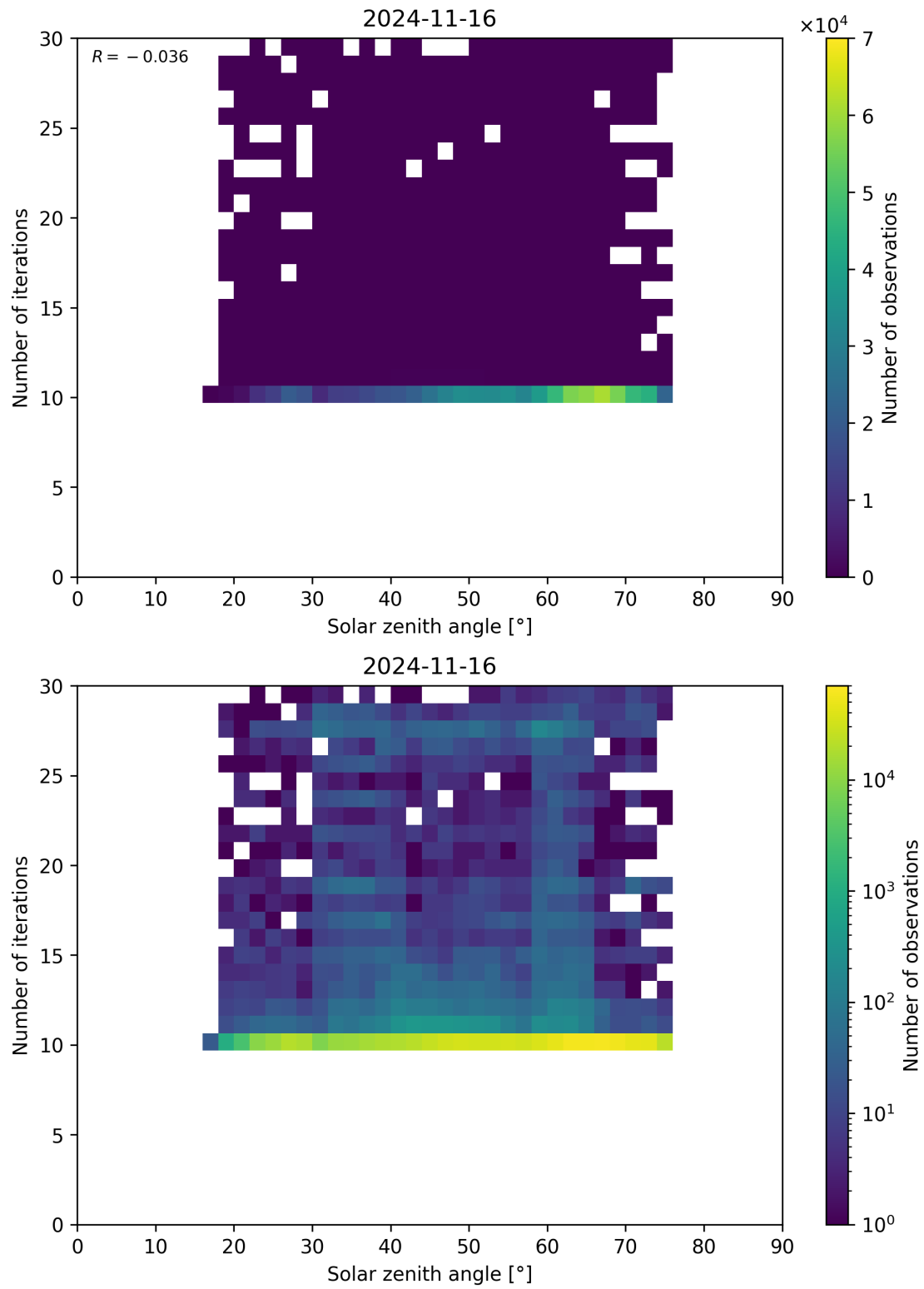
Figure 102: Scatter density plot of “Solar zenith angle” against “Number of iterations” for 2024-11-15 to 2024-11-17.
