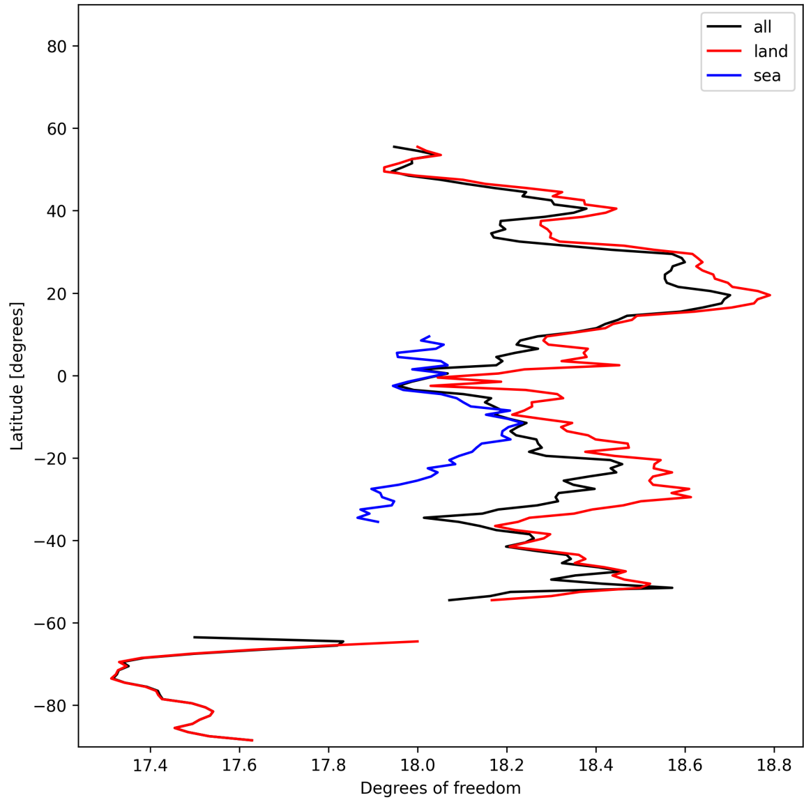
Figure 19: Zonal average of “Degrees of freedom” for 2024-11-15 to 2024-11-17.
