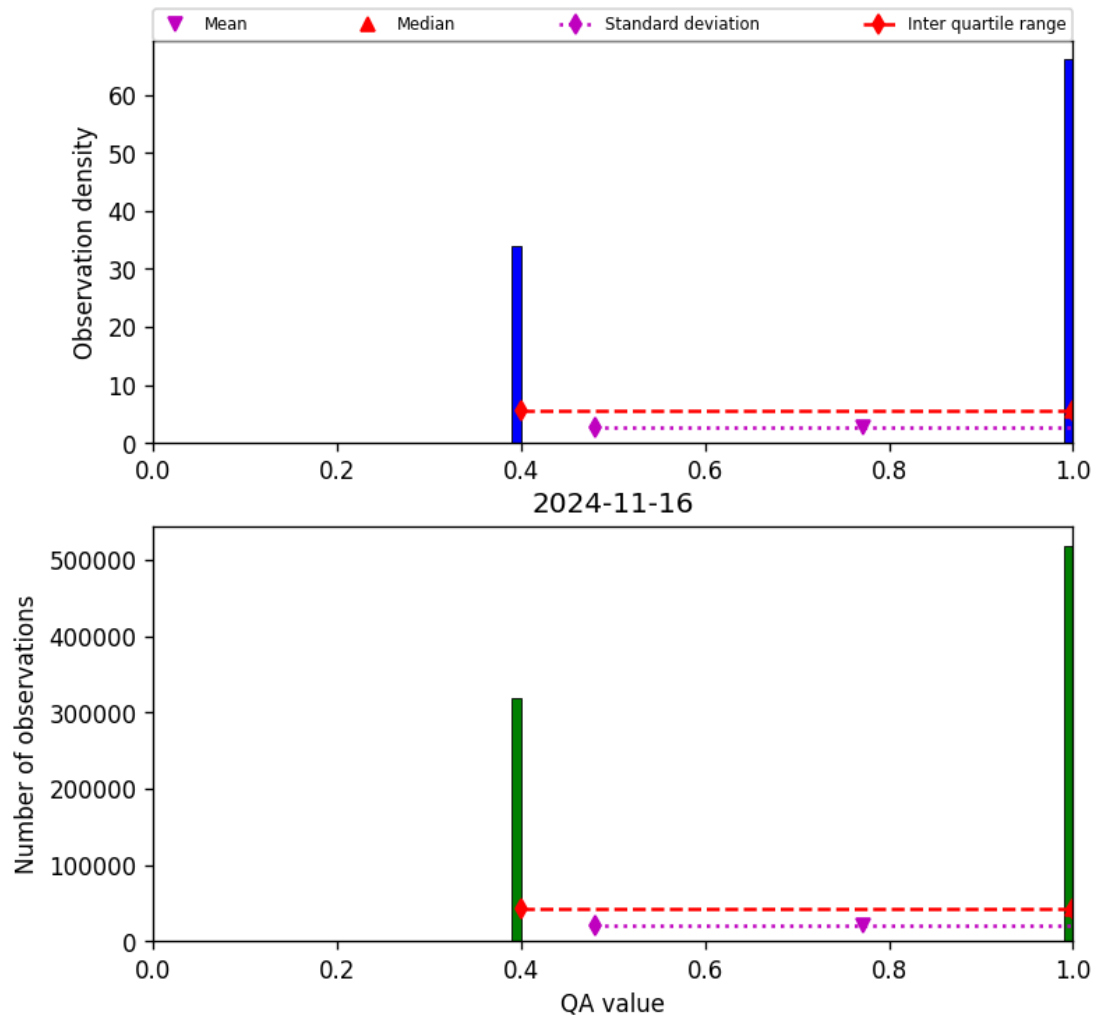
Figure 22: Histogram of “QA value” for 2024-11-15 to 2024-11-17
