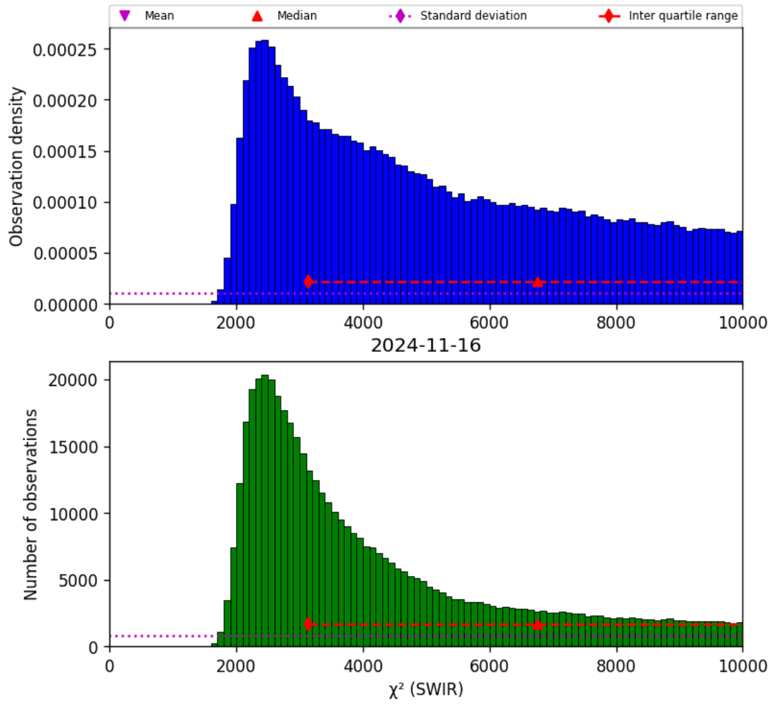
Figure 28: Histogram of “ \chi^2 (SWIR)” for 2024-11-15 to 2024-11-17
