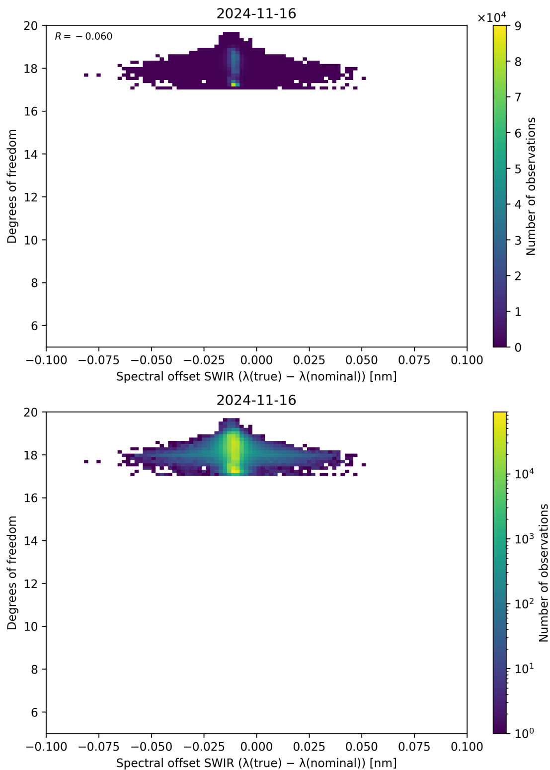
Figure 119: Scatter density plot of “Spectral offset SWIR ( \lambda_{\text{true}} - \lambda_{\text{nominal}} )” against “Degrees of freedom” for 2024-11-15 to 2024-11-17.
