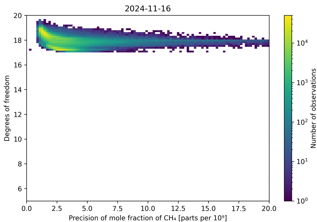
Figure 80: Scatter density plot of “Precision of mole fraction of CH 4 ” against “Degrees of freedom” for 2024-11-15 to 2024-11-17.
