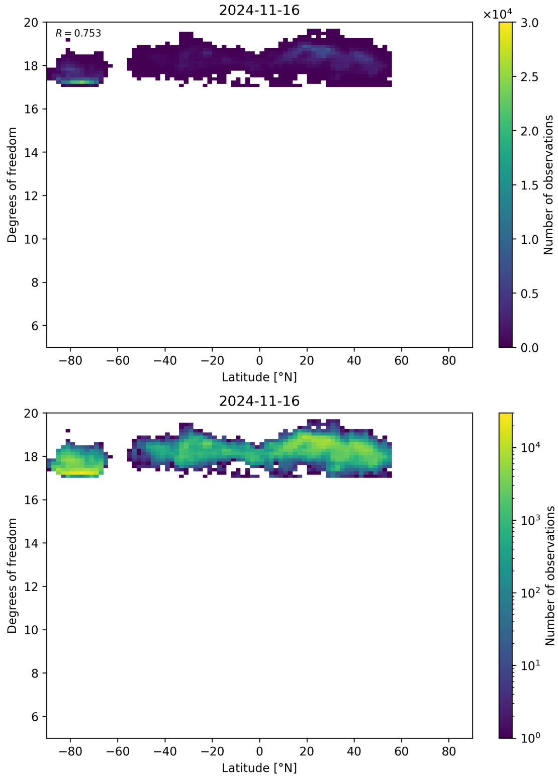
Figure 55: Scatter density plot of “Latitude” against “Degrees of freedom” for 2024-11-15 to 2024-11-17.
