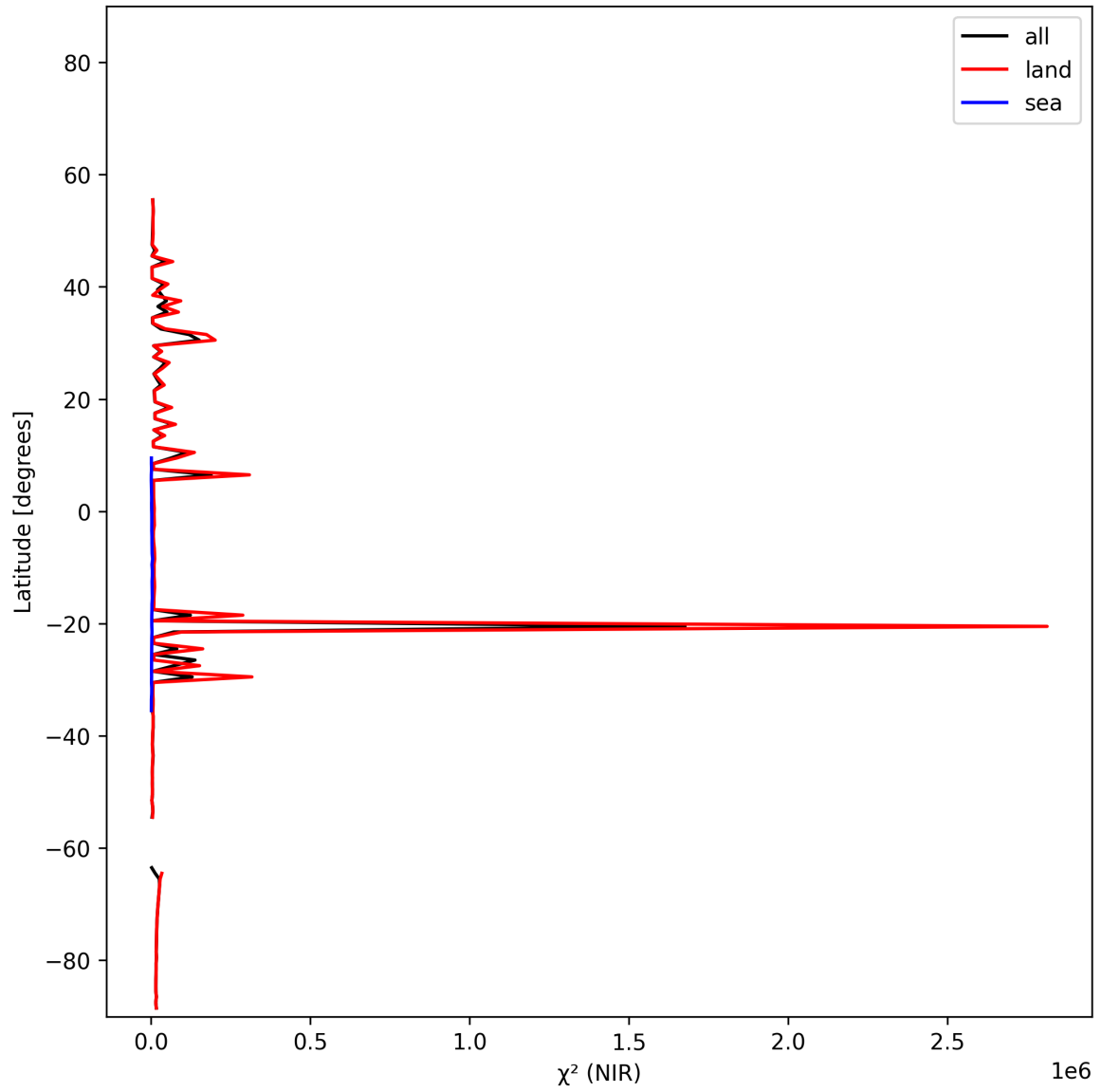
Figure 18: Zonal average of “ \chi^2 (NIR)” for 2024-11-15 to 2024-11-17.
