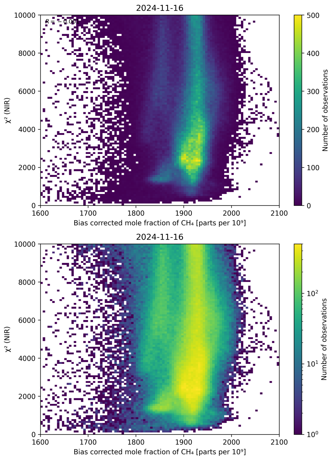
Figure 63: Scatter density plot of “Bias corrected mole fraction of CH 4 ” against “ \chi^2 (NIR)” for 2024-11-15 to 2024-11-17.
