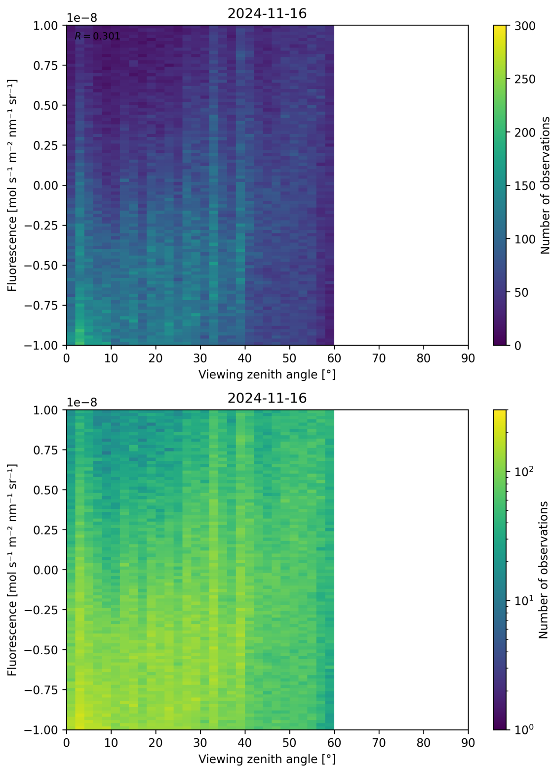
Figure 108: Scatter density plot of “Viewing zenith angle” against “Fluorescence” for 2024-11-15 to 2024-11-17.
