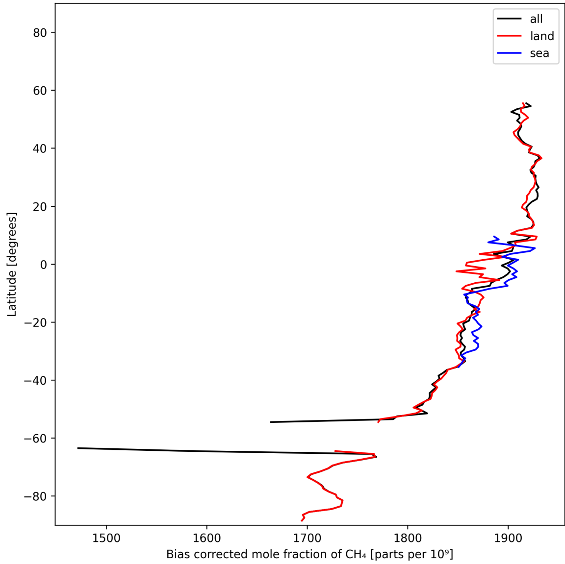
Figure 14: Zonal average of “Bias corrected mole fraction of CH 4 ” for 2024-11-15 to 2024-11-17.
