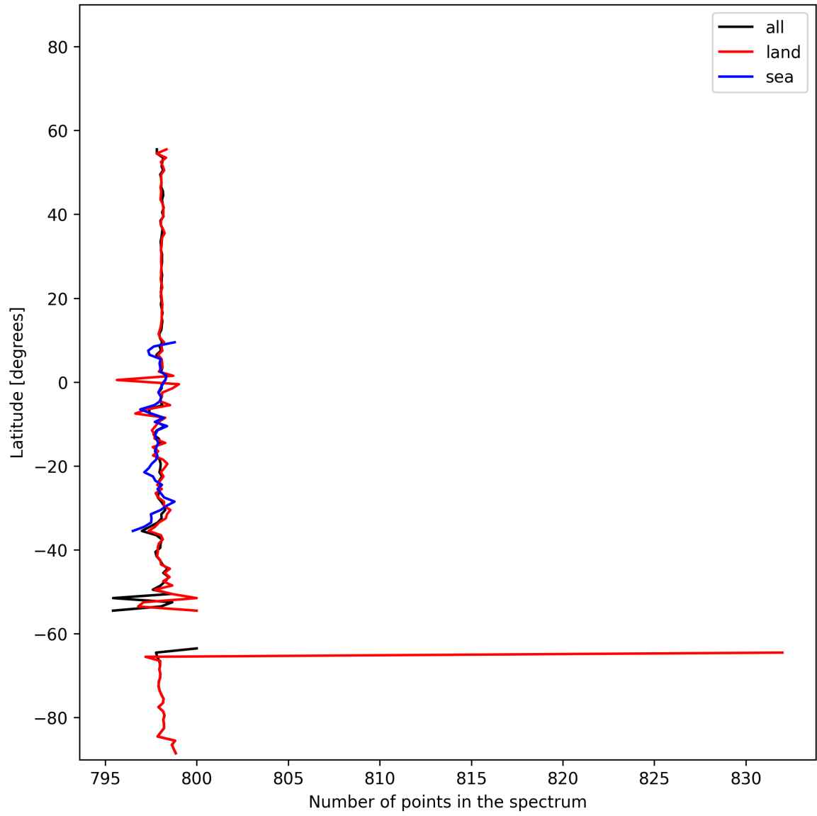
Figure 15: Zonal average of “Number of points in the spectrum” for 2024-11-15 to 2024-11-17.
