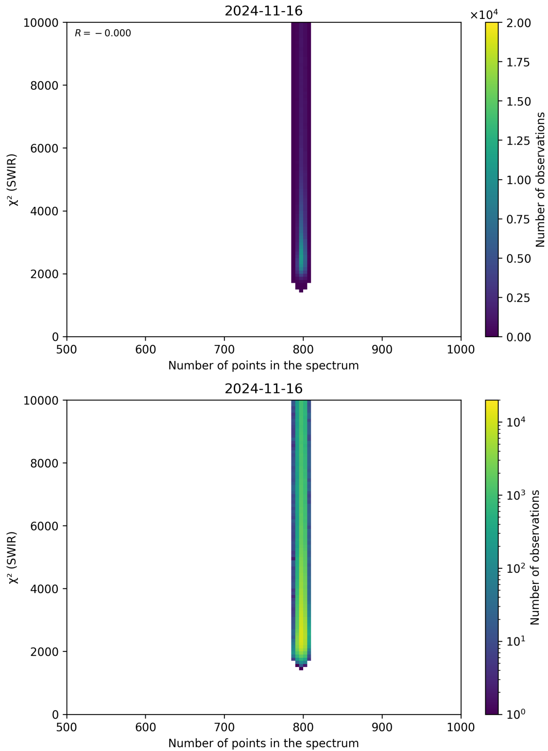
Figure 89: Scatter density plot of “Number of points in the spectrum” against “ \chi^2 (SWIR)” for 2024-11-15 to 2024-11-17.
