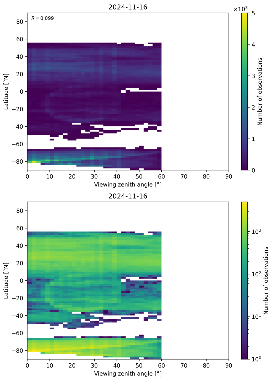
Figure 109: Scatter density plot of “Viewing zenith angle” against “Latitude” for 2024-11-15 to 2024-11-17.
