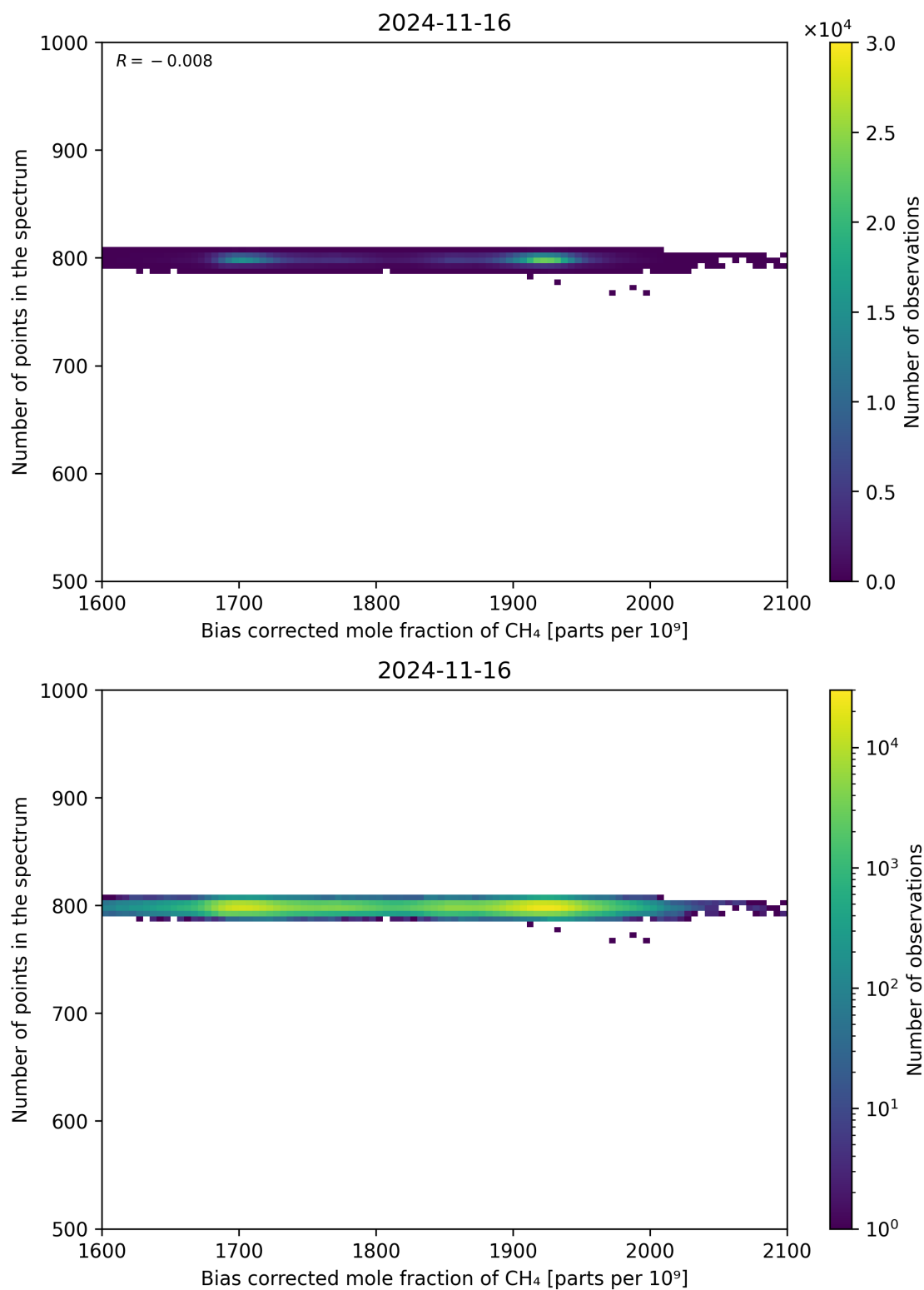
Figure 68: Scatter density plot of “Bias corrected mole fraction of CH 4 ” against “Number of points in the spectrum” for 2024-11-15 to 2024-11-17.
