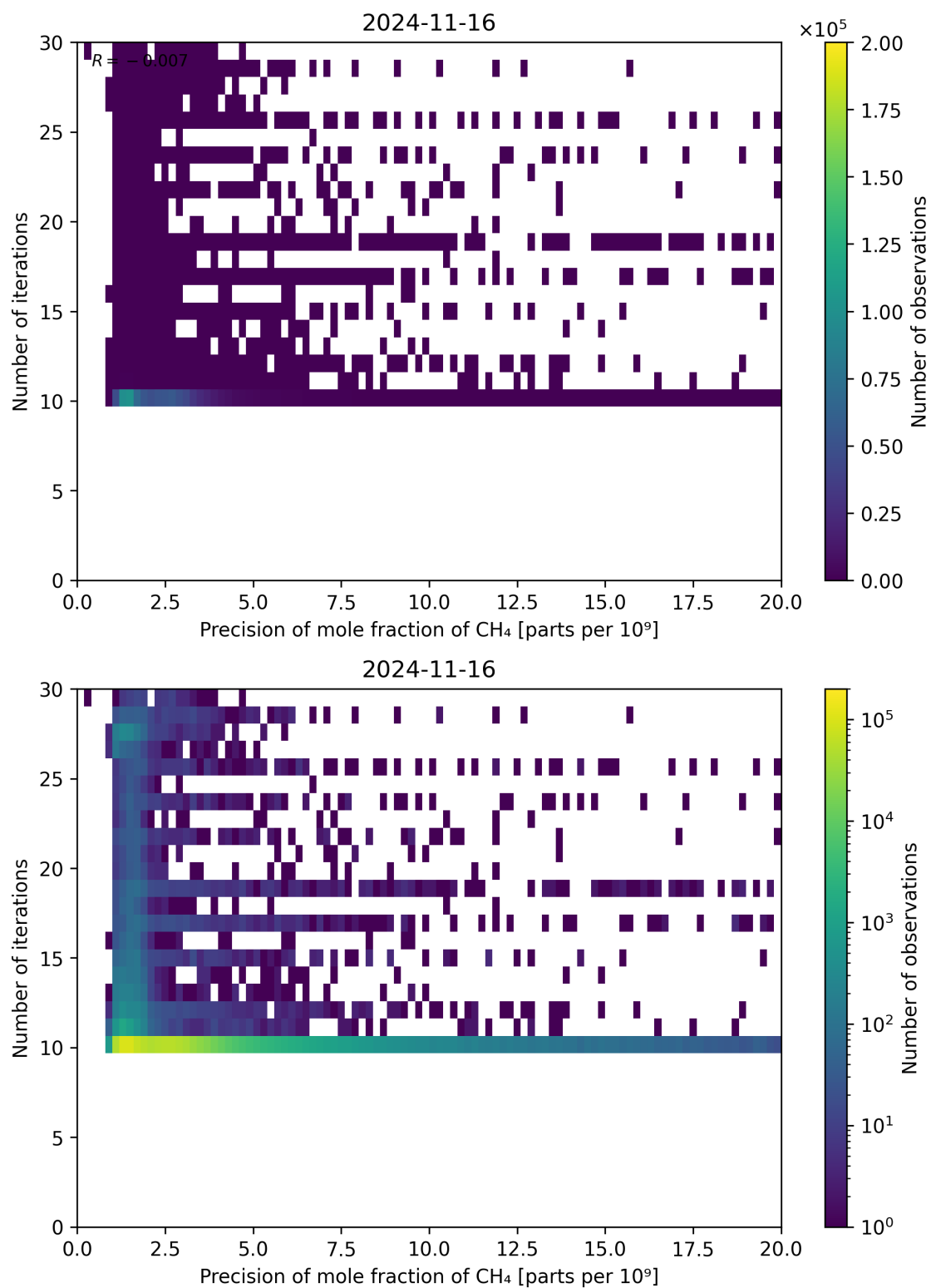
Figure 83: Scatter density plot of “Precision of mole fraction of CH 4 ” against “Number of iterations” for 2024-11-15 to 2024-11-17.
