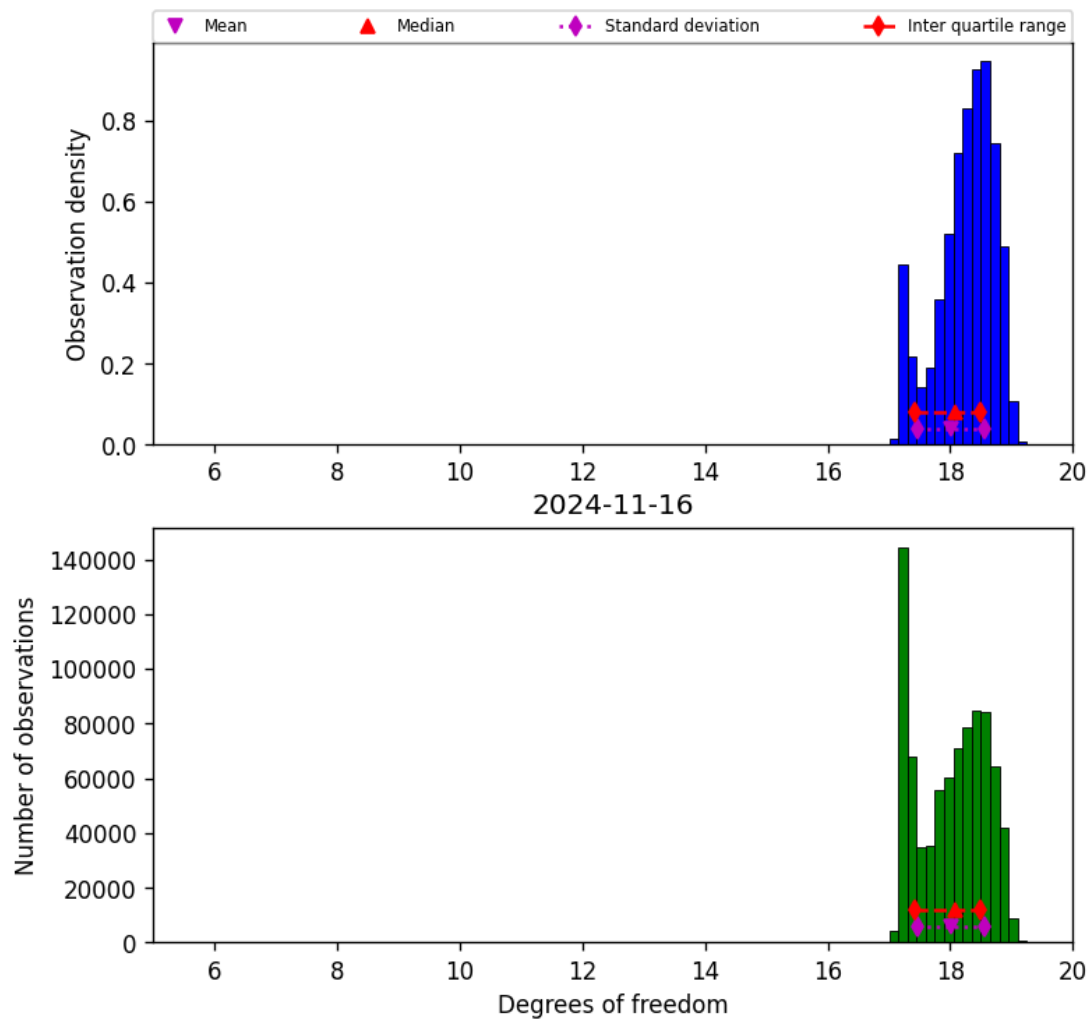
Figure 30: Histogram of “Degrees of freedom” for 2024-11-15 to 2024-11-17
