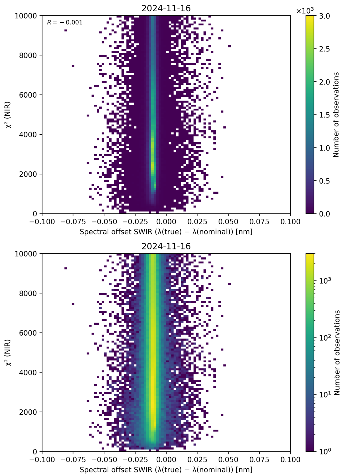
Figure 117: Scatter density plot of “Spectral offset SWIR ( \lambda_{\text{true}} - \lambda_{\text{nominal}} )” against “ \chi^2 (NIR)” for 2024-11-15 to 2024-11-17.
