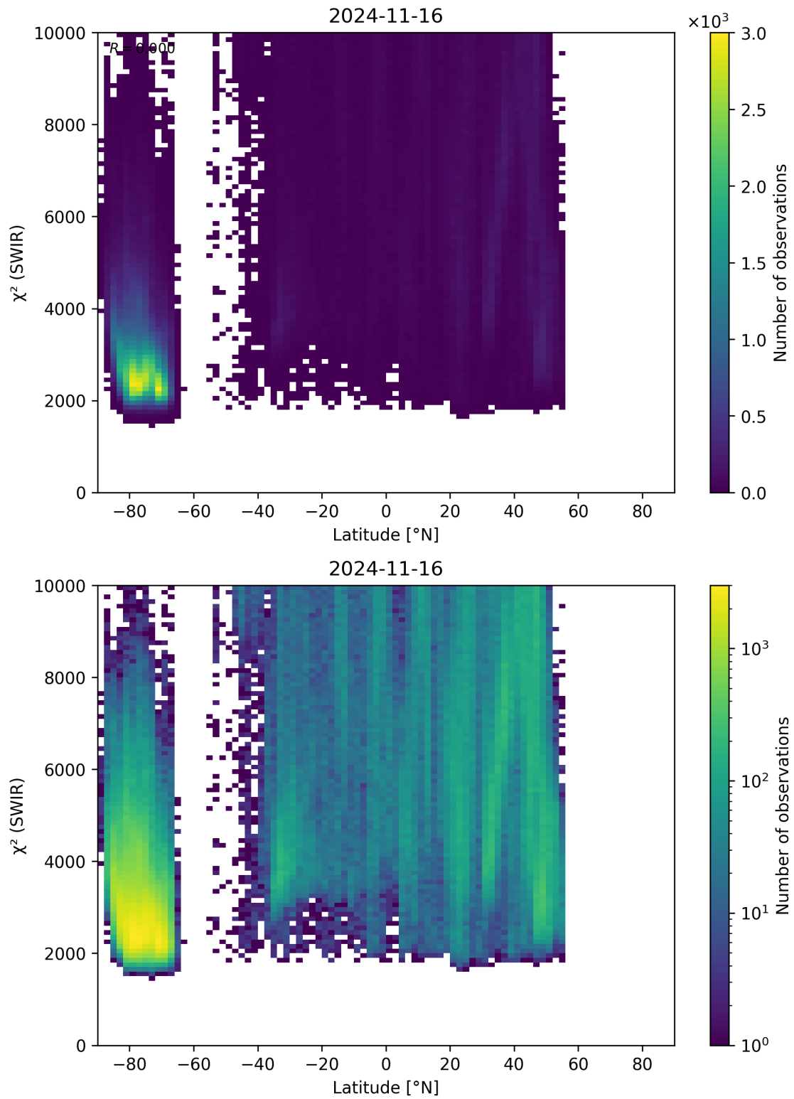
Figure 54: Scatter density plot of “Latitude” against “ \chi^2 (SWIR)” for 2024-11-15 to 2024-11-17.
