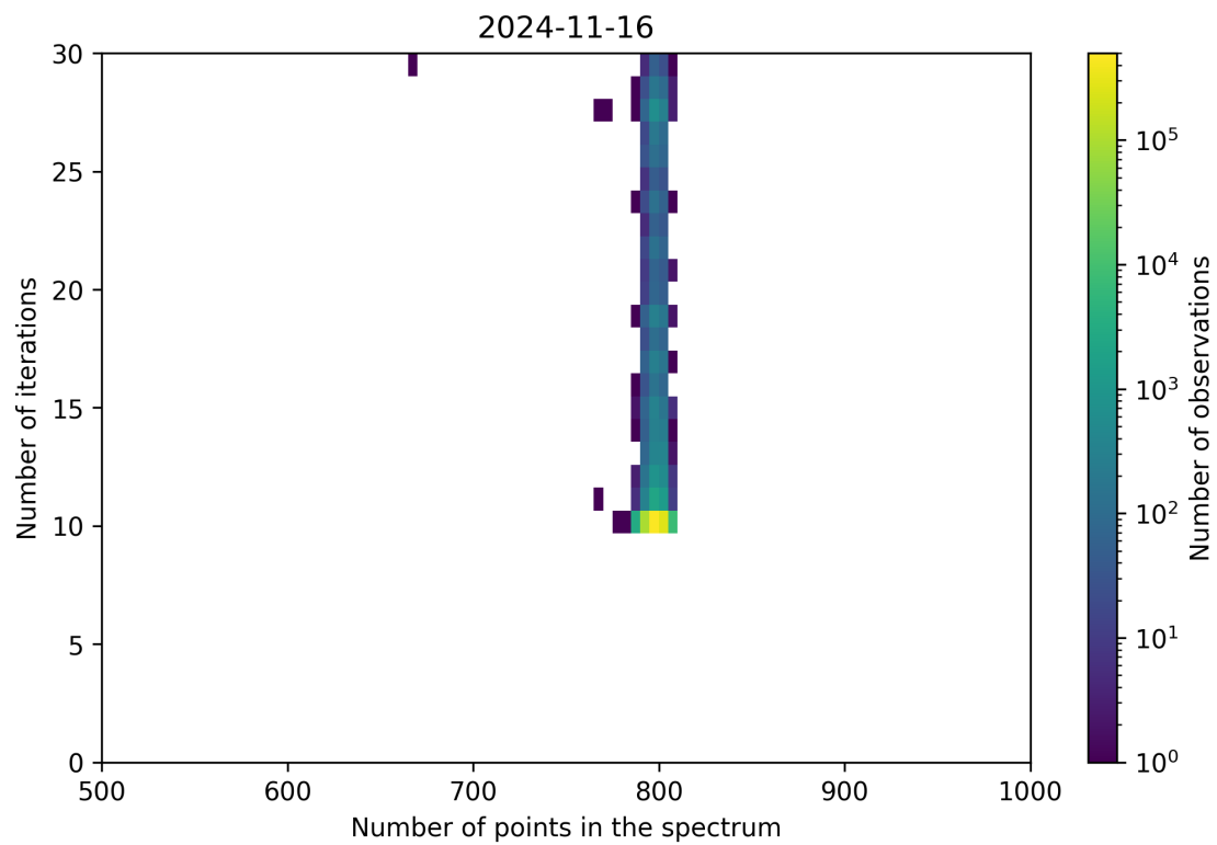
Figure 92: Scatter density plot of “Number of points in the spectrum” against “Number of iterations” for 2024-11-15 to 2024-11-17.
