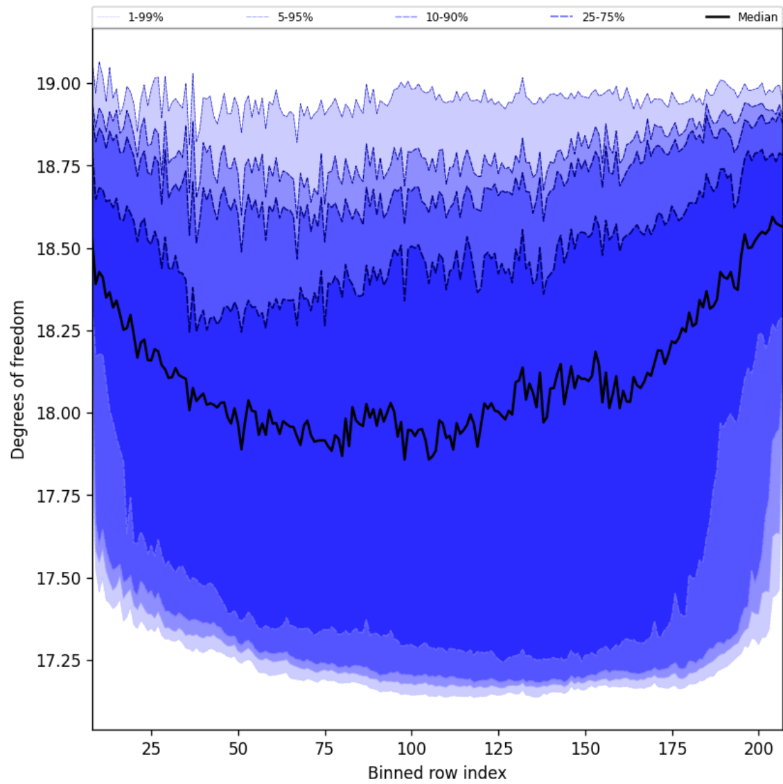
Figure 41: Along track statistics of “Degrees of freedom” for 2024-11-15 to 2024-11-17
