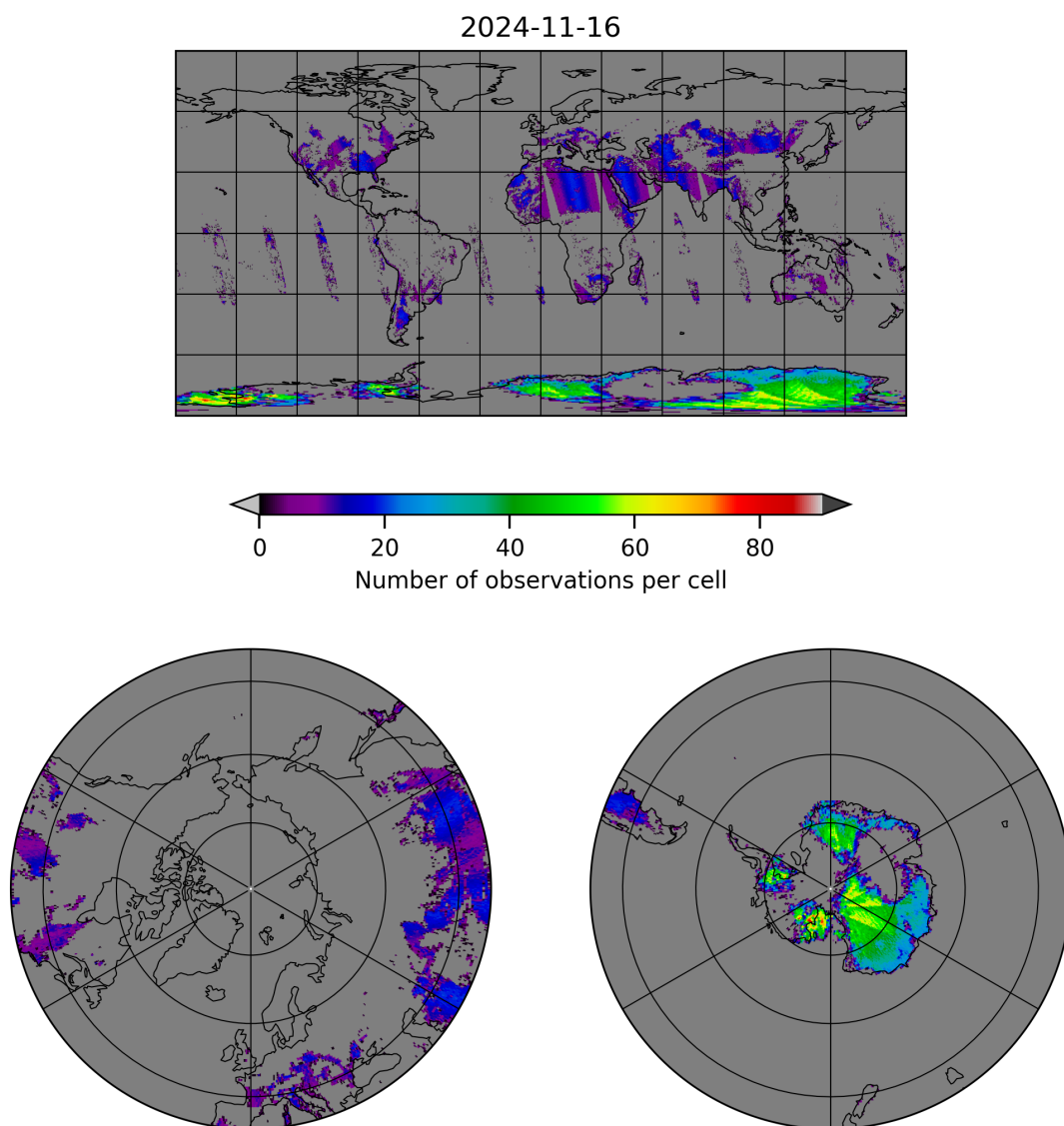
Figure 10: Map of the number of observations for 2024-11-15 to 2024-11-17
