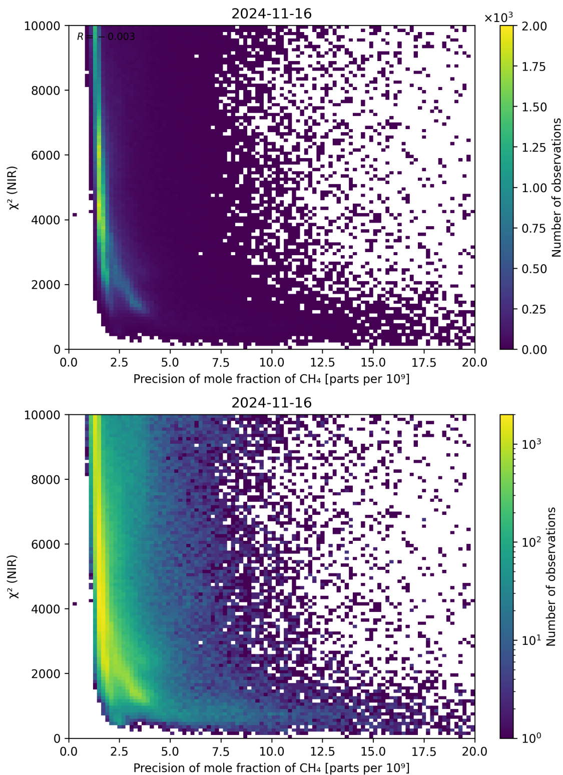
Figure 78: Scatter density plot of “Precision of mole fraction of CH 4 ” against “ \chi^2 (NIR)” for 2024-11-15 to 2024-11-17.
