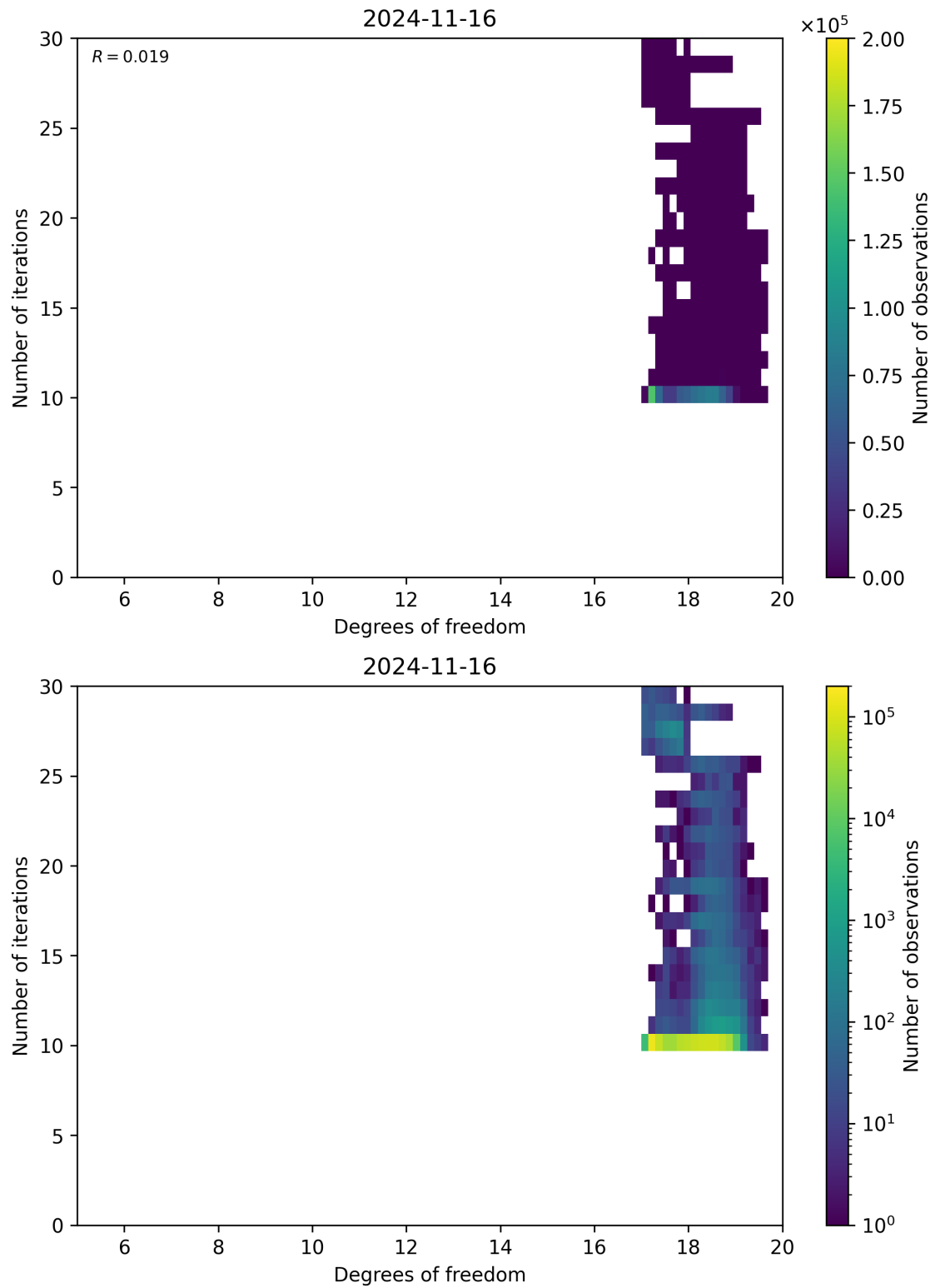
Figure 52: Scatter density plot of “Degrees of freedom” against “Number of iterations” for 2024-11-15 to 2024-11-17.
