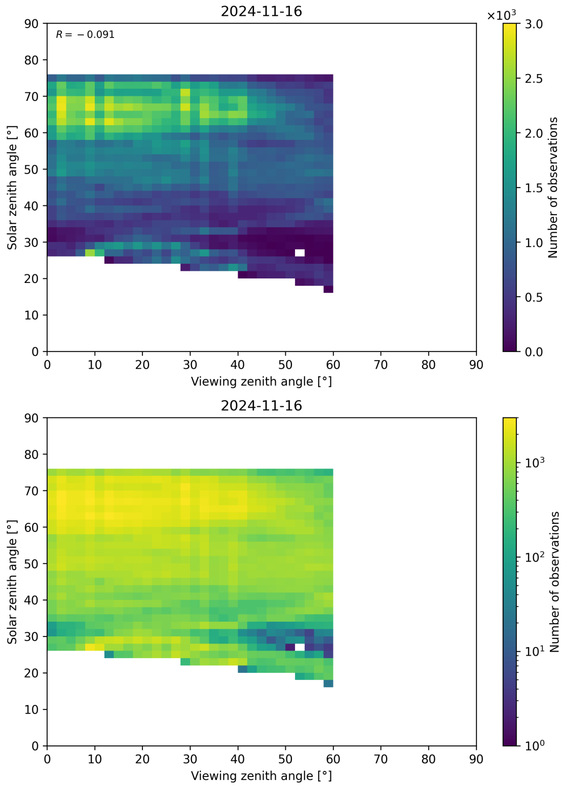
Figure 115: Scatter density plot of “Viewing zenith angle” against “Solar zenith angle” for 2024-11-15 to 2024-11-17.
