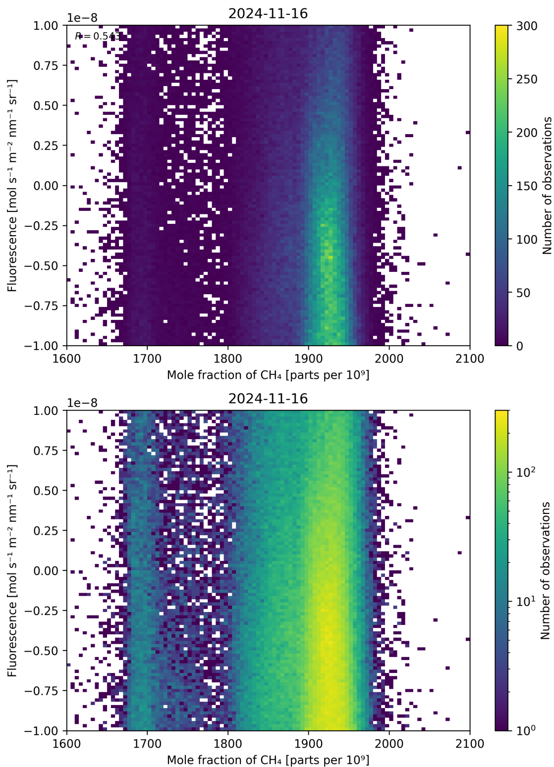
Figure 73: Scatter density plot of “Mole fraction of \text{CH}_4 ” against “Fluorescence” for 2024-11-15 to 2024-11-17.
