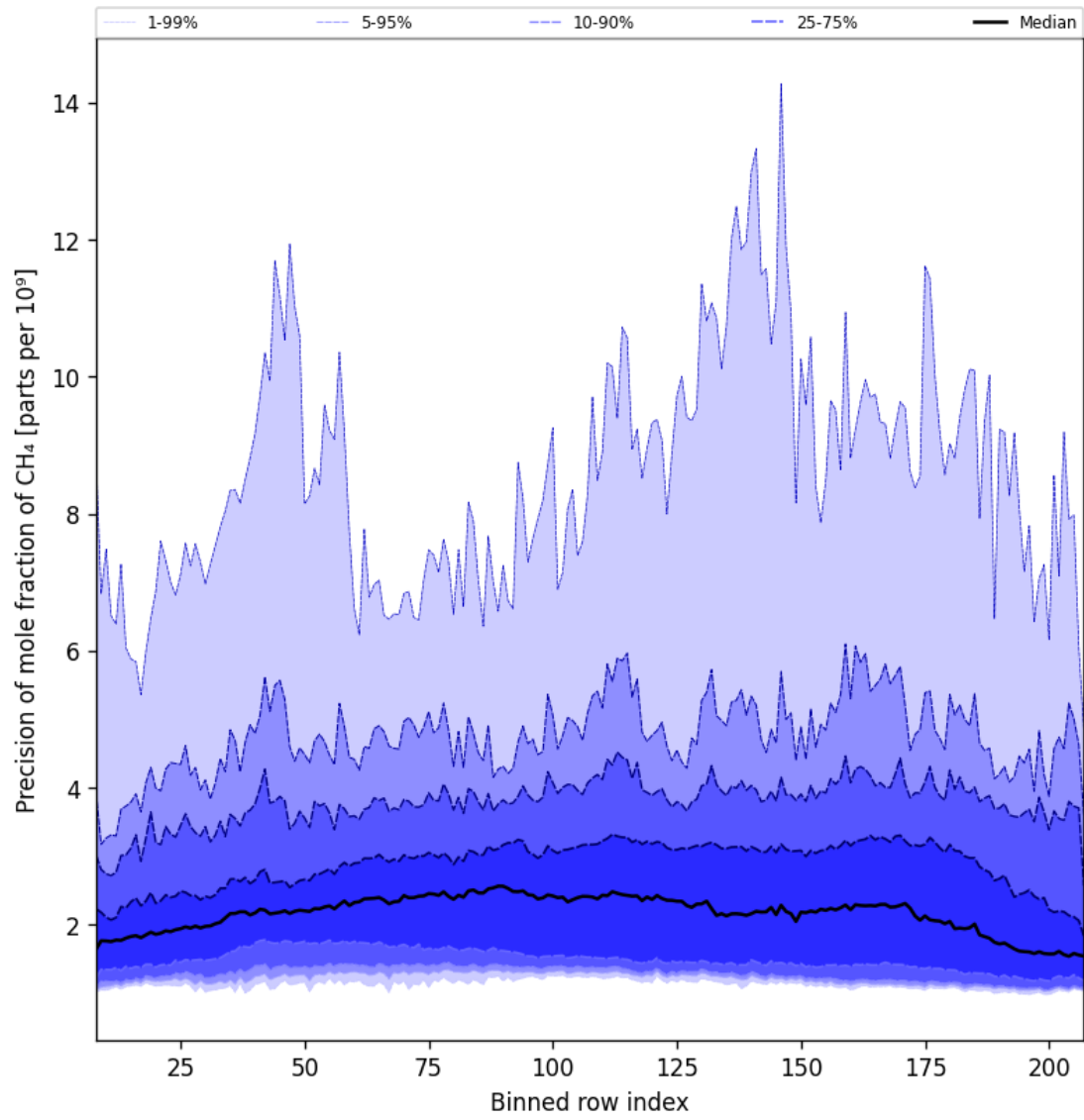
Figure 35: Along track statistics of “Precision of mole fraction of CH 4 ” for 2024-11-15 to 2024-11-17
