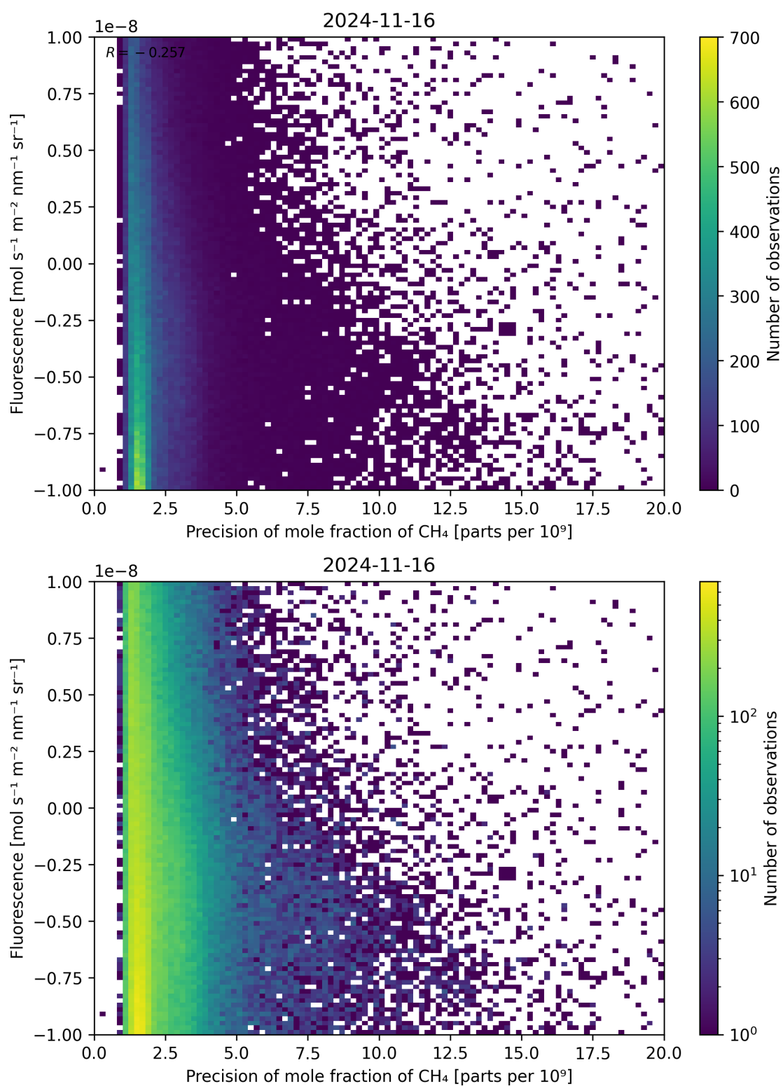
Figure 81: Scatter density plot of “Precision of mole fraction of \text{CH}_4 ” against “Fluorescence” for 2024-11-15 to 2024-11-17.
