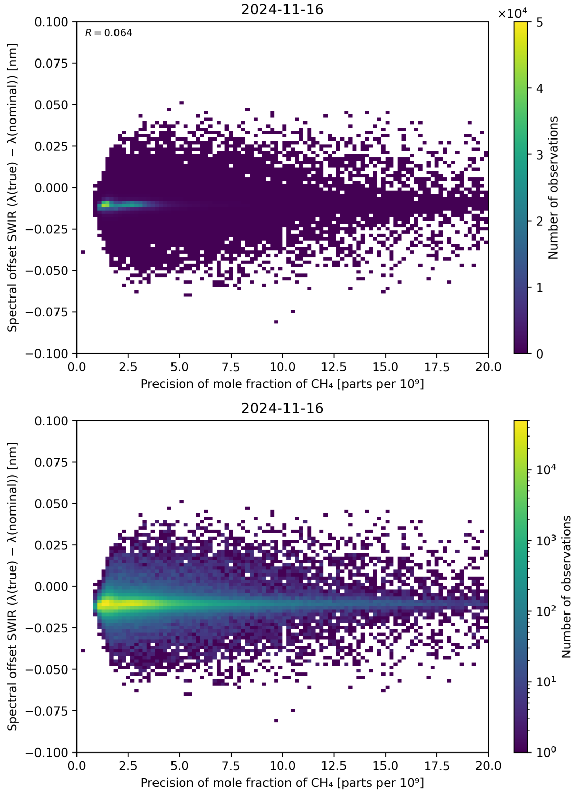
Figure 85: Scatter density plot of “Precision of mole fraction of CH 4 ” against “Spectral offset SWIR ( \lambda_{\text{true}} - \lambda_{\text{nominal}} )” for 2024-11-15 to 2024-11-17.
