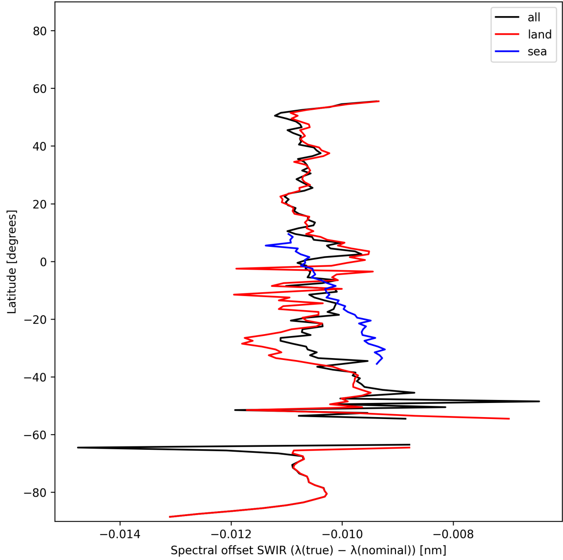
Figure 16: Zonal average of “Spectral offset SWIR ( \lambda_{\text{true}} - \lambda_{\text{nominal}} )” for 2024-11-15 to 2024-11-17.
