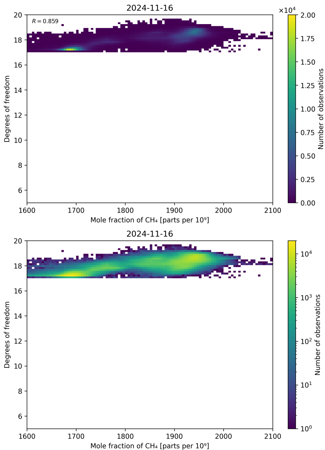
Figure 72: Scatter density plot of “Mole fraction of CH 4 ” against “Degrees of freedom” for 2024-11-15 to 2024-11-17.
