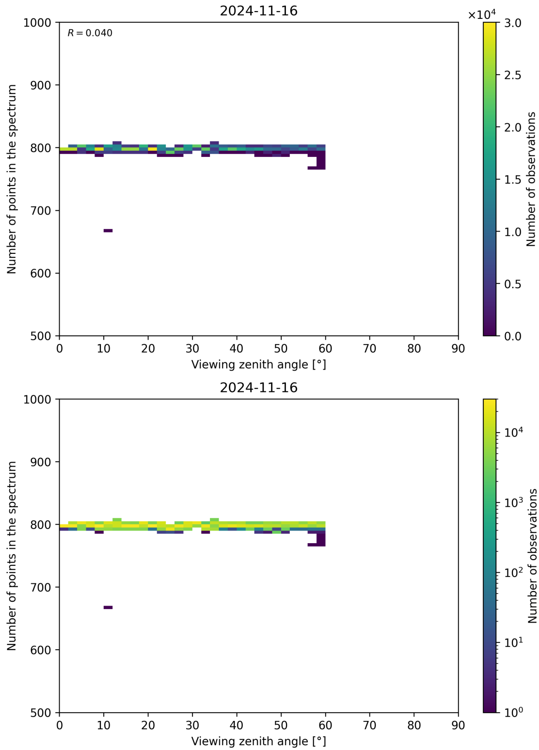
Figure 114: Scatter density plot of “Viewing zenith angle” against “Number of points in the spectrum” for 2024-11-15 to 2024-11-17.
