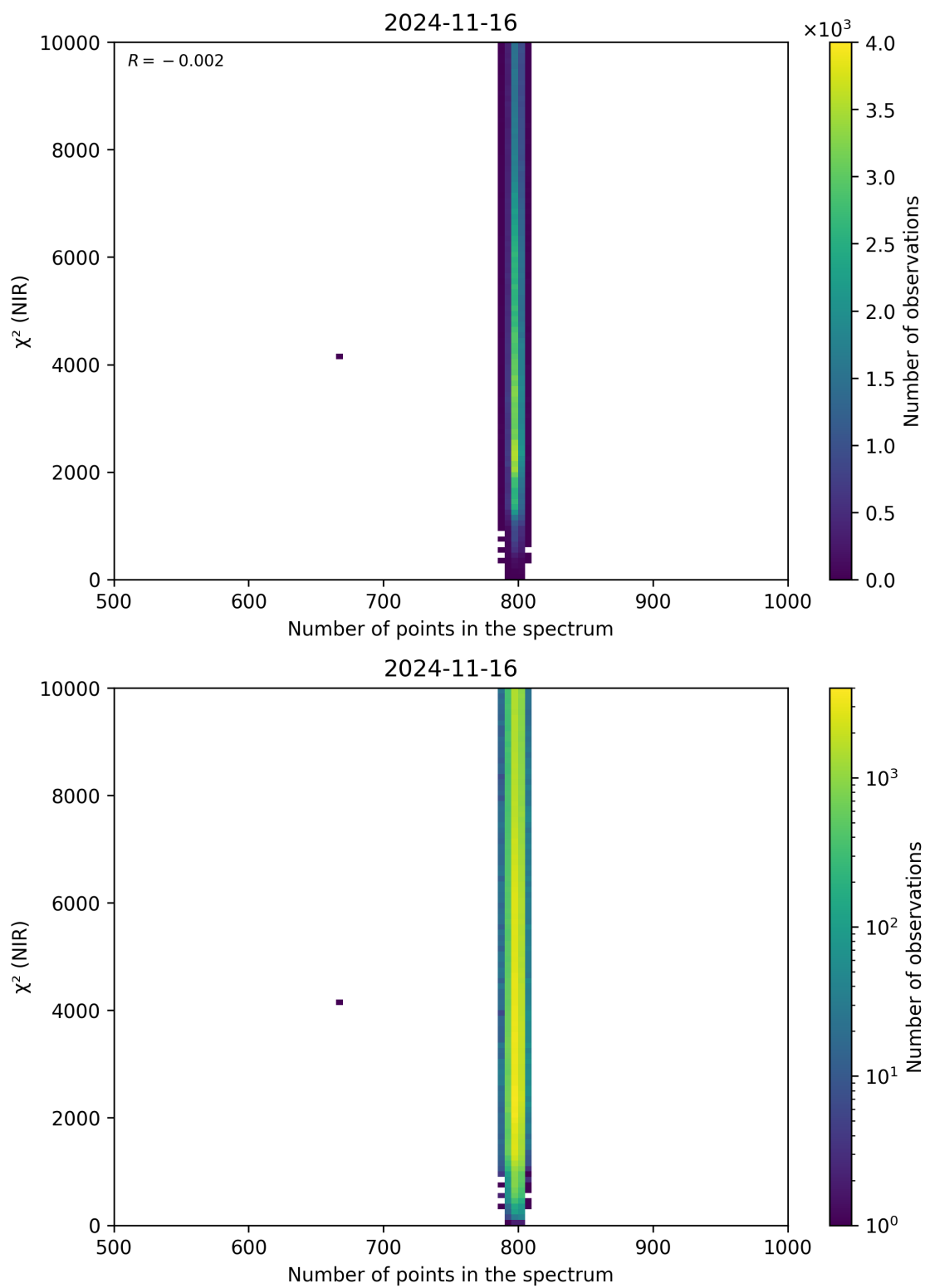
Figure 88: Scatter density plot of “Number of points in the spectrum” against “ \chi^2 (NIR)” for 2024-11-15 to 2024-11-17.
