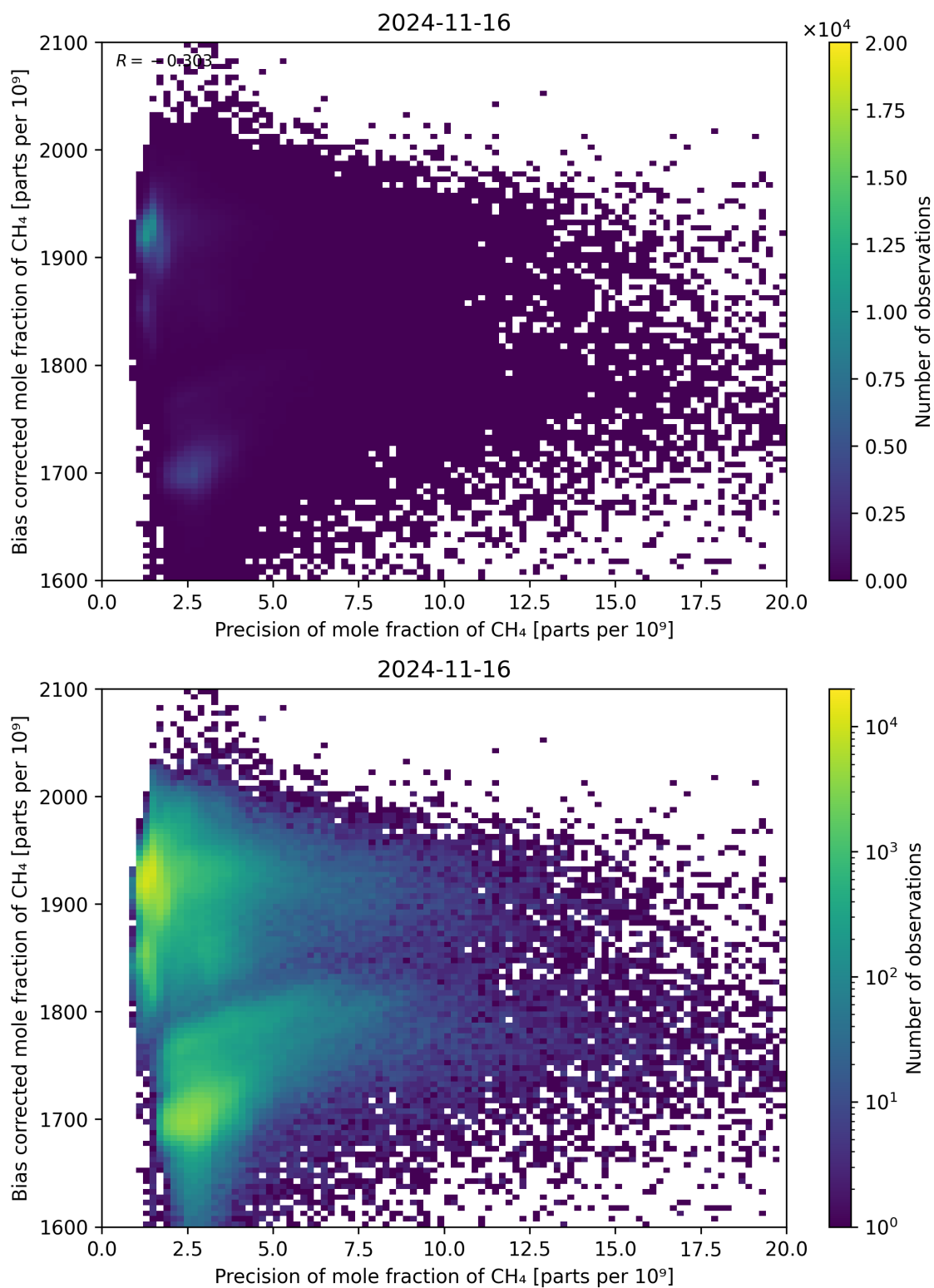
Figure 82: Scatter density plot of “Precision of mole fraction of CH 4 ” against “Bias corrected mole fraction of CH 4 ” for 2024-11-15 to 2024-11-17.
