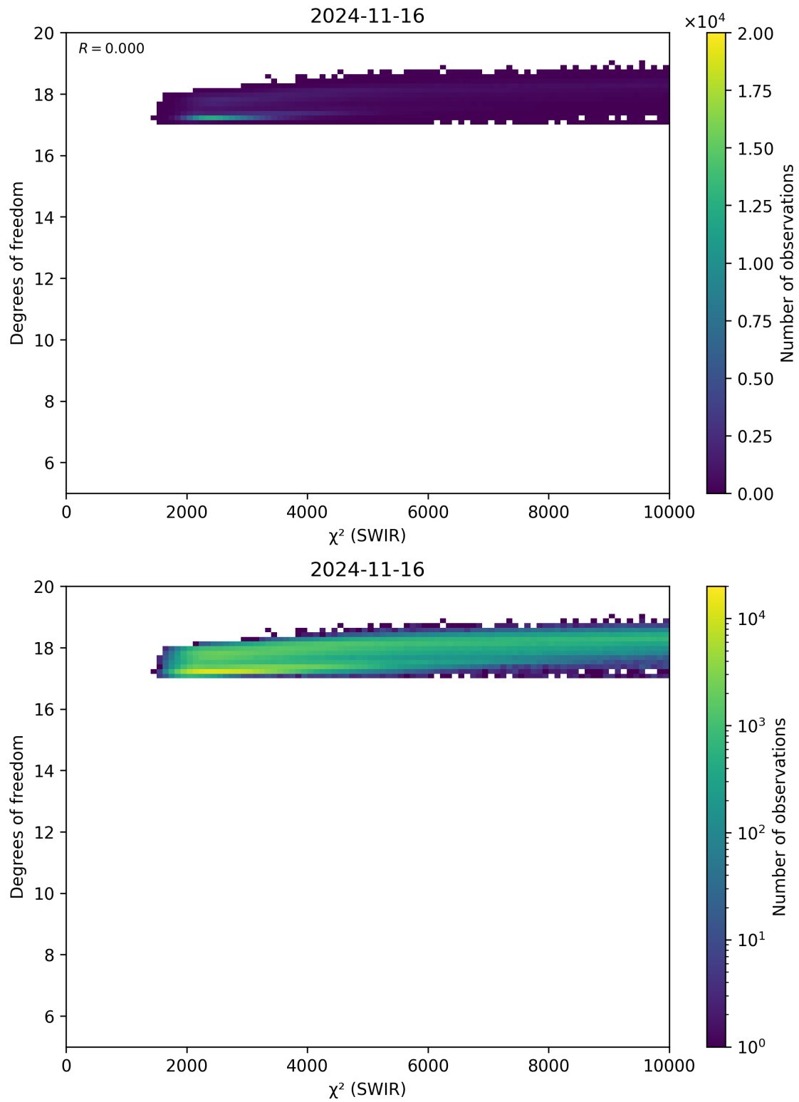
Figure 48: Scatter density plot of “ \chi^2 (SWIR)” against “Degrees of freedom” for 2024-11-15 to 2024-11-17.
