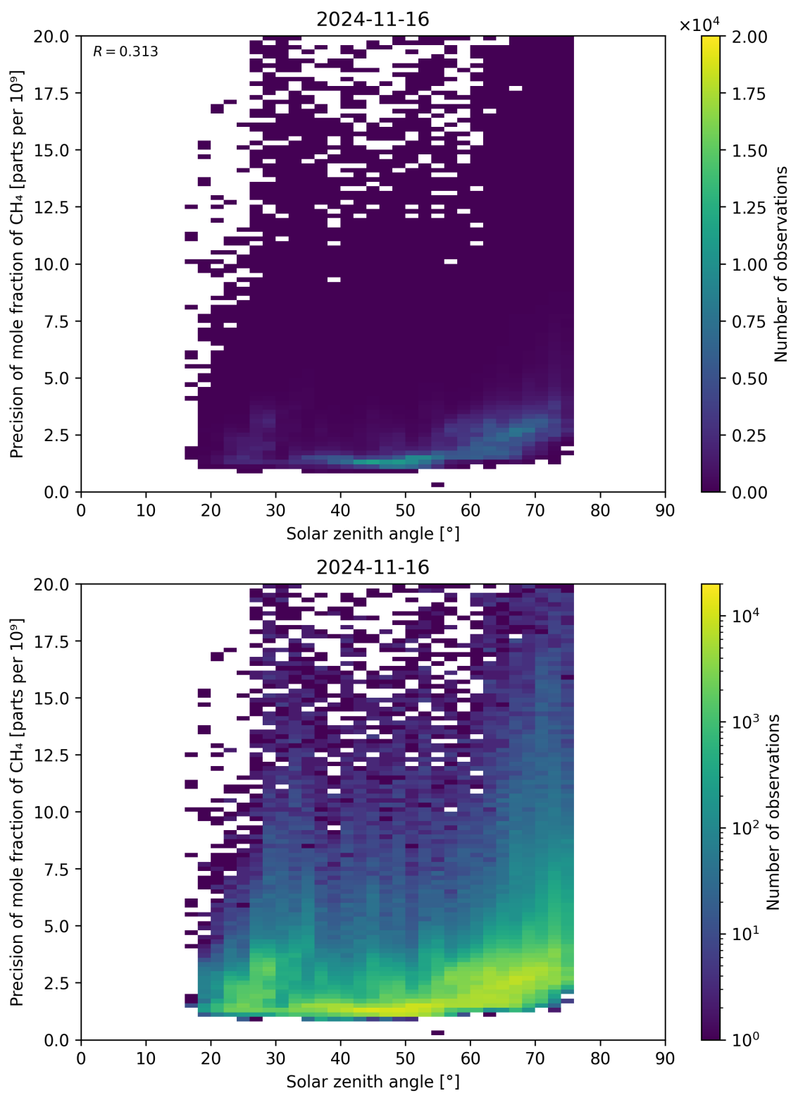
Figure 101: Scatter density plot of “Solar zenith angle” against “Precision of mole fraction of \text{CH}_4 ” for 2024-11-15 to 2024-11-17.
