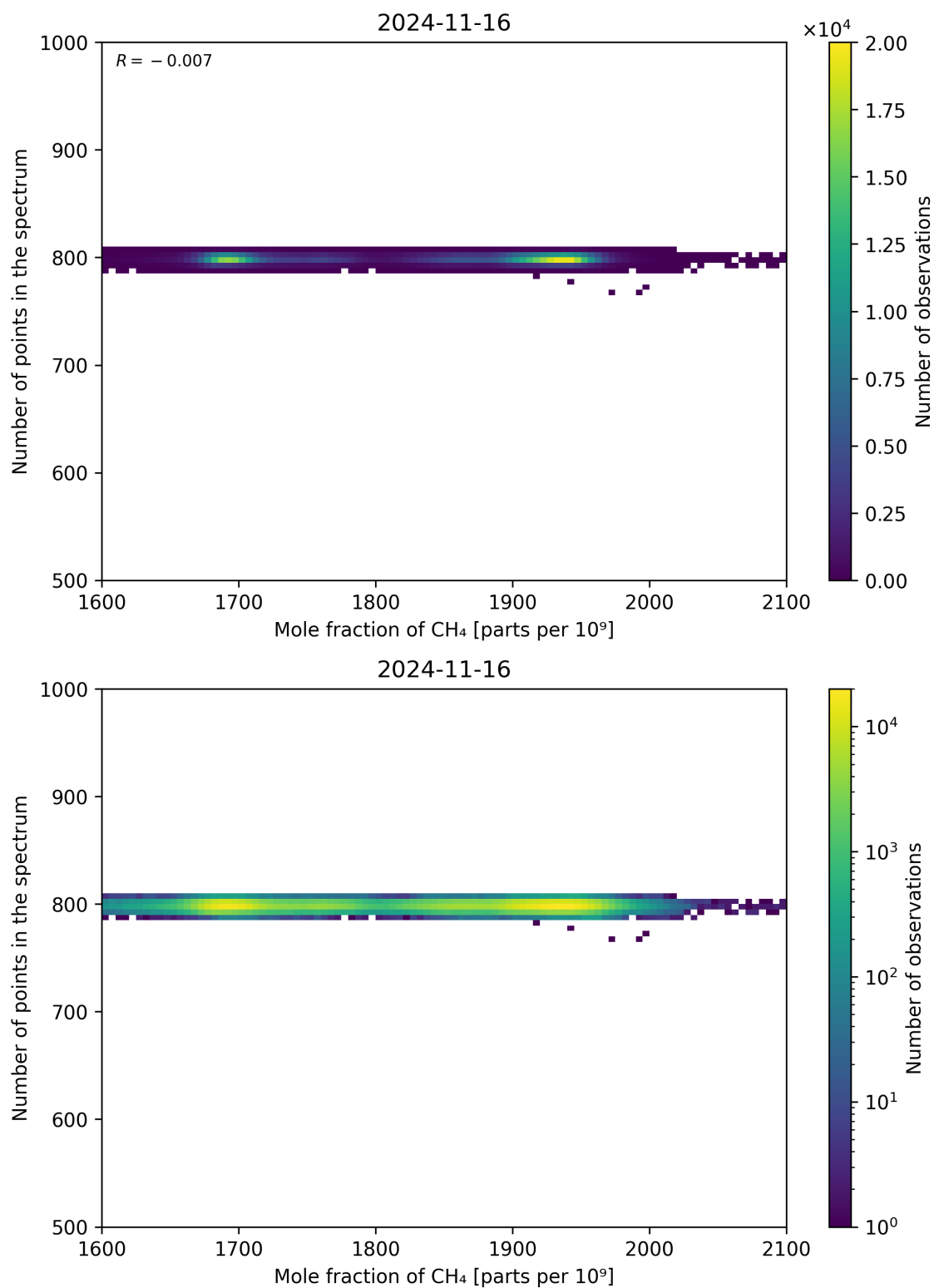
Figure 77: Scatter density plot of “Mole fraction of CH 4 ” against “Number of points in the spectrum” for 2024-11-15 to 2024-11-17.
