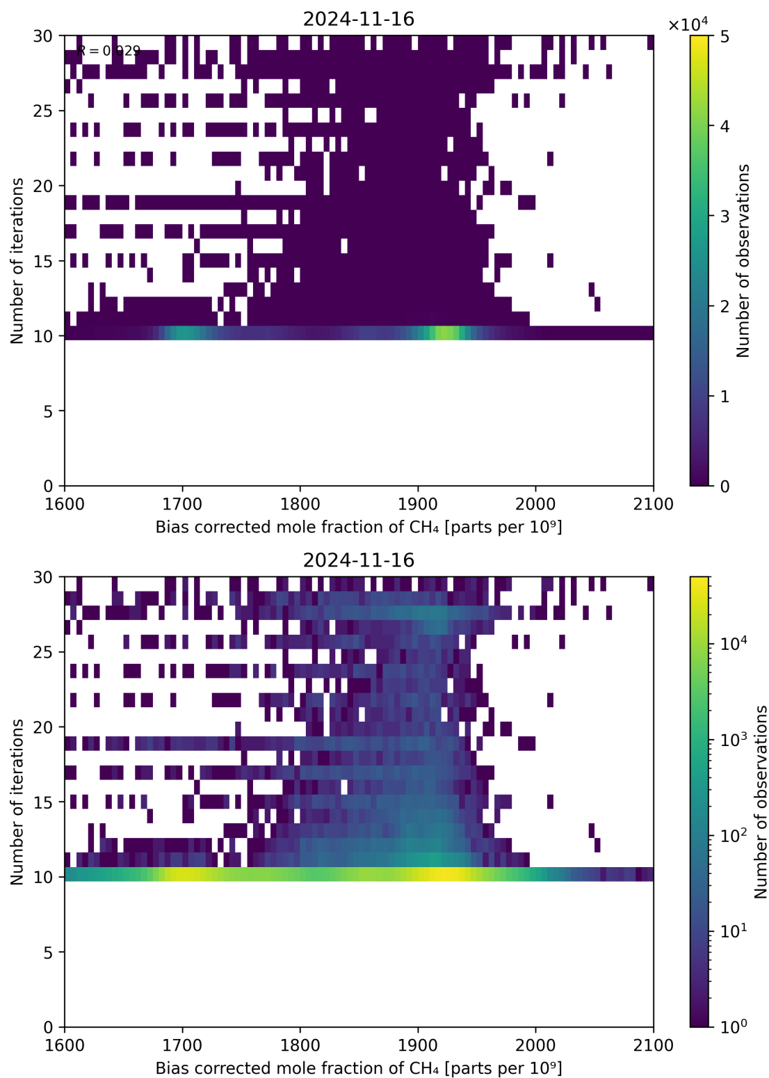
Figure 67: Scatter density plot of “Bias corrected mole fraction of \text{CH}_4 ” against “Number of iterations” for 2024-11-15 to 2024-11-17.
