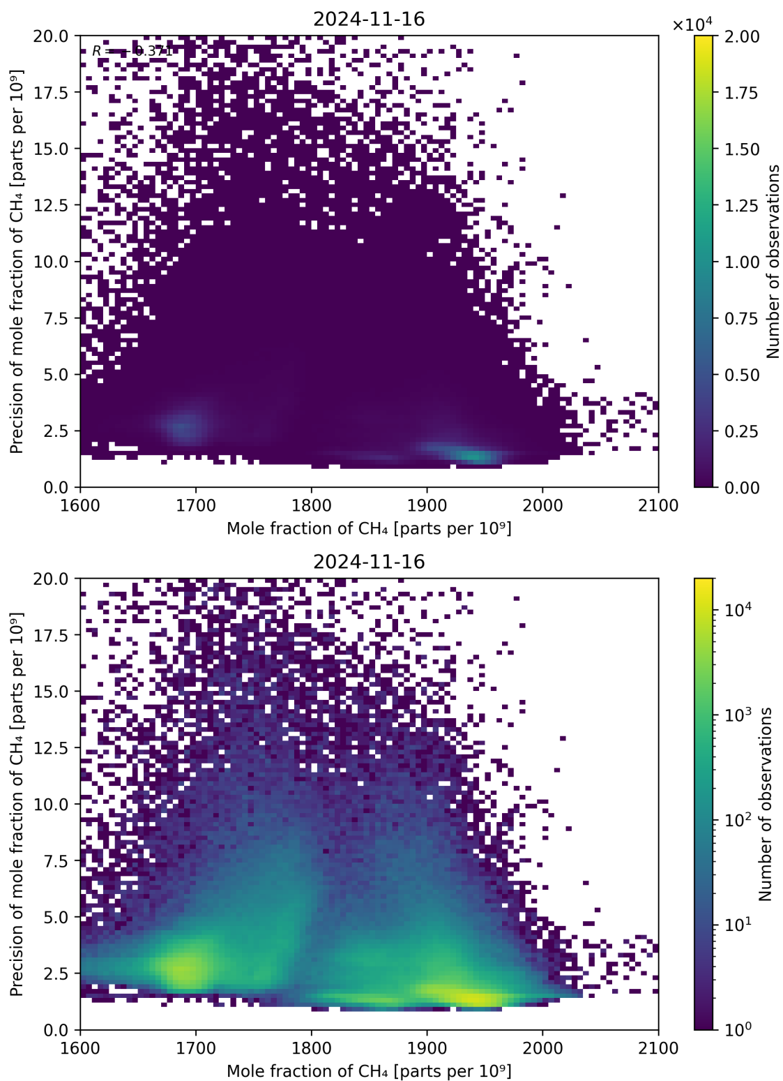
Figure 75: Scatter density plot of “Mole fraction of CH 4 ” against “Precision of mole fraction of CH 4 ” for 2024-11-15 to 2024-11-17.
