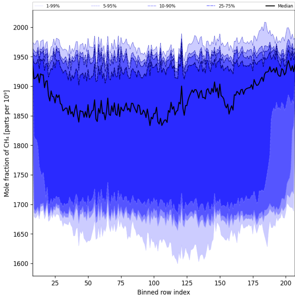
Figure 34: Along track statistics of “Mole fraction of CH 4 ” for 2024-11-15 to 2024-11-17
