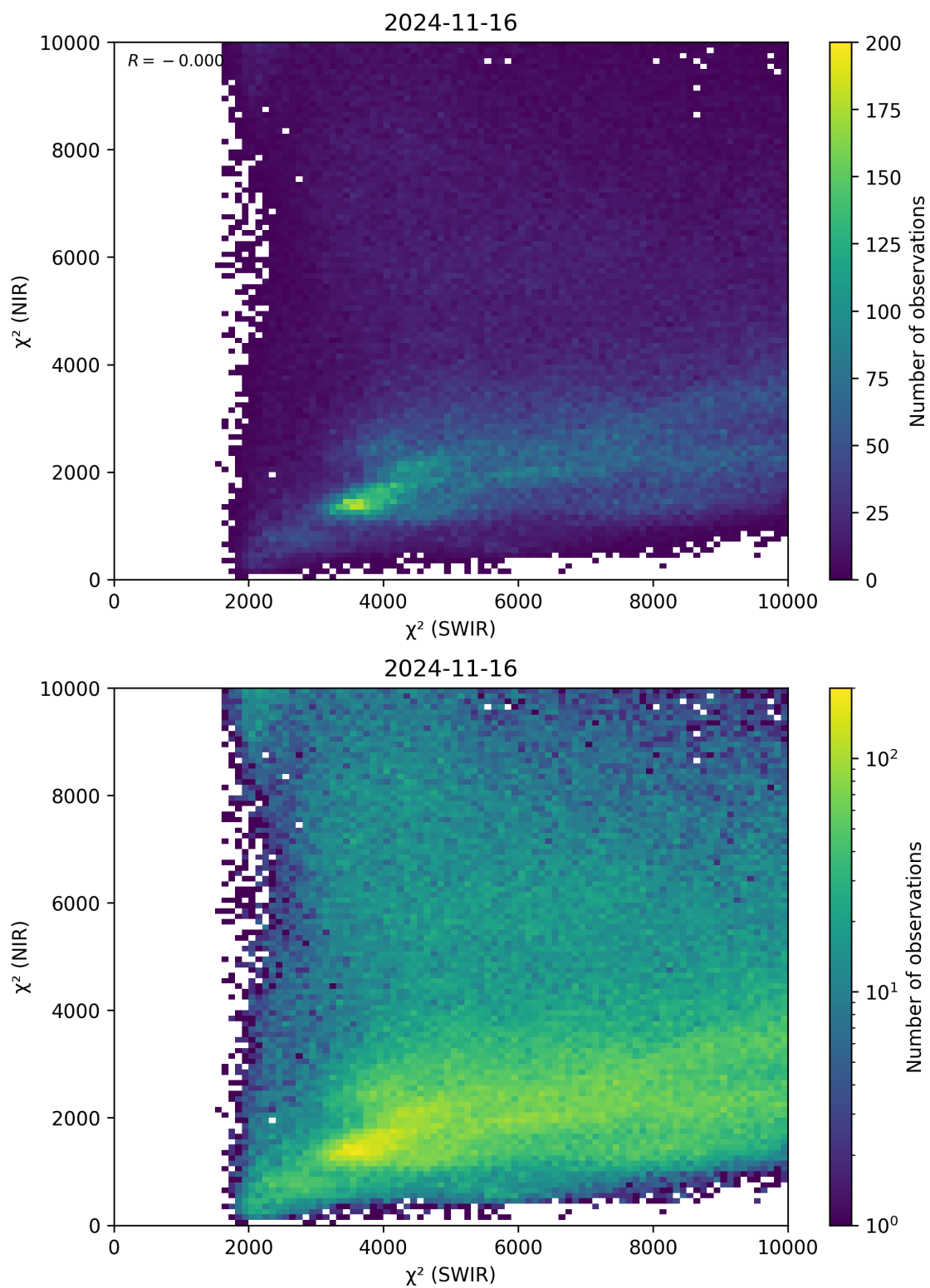
Figure 47: Scatter density plot of “ \chi^2 (SWIR)” against “ \chi^2 (NIR)” for 2024-11-15 to 2024-11-17.
