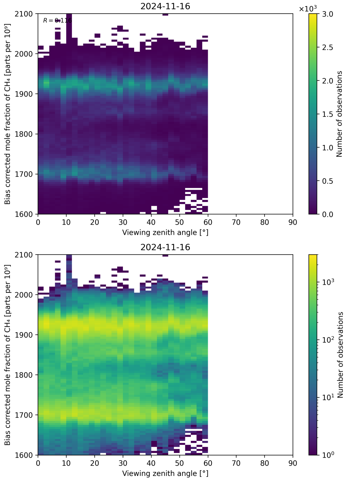
Figure 111: Scatter density plot of “Viewing zenith angle” against “Bias corrected mole fraction of CH 4 ” for 2024-11-15 to 2024-11-17.
