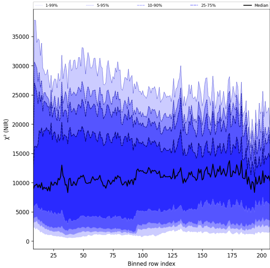
Figure 40: Along track statistics of “ \chi^2 (NIR)” for 2024-11-15 to 2024-11-17
