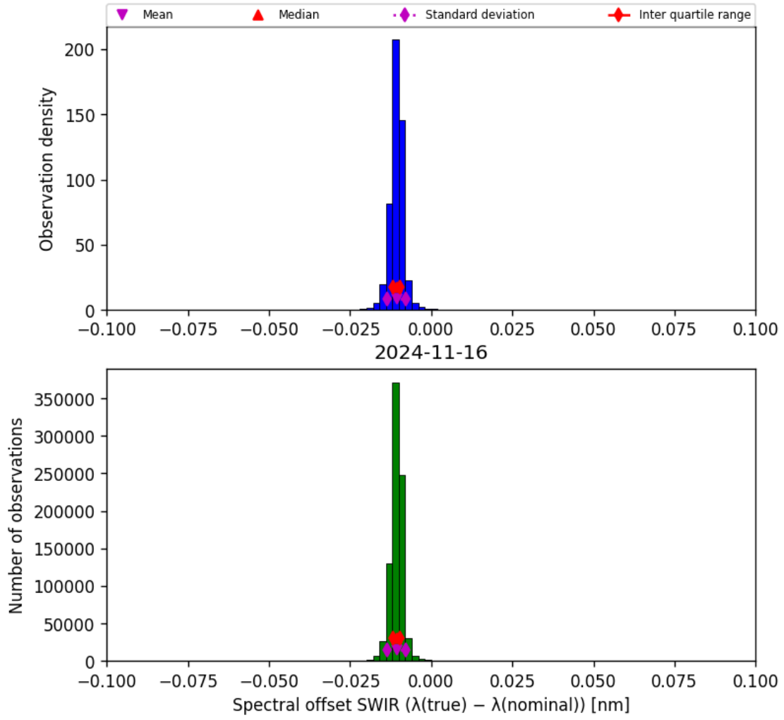
Figure 27: Histogram of “Spectral offset SWIR ( \lambda_{\text{true}} - \lambda_{\text{nominal}} )” for 2024-11-15 to 2024-11-17
