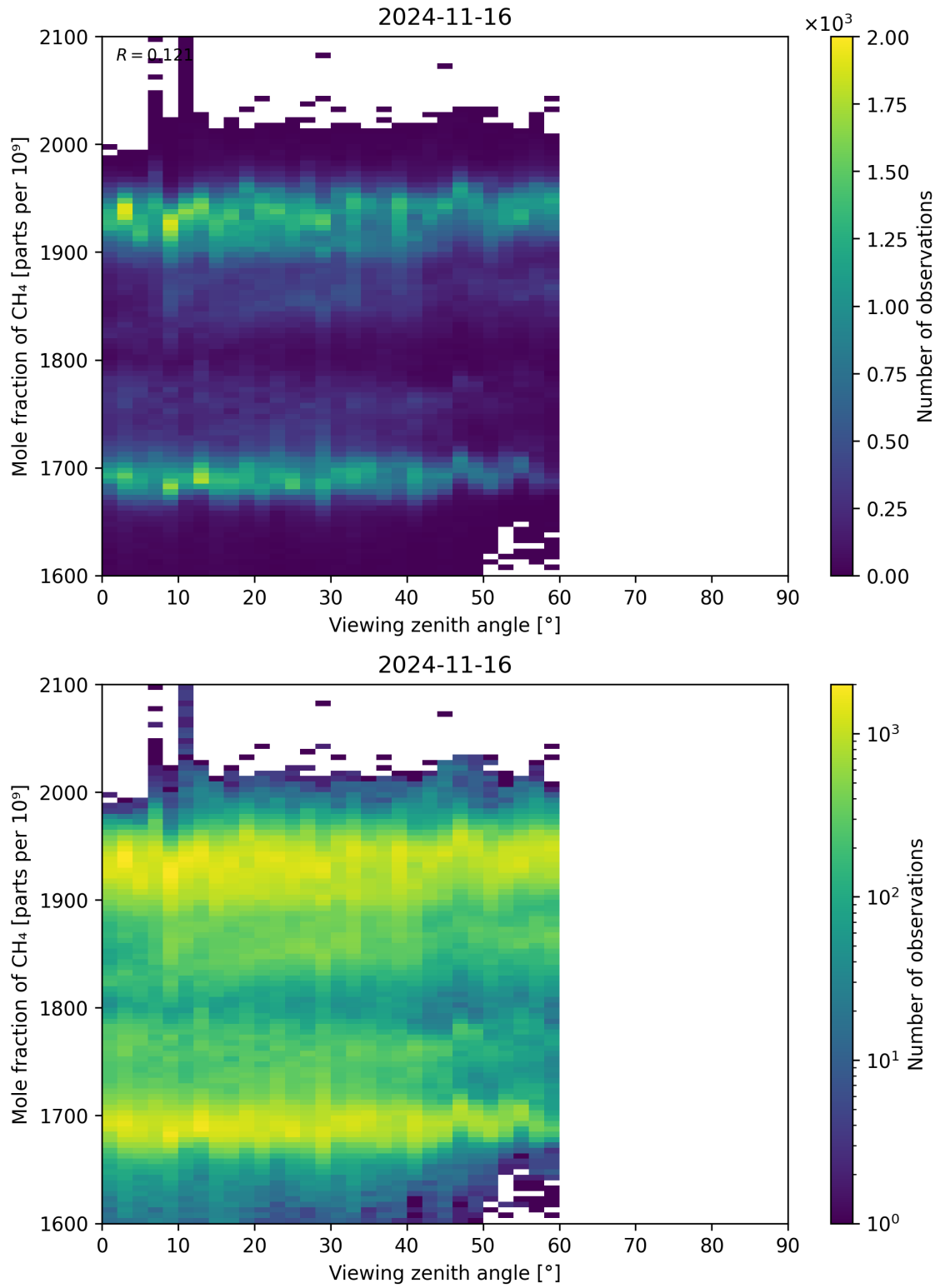
Figure 110: Scatter density plot of “Viewing zenith angle” against “Mole fraction of CH 4 ” for 2024-11-15 to 2024-11-17.
