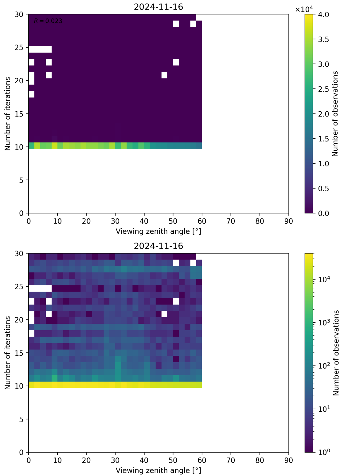
Figure 113: Scatter density plot of “Viewing zenith angle” against “Number of iterations” for 2024-11-15 to 2024-11-17.
