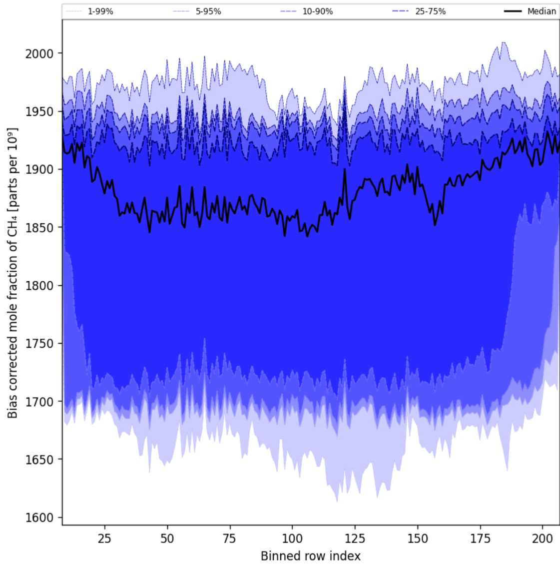
Figure 36: Along track statistics of “Bias corrected mole fraction of CH 4 ” for 2024-11-15 to 2024-11-17
