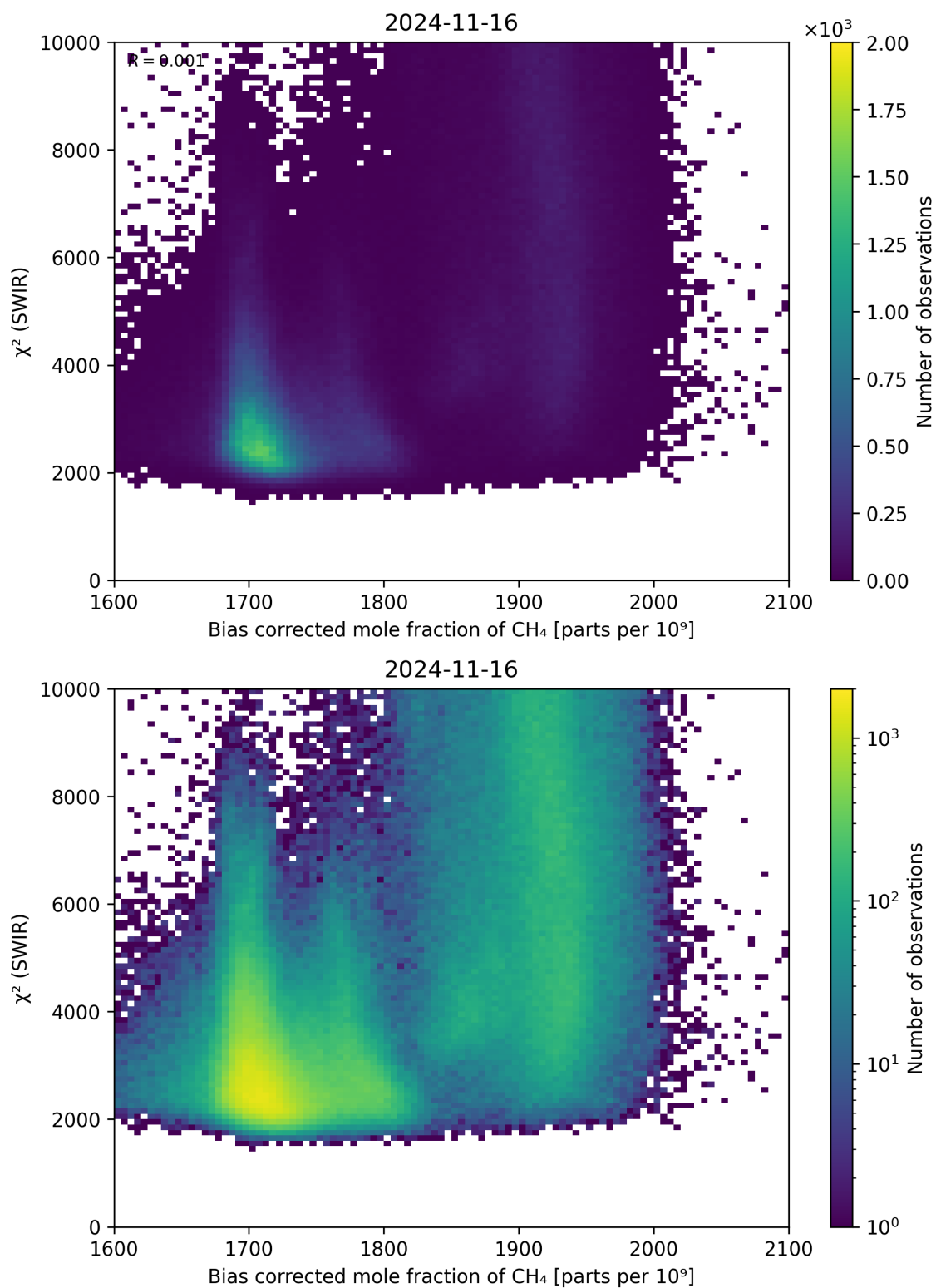
Figure 64: Scatter density plot of “Bias corrected mole fraction of \text{CH}_4 ” against “ \chi^2 (SWIR)” for 2024-11-15 to 2024-11-17.
