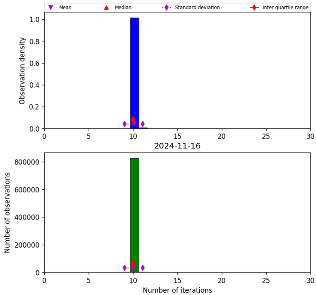
Figure 31: Histogram of “Number of iterations” for 2024-11-15 to 2024-11-17
