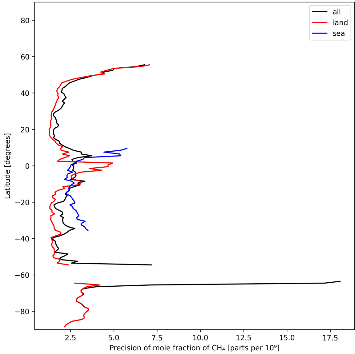
Figure 13: Zonal average of “Precision of mole fraction of CH 4 ” for 2024-11-15 to 2024-11-17.
