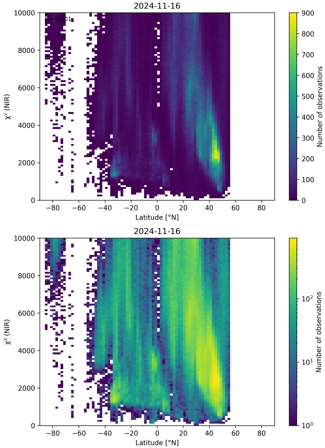
Figure 53: Scatter density plot of “Latitude” against “ \chi^2 (NIR)” for 2024-11-15 to 2024-11-17.
