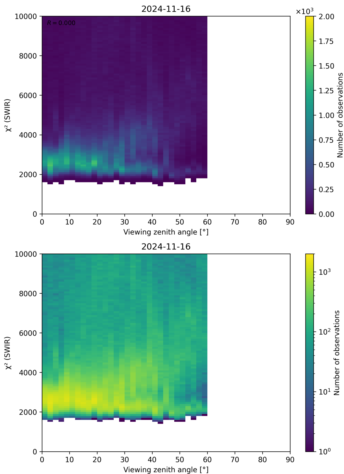
Figure 106: Scatter density plot of “Viewing zenith angle” against “ \chi^2 (SWIR)” for 2024-11-15 to 2024-11-17.
