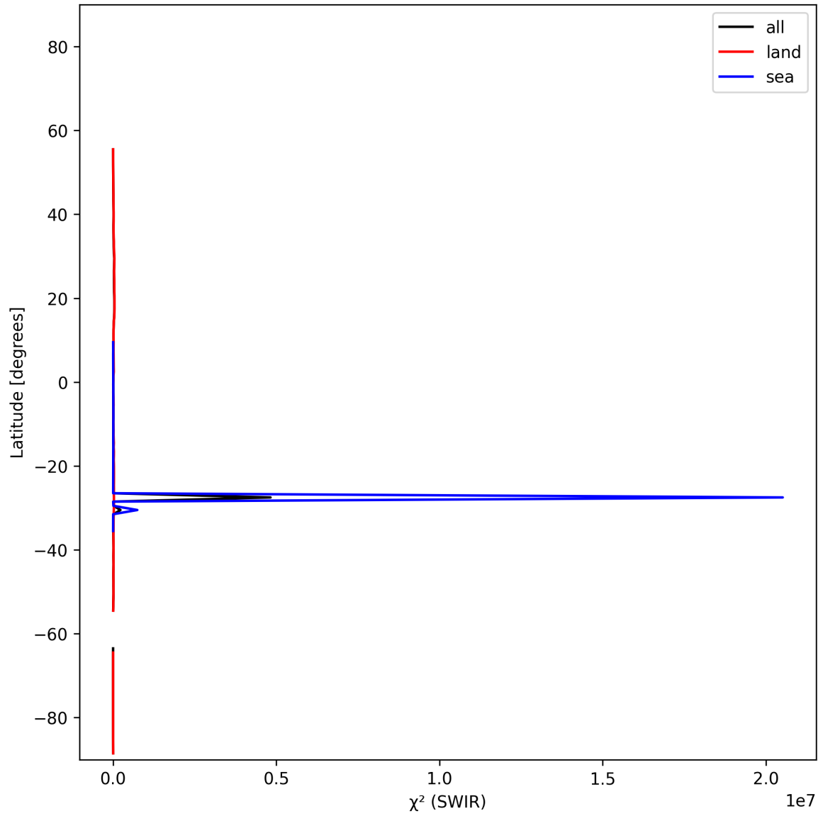
Figure 17: Zonal average of “ \chi^2 (SWIR)” for 2024-11-15 to 2024-11-17.
