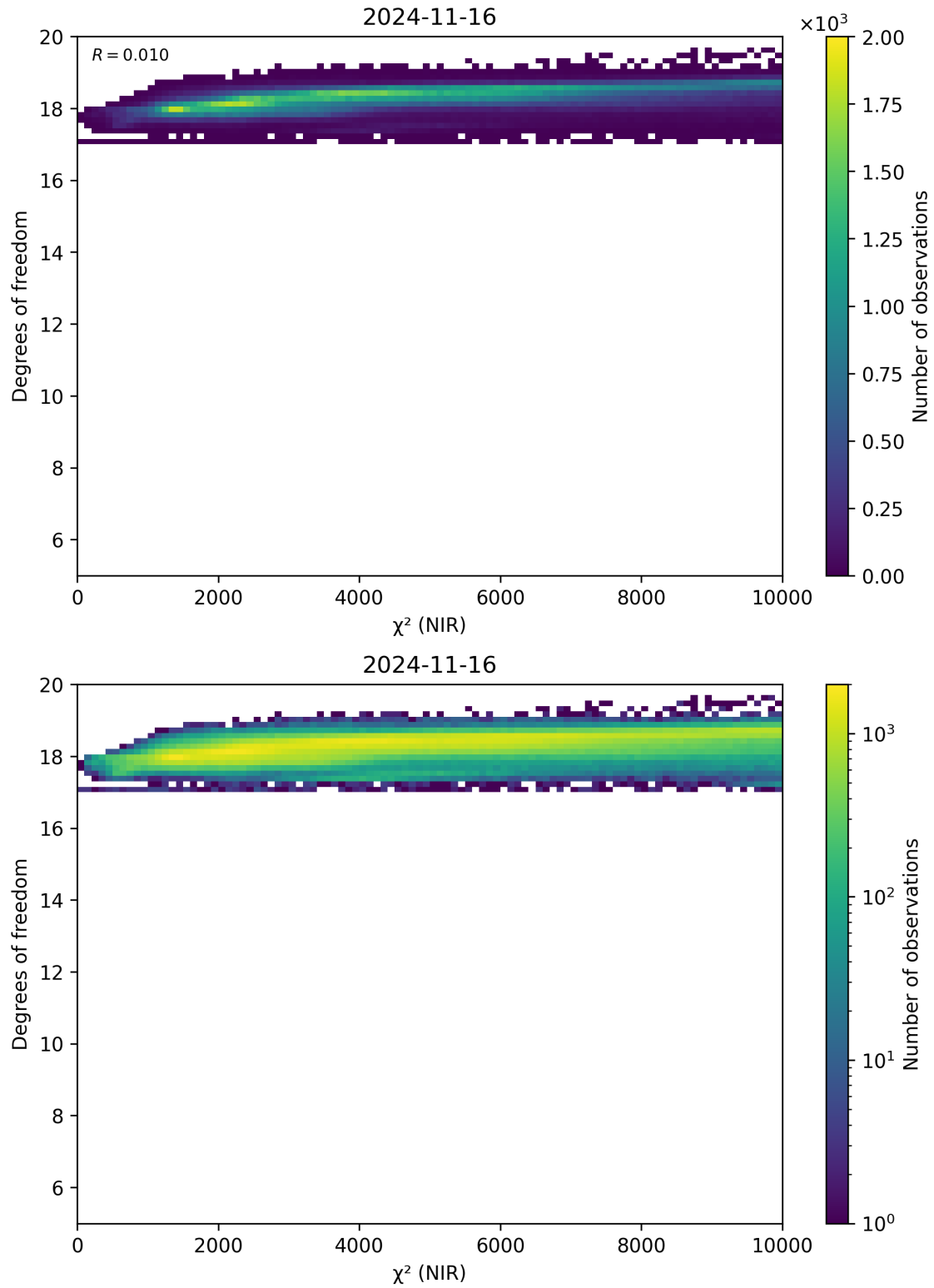
Figure 44: Scatter density plot of “ \chi^2 (NIR)” against “Degrees of freedom” for 2024-11-15 to 2024-11-17.
