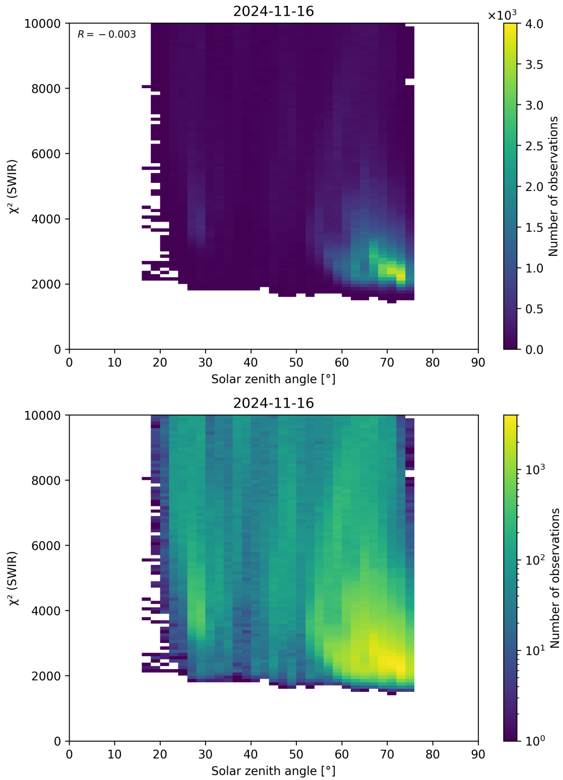
Figure 95: Scatter density plot of “Solar zenith angle” against “ \chi^2 (SWIR)” for 2024-11-15 to 2024-11-17.
