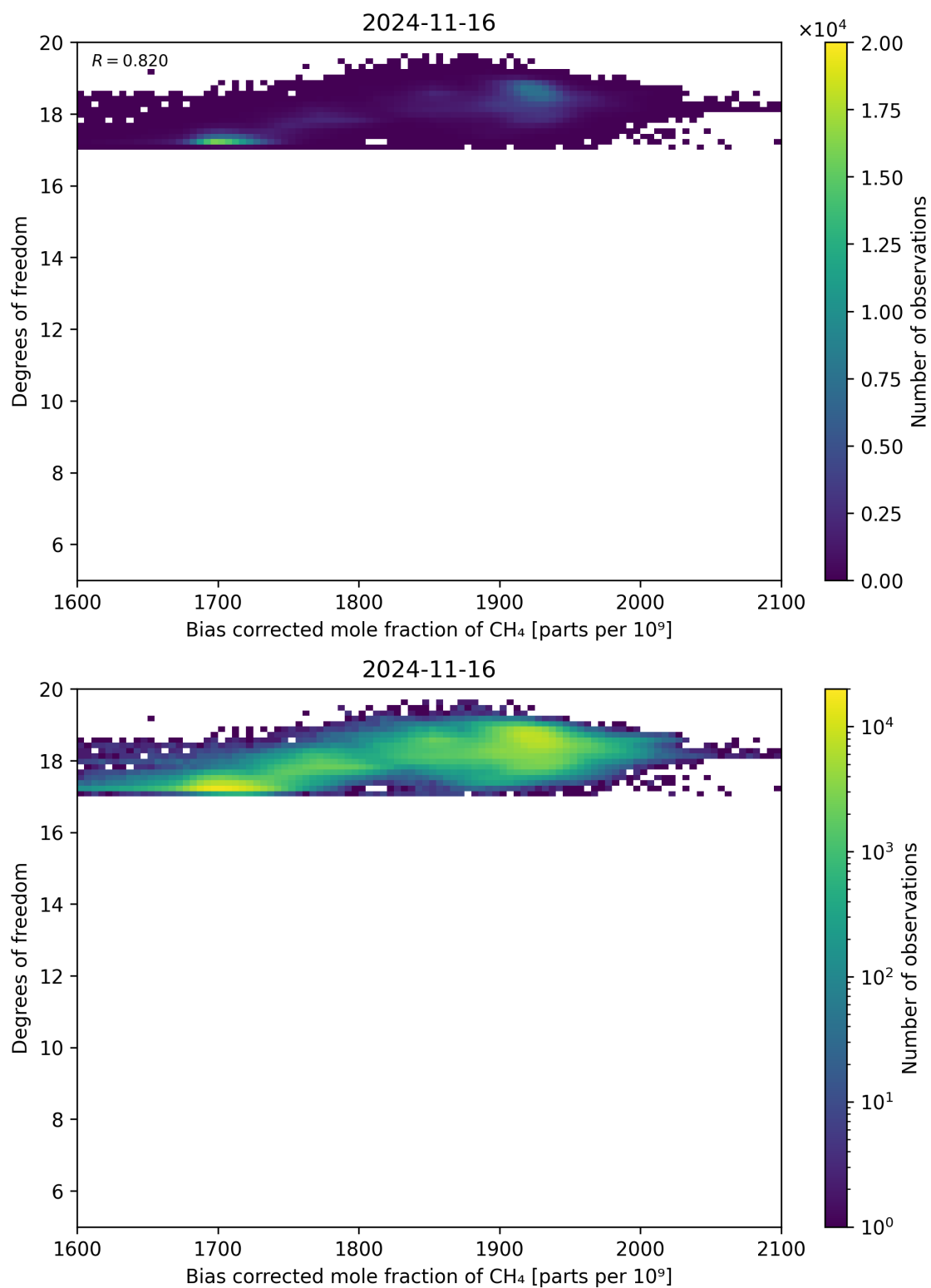
Figure 65: Scatter density plot of “Bias corrected mole fraction of CH 4 ” against “Degrees of freedom” for 2024-11-15 to 2024-11-17.
