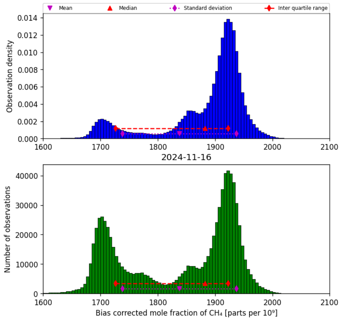
Figure 25: Histogram of “Bias corrected mole fraction of CH 4 ” for 2024-11-15 to 2024-11-17
