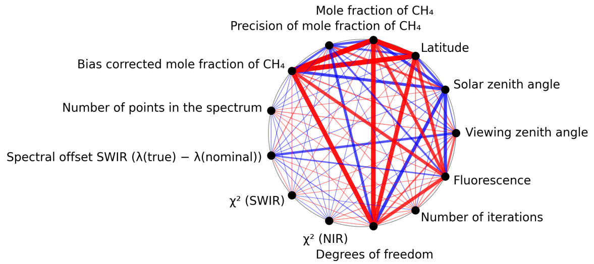
Figure 1: Map of correlation graph for 2024-11-15 to 2024-11-17.
