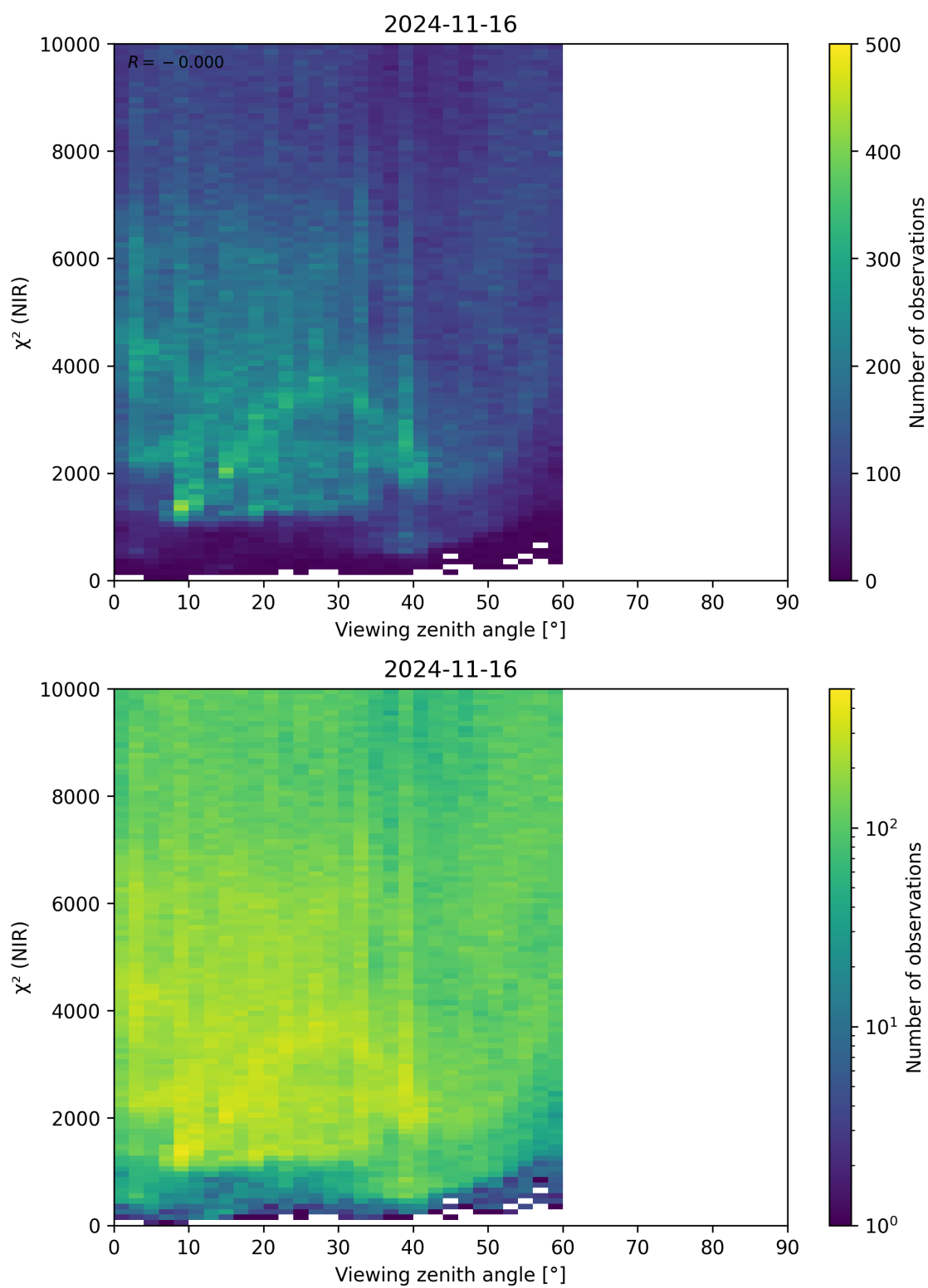
Figure 105: Scatter density plot of “Viewing zenith angle” against “ \chi^2 (NIR)” for 2024-11-15 to 2024-11-17.
