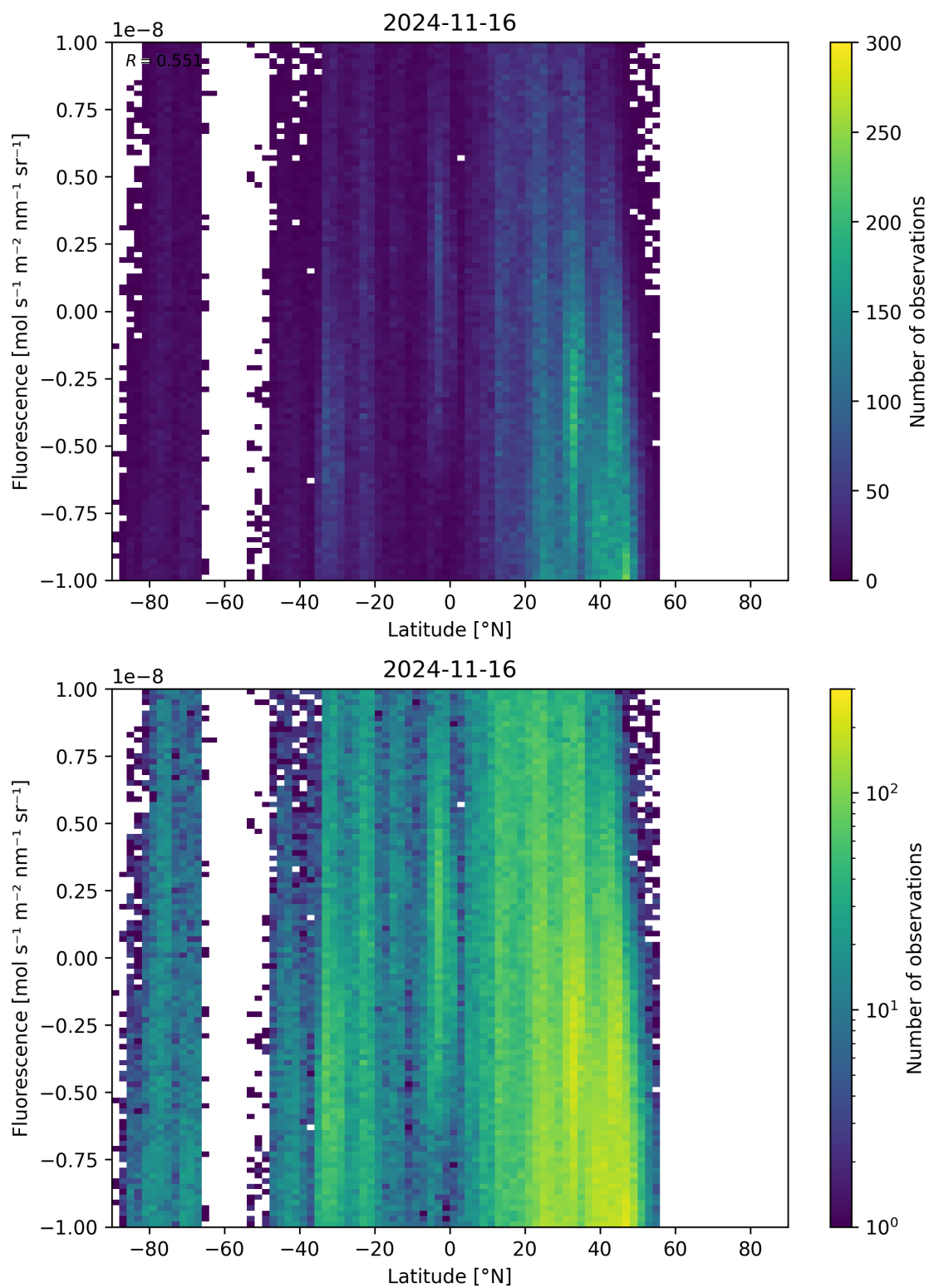
Figure 56: Scatter density plot of “Latitude” against “Fluorescence” for 2024-11-15 to 2024-11-17.
