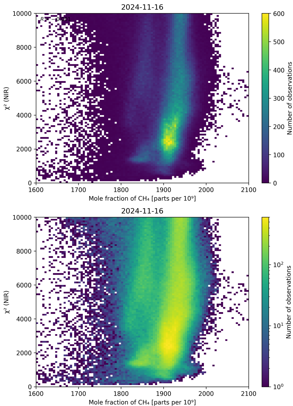
Figure 70: Scatter density plot of “Mole fraction of \text{CH}_4 ” against “ \chi^2 (NIR)” for 2024-11-15 to 2024-11-17.
