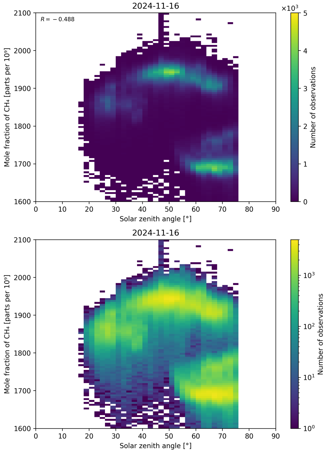
Figure 99: Scatter density plot of “Solar zenith angle” against “Mole fraction of CH 4 ” for 2024-11-15 to 2024-11-17.
