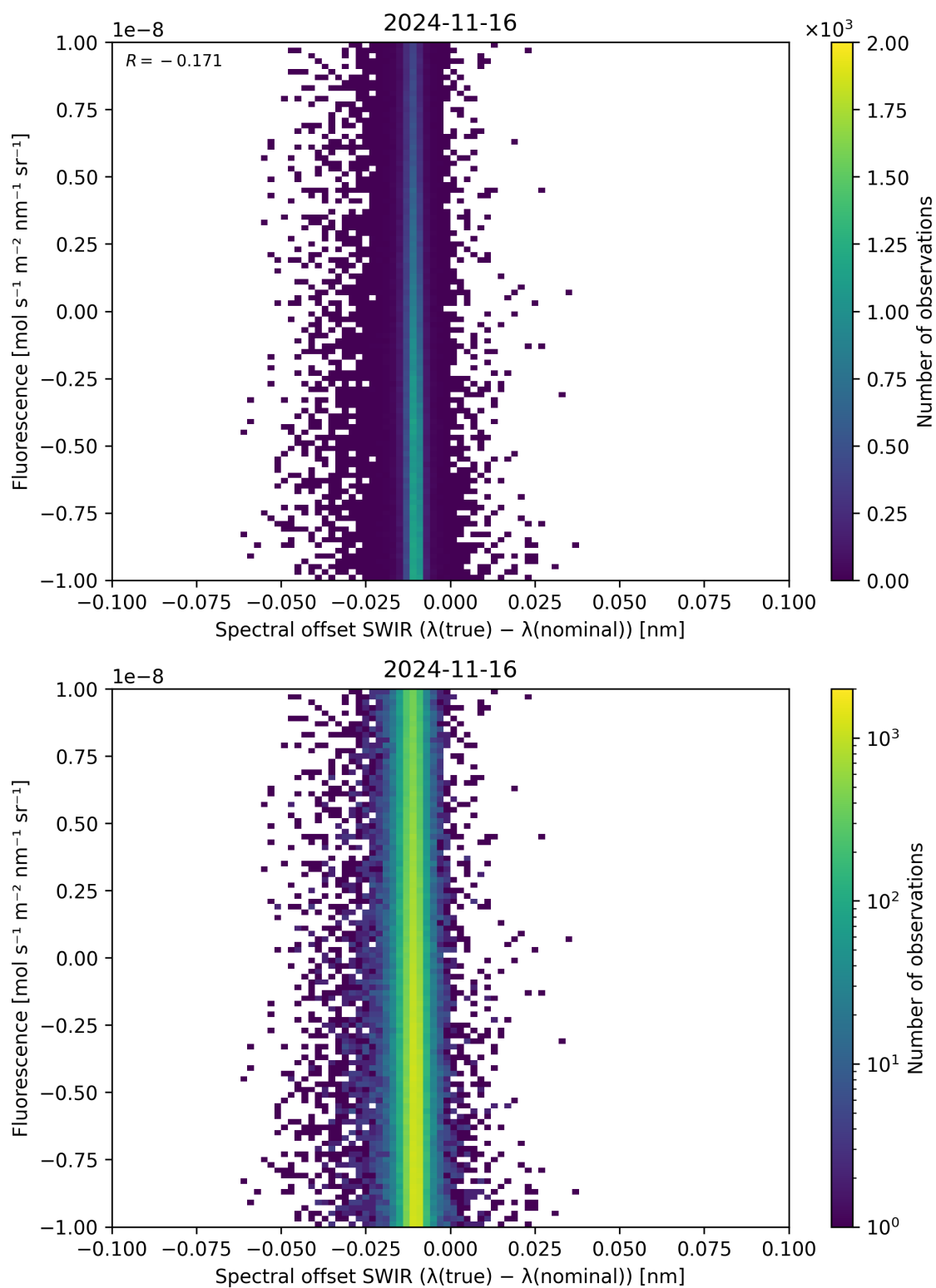
Figure 120: Scatter density plot of “Spectral offset SWIR ( \lambda_{\text{true}} - \lambda_{\text{nominal}} )” against “Fluorescence” for 2024-11-15 to 2024-11-17.
