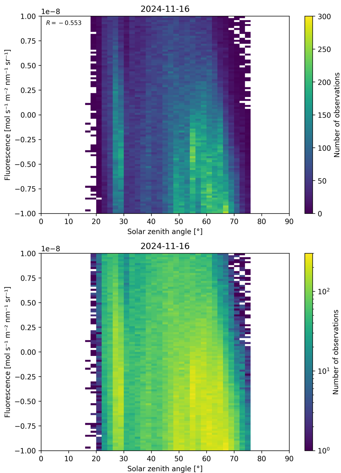
Figure 97: Scatter density plot of “Solar zenith angle” against “Fluorescence” for 2024-11-15 to 2024-11-17.
