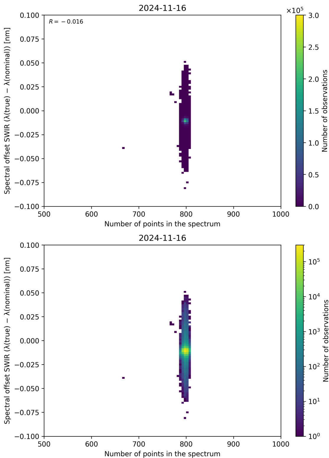
Figure 93: Scatter density plot of “Number of points in the spectrum” against “Spectral offset SWIR ( \lambda_{\text{true}} - \lambda_{\text{nominal}} )” for 2024-11-15 to 2024-11-17.
