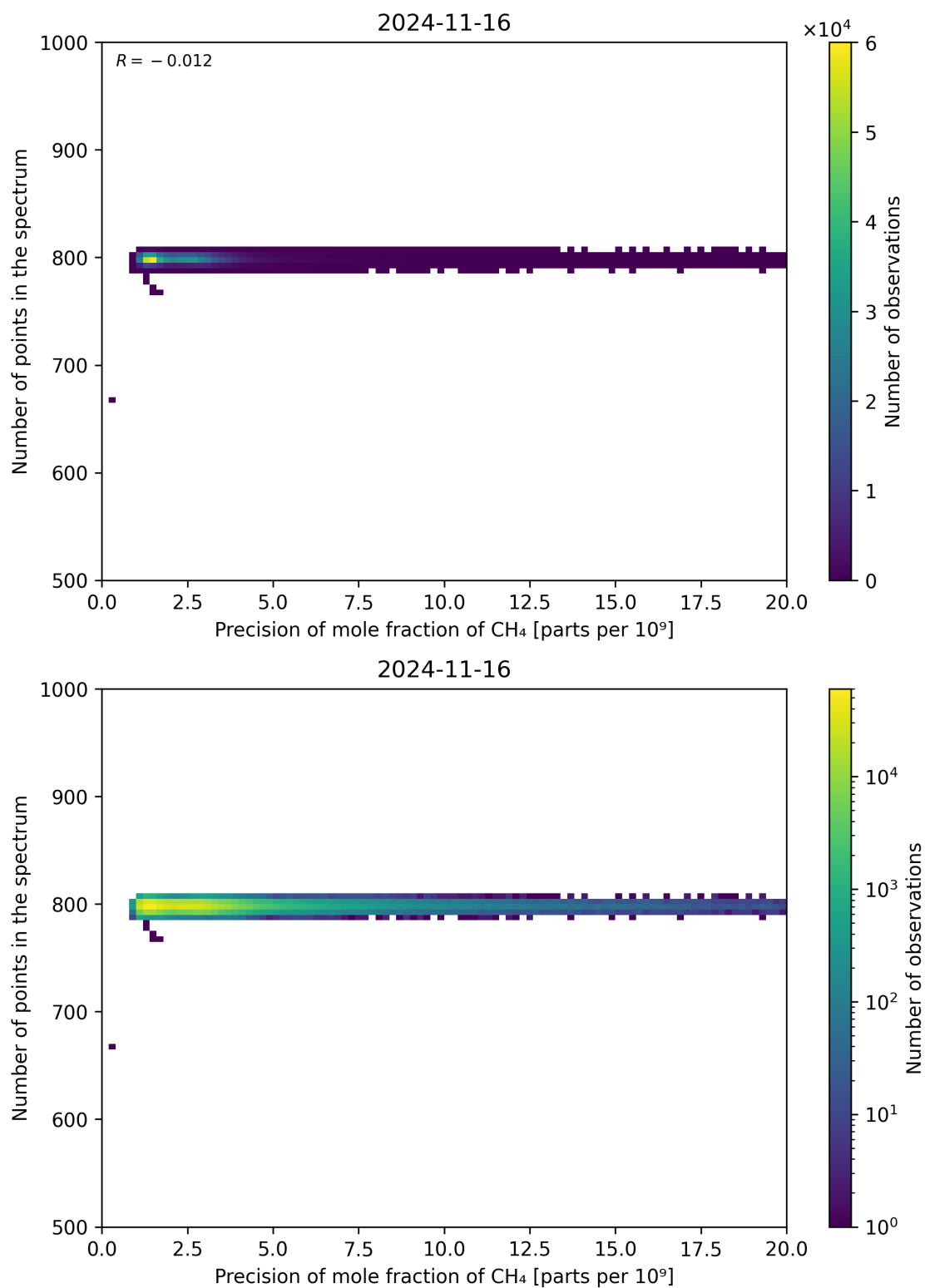
Figure 84: Scatter density plot of “Precision of mole fraction of CH 4 ” against “Number of points in the spectrum” for 2024-11-15 to 2024-11-17.
