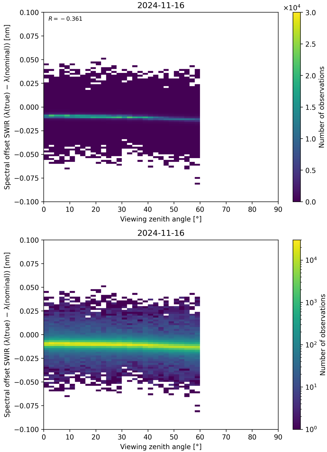
Figure 116: Scatter density plot of “Viewing zenith angle” against “Spectral offset SWIR ( \lambda_{\text{true}} - \lambda_{\text{nominal}} )” for 2024-11-15 to 2024-11-17.
