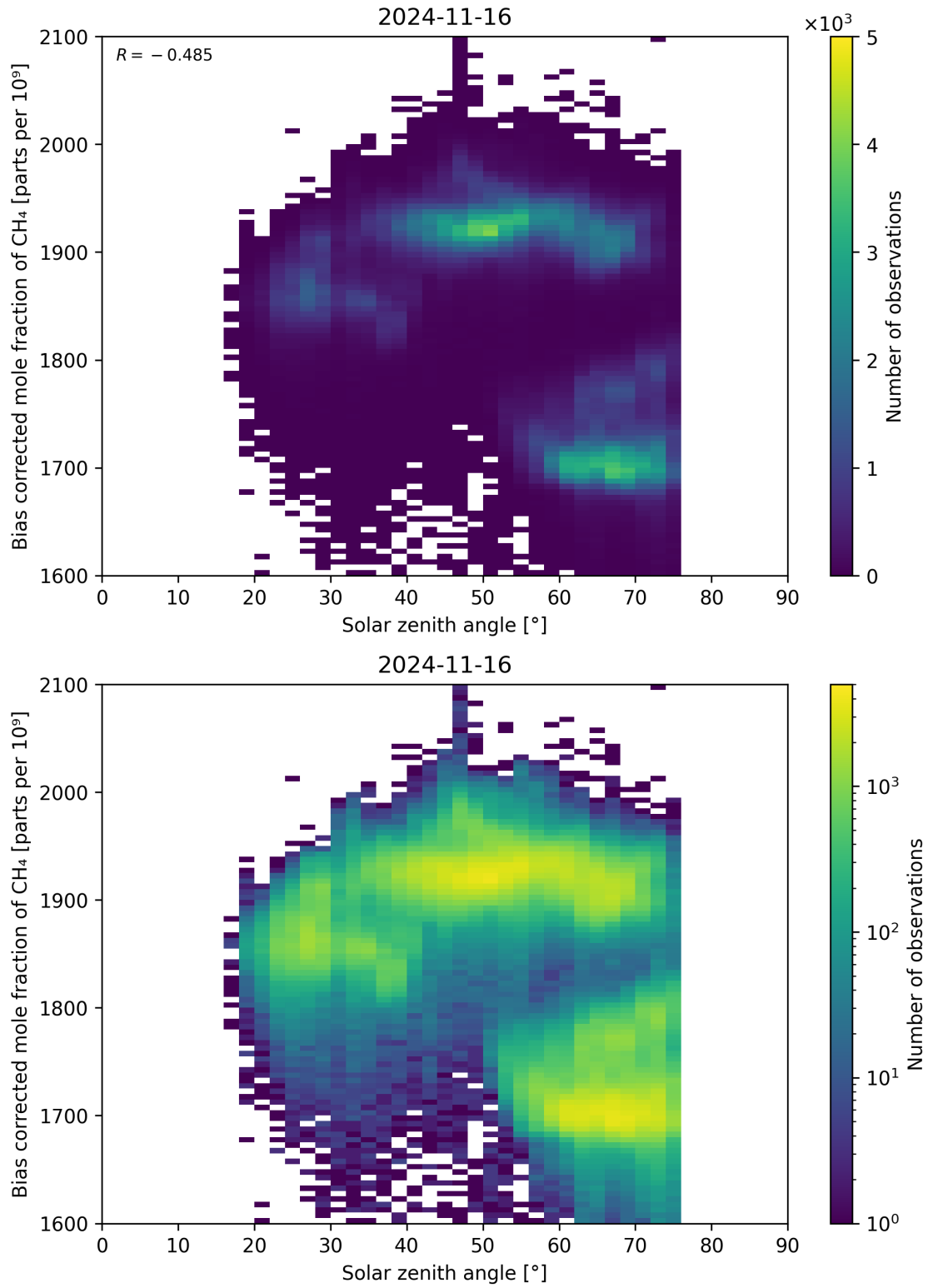
Figure 100: Scatter density plot of “Solar zenith angle” against “Bias corrected mole fraction of CH 4 ” for 2024-11-15 to 2024-11-17.
