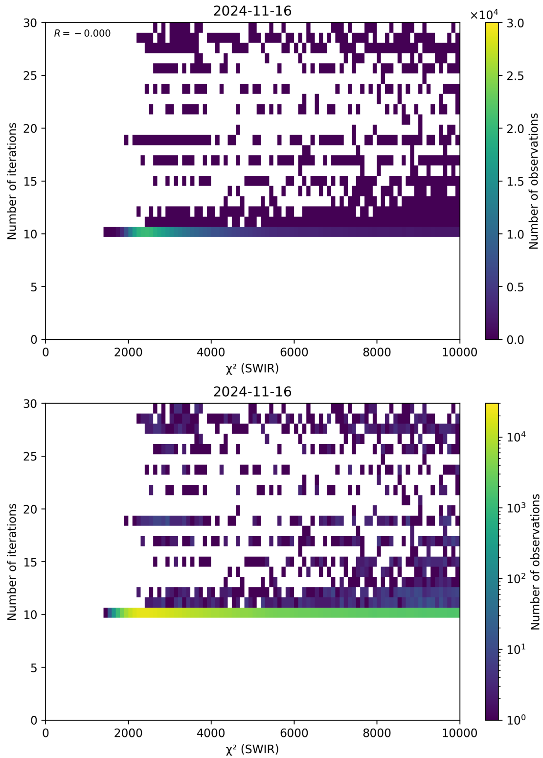
Figure 50: Scatter density plot of “ \chi^2 (SWIR)” against “Number of iterations” for 2024-11-15 to 2024-11-17.
