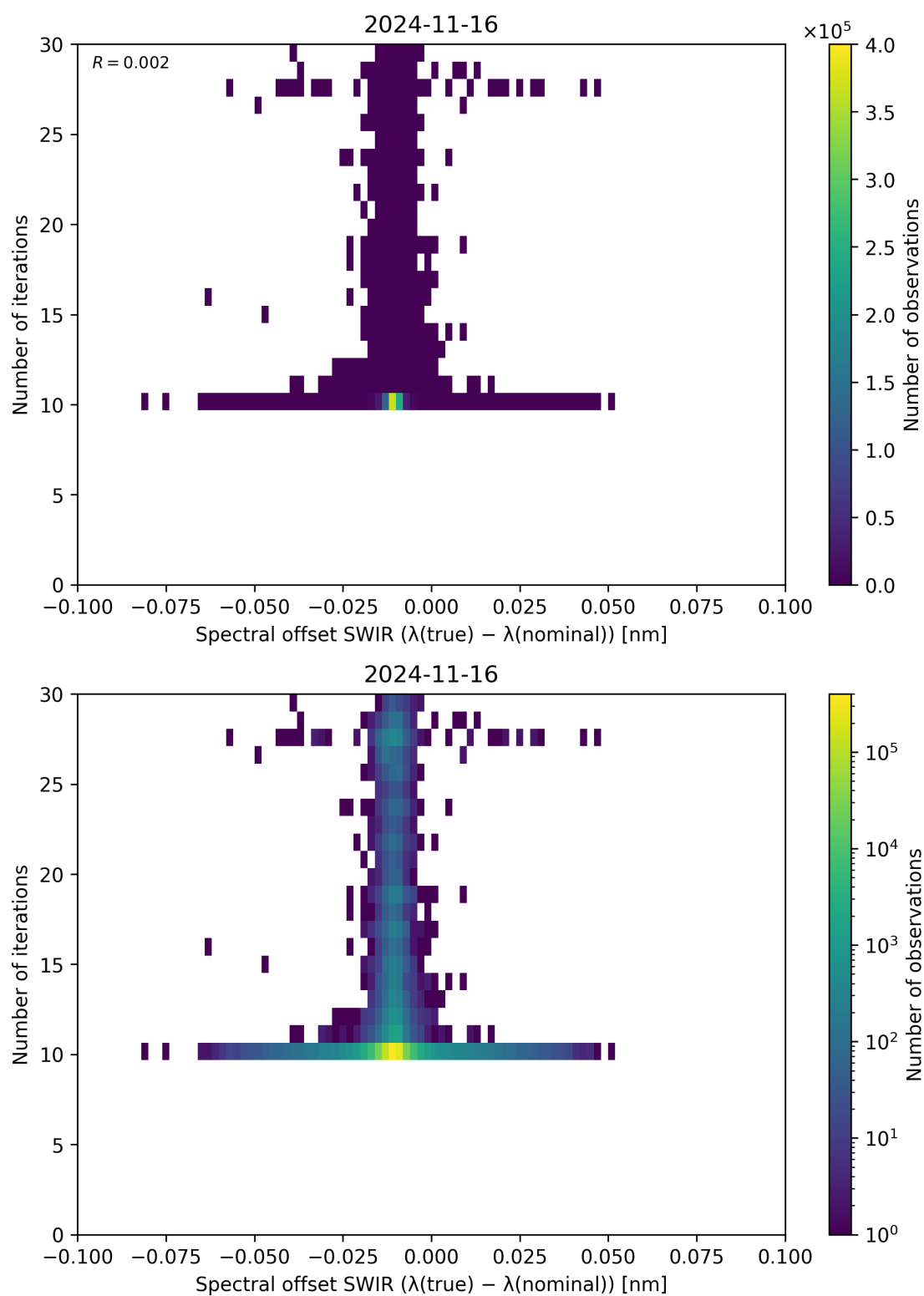
Figure 121: Scatter density plot of “Spectral offset SWIR ( \lambda_{\text{true}} - \lambda_{\text{nominal}} )” against “Number of iterations” for 2024-11-15 to 2024-11-17.
