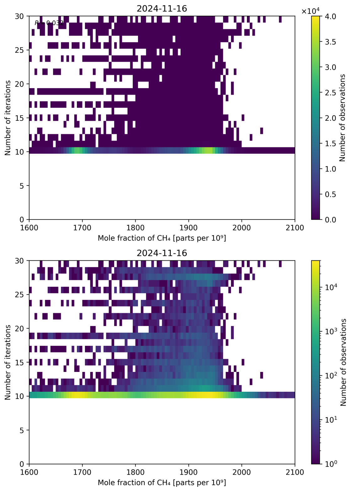
Figure 76: Scatter density plot of “Mole fraction of CH 4 ” against “Number of iterations” for 2024-11-15 to 2024-11-17.
