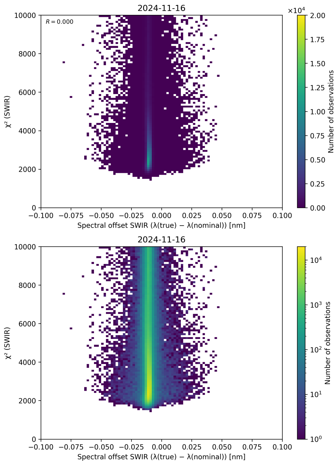
Figure 118: Scatter density plot of “Spectral offset SWIR ( \lambda_{\text{true}} - \lambda_{\text{nominal}} )” against “ \chi^2 (SWIR)” for 2024-11-15 to 2024-11-17.
