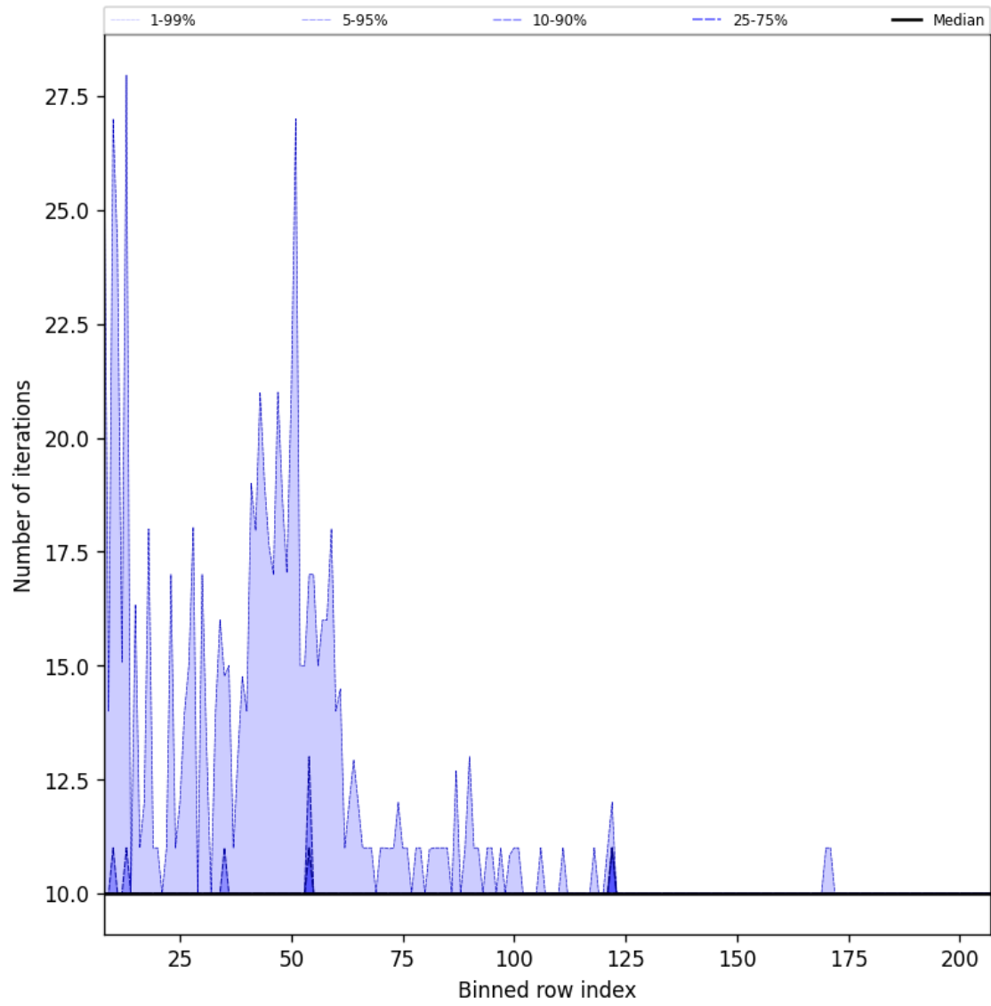
Figure 42: Along track statistics of “Number of iterations” for 2024-11-15 to 2024-11-17
