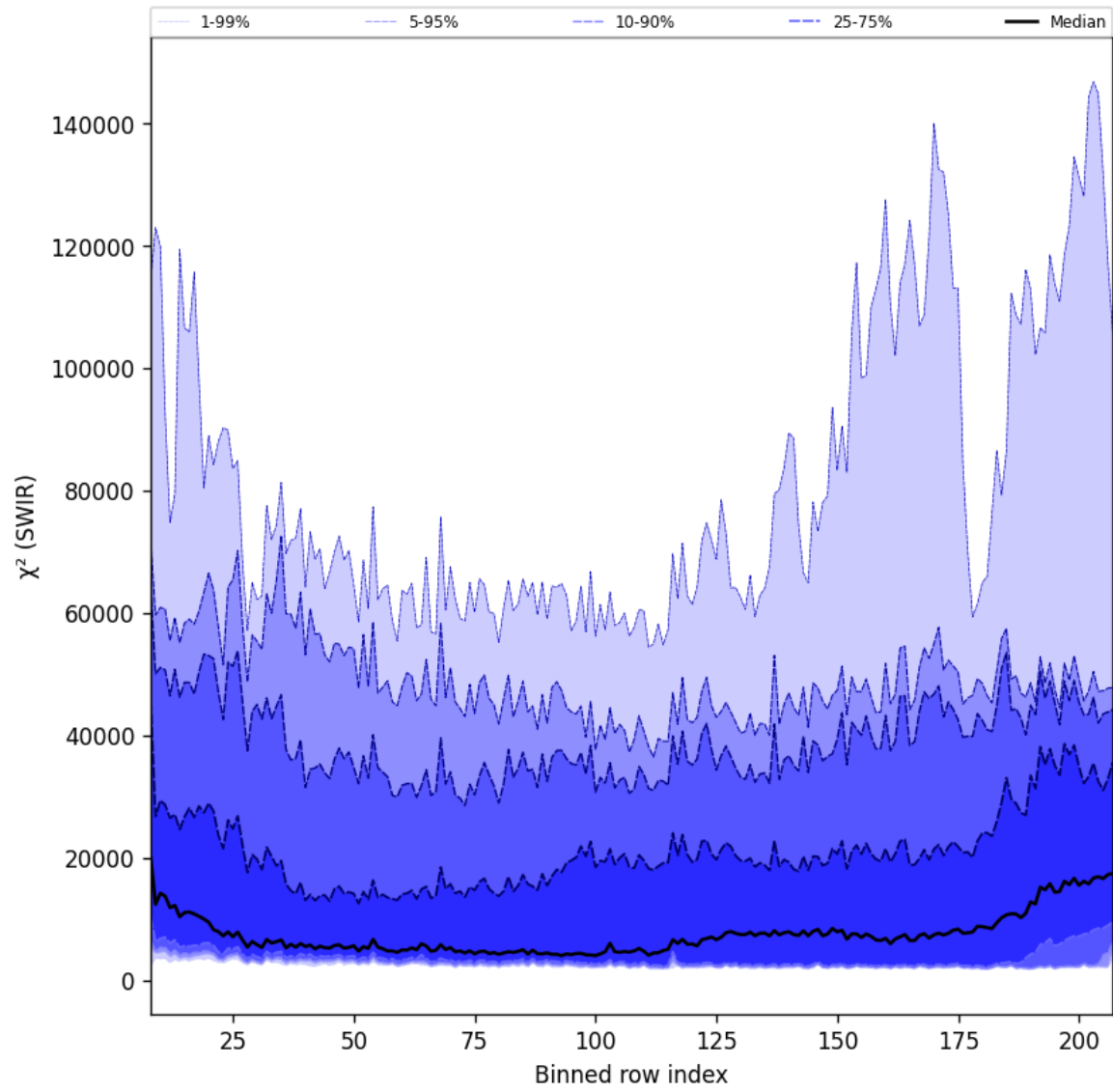
Figure 39: Along track statistics of " \chi^2 (SWIR)" for 2024-11-15 to 2024-11-17
