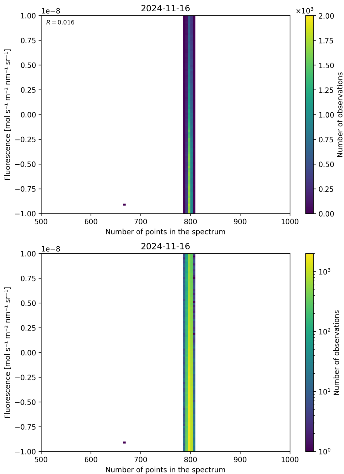
Figure 91: Scatter density plot of “Number of points in the spectrum” against “Fluorescence” for 2024-11-15 to 2024-11-17.
