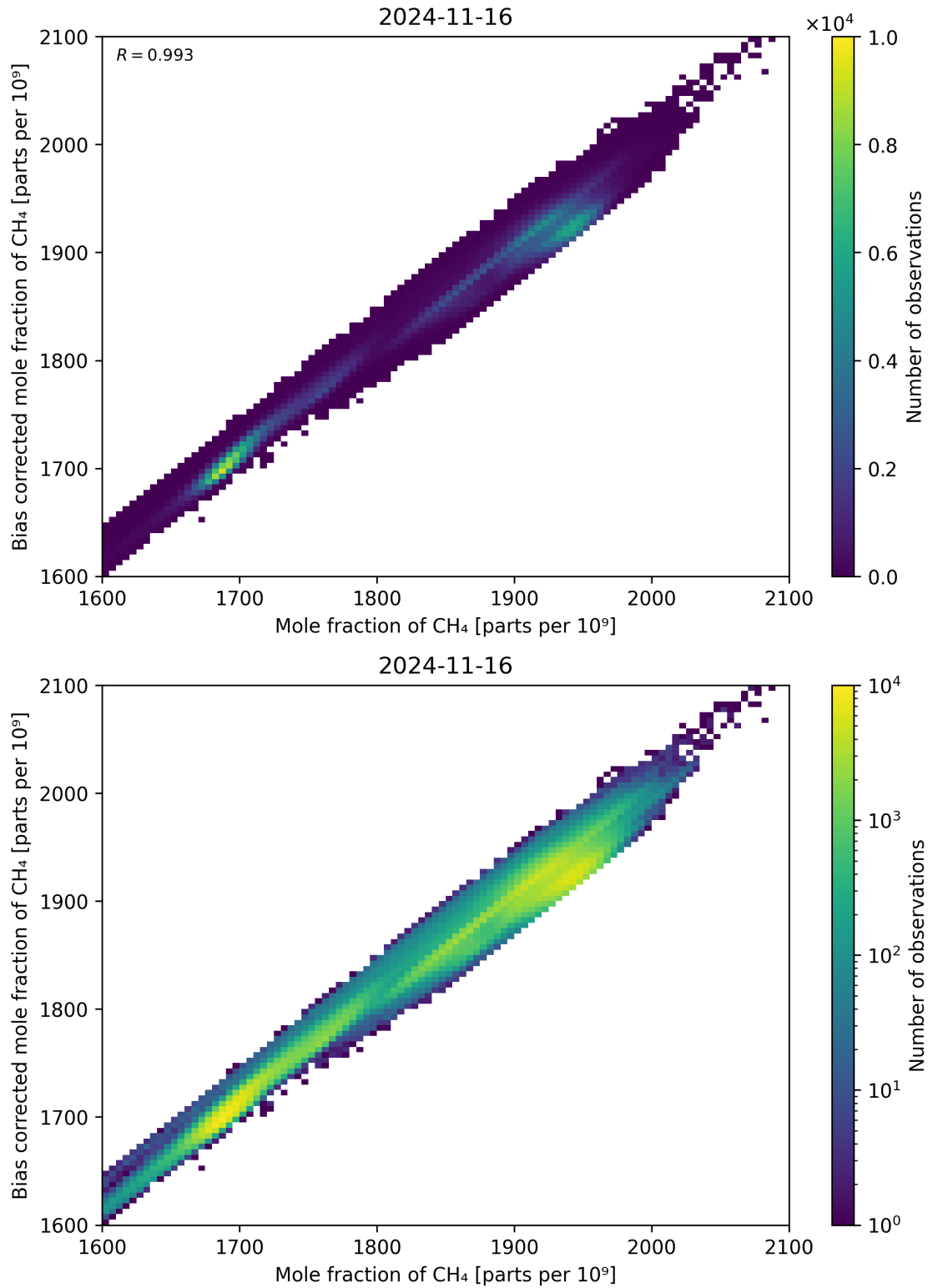
Figure 74: Scatter density plot of “Mole fraction of CH 4 ” against “Bias corrected mole fraction of CH 4 ” for 2024-11-15 to 2024-11-17.
