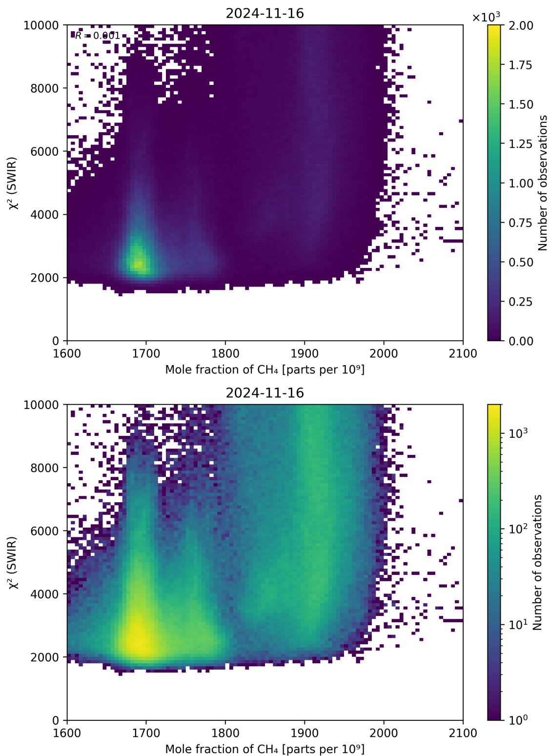
Figure 71: Scatter density plot of “Mole fraction of \text{CH}_4 ” against “ \chi^2 (SWIR)” for 2024-11-15 to 2024-11-17.
