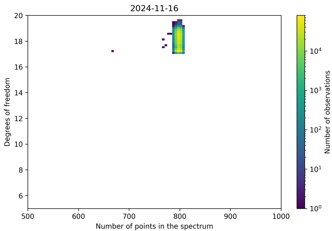
Figure 90: Scatter density plot of “Number of points in the spectrum” against “Degrees of freedom” for 2024-11-15 to 2024-11-17.
