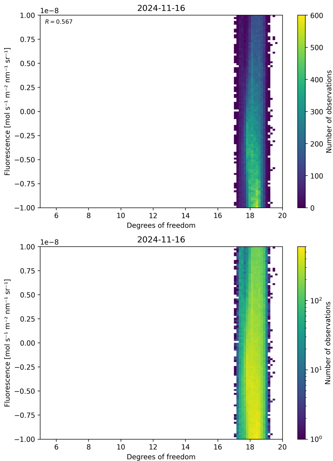
Figure 51: Scatter density plot of “Degrees of freedom” against “Fluorescence” for 2024-11-15 to 2024-11-17.
