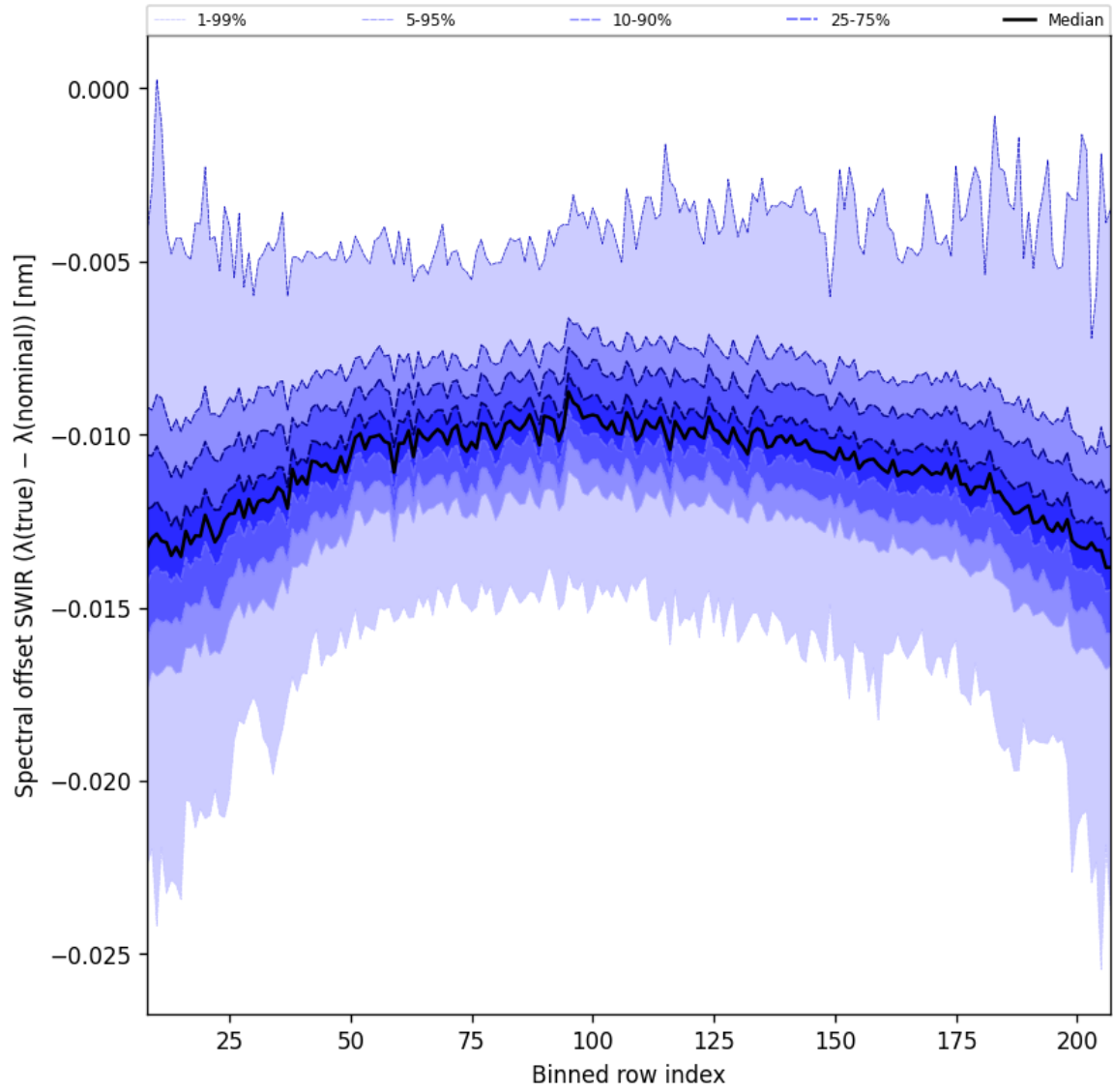
Figure 38: Along track statistics of “Spectral offset SWIR ( \lambda_{\text{true}} - \lambda_{\text{nominal}} )” for 2024-11-15 to 2024-11-17
