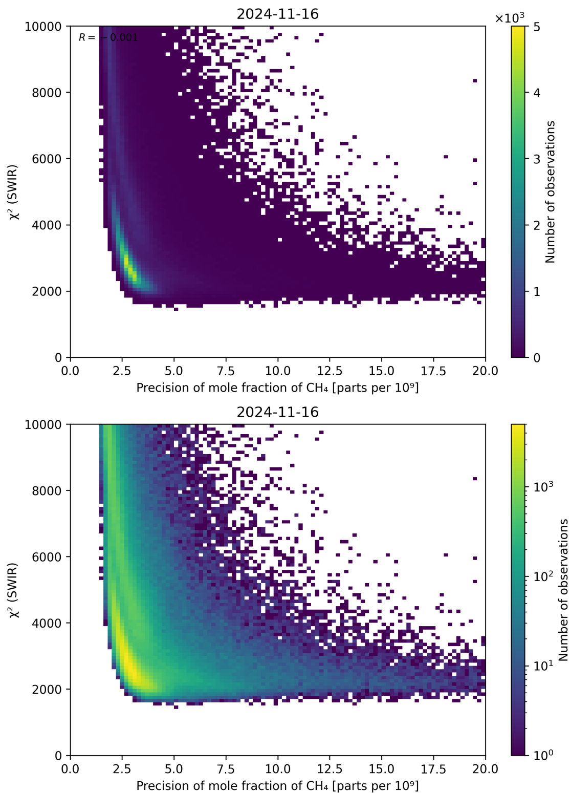
Figure 79: Scatter density plot of “Precision of mole fraction of \text{CH}_4 ” against “ \chi^2 (SWIR)” for 2024-11-15 to 2024-11-17.
