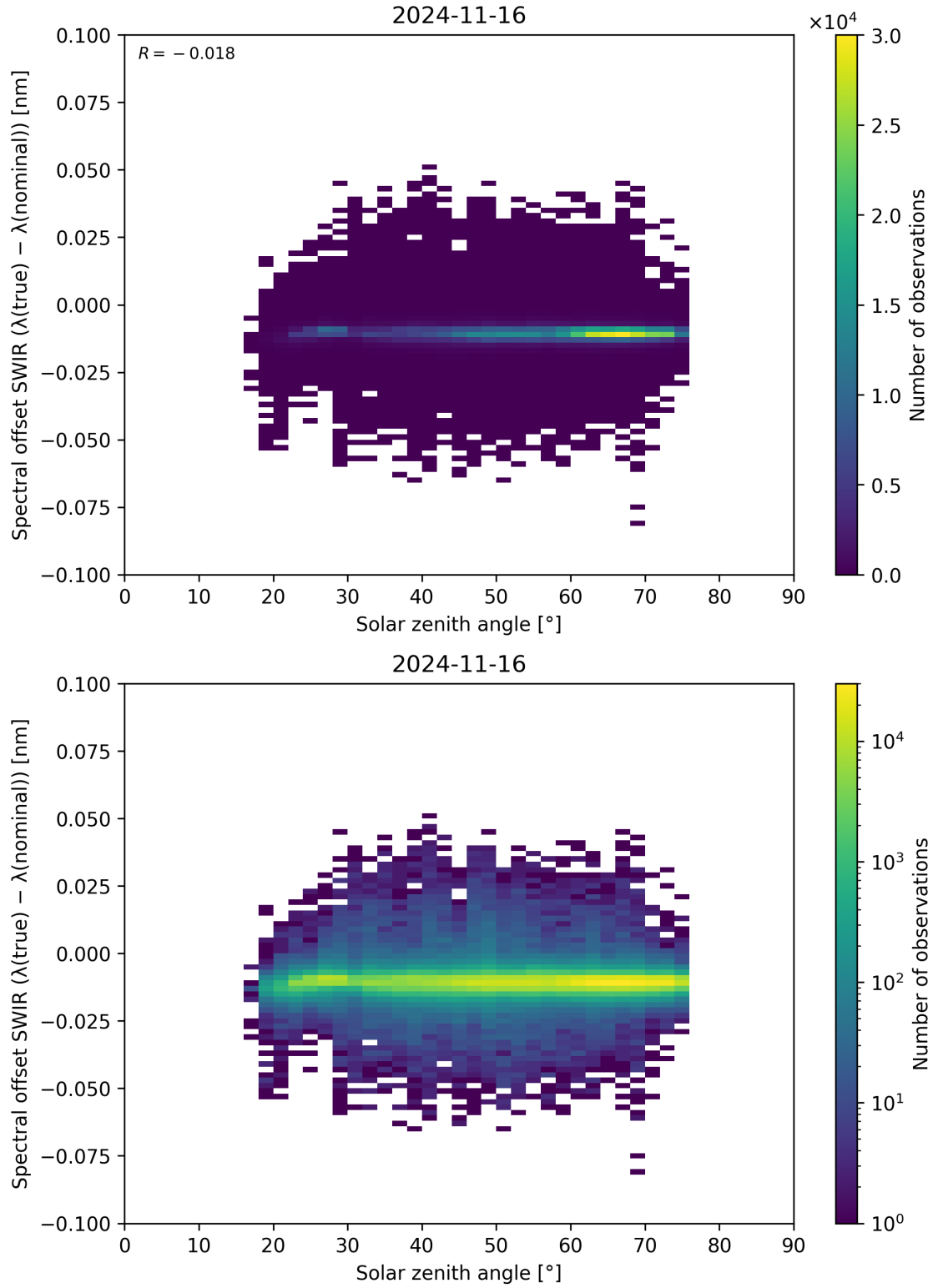
Figure 104: Scatter density plot of “Solar zenith angle” against “Spectral offset SWIR ( \lambda_{\text{true}} - \lambda_{\text{nominal}} )” for 2024-11-15 to 2024-11-17.
