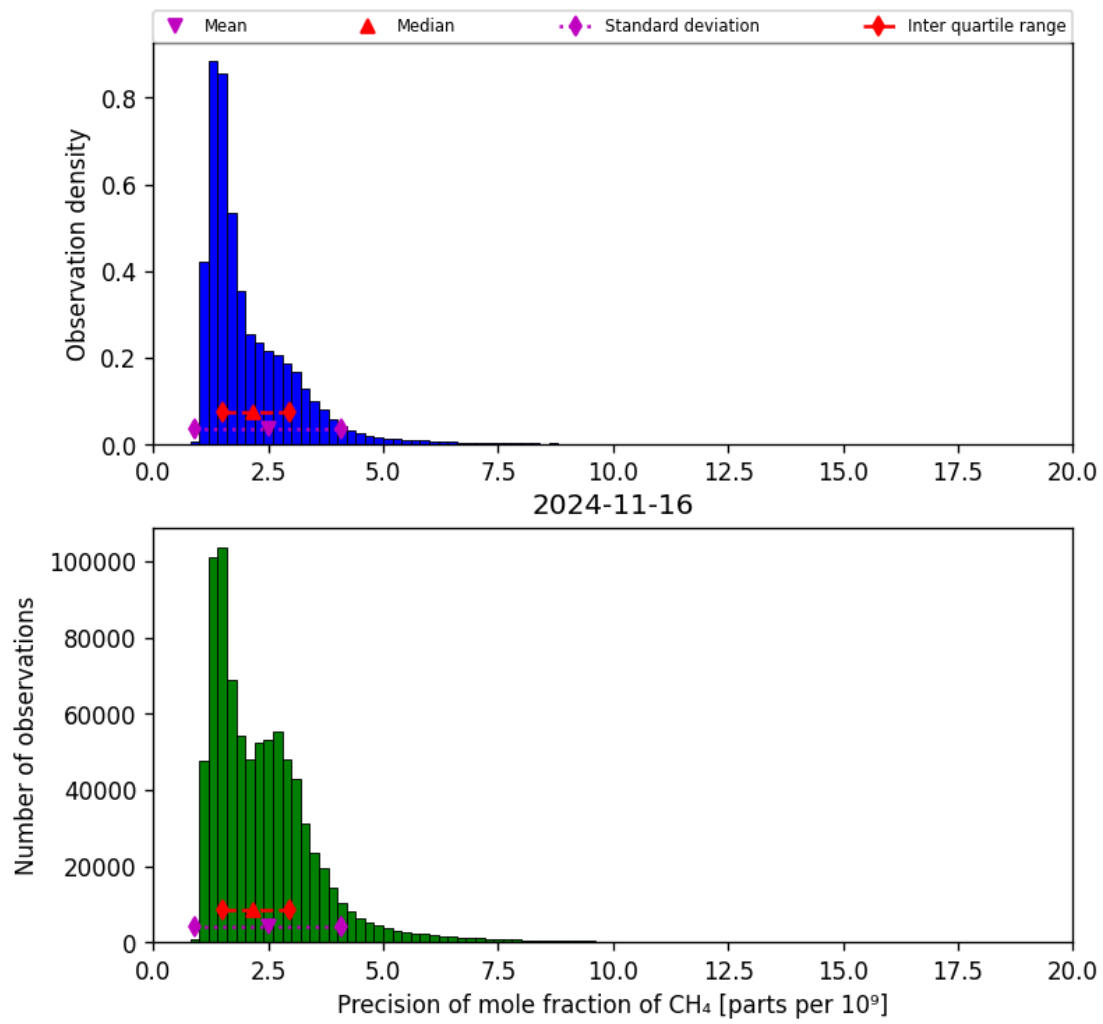
Figure 24: Histogram of “Precision of mole fraction of CH 4 ” for 2024-11-15 to 2024-11-17
