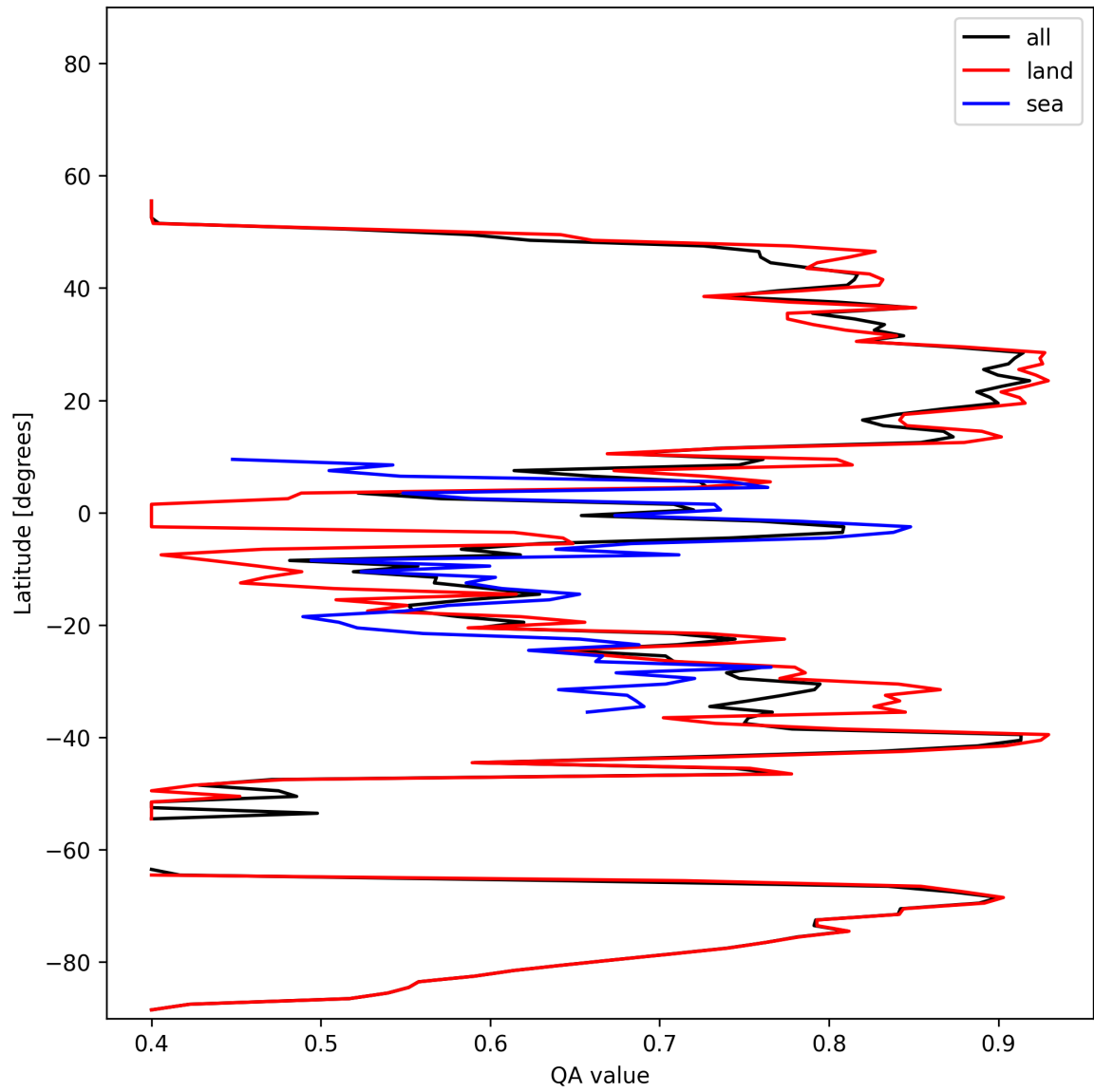
Figure 11: Zonal average of “QA value” for 2024-11-15 to 2024-11-17.
