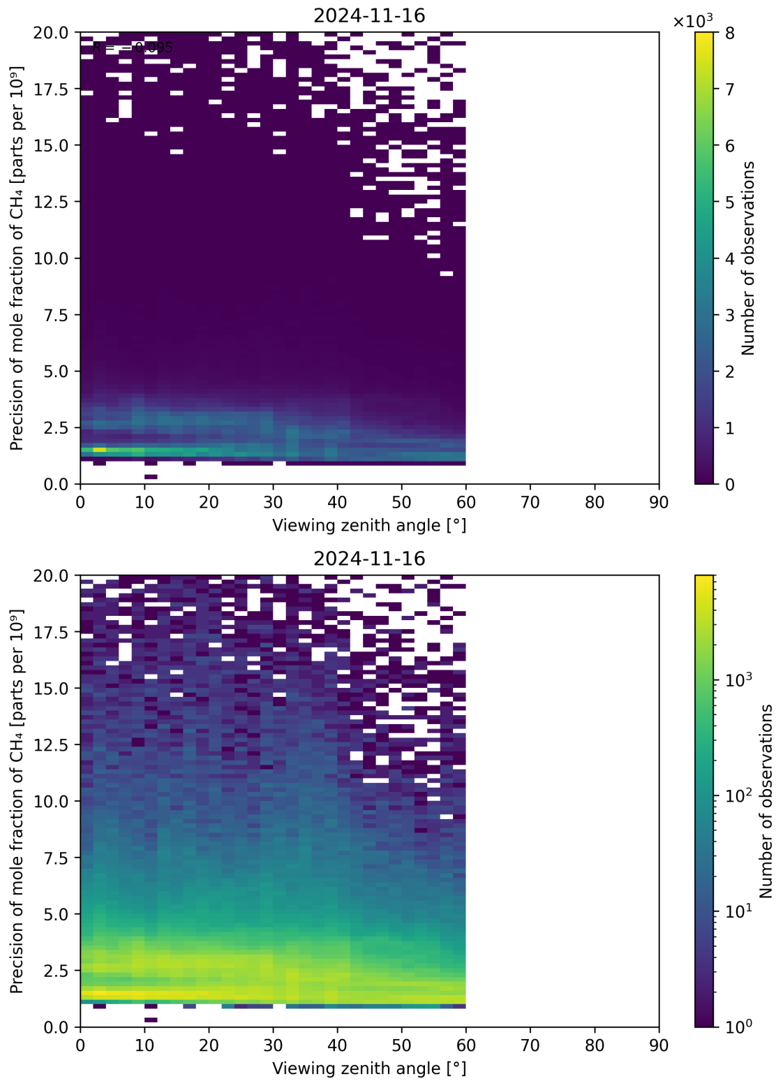
Figure 112: Scatter density plot of “Viewing zenith angle” against “Precision of mole fraction of CH 4 ” for 2024-11-15 to 2024-11-17.
