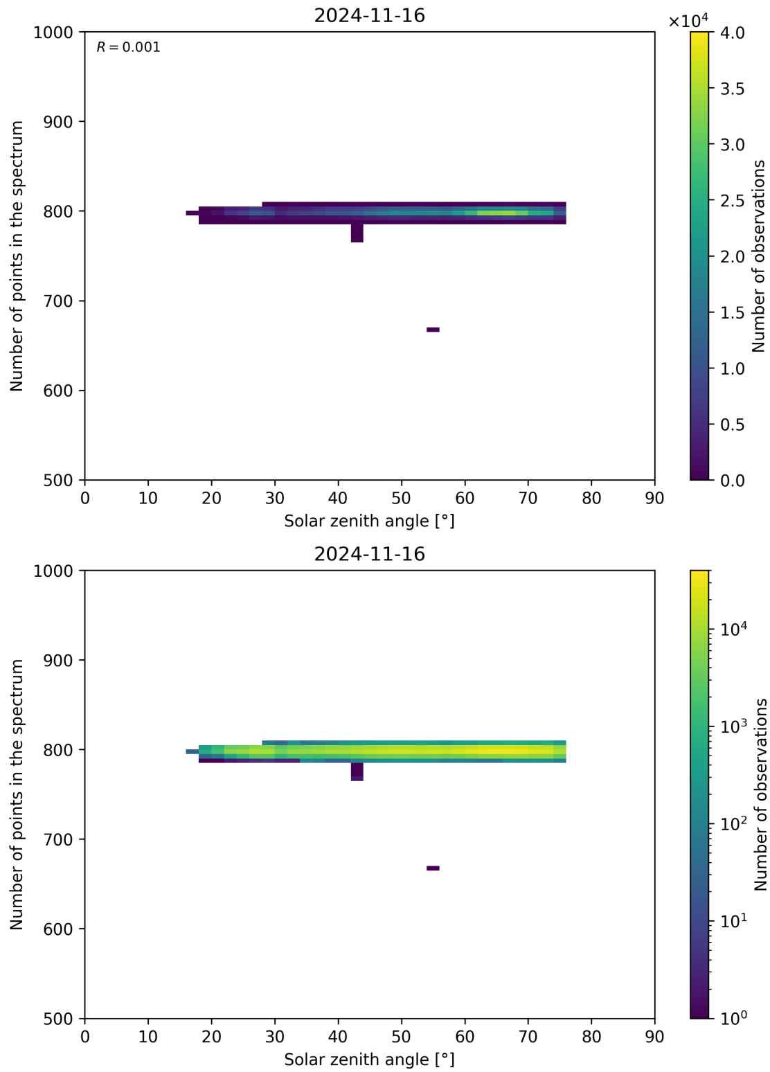
Figure 103: Scatter density plot of “Solar zenith angle” against “Number of points in the spectrum” for 2024-11-15 to 2024-11-17.
