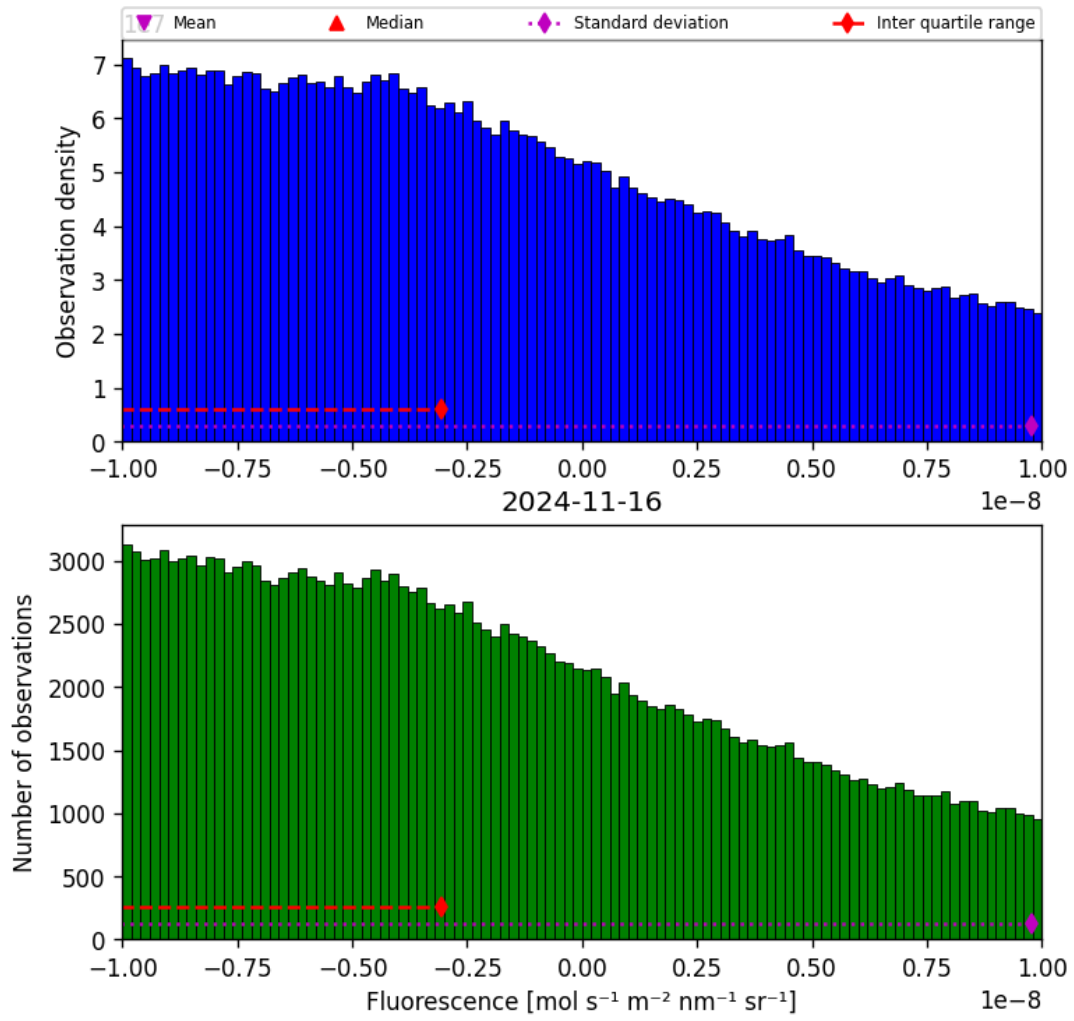
Figure 32: Histogram of “Fluorescence” for 2024-11-15 to 2024-11-17
