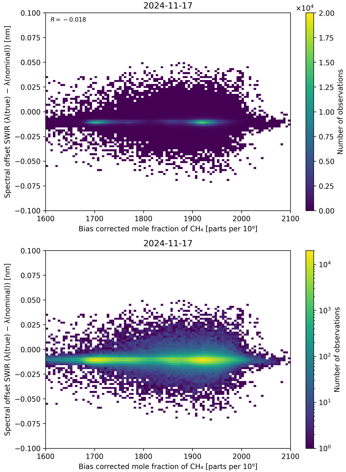
Figure 69: Scatter density plot of “Bias corrected mole fraction of \text{CH}_4 ” against “Spectral offset SWIR ( \lambda_{\text{true}} - \lambda_{\text{nominal}} )” for 2024-11-17 to 2024-11-18.
