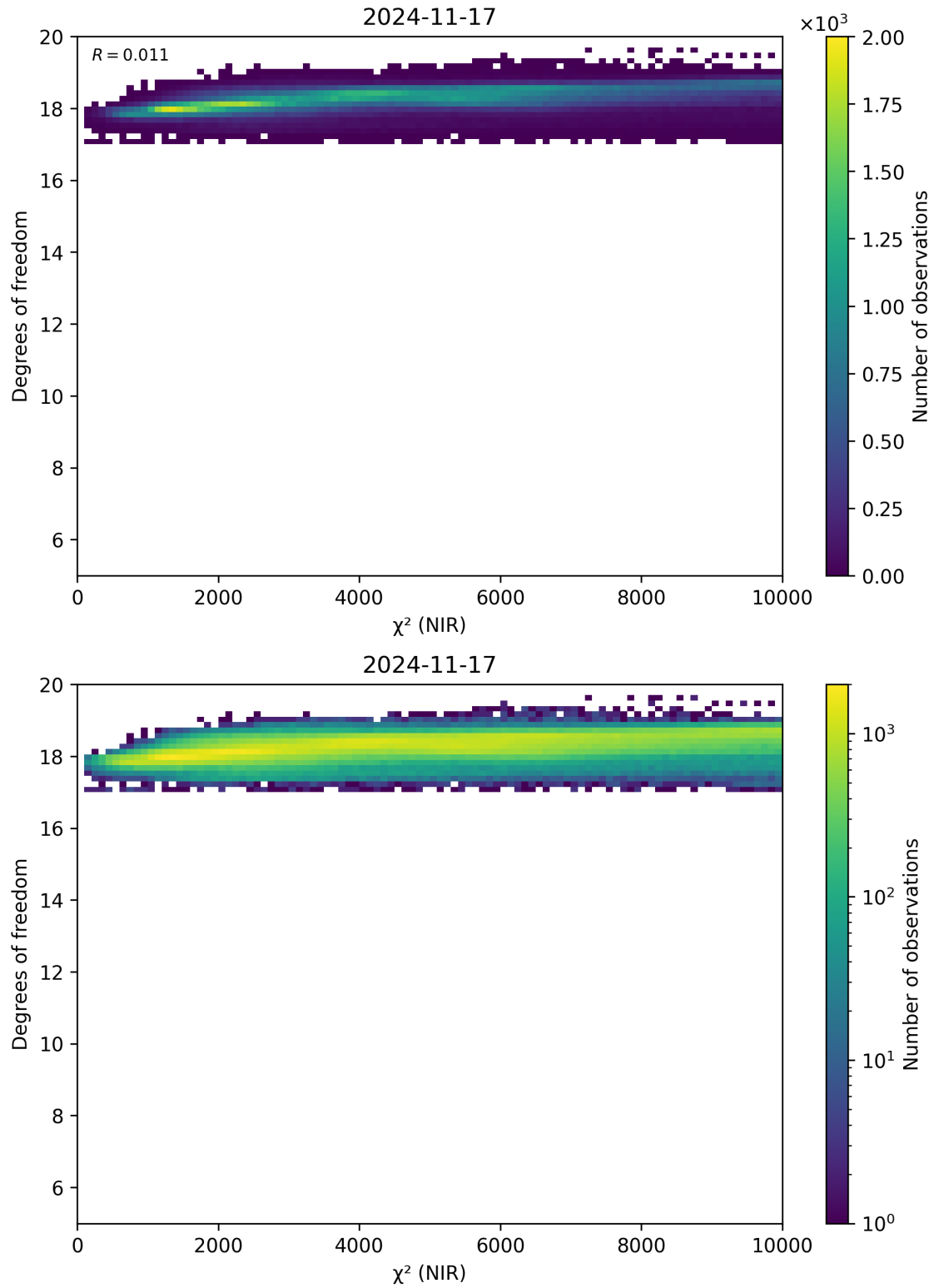
Figure 44: Scatter density plot of “ \chi^2 (NIR)” against “Degrees of freedom” for 2024-11-17 to 2024-11-18.
