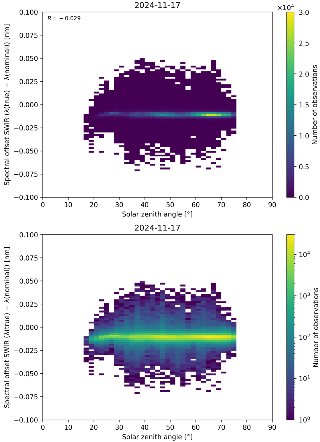
Figure 104: Scatter density plot of “Solar zenith angle” against “Spectral offset SWIR ( \lambda_{\text{true}} - \lambda_{\text{nominal}} )” for 2024-11-17 to 2024-11-18.
