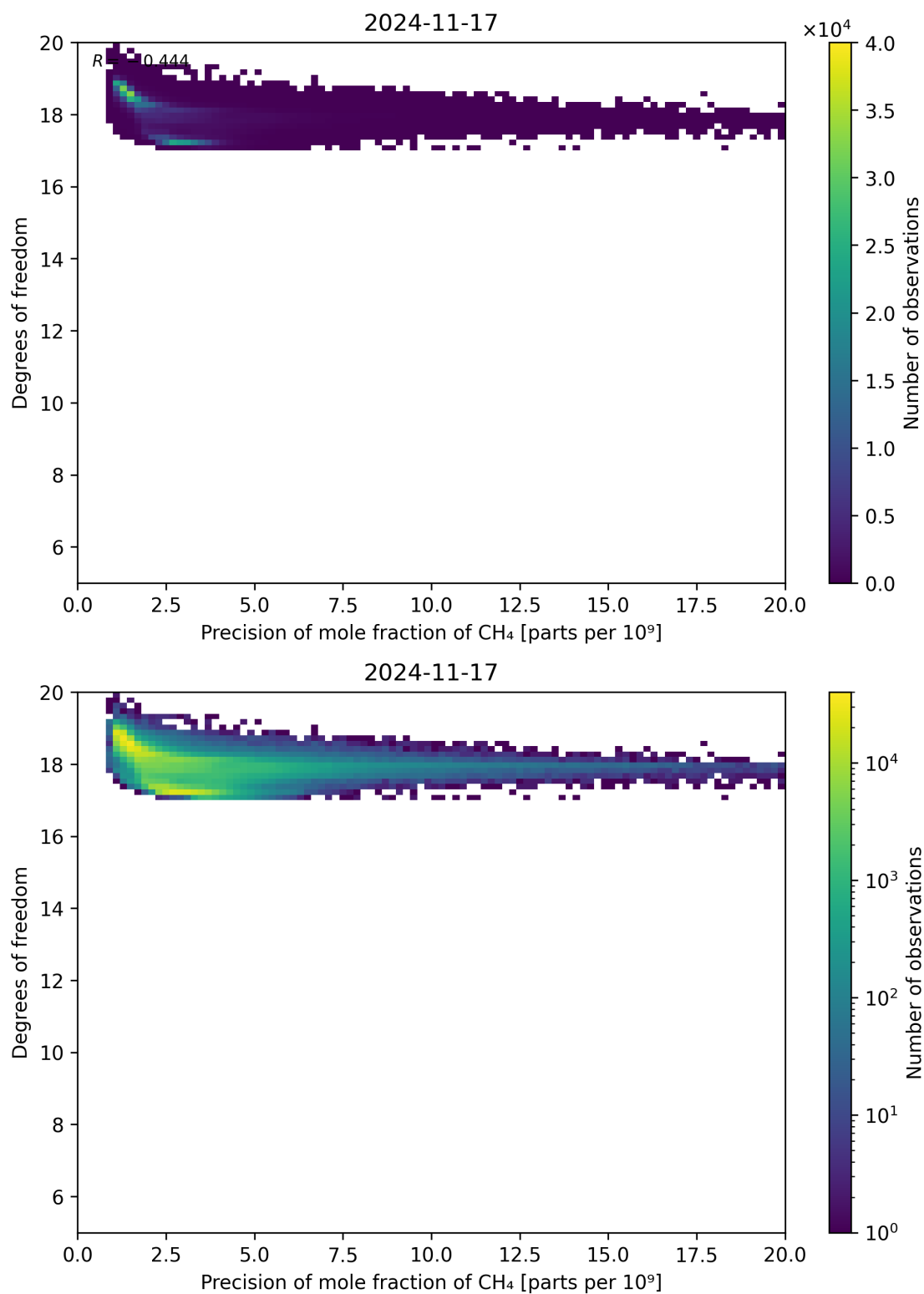
Figure 80: Scatter density plot of “Precision of mole fraction of CH 4 ” against “Degrees of freedom” for 2024-11-17 to 2024-11-18.
