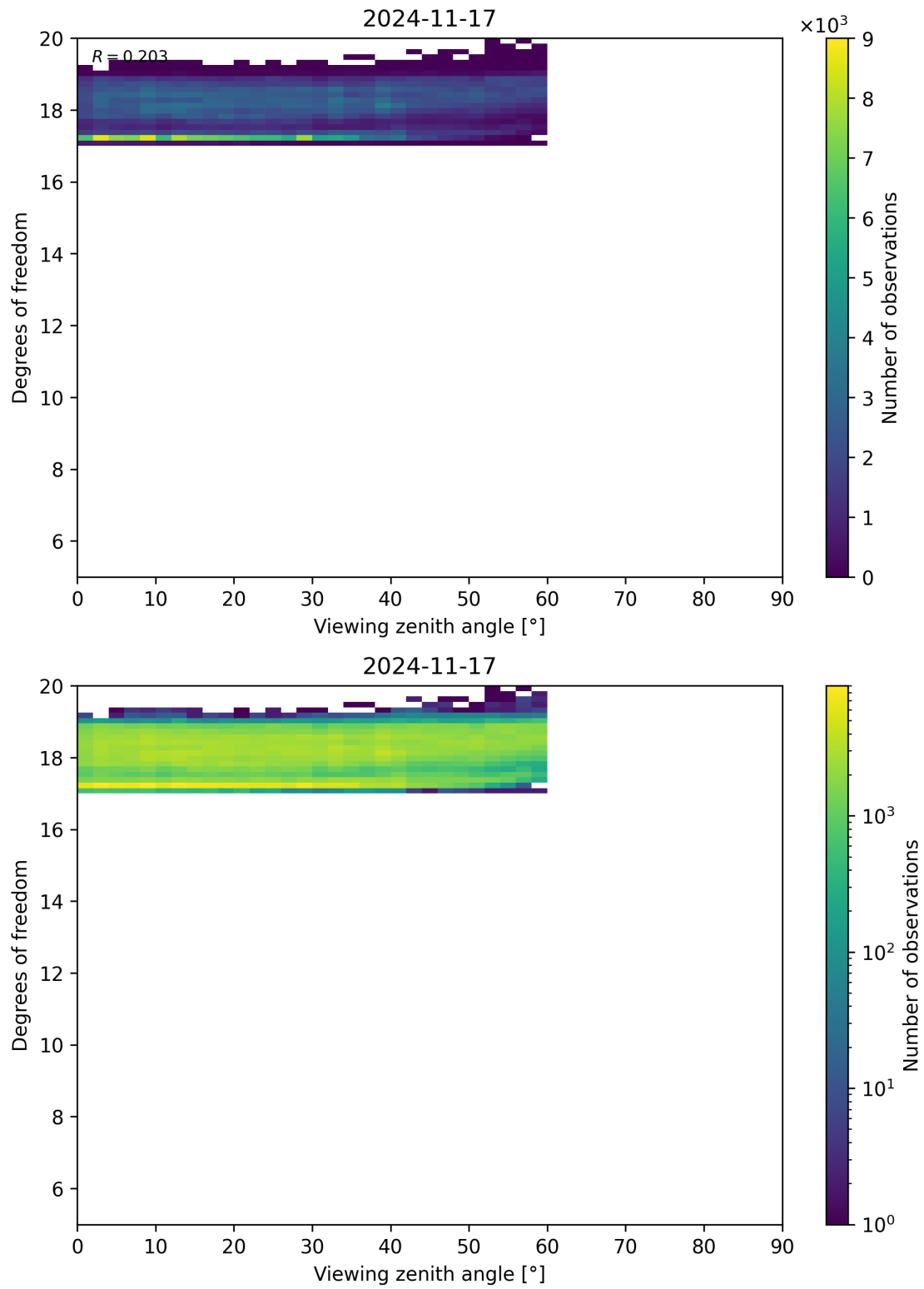
Figure 107: Scatter density plot of “Viewing zenith angle” against “Degrees of freedom” for 2024-11-17 to 2024-11-18.
