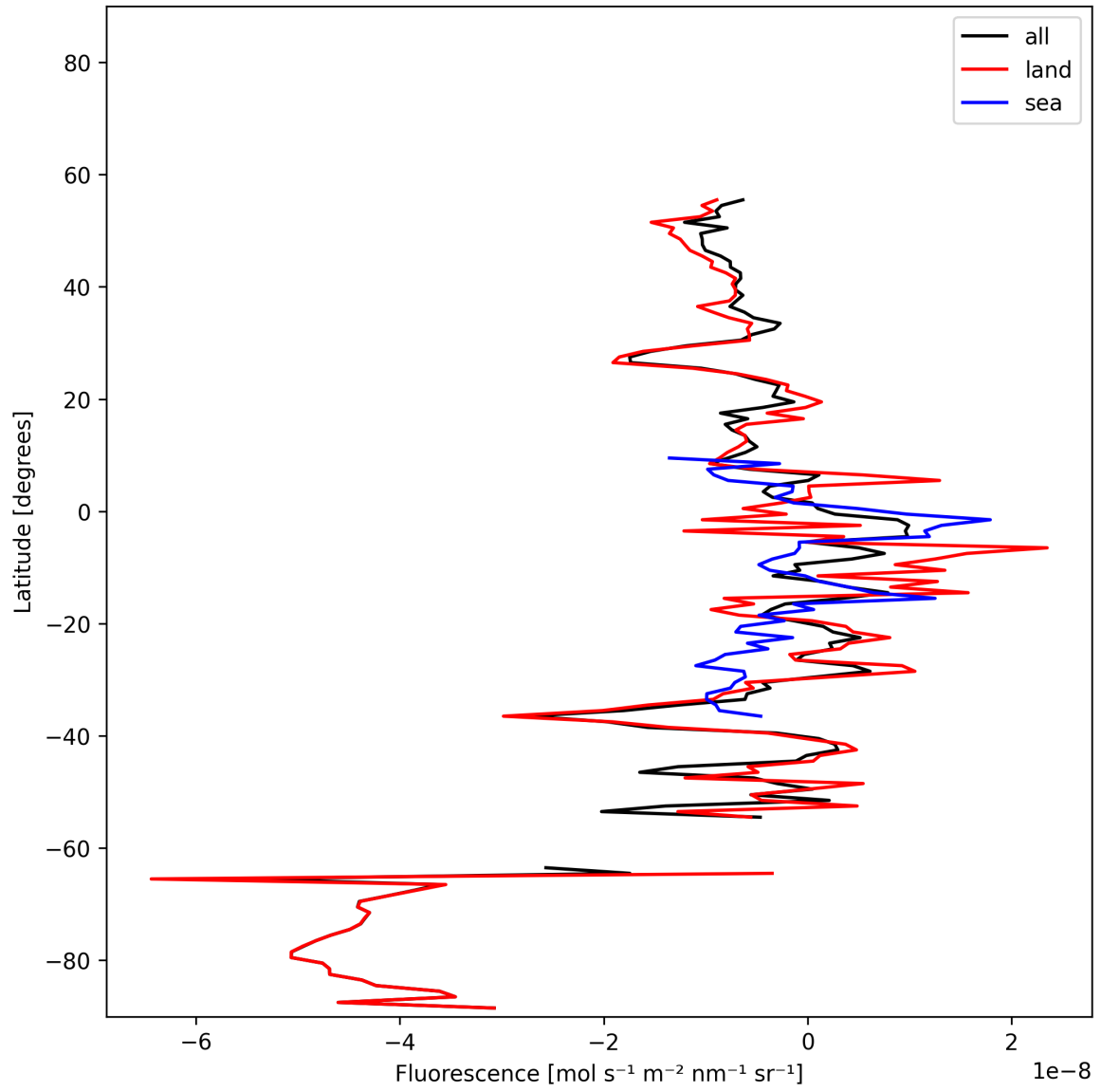
Figure 21: Zonal average of “Fluorescence” for 2024-11-17 to 2024-11-18.
