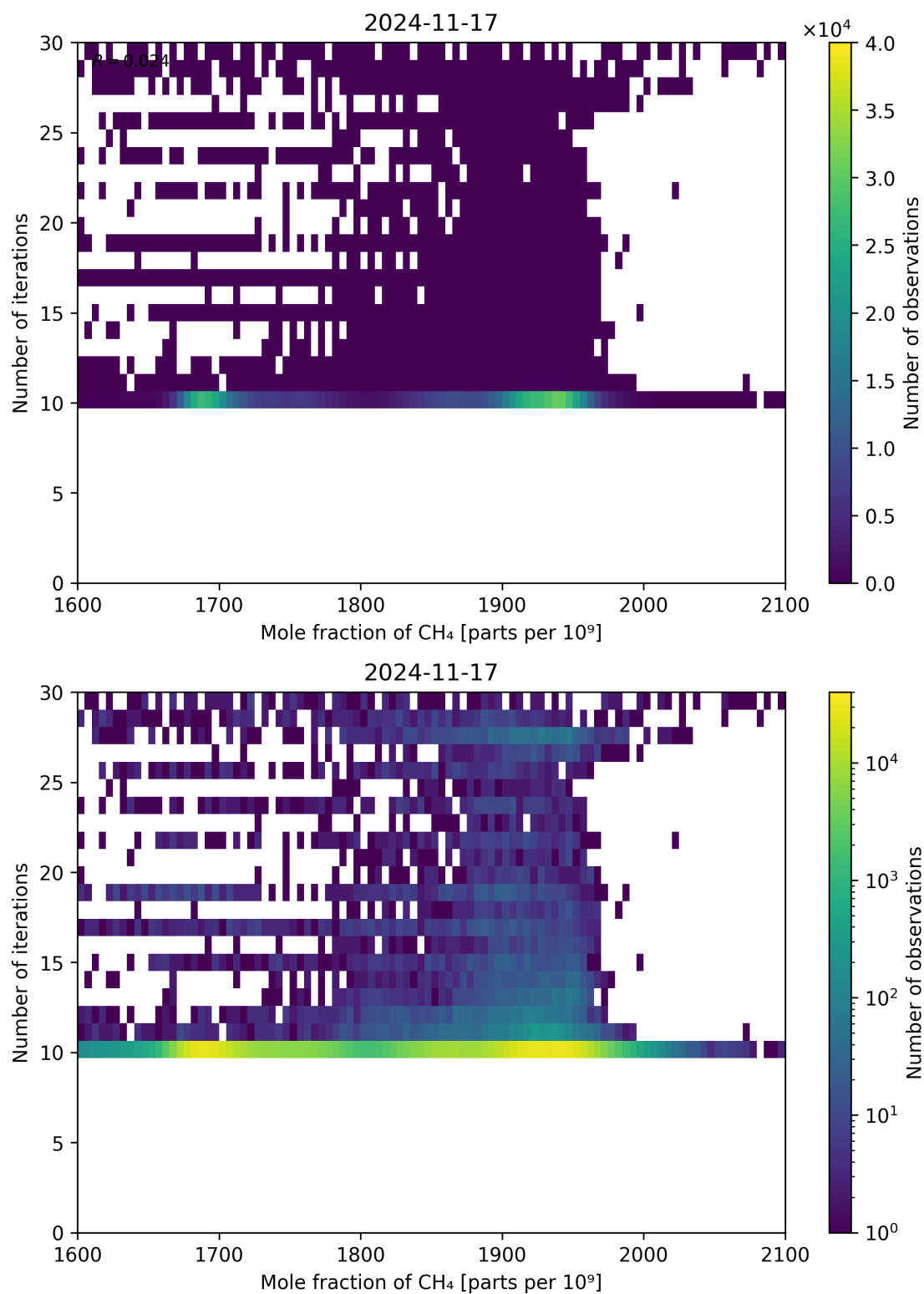
Figure 76: Scatter density plot of “Mole fraction of CH 4 ” against “Number of iterations” for 2024-11-17 to 2024-11-18.
