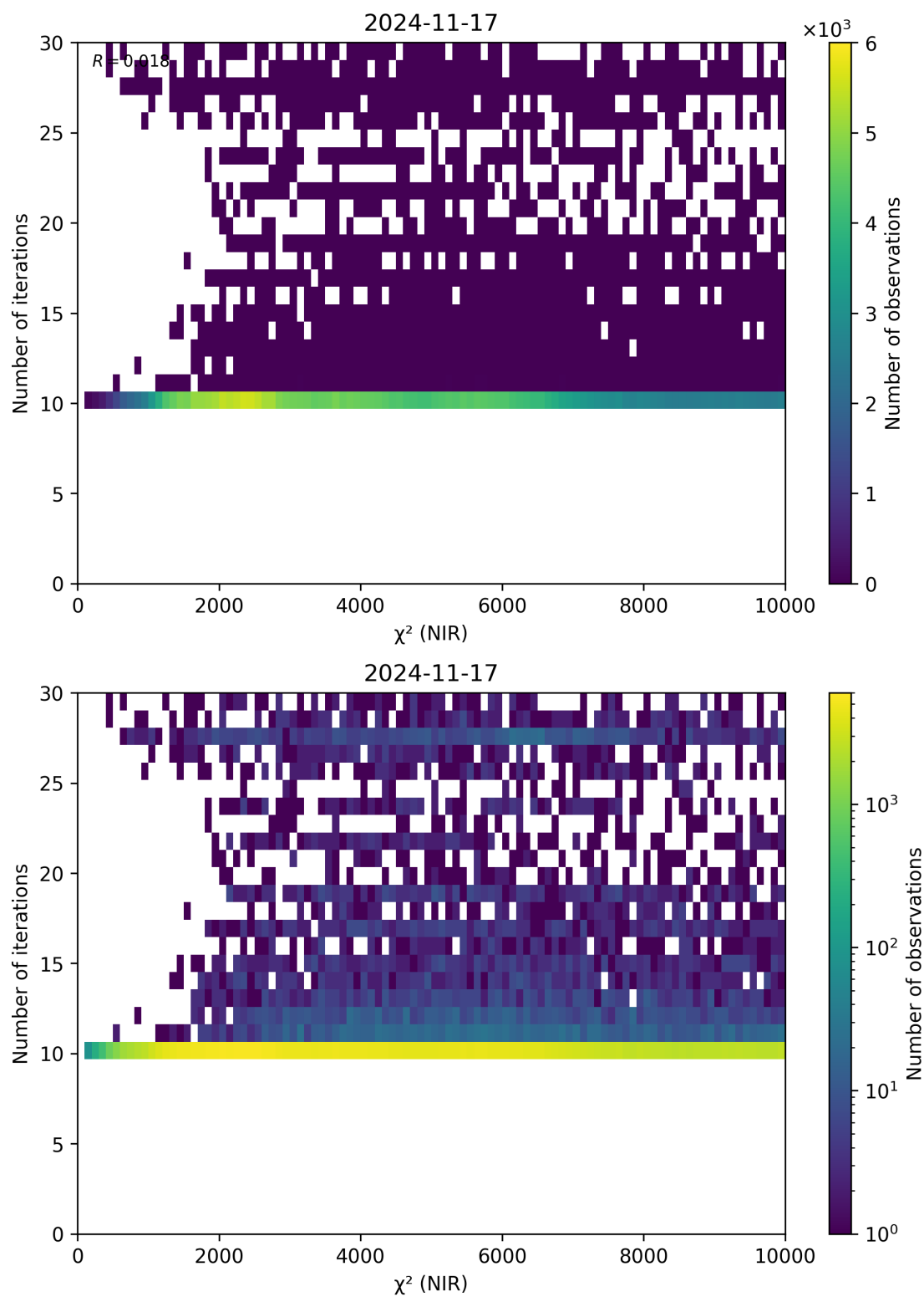
Figure 46: Scatter density plot of “ \chi^2 (NIR)” against “Number of iterations” for 2024-11-17 to 2024-11-18.
