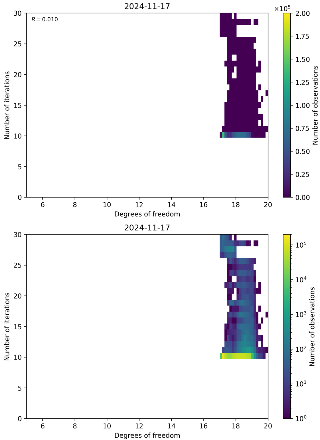
Figure 52: Scatter density plot of “Degrees of freedom” against “Number of iterations” for 2024-11-17 to 2024-11-18.
