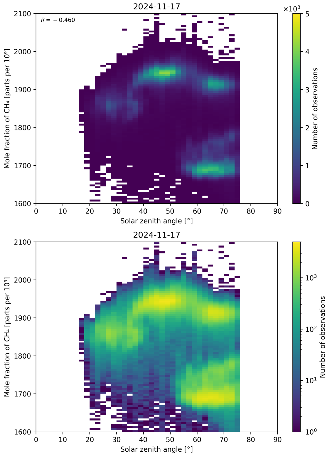
Figure 99: Scatter density plot of “Solar zenith angle” against “Mole fraction of \text{CH}_4 ” for 2024-11-17 to 2024-11-18.
