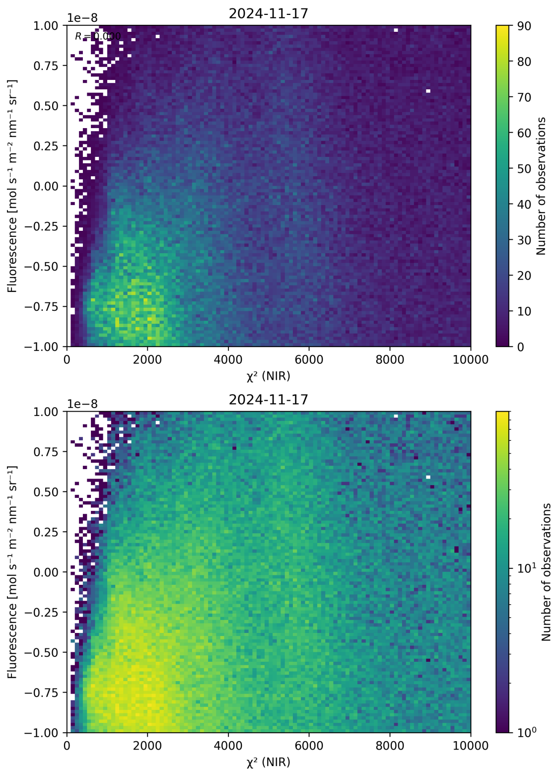
Figure 45: Scatter density plot of “ \chi^2 (NIR)” against “Fluorescence” for 2024-11-17 to 2024-11-18.
