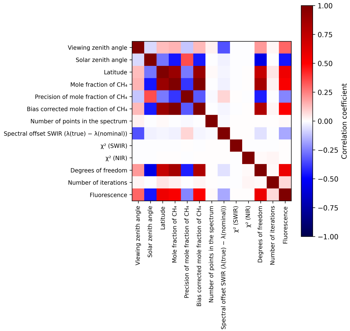
Figure 2: Map of correlation matrix for 2024-11-17 to 2024-11-18.
