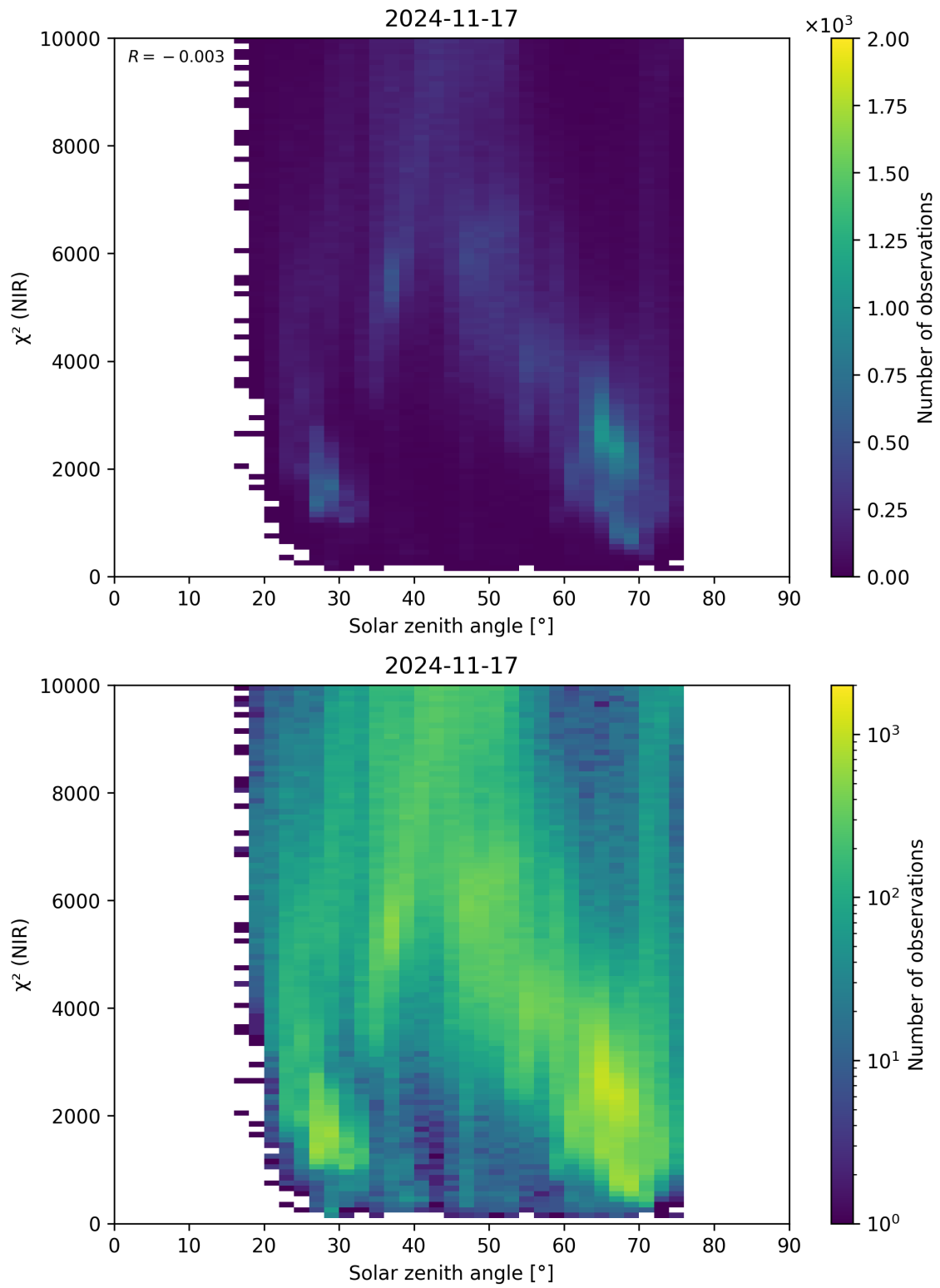
Figure 94: Scatter density plot of “Solar zenith angle” against “ \chi^2 (NIR)” for 2024-11-17 to 2024-11-18.
