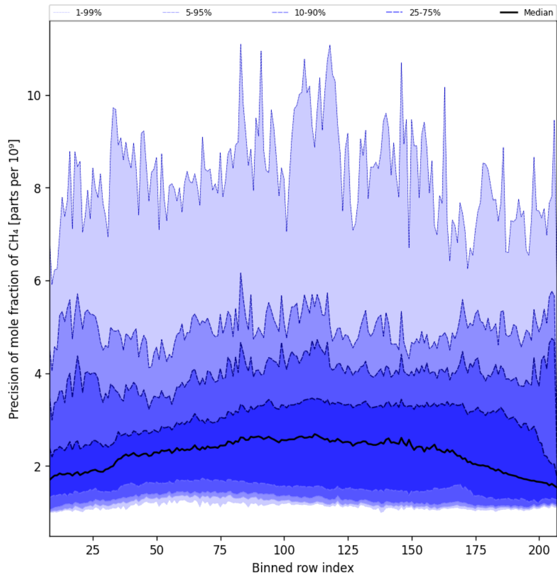
Figure 35: Along track statistics of “Precision of mole fraction of CH 4 ” for 2024-11-17 to 2024-11-18
