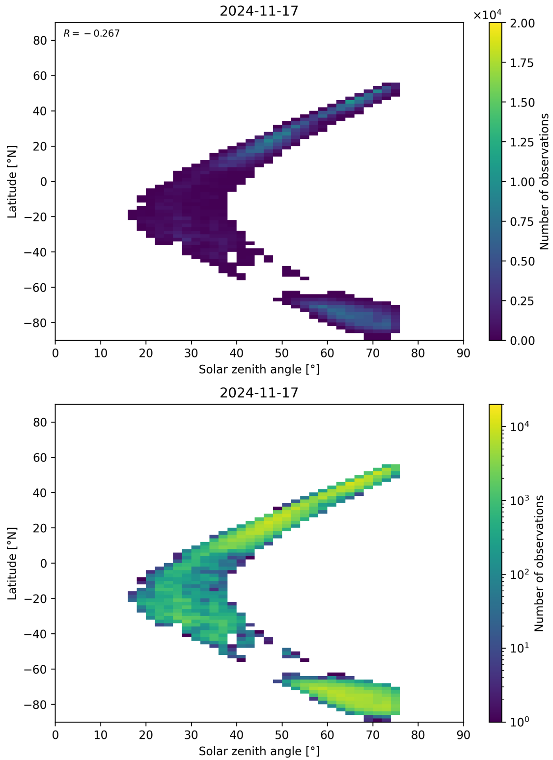
Figure 98: Scatter density plot of “Solar zenith angle” against “Latitude” for 2024-11-17 to 2024-11-18.
