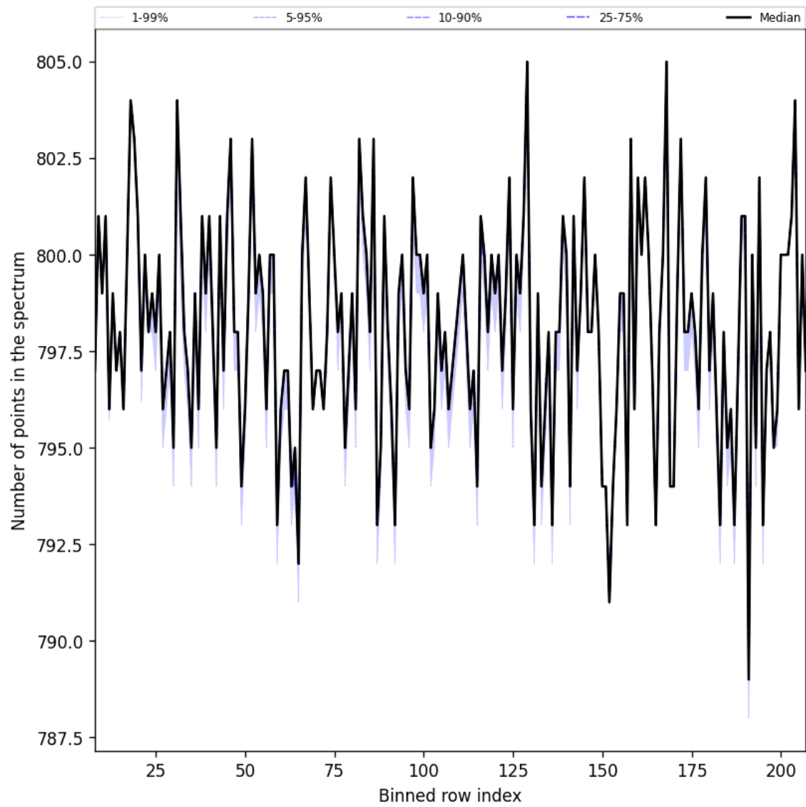
Figure 37: Along track statistics of “Number of points in the spectrum” for 2024-11-17 to 2024-11-18
