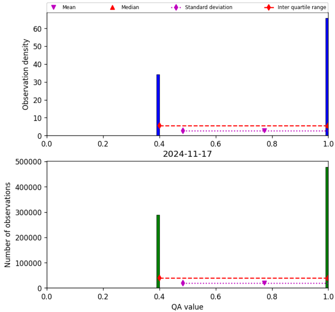
Figure 22: Histogram of “QA value” for 2024-11-17 to 2024-11-18
