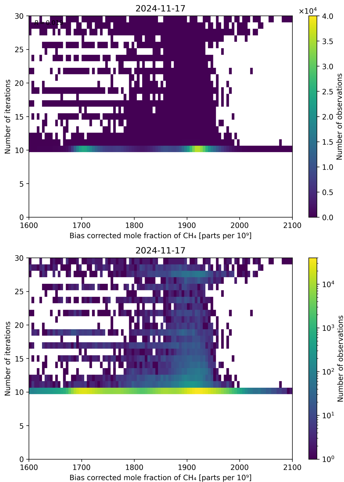
Figure 67: Scatter density plot of “Bias corrected mole fraction of \text{CH}_4 ” against “Number of iterations” for 2024-11-17 to 2024-11-18.
