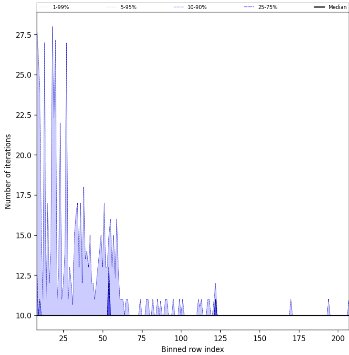
Figure 42: Along track statistics of “Number of iterations” for 2024-11-17 to 2024-11-18
