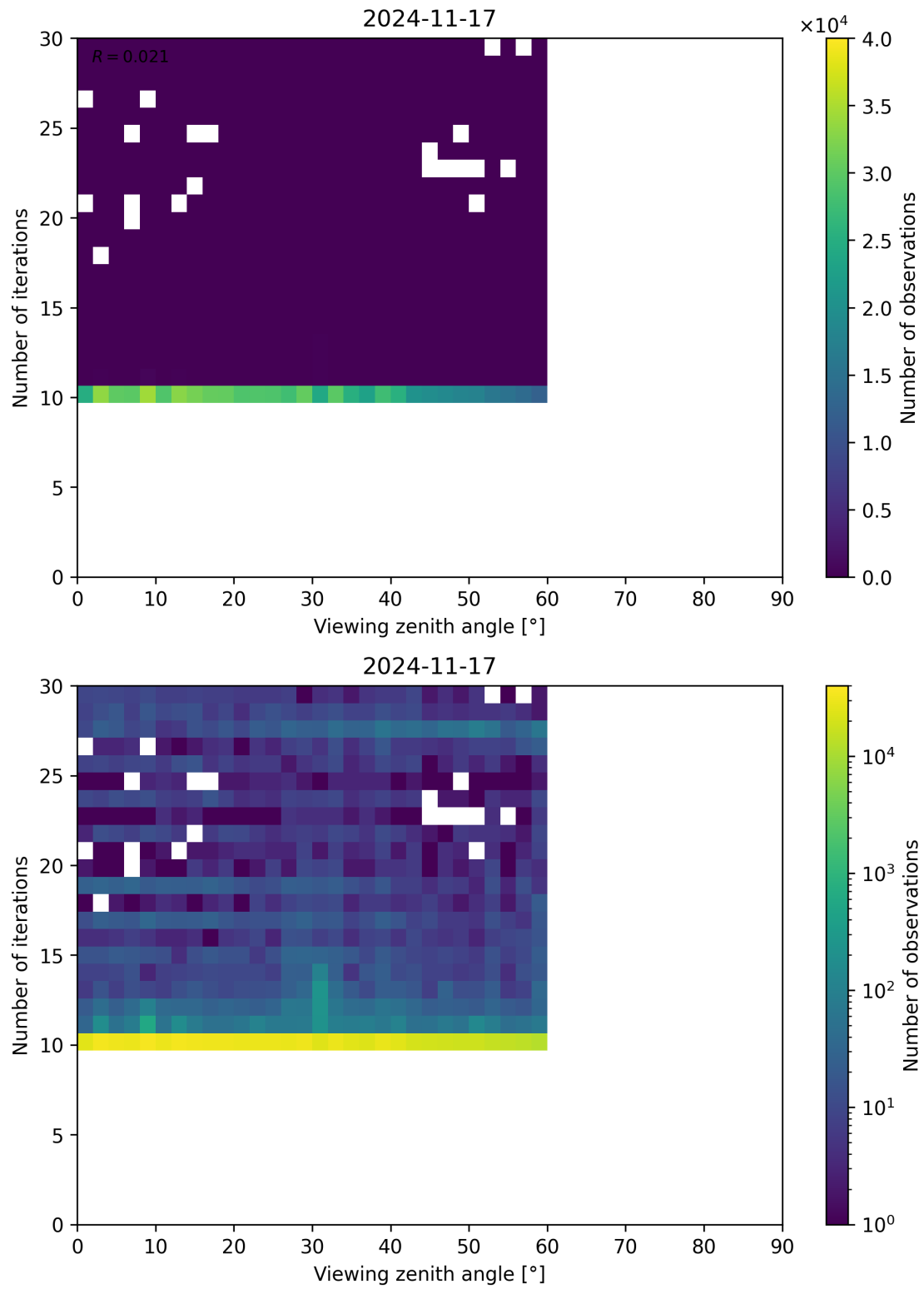
Figure 113: Scatter density plot of “Viewing zenith angle” against “Number of iterations” for 2024-11-17 to 2024-11-18.
