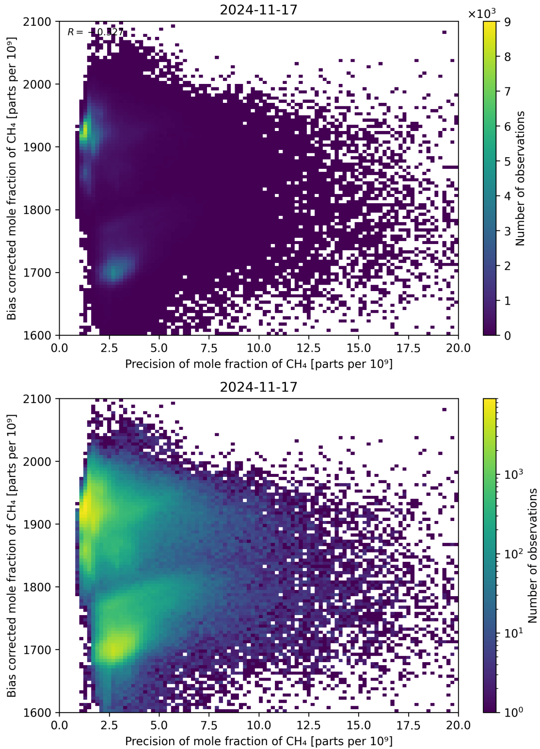
Figure 82: Scatter density plot of “Precision of mole fraction of CH 4 ” against “Bias corrected mole fraction of CH 4 ” for 2024-11-17 to 2024-11-18.
