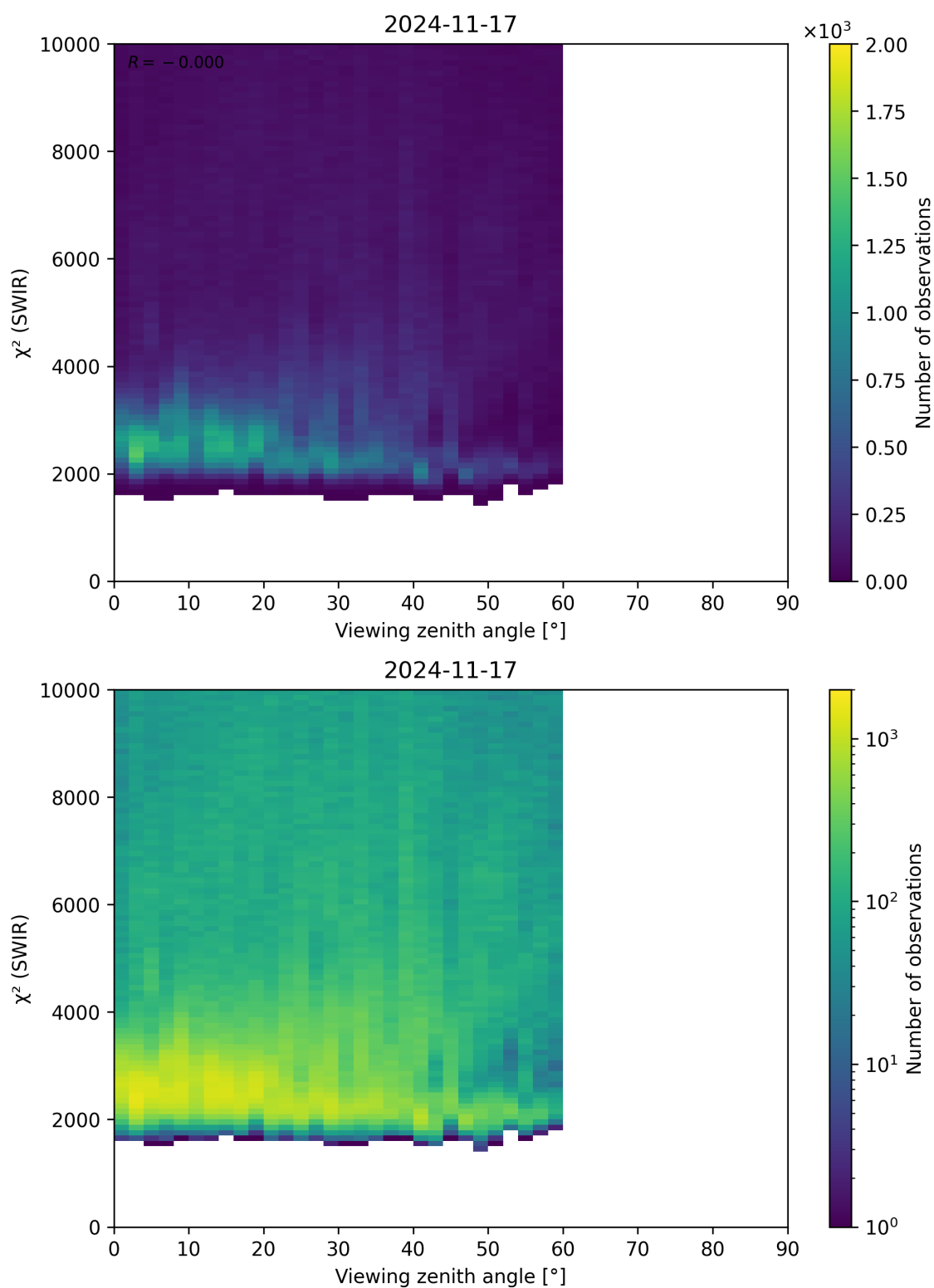
Figure 106: Scatter density plot of “Viewing zenith angle” against “ \chi^2 (SWIR)” for 2024-11-17 to 2024-11-18.
