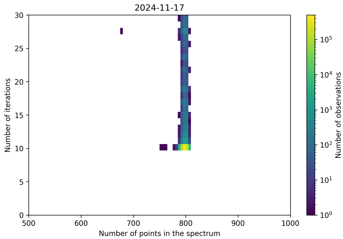
Figure 92: Scatter density plot of “Number of points in the spectrum” against “Number of iterations” for 2024-11-17 to 2024-11-18.
