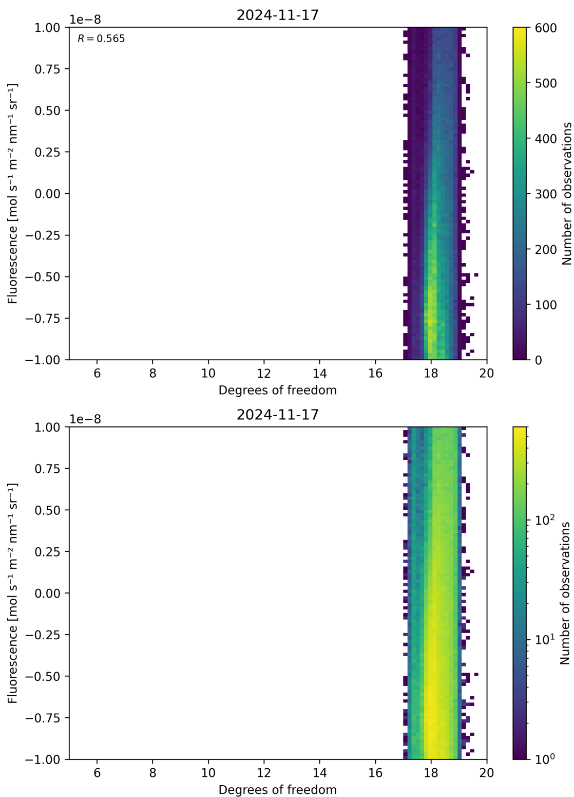
Figure 51: Scatter density plot of “Degrees of freedom” against “Fluorescence” for 2024-11-17 to 2024-11-18.
