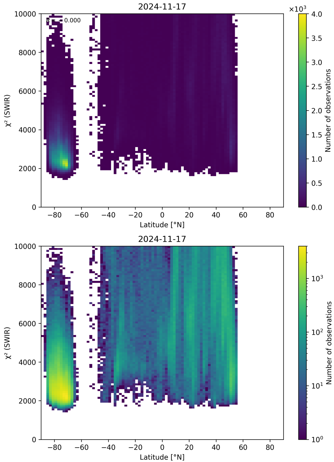
Figure 54: Scatter density plot of “Latitude” against “ \chi^2 (SWIR)” for 2024-11-17 to 2024-11-18.
