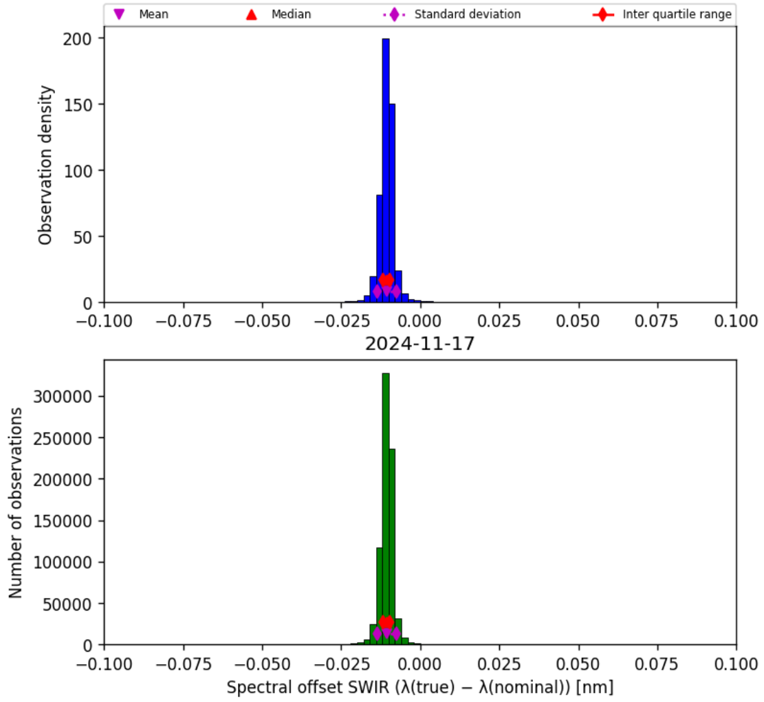
Figure 27: Histogram of “Spectral offset SWIR ( \lambda_{\text{true}} - \lambda_{\text{nominal}} )” for 2024-11-17 to 2024-11-18
