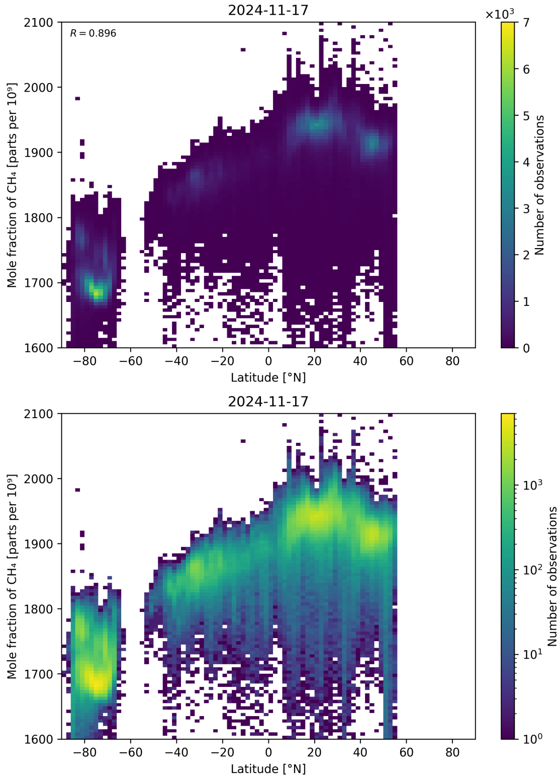
Figure 57: Scatter density plot of “Latitude” against “Mole fraction of CH 4 ” for 2024-11-17 to 2024-11-18.
