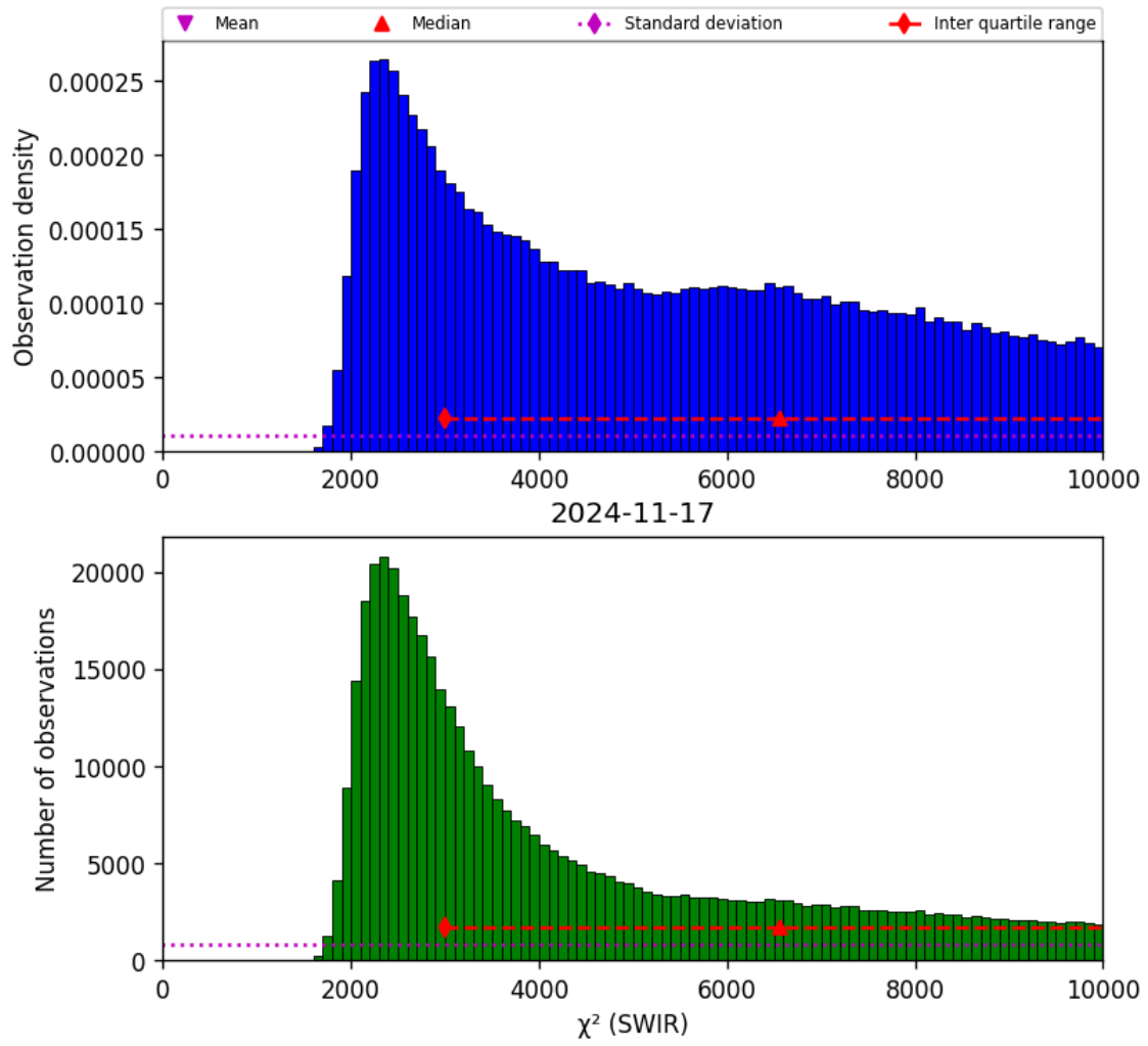
Figure 28: Histogram of “ \chi^2 (SWIR)” for 2024-11-17 to 2024-11-18
