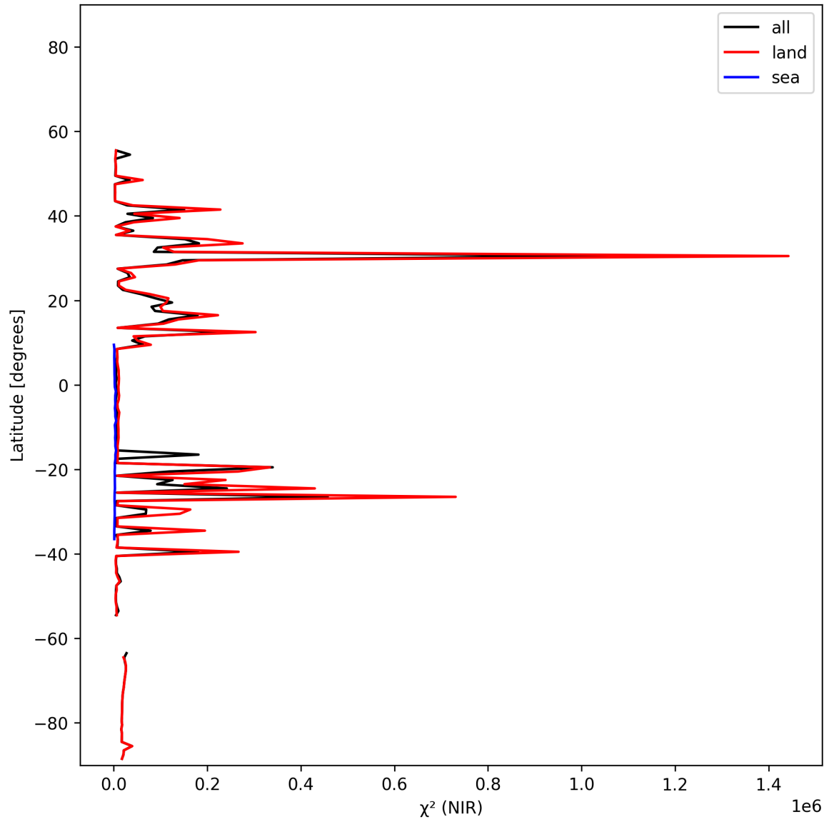
Figure 18: Zonal average of “ \chi^2 (NIR)” for 2024-11-17 to 2024-11-18.
