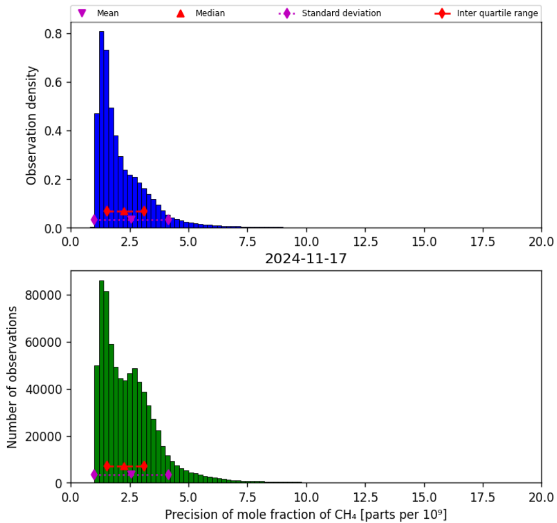
Figure 24: Histogram of “Precision of mole fraction of CH 4 ” for 2024-11-17 to 2024-11-18
