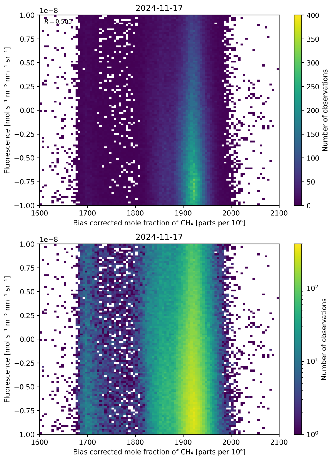
Figure 66: Scatter density plot of “Bias corrected mole fraction of \text{CH}_4 ” against “Fluorescence” for 2024-11-17 to 2024-11-18.
