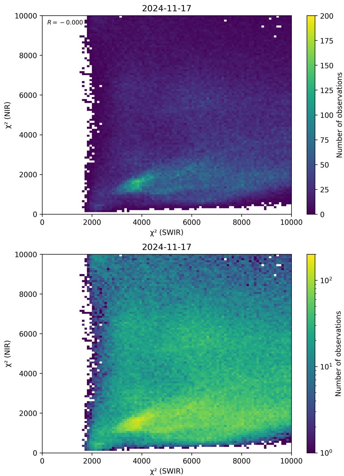
Figure 47: Scatter density plot of “ \chi^2 (SWIR)” against “ \chi^2 (NIR)” for 2024-11-17 to 2024-11-18.
