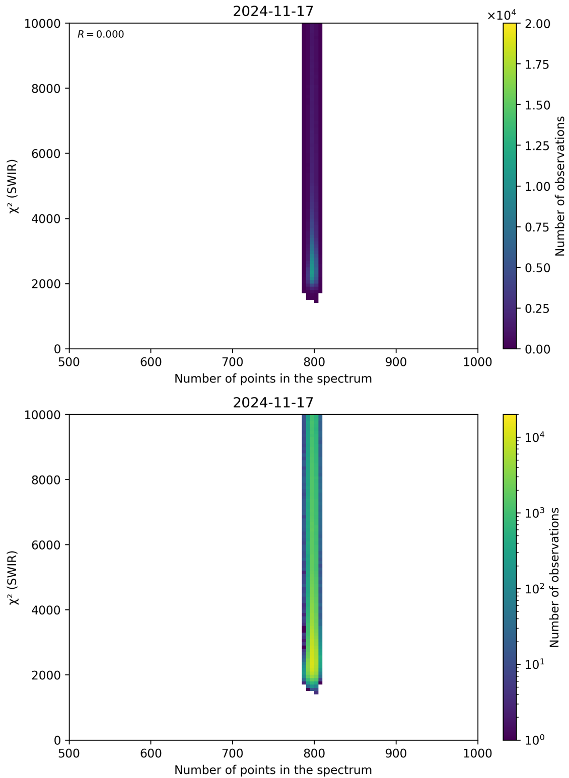
Figure 89: Scatter density plot of “Number of points in the spectrum” against “ \chi^2 (SWIR)” for 2024-11-17 to 2024-11-18.
