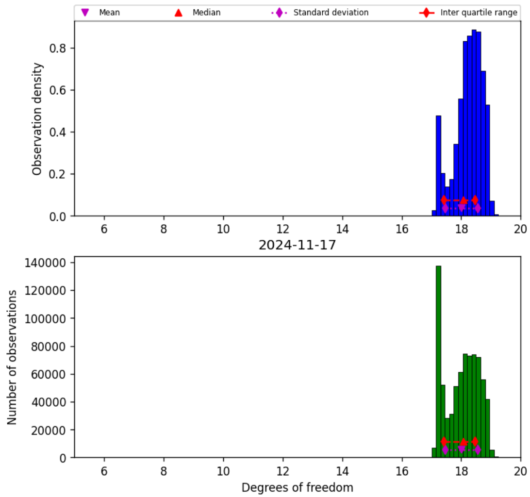
Figure 30: Histogram of “Degrees of freedom” for 2024-11-17 to 2024-11-18
