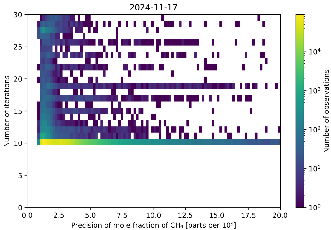
Figure 83: Scatter density plot of “Precision of mole fraction of CH 4 ” against “Number of iterations” for 2024-11-17 to 2024-11-18.
