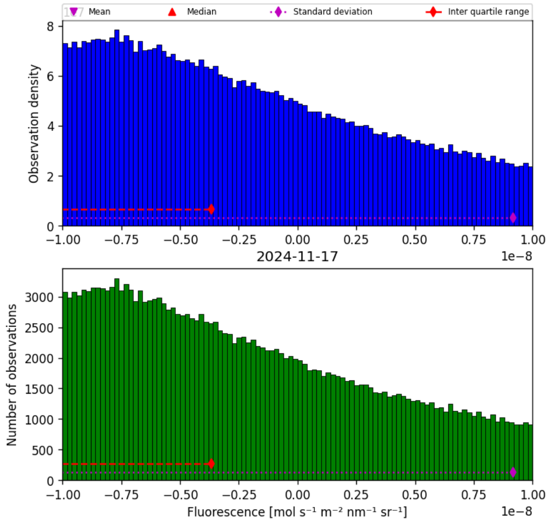
Figure 32: Histogram of “Fluorescence” for 2024-11-17 to 2024-11-18
