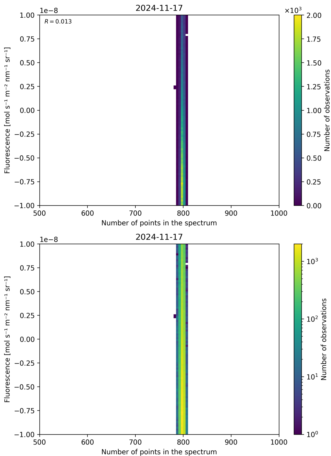
Figure 91: Scatter density plot of “Number of points in the spectrum” against “Fluorescence” for 2024-11-17 to 2024-11-18.
