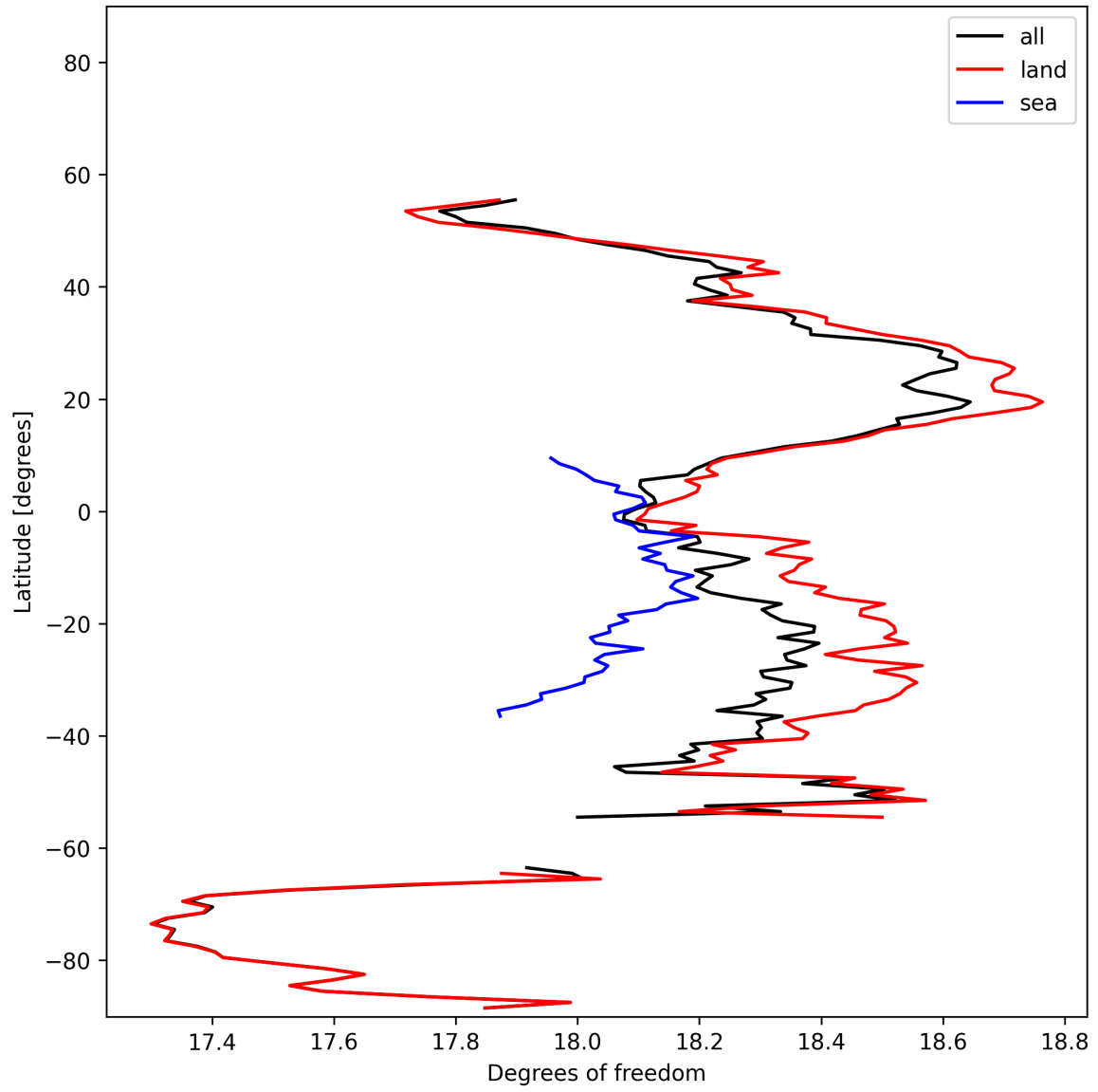
Figure 19: Zonal average of “Degrees of freedom” for 2024-11-17 to 2024-11-18.
