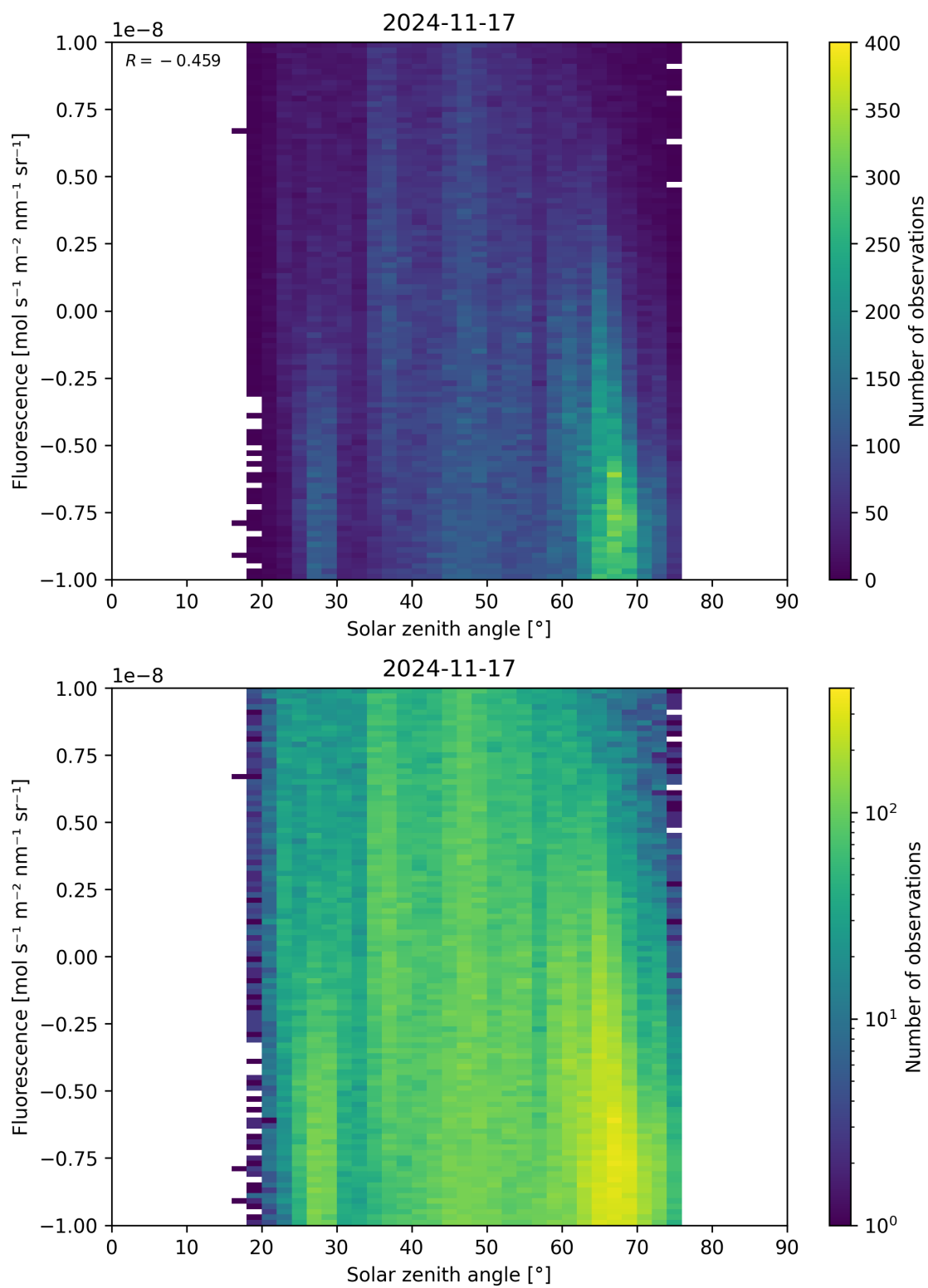
Figure 97: Scatter density plot of “Solar zenith angle” against “Fluorescence” for 2024-11-17 to 2024-11-18.
