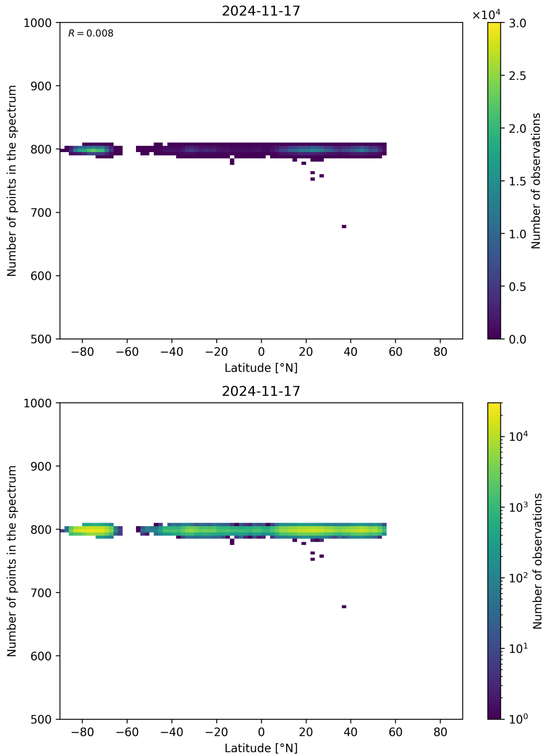
Figure 61: Scatter density plot of “Latitude” against “Number of points in the spectrum” for 2024-11-17 to 2024-11-18.
