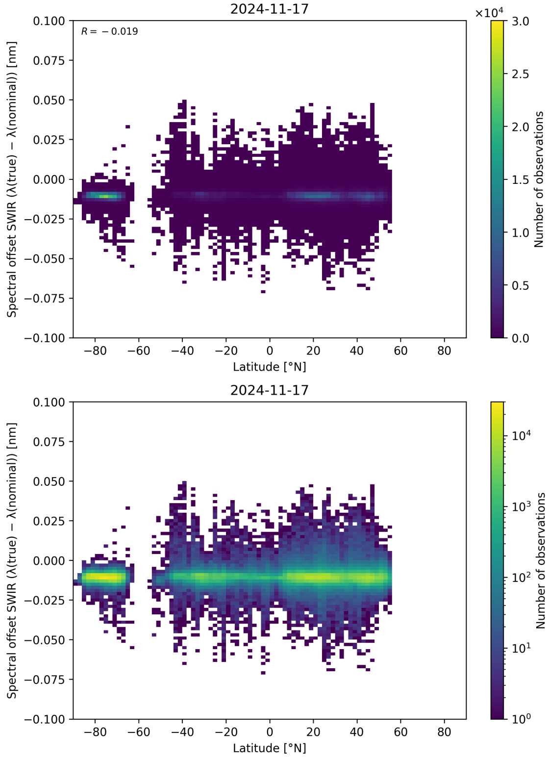
Figure 62: Scatter density plot of “Latitude” against “Spectral offset SWIR ( \lambda_{\text{true}} - \lambda_{\text{nominal}} )” for 2024-11-17 to 2024-11-18.
