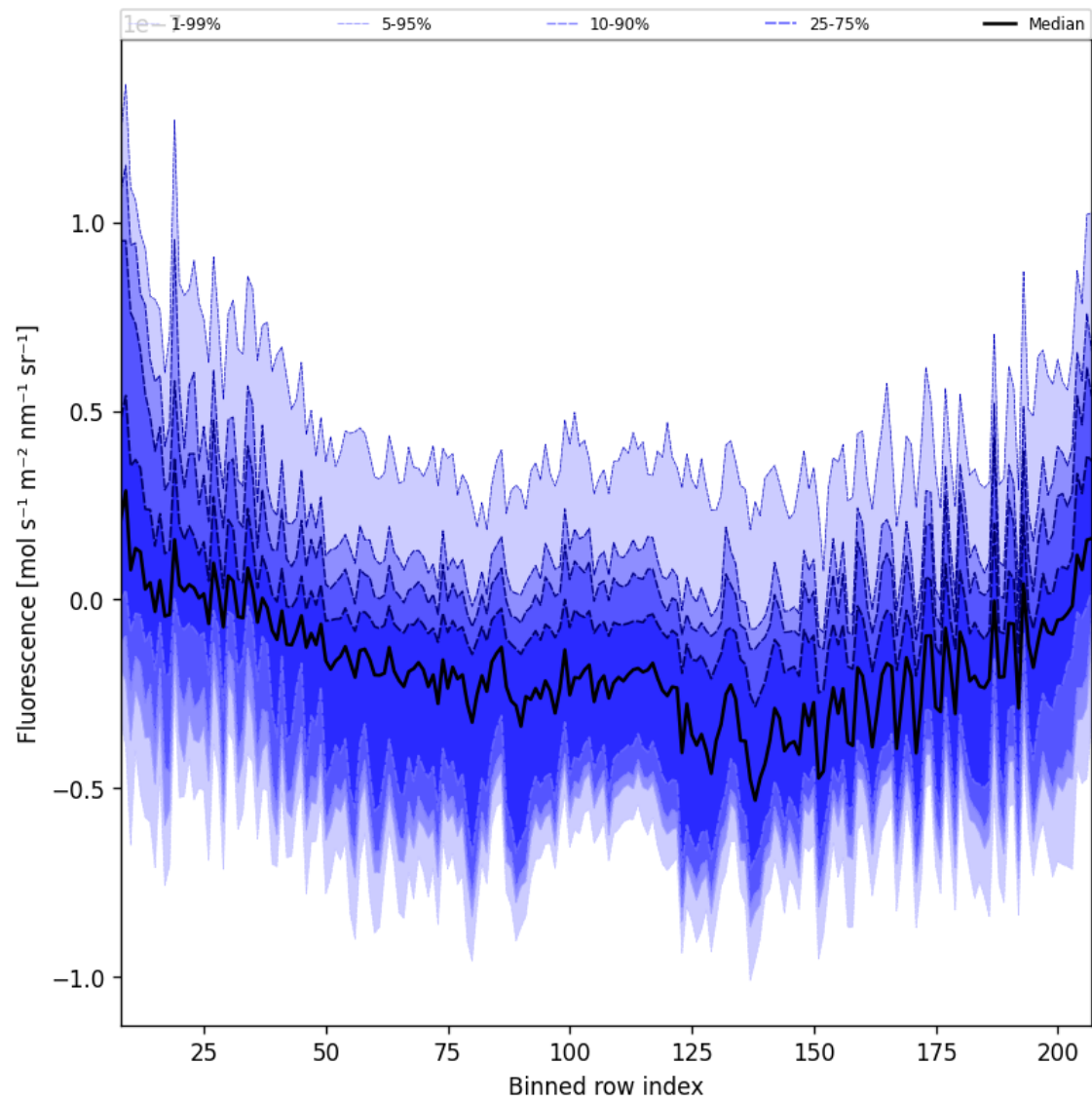
Figure 43: Along track statistics of “Fluorescence” for 2024-11-17 to 2024-11-18
