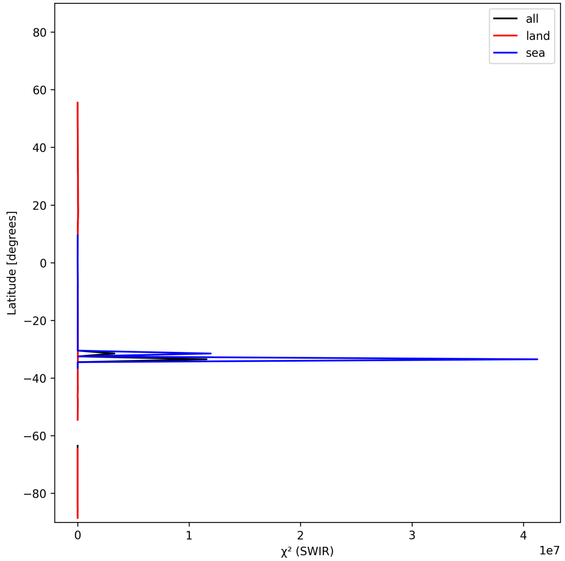
Figure 17: Zonal average of “ \chi^2 (SWIR)” for 2024-11-17 to 2024-11-18.
