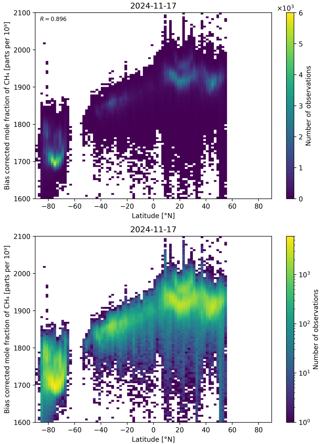
Figure 58: Scatter density plot of “Latitude” against “Bias corrected mole fraction of CH 4 ” for 2024-11-17 to 2024-11-18.
