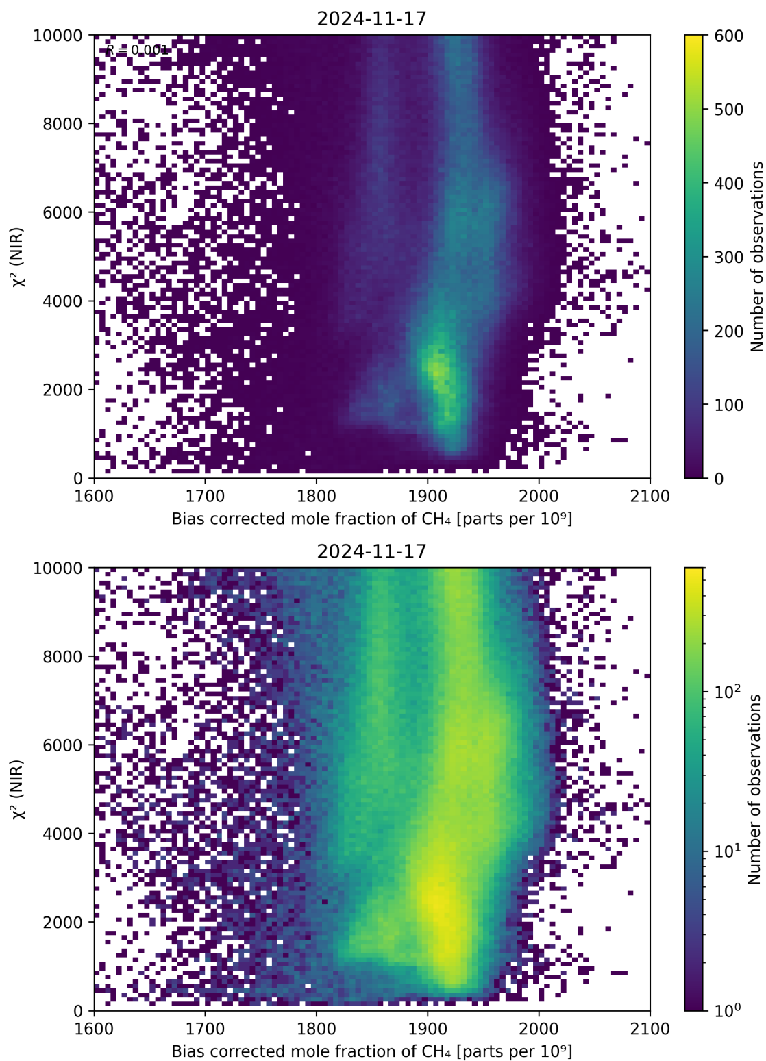
Figure 63: Scatter density plot of “Bias corrected mole fraction of \text{CH}_4 ” against “ \chi^2 (NIR)” for 2024-11-17 to 2024-11-18.
