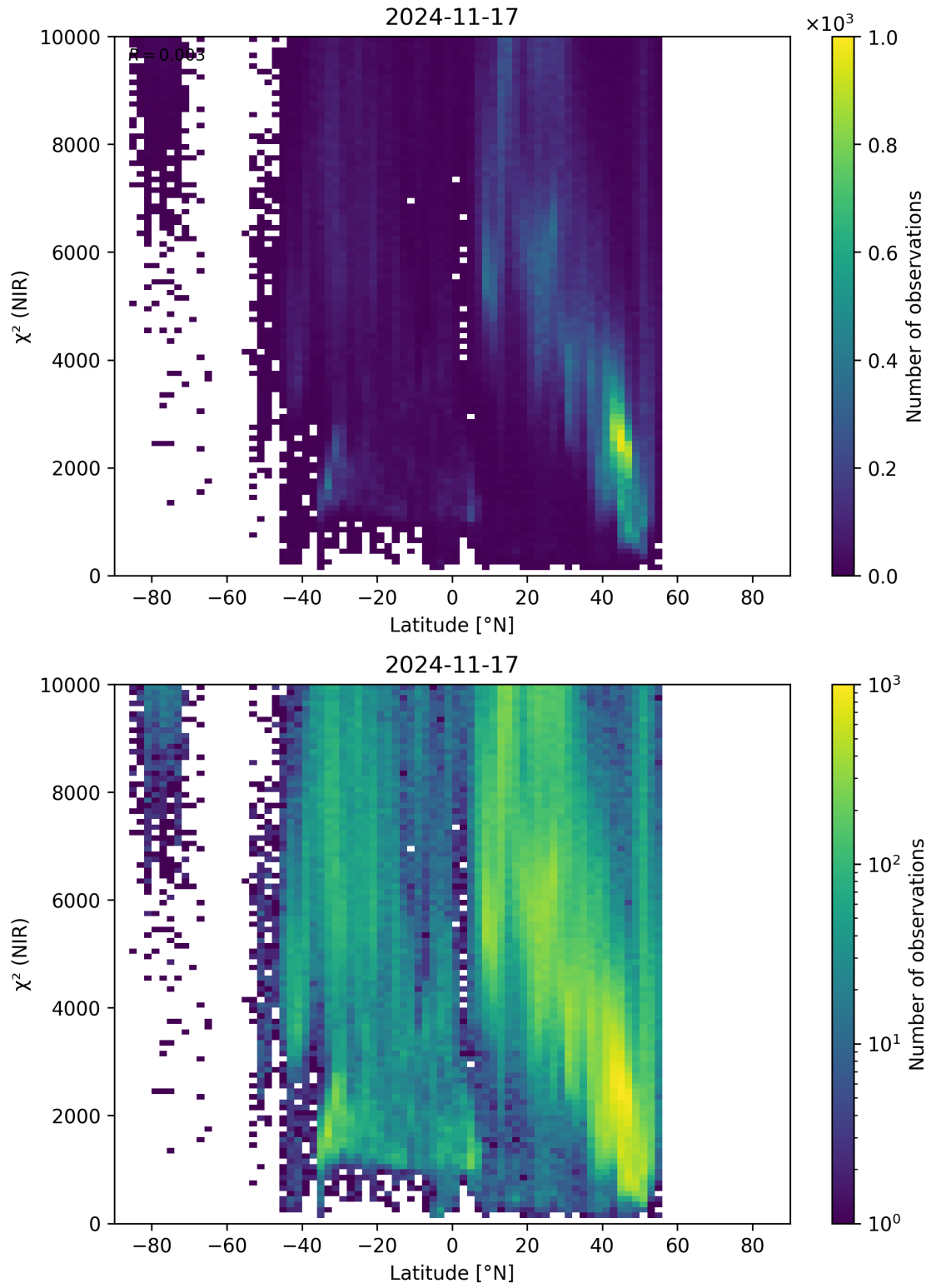
Figure 53: Scatter density plot of “Latitude” against “ \chi^2 (NIR)” for 2024-11-17 to 2024-11-18.
