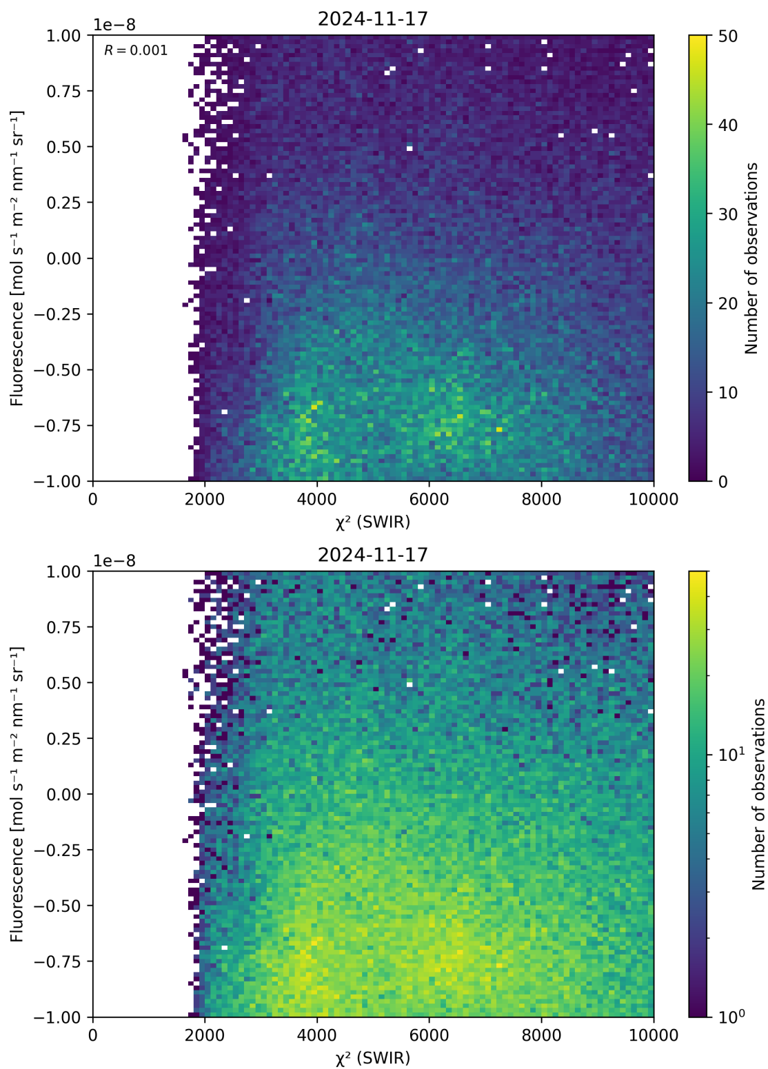
Figure 49: Scatter density plot of “ \chi^2 (SWIR)” against “Fluorescence” for 2024-11-17 to 2024-11-18.
