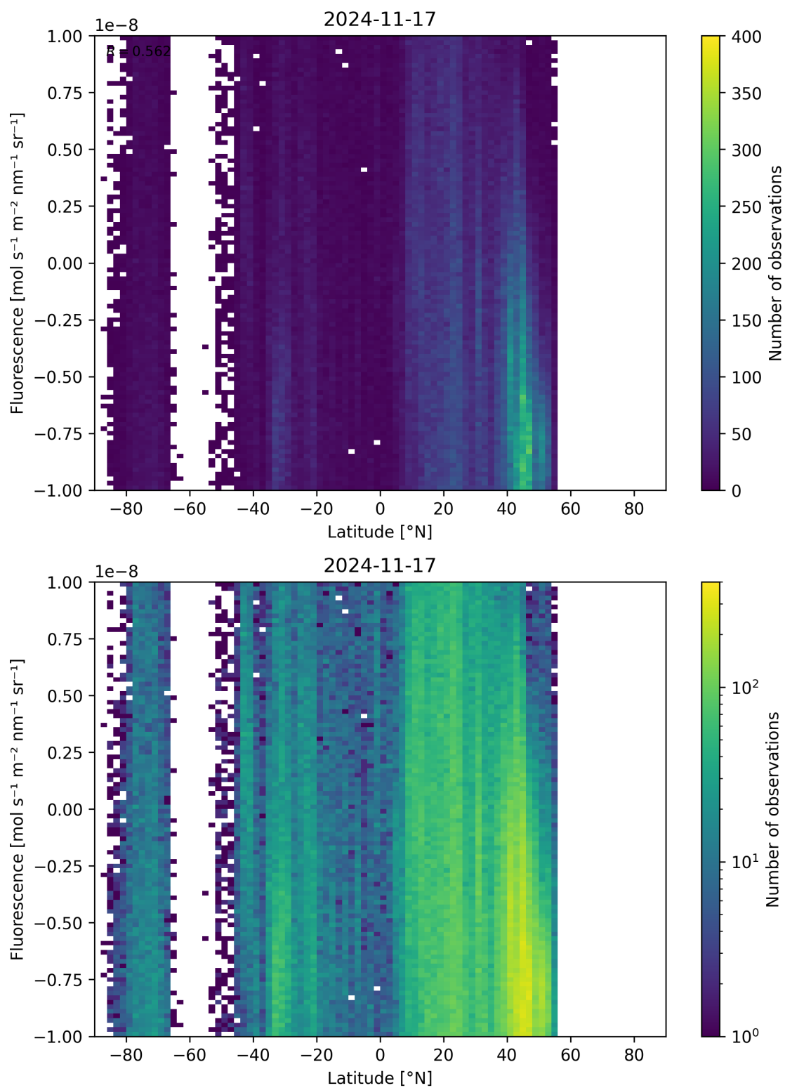
Figure 56: Scatter density plot of “Latitude” against “Fluorescence” for 2024-11-17 to 2024-11-18.
