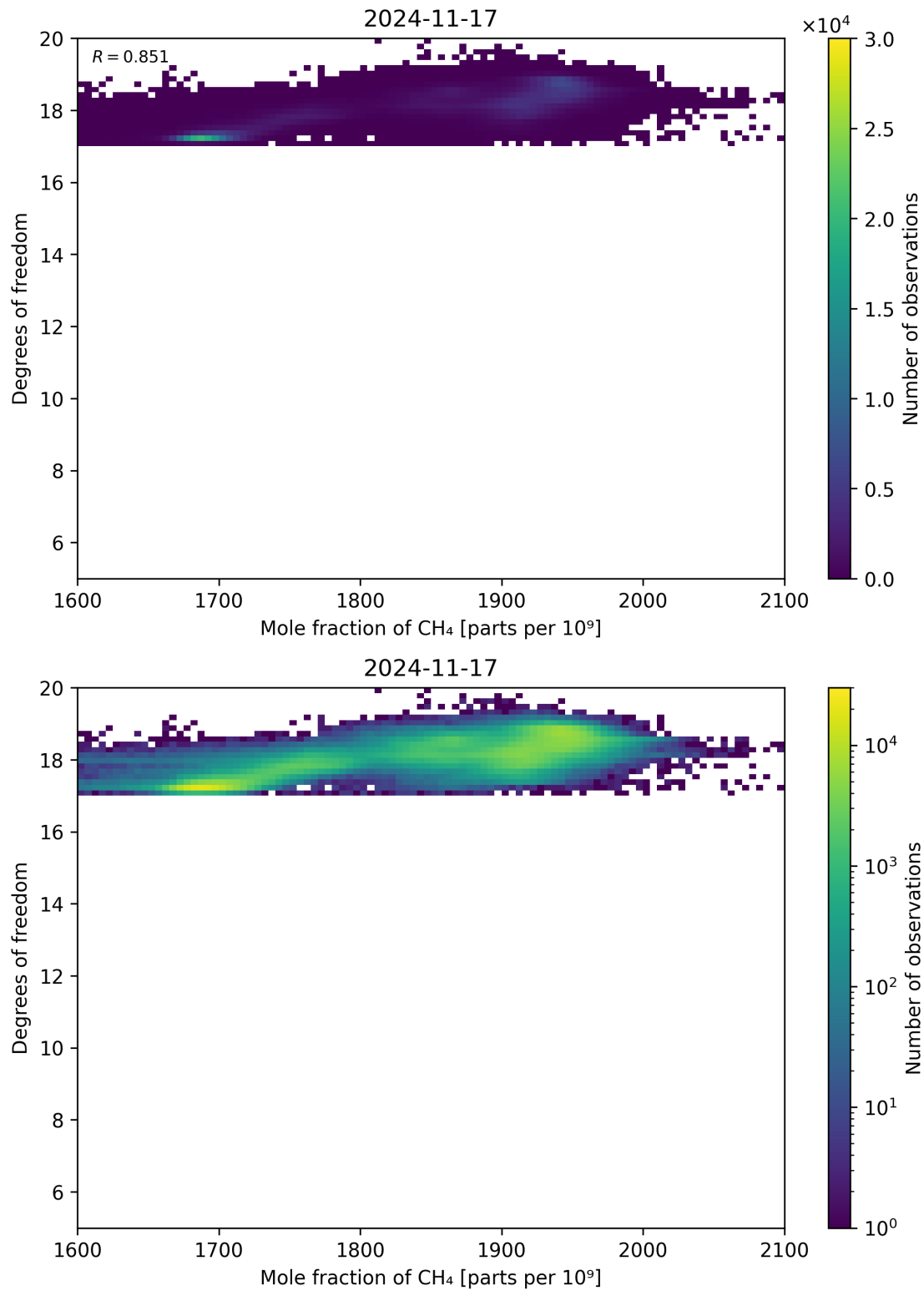
Figure 72: Scatter density plot of “Mole fraction of CH 4 ” against “Degrees of freedom” for 2024-11-17 to 2024-11-18.
