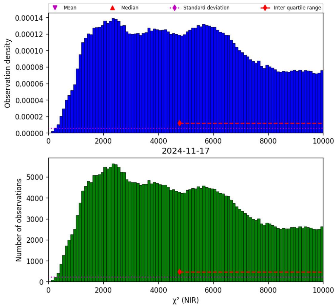
Figure 29: Histogram of " \chi^2 (NIR)" for 2024-11-17 to 2024-11-18
