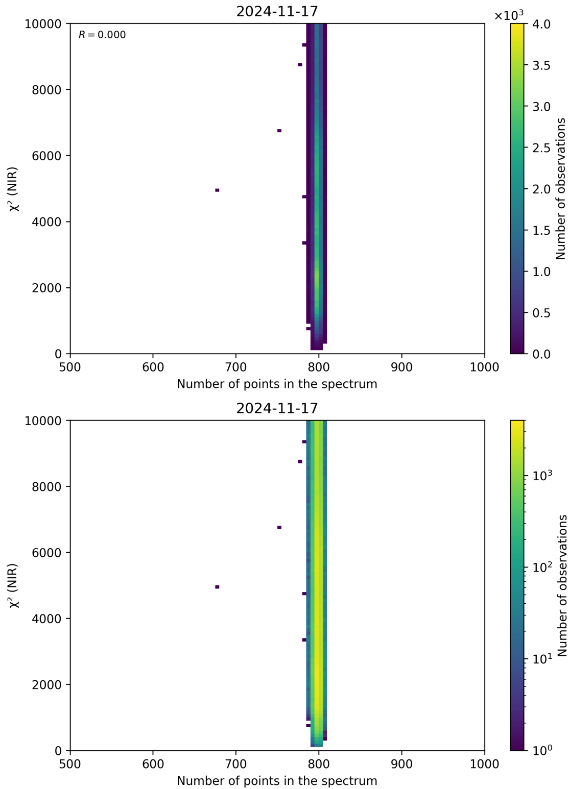
Figure 88: Scatter density plot of “Number of points in the spectrum” against “ \chi^2 (NIR)” for 2024-11-17 to 2024-11-18.
