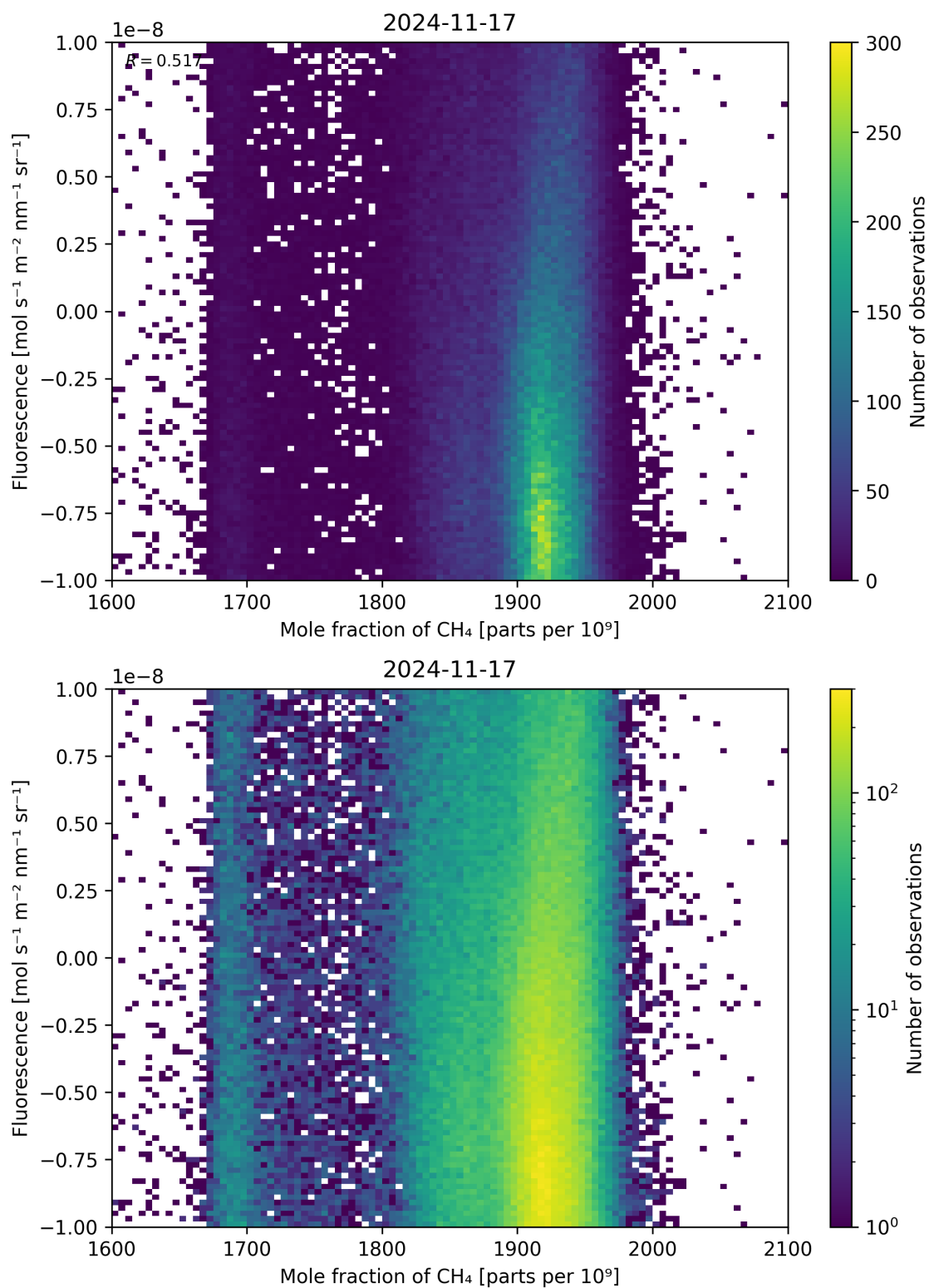
Figure 73: Scatter density plot of “Mole fraction of \text{CH}_4 ” against “Fluorescence” for 2024-11-17 to 2024-11-18.
