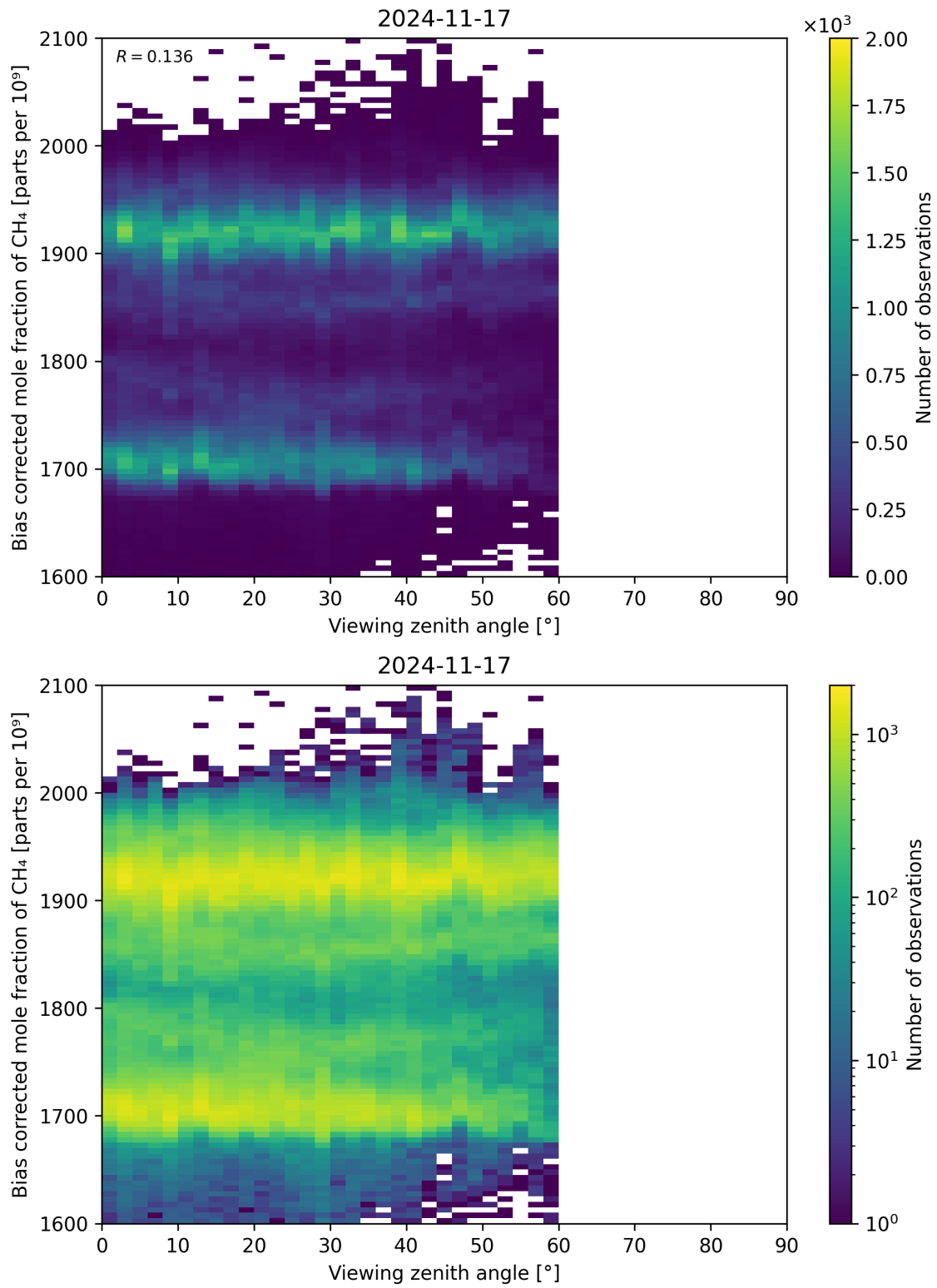
Figure 111: Scatter density plot of “Viewing zenith angle” against “Bias corrected mole fraction of CH 4 ” for 2024-11-17 to 2024-11-18.
