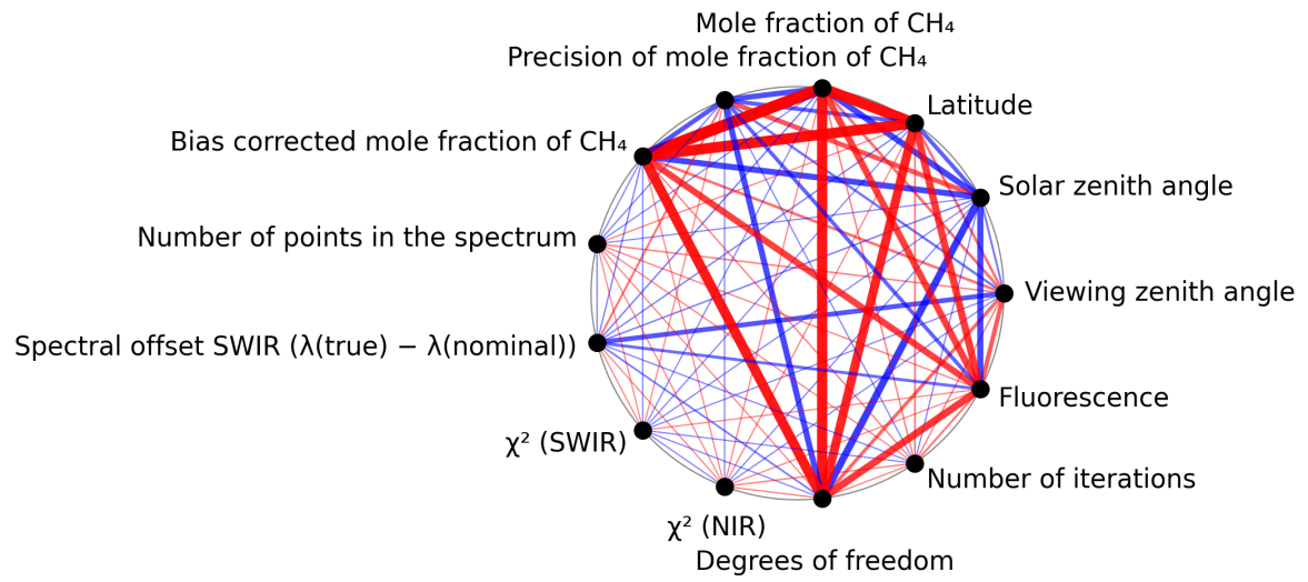
Figure 1: Map of correlation graph for 2024-11-17 to 2024-11-18.
