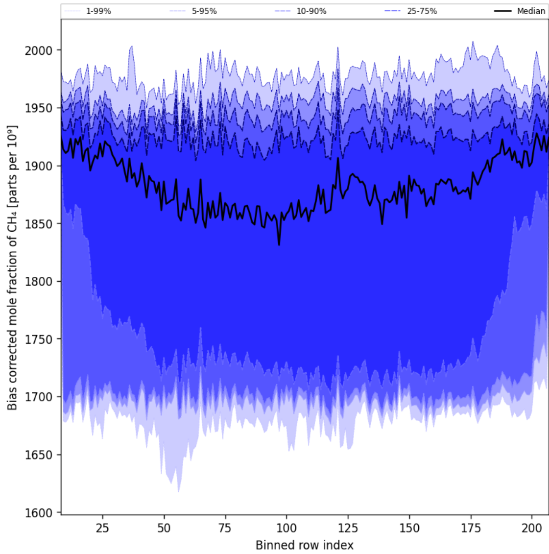
Figure 36: Along track statistics of “Bias corrected mole fraction of CH 4 ” for 2024-11-17 to 2024-11-18
