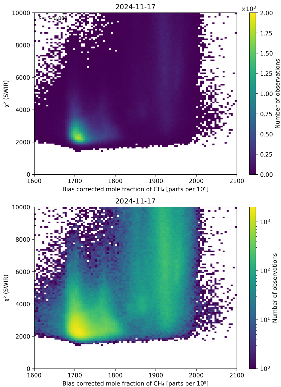
Figure 64: Scatter density plot of “Bias corrected mole fraction of CH 4 ” against “ \chi^2 (SWIR)” for 2024-11-17 to 2024-11-18.
