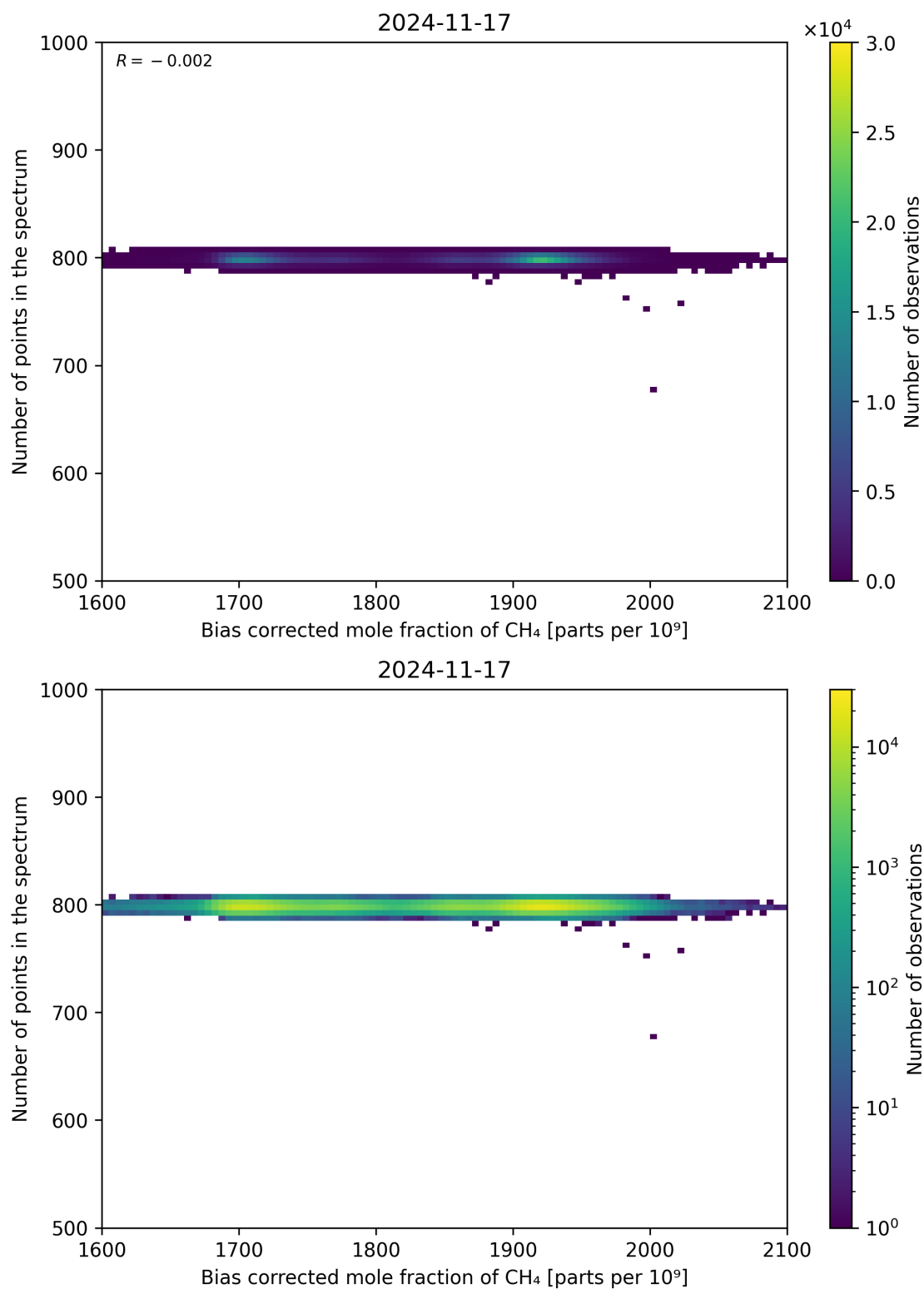
Figure 68: Scatter density plot of “Bias corrected mole fraction of CH 4 ” against “Number of points in the spectrum” for 2024-11-17 to 2024-11-18.
