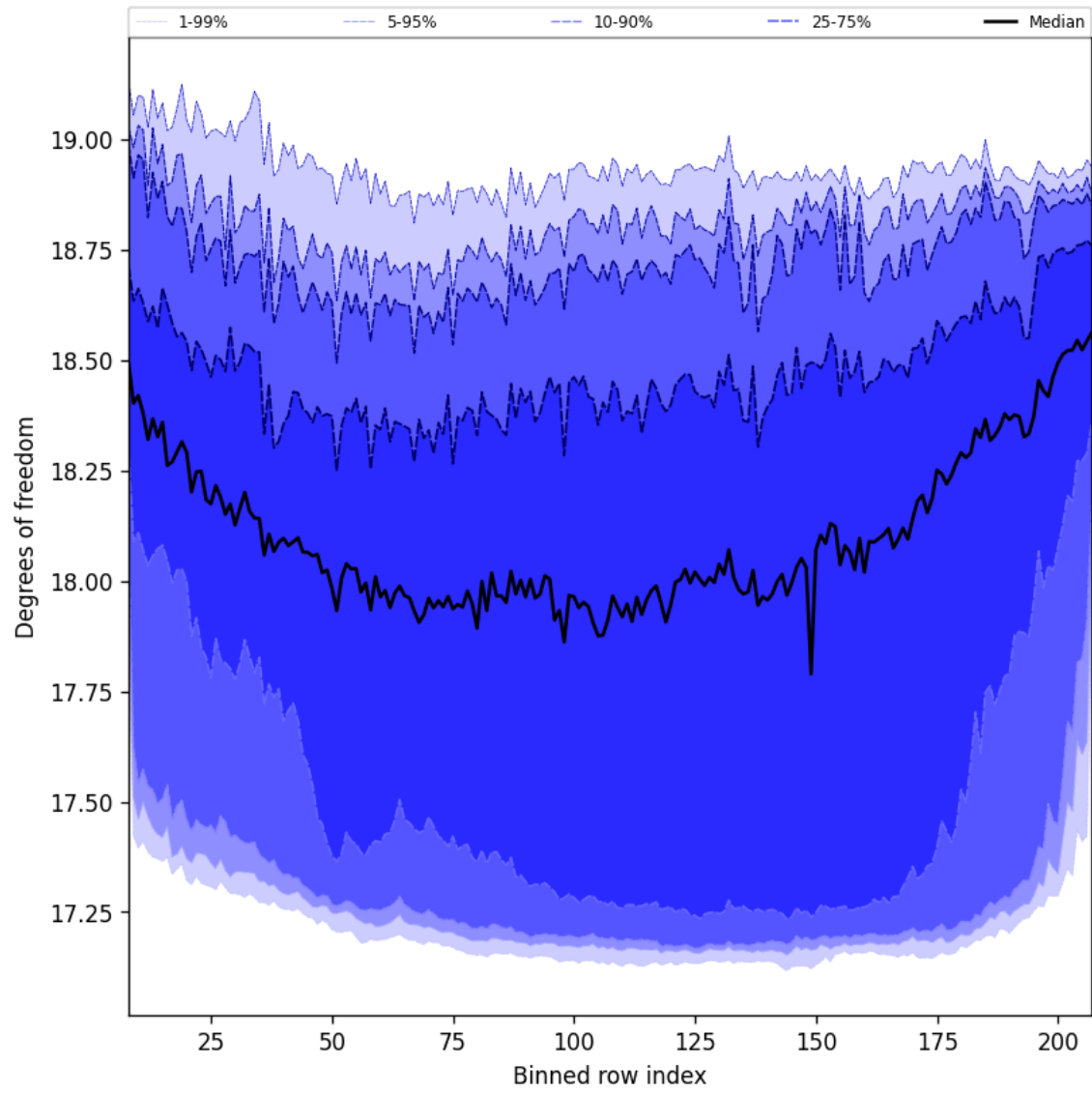
Figure 41: Along track statistics of “Degrees of freedom” for 2024-11-17 to 2024-11-18
