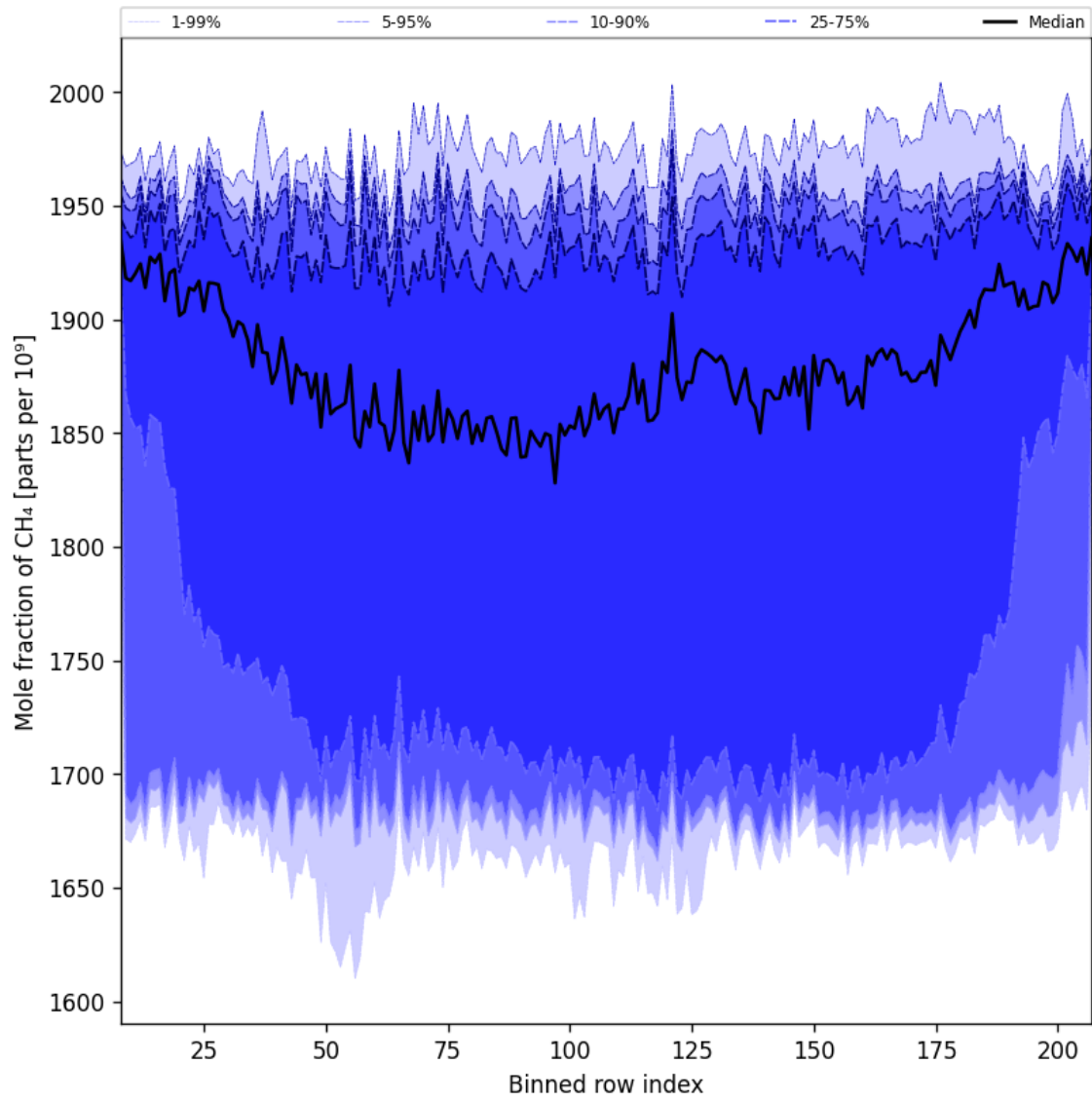
Figure 34: Along track statistics of “Mole fraction of CH 4 ” for 2024-11-17 to 2024-11-18
