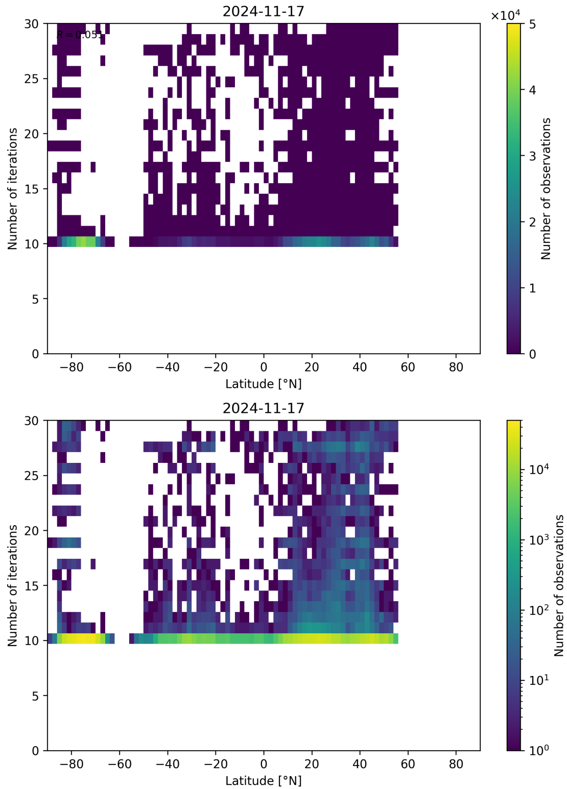
Figure 60: Scatter density plot of “Latitude” against “Number of iterations” for 2024-11-17 to 2024-11-18.
