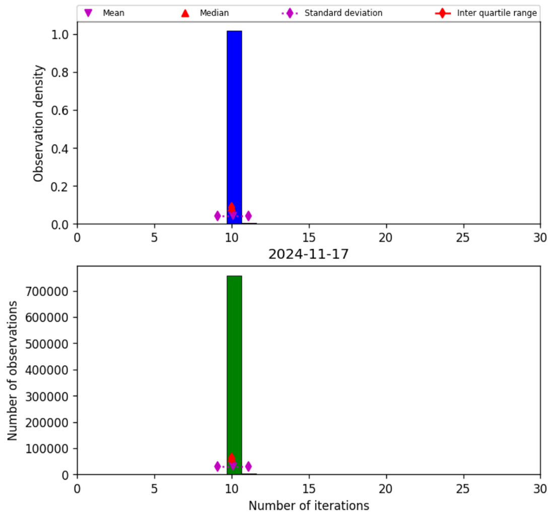
Figure 31: Histogram of “Number of iterations” for 2024-11-17 to 2024-11-18
