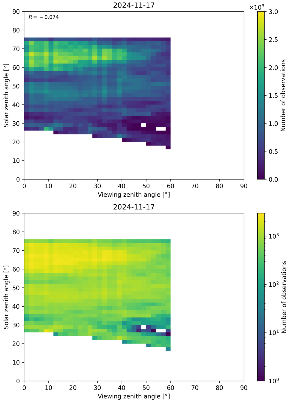
Figure 115: Scatter density plot of “Viewing zenith angle” against “Solar zenith angle” for 2024-11-17 to 2024-11-18.
