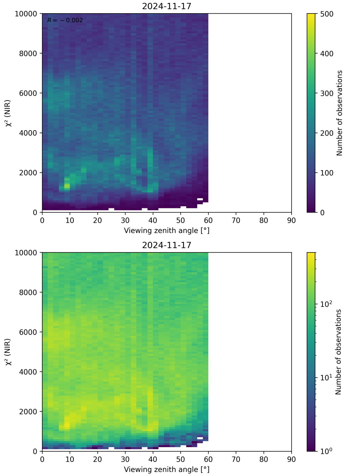
Figure 105: Scatter density plot of “Viewing zenith angle” against “ \chi^2 (NIR)” for 2024-11-17 to 2024-11-18.
