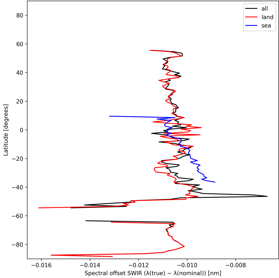
Figure 16: Zonal average of “Spectral offset SWIR ( \lambda_{\text{true}} - \lambda_{\text{nominal}} )” for 2024-11-17 to 2024-11-18.
