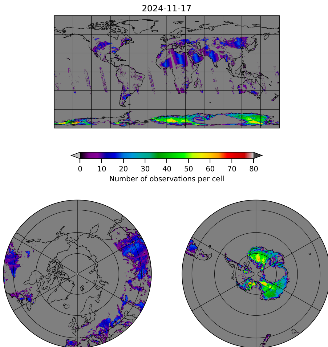
Figure 10: Map of the number of observations for 2024-11-17 to 2024-11-18
