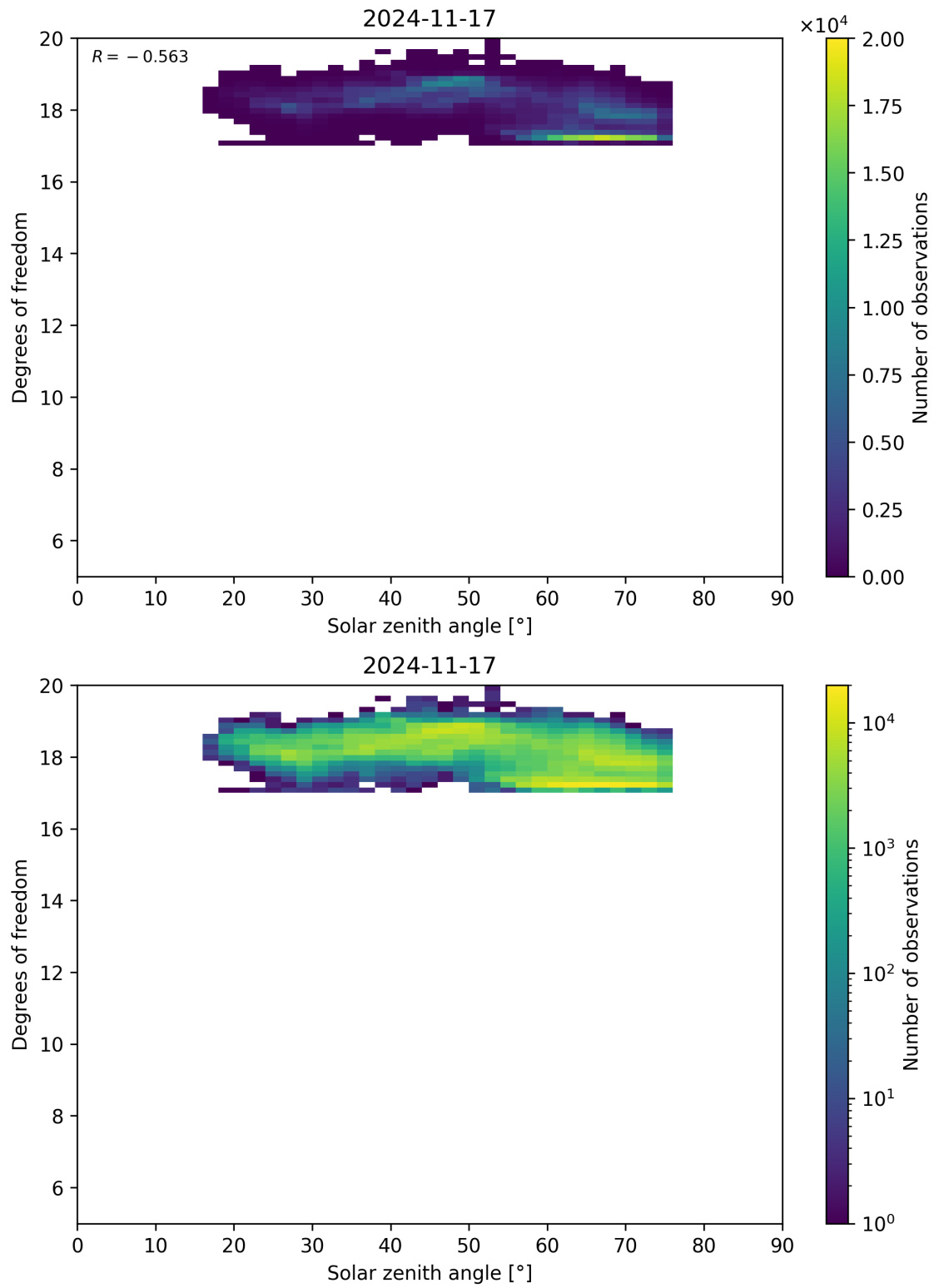
Figure 96: Scatter density plot of “Solar zenith angle” against “Degrees of freedom” for 2024-11-17 to 2024-11-18.
