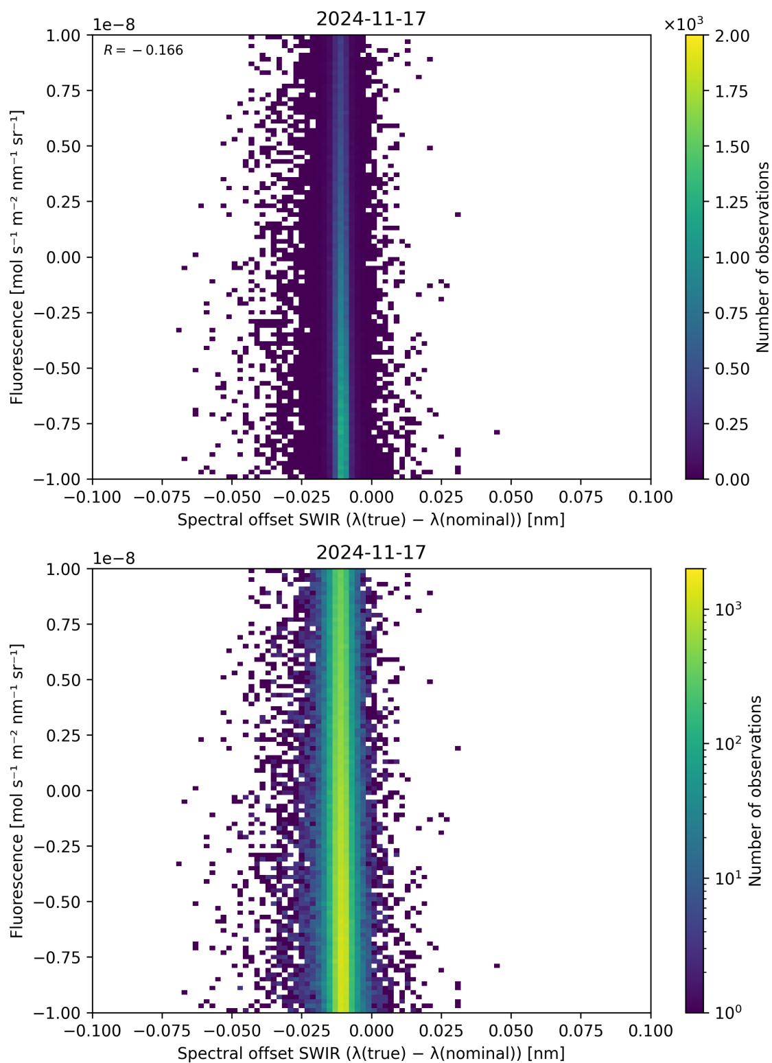
Figure 120: Scatter density plot of “Spectral offset SWIR ( \lambda_{\text{true}} - \lambda_{\text{nominal}} )” against “Fluorescence” for 2024-11-17 to 2024-11-18.
