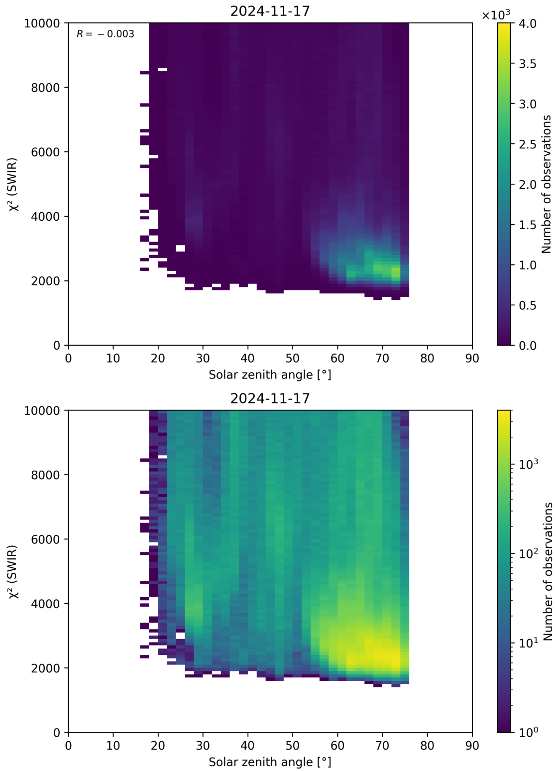
Figure 95: Scatter density plot of “Solar zenith angle” against “ \chi^2 (SWIR)” for 2024-11-17 to 2024-11-18.
