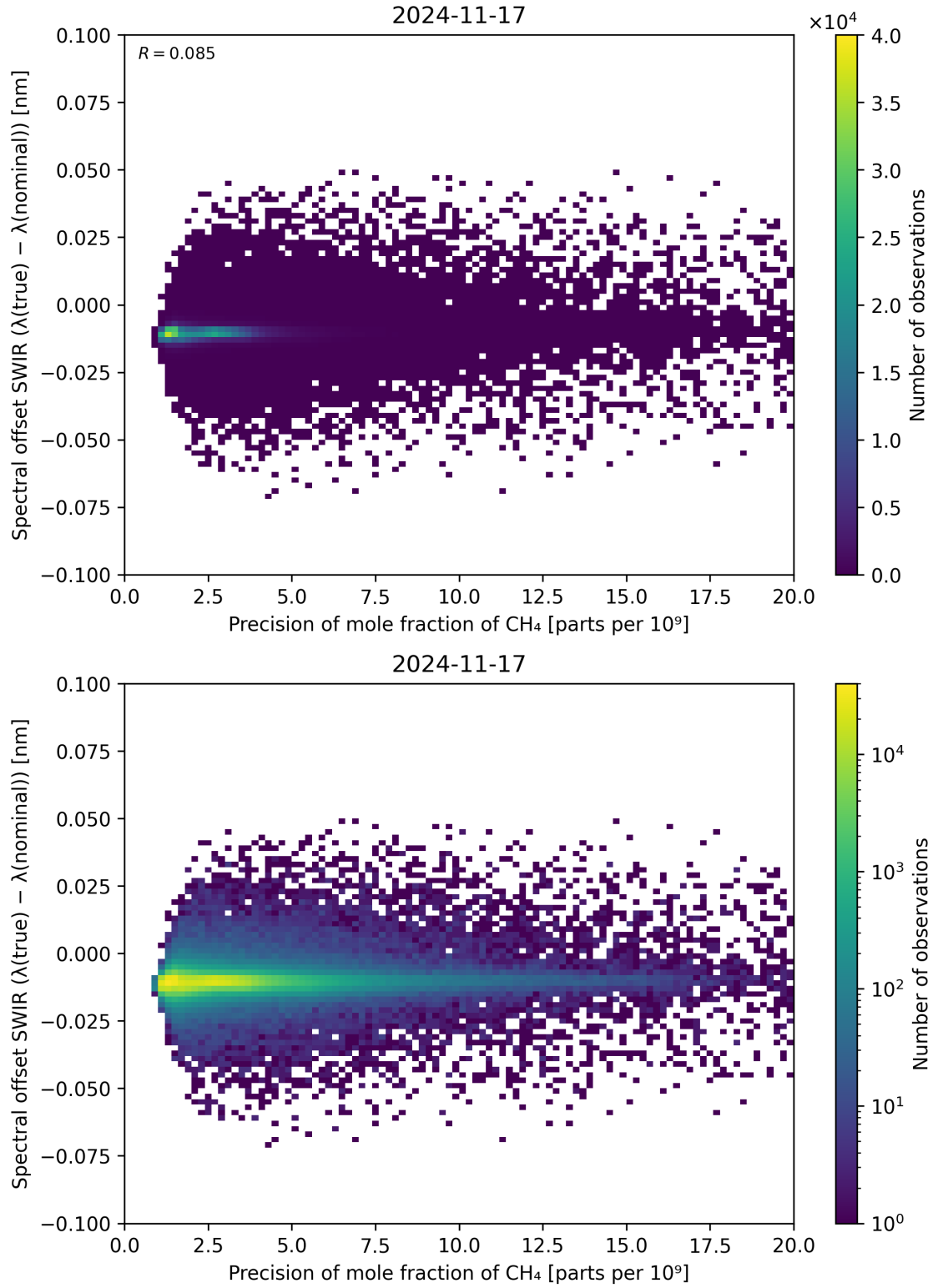
Figure 85: Scatter density plot of “Precision of mole fraction of CH 4 ” against “Spectral offset SWIR ( \lambda_{\text{true}} - \lambda_{\text{nominal}} )” for 2024-11-17 to 2024-11-18.
