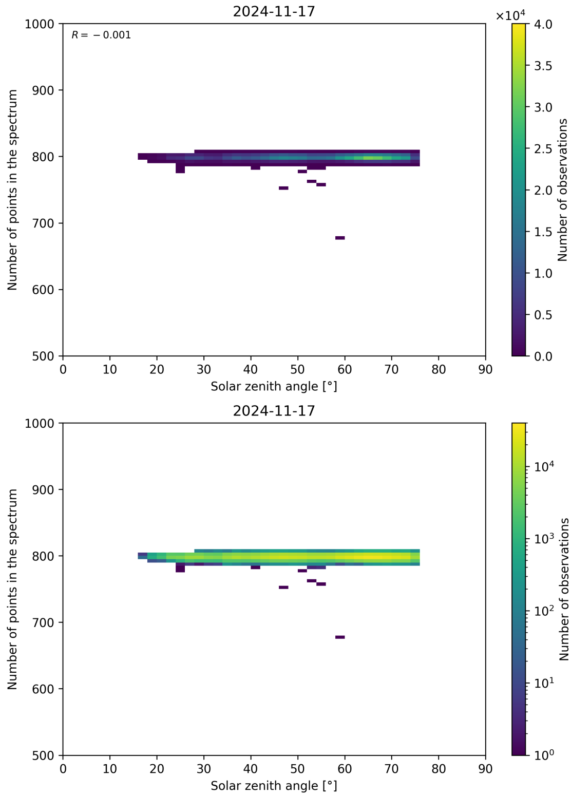
Figure 103: Scatter density plot of “Solar zenith angle” against “Number of points in the spectrum” for 2024-11-17 to 2024-11-18.
