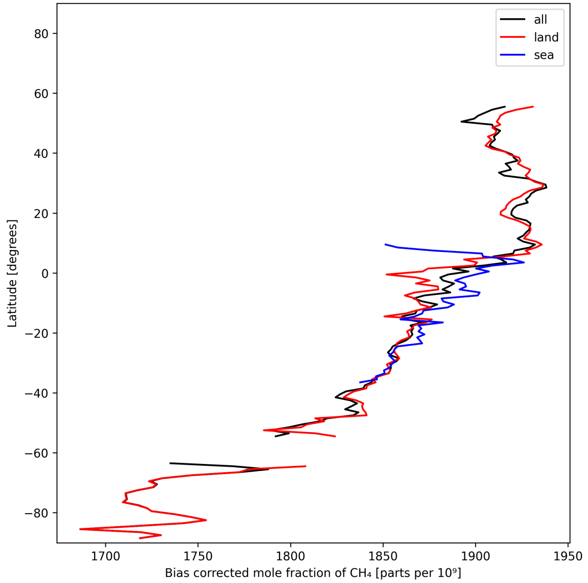
Figure 14: Zonal average of “Bias corrected mole fraction of CH 4 ” for 2024-11-17 to 2024-11-18.
