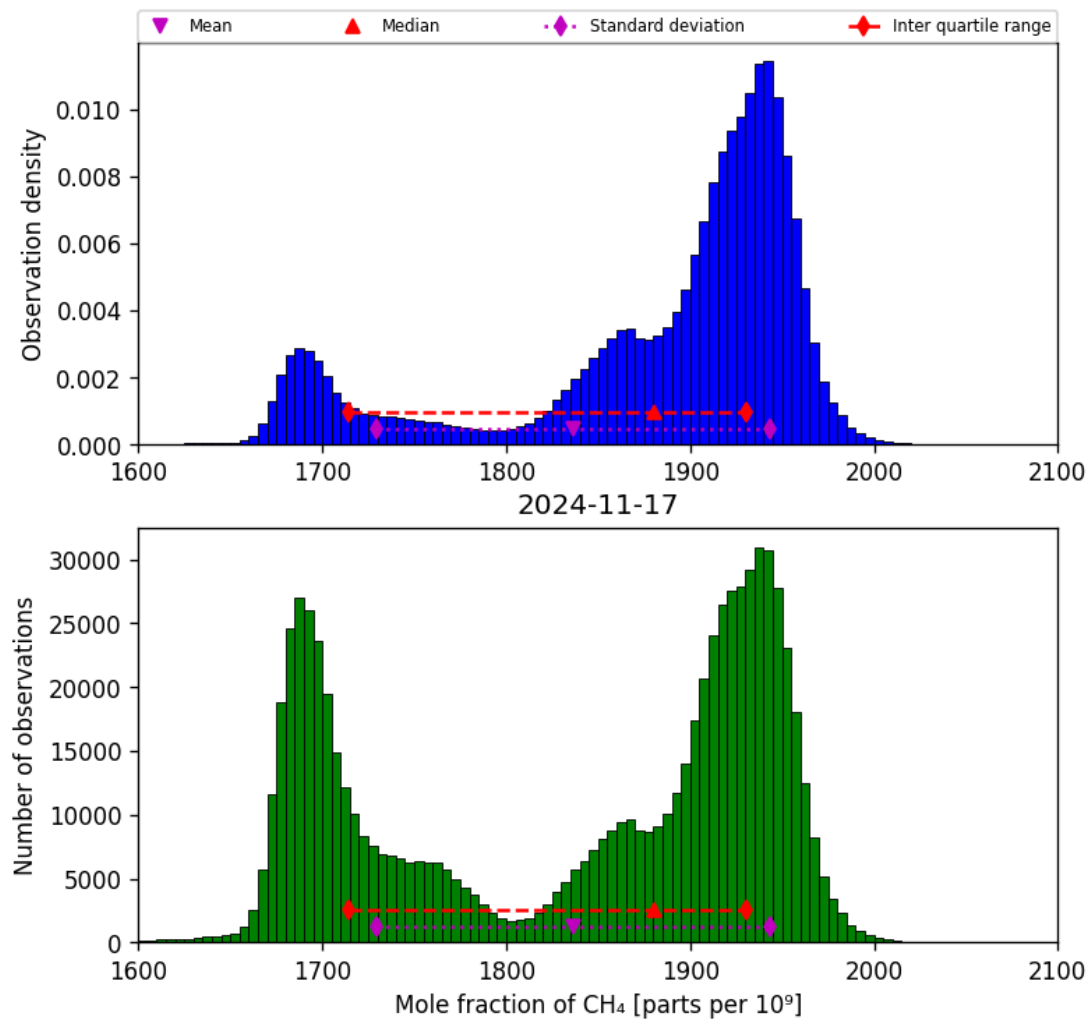
Figure 23: Histogram of “Mole fraction of CH 4 ” for 2024-11-17 to 2024-11-18
