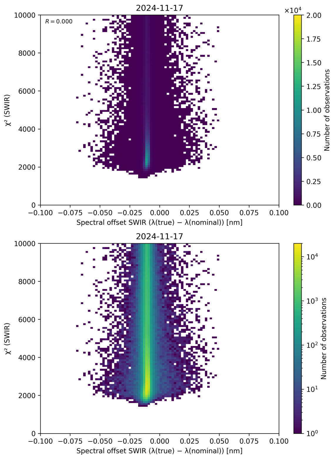
Figure 118: Scatter density plot of “Spectral offset SWIR ( \lambda_{\text{true}} - \lambda_{\text{nominal}} )” against “ \chi^2 (SWIR)” for 2024-11-17 to 2024-11-18.
