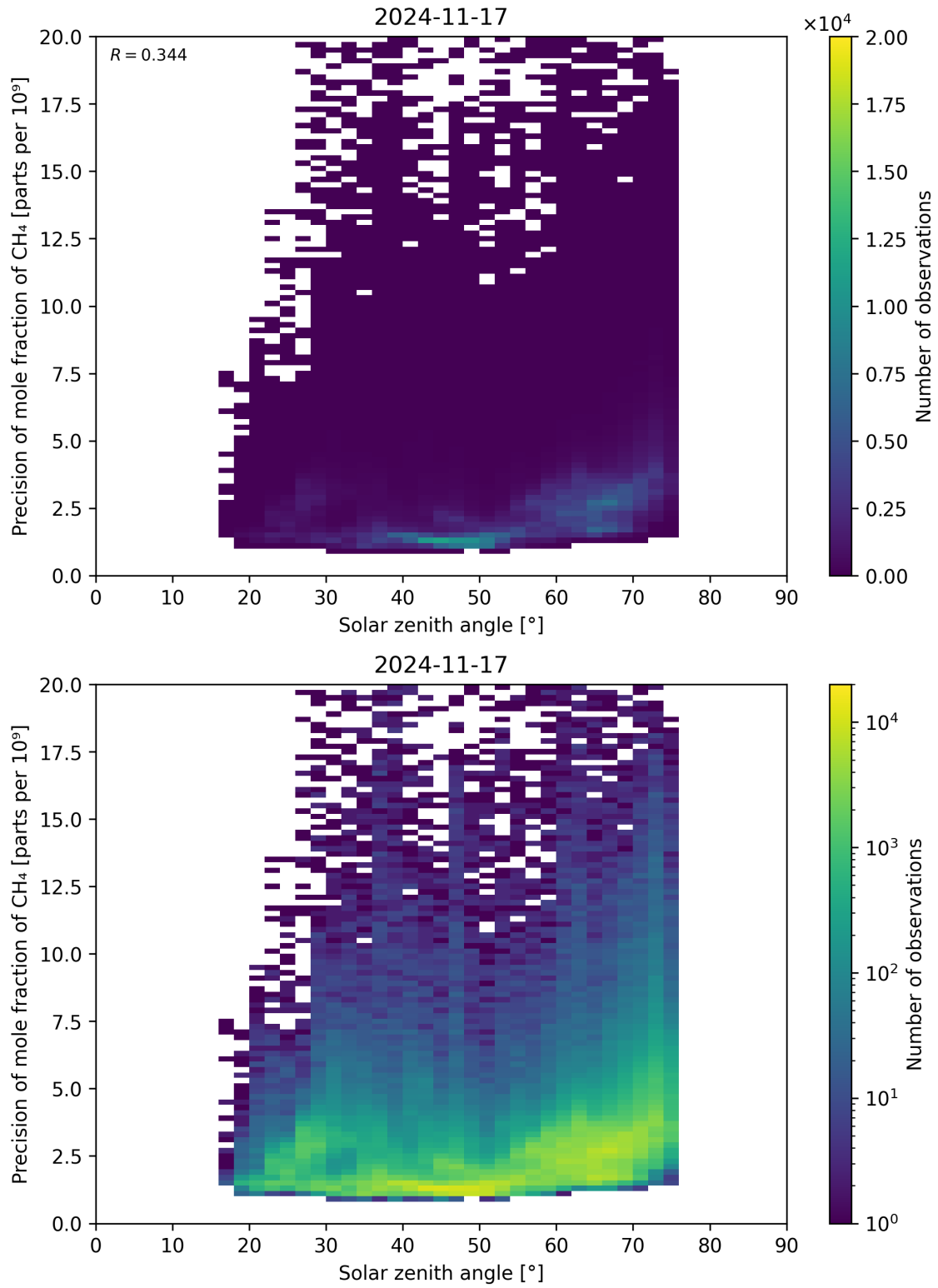
Figure 101: Scatter density plot of “Solar zenith angle” against “Precision of mole fraction of \text{CH}_4 ” for 2024-11-17 to 2024-11-18.
