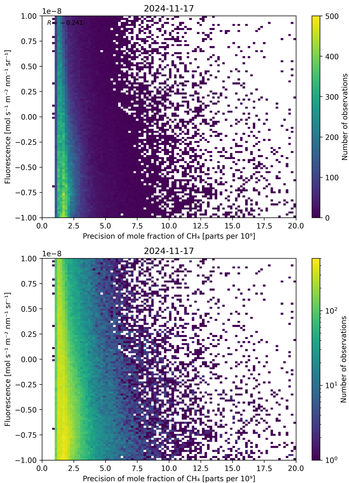
Figure 81: Scatter density plot of “Precision of mole fraction of \text{CH}_4 ” against “Fluorescence” for 2024-11-17 to 2024-11-18.
