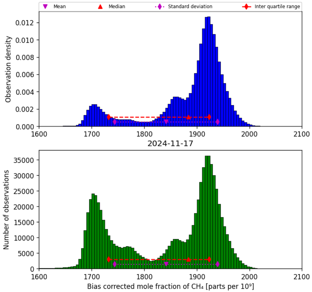
Figure 25: Histogram of “Bias corrected mole fraction of CH 4 ” for 2024-11-17 to 2024-11-18
