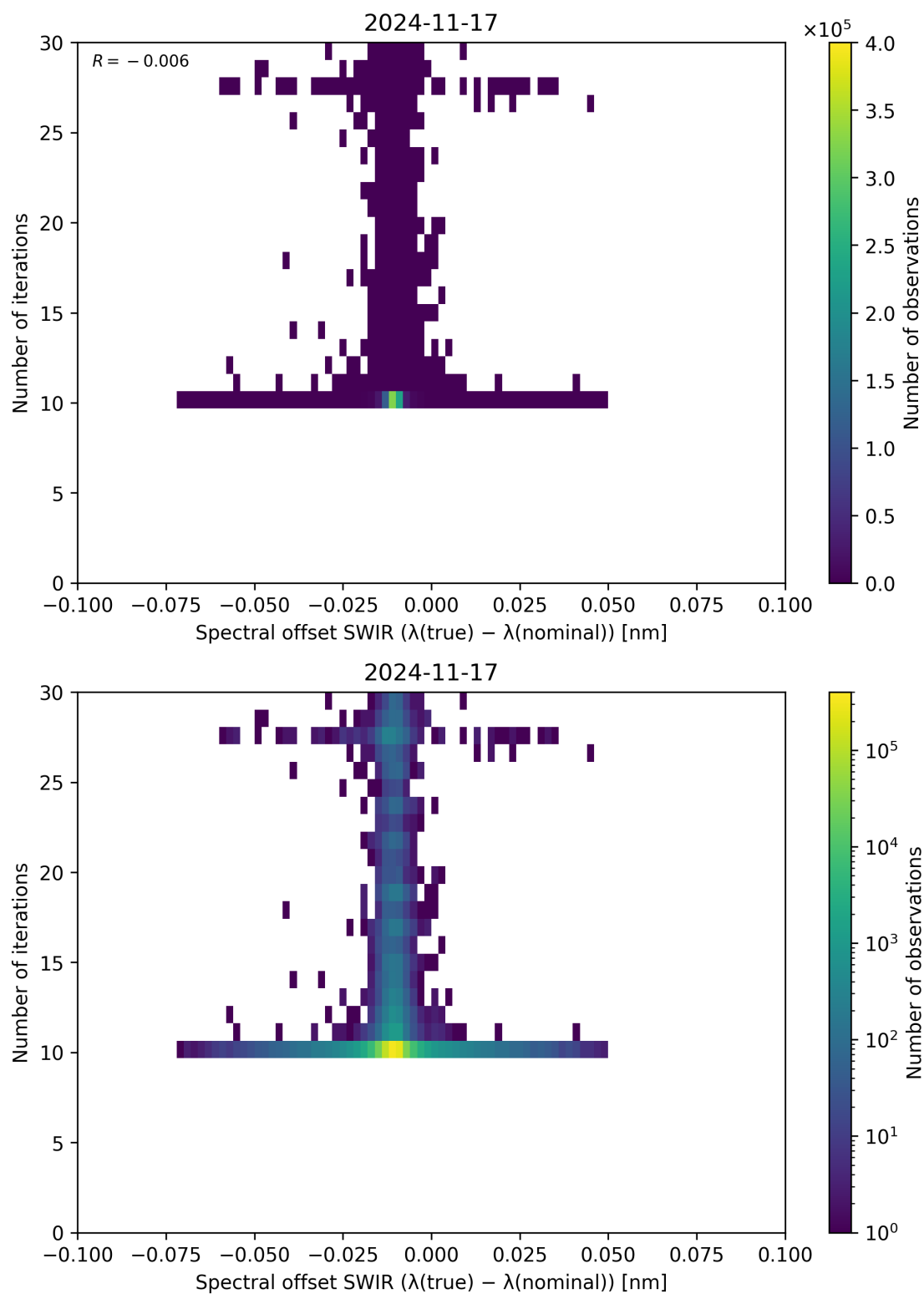
Figure 121: Scatter density plot of “Spectral offset SWIR ( \lambda_{\text{true}} - \lambda_{\text{nominal}} )” against “Number of iterations” for 2024-11-17 to 2024-11-18.
