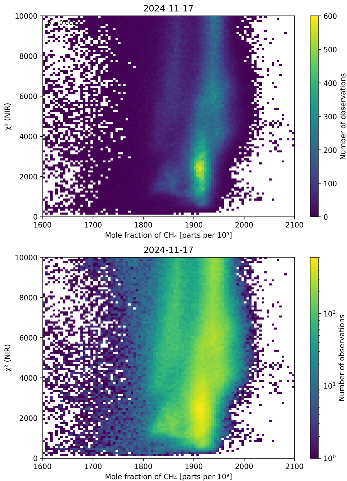
Figure 70: Scatter density plot of “Mole fraction of \text{CH}_4 ” against “ \chi^2 (NIR)” for 2024-11-17 to 2024-11-18.
