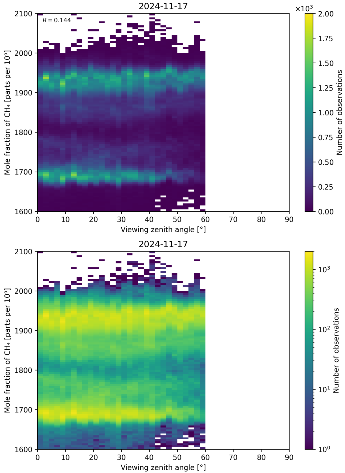
Figure 110: Scatter density plot of “Viewing zenith angle” against “Mole fraction of CH 4 ” for 2024-11-17 to 2024-11-18.
