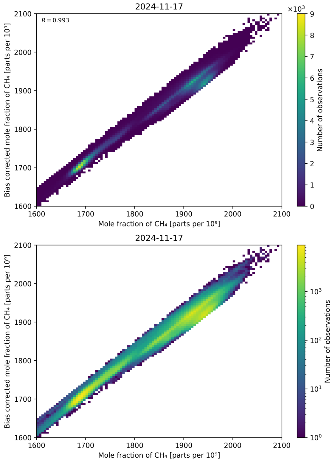
Figure 74: Scatter density plot of “Mole fraction of CH 4 ” against “Bias corrected mole fraction of CH 4 ” for 2024-11-17 to 2024-11-18.
