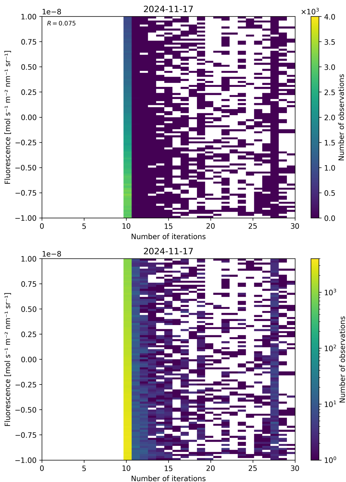
Figure 87: Scatter density plot of “Number of iterations” against “Fluorescence” for 2024-11-17 to 2024-11-18.
