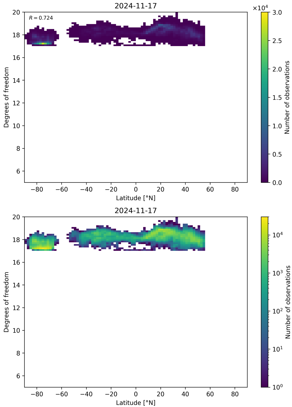
Figure 55: Scatter density plot of “Latitude” against “Degrees of freedom” for 2024-11-17 to 2024-11-18.
