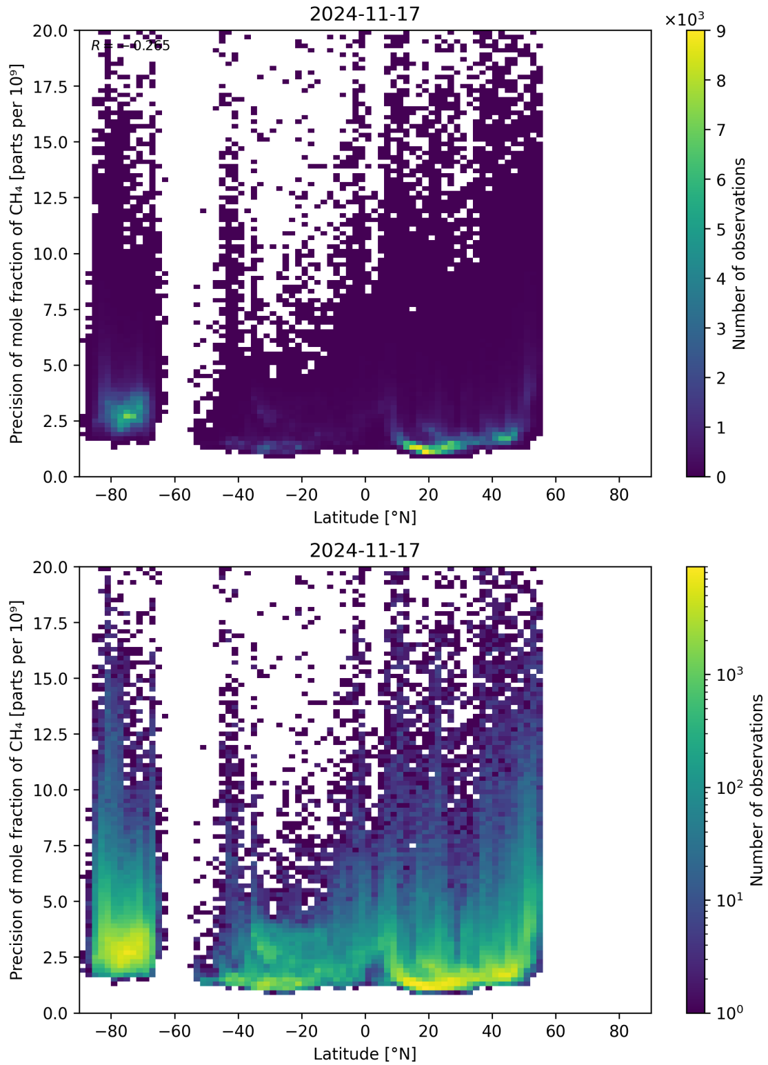
Figure 59: Scatter density plot of “Latitude” against “Precision of mole fraction of CH 4 ” for 2024-11-17 to 2024-11-18.
