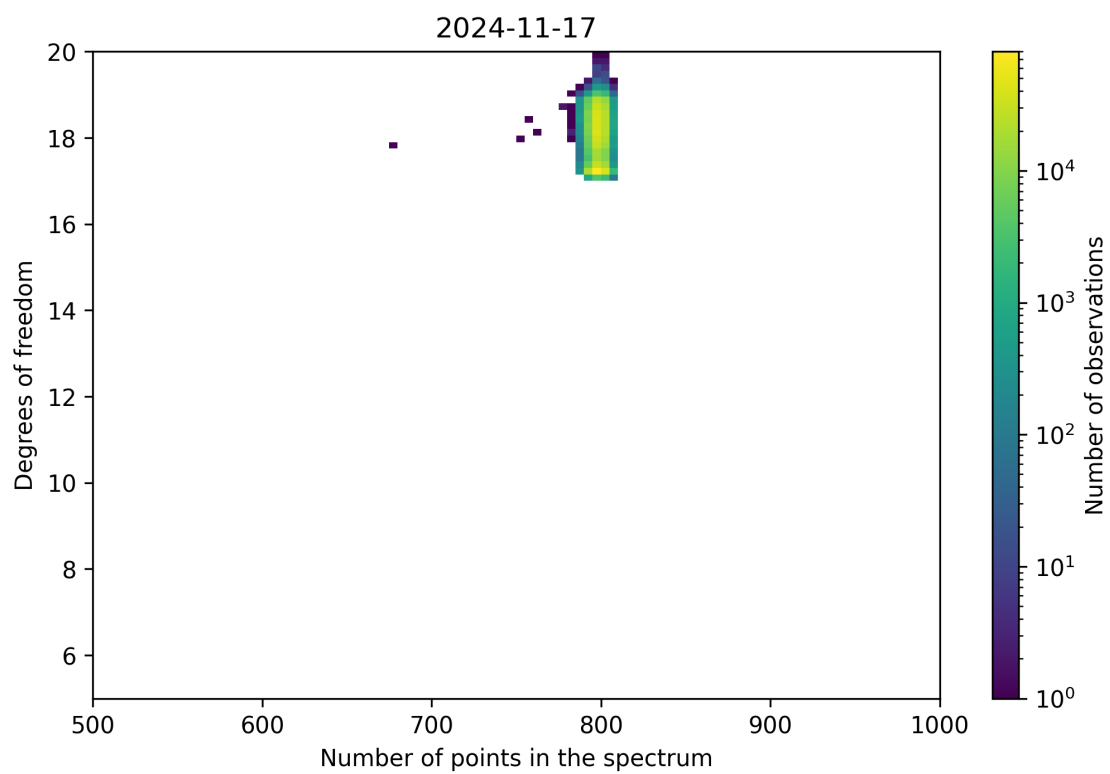
Figure 90: Scatter density plot of “Number of points in the spectrum” against “Degrees of freedom” for 2024-11-17 to 2024-11-18.
