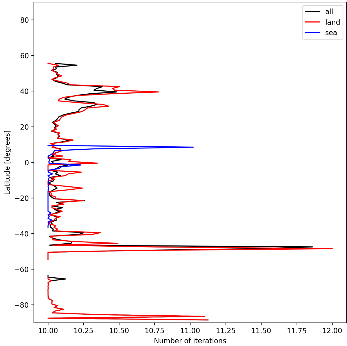
Figure 20: Zonal average of “Number of iterations” for 2024-11-17 to 2024-11-18.
