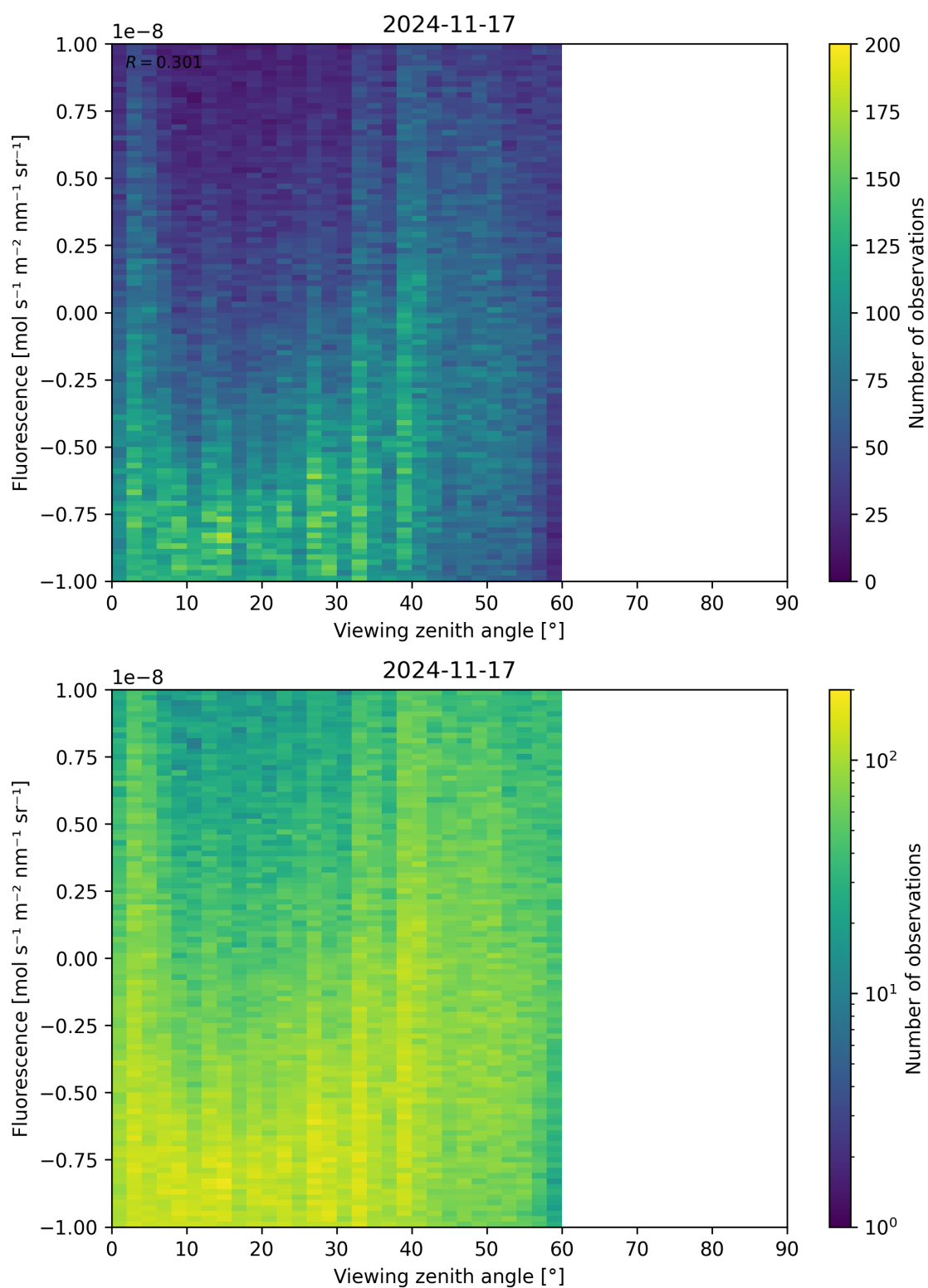
Figure 108: Scatter density plot of “Viewing zenith angle” against “Fluorescence” for 2024-11-17 to 2024-11-18.
