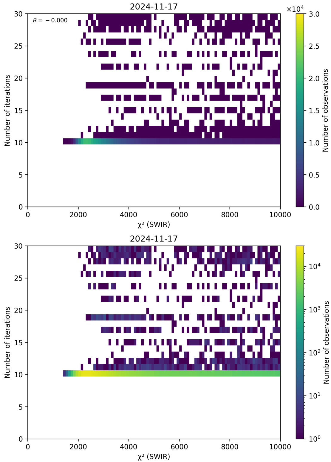
Figure 50: Scatter density plot of “ \chi^2 (SWIR)” against “Number of iterations” for 2024-11-17 to 2024-11-18.
