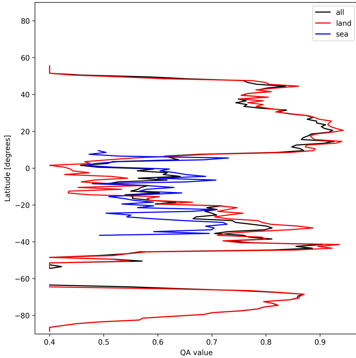
Figure 11: Zonal average of “QA value” for 2024-11-17 to 2024-11-18.
