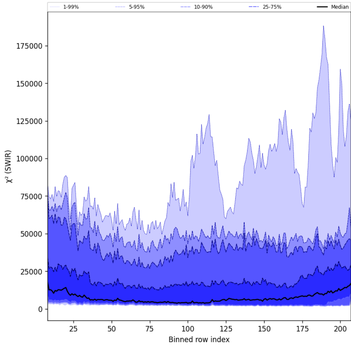
Figure 39: Along track statistics of “ \chi^2 (SWIR)” for 2024-11-17 to 2024-11-18
