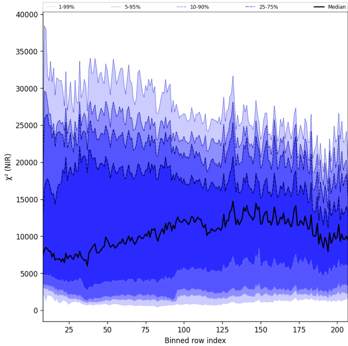
Figure 40: Along track statistics of “ \chi^2 (NIR)” for 2024-11-17 to 2024-11-18
