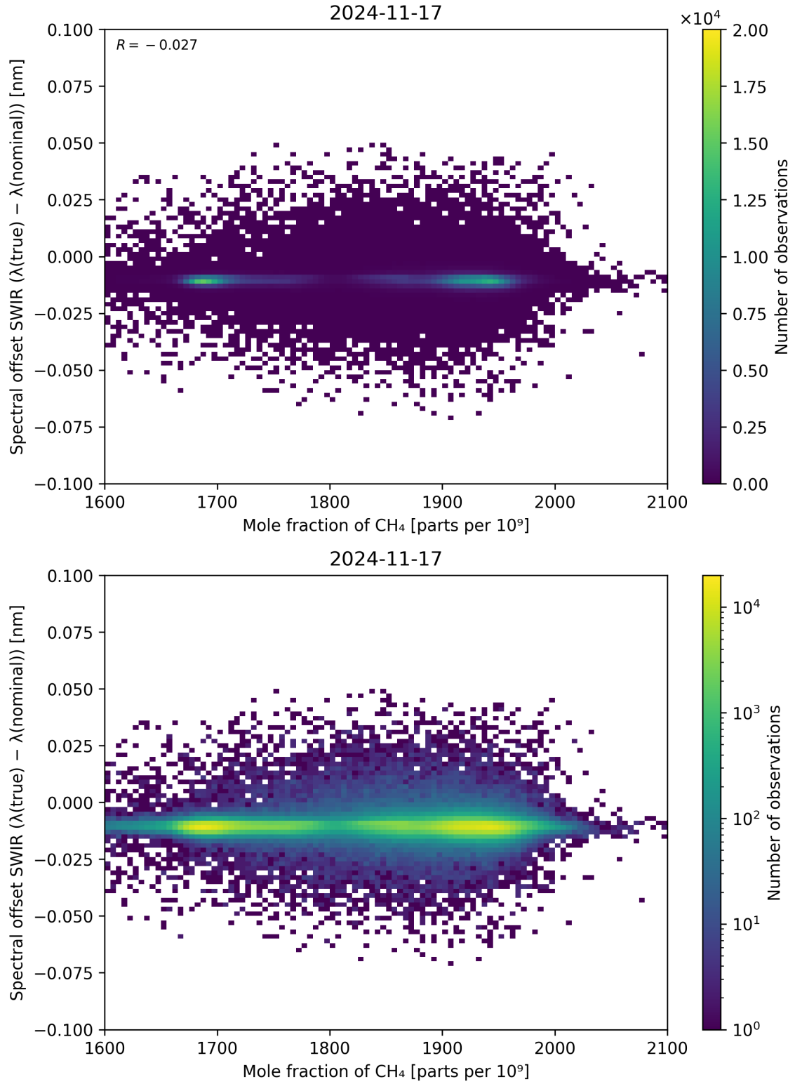
Figure 86: Scatter density plot of “Mole fraction of CH 4 ” against “Spectral offset SWIR ( \lambda_{\text{true}} - \lambda_{\text{nominal}} )” for 2024-11-17 to 2024-11-18.
