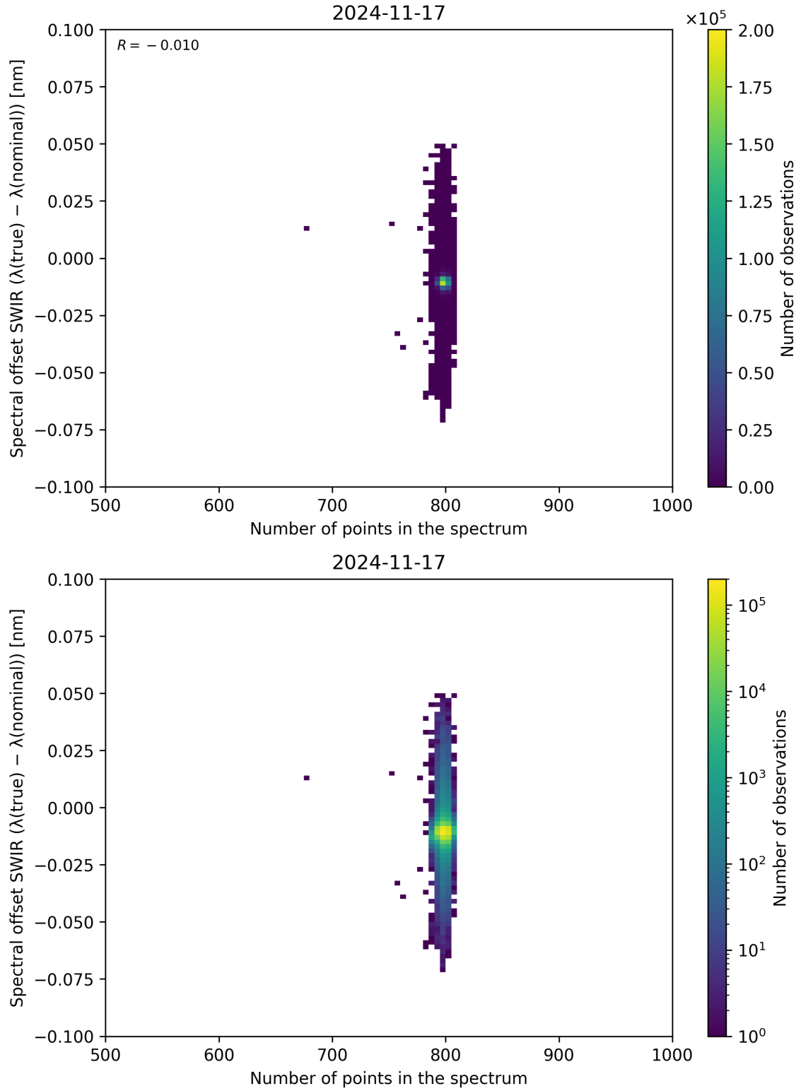
Figure 93: Scatter density plot of “Number of points in the spectrum” against “Spectral offset SWIR ( \lambda_{\text{true}} - \lambda_{\text{nominal}} )” for 2024-11-17 to 2024-11-18.
