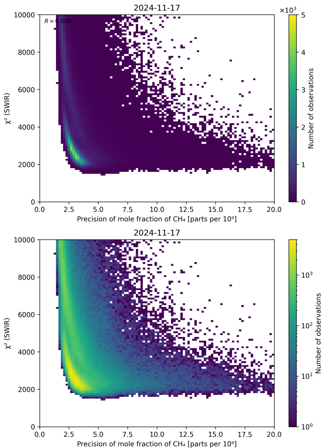
Figure 79: Scatter density plot of “Precision of mole fraction of \text{CH}_4 ” against “ \chi^2 (SWIR)” for 2024-11-17 to 2024-11-18.
