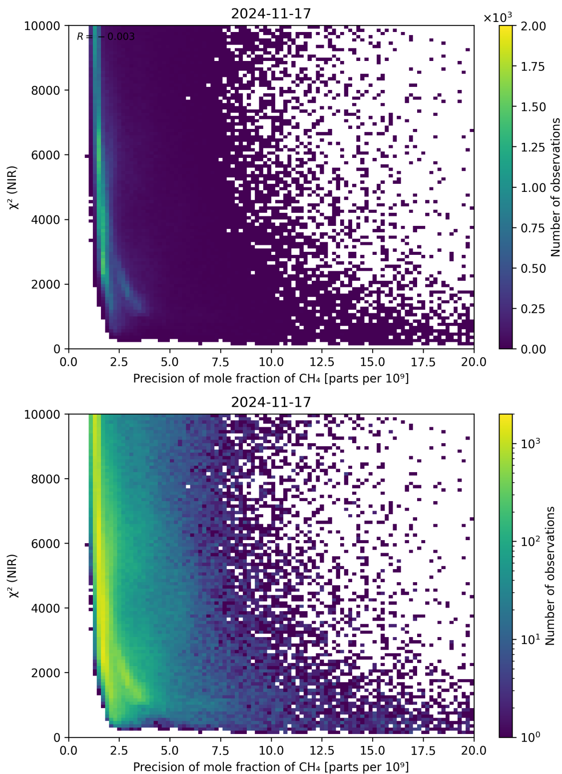
Figure 78: Scatter density plot of “Precision of mole fraction of CH 4 ” against “ \chi^2 (NIR)” for 2024-11-17 to 2024-11-18.
