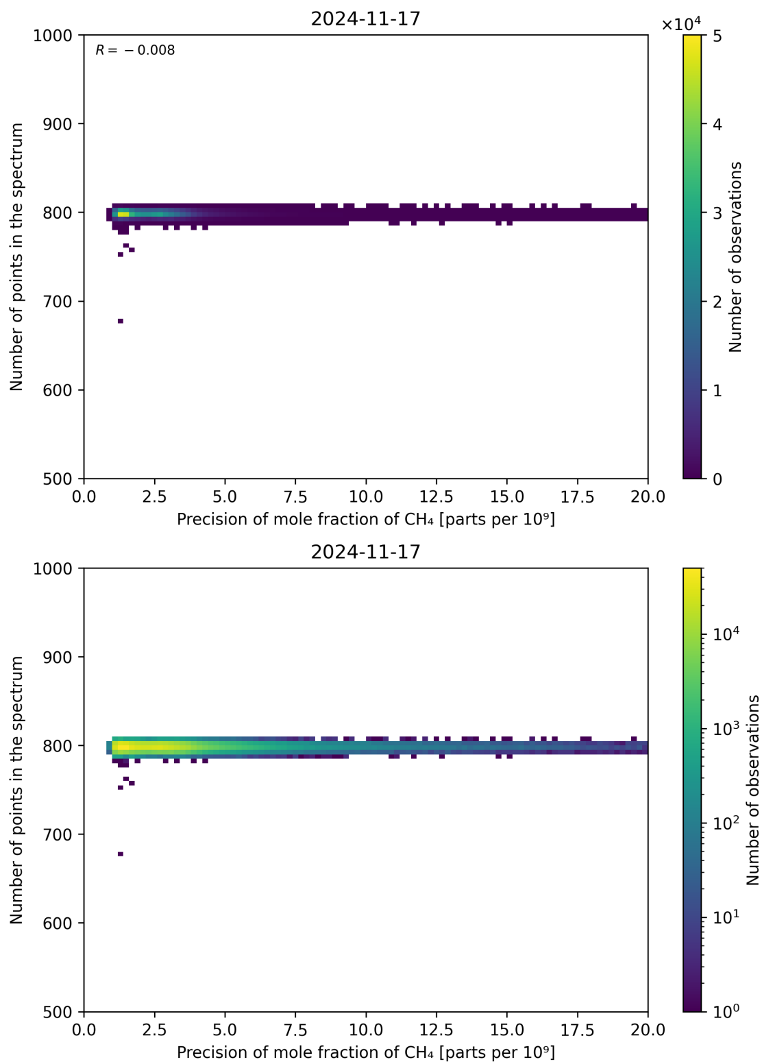
Figure 84: Scatter density plot of “Precision of mole fraction of CH 4 ” against “Number of points in the spectrum” for 2024-11-17 to 2024-11-18.
