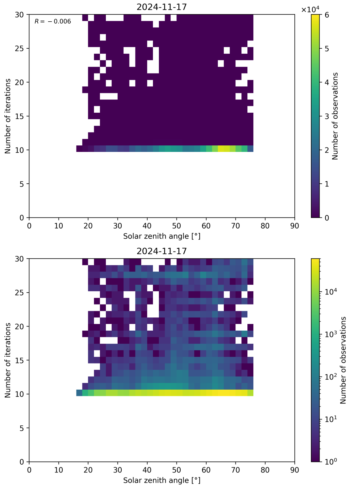
Figure 102: Scatter density plot of “Solar zenith angle” against “Number of iterations” for 2024-11-17 to 2024-11-18.
