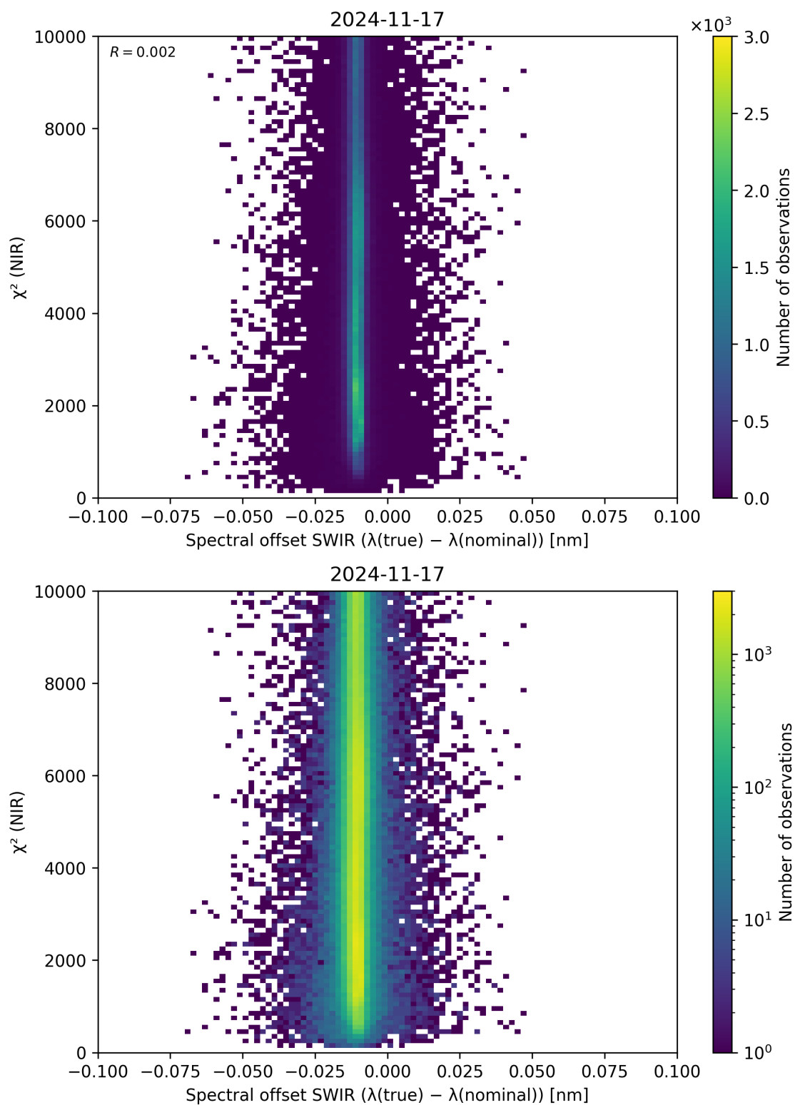
Figure 117: Scatter density plot of “Spectral offset SWIR ( \lambda_{\text{true}} - \lambda_{\text{nominal}} )” against “ \chi^2 (NIR)” for 2024-11-17 to 2024-11-18.
