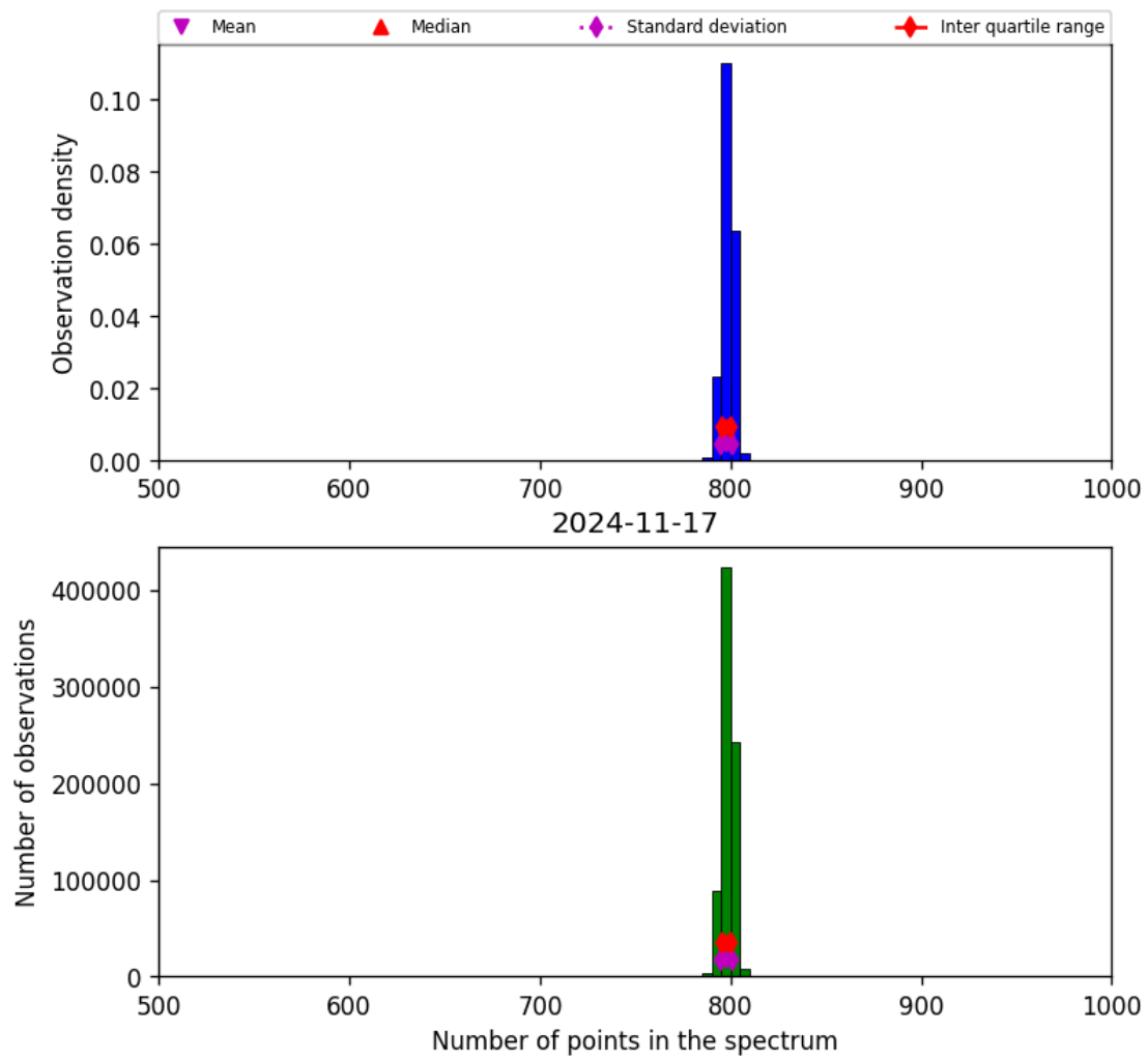
Figure 26: Histogram of “Number of points in the spectrum” for 2024-11-17 to 2024-11-18
