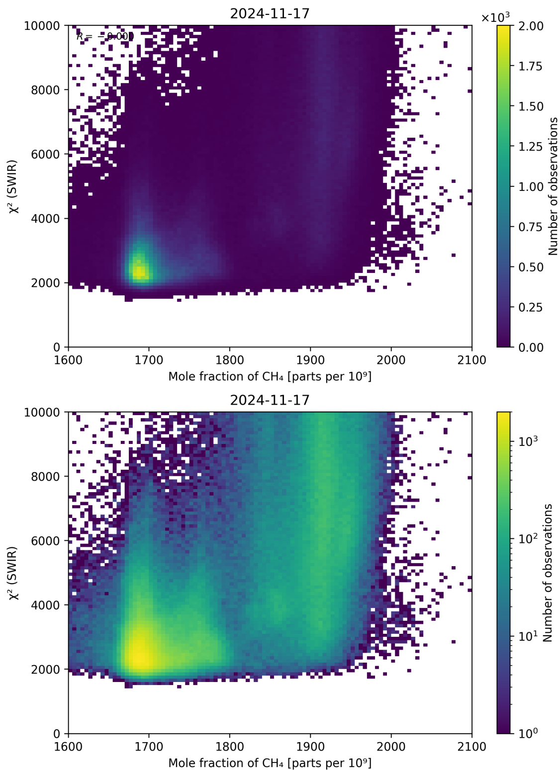
Figure 71: Scatter density plot of “Mole fraction of CH 4 ” against “ \chi^2 (SWIR)” for 2024-11-17 to 2024-11-18.
