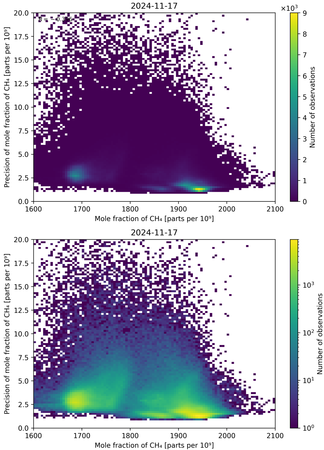
Figure 75: Scatter density plot of “Mole fraction of CH 4 ” against “Precision of mole fraction of CH 4 ” for 2024-11-17 to 2024-11-18.
