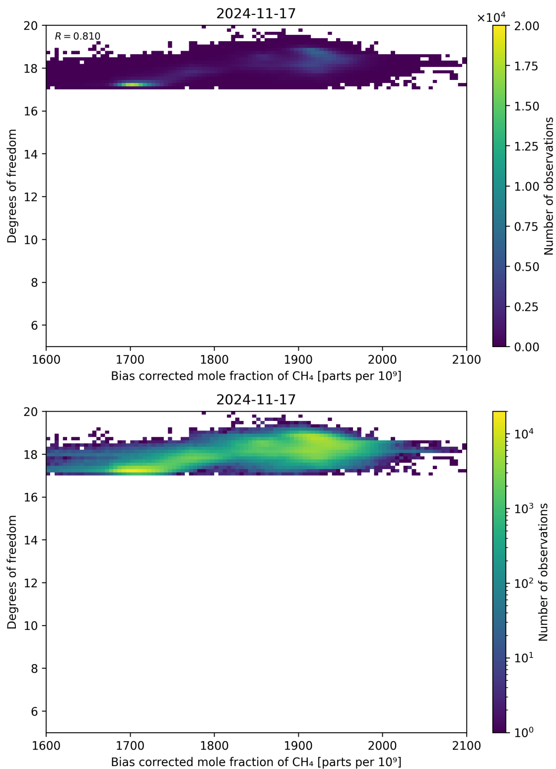
Figure 65: Scatter density plot of “Bias corrected mole fraction of CH 4 ” against “Degrees of freedom” for 2024-11-17 to 2024-11-18.
