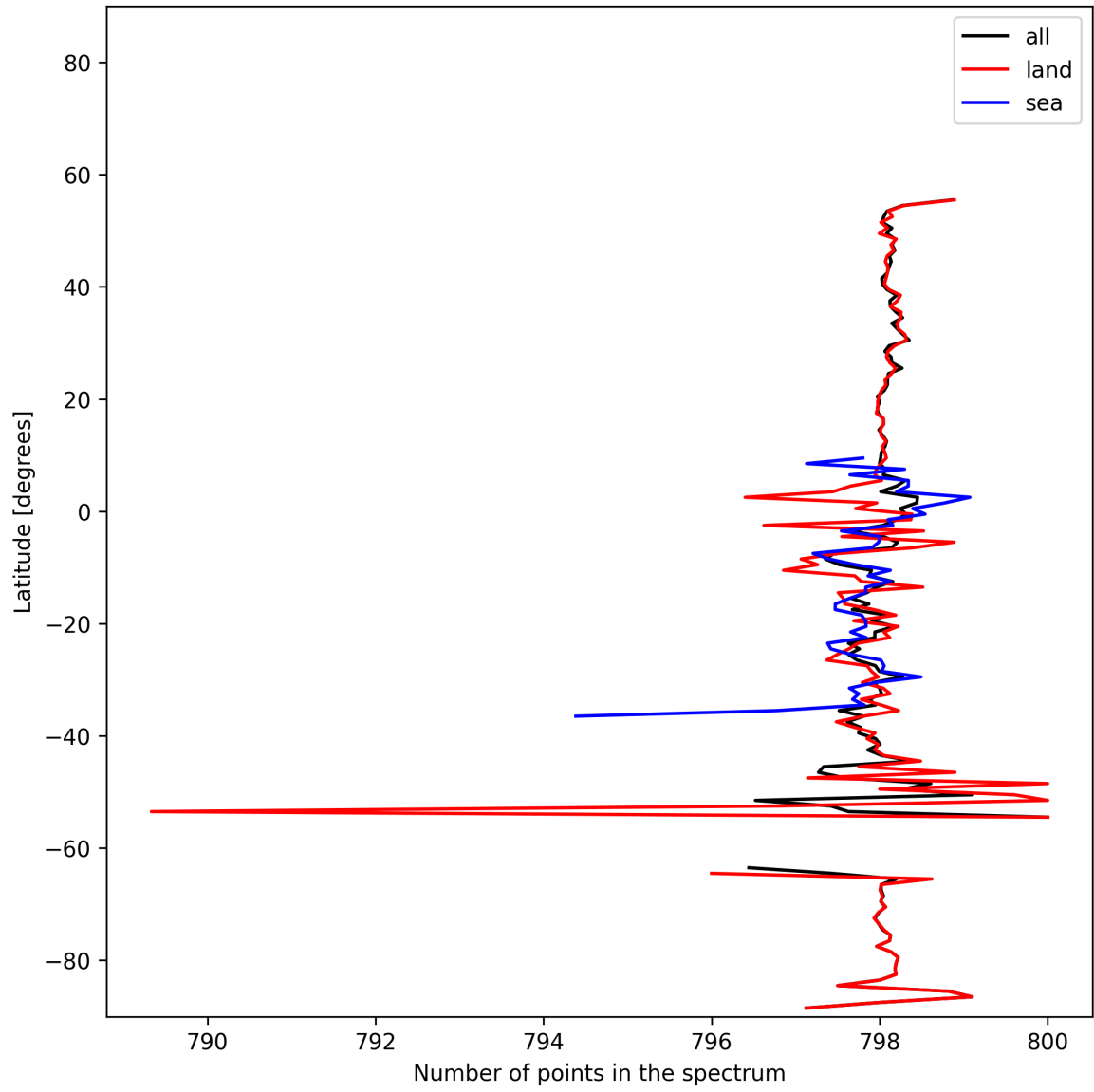
Figure 15: Zonal average of “Number of points in the spectrum” for 2024-11-17 to 2024-11-18.
