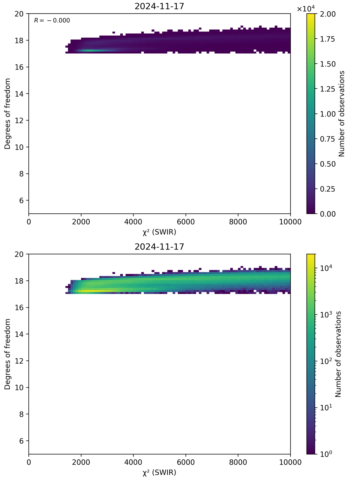
Figure 48: Scatter density plot of “ \chi^2 (SWIR)” against “Degrees of freedom” for 2024-11-17 to 2024-11-18.
