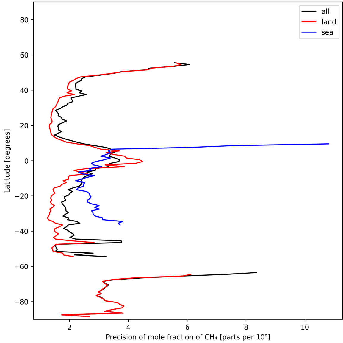
Figure 13: Zonal average of “Precision of mole fraction of CH 4 ” for 2024-11-17 to 2024-11-18.
