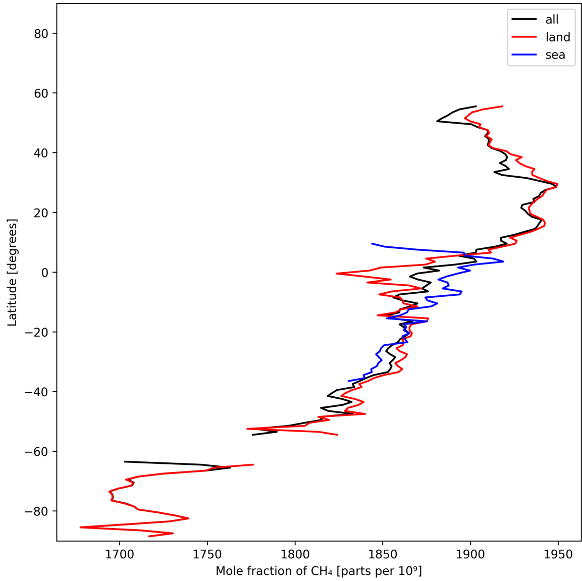
Figure 12: Zonal average of “Mole fraction of CH 4 ” for 2024-11-17 to 2024-11-18.
