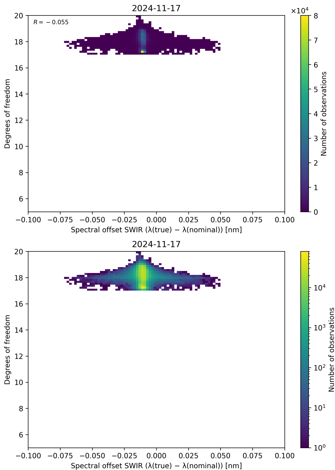
Figure 119: Scatter density plot of “Spectral offset SWIR ( \lambda_{\text{true}} - \lambda_{\text{nominal}} )” against “Degrees of freedom” for 2024-11-17 to 2024-11-18.
