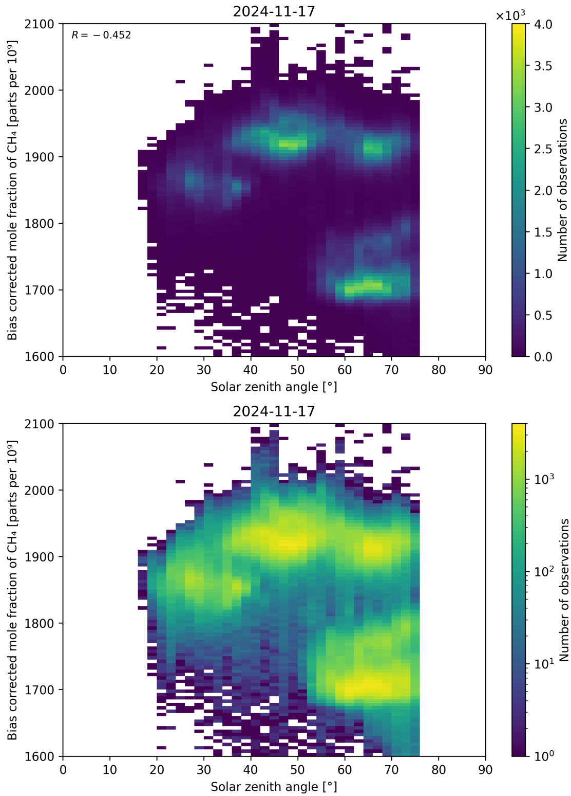
Figure 100: Scatter density plot of “Solar zenith angle” against “Bias corrected mole fraction of CH 4 ” for 2024-11-17 to 2024-11-18.
