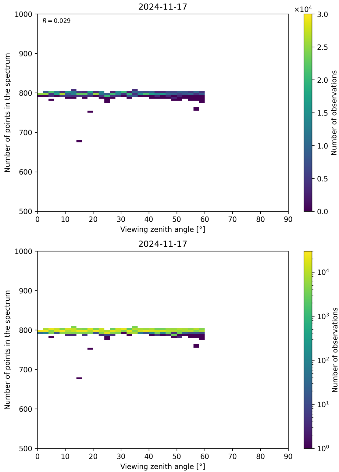
Figure 114: Scatter density plot of “Viewing zenith angle” against “Number of points in the spectrum” for 2024-11-17 to 2024-11-18.
