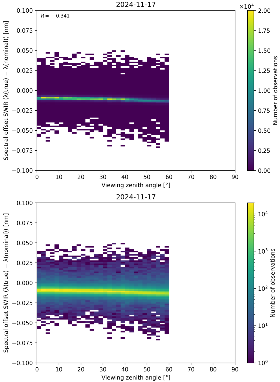
Figure 116: Scatter density plot of “Viewing zenith angle” against “Spectral offset SWIR ( \lambda_{\text{true}} - \lambda_{\text{nominal}} )” for 2024-11-17 to 2024-11-18.
