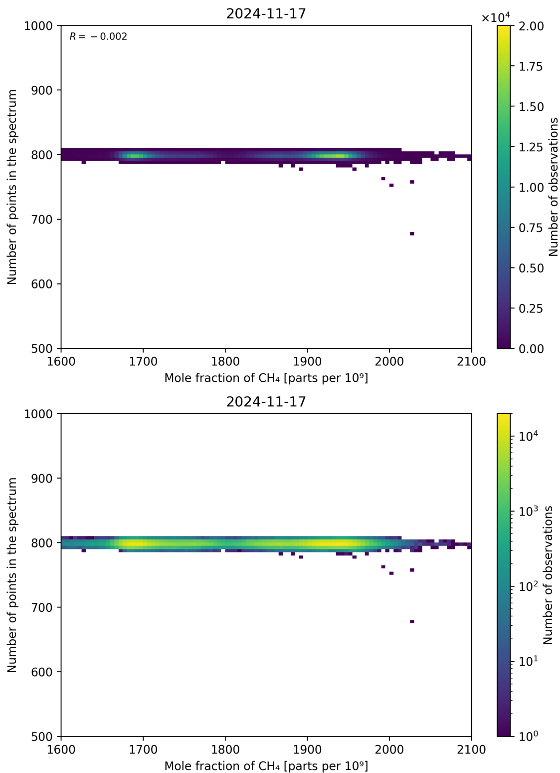
Figure 77: Scatter density plot of “Mole fraction of CH 4 ” against “Number of points in the spectrum” for 2024-11-17 to 2024-11-18.
