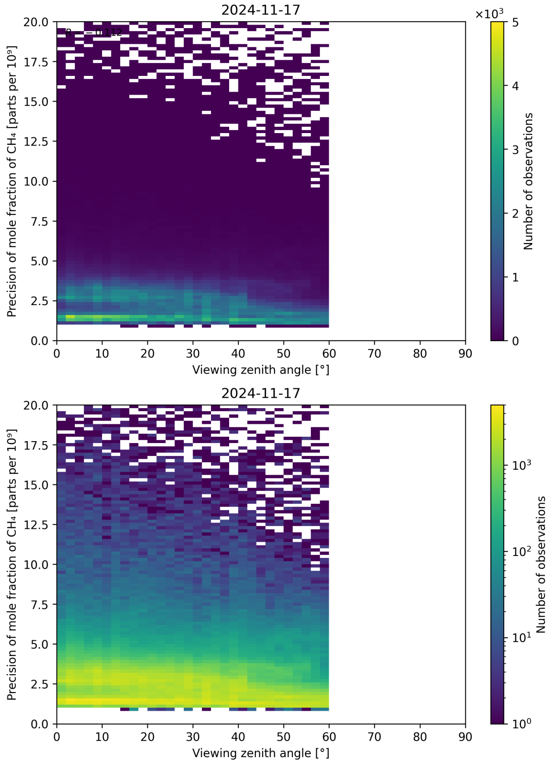
Figure 112: Scatter density plot of “Viewing zenith angle” against “Precision of mole fraction of CH 4 ” for 2024-11-17 to 2024-11-18.
