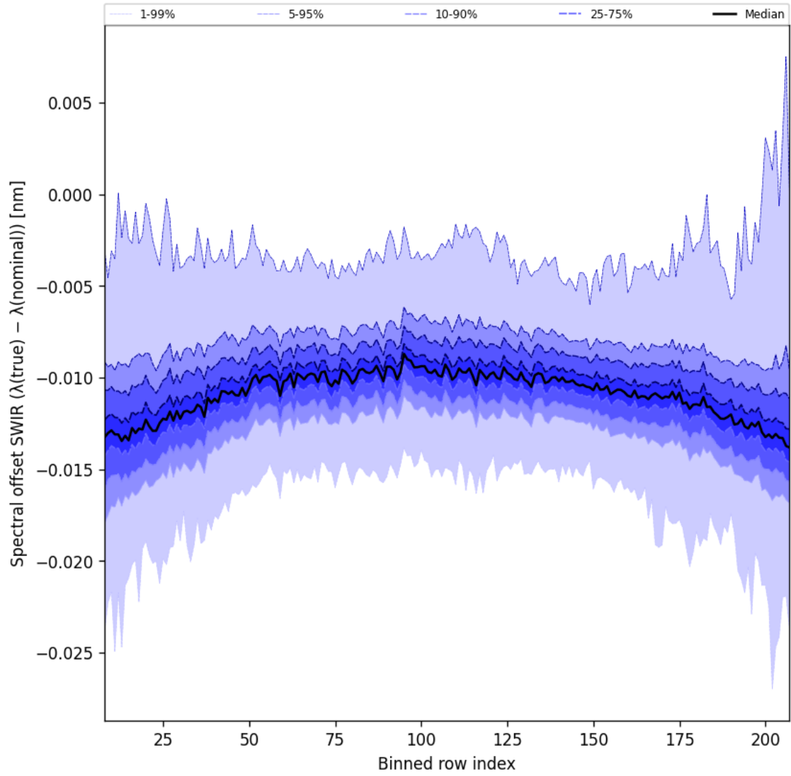
Figure 38: Along track statistics of “Spectral offset SWIR ( \lambda_{\text{true}} - \lambda_{\text{nominal}} )” for 2024-11-17 to 2024-11-18
