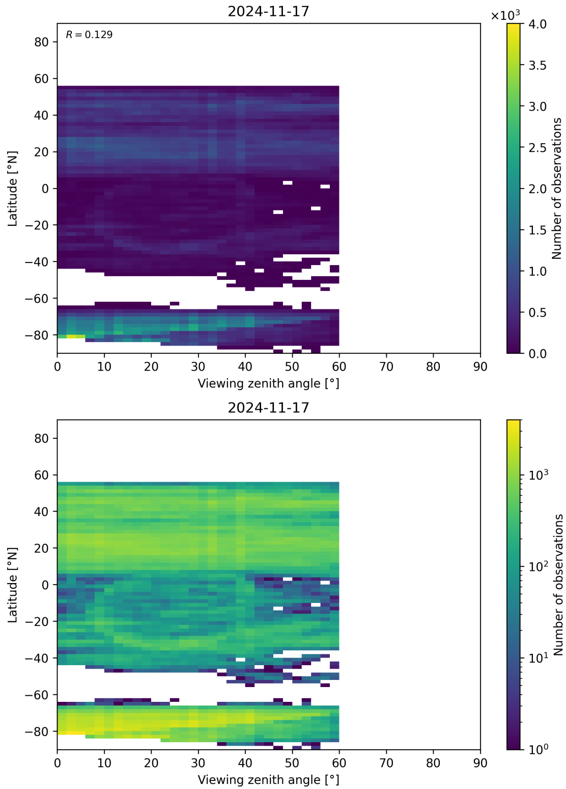
Figure 109: Scatter density plot of “Viewing zenith angle” against “Latitude” for 2024-11-17 to 2024-11-18.
