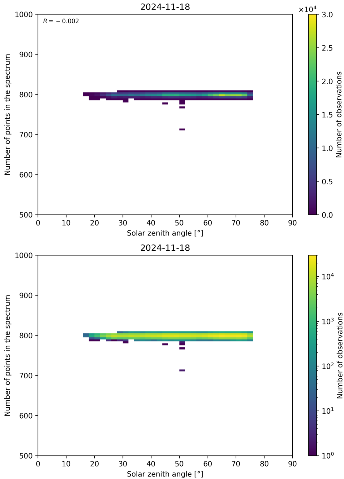
Figure 103: Scatter density plot of “Solar zenith angle” against “Number of points in the spectrum” for 2024-11-17 to 2024-11-19.
