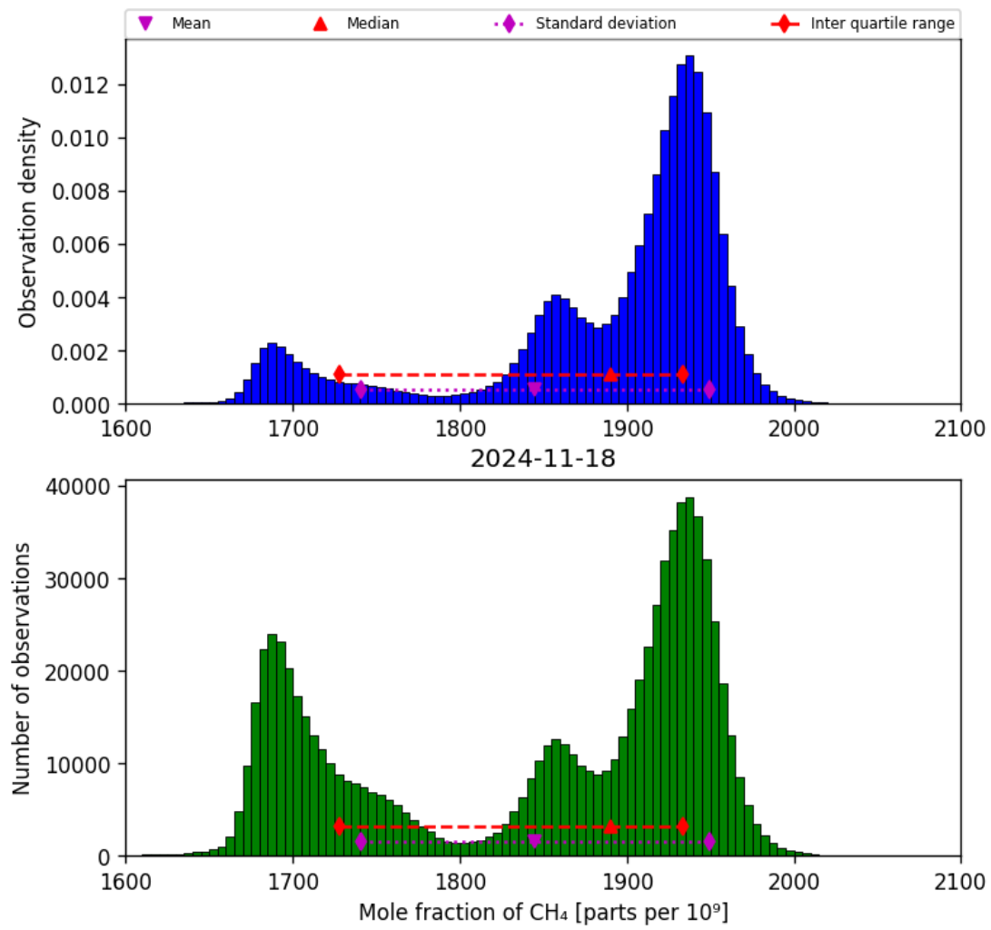
Figure 23: Histogram of “Mole fraction of CH 4 ” for 2024-11-17 to 2024-11-19
