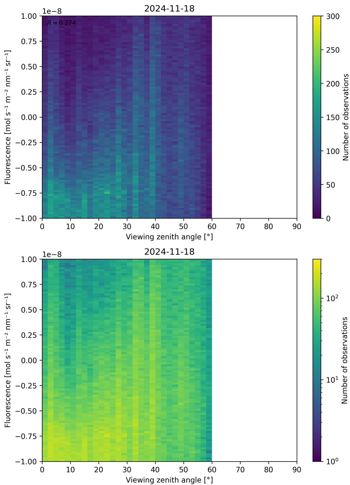
Figure 108: Scatter density plot of “Viewing zenith angle” against “Fluorescence” for 2024-11-17 to 2024-11-19.
