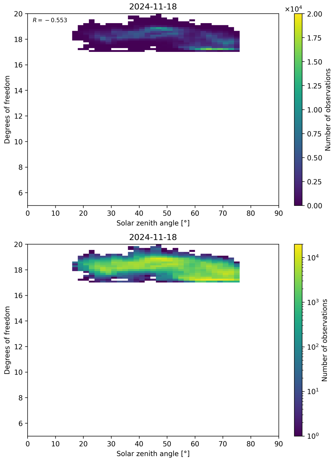
Figure 96: Scatter density plot of “Solar zenith angle” against “Degrees of freedom” for 2024-11-17 to 2024-11-19.
