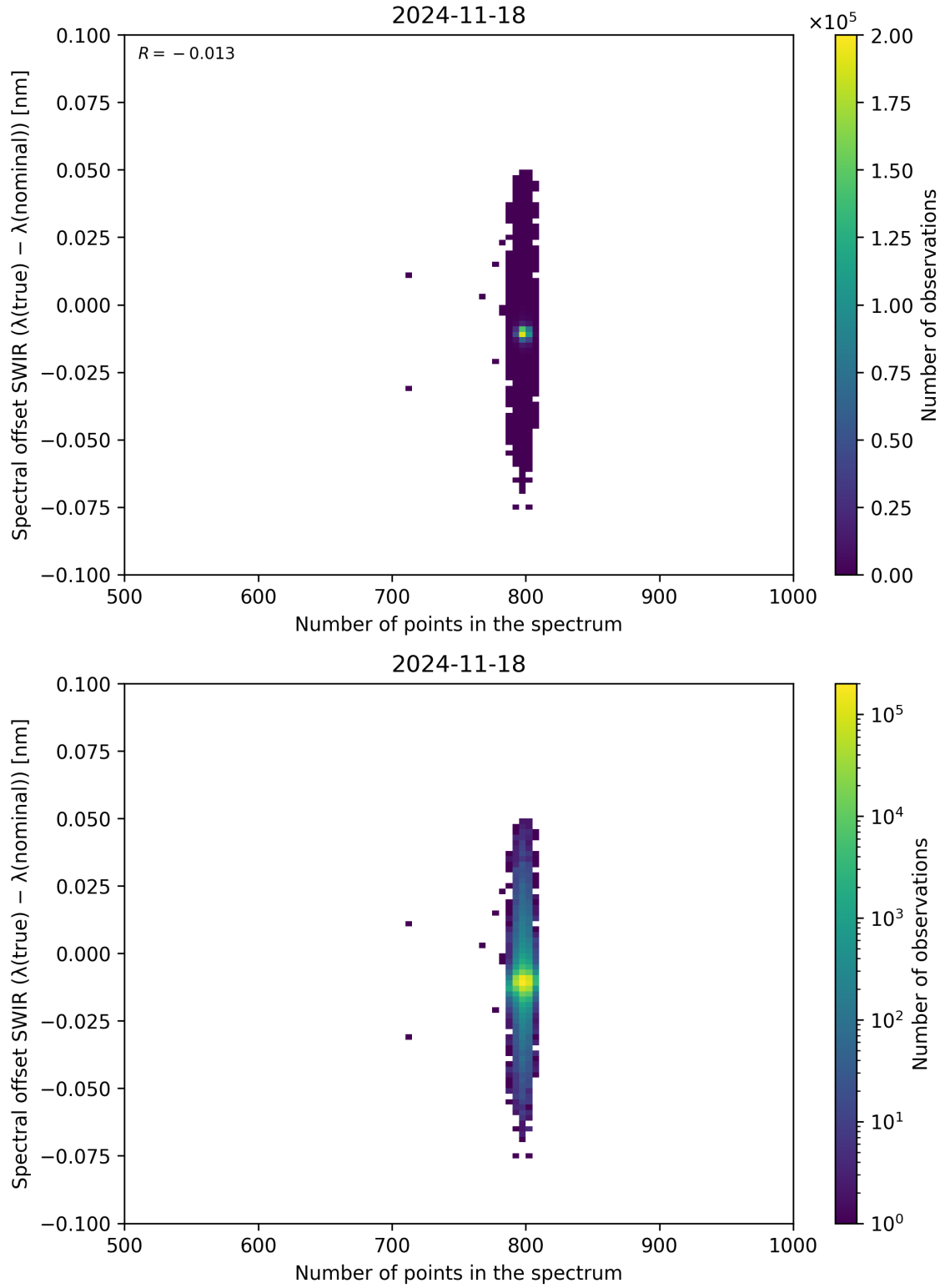
Figure 93: Scatter density plot of “Number of points in the spectrum” against “Spectral offset SWIR ( \lambda_{\text{true}} - \lambda_{\text{nominal}} )” for 2024-11-17 to 2024-11-19.
