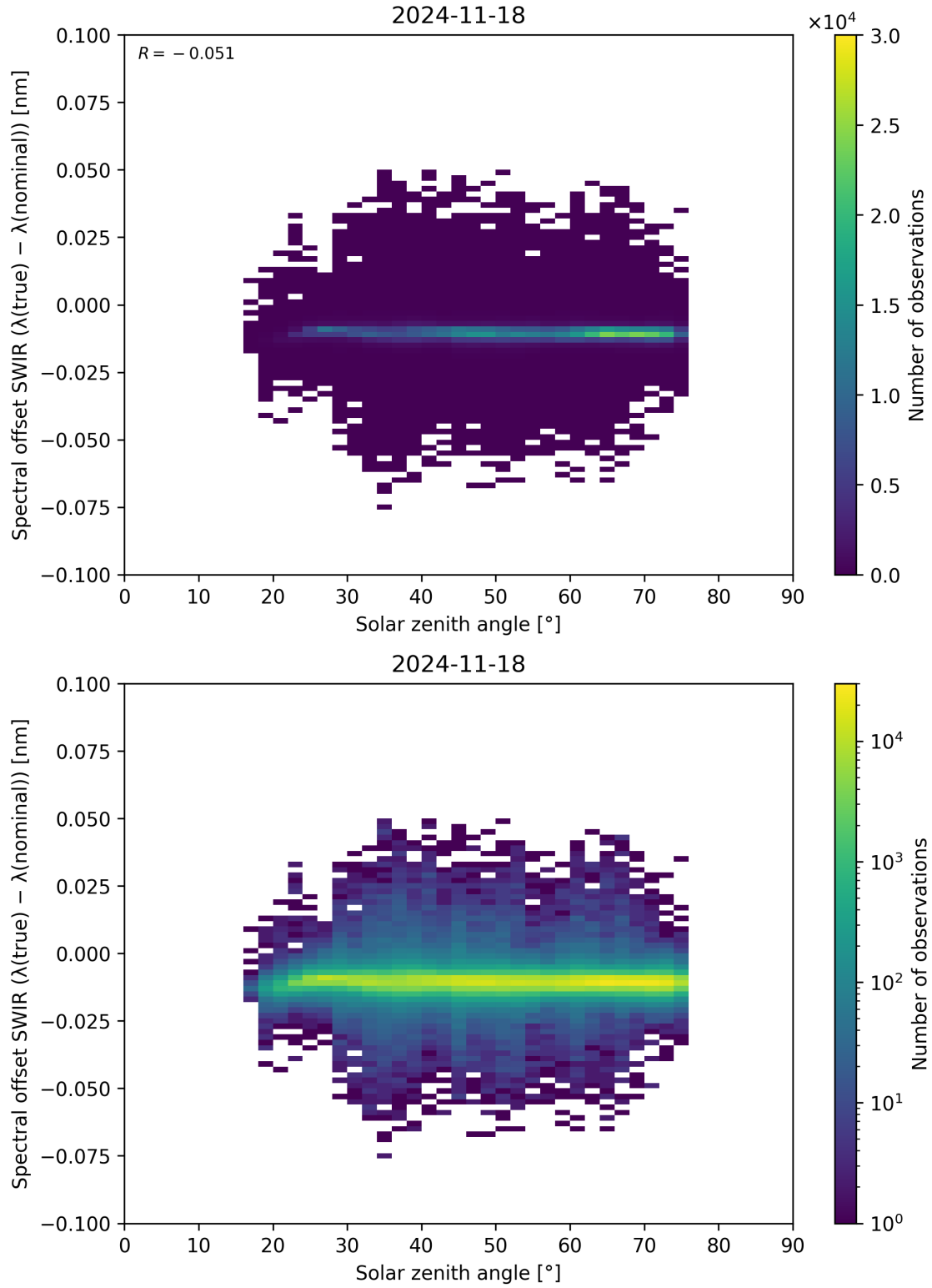
Figure 104: Scatter density plot of “Solar zenith angle” against “Spectral offset SWIR ( \lambda_{\text{true}} - \lambda_{\text{nominal}} )” for 2024-11-17 to 2024-11-19.
