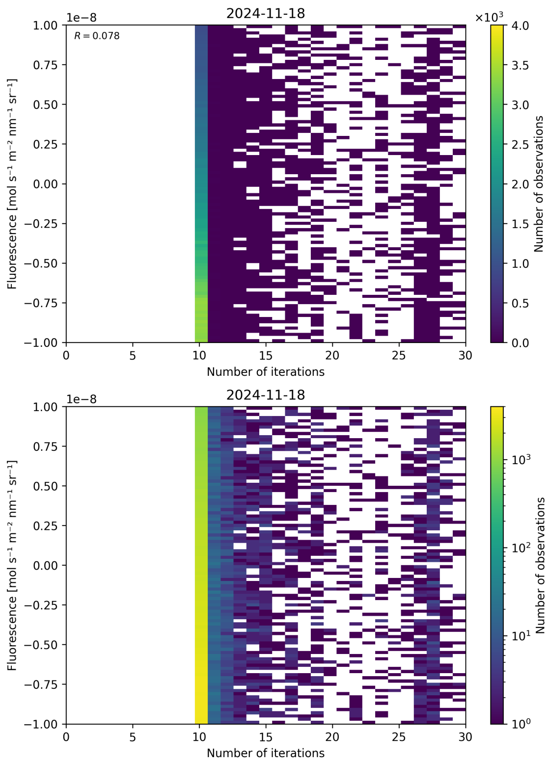
Figure 87: Scatter density plot of “Number of iterations” against “Fluorescence” for 2024-11-17 to 2024-11-19.
