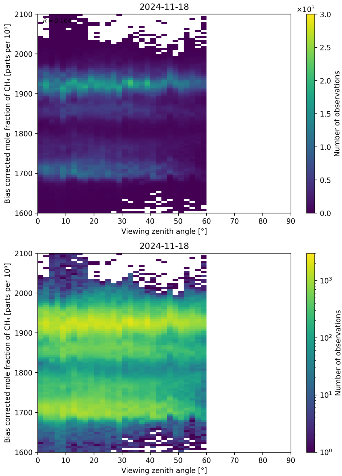
Figure 111: Scatter density plot of “Viewing zenith angle” against “Bias corrected mole fraction of CH 4 ” for 2024-11-17 to 2024-11-19.
