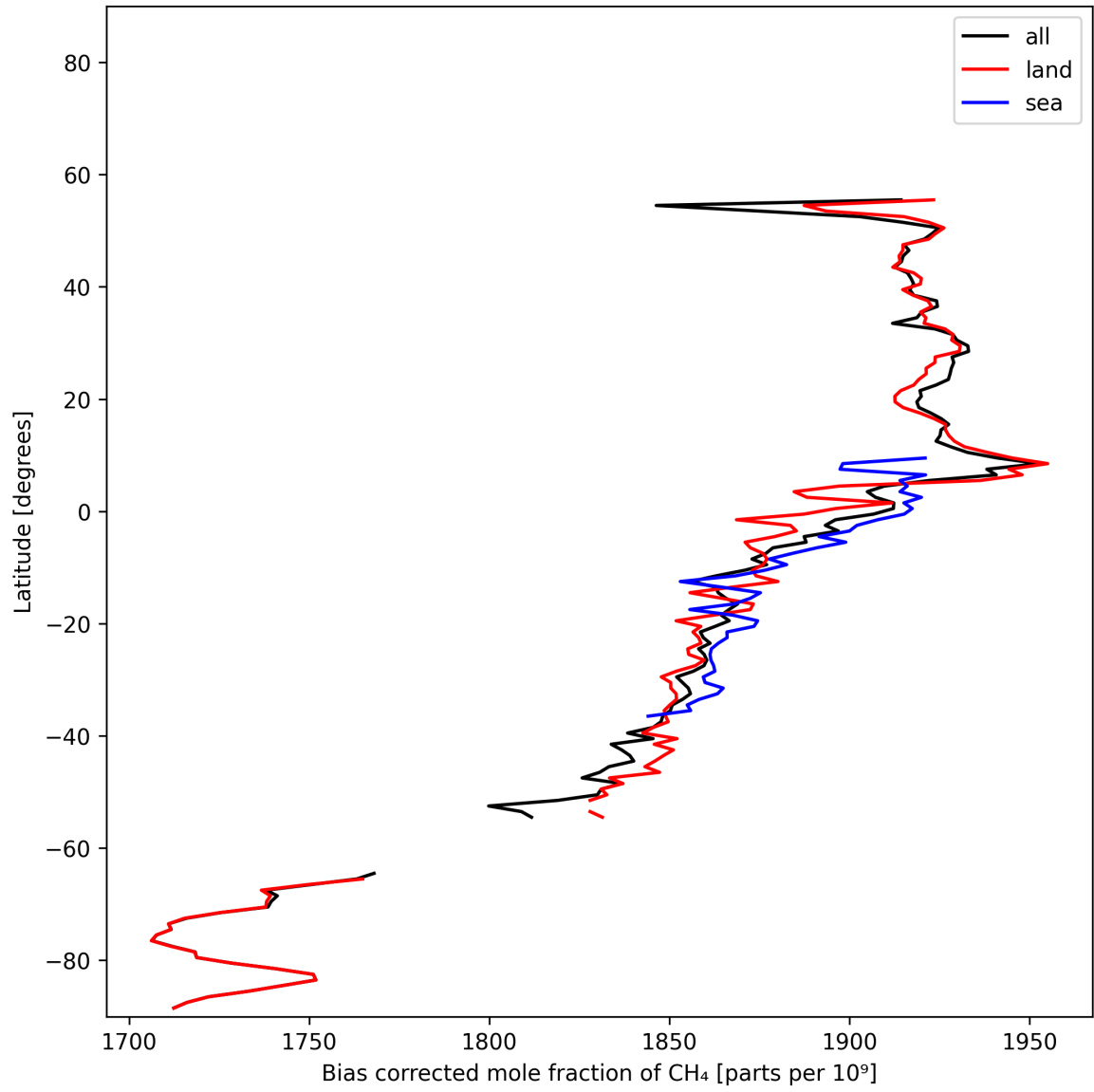
Figure 14: Zonal average of “Bias corrected mole fraction of CH 4 ” for 2024-11-17 to 2024-11-19.
