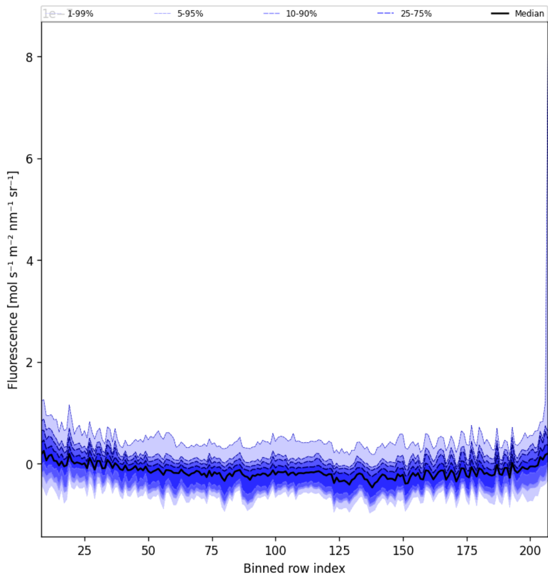
Figure 43: Along track statistics of “Fluorescence” for 2024-11-17 to 2024-11-19
