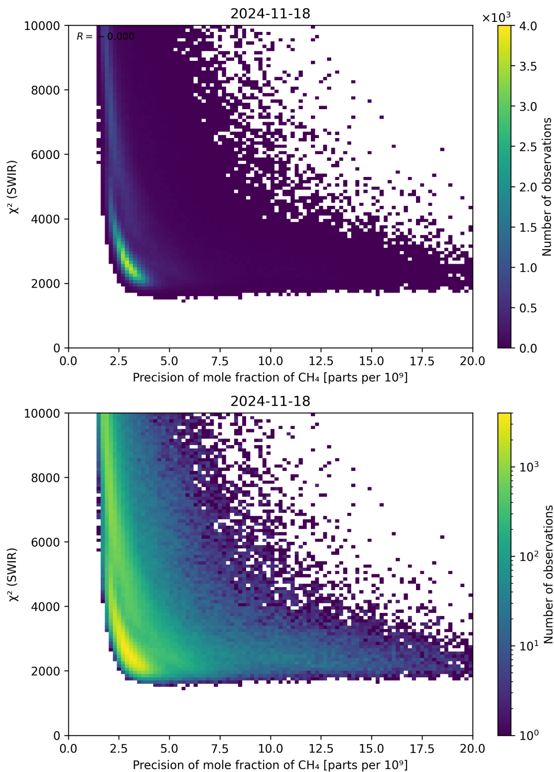
Figure 79: Scatter density plot of “Precision of mole fraction of \text{CH}_4 ” against “ \chi^2 (SWIR)” for 2024-11-17 to 2024-11-19.
