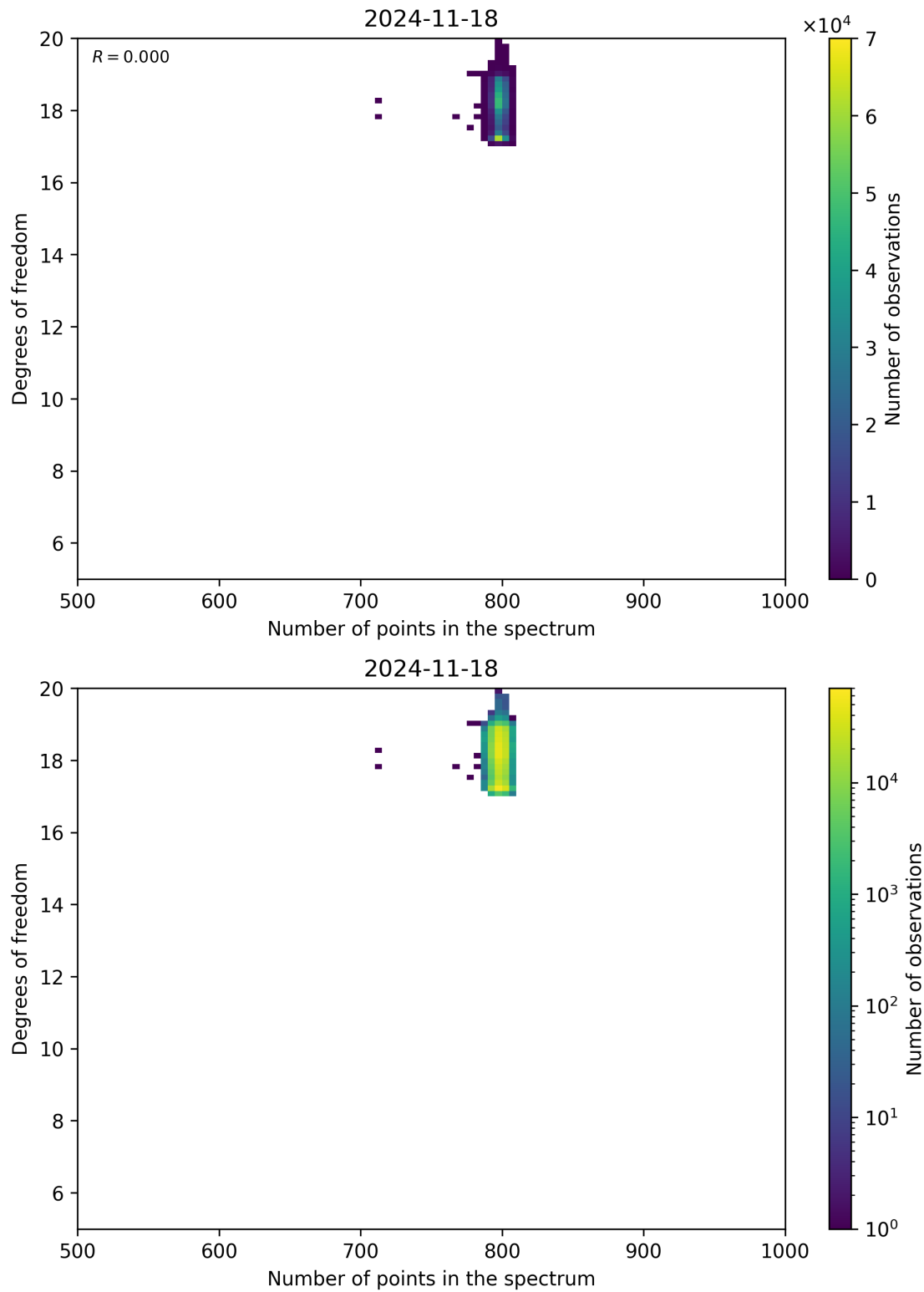
Figure 90: Scatter density plot of “Number of points in the spectrum” against “Degrees of freedom” for 2024-11-17 to 2024-11-19.
