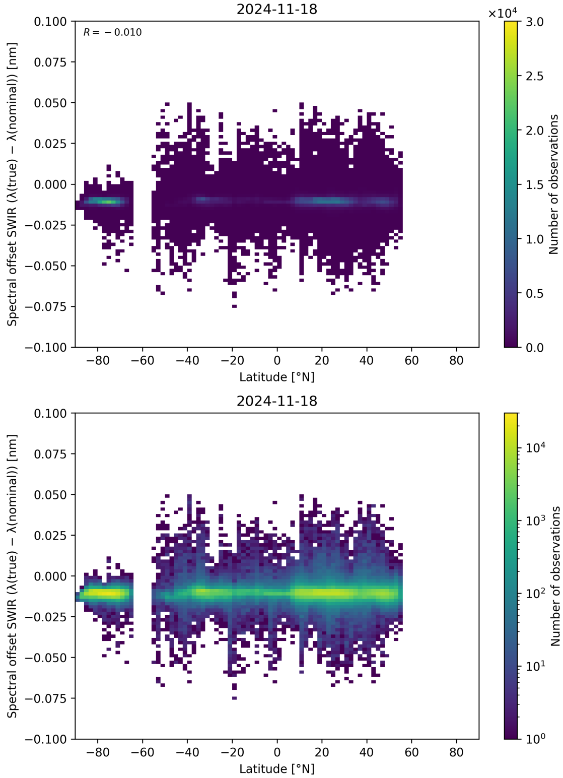
Figure 62: Scatter density plot of “Latitude” against “Spectral offset SWIR ( \lambda_{\text{true}} - \lambda_{\text{nominal}} )” for 2024-11-17 to 2024-11-19.
