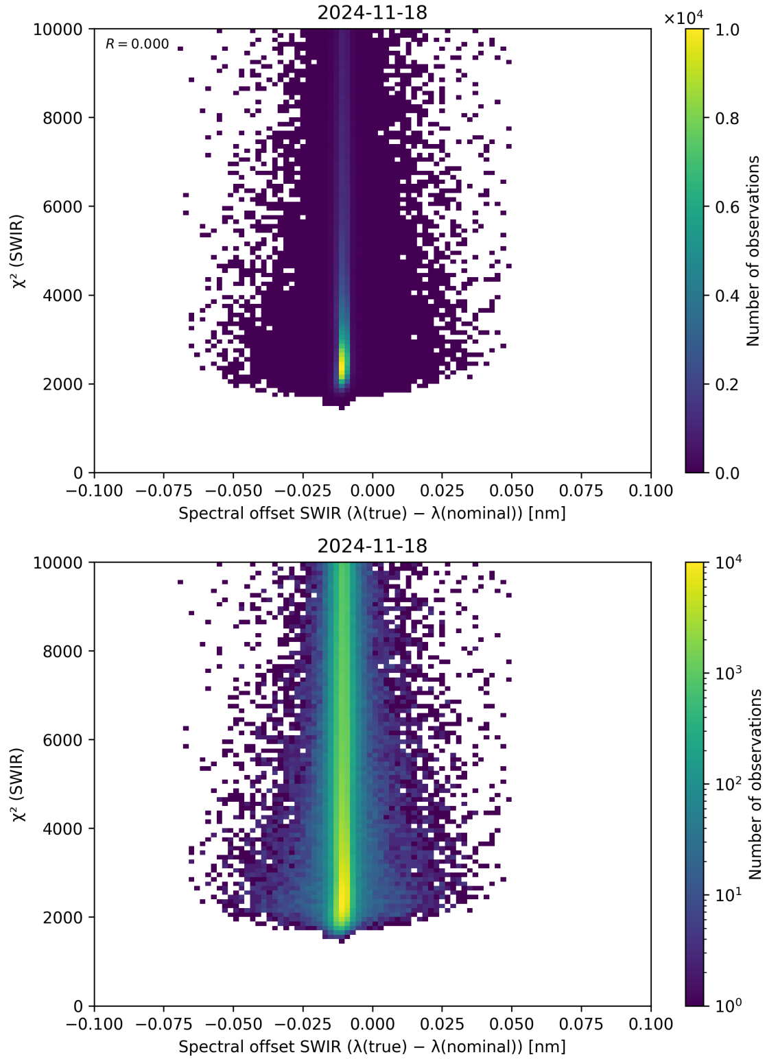
Figure 118: Scatter density plot of “Spectral offset SWIR ( \lambda_{\text{true}} - \lambda_{\text{nominal}} )” against “ \chi^2 (SWIR)” for 2024-11-17 to 2024-11-19.
