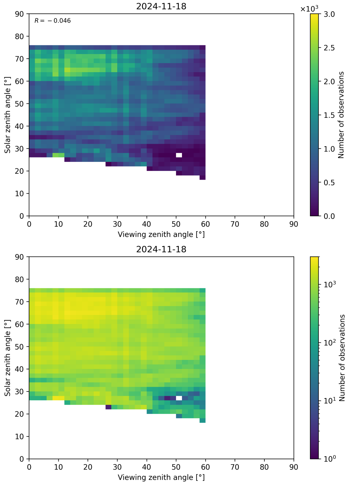
Figure 115: Scatter density plot of “Viewing zenith angle” against “Solar zenith angle” for 2024-11-17 to 2024-11-19.
