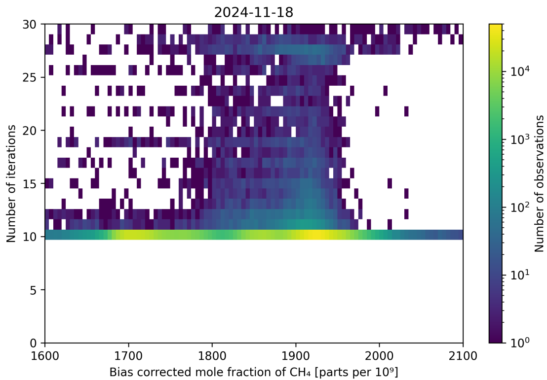
Figure 67: Scatter density plot of “Bias corrected mole fraction of CH 4 ” against “Number of iterations” for 2024-11-17 to 2024-11-19.
