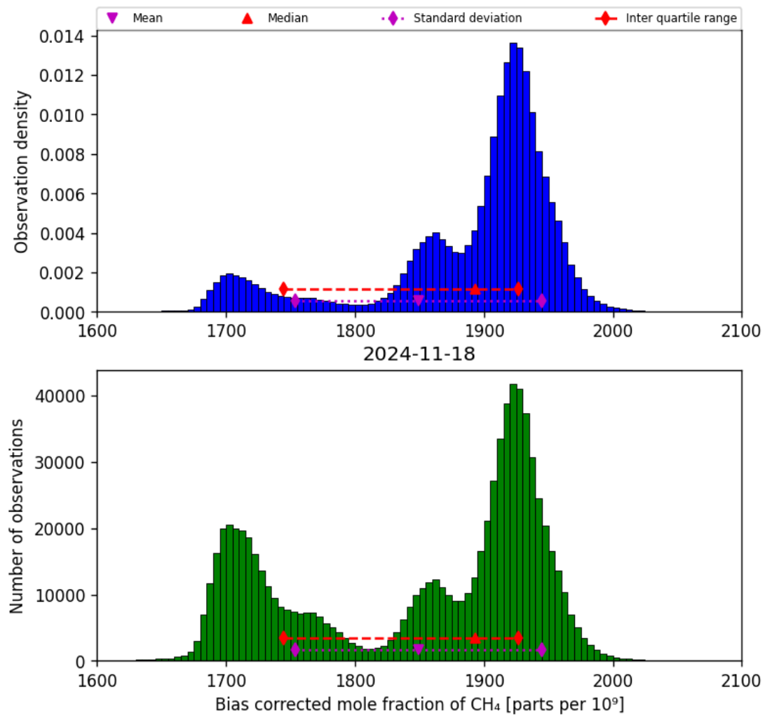
Figure 25: Histogram of “Bias corrected mole fraction of CH 4 ” for 2024-11-17 to 2024-11-19
