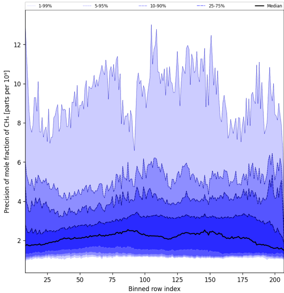
Figure 35: Along track statistics of “Precision of mole fraction of CH 4 ” for 2024-11-17 to 2024-11-19
