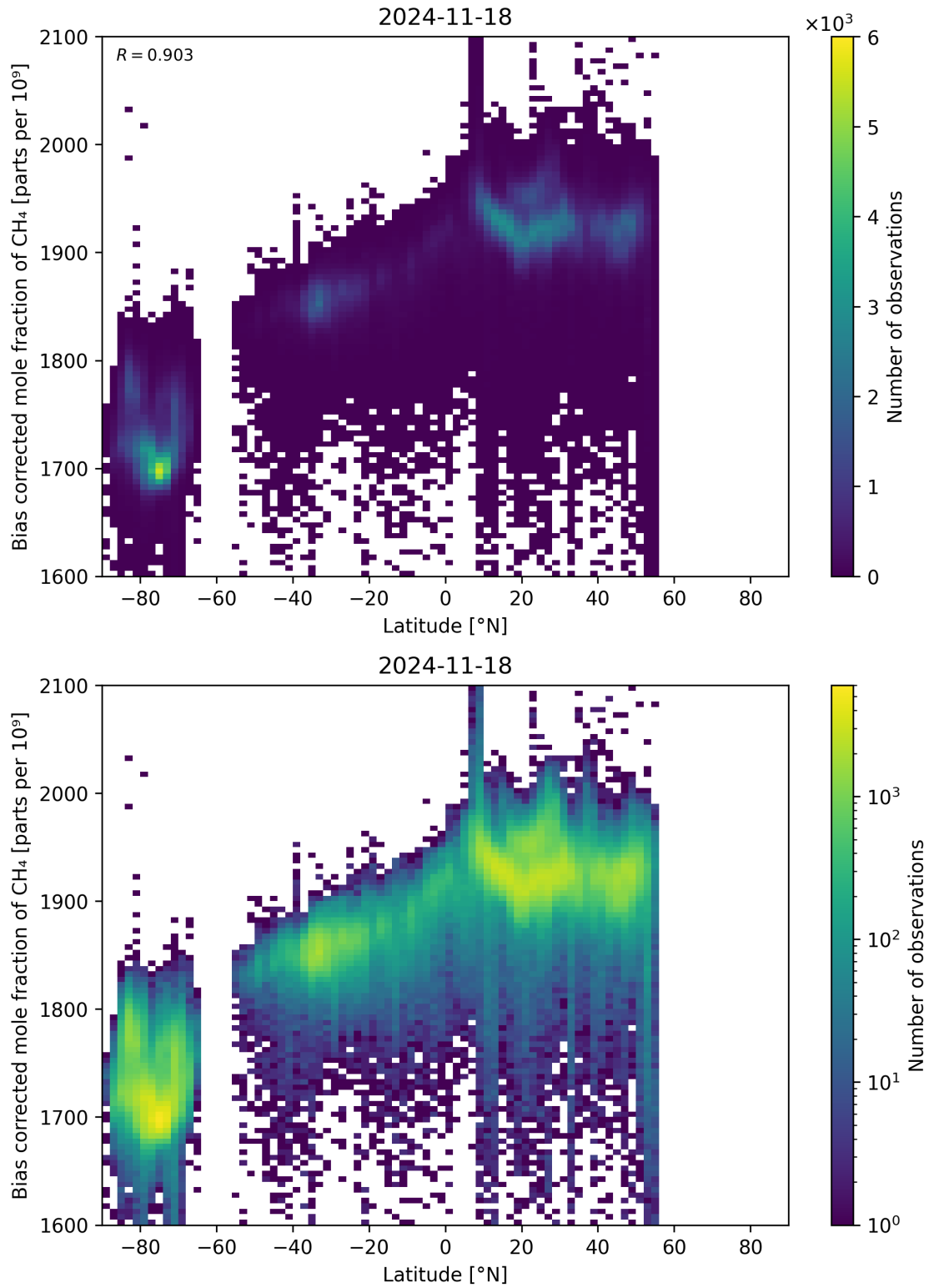
Figure 58: Scatter density plot of “Latitude” against “Bias corrected mole fraction of CH 4 ” for 2024-11-17 to 2024-11-19.
