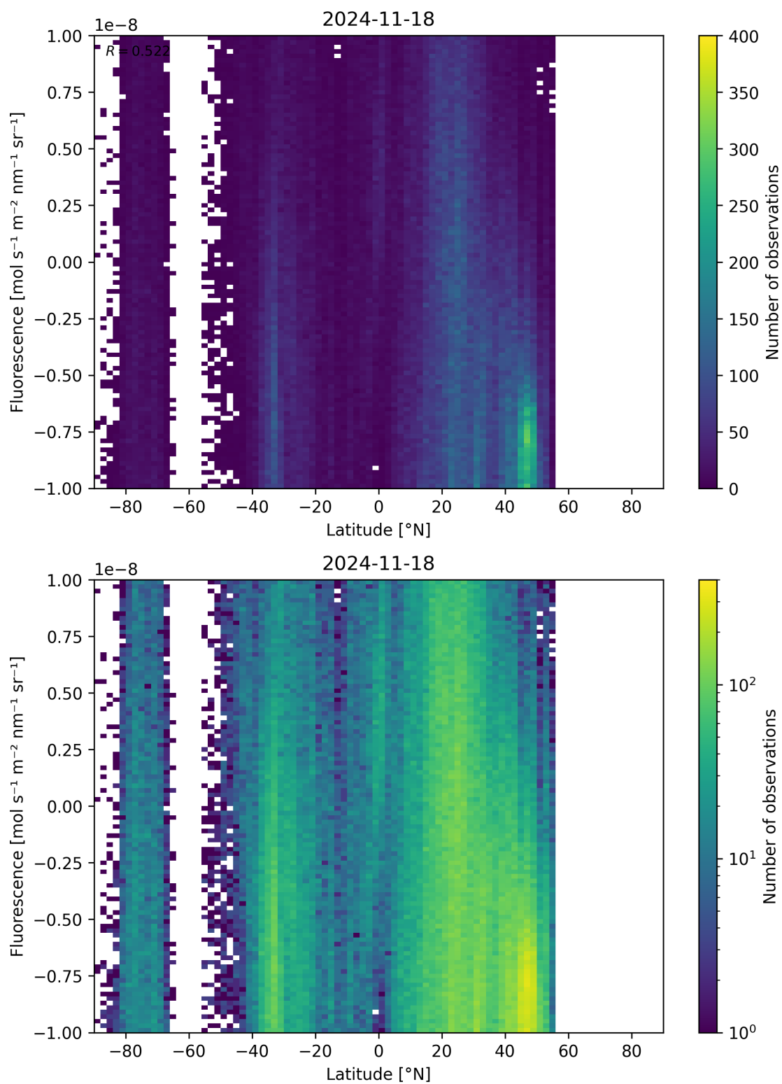
Figure 56: Scatter density plot of “Latitude” against “Fluorescence” for 2024-11-17 to 2024-11-19.
