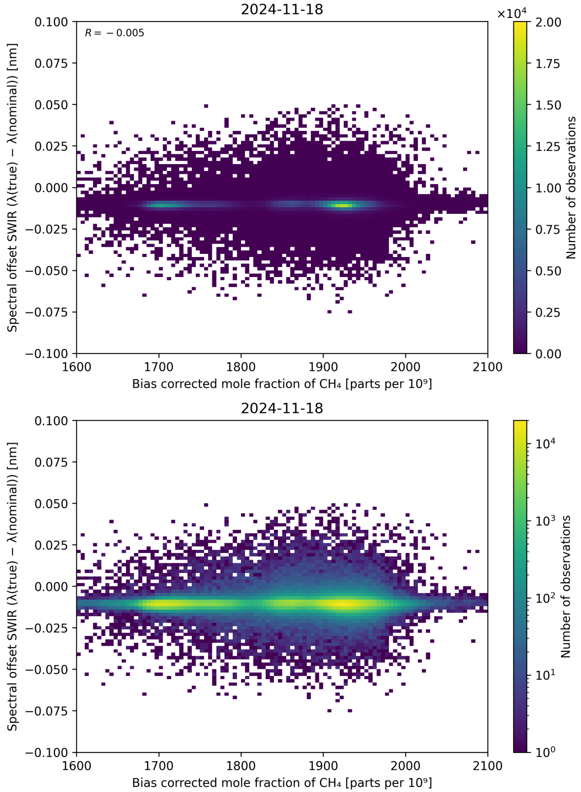
Figure 69: Scatter density plot of “Bias corrected mole fraction of \text{CH}_4 ” against “Spectral offset SWIR ( \lambda_{\text{true}} - \lambda_{\text{nominal}} )” for 2024-11-17 to 2024-11-19.
