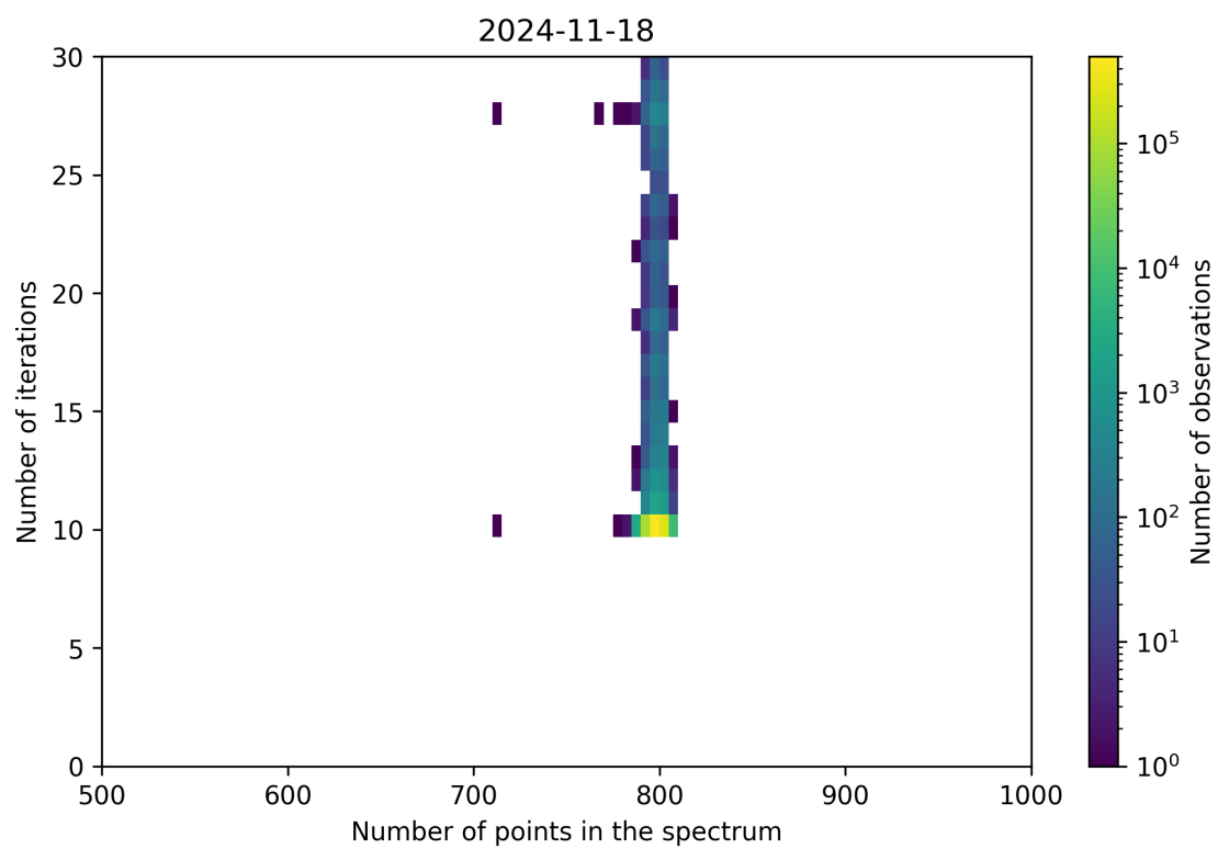
Figure 92: Scatter density plot of “Number of points in the spectrum” against “Number of iterations” for 2024-11-17 to 2024-11-19.
