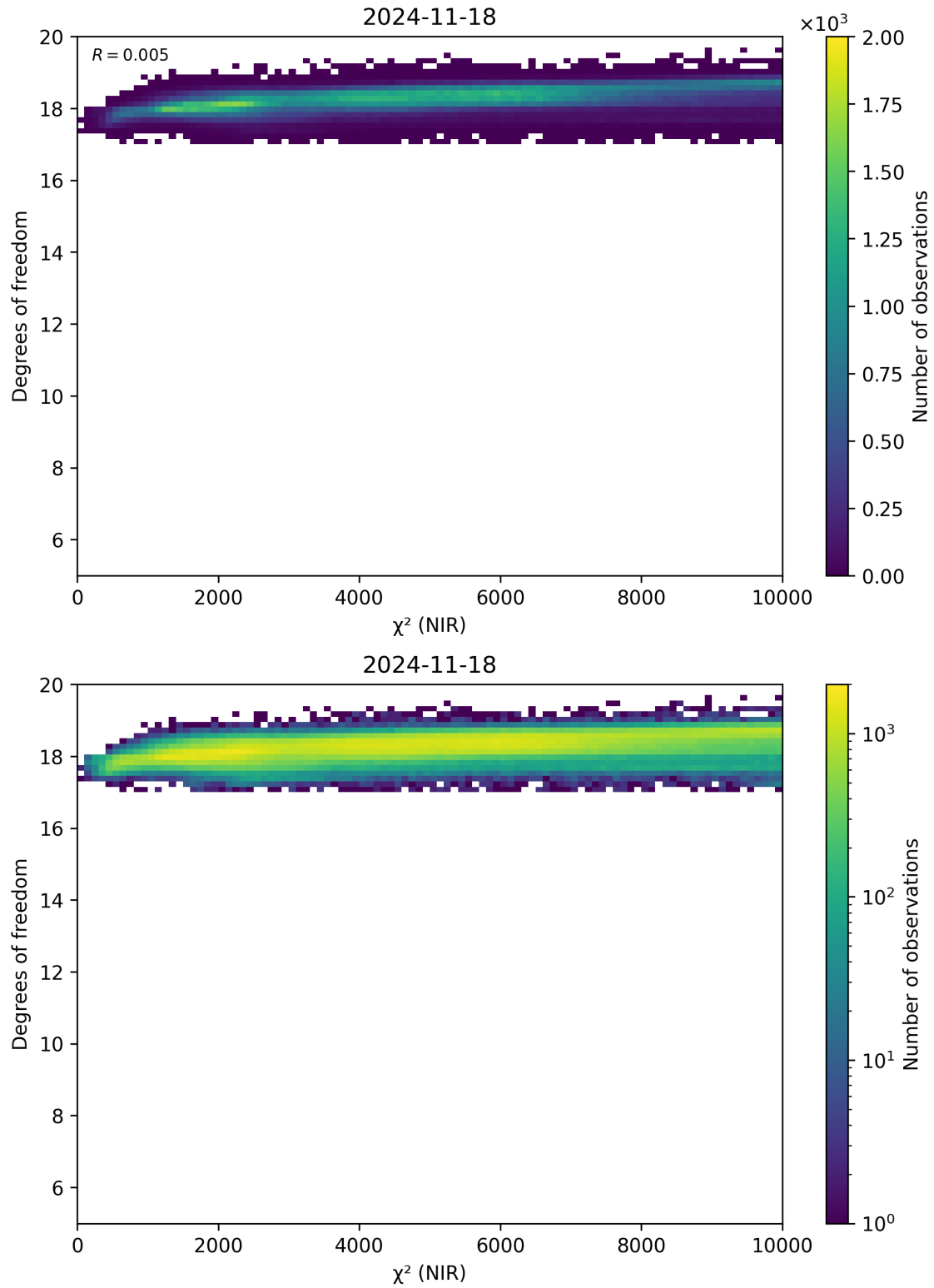
Figure 44: Scatter density plot of “ \chi^2 (NIR)” against “Degrees of freedom” for 2024-11-17 to 2024-11-19.
