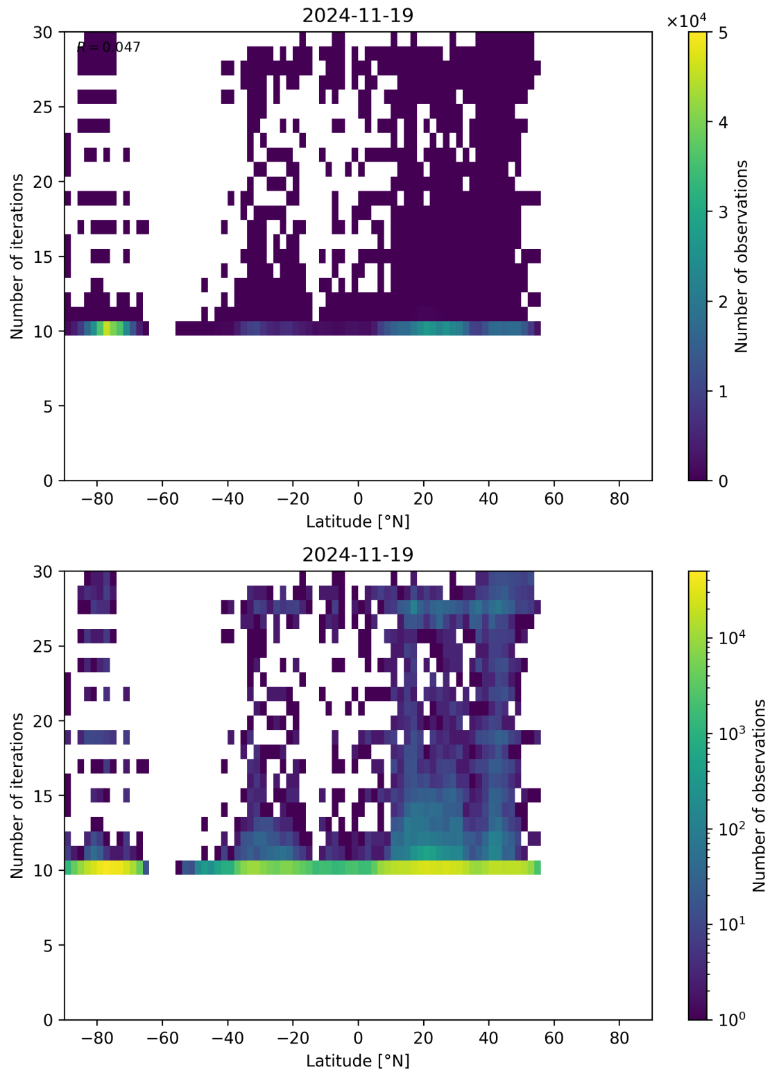
Figure 60: Scatter density plot of “Latitude” against “Number of iterations” for 2024-11-18 to 2024-11-20.
