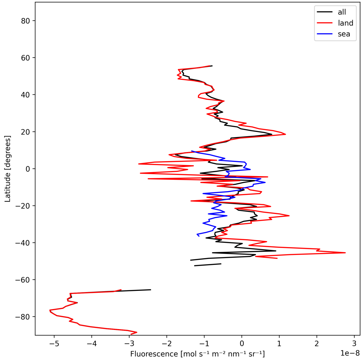
Figure 21: Zonal average of “Fluorescence” for 2024-11-18 to 2024-11-20.
