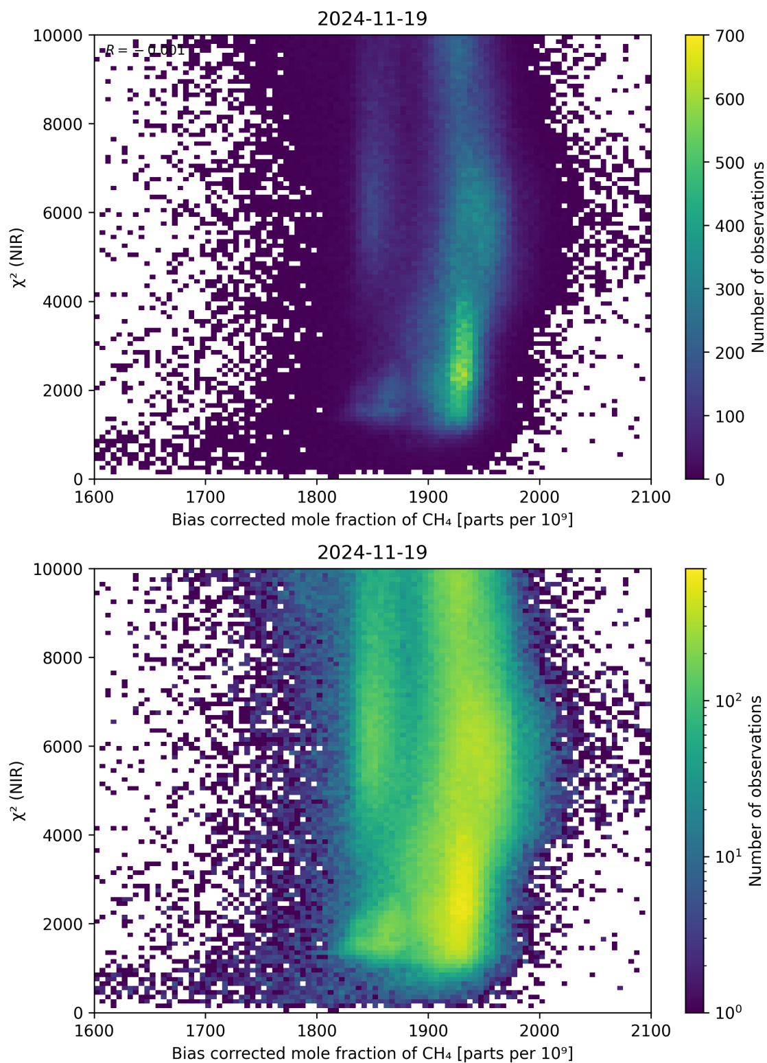
Figure 63: Scatter density plot of “Bias corrected mole fraction of CH 4 ” against “ \chi^2 (NIR)” for 2024-11-18 to 2024-11-20.
