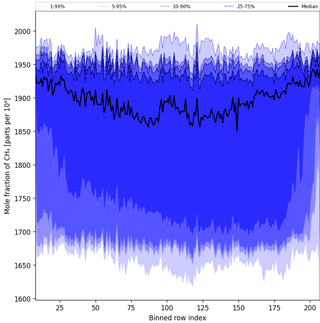
Figure 34: Along track statistics of “Mole fraction of CH 4 ” for 2024-11-18 to 2024-11-20
