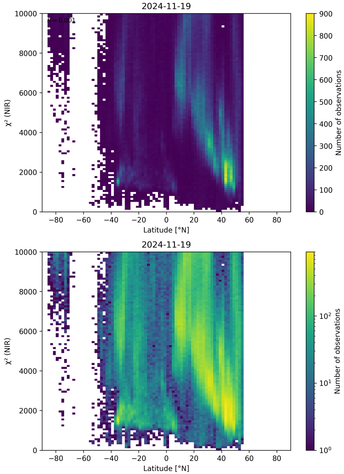
Figure 53: Scatter density plot of “Latitude” against “ \chi^2 (NIR)” for 2024-11-18 to 2024-11-20.
