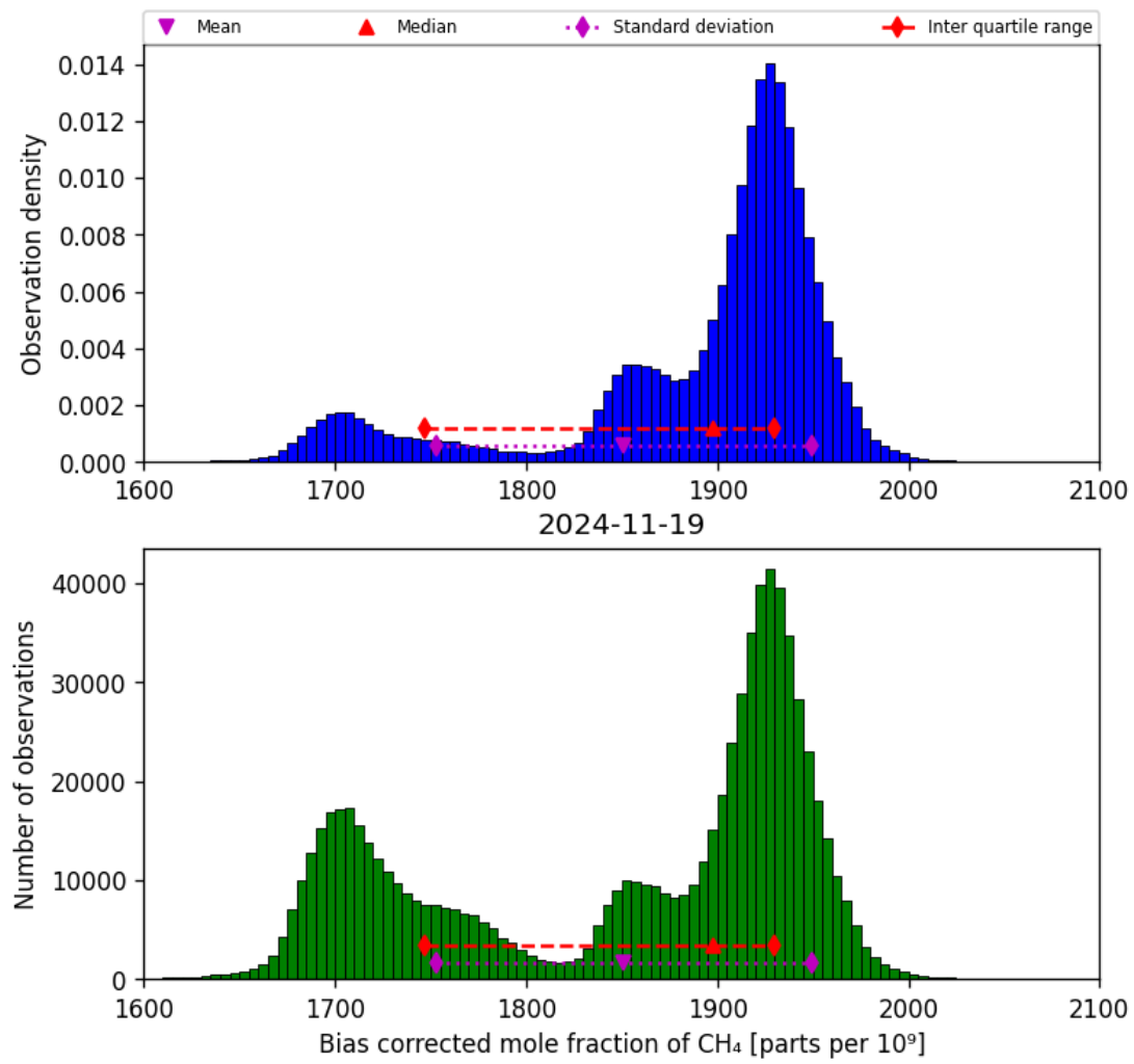
Figure 25: Histogram of “Bias corrected mole fraction of CH 4 ” for 2024-11-18 to 2024-11-20
