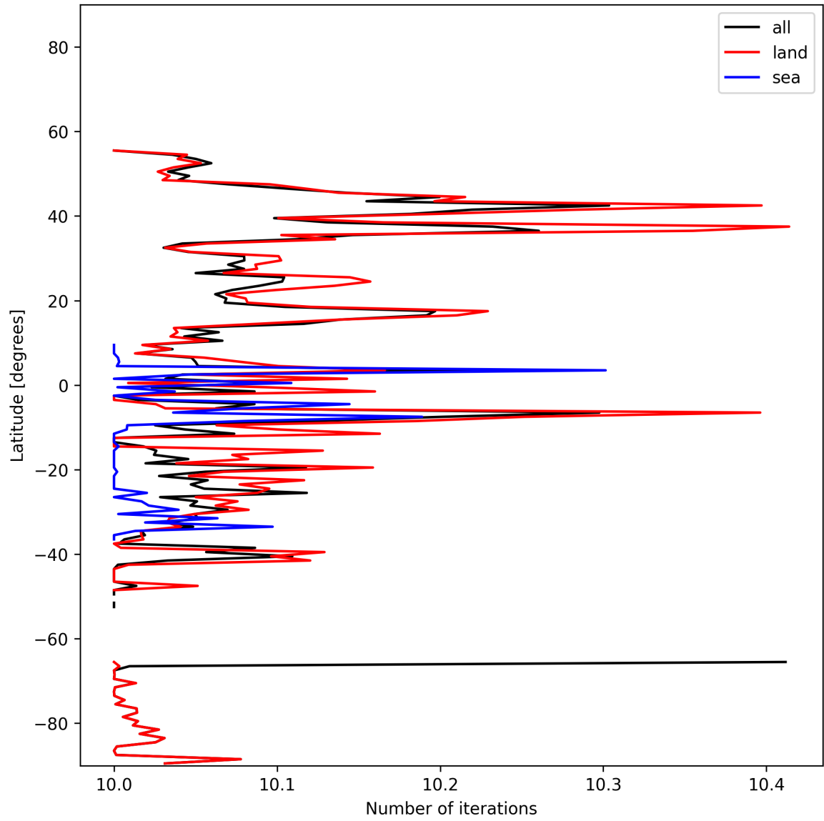
Figure 20: Zonal average of “Number of iterations” for 2024-11-18 to 2024-11-20.
