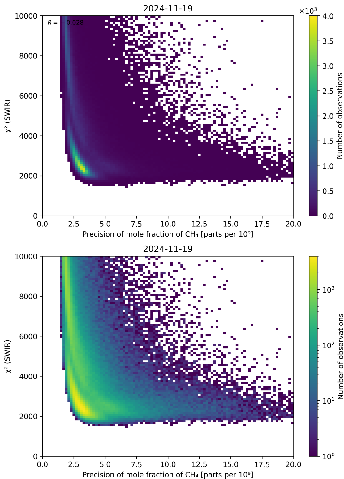
Figure 79: Scatter density plot of “Precision of mole fraction of \text{CH}_4 ” against “ \chi^2 (SWIR)” for 2024-11-18 to 2024-11-20.
