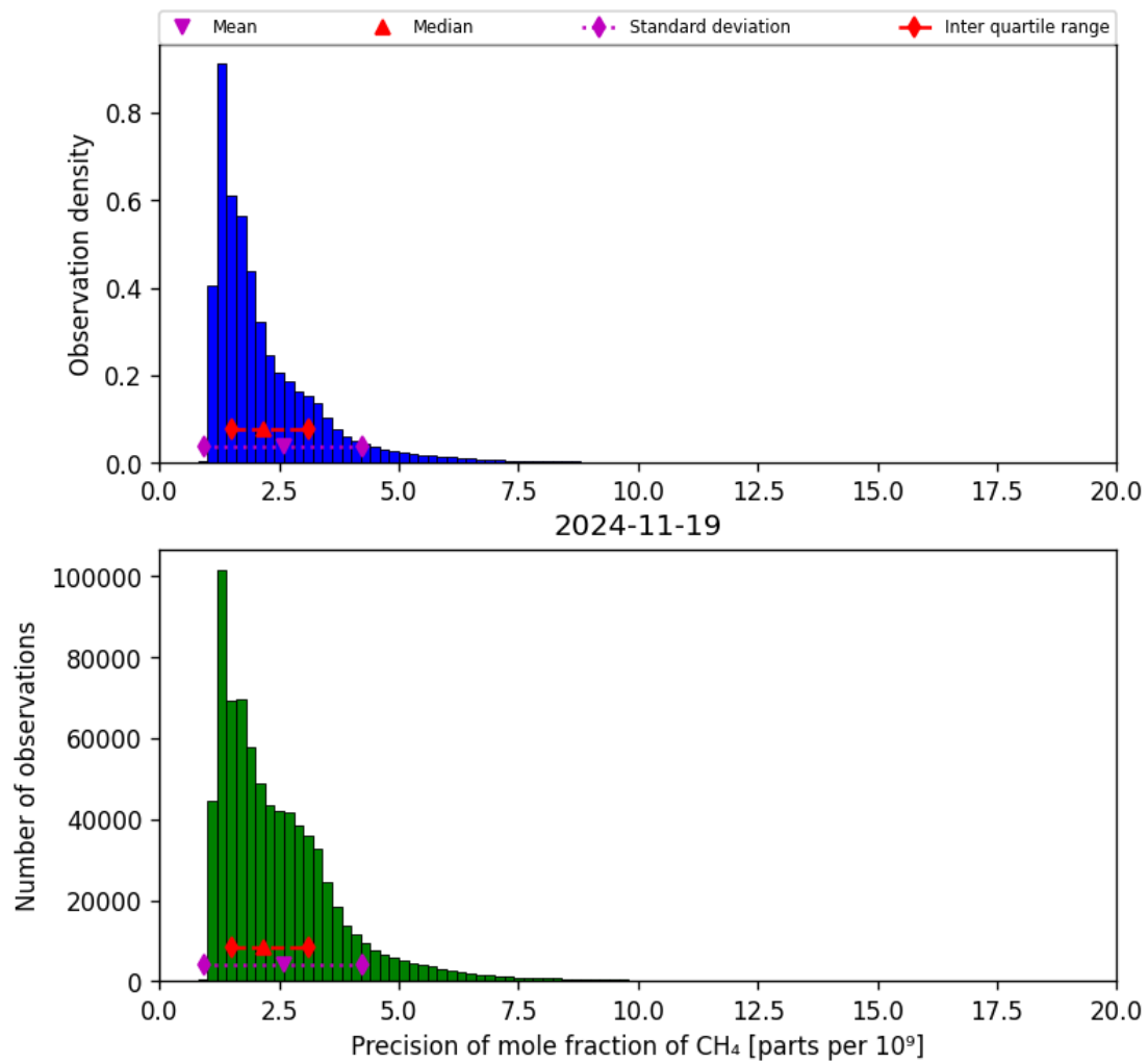
Figure 24: Histogram of “Precision of mole fraction of CH 4 ” for 2024-11-18 to 2024-11-20
