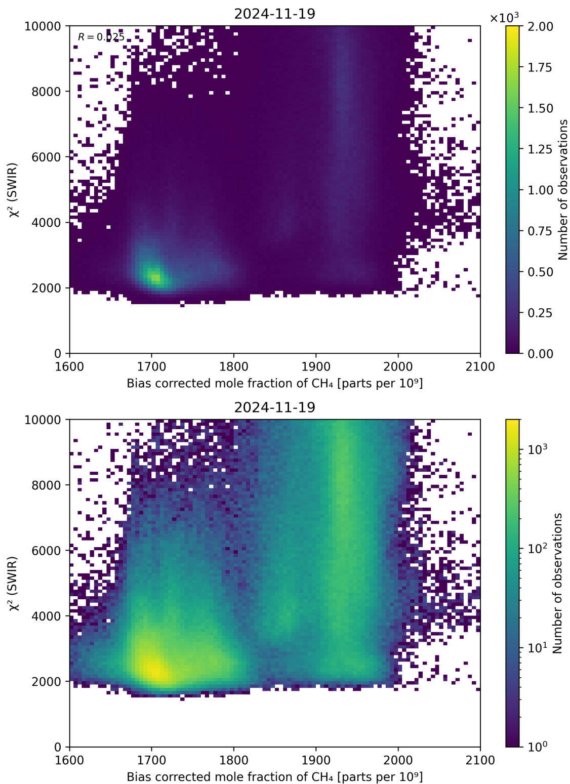
Figure 64: Scatter density plot of “Bias corrected mole fraction of \text{CH}_4 ” against “ \chi^2 (SWIR)” for 2024-11-18 to 2024-11-20.
