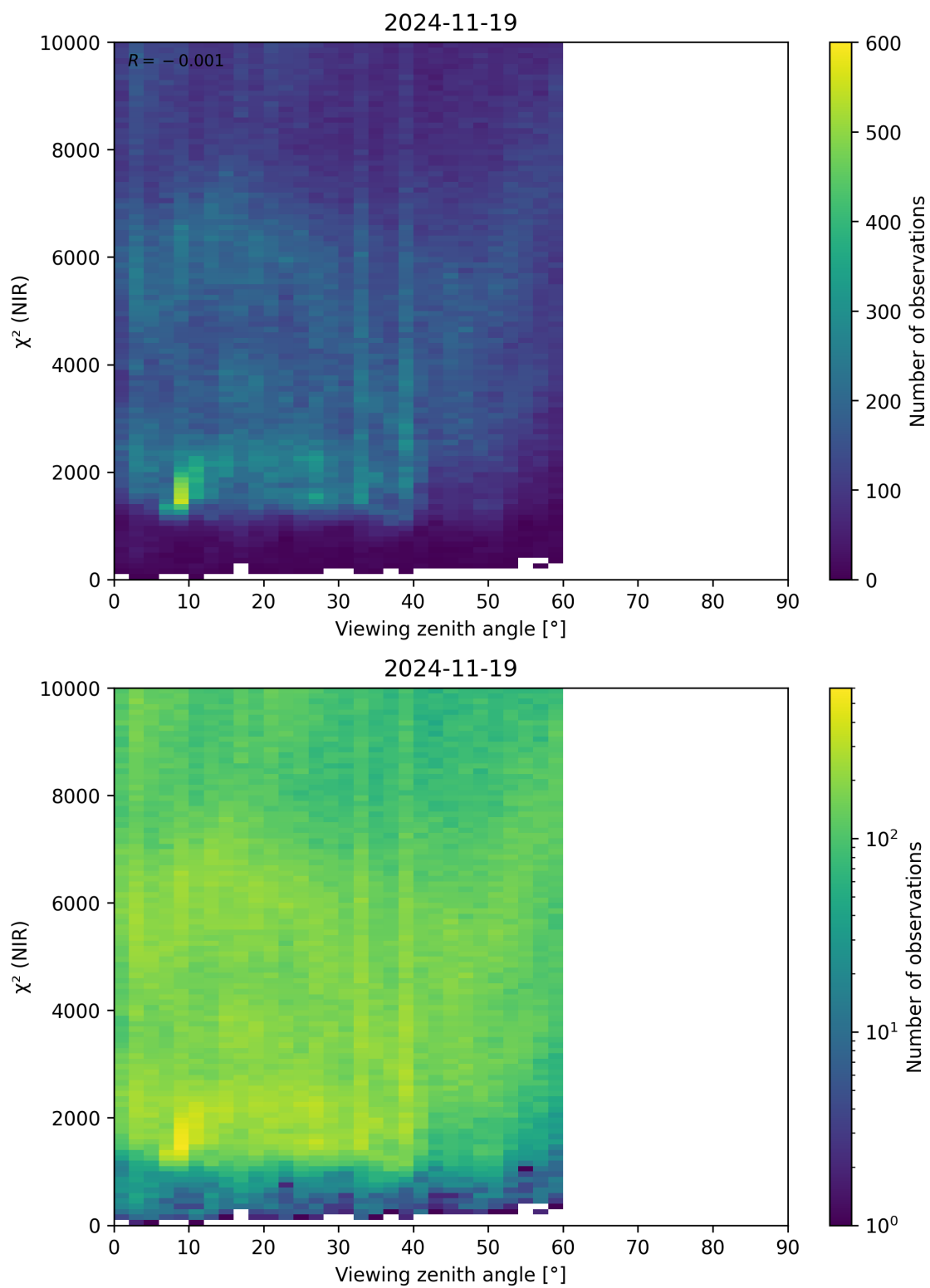
Figure 105: Scatter density plot of “Viewing zenith angle” against “ \chi^2 (NIR)” for 2024-11-18 to 2024-11-20.
