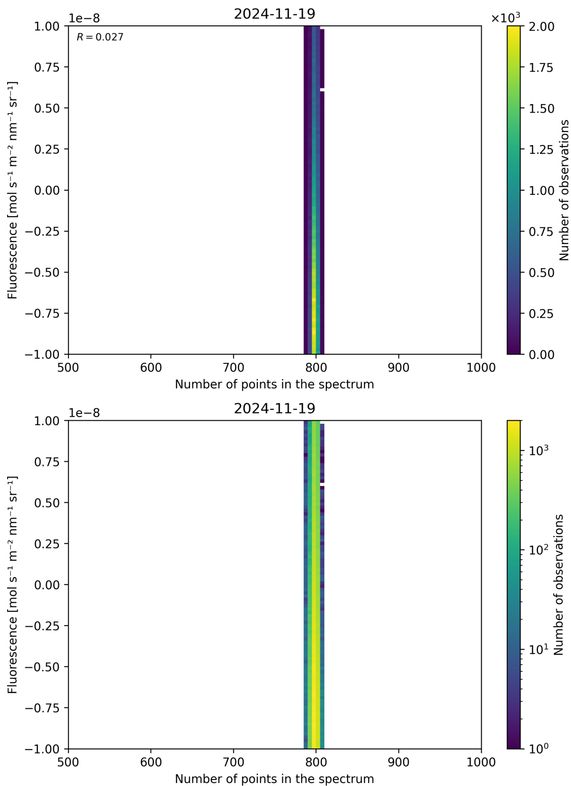
Figure 91: Scatter density plot of “Number of points in the spectrum” against “Fluorescence” for 2024-11-18 to 2024-11-20.
