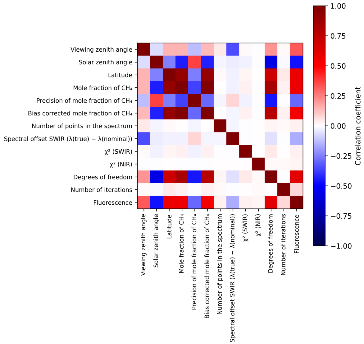
Figure 2: Map of correlation matrix for 2024-11-18 to 2024-11-20.
