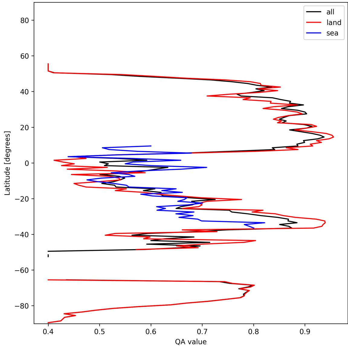
Figure 11: Zonal average of “QA value” for 2024-11-18 to 2024-11-20.
