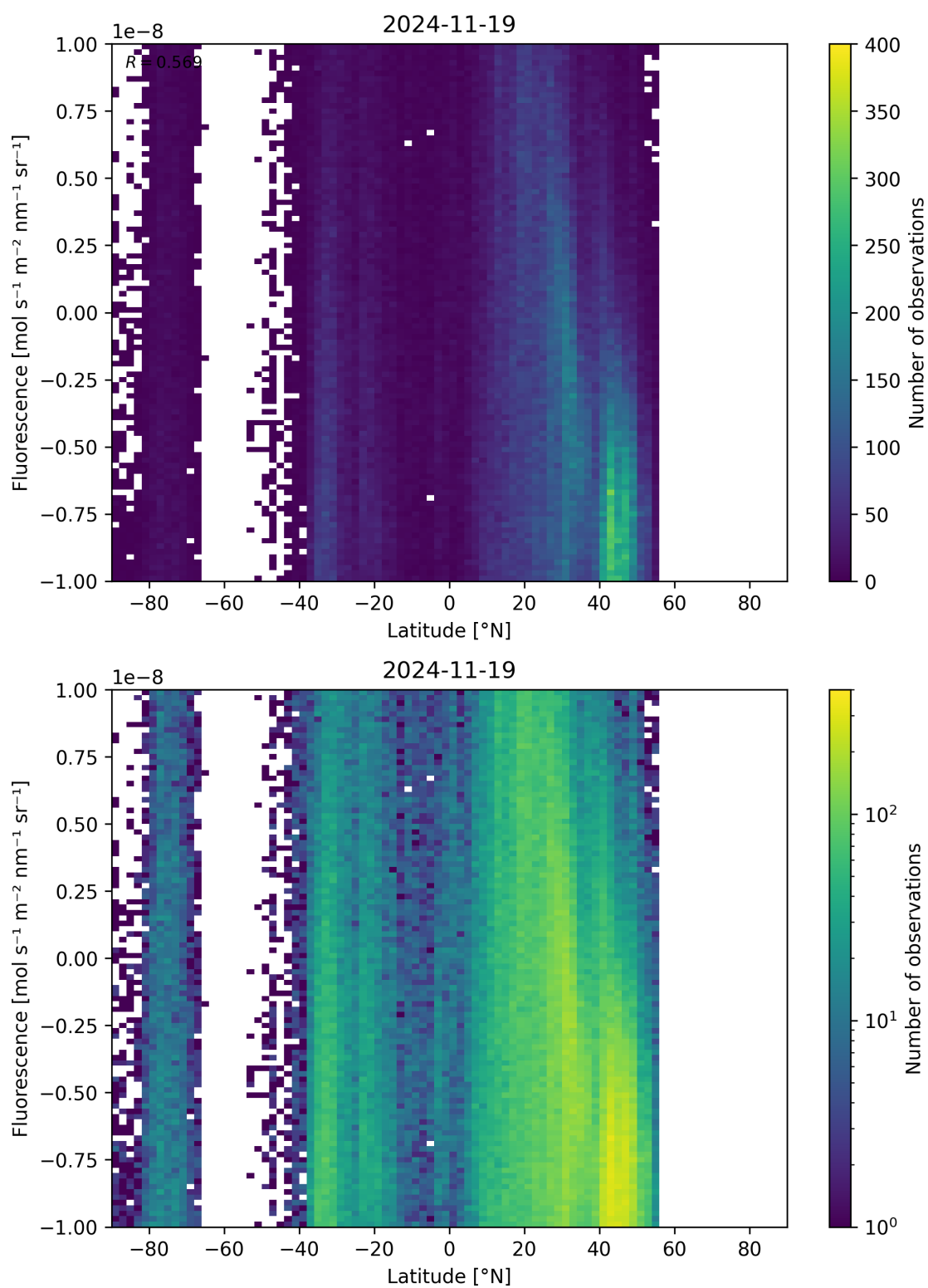
Figure 56: Scatter density plot of “Latitude” against “Fluorescence” for 2024-11-18 to 2024-11-20.
