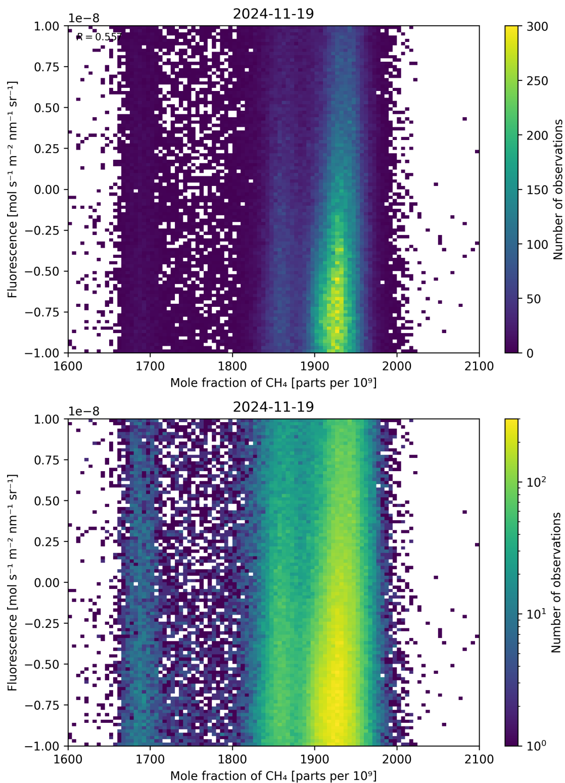
Figure 73: Scatter density plot of “Mole fraction of \text{CH}_4 ” against “Fluorescence” for 2024-11-18 to 2024-11-20.
