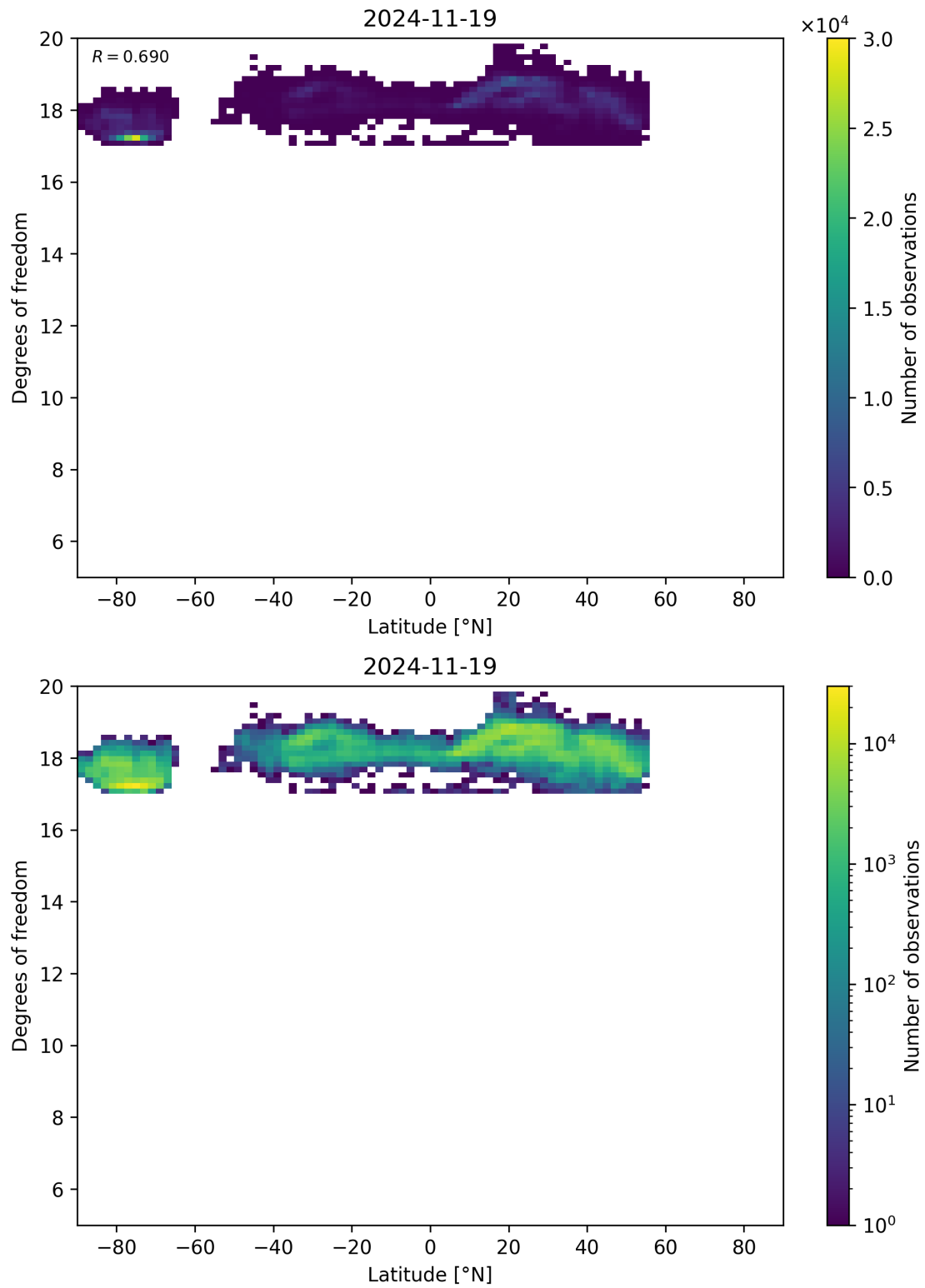
Figure 55: Scatter density plot of “Latitude” against “Degrees of freedom” for 2024-11-18 to 2024-11-20.
