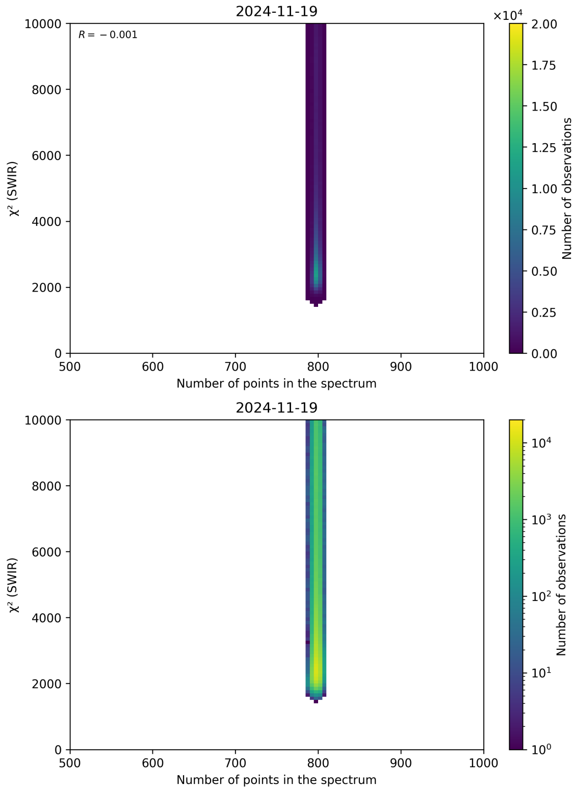
Figure 89: Scatter density plot of “Number of points in the spectrum” against “ \chi^2 (SWIR)” for 2024-11-18 to 2024-11-20.
