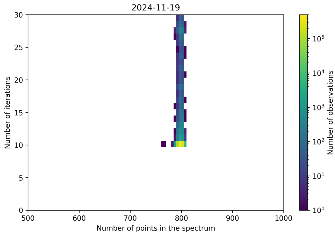
Figure 92: Scatter density plot of “Number of points in the spectrum” against “Number of iterations” for 2024-11-18 to 2024-11-20.
