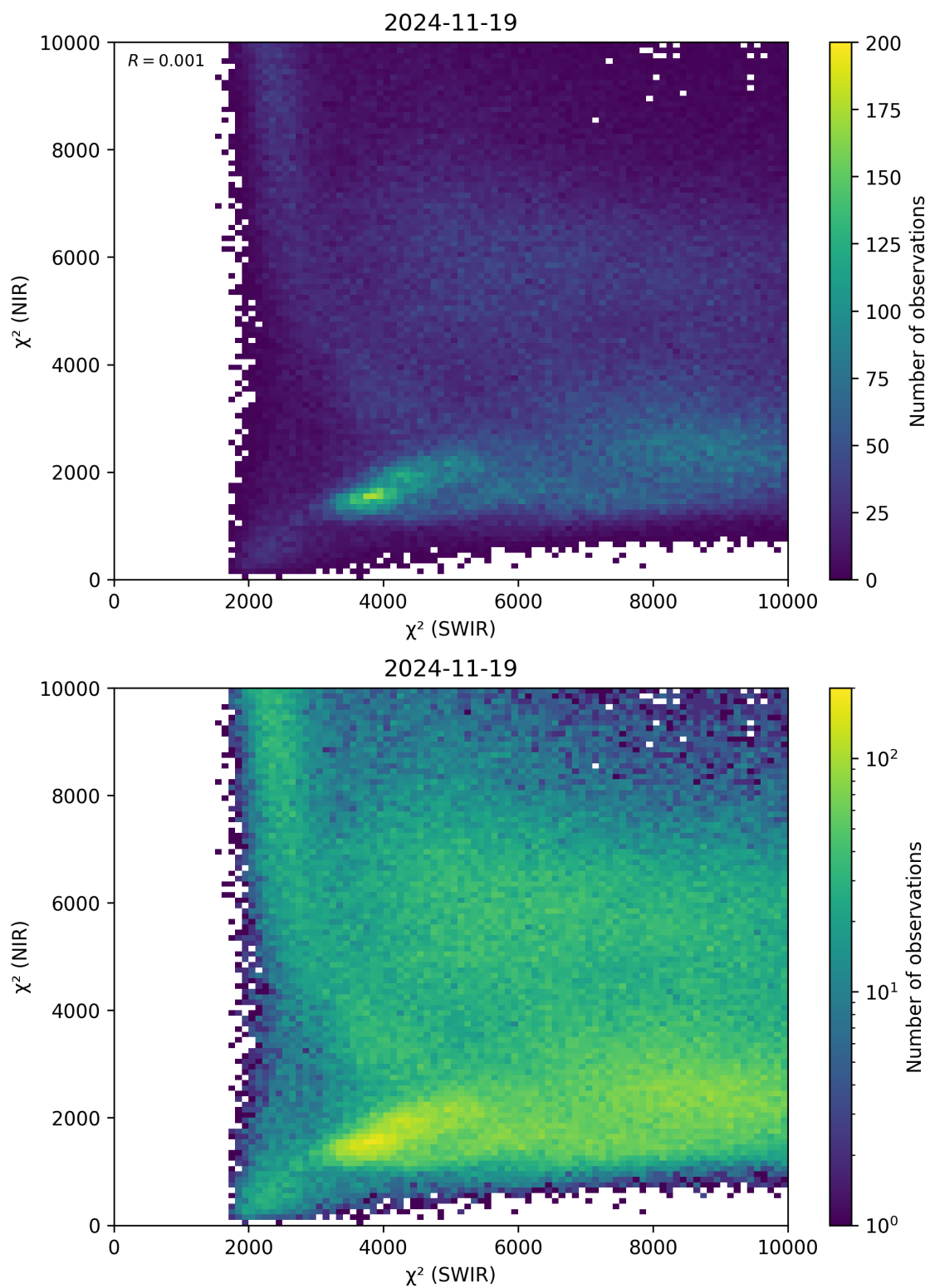
Figure 47: Scatter density plot of “ \chi^2 (SWIR)” against “ \chi^2 (NIR)” for 2024-11-18 to 2024-11-20.
