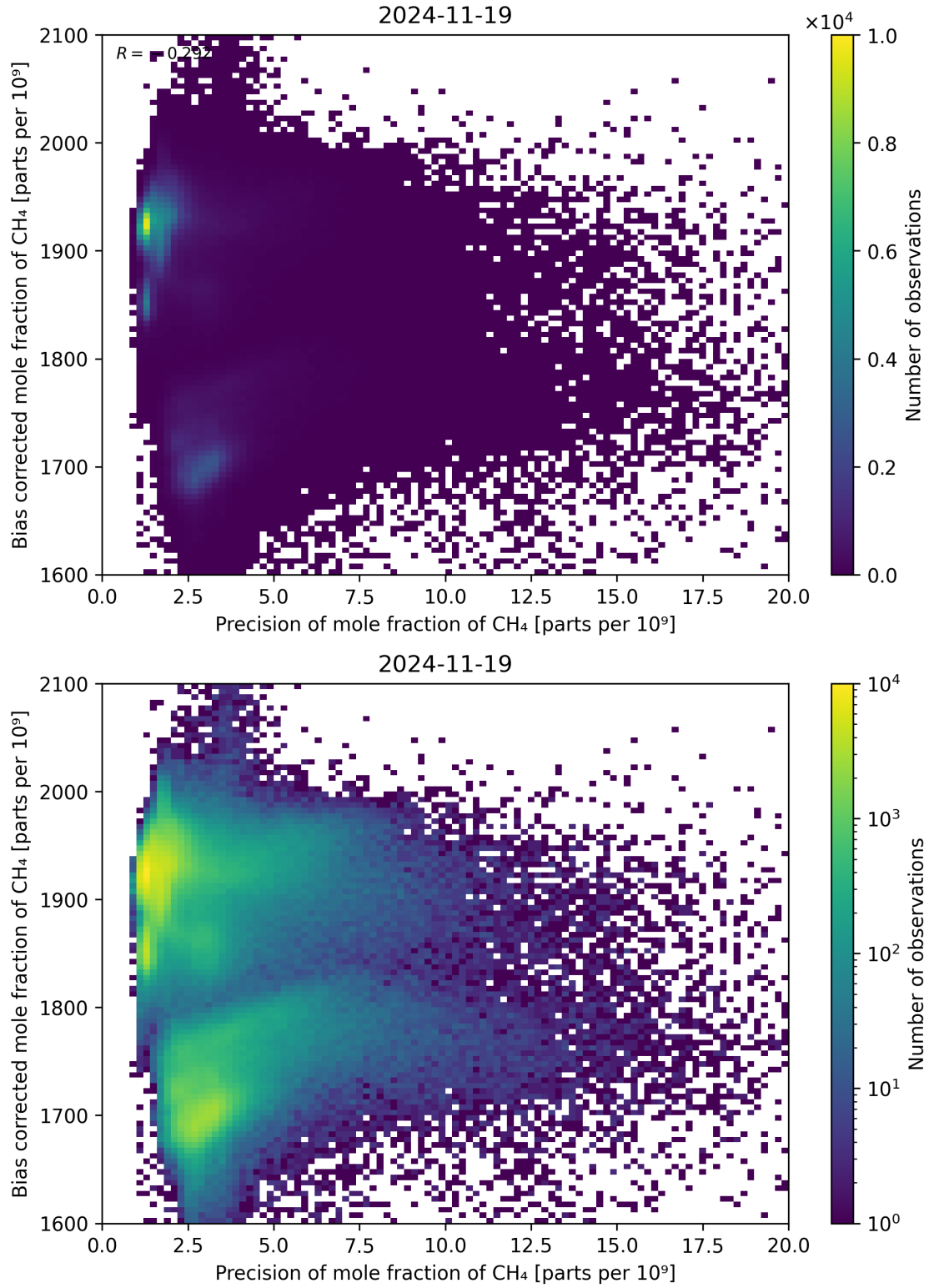
Figure 82: Scatter density plot of “Precision of mole fraction of CH 4 ” against “Bias corrected mole fraction of CH 4 ” for 2024-11-18 to 2024-11-20.
