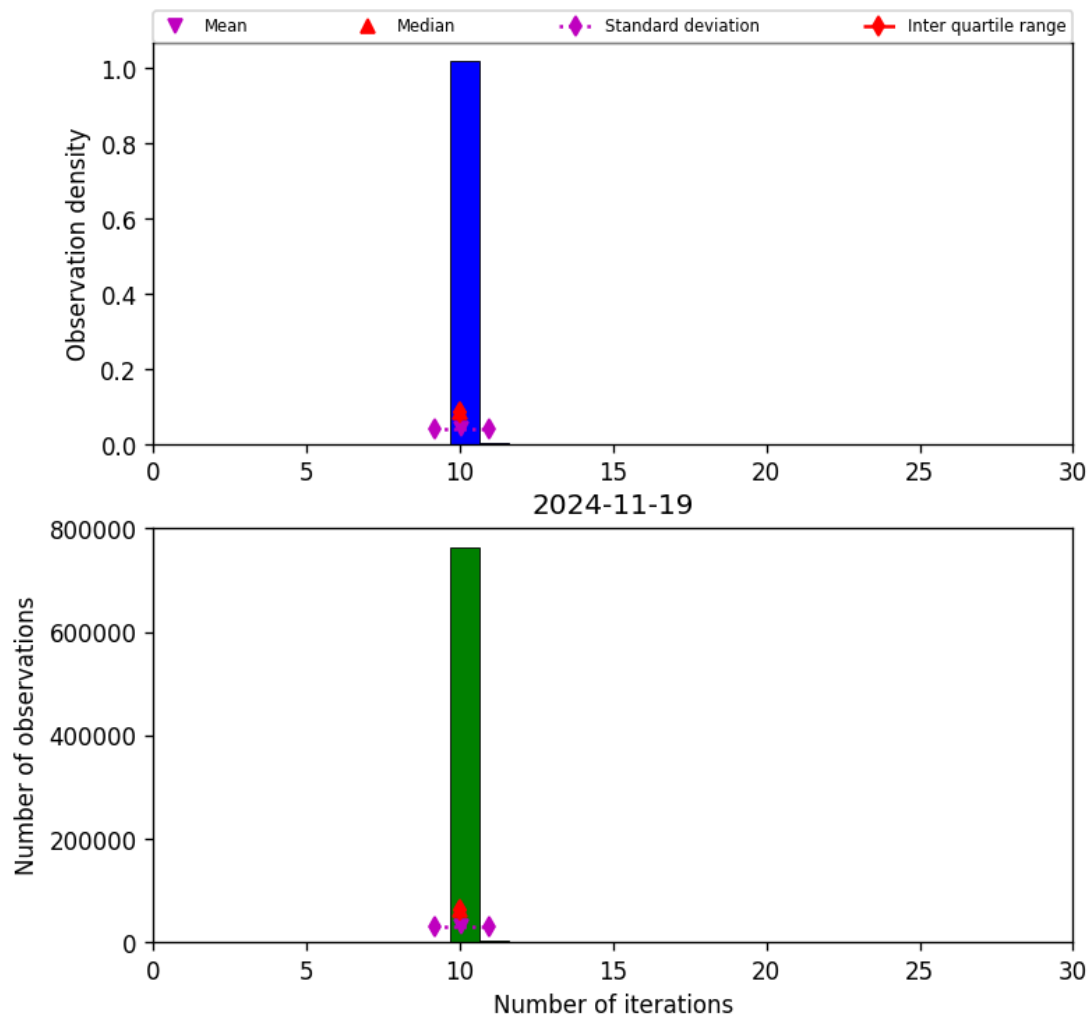
Figure 31: Histogram of “Number of iterations” for 2024-11-18 to 2024-11-20
