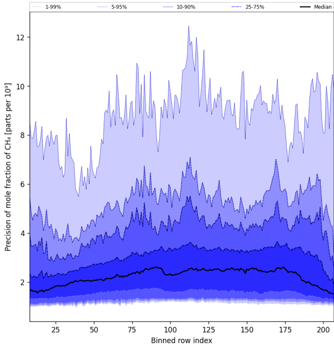
Figure 35: Along track statistics of “Precision of mole fraction of CH 4 ” for 2024-11-18 to 2024-11-20
