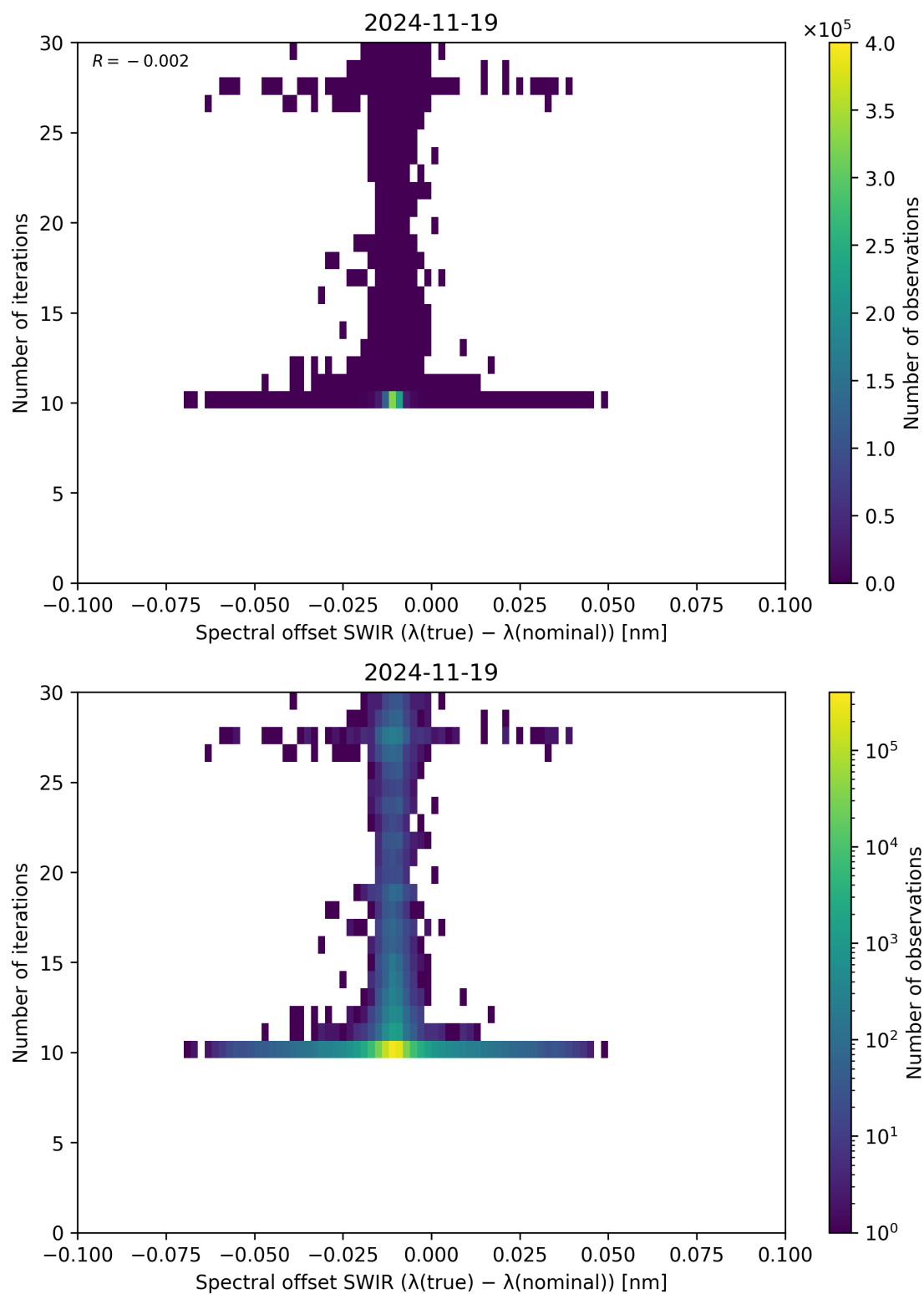
Figure 121: Scatter density plot of “Spectral offset SWIR ( \lambda_{\text{true}} - \lambda_{\text{nominal}} )” against “Number of iterations” for 2024-11-18 to 2024-11-20.
