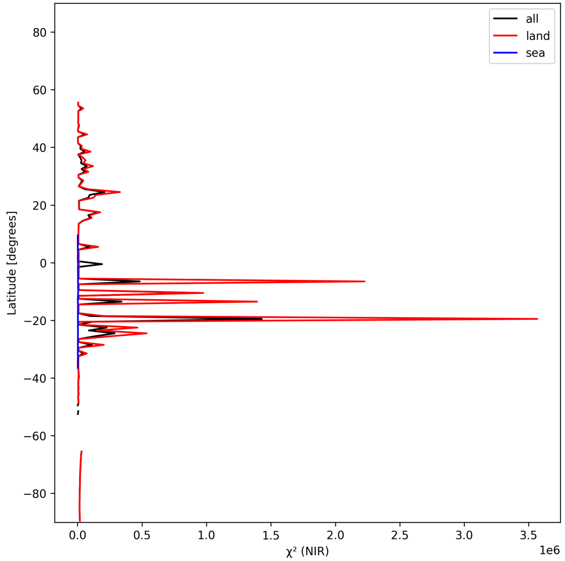
Figure 18: Zonal average of “ \chi^2 (NIR)” for 2024-11-18 to 2024-11-20.
