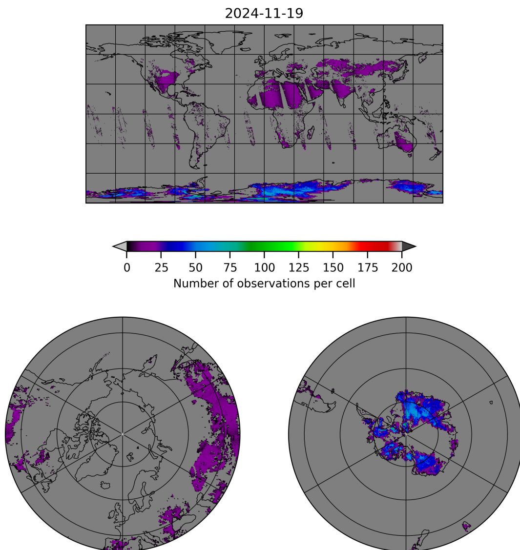
Figure 10: Map of the number of observations for 2024-11-18 to 2024-11-20
