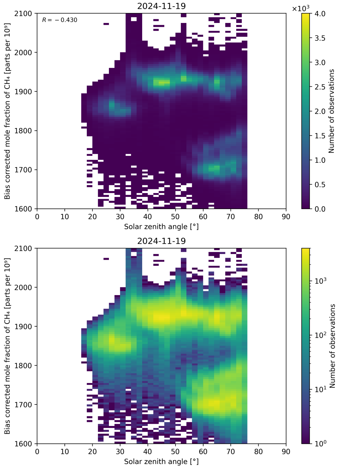
Figure 100: Scatter density plot of “Solar zenith angle” against “Bias corrected mole fraction of CH 4 ” for 2024-11-18 to 2024-11-20.
