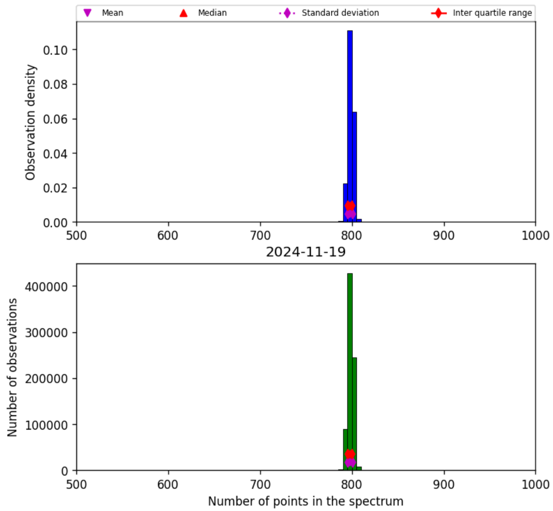
Figure 26: Histogram of “Number of points in the spectrum” for 2024-11-18 to 2024-11-20
