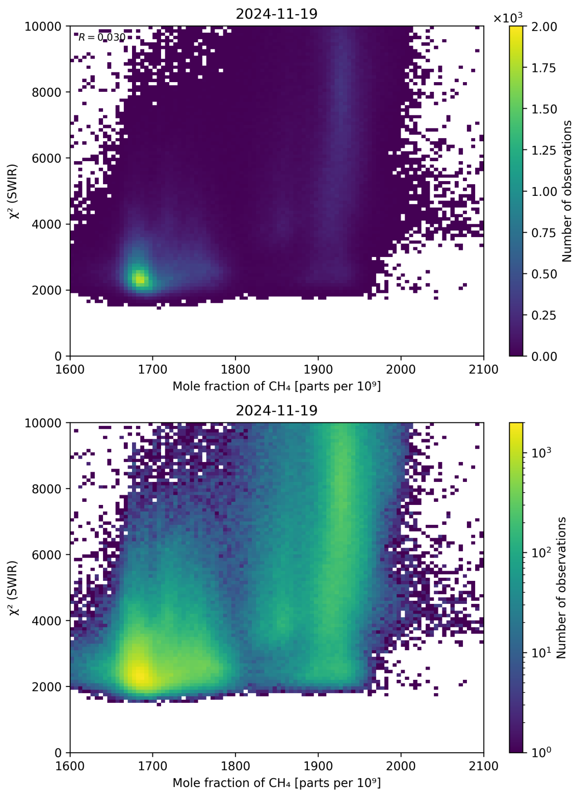
Figure 71: Scatter density plot of “Mole fraction of CH 4 ” against “ \chi^2 (SWIR)” for 2024-11-18 to 2024-11-20.
