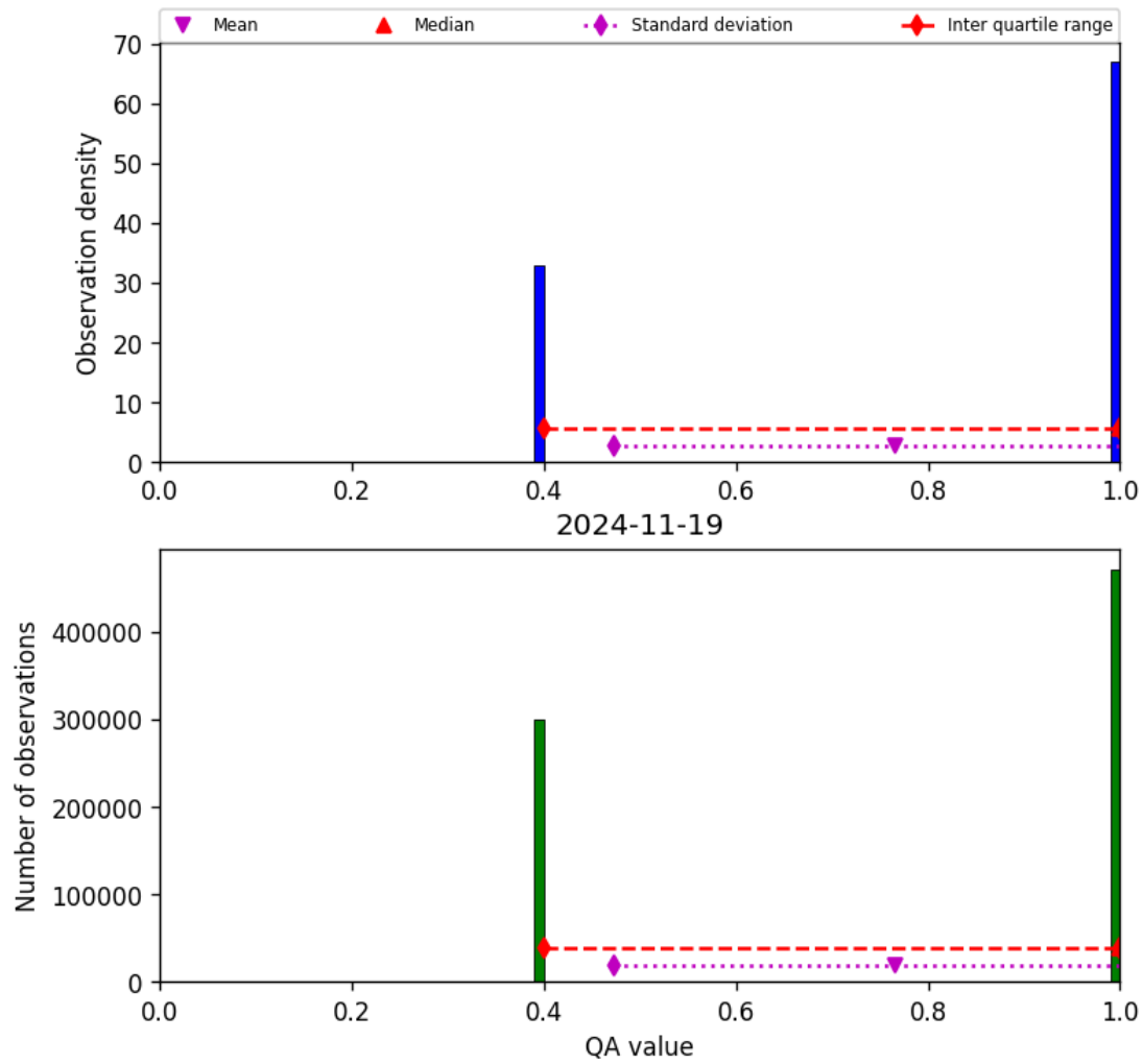
Figure 22: Histogram of “QA value” for 2024-11-18 to 2024-11-20
