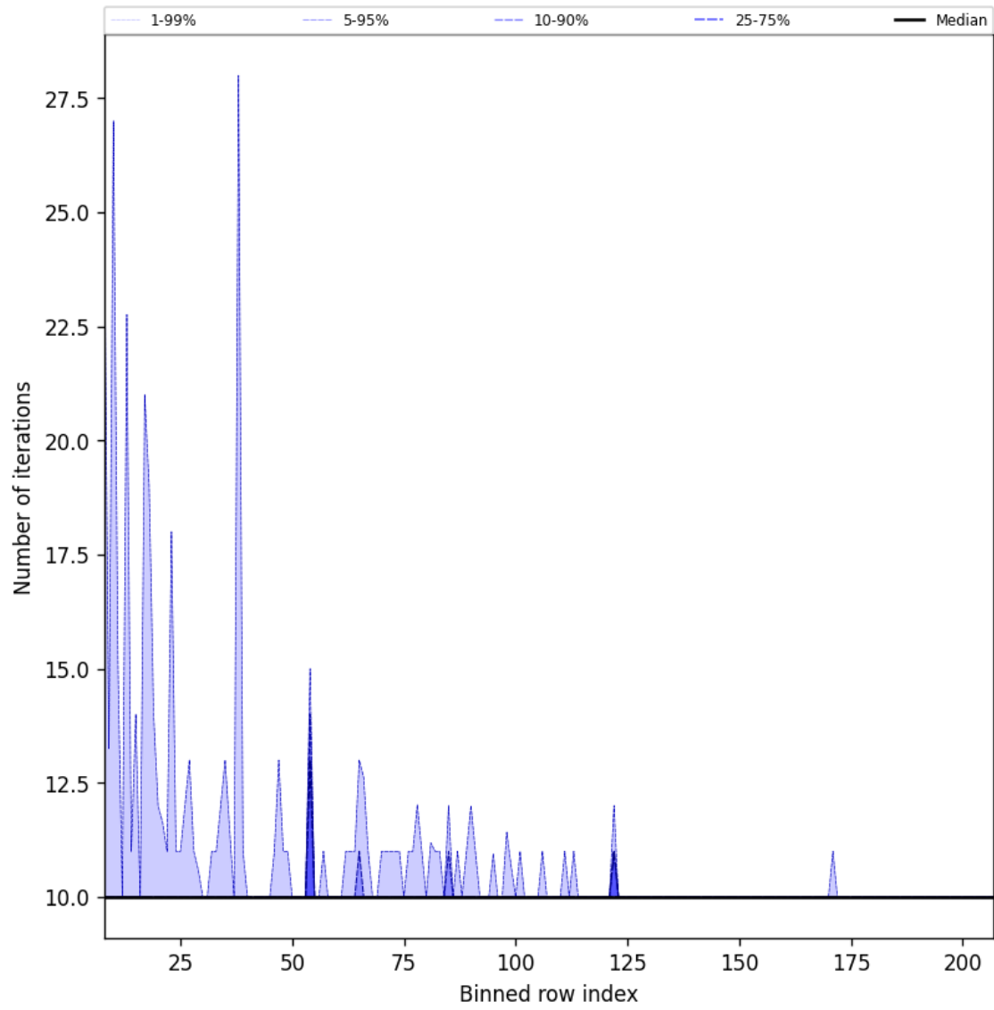
Figure 42: Along track statistics of “Number of iterations” for 2024-11-18 to 2024-11-20
