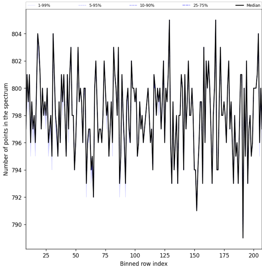
Figure 37: Along track statistics of “Number of points in the spectrum” for 2024-11-18 to 2024-11-20
