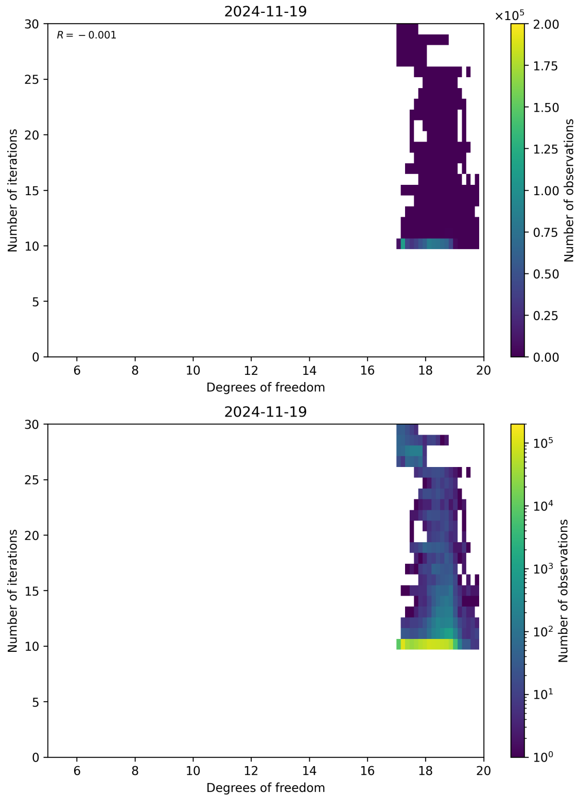
Figure 52: Scatter density plot of “Degrees of freedom” against “Number of iterations” for 2024-11-18 to 2024-11-20.
