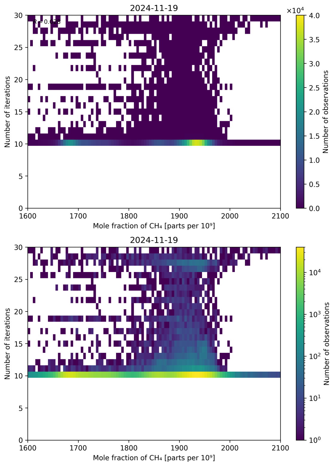
Figure 76: Scatter density plot of “Mole fraction of CH 4 ” against “Number of iterations” for 2024-11-18 to 2024-11-20.
