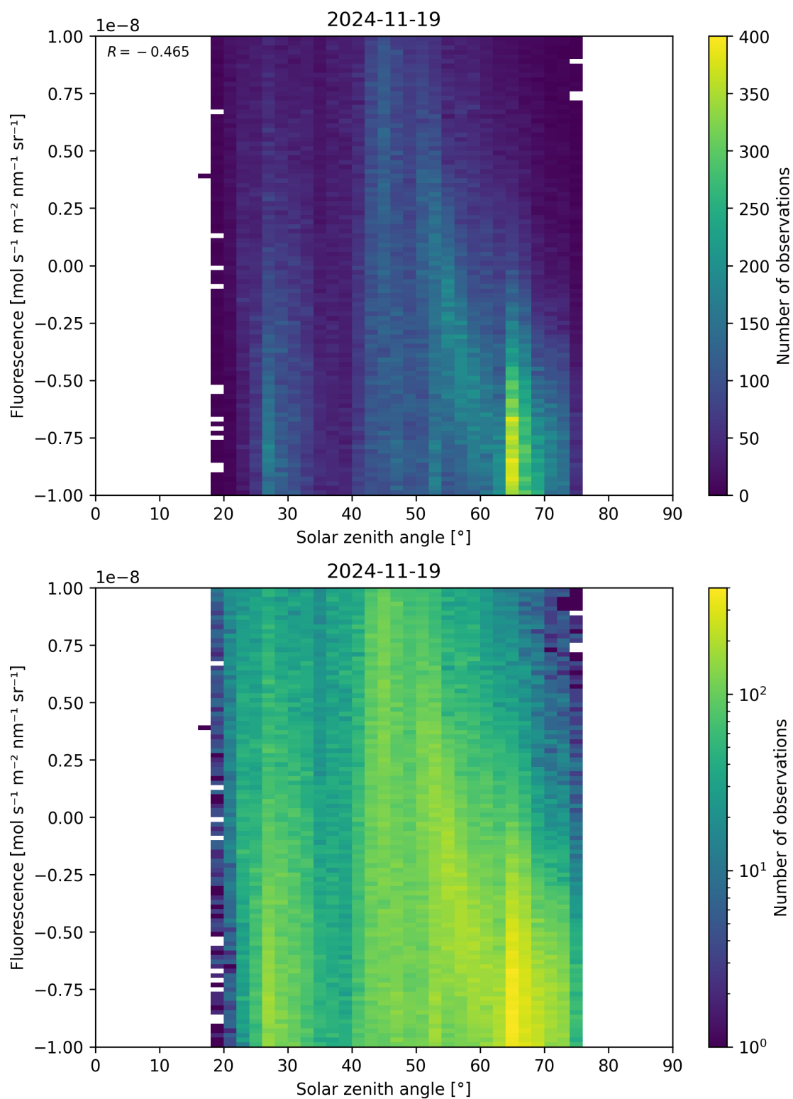
Figure 97: Scatter density plot of “Solar zenith angle” against “Fluorescence” for 2024-11-18 to 2024-11-20.
