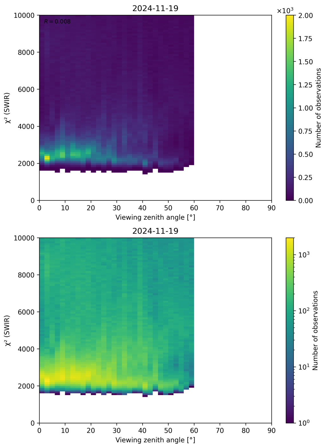
Figure 106: Scatter density plot of “Viewing zenith angle” against “ \chi^2 (SWIR)” for 2024-11-18 to 2024-11-20.
