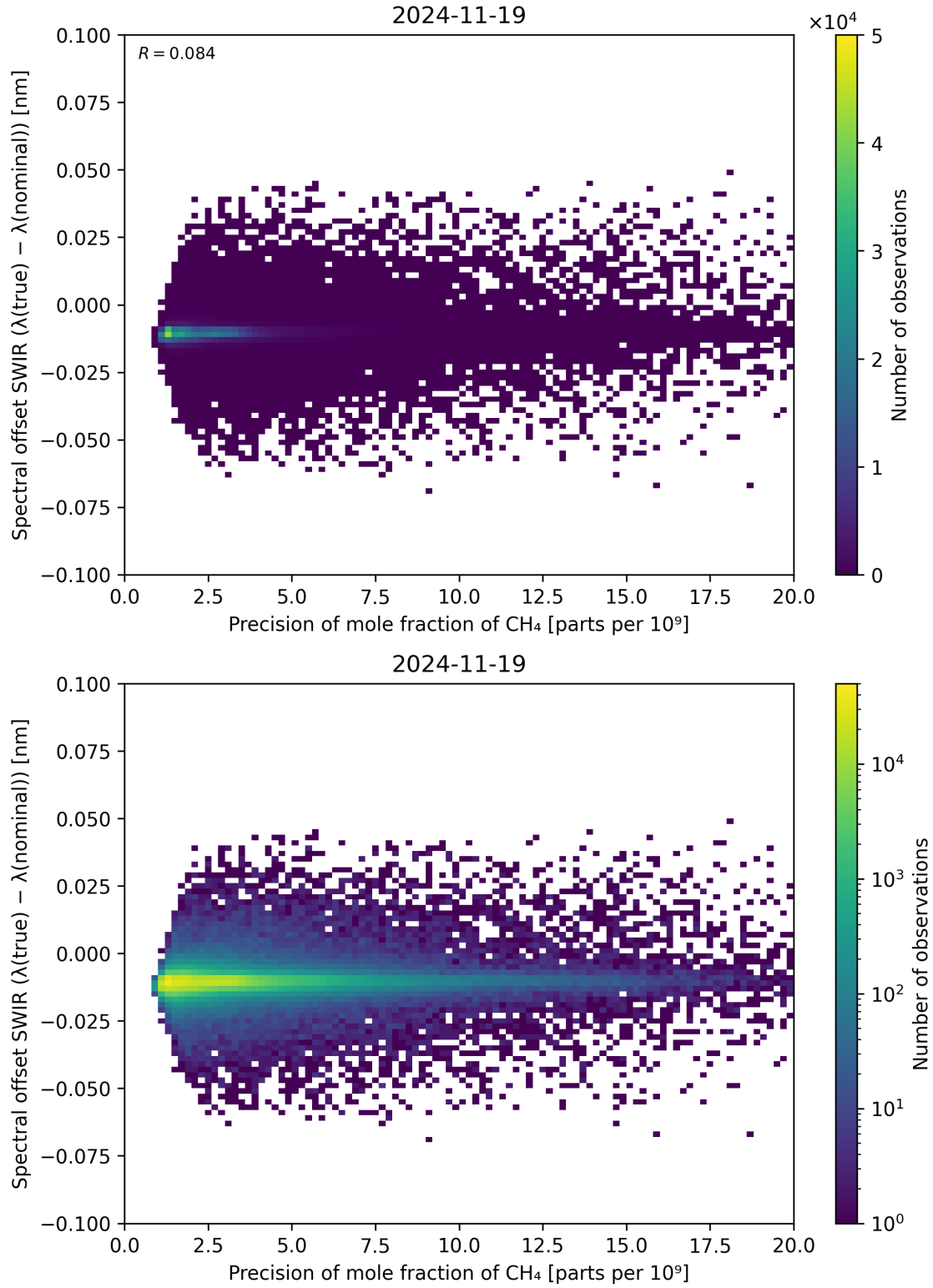
Figure 85: Scatter density plot of “Precision of mole fraction of \text{CH}_4 ” against “Spectral offset SWIR ( \lambda_{\text{true}} - \lambda_{\text{nominal}} )” for 2024-11-18 to 2024-11-20.
