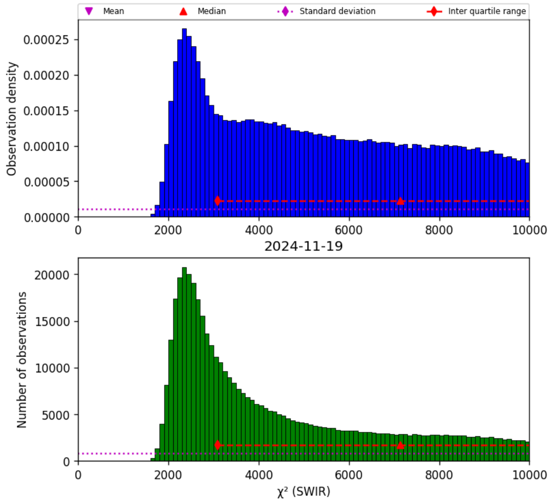
Figure 28: Histogram of “ \chi^2 (SWIR)” for 2024-11-18 to 2024-11-20
