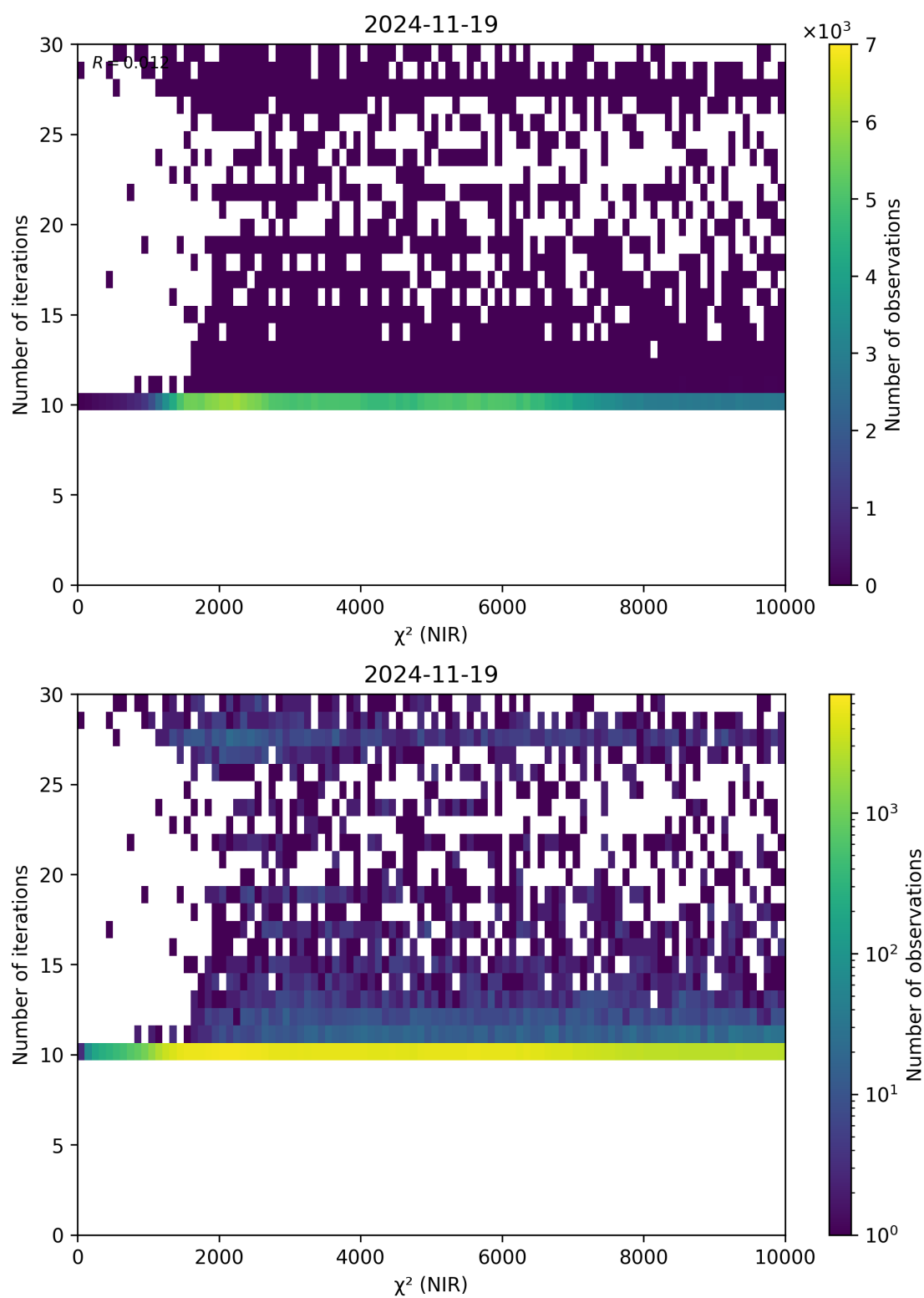
Figure 46: Scatter density plot of “ \chi^2 (NIR)” against “Number of iterations” for 2024-11-18 to 2024-11-20.
