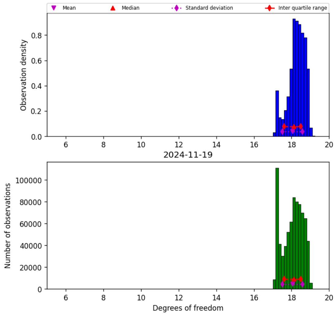
Figure 30: Histogram of “Degrees of freedom” for 2024-11-18 to 2024-11-20
