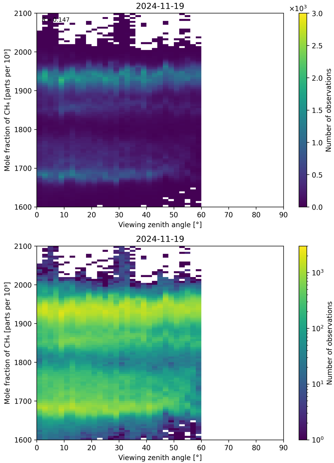
Figure 110: Scatter density plot of “Viewing zenith angle” against “Mole fraction of CH 4 ” for 2024-11-18 to 2024-11-20.
