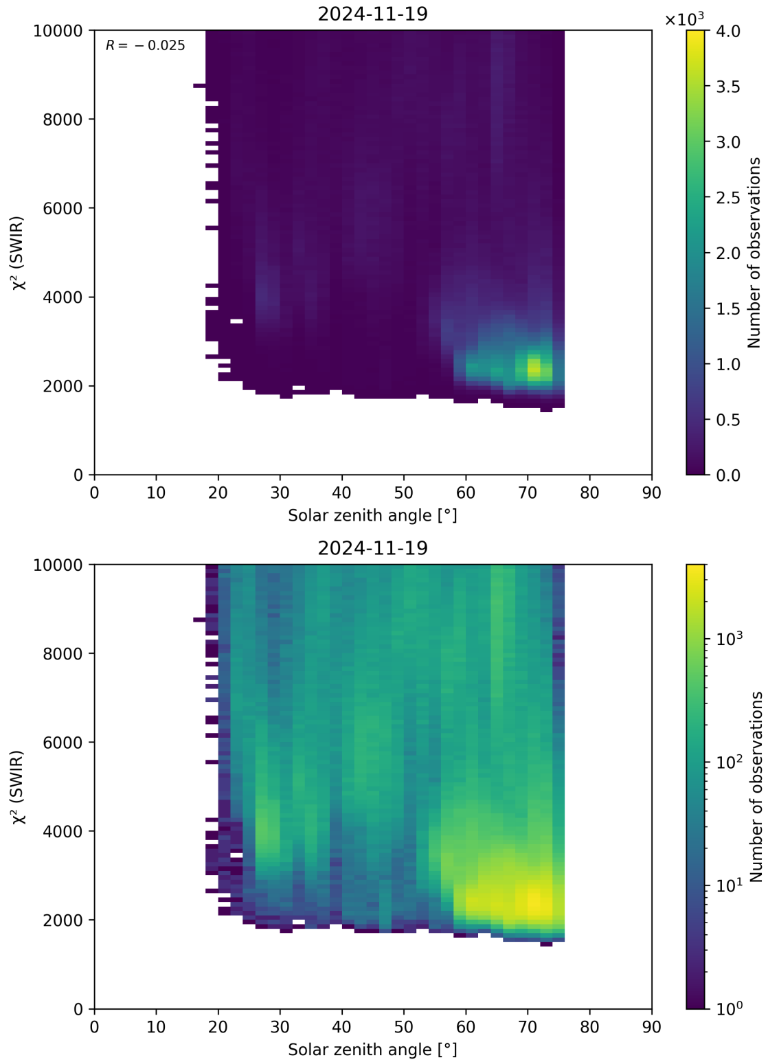
Figure 95: Scatter density plot of “Solar zenith angle” against “ \chi^2 (SWIR)” for 2024-11-18 to 2024-11-20.
