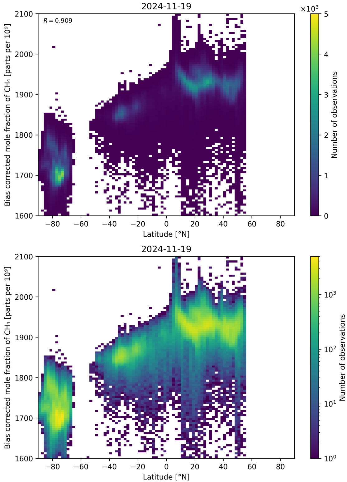
Figure 58: Scatter density plot of “Latitude” against “Bias corrected mole fraction of CH 4 ” for 2024-11-18 to 2024-11-20.
