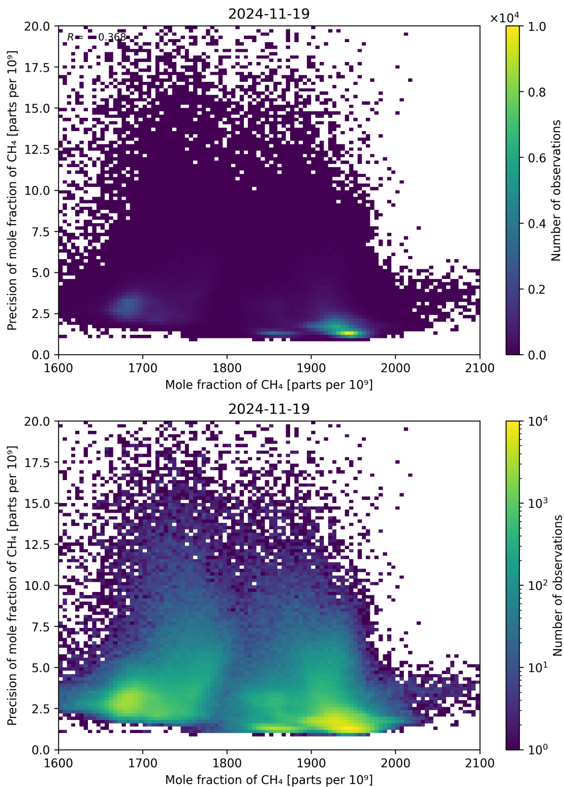
Figure 75: Scatter density plot of “Mole fraction of CH 4 ” against “Precision of mole fraction of CH 4 ” for 2024-11-18 to 2024-11-20.
