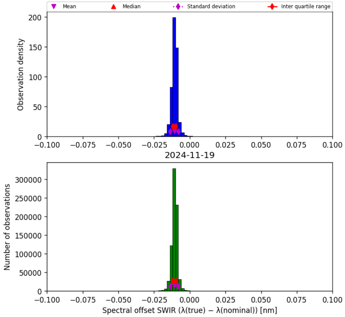
Figure 27: Histogram of “Spectral offset SWIR ( \lambda_{\text{true}} - \lambda_{\text{nominal}} )” for 2024-11-18 to 2024-11-20
