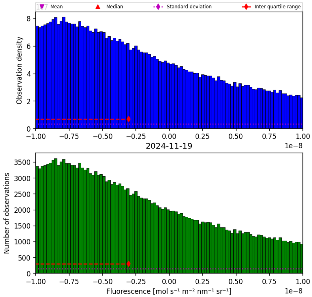
Figure 32: Histogram of “Fluorescence” for 2024-11-18 to 2024-11-20
