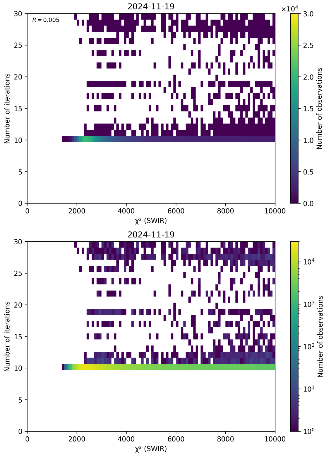
Figure 50: Scatter density plot of “ \chi^2 (SWIR)” against “Number of iterations” for 2024-11-18 to 2024-11-20.
