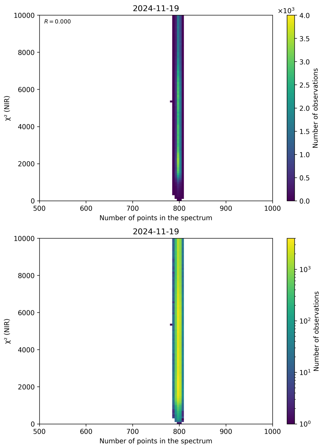
Figure 88: Scatter density plot of “Number of points in the spectrum” against “ \chi^2 (NIR)” for 2024-11-18 to 2024-11-20.
