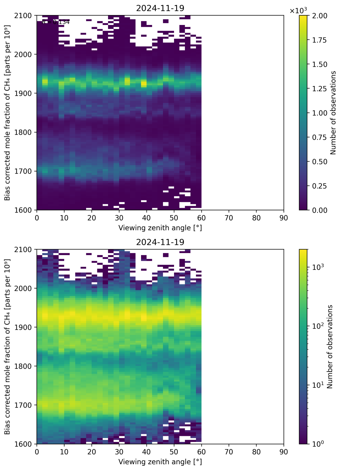
Figure 111: Scatter density plot of “Viewing zenith angle” against “Bias corrected mole fraction of CH 4 ” for 2024-11-18 to 2024-11-20.
