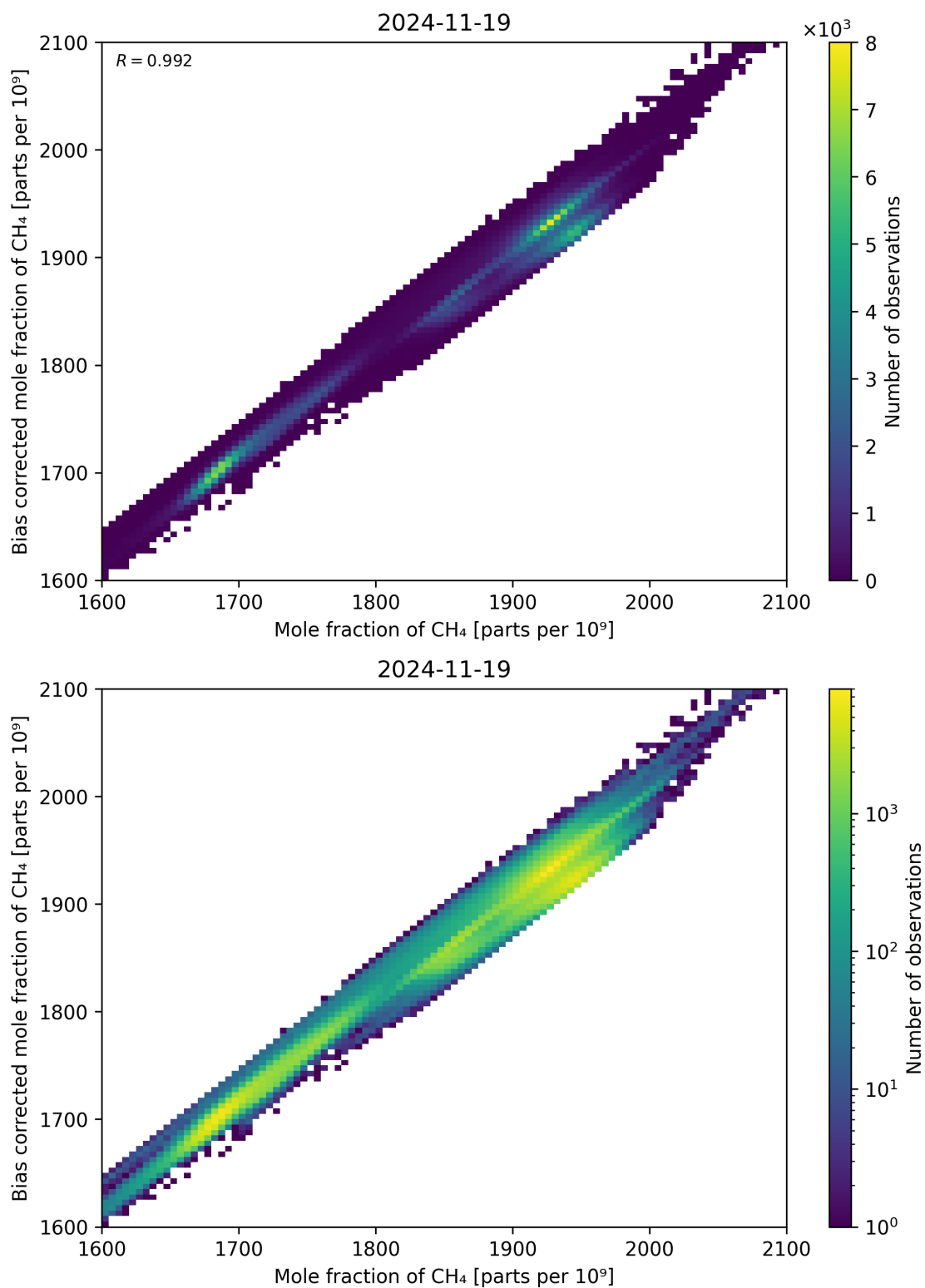
Figure 74: Scatter density plot of “Mole fraction of CH 4 ” against “Bias corrected mole fraction of CH 4 ” for 2024-11-18 to 2024-11-20.
