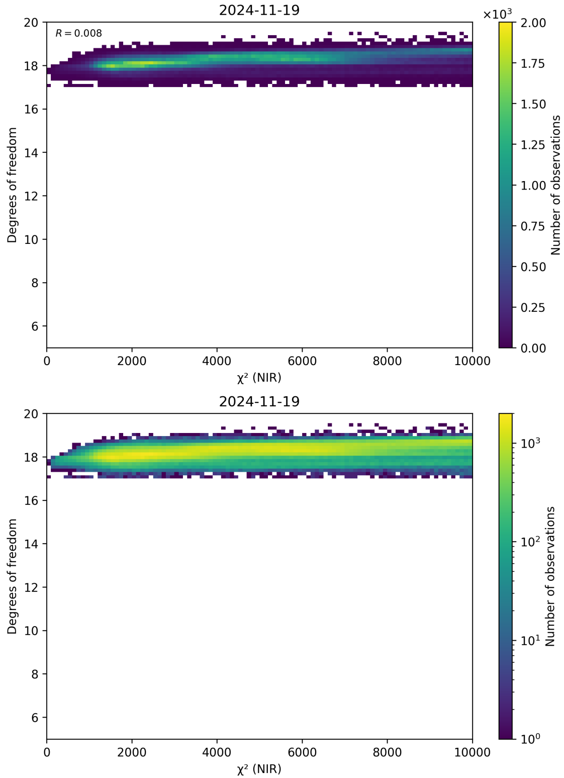
Figure 44: Scatter density plot of “ \chi^2 (NIR)” against “Degrees of freedom” for 2024-11-18 to 2024-11-20.
