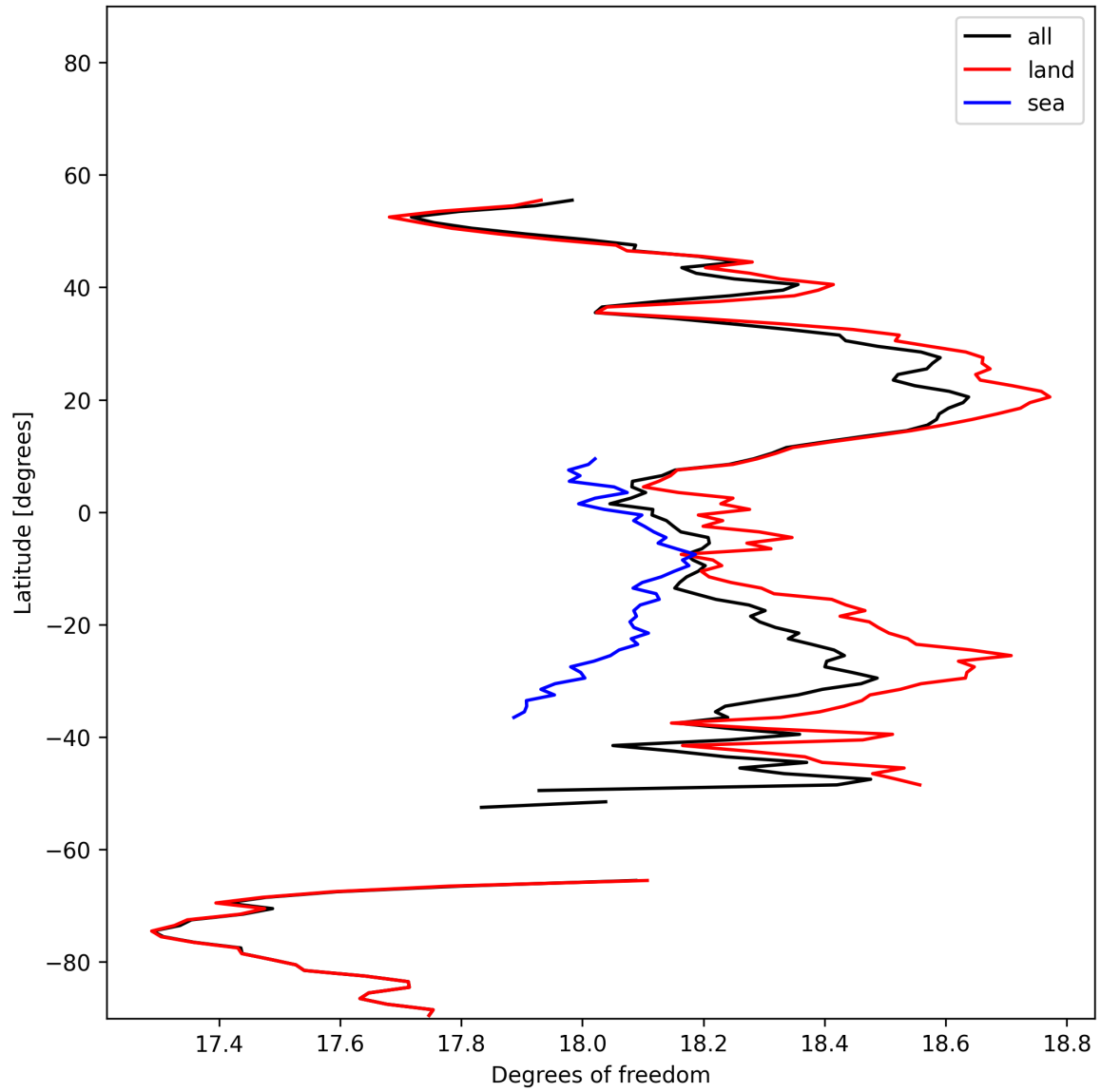
Figure 19: Zonal average of “Degrees of freedom” for 2024-11-18 to 2024-11-20.
