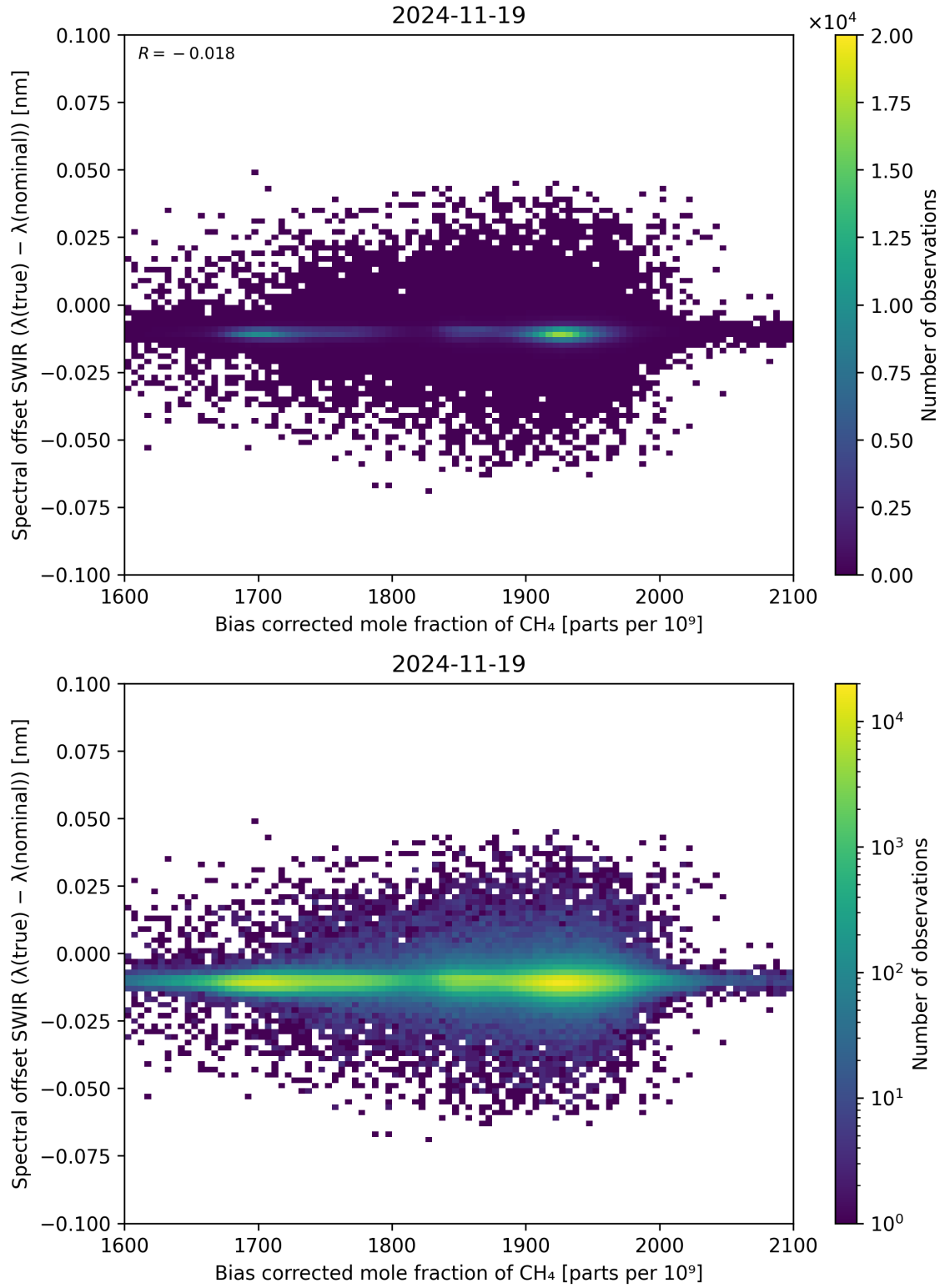
Figure 69: Scatter density plot of “Bias corrected mole fraction of \text{CH}_4 ” against “Spectral offset SWIR ( \lambda_{\text{true}} - \lambda_{\text{nominal}} )” for 2024-11-18 to 2024-11-20.
