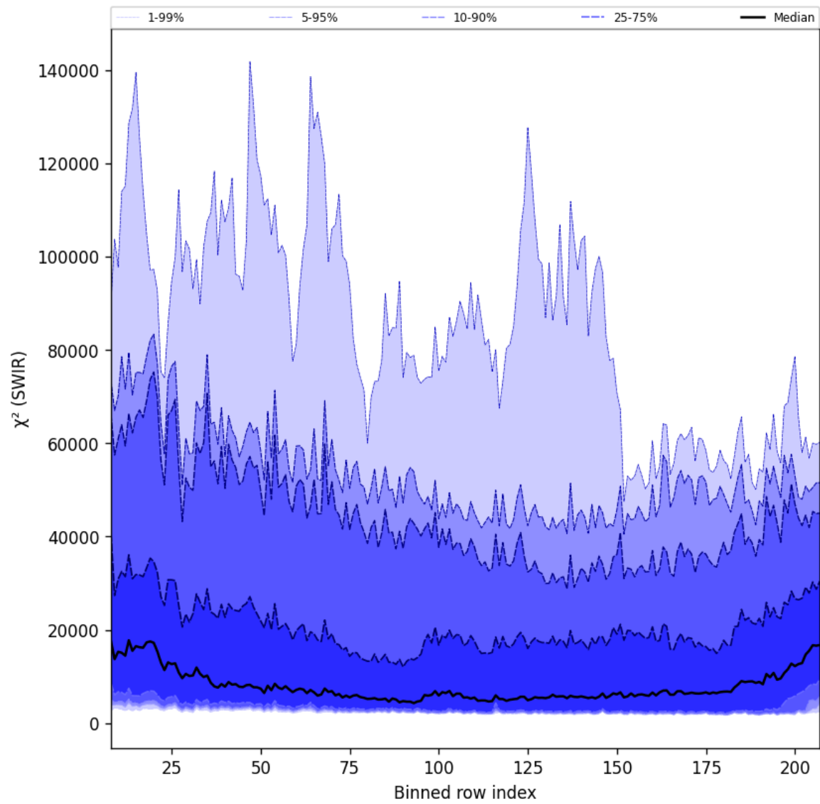
Figure 39: Along track statistics of “ \chi^2 (SWIR)” for 2024-11-18 to 2024-11-20
