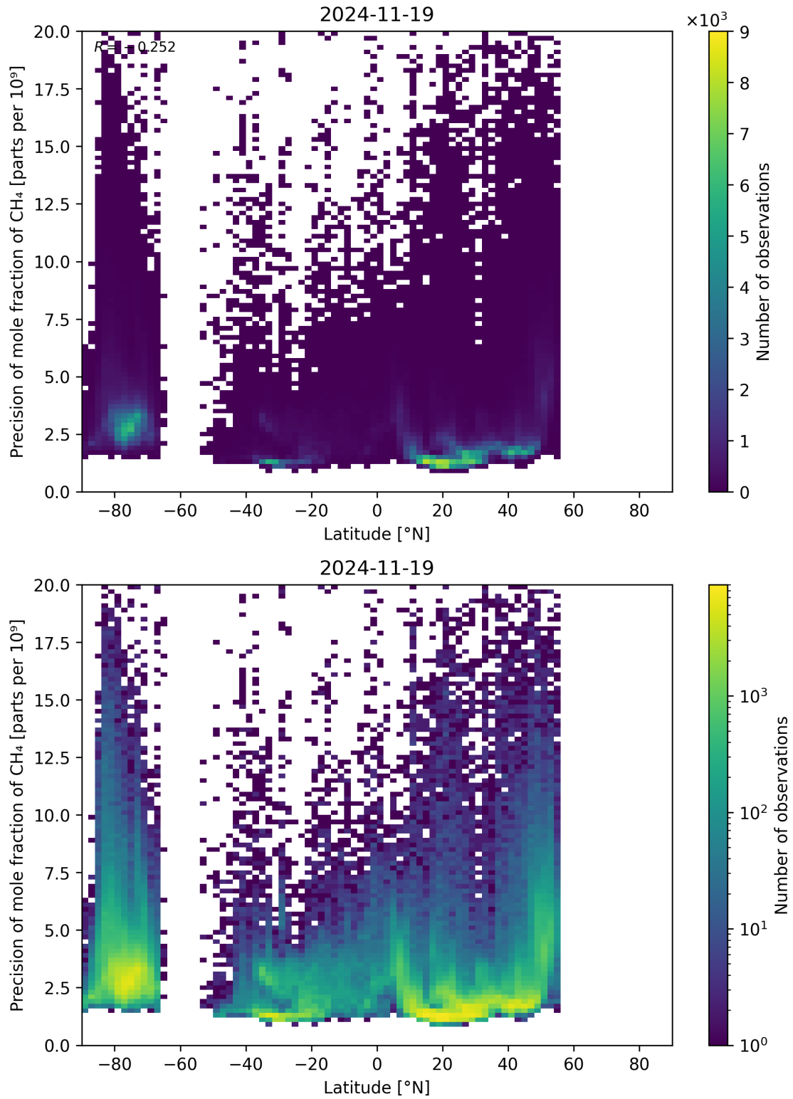
Figure 59: Scatter density plot of “Latitude” against “Precision of mole fraction of CH 4 ” for 2024-11-18 to 2024-11-20.
