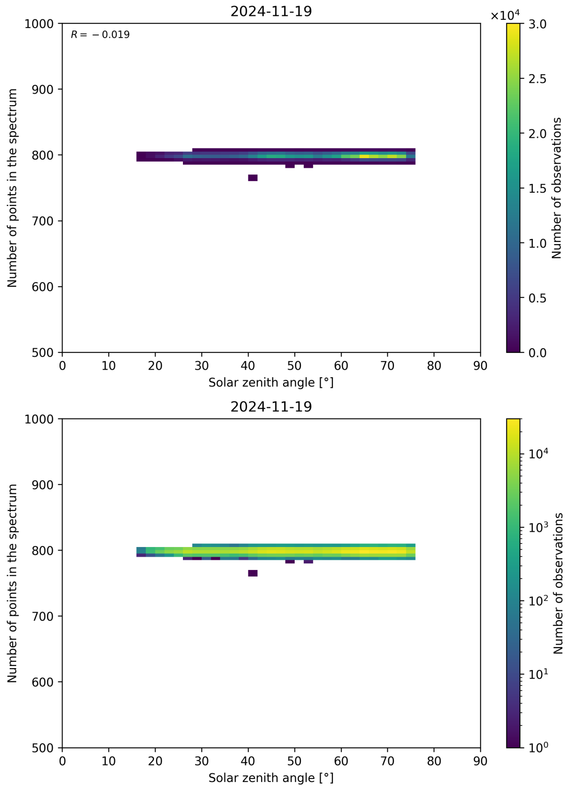
Figure 103: Scatter density plot of “Solar zenith angle” against “Number of points in the spectrum” for 2024-11-18 to 2024-11-20.
