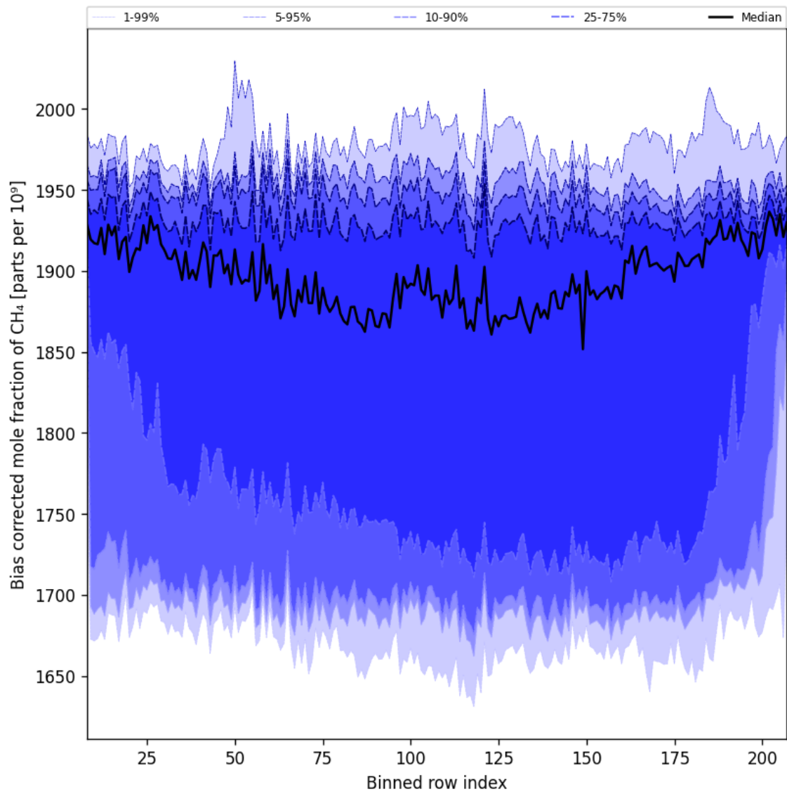
Figure 36: Along track statistics of “Bias corrected mole fraction of CH 4 ” for 2024-11-18 to 2024-11-20
