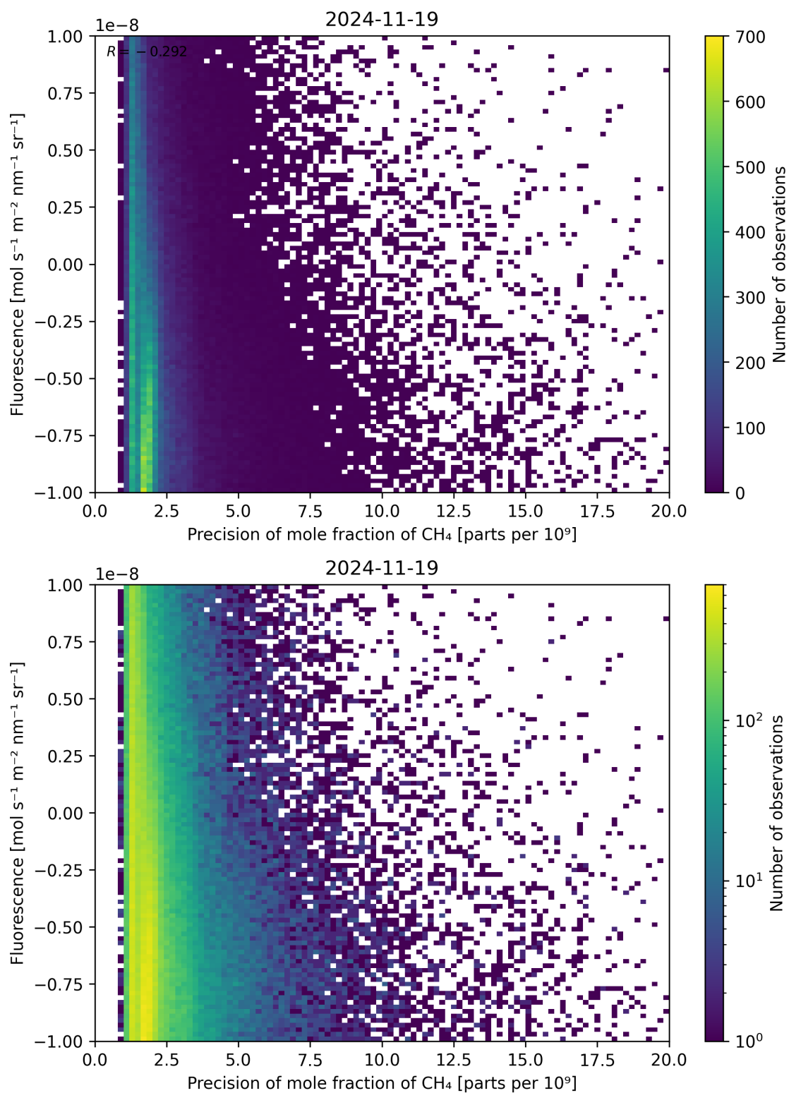
Figure 81: Scatter density plot of “Precision of mole fraction of \text{CH}_4 ” against “Fluorescence” for 2024-11-18 to 2024-11-20.
