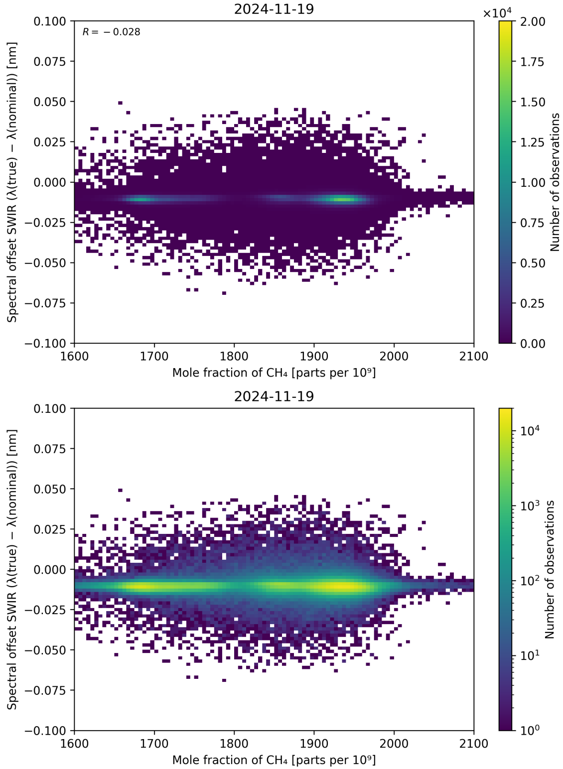
Figure 86: Scatter density plot of “Mole fraction of \text{CH}_4 ” against “Spectral offset SWIR ( \lambda_{\text{true}} - \lambda_{\text{nominal}} )” for 2024-11-18 to 2024-11-20.
