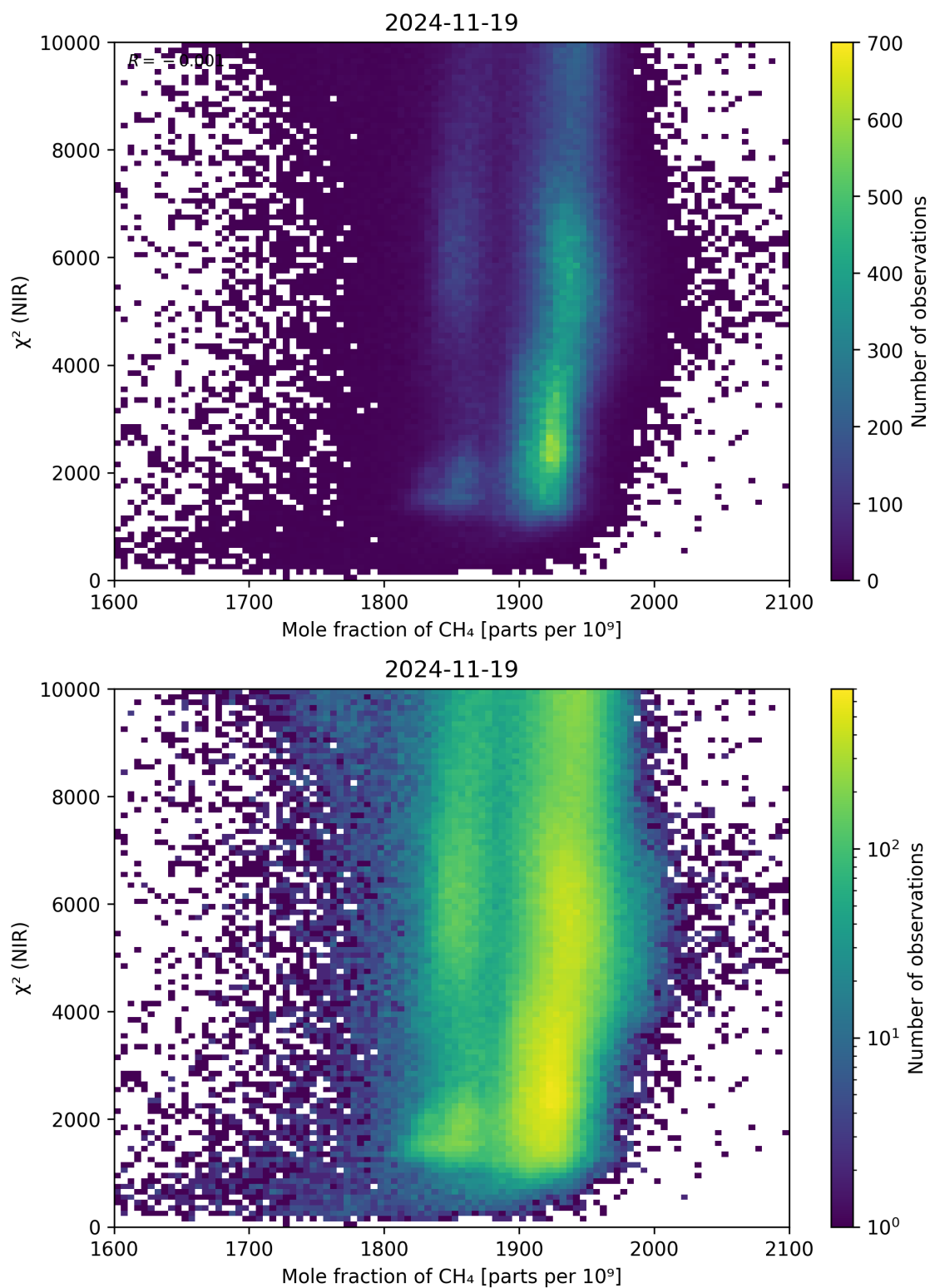
Figure 70: Scatter density plot of “Mole fraction of \text{CH}_4 ” against “ \chi^2 (NIR)” for 2024-11-18 to 2024-11-20.
