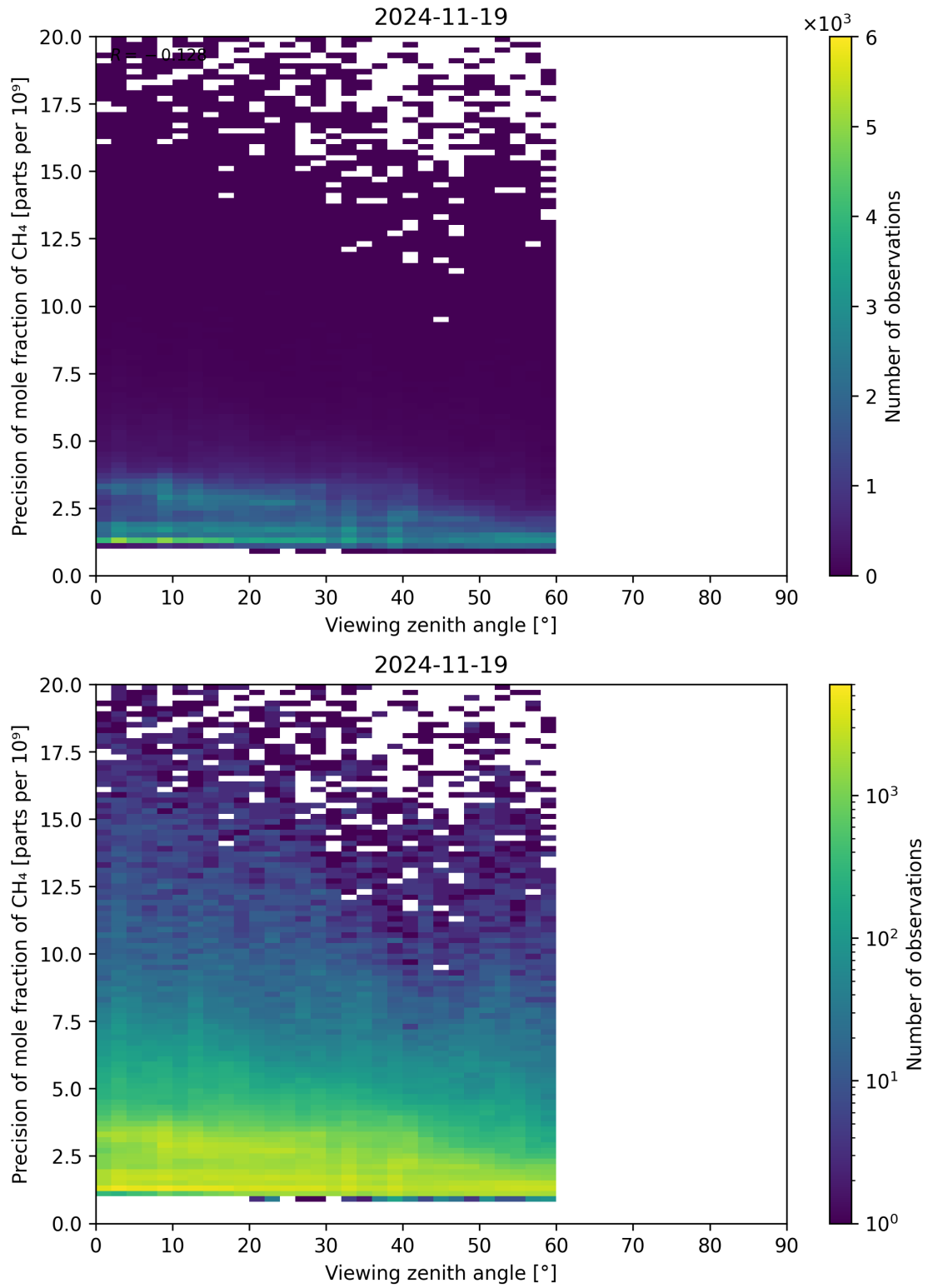
Figure 112: Scatter density plot of “Viewing zenith angle” against “Precision of mole fraction of CH 4 ” for 2024-11-18 to 2024-11-20.
