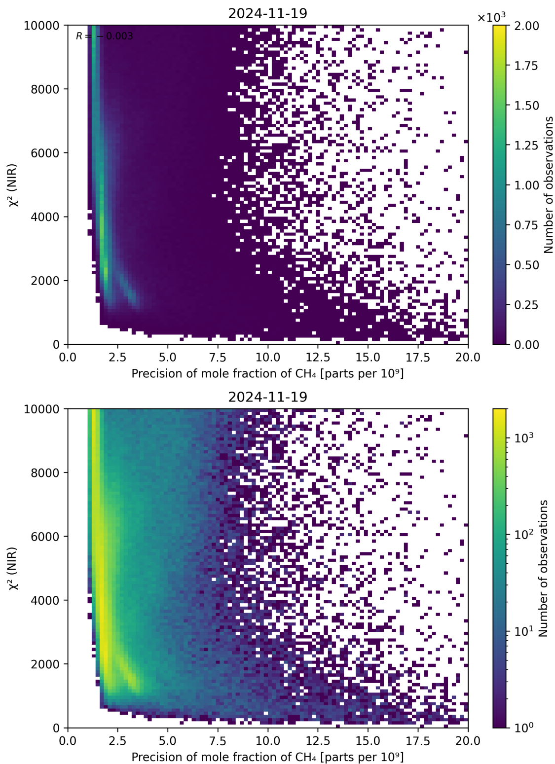
Figure 78: Scatter density plot of “Precision of mole fraction of CH 4 ” against “ \chi^2 (NIR)” for 2024-11-18 to 2024-11-20.
