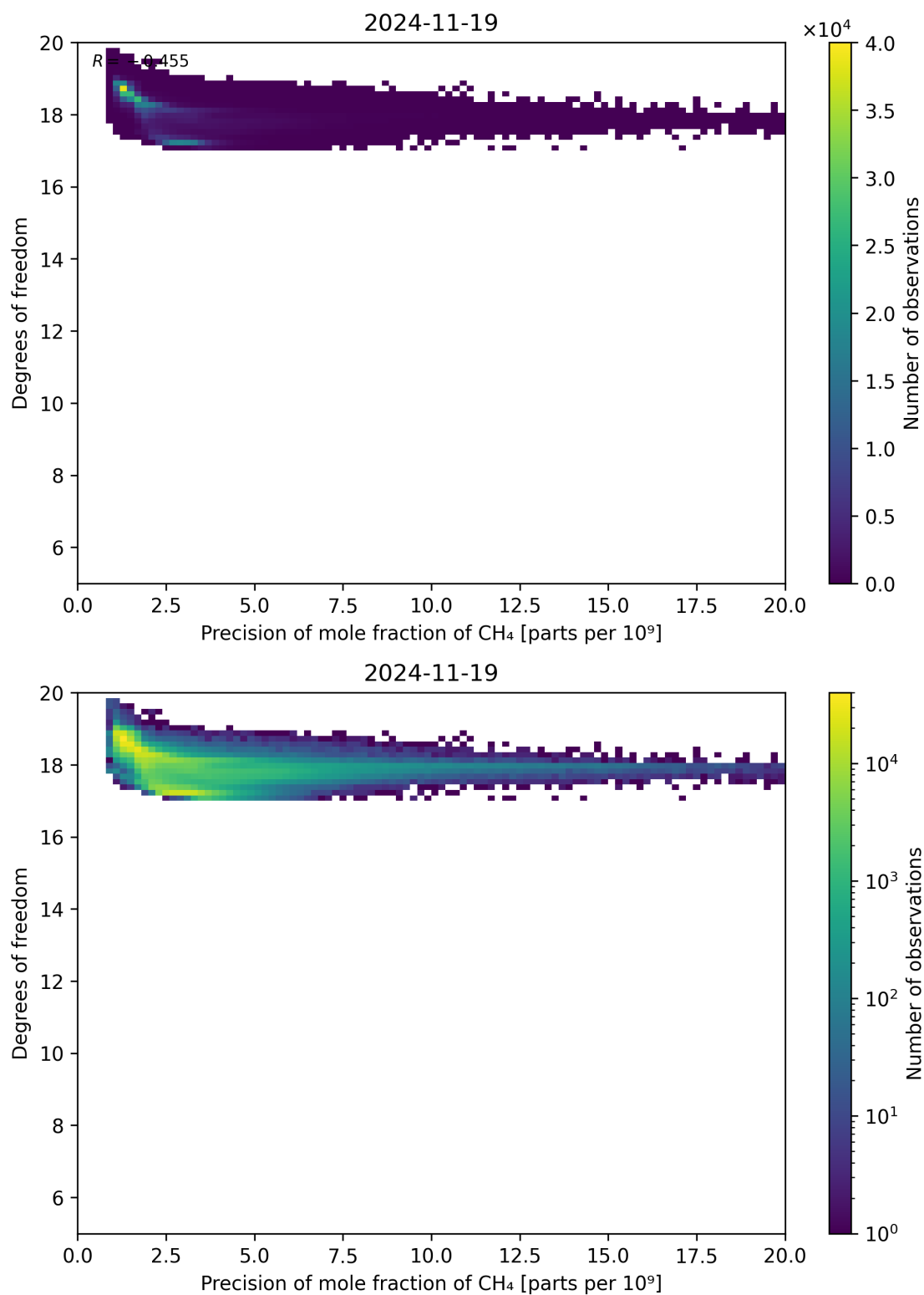
Figure 80: Scatter density plot of “Precision of mole fraction of \text{CH}_4 ” against “Degrees of freedom” for 2024-11-18 to 2024-11-20.
