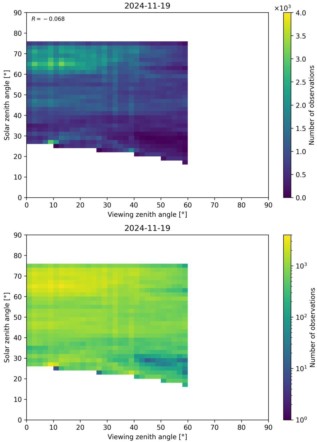
Figure 115: Scatter density plot of “Viewing zenith angle” against “Solar zenith angle” for 2024-11-18 to 2024-11-20.
