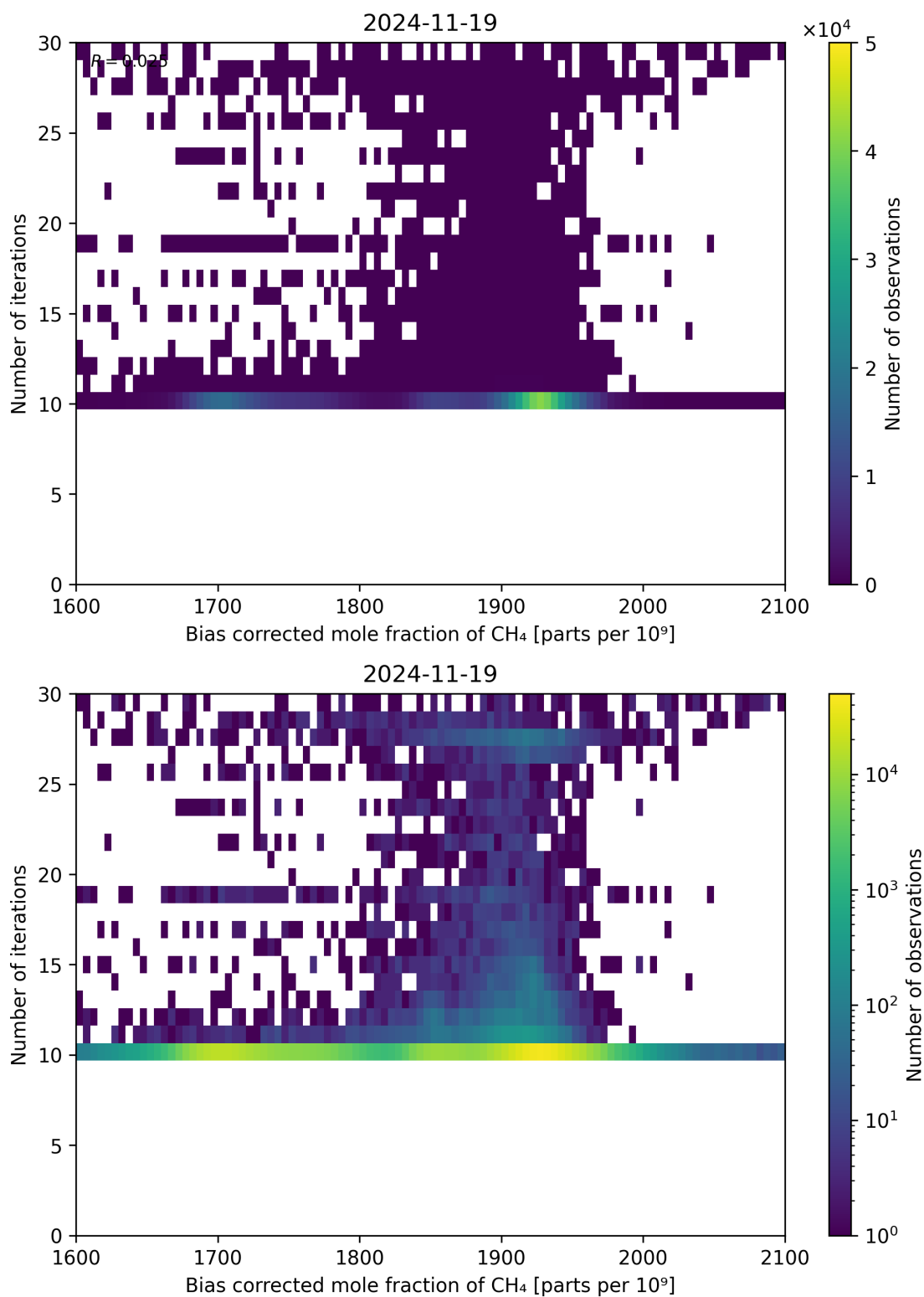
Figure 67: Scatter density plot of “Bias corrected mole fraction of CH 4 ” against “Number of iterations” for 2024-11-18 to 2024-11-20.
