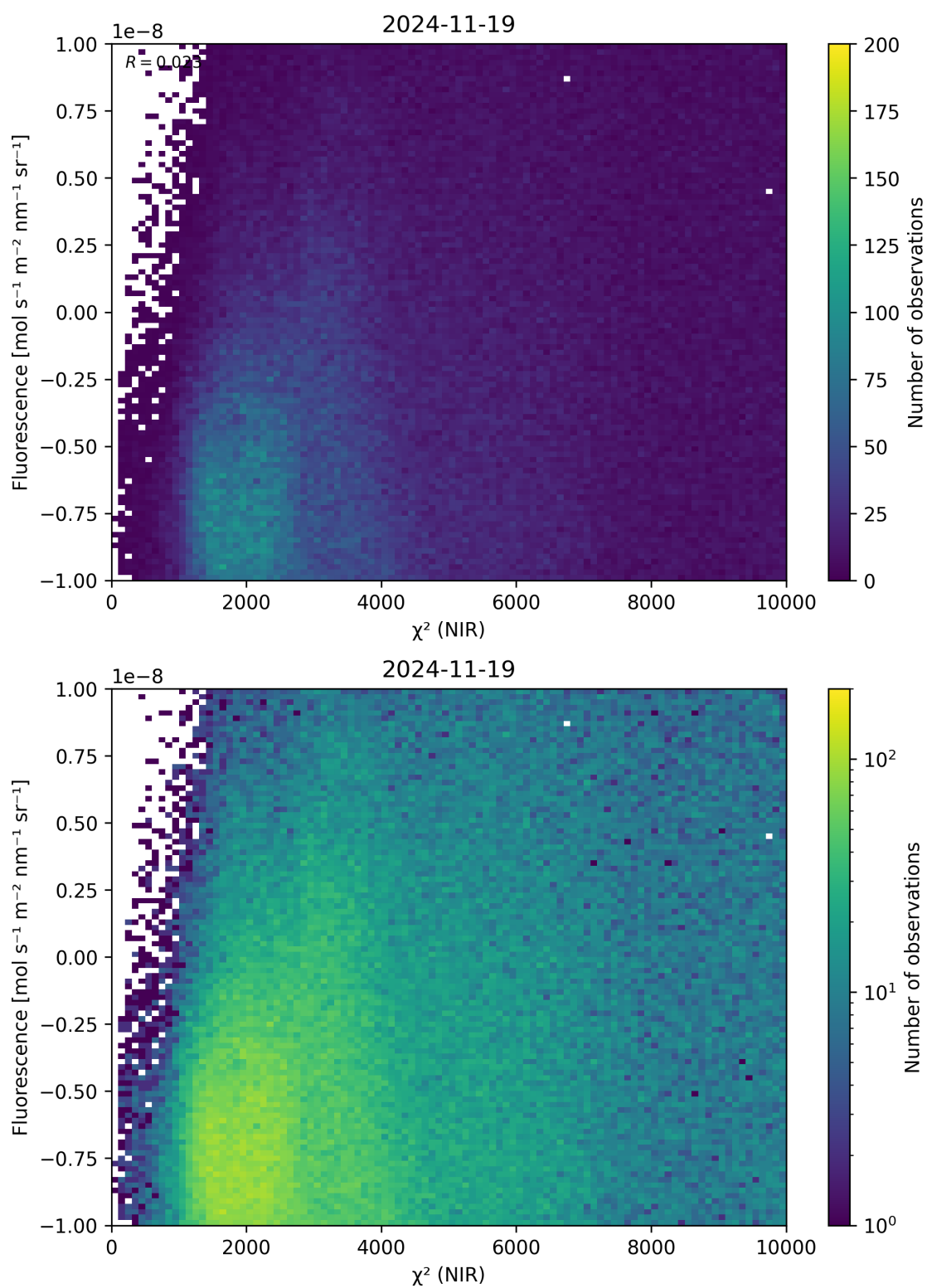
Figure 45: Scatter density plot of “ \chi^2 (NIR)” against “Fluorescence” for 2024-11-18 to 2024-11-20.
