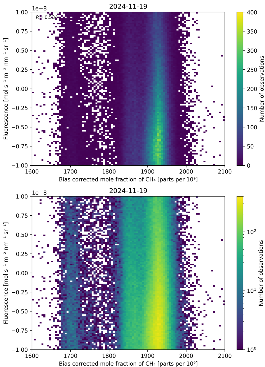
Figure 66: Scatter density plot of “Bias corrected mole fraction of \text{CH}_4 ” against “Fluorescence” for 2024-11-18 to 2024-11-20.
