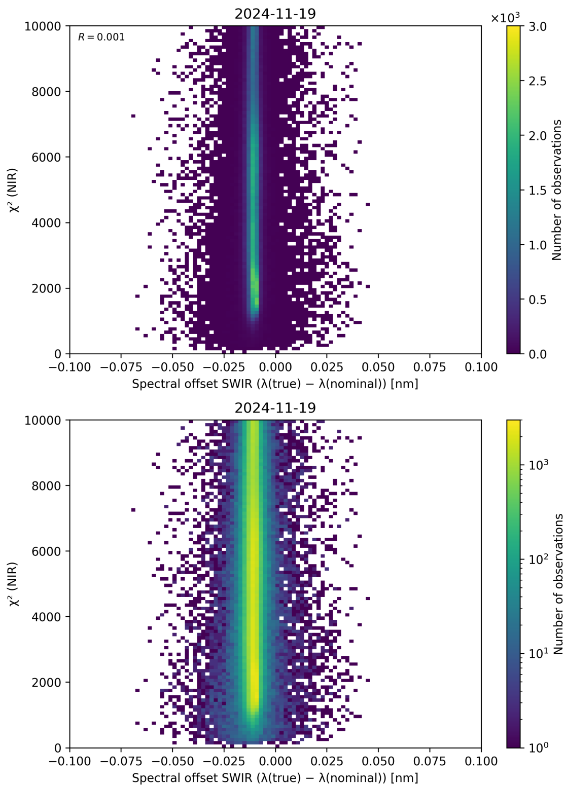
Figure 117: Scatter density plot of “Spectral offset SWIR ( \lambda_{\text{true}} - \lambda_{\text{nominal}} )” against “ \chi^2 (NIR)” for 2024-11-18 to 2024-11-20.
