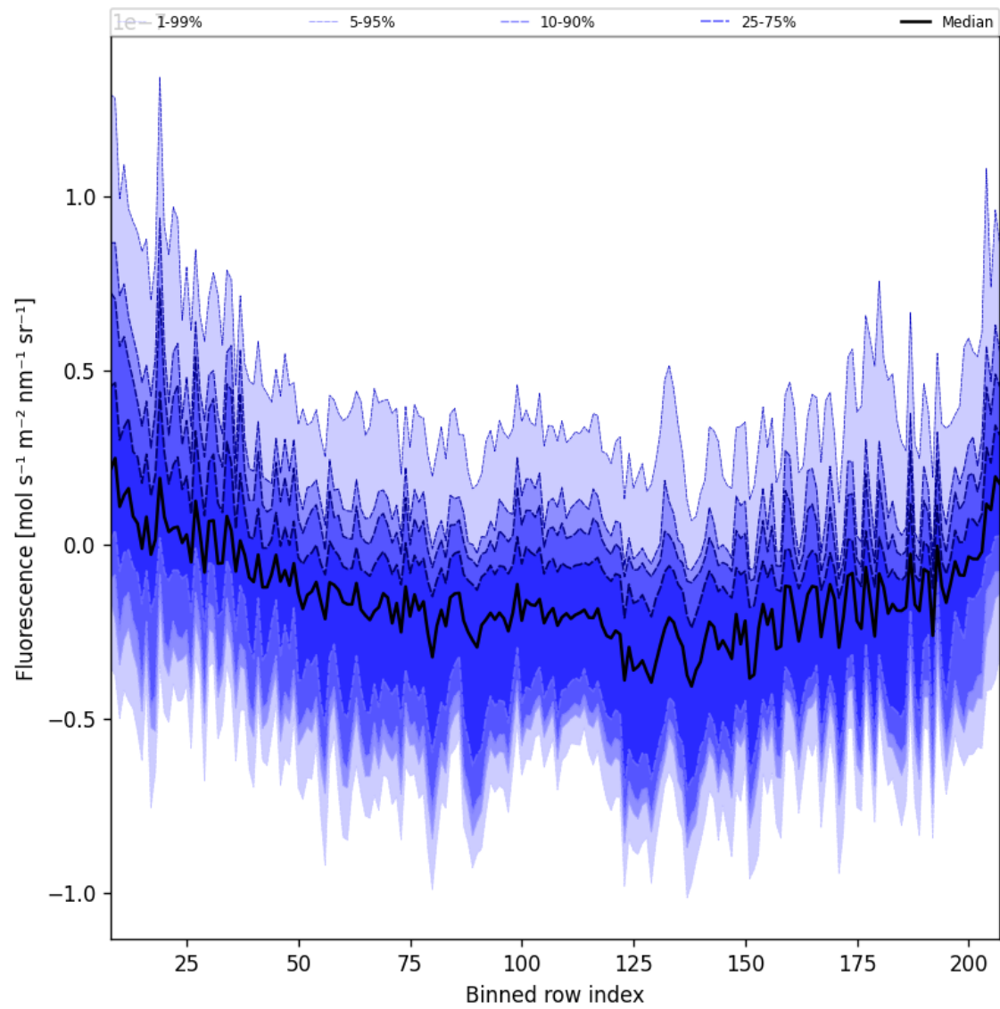
Figure 43: Along track statistics of “Fluorescence” for 2024-11-18 to 2024-11-20
