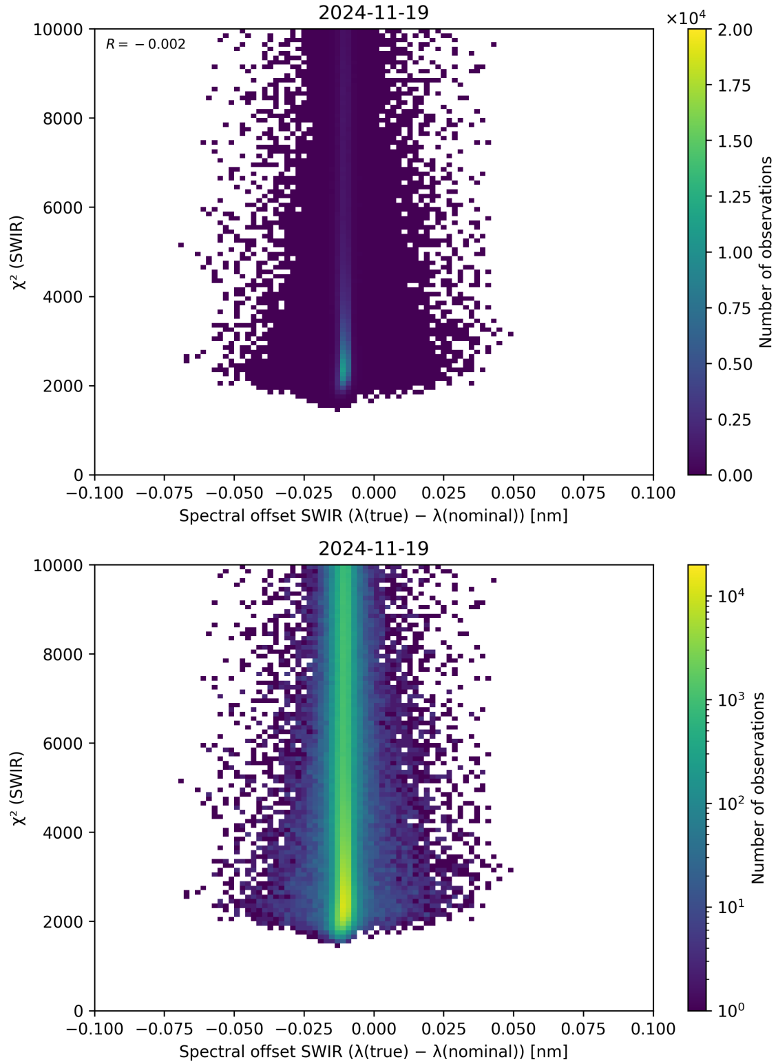
Figure 118: Scatter density plot of “Spectral offset SWIR ( \lambda_{\text{true}} - \lambda_{\text{nominal}} )” against “ \chi^2 (SWIR)” for 2024-11-18 to 2024-11-20.
