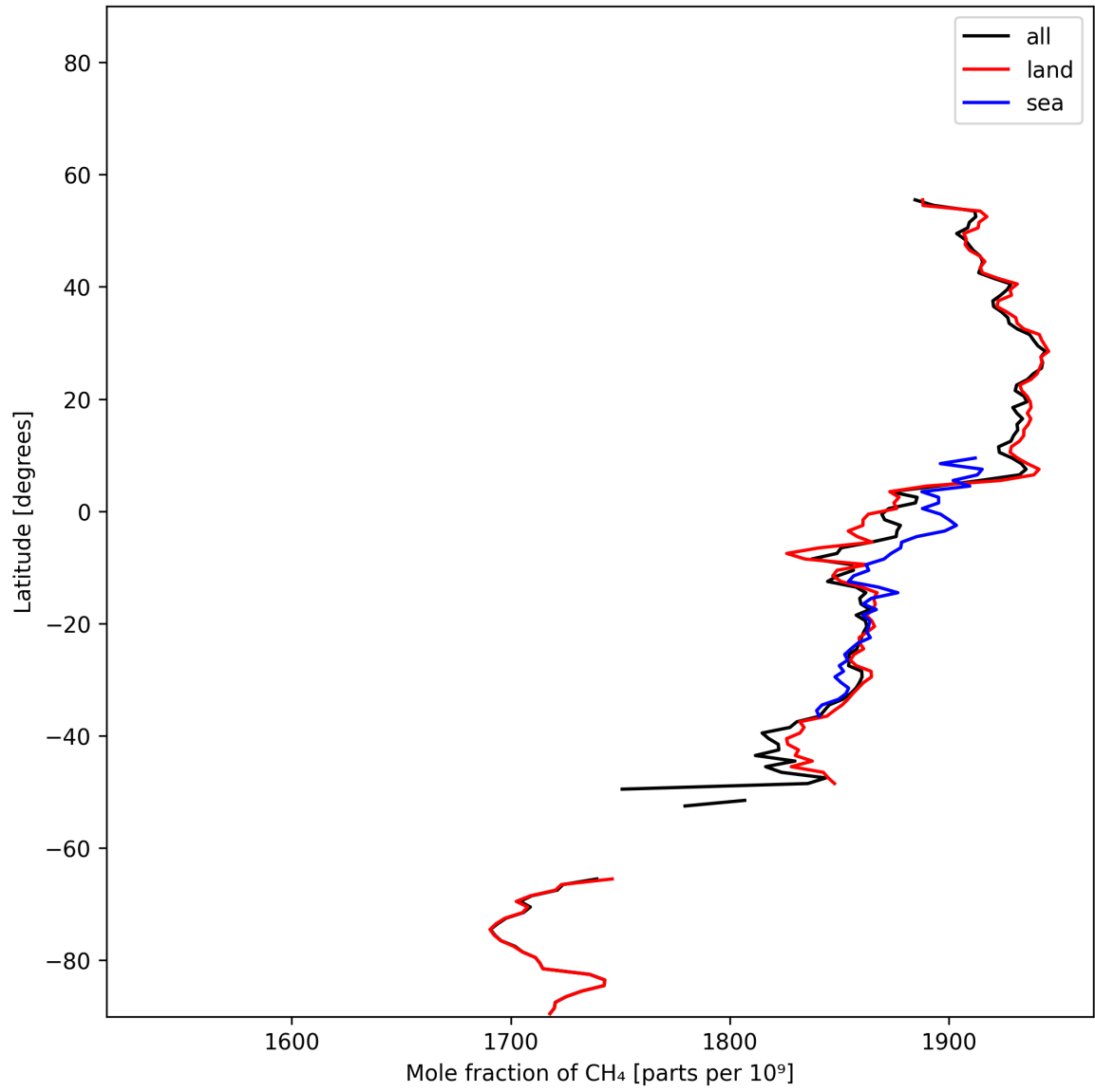
Figure 12: Zonal average of “Mole fraction of \text{CH}_4 ” for 2024-11-18 to 2024-11-20.
