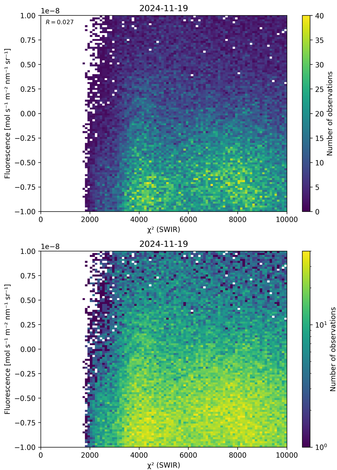
Figure 49: Scatter density plot of “ \chi^2 (SWIR)” against “Fluorescence” for 2024-11-18 to 2024-11-20.
