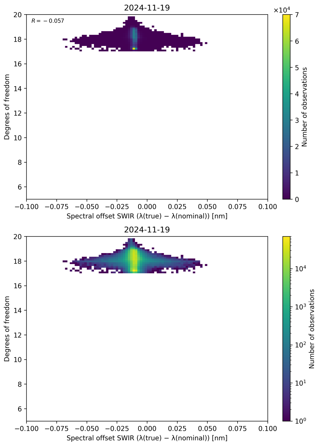
Figure 119: Scatter density plot of “Spectral offset SWIR ( \lambda_{\text{true}} - \lambda_{\text{nominal}} )” against “Degrees of freedom” for 2024-11-18 to 2024-11-20.
