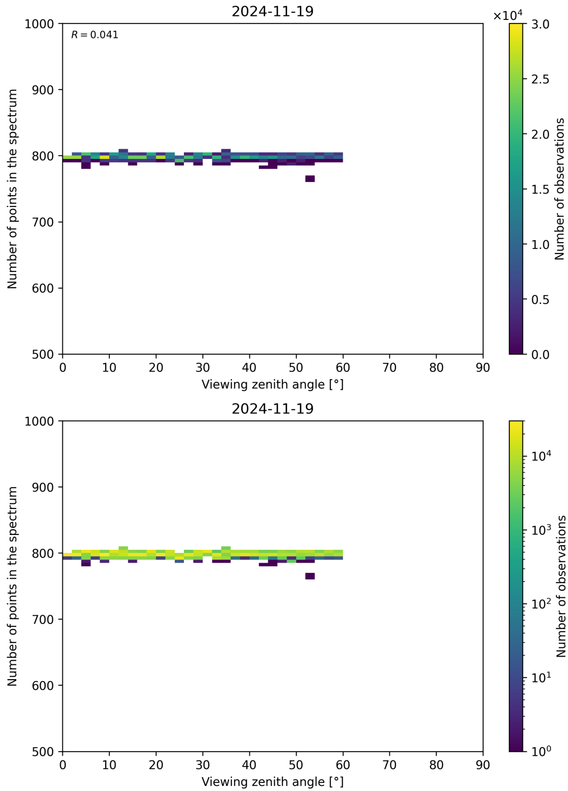
Figure 114: Scatter density plot of “Viewing zenith angle” against “Number of points in the spectrum” for 2024-11-18 to 2024-11-20.
