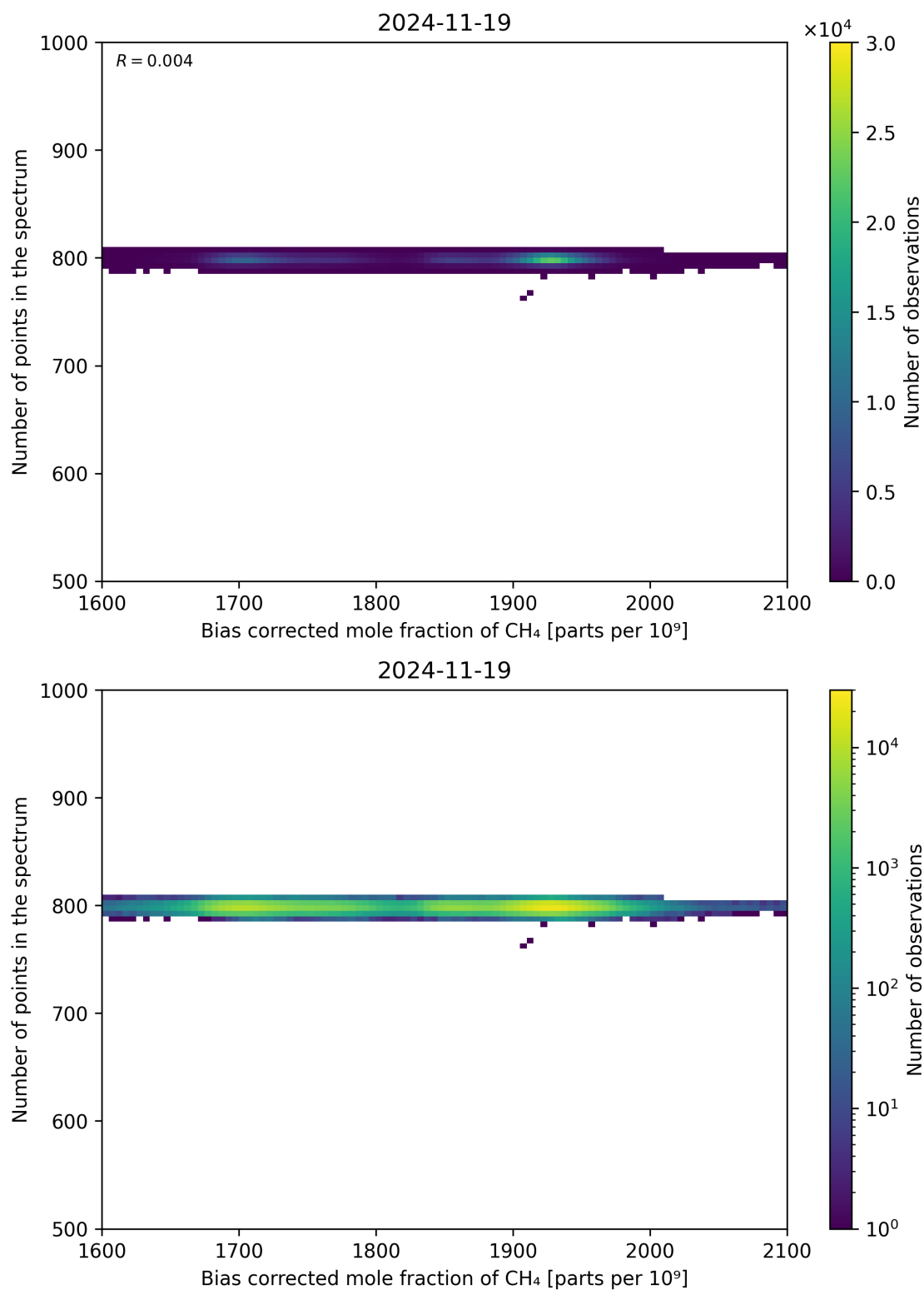
Figure 68: Scatter density plot of “Bias corrected mole fraction of CH 4 ” against “Number of points in the spectrum” for 2024-11-18 to 2024-11-20.
