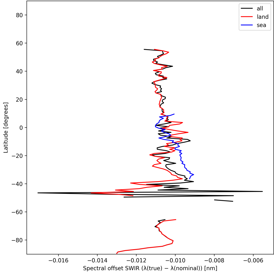
Figure 16: Zonal average of “Spectral offset SWIR ( \lambda_{\text{true}} - \lambda_{\text{nominal}} )” for 2024-11-18 to 2024-11-20.
