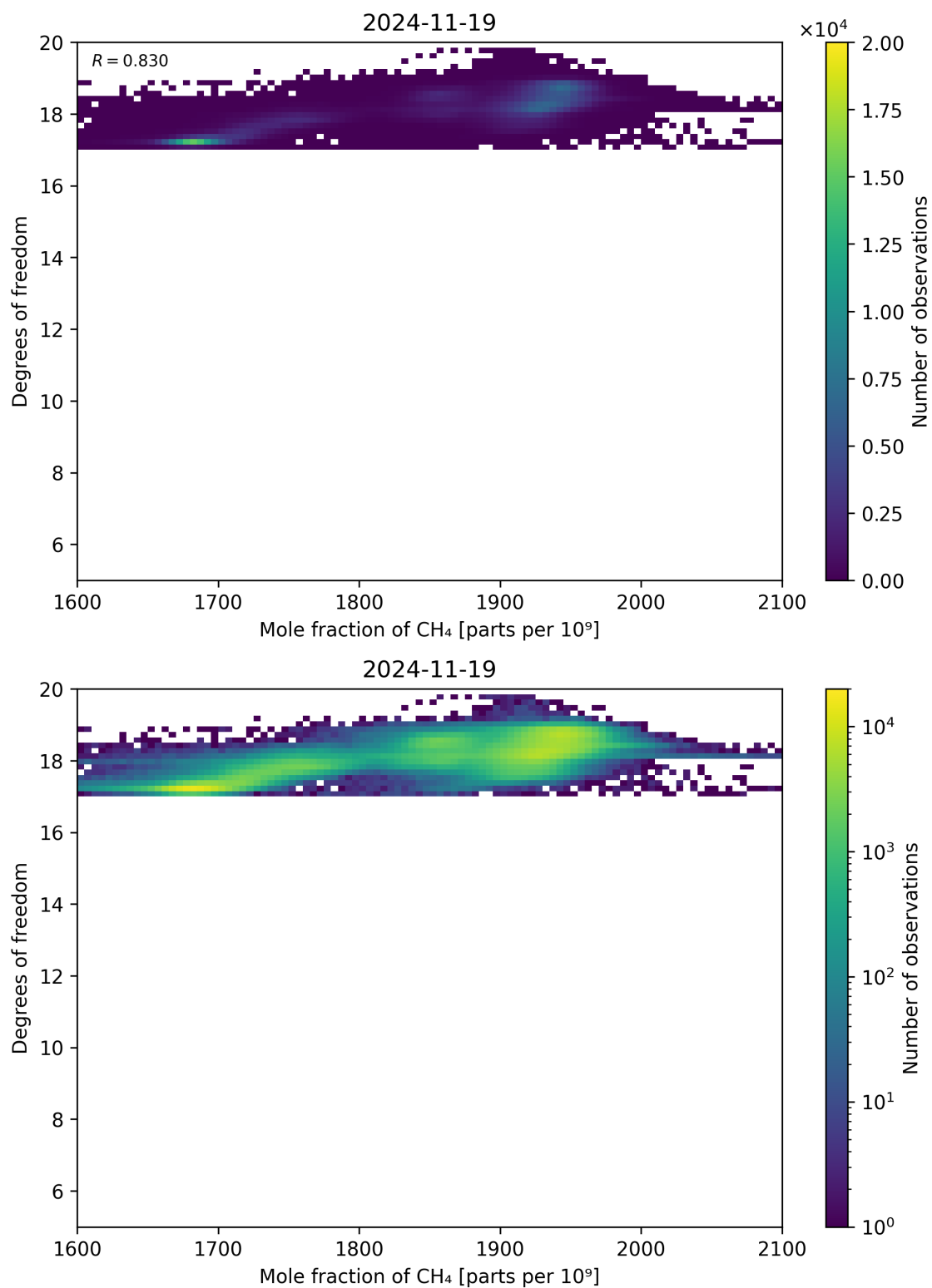
Figure 72: Scatter density plot of “Mole fraction of CH 4 ” against “Degrees of freedom” for 2024-11-18 to 2024-11-20.
