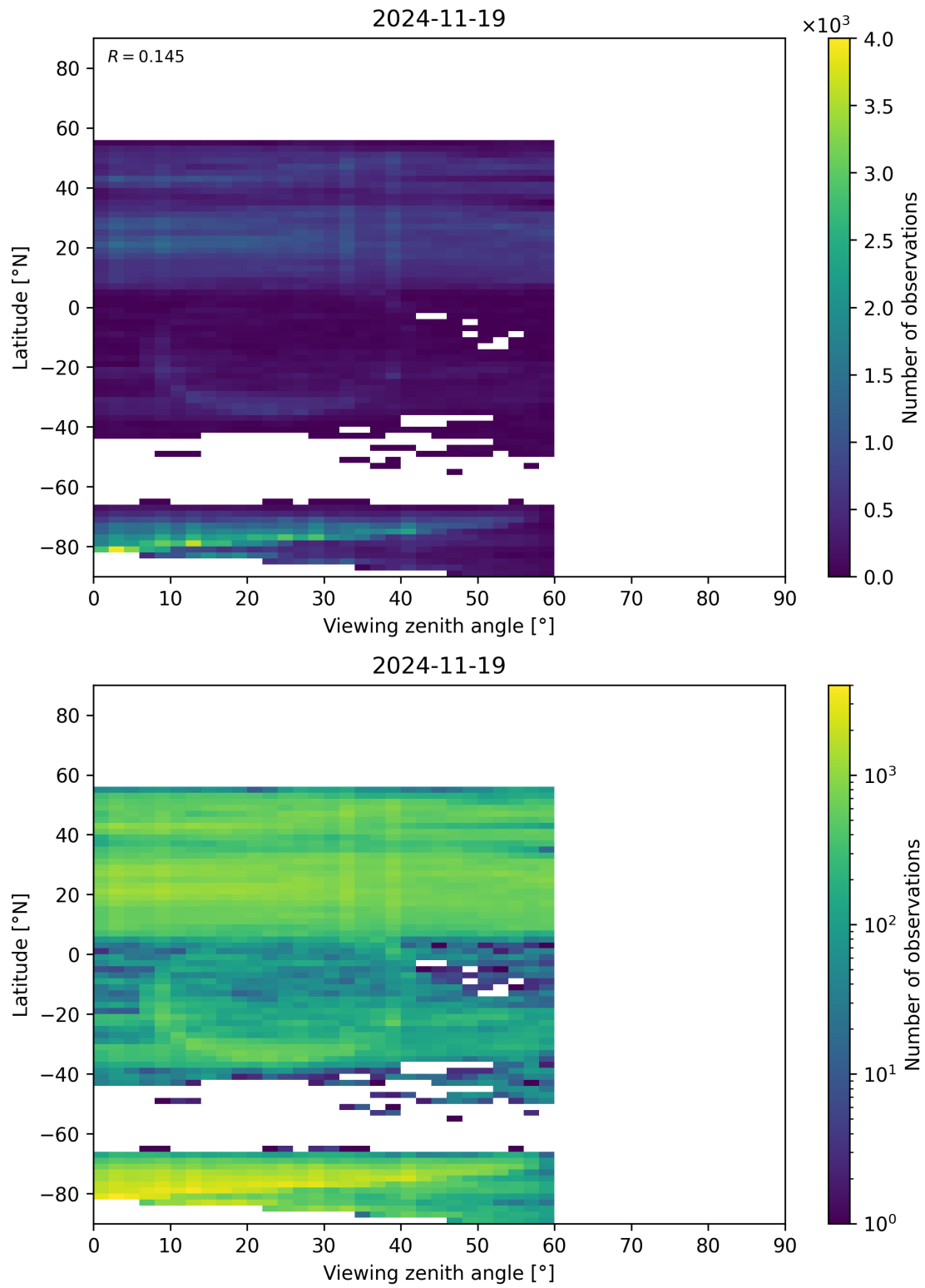
Figure 109: Scatter density plot of “Viewing zenith angle” against “Latitude” for 2024-11-18 to 2024-11-20.
