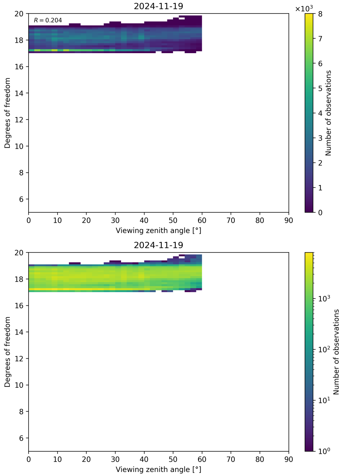
Figure 107: Scatter density plot of “Viewing zenith angle” against “Degrees of freedom” for 2024-11-18 to 2024-11-20.
