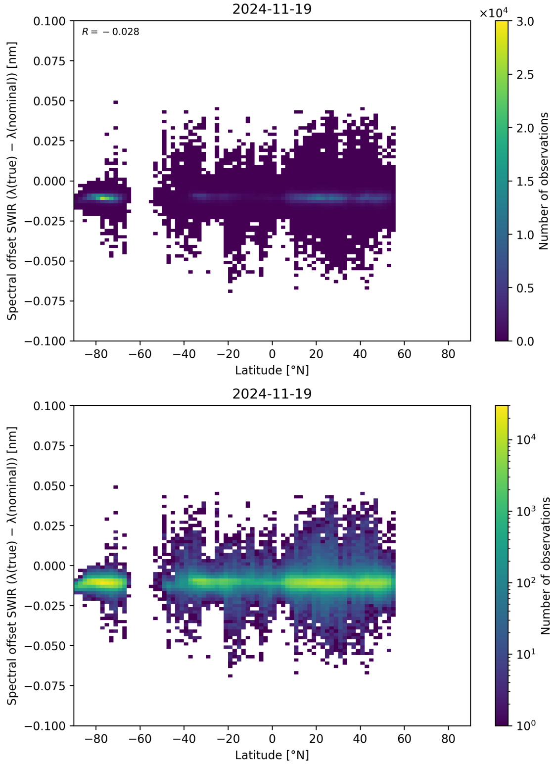
Figure 62: Scatter density plot of “Latitude” against “Spectral offset SWIR ( \lambda_{\text{true}} - \lambda_{\text{nominal}} )” for 2024-11-18 to 2024-11-20.
