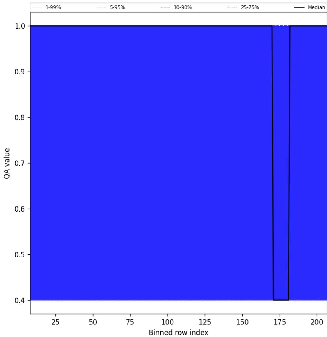
Figure 33: Along track statistics of “QA value” for 2024-11-18 to 2024-11-20
