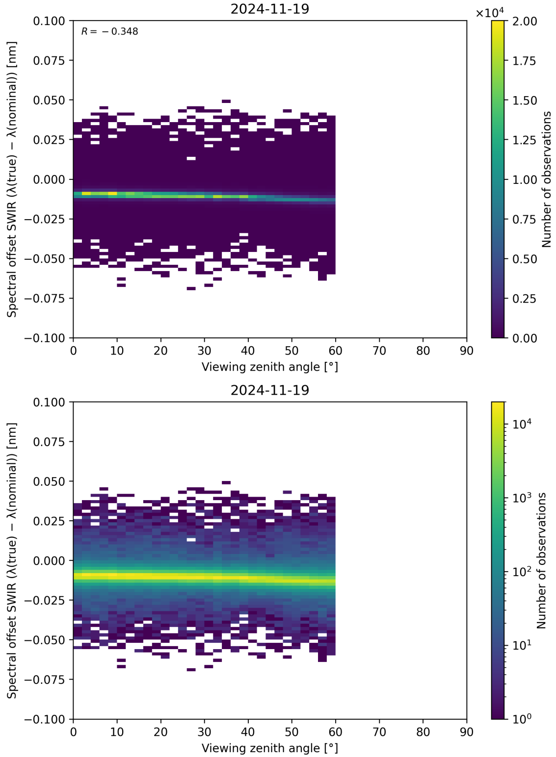
Figure 116: Scatter density plot of “Viewing zenith angle” against “Spectral offset SWIR ( \lambda_{\text{true}} - \lambda_{\text{nominal}} )” for 2024-11-18 to 2024-11-20.
