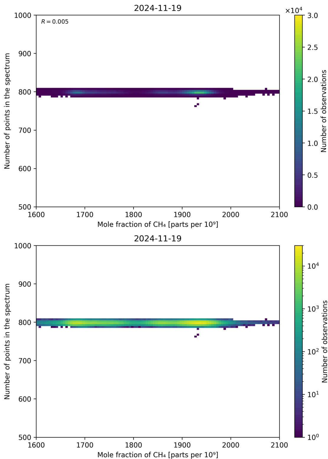
Figure 77: Scatter density plot of “Mole fraction of CH 4 ” against “Number of points in the spectrum” for 2024-11-18 to 2024-11-20.
