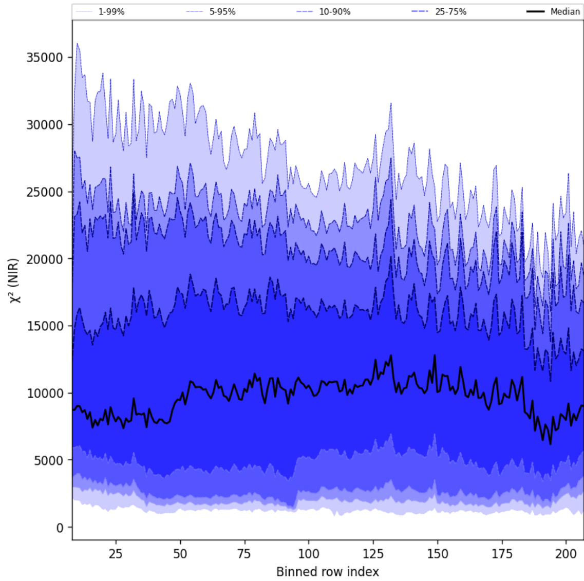
Figure 40: Along track statistics of “ \chi^2 (NIR)” for 2024-11-18 to 2024-11-20
