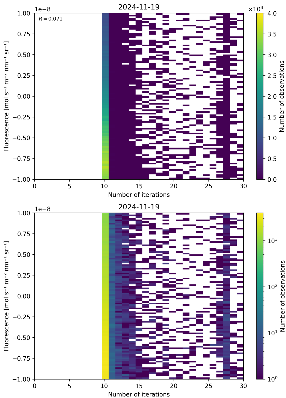
Figure 87: Scatter density plot of “Number of iterations” against “Fluorescence” for 2024-11-18 to 2024-11-20.
