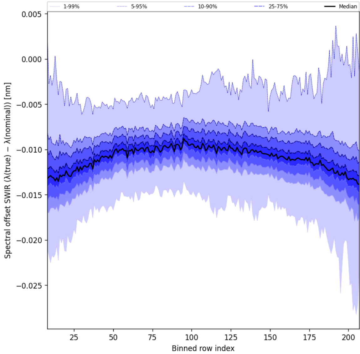
Figure 38: Along track statistics of “Spectral offset SWIR ( \lambda_{\text{true}} - \lambda_{\text{nominal}} )” for 2024-11-18 to 2024-11-20
