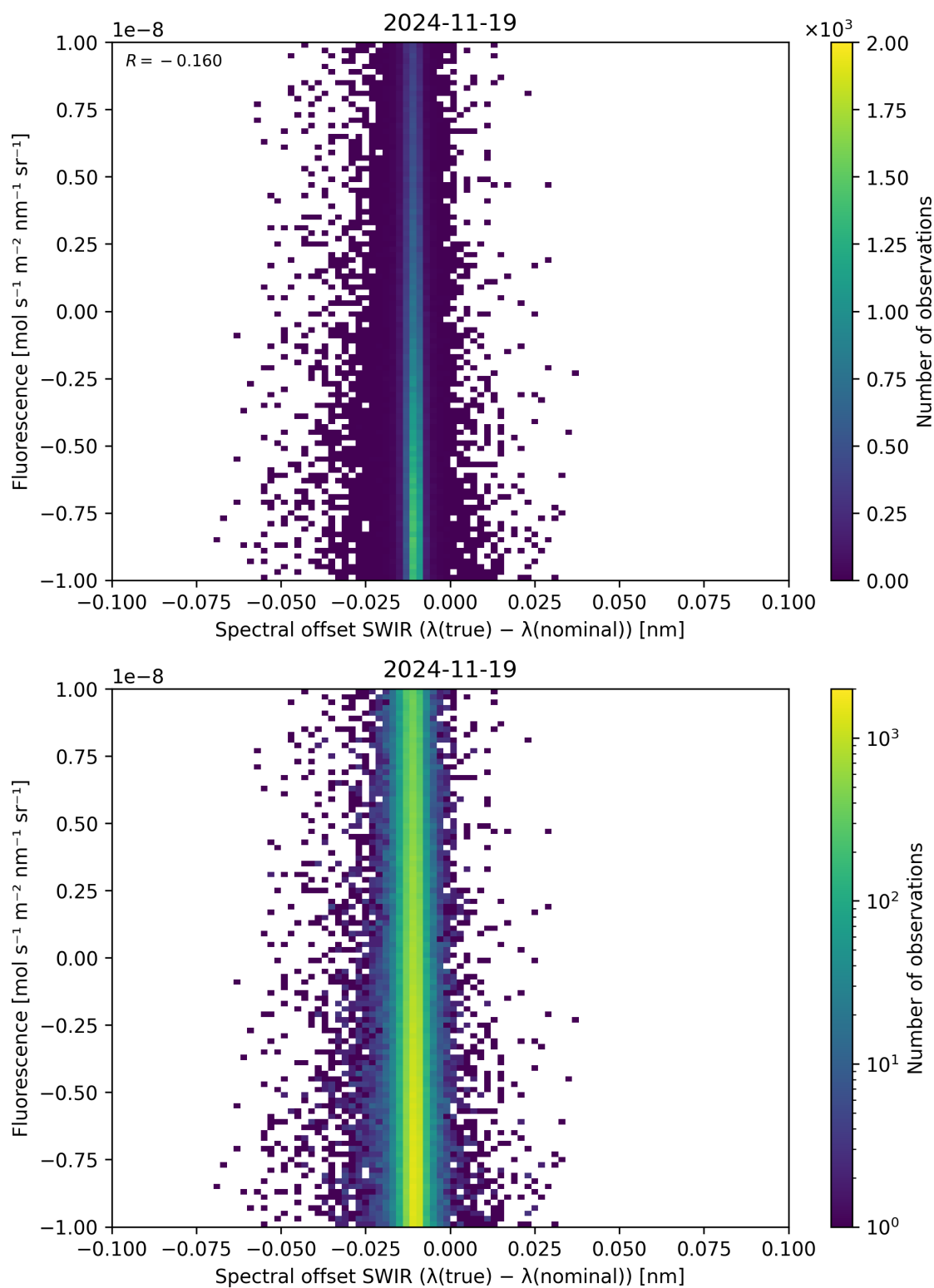
Figure 120: Scatter density plot of “Spectral offset SWIR ( \lambda_{\text{true}} - \lambda_{\text{nominal}} )” against “Fluorescence” for 2024-11-18 to 2024-11-20.
