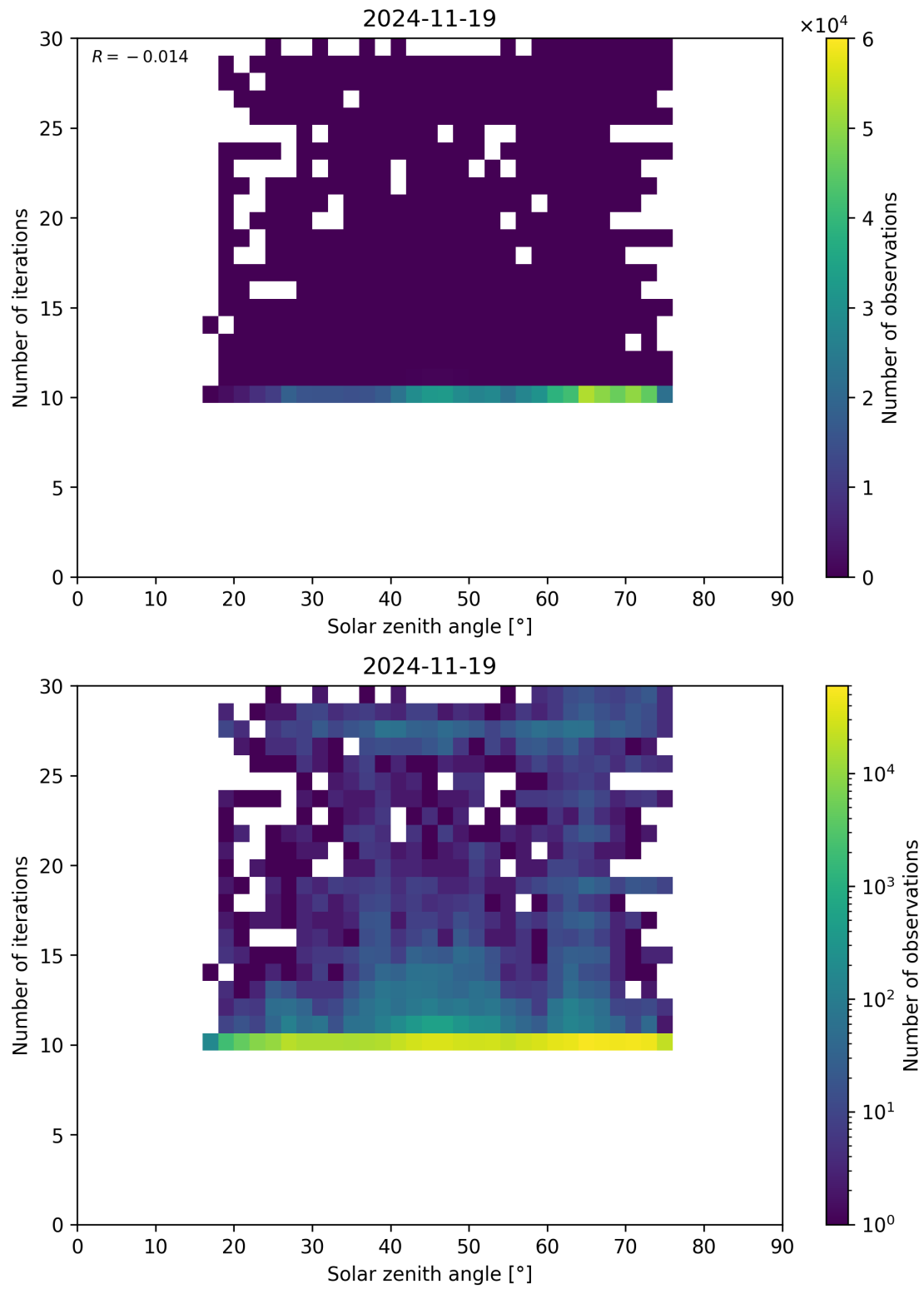
Figure 102: Scatter density plot of “Solar zenith angle” against “Number of iterations” for 2024-11-18 to 2024-11-20.
