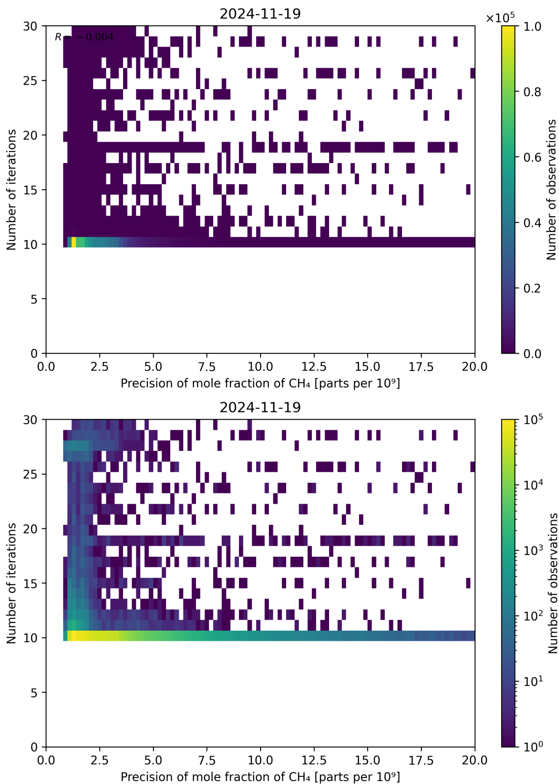
Figure 83: Scatter density plot of “Precision of mole fraction of CH 4 ” against “Number of iterations” for 2024-11-18 to 2024-11-20.
