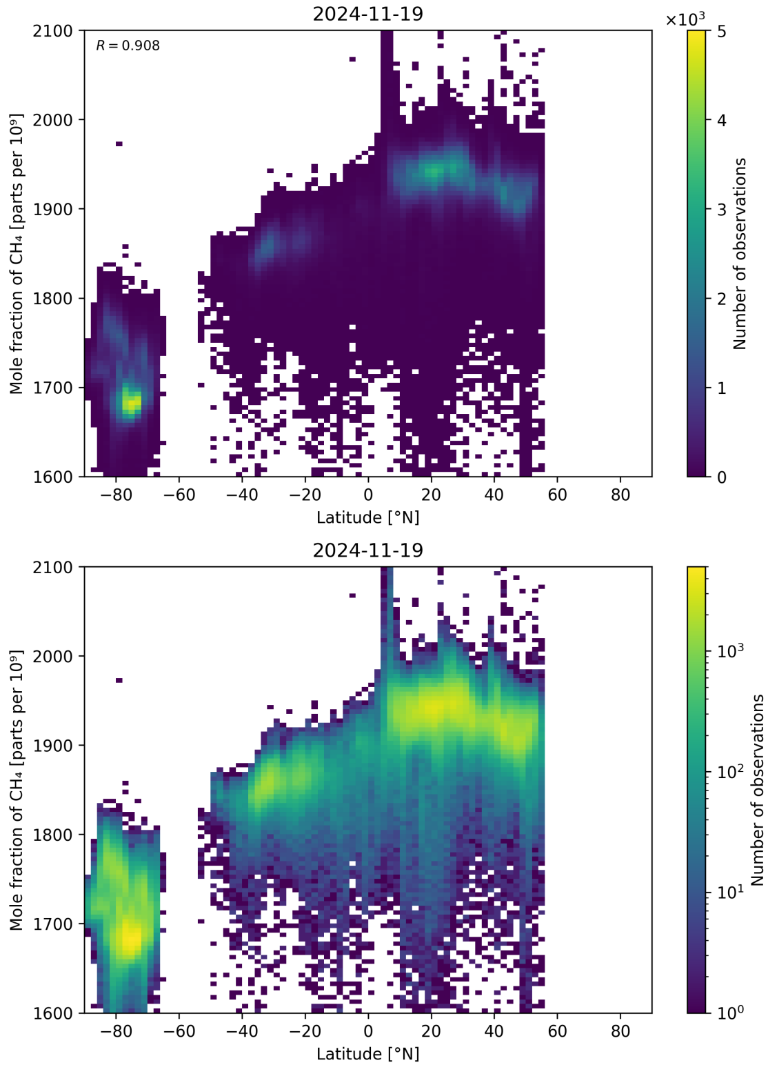
Figure 57: Scatter density plot of “Latitude” against “Mole fraction of CH 4 ” for 2024-11-18 to 2024-11-20.
