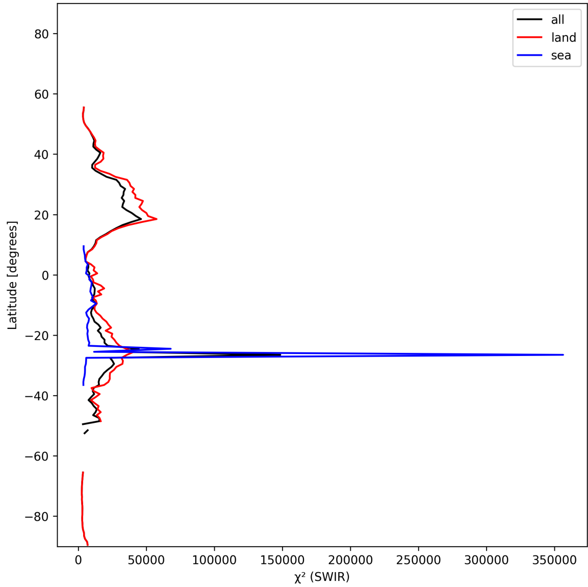
Figure 17: Zonal average of “ \chi^2 (SWIR)” for 2024-11-18 to 2024-11-20.
