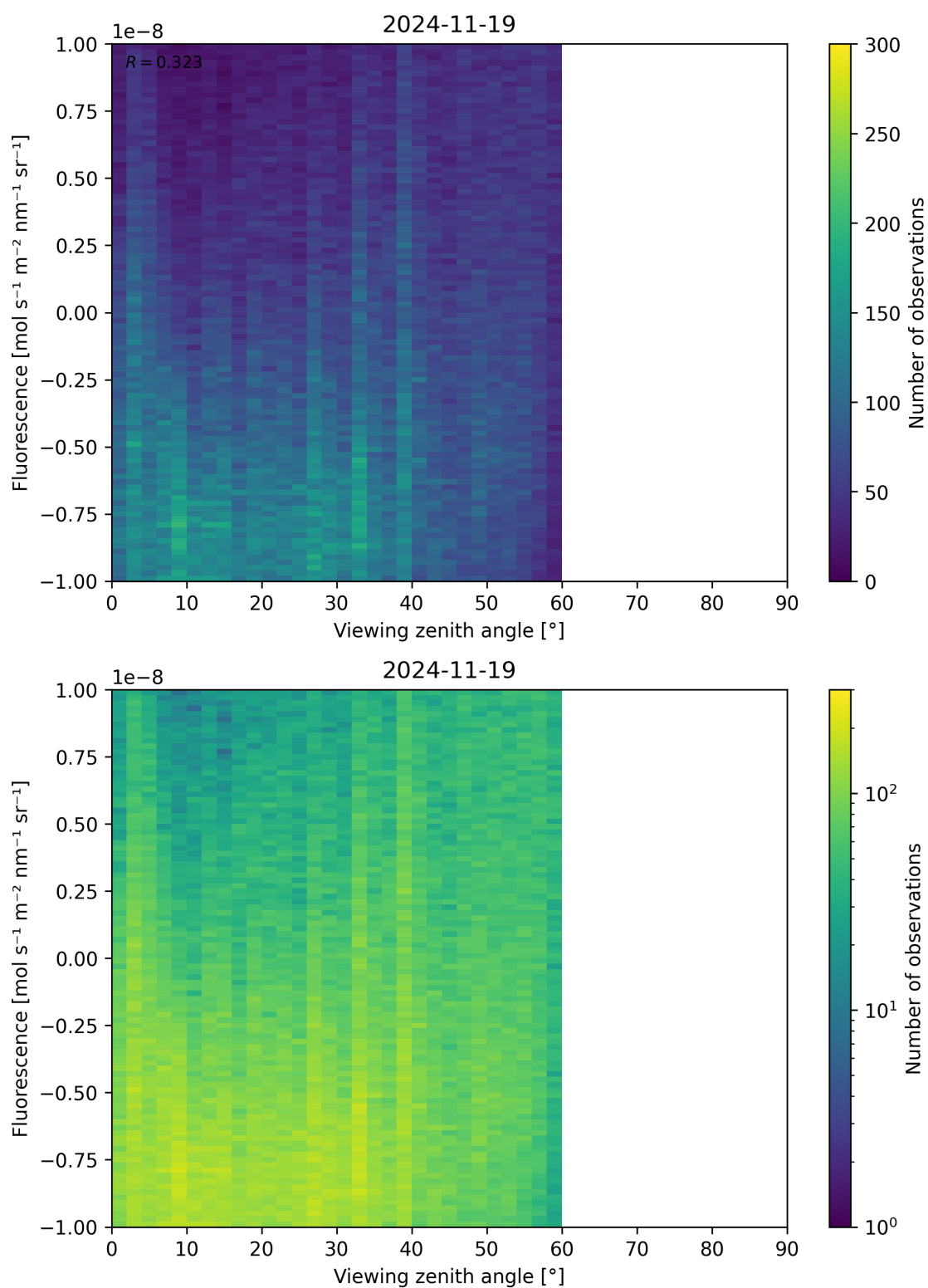
Figure 108: Scatter density plot of “Viewing zenith angle” against “Fluorescence” for 2024-11-18 to 2024-11-20.
