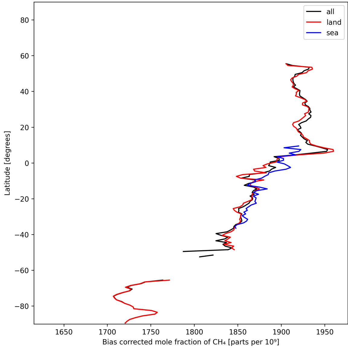
Figure 14: Zonal average of “Bias corrected mole fraction of CH 4 ” for 2024-11-18 to 2024-11-20.
