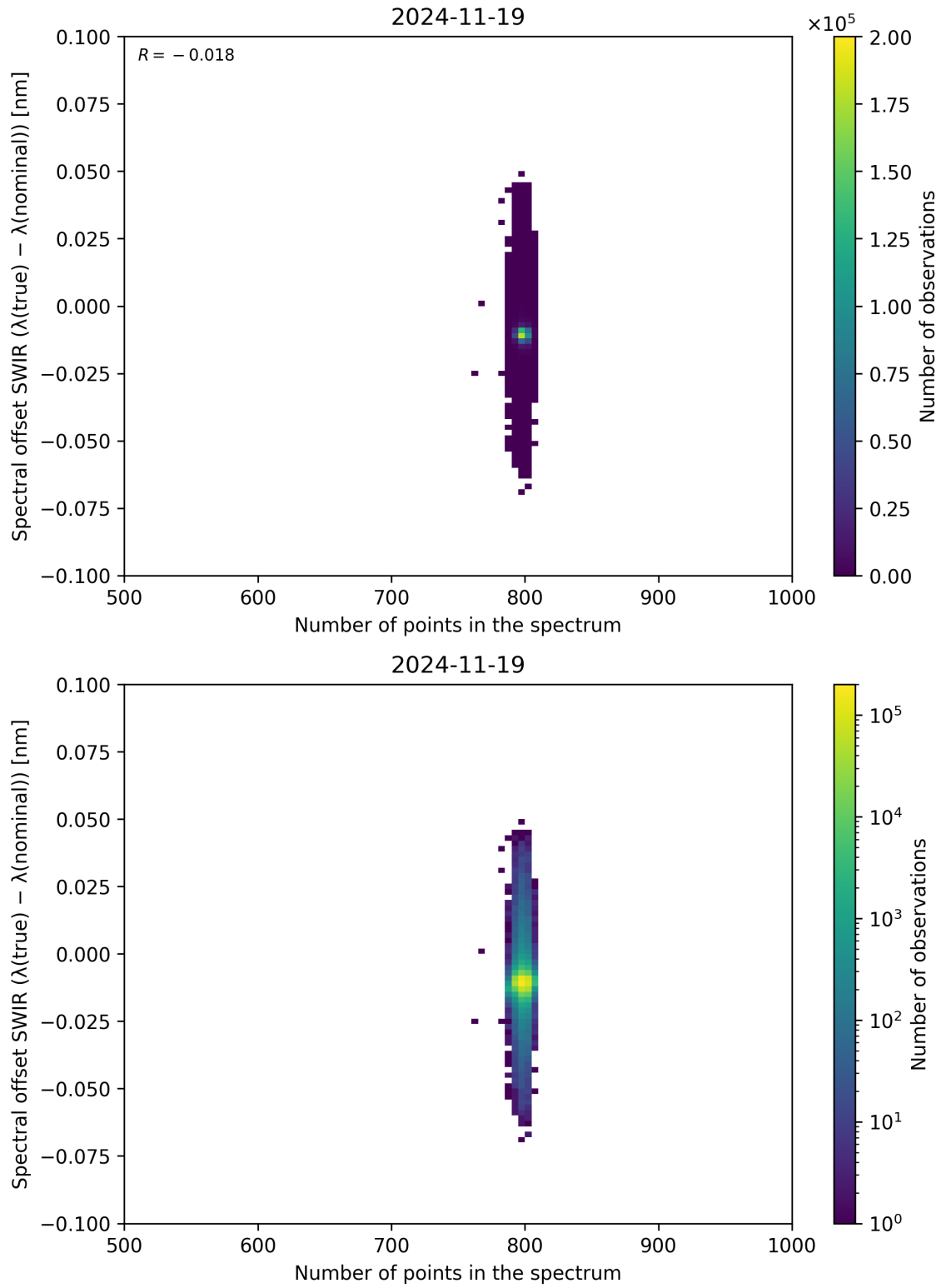
Figure 93: Scatter density plot of “Number of points in the spectrum” against “Spectral offset SWIR ( \lambda_{\text{true}} - \lambda_{\text{nominal}} )” for 2024-11-18 to 2024-11-20.
