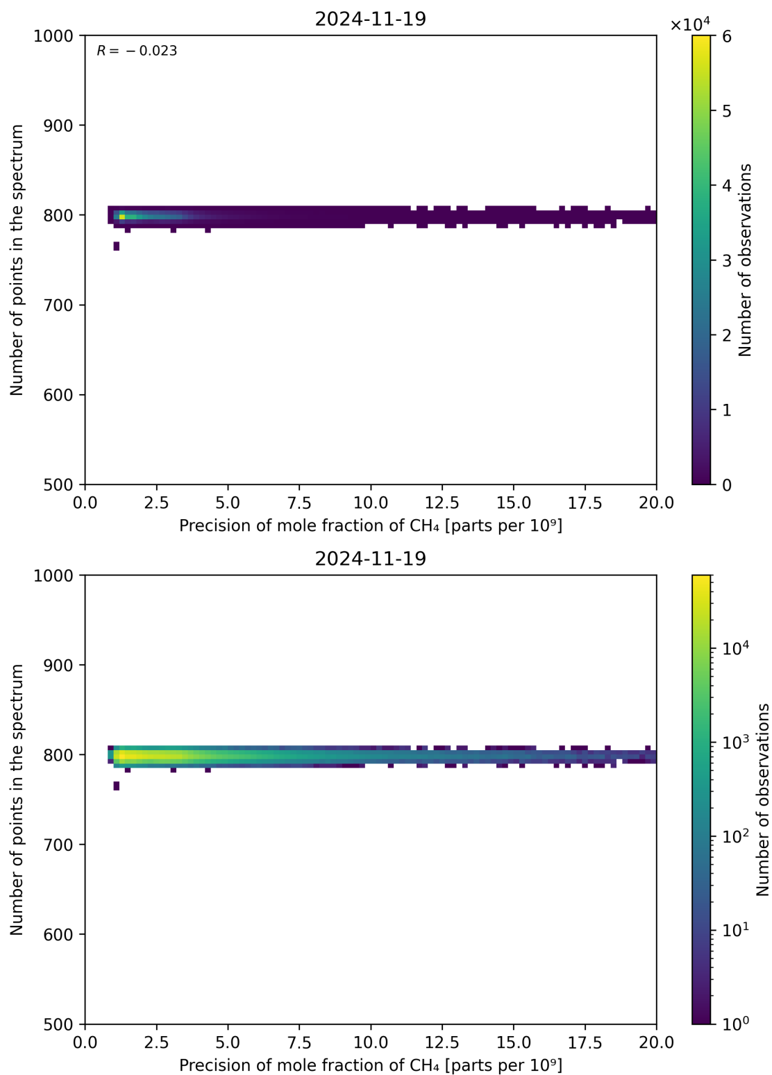
Figure 84: Scatter density plot of “Precision of mole fraction of CH 4 ” against “Number of points in the spectrum” for 2024-11-18 to 2024-11-20.
