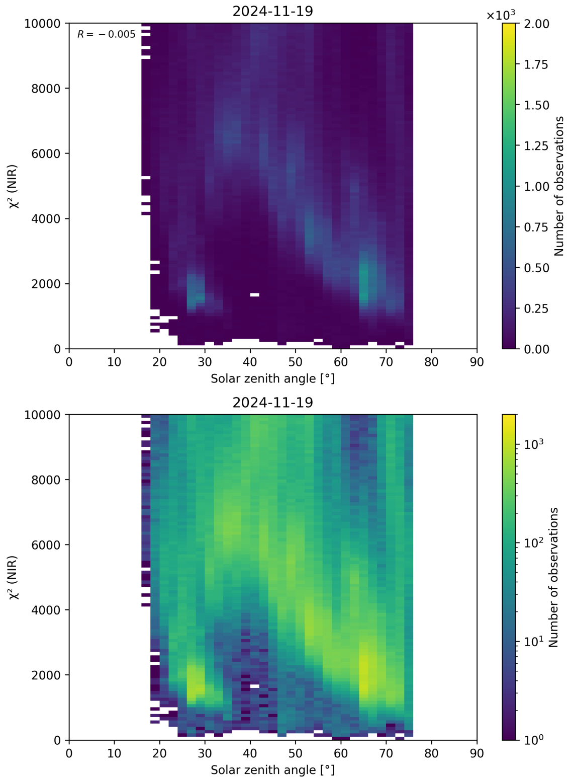
Figure 94: Scatter density plot of “Solar zenith angle” against “ \chi^2 (NIR)” for 2024-11-18 to 2024-11-20.
