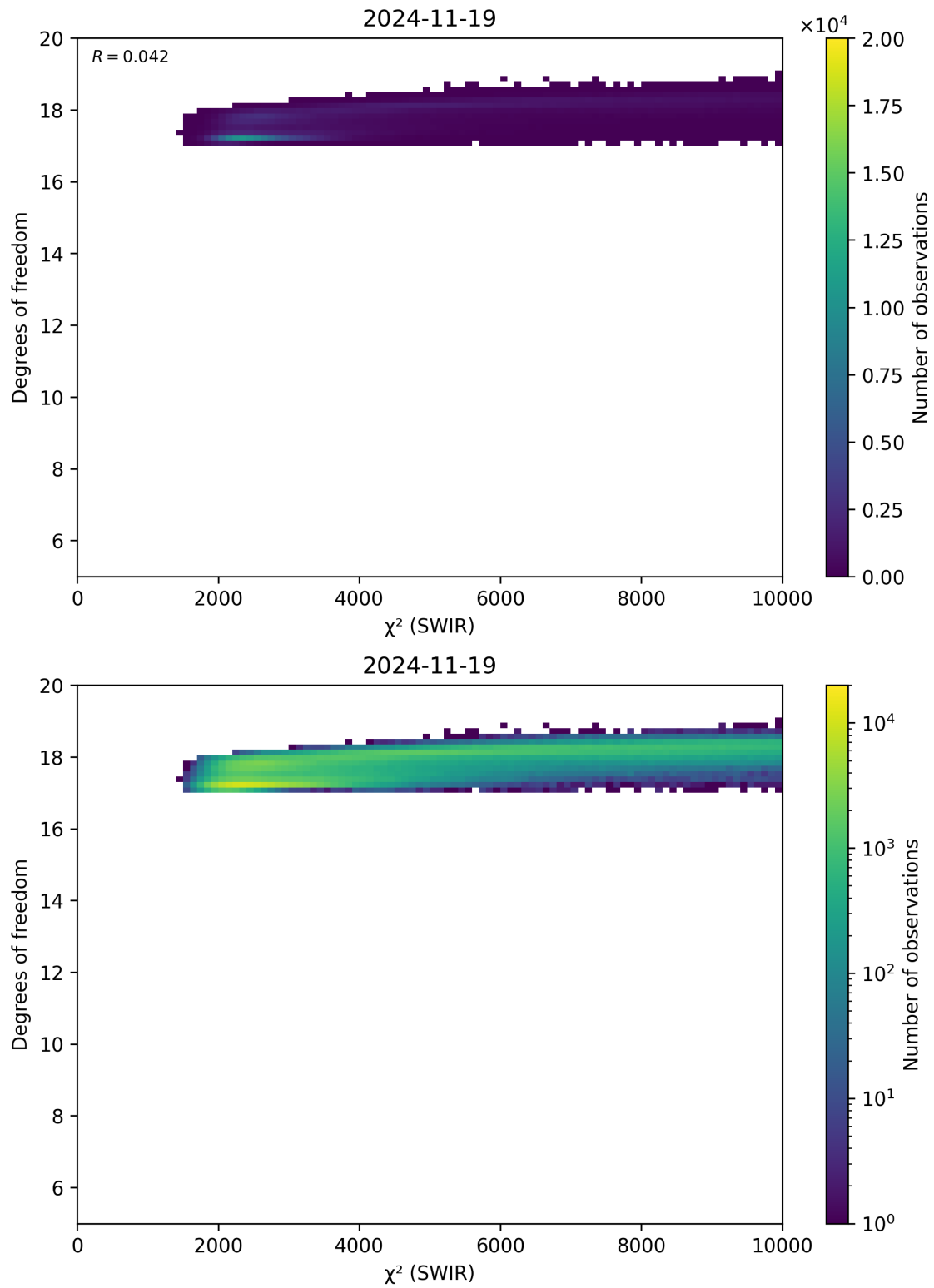
Figure 48: Scatter density plot of “ \chi^2 (SWIR)” against “Degrees of freedom” for 2024-11-18 to 2024-11-20.
