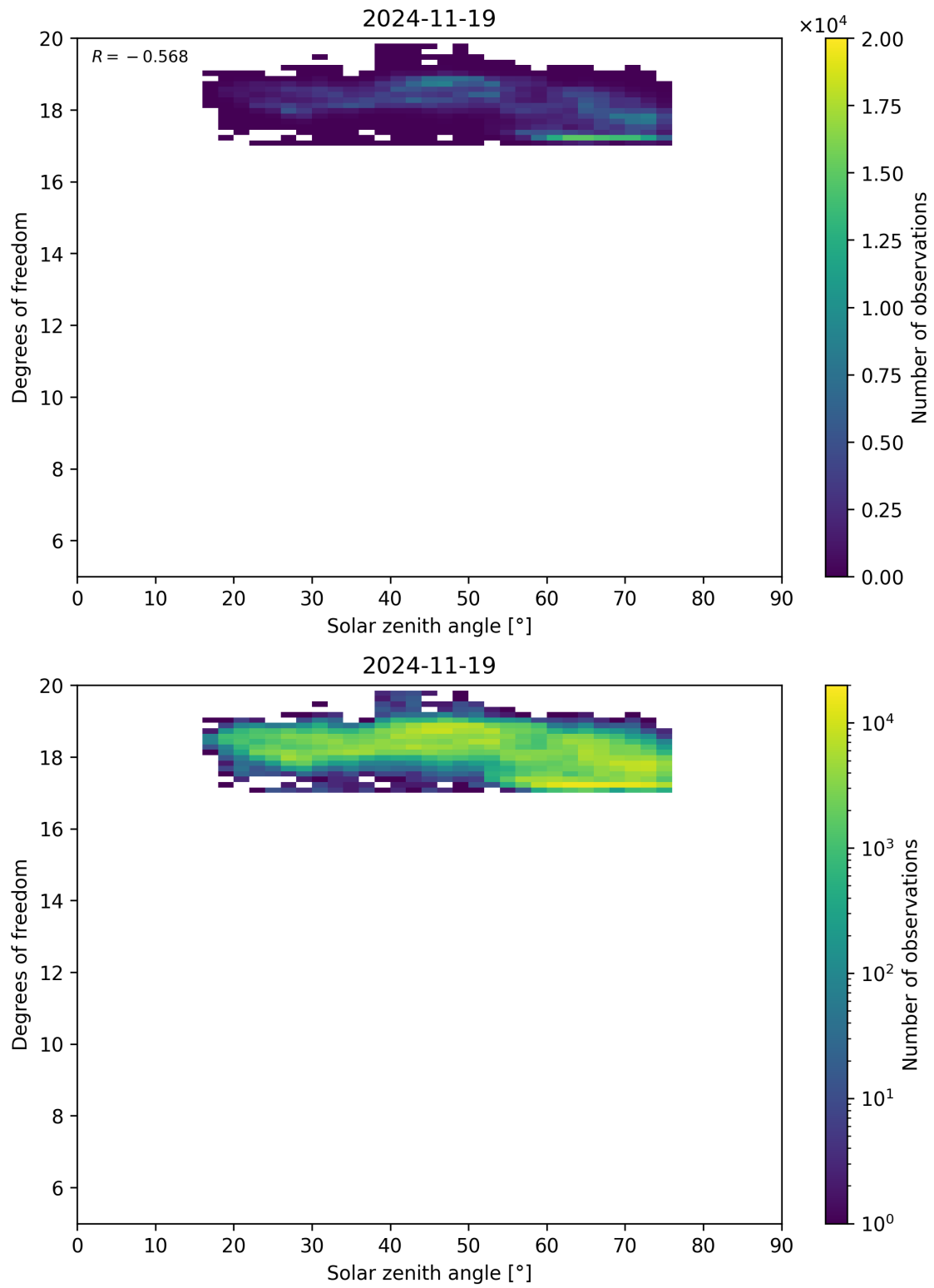
Figure 96: Scatter density plot of “Solar zenith angle” against “Degrees of freedom” for 2024-11-18 to 2024-11-20.
