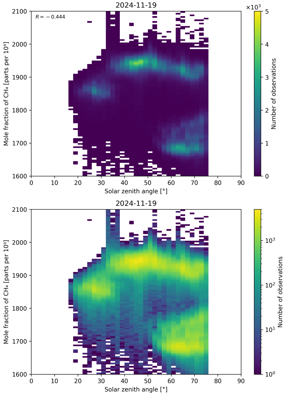
Figure 99: Scatter density plot of “Solar zenith angle” against “Mole fraction of CH 4 ” for 2024-11-18 to 2024-11-20.
