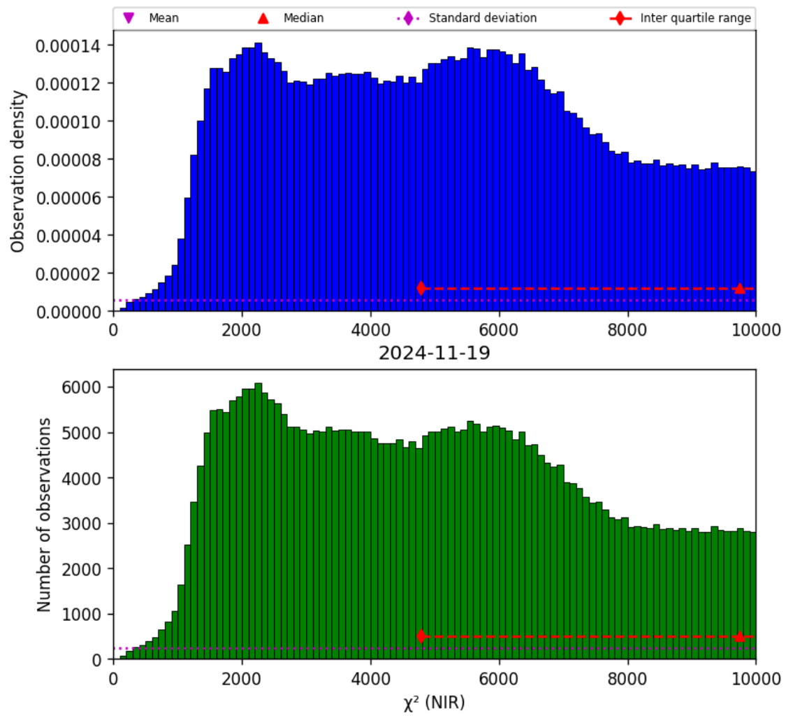
Figure 29: Histogram of “ \chi^2 (NIR)” for 2024-11-18 to 2024-11-20
