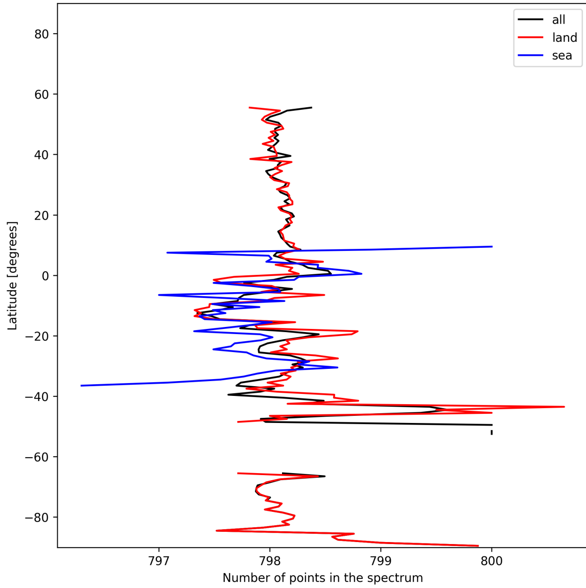
Figure 15: Zonal average of “Number of points in the spectrum” for 2024-11-18 to 2024-11-20.
