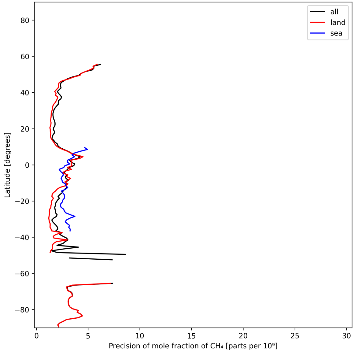
Figure 13: Zonal average of “Precision of mole fraction of CH 4 ” for 2024-11-18 to 2024-11-20.
