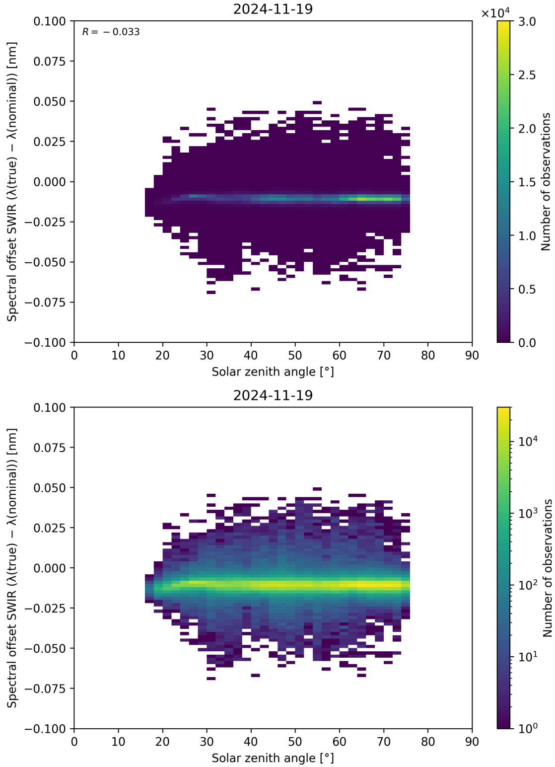
Figure 104: Scatter density plot of “Solar zenith angle” against “Spectral offset SWIR ( \lambda_{\text{true}} - \lambda_{\text{nominal}} )” for 2024-11-18 to 2024-11-20.
