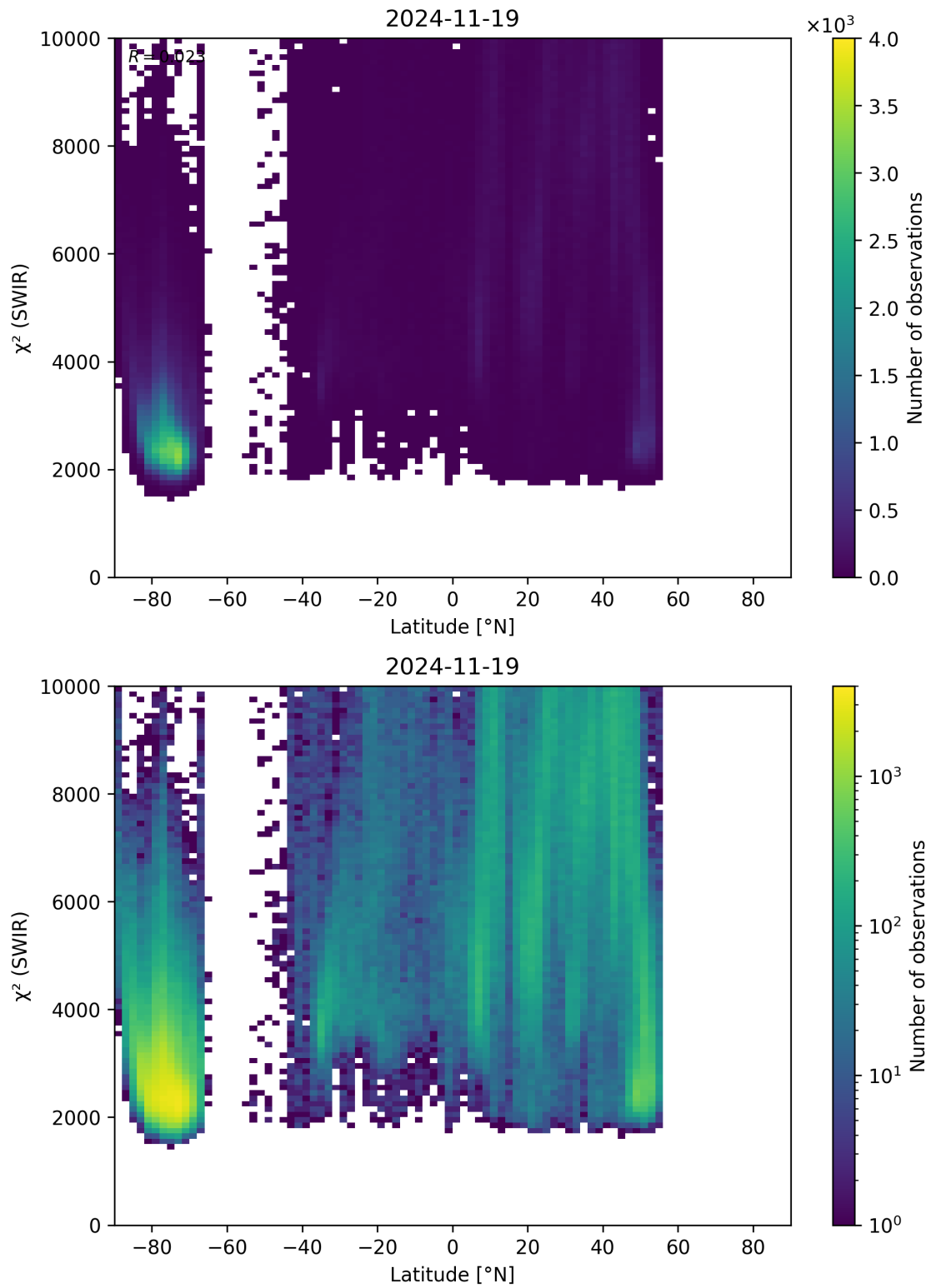
Figure 54: Scatter density plot of “Latitude” against “ \chi^2 (SWIR)” for 2024-11-18 to 2024-11-20.
