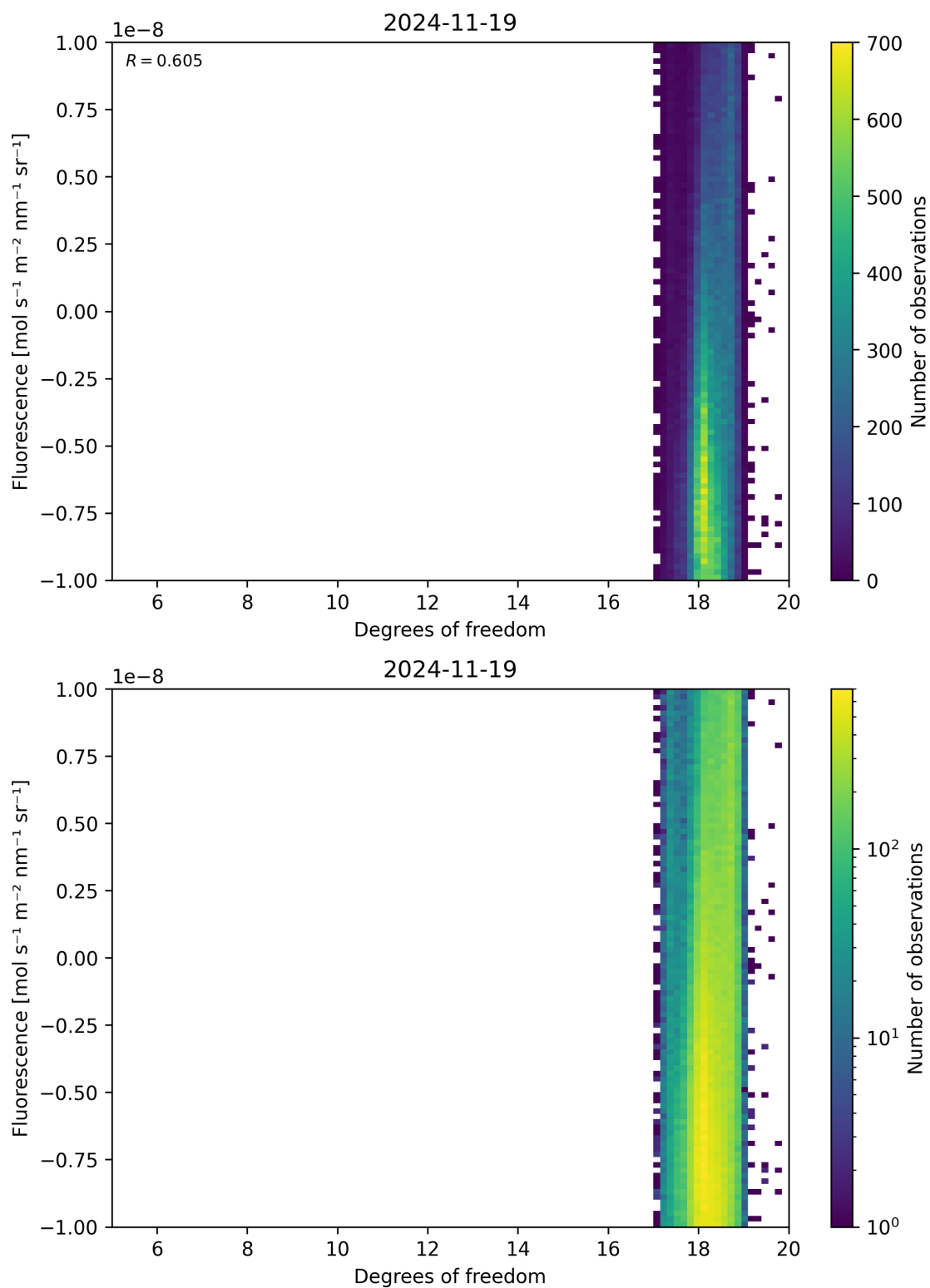
Figure 51: Scatter density plot of “Degrees of freedom” against “Fluorescence” for 2024-11-18 to 2024-11-20.
