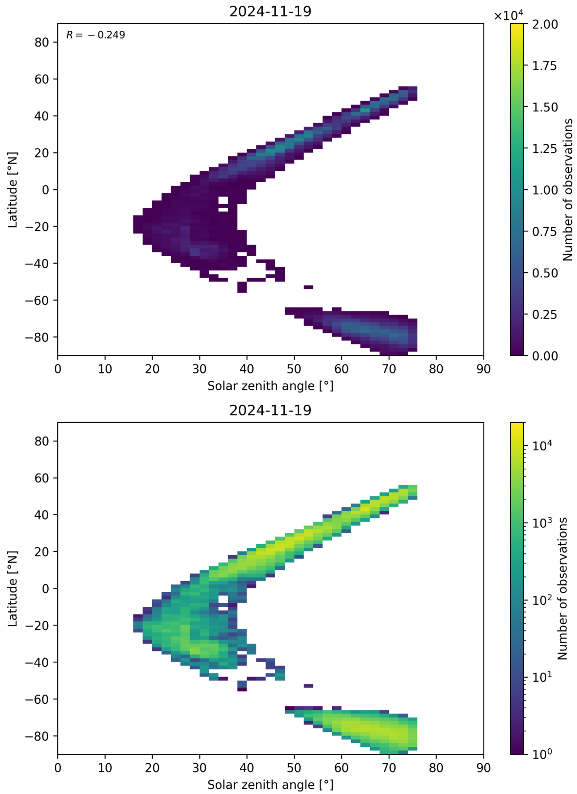
Figure 98: Scatter density plot of “Solar zenith angle” against “Latitude” for 2024-11-18 to 2024-11-20.
