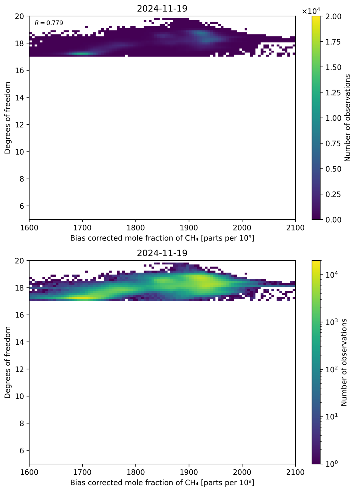
Figure 65: Scatter density plot of “Bias corrected mole fraction of CH 4 ” against “Degrees of freedom” for 2024-11-18 to 2024-11-20.
