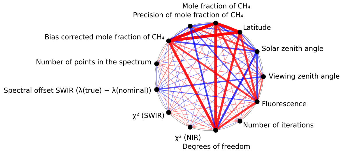
Figure 1: Map of correlation graph for 2024-11-18 to 2024-11-20.
