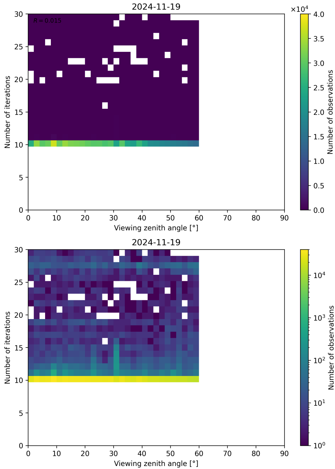
Figure 113: Scatter density plot of “Viewing zenith angle” against “Number of iterations” for 2024-11-18 to 2024-11-20.
