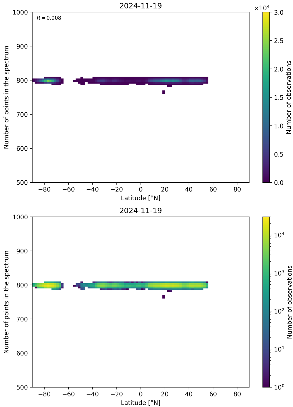
Figure 61: Scatter density plot of “Latitude” against “Number of points in the spectrum” for 2024-11-18 to 2024-11-20.
