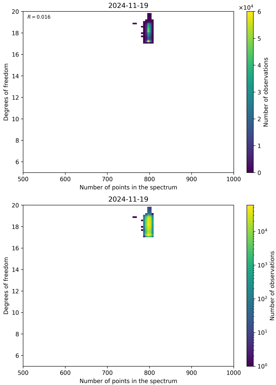
Figure 90: Scatter density plot of “Number of points in the spectrum” against “Degrees of freedom” for 2024-11-18 to 2024-11-20.
