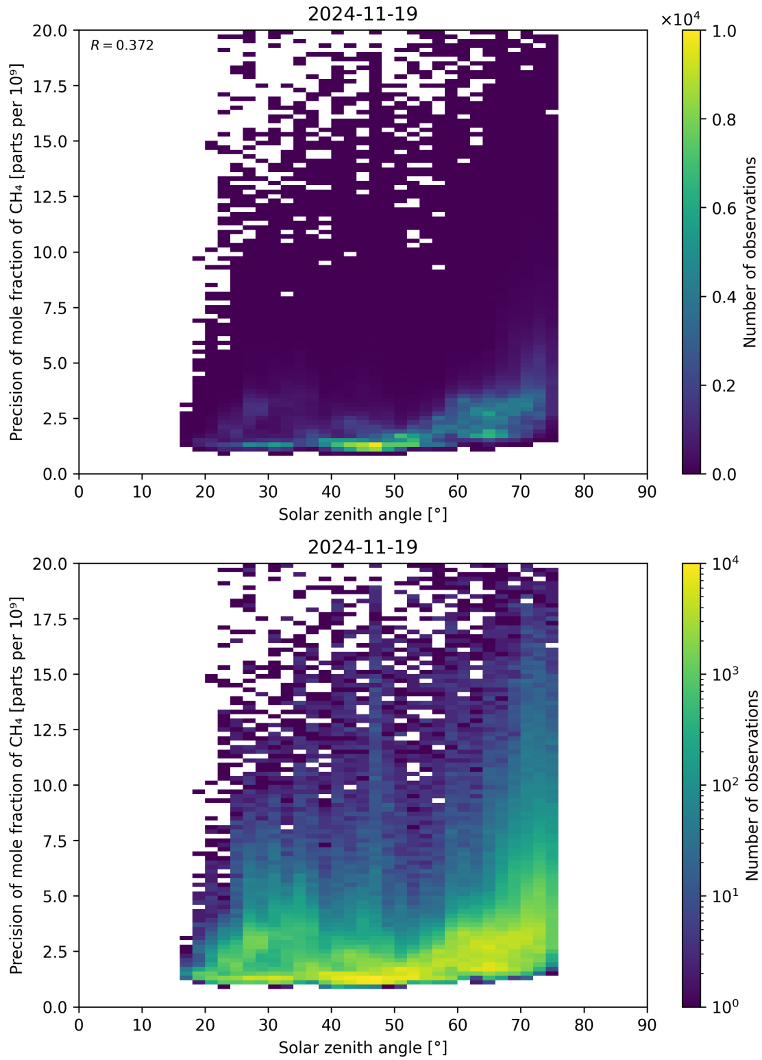
Figure 101: Scatter density plot of “Solar zenith angle” against “Precision of mole fraction of \text{CH}_4 ” for 2024-11-18 to 2024-11-20.
