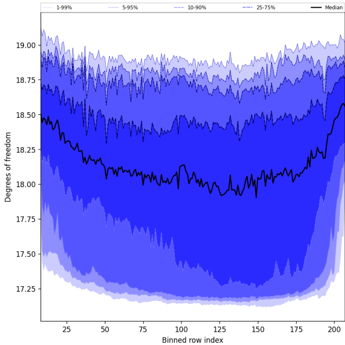
Figure 41: Along track statistics of “Degrees of freedom” for 2024-11-18 to 2024-11-20
