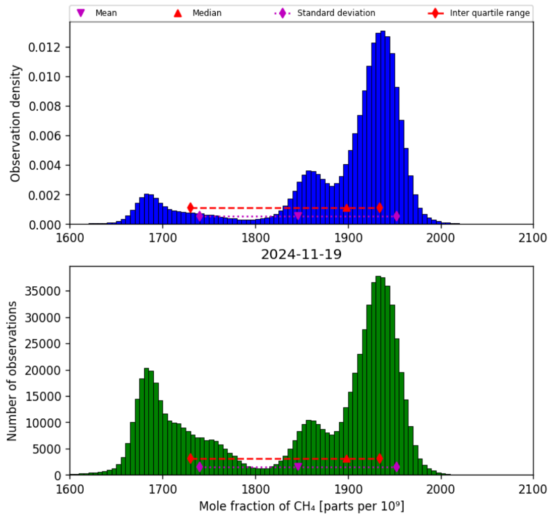
Figure 23: Histogram of “Mole fraction of CH 4 ” for 2024-11-18 to 2024-11-20
