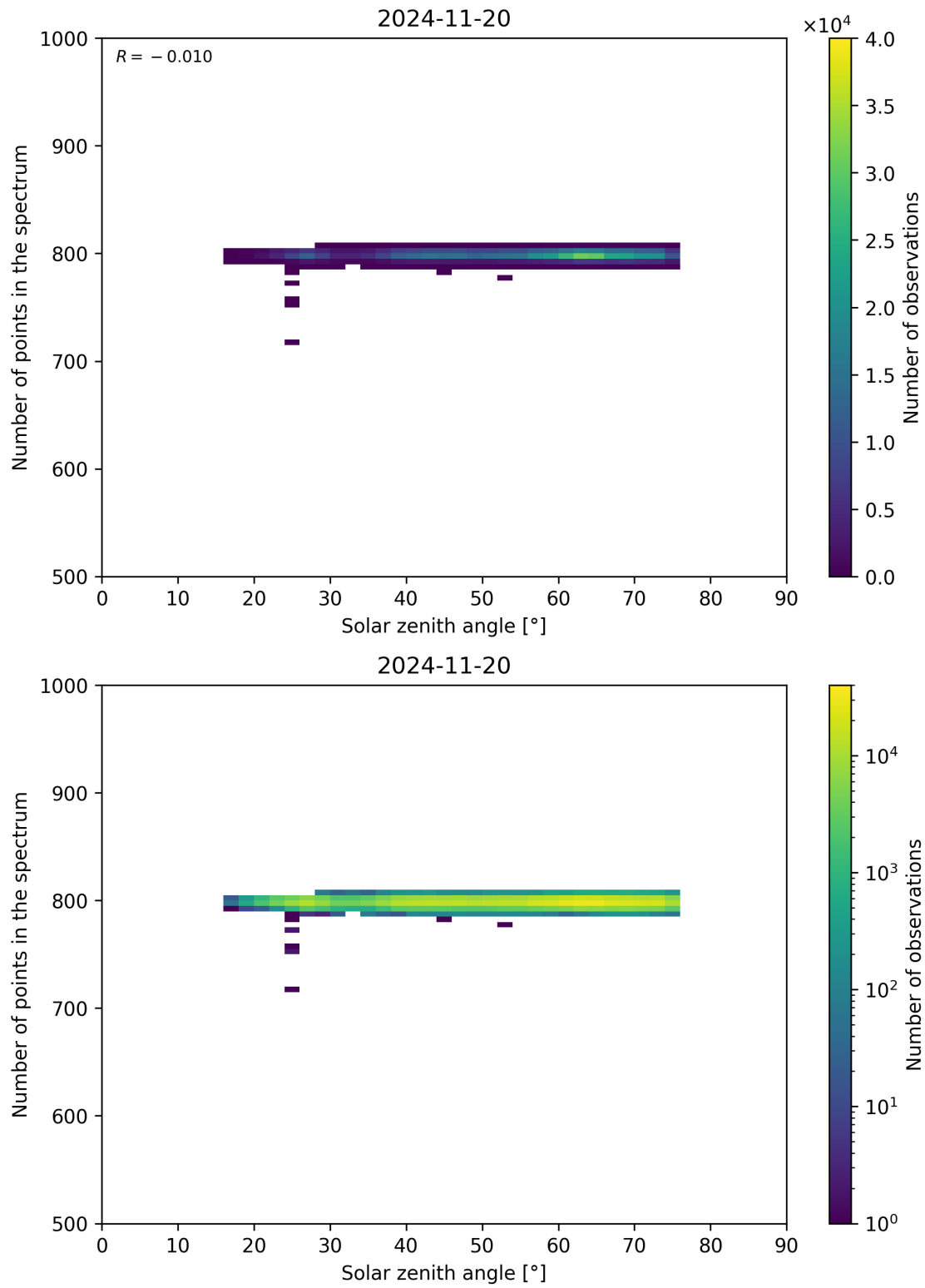
Figure 103: Scatter density plot of “Solar zenith angle” against “Number of points in the spectrum” for 2024-11-20 to 2024-11-21.
