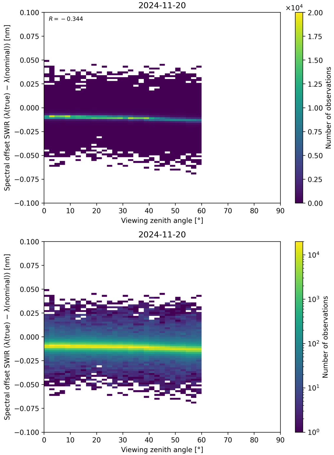
Figure 116: Scatter density plot of “Viewing zenith angle” against “Spectral offset SWIR ( \lambda_{\text{true}} - \lambda_{\text{nominal}} )” for 2024-11-20 to 2024-11-21.
