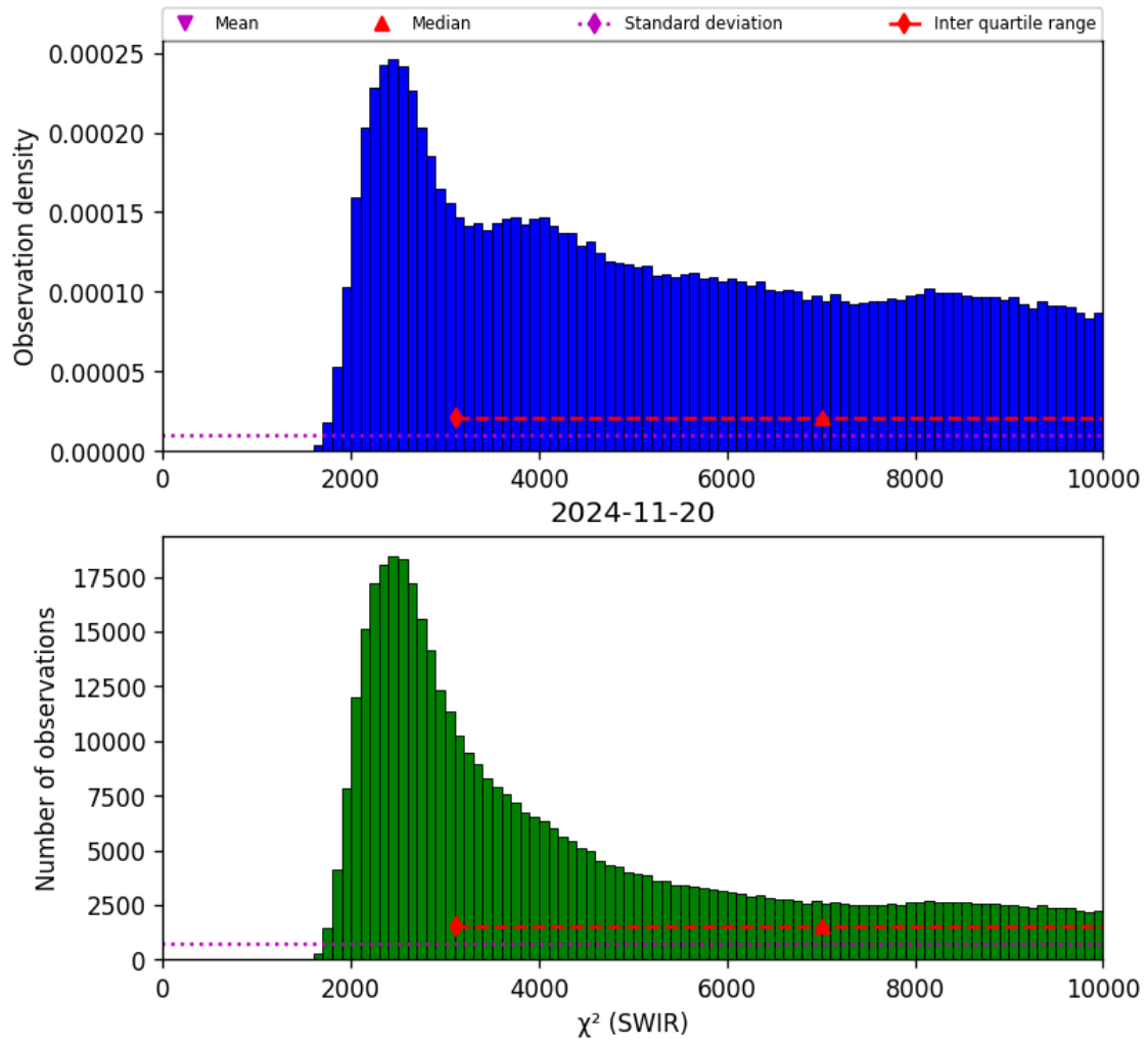
Figure 28: Histogram of “ \chi^2 (SWIR)” for 2024-11-20 to 2024-11-21
