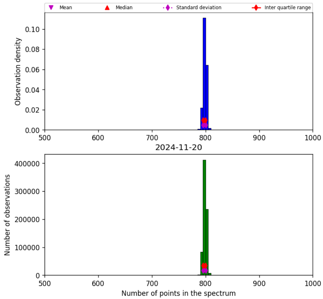
Figure 26: Histogram of “Number of points in the spectrum” for 2024-11-20 to 2024-11-21
