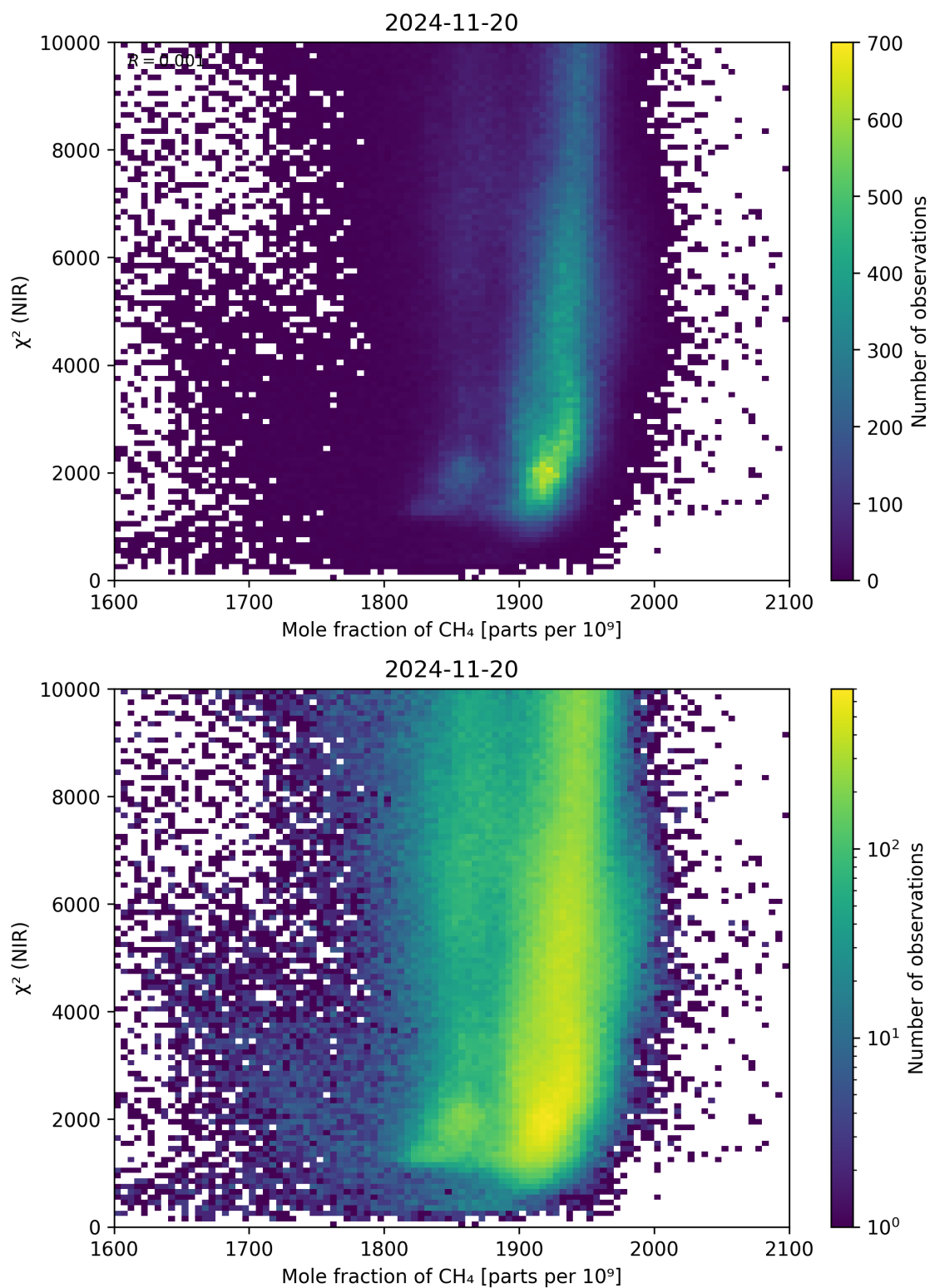
Figure 70: Scatter density plot of “Mole fraction of \text{CH}_4 ” against “ \chi^2 (NIR)” for 2024-11-20 to 2024-11-21.
