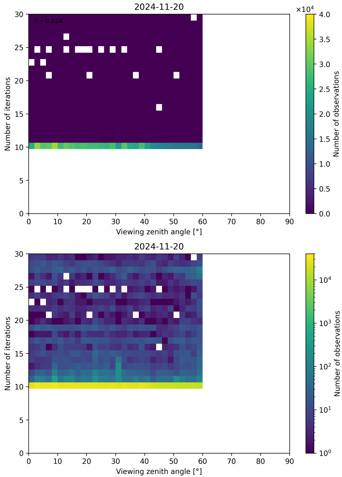
Figure 113: Scatter density plot of “Viewing zenith angle” against “Number of iterations” for 2024-11-20 to 2024-11-21.
