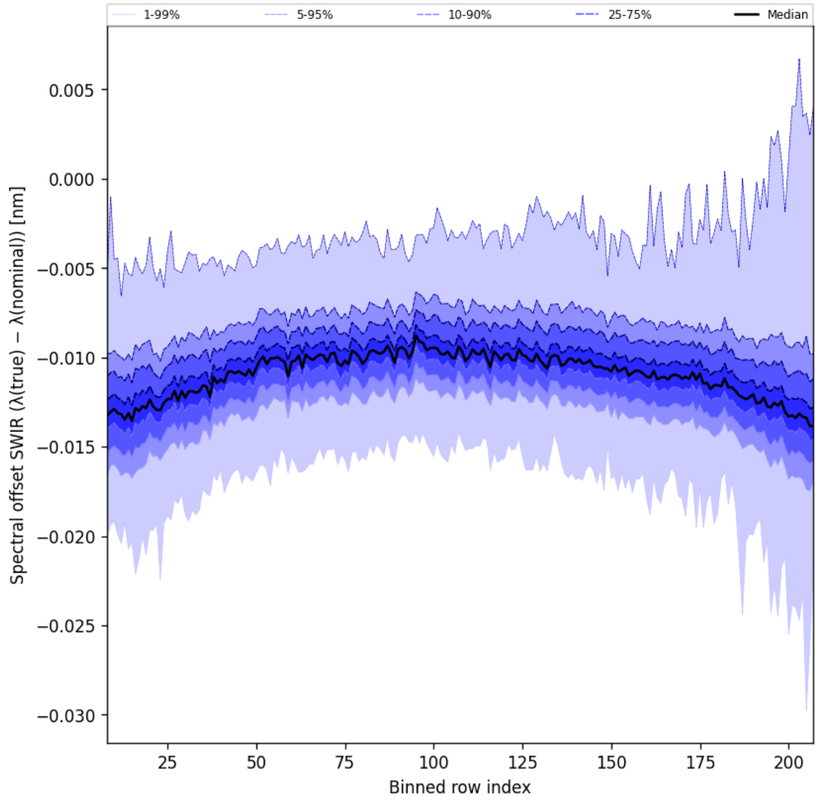
Figure 38: Along track statistics of “Spectral offset SWIR ( \lambda_{\text{true}} - \lambda_{\text{nominal}} )” for 2024-11-20 to 2024-11-21
