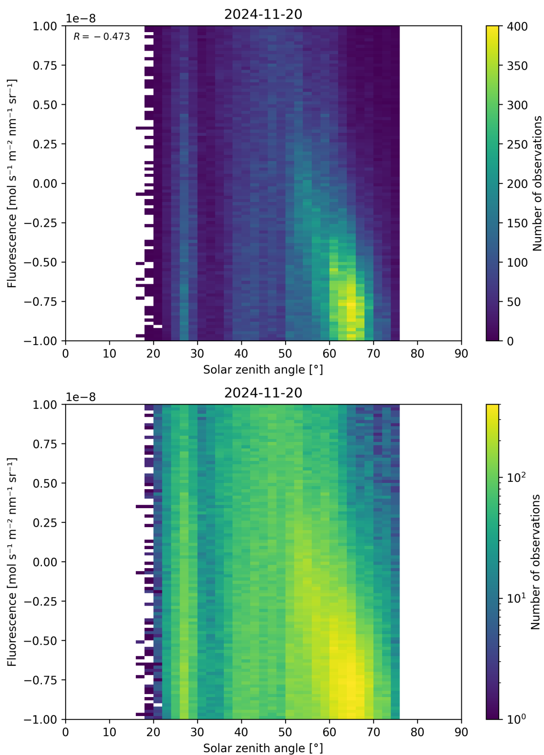
Figure 97: Scatter density plot of “Solar zenith angle” against “Fluorescence” for 2024-11-20 to 2024-11-21.
