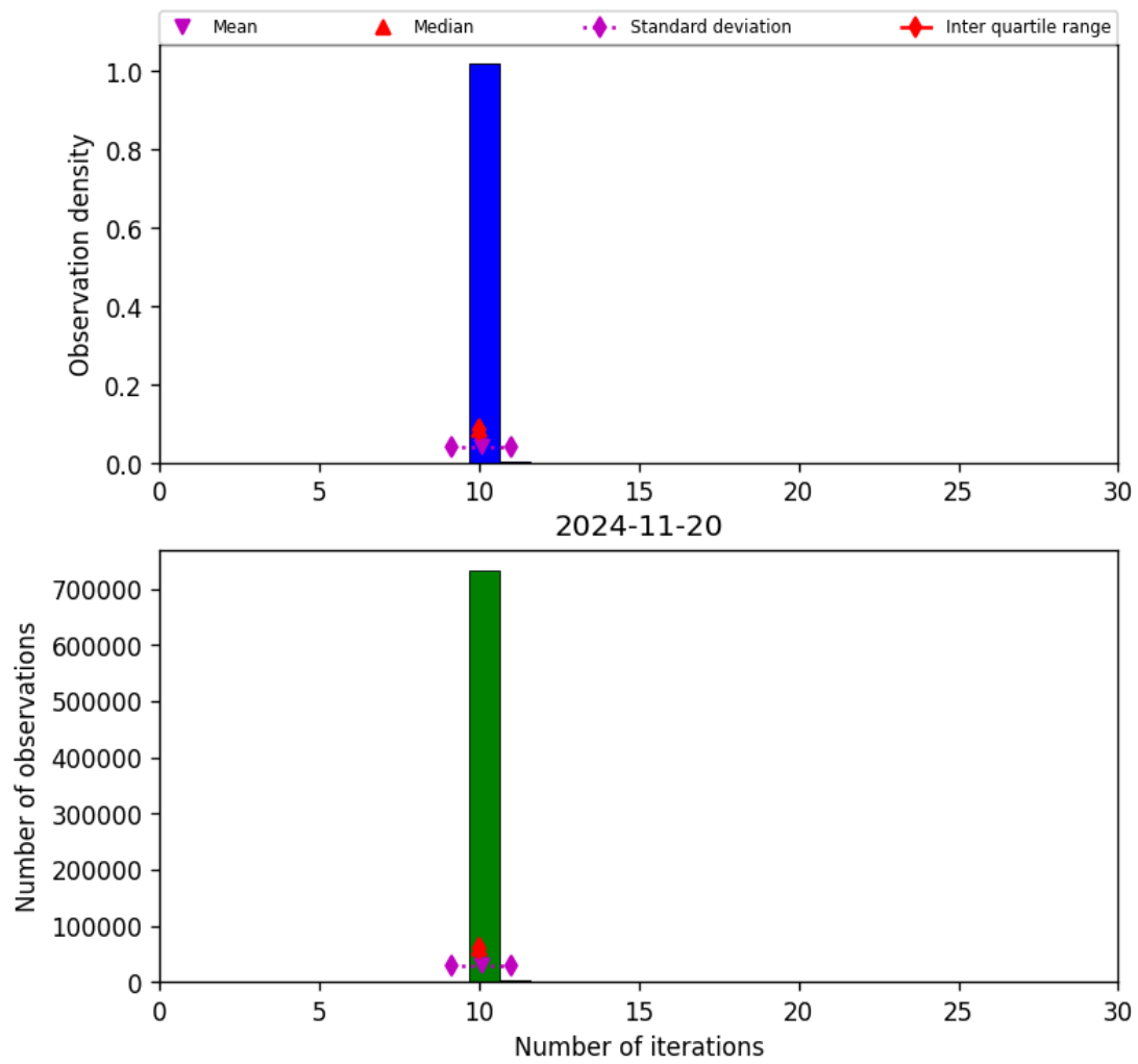
Figure 31: Histogram of “Number of iterations” for 2024-11-20 to 2024-11-21
