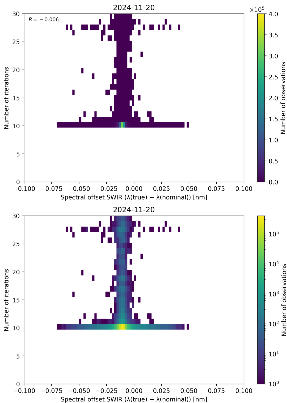
Figure 121: Scatter density plot of “Spectral offset SWIR ( \lambda_{\text{true}} - \lambda_{\text{nominal}} )” against “Number of iterations” for 2024-11-20 to 2024-11-21.
