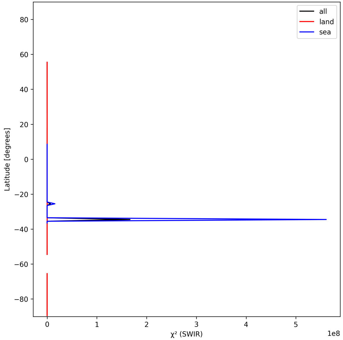
Figure 17: Zonal average of “ \chi^2 (SWIR)” for 2024-11-20 to 2024-11-21.
