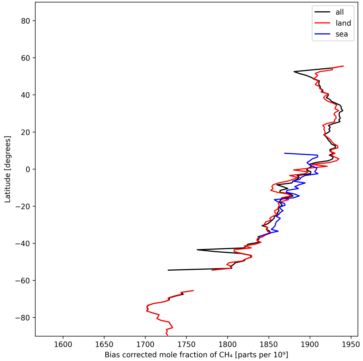
Figure 14: Zonal average of “Bias corrected mole fraction of CH 4 ” for 2024-11-20 to 2024-11-21.
