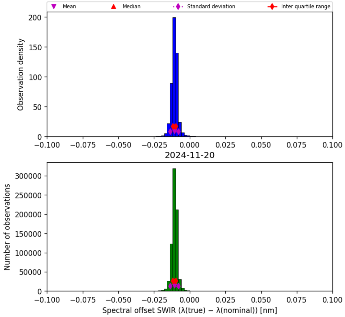
Figure 27: Histogram of “Spectral offset SWIR ( \lambda_{\text{true}} - \lambda_{\text{nominal}} )” for 2024-11-20 to 2024-11-21
