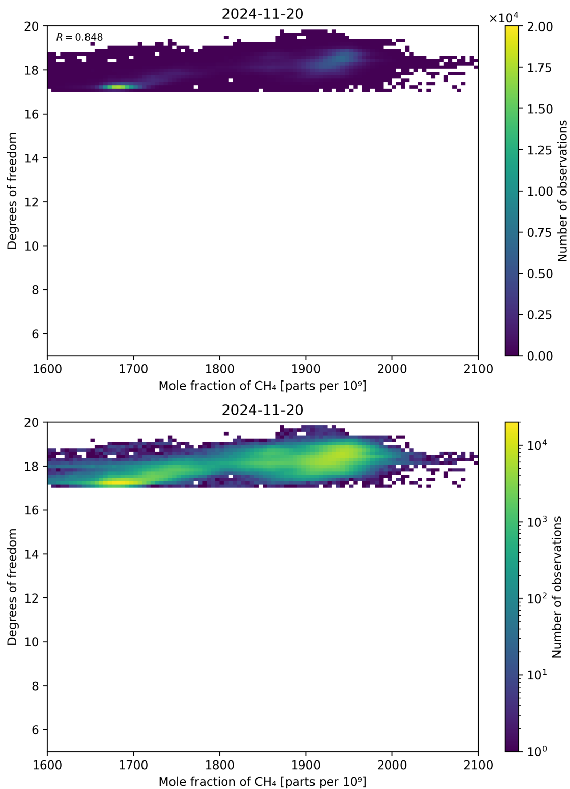
Figure 72: Scatter density plot of “Mole fraction of CH 4 ” against “Degrees of freedom” for 2024-11-20 to 2024-11-21.
