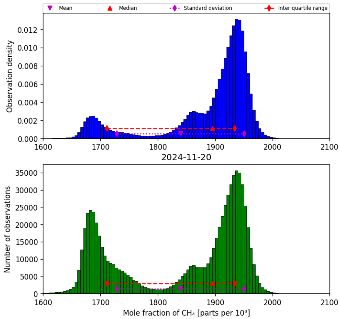
Figure 23: Histogram of “Mole fraction of CH 4 ” for 2024-11-20 to 2024-11-21
