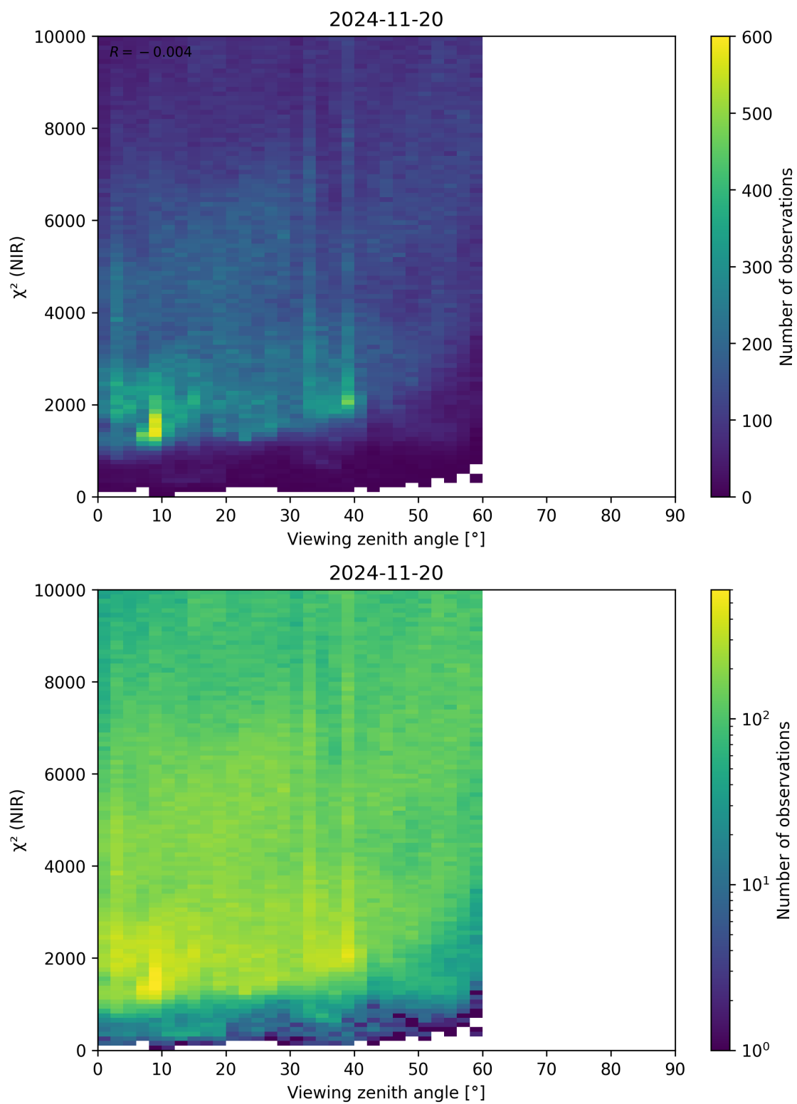
Figure 105: Scatter density plot of “Viewing zenith angle” against “ \chi^2 (NIR)” for 2024-11-20 to 2024-11-21.
