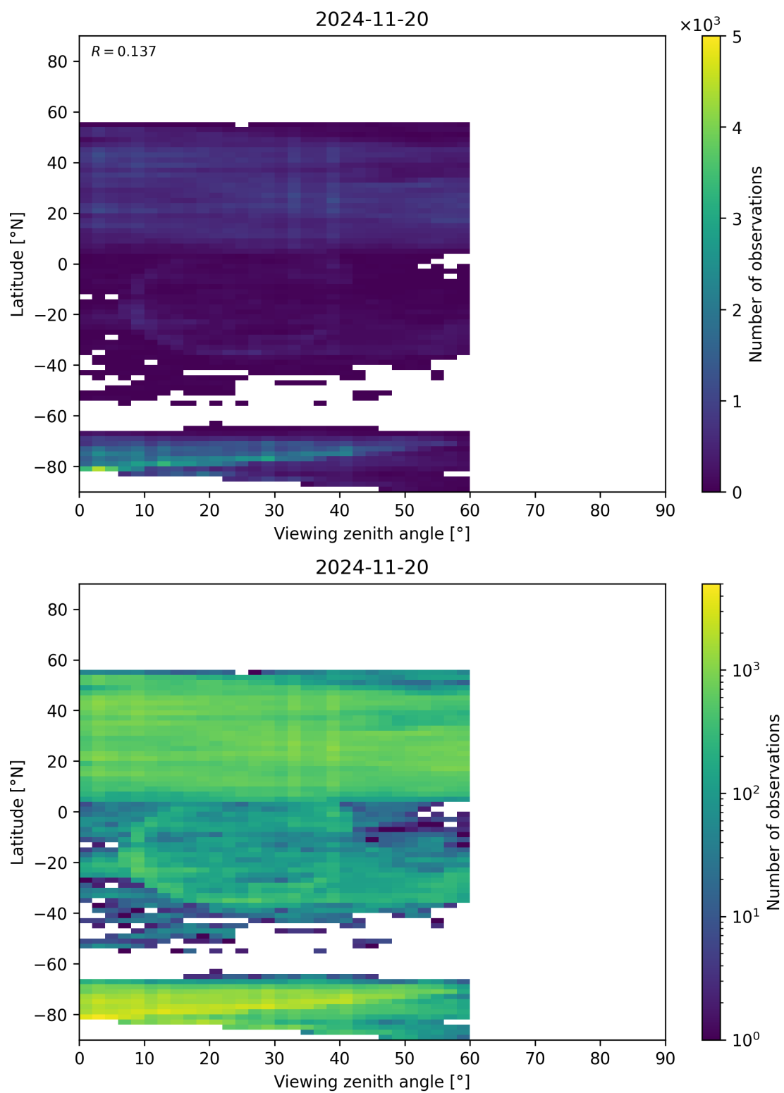
Figure 109: Scatter density plot of “Viewing zenith angle” against “Latitude” for 2024-11-20 to 2024-11-21.
