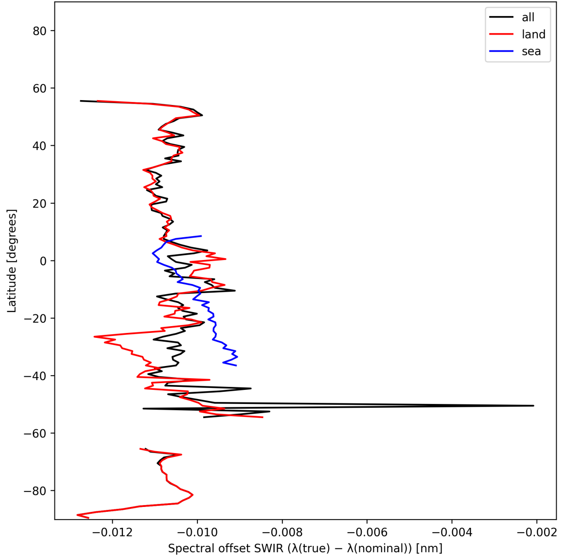
Figure 16: Zonal average of “Spectral offset SWIR ( \lambda_{\text{true}} - \lambda_{\text{nominal}} )” for 2024-11-20 to 2024-11-21.
