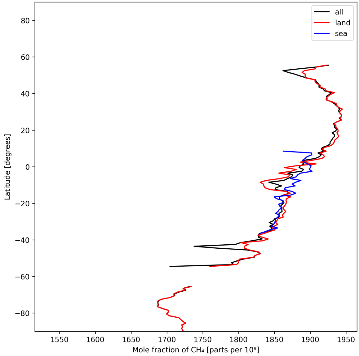
Figure 12: Zonal average of “Mole fraction of \text{CH}_4 ” for 2024-11-20 to 2024-11-21.
