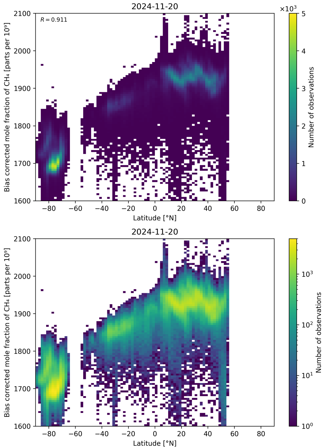
Figure 58: Scatter density plot of “Latitude” against “Bias corrected mole fraction of CH 4 ” for 2024-11-20 to 2024-11-21.
