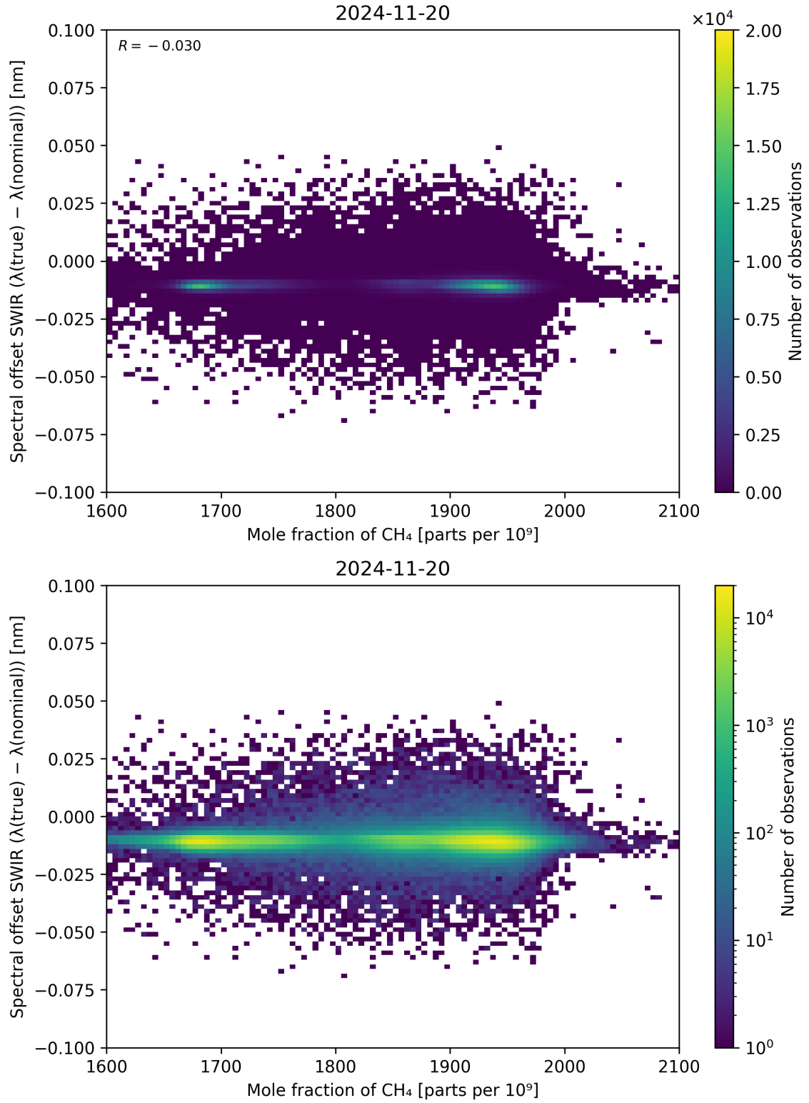
Figure 86: Scatter density plot of “Mole fraction of CH 4 ” against “Spectral offset SWIR ( \lambda_{\text{true}} - \lambda_{\text{nominal}} )” for 2024-11-20 to 2024-11-21.
