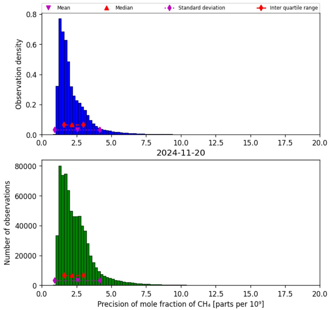
Figure 24: Histogram of “Precision of mole fraction of CH 4 ” for 2024-11-20 to 2024-11-21
