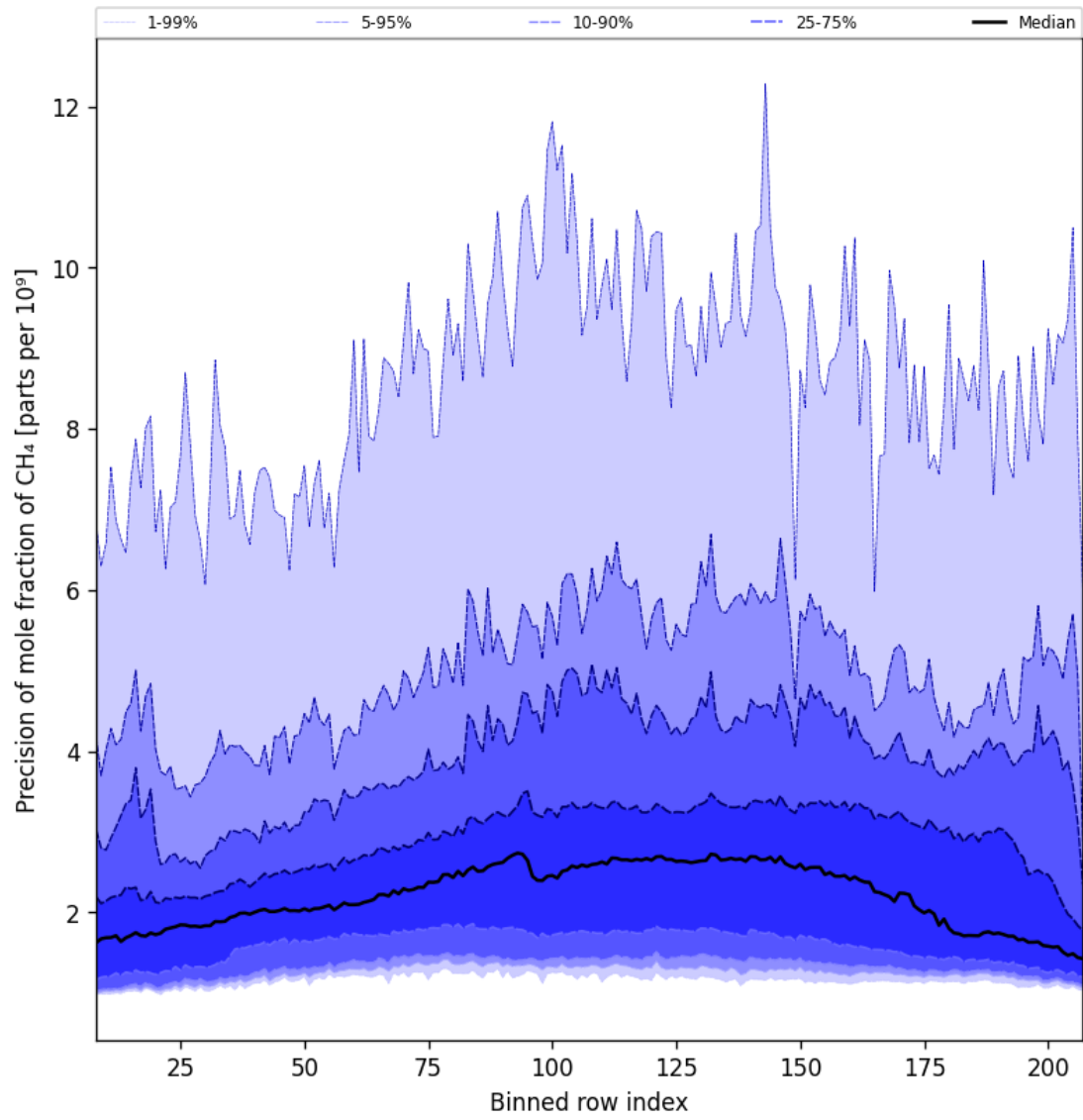
Figure 35: Along track statistics of “Precision of mole fraction of CH 4 ” for 2024-11-20 to 2024-11-21
