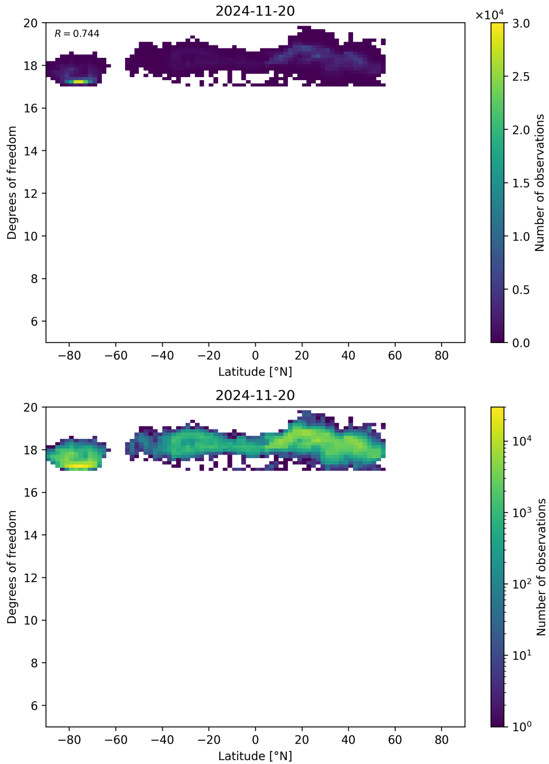
Figure 55: Scatter density plot of “Latitude” against “Degrees of freedom” for 2024-11-20 to 2024-11-21.
