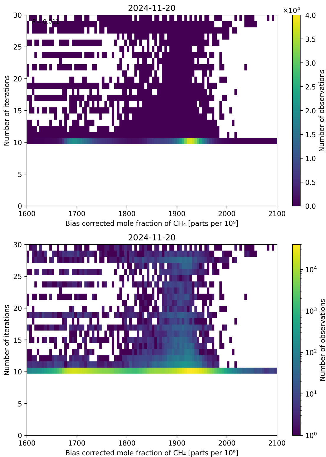
Figure 67: Scatter density plot of “Bias corrected mole fraction of \text{CH}_4 ” against “Number of iterations” for 2024-11-20 to 2024-11-21.
