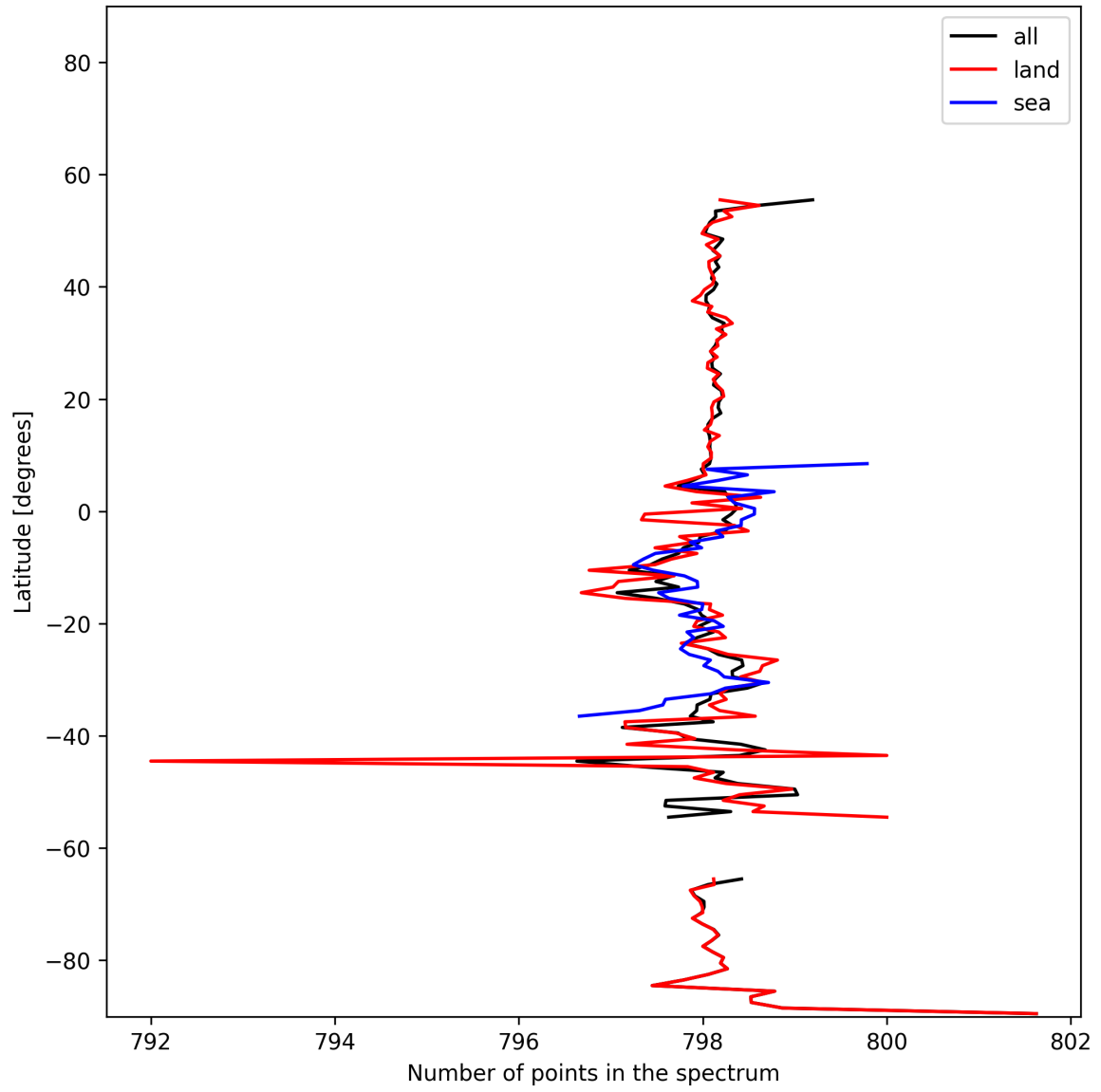
Figure 15: Zonal average of “Number of points in the spectrum” for 2024-11-20 to 2024-11-21.
