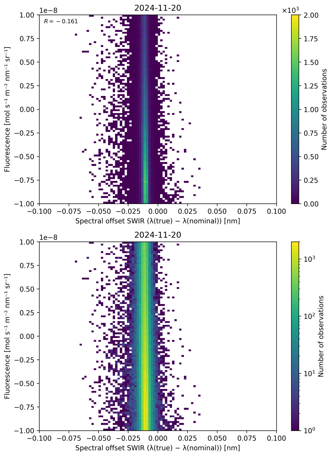
Figure 120: Scatter density plot of “Spectral offset SWIR ( \lambda_{\text{true}} - \lambda_{\text{nominal}} )” against “Fluorescence” for 2024-11-20 to 2024-11-21.
