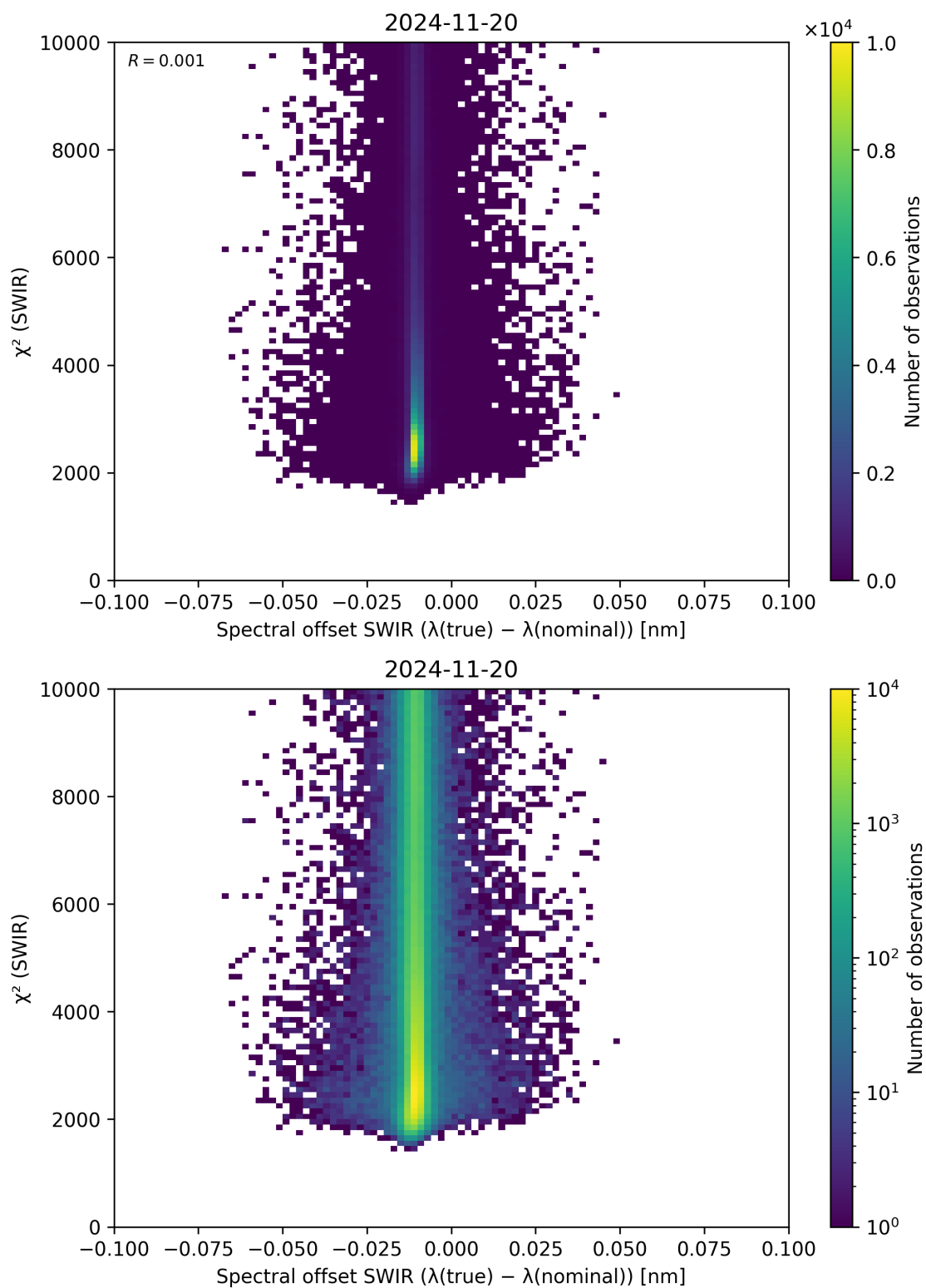
Figure 118: Scatter density plot of “Spectral offset SWIR ( \lambda_{\text{true}} - \lambda_{\text{nominal}} )” against “ \chi^2 (SWIR)” for 2024-11-20 to 2024-11-21.
