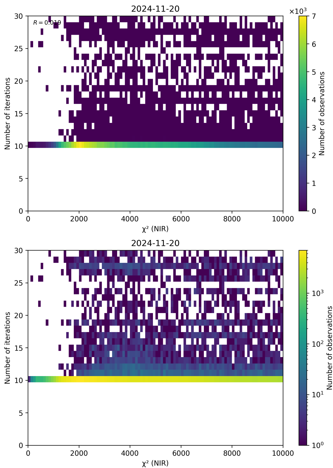
Figure 46: Scatter density plot of “ \chi^2 (NIR)” against “Number of iterations” for 2024-11-20 to 2024-11-21.
