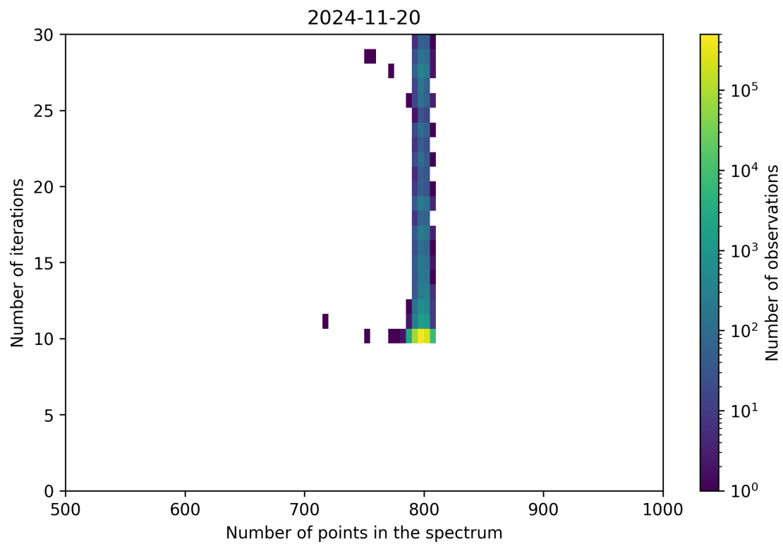
Figure 92: Scatter density plot of “Number of points in the spectrum” against “Number of iterations” for 2024-11-20 to 2024-11-21.
