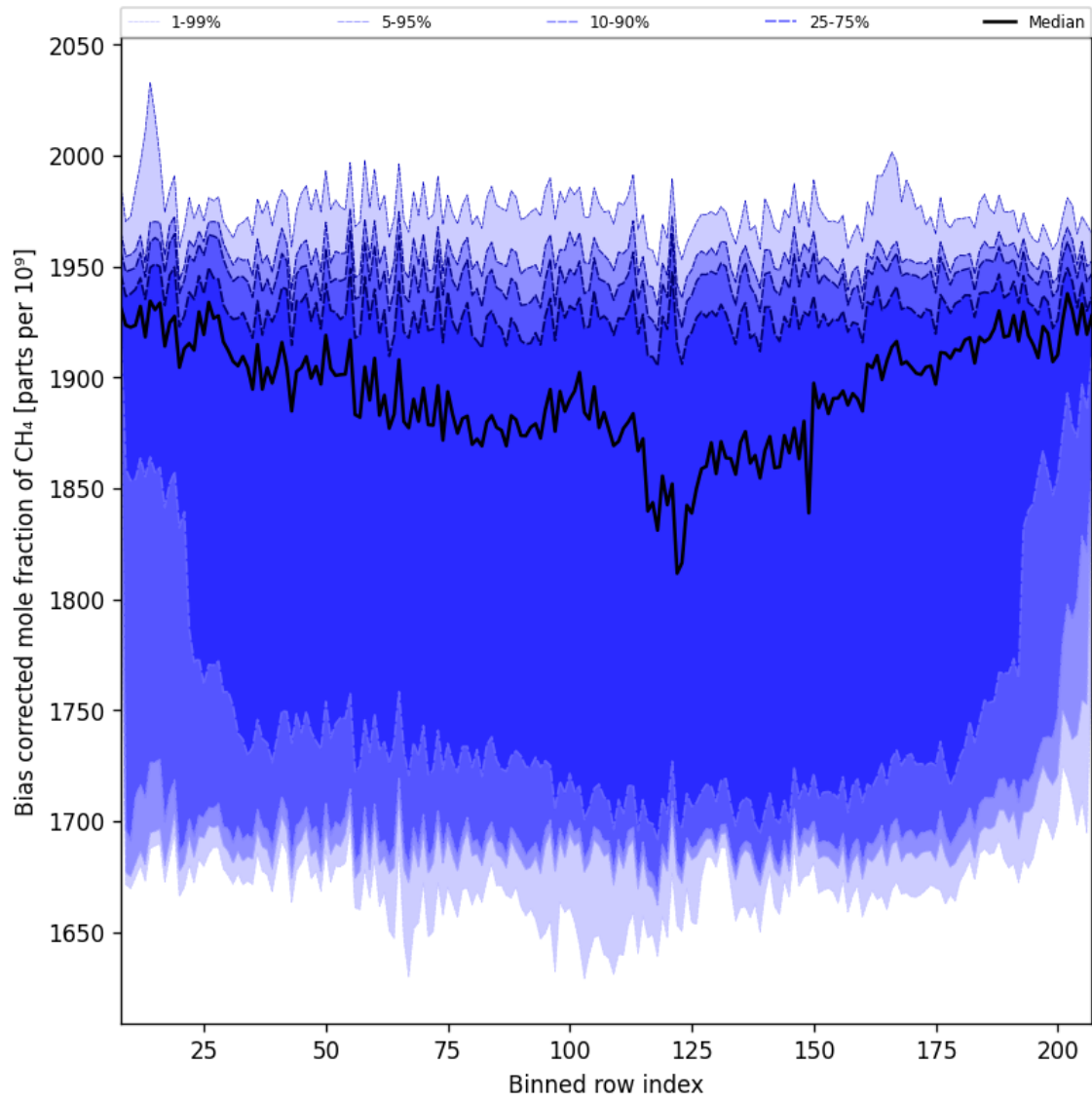
Figure 36: Along track statistics of “Bias corrected mole fraction of CH 4 ” for 2024-11-20 to 2024-11-21
