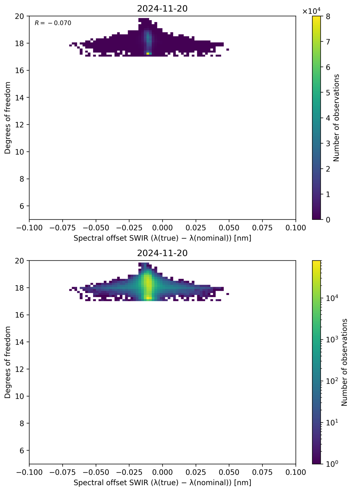
Figure 119: Scatter density plot of “Spectral offset SWIR ( \lambda_{\text{true}} - \lambda_{\text{nominal}} )” against “Degrees of freedom” for 2024-11-20 to 2024-11-21.
