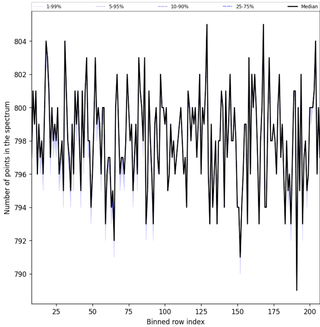
Figure 37: Along track statistics of “Number of points in the spectrum” for 2024-11-20 to 2024-11-21
