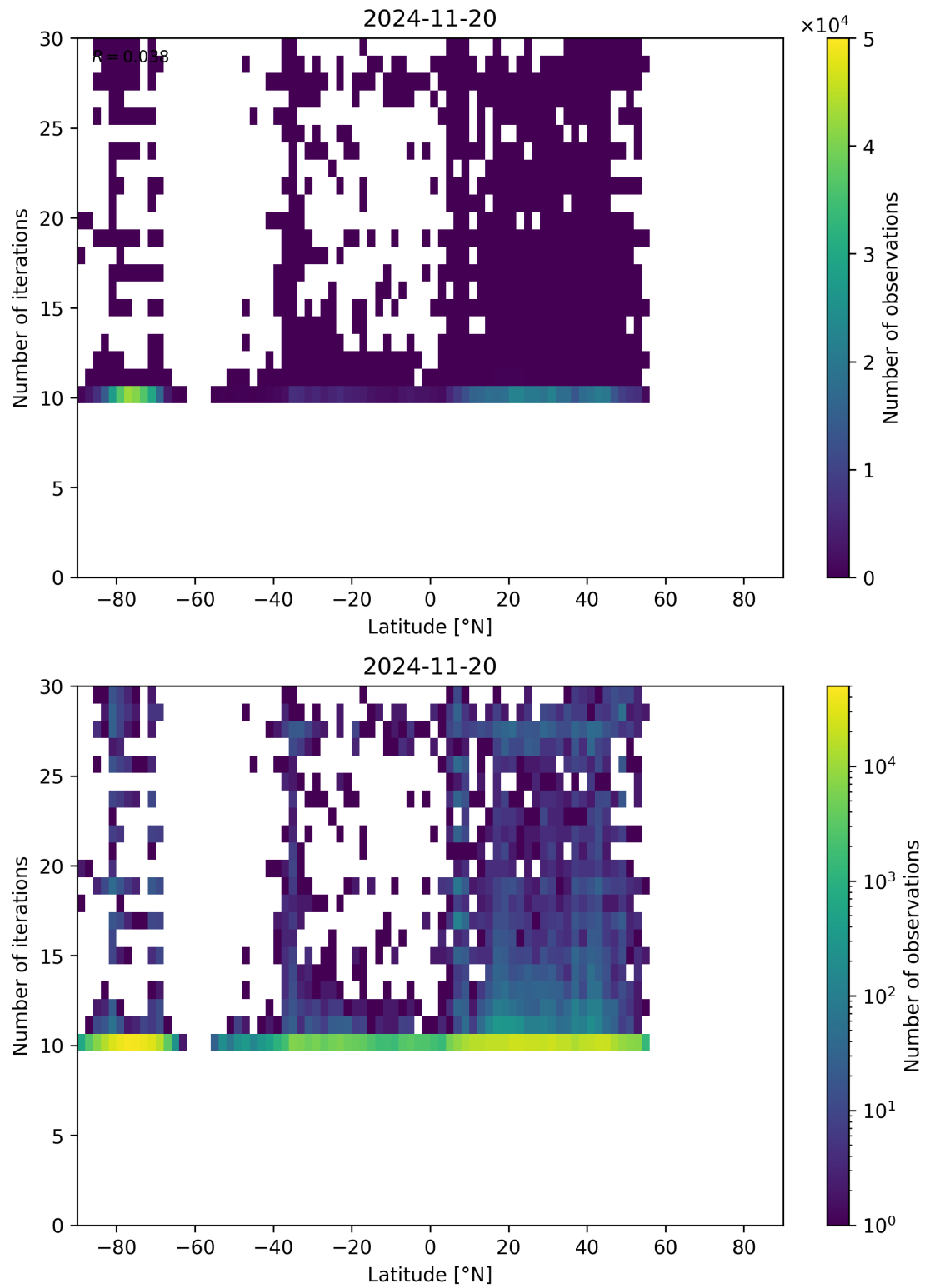
Figure 60: Scatter density plot of “Latitude” against “Number of iterations” for 2024-11-20 to 2024-11-21.
