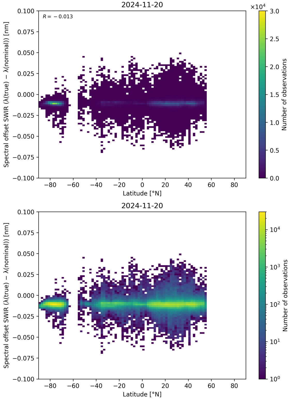
Figure 62: Scatter density plot of “Latitude” against “Spectral offset SWIR ( \lambda_{\text{true}} - \lambda_{\text{nominal}} )” for 2024-11-20 to 2024-11-21.
