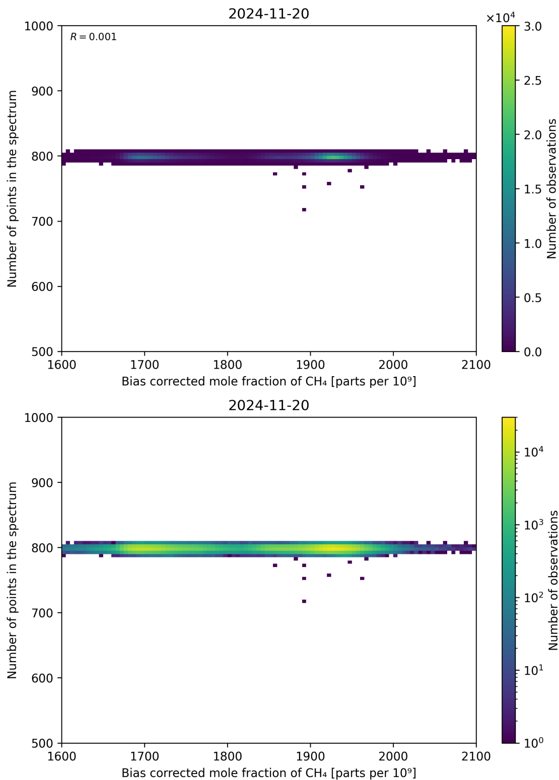
Figure 68: Scatter density plot of “Bias corrected mole fraction of CH 4 ” against “Number of points in the spectrum” for 2024-11-20 to 2024-11-21.
