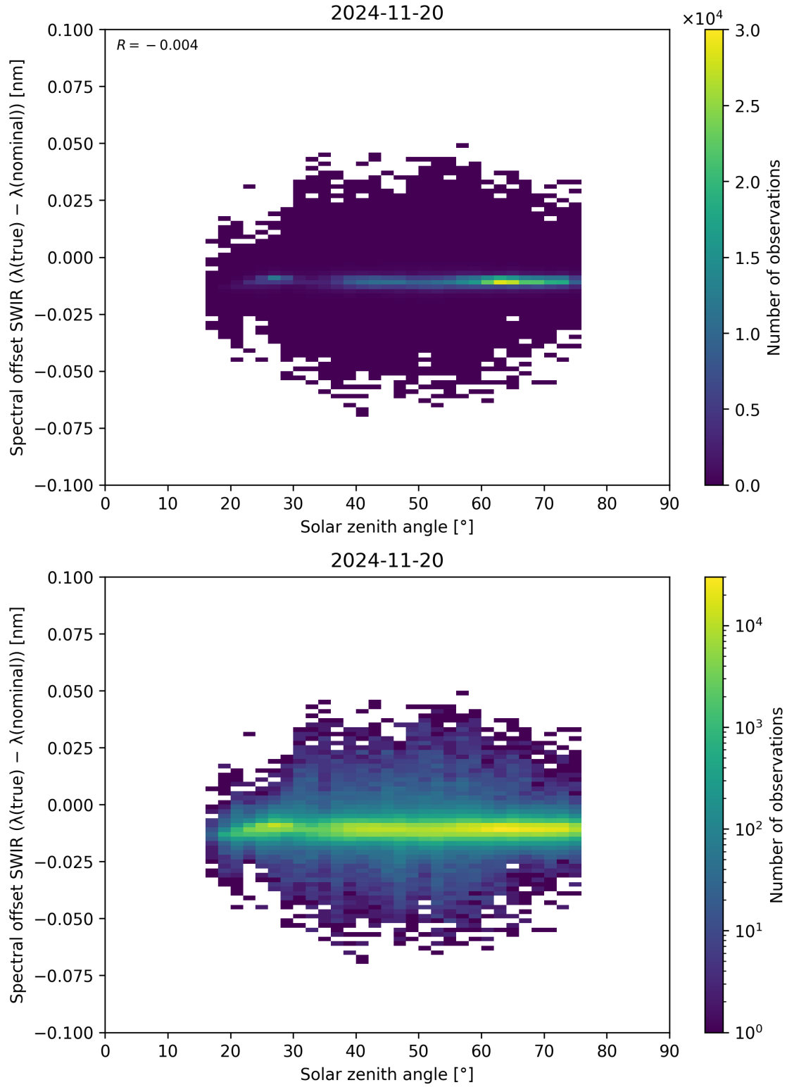
Figure 104: Scatter density plot of “Solar zenith angle” against “Spectral offset SWIR ( \lambda_{\text{true}} - \lambda_{\text{nominal}} )” for 2024-11-20 to 2024-11-21.
