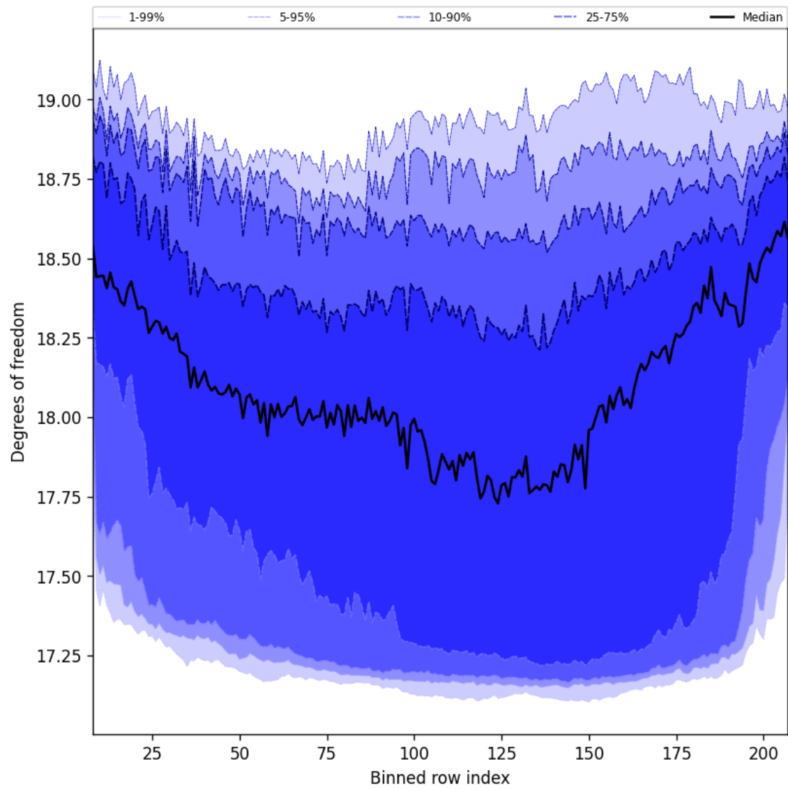
Figure 41: Along track statistics of “Degrees of freedom” for 2024-11-20 to 2024-11-21
