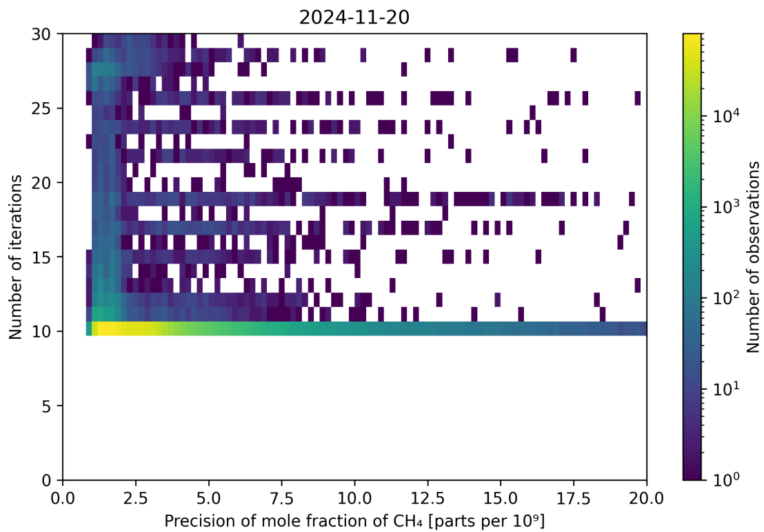
Figure 83: Scatter density plot of “Precision of mole fraction of CH 4 ” against “Number of iterations” for 2024-11-20 to 2024-11-21.
