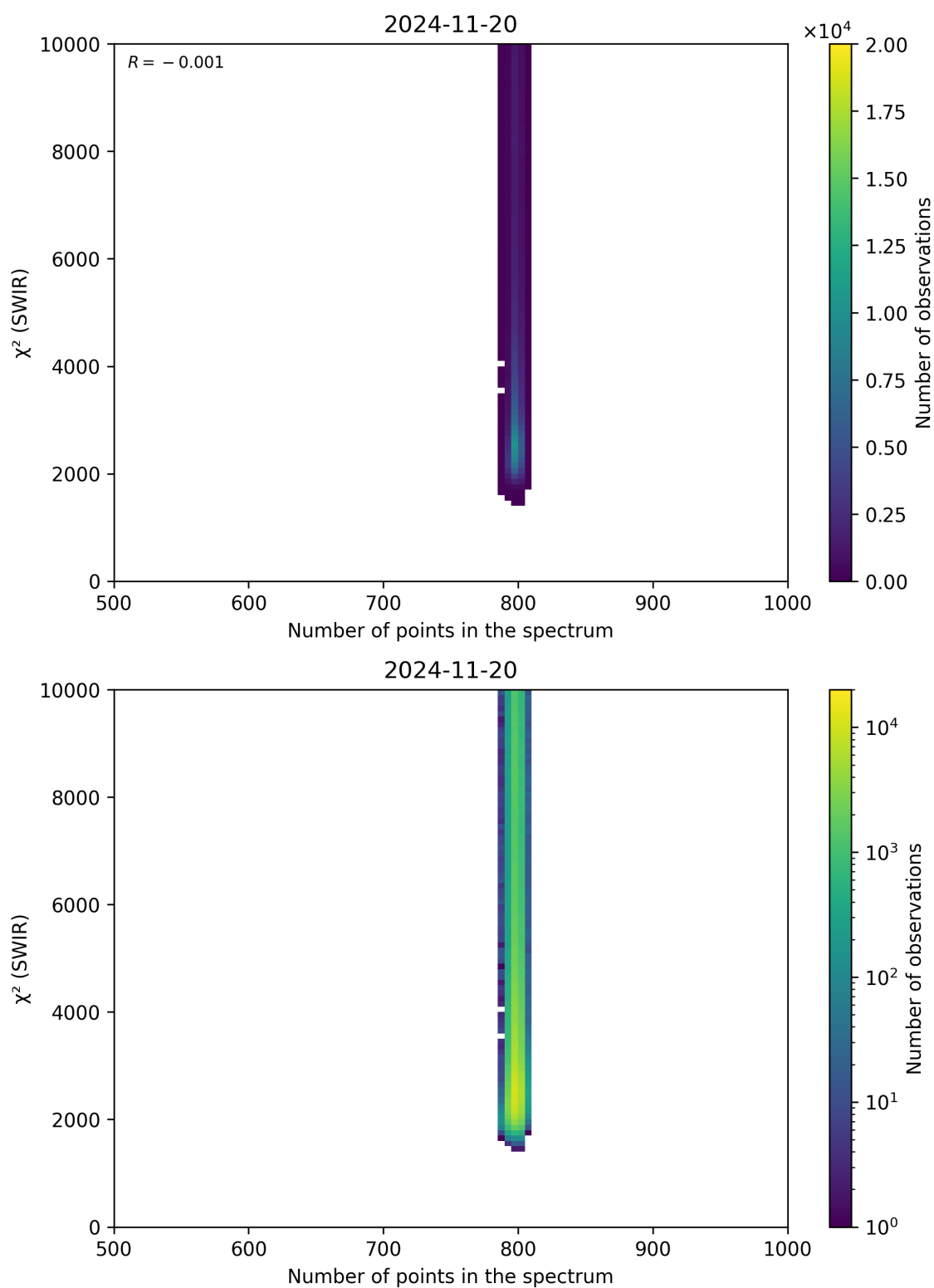
Figure 89: Scatter density plot of “Number of points in the spectrum” against “ \chi^2 (SWIR)” for 2024-11-20 to 2024-11-21.
