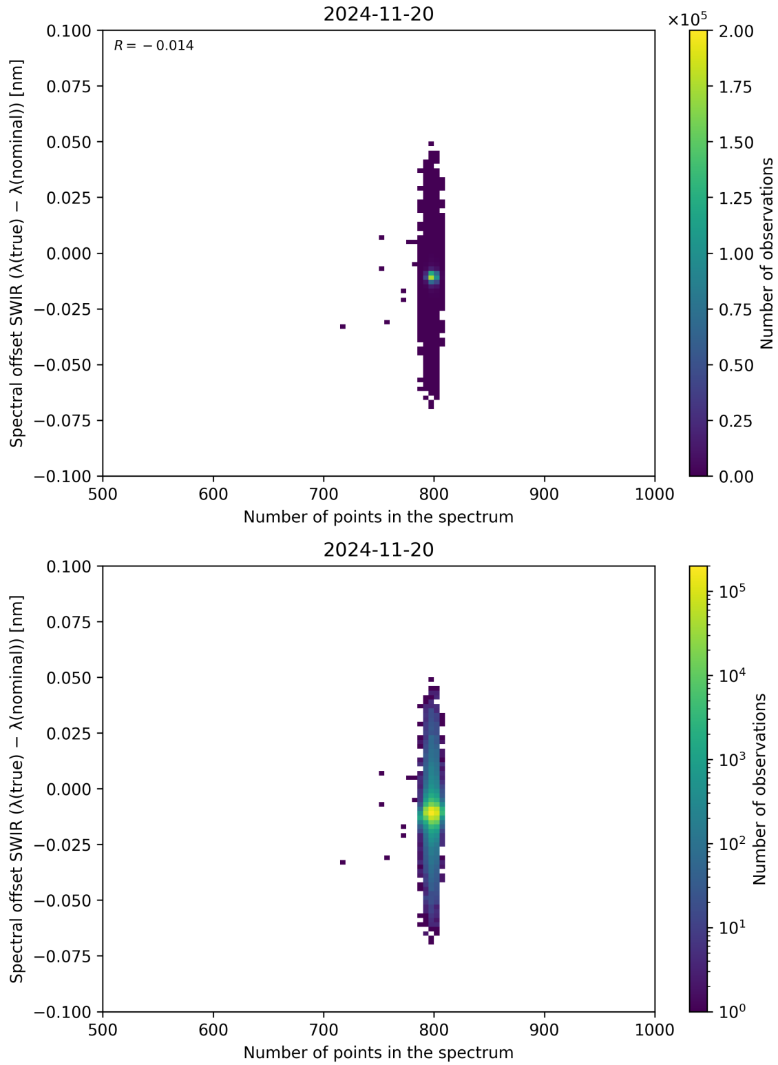
Figure 93: Scatter density plot of “Number of points in the spectrum” against “Spectral offset SWIR ( \lambda_{\text{true}} - \lambda_{\text{nominal}} )” for 2024-11-20 to 2024-11-21.
