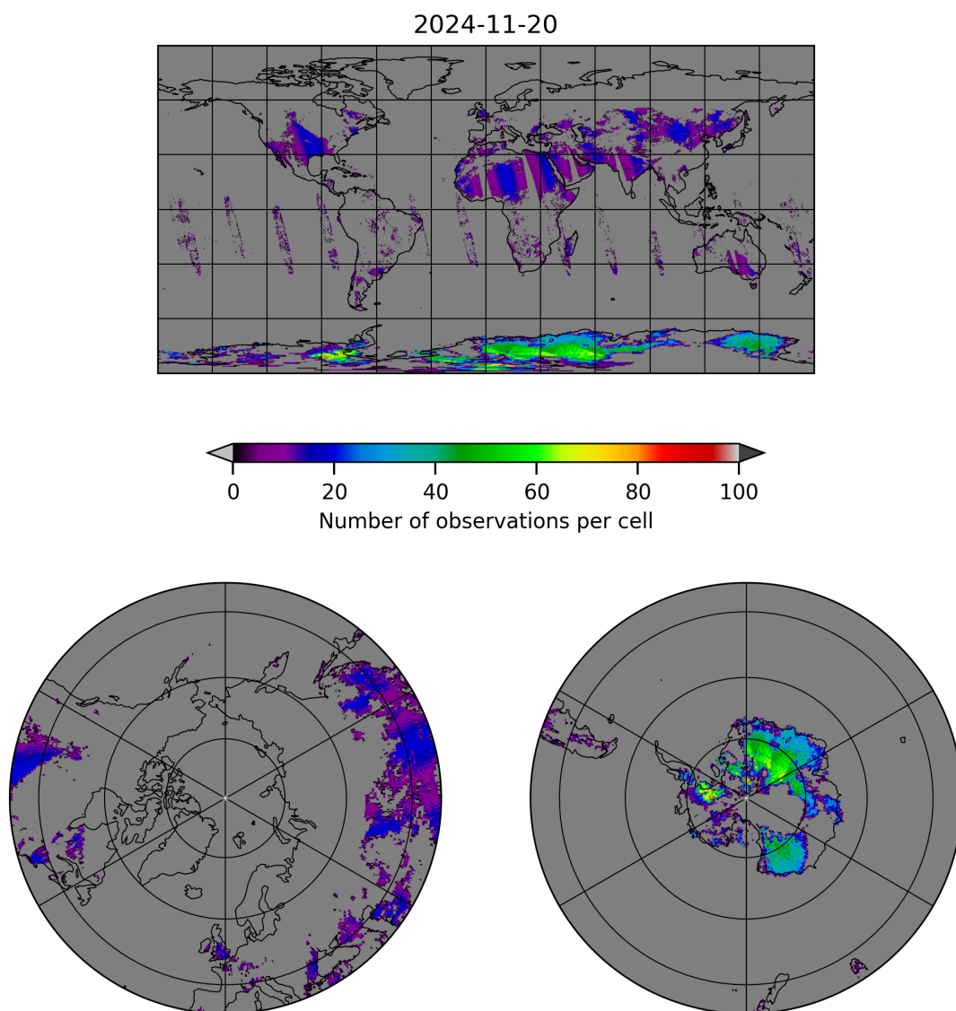
Figure 10: Map of the number of observations for 2024-11-20 to 2024-11-21
