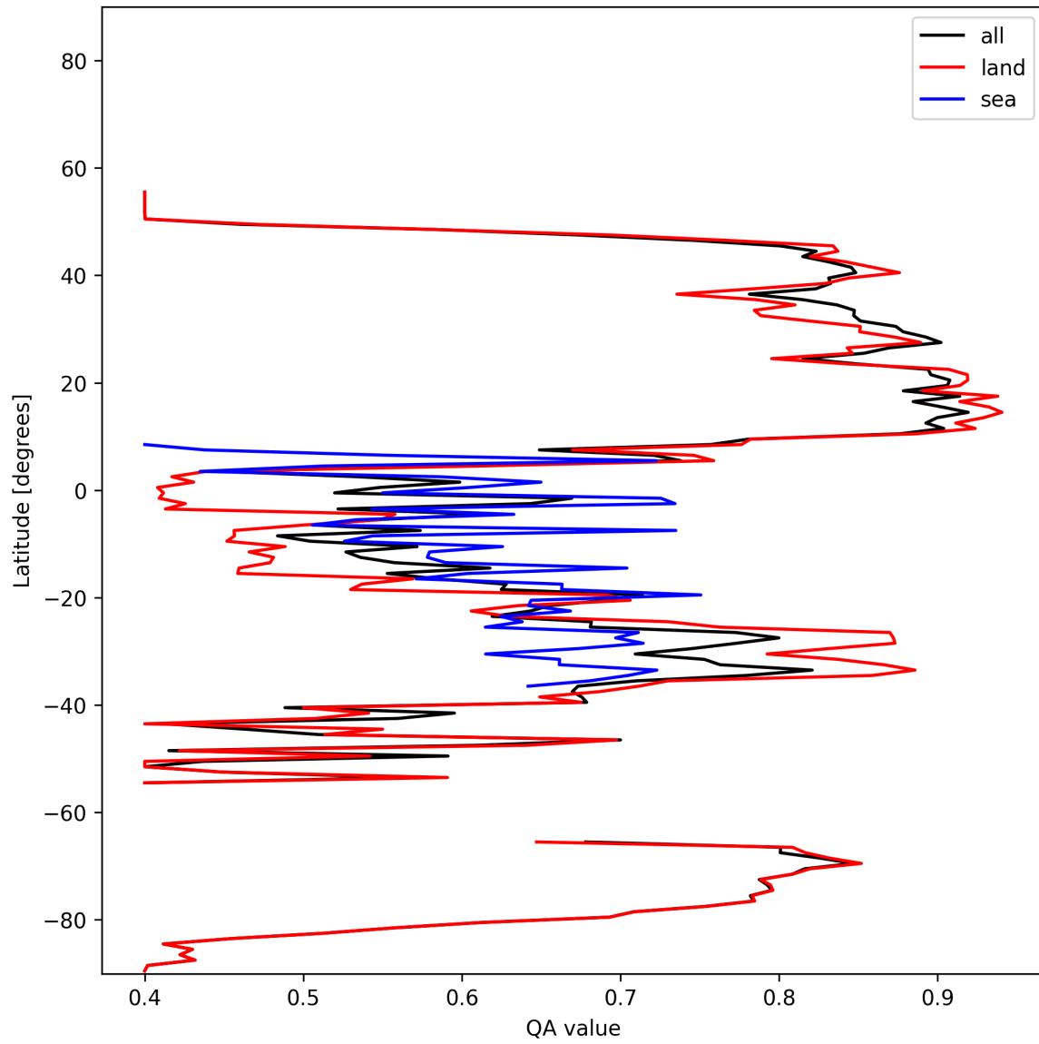
Figure 11: Zonal average of “QA value” for 2024-11-20 to 2024-11-21.
