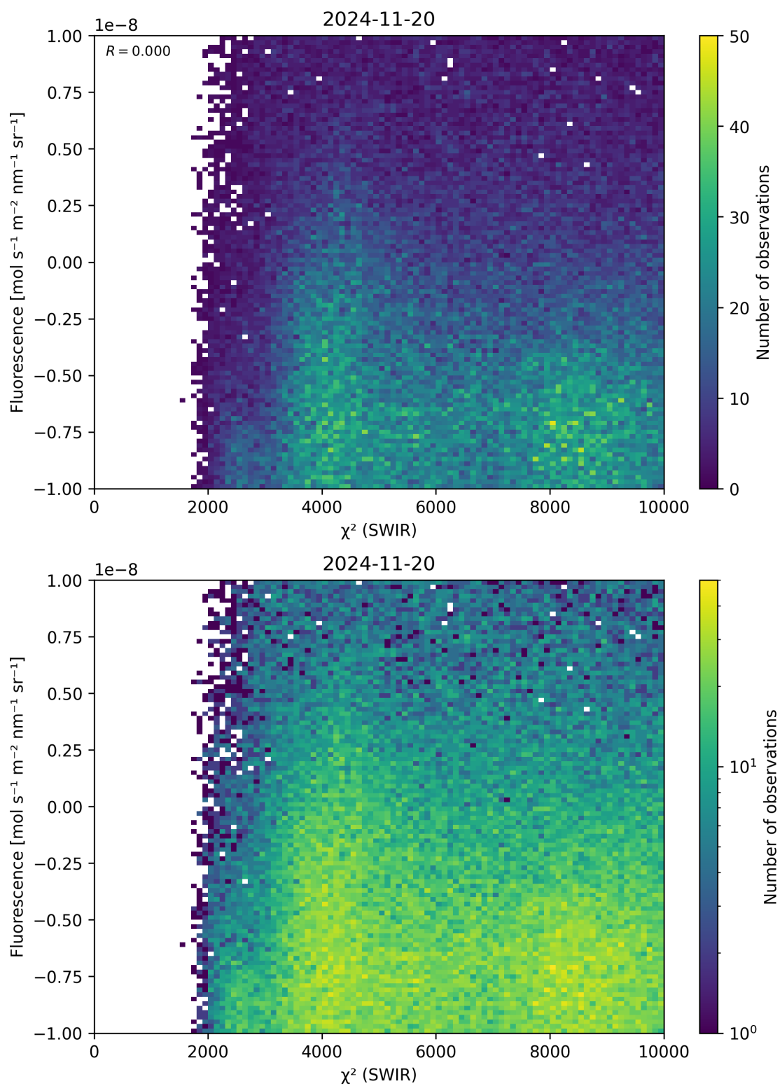
Figure 49: Scatter density plot of “ \chi^2 (SWIR)” against “Fluorescence” for 2024-11-20 to 2024-11-21.
