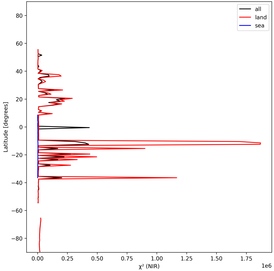
Figure 18: Zonal average of “ \chi^2 (NIR)” for 2024-11-20 to 2024-11-21.
