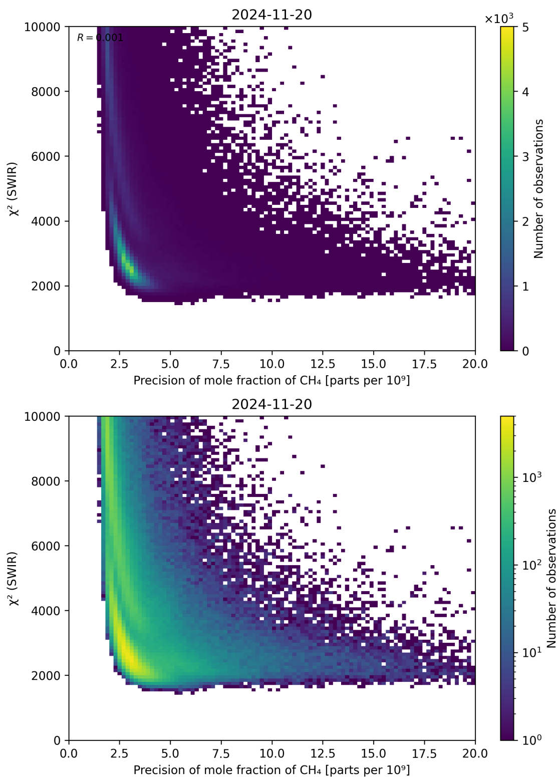
Figure 79: Scatter density plot of “Precision of mole fraction of \text{CH}_4 ” against “ \chi^2 (SWIR)” for 2024-11-20 to 2024-11-21.
