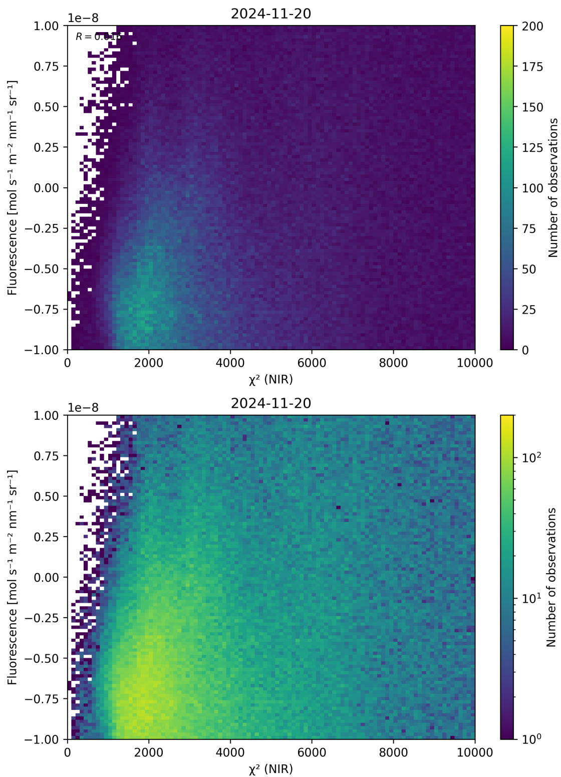
Figure 45: Scatter density plot of “ \chi^2 (NIR)” against “Fluorescence” for 2024-11-20 to 2024-11-21.
