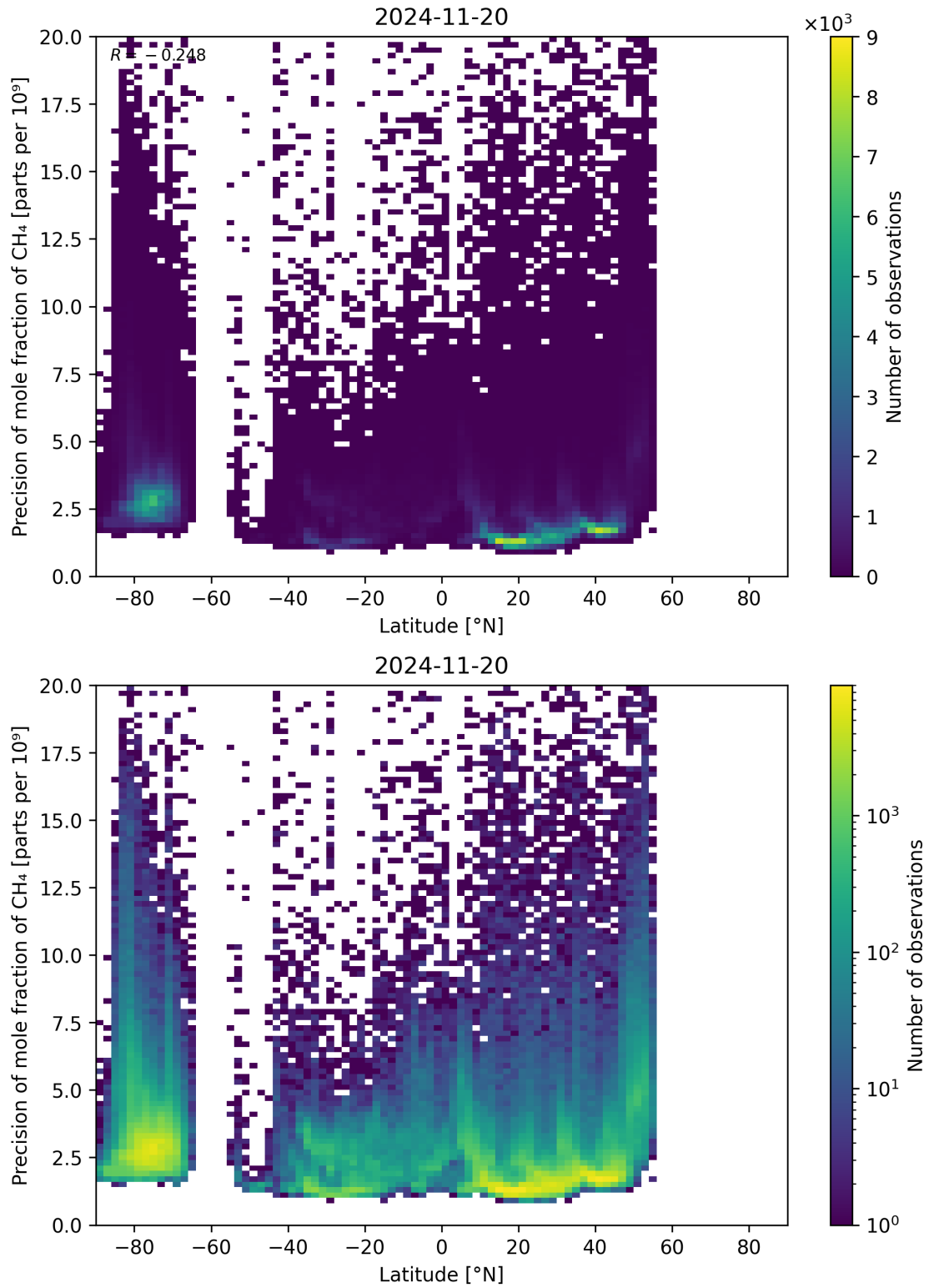
Figure 59: Scatter density plot of “Latitude” against “Precision of mole fraction of CH 4 ” for 2024-11-20 to 2024-11-21.
