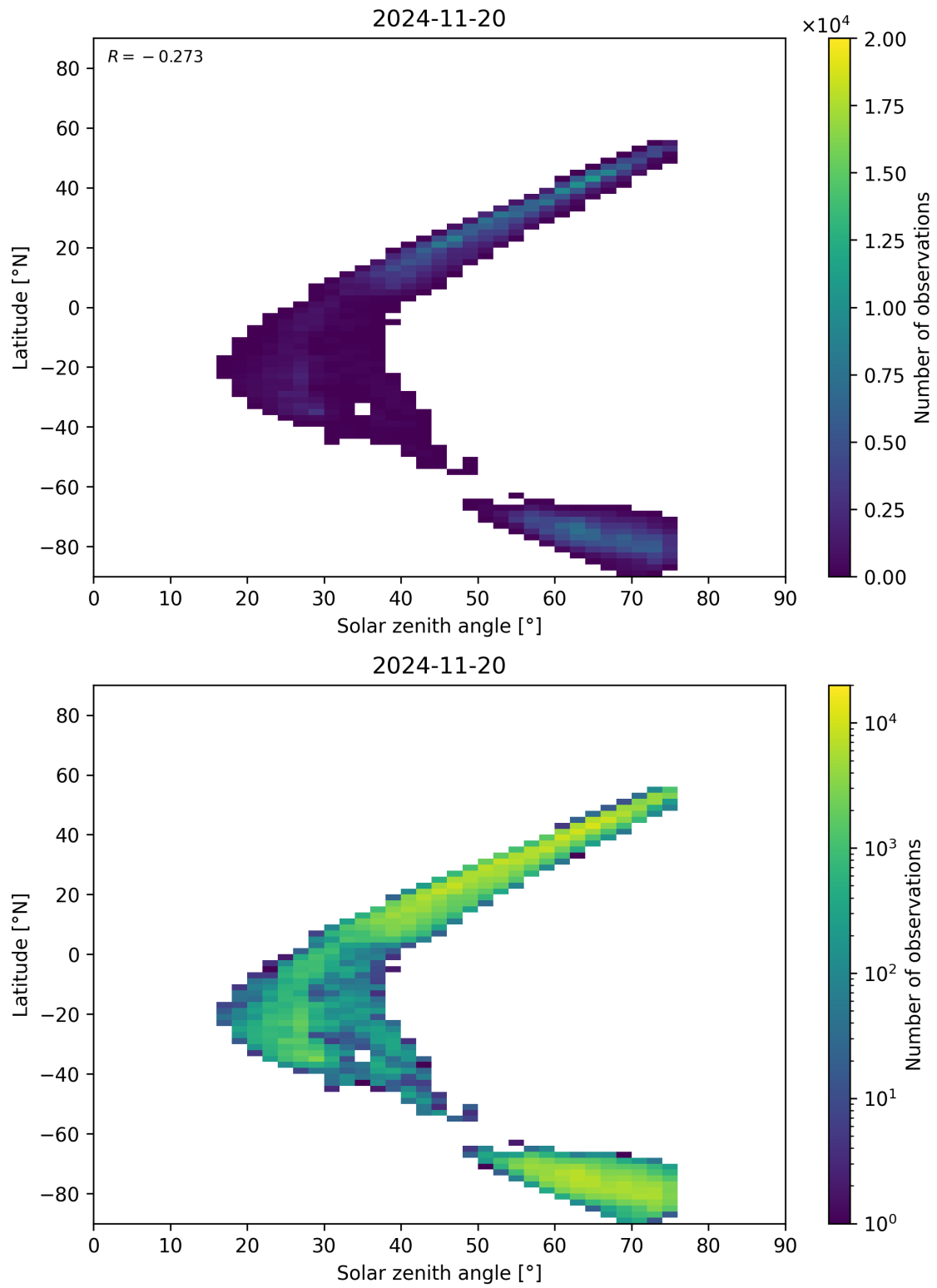
Figure 98: Scatter density plot of “Solar zenith angle” against “Latitude” for 2024-11-20 to 2024-11-21.
