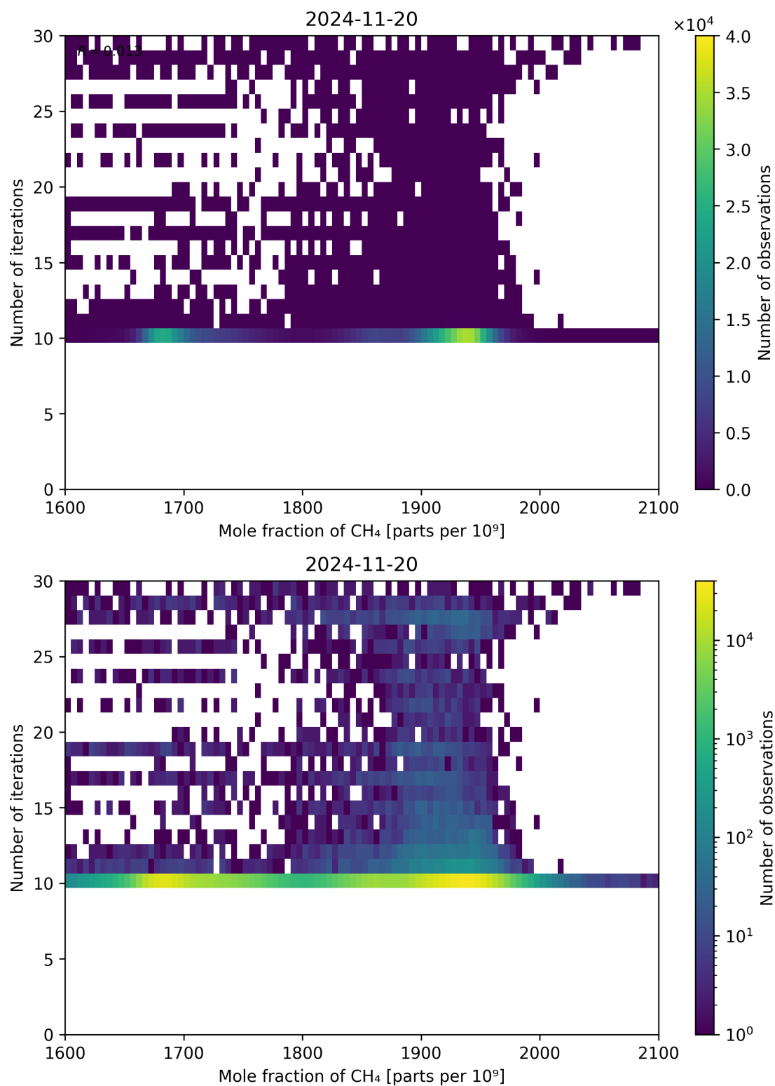
Figure 76: Scatter density plot of “Mole fraction of CH 4 ” against “Number of iterations” for 2024-11-20 to 2024-11-21.
