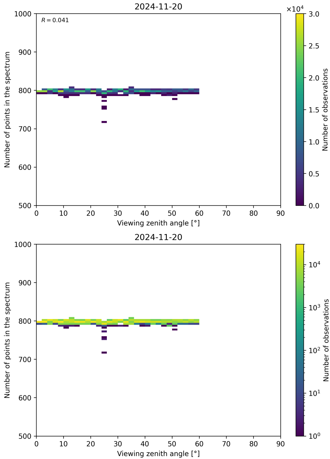
Figure 114: Scatter density plot of “Viewing zenith angle” against “Number of points in the spectrum” for 2024-11-20 to 2024-11-21.
