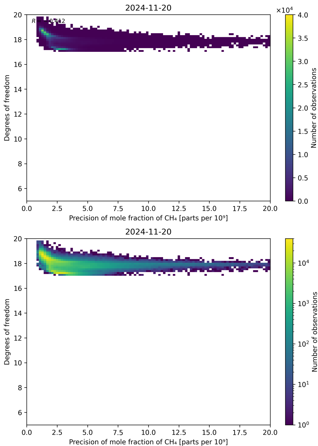
Figure 80: Scatter density plot of “Precision of mole fraction of CH 4 ” against “Degrees of freedom” for 2024-11-20 to 2024-11-21.
