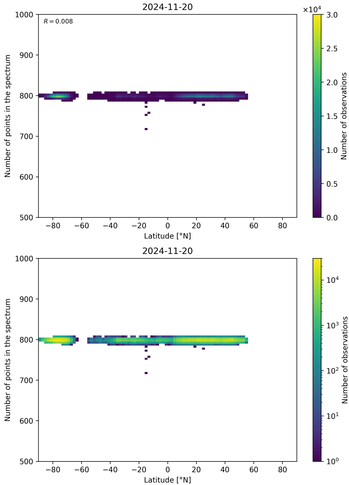
Figure 61: Scatter density plot of “Latitude” against “Number of points in the spectrum” for 2024-11-20 to 2024-11-21.
