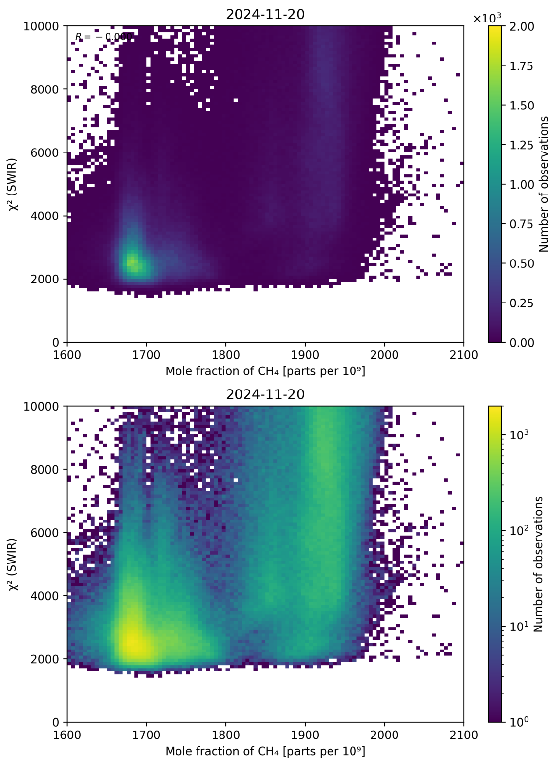
Figure 71: Scatter density plot of “Mole fraction of \text{CH}_4 ” against “ \chi^2 (SWIR)” for 2024-11-20 to 2024-11-21.
