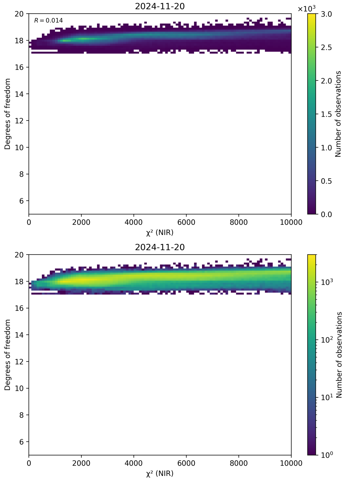
Figure 44: Scatter density plot of “ \chi^2 (NIR)” against “Degrees of freedom” for 2024-11-20 to 2024-11-21.
