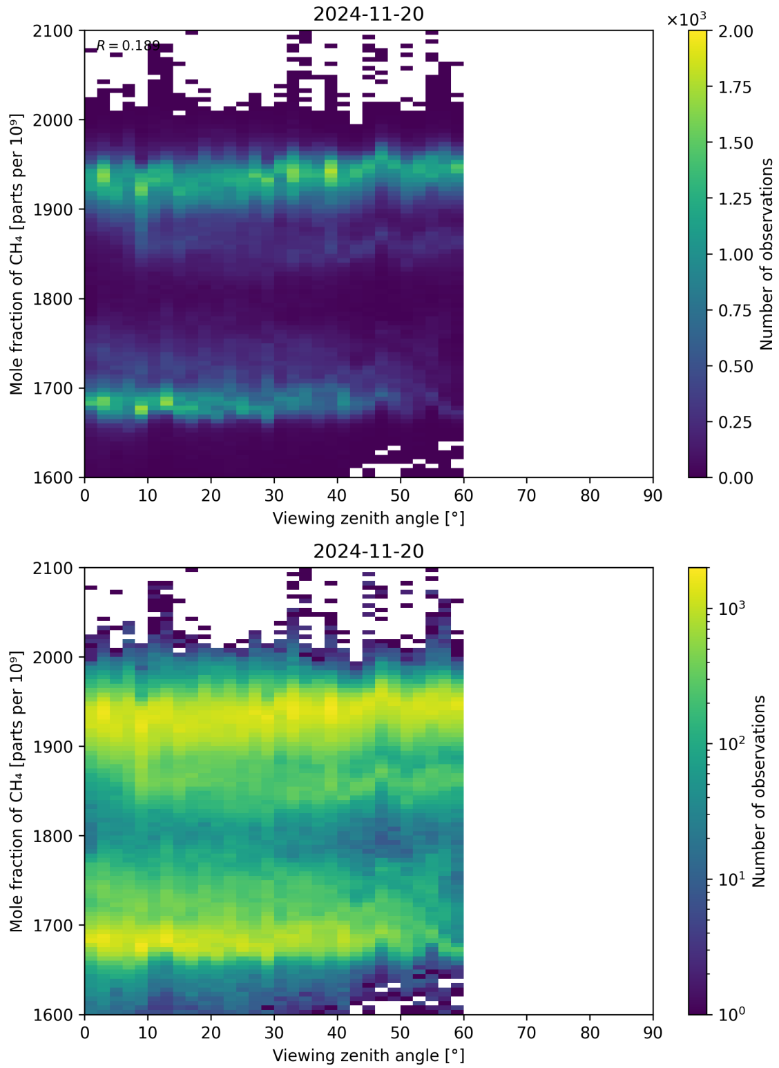
Figure 110: Scatter density plot of “Viewing zenith angle” against “Mole fraction of CH 4 ” for 2024-11-20 to 2024-11-21.
