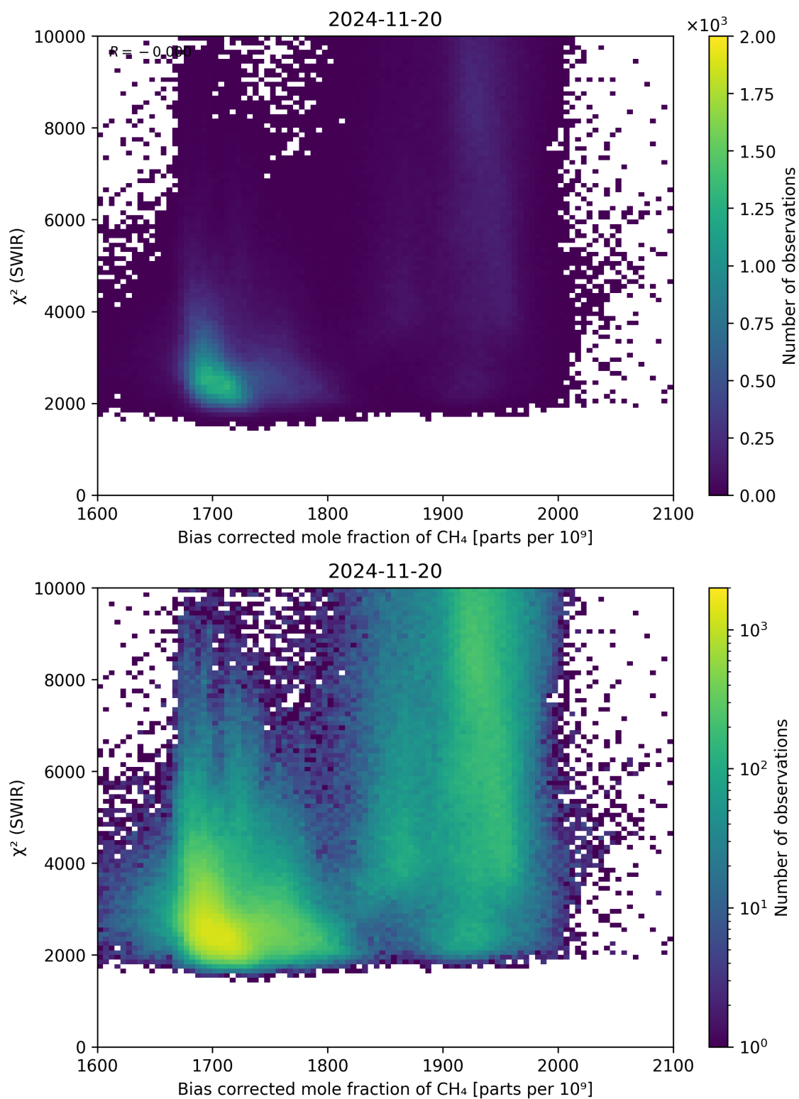
Figure 64: Scatter density plot of “Bias corrected mole fraction of \text{CH}_4 ” against “ \chi^2 (SWIR)” for 2024-11-20 to 2024-11-21.
