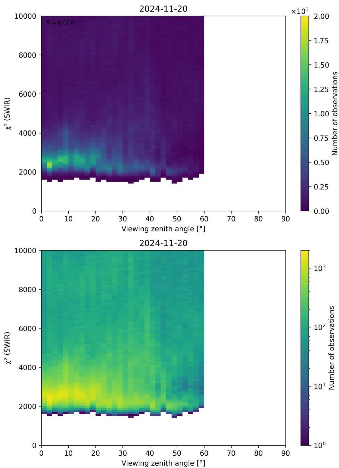
Figure 106: Scatter density plot of “Viewing zenith angle” against “ \chi^2 (SWIR)” for 2024-11-20 to 2024-11-21.
