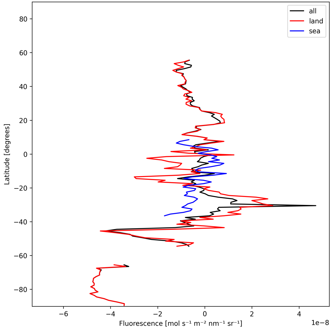
Figure 21: Zonal average of “Fluorescence” for 2024-11-20 to 2024-11-21.
