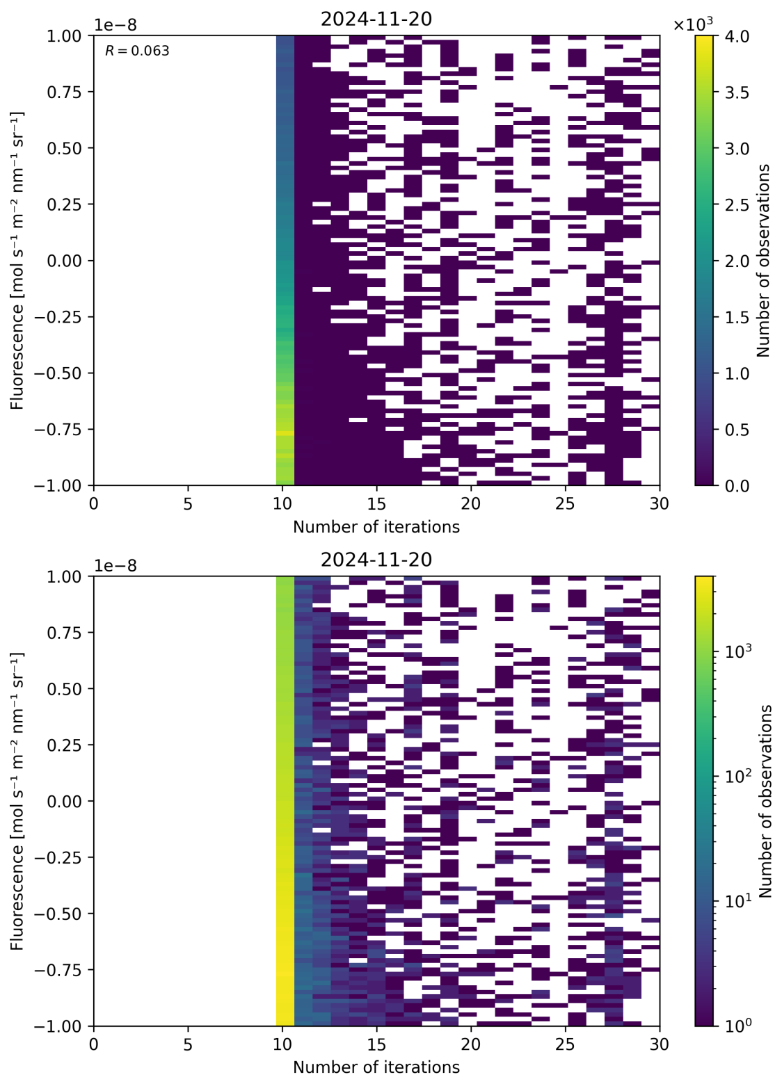
Figure 87: Scatter density plot of “Number of iterations” against “Fluorescence” for 2024-11-20 to 2024-11-21.
