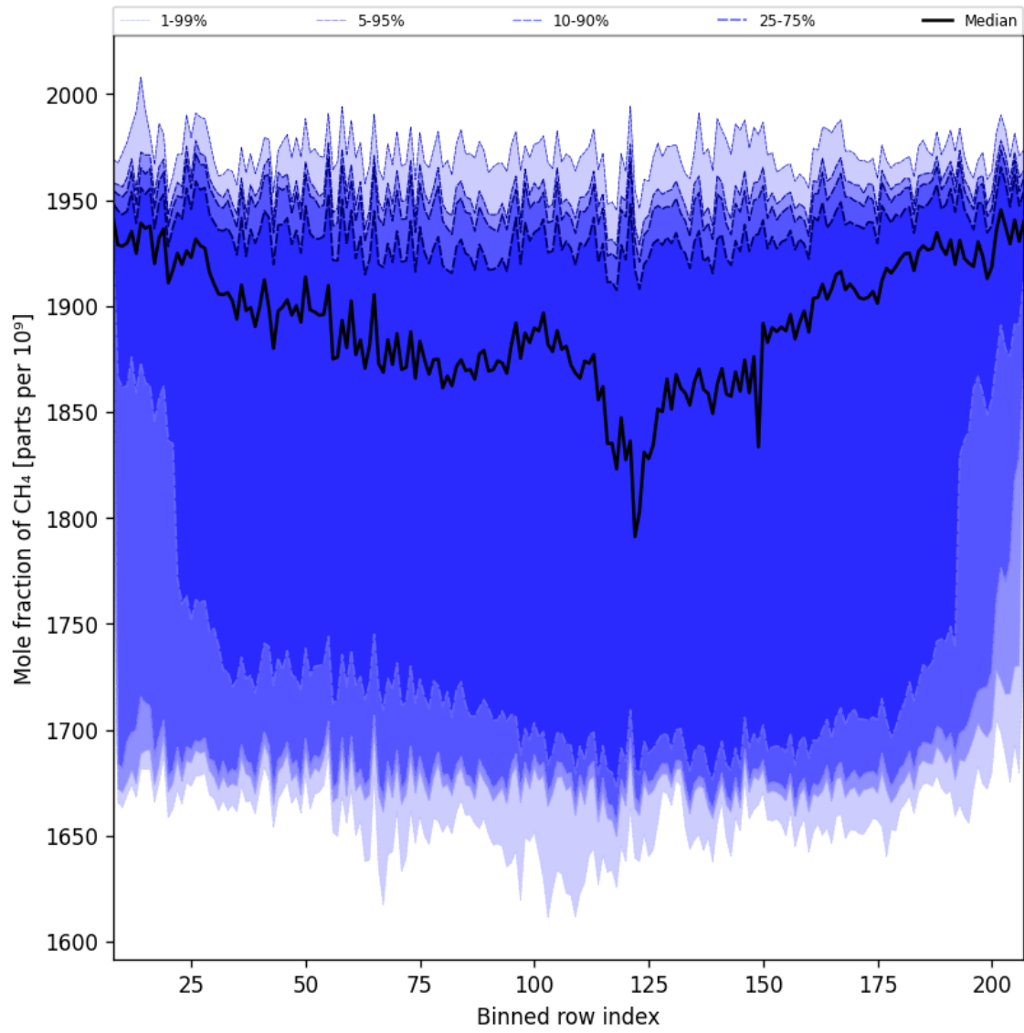
Figure 34: Along track statistics of “Mole fraction of CH 4 ” for 2024-11-20 to 2024-11-21
