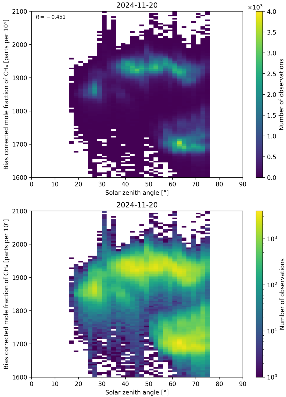
Figure 100: Scatter density plot of “Solar zenith angle” against “Bias corrected mole fraction of CH 4 ” for 2024-11-20 to 2024-11-21.
