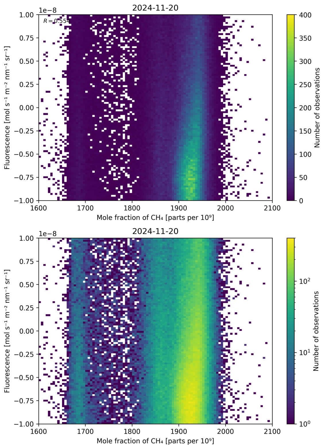
Figure 73: Scatter density plot of “Mole fraction of \text{CH}_4 ” against “Fluorescence” for 2024-11-20 to 2024-11-21.
