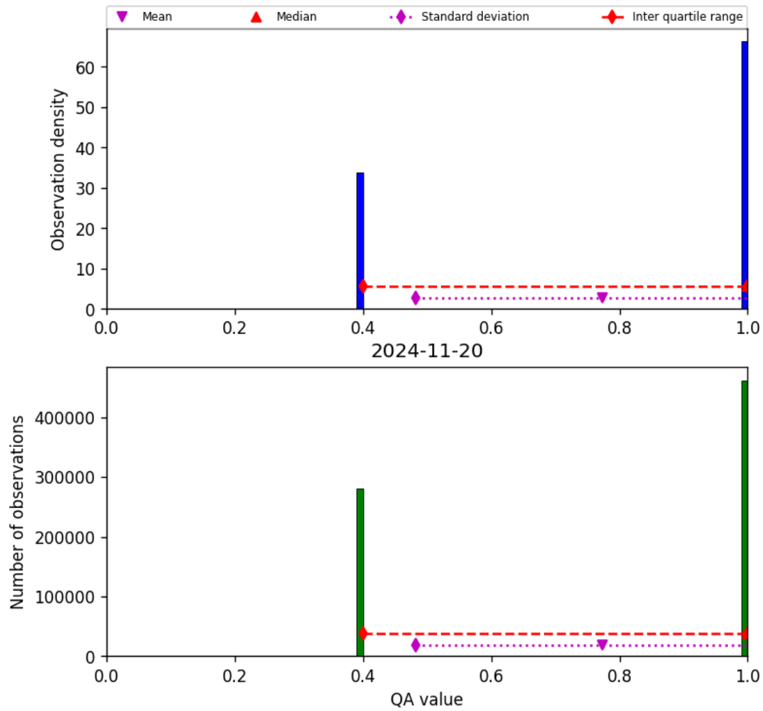
Figure 22: Histogram of “QA value” for 2024-11-20 to 2024-11-21
