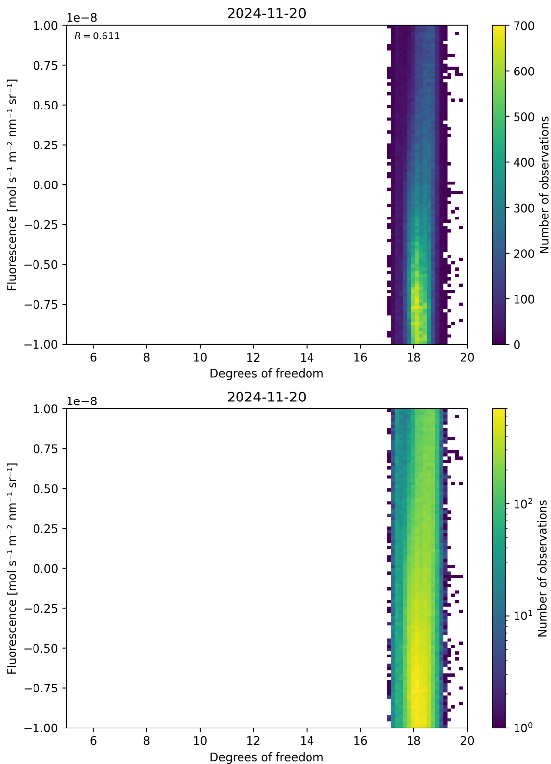
Figure 51: Scatter density plot of “Degrees of freedom” against “Fluorescence” for 2024-11-20 to 2024-11-21.
