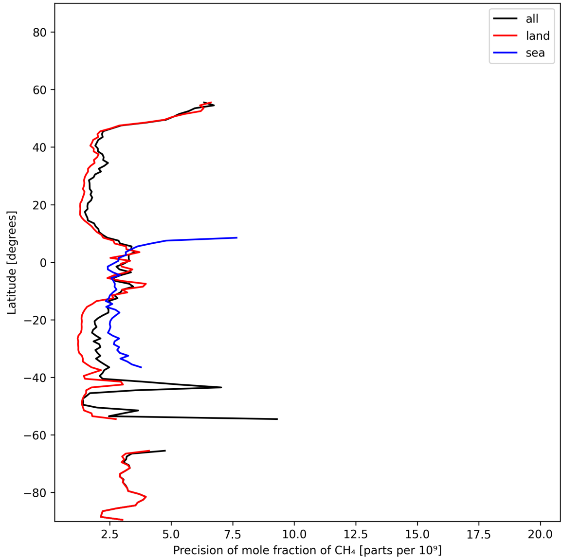
Figure 13: Zonal average of “Precision of mole fraction of CH 4 ” for 2024-11-20 to 2024-11-21.
