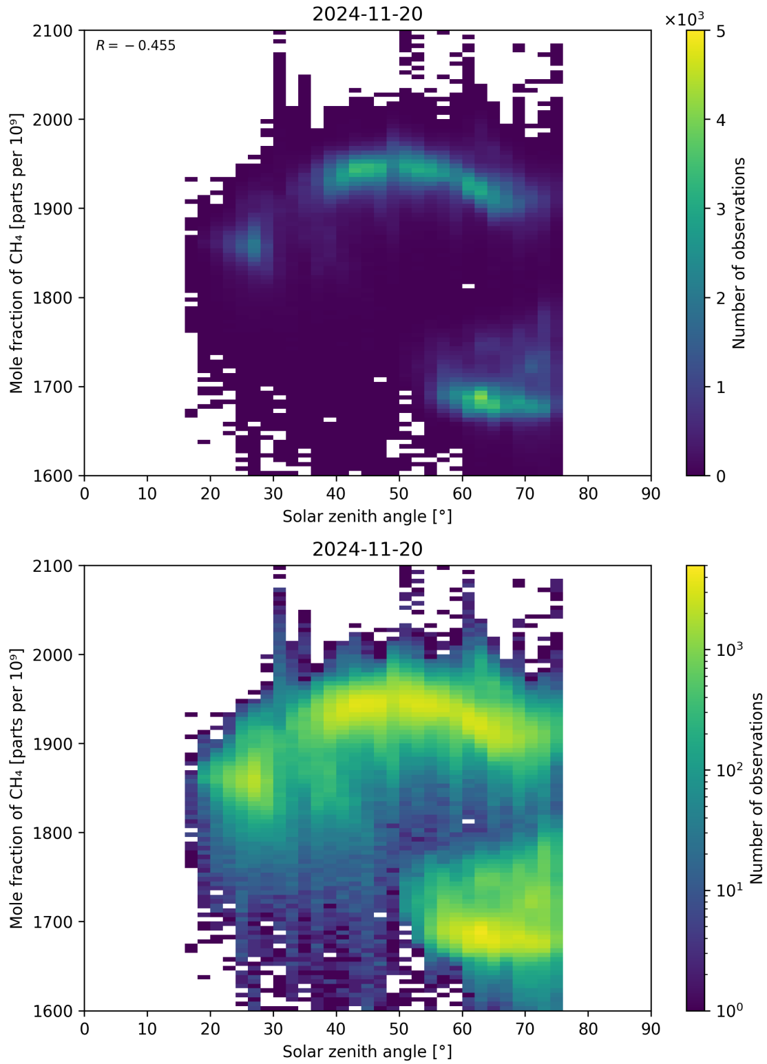
Figure 99: Scatter density plot of “Solar zenith angle” against “Mole fraction of CH 4 ” for 2024-11-20 to 2024-11-21.
