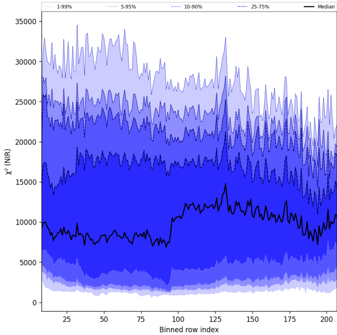
Figure 40: Along track statistics of “ \chi^2 (NIR)” for 2024-11-20 to 2024-11-21
