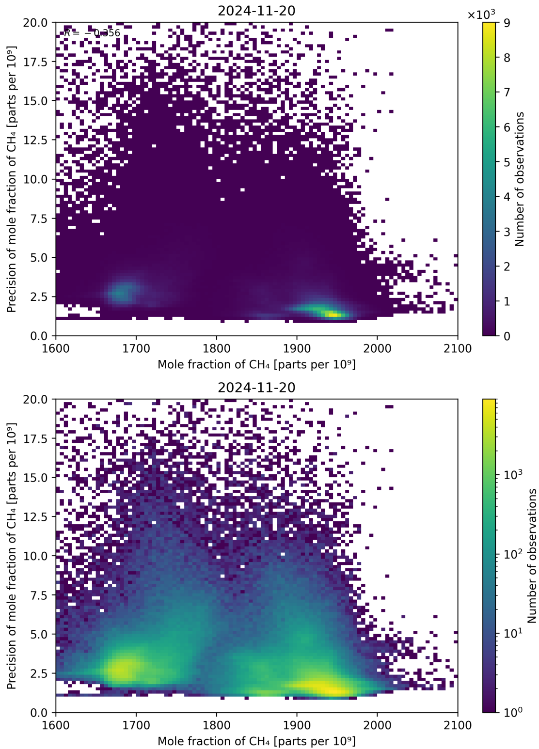
Figure 75: Scatter density plot of “Mole fraction of CH 4 ” against “Precision of mole fraction of CH 4 ” for 2024-11-20 to 2024-11-21.
