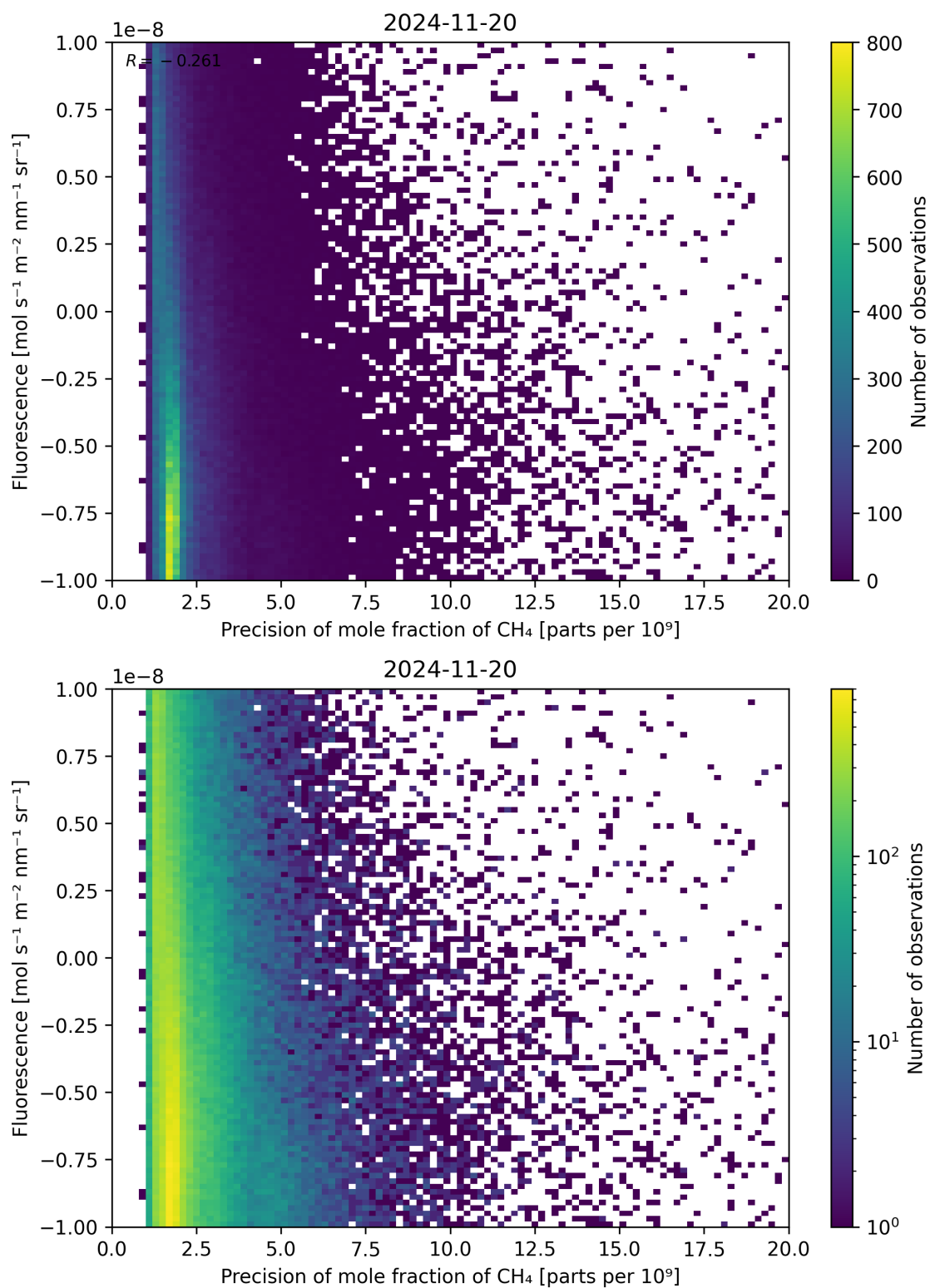
Figure 81: Scatter density plot of “Precision of mole fraction of \text{CH}_4 ” against “Fluorescence” for 2024-11-20 to 2024-11-21.
