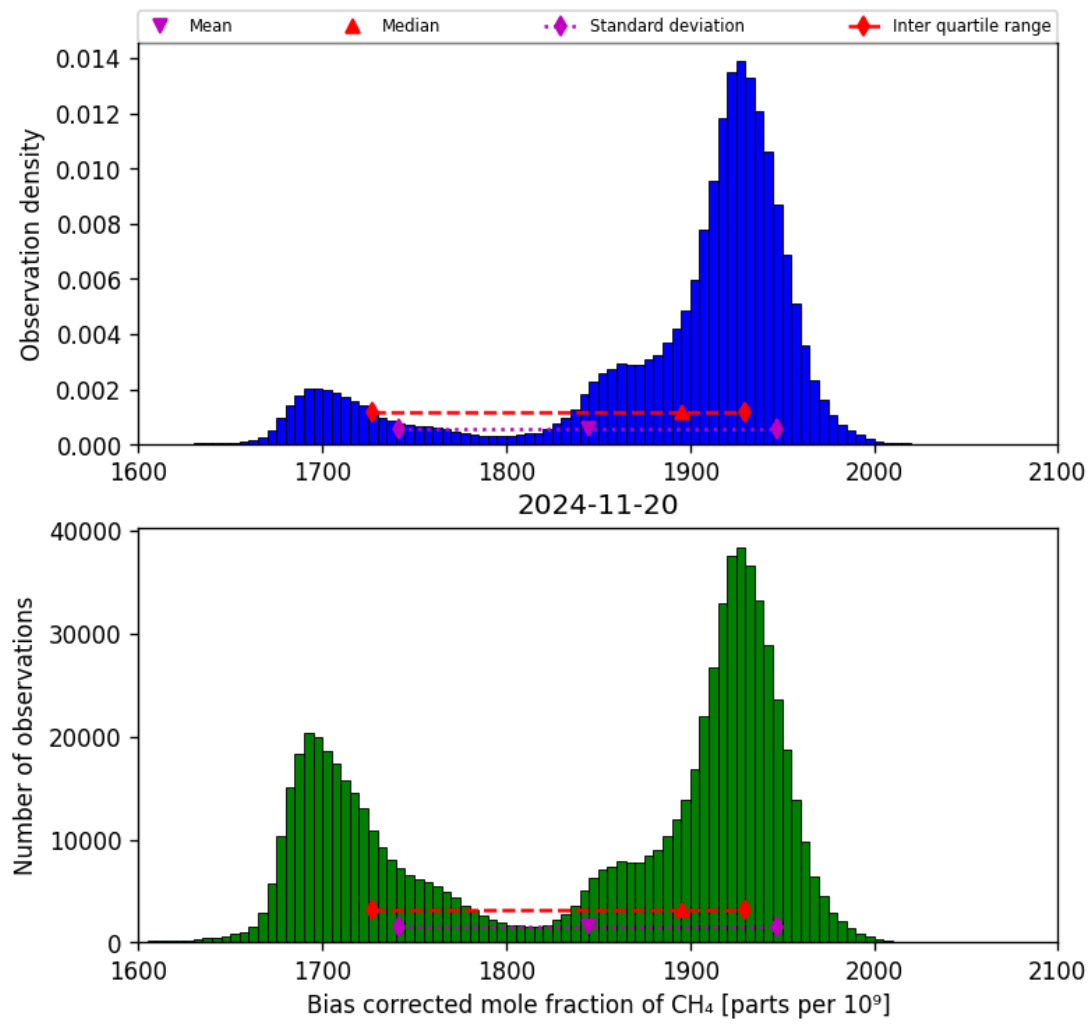
Figure 25: Histogram of “Bias corrected mole fraction of CH 4 ” for 2024-11-20 to 2024-11-21
