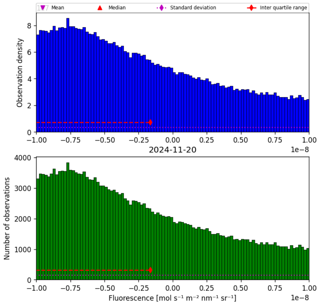
Figure 32: Histogram of “Fluorescence” for 2024-11-20 to 2024-11-21
