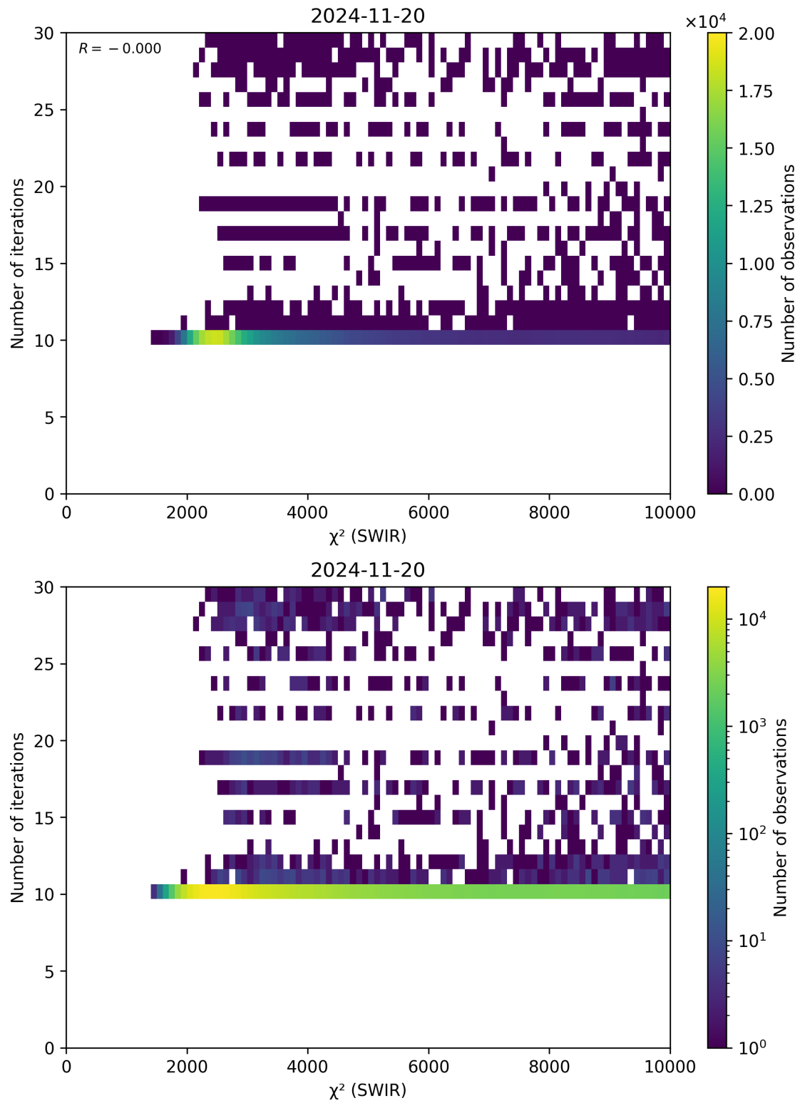
Figure 50: Scatter density plot of " \chi^2 (SWIR)" against "Number of iterations" for 2024-11-20 to 2024-11-21.
