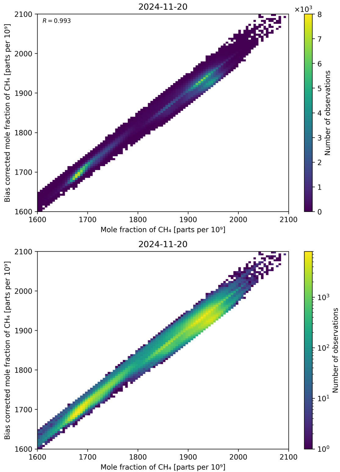
Figure 74: Scatter density plot of “Mole fraction of CH 4 ” against “Bias corrected mole fraction of CH 4 ” for 2024-11-20 to 2024-11-21.
