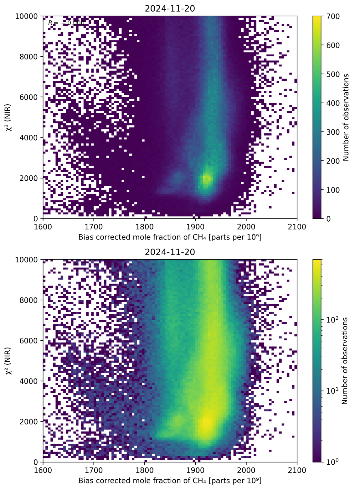
Figure 63: Scatter density plot of “Bias corrected mole fraction of CH 4 ” against “ \chi^2 (NIR)” for 2024-11-20 to 2024-11-21.
