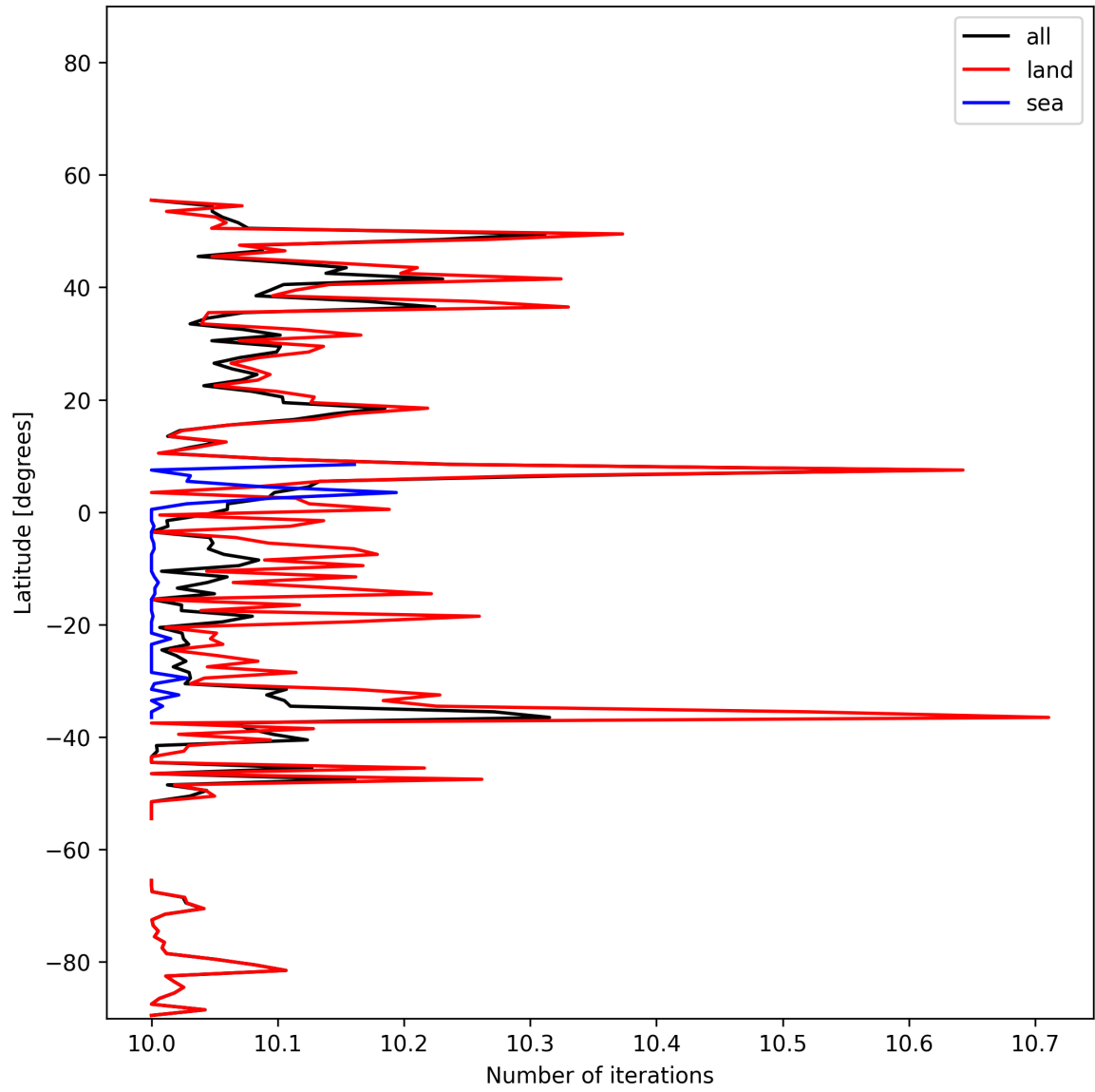
Figure 20: Zonal average of “Number of iterations” for 2024-11-20 to 2024-11-21.
