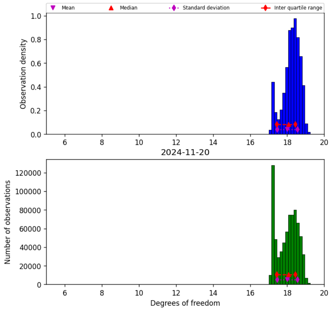
Figure 30: Histogram of “Degrees of freedom” for 2024-11-20 to 2024-11-21
