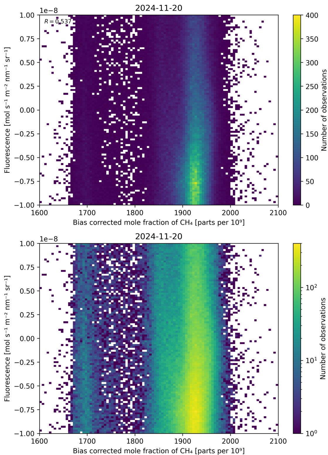
Figure 66: Scatter density plot of “Bias corrected mole fraction of \text{CH}_4 ” against “Fluorescence” for 2024-11-20 to 2024-11-21.
