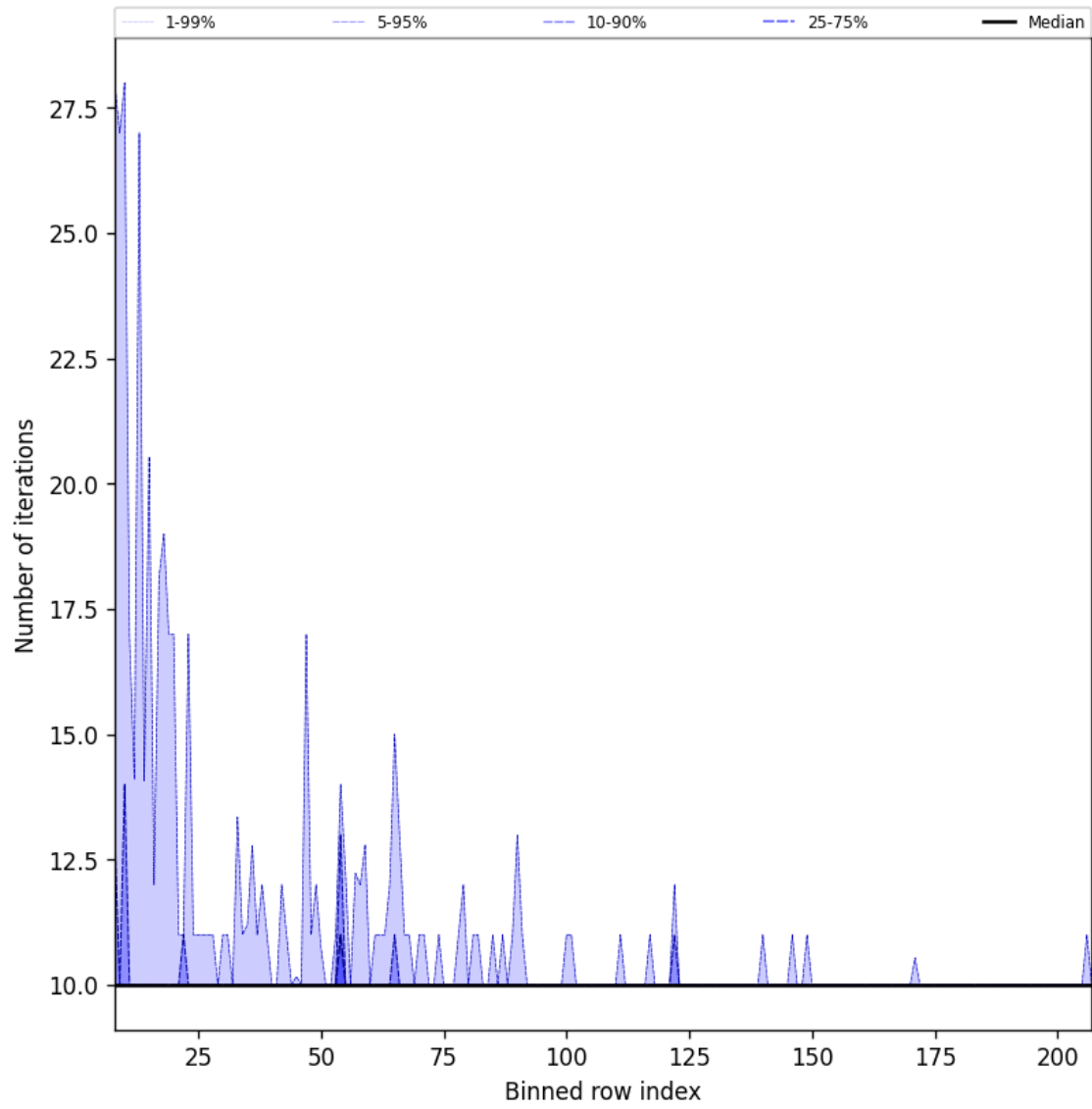
Figure 42: Along track statistics of “Number of iterations” for 2024-11-20 to 2024-11-21
