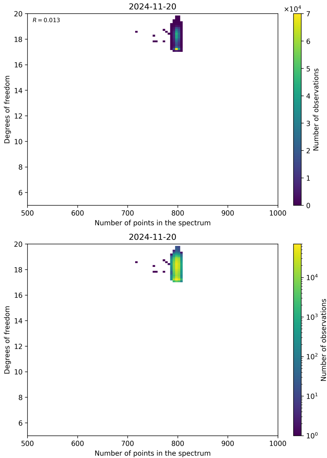
Figure 90: Scatter density plot of “Number of points in the spectrum” against “Degrees of freedom” for 2024-11-20 to 2024-11-21.
