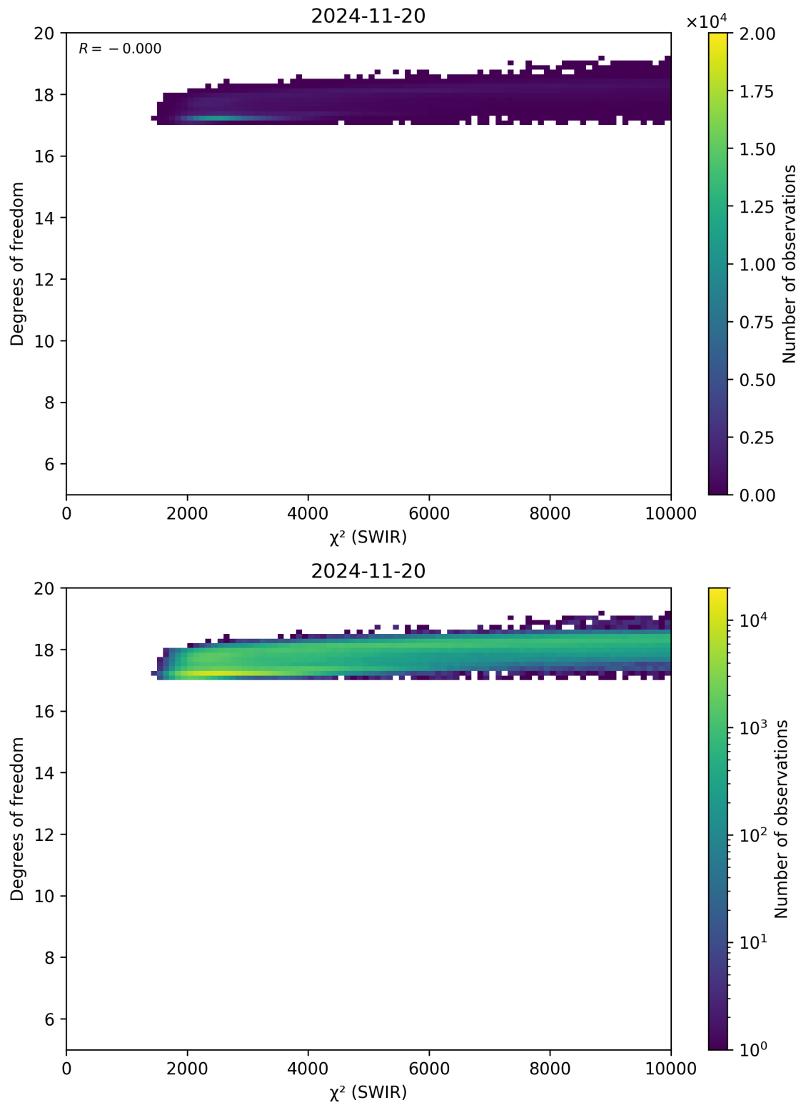
Figure 48: Scatter density plot of “ \chi^2 (SWIR)” against “Degrees of freedom” for 2024-11-20 to 2024-11-21.
