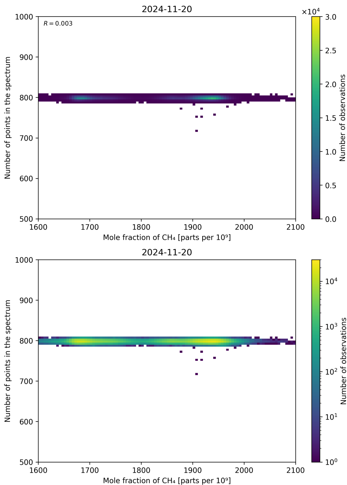
Figure 77: Scatter density plot of “Mole fraction of CH 4 ” against “Number of points in the spectrum” for 2024-11-20 to 2024-11-21.
