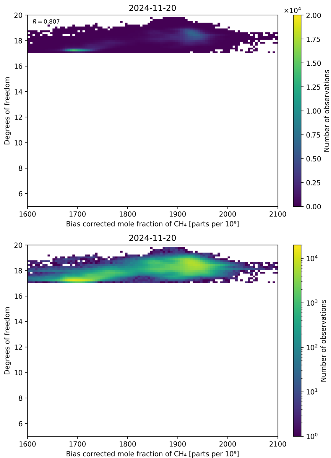
Figure 65: Scatter density plot of “Bias corrected mole fraction of CH 4 ” against “Degrees of freedom” for 2024-11-20 to 2024-11-21.
