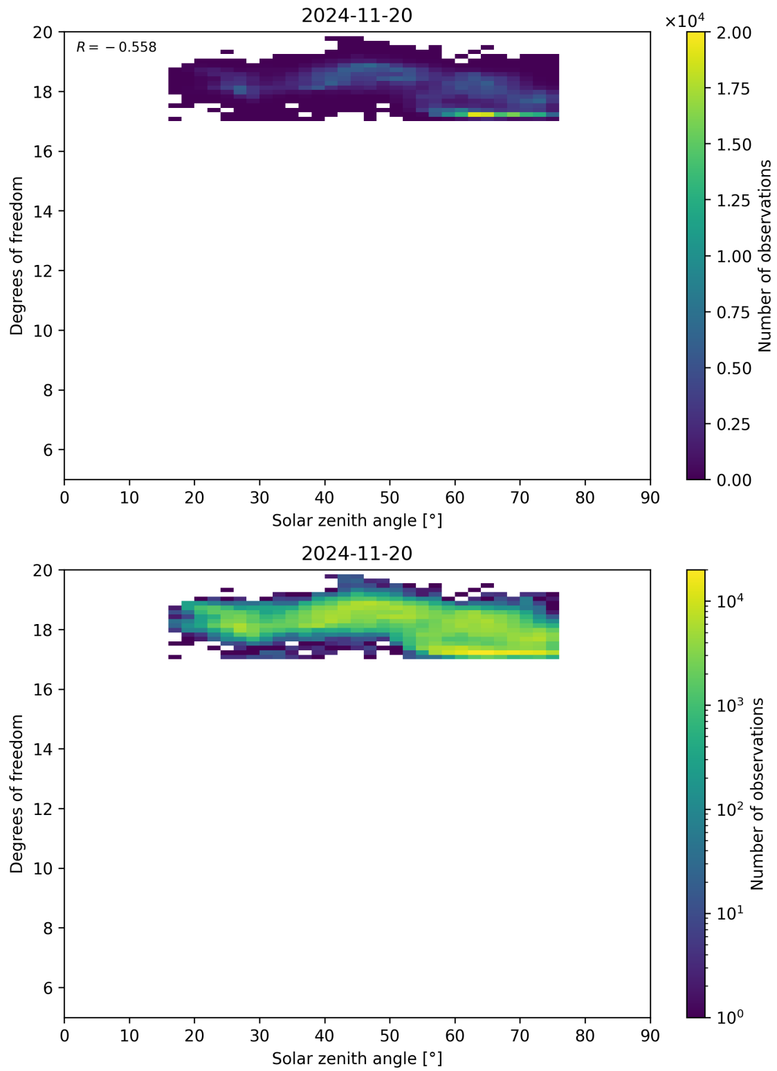
Figure 96: Scatter density plot of “Solar zenith angle” against “Degrees of freedom” for 2024-11-20 to 2024-11-21.
