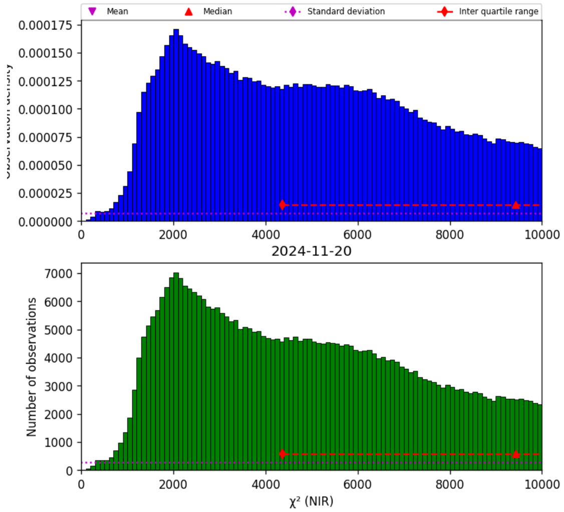
Figure 29: Histogram of “ \chi^2 (NIR)” for 2024-11-20 to 2024-11-21
