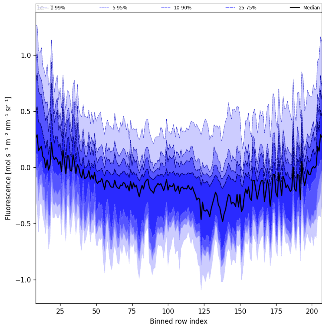
Figure 43: Along track statistics of “Fluorescence” for 2024-11-20 to 2024-11-21
