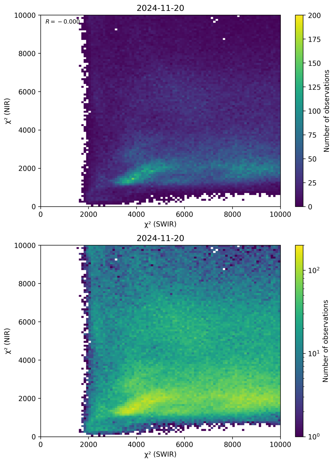
Figure 47: Scatter density plot of “ \chi^2 (SWIR)” against “ \chi^2 (NIR)” for 2024-11-20 to 2024-11-21.
