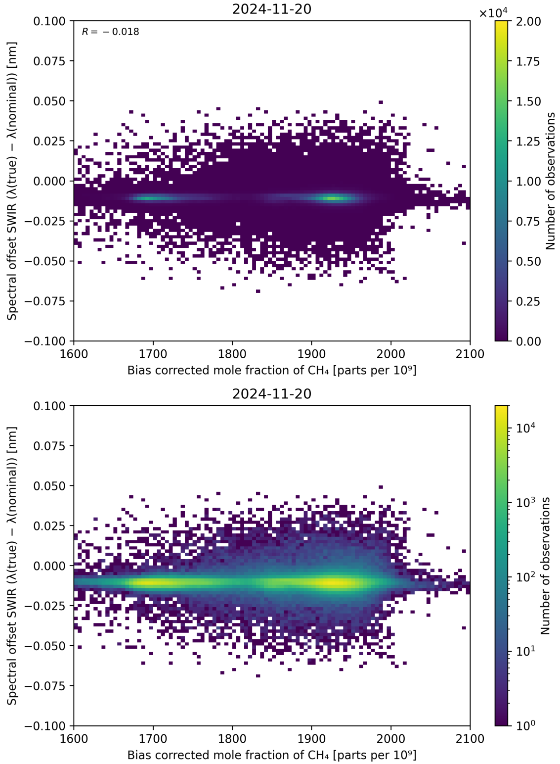
Figure 69: Scatter density plot of “Bias corrected mole fraction of \text{CH}_4 ” against “Spectral offset SWIR ( \lambda_{\text{true}} - \lambda_{\text{nominal}} )” for 2024-11-20 to 2024-11-21.
