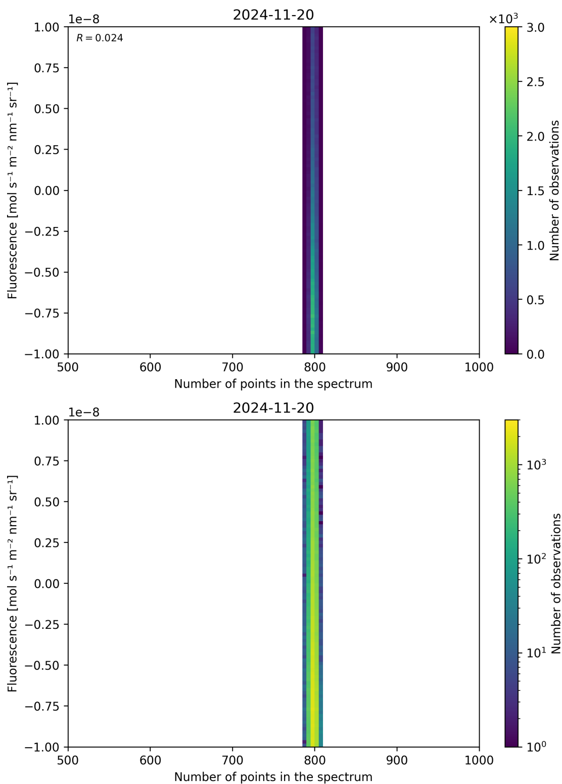
Figure 91: Scatter density plot of “Number of points in the spectrum” against “Fluorescence” for 2024-11-20 to 2024-11-21.
