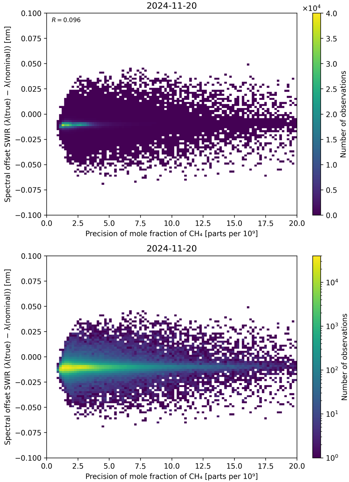
Figure 85: Scatter density plot of “Precision of mole fraction of \text{CH}_4 ” against “Spectral offset SWIR ( \lambda_{\text{true}} - \lambda_{\text{nominal}} )” for 2024-11-20 to 2024-11-21.
