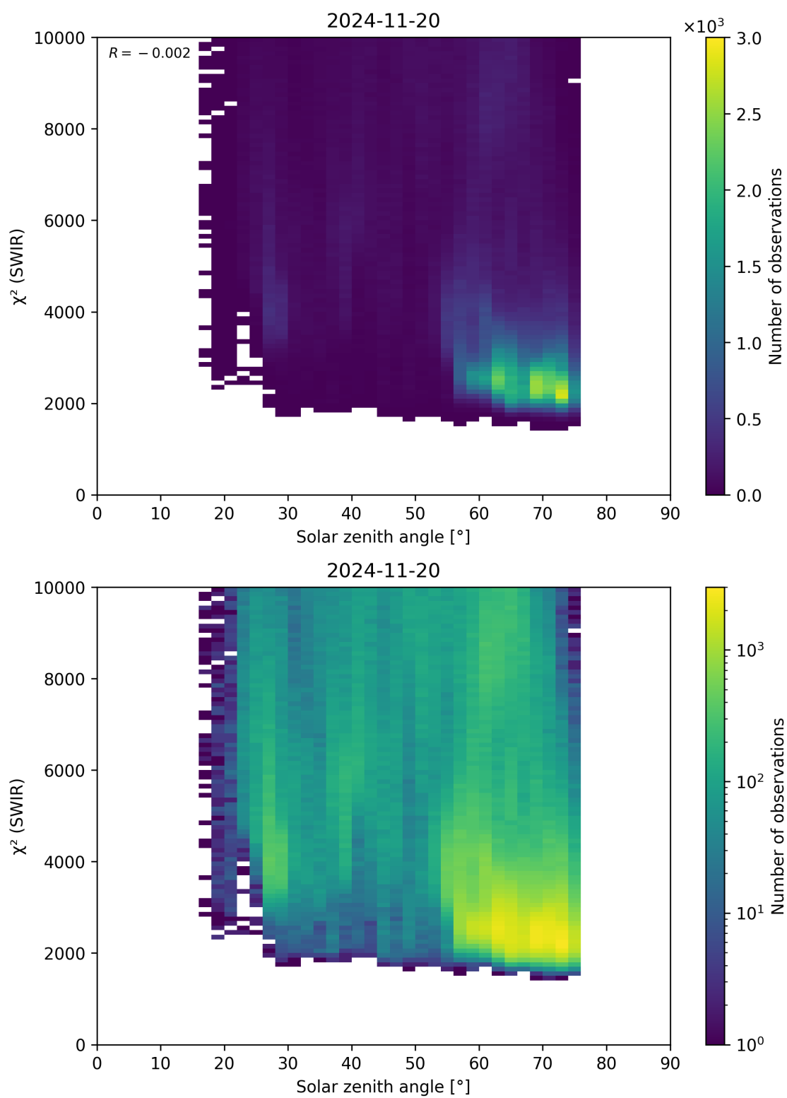
Figure 95: Scatter density plot of “Solar zenith angle” against “ \chi^2 (SWIR)” for 2024-11-20 to 2024-11-21.
