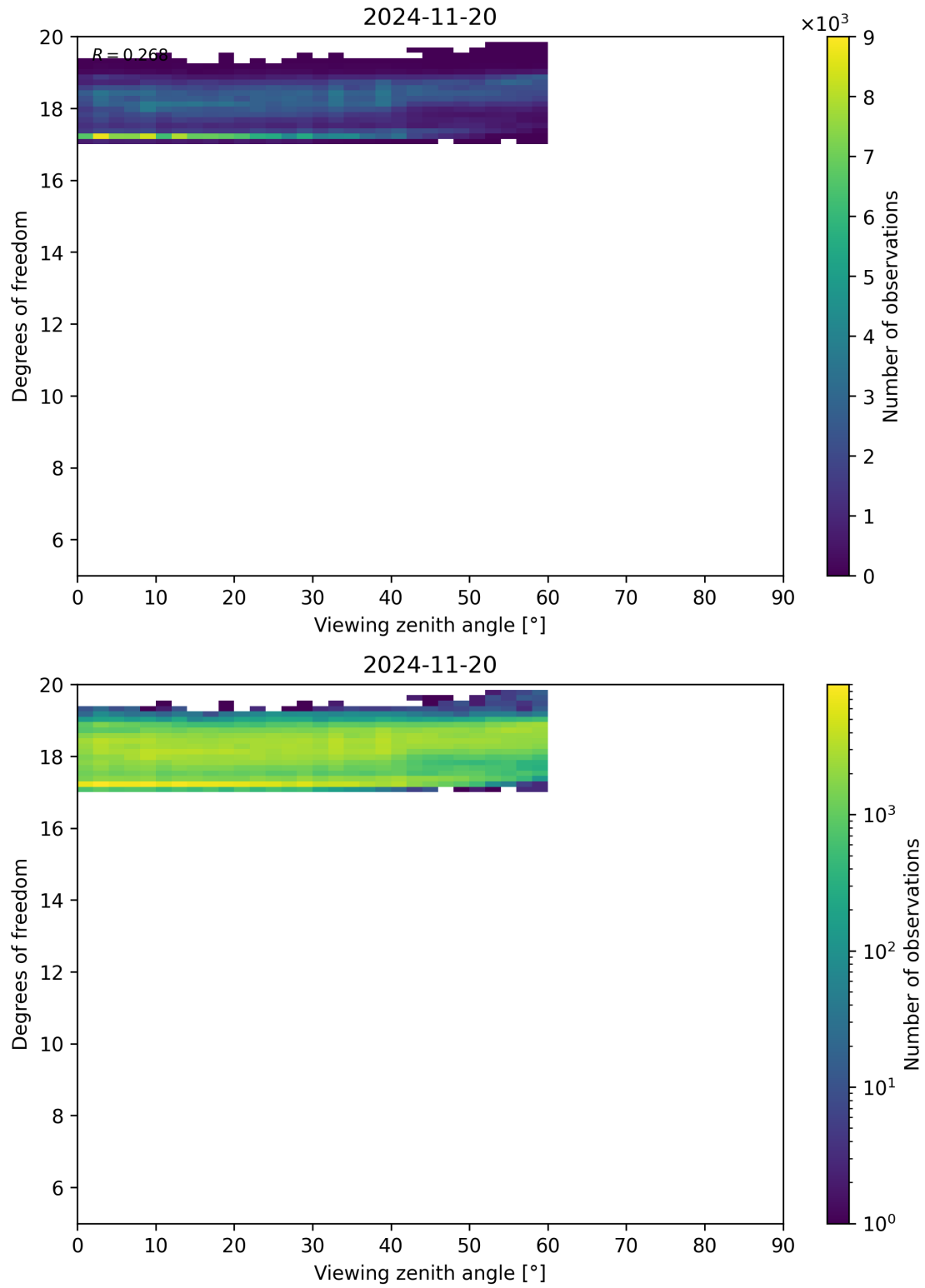
Figure 107: Scatter density plot of “Viewing zenith angle” against “Degrees of freedom” for 2024-11-20 to 2024-11-21.
