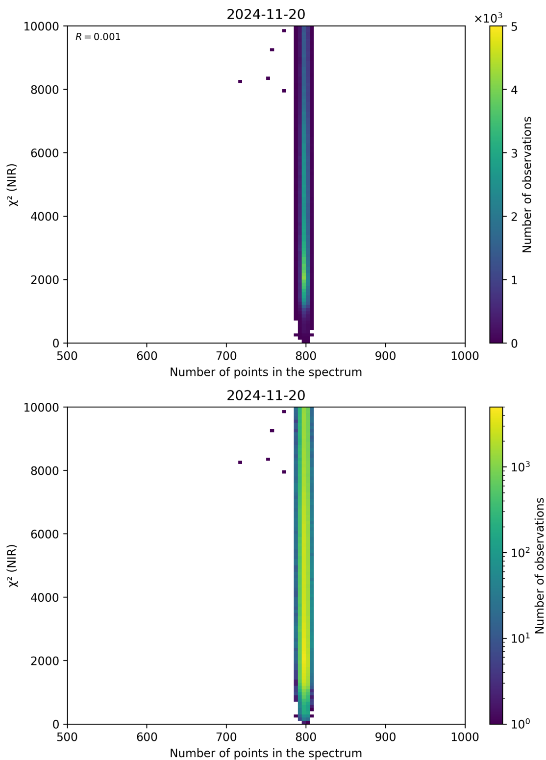
Figure 88: Scatter density plot of “Number of points in the spectrum” against “ \chi^2 (NIR)” for 2024-11-20 to 2024-11-21.
