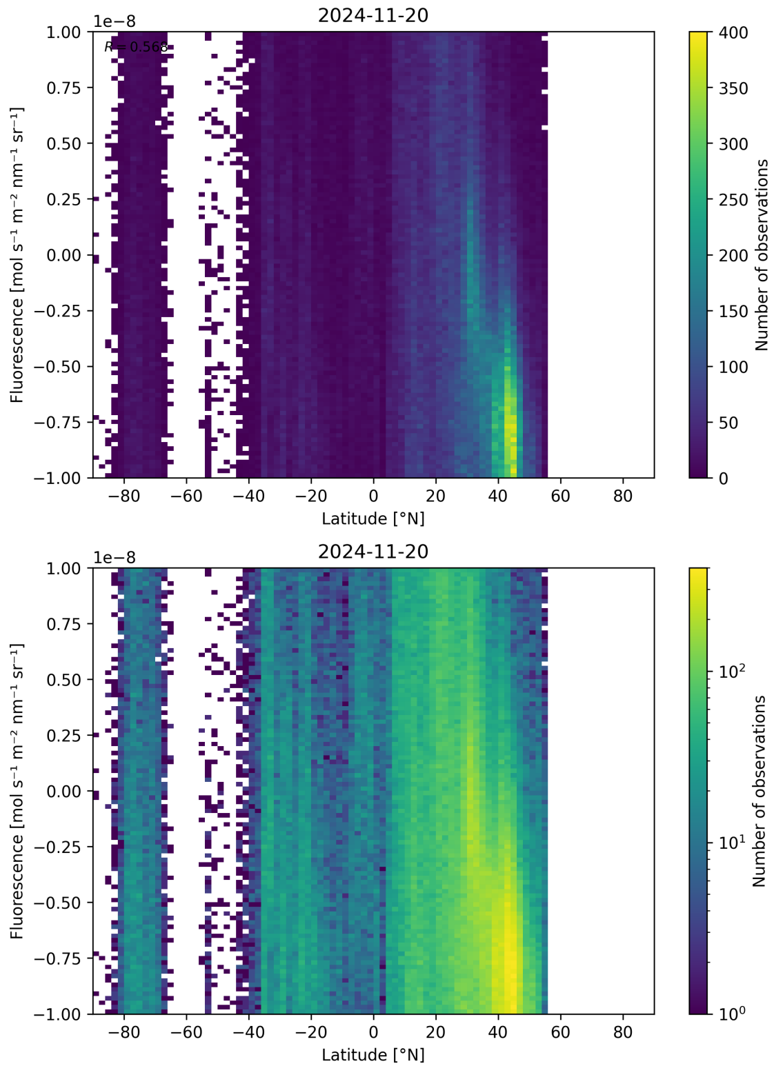
Figure 56: Scatter density plot of “Latitude” against “Fluorescence” for 2024-11-20 to 2024-11-21.
