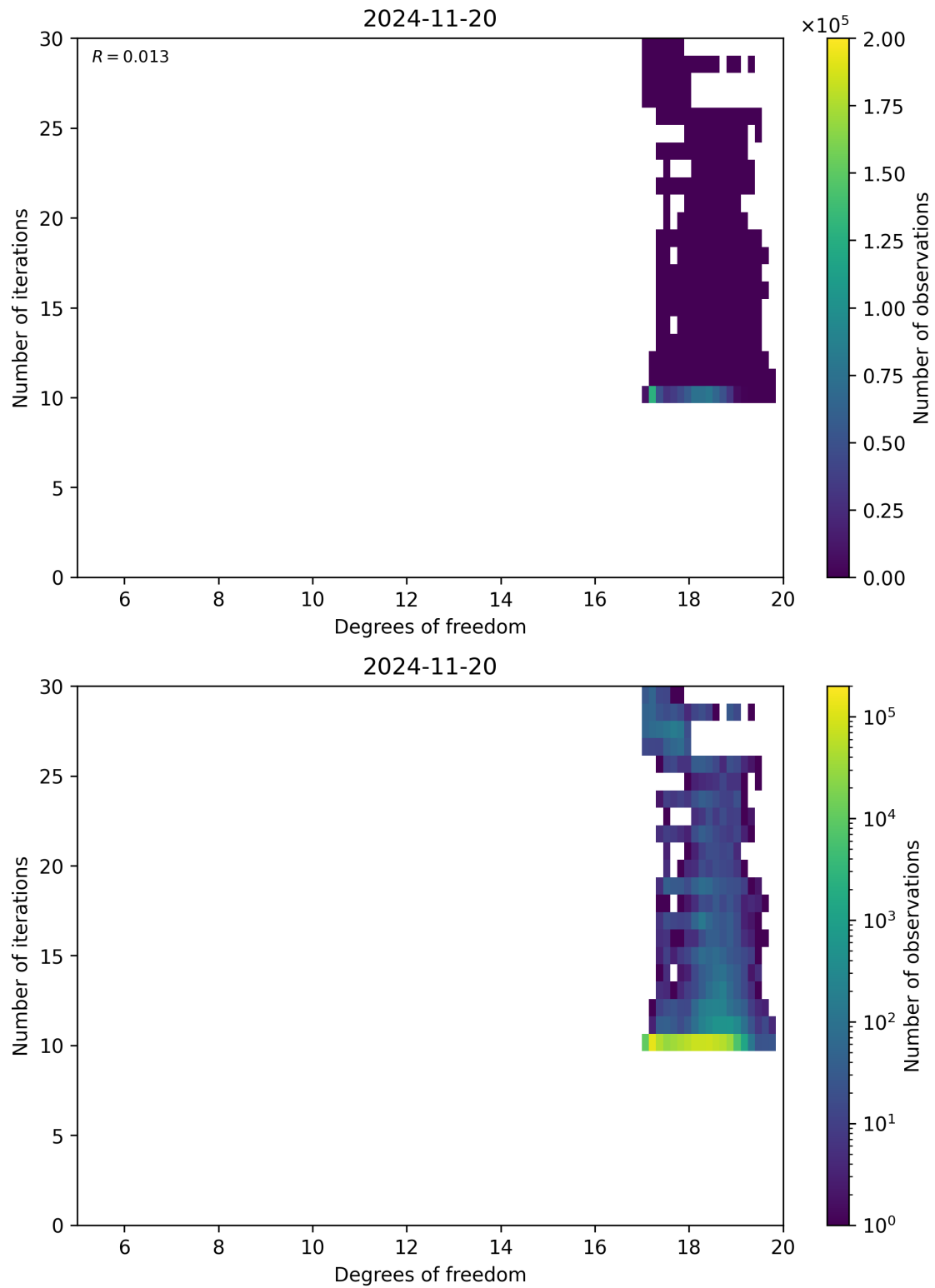
Figure 52: Scatter density plot of “Degrees of freedom” against “Number of iterations” for 2024-11-20 to 2024-11-21.
