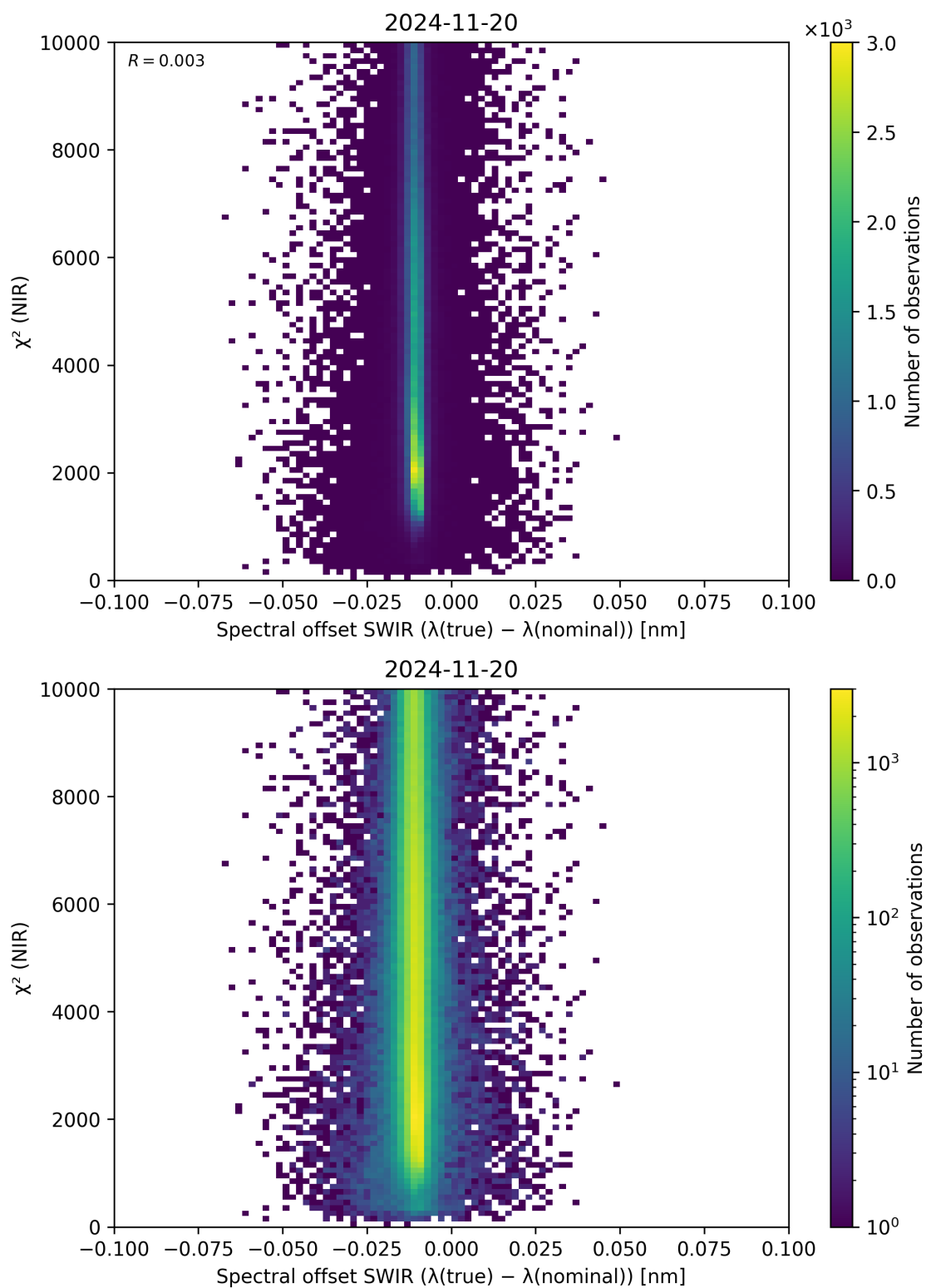
Figure 117: Scatter density plot of “Spectral offset SWIR ( \lambda_{\text{true}} - \lambda_{\text{nominal}} )” against “ \chi^2 (NIR)” for 2024-11-20 to 2024-11-21.
