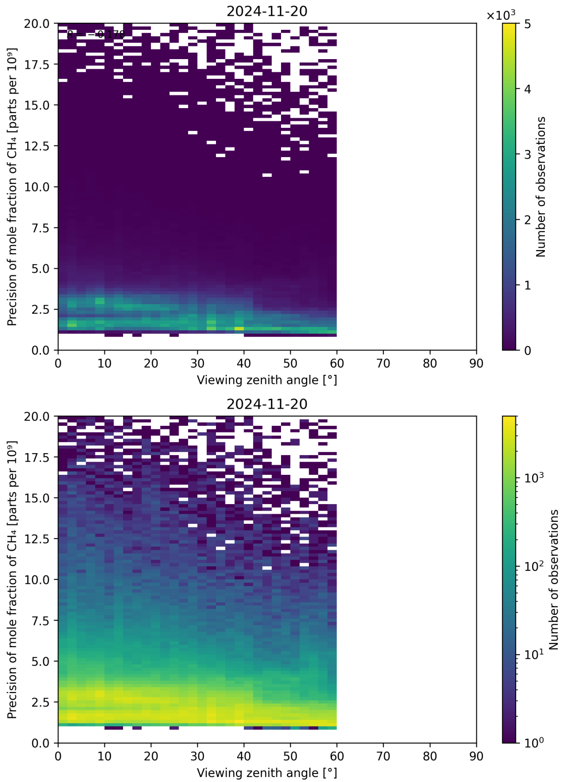
Figure 112: Scatter density plot of “Viewing zenith angle” against “Precision of mole fraction of CH 4 ” for 2024-11-20 to 2024-11-21.
