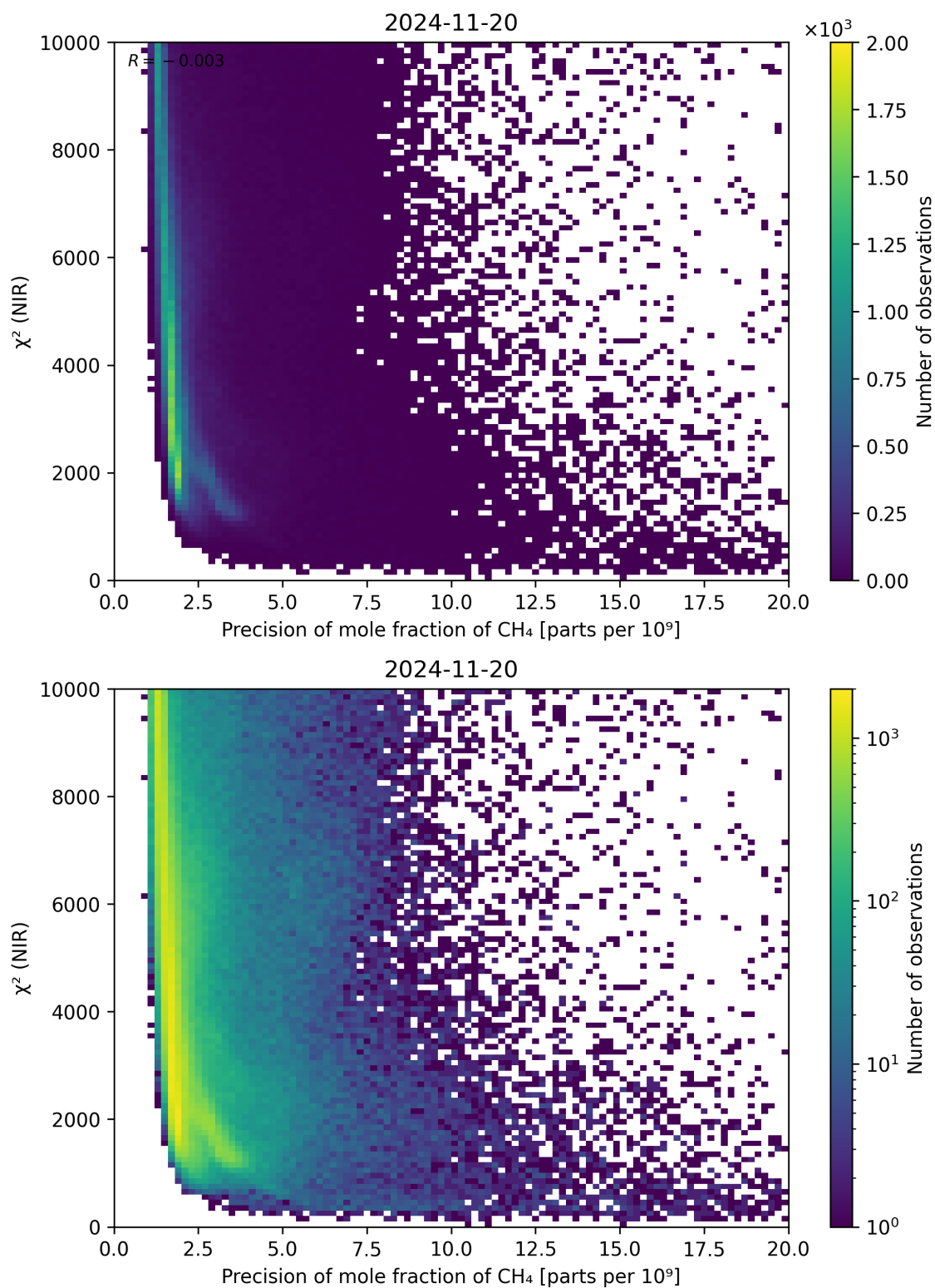
Figure 78: Scatter density plot of “Precision of mole fraction of \text{CH}_4 ” against “ \chi^2 (NIR)” for 2024-11-20 to 2024-11-21.
