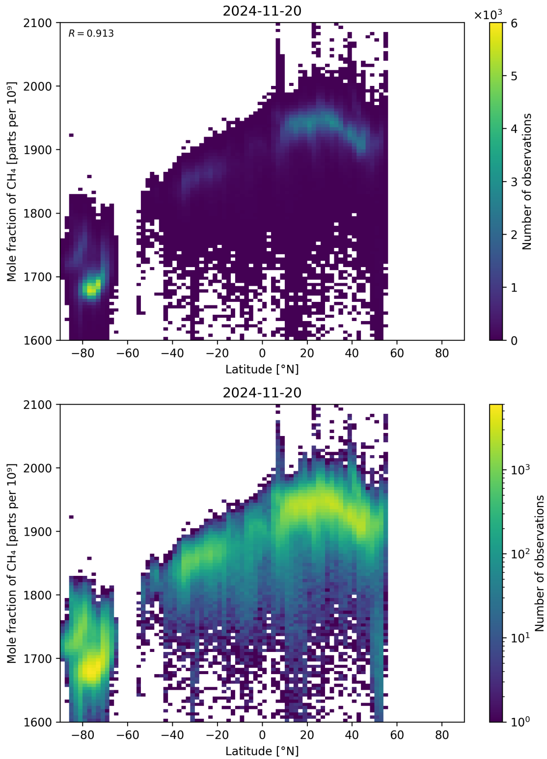
Figure 57: Scatter density plot of “Latitude” against “Mole fraction of CH 4 ” for 2024-11-20 to 2024-11-21.
