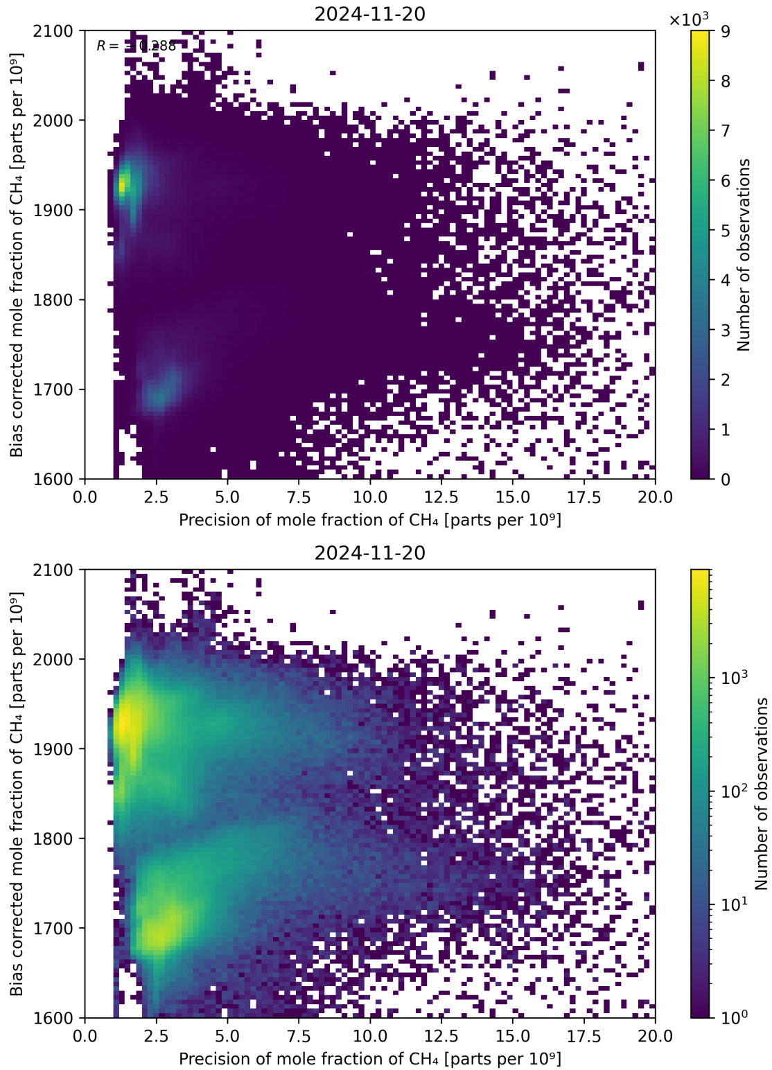
Figure 82: Scatter density plot of “Precision of mole fraction of \text{CH}_4 ” against “Bias corrected mole fraction of \text{CH}_4 ” for 2024-11-20 to 2024-11-21.
