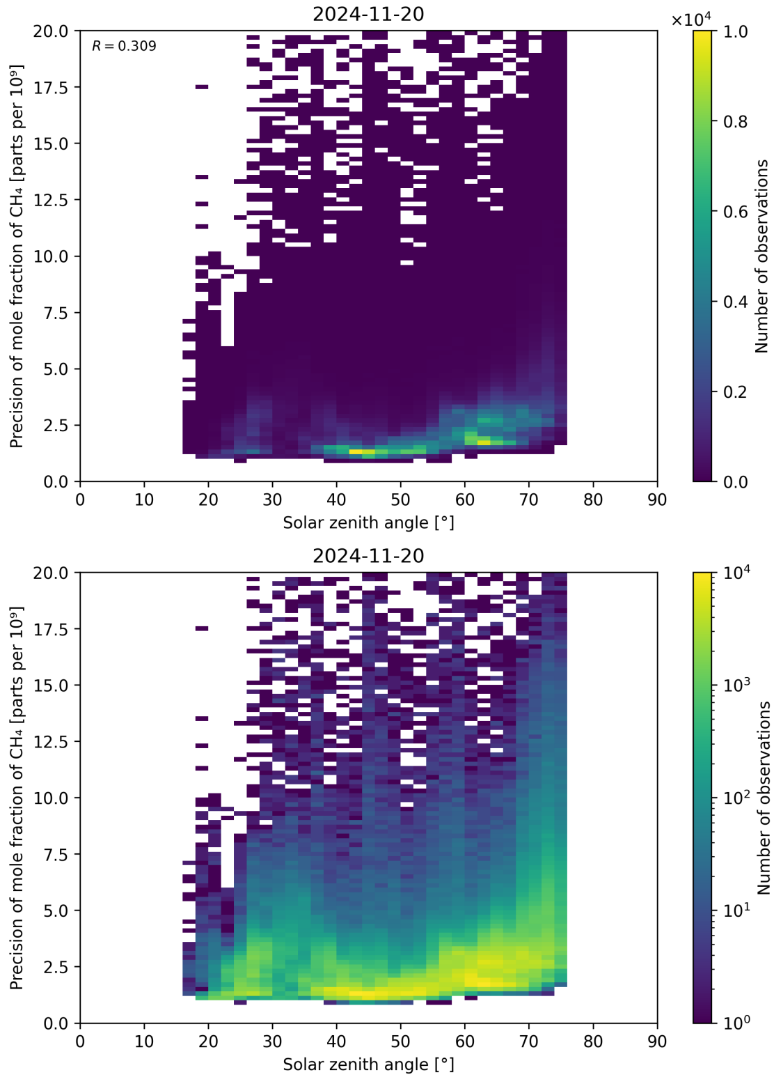
Figure 101: Scatter density plot of “Solar zenith angle” against “Precision of mole fraction of \text{CH}_4 ” for 2024-11-20 to 2024-11-21.
