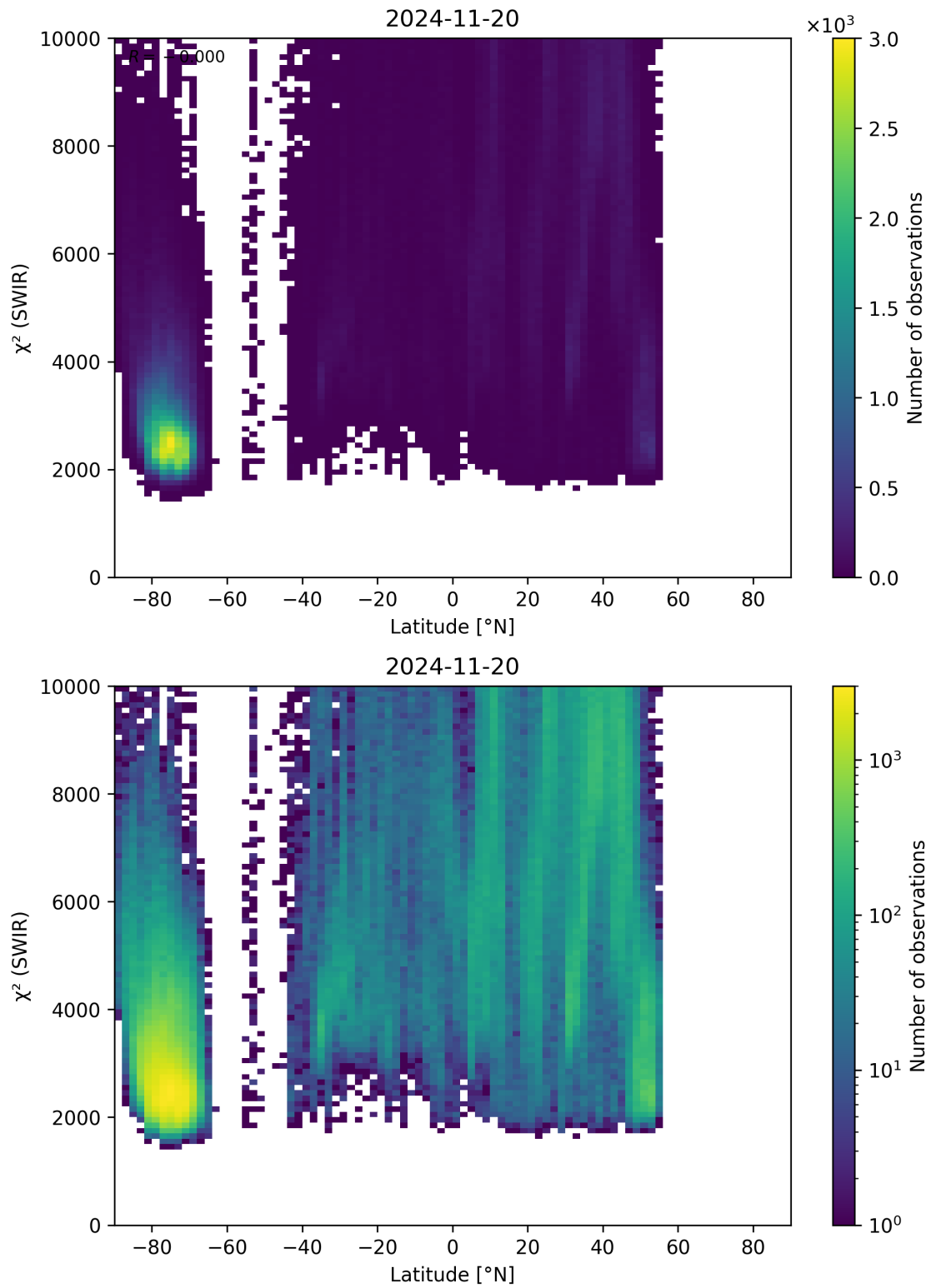
Figure 54: Scatter density plot of “Latitude” against “ \chi^2 (SWIR)” for 2024-11-20 to 2024-11-21.
