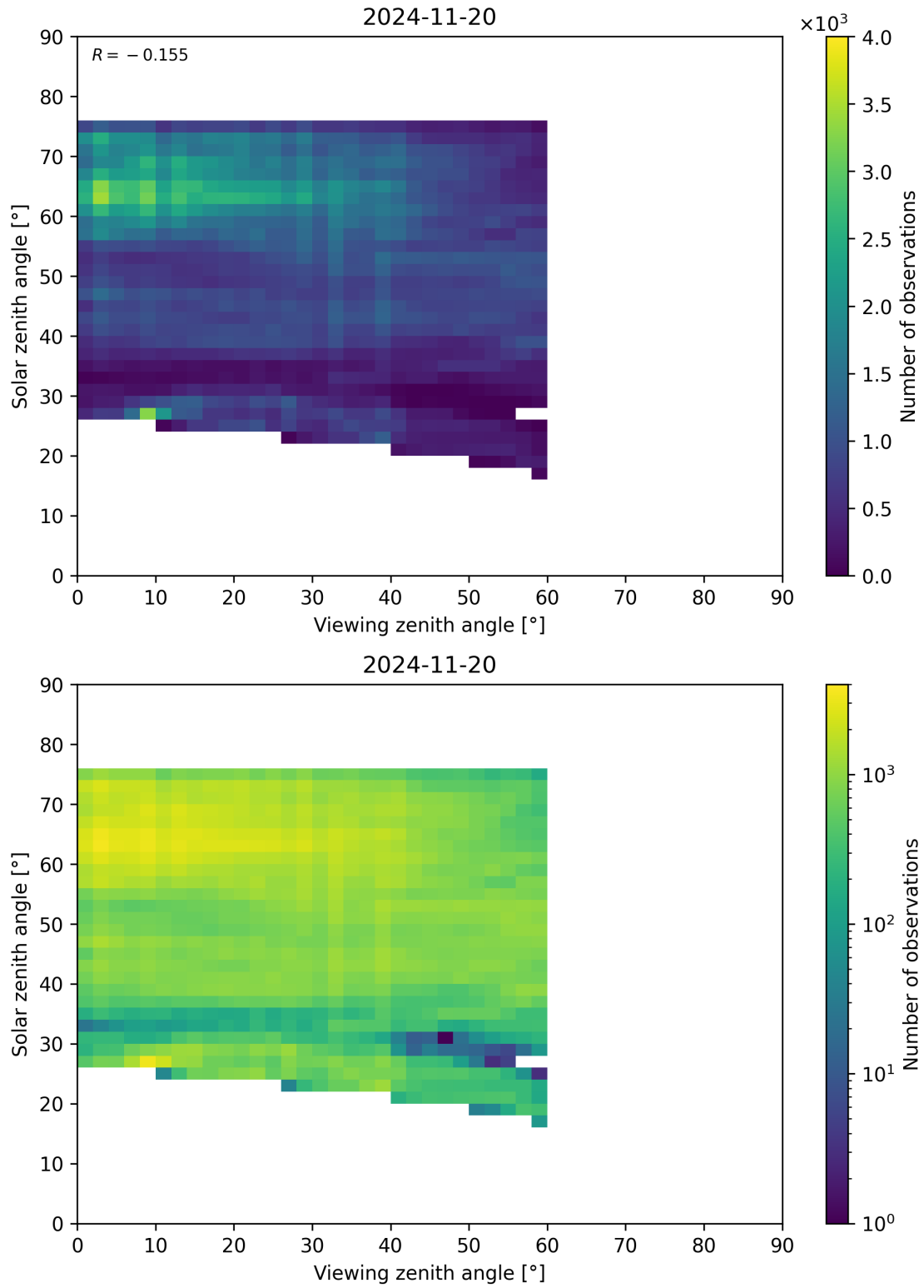
Figure 115: Scatter density plot of “Viewing zenith angle” against “Solar zenith angle” for 2024-11-20 to 2024-11-21.
