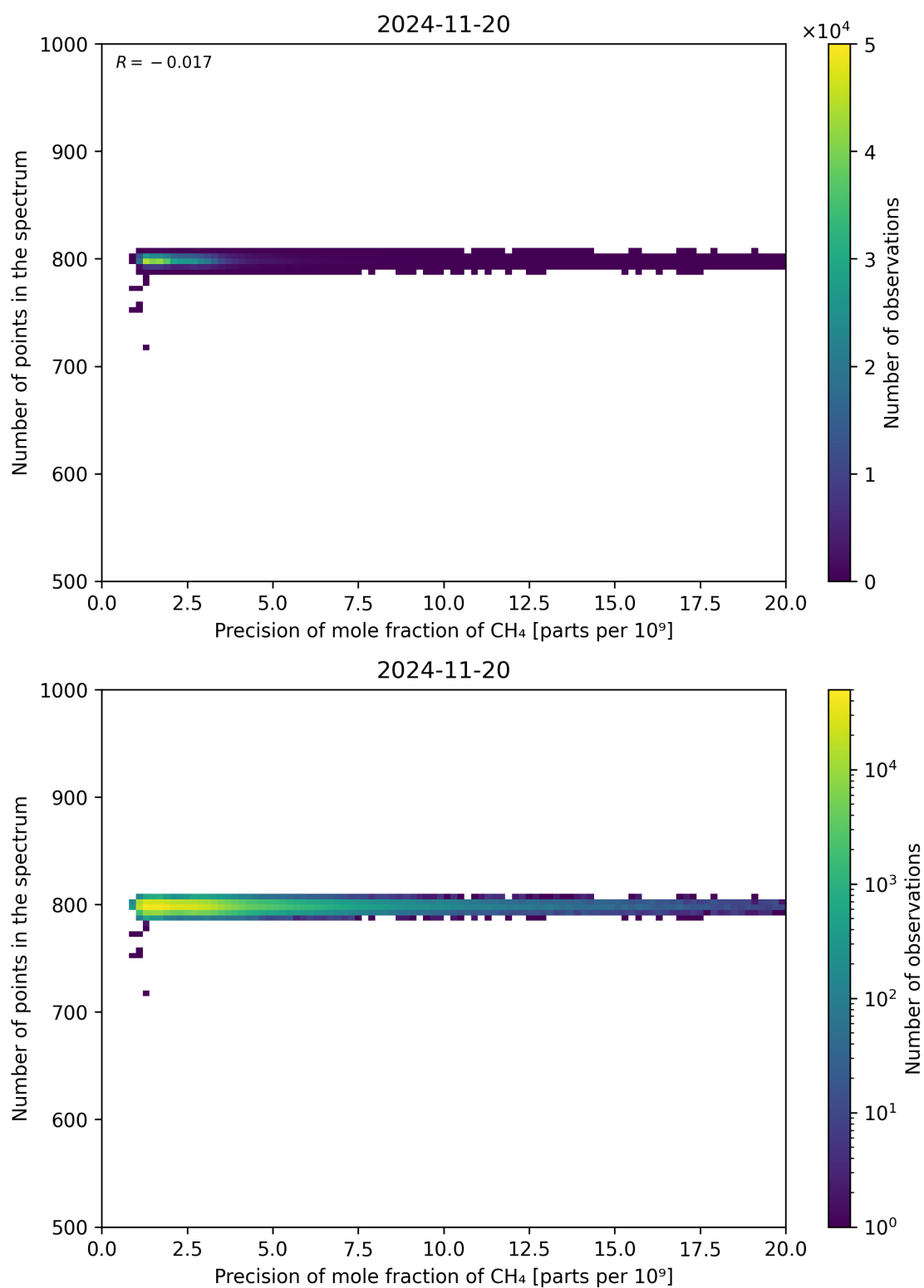
Figure 84: Scatter density plot of “Precision of mole fraction of CH 4 ” against “Number of points in the spectrum” for 2024-11-20 to 2024-11-21.
