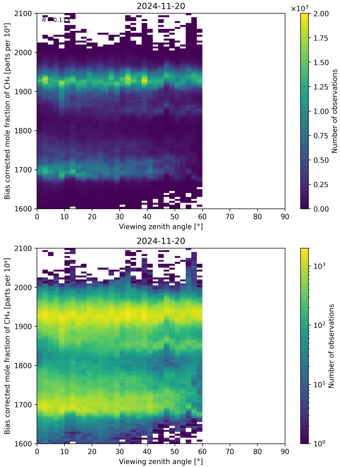
Figure 111: Scatter density plot of “Viewing zenith angle” against “Bias corrected mole fraction of CH 4 ” for 2024-11-20 to 2024-11-21.
