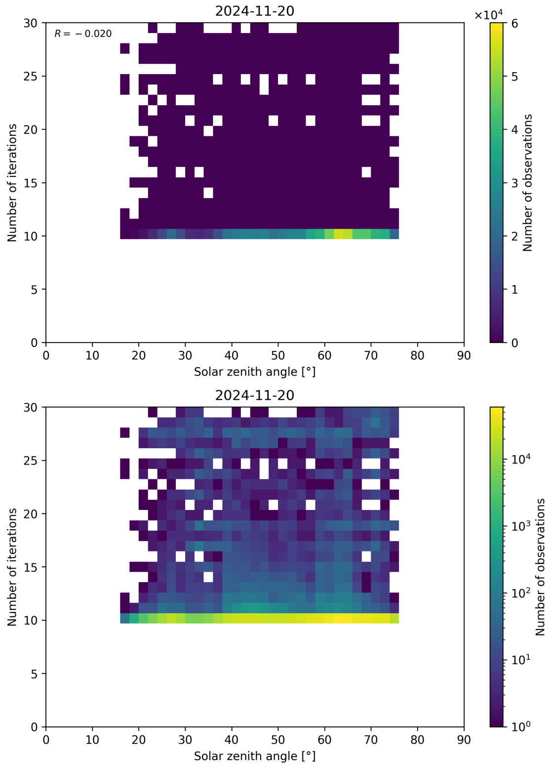
Figure 102: Scatter density plot of “Solar zenith angle” against “Number of iterations” for 2024-11-20 to 2024-11-21.
