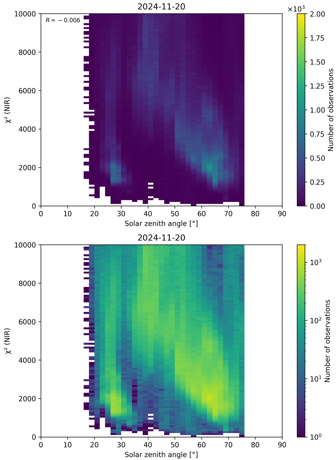
Figure 94: Scatter density plot of “Solar zenith angle” against “ \chi^2 (NIR)” for 2024-11-20 to 2024-11-21.
