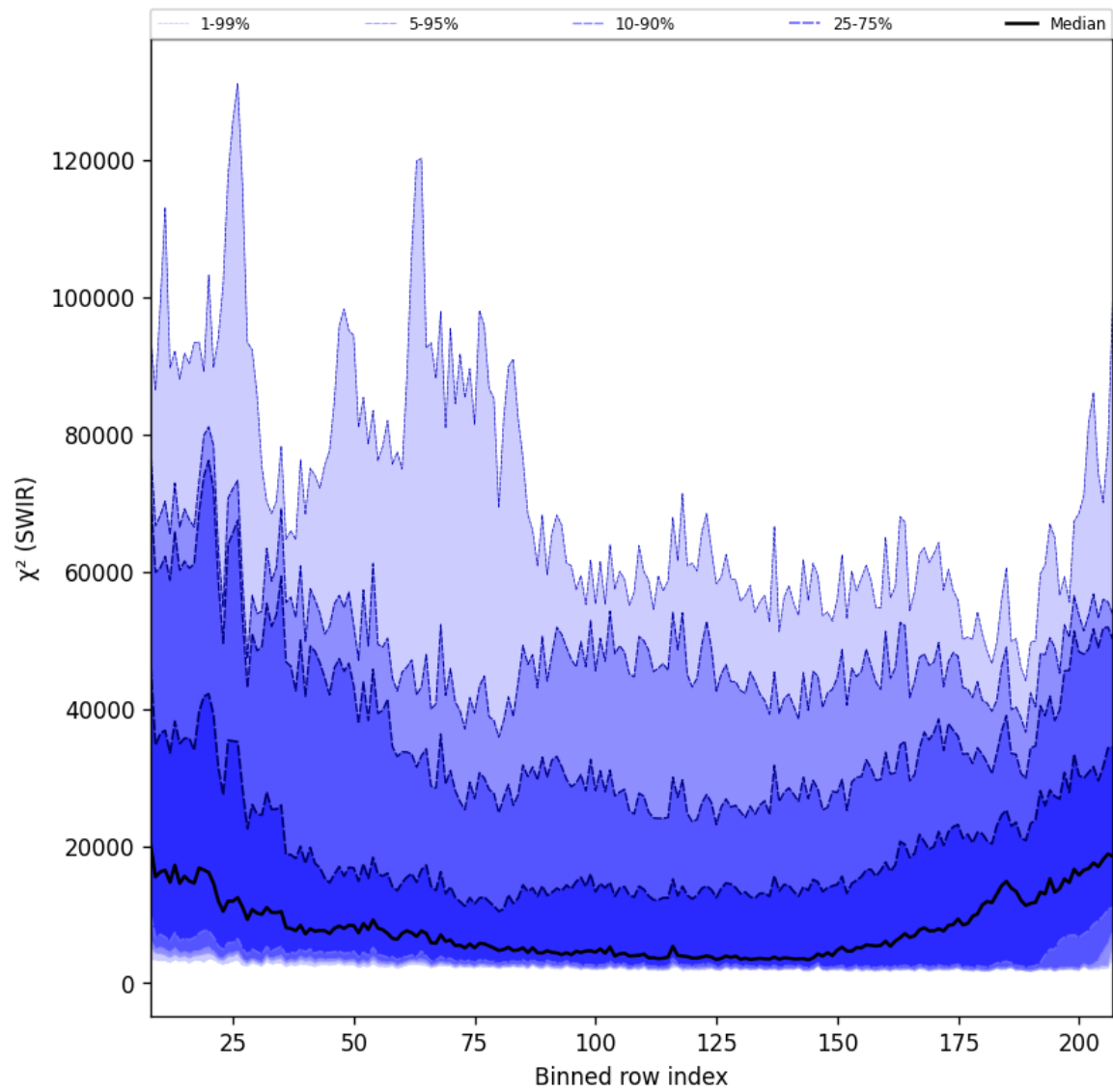
Figure 39: Along track statistics of “ \chi^2 (SWIR)” for 2024-11-20 to 2024-11-21
