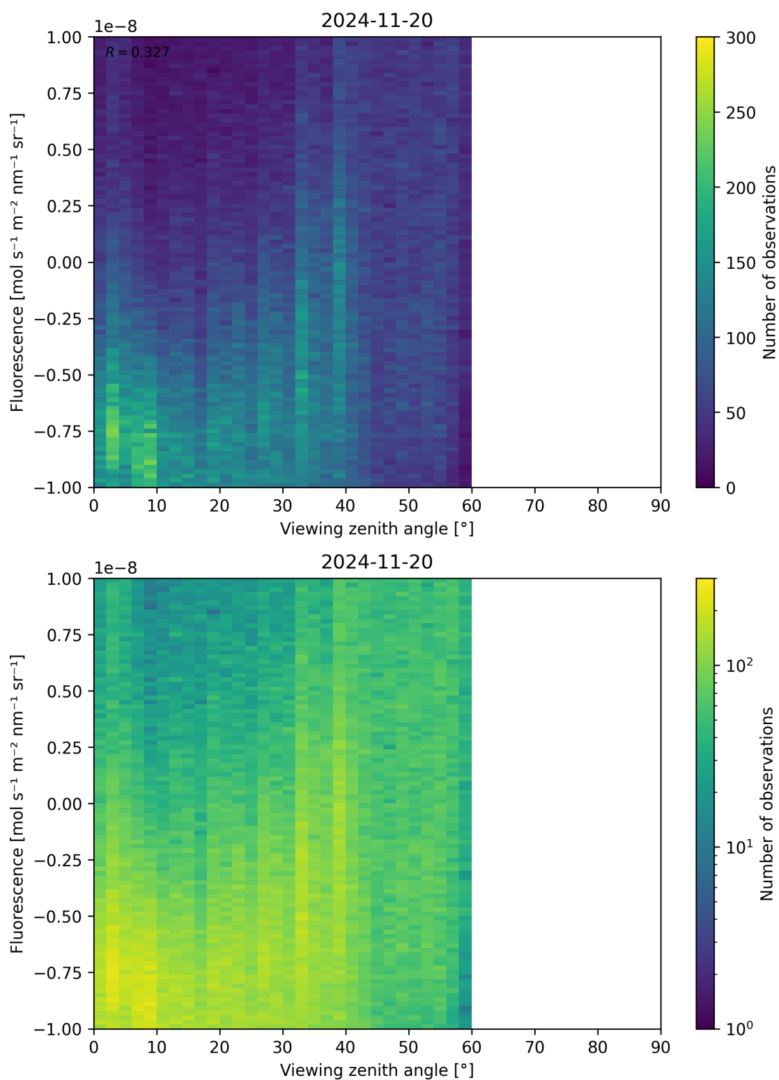
Figure 108: Scatter density plot of “Viewing zenith angle” against “Fluorescence” for 2024-11-20 to 2024-11-21.
