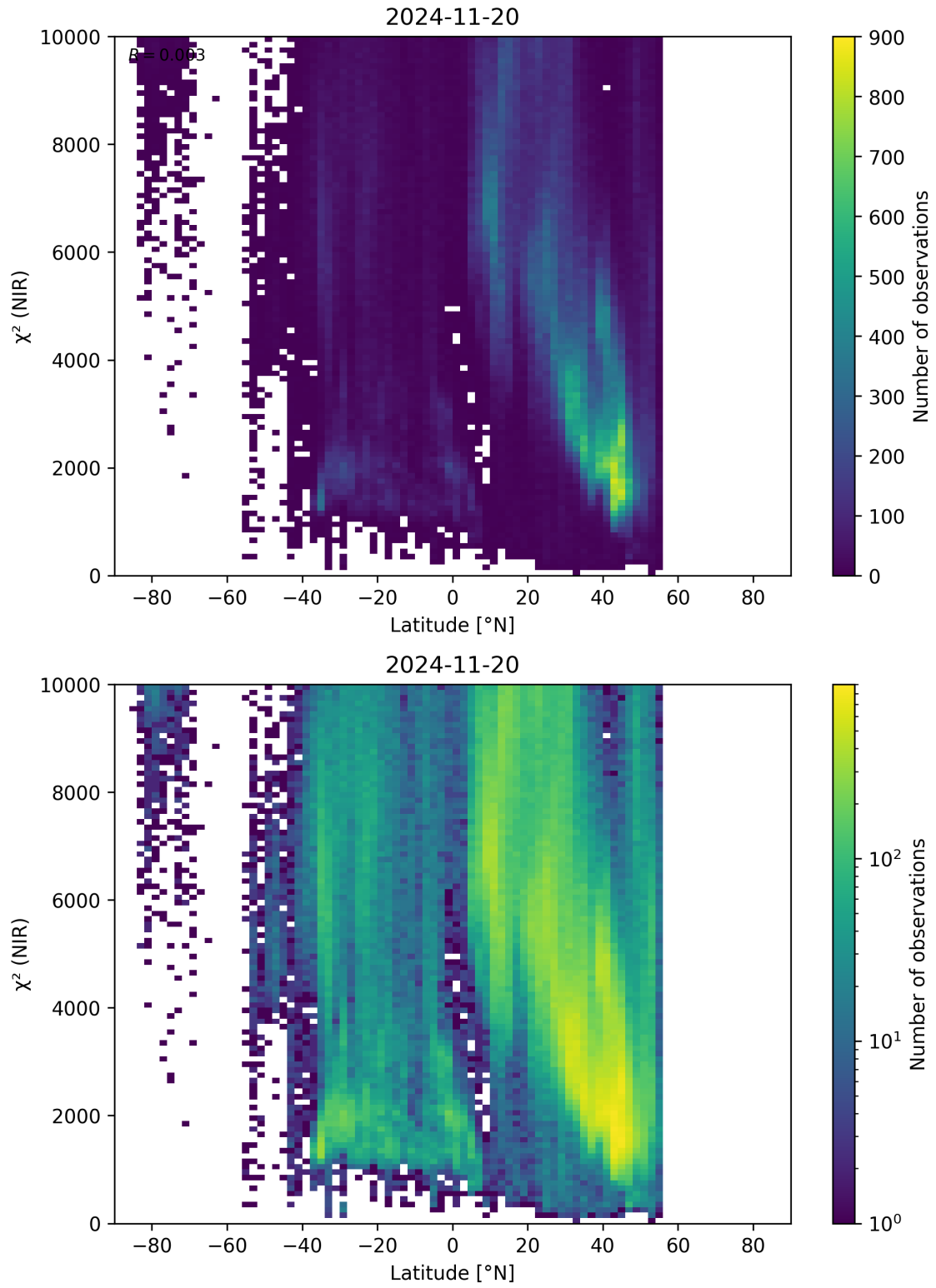
Figure 53: Scatter density plot of “Latitude” against “ \chi^2 (NIR)” for 2024-11-20 to 2024-11-21.
