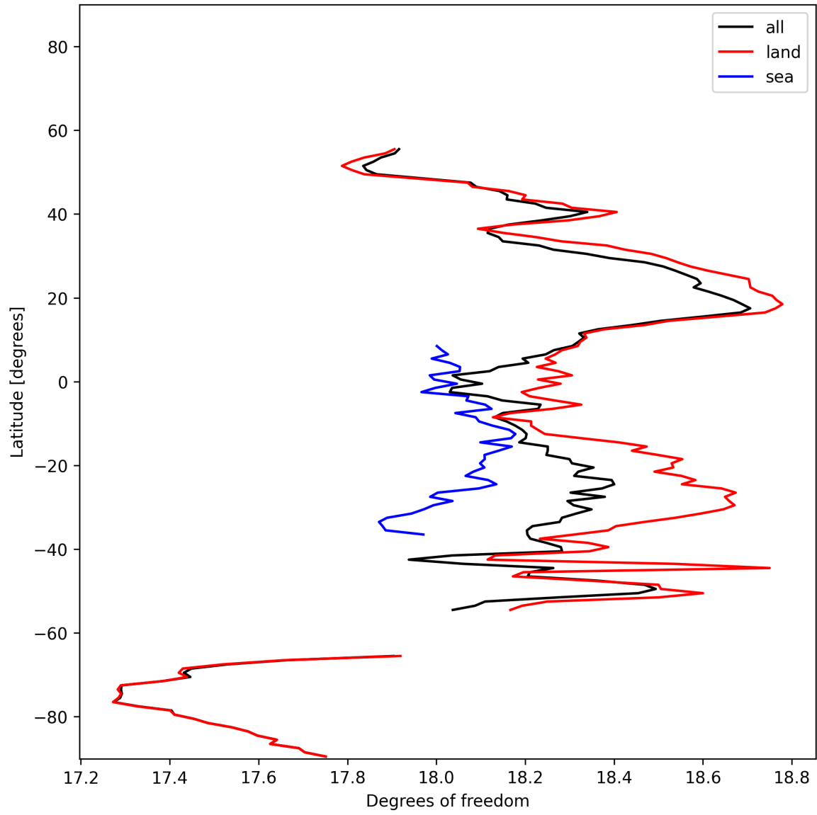
Figure 19: Zonal average of “Degrees of freedom” for 2024-11-20 to 2024-11-21.
