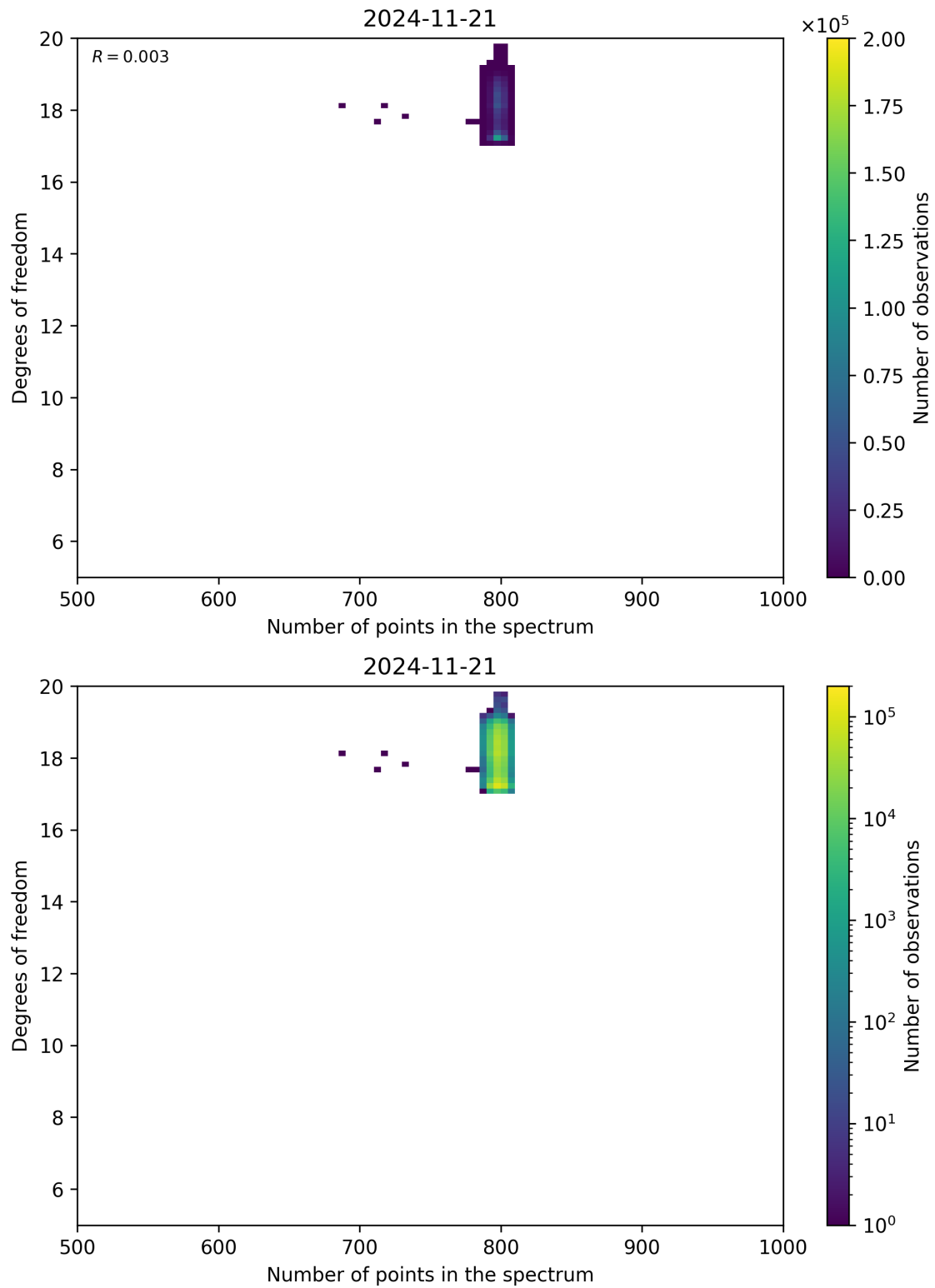
Figure 90: Scatter density plot of “Number of points in the spectrum” against “Degrees of freedom” for 2024-11-20 to 2024-11-22.
