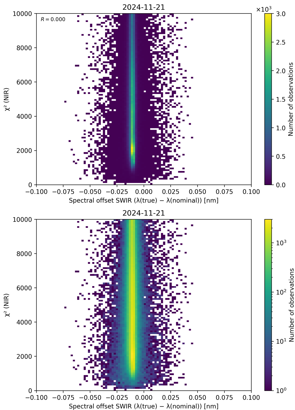
Figure 117: Scatter density plot of “Spectral offset SWIR ( \lambda_{\text{true}} - \lambda_{\text{nominal}} )” against “ \chi^2 (NIR)” for 2024-11-20 to 2024-11-22.
