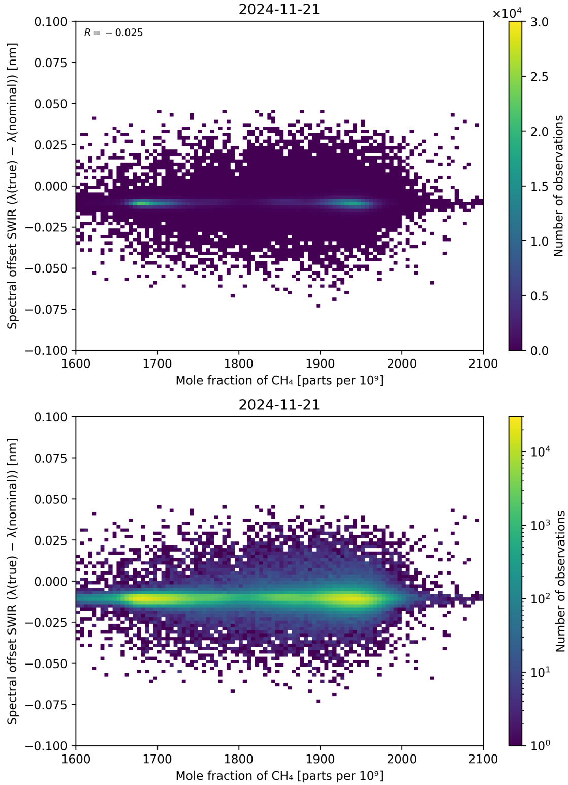
Figure 86: Scatter density plot of “Mole fraction of CH 4 ” against “Spectral offset SWIR ( \lambda_{\text{true}} - \lambda_{\text{nominal}} )” for 2024-11-20 to 2024-11-22.
