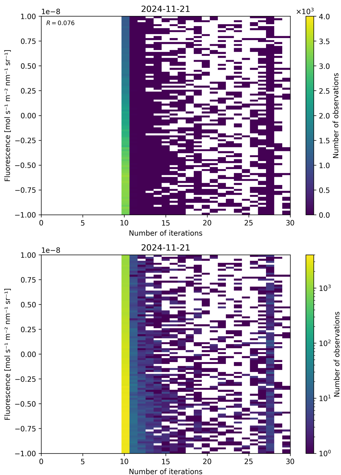
Figure 87: Scatter density plot of “Number of iterations” against “Fluorescence” for 2024-11-20 to 2024-11-22.
