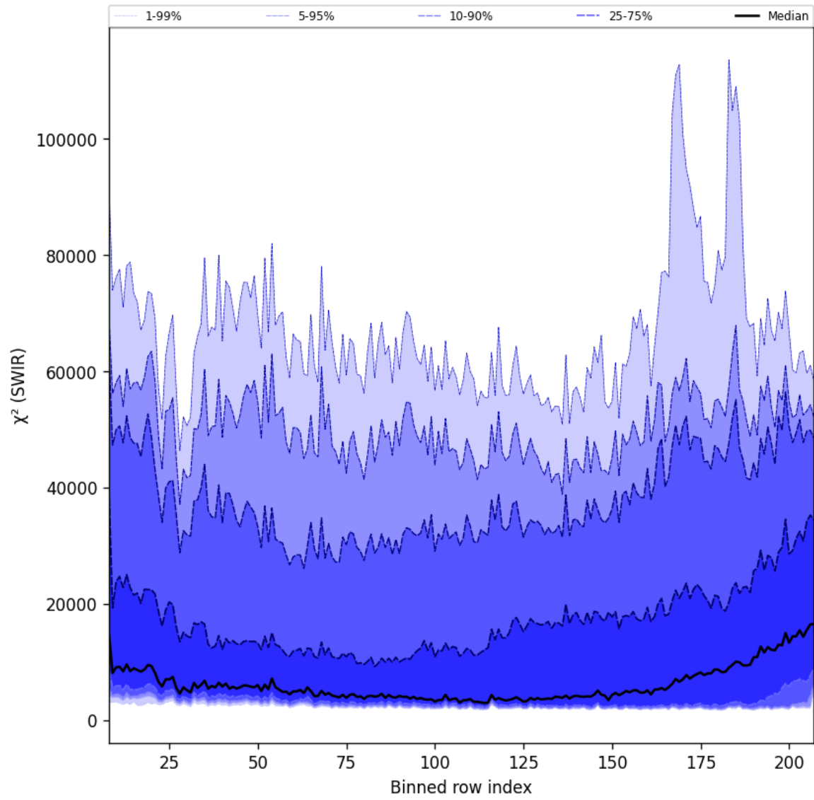
Figure 39: Along track statistics of " \chi^2 (SWIR)" for 2024-11-20 to 2024-11-22
