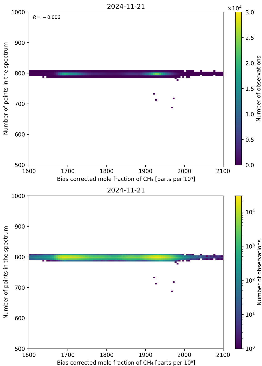
Figure 68: Scatter density plot of “Bias corrected mole fraction of CH 4 ” against “Number of points in the spectrum” for 2024-11-20 to 2024-11-22.
