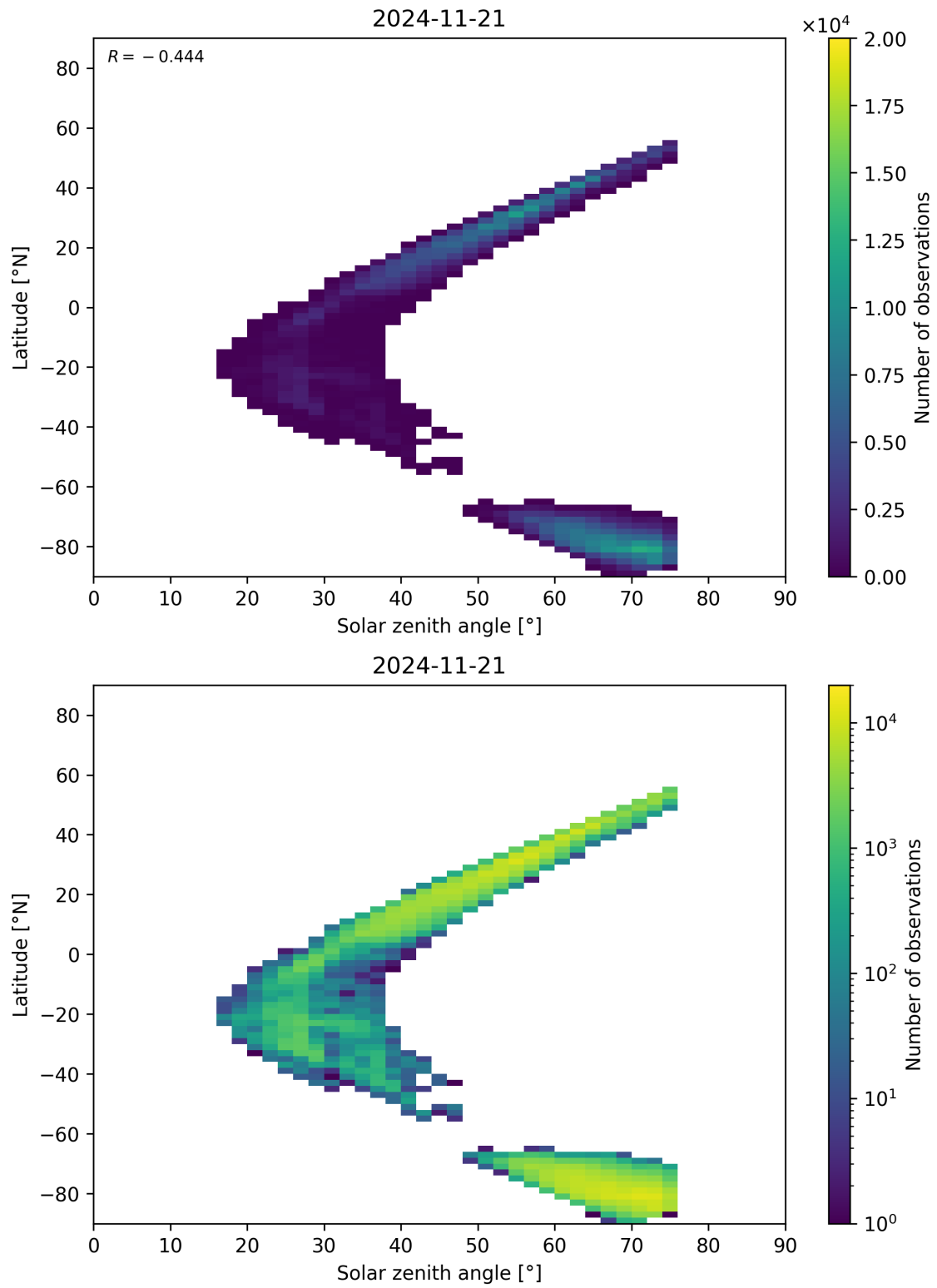
Figure 98: Scatter density plot of “Solar zenith angle” against “Latitude” for 2024-11-20 to 2024-11-22.
