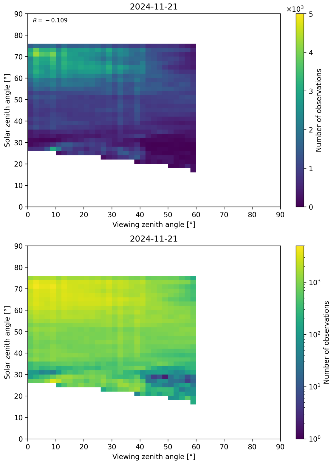
Figure 115: Scatter density plot of “Viewing zenith angle” against “Solar zenith angle” for 2024-11-20 to 2024-11-22.
