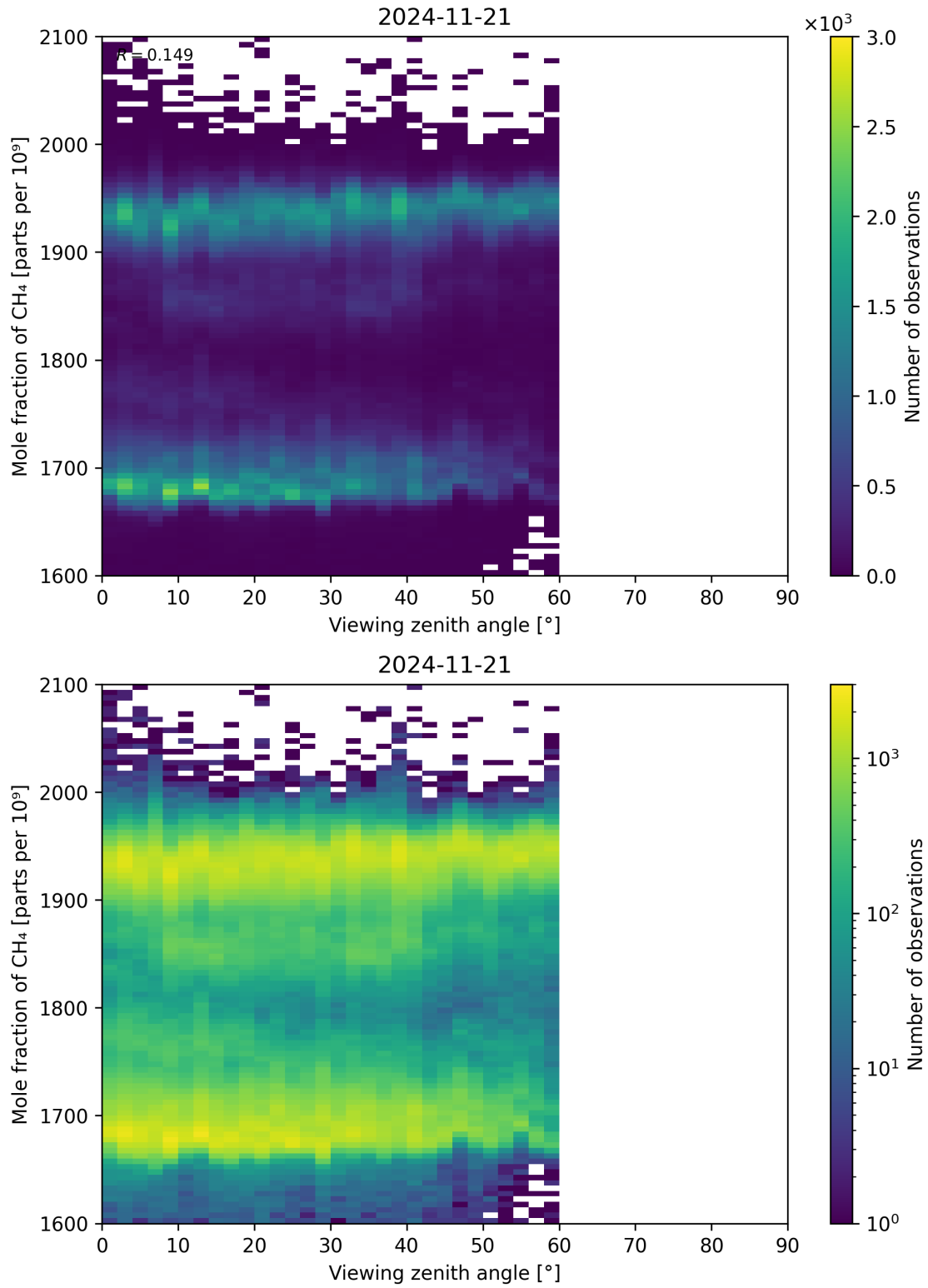
Figure 110: Scatter density plot of “Viewing zenith angle” against “Mole fraction of CH 4 ” for 2024-11-20 to 2024-11-22.
