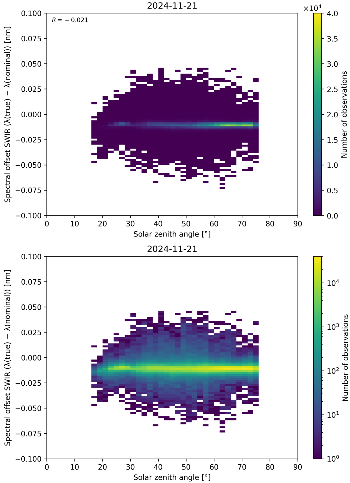
Figure 104: Scatter density plot of “Solar zenith angle” against “Spectral offset SWIR ( \lambda_{\text{true}} - \lambda_{\text{nominal}} )” for 2024-11-20 to 2024-11-22.
