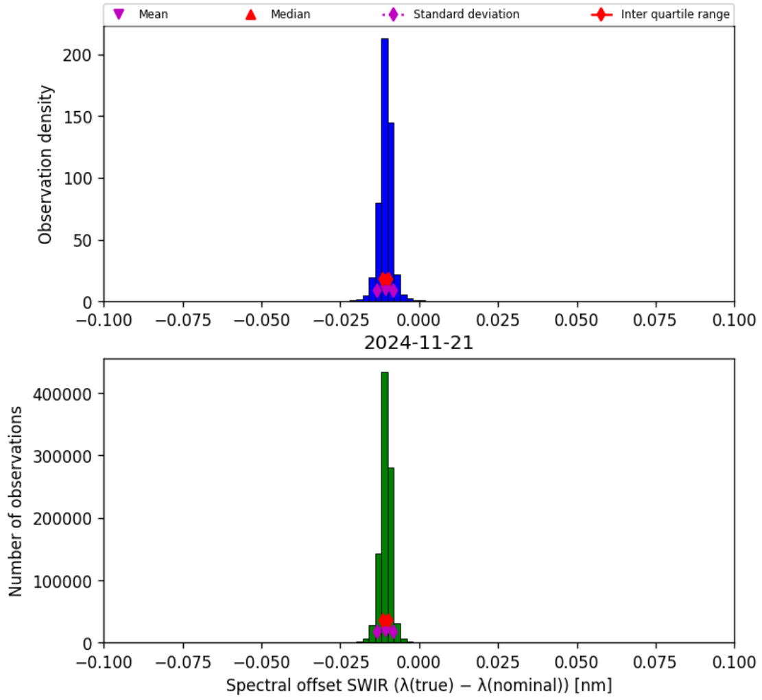
Figure 27: Histogram of “Spectral offset SWIR ( \lambda_{\text{true}} - \lambda_{\text{nominal}} )” for 2024-11-20 to 2024-11-22
