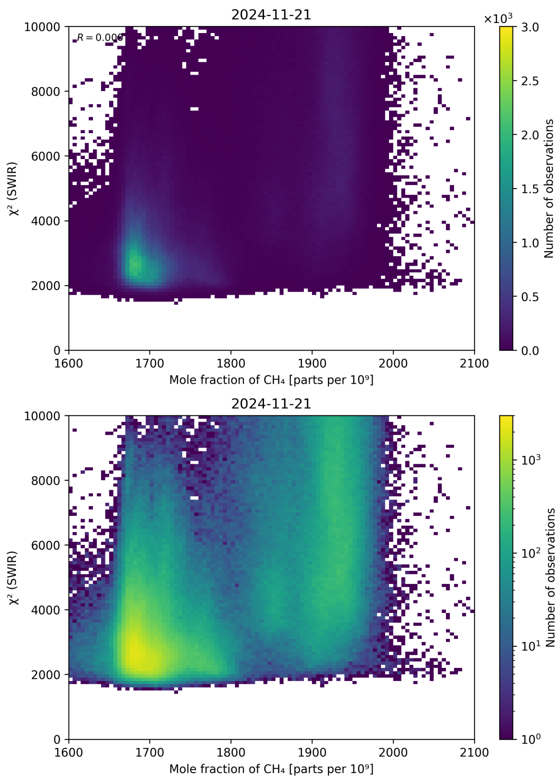
Figure 71: Scatter density plot of “Mole fraction of \text{CH}_4 ” against “ \chi^2 (SWIR)” for 2024-11-20 to 2024-11-22.
