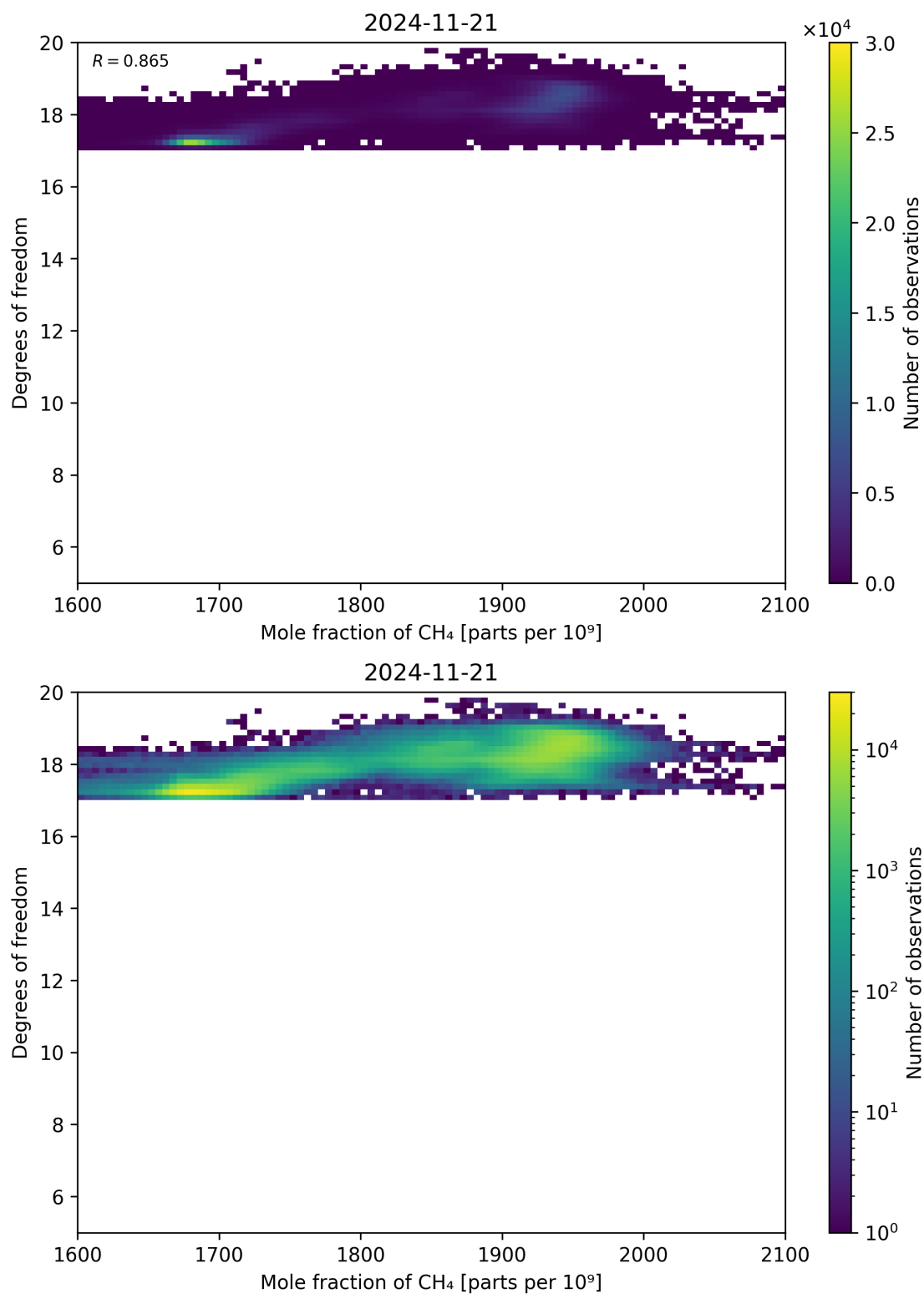
Figure 72: Scatter density plot of “Mole fraction of CH 4 ” against “Degrees of freedom” for 2024-11-20 to 2024-11-22.
