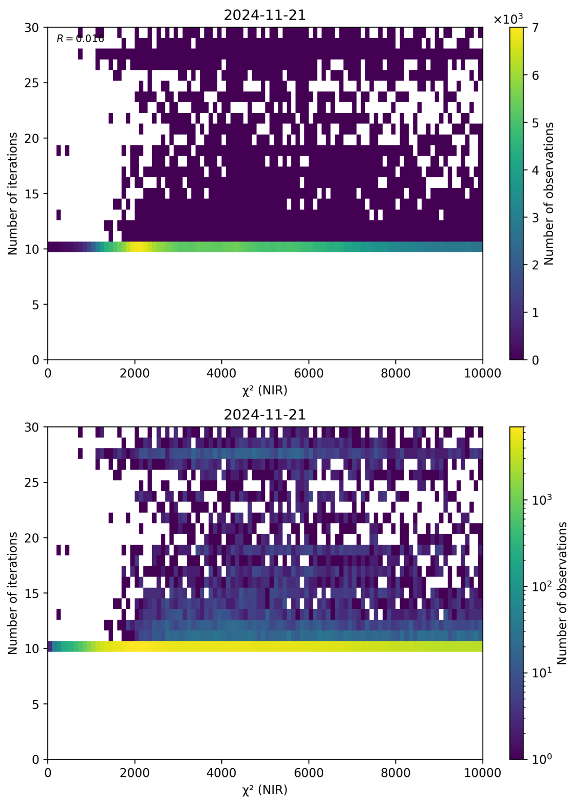
Figure 46: Scatter density plot of “ \chi^2 (NIR)” against “Number of iterations” for 2024-11-20 to 2024-11-22.
