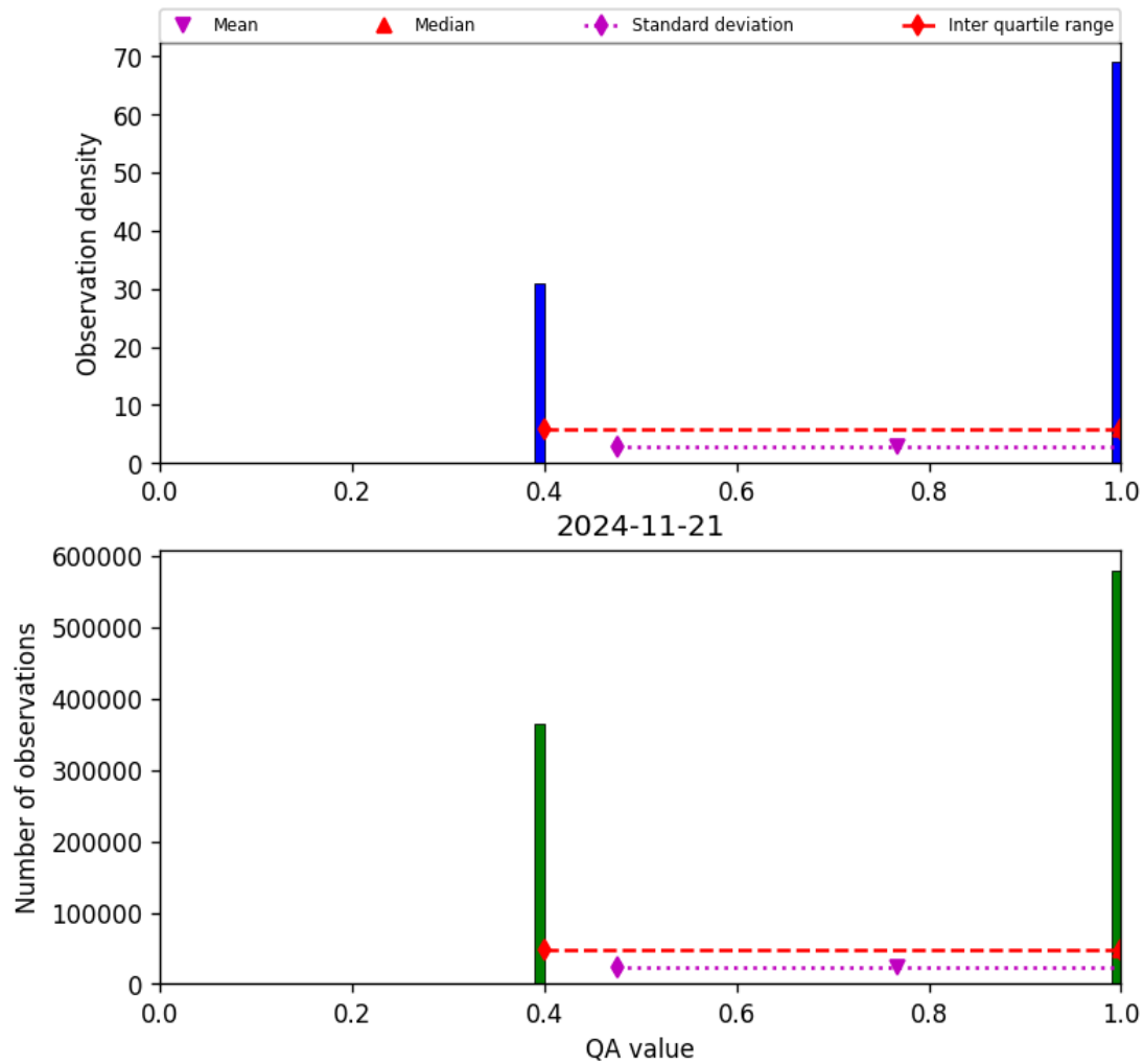
Figure 22: Histogram of “QA value” for 2024-11-20 to 2024-11-22
