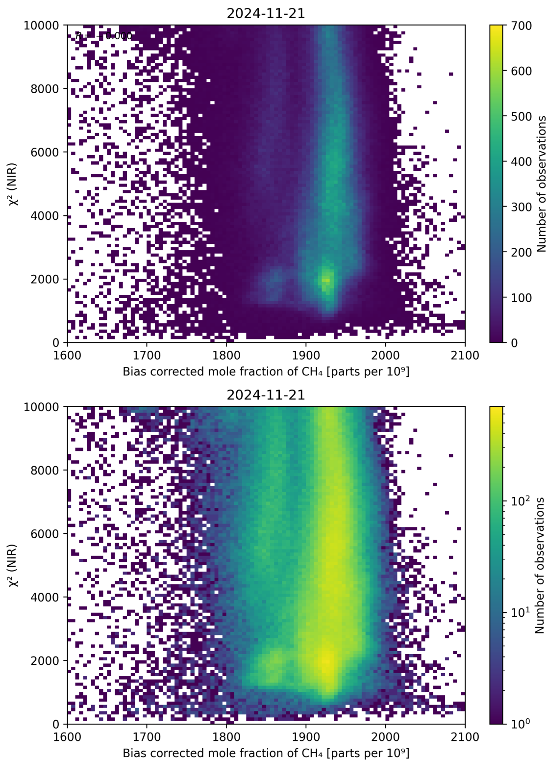
Figure 63: Scatter density plot of “Bias corrected mole fraction of \text{CH}_4 ” against “ \chi^2 (NIR)” for 2024-11-20 to 2024-11-22.
