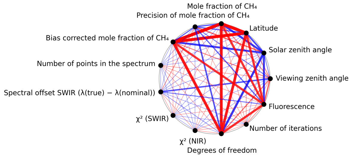
Figure 1: Map of correlation graph for 2024-11-20 to 2024-11-22.
