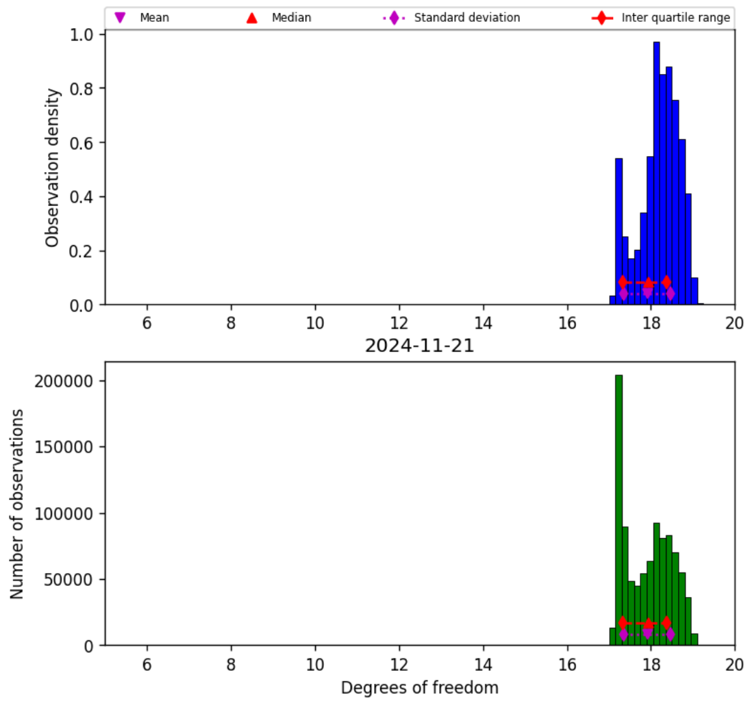
Figure 30: Histogram of “Degrees of freedom” for 2024-11-20 to 2024-11-22
