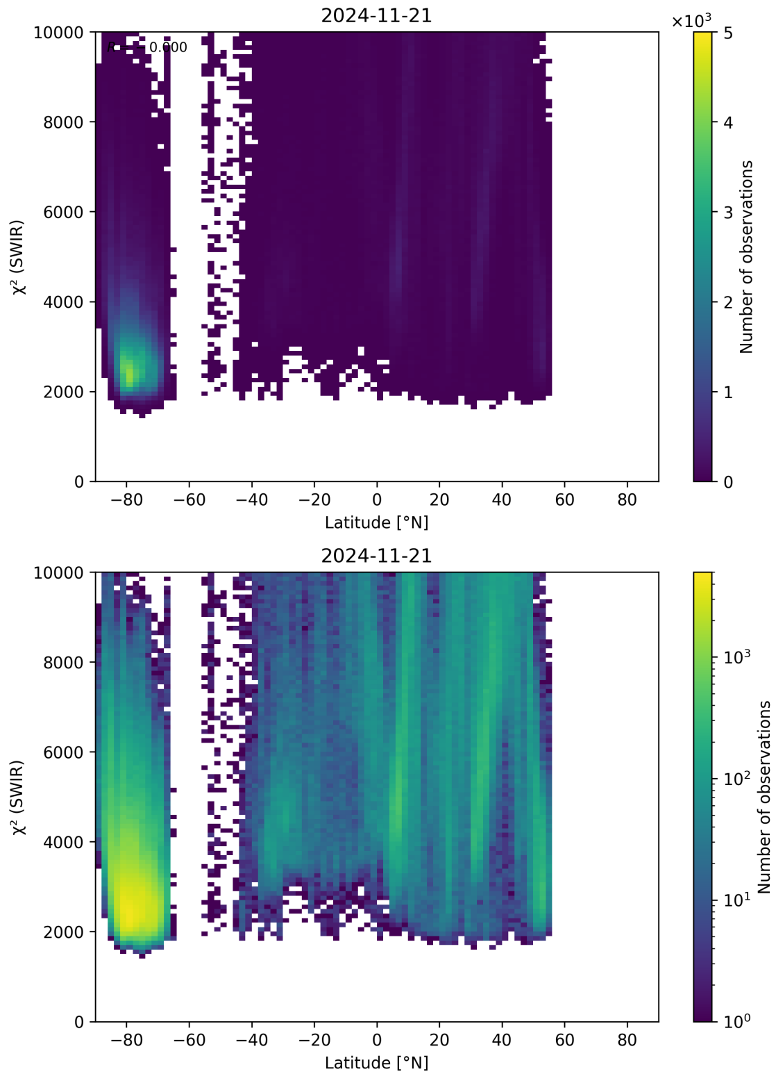
Figure 54: Scatter density plot of “Latitude” against “ \chi^2 (SWIR)” for 2024-11-20 to 2024-11-22.
