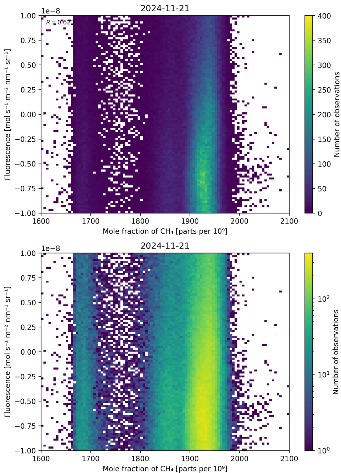
Figure 73: Scatter density plot of “Mole fraction of \text{CH}_4 ” against “Fluorescence” for 2024-11-20 to 2024-11-22.
