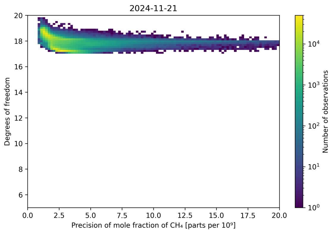
Figure 80: Scatter density plot of “Precision of mole fraction of CH 4 ” against “Degrees of freedom” for 2024-11-20 to 2024-11-22.
