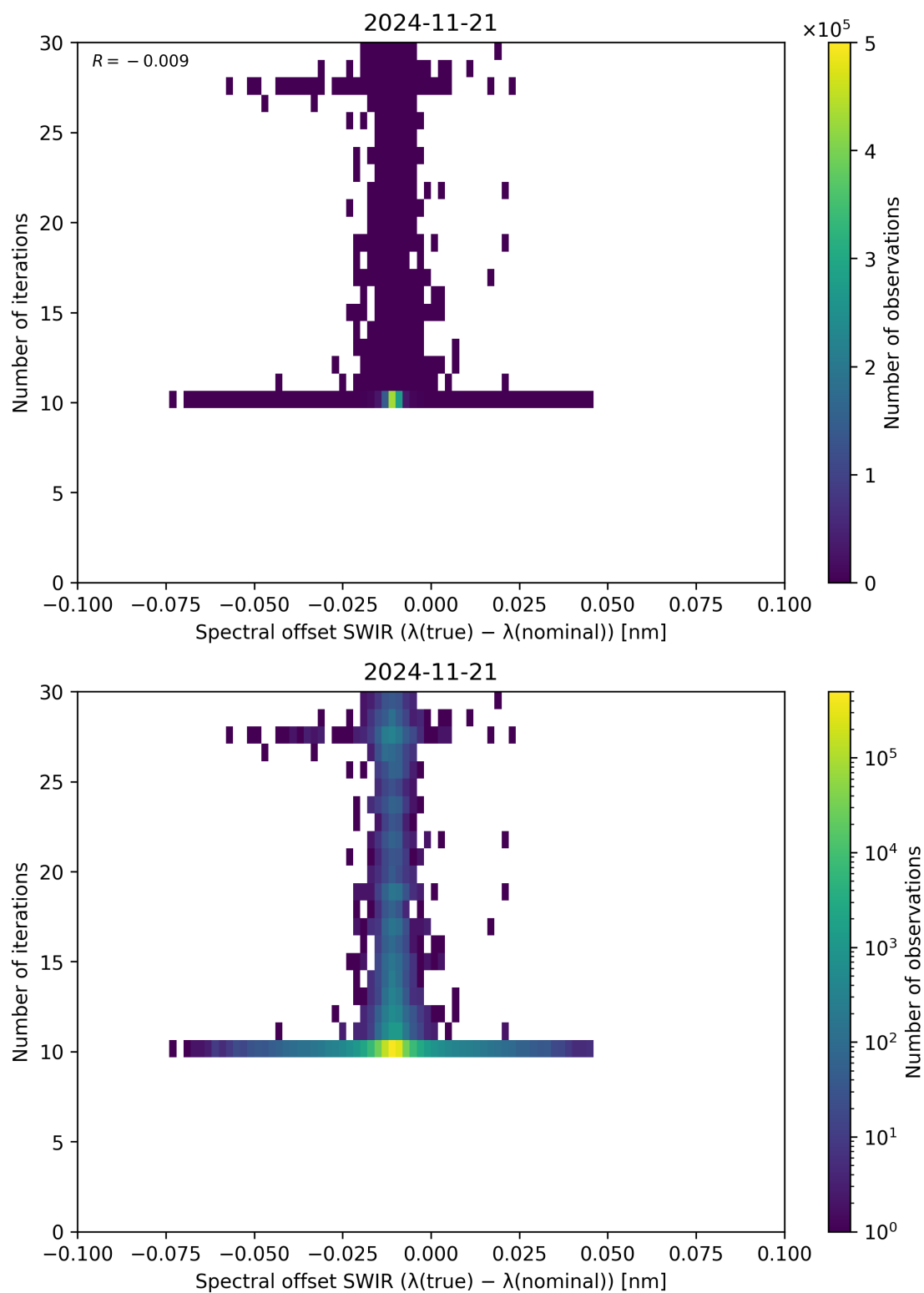
Figure 121: Scatter density plot of “Spectral offset SWIR ( \lambda_{\text{true}} - \lambda_{\text{nominal}} )” against “Number of iterations” for 2024-11-20 to 2024-11-22.
