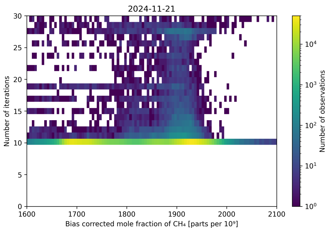
Figure 67: Scatter density plot of “Bias corrected mole fraction of \text{CH}_4 ” against “Number of iterations” for 2024-11-20 to 2024-11-22.
