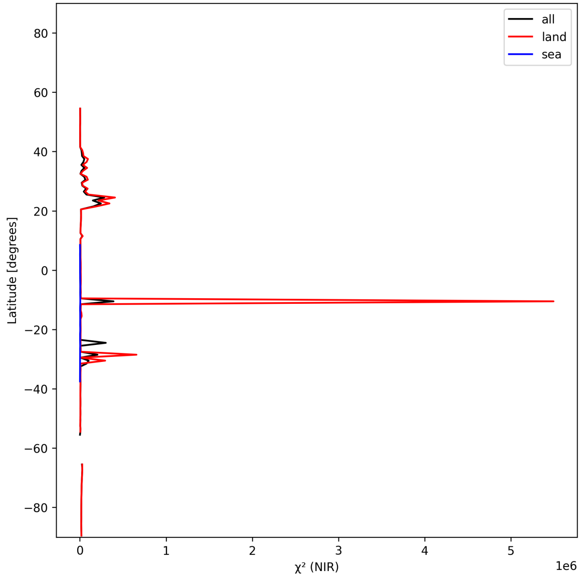
Figure 18: Zonal average of “ \chi^2 (NIR)” for 2024-11-20 to 2024-11-22.
