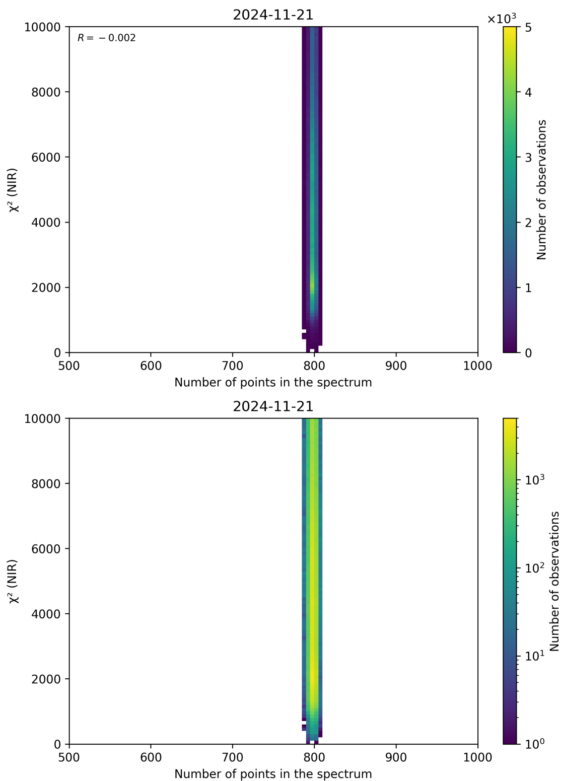
Figure 88: Scatter density plot of “Number of points in the spectrum” against “ \chi^2 (NIR)” for 2024-11-20 to 2024-11-22.
