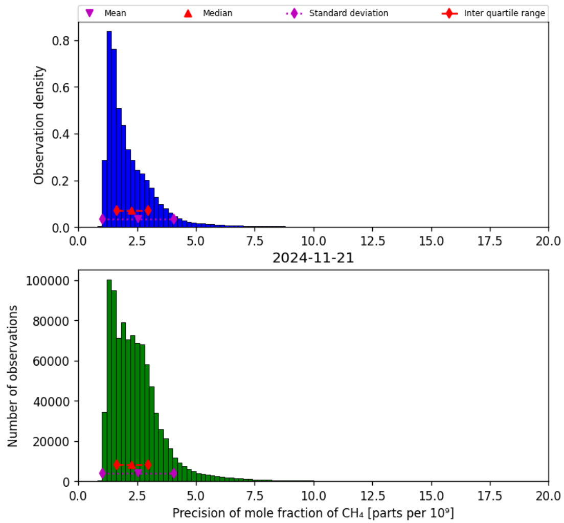
Figure 24: Histogram of “Precision of mole fraction of CH 4 ” for 2024-11-20 to 2024-11-22
