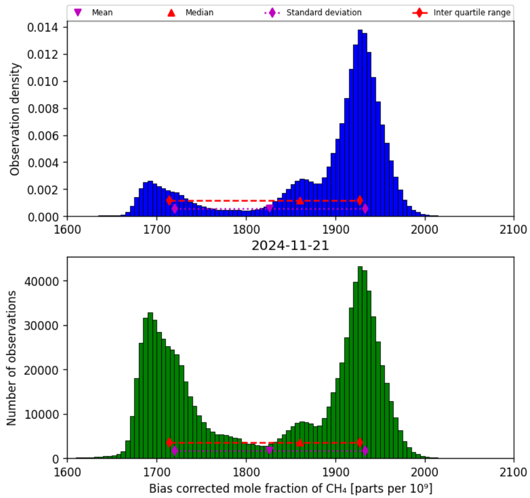
Figure 25: Histogram of “Bias corrected mole fraction of CH 4 ” for 2024-11-20 to 2024-11-22
