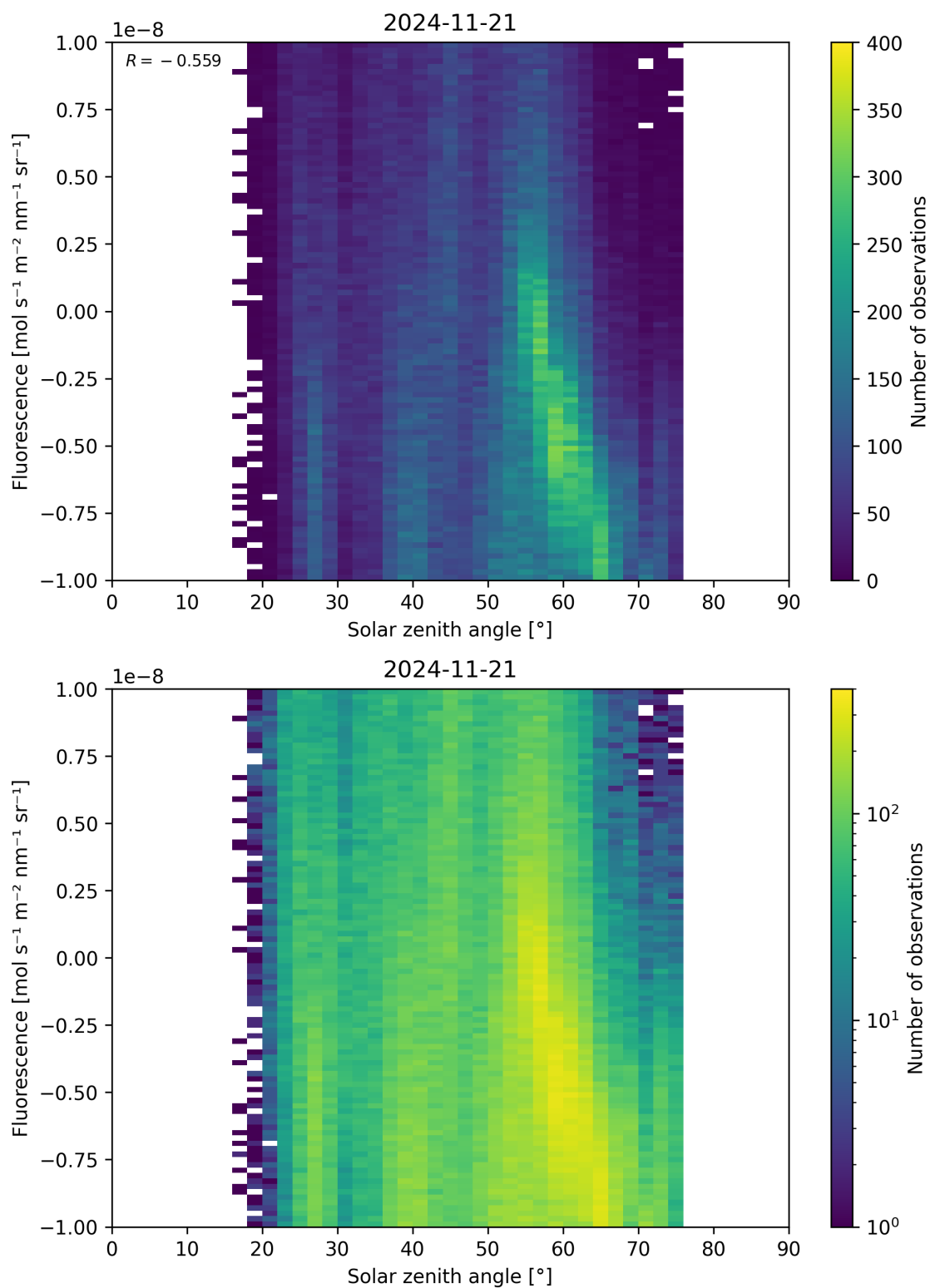
Figure 97: Scatter density plot of “Solar zenith angle” against “Fluorescence” for 2024-11-20 to 2024-11-22.
