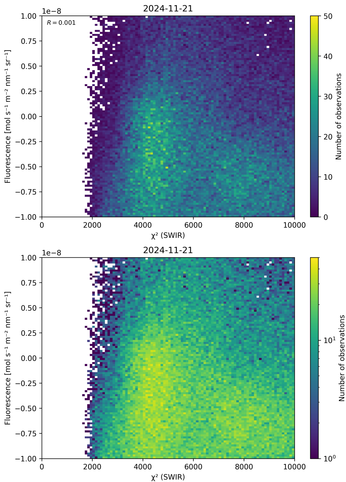
Figure 49: Scatter density plot of “ \chi^2 (SWIR)” against “Fluorescence” for 2024-11-20 to 2024-11-22.
