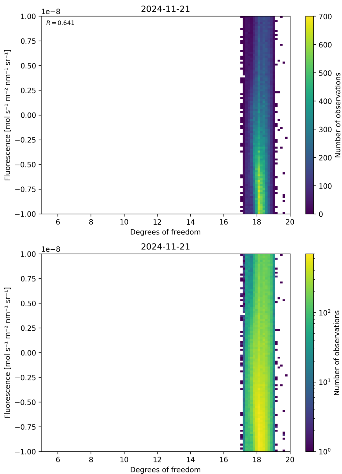
Figure 51: Scatter density plot of “Degrees of freedom” against “Fluorescence” for 2024-11-20 to 2024-11-22.
