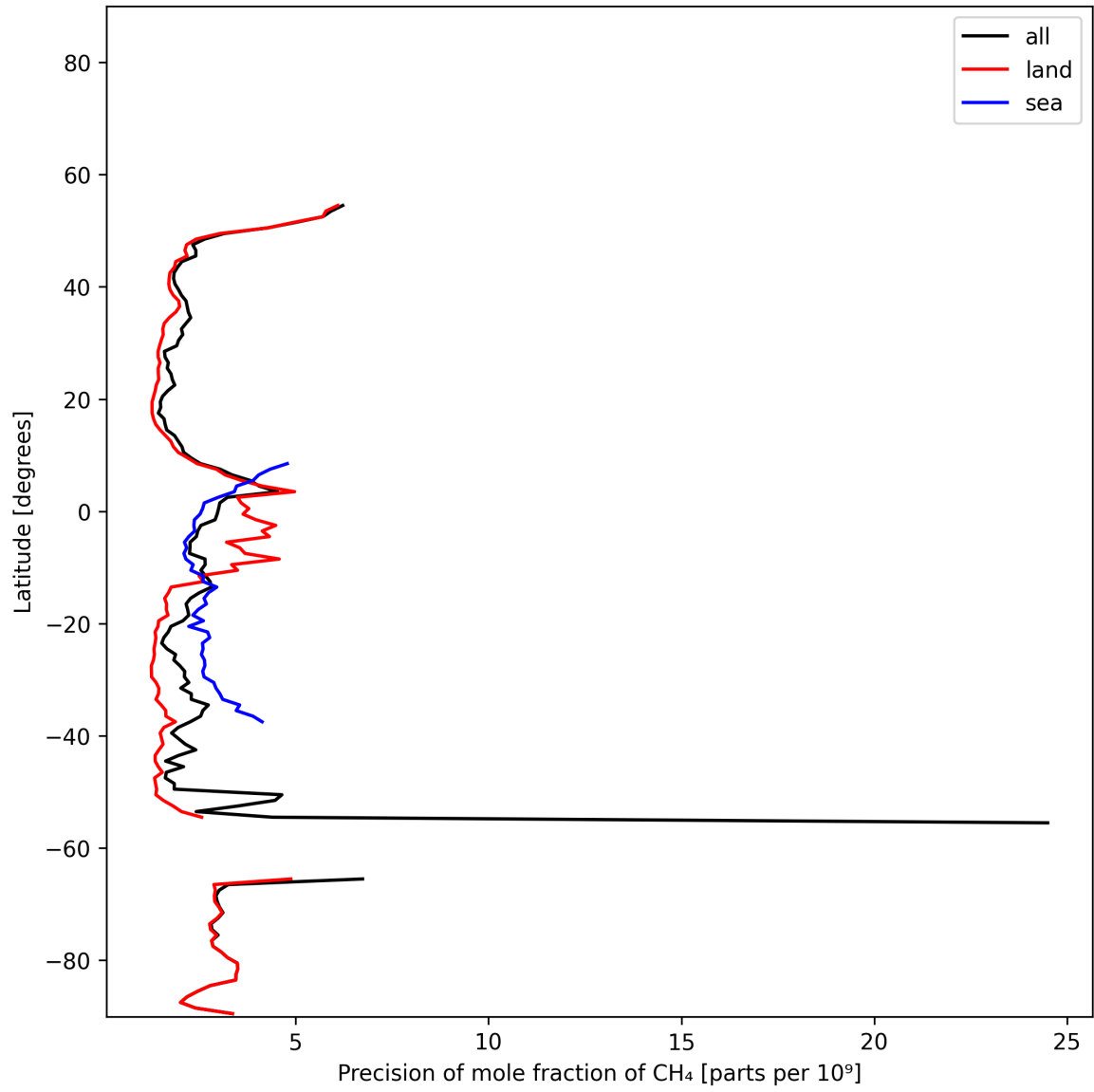
Figure 13: Zonal average of “Precision of mole fraction of CH 4 ” for 2024-11-20 to 2024-11-22.
