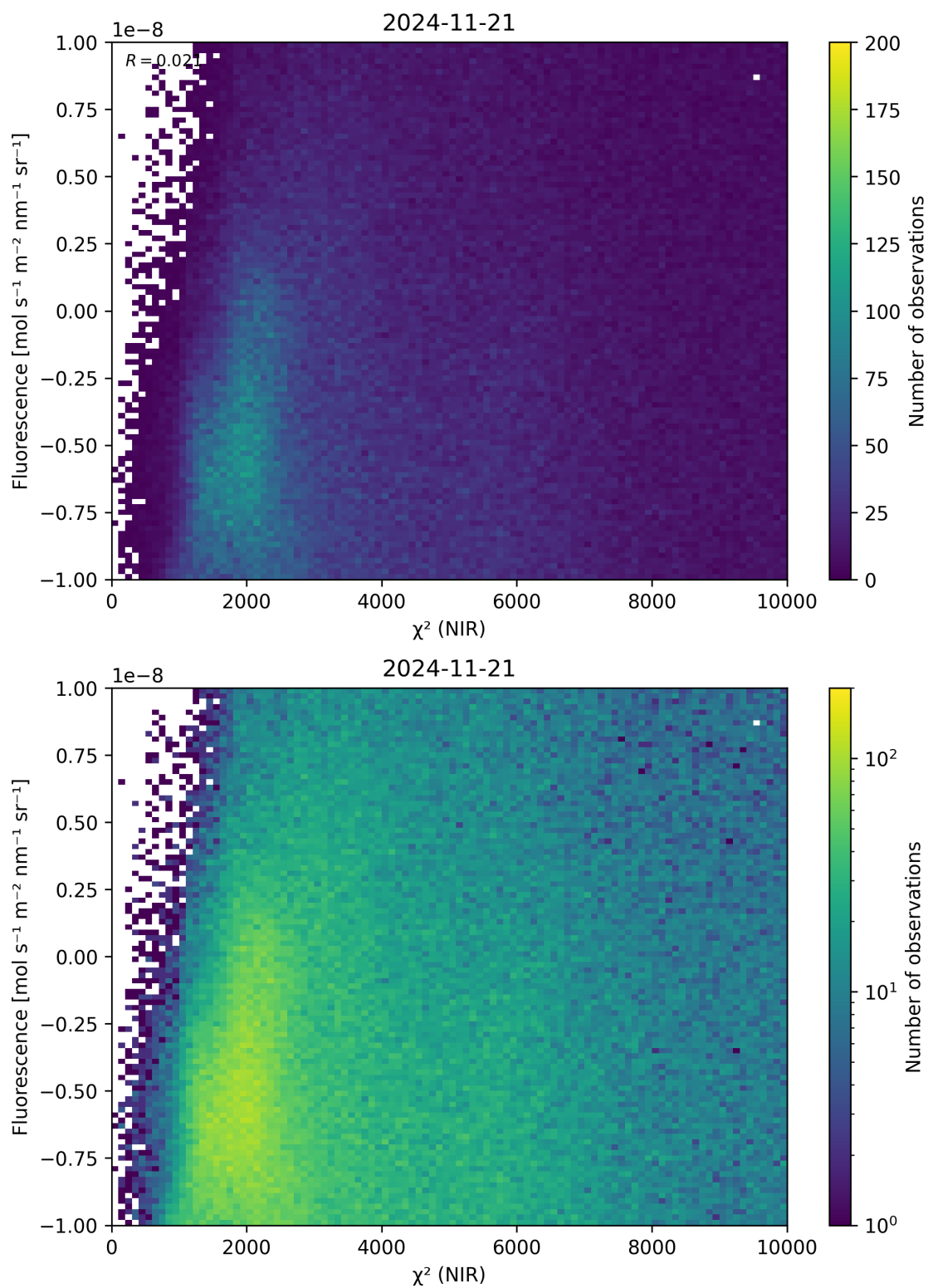
Figure 45: Scatter density plot of “ \chi^2 (NIR)” against “Fluorescence” for 2024-11-20 to 2024-11-22.
