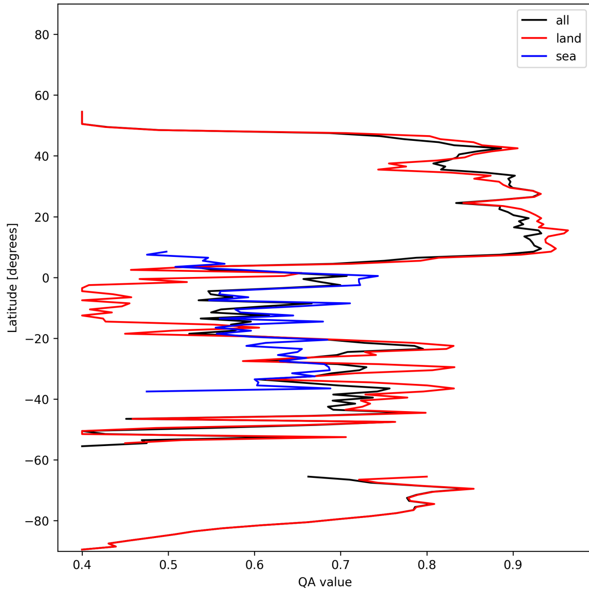
Figure 11: Zonal average of “QA value” for 2024-11-20 to 2024-11-22.
