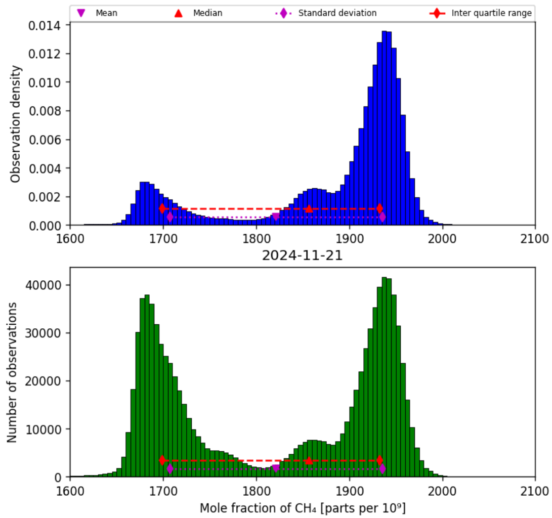
Figure 23: Histogram of “Mole fraction of CH 4 ” for 2024-11-20 to 2024-11-22
