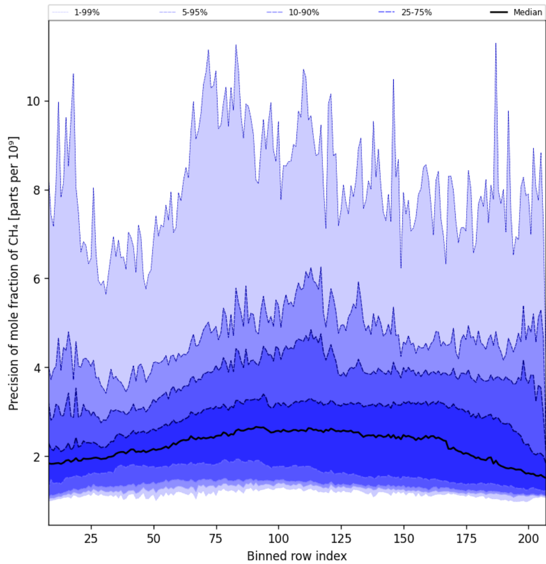
Figure 35: Along track statistics of “Precision of mole fraction of CH 4 ” for 2024-11-20 to 2024-11-22
