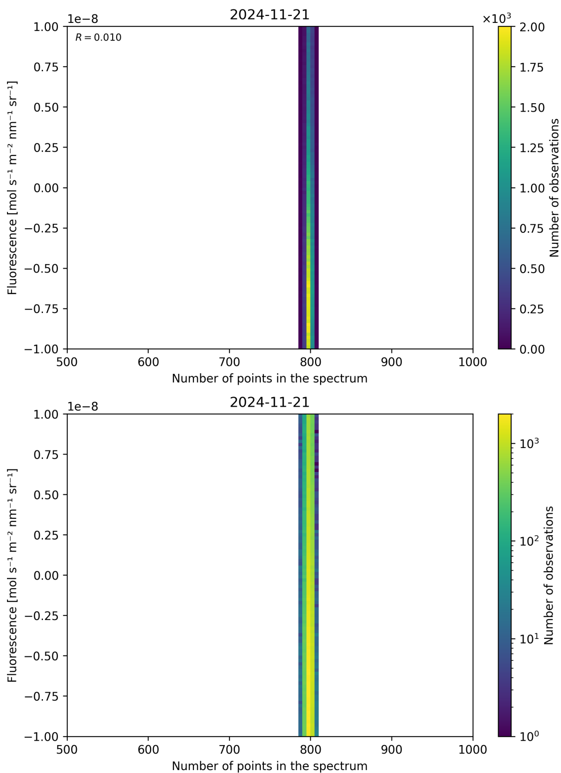
Figure 91: Scatter density plot of “Number of points in the spectrum” against “Fluorescence” for 2024-11-20 to 2024-11-22.
