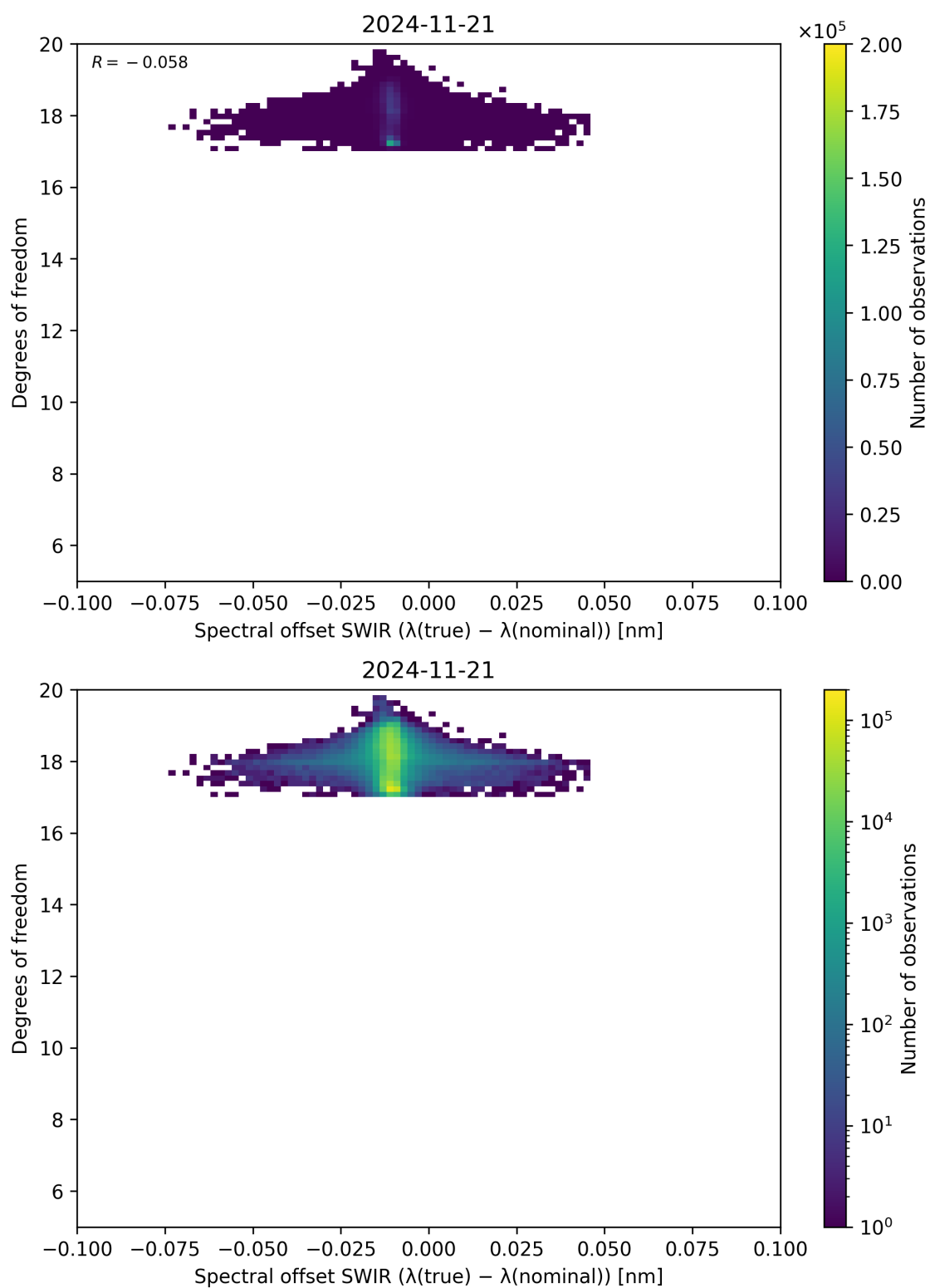
Figure 119: Scatter density plot of “Spectral offset SWIR ( \lambda_{\text{true}} - \lambda_{\text{nominal}} )” against “Degrees of freedom” for 2024-11-20 to 2024-11-22.
