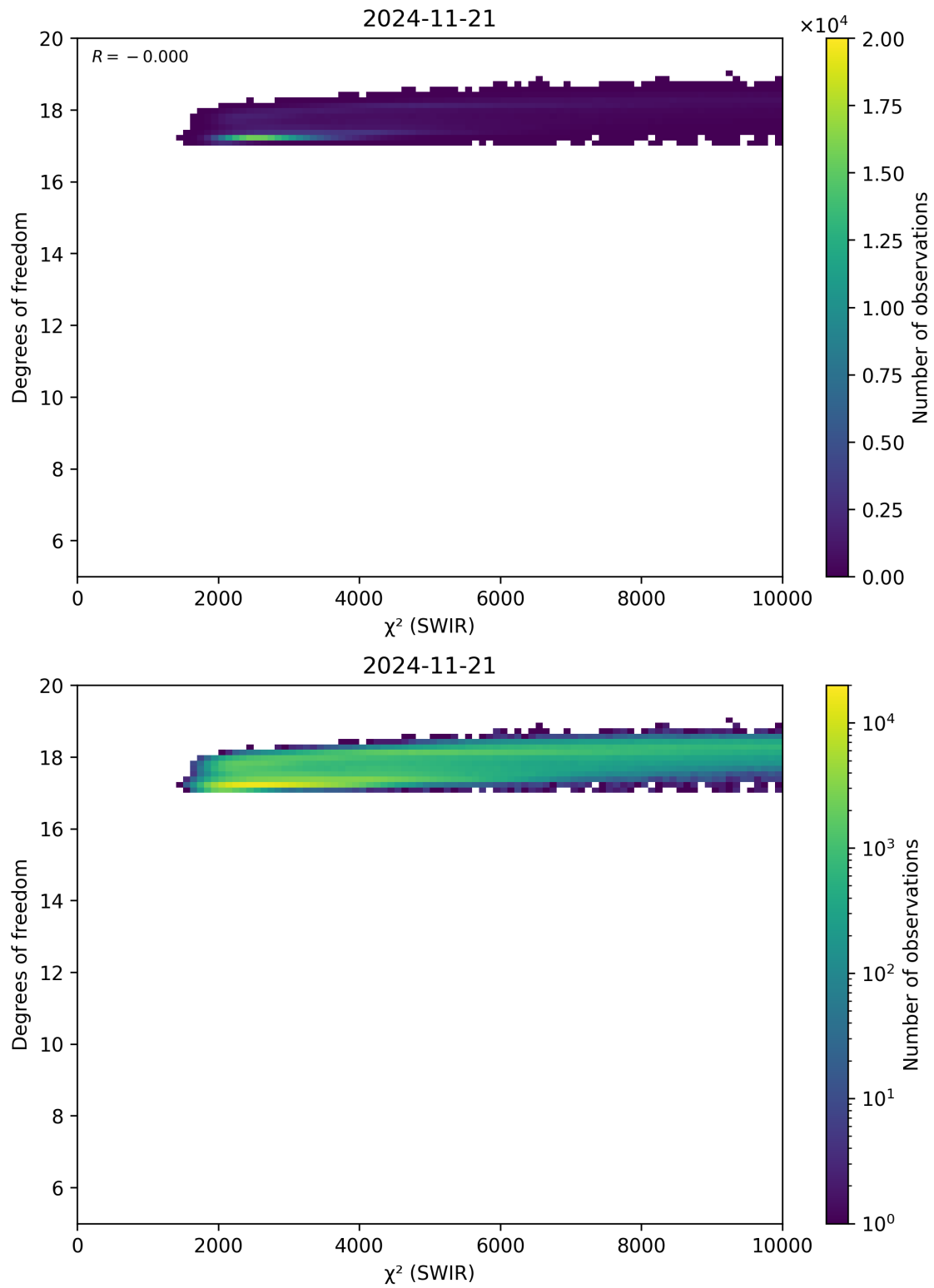
Figure 48: Scatter density plot of “ \chi^2 (SWIR)” against “Degrees of freedom” for 2024-11-20 to 2024-11-22.
