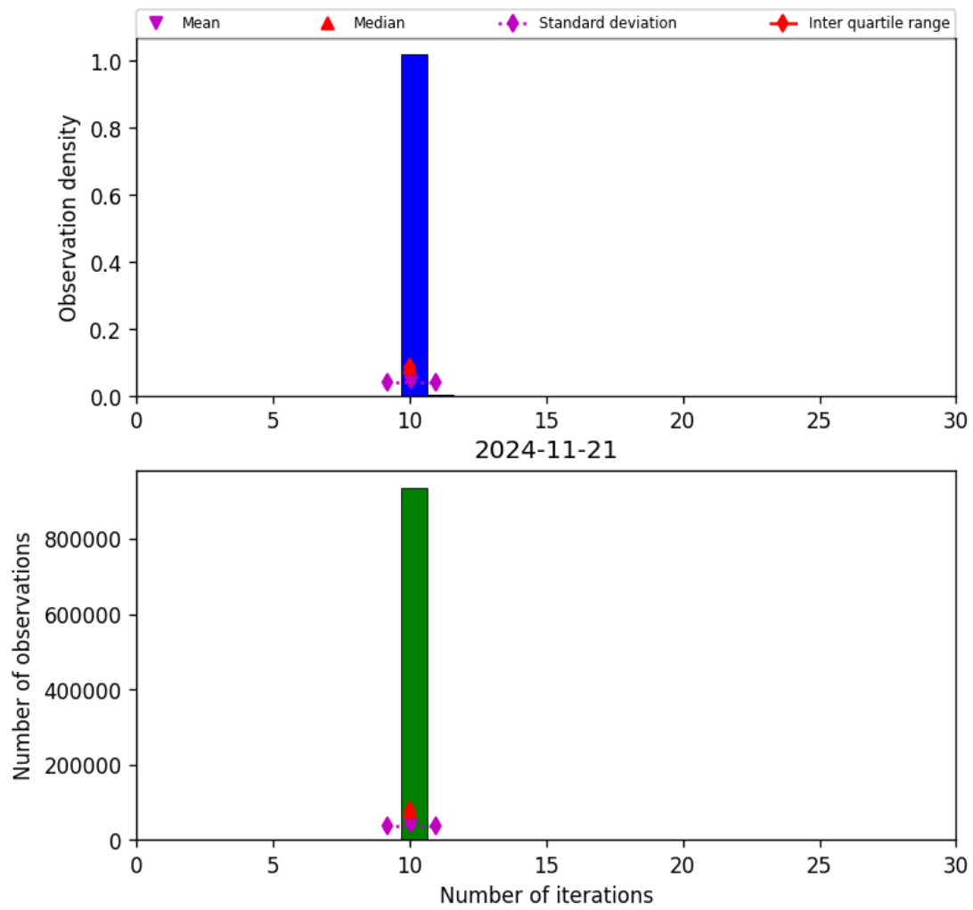
Figure 31: Histogram of “Number of iterations” for 2024-11-20 to 2024-11-22
