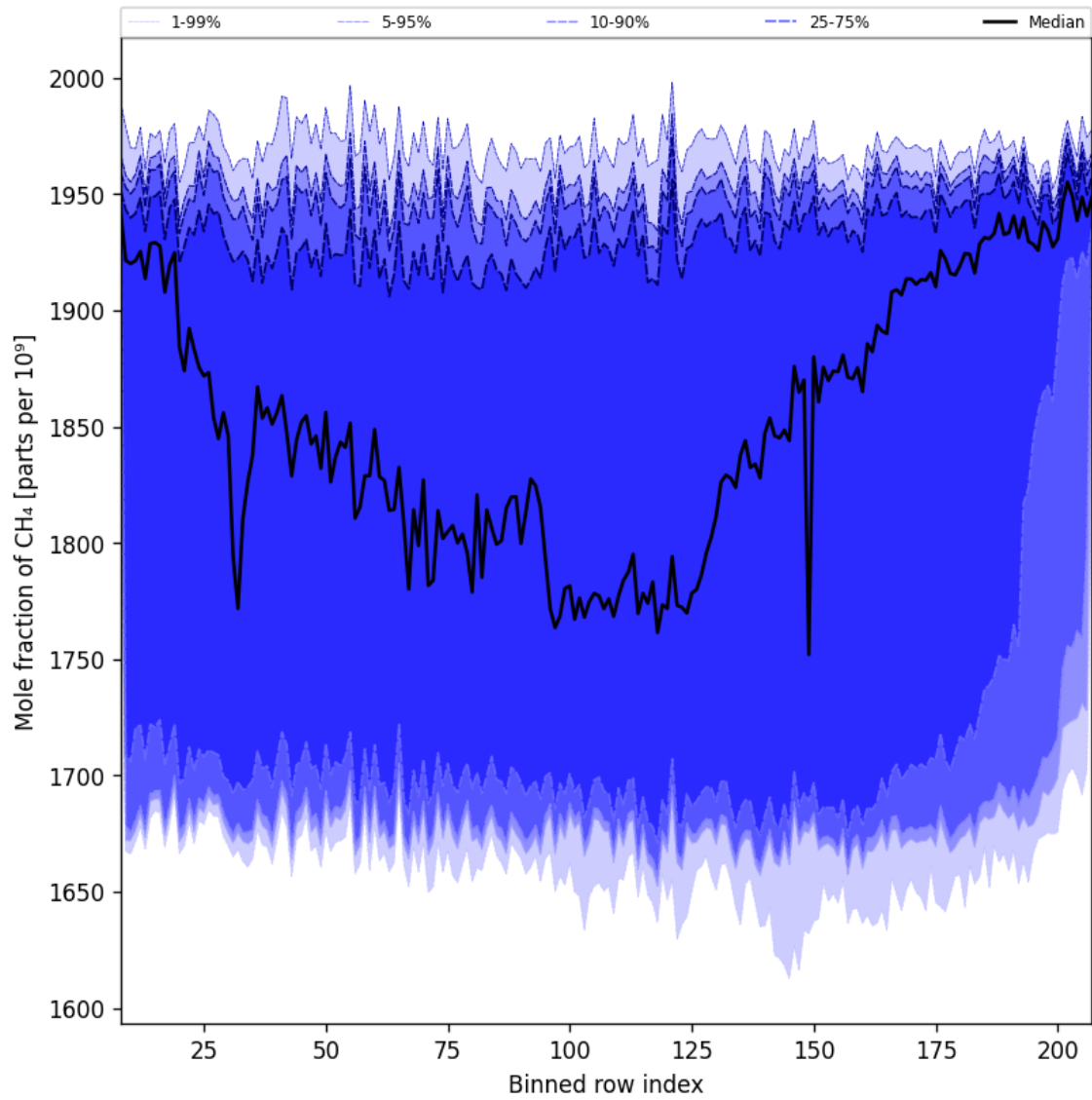
Figure 34: Along track statistics of “Mole fraction of CH 4 ” for 2024-11-20 to 2024-11-22
