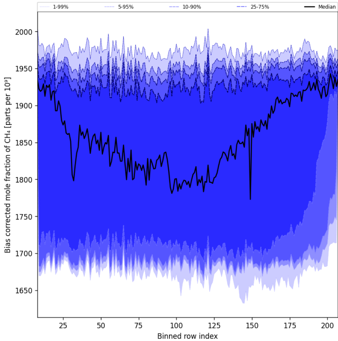
Figure 36: Along track statistics of “Bias corrected mole fraction of CH 4 ” for 2024-11-20 to 2024-11-22
