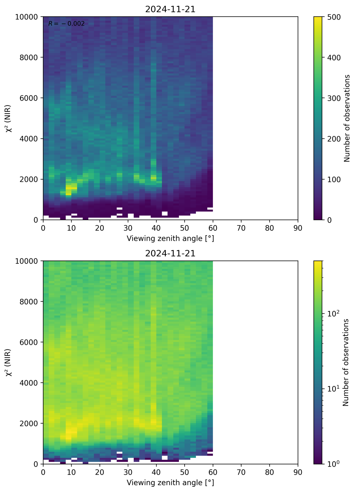
Figure 105: Scatter density plot of “Viewing zenith angle” against “ \chi^2 (NIR)” for 2024-11-20 to 2024-11-22.
