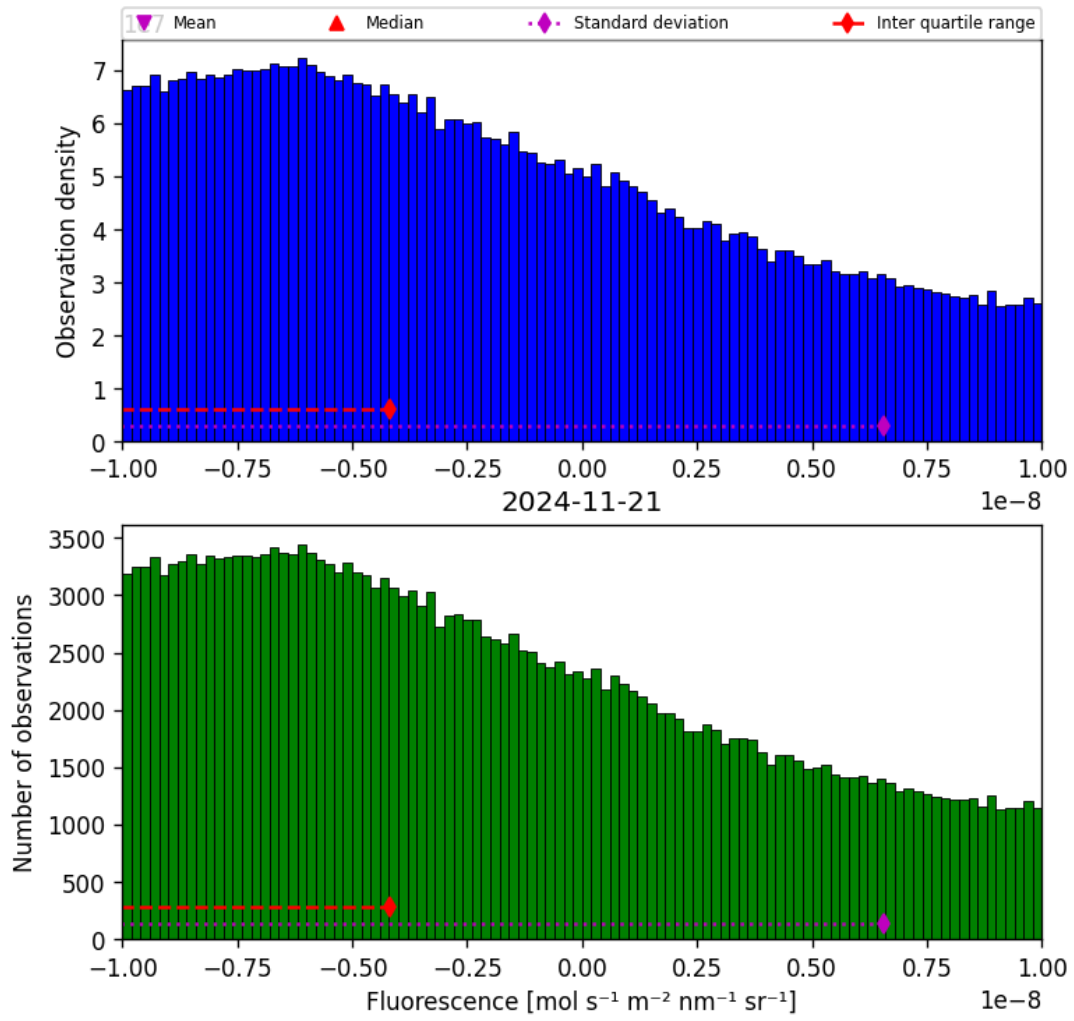
Figure 32: Histogram of “Fluorescence” for 2024-11-20 to 2024-11-22
