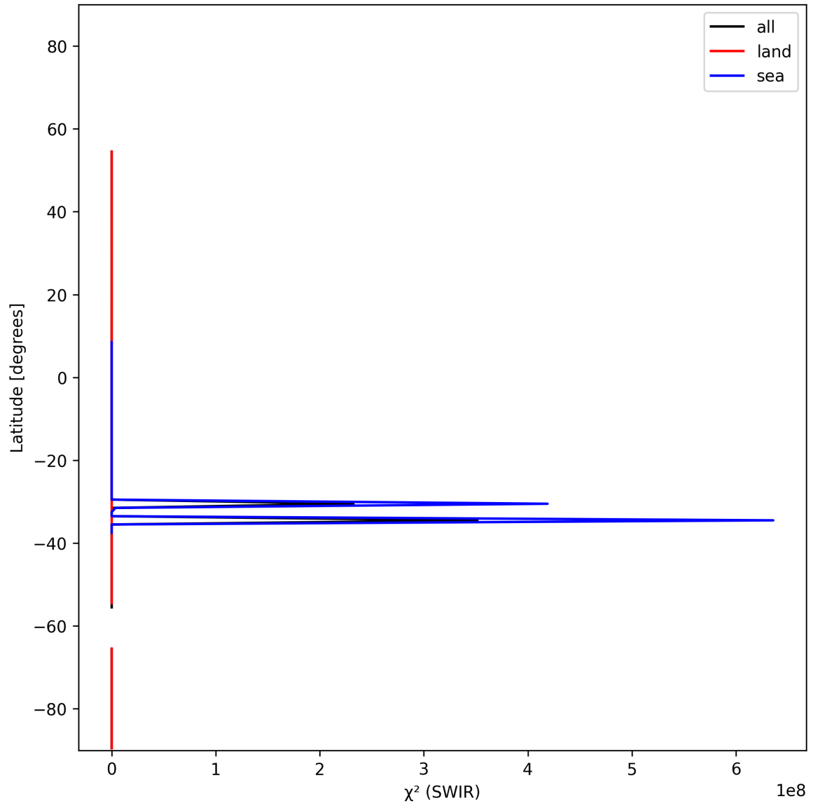
Figure 17: Zonal average of “ \chi^2 (SWIR)” for 2024-11-20 to 2024-11-22.
