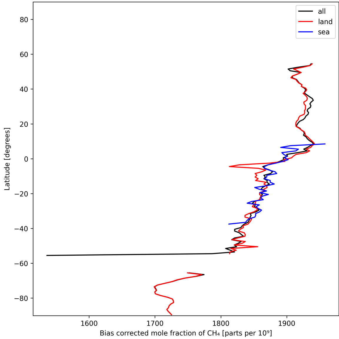
Figure 14: Zonal average of “Bias corrected mole fraction of CH 4 ” for 2024-11-20 to 2024-11-22.
