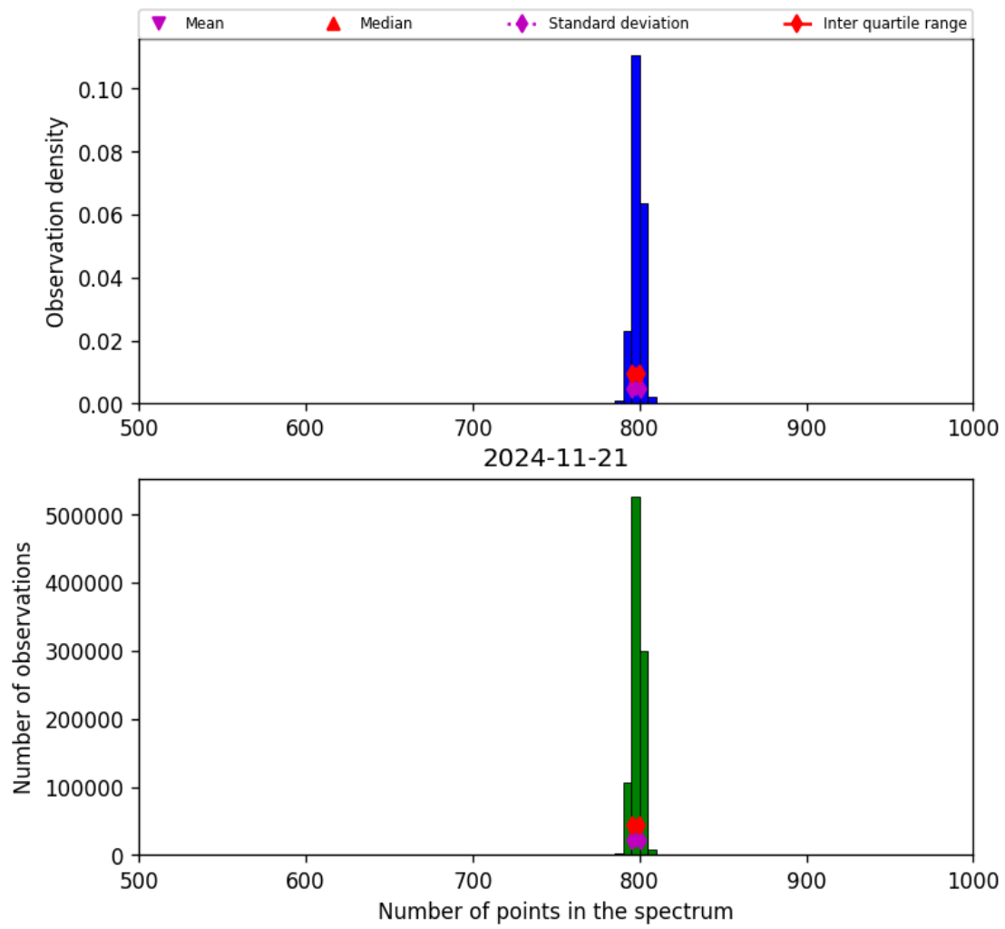
Figure 26: Histogram of “Number of points in the spectrum” for 2024-11-20 to 2024-11-22
