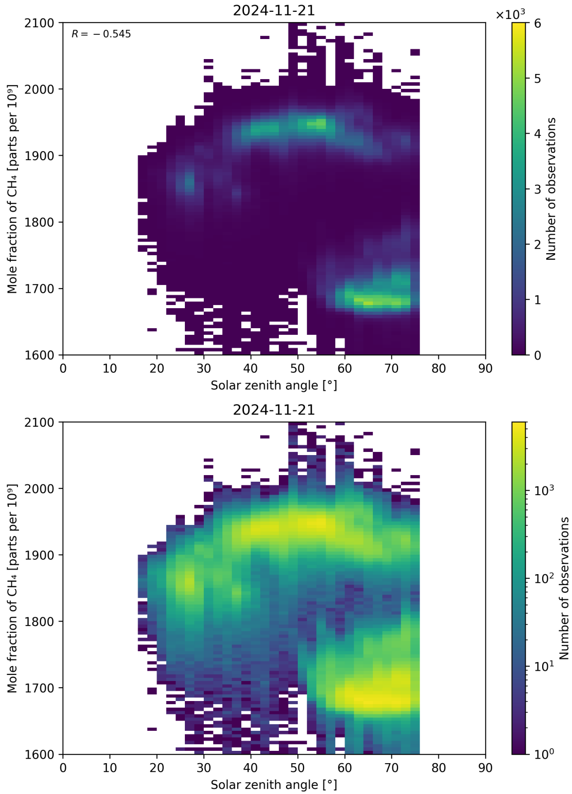
Figure 99: Scatter density plot of “Solar zenith angle” against “Mole fraction of CH 4 ” for 2024-11-20 to 2024-11-22.
