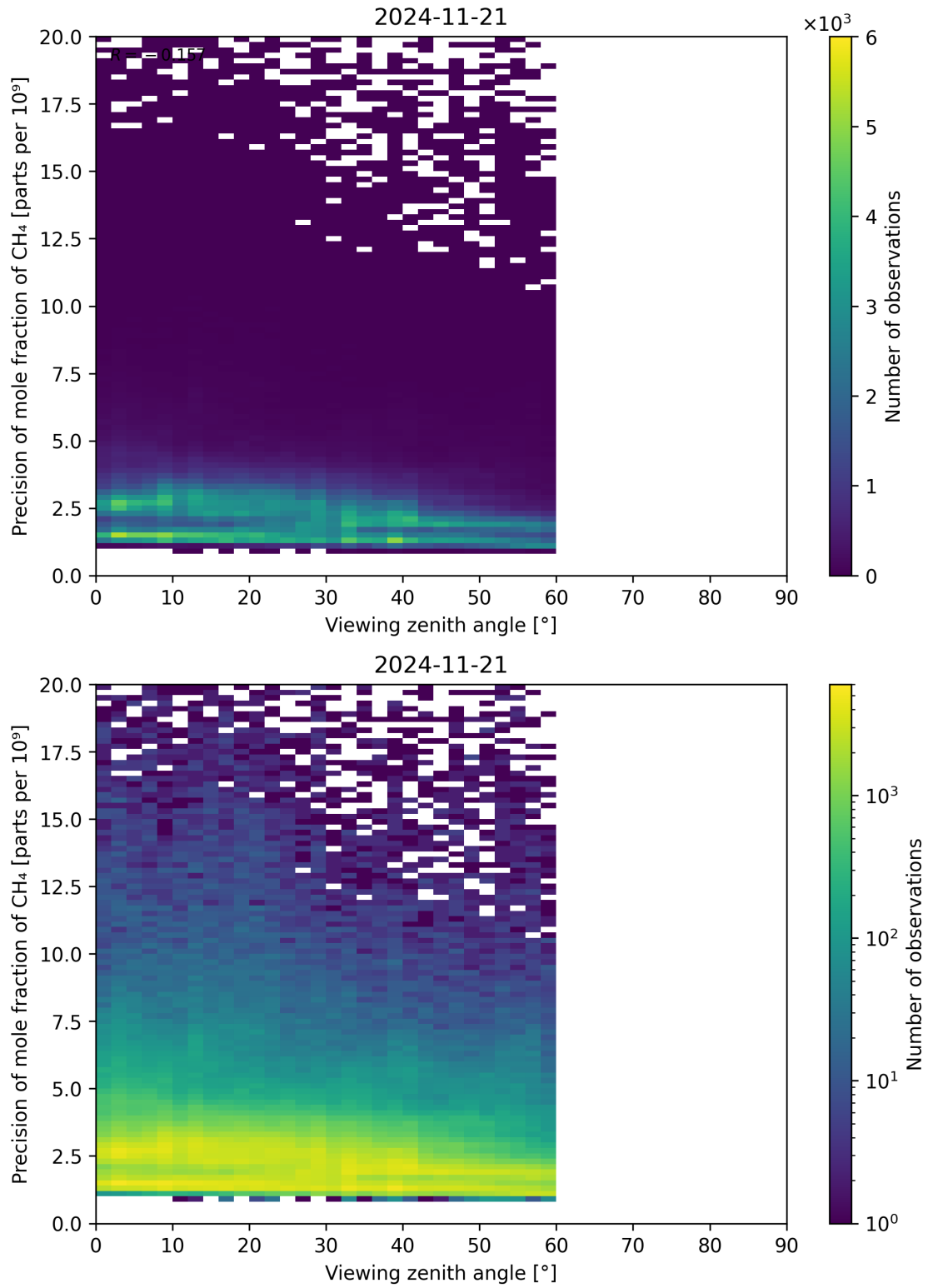
Figure 112: Scatter density plot of “Viewing zenith angle” against “Precision of mole fraction of CH 4 ” for 2024-11-20 to 2024-11-22.
