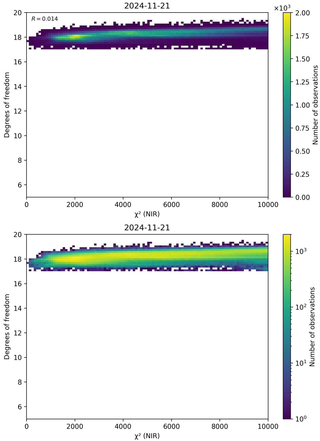
Figure 44: Scatter density plot of “ \chi^2 (NIR)” against “Degrees of freedom” for 2024-11-20 to 2024-11-22.
