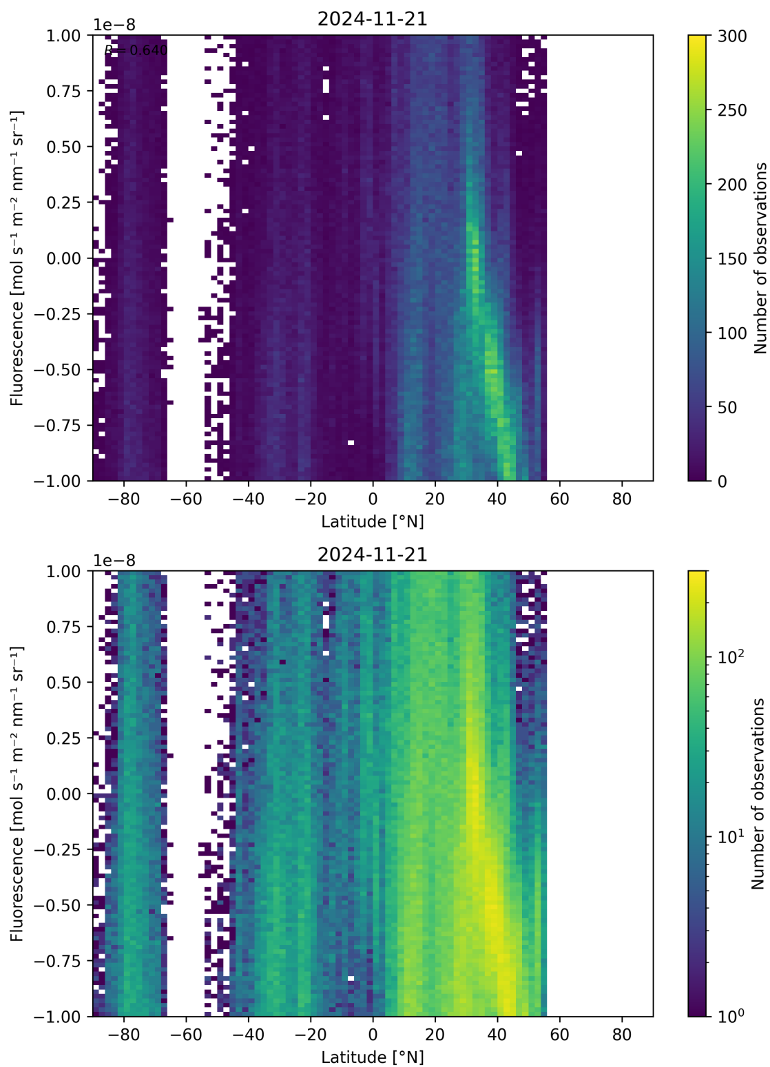
Figure 56: Scatter density plot of “Latitude” against “Fluorescence” for 2024-11-20 to 2024-11-22.
