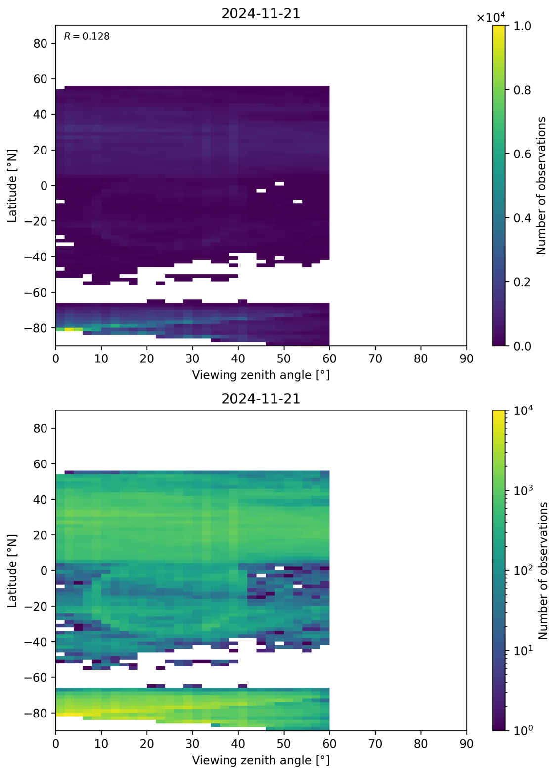
Figure 109: Scatter density plot of “Viewing zenith angle” against “Latitude” for 2024-11-20 to 2024-11-22.
