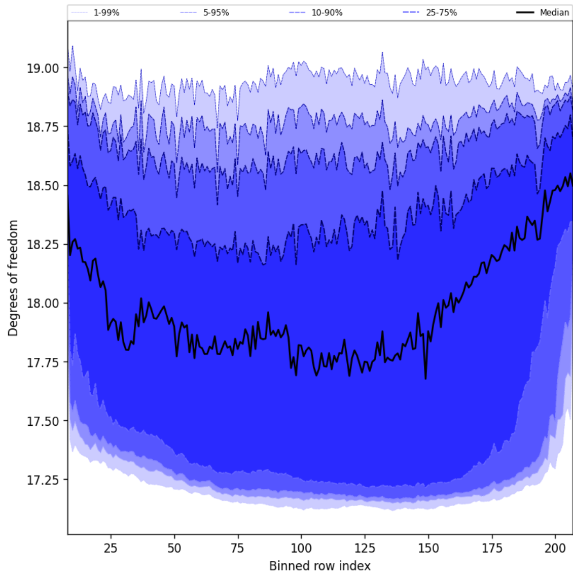
Figure 41: Along track statistics of “Degrees of freedom” for 2024-11-20 to 2024-11-22
