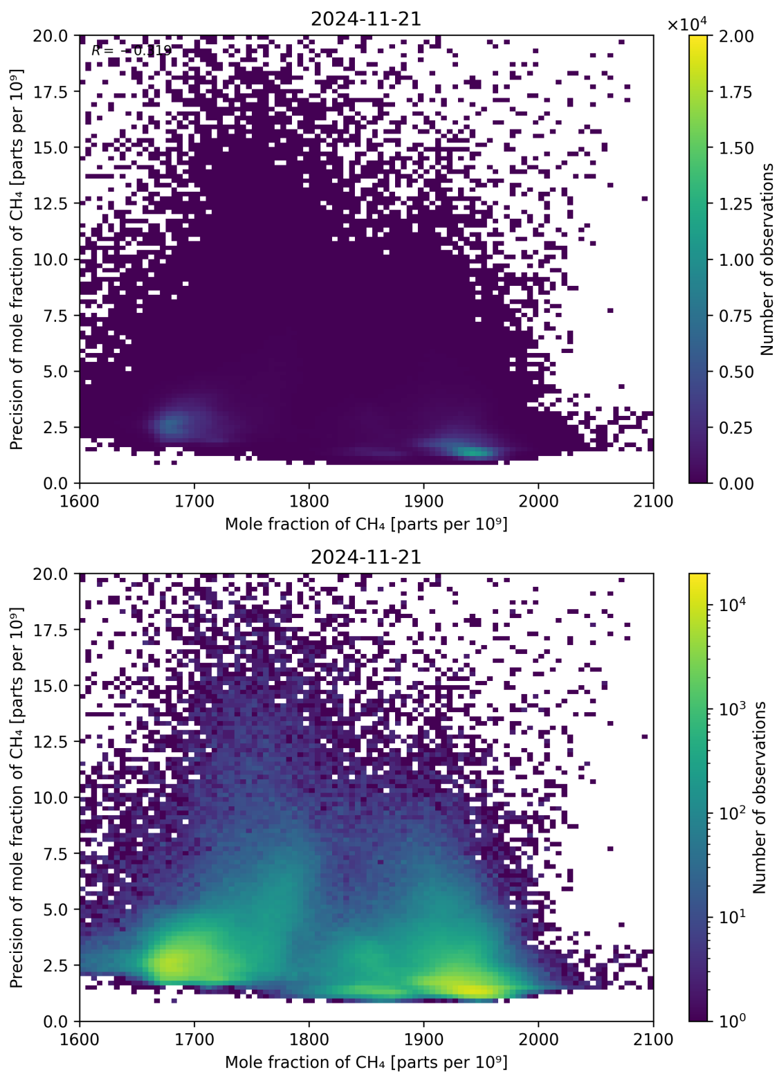
Figure 75: Scatter density plot of “Mole fraction of CH 4 ” against “Precision of mole fraction of CH 4 ” for 2024-11-20 to 2024-11-22.
