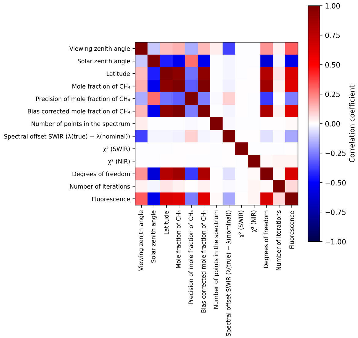
Figure 2: Map of correlation matrix for 2024-11-20 to 2024-11-22.
