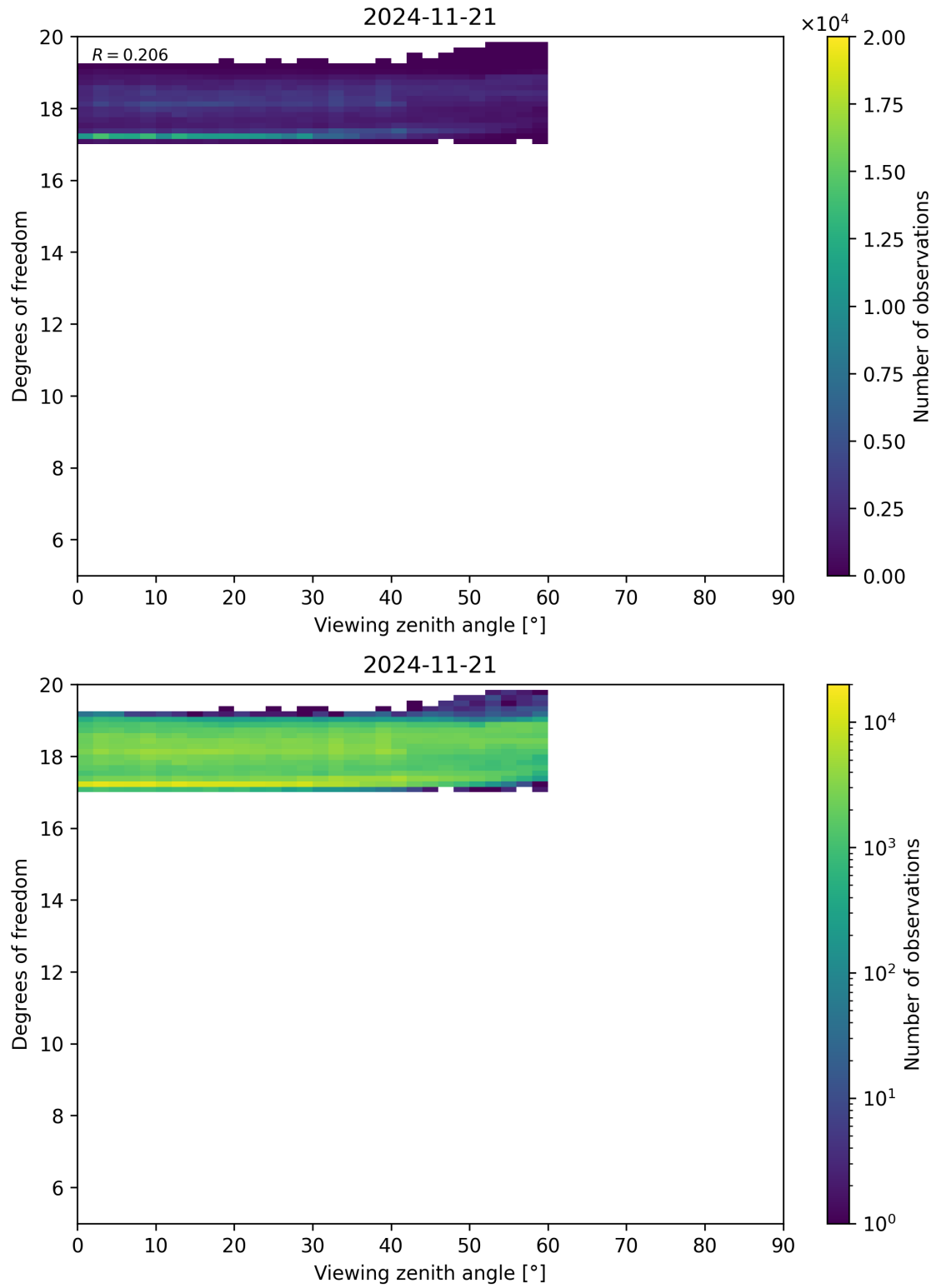
Figure 107: Scatter density plot of “Viewing zenith angle” against “Degrees of freedom” for 2024-11-20 to 2024-11-22.
