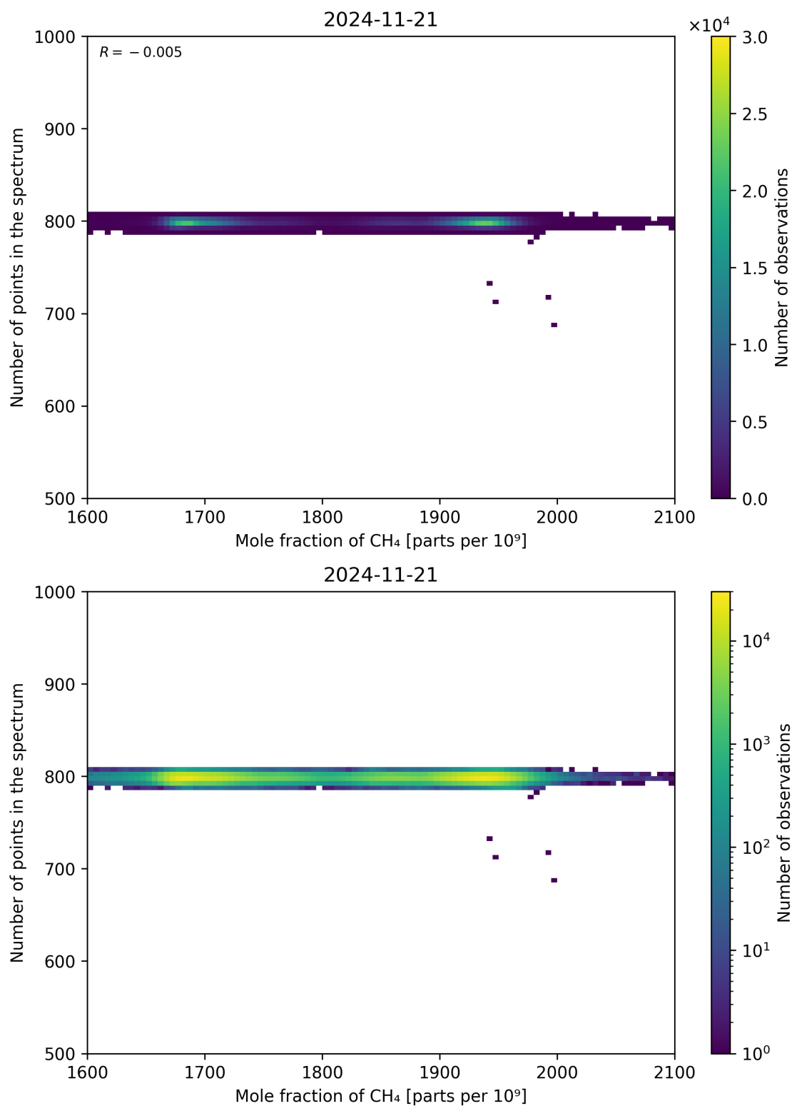
Figure 77: Scatter density plot of “Mole fraction of CH 4 ” against “Number of points in the spectrum” for 2024-11-20 to 2024-11-22.
