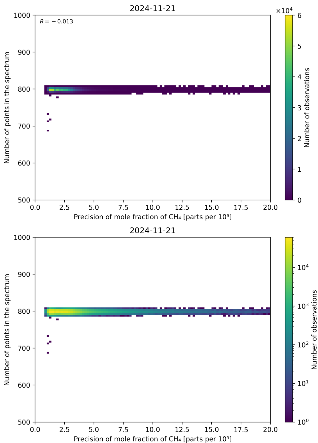
Figure 84: Scatter density plot of “Precision of mole fraction of CH 4 ” against “Number of points in the spectrum” for 2024-11-20 to 2024-11-22.
