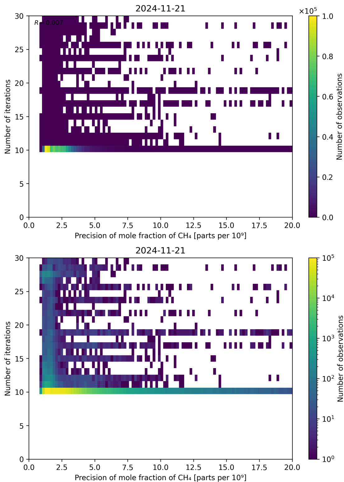
Figure 83: Scatter density plot of “Precision of mole fraction of CH 4 ” against “Number of iterations” for 2024-11-20 to 2024-11-22.
