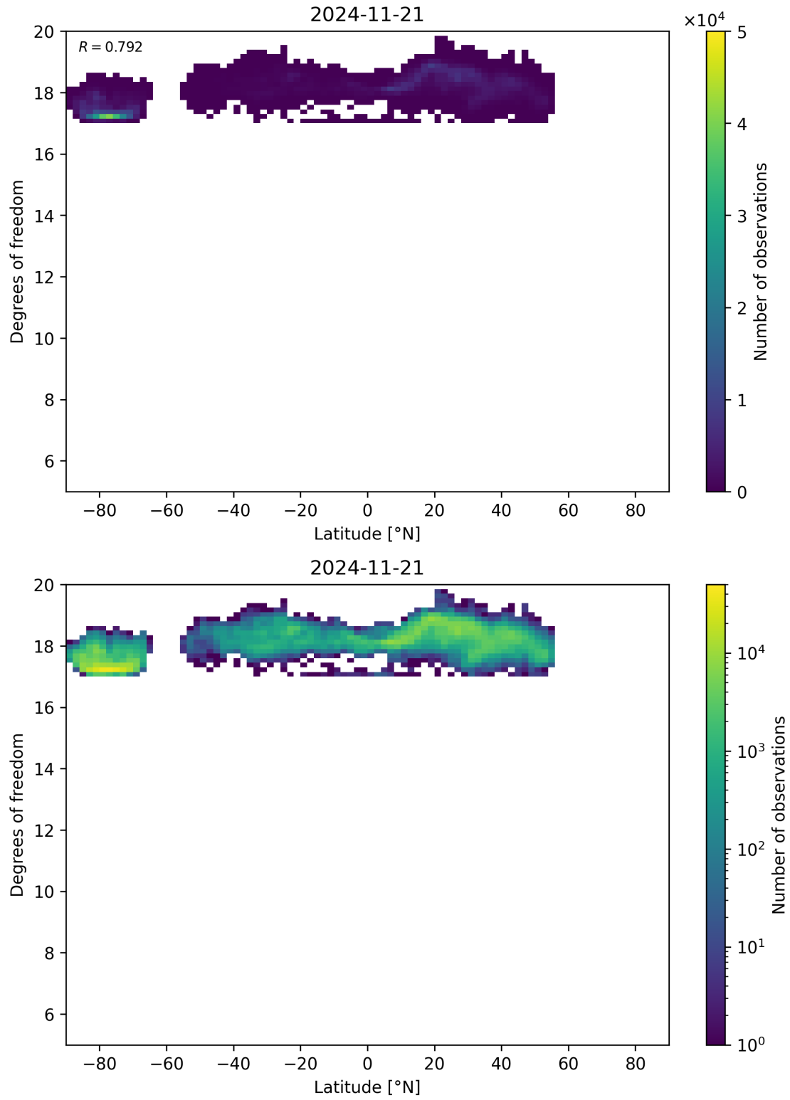
Figure 55: Scatter density plot of “Latitude” against “Degrees of freedom” for 2024-11-20 to 2024-11-22.
