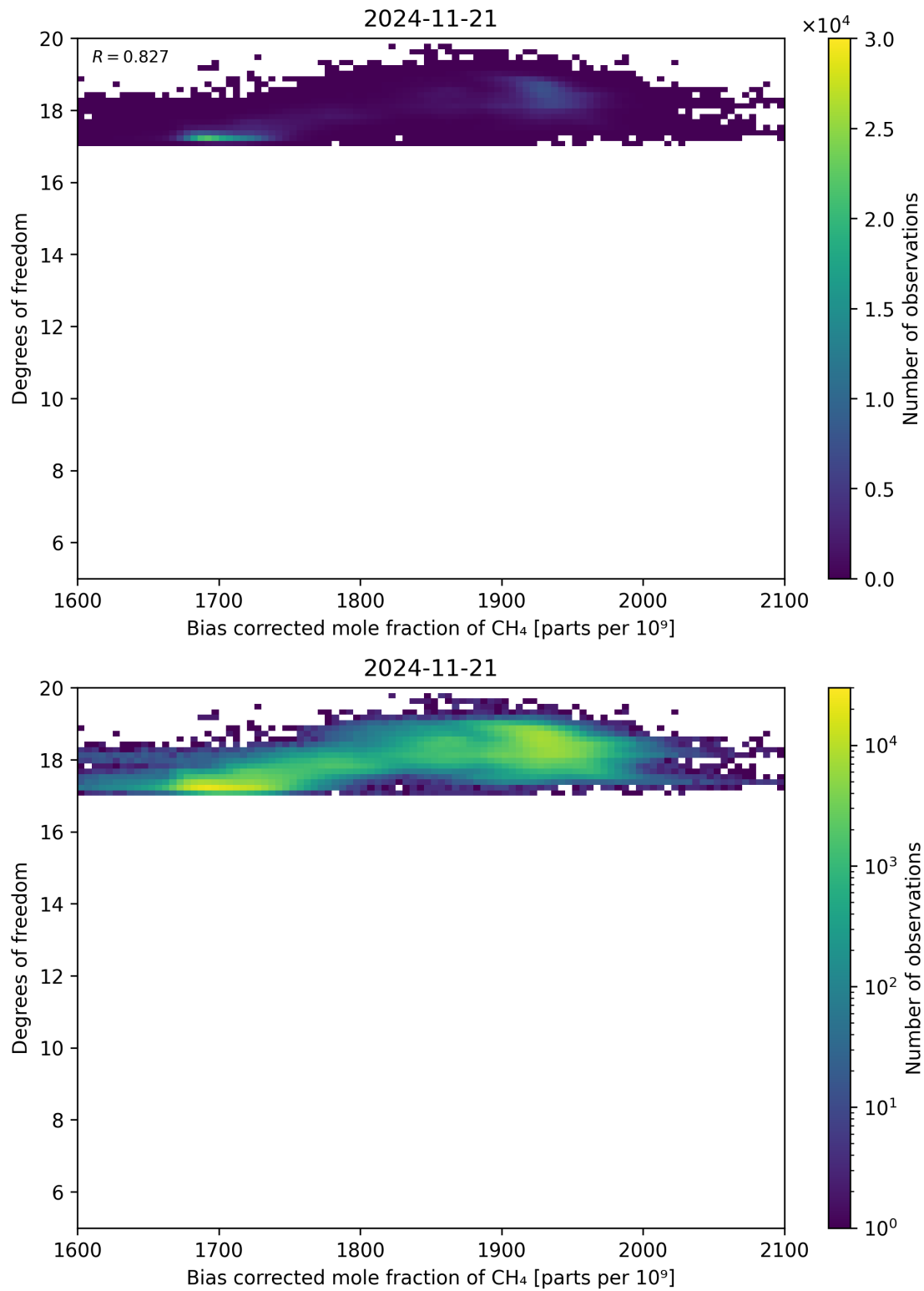
Figure 65: Scatter density plot of “Bias corrected mole fraction of CH 4 ” against “Degrees of freedom” for 2024-11-20 to 2024-11-22.
