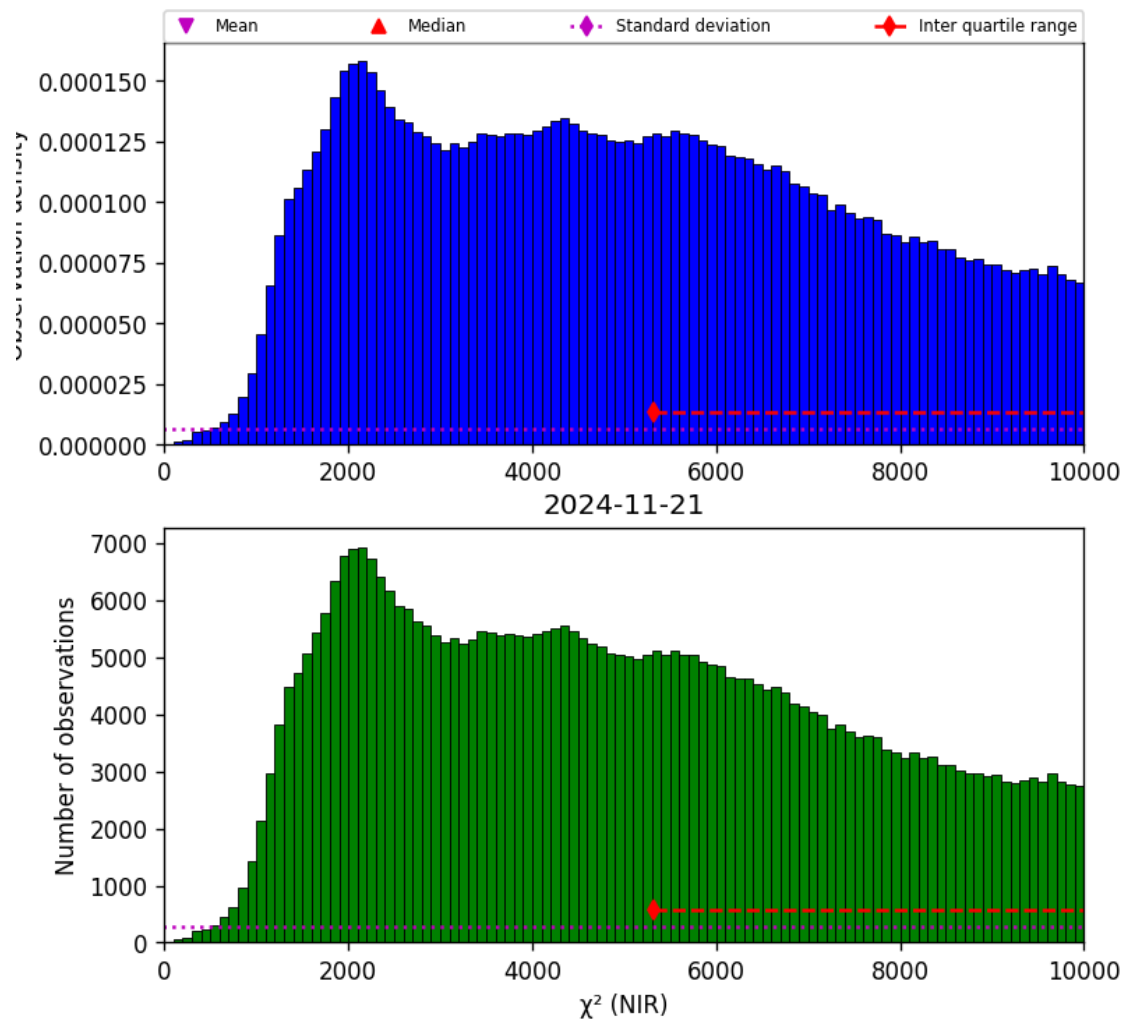
Figure 29: Histogram of “ \chi^2 (NIR)” for 2024-11-20 to 2024-11-22
