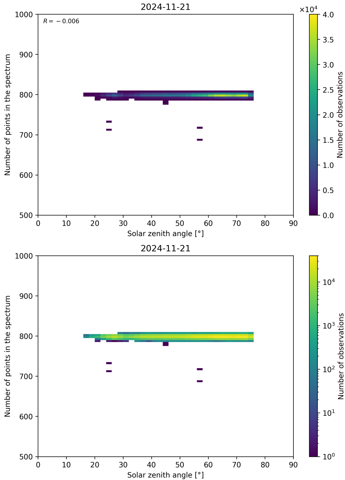
Figure 103: Scatter density plot of “Solar zenith angle” against “Number of points in the spectrum” for 2024-11-20 to 2024-11-22.
