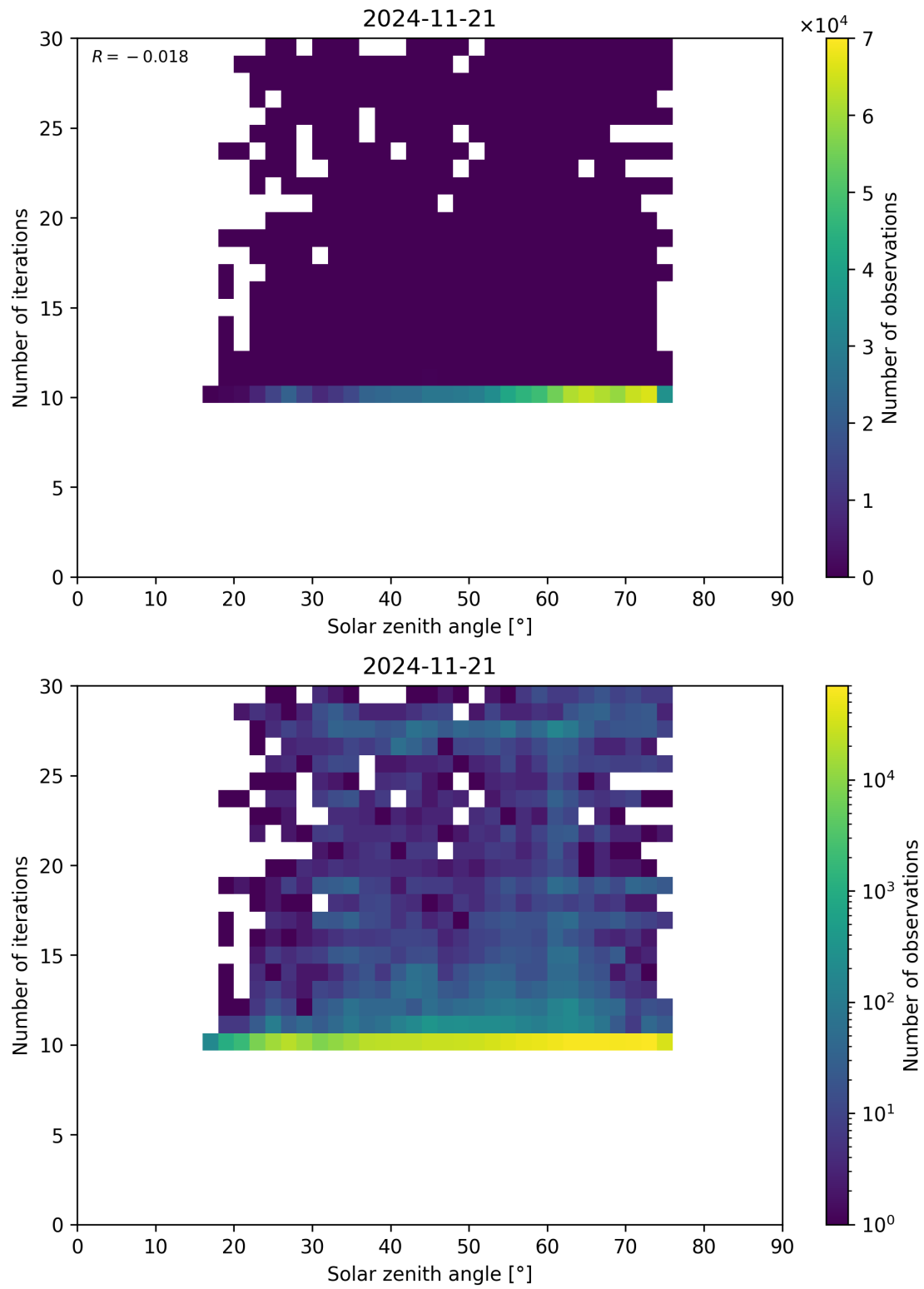
Figure 102: Scatter density plot of “Solar zenith angle” against “Number of iterations” for 2024-11-20 to 2024-11-22.
