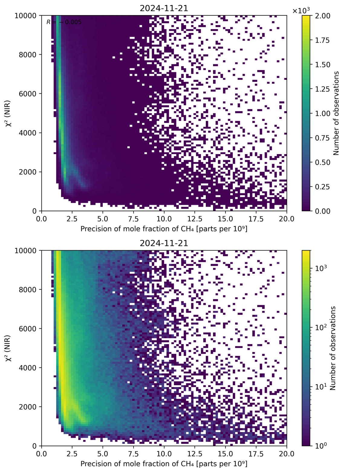
Figure 78: Scatter density plot of “Precision of mole fraction of CH 4 ” against “ \chi^2 (NIR)” for 2024-11-20 to 2024-11-22.
