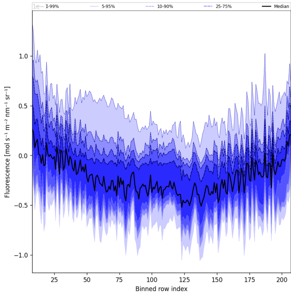
Figure 43: Along track statistics of “Fluorescence” for 2024-11-20 to 2024-11-22
