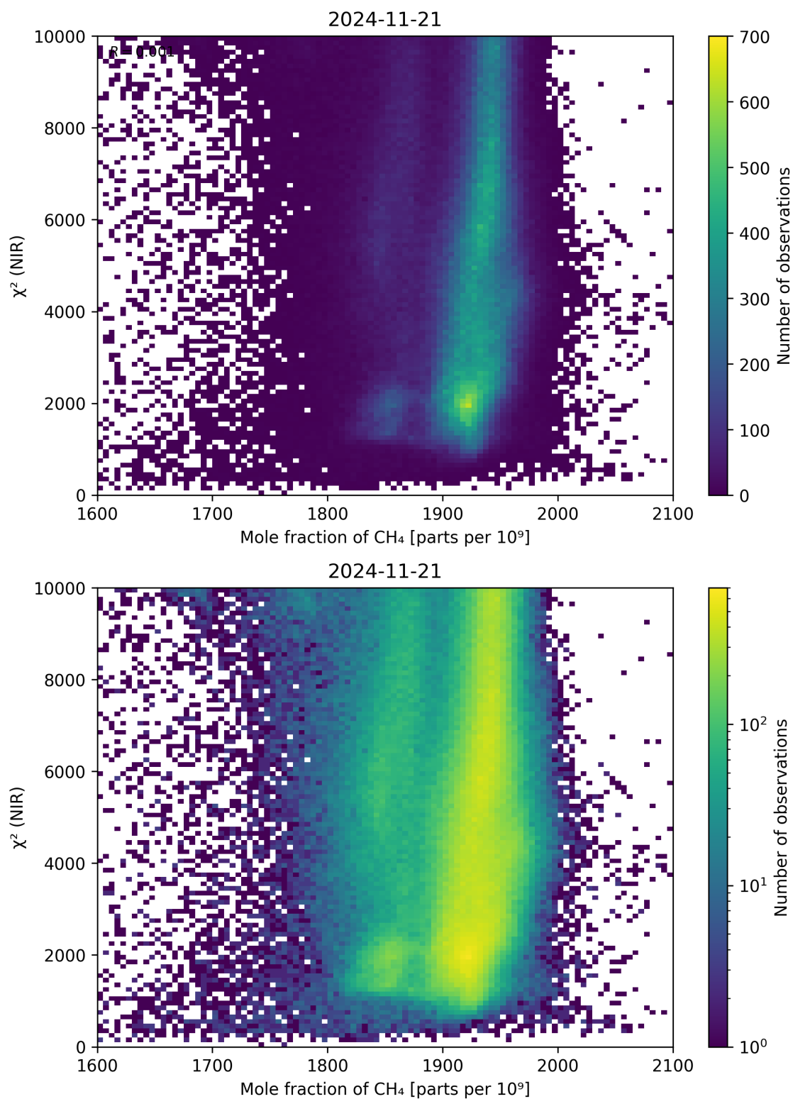
Figure 70: Scatter density plot of “Mole fraction of \text{CH}_4 ” against “ \chi^2 (NIR)” for 2024-11-20 to 2024-11-22.
