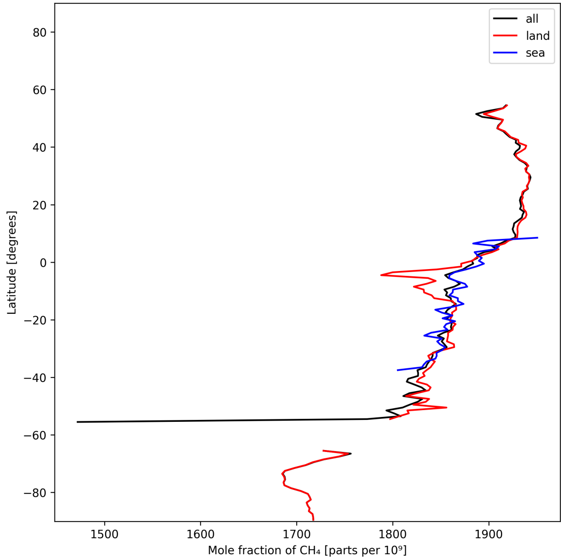
Figure 12: Zonal average of “Mole fraction of CH 4 ” for 2024-11-20 to 2024-11-22.
