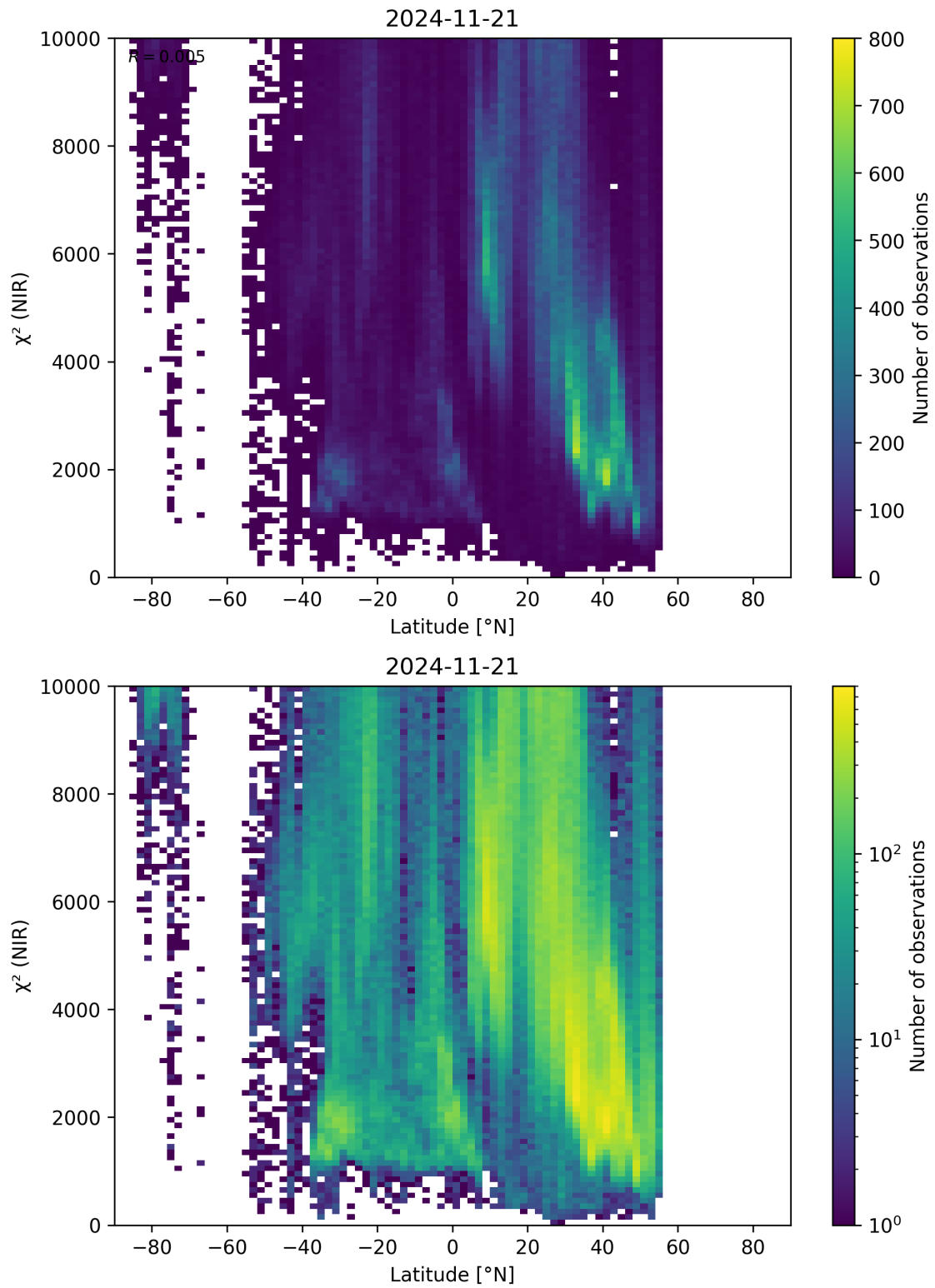
Figure 53: Scatter density plot of “Latitude” against “ \chi^2 (NIR)” for 2024-11-20 to 2024-11-22.
