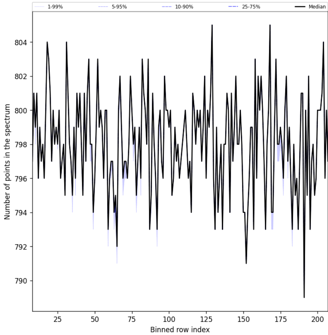
Figure 37: Along track statistics of “Number of points in the spectrum” for 2024-11-20 to 2024-11-22
