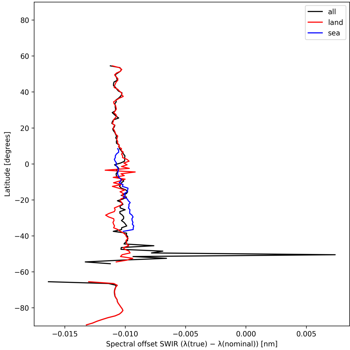
Figure 16: Zonal average of “Spectral offset SWIR ( \lambda_{\text{true}} - \lambda_{\text{nominal}} )” for 2024-11-20 to 2024-11-22.
