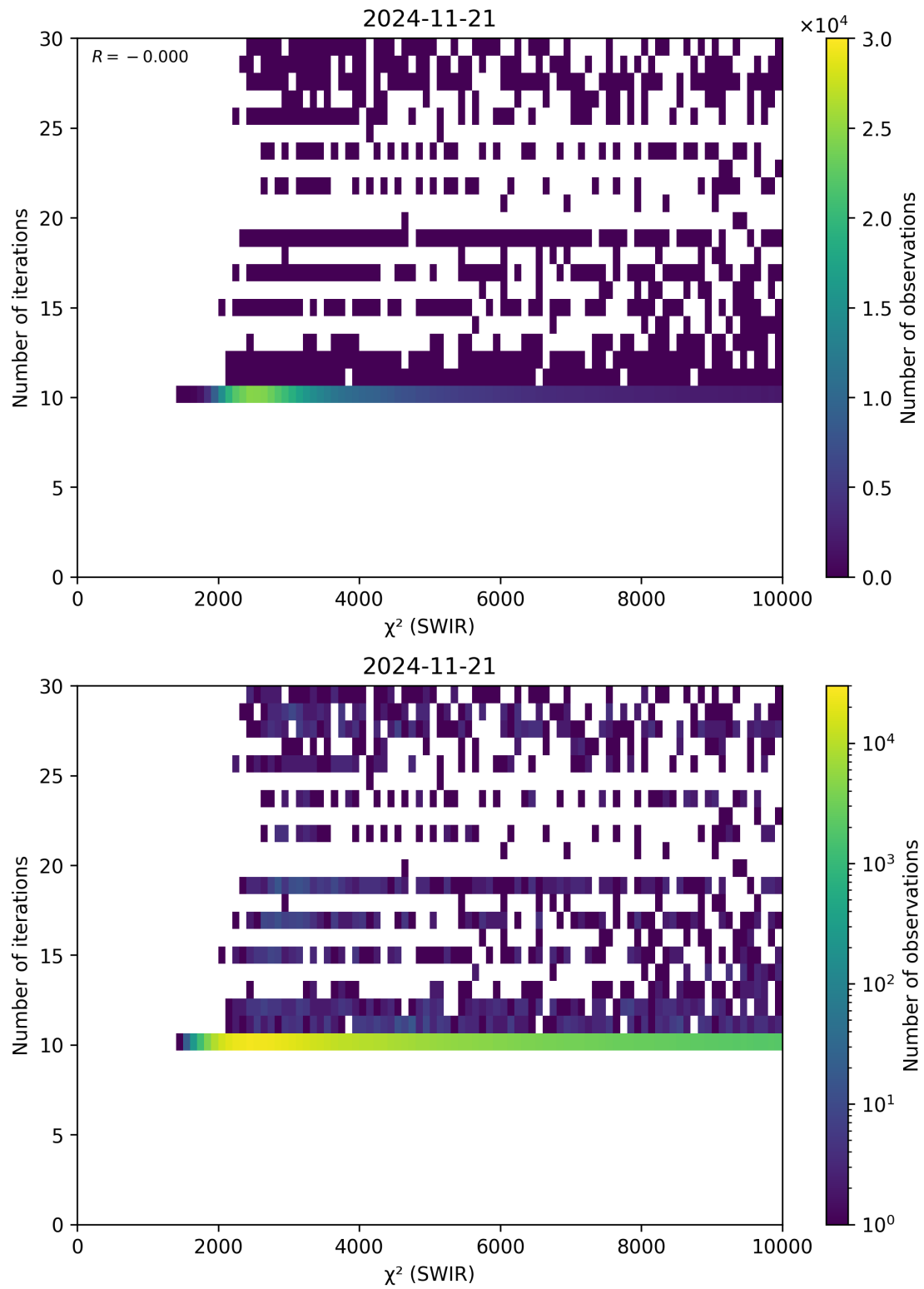
Figure 50: Scatter density plot of “ \chi^2 (SWIR)” against “Number of iterations” for 2024-11-20 to 2024-11-22.
