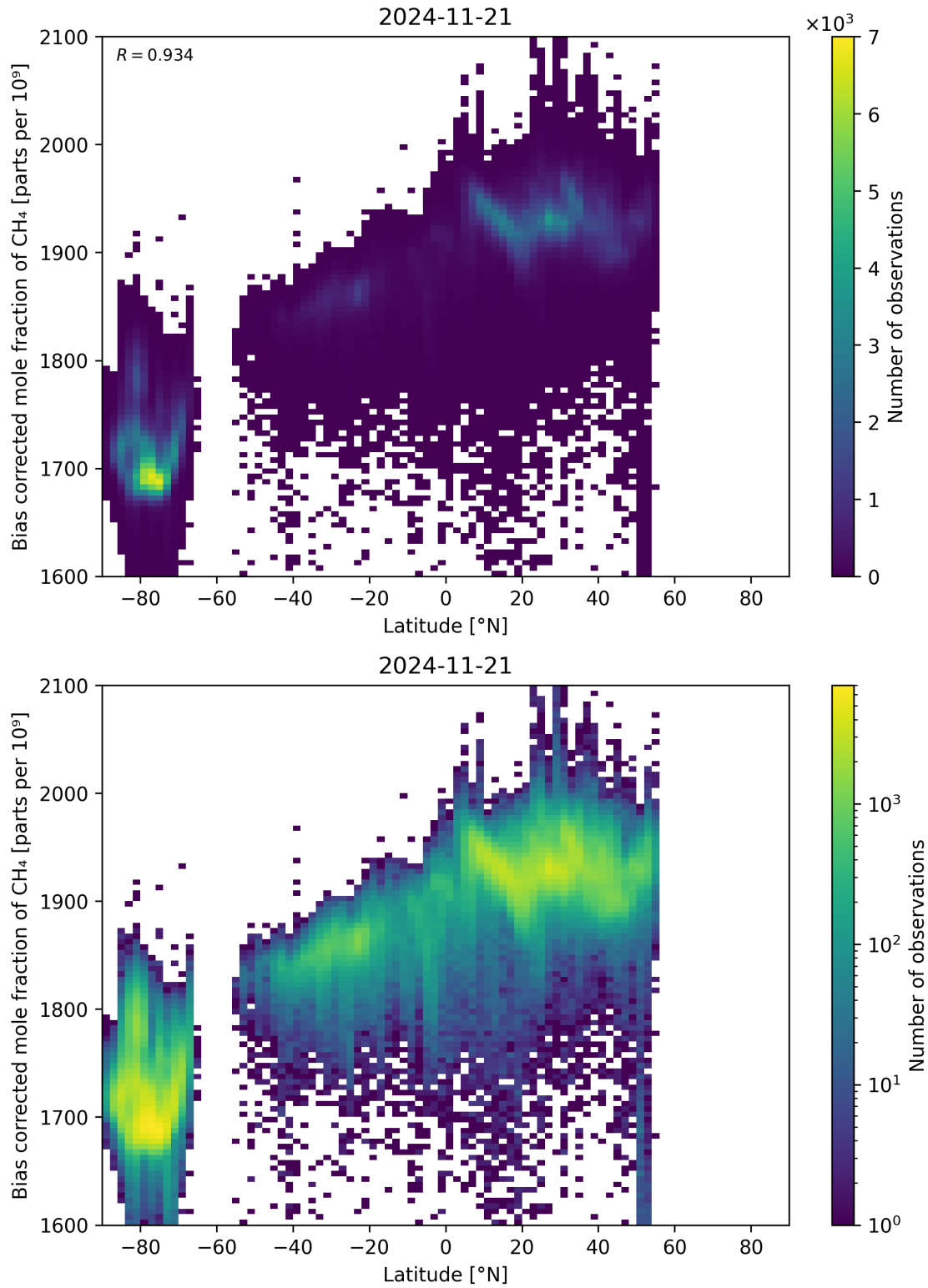
Figure 58: Scatter density plot of “Latitude” against “Bias corrected mole fraction of CH 4 ” for 2024-11-20 to 2024-11-22.
