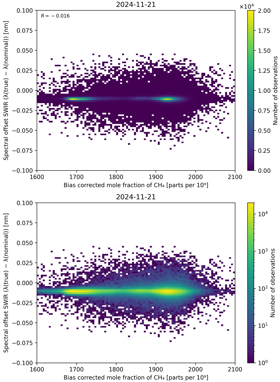
Figure 69: Scatter density plot of “Bias corrected mole fraction of \text{CH}_4 ” against “Spectral offset SWIR ( \lambda_{\text{true}} - \lambda_{\text{nominal}} )” for 2024-11-20 to 2024-11-22.
