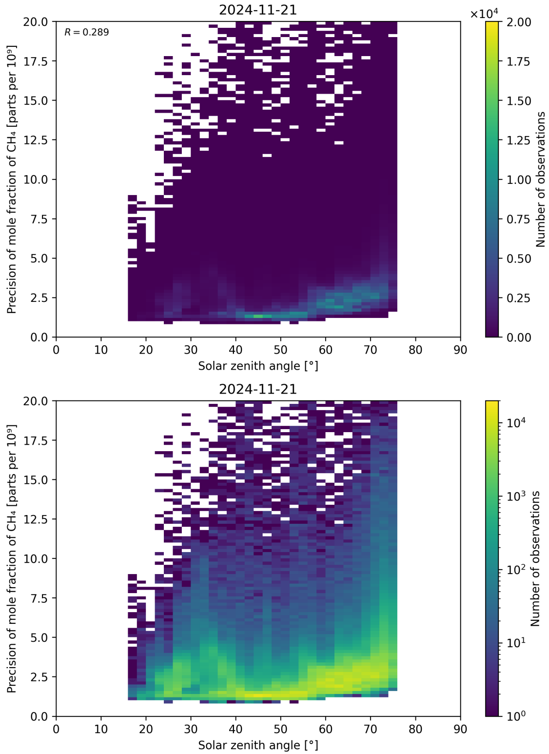
Figure 101: Scatter density plot of “Solar zenith angle” against “Precision of mole fraction of CH 4 ” for 2024-11-20 to 2024-11-22.
