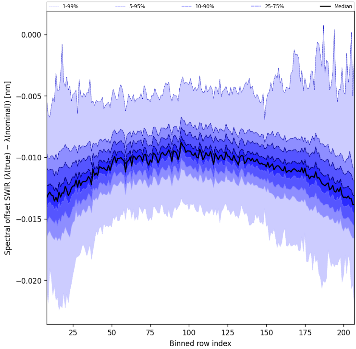
Figure 38: Along track statistics of “Spectral offset SWIR ( \lambda_{\text{true}} - \lambda_{\text{nominal}} )” for 2024-11-20 to 2024-11-22
