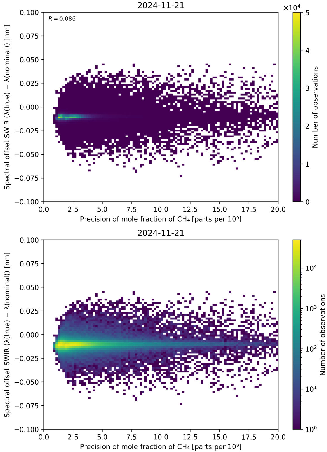
Figure 85: Scatter density plot of “Precision of mole fraction of \text{CH}_4 ” against “Spectral offset SWIR ( \lambda_{\text{true}} - \lambda_{\text{nominal}} )” for 2024-11-20 to 2024-11-22.
