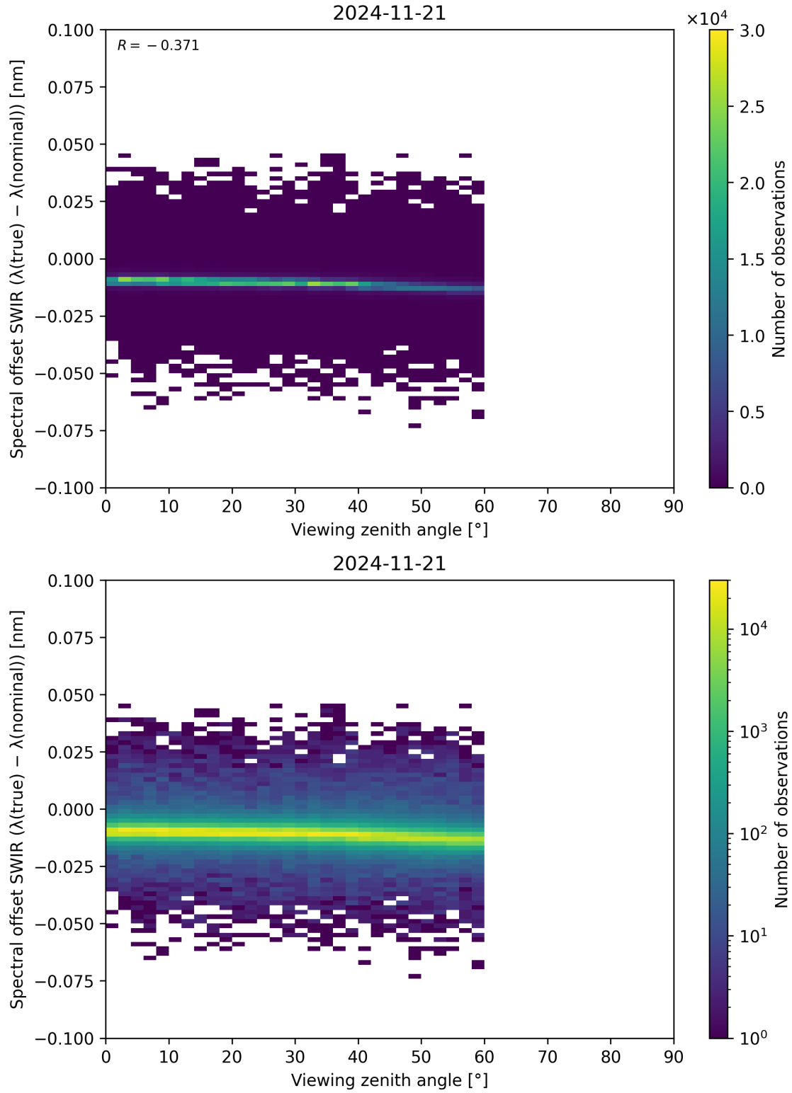
Figure 116: Scatter density plot of “Viewing zenith angle” against “Spectral offset SWIR ( \lambda_{\text{true}} - \lambda_{\text{nominal}} )” for 2024-11-20 to 2024-11-22.
