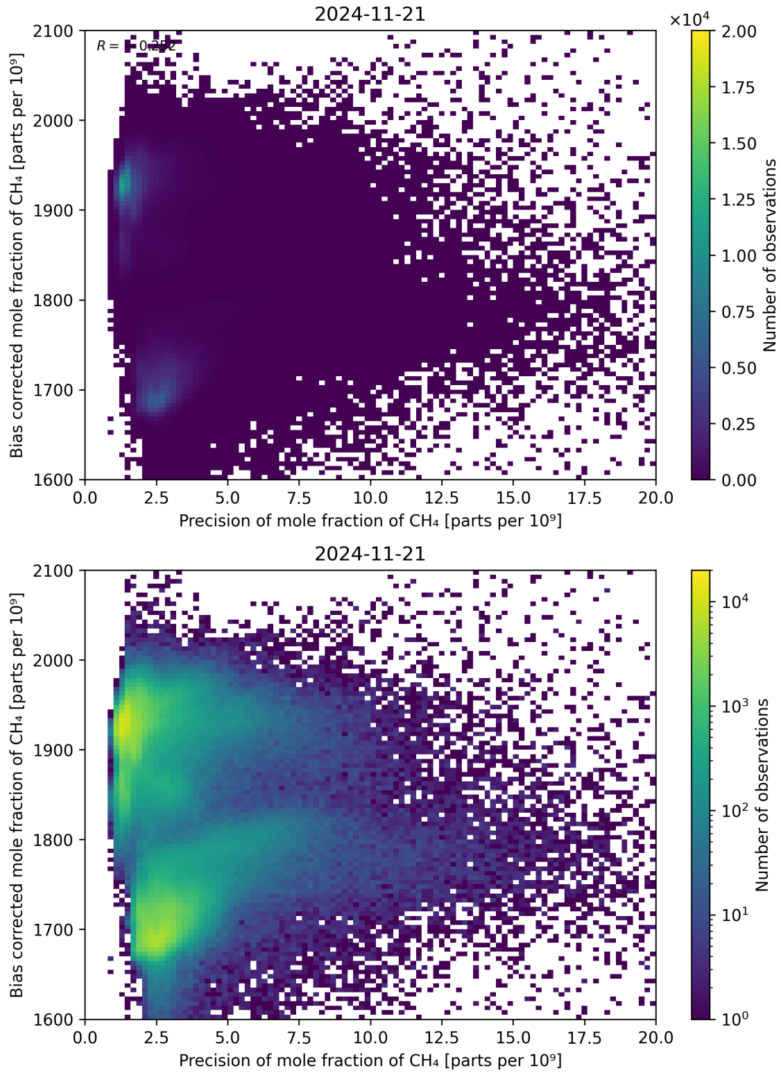
Figure 82: Scatter density plot of “Precision of mole fraction of \text{CH}_4 ” against “Bias corrected mole fraction of \text{CH}_4 ” for 2024-11-20 to 2024-11-22.
