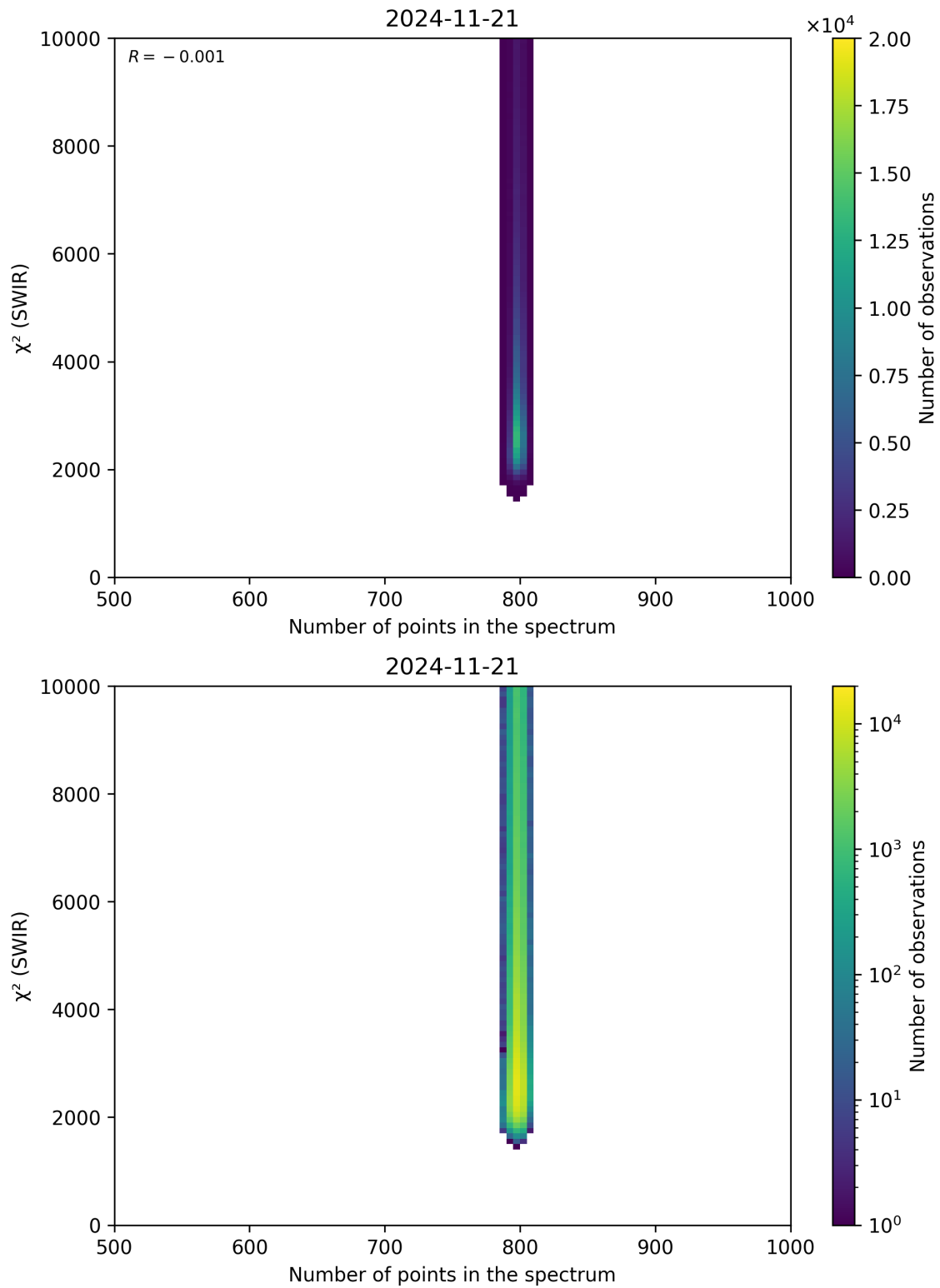
Figure 89: Scatter density plot of “Number of points in the spectrum” against “ \chi^2 (SWIR)” for 2024-11-20 to 2024-11-22.
