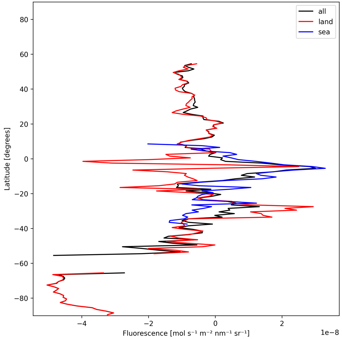
Figure 21: Zonal average of “Fluorescence” for 2024-11-20 to 2024-11-22.
