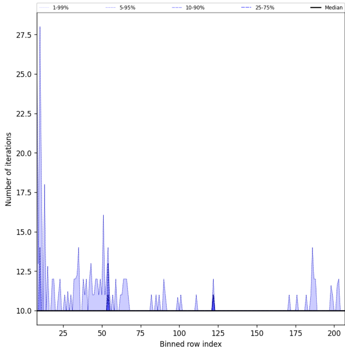
Figure 42: Along track statistics of “Number of iterations” for 2024-11-20 to 2024-11-22
