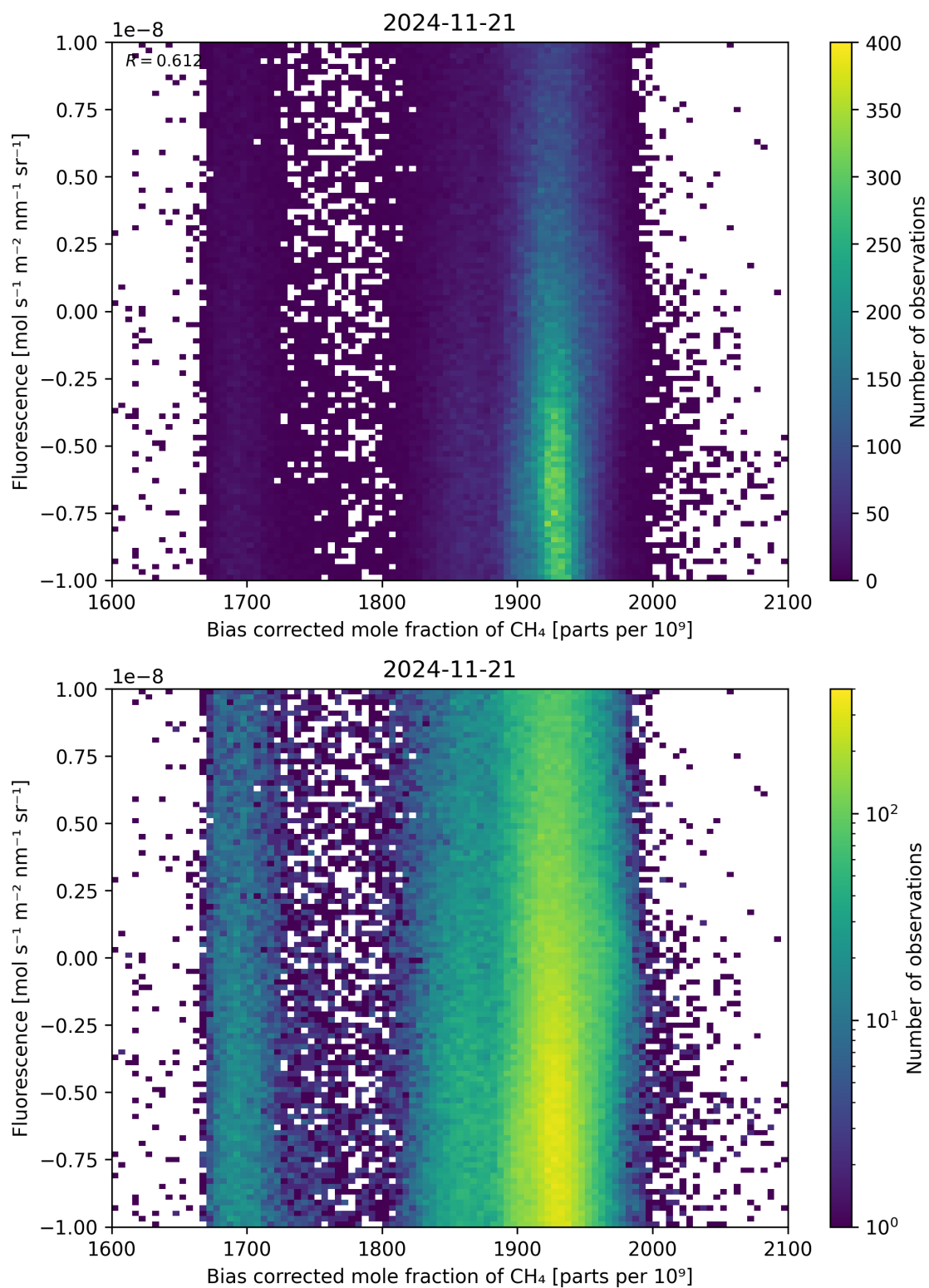
Figure 66: Scatter density plot of “Bias corrected mole fraction of CH 4 ” against “Fluorescence” for 2024-11-20 to 2024-11-22.
