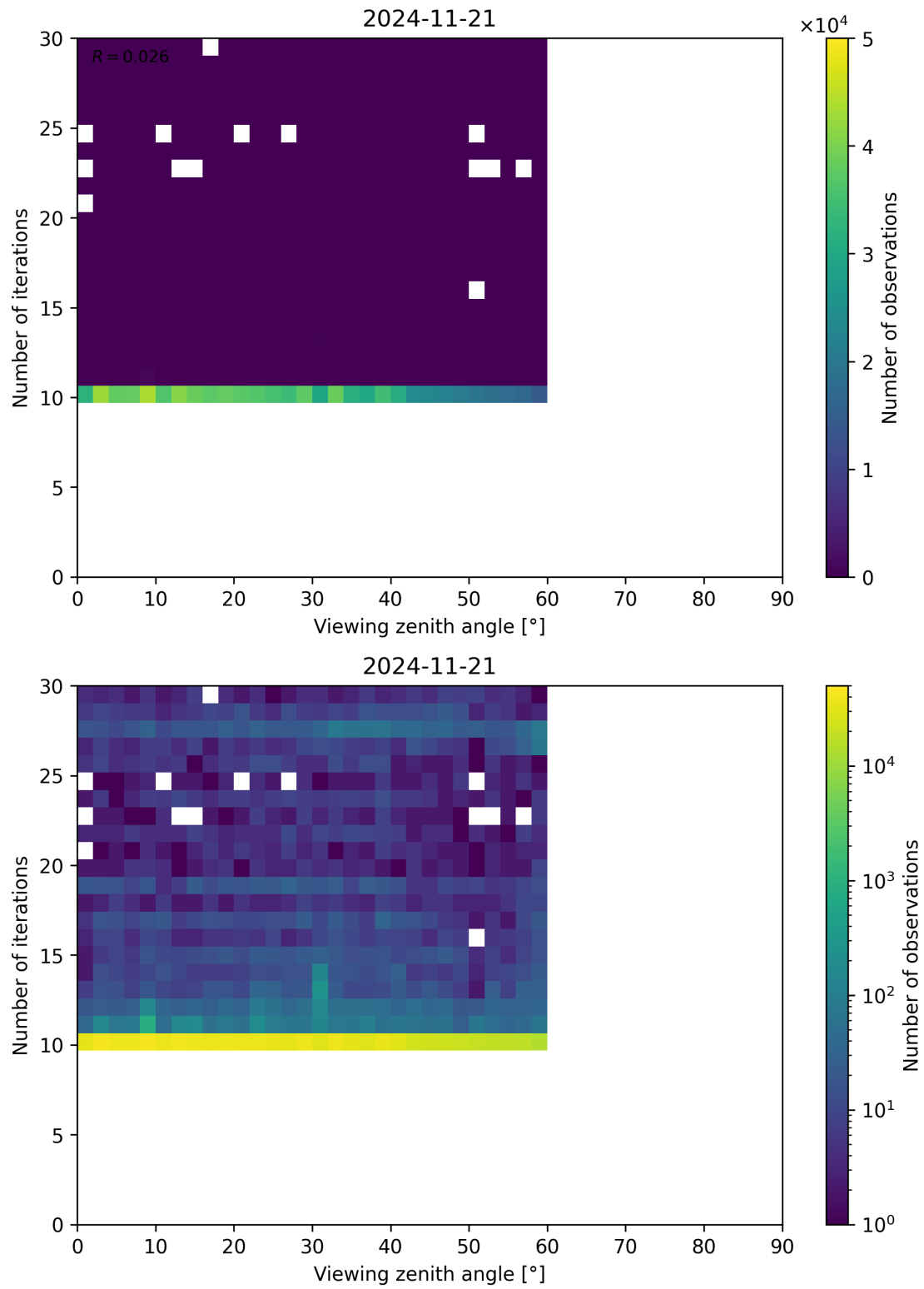
Figure 113: Scatter density plot of “Viewing zenith angle” against “Number of iterations” for 2024-11-20 to 2024-11-22.
