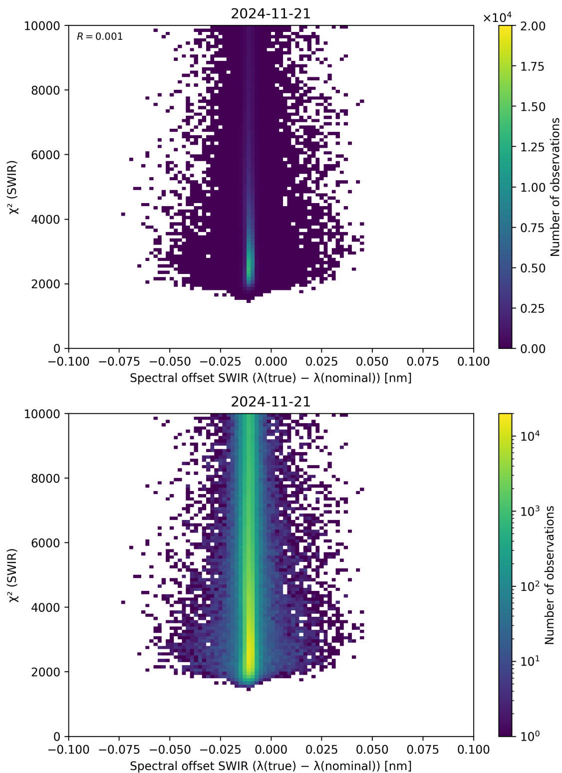
Figure 118: Scatter density plot of “Spectral offset SWIR ( \lambda_{\text{true}} - \lambda_{\text{nominal}} )” against “ \chi^2 (SWIR)” for 2024-11-20 to 2024-11-22.
