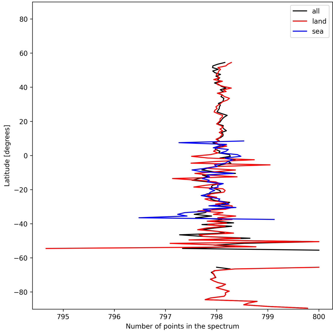
Figure 15: Zonal average of “Number of points in the spectrum” for 2024-11-20 to 2024-11-22.
