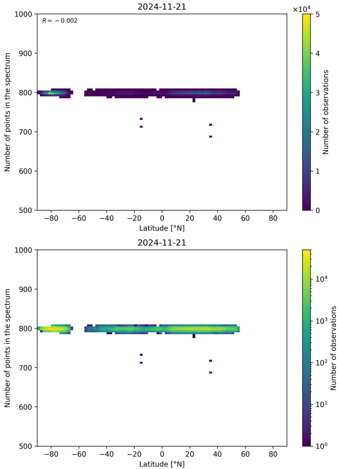
Figure 61: Scatter density plot of “Latitude” against “Number of points in the spectrum” for 2024-11-20 to 2024-11-22.
