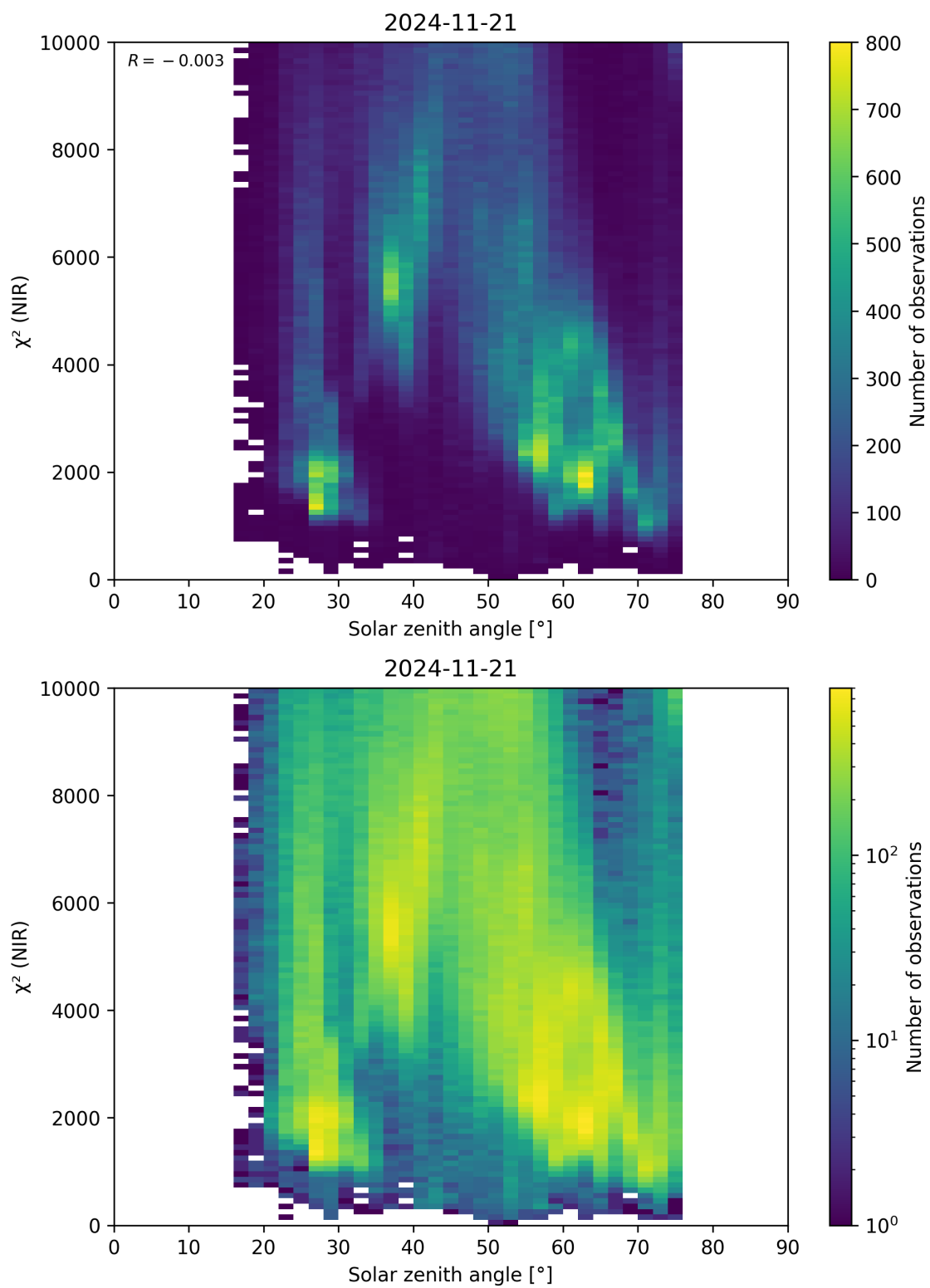
Figure 94: Scatter density plot of “Solar zenith angle” against “ \chi^2 (NIR)” for 2024-11-20 to 2024-11-22.
