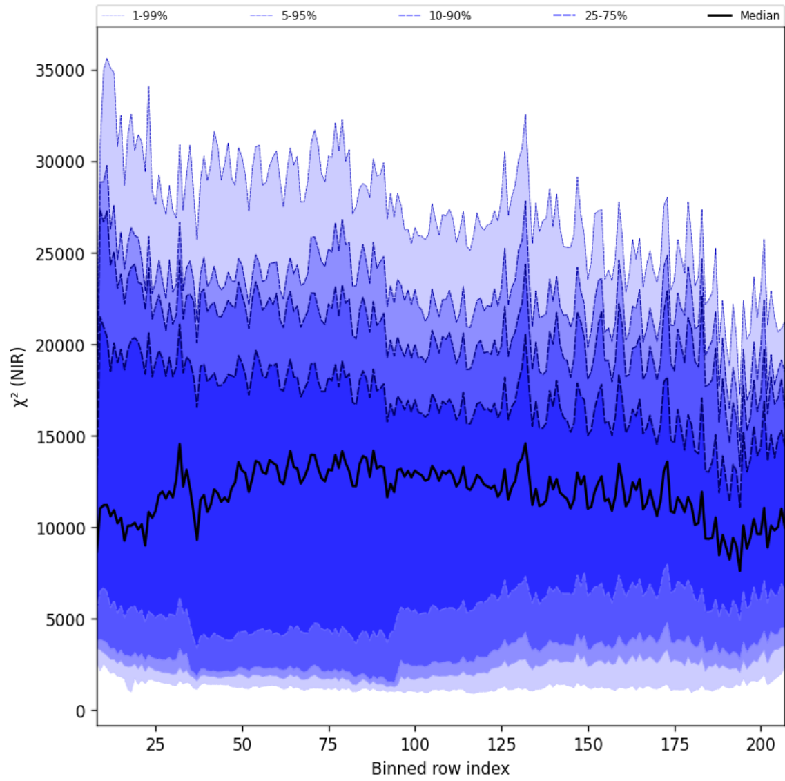
Figure 40: Along track statistics of “ \chi^2 (NIR)” for 2024-11-20 to 2024-11-22
