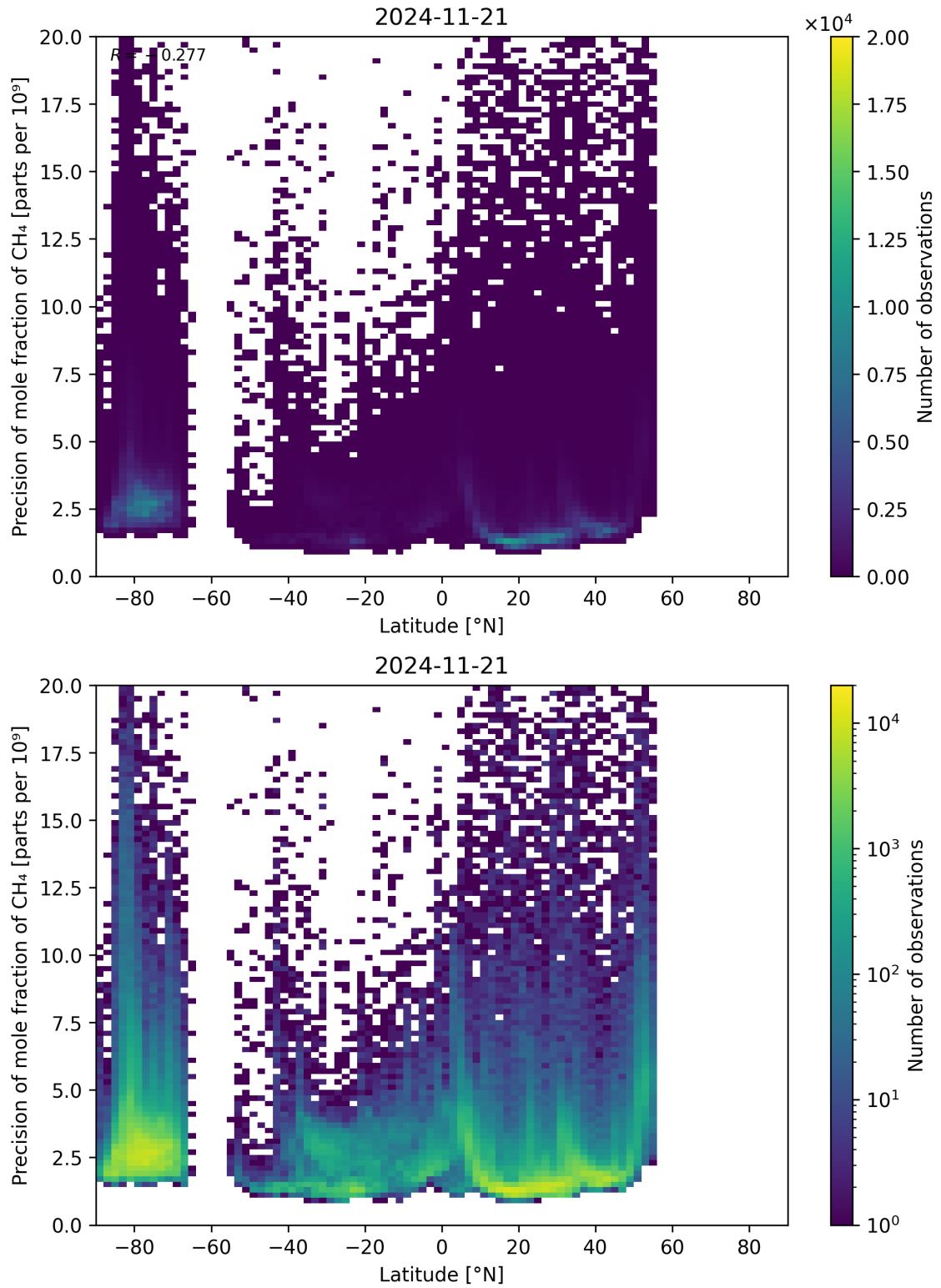
Figure 59: Scatter density plot of “Latitude” against “Precision of mole fraction of CH 4 ” for 2024-11-20 to 2024-11-22.
