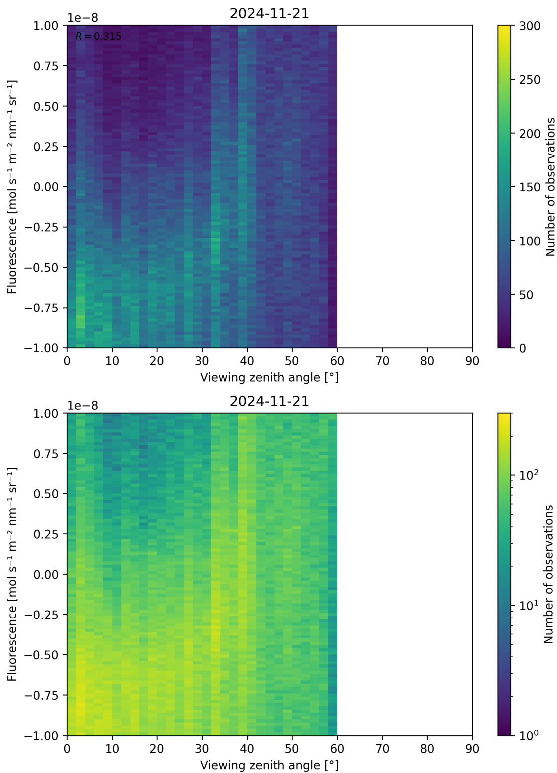
Figure 108: Scatter density plot of “Viewing zenith angle” against “Fluorescence” for 2024-11-20 to 2024-11-22.
