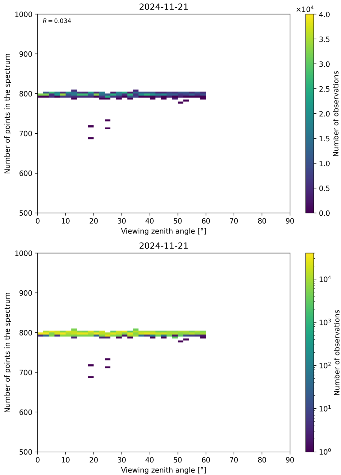
Figure 114: Scatter density plot of “Viewing zenith angle” against “Number of points in the spectrum” for 2024-11-20 to 2024-11-22.
