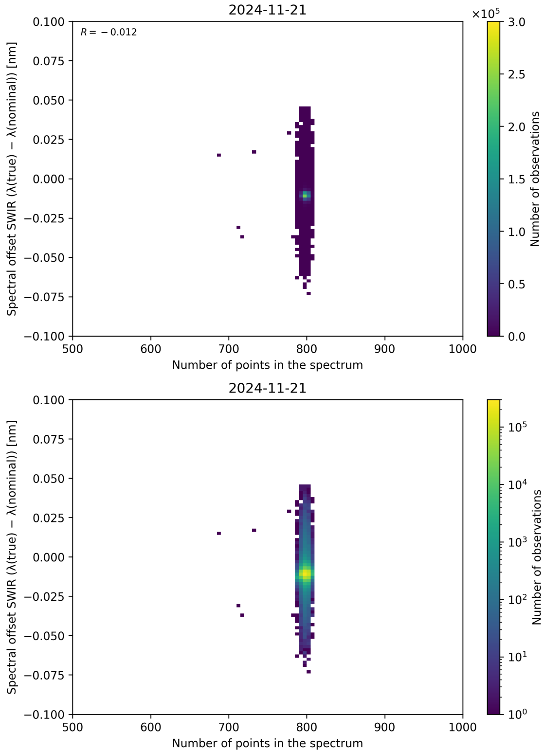
Figure 93: Scatter density plot of “Number of points in the spectrum” against “Spectral offset SWIR ( \lambda_{\text{true}} - \lambda_{\text{nominal}} )” for 2024-11-20 to 2024-11-22.
