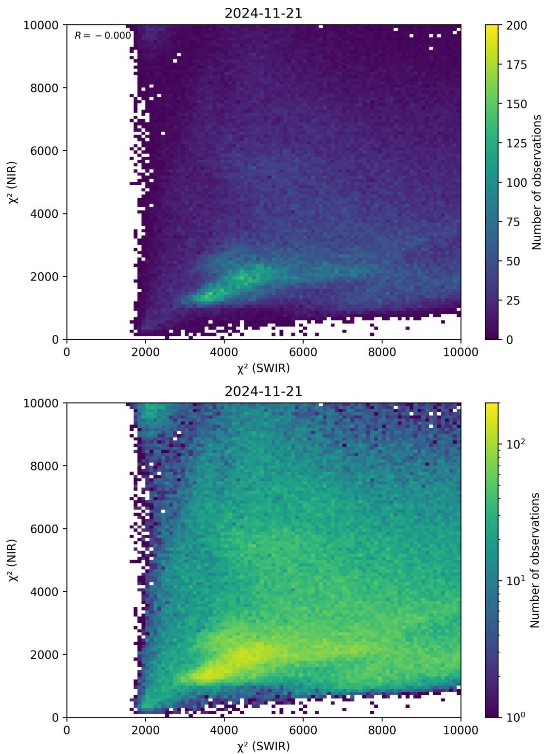
Figure 47: Scatter density plot of “ \chi^2 (SWIR)” against “ \chi^2 (NIR)” for 2024-11-20 to 2024-11-22.
