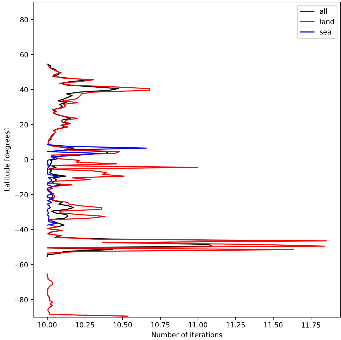
Figure 20: Zonal average of “Number of iterations” for 2024-11-20 to 2024-11-22.
