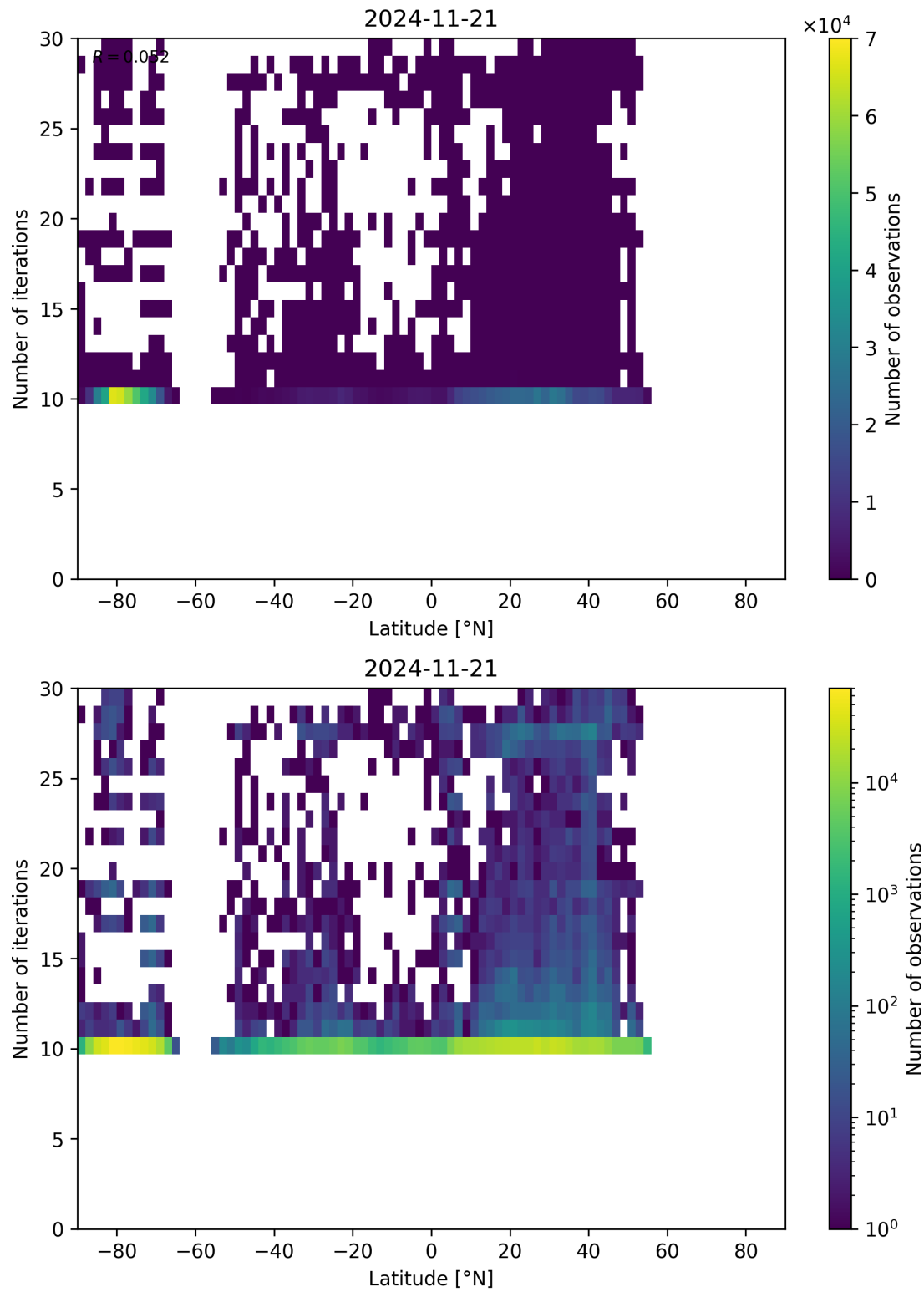
Figure 60: Scatter density plot of “Latitude” against “Number of iterations” for 2024-11-20 to 2024-11-22.
