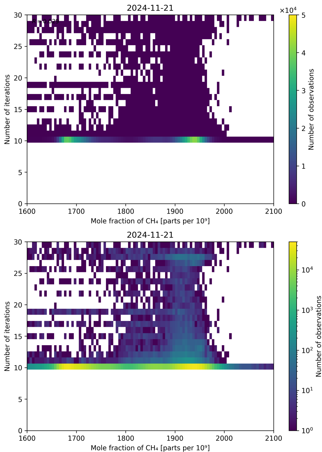
Figure 76: Scatter density plot of “Mole fraction of CH 4 ” against “Number of iterations” for 2024-11-20 to 2024-11-22.
