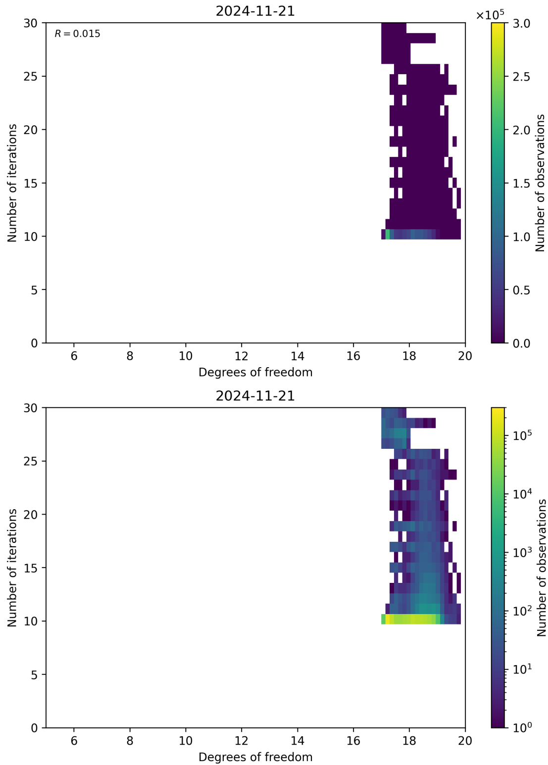
Figure 52: Scatter density plot of “Degrees of freedom” against “Number of iterations” for 2024-11-20 to 2024-11-22.
