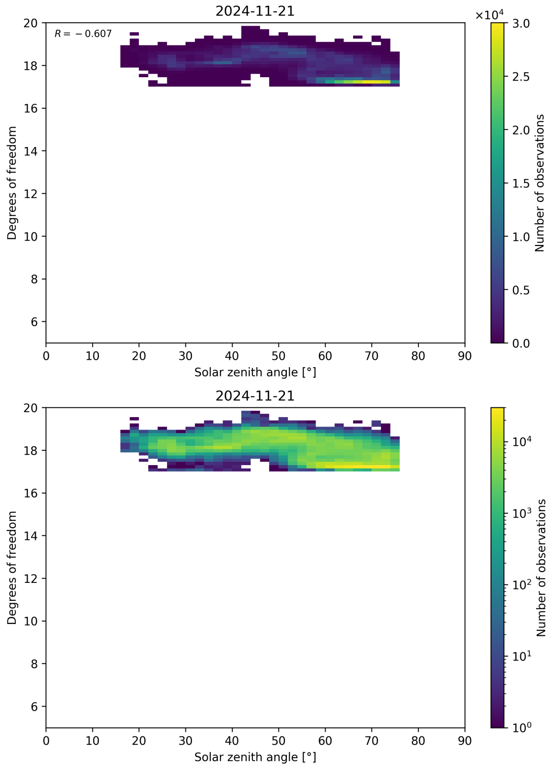
Figure 96: Scatter density plot of “Solar zenith angle” against “Degrees of freedom” for 2024-11-20 to 2024-11-22.
