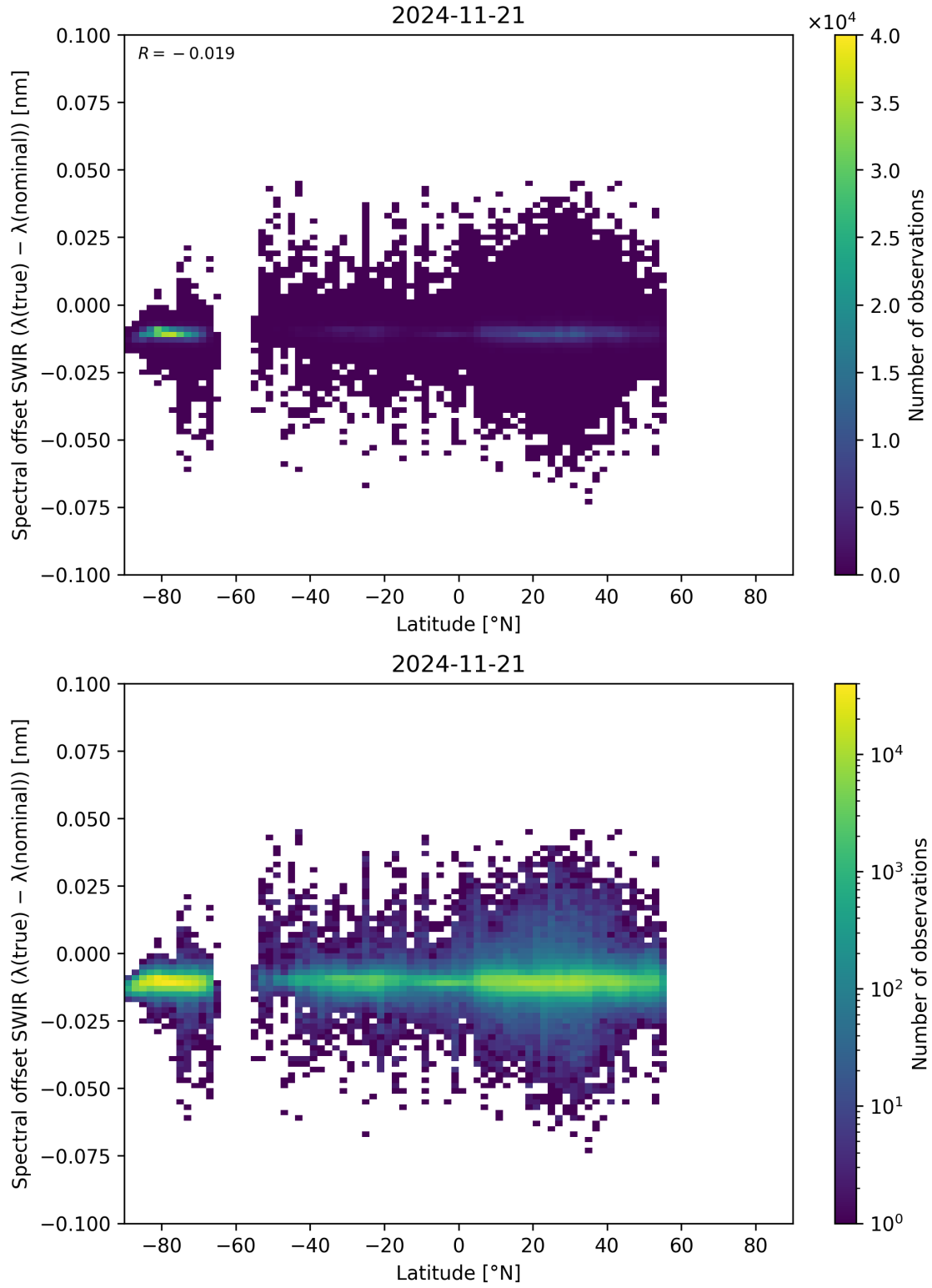
Figure 62: Scatter density plot of “Latitude” against “Spectral offset SWIR ( \lambda_{\text{true}} - \lambda_{\text{nominal}} )” for 2024-11-20 to 2024-11-22.
