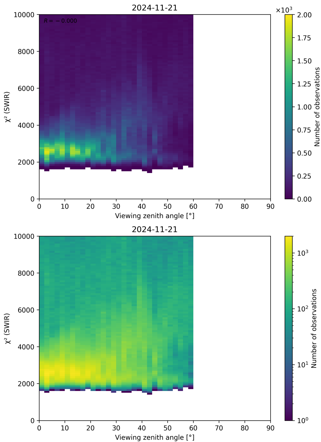
Figure 106: Scatter density plot of “Viewing zenith angle” against “ \chi^2 (SWIR)” for 2024-11-20 to 2024-11-22.
