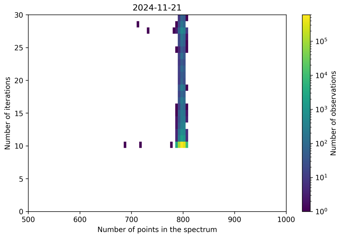
Figure 92: Scatter density plot of “Number of points in the spectrum” against “Number of iterations” for 2024-11-20 to 2024-11-22.
