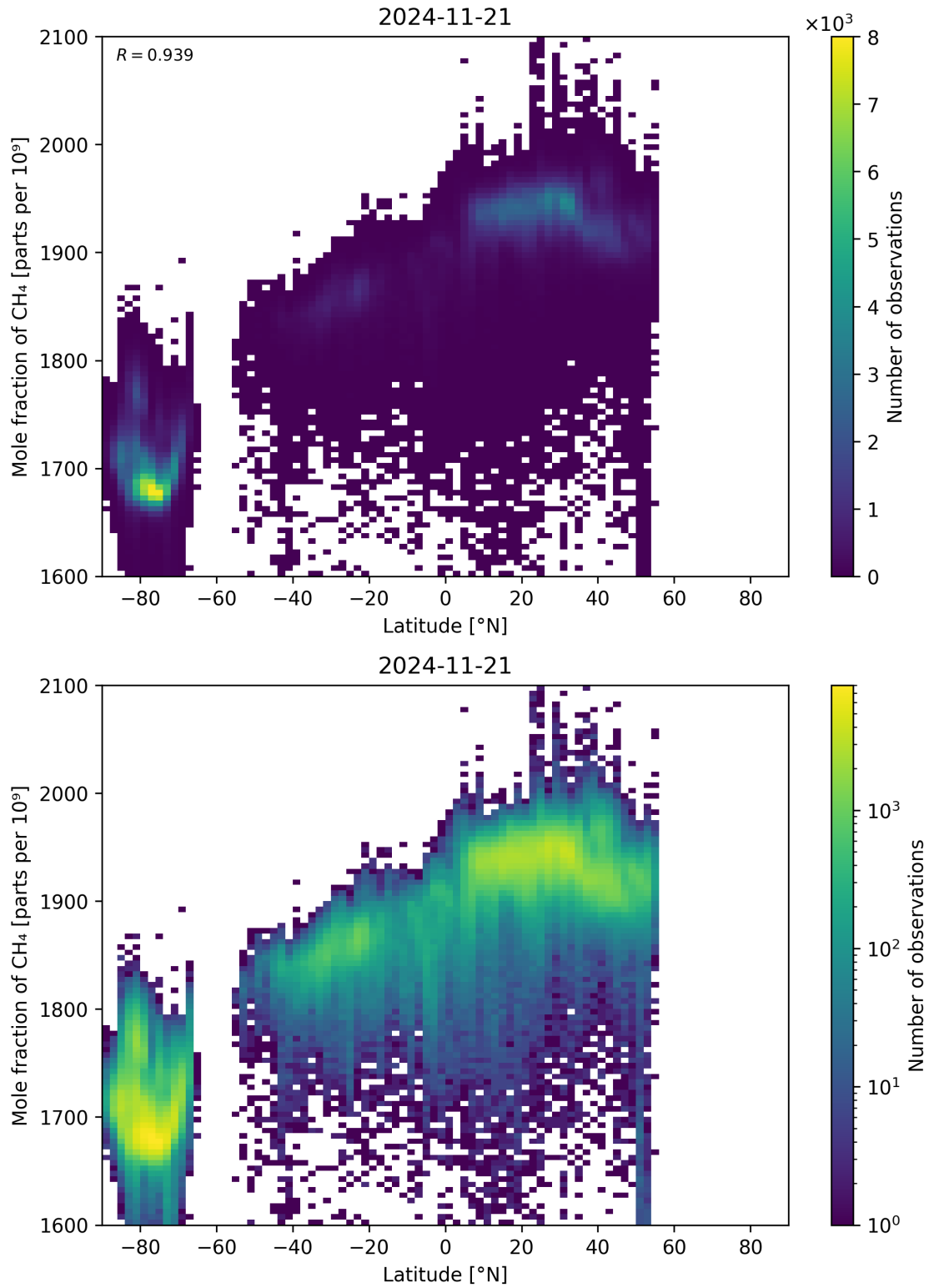
Figure 57: Scatter density plot of “Latitude” against “Mole fraction of \text{CH}_4 ” for 2024-11-20 to 2024-11-22.
