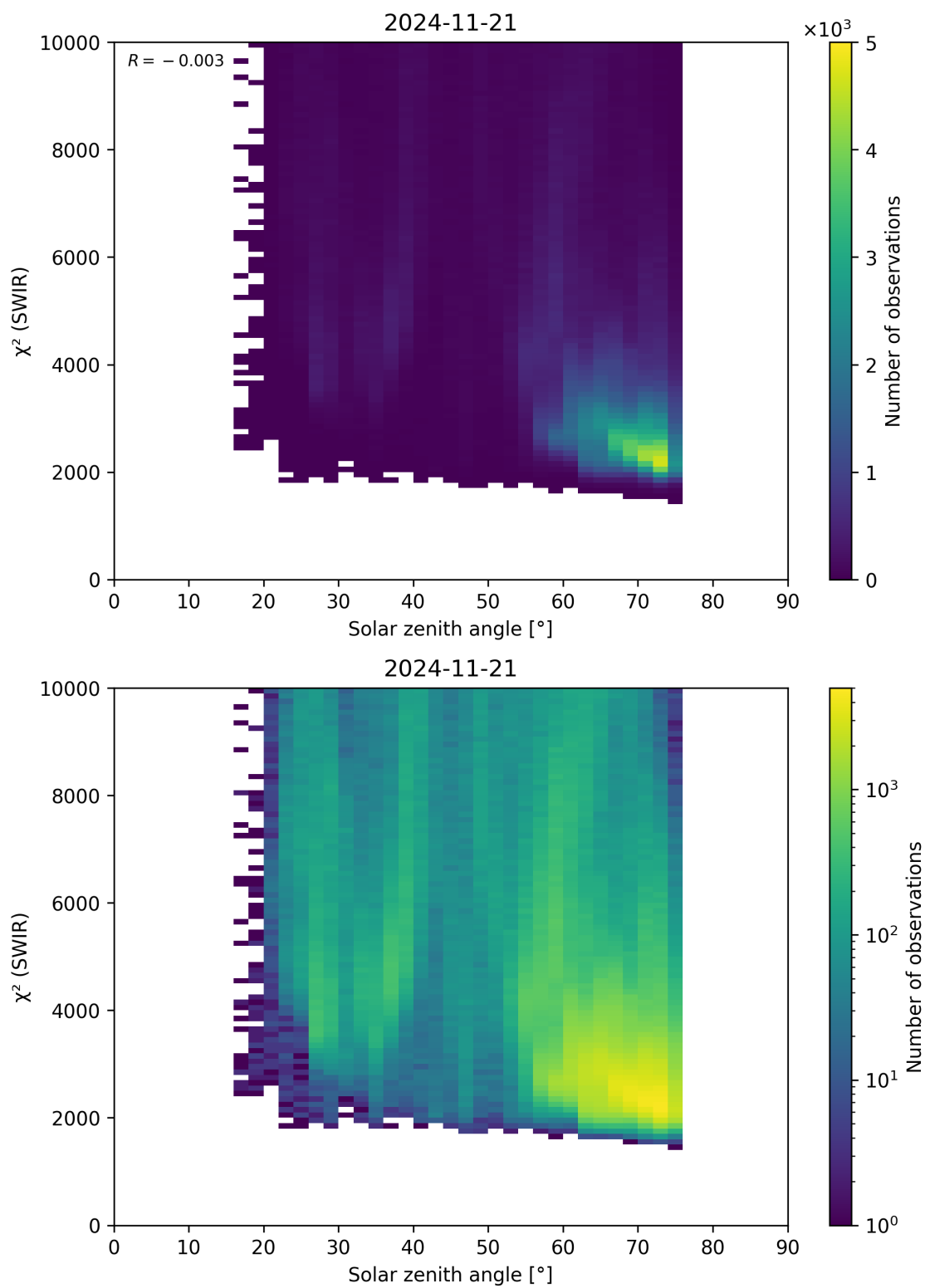
Figure 95: Scatter density plot of “Solar zenith angle” against “ \chi^2 (SWIR)” for 2024-11-20 to 2024-11-22.
