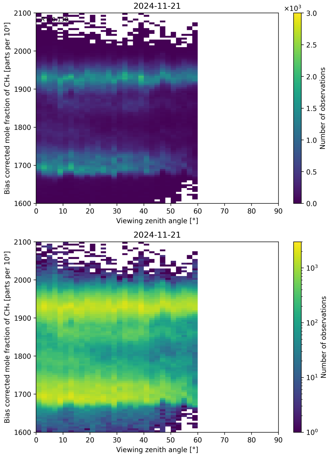
Figure 111: Scatter density plot of “Viewing zenith angle” against “Bias corrected mole fraction of CH 4 ” for 2024-11-20 to 2024-11-22.
