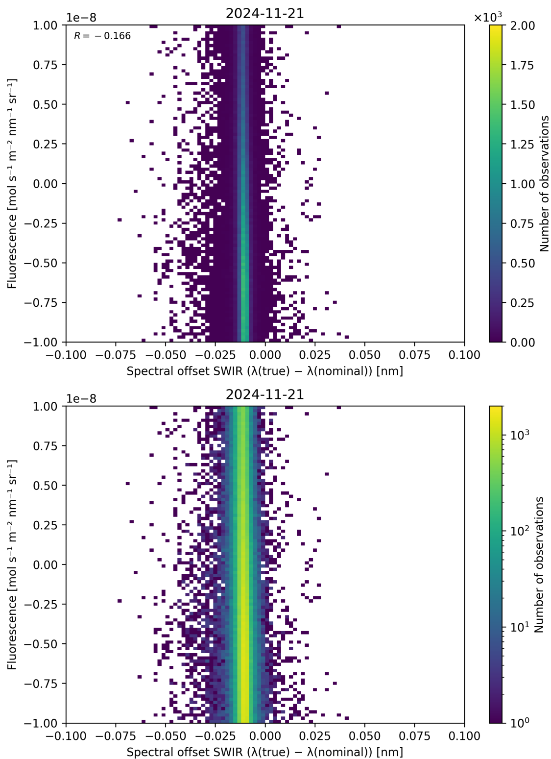
Figure 120: Scatter density plot of “Spectral offset SWIR ( \lambda_{\text{true}} - \lambda_{\text{nominal}} )” against “Fluorescence” for 2024-11-20 to 2024-11-22.
