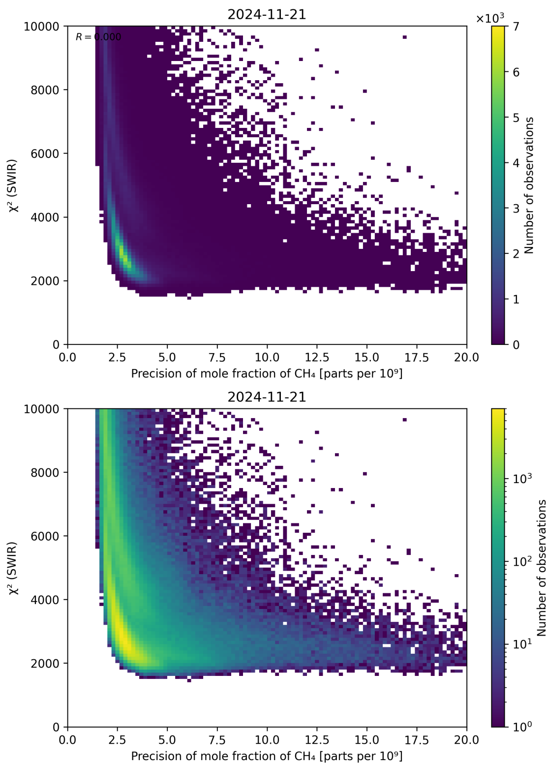
Figure 79: Scatter density plot of “Precision of mole fraction of \text{CH}_4 ” against “ \chi^2 (SWIR)” for 2024-11-20 to 2024-11-22.
