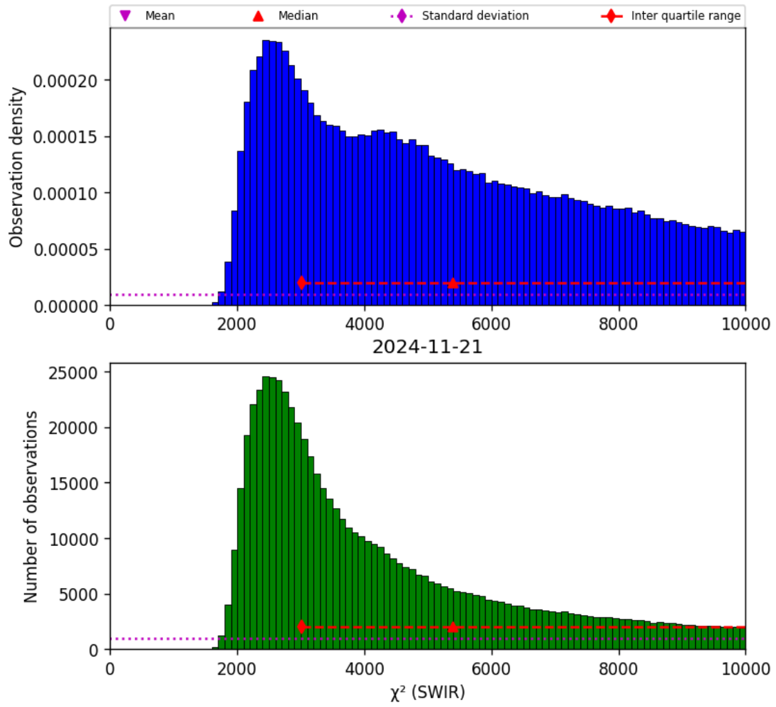
Figure 28: Histogram of " \chi^2 (SWIR)" for 2024-11-20 to 2024-11-22
