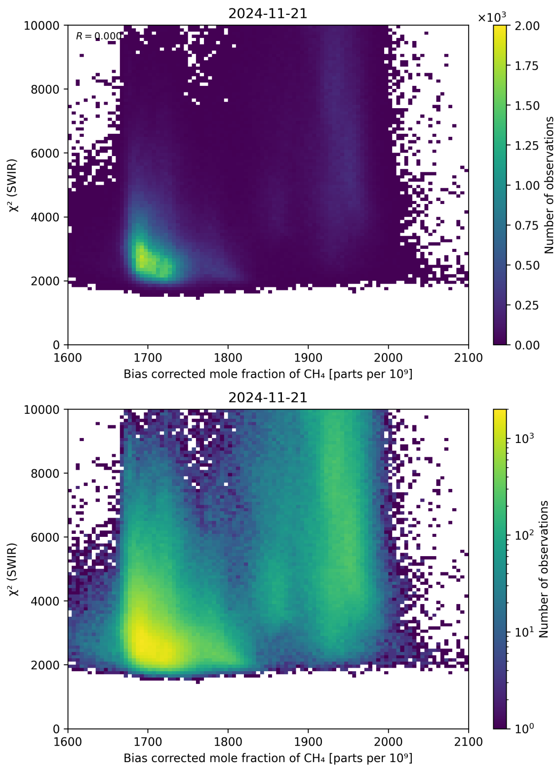
Figure 64: Scatter density plot of “Bias corrected mole fraction of \text{CH}_4 ” against “ \chi^2 (SWIR)” for 2024-11-20 to 2024-11-22.
