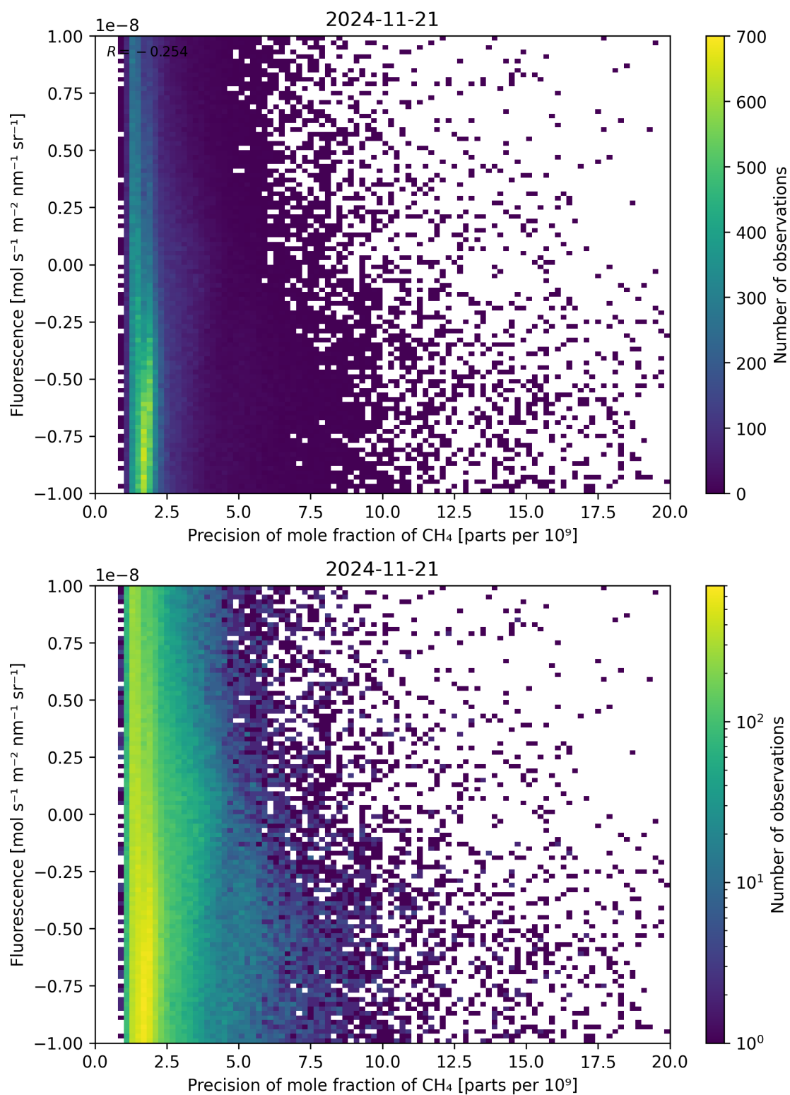
Figure 81: Scatter density plot of “Precision of mole fraction of \text{CH}_4 ” against “Fluorescence” for 2024-11-20 to 2024-11-22.
