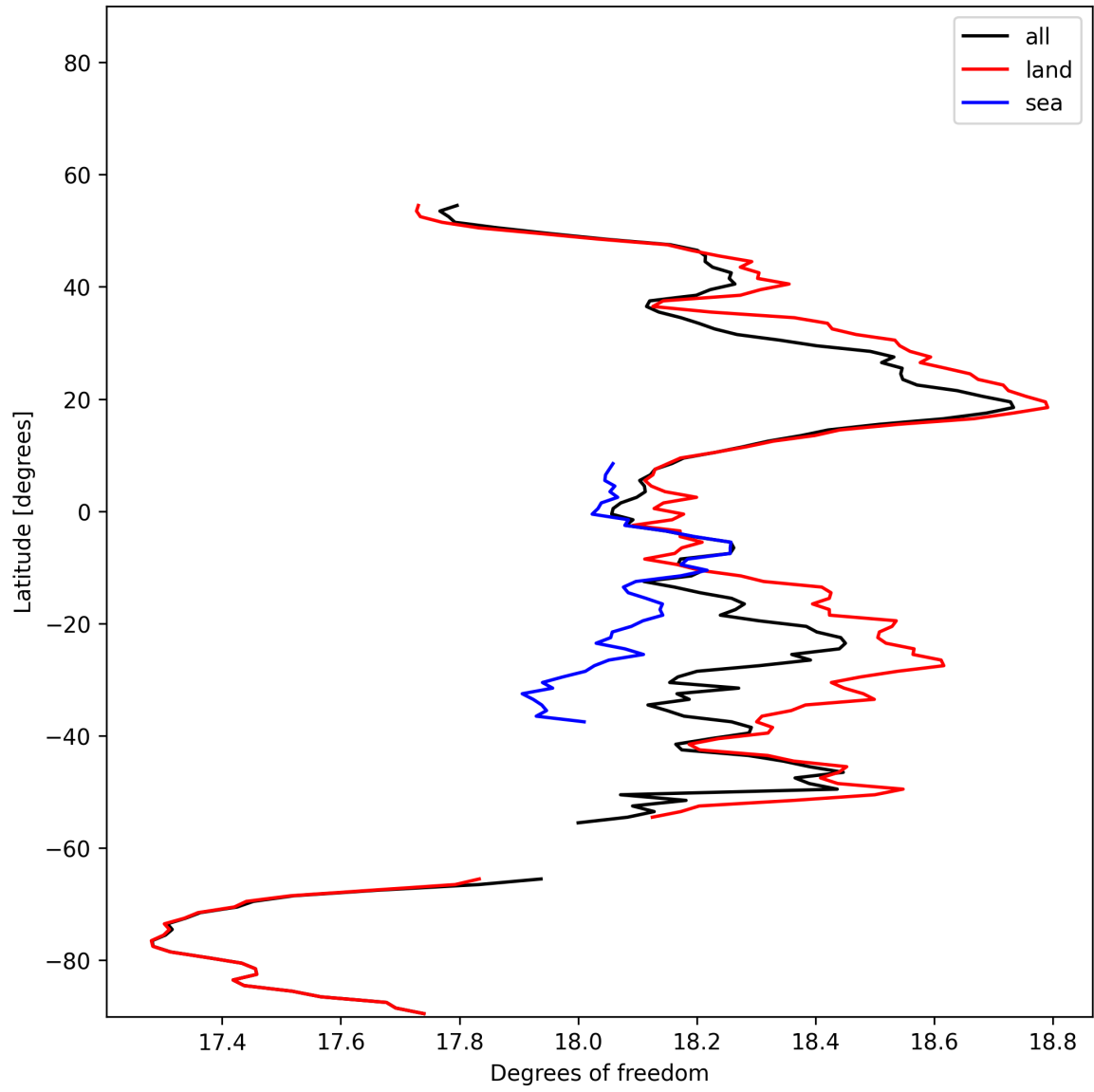
Figure 19: Zonal average of “Degrees of freedom” for 2024-11-20 to 2024-11-22.
