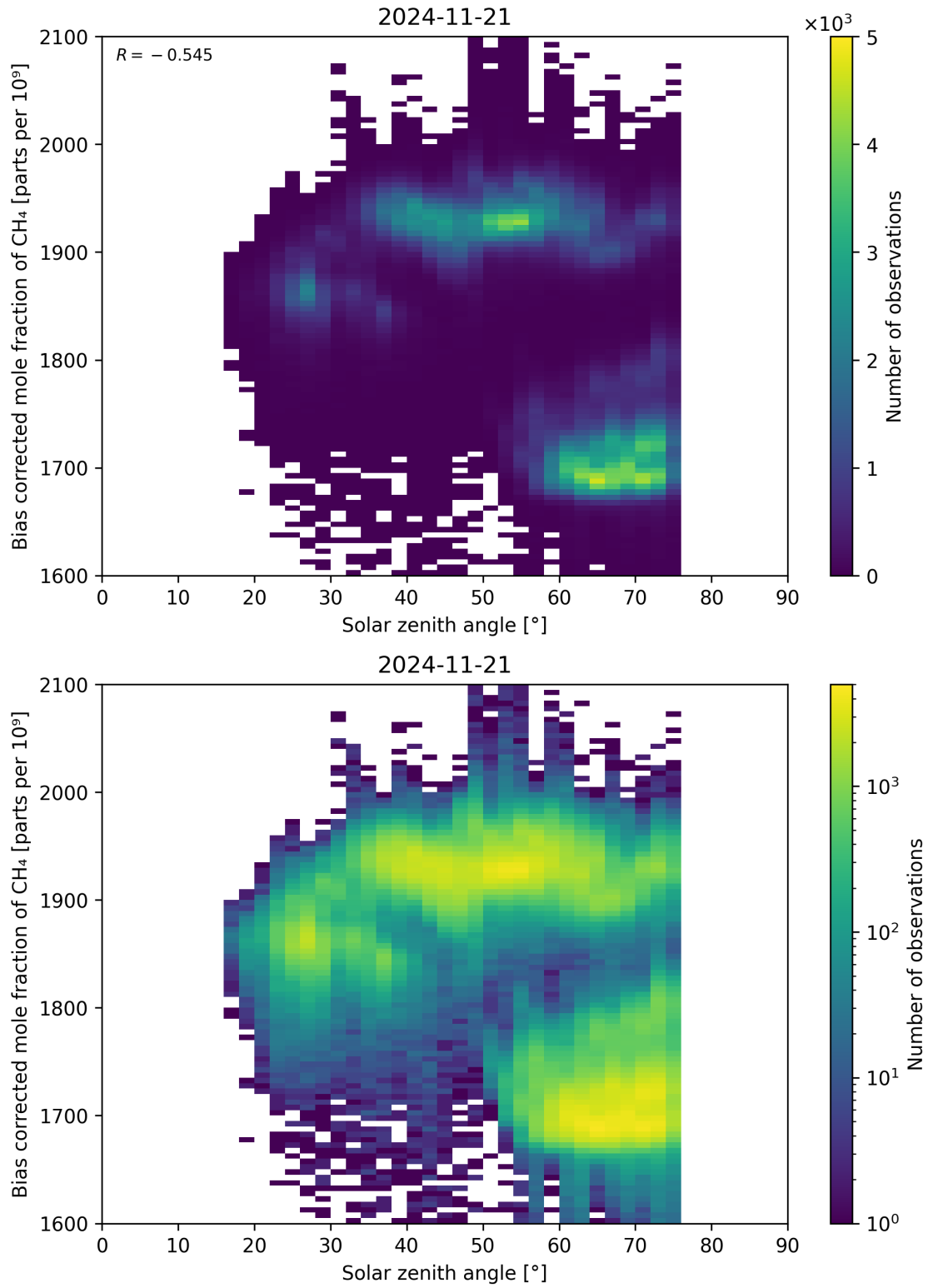
Figure 100: Scatter density plot of “Solar zenith angle” against “Bias corrected mole fraction of \text{CH}_4 ” for 2024-11-20 to 2024-11-22.
