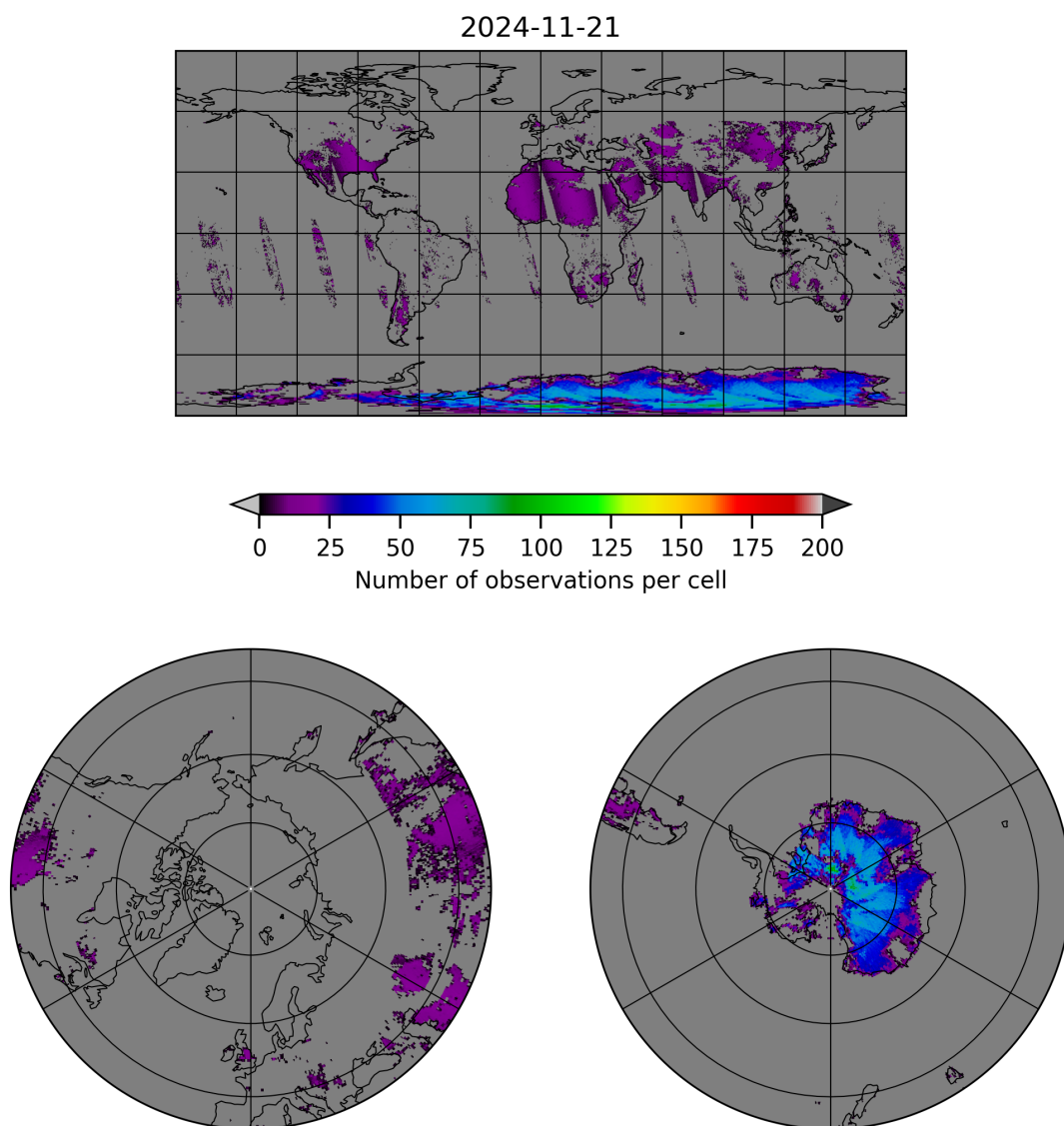
Figure 10: Map of the number of observations for 2024-11-20 to 2024-11-22
