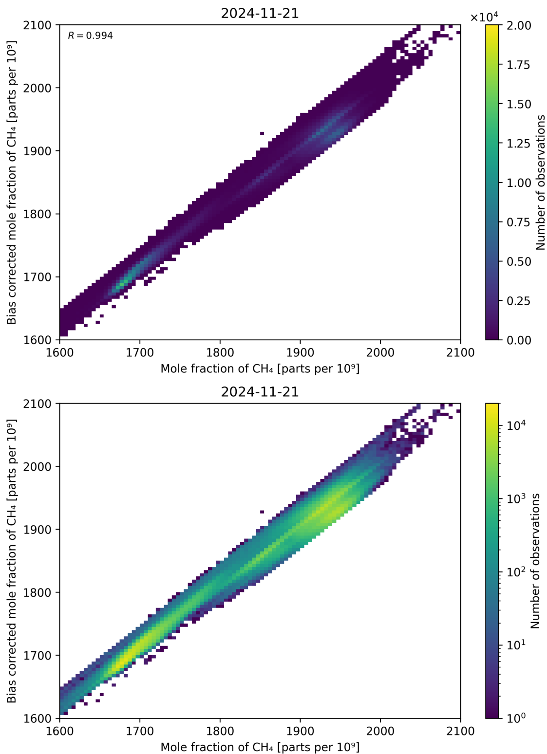
Figure 74: Scatter density plot of “Mole fraction of CH 4 ” against “Bias corrected mole fraction of CH 4 ” for 2024-11-20 to 2024-11-22.
