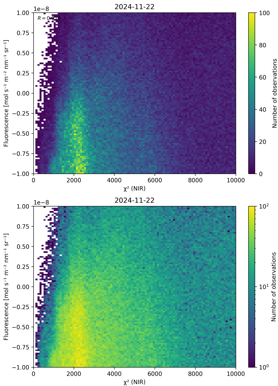
Figure 45: Scatter density plot of “ \chi^2 (NIR)” against “Fluorescence” for 2024-11-21 to 2024-11-23.
