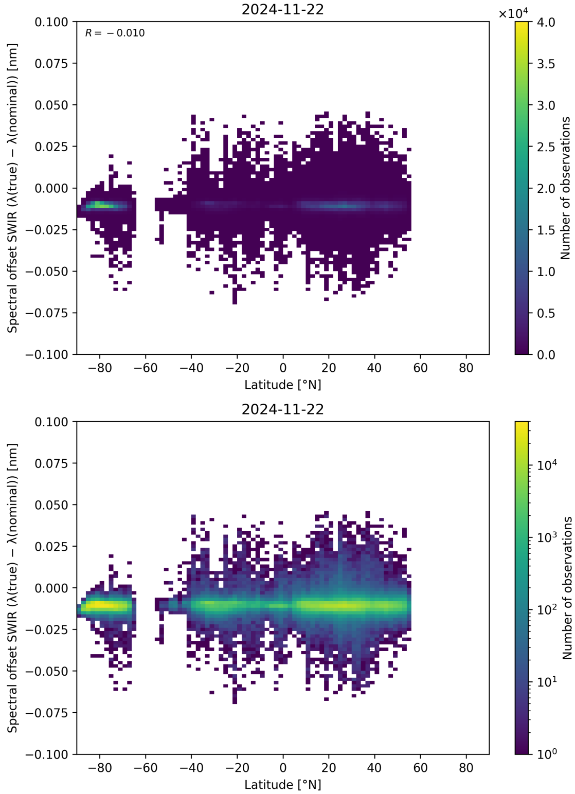
Figure 62: Scatter density plot of “Latitude” against “Spectral offset SWIR ( \lambda_{\text{true}} - \lambda_{\text{nominal}} )” for 2024-11-21 to 2024-11-23.
