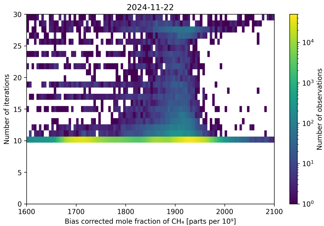
Figure 67: Scatter density plot of “Bias corrected mole fraction of \text{CH}_4 ” against “Number of iterations” for 2024-11-21 to 2024-11-23.
