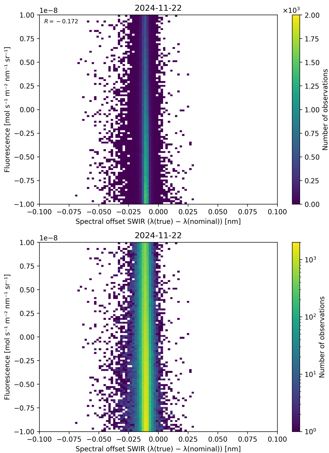
Figure 120: Scatter density plot of “Spectral offset SWIR ( \lambda_{\text{true}} - \lambda_{\text{nominal}} )” against “Fluorescence” for 2024-11-21 to 2024-11-23.
