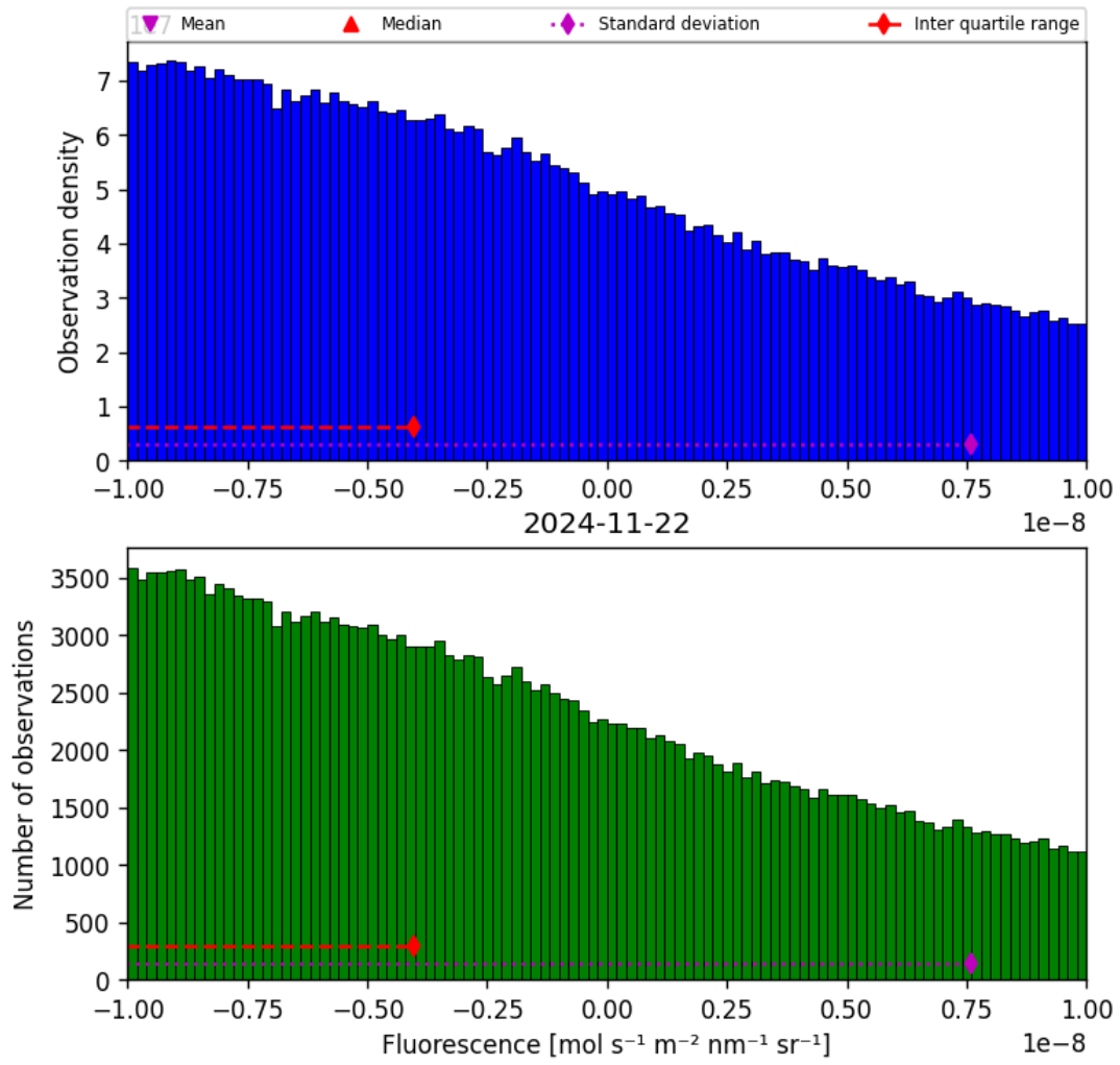
Figure 32: Histogram of “Fluorescence” for 2024-11-21 to 2024-11-23
