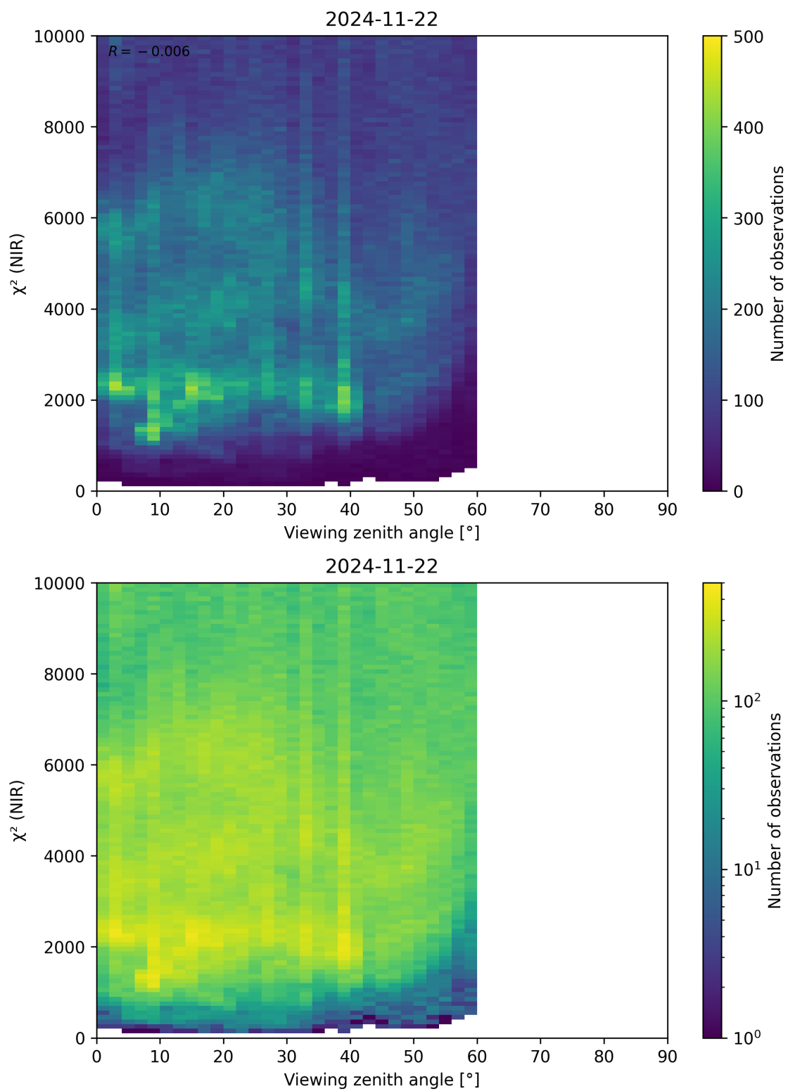
Figure 105: Scatter density plot of “Viewing zenith angle” against “ \chi^2 (NIR)” for 2024-11-21 to 2024-11-23.
