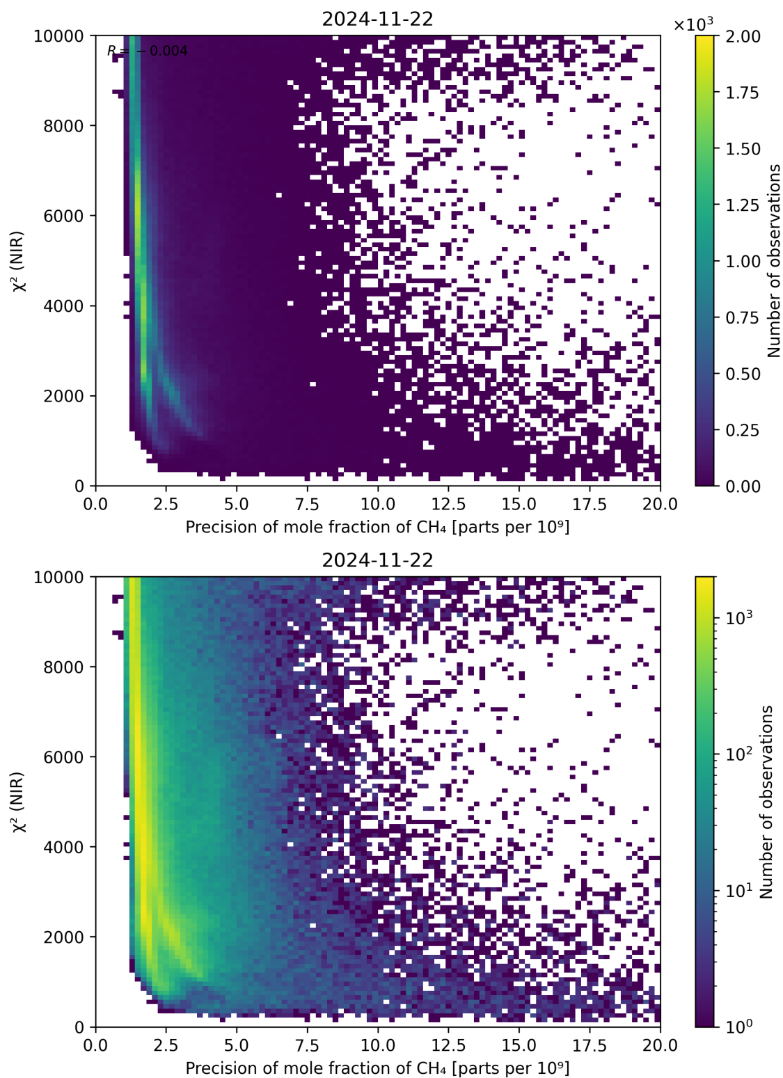
Figure 78: Scatter density plot of “Precision of mole fraction of CH 4 ” against “ \chi^2 (NIR)” for 2024-11-21 to 2024-11-23.
