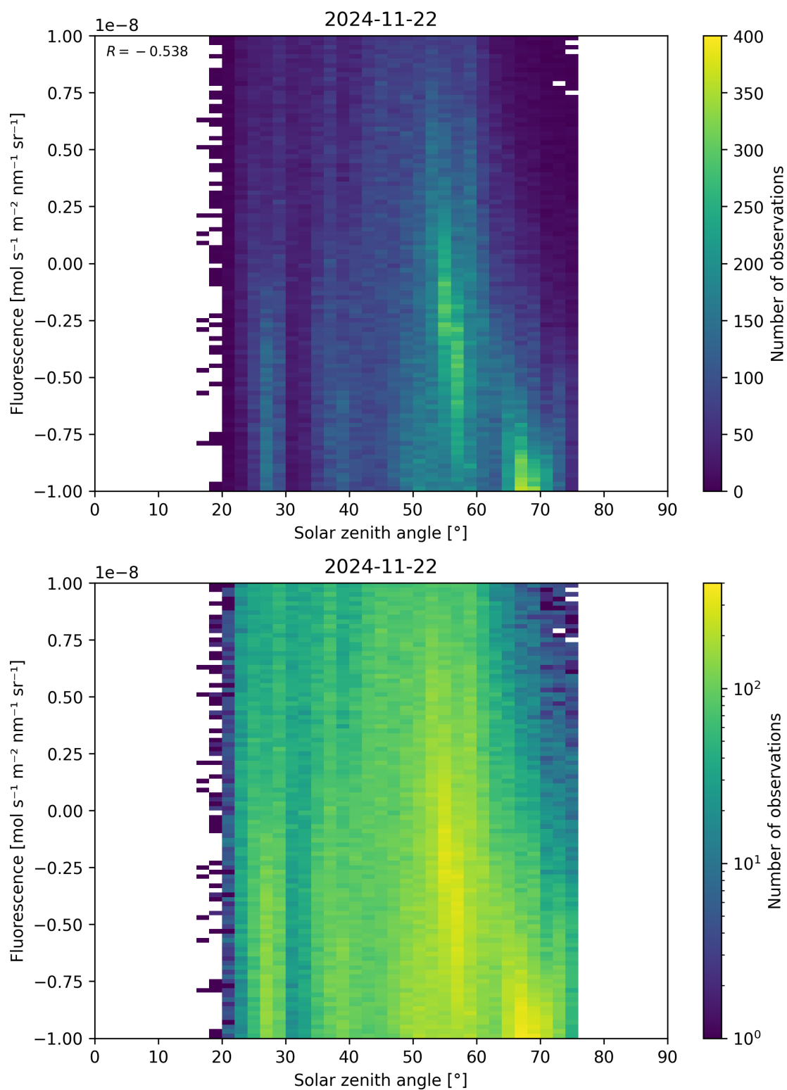
Figure 97: Scatter density plot of “Solar zenith angle” against “Fluorescence” for 2024-11-21 to 2024-11-23.
