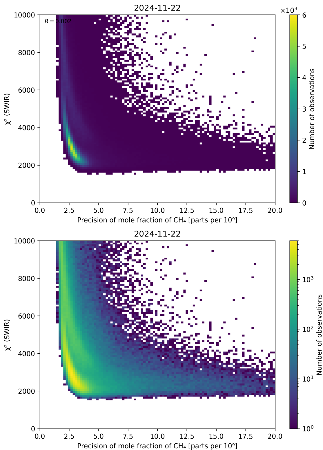
Figure 79: Scatter density plot of “Precision of mole fraction of \text{CH}_4 ” against “ \chi^2 (SWIR)” for 2024-11-21 to 2024-11-23.
