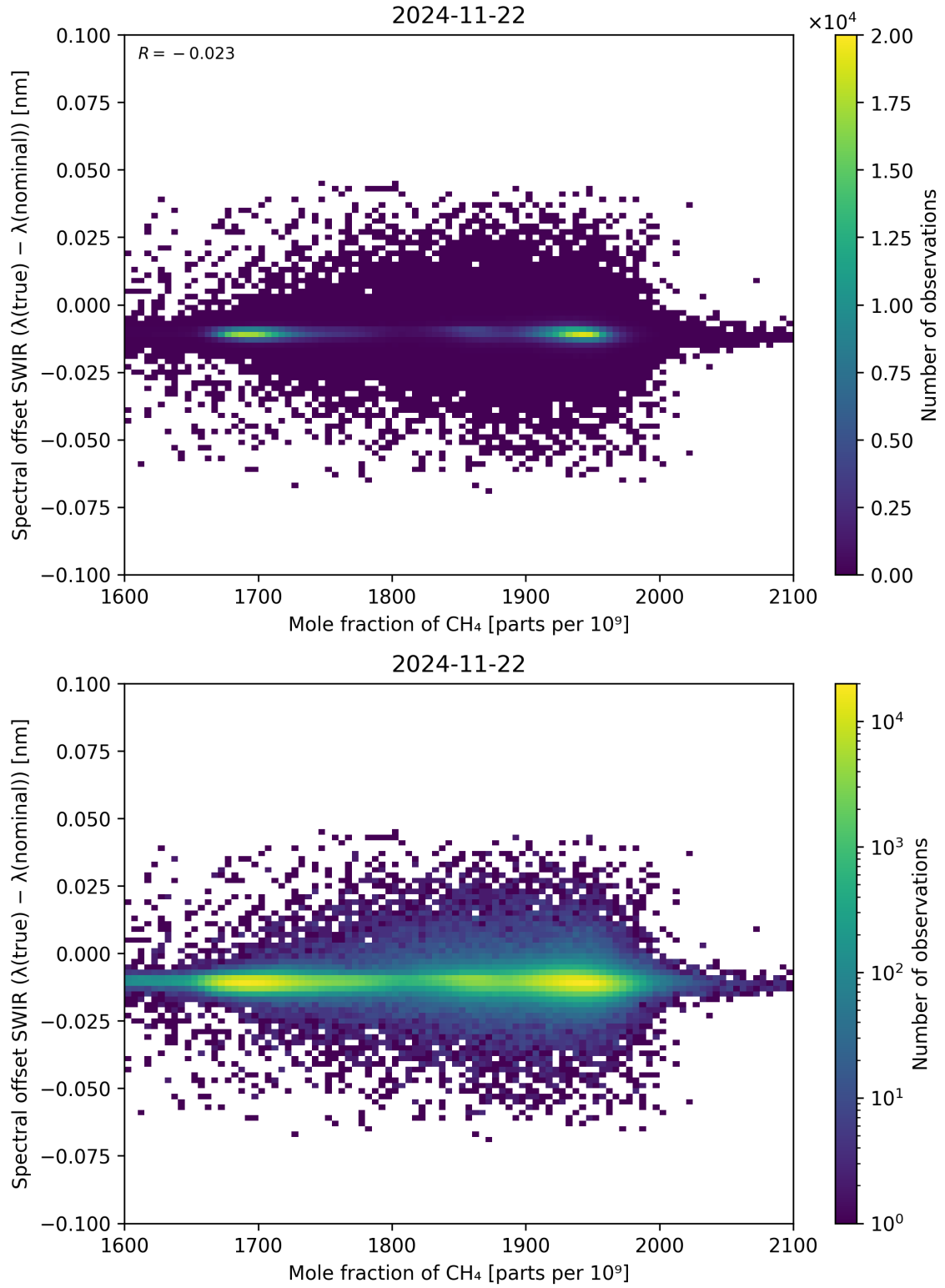
Figure 86: Scatter density plot of “Mole fraction of CH 4 ” against “Spectral offset SWIR ( \lambda_{\text{true}} - \lambda_{\text{nominal}} )” for 2024-11-21 to 2024-11-23.
