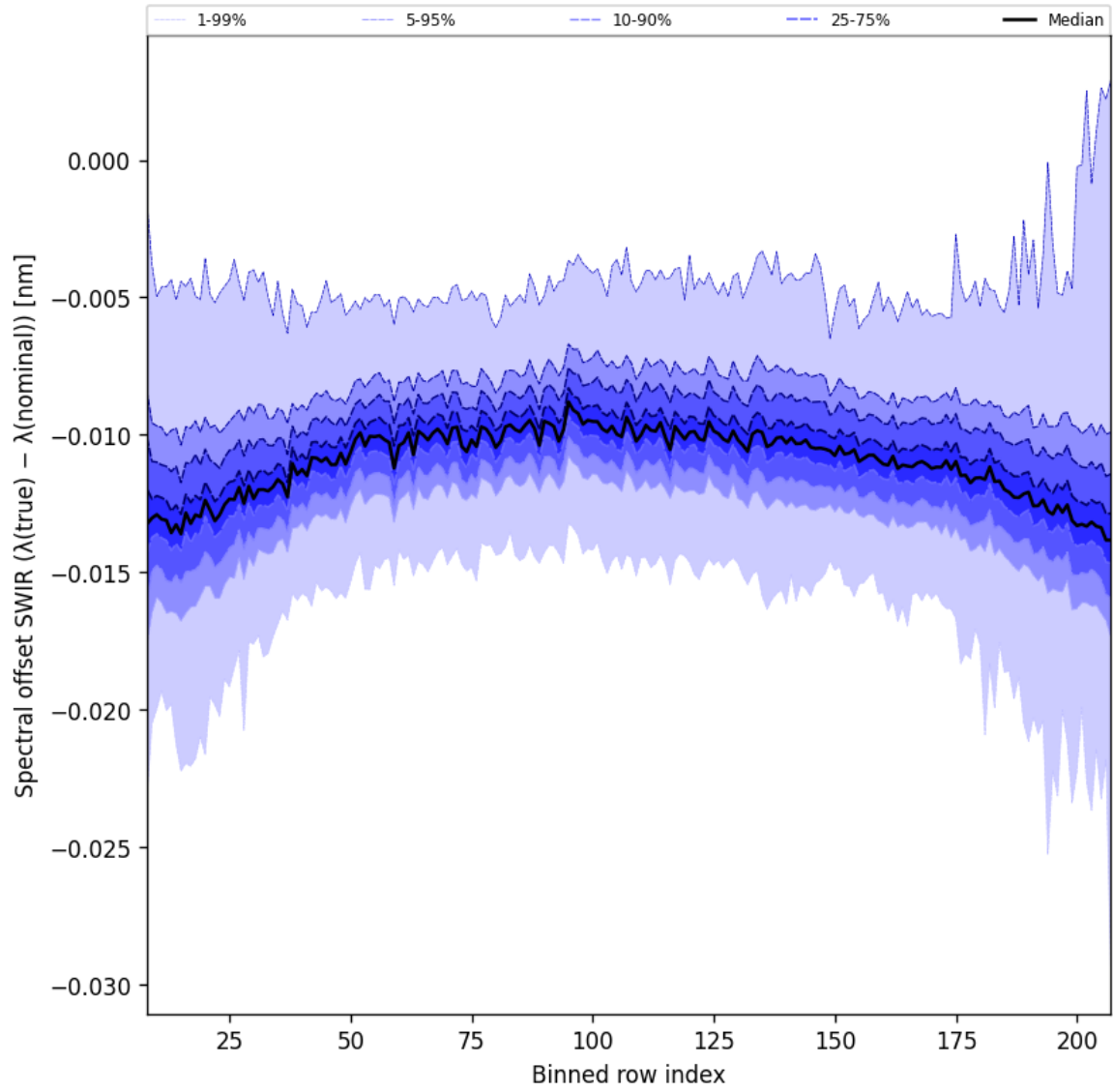
Figure 38: Along track statistics of “Spectral offset SWIR ( \lambda_{\text{true}} - \lambda_{\text{nominal}} )” for 2024-11-21 to 2024-11-23
