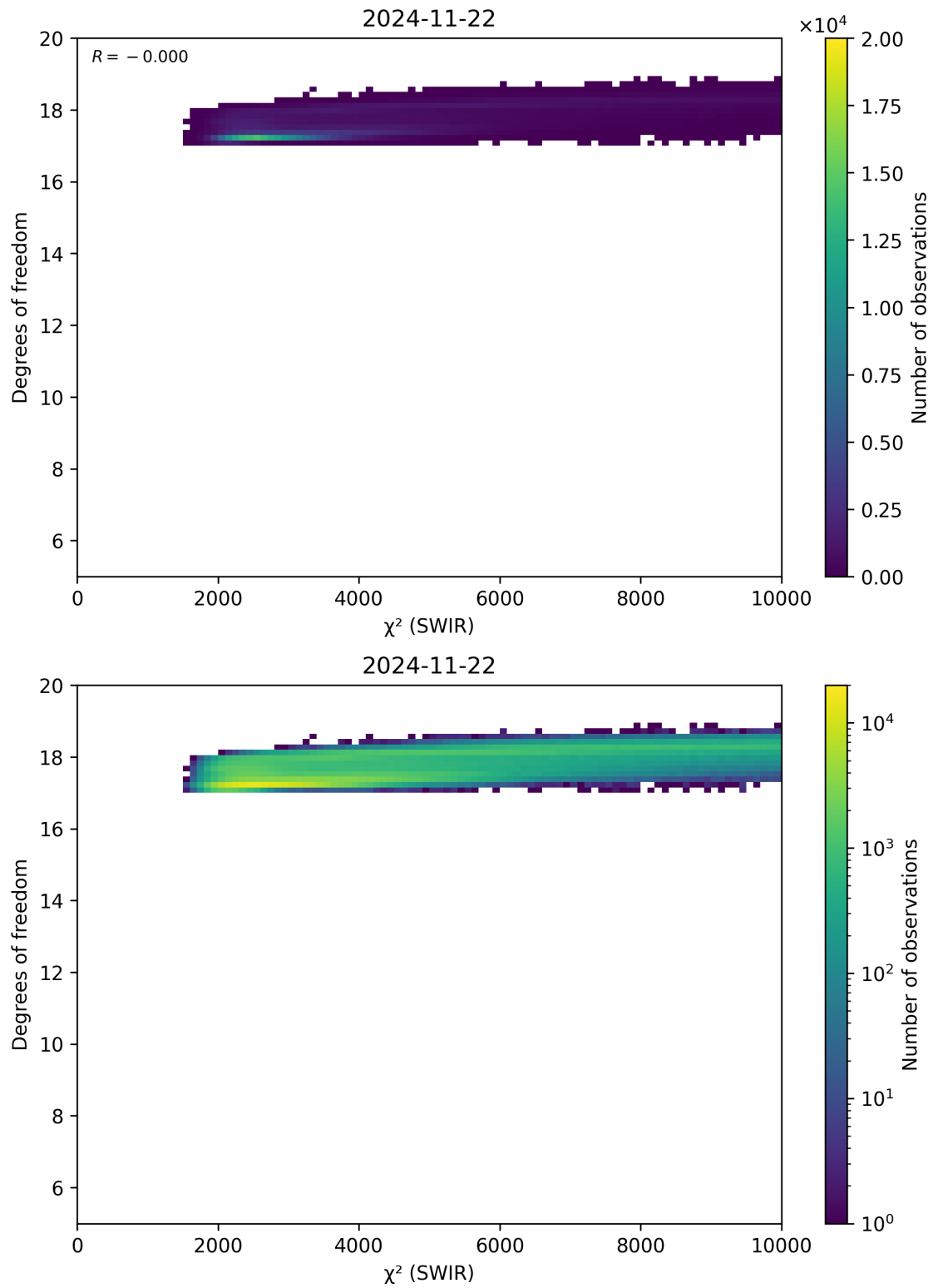
Figure 48: Scatter density plot of “ \chi^2 (SWIR)” against “Degrees of freedom” for 2024-11-21 to 2024-11-23.
