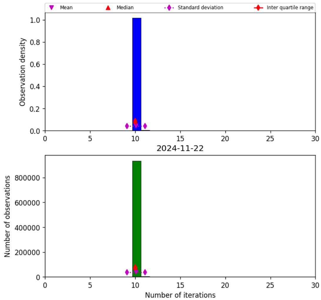
Figure 31: Histogram of “Number of iterations” for 2024-11-21 to 2024-11-23
