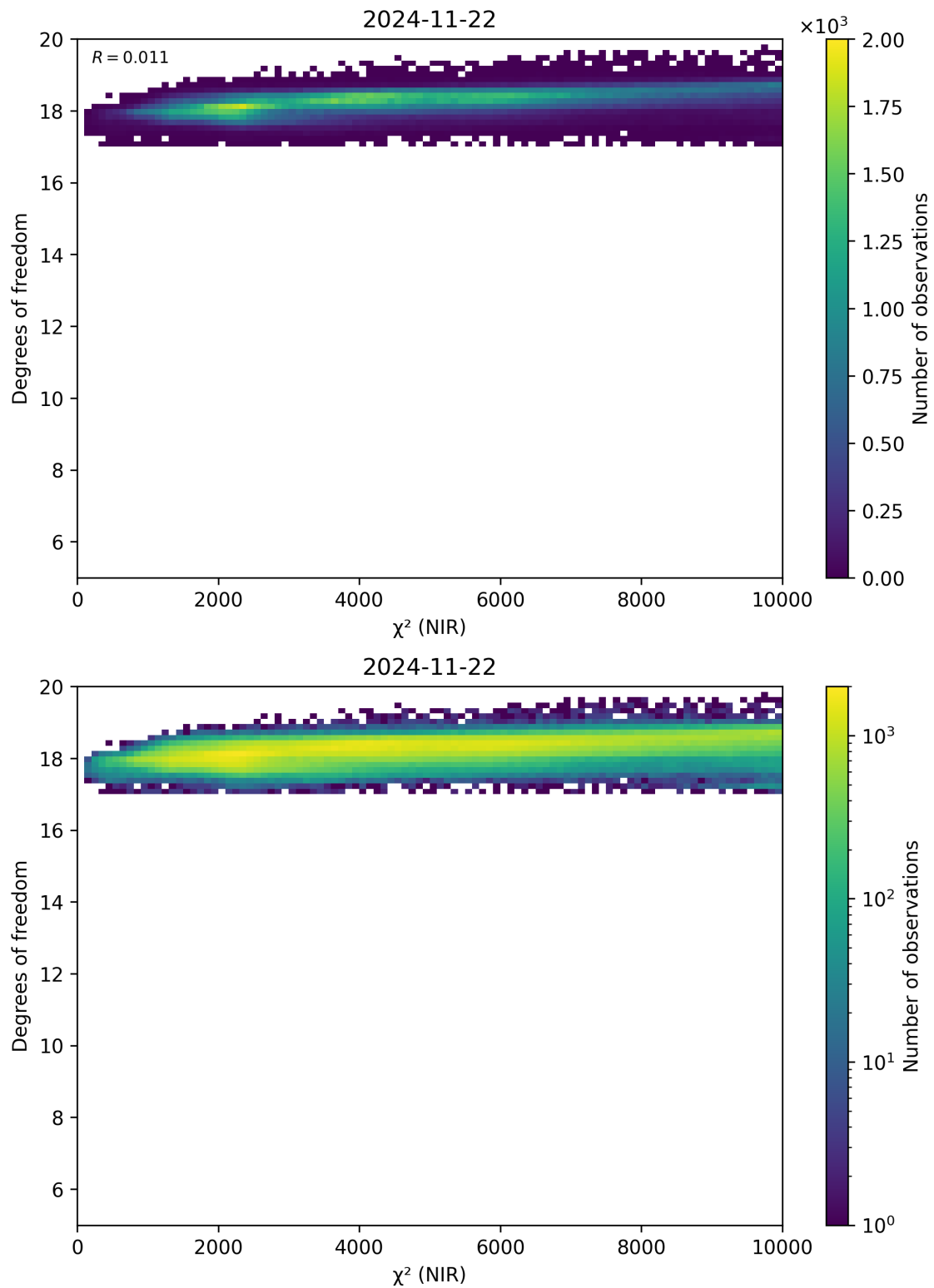
Figure 44: Scatter density plot of “ \chi^2 (NIR)” against “Degrees of freedom” for 2024-11-21 to 2024-11-23.
