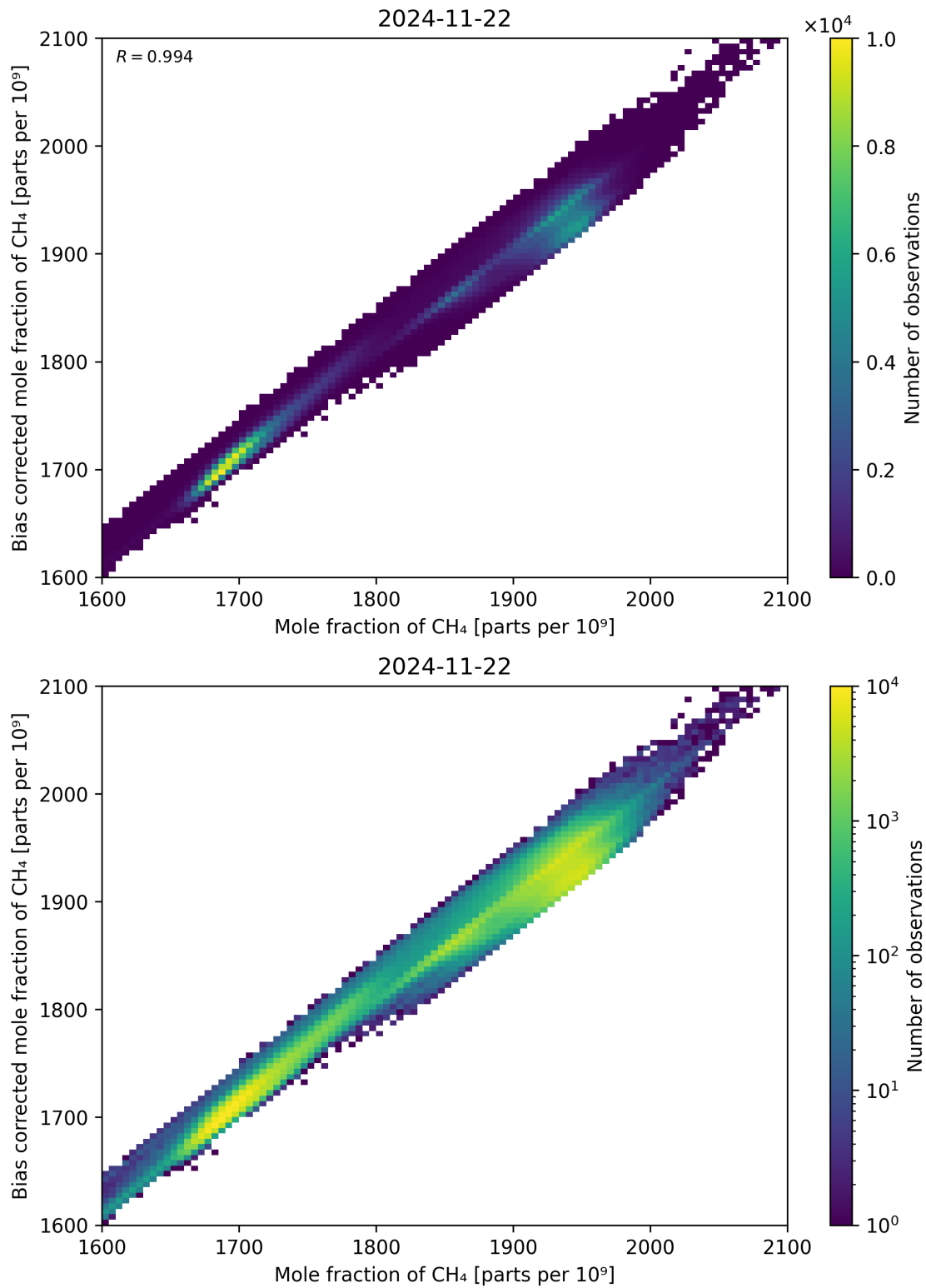
Figure 74: Scatter density plot of “Mole fraction of CH 4 ” against “Bias corrected mole fraction of CH 4 ” for 2024-11-21 to 2024-11-23.
