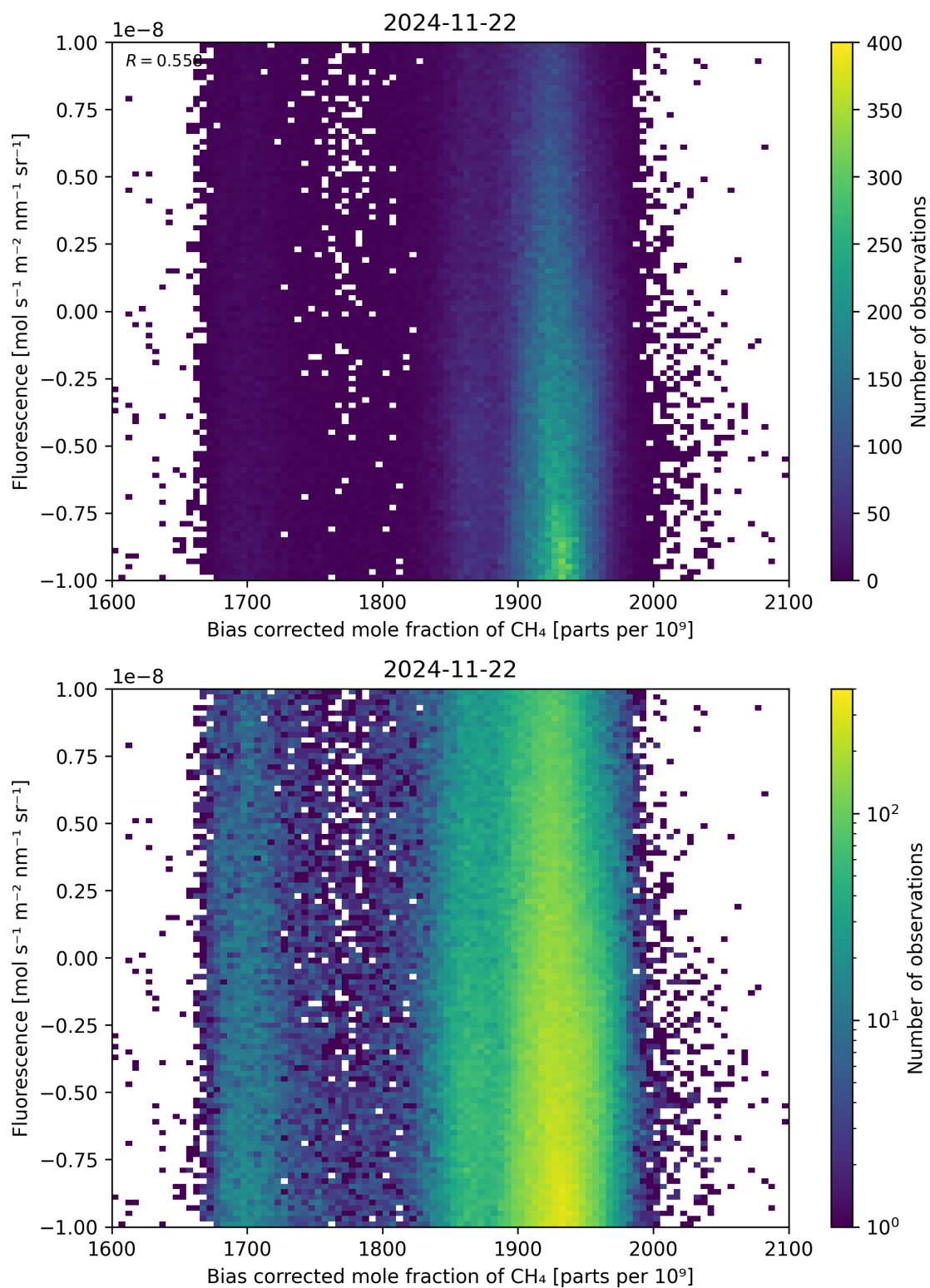
Figure 66: Scatter density plot of “Bias corrected mole fraction of CH 4 ” against “Fluorescence” for 2024-11-21 to 2024-11-23.
