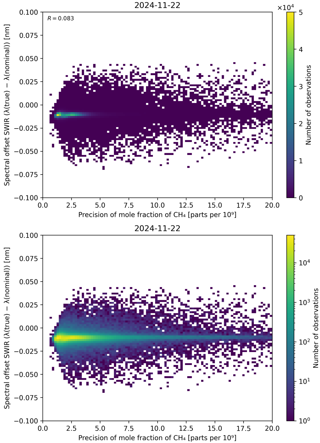
Figure 85: Scatter density plot of “Precision of mole fraction of CH 4 ” against “Spectral offset SWIR ( \lambda_{\text{true}} - \lambda_{\text{nominal}} )” for 2024-11-21 to 2024-11-23.
