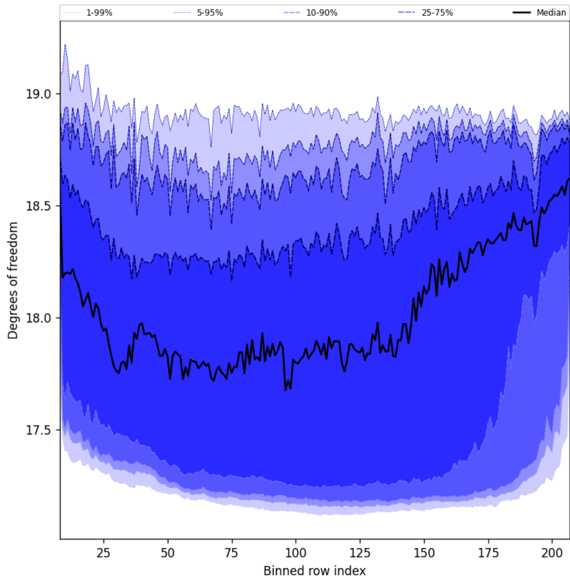
Figure 41: Along track statistics of “Degrees of freedom” for 2024-11-21 to 2024-11-23
