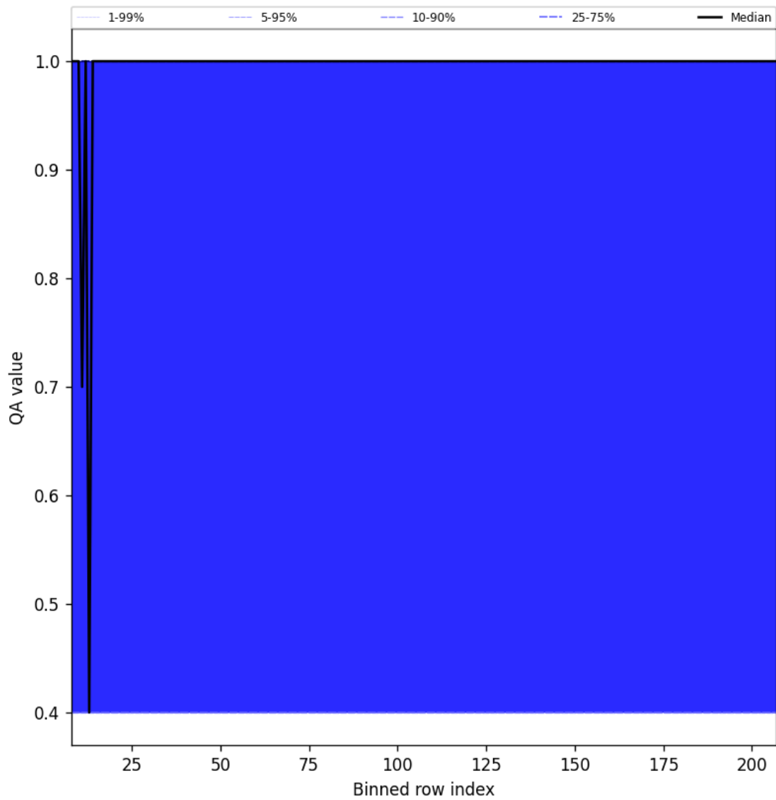
Figure 33: Along track statistics of “QA value” for 2024-11-21 to 2024-11-23
