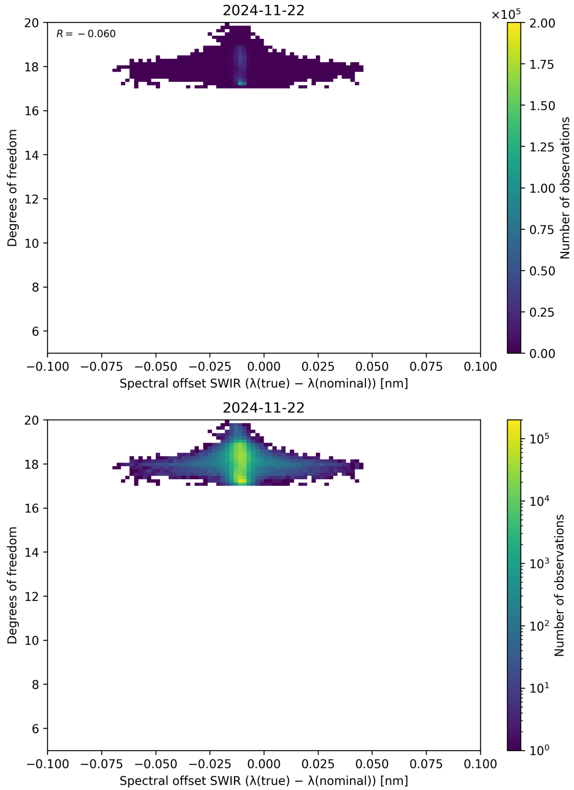
Figure 119: Scatter density plot of “Spectral offset SWIR ( \lambda_{\text{true}} - \lambda_{\text{nominal}} )” against “Degrees of freedom” for 2024-11-21 to 2024-11-23.
