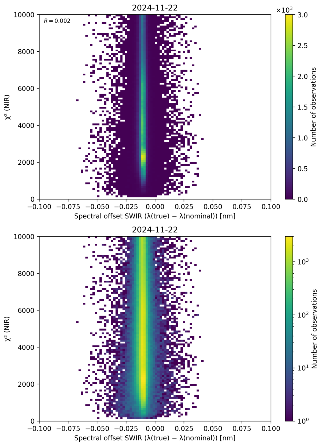
Figure 117: Scatter density plot of “Spectral offset SWIR ( \lambda_{\text{true}} - \lambda_{\text{nominal}} )” against “ \chi^2 (NIR)” for 2024-11-21 to 2024-11-23.
