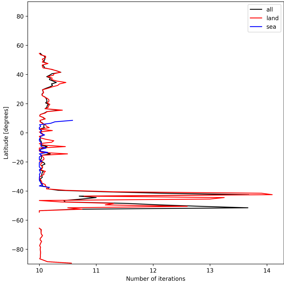
Figure 20: Zonal average of “Number of iterations” for 2024-11-21 to 2024-11-23.
