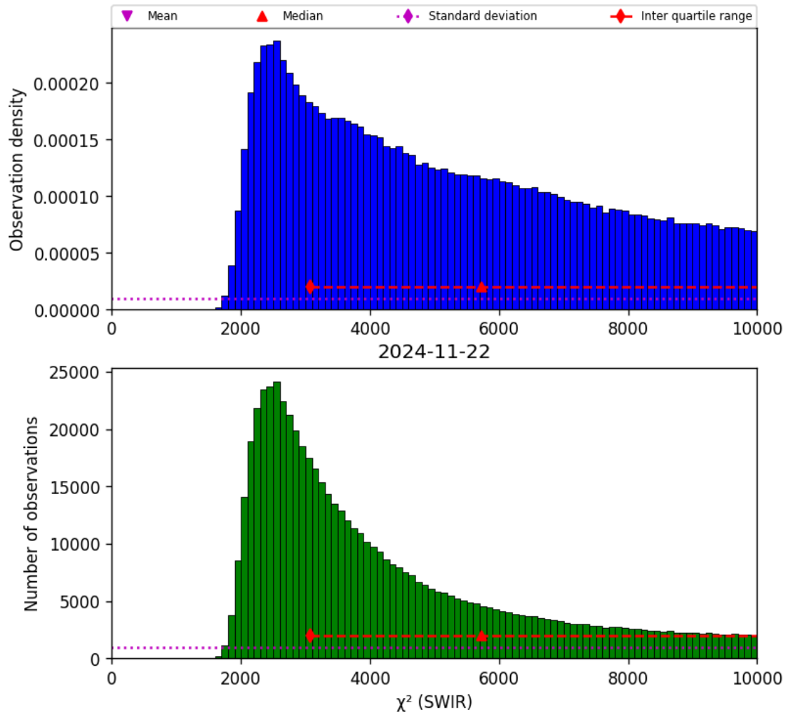
Figure 28: Histogram of “ \chi^2 (SWIR)” for 2024-11-21 to 2024-11-23
