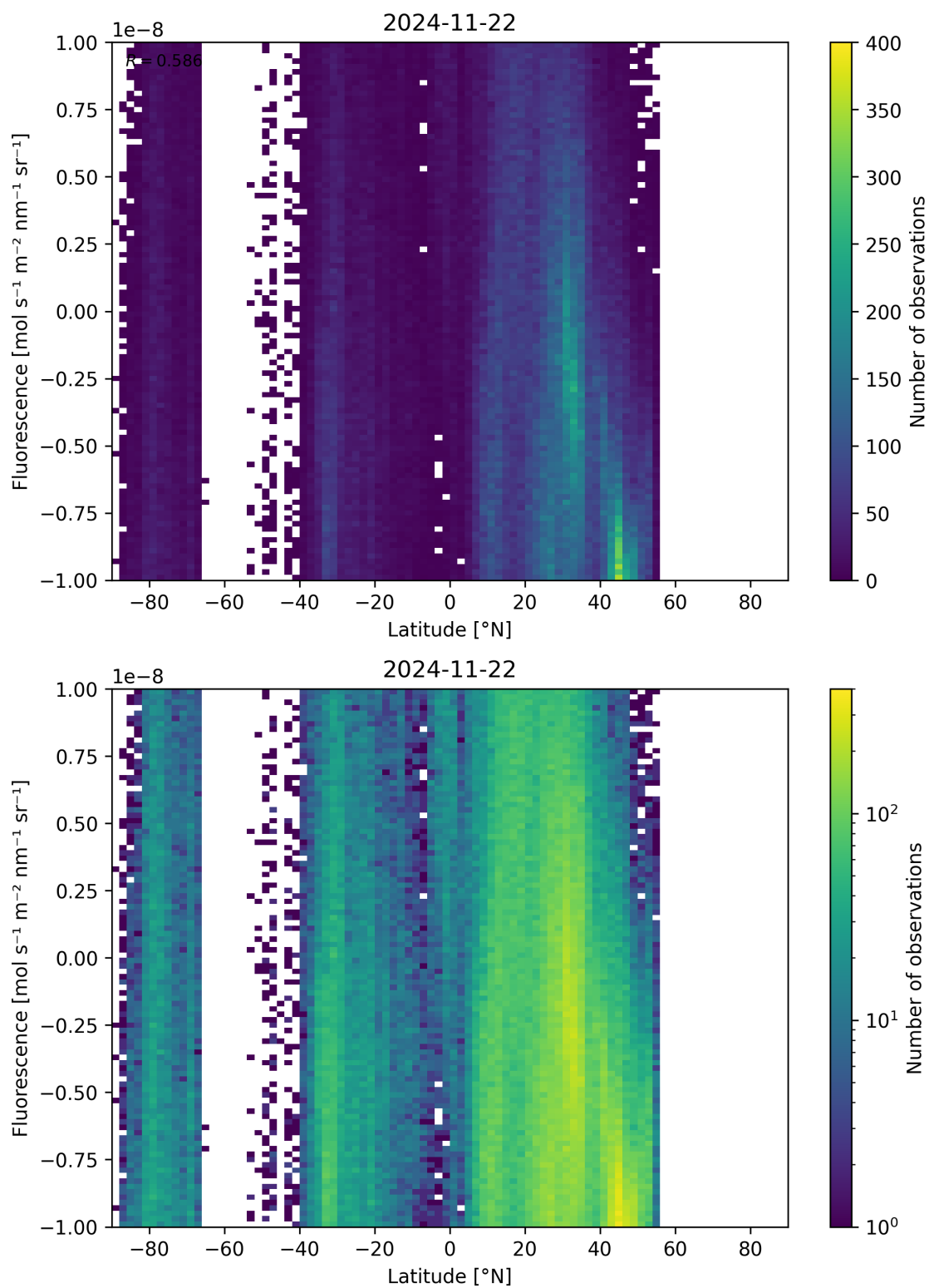
Figure 56: Scatter density plot of “Latitude” against “Fluorescence” for 2024-11-21 to 2024-11-23.
