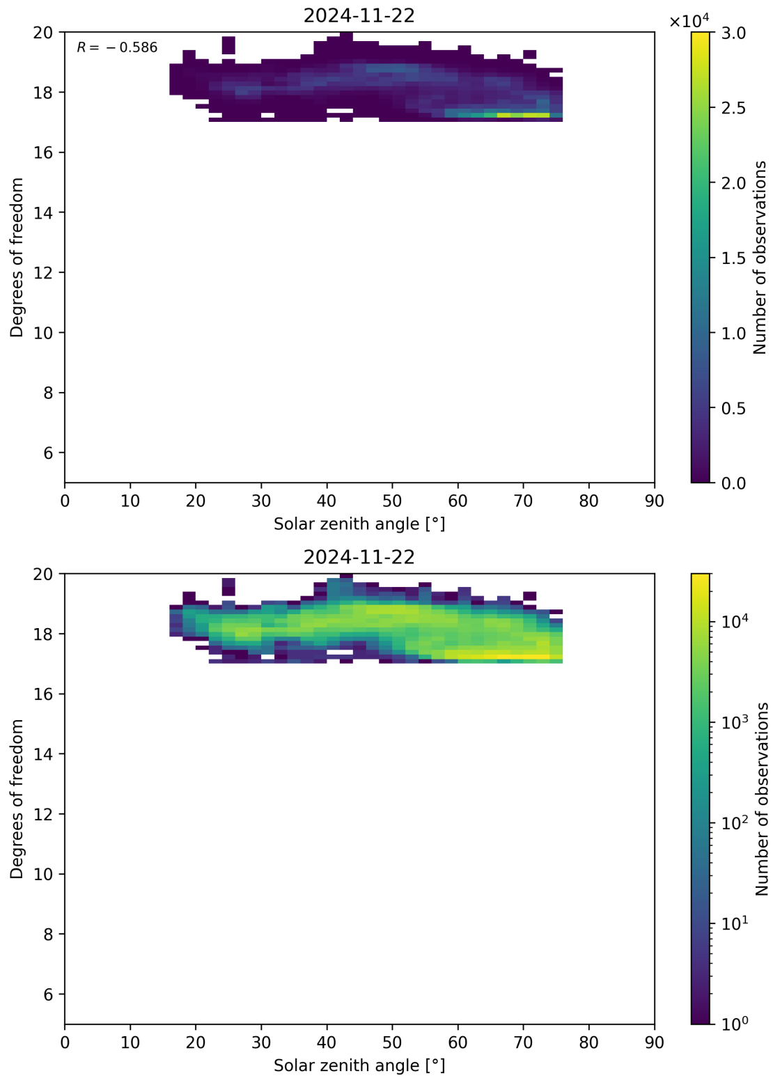
Figure 96: Scatter density plot of “Solar zenith angle” against “Degrees of freedom” for 2024-11-21 to 2024-11-23.
