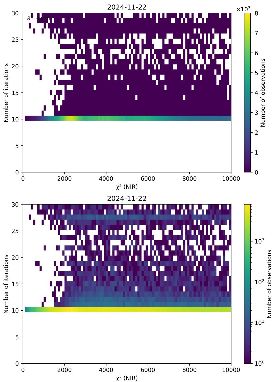
Figure 46: Scatter density plot of “ \chi^2 (NIR)” against “Number of iterations” for 2024-11-21 to 2024-11-23.
