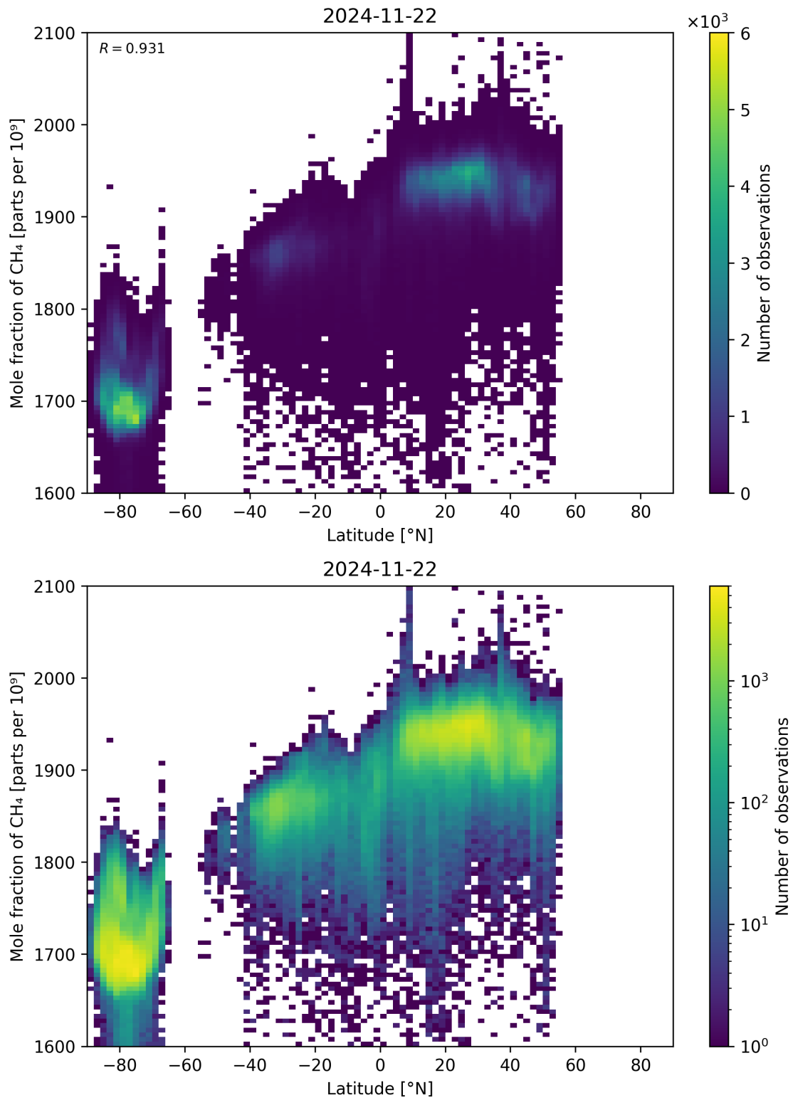
Figure 57: Scatter density plot of “Latitude” against “Mole fraction of \text{CH}_4 ” for 2024-11-21 to 2024-11-23.
