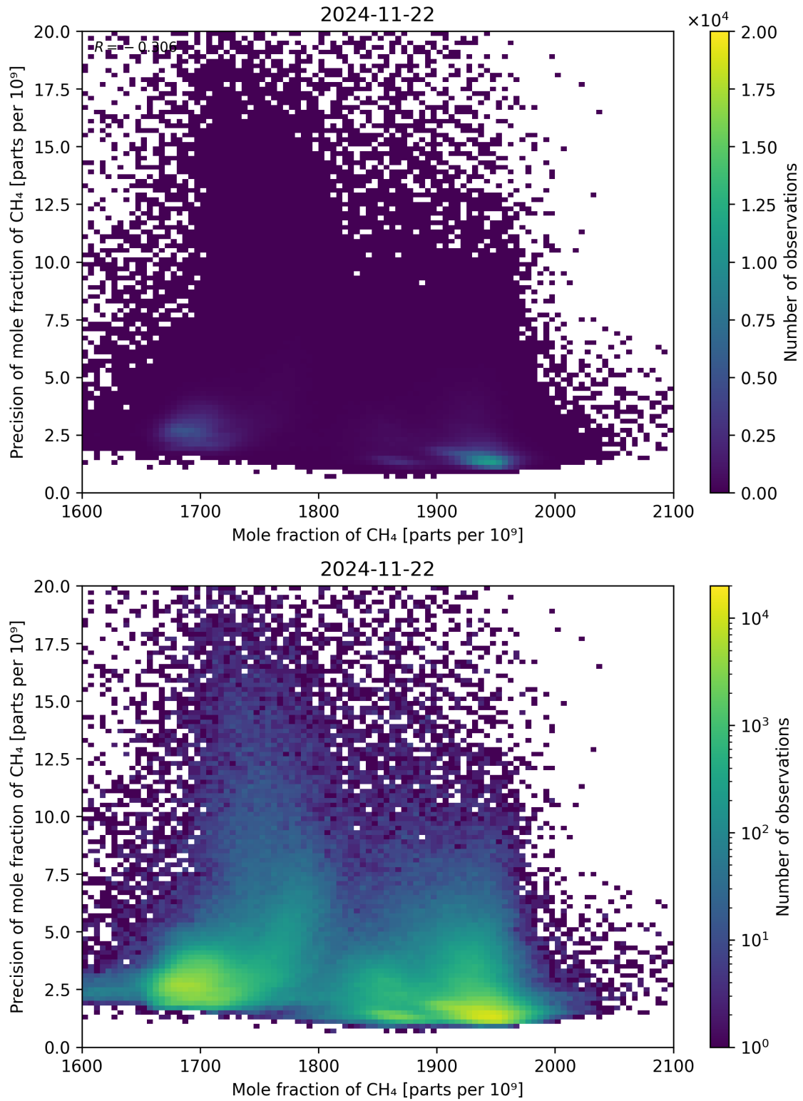
Figure 75: Scatter density plot of “Mole fraction of CH 4 ” against “Precision of mole fraction of CH 4 ” for 2024-11-21 to 2024-11-23.
