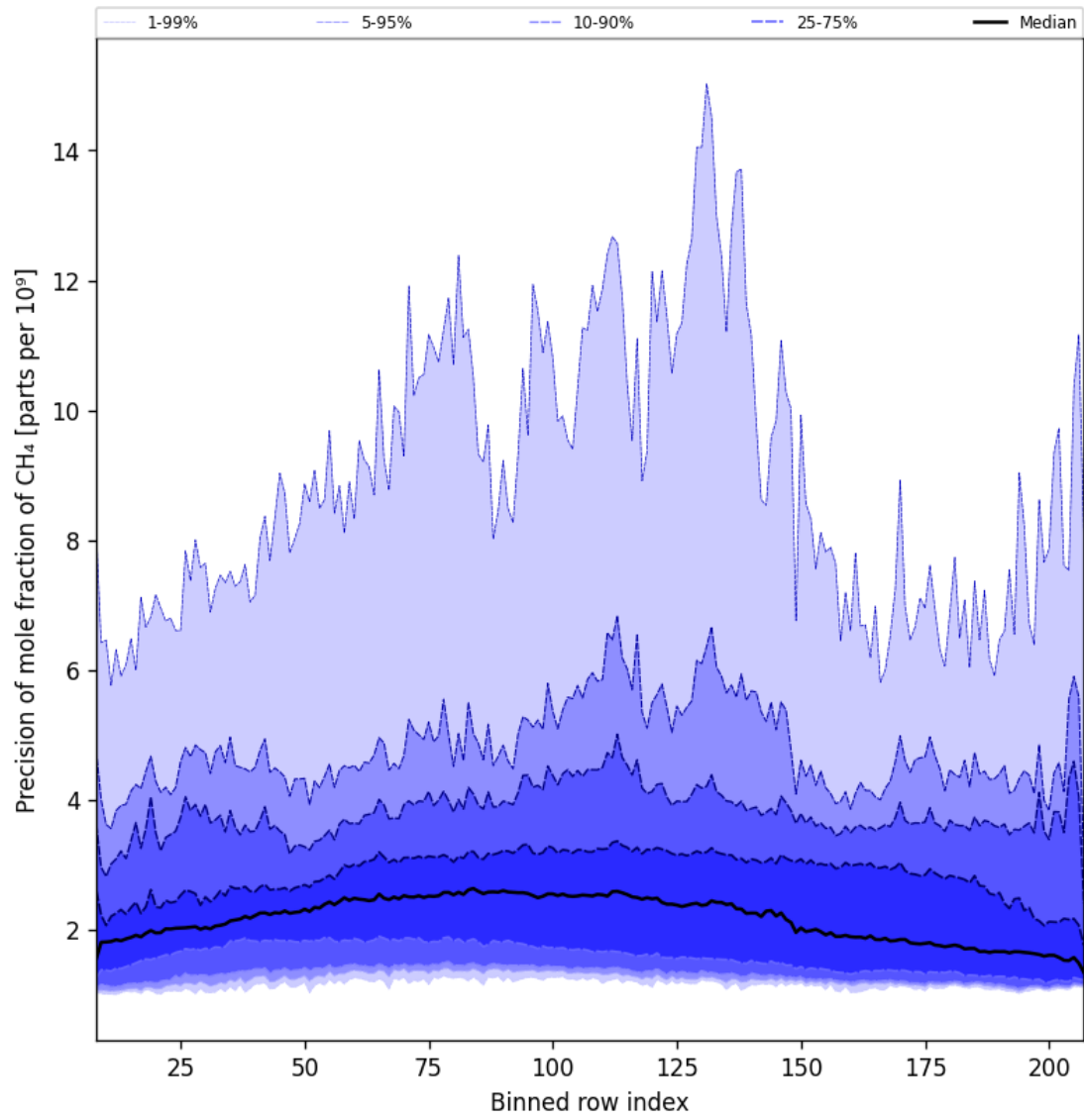
Figure 35: Along track statistics of “Precision of mole fraction of CH 4 ” for 2024-11-21 to 2024-11-23
