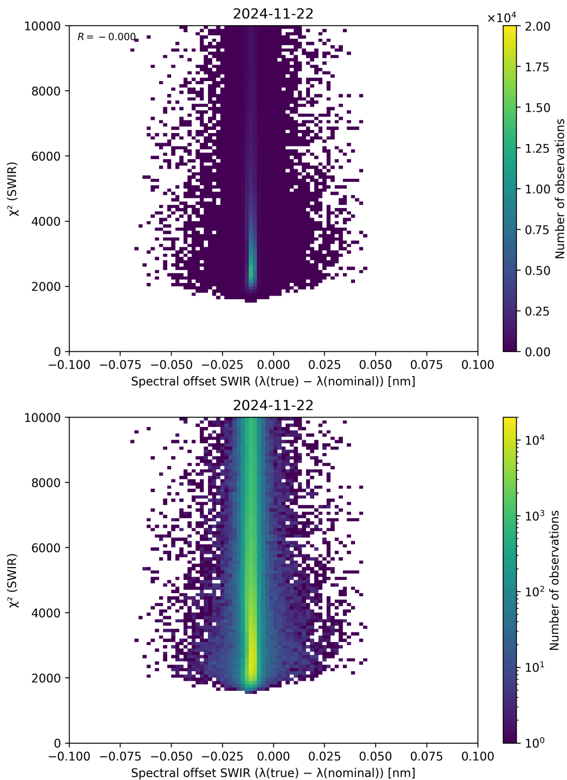
Figure 118: Scatter density plot of “Spectral offset SWIR ( \lambda_{\text{true}} - \lambda_{\text{nominal}} )” against “ \chi^2 (SWIR)” for 2024-11-21 to 2024-11-23.
