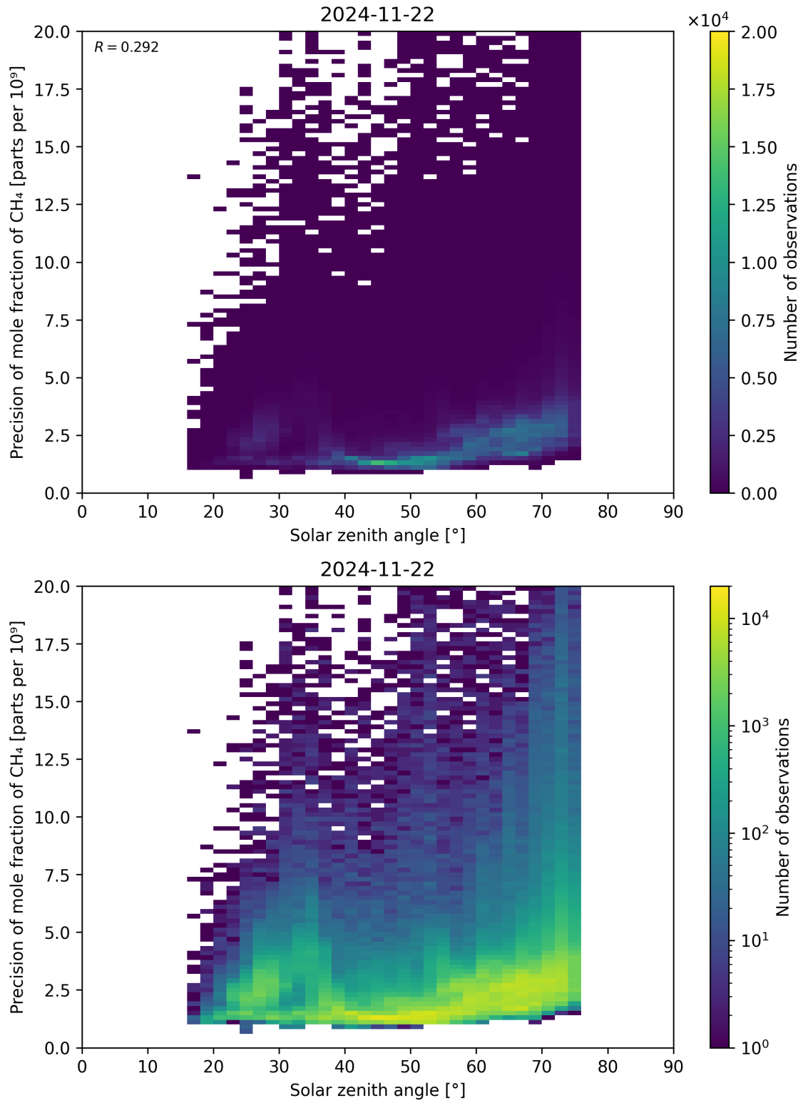
Figure 101: Scatter density plot of “Solar zenith angle” against “Precision of mole fraction of \text{CH}_4 ” for 2024-11-21 to 2024-11-23.
