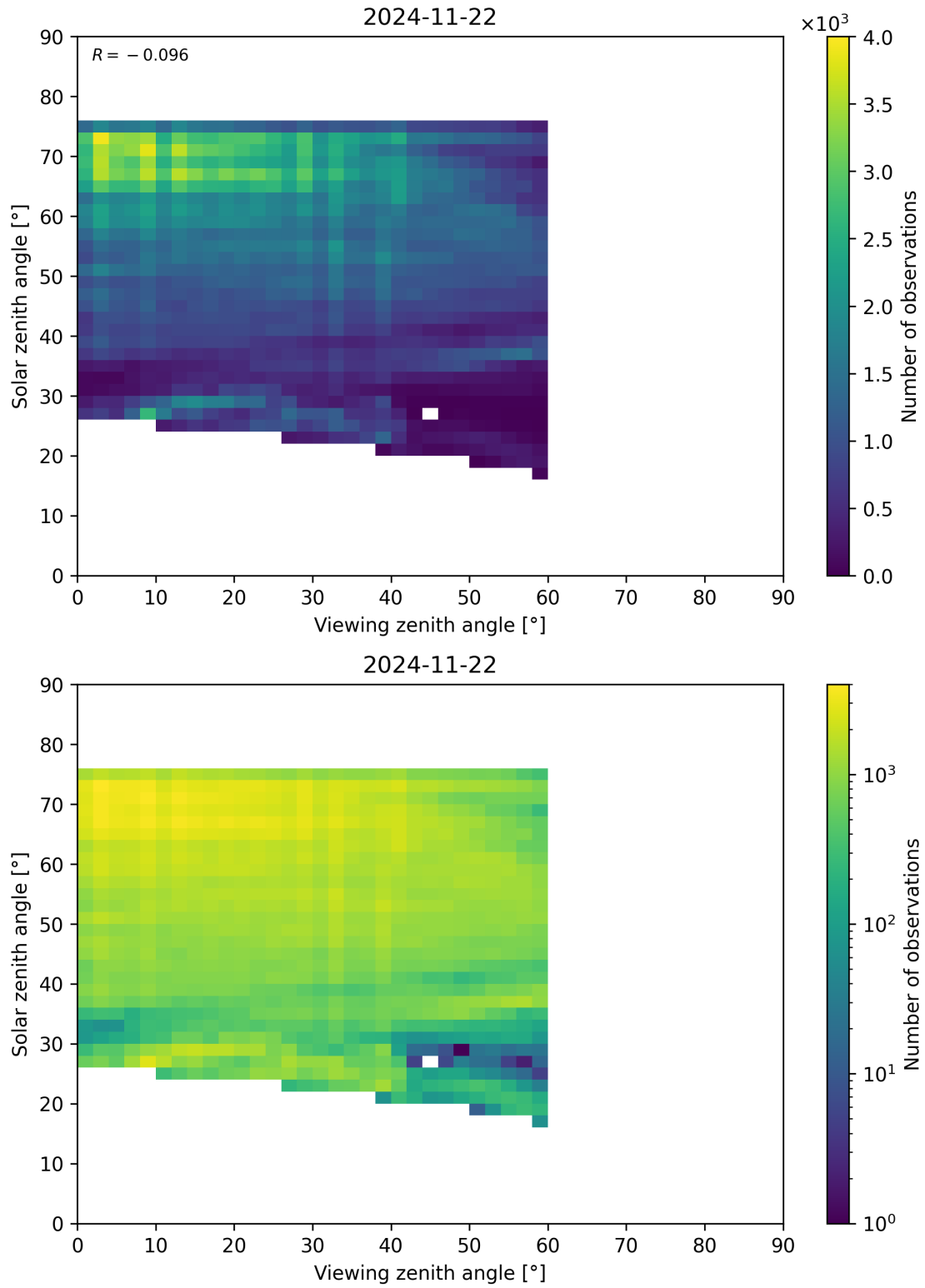
Figure 115: Scatter density plot of “Viewing zenith angle” against “Solar zenith angle” for 2024-11-21 to 2024-11-23.
