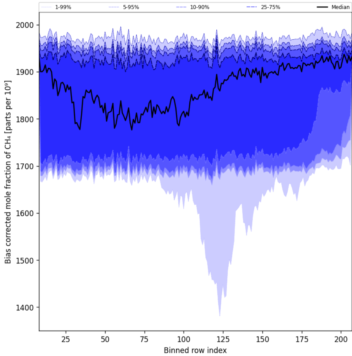
Figure 36: Along track statistics of “Bias corrected mole fraction of CH 4 ” for 2024-11-21 to 2024-11-23
