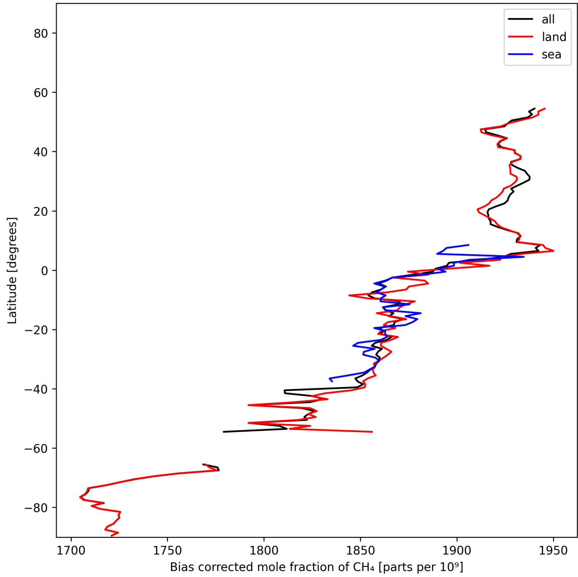
Figure 14: Zonal average of “Bias corrected mole fraction of CH 4 ” for 2024-11-21 to 2024-11-23.
