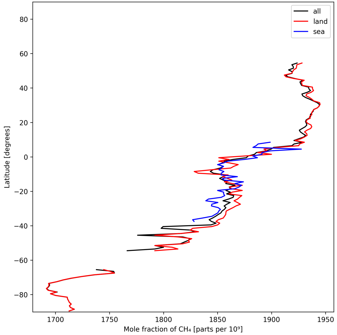
Figure 12: Zonal average of “Mole fraction of CH 4 ” for 2024-11-21 to 2024-11-23.
