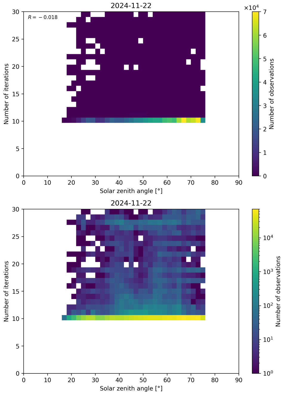
Figure 102: Scatter density plot of “Solar zenith angle” against “Number of iterations” for 2024-11-21 to 2024-11-23.
