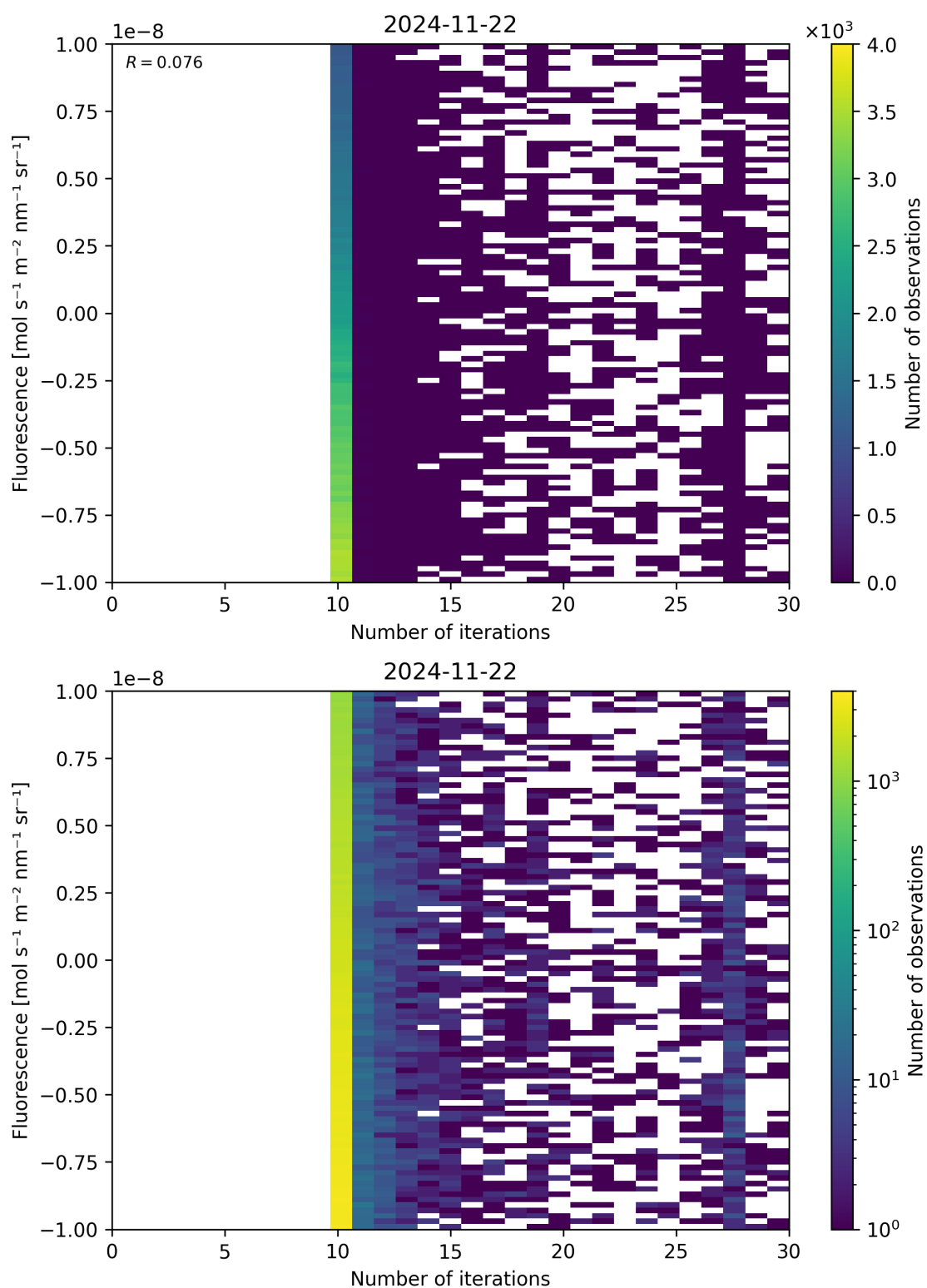
Figure 87: Scatter density plot of “Number of iterations” against “Fluorescence” for 2024-11-21 to 2024-11-23.
