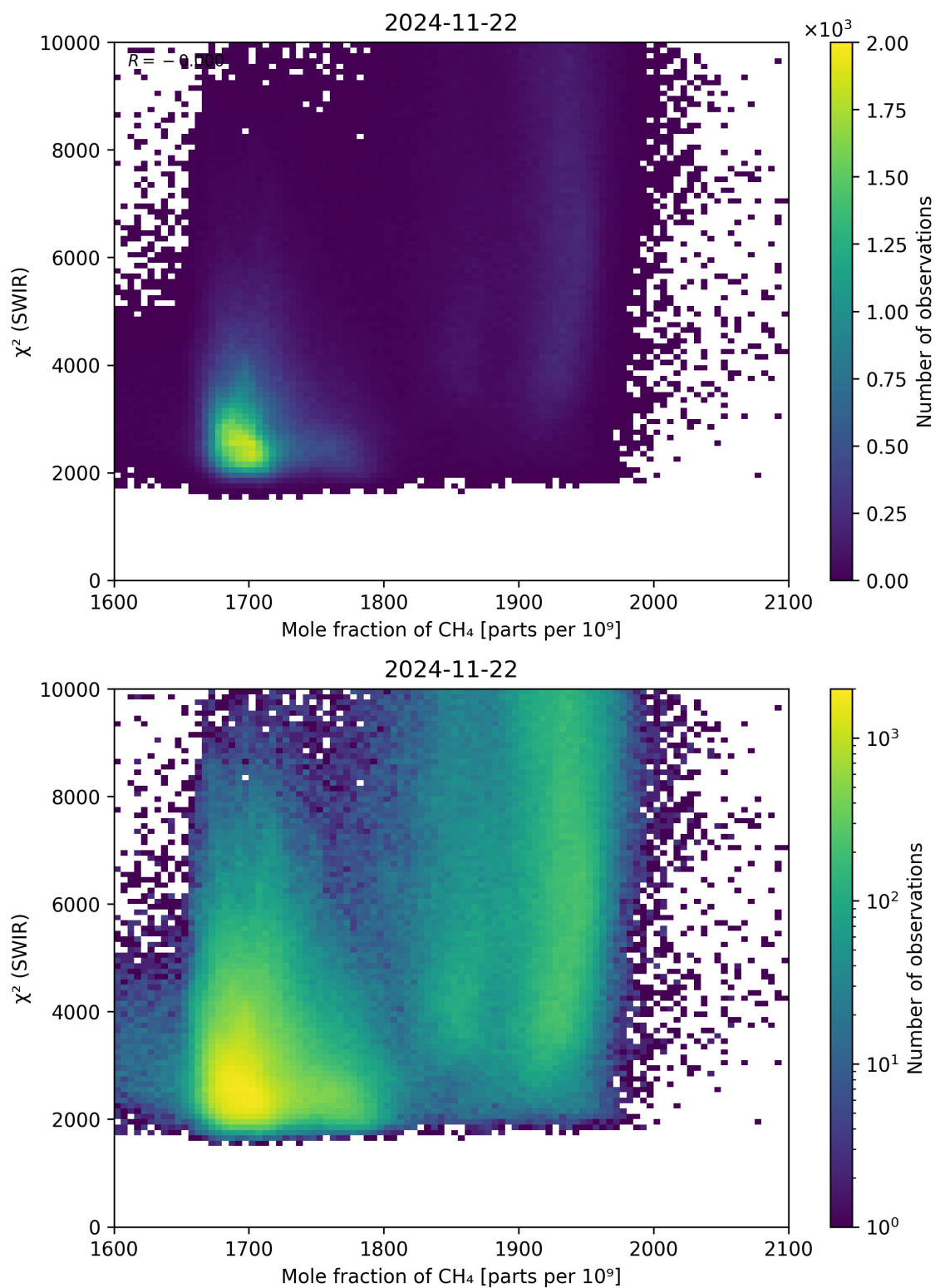
Figure 71: Scatter density plot of “Mole fraction of \text{CH}_4 ” against “ \chi^2 (SWIR)” for 2024-11-21 to 2024-11-23.
