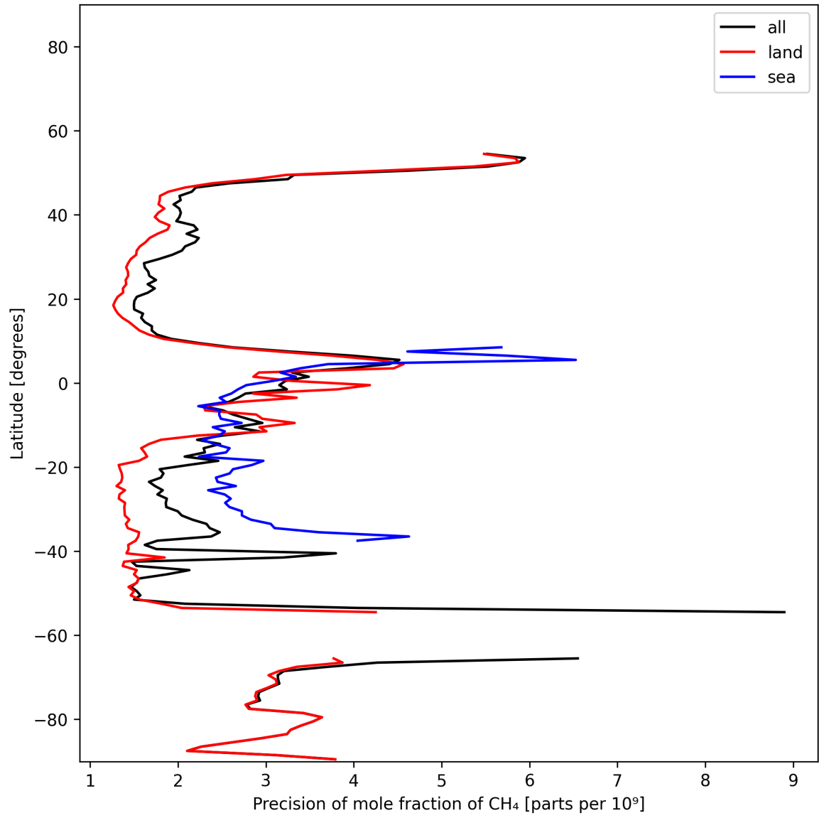
Figure 13: Zonal average of “Precision of mole fraction of CH 4 ” for 2024-11-21 to 2024-11-23.
