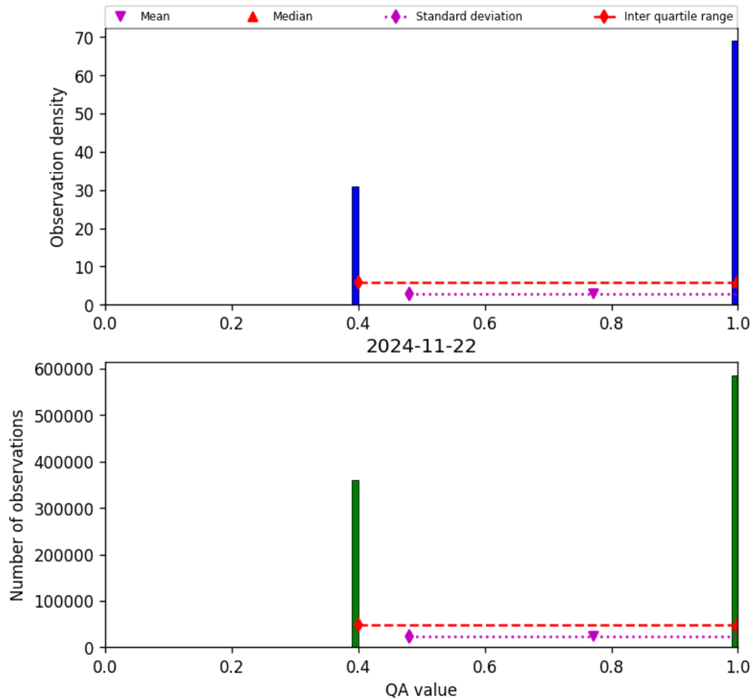
Figure 22: Histogram of “QA value” for 2024-11-21 to 2024-11-23
