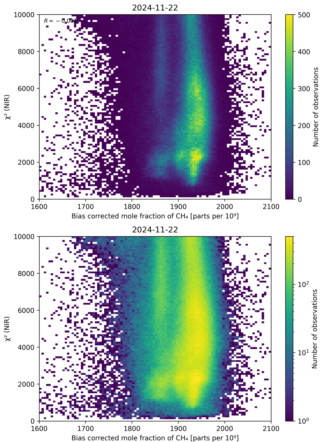
Figure 63: Scatter density plot of “Bias corrected mole fraction of CH 4 ” against “ \chi^2 (NIR)” for 2024-11-21 to 2024-11-23.
