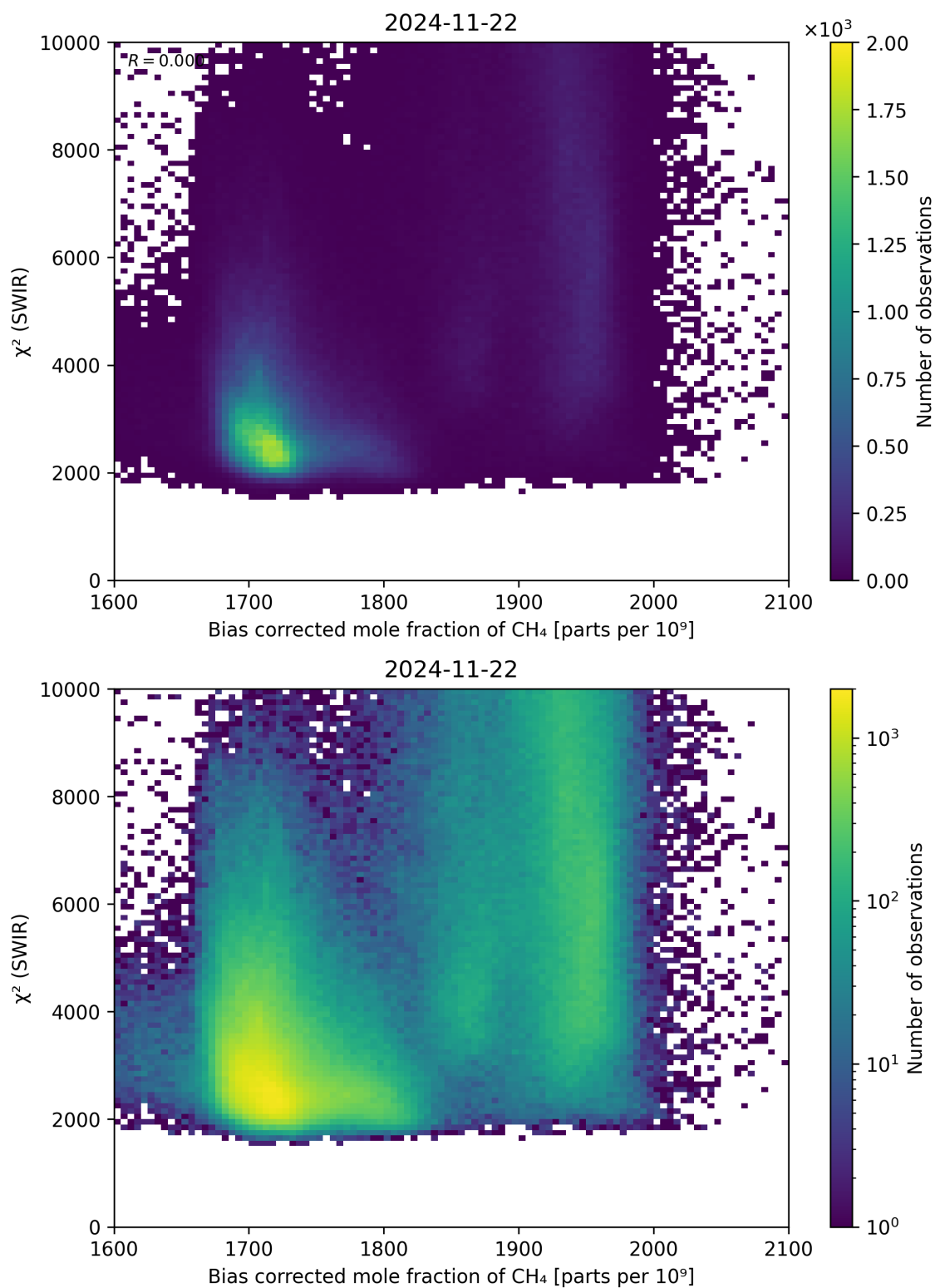
Figure 64: Scatter density plot of “Bias corrected mole fraction of CH 4 ” against “ \chi^2 (SWIR)” for 2024-11-21 to 2024-11-23.
