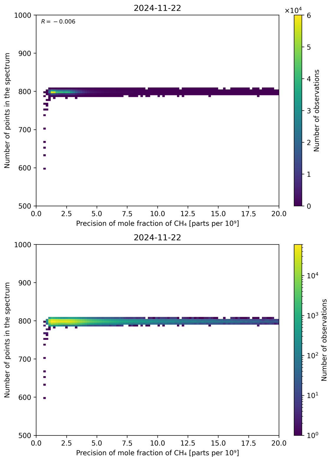
Figure 84: Scatter density plot of “Precision of mole fraction of CH 4 ” against “Number of points in the spectrum” for 2024-11-21 to 2024-11-23.
