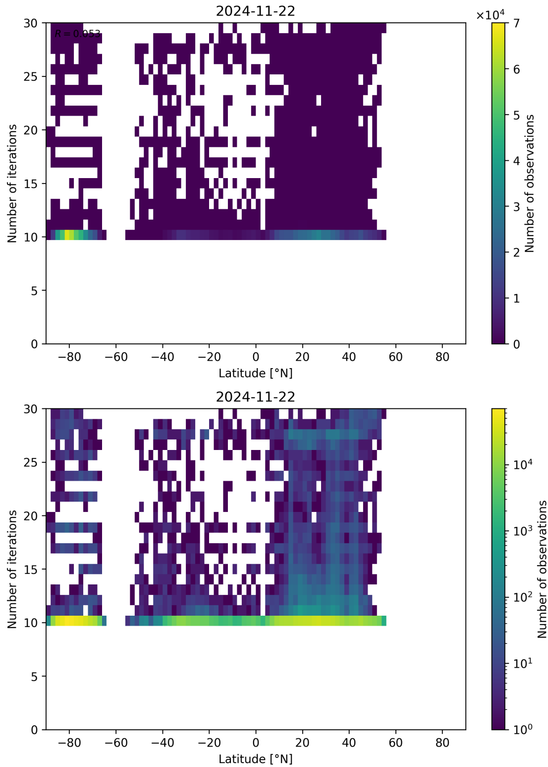
Figure 60: Scatter density plot of “Latitude” against “Number of iterations” for 2024-11-21 to 2024-11-23.
