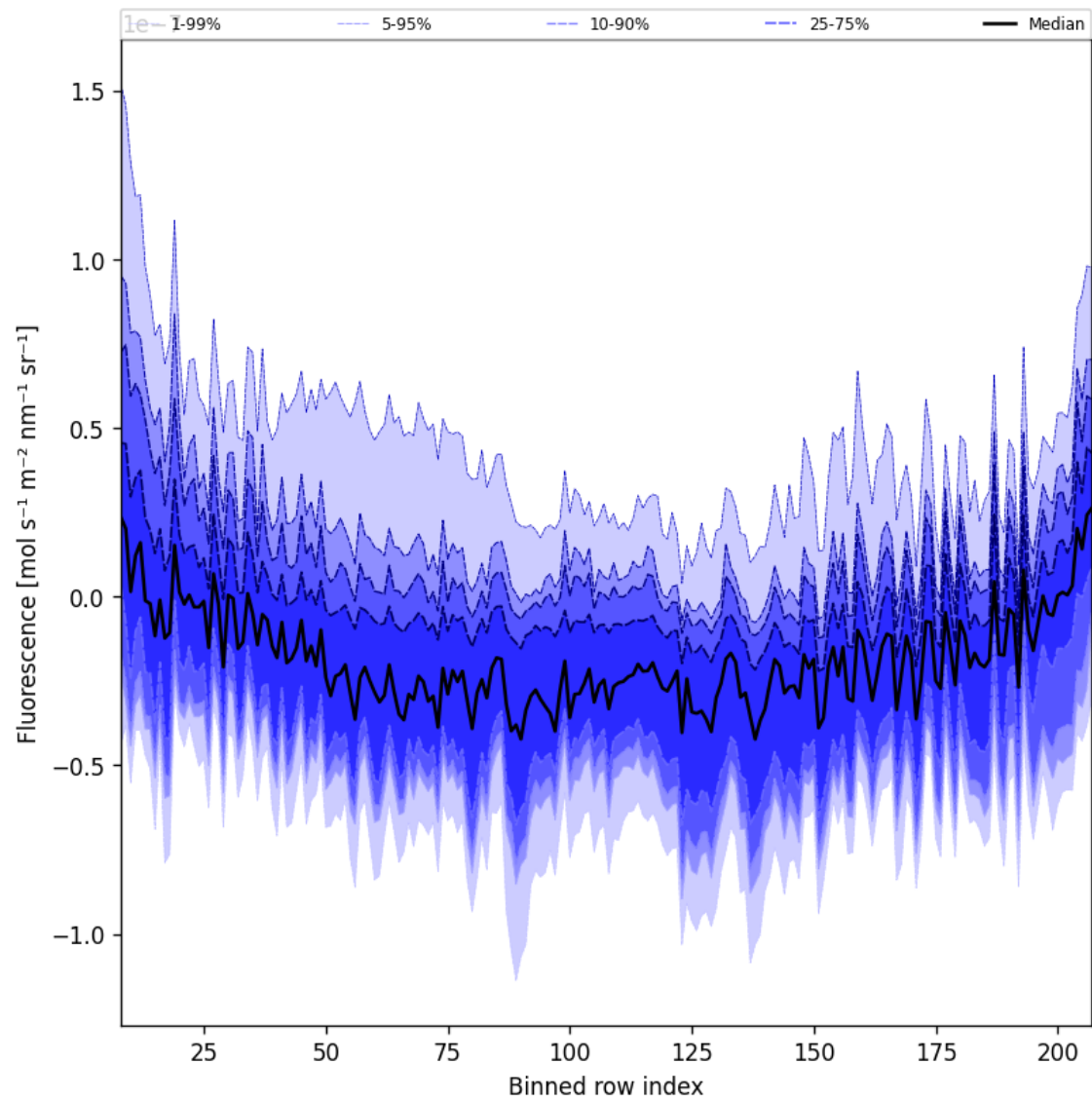
Figure 43: Along track statistics of “Fluorescence” for 2024-11-21 to 2024-11-23
