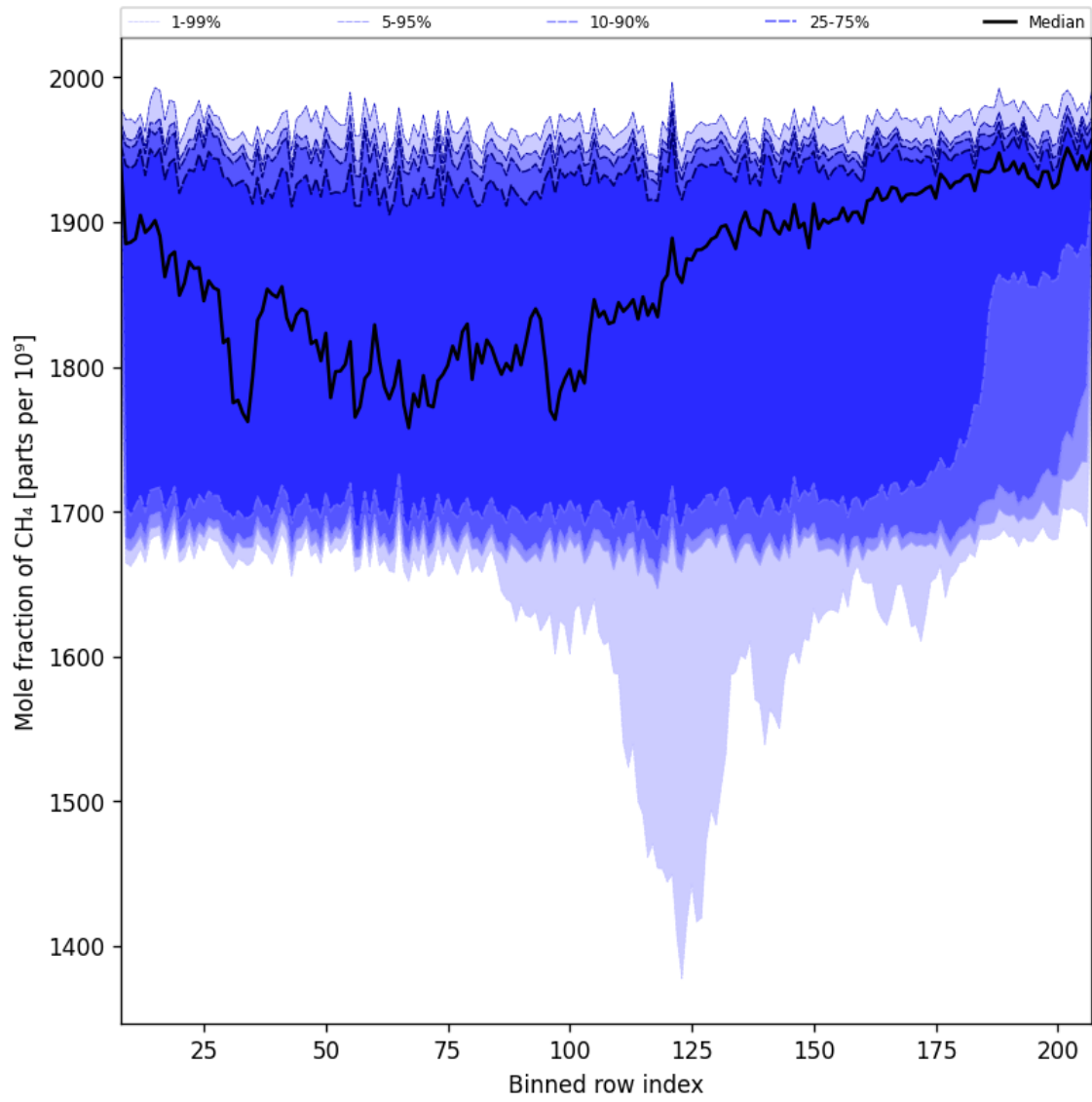
Figure 34: Along track statistics of “Mole fraction of CH 4 ” for 2024-11-21 to 2024-11-23
