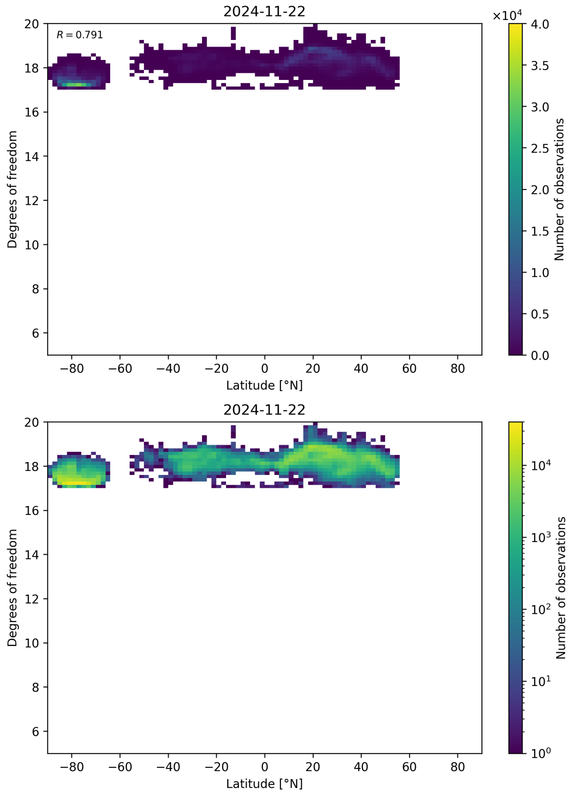
Figure 55: Scatter density plot of “Latitude” against “Degrees of freedom” for 2024-11-21 to 2024-11-23.
