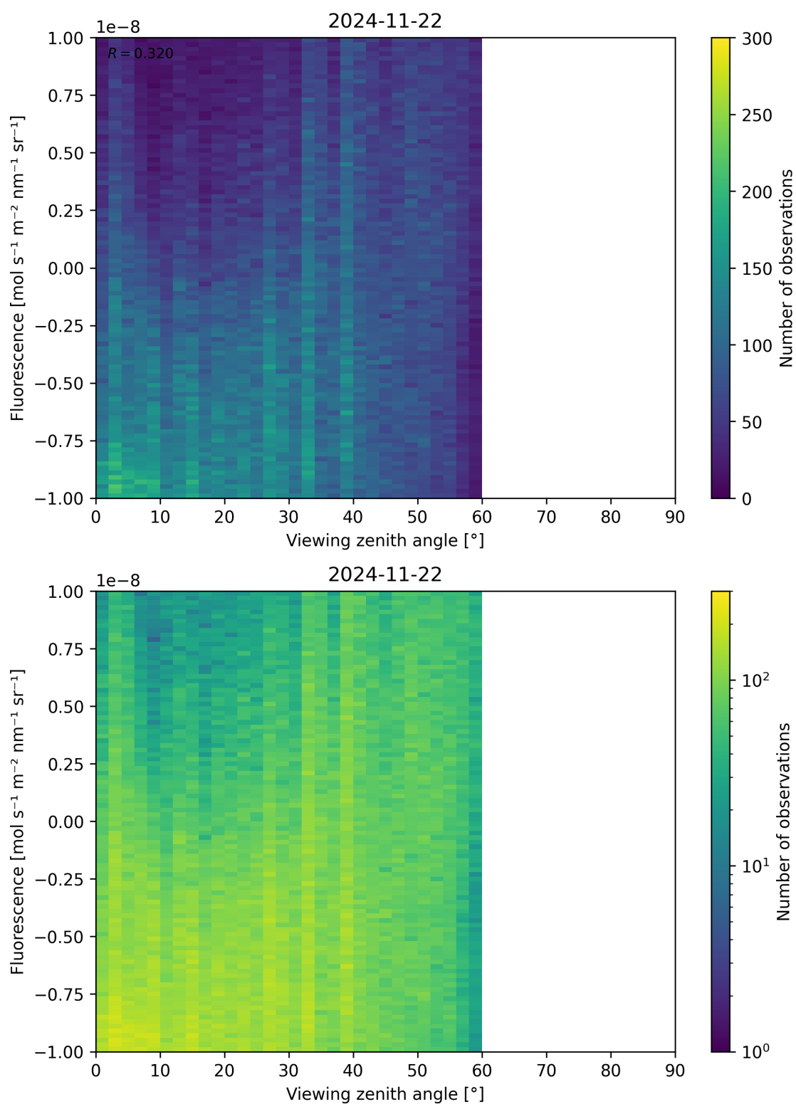
Figure 108: Scatter density plot of “Viewing zenith angle” against “Fluorescence” for 2024-11-21 to 2024-11-23.
