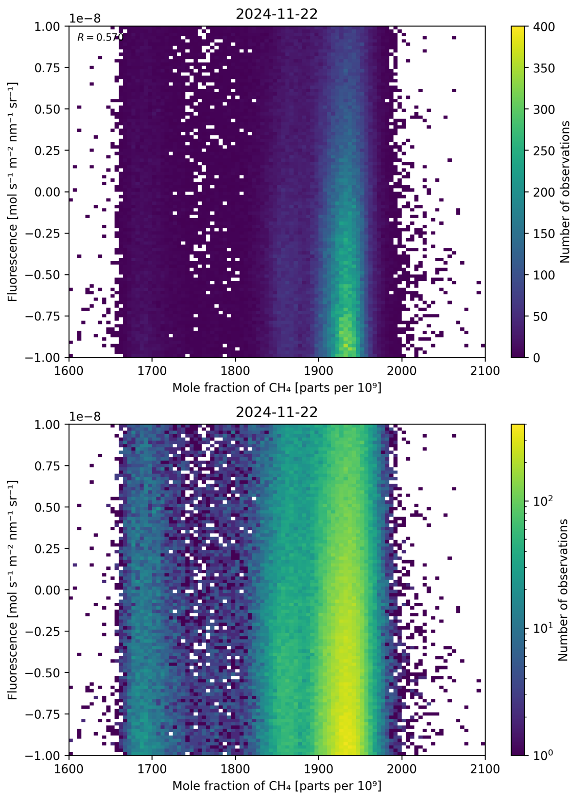
Figure 73: Scatter density plot of “Mole fraction of \text{CH}_4 ” against “Fluorescence” for 2024-11-21 to 2024-11-23.
