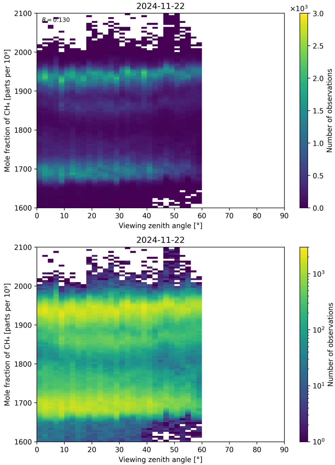
Figure 110: Scatter density plot of “Viewing zenith angle” against “Mole fraction of CH 4 ” for 2024-11-21 to 2024-11-23.
