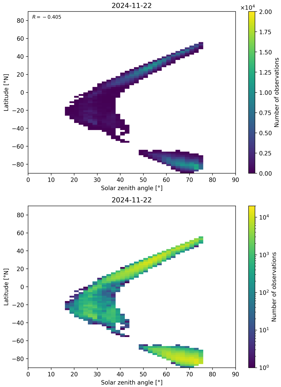
Figure 98: Scatter density plot of “Solar zenith angle” against “Latitude” for 2024-11-21 to 2024-11-23.
