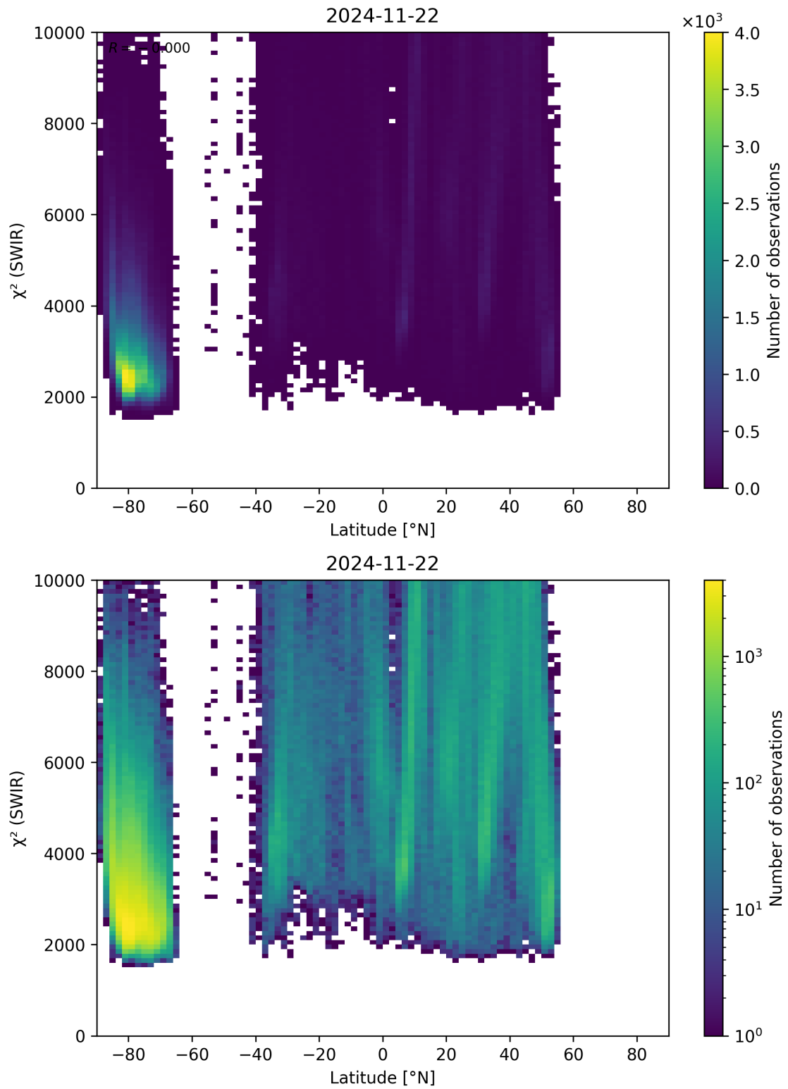
Figure 54: Scatter density plot of “Latitude” against “ \chi^2 (SWIR)” for 2024-11-21 to 2024-11-23.
