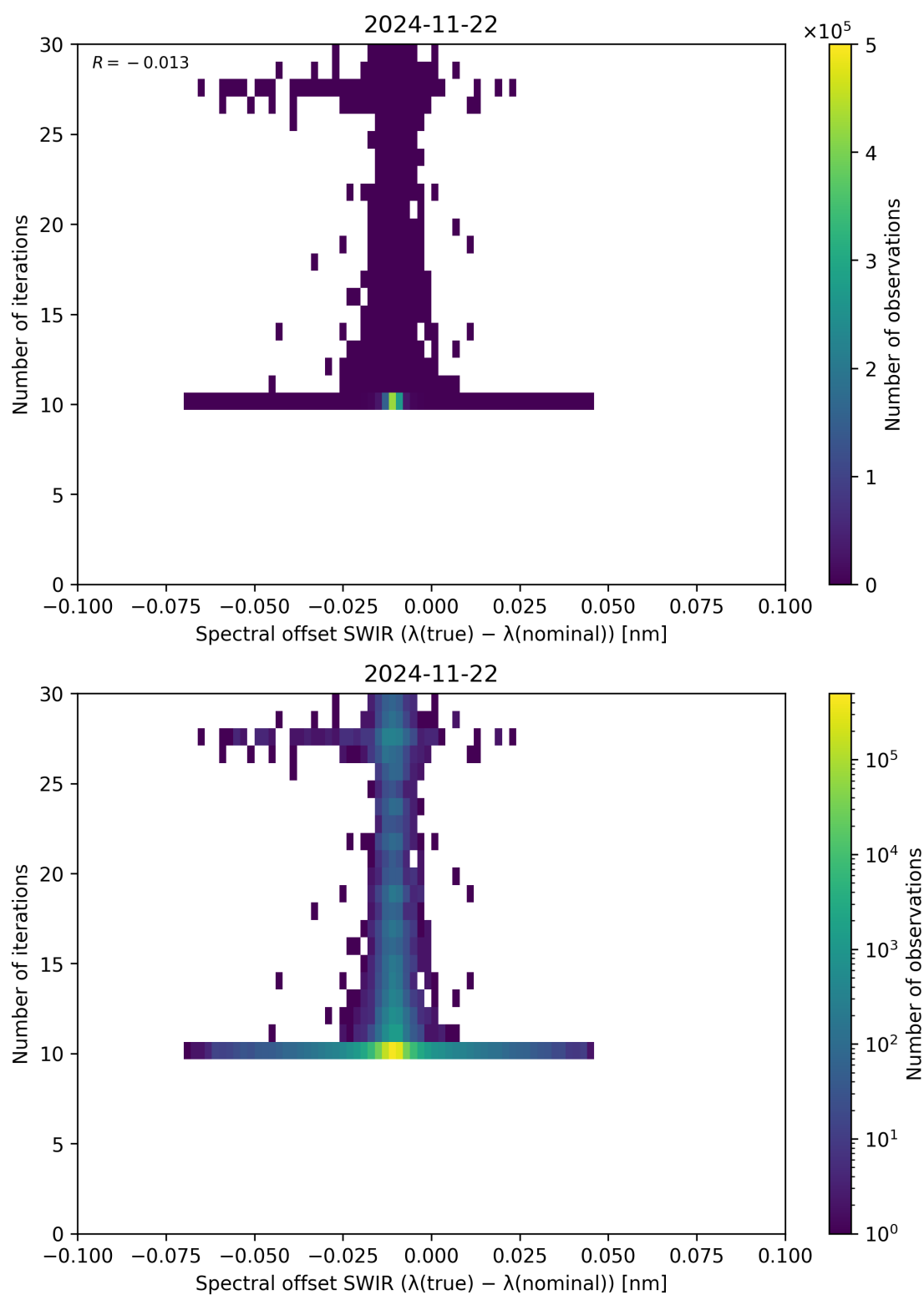
Figure 121: Scatter density plot of “Spectral offset SWIR ( \lambda_{\text{true}} - \lambda_{\text{nominal}} )” against “Number of iterations” for 2024-11-21 to 2024-11-23.
