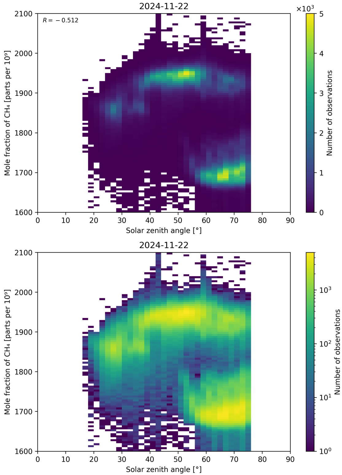
Figure 99: Scatter density plot of “Solar zenith angle” against “Mole fraction of CH 4 ” for 2024-11-21 to 2024-11-23.
