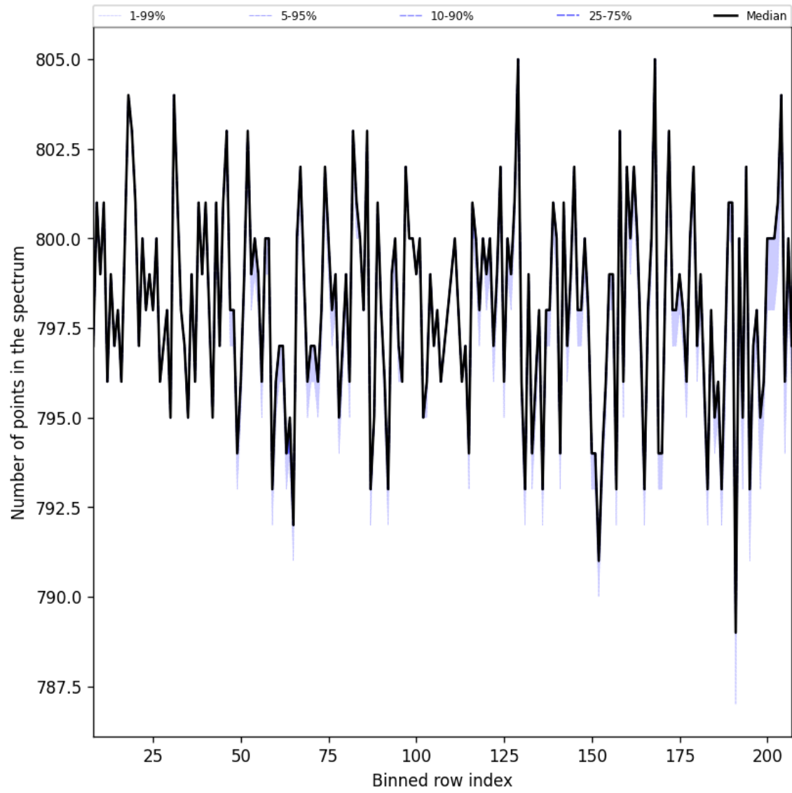
Figure 37: Along track statistics of “Number of points in the spectrum” for 2024-11-21 to 2024-11-23
