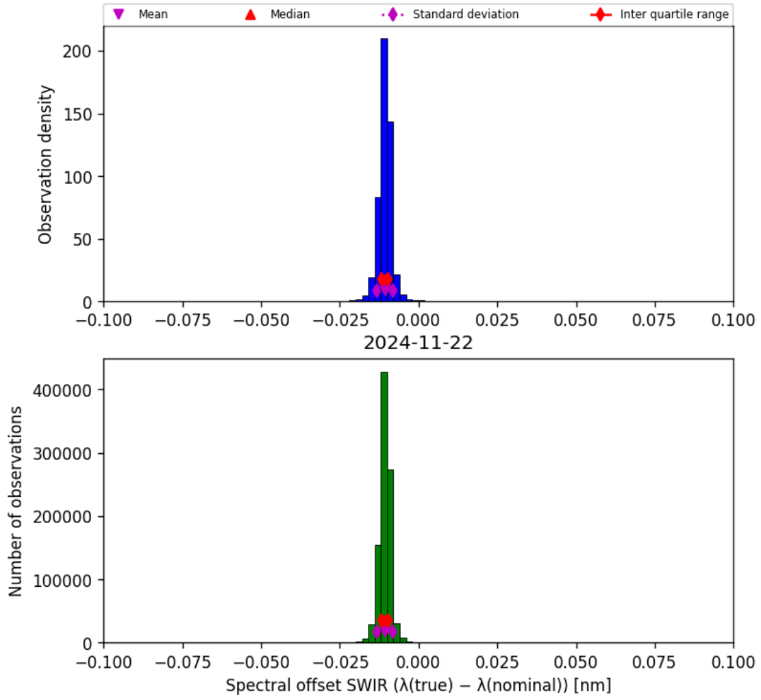
Figure 27: Histogram of “Spectral offset SWIR ( \lambda_{\text{true}} - \lambda_{\text{nominal}} )” for 2024-11-21 to 2024-11-23
