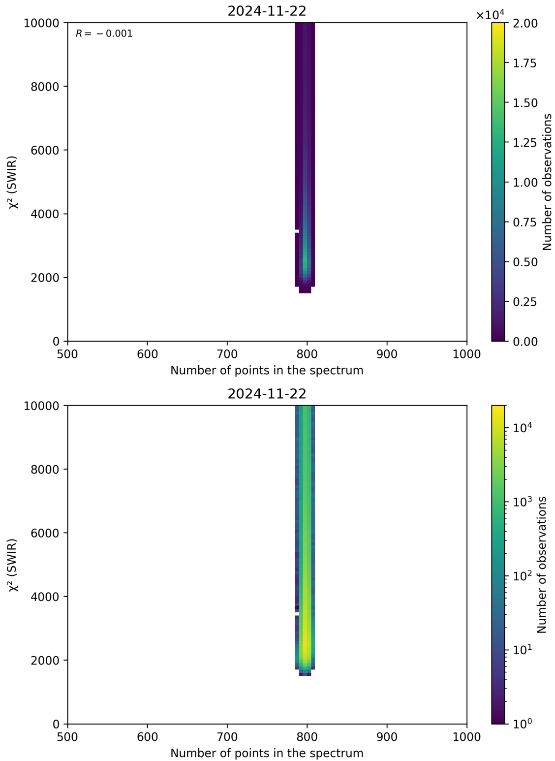
Figure 89: Scatter density plot of “Number of points in the spectrum” against “ \chi^2 (SWIR)” for 2024-11-21 to 2024-11-23.
