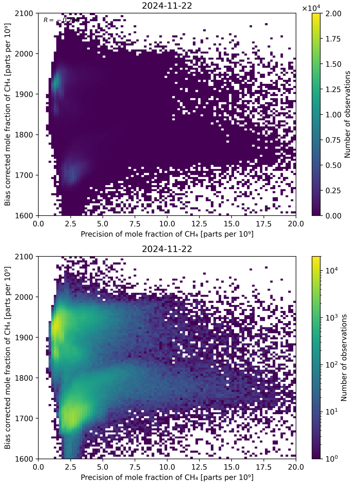
Figure 82: Scatter density plot of “Precision of mole fraction of CH 4 ” against “Bias corrected mole fraction of CH 4 ” for 2024-11-21 to 2024-11-23.
