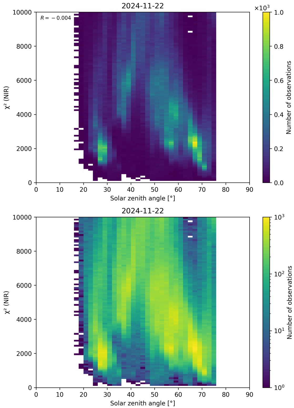
Figure 94: Scatter density plot of “Solar zenith angle” against “ \chi^2 (NIR)” for 2024-11-21 to 2024-11-23.
