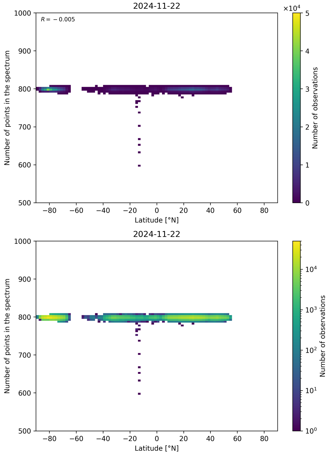
Figure 61: Scatter density plot of “Latitude” against “Number of points in the spectrum” for 2024-11-21 to 2024-11-23.
