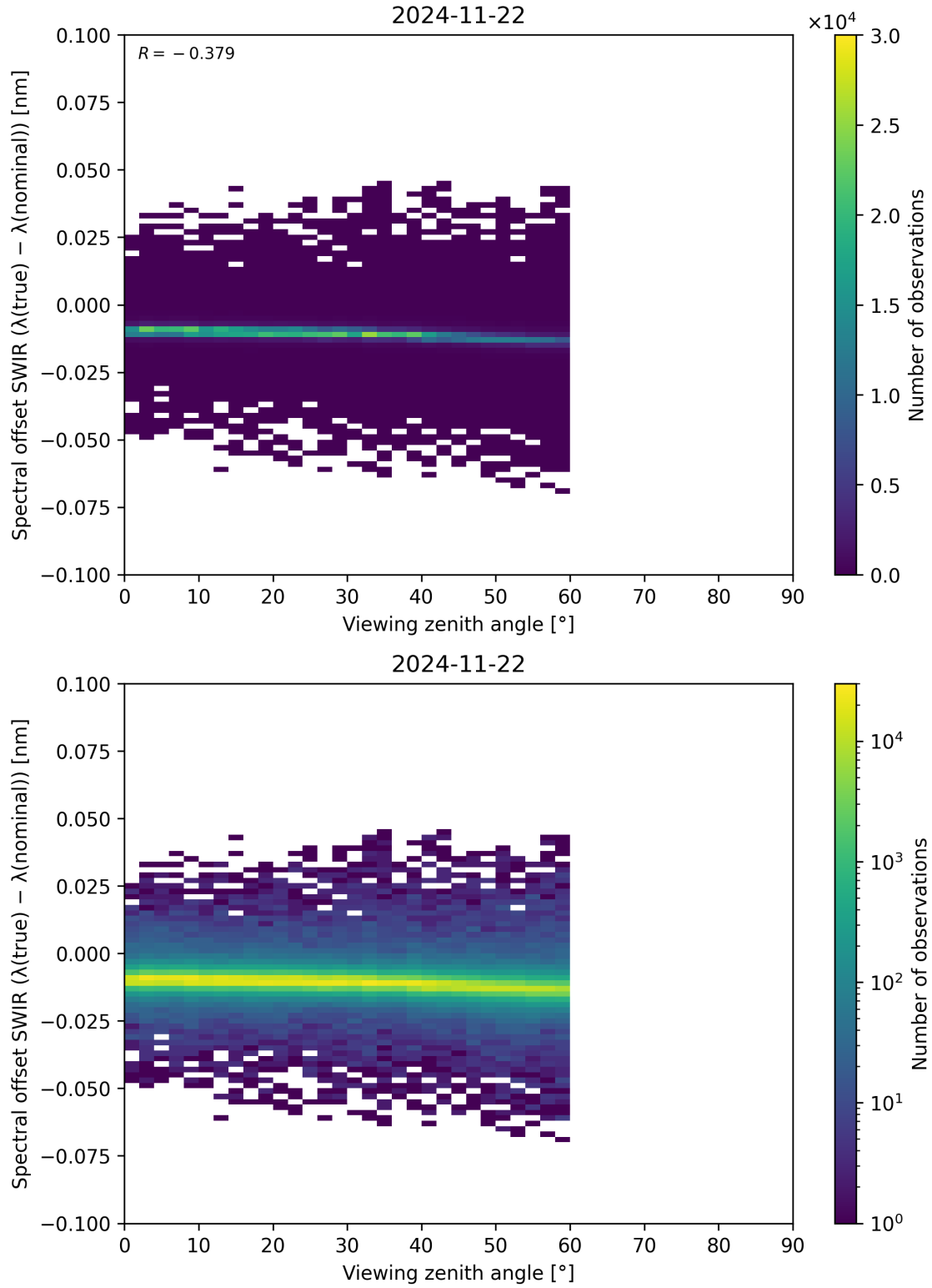
Figure 116: Scatter density plot of “Viewing zenith angle” against “Spectral offset SWIR ( \lambda_{\text{true}} - \lambda_{\text{nominal}} )” for 2024-11-21 to 2024-11-23.
