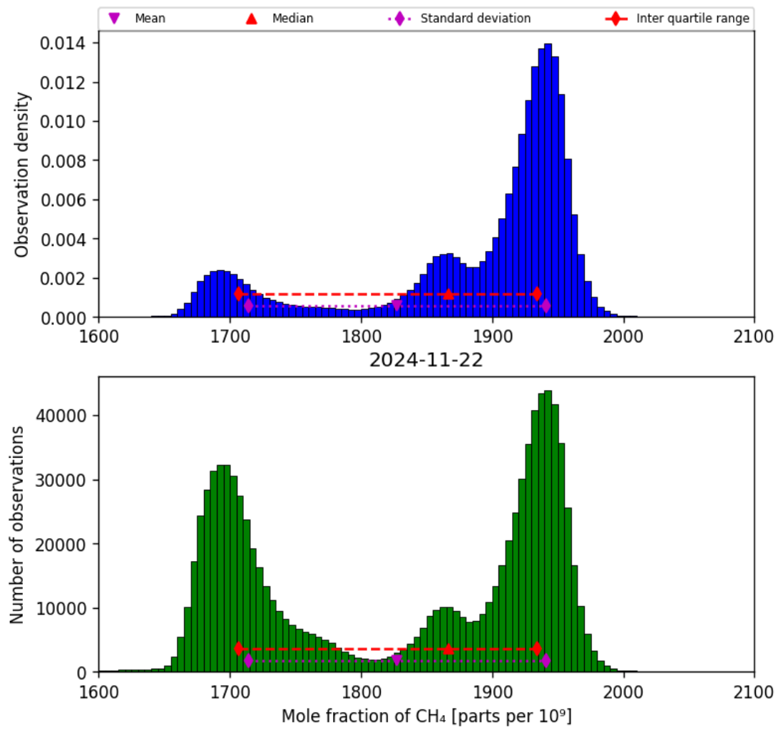
Figure 23: Histogram of “Mole fraction of CH 4 ” for 2024-11-21 to 2024-11-23
