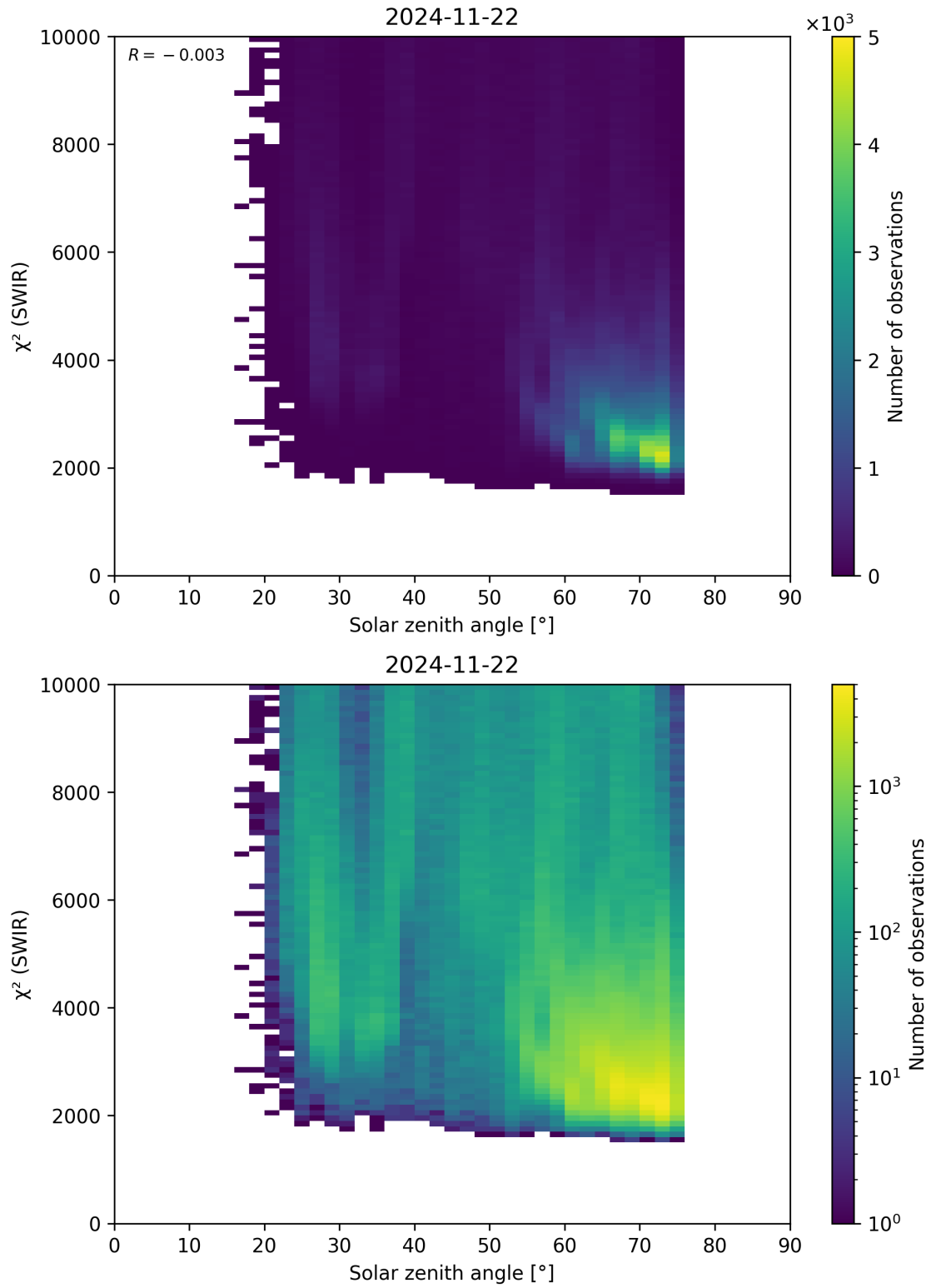
Figure 95: Scatter density plot of “Solar zenith angle” against “ \chi^2 (SWIR)” for 2024-11-21 to 2024-11-23.
