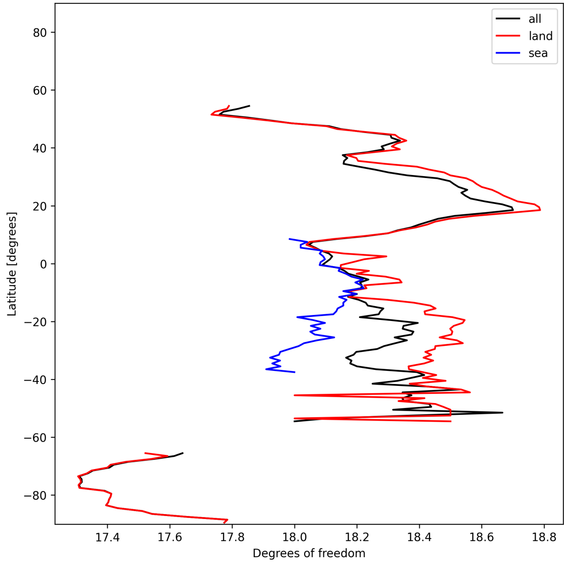
Figure 19: Zonal average of “Degrees of freedom” for 2024-11-21 to 2024-11-23.
