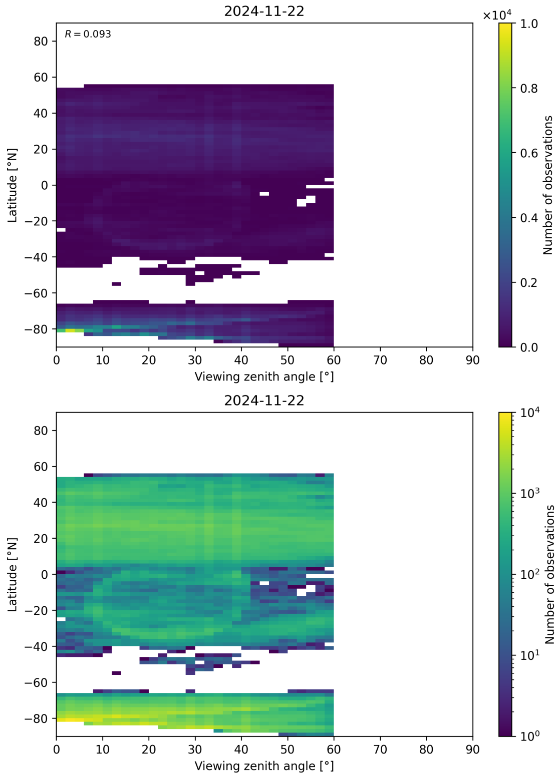
Figure 109: Scatter density plot of “Viewing zenith angle” against “Latitude” for 2024-11-21 to 2024-11-23.
