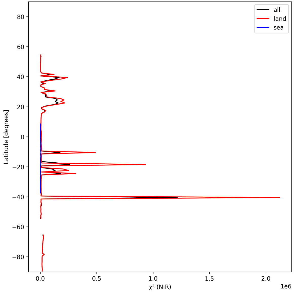
Figure 18: Zonal average of “ \chi^2 (NIR)” for 2024-11-21 to 2024-11-23.
