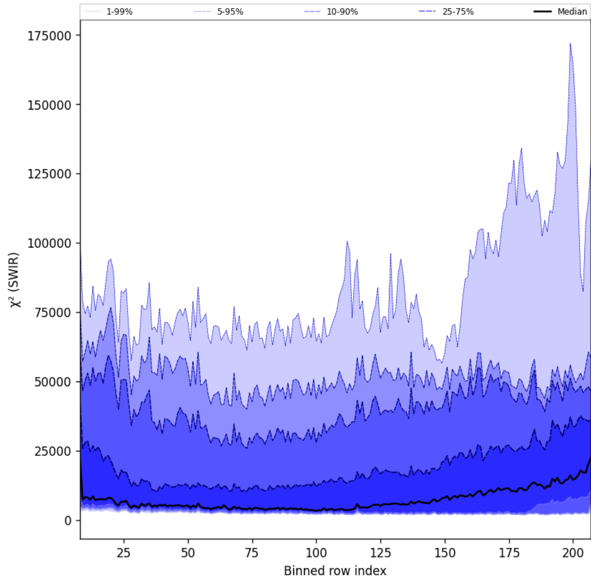
Figure 39: Along track statistics of “ \chi^2 (SWIR)” for 2024-11-21 to 2024-11-23
