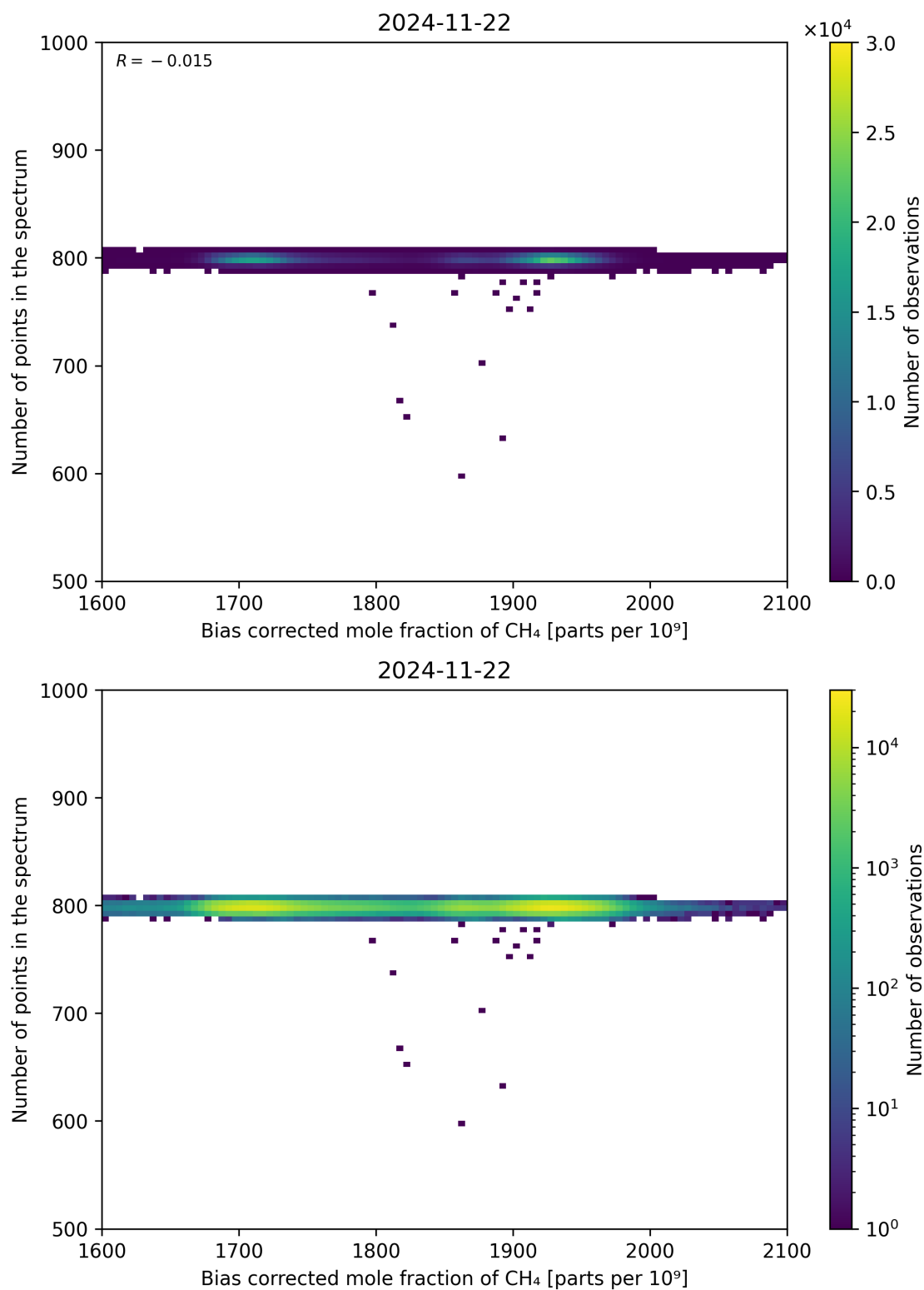
Figure 68: Scatter density plot of “Bias corrected mole fraction of CH 4 ” against “Number of points in the spectrum” for 2024-11-21 to 2024-11-23.
