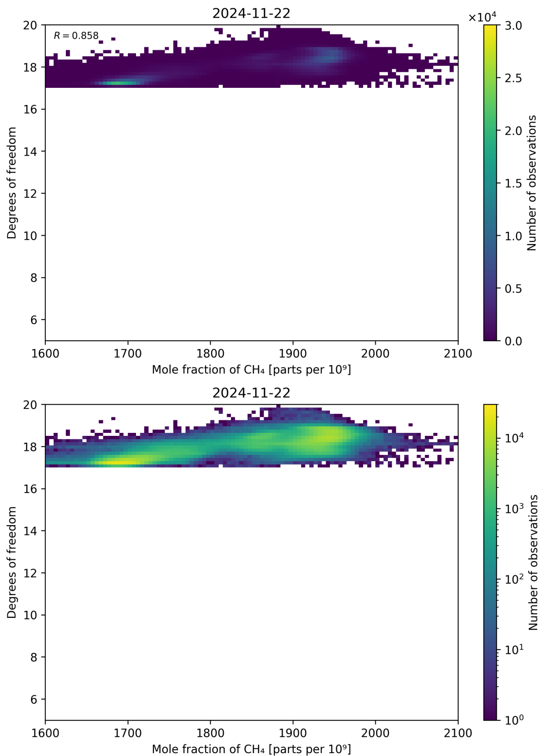
Figure 72: Scatter density plot of “Mole fraction of CH 4 ” against “Degrees of freedom” for 2024-11-21 to 2024-11-23.
