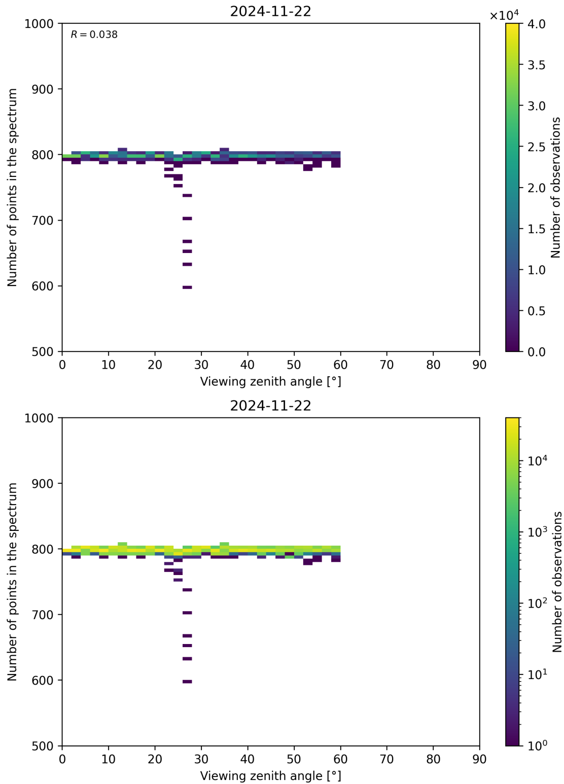
Figure 114: Scatter density plot of “Viewing zenith angle” against “Number of points in the spectrum” for 2024-11-21 to 2024-11-23.
