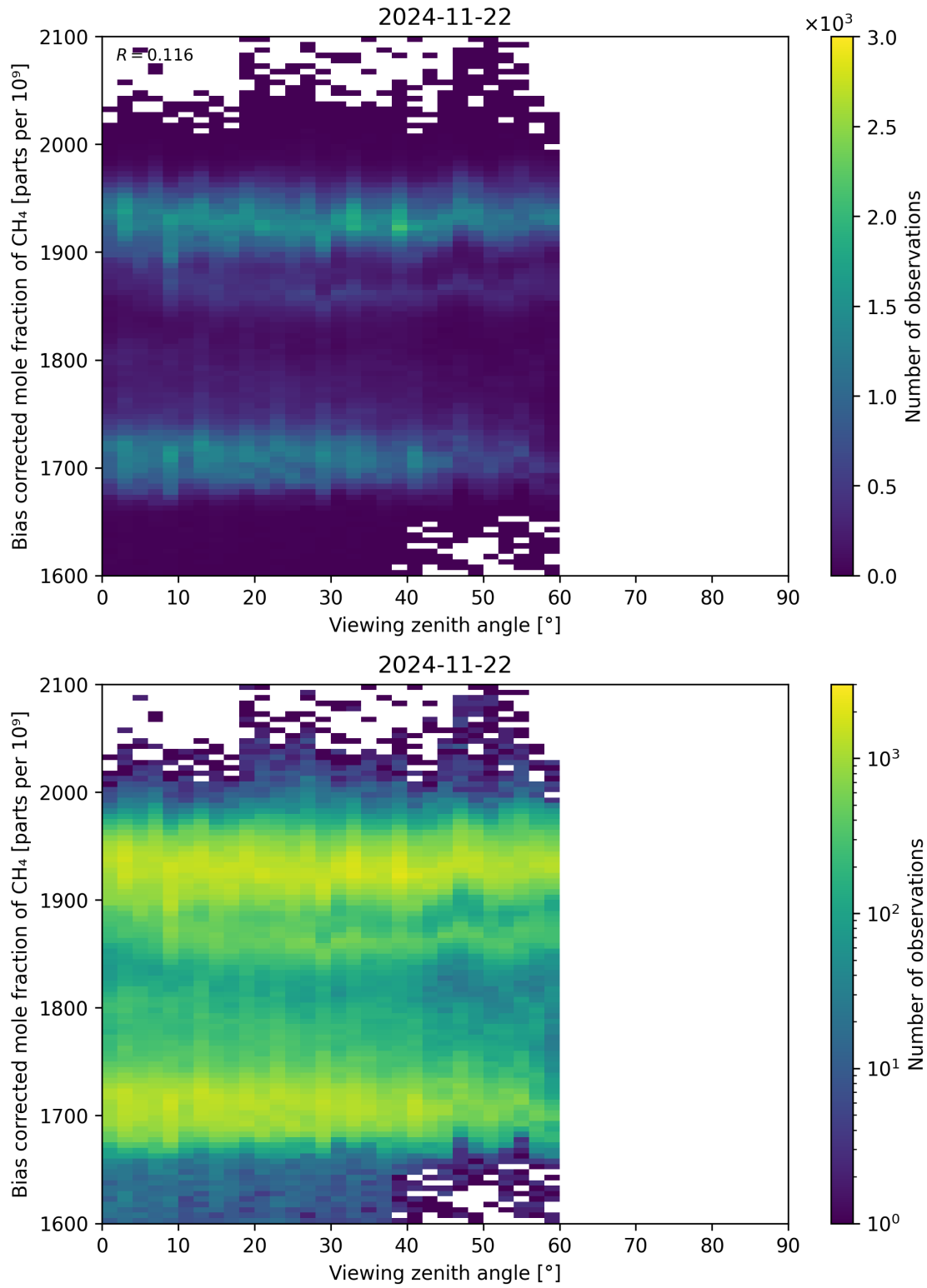
Figure 111: Scatter density plot of “Viewing zenith angle” against “Bias corrected mole fraction of CH 4 ” for 2024-11-21 to 2024-11-23.
