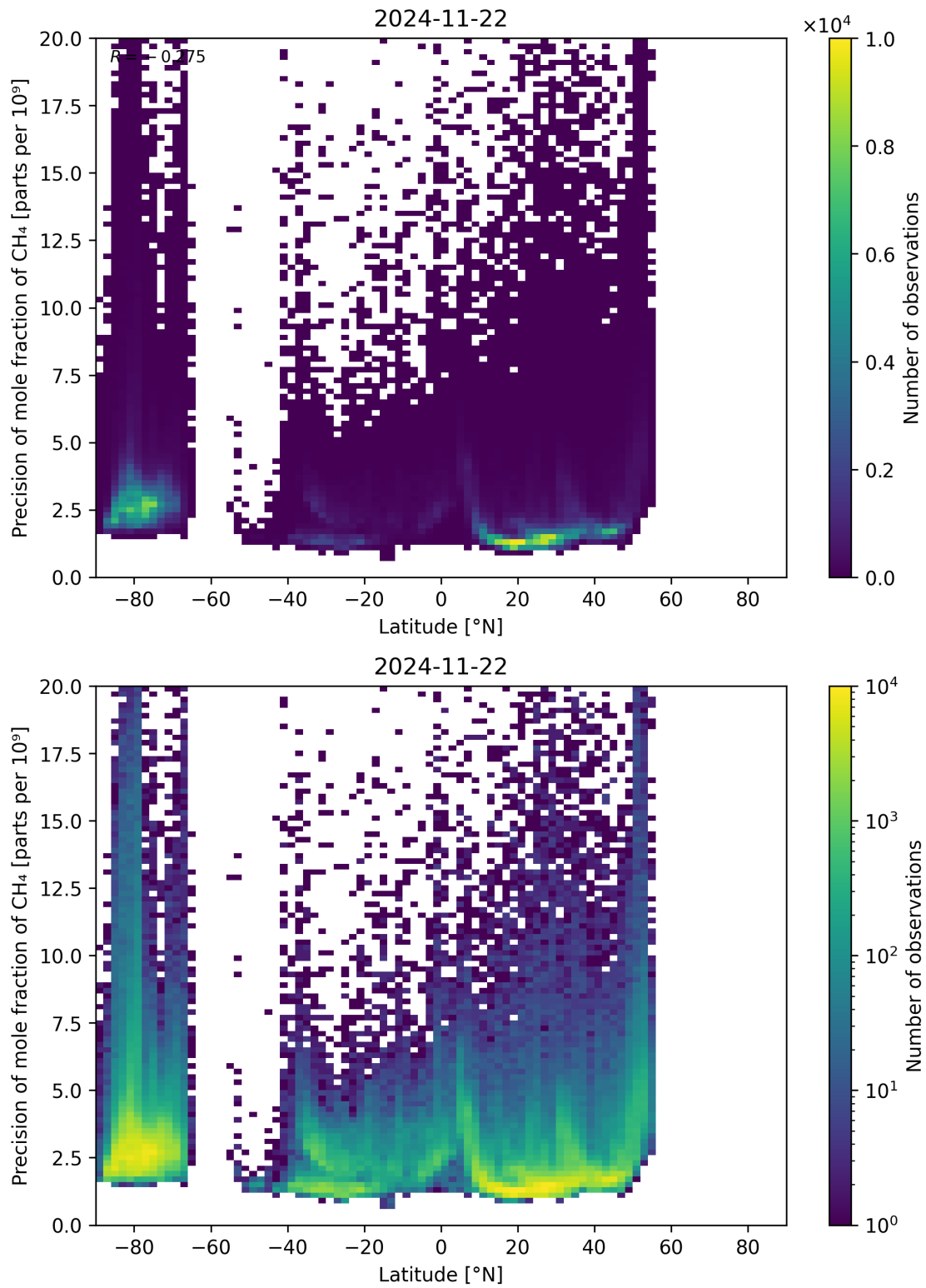
Figure 59: Scatter density plot of “Latitude” against “Precision of mole fraction of \text{CH}_4 ” for 2024-11-21 to 2024-11-23.
