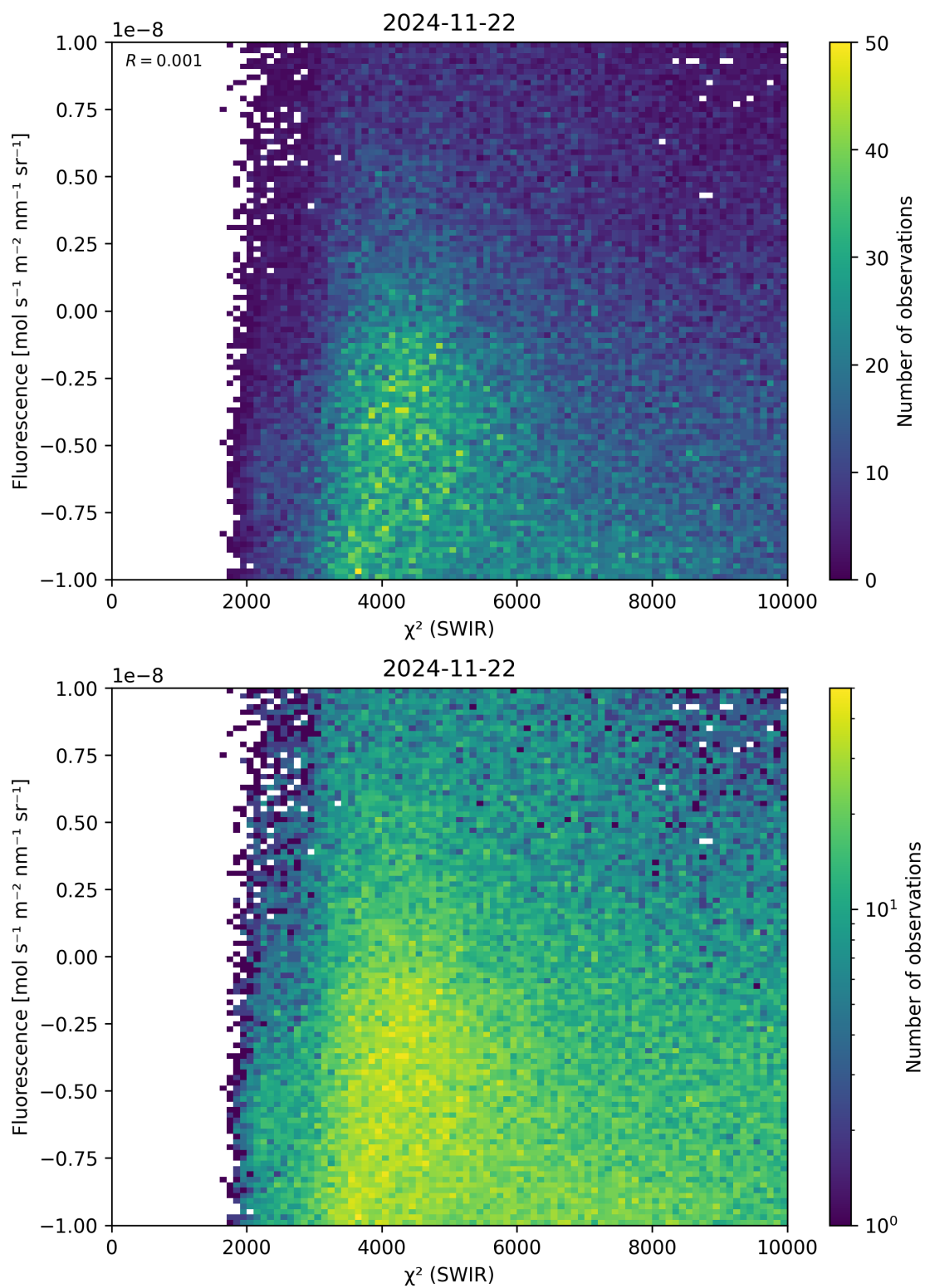
Figure 49: Scatter density plot of “ \chi^2 (SWIR)” against “Fluorescence” for 2024-11-21 to 2024-11-23.
