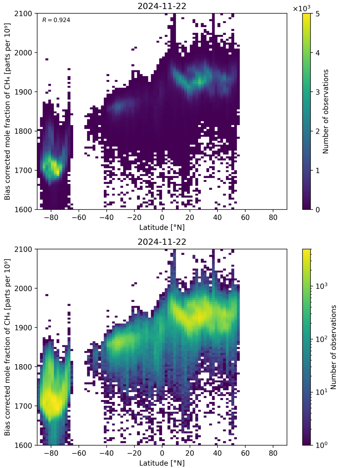
Figure 58: Scatter density plot of “Latitude” against “Bias corrected mole fraction of CH 4 ” for 2024-11-21 to 2024-11-23.
