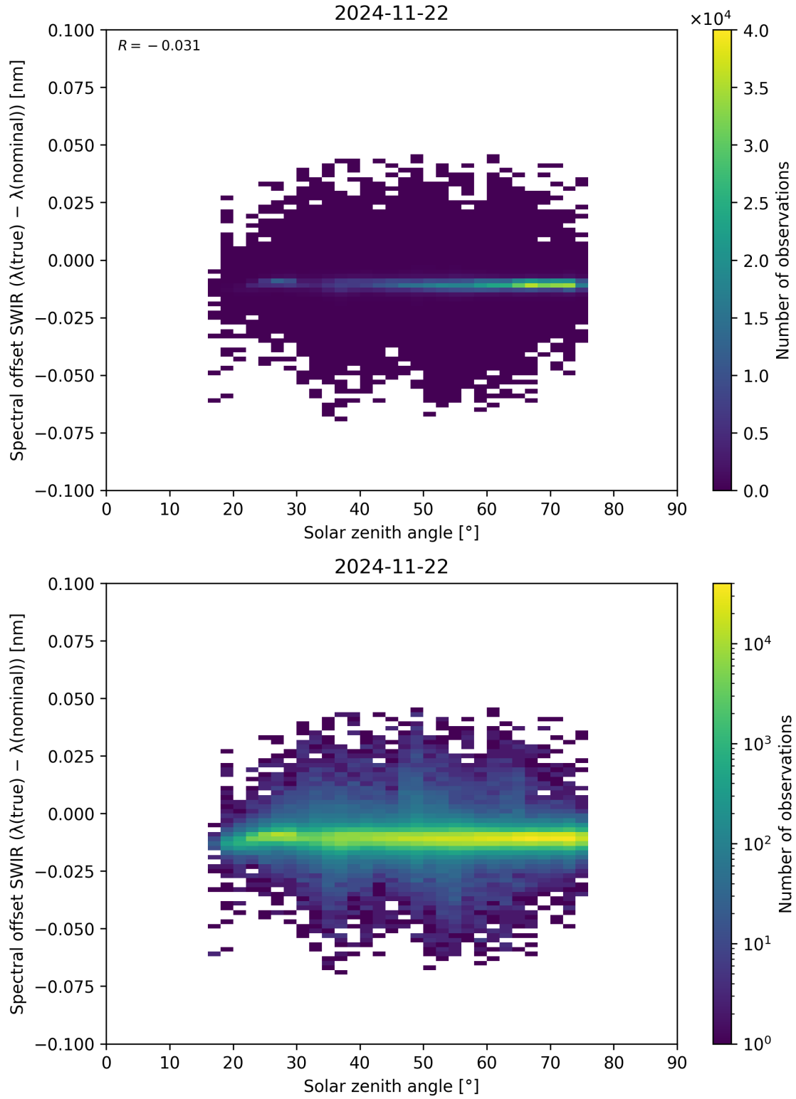
Figure 104: Scatter density plot of “Solar zenith angle” against “Spectral offset SWIR ( \lambda_{\text{true}} - \lambda_{\text{nominal}} )” for 2024-11-21 to 2024-11-23.
