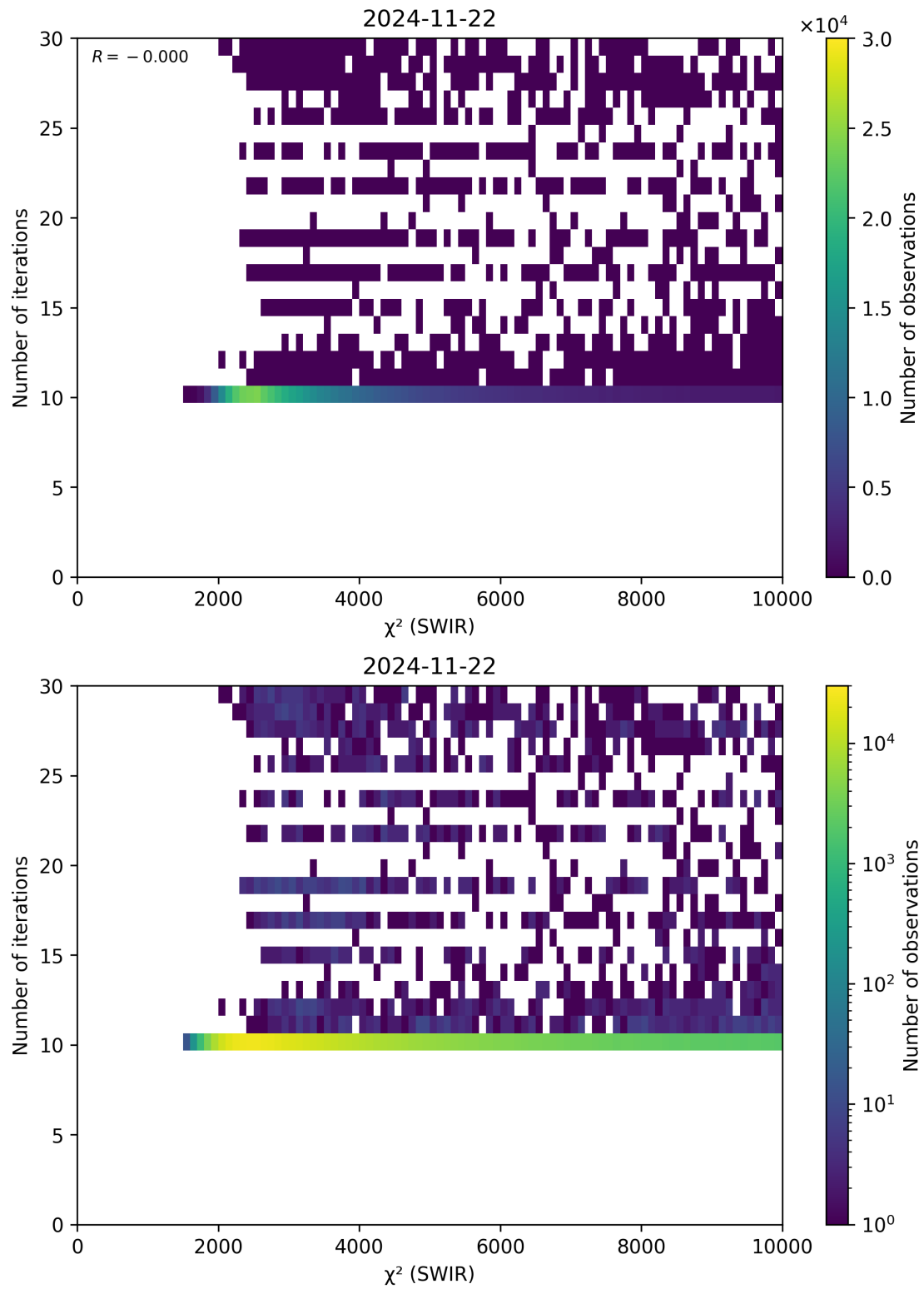
Figure 50: Scatter density plot of “ \chi^2 (SWIR)” against “Number of iterations” for 2024-11-21 to 2024-11-23.
