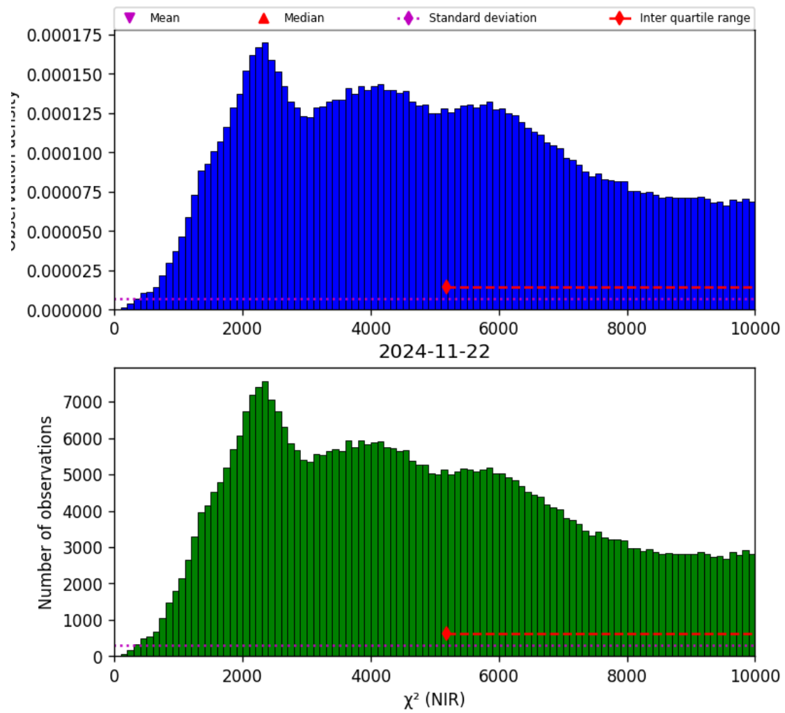
Figure 29: Histogram of “ \chi^2 (NIR)” for 2024-11-21 to 2024-11-23
