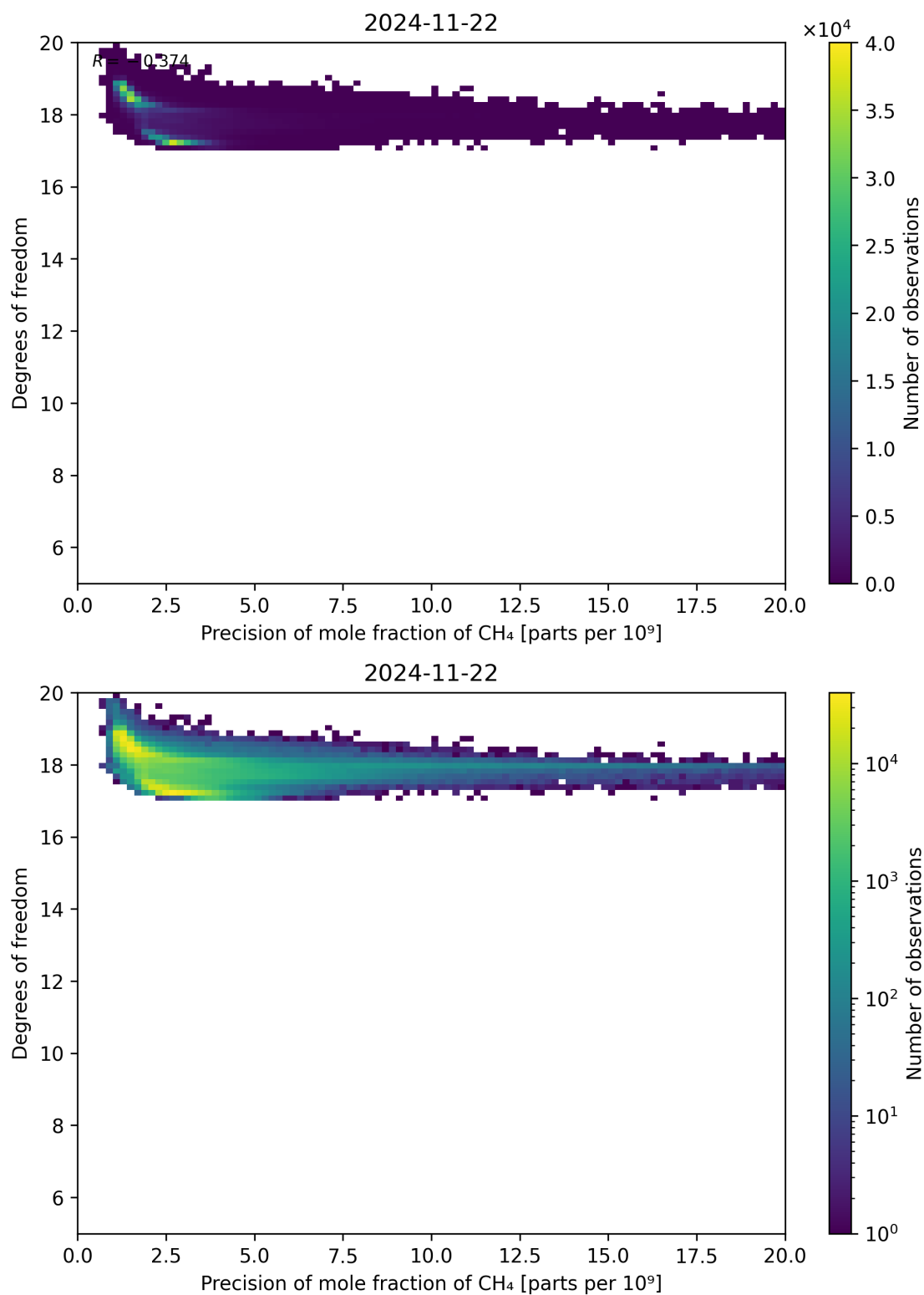
Figure 80: Scatter density plot of “Precision of mole fraction of CH 4 ” against “Degrees of freedom” for 2024-11-21 to 2024-11-23.
