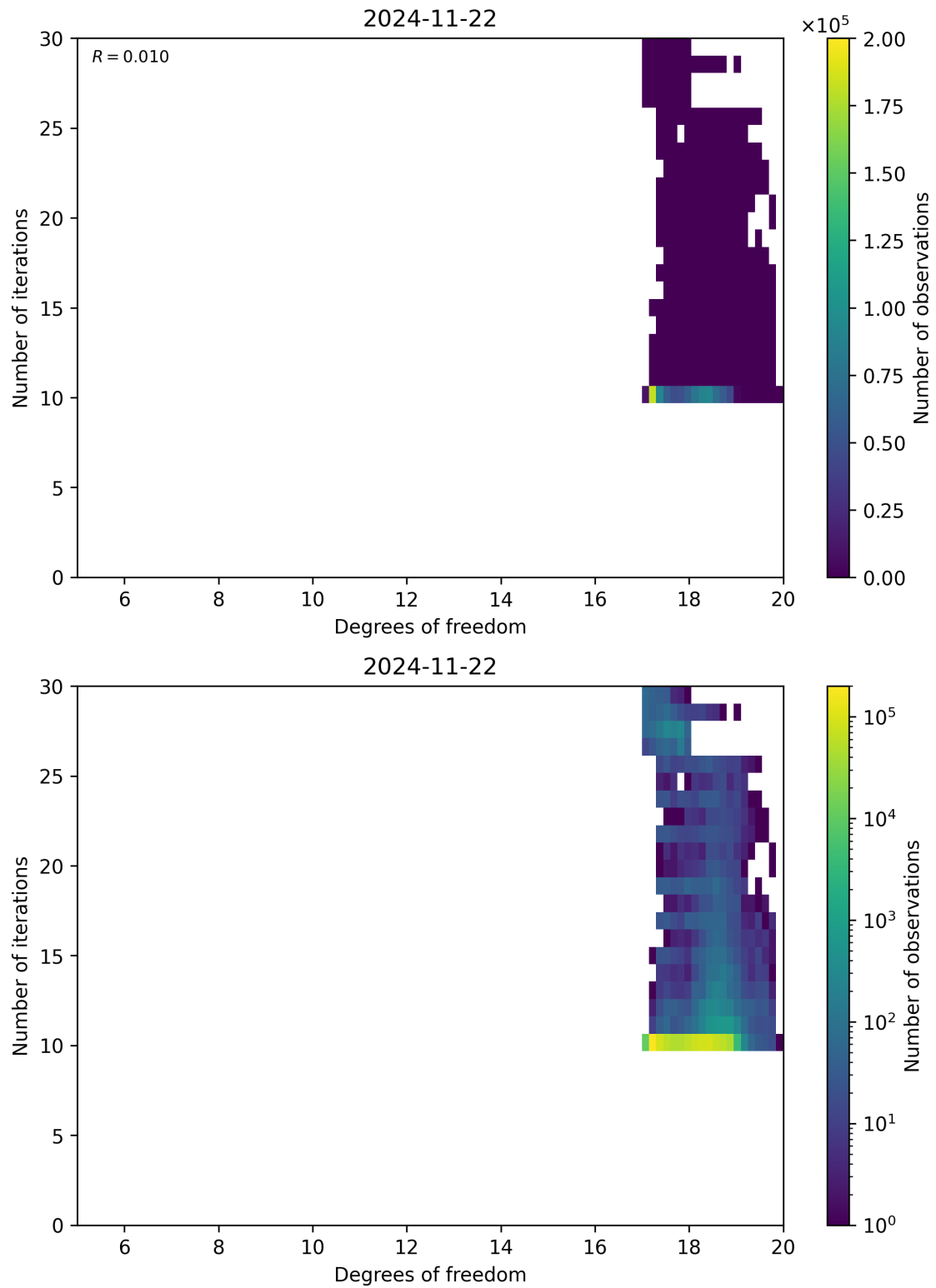
Figure 52: Scatter density plot of “Degrees of freedom” against “Number of iterations” for 2024-11-21 to 2024-11-23.
