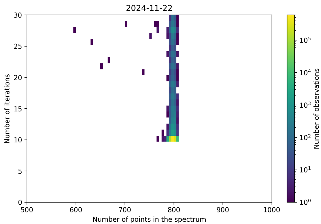
Figure 92: Scatter density plot of “Number of points in the spectrum” against “Number of iterations” for 2024-11-21 to 2024-11-23.
