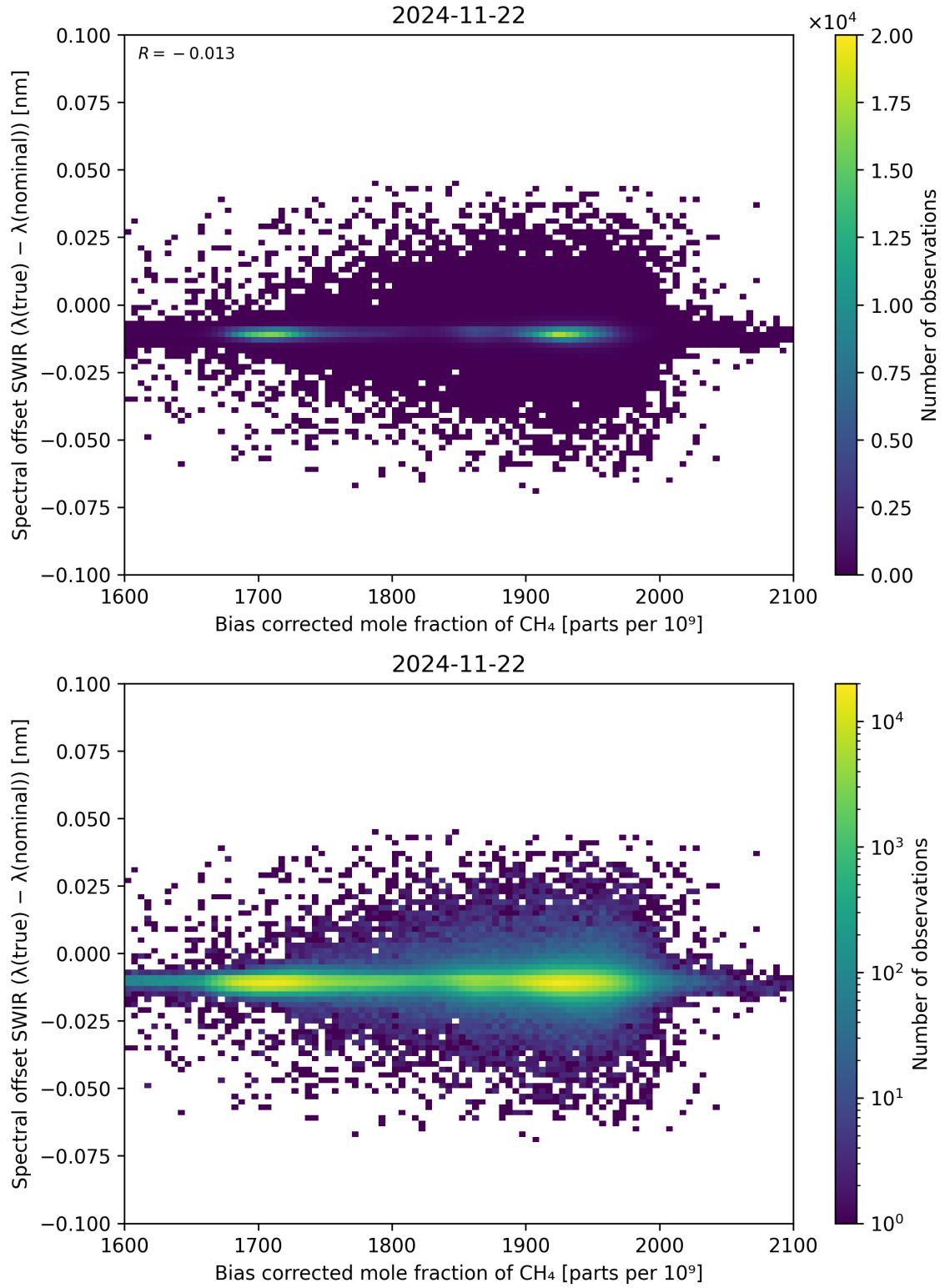
Figure 69: Scatter density plot of “Bias corrected mole fraction of \text{CH}_4 ” against “Spectral offset SWIR ( \lambda_{\text{true}} - \lambda_{\text{nominal}} )” for 2024-11-21 to 2024-11-23.
