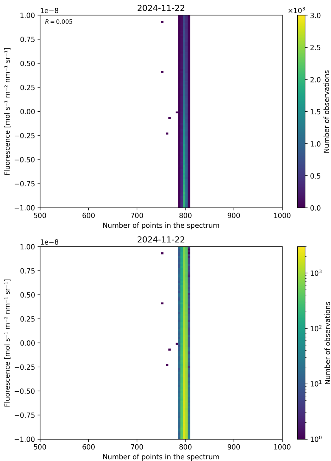
Figure 91: Scatter density plot of “Number of points in the spectrum” against “Fluorescence” for 2024-11-21 to 2024-11-23.
