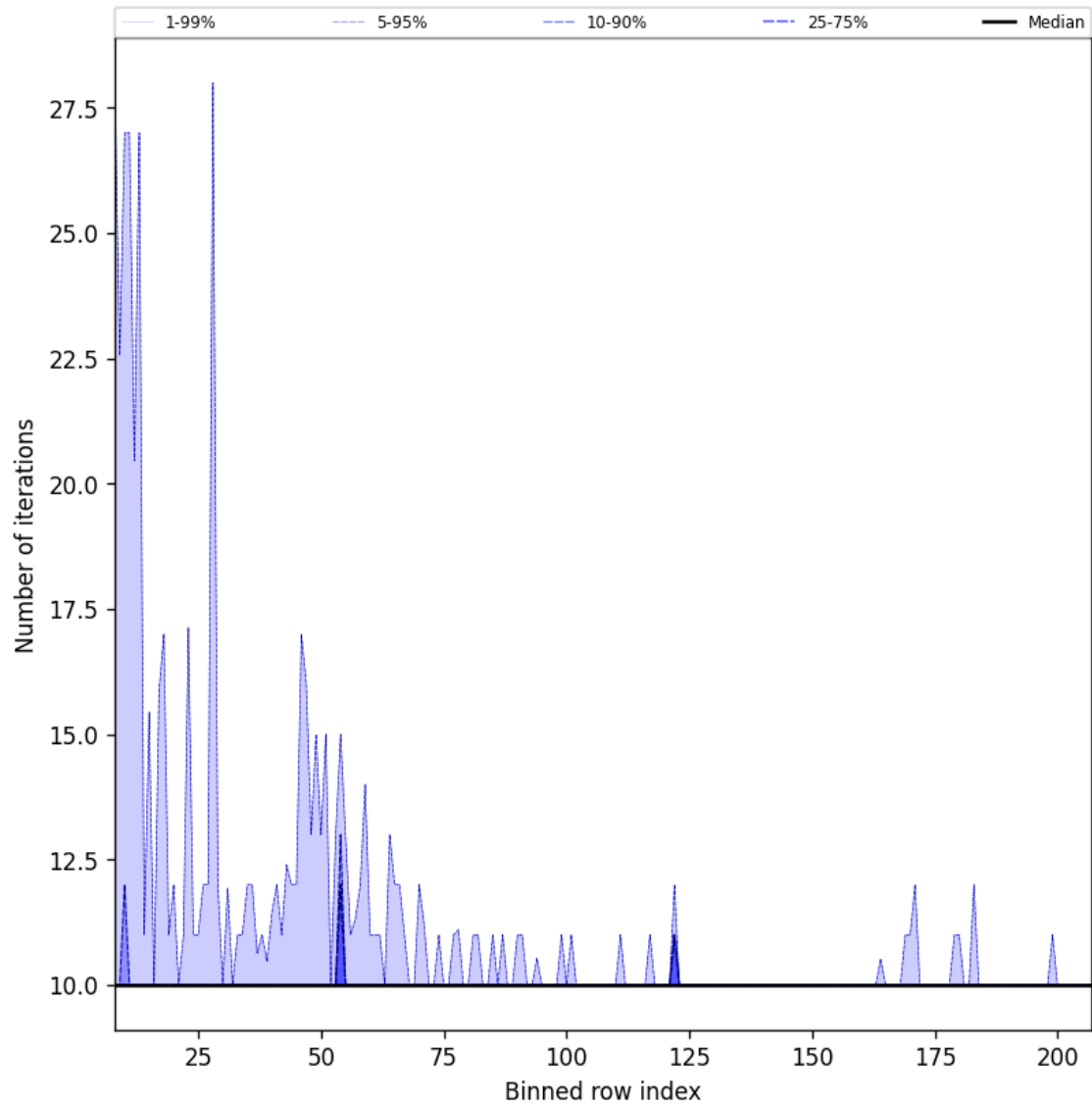
Figure 42: Along track statistics of “Number of iterations” for 2024-11-21 to 2024-11-23
