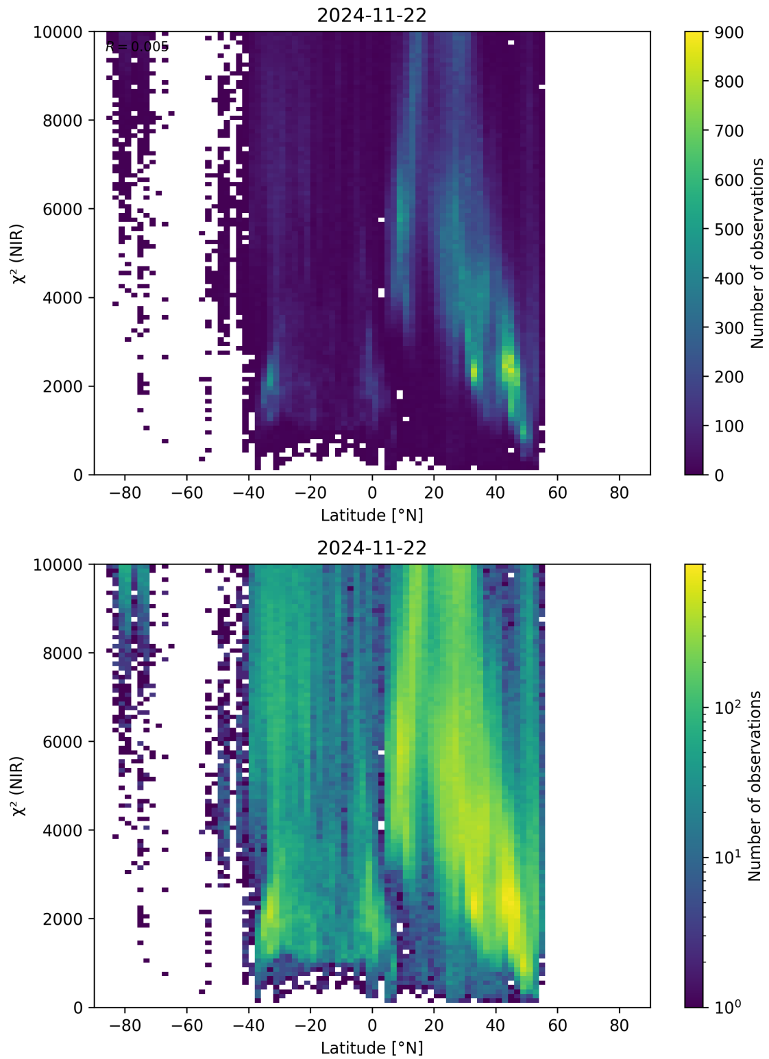
Figure 53: Scatter density plot of “Latitude” against “ \chi^2 (NIR)” for 2024-11-21 to 2024-11-23.
