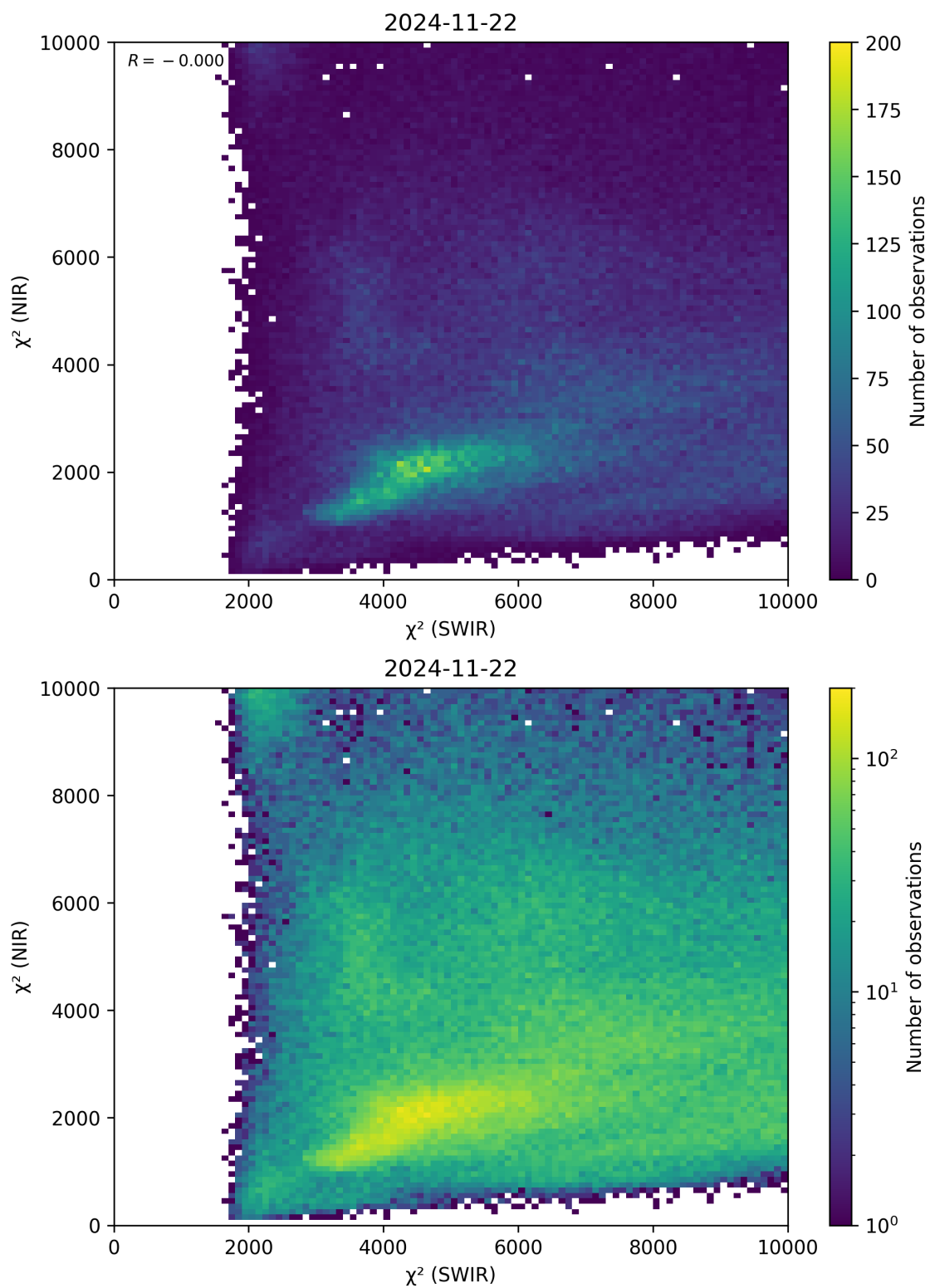
Figure 47: Scatter density plot of “ \chi^2 (SWIR)” against “ \chi^2 (NIR)” for 2024-11-21 to 2024-11-23.
