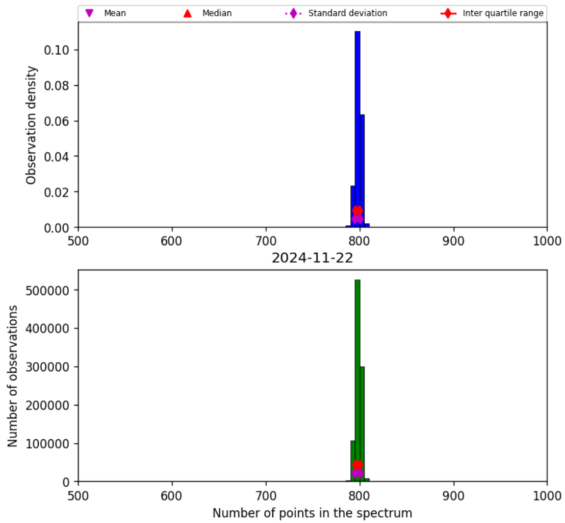
Figure 26: Histogram of “Number of points in the spectrum” for 2024-11-21 to 2024-11-23
