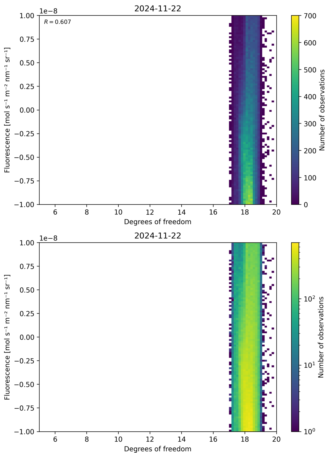
Figure 51: Scatter density plot of “Degrees of freedom” against “Fluorescence” for 2024-11-21 to 2024-11-23.
