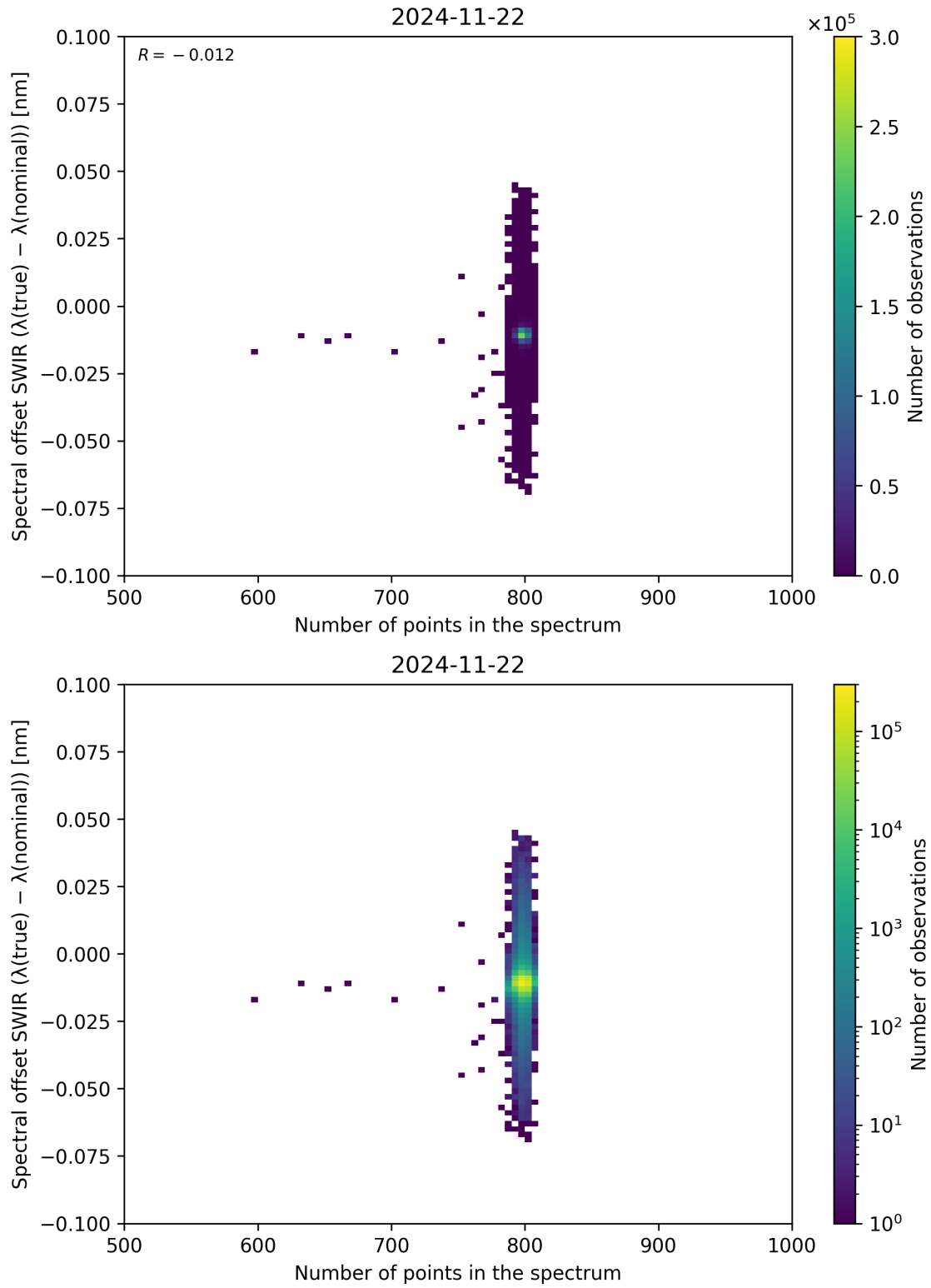
Figure 93: Scatter density plot of “Number of points in the spectrum” against “Spectral offset SWIR ( \lambda_{\text{true}} - \lambda_{\text{nominal}} )” for 2024-11-21 to 2024-11-23.
