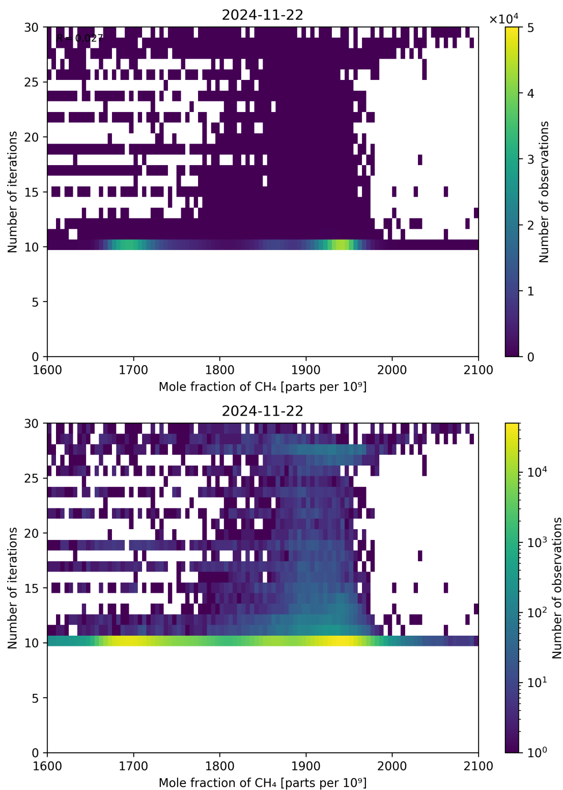
Figure 76: Scatter density plot of “Mole fraction of CH 4 ” against “Number of iterations” for 2024-11-21 to 2024-11-23.
