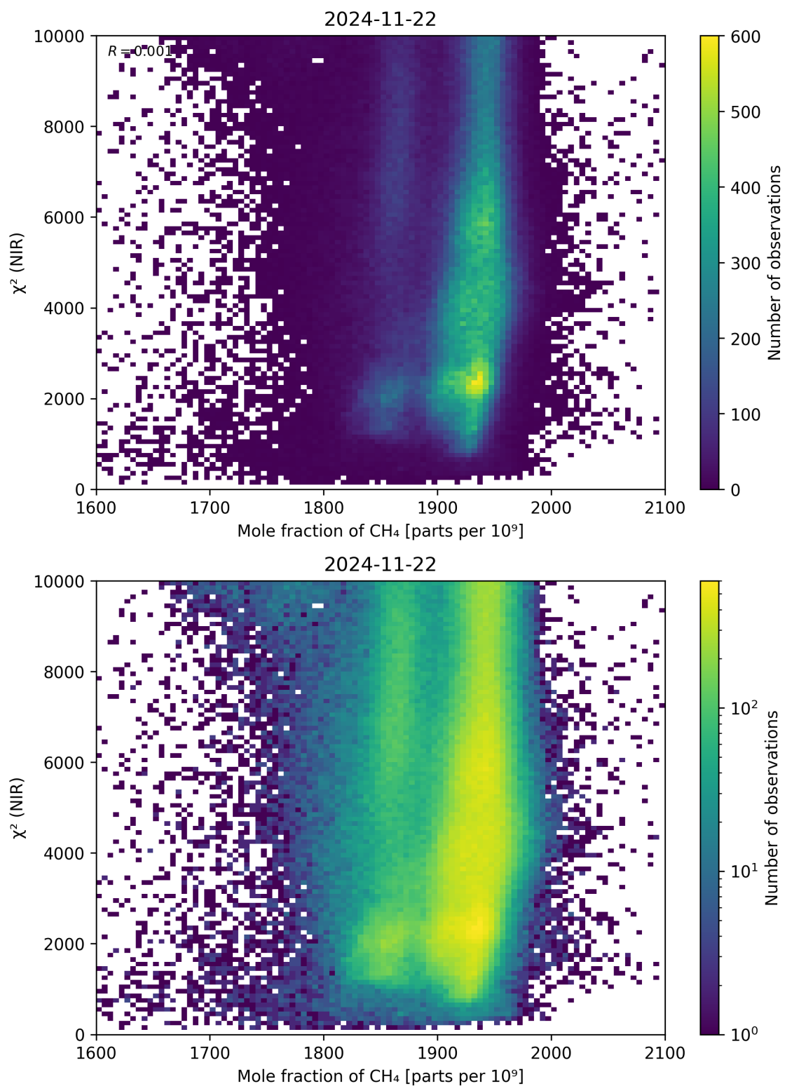
Figure 70: Scatter density plot of “Mole fraction of \text{CH}_4 ” against “ \chi^2 (NIR)” for 2024-11-21 to 2024-11-23.
