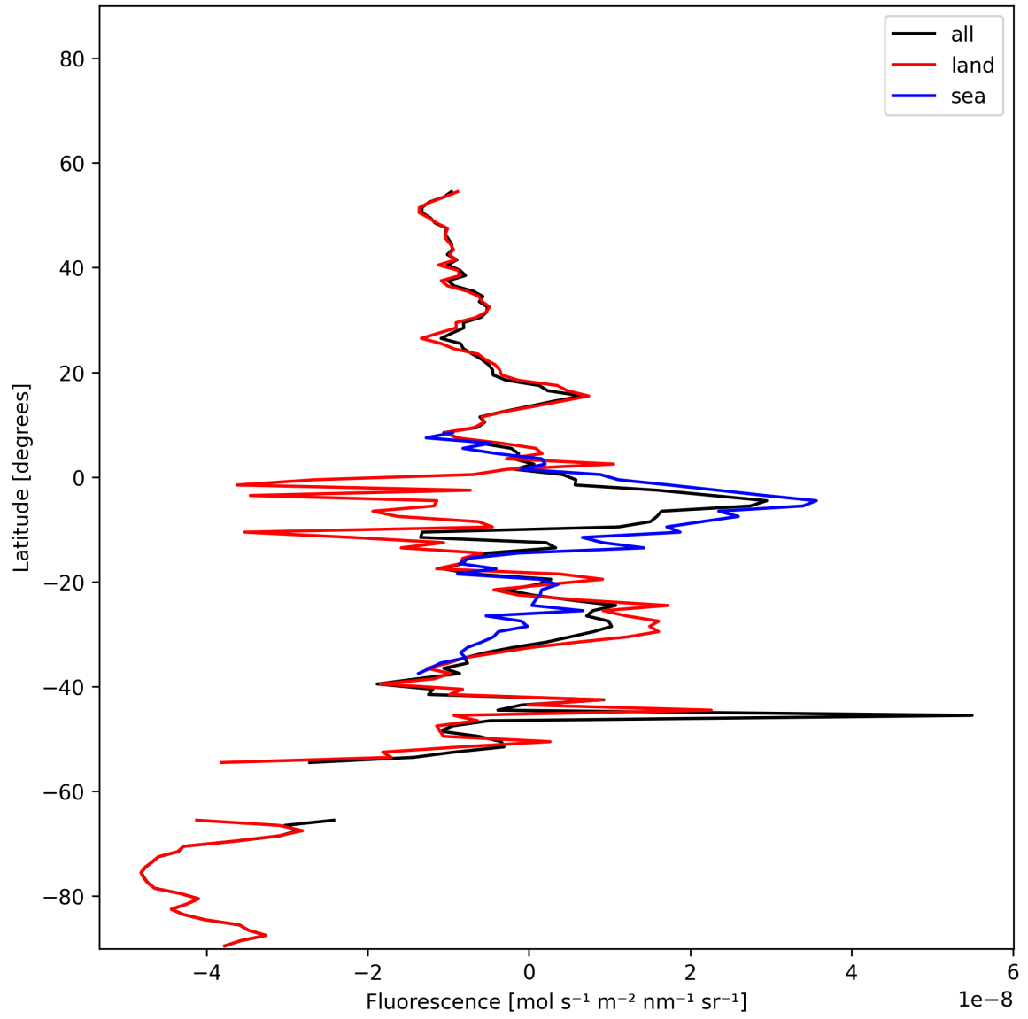
Figure 21: Zonal average of “Fluorescence” for 2024-11-21 to 2024-11-23.
