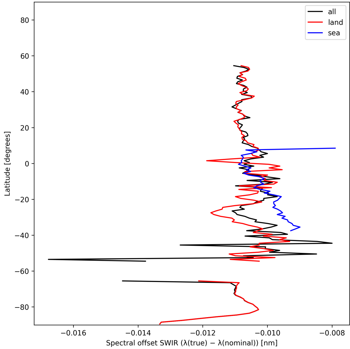
Figure 16: Zonal average of “Spectral offset SWIR ( \lambda_{\text{true}} - \lambda_{\text{nominal}} )” for 2024-11-21 to 2024-11-23.
