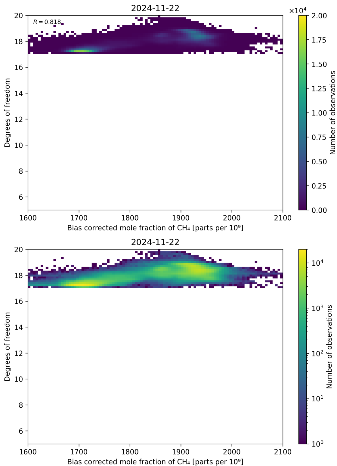
Figure 65: Scatter density plot of “Bias corrected mole fraction of CH 4 ” against “Degrees of freedom” for 2024-11-21 to 2024-11-23.
