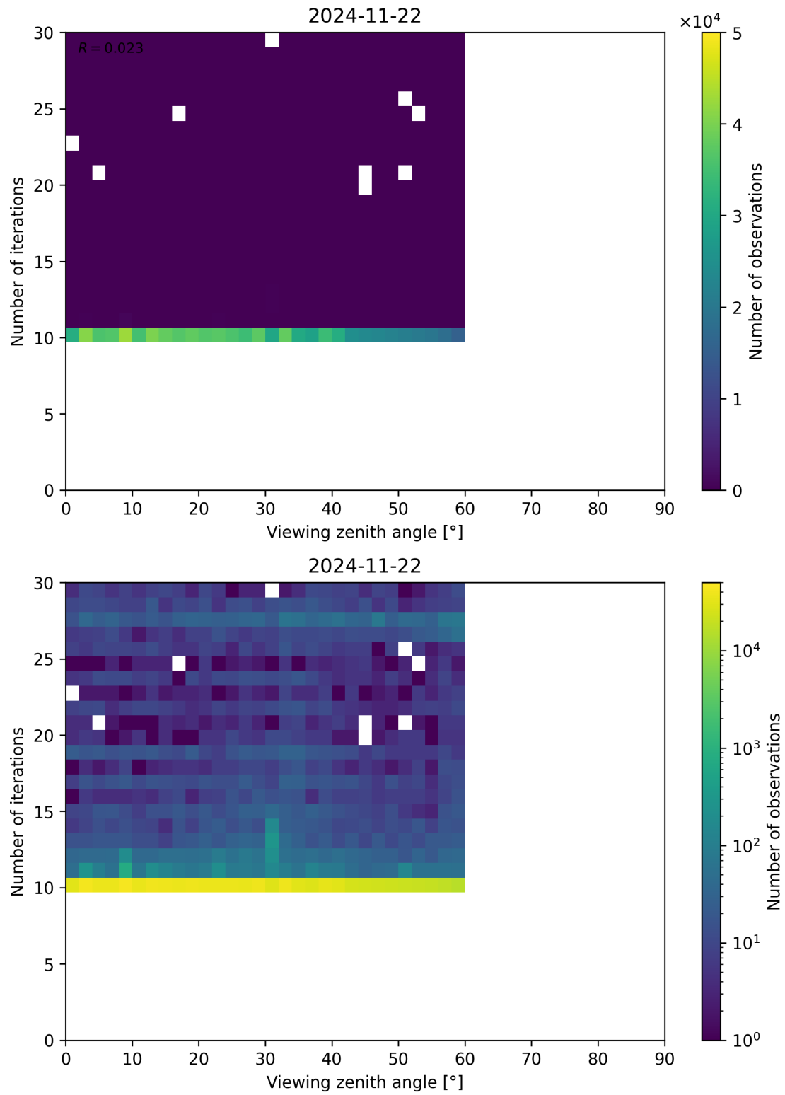
Figure 113: Scatter density plot of “Viewing zenith angle” against “Number of iterations” for 2024-11-21 to 2024-11-23.
