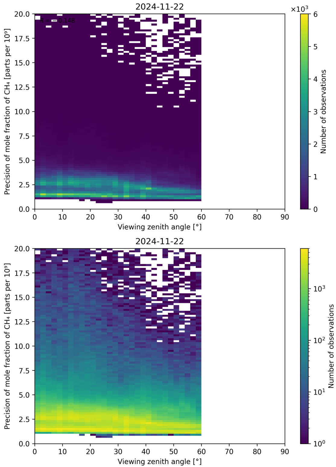
Figure 112: Scatter density plot of “Viewing zenith angle” against “Precision of mole fraction of \text{CH}_4 ” for 2024-11-21 to 2024-11-23.
