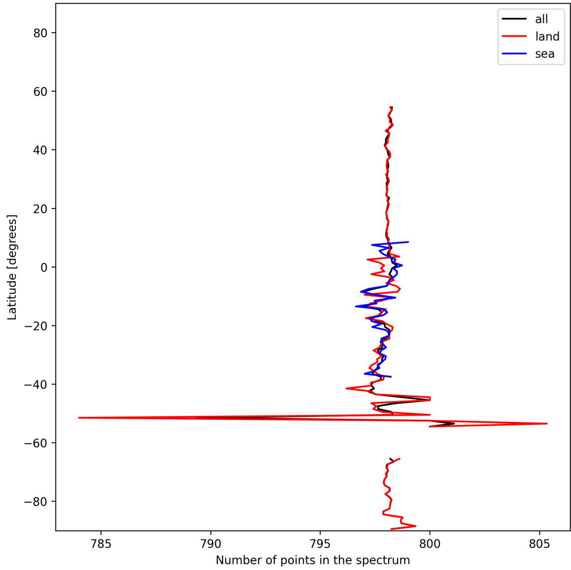
Figure 15: Zonal average of “Number of points in the spectrum” for 2024-11-21 to 2024-11-23.
