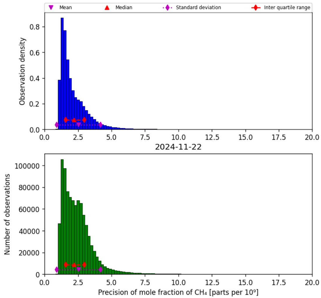
Figure 24: Histogram of “Precision of mole fraction of CH 4 ” for 2024-11-21 to 2024-11-23
