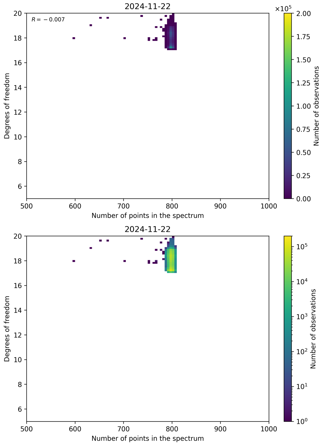
Figure 90: Scatter density plot of “Number of points in the spectrum” against “Degrees of freedom” for 2024-11-21 to 2024-11-23.
