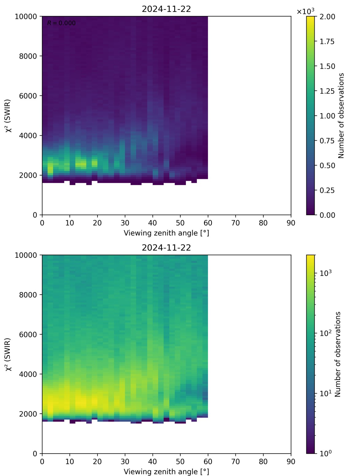
Figure 106: Scatter density plot of “Viewing zenith angle” against “ \chi^2 (SWIR)” for 2024-11-21 to 2024-11-23.
