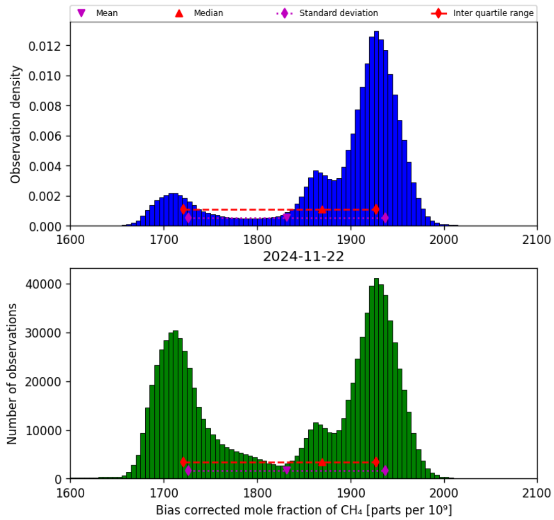
Figure 25: Histogram of “Bias corrected mole fraction of CH 4 ” for 2024-11-21 to 2024-11-23
