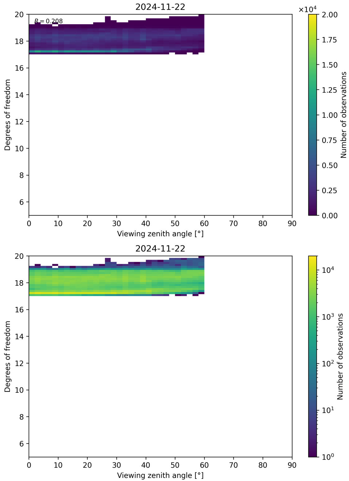
Figure 107: Scatter density plot of “Viewing zenith angle” against “Degrees of freedom” for 2024-11-21 to 2024-11-23.
