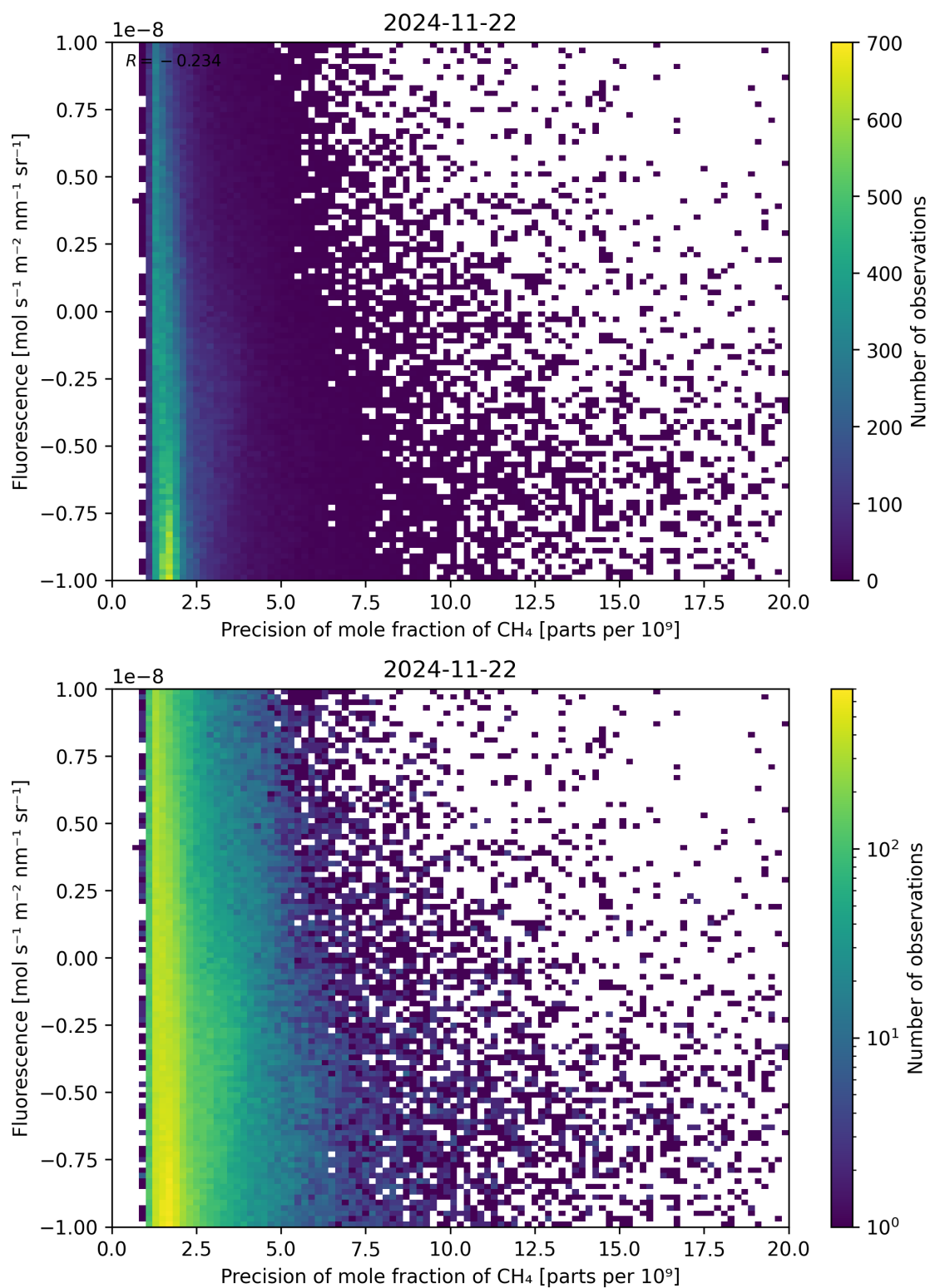
Figure 81: Scatter density plot of “Precision of mole fraction of \text{CH}_4 ” against “Fluorescence” for 2024-11-21 to 2024-11-23.
