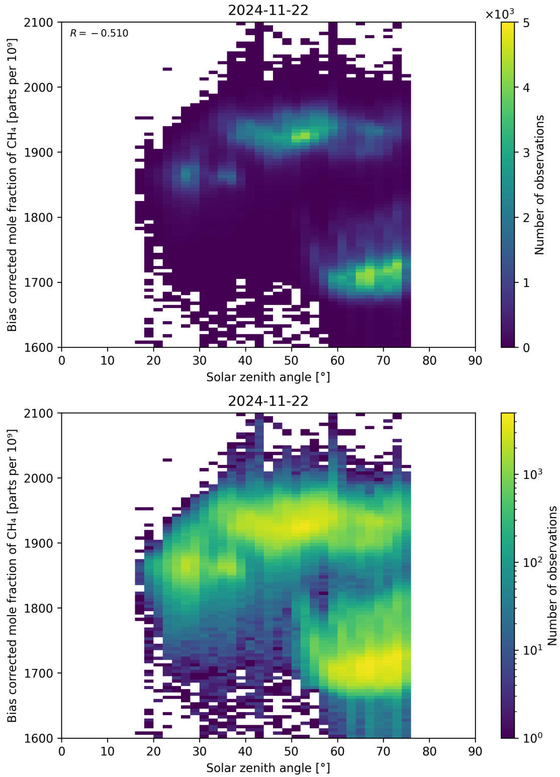
Figure 100: Scatter density plot of “Solar zenith angle” against “Bias corrected mole fraction of CH 4 ” for 2024-11-21 to 2024-11-23.
