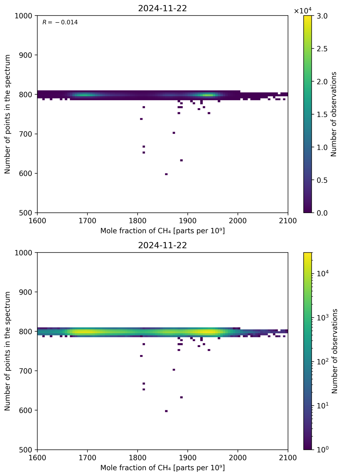
Figure 77: Scatter density plot of “Mole fraction of CH 4 ” against “Number of points in the spectrum” for 2024-11-21 to 2024-11-23.
