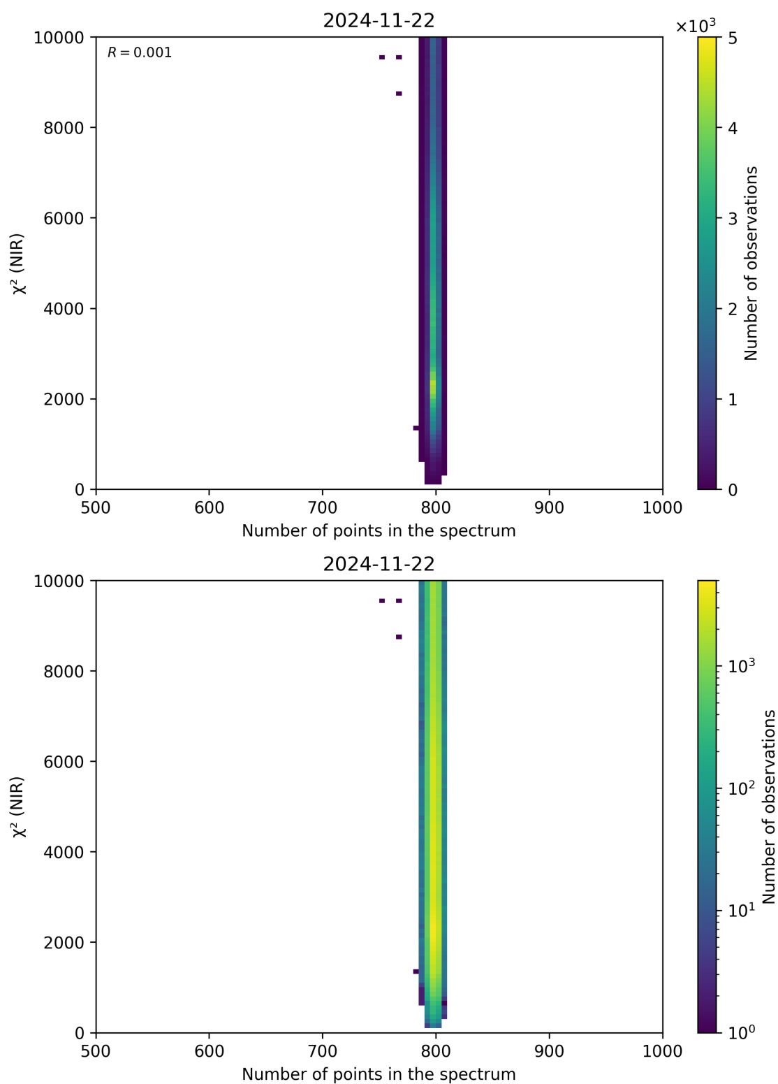
Figure 88: Scatter density plot of “Number of points in the spectrum” against “ \chi^2 (NIR)” for 2024-11-21 to 2024-11-23.
