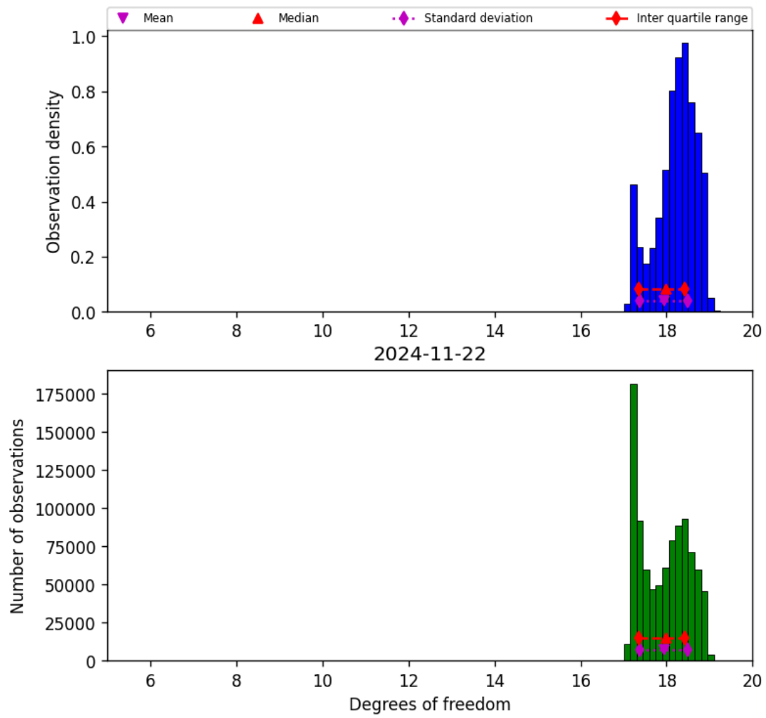
Figure 30: Histogram of “Degrees of freedom” for 2024-11-21 to 2024-11-23
