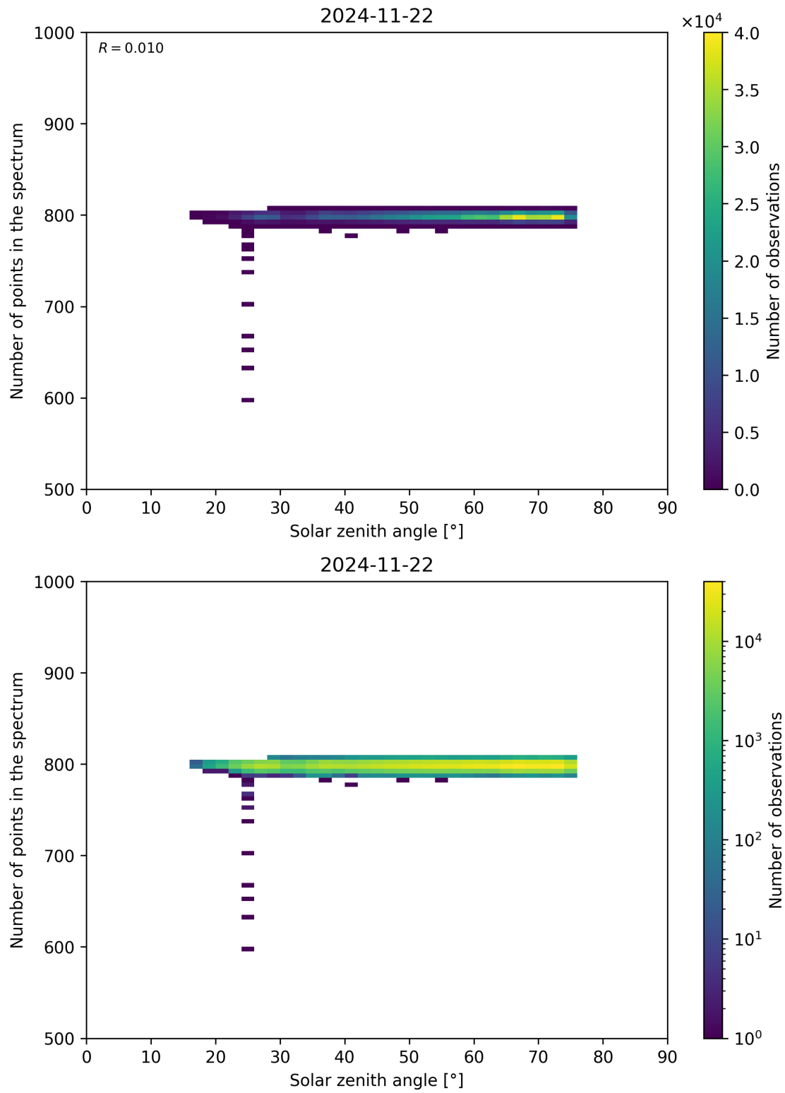
Figure 103: Scatter density plot of “Solar zenith angle” against “Number of points in the spectrum” for 2024-11-21 to 2024-11-23.
