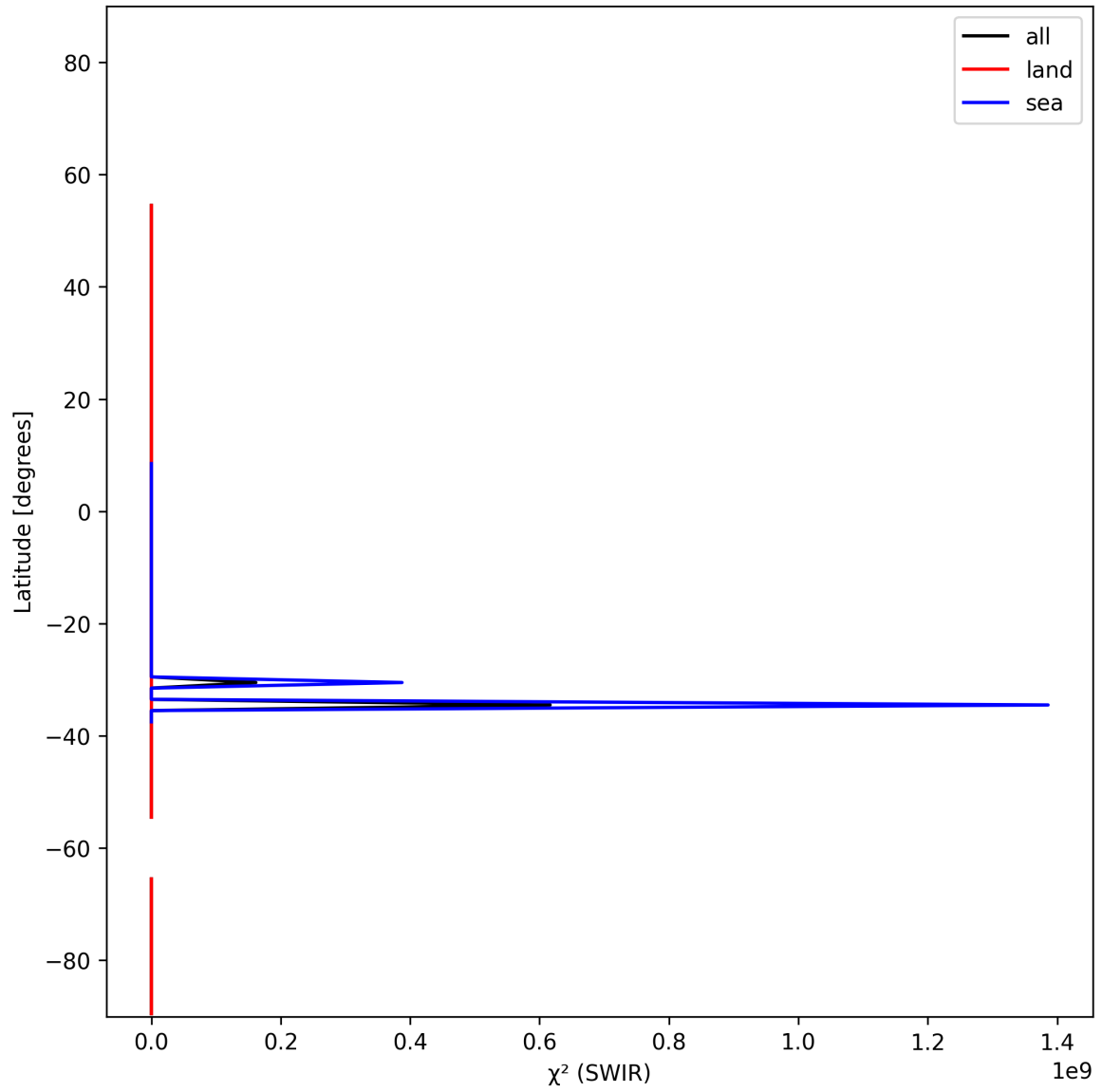
Figure 17: Zonal average of “ \chi^2 (SWIR)” for 2024-11-21 to 2024-11-23.
