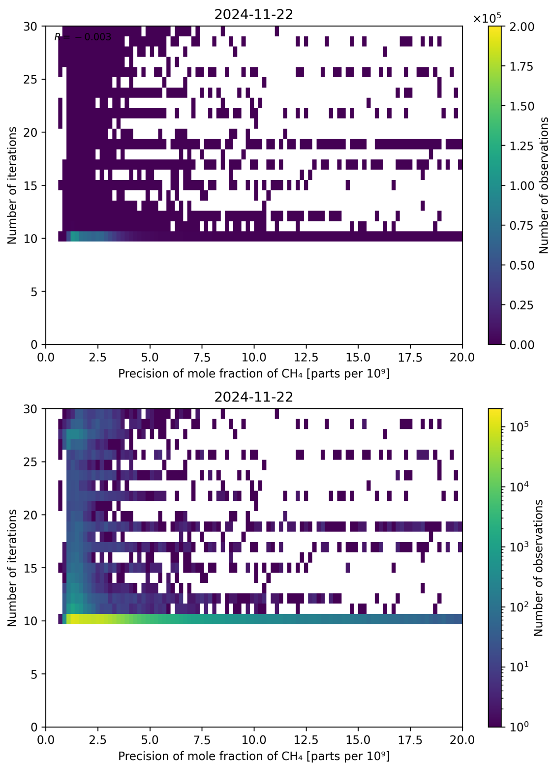
Figure 83: Scatter density plot of “Precision of mole fraction of CH 4 ” against “Number of iterations” for 2024-11-21 to 2024-11-23.
