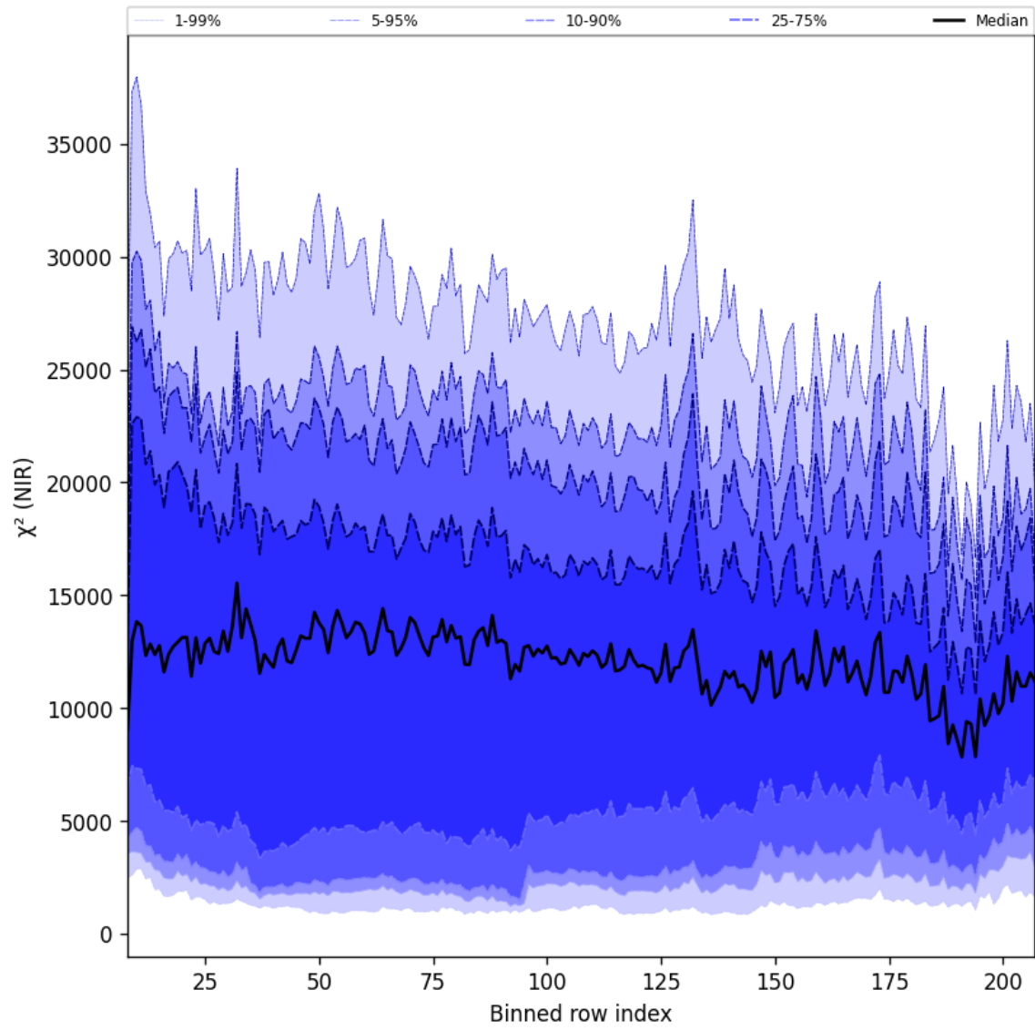
Figure 40: Along track statistics of “ \chi^2 (NIR)” for 2024-11-21 to 2024-11-23
