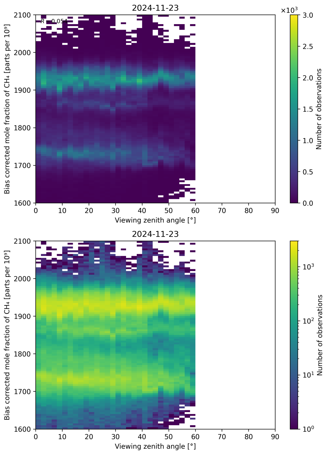
Figure 111: Scatter density plot of “Viewing zenith angle” against “Bias corrected mole fraction of CH 4 ” for 2024-11-22 to 2024-11-24.
