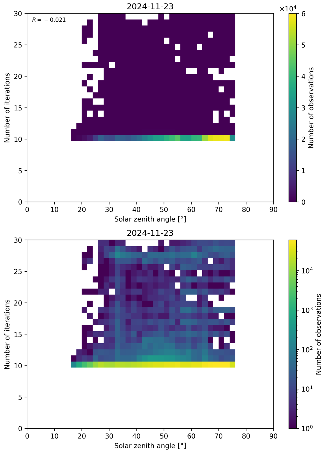
Figure 102: Scatter density plot of “Solar zenith angle” against “Number of iterations” for 2024-11-22 to 2024-11-24.
