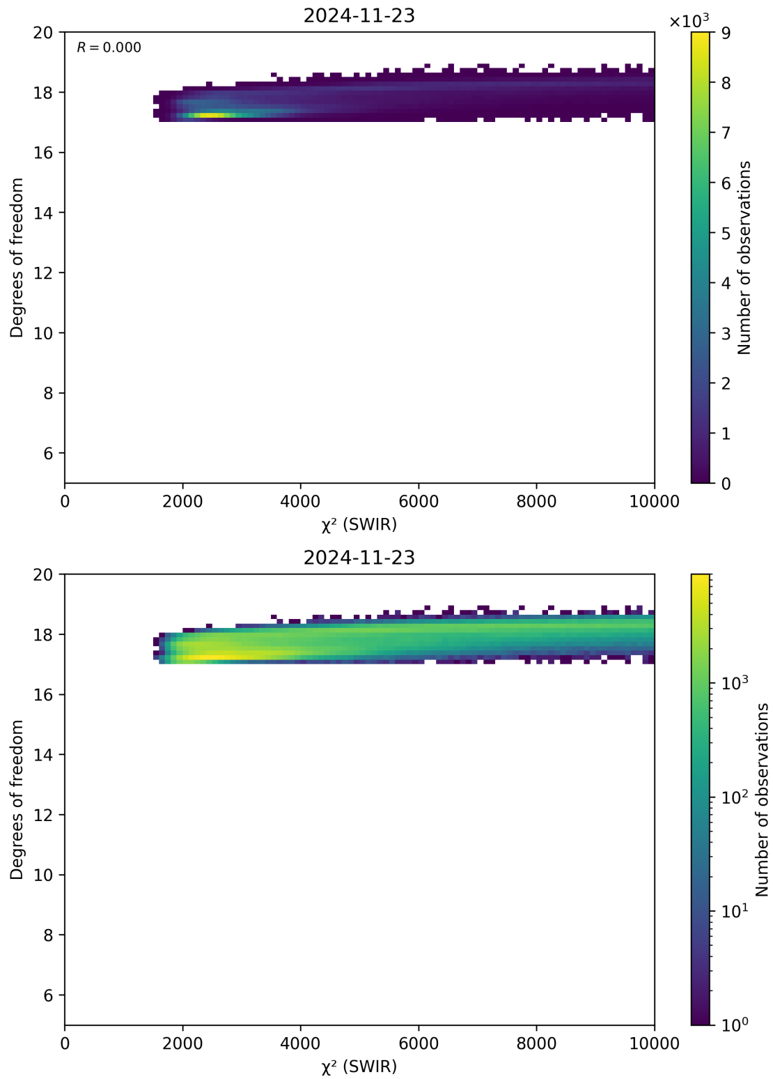
Figure 48: Scatter density plot of “ \chi^2 (SWIR)” against “Degrees of freedom” for 2024-11-22 to 2024-11-24.
