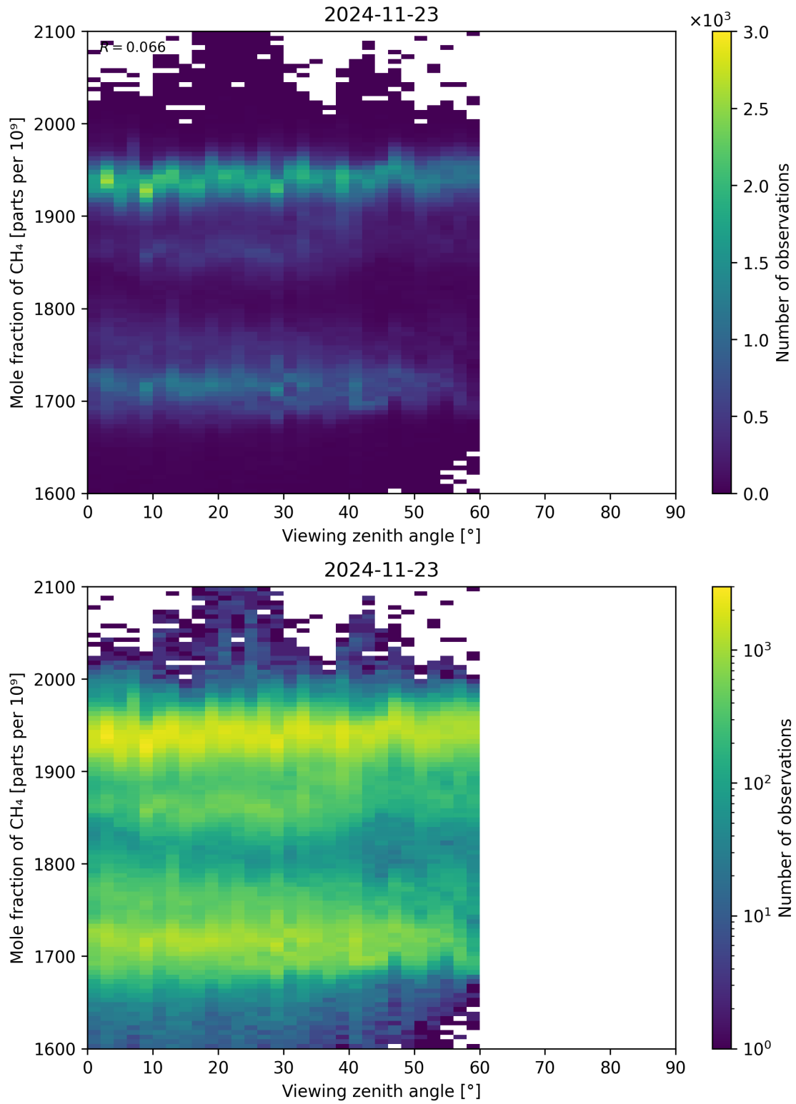
Figure 110: Scatter density plot of “Viewing zenith angle” against “Mole fraction of CH 4 ” for 2024-11-22 to 2024-11-24.
