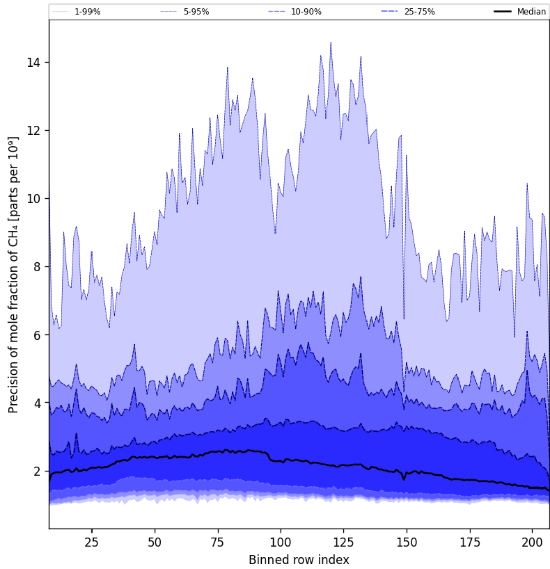
Figure 35: Along track statistics of “Precision of mole fraction of CH 4 ” for 2024-11-22 to 2024-11-24
