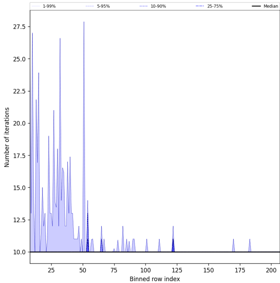
Figure 42: Along track statistics of “Number of iterations” for 2024-11-22 to 2024-11-24
