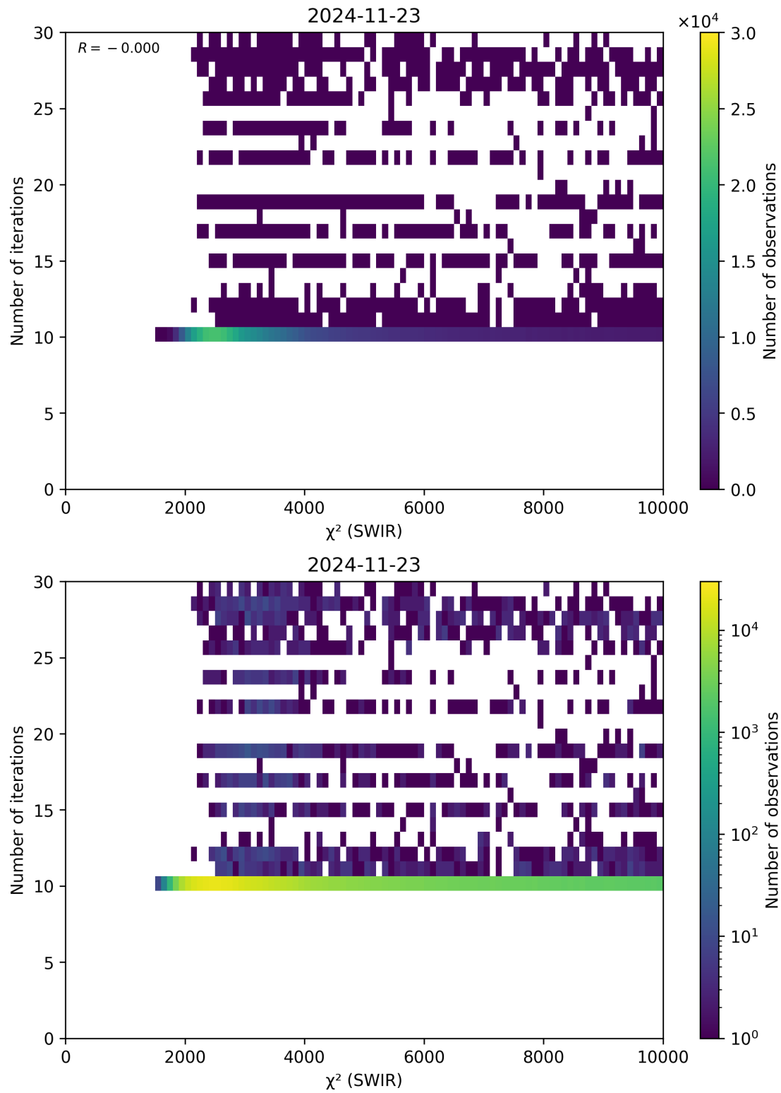
Figure 50: Scatter density plot of “ \chi^2 (SWIR)” against “Number of iterations” for 2024-11-22 to 2024-11-24.
