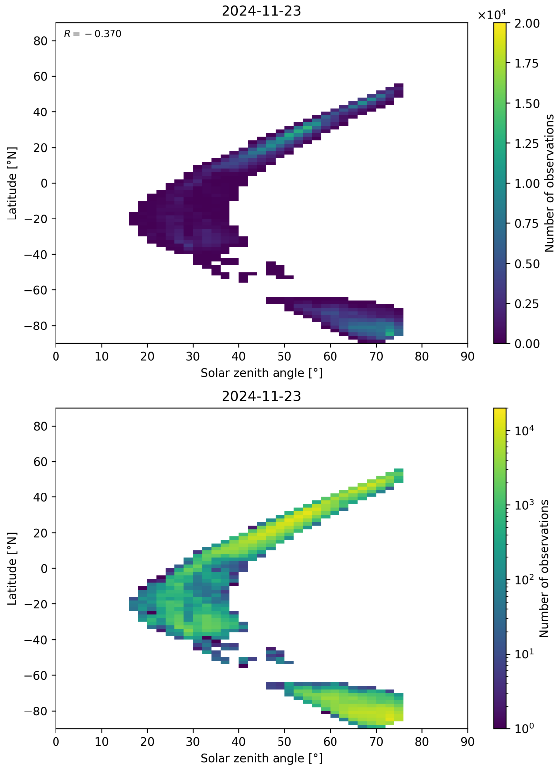
Figure 98: Scatter density plot of “Solar zenith angle” against “Latitude” for 2024-11-22 to 2024-11-24.
