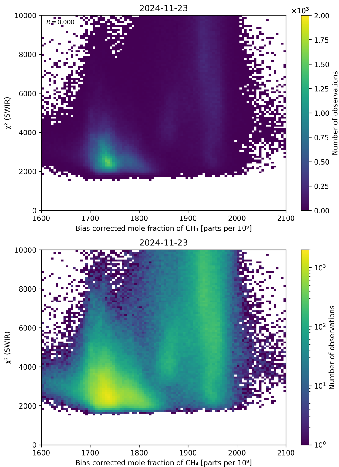
Figure 64: Scatter density plot of “Bias corrected mole fraction of \text{CH}_4 ” against “ \chi^2 (SWIR)” for 2024-11-22 to 2024-11-24.
