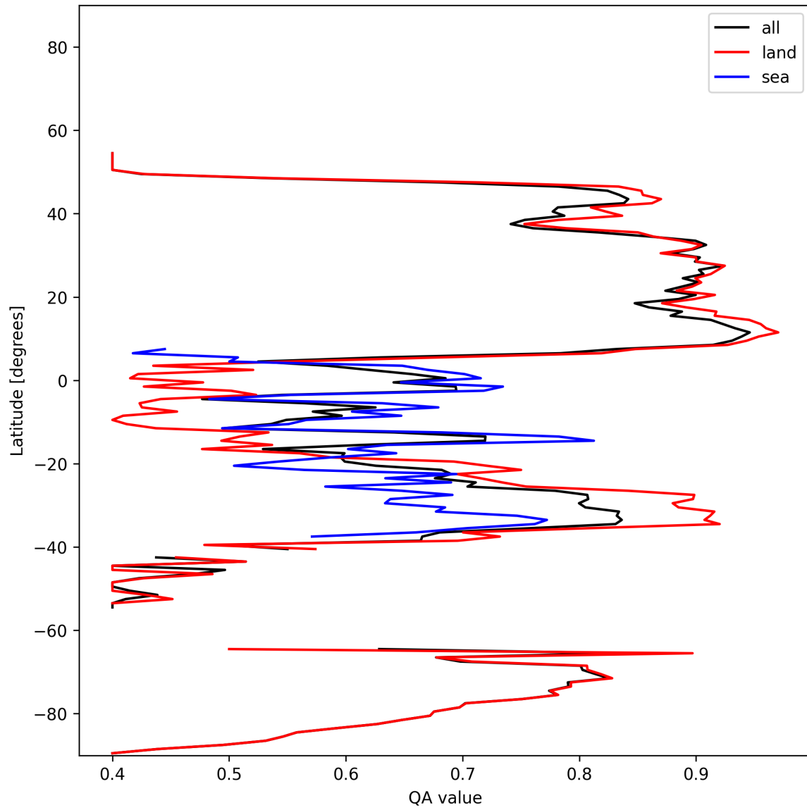
Figure 11: Zonal average of “QA value” for 2024-11-22 to 2024-11-24.
