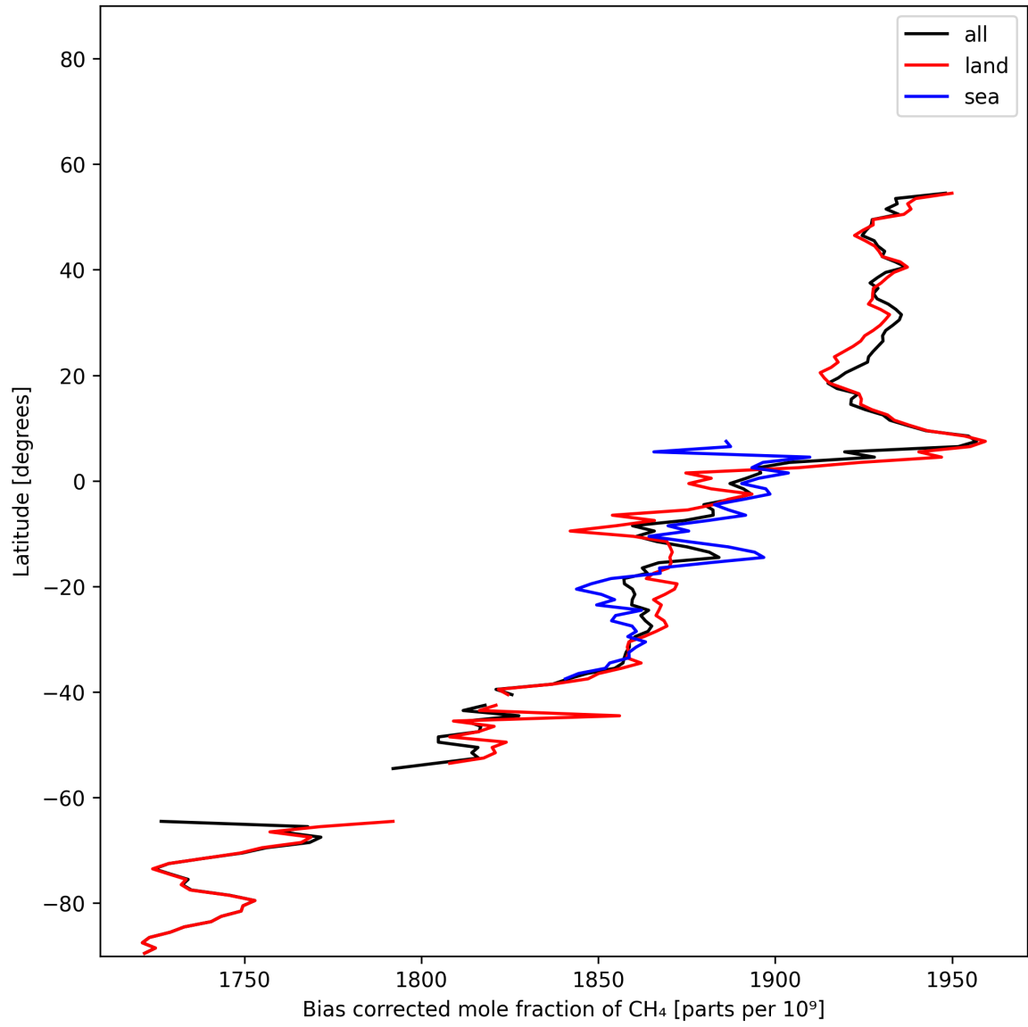
Figure 14: Zonal average of “Bias corrected mole fraction of CH 4 ” for 2024-11-22 to 2024-11-24.
