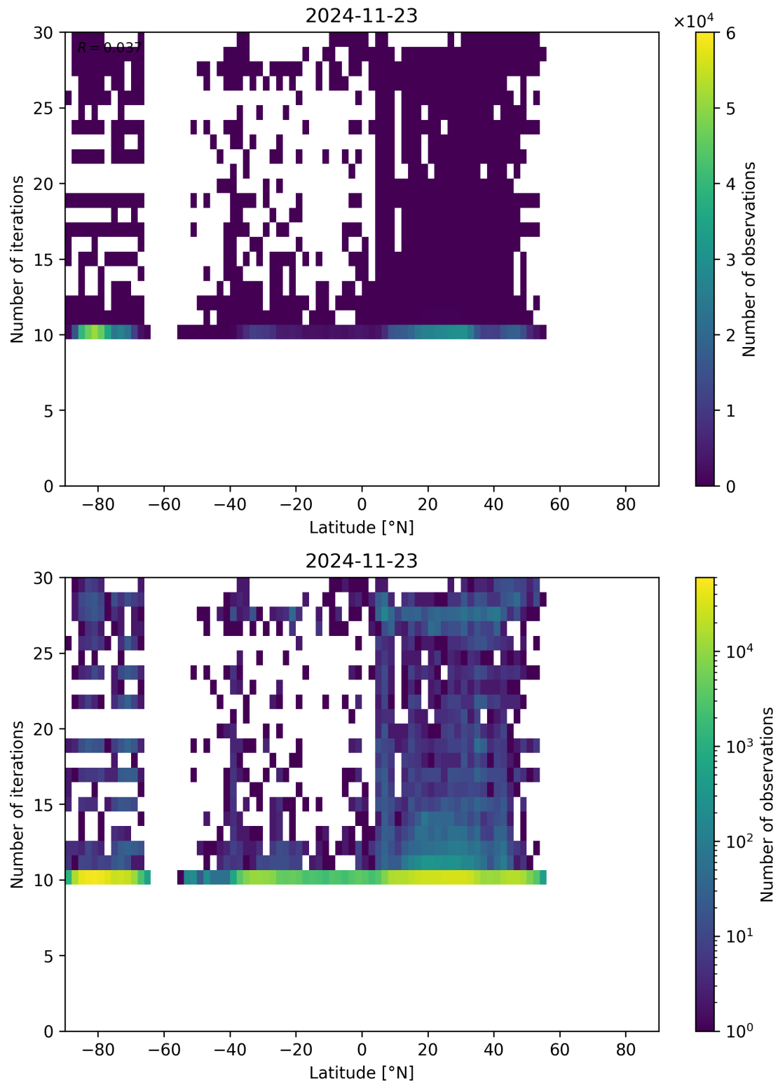
Figure 60: Scatter density plot of “Latitude” against “Number of iterations” for 2024-11-22 to 2024-11-24.
