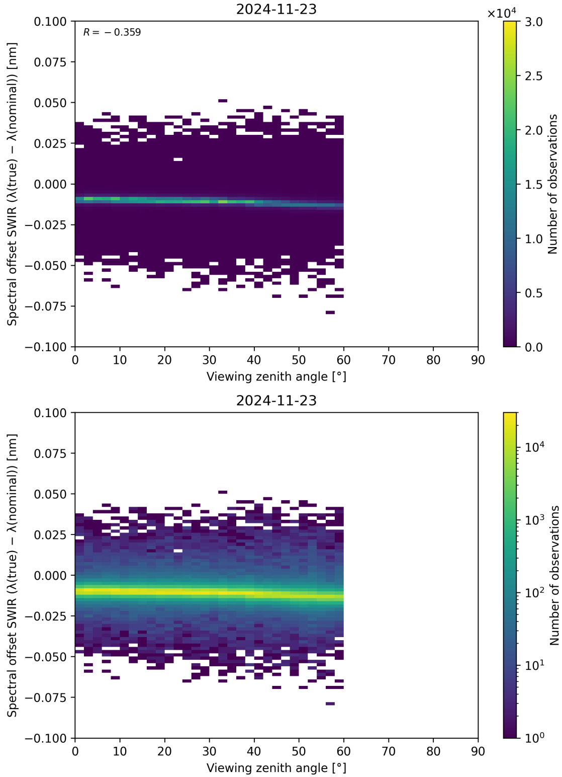
Figure 116: Scatter density plot of “Viewing zenith angle” against “Spectral offset SWIR ( \lambda_{\text{true}} - \lambda_{\text{nominal}} )” for 2024-11-22 to 2024-11-24.
