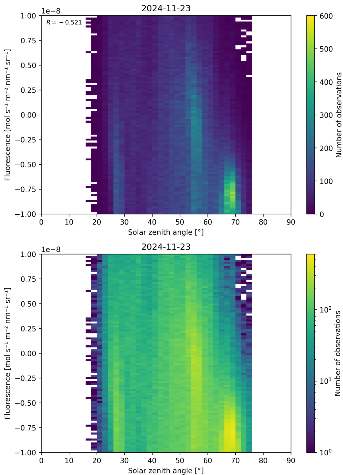
Figure 97: Scatter density plot of “Solar zenith angle” against “Fluorescence” for 2024-11-22 to 2024-11-24.
