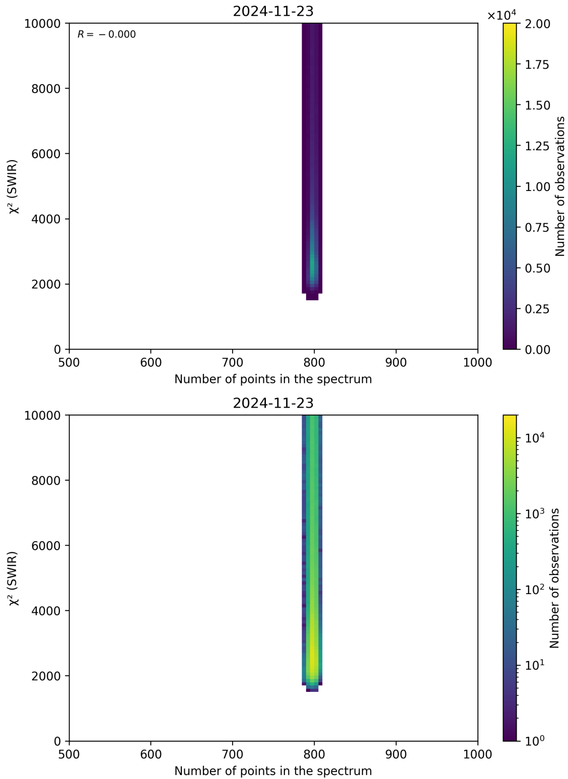
Figure 89: Scatter density plot of “Number of points in the spectrum” against “ \chi^2 (SWIR)” for 2024-11-22 to 2024-11-24.
