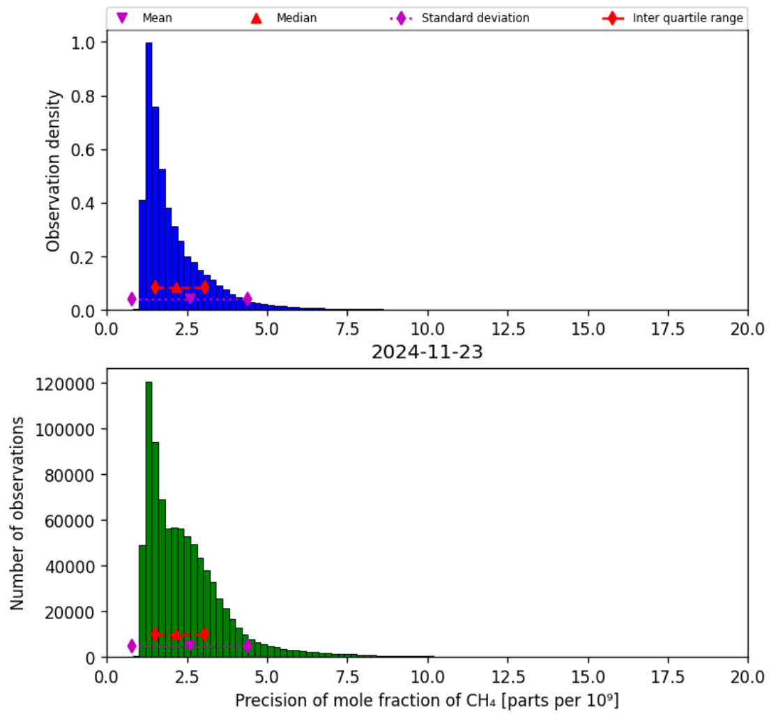
Figure 24: Histogram of “Precision of mole fraction of CH 4 ” for 2024-11-22 to 2024-11-24
