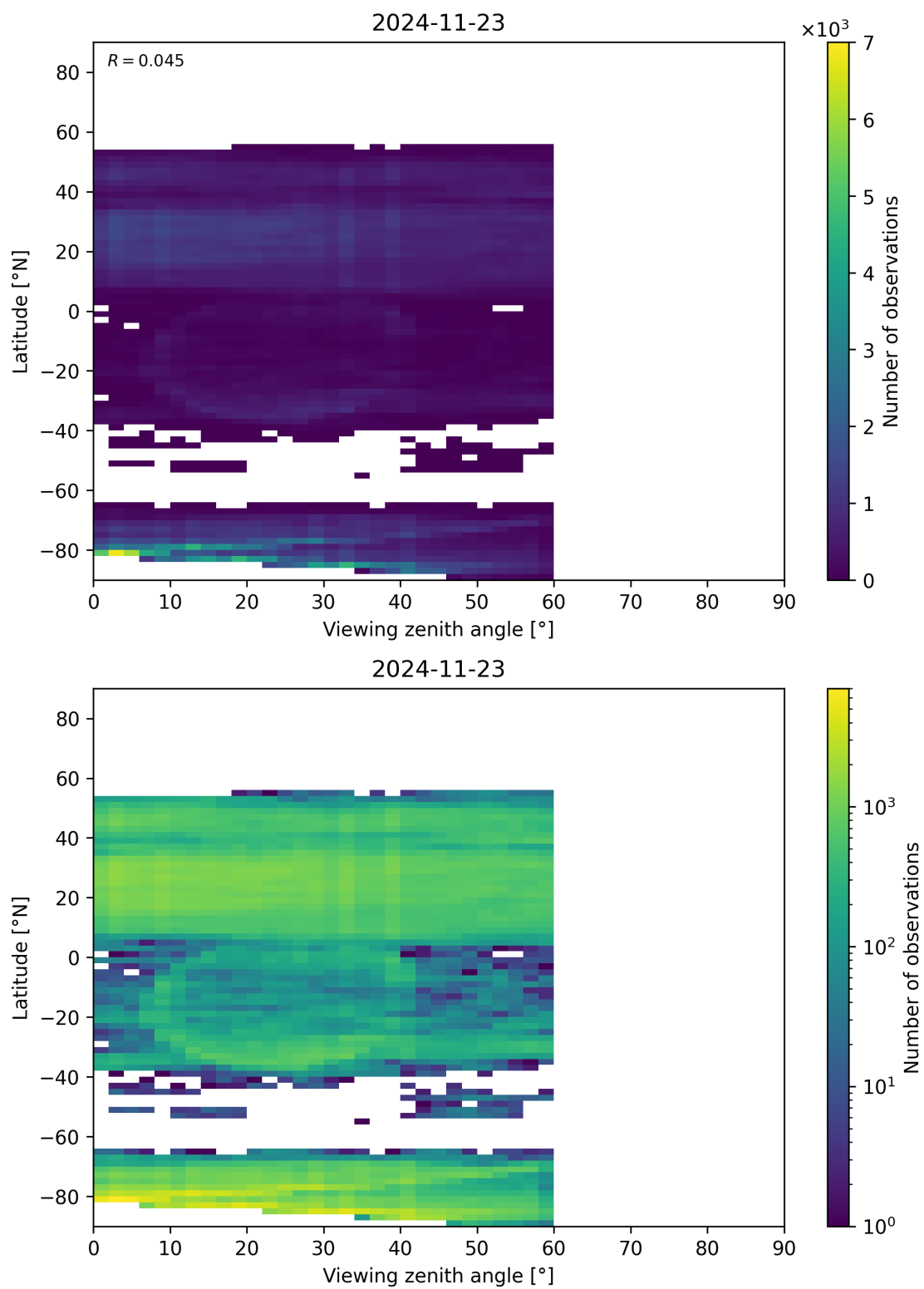
Figure 109: Scatter density plot of “Viewing zenith angle” against “Latitude” for 2024-11-22 to 2024-11-24.
