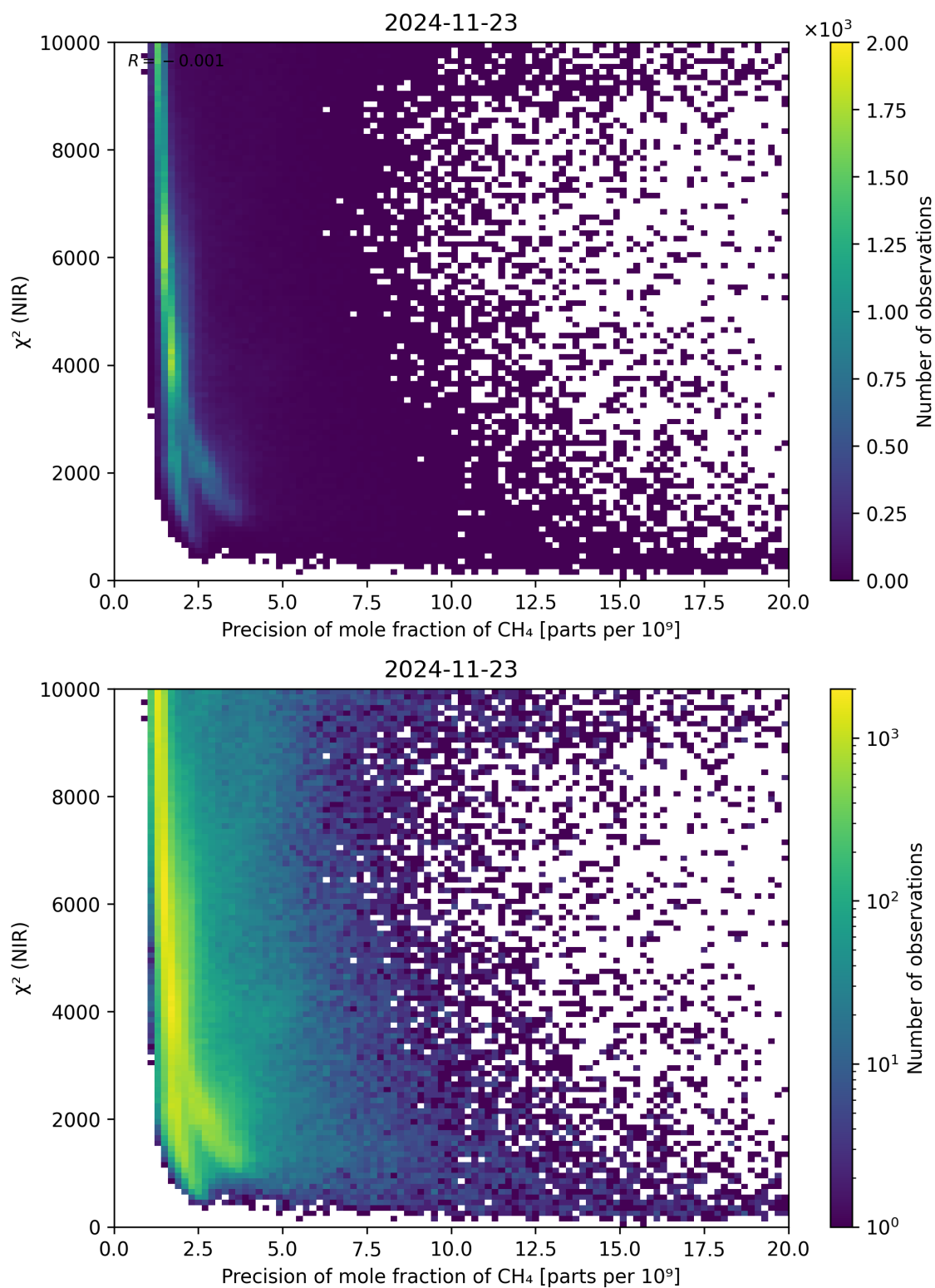
Figure 78: Scatter density plot of “Precision of mole fraction of CH 4 ” against “ \chi^2 (NIR)” for 2024-11-22 to 2024-11-24.
