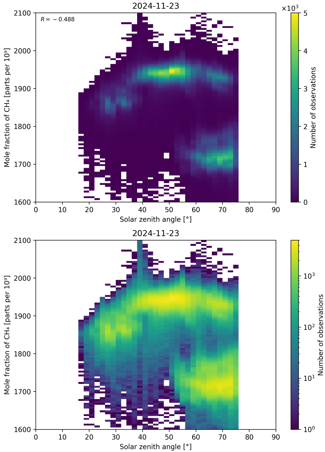
Figure 99: Scatter density plot of “Solar zenith angle” against “Mole fraction of CH 4 ” for 2024-11-22 to 2024-11-24.
