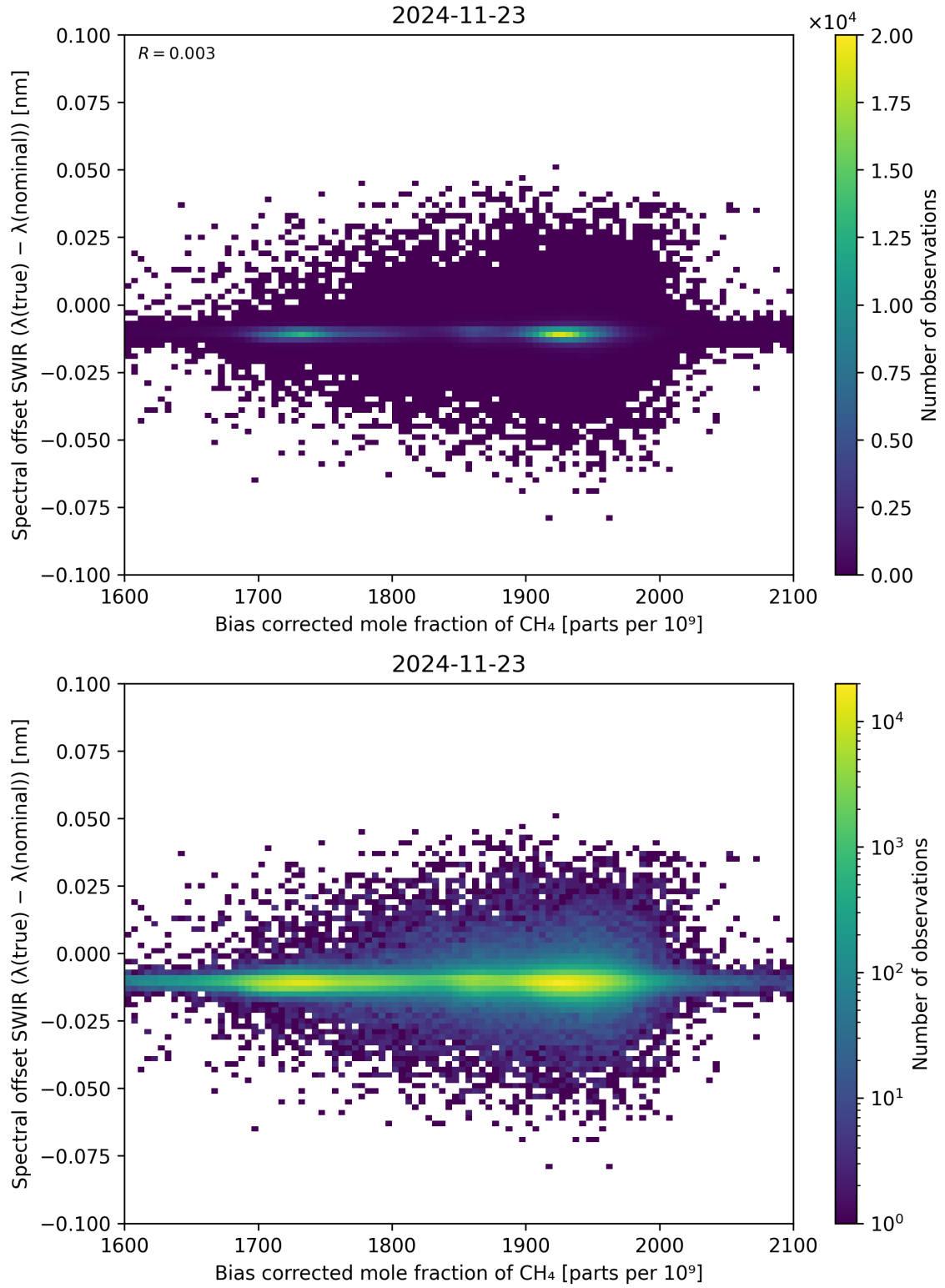
Figure 69: Scatter density plot of “Bias corrected mole fraction of \text{CH}_4 ” against “Spectral offset SWIR ( \lambda_{\text{true}} - \lambda_{\text{nominal}} )” for 2024-11-22 to 2024-11-24.
