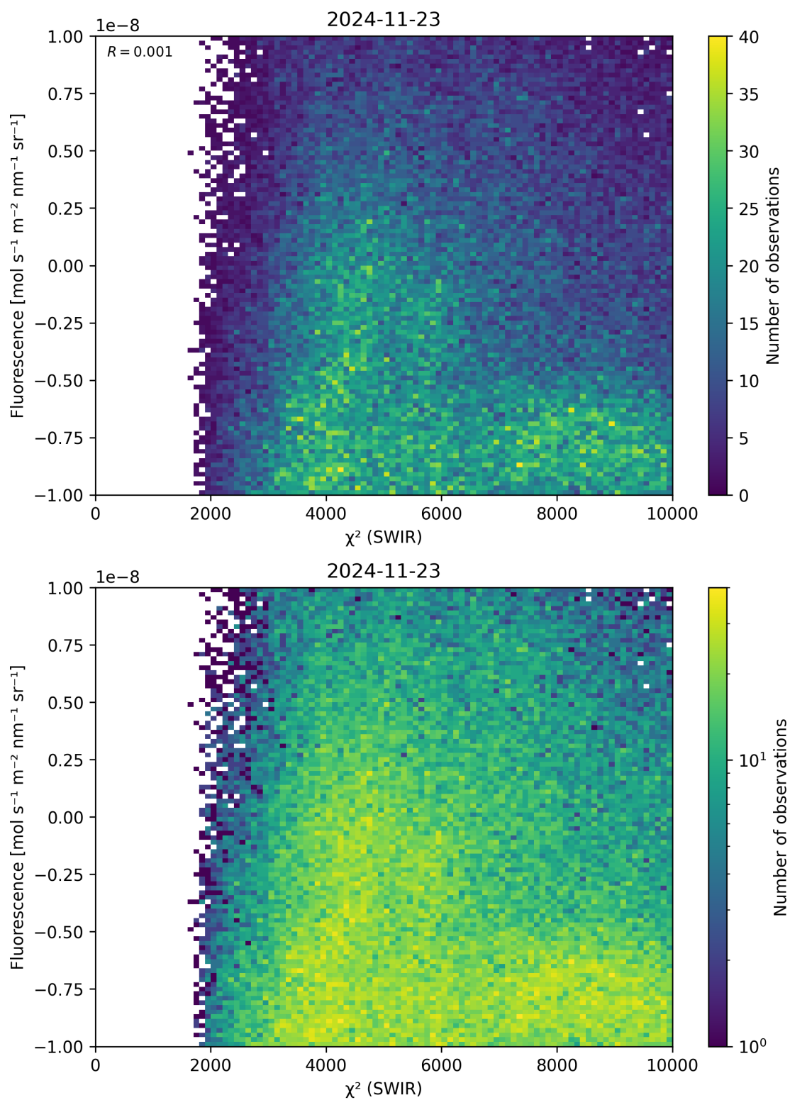
Figure 49: Scatter density plot of “ \chi^2 (SWIR)” against “Fluorescence” for 2024-11-22 to 2024-11-24.
