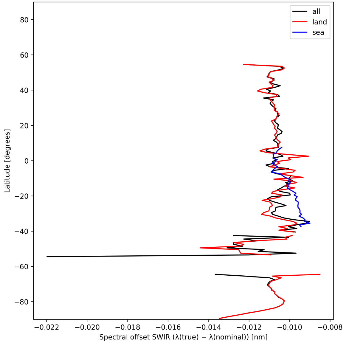
Figure 16: Zonal average of “Spectral offset SWIR ( \lambda_{\text{true}} - \lambda_{\text{nominal}} )” for 2024-11-22 to 2024-11-24.
