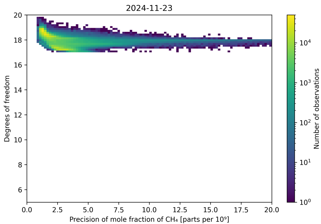
Figure 80: Scatter density plot of “Precision of mole fraction of CH 4 ” against “Degrees of freedom” for 2024-11-22 to 2024-11-24.
