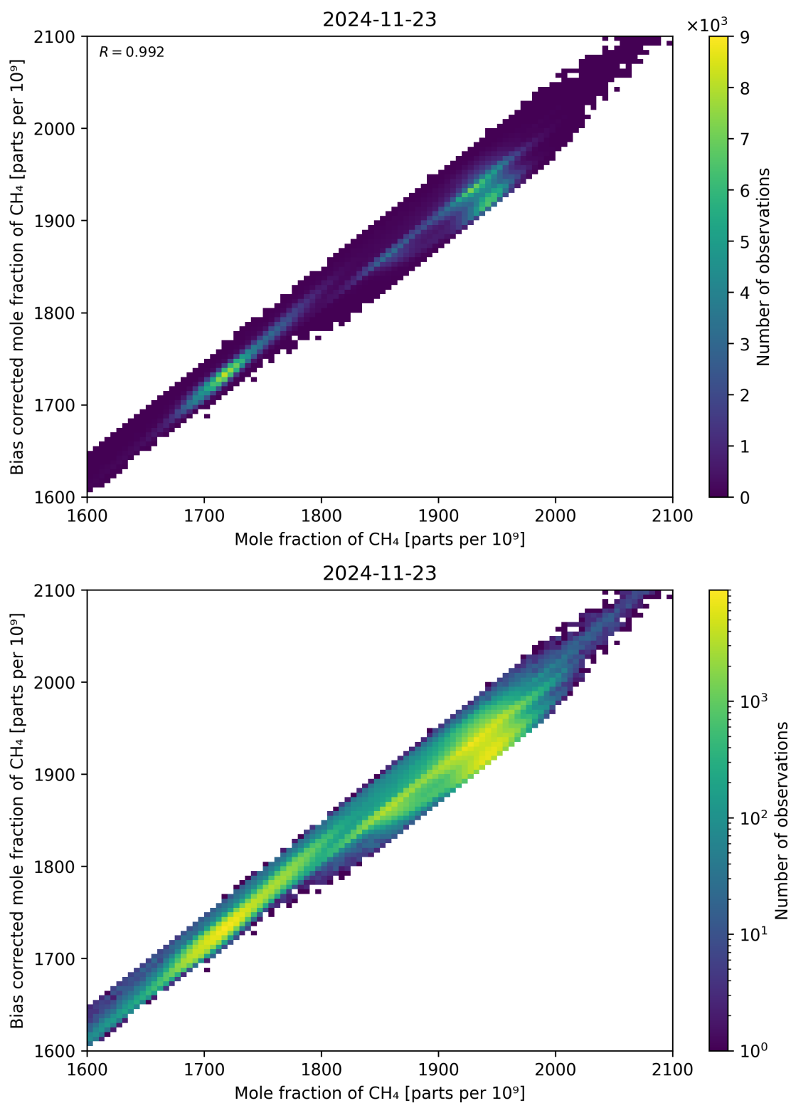
Figure 74: Scatter density plot of “Mole fraction of CH 4 ” against “Bias corrected mole fraction of CH 4 ” for 2024-11-22 to 2024-11-24.
