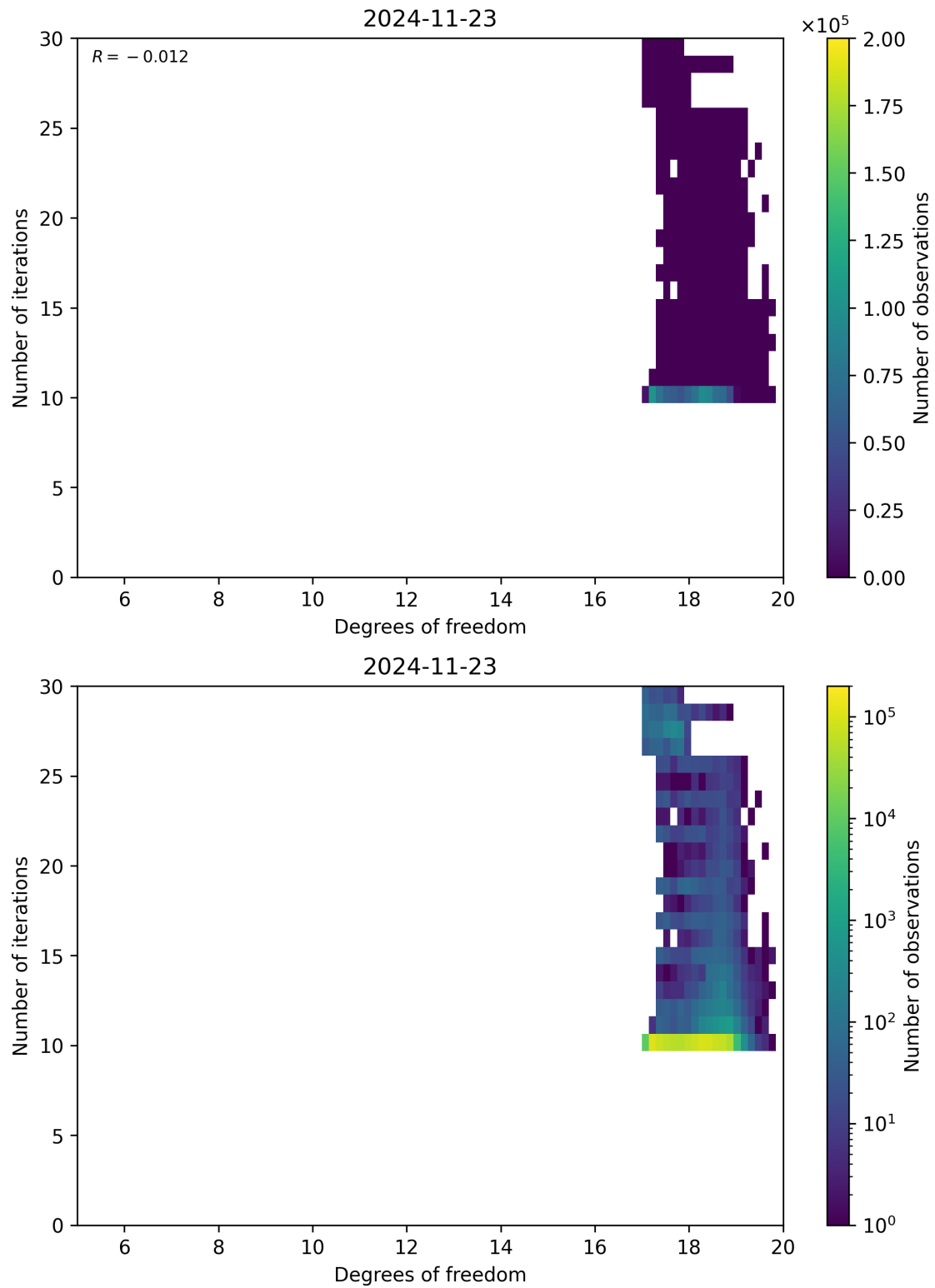
Figure 52: Scatter density plot of “Degrees of freedom” against “Number of iterations” for 2024-11-22 to 2024-11-24.
