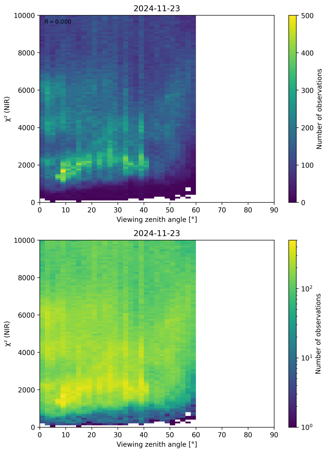
Figure 105: Scatter density plot of “Viewing zenith angle” against “ \chi^2 (NIR)” for 2024-11-22 to 2024-11-24.
