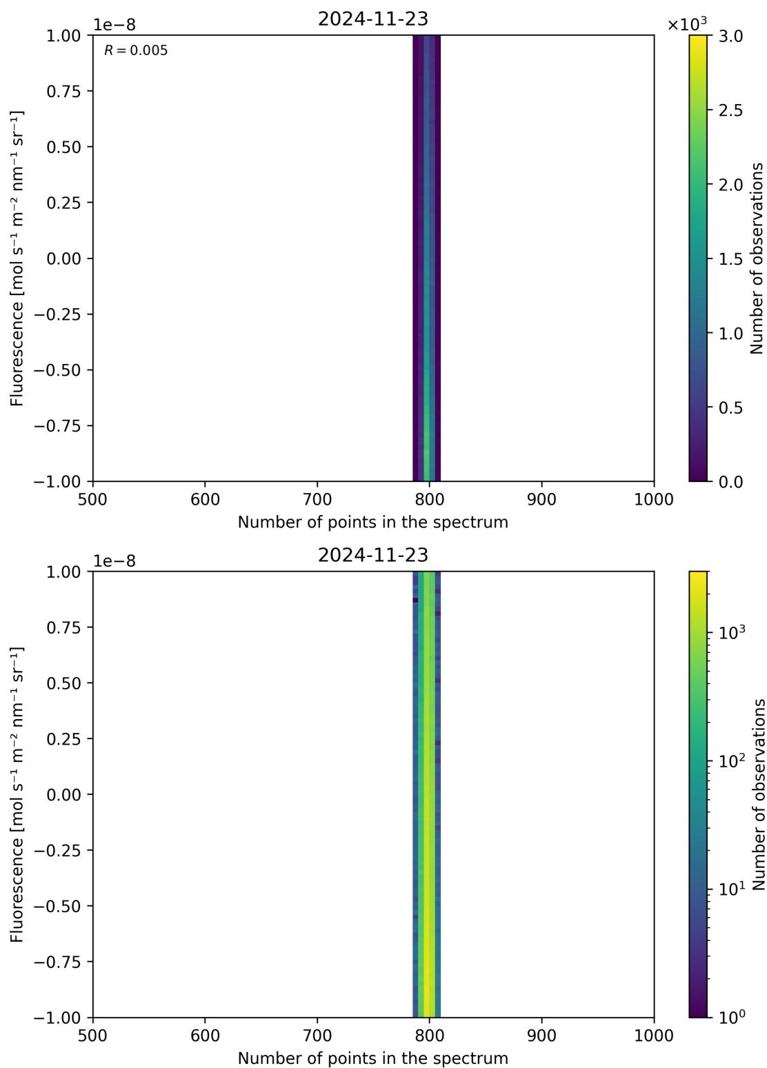
Figure 91: Scatter density plot of “Number of points in the spectrum” against “Fluorescence” for 2024-11-22 to 2024-11-24.
