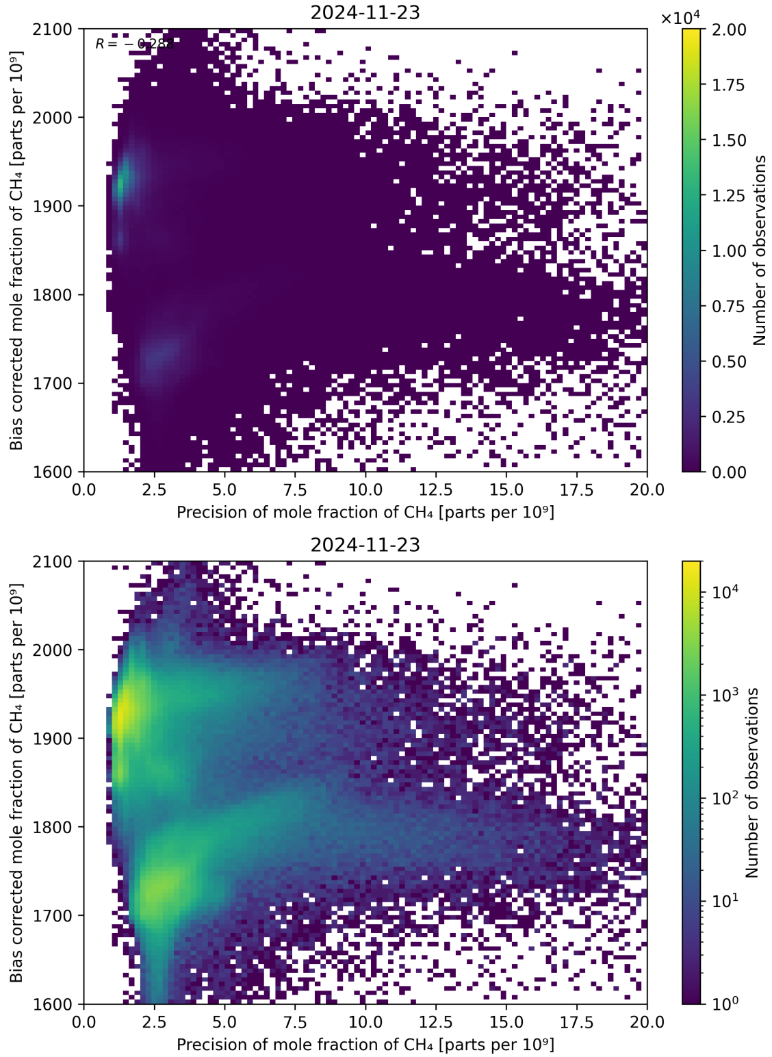
Figure 82: Scatter density plot of “Precision of mole fraction of CH 4 ” against “Bias corrected mole fraction of CH 4 ” for 2024-11-22 to 2024-11-24.
