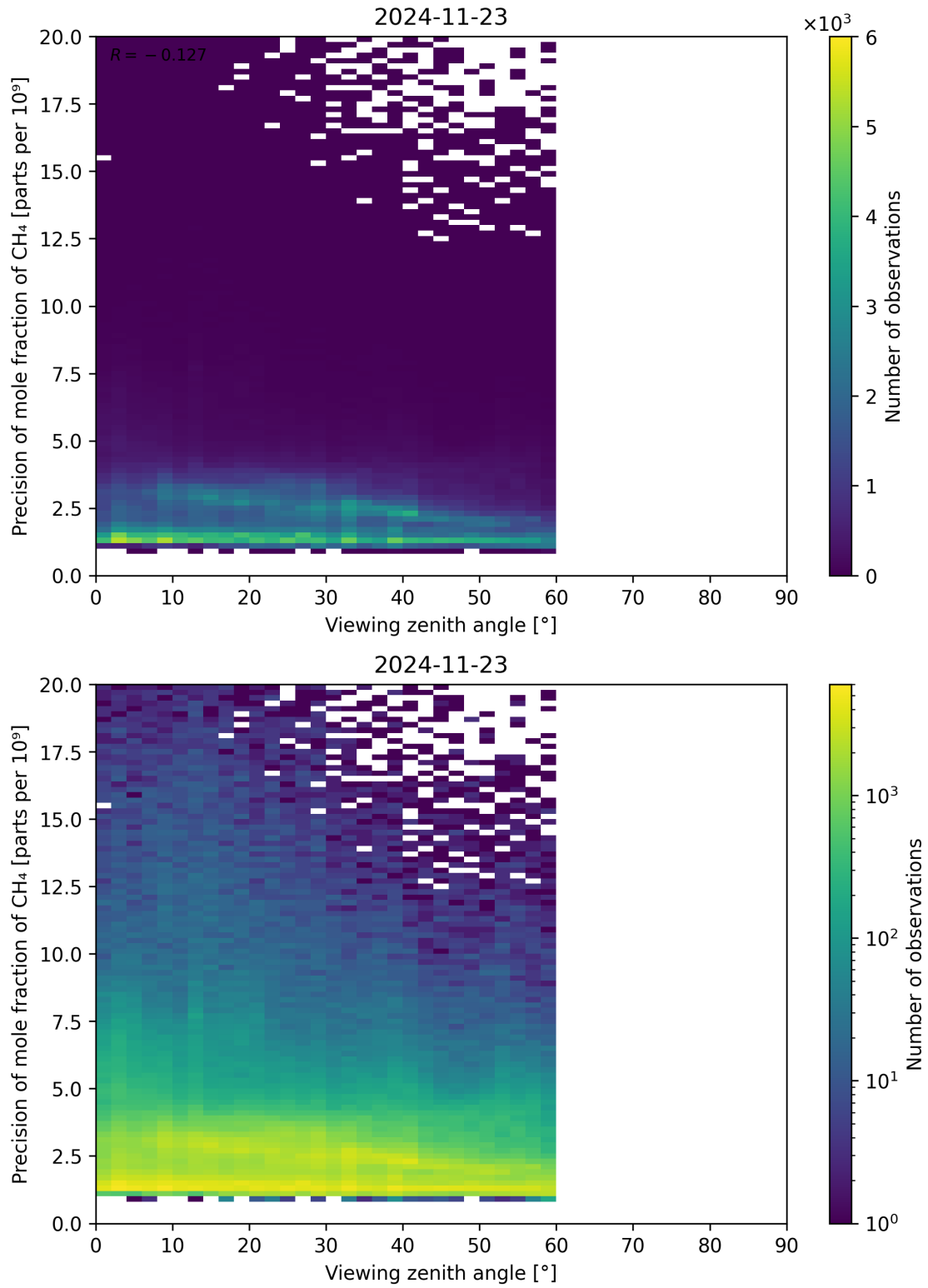
Figure 112: Scatter density plot of “Viewing zenith angle” against “Precision of mole fraction of \text{CH}_4 ” for 2024-11-22 to 2024-11-24.
