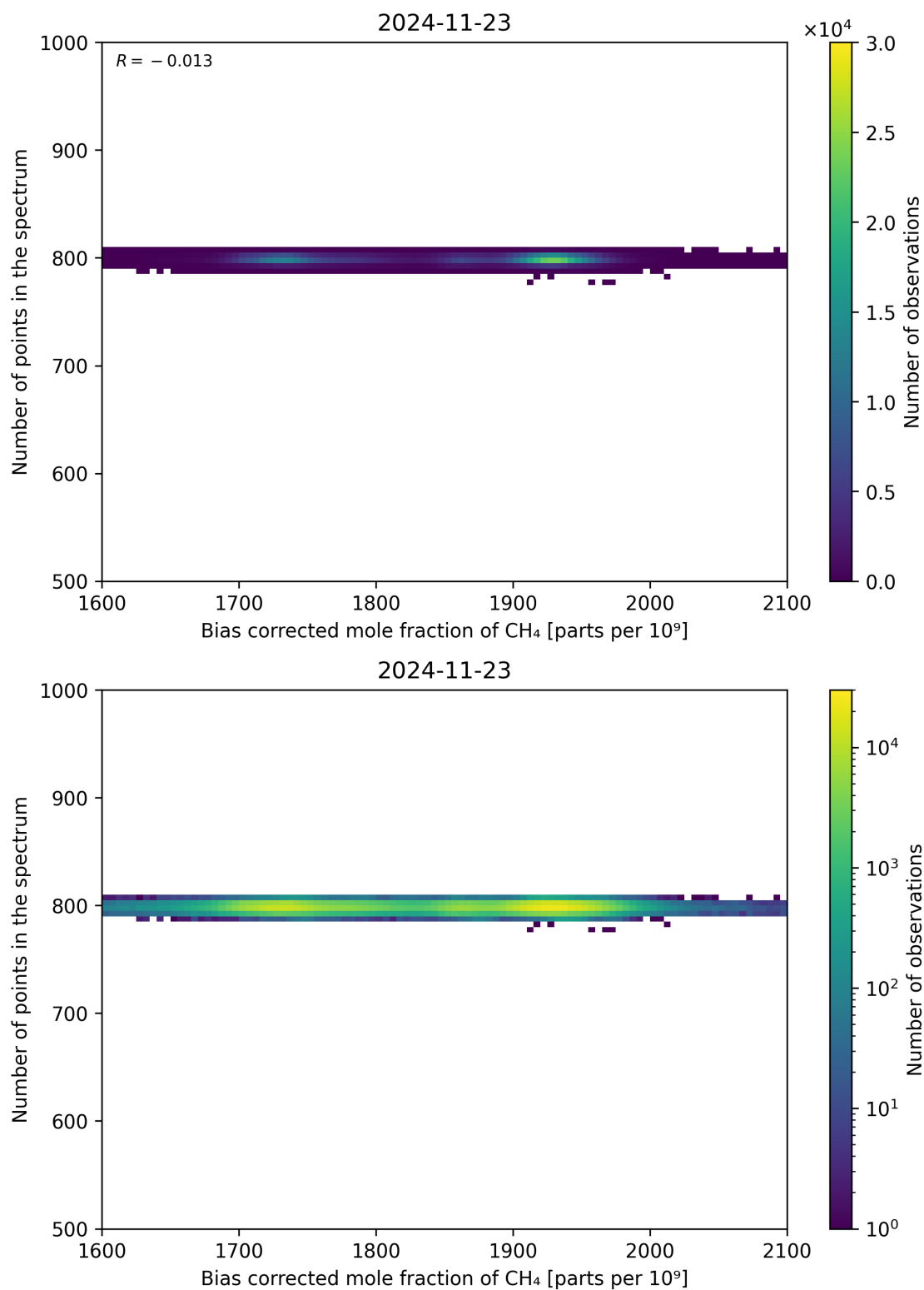
Figure 68: Scatter density plot of “Bias corrected mole fraction of CH 4 ” against “Number of points in the spectrum” for 2024-11-22 to 2024-11-24.
