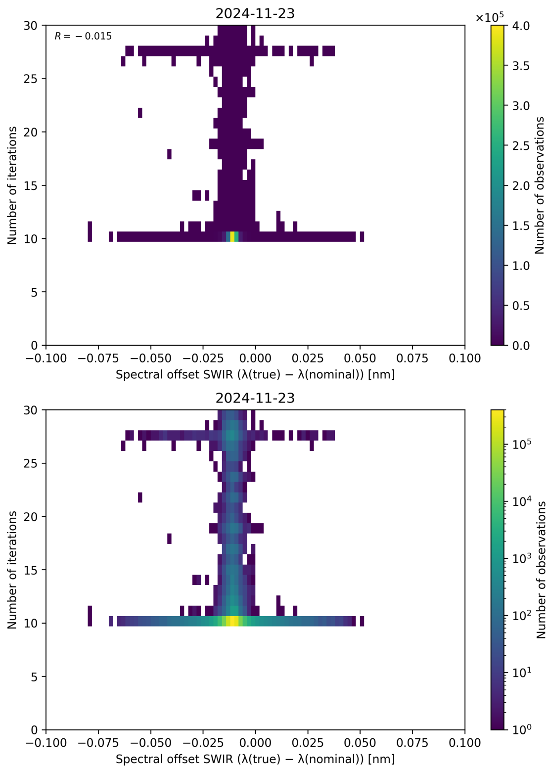
Figure 121: Scatter density plot of “Spectral offset SWIR ( \lambda_{\text{true}} - \lambda_{\text{nominal}} )” against “Number of iterations” for 2024-11-22 to 2024-11-24.
