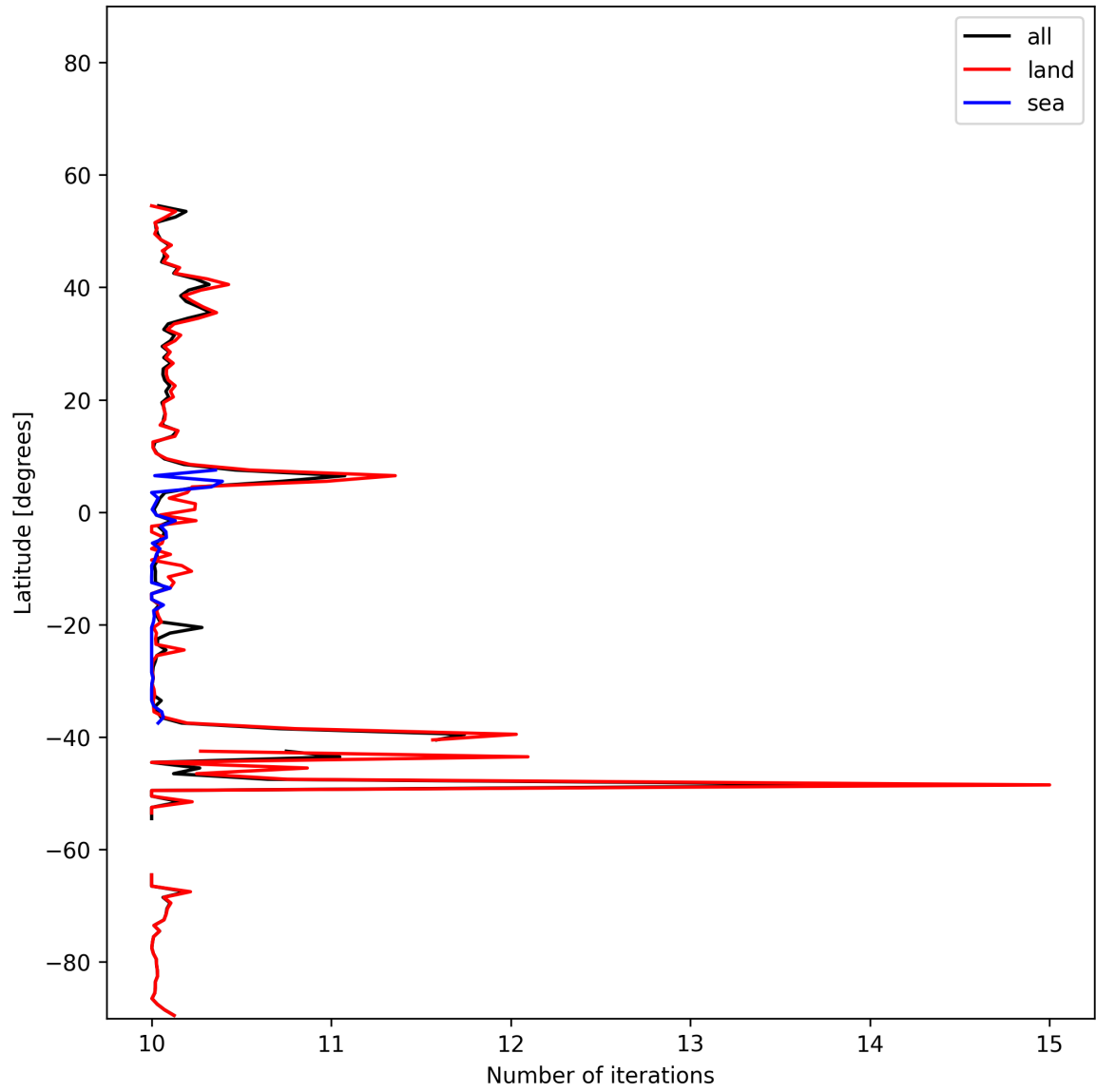
Figure 20: Zonal average of “Number of iterations” for 2024-11-22 to 2024-11-24.
