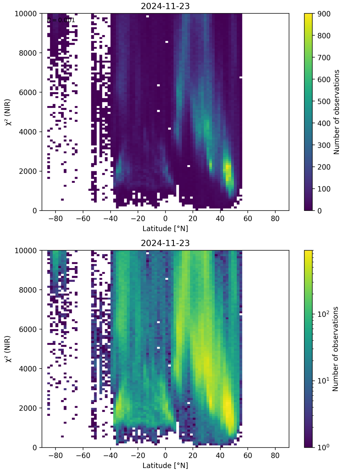
Figure 53: Scatter density plot of “Latitude” against “ \chi^2 (NIR)” for 2024-11-22 to 2024-11-24.
