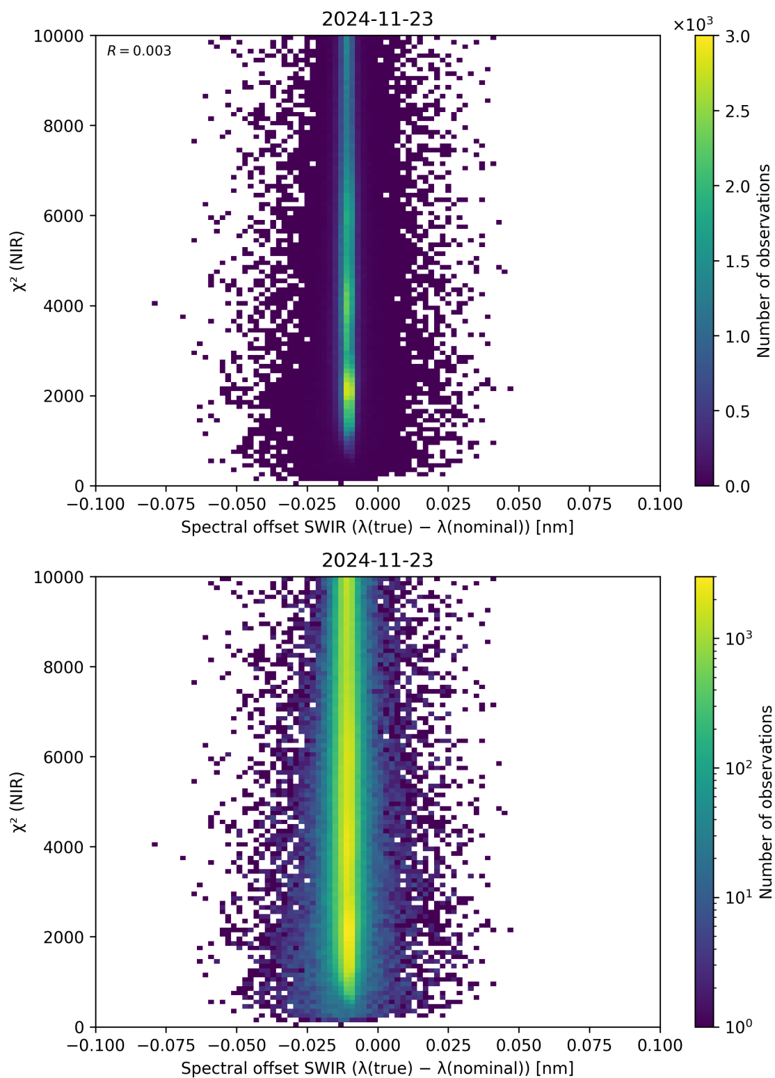
Figure 117: Scatter density plot of “Spectral offset SWIR ( \lambda_{\text{true}} - \lambda_{\text{nominal}} )” against “ \chi^2 (NIR)” for 2024-11-22 to 2024-11-24.
