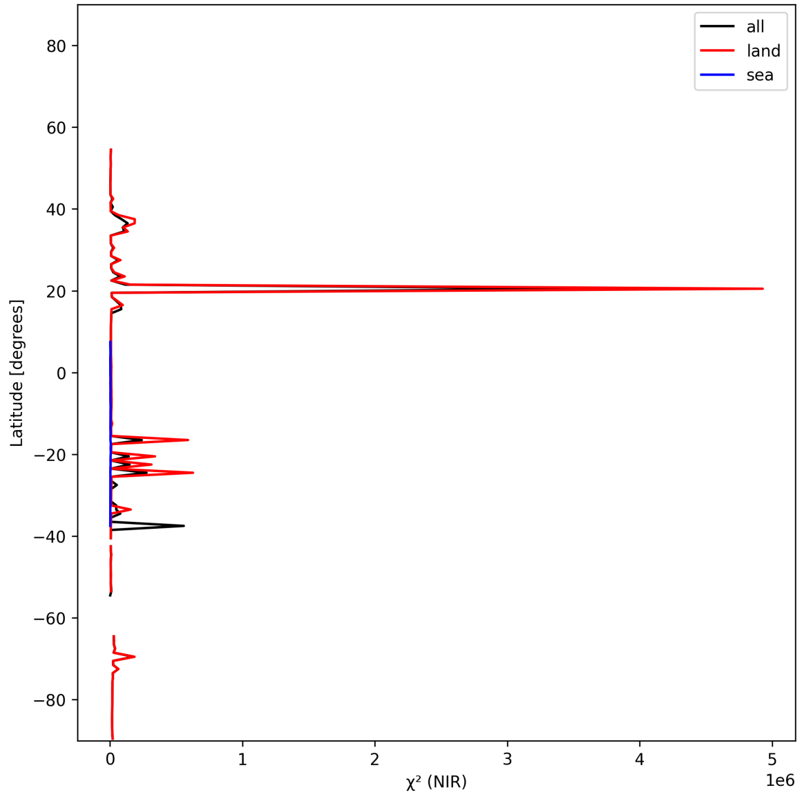
Figure 18: Zonal average of “ \chi^2 (NIR)” for 2024-11-22 to 2024-11-24.
