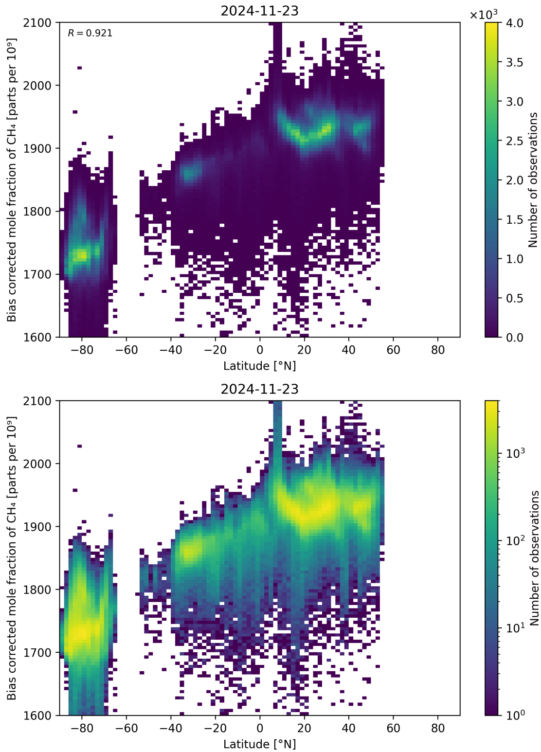
Figure 58: Scatter density plot of “Latitude” against “Bias corrected mole fraction of \text{CH}_4 ” for 2024-11-22 to 2024-11-24.
