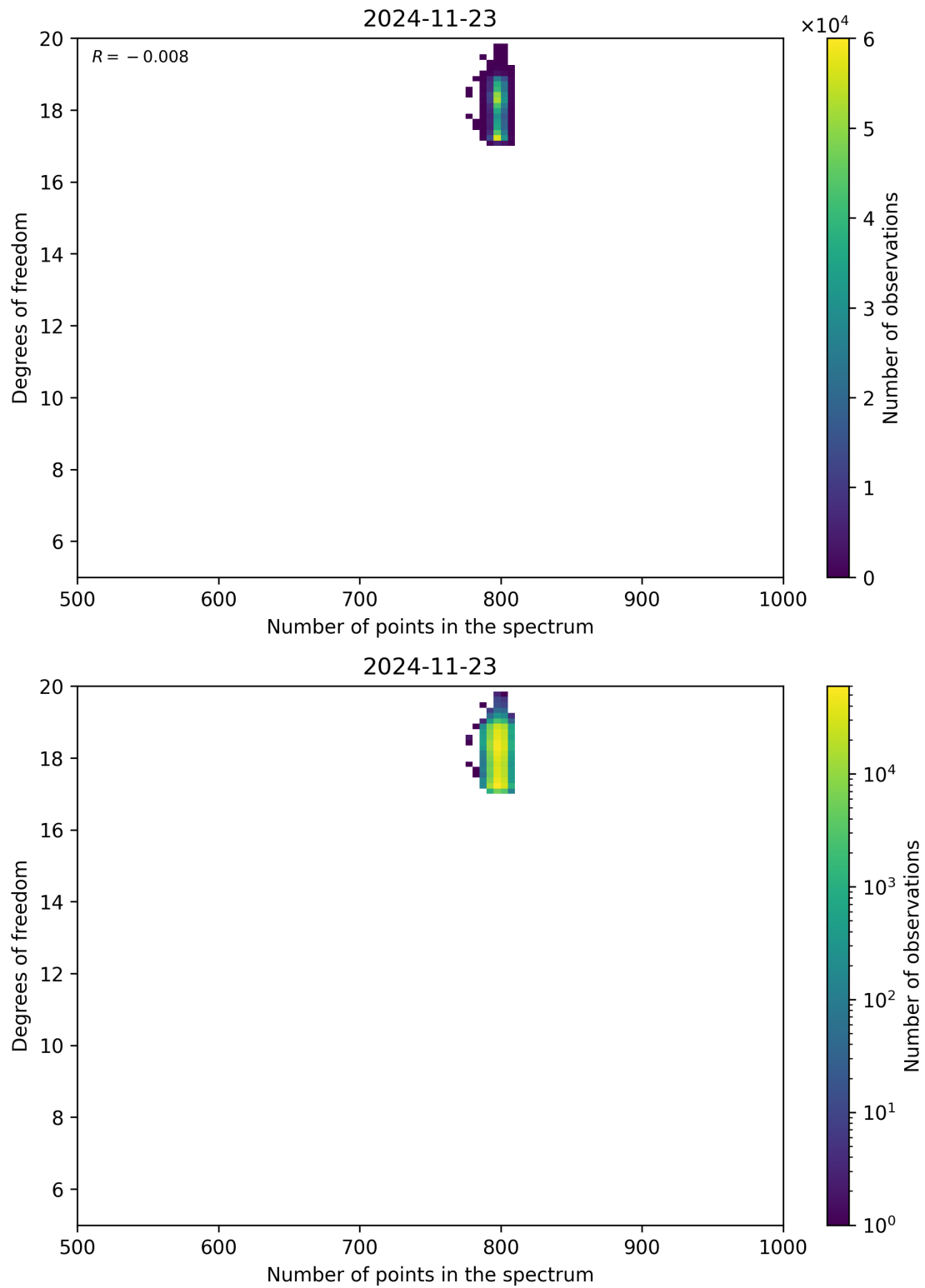
Figure 90: Scatter density plot of “Number of points in the spectrum” against “Degrees of freedom” for 2024-11-22 to 2024-11-24.
