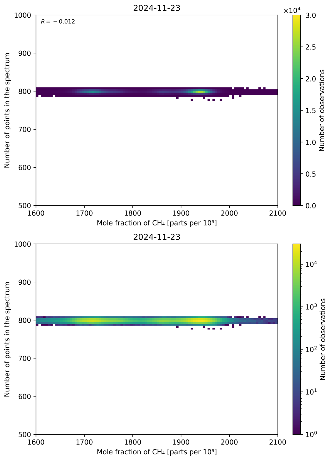
Figure 77: Scatter density plot of “Mole fraction of CH 4 ” against “Number of points in the spectrum” for 2024-11-22 to 2024-11-24.
