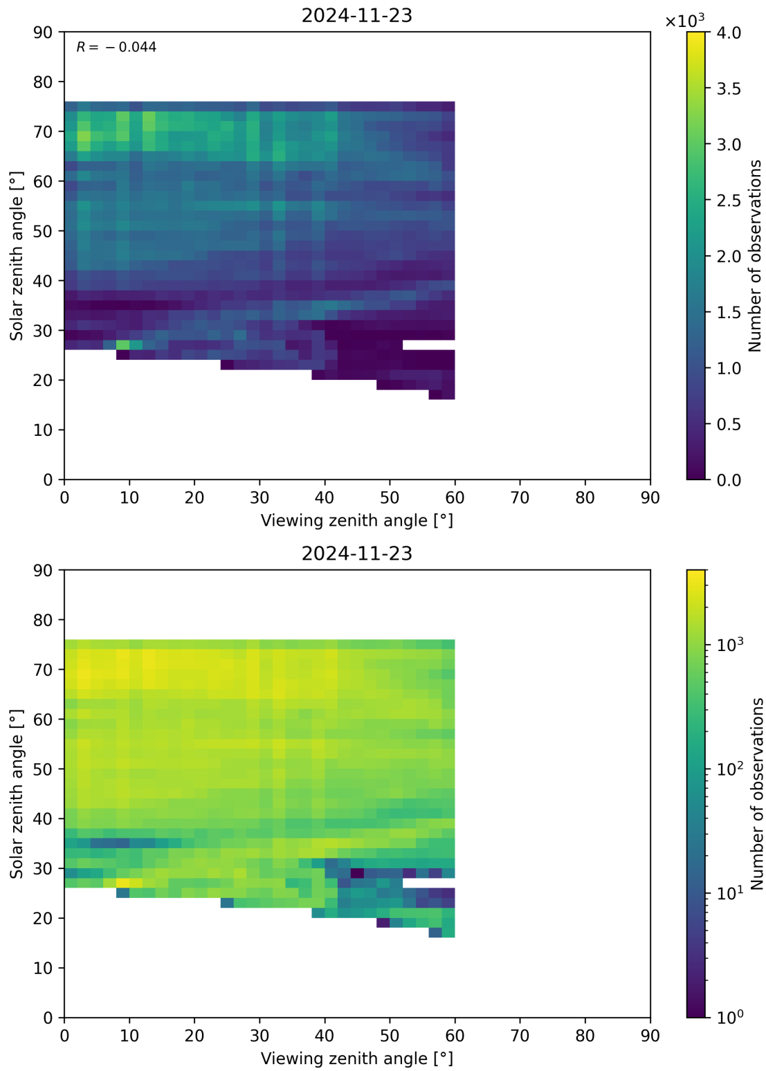
Figure 115: Scatter density plot of “Viewing zenith angle” against “Solar zenith angle” for 2024-11-22 to 2024-11-24.
