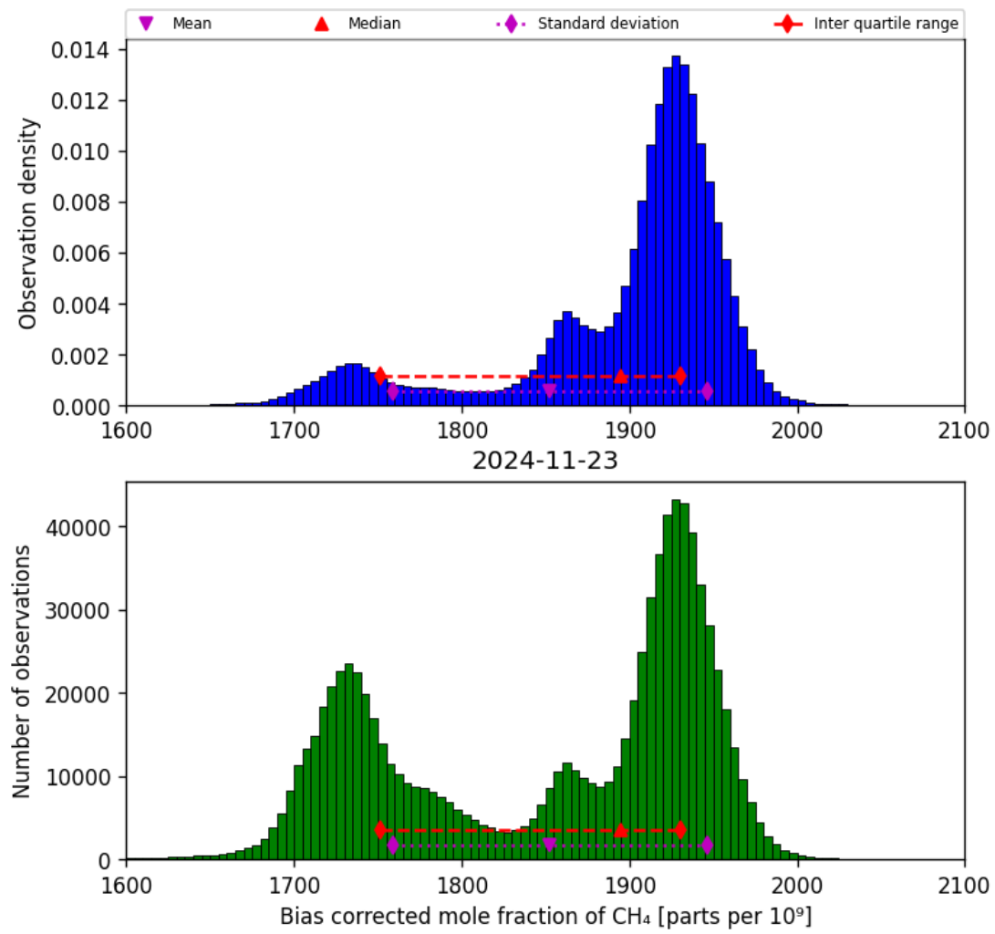
Figure 25: Histogram of “Bias corrected mole fraction of CH 4 ” for 2024-11-22 to 2024-11-24
