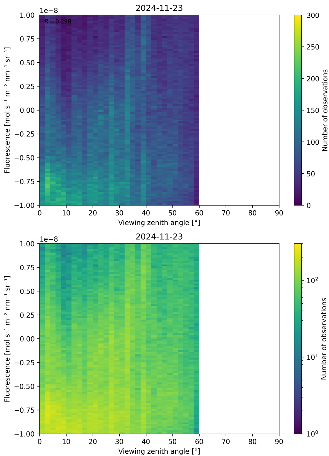
Figure 108: Scatter density plot of “Viewing zenith angle” against “Fluorescence” for 2024-11-22 to 2024-11-24.
