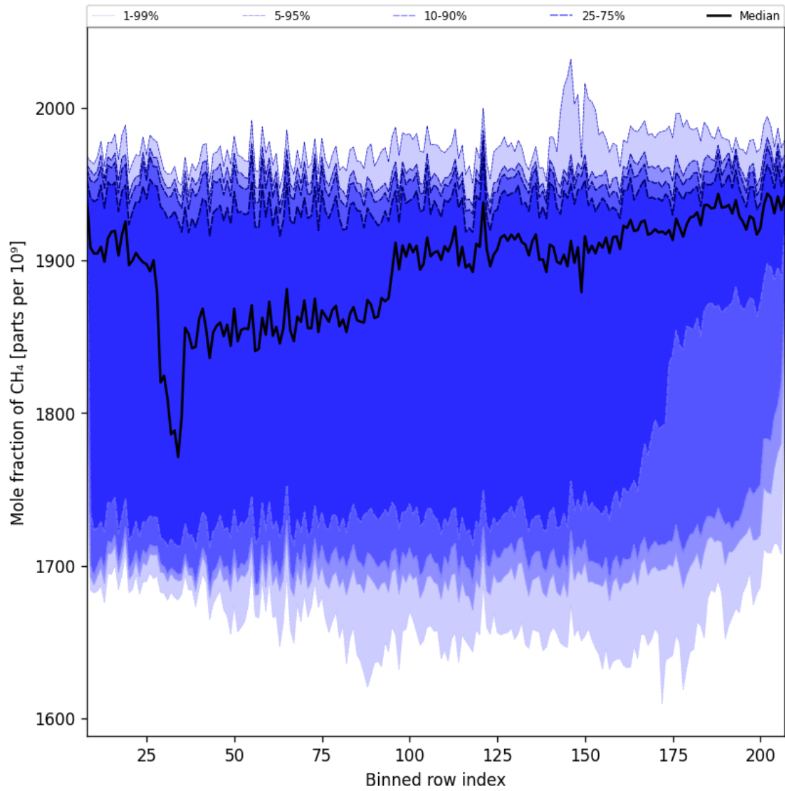
Figure 34: Along track statistics of “Mole fraction of CH 4 ” for 2024-11-22 to 2024-11-24
