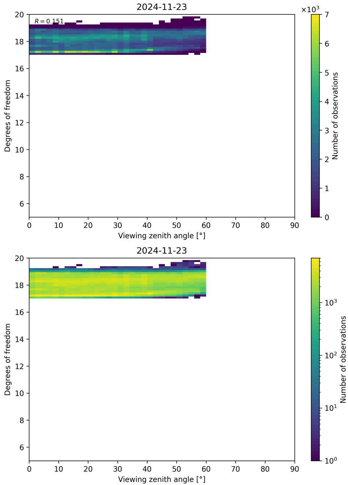
Figure 107: Scatter density plot of “Viewing zenith angle” against “Degrees of freedom” for 2024-11-22 to 2024-11-24.
