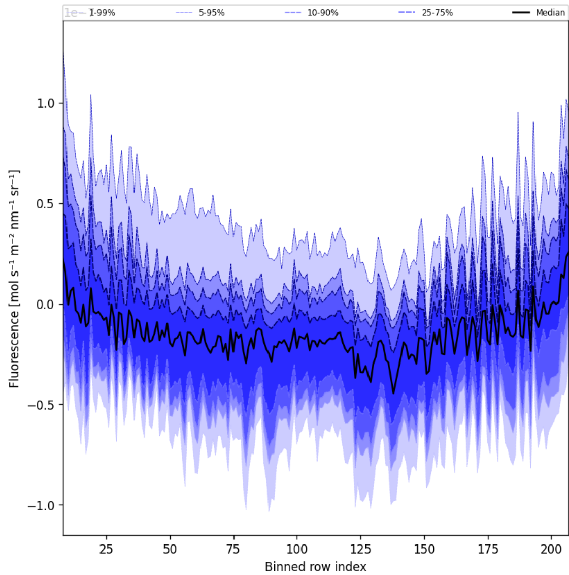
Figure 43: Along track statistics of “Fluorescence” for 2024-11-22 to 2024-11-24
