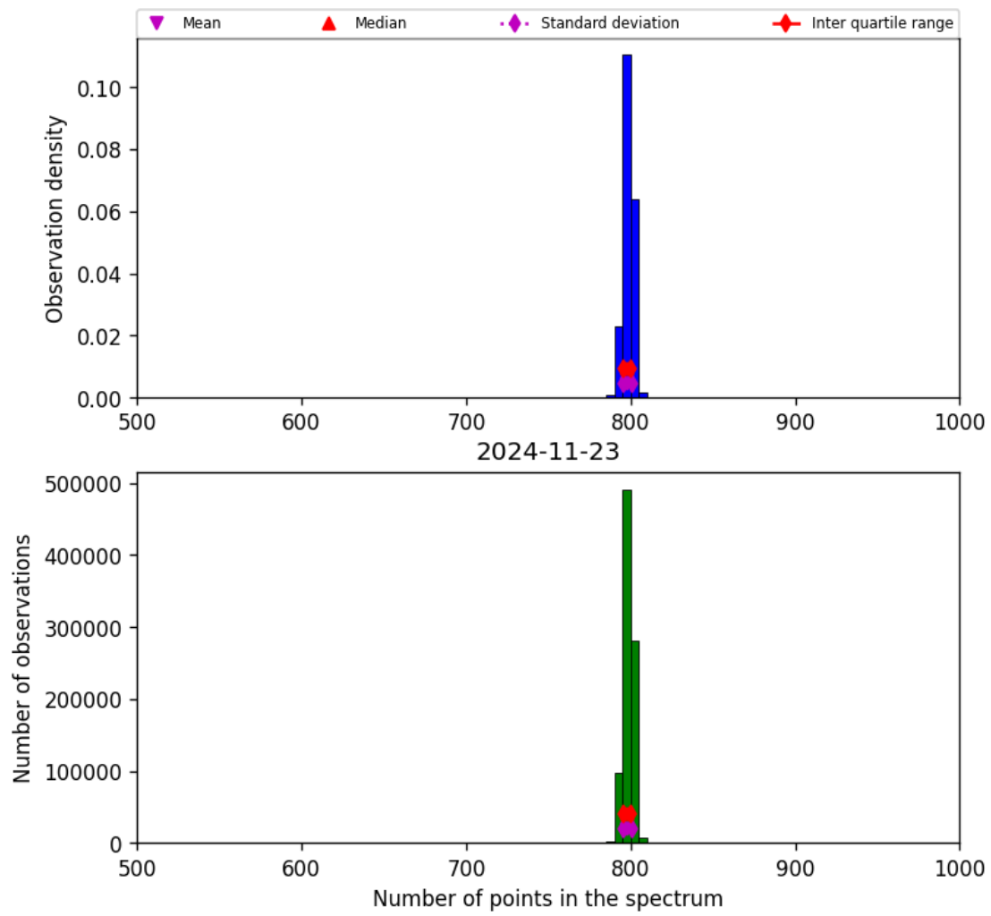
Figure 26: Histogram of “Number of points in the spectrum” for 2024-11-22 to 2024-11-24
