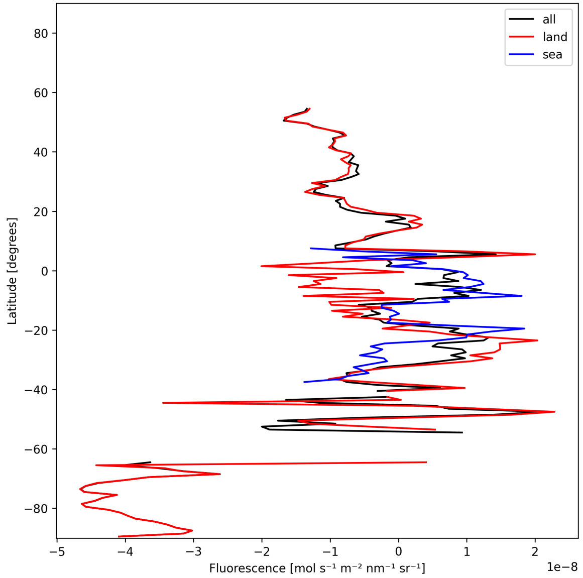
Figure 21: Zonal average of “Fluorescence” for 2024-11-22 to 2024-11-24.
