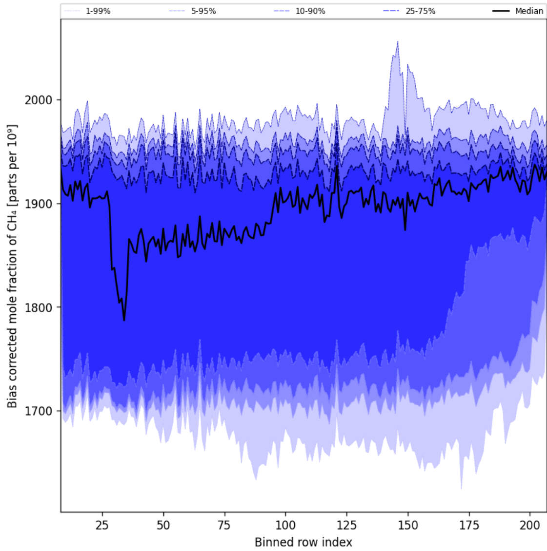
Figure 36: Along track statistics of “Bias corrected mole fraction of CH 4 ” for 2024-11-22 to 2024-11-24
