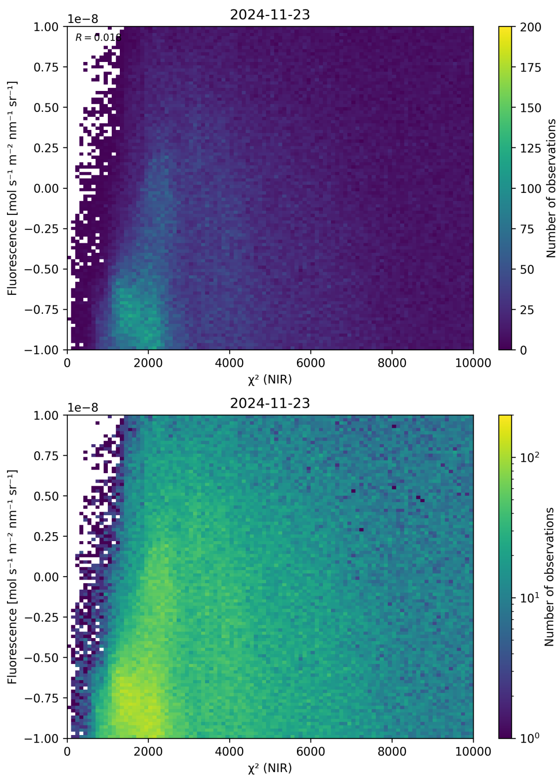
Figure 45: Scatter density plot of “ \chi^2 (NIR)” against “Fluorescence” for 2024-11-22 to 2024-11-24.
