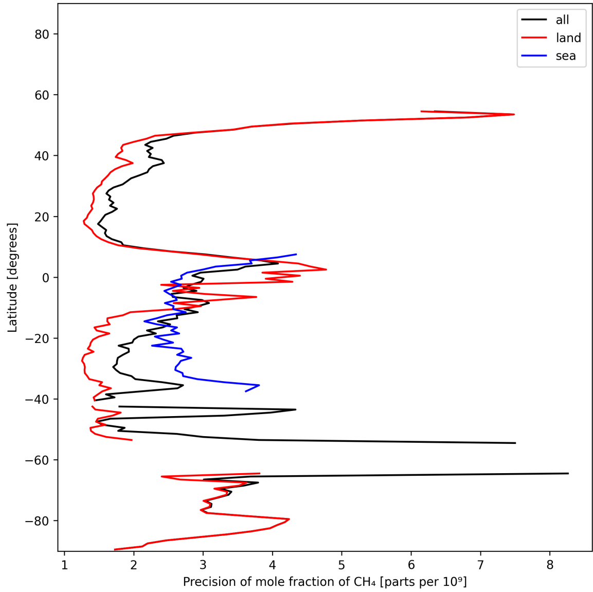
Figure 13: Zonal average of “Precision of mole fraction of CH 4 ” for 2024-11-22 to 2024-11-24.
