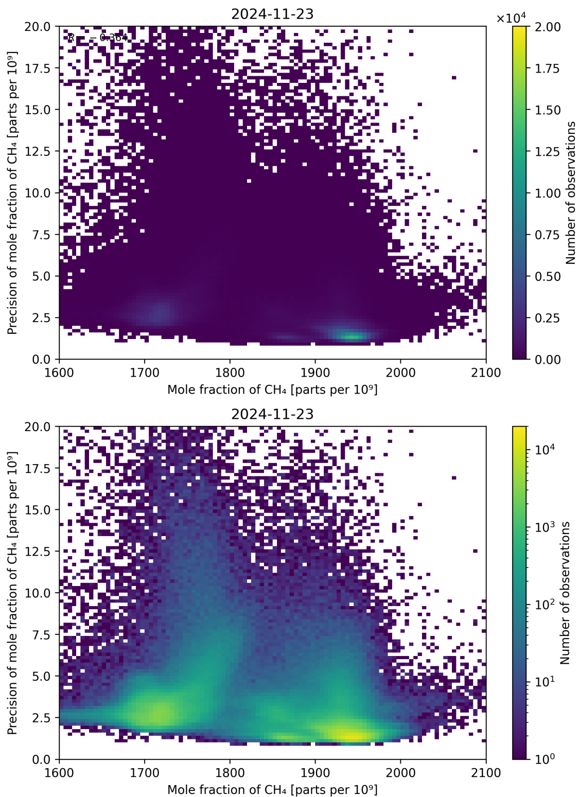
Figure 75: Scatter density plot of “Mole fraction of CH 4 ” against “Precision of mole fraction of CH 4 ” for 2024-11-22 to 2024-11-24.
