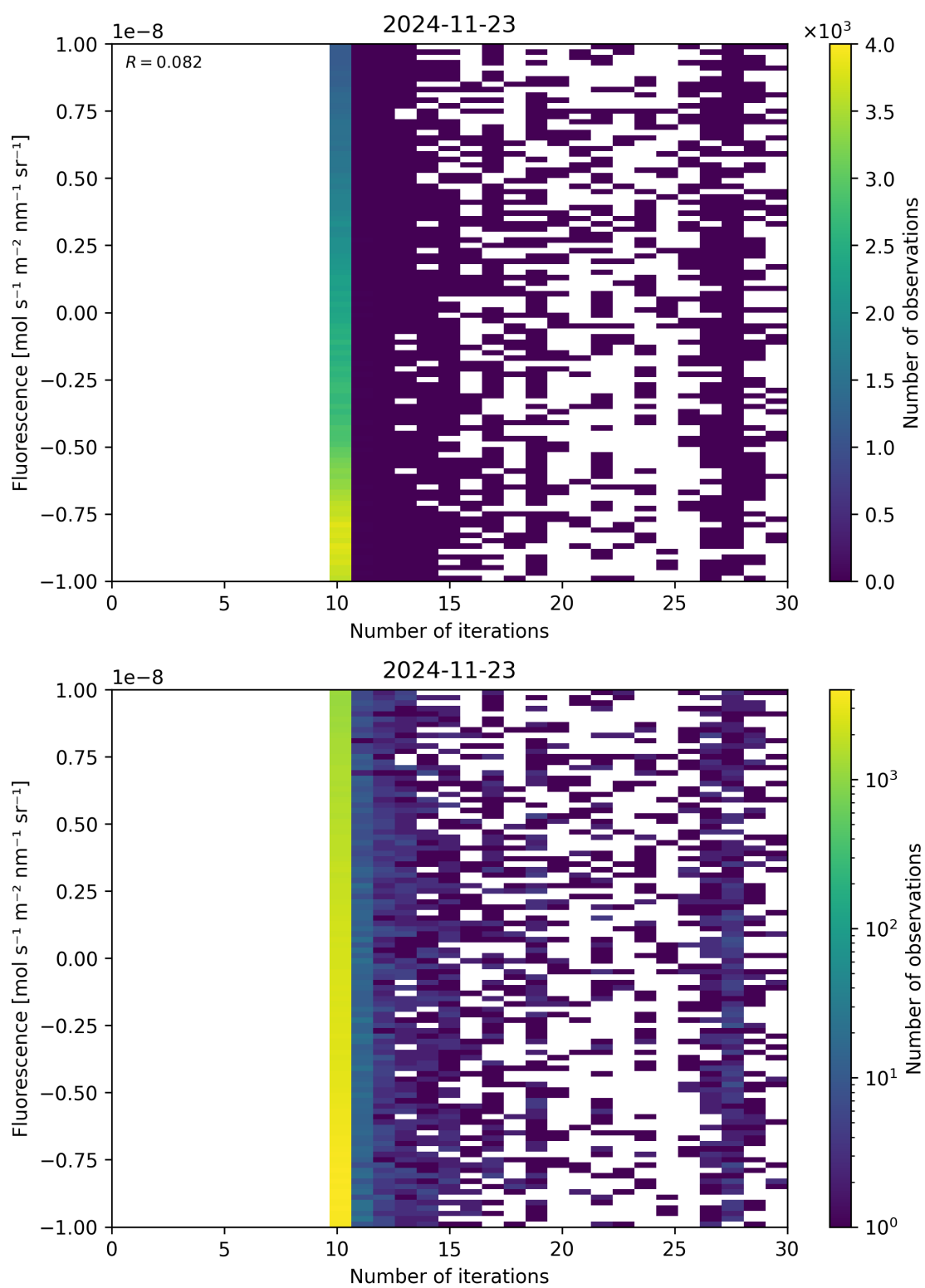
Figure 87: Scatter density plot of “Number of iterations” against “Fluorescence” for 2024-11-22 to 2024-11-24.
