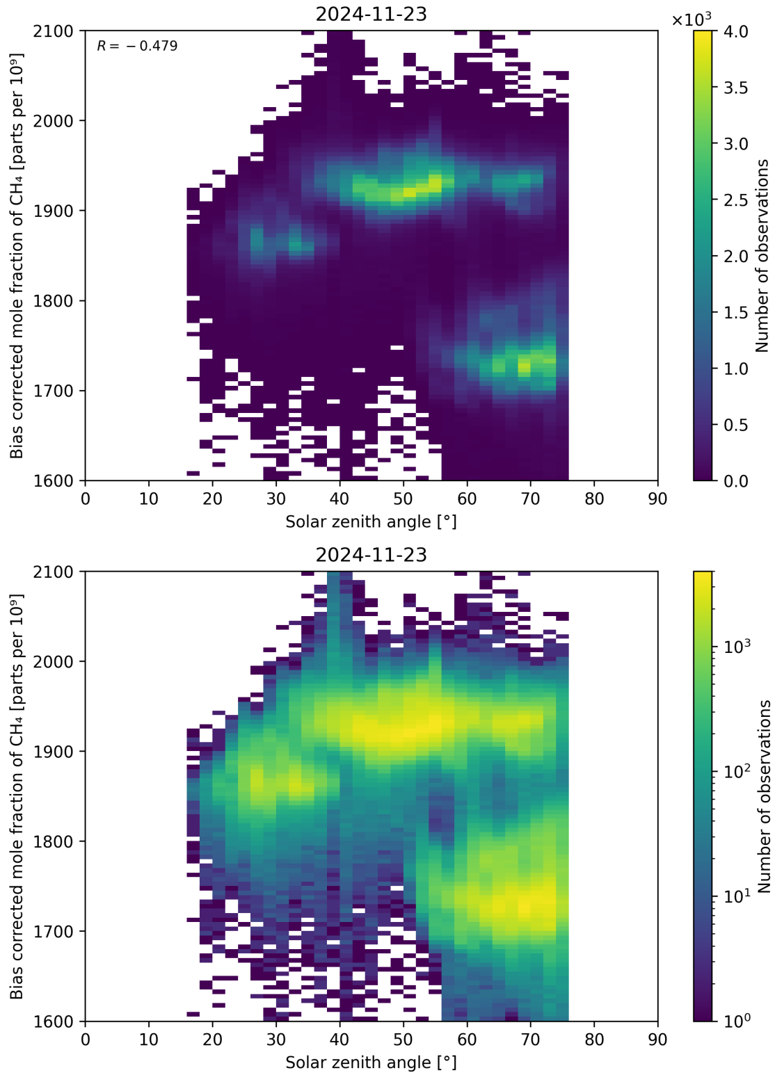
Figure 100: Scatter density plot of “Solar zenith angle” against “Bias corrected mole fraction of CH 4 ” for 2024-11-22 to 2024-11-24.
