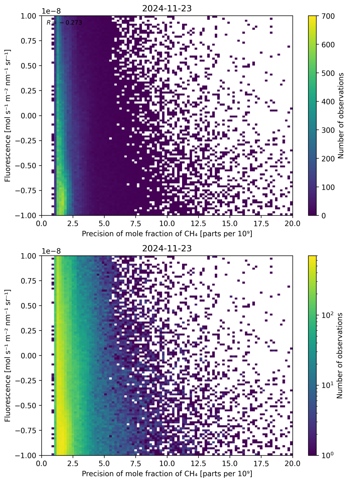
Figure 81: Scatter density plot of “Precision of mole fraction of CH 4 ” against “Fluorescence” for 2024-11-22 to 2024-11-24.
