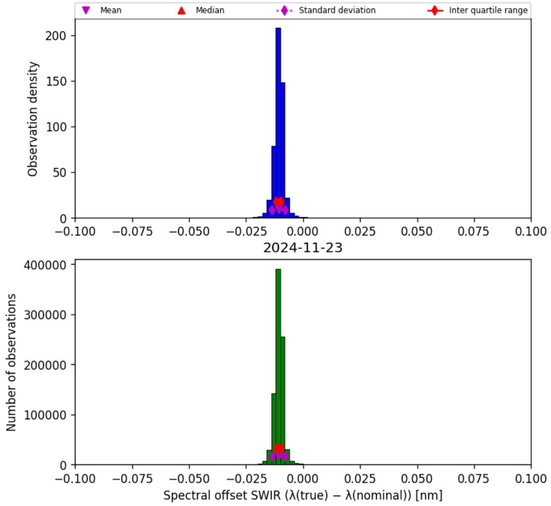
Figure 27: Histogram of “Spectral offset SWIR ( \lambda_{\text{true}} - \lambda_{\text{nominal}} )” for 2024-11-22 to 2024-11-24
