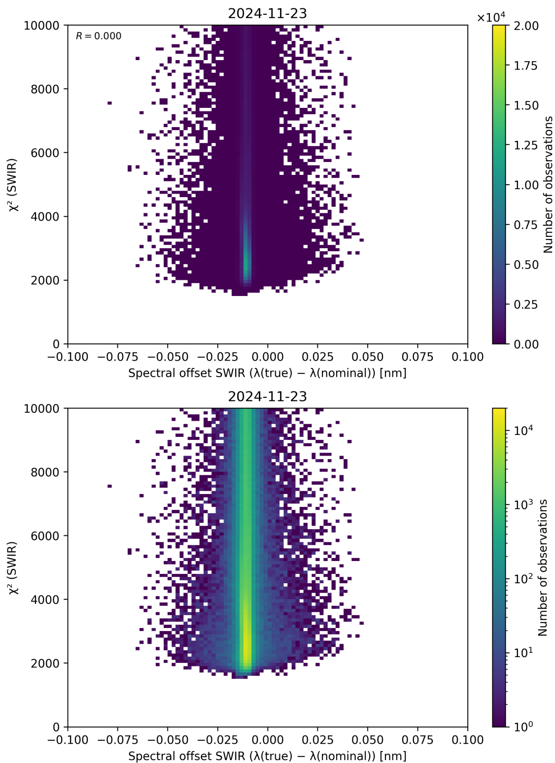
Figure 118: Scatter density plot of “Spectral offset SWIR ( \lambda_{\text{true}} - \lambda_{\text{nominal}} )” against “ \chi^2 (SWIR)” for 2024-11-22 to 2024-11-24.
