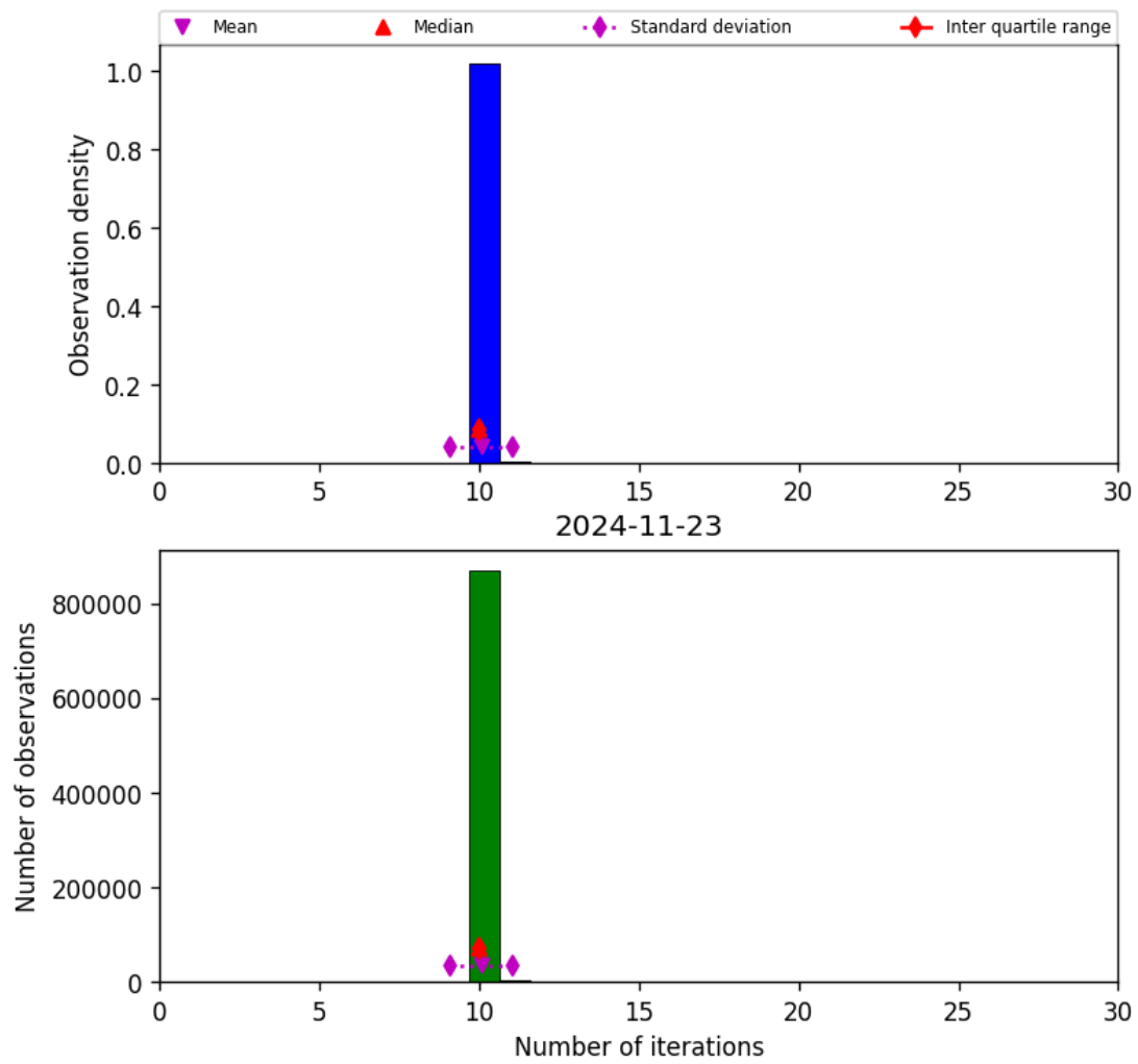
Figure 31: Histogram of “Number of iterations” for 2024-11-22 to 2024-11-24
