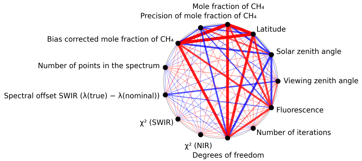
Figure 1: Map of correlation graph for 2024-11-22 to 2024-11-24.
