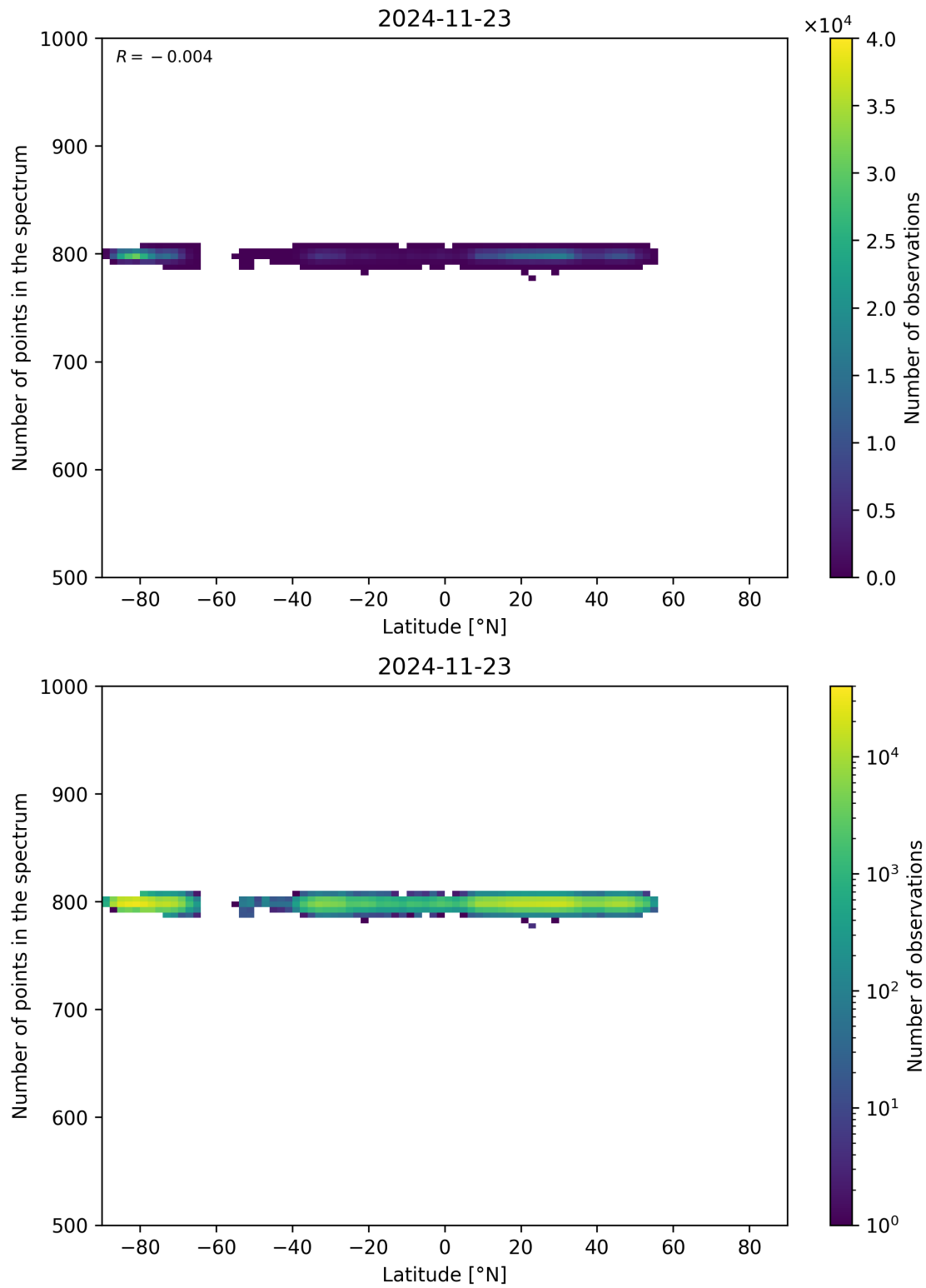
Figure 61: Scatter density plot of “Latitude” against “Number of points in the spectrum” for 2024-11-22 to 2024-11-24.
