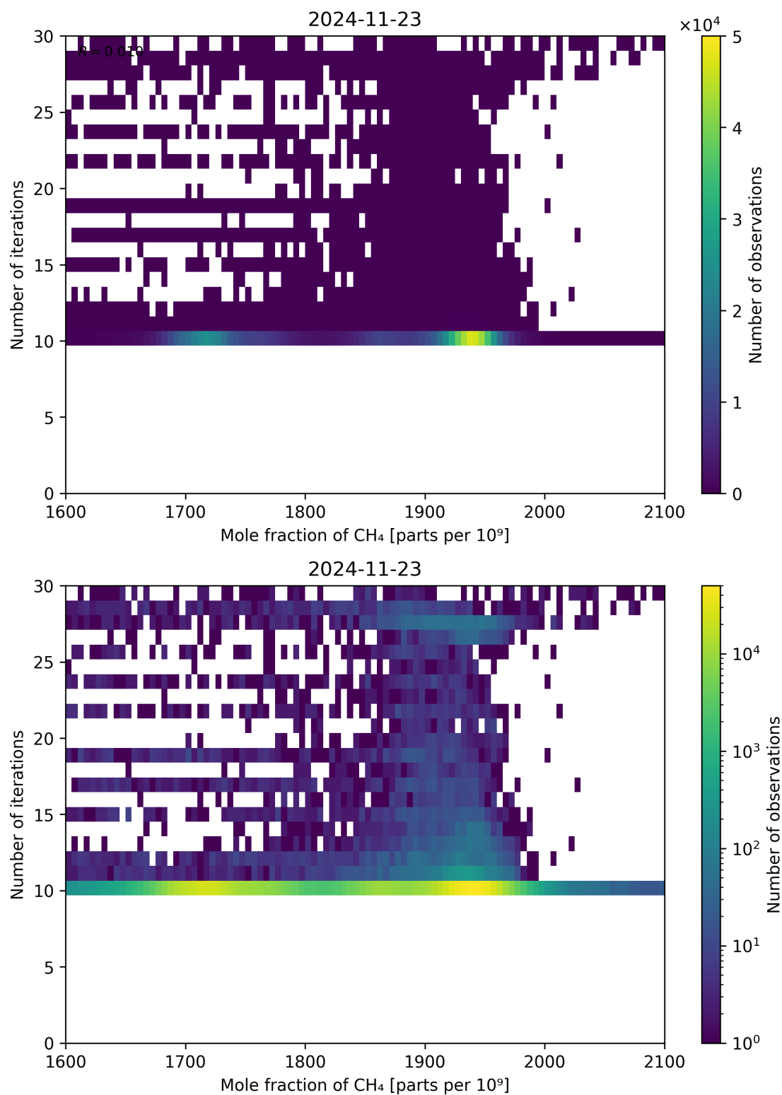
Figure 76: Scatter density plot of “Mole fraction of CH 4 ” against “Number of iterations” for 2024-11-22 to 2024-11-24.
