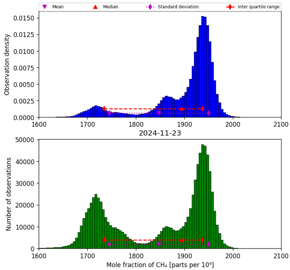
Figure 23: Histogram of “Mole fraction of CH 4 ” for 2024-11-22 to 2024-11-24
