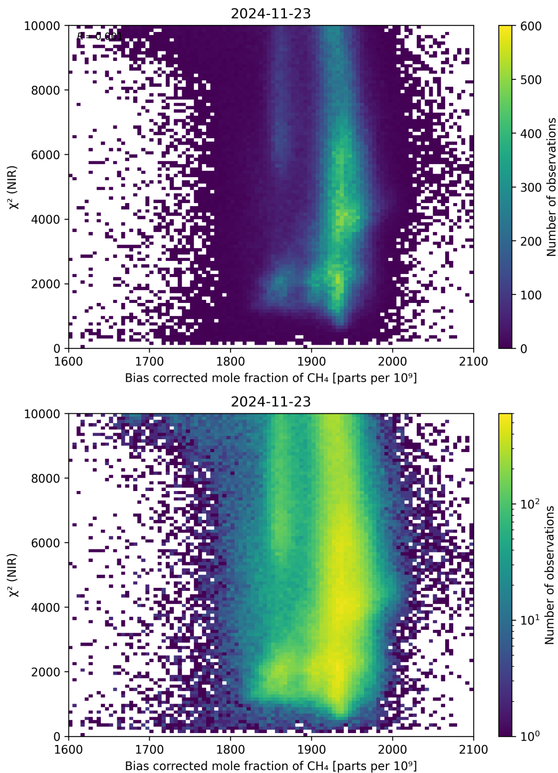
Figure 63: Scatter density plot of “Bias corrected mole fraction of CH 4 ” against “ \chi^2 (NIR)” for 2024-11-22 to 2024-11-24.
