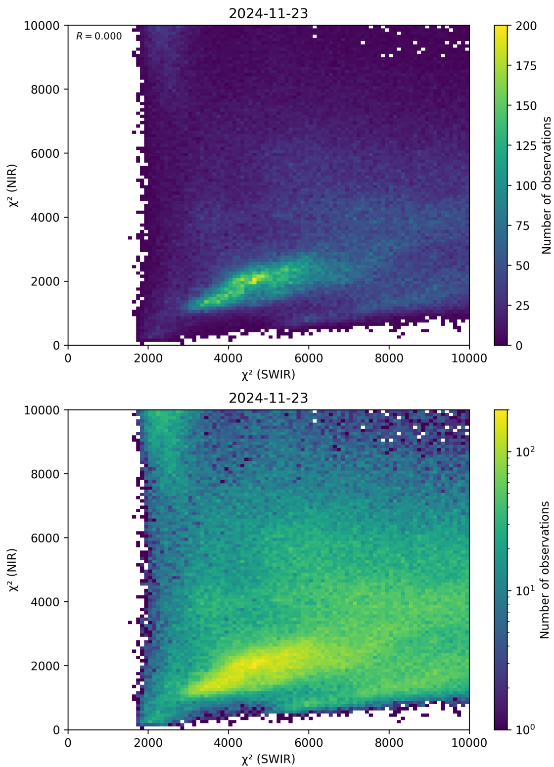
Figure 47: Scatter density plot of “ \chi^2 (SWIR)” against “ \chi^2 (NIR)” for 2024-11-22 to 2024-11-24.
