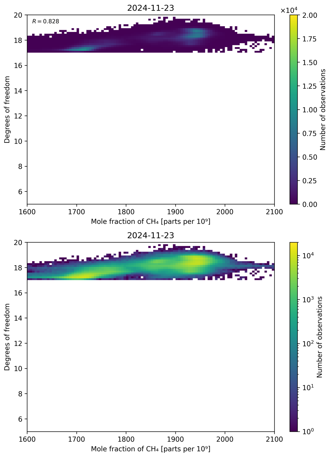
Figure 72: Scatter density plot of “Mole fraction of CH 4 ” against “Degrees of freedom” for 2024-11-22 to 2024-11-24.
