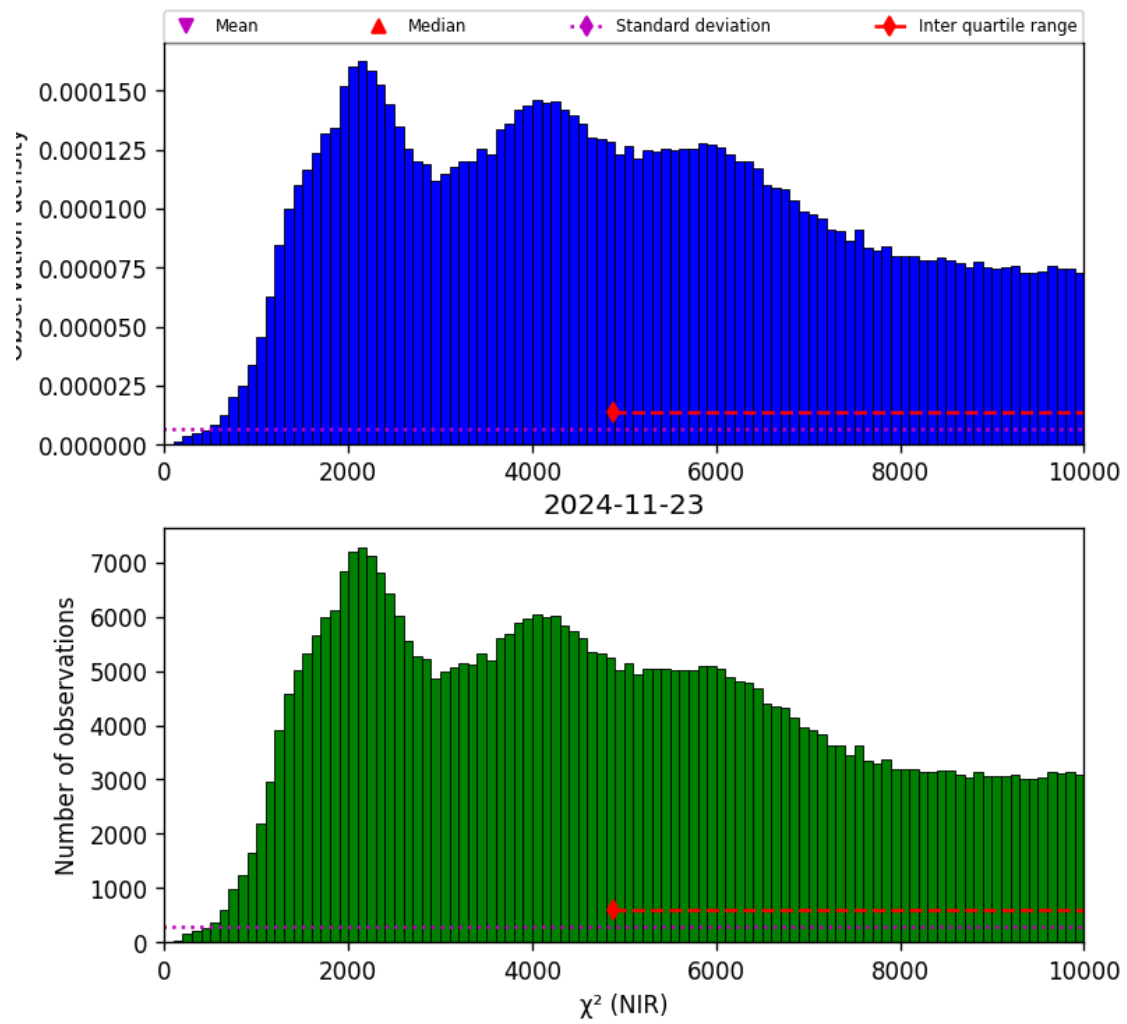
Figure 29: Histogram of “ \chi^2 (NIR)” for 2024-11-22 to 2024-11-24
