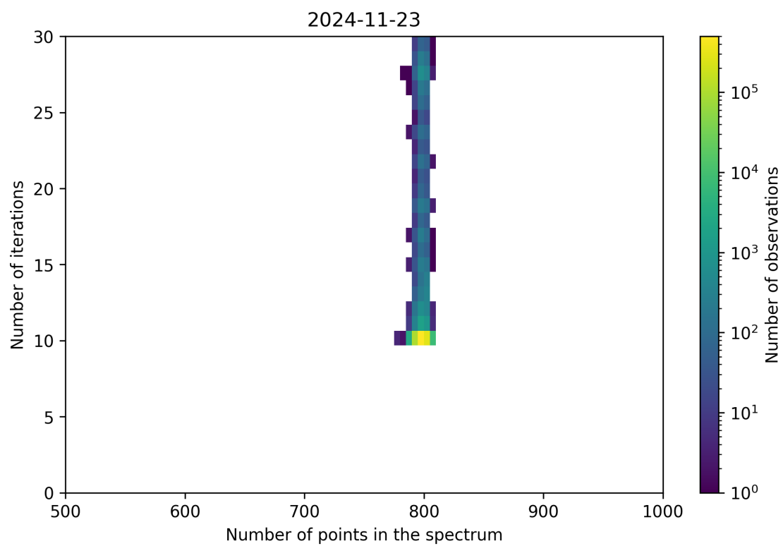
Figure 92: Scatter density plot of “Number of points in the spectrum” against “Number of iterations” for 2024-11-22 to 2024-11-24.
