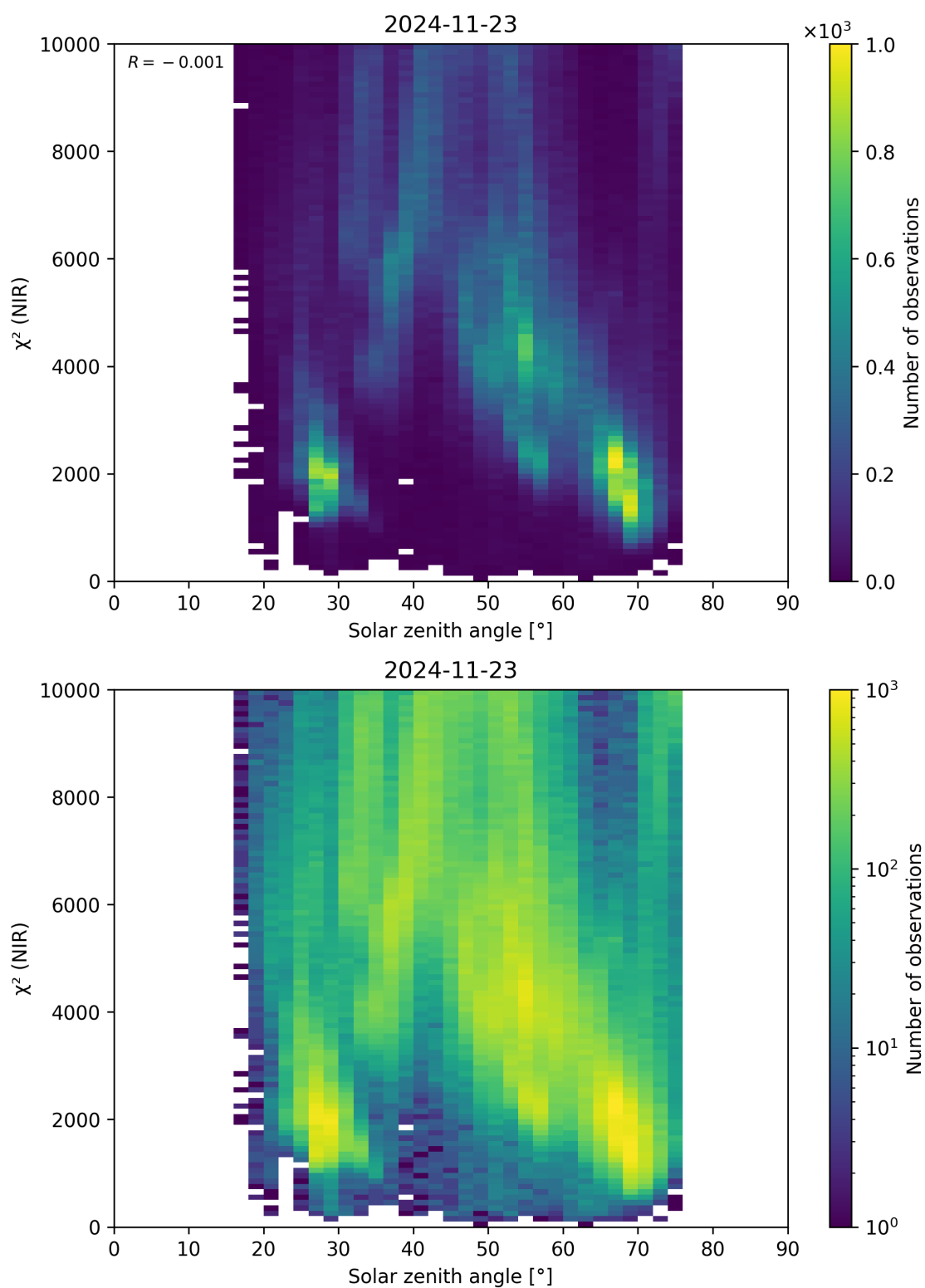
Figure 94: Scatter density plot of “Solar zenith angle” against “ \chi^2 (NIR)” for 2024-11-22 to 2024-11-24.
