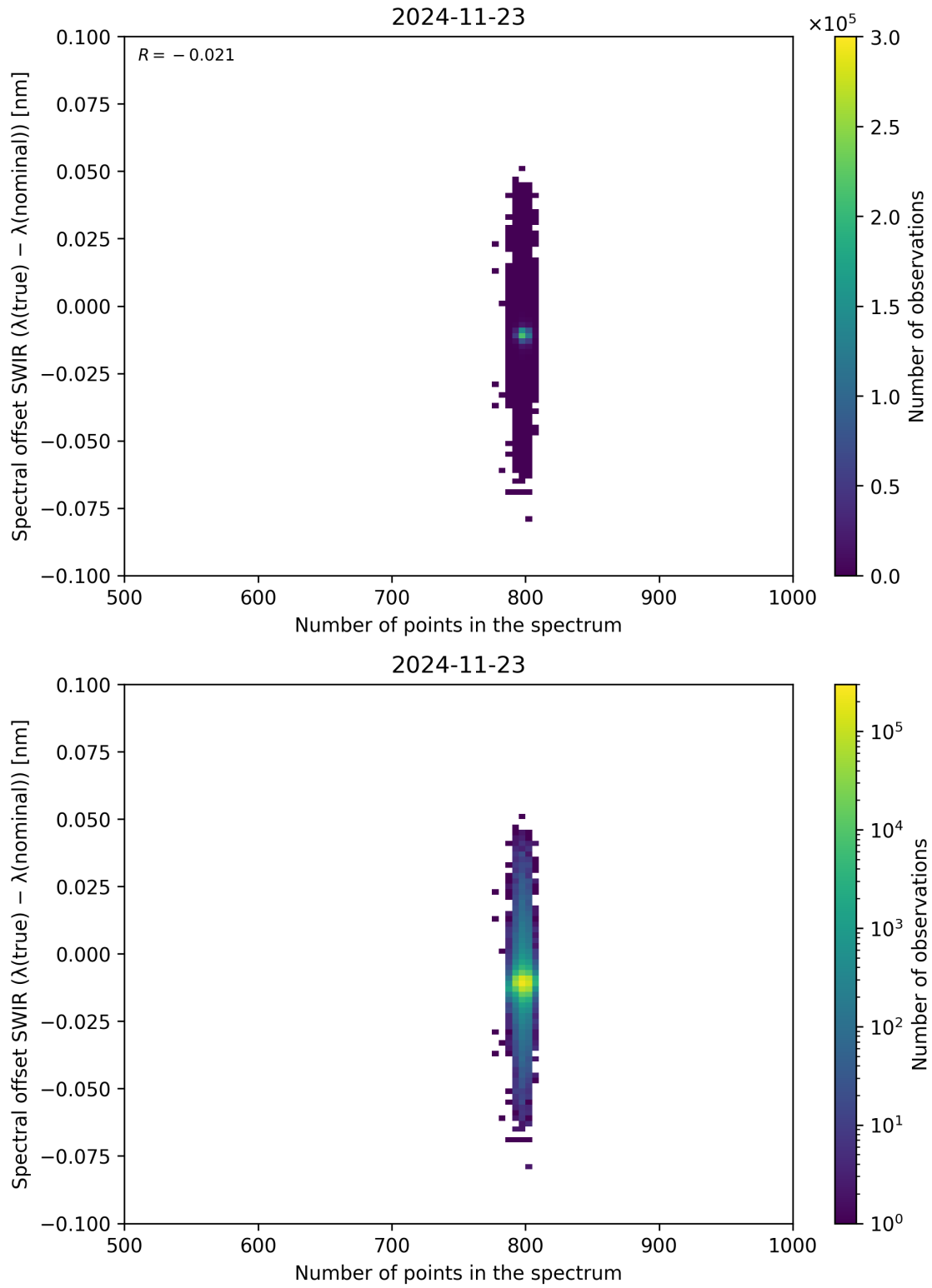
Figure 93: Scatter density plot of “Number of points in the spectrum” against “Spectral offset SWIR ( \lambda_{\text{true}} - \lambda_{\text{nominal}} )” for 2024-11-22 to 2024-11-24.
