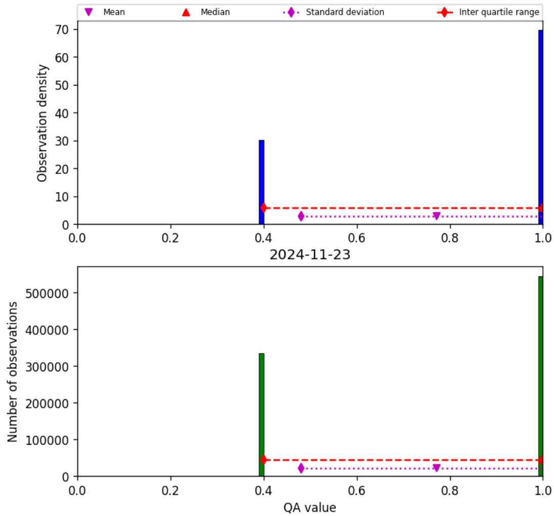
Figure 22: Histogram of “QA value” for 2024-11-22 to 2024-11-24
