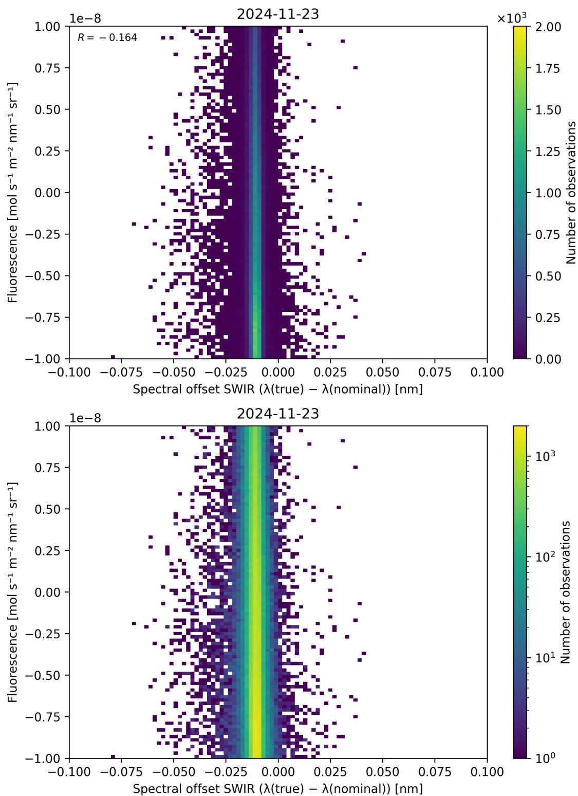
Figure 120: Scatter density plot of “Spectral offset SWIR ( \lambda_{\text{true}} - \lambda_{\text{nominal}} )” against “Fluorescence” for 2024-11-22 to 2024-11-24.
