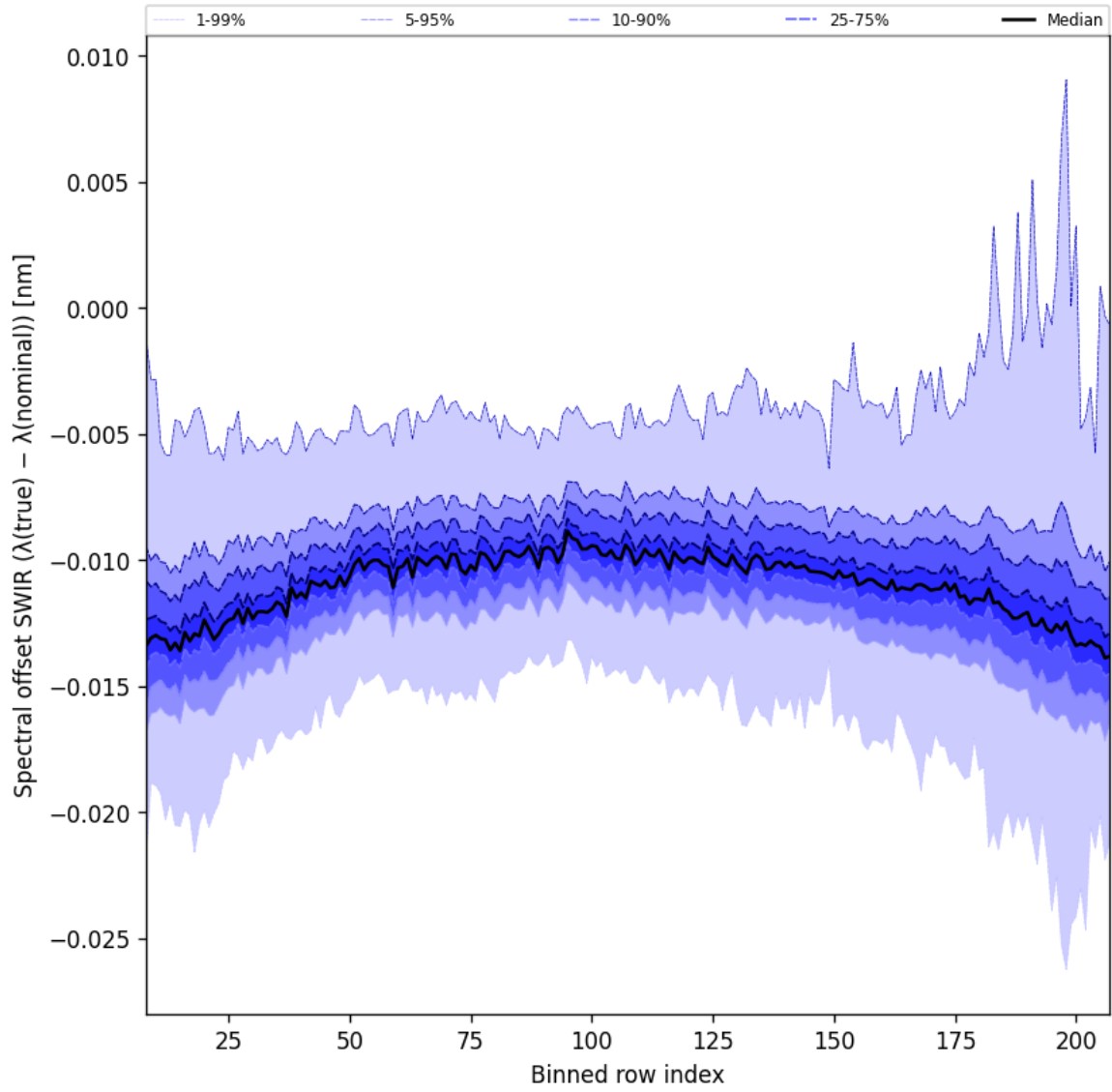
Figure 38: Along track statistics of “Spectral offset SWIR ( \lambda_{\text{true}} - \lambda_{\text{nominal}} )” for 2024-11-22 to 2024-11-24
