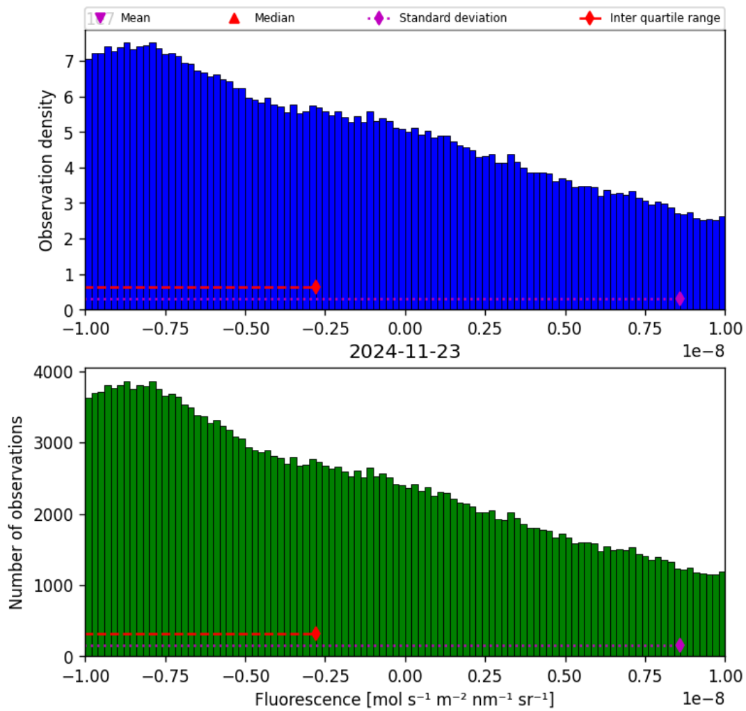
Figure 32: Histogram of “Fluorescence” for 2024-11-22 to 2024-11-24
