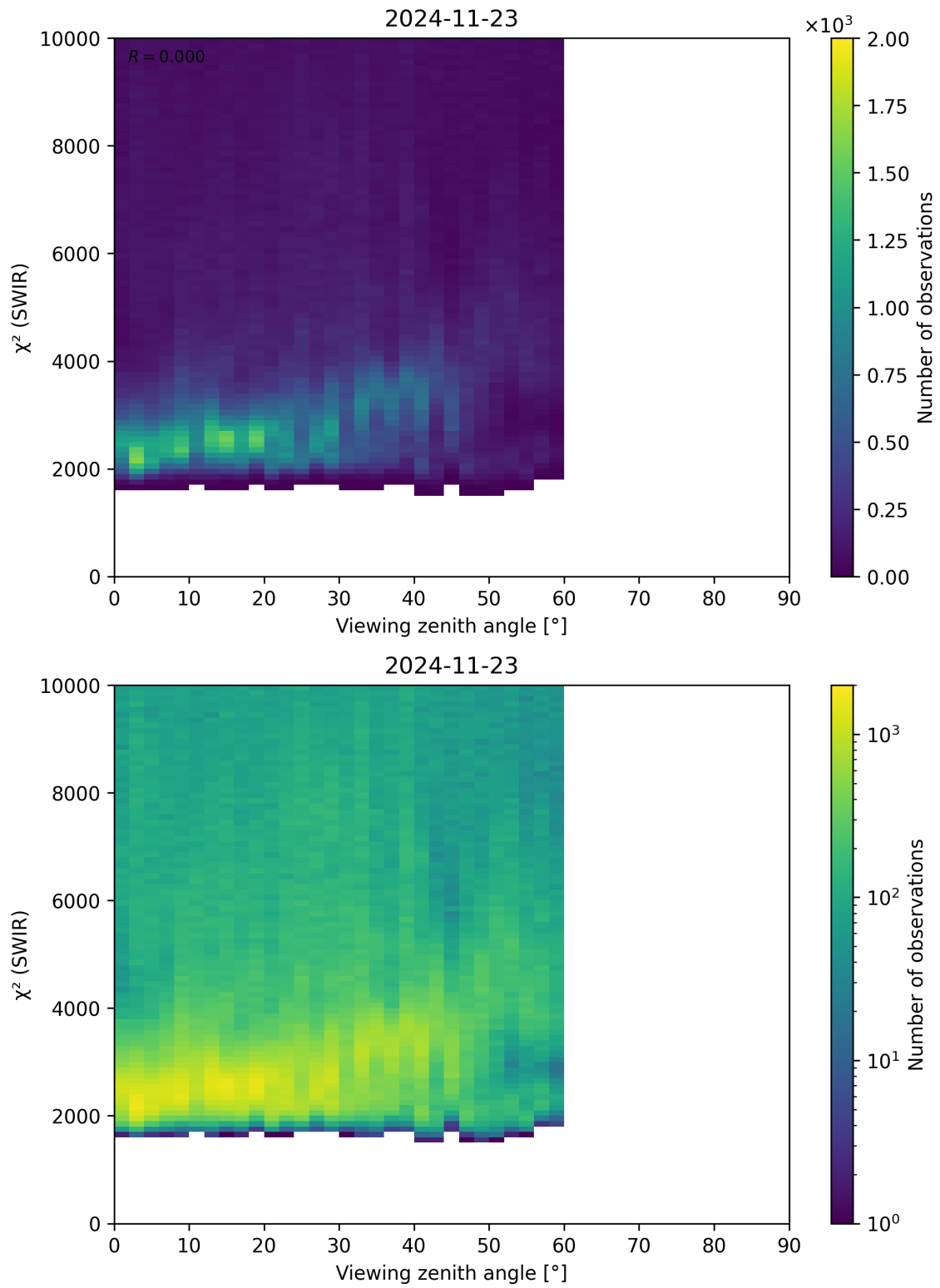
Figure 106: Scatter density plot of “Viewing zenith angle” against “ \chi^2 (SWIR)” for 2024-11-22 to 2024-11-24.
