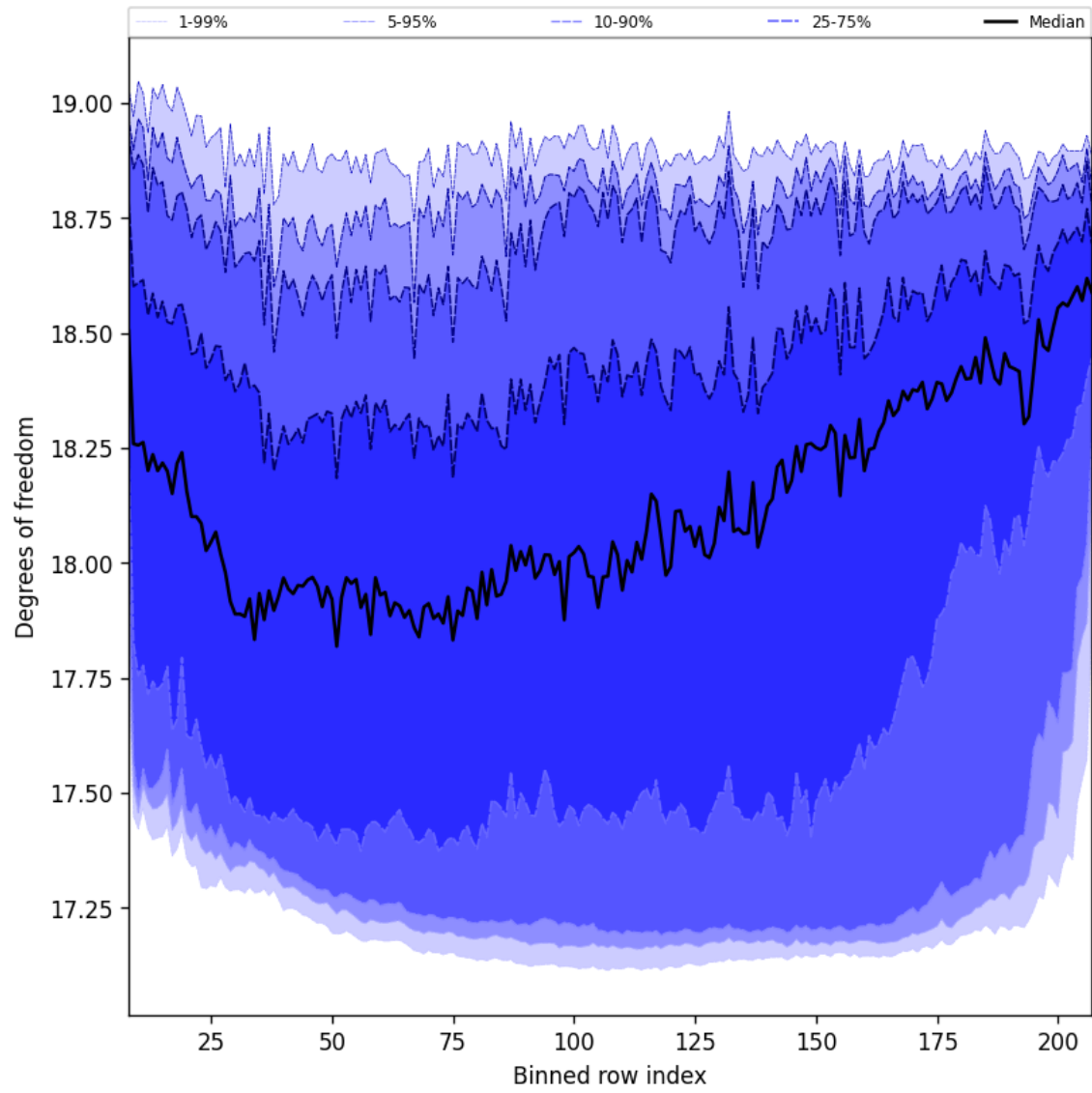
Figure 41: Along track statistics of “Degrees of freedom” for 2024-11-22 to 2024-11-24
