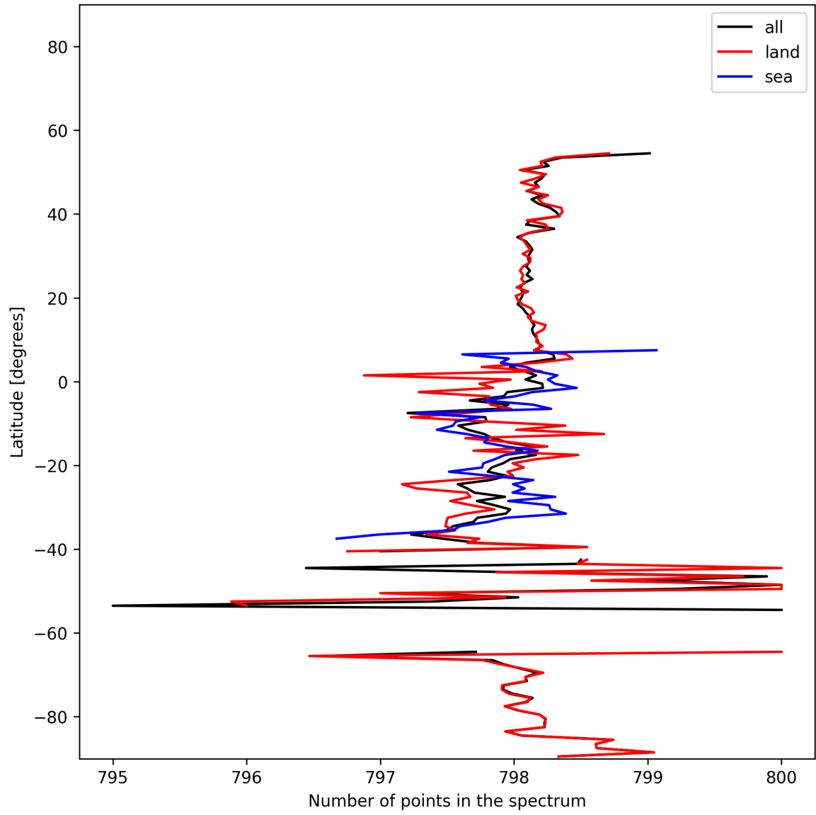
Figure 15: Zonal average of “Number of points in the spectrum” for 2024-11-22 to 2024-11-24.
