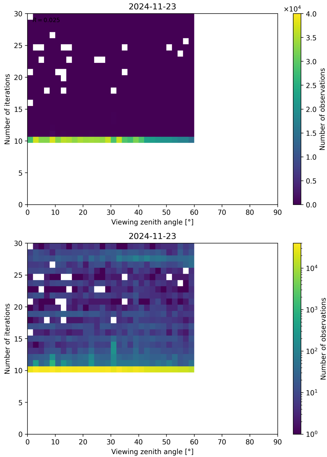
Figure 113: Scatter density plot of “Viewing zenith angle” against “Number of iterations” for 2024-11-22 to 2024-11-24.
