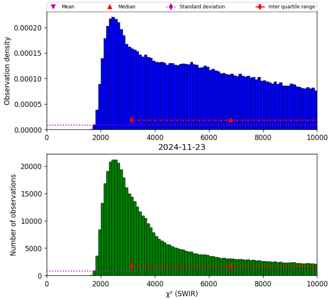
Figure 28: Histogram of “ \chi^2 (SWIR)” for 2024-11-22 to 2024-11-24
