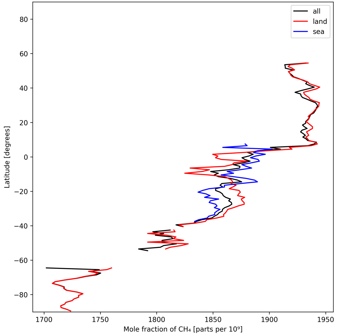
Figure 12: Zonal average of “Mole fraction of CH 4 ” for 2024-11-22 to 2024-11-24.
