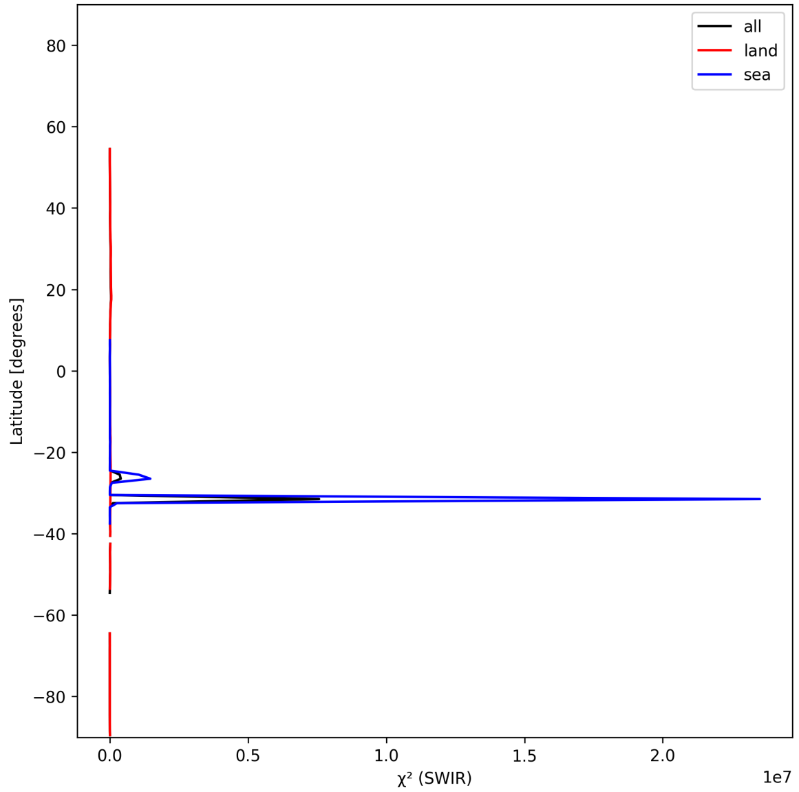
Figure 17: Zonal average of “ \chi^2 (SWIR)” for 2024-11-22 to 2024-11-24.
