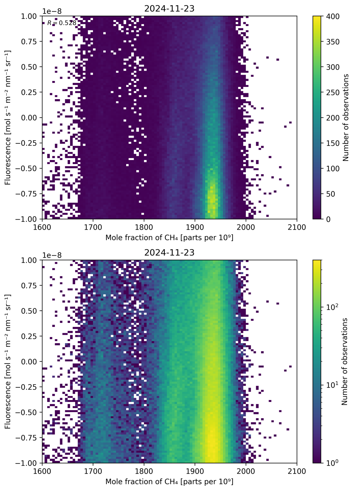
Figure 73: Scatter density plot of “Mole fraction of \text{CH}_4 ” against “Fluorescence” for 2024-11-22 to 2024-11-24.
