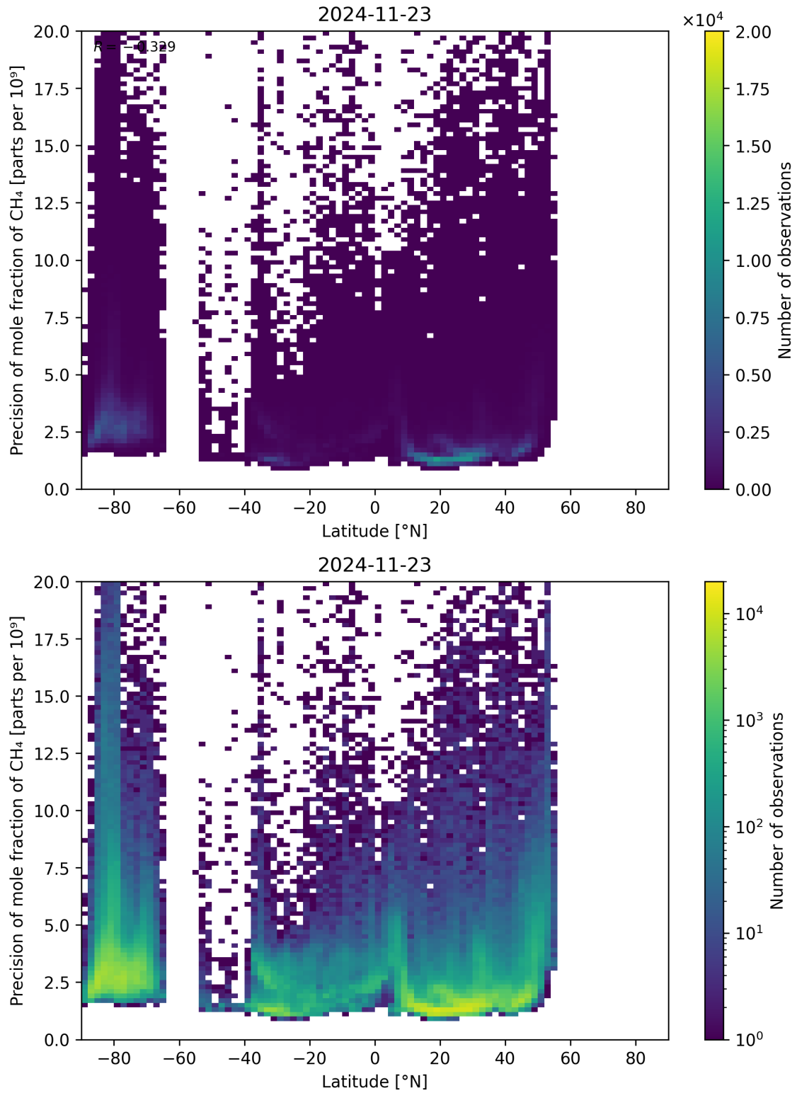
Figure 59: Scatter density plot of “Latitude” against “Precision of mole fraction of CH 4 ” for 2024-11-22 to 2024-11-24.
