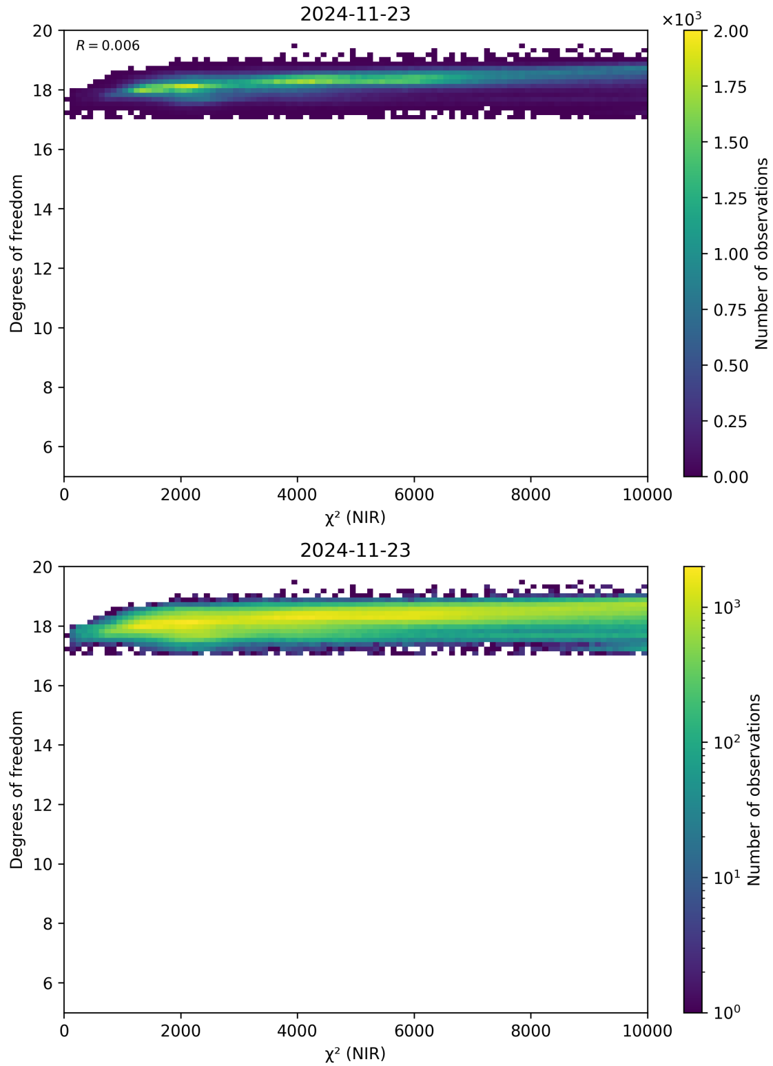
Figure 44: Scatter density plot of “ \chi^2 (NIR)” against “Degrees of freedom” for 2024-11-22 to 2024-11-24.
