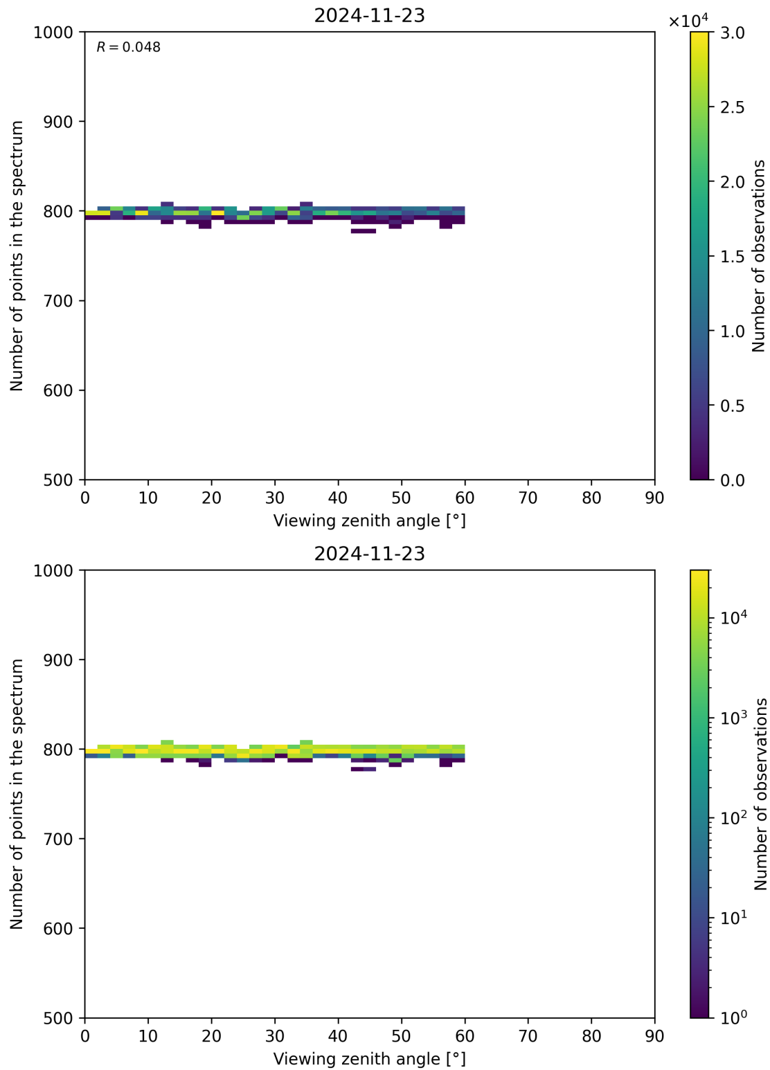
Figure 114: Scatter density plot of “Viewing zenith angle” against “Number of points in the spectrum” for 2024-11-22 to 2024-11-24.
