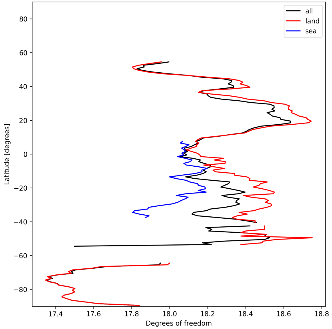
Figure 19: Zonal average of “Degrees of freedom” for 2024-11-22 to 2024-11-24.
