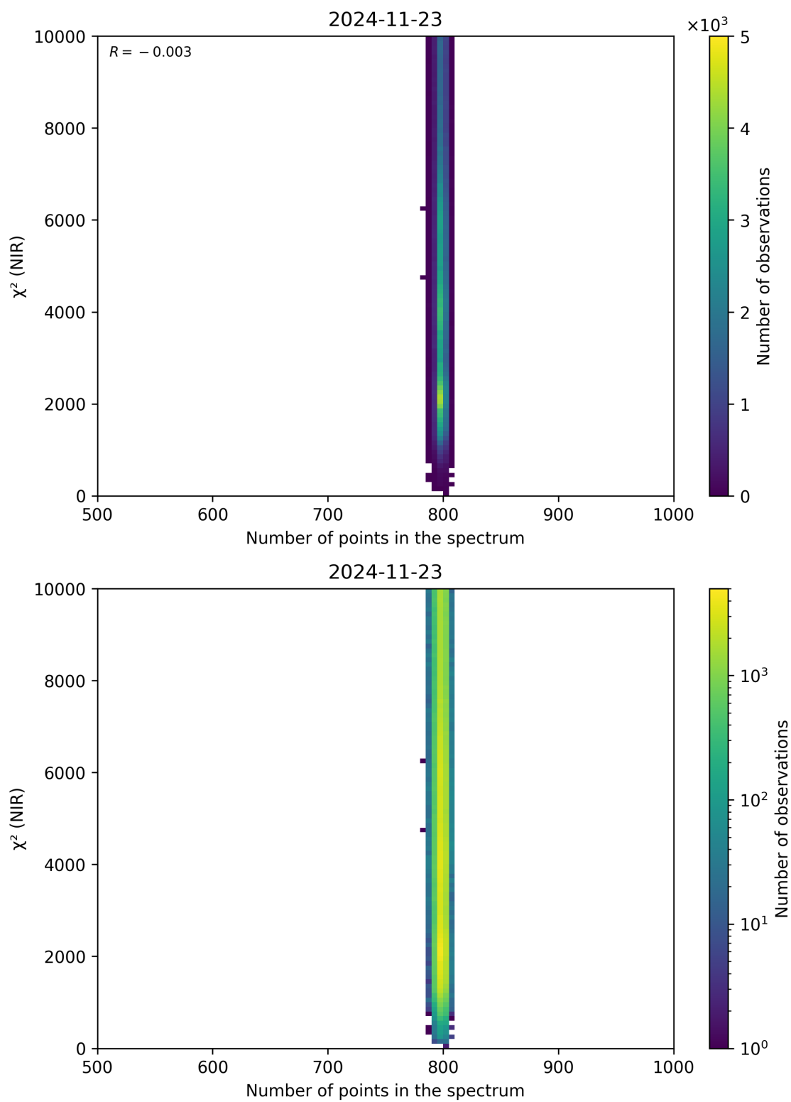
Figure 88: Scatter density plot of “Number of points in the spectrum” against “ \chi^2 (NIR)” for 2024-11-22 to 2024-11-24.
