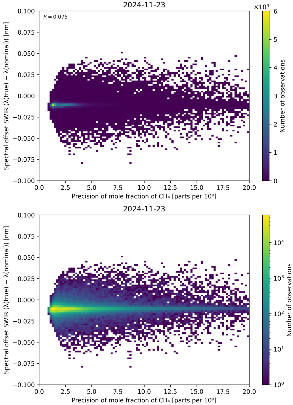
Figure 85: Scatter density plot of “Precision of mole fraction of \text{CH}_4 ” against “Spectral offset SWIR ( \lambda_{\text{true}} - \lambda_{\text{nominal}} )” for 2024-11-22 to 2024-11-24.
