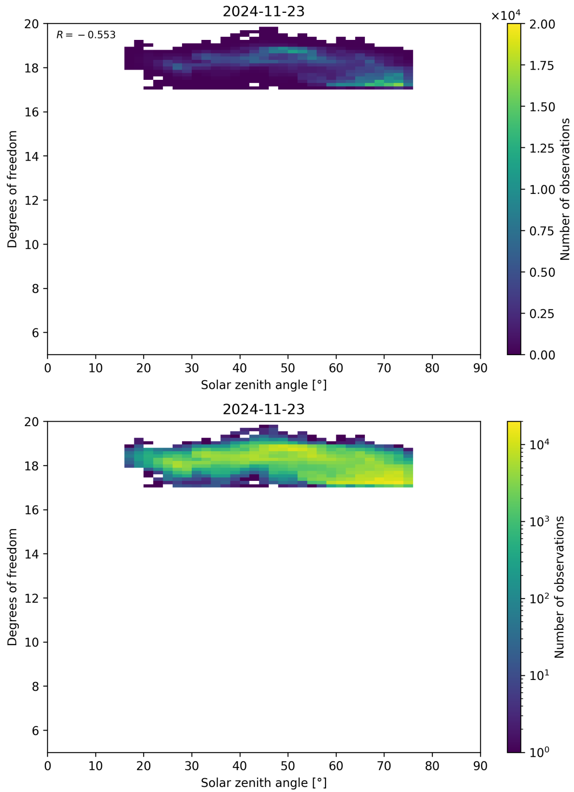
Figure 96: Scatter density plot of “Solar zenith angle” against “Degrees of freedom” for 2024-11-22 to 2024-11-24.
