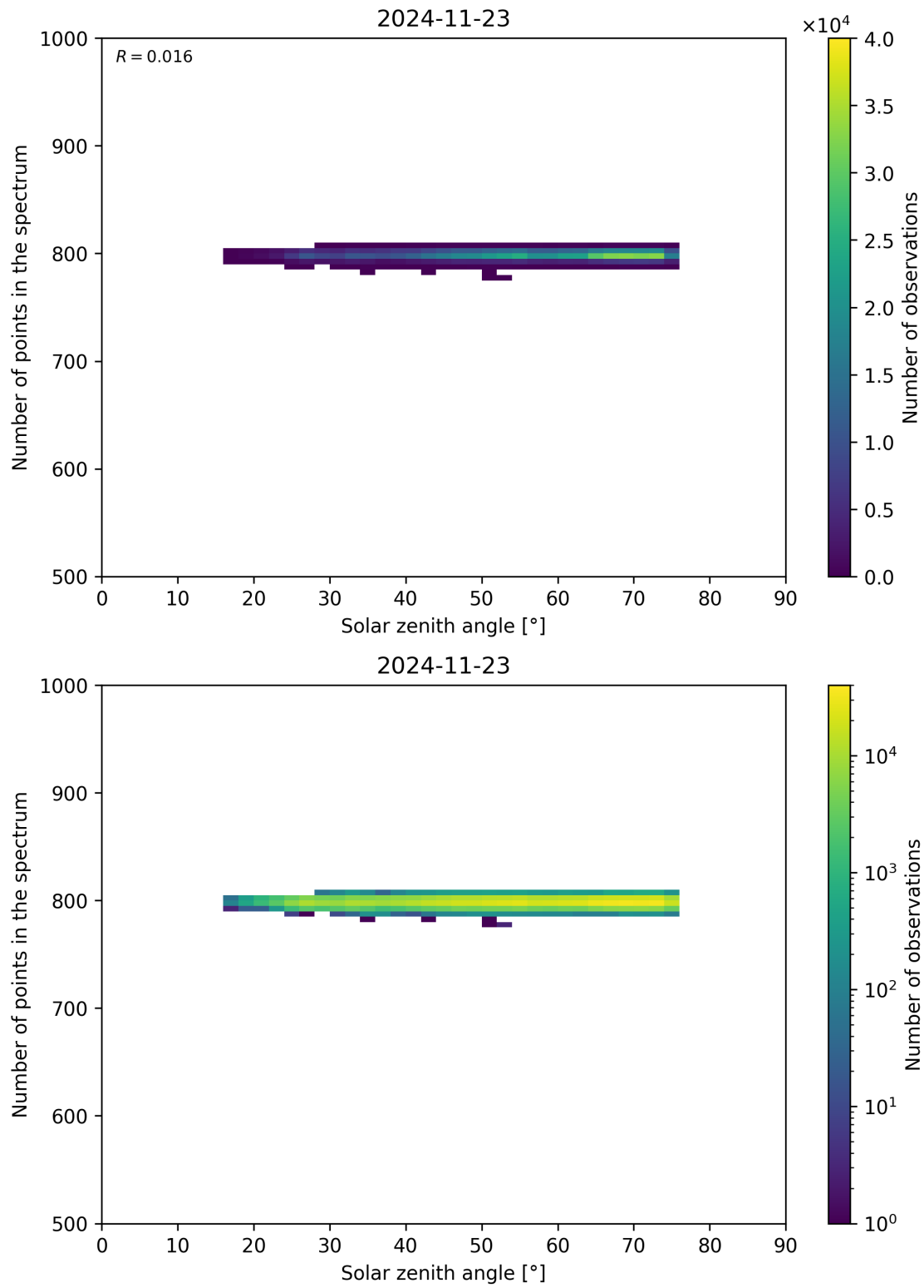
Figure 103: Scatter density plot of “Solar zenith angle” against “Number of points in the spectrum” for 2024-11-22 to 2024-11-24.
