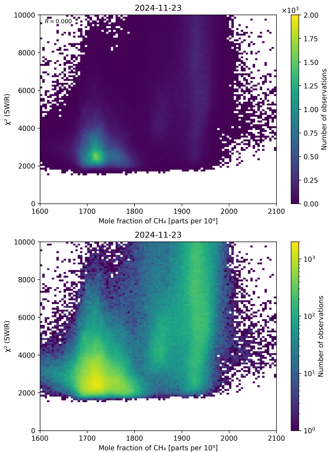
Figure 71: Scatter density plot of “Mole fraction of CH 4 ” against “ \chi^2 (SWIR)” for 2024-11-22 to 2024-11-24.
