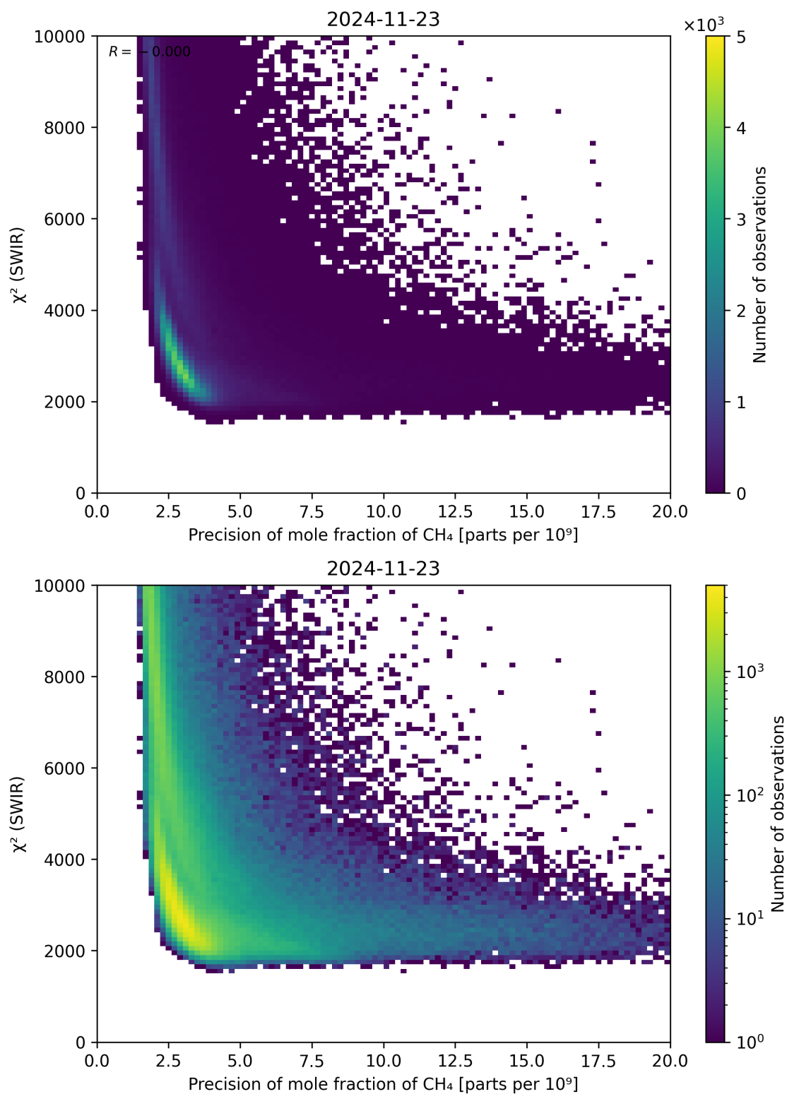
Figure 79: Scatter density plot of “Precision of mole fraction of CH 4 ” against “ \chi^2 (SWIR)” for 2024-11-22 to 2024-11-24.
