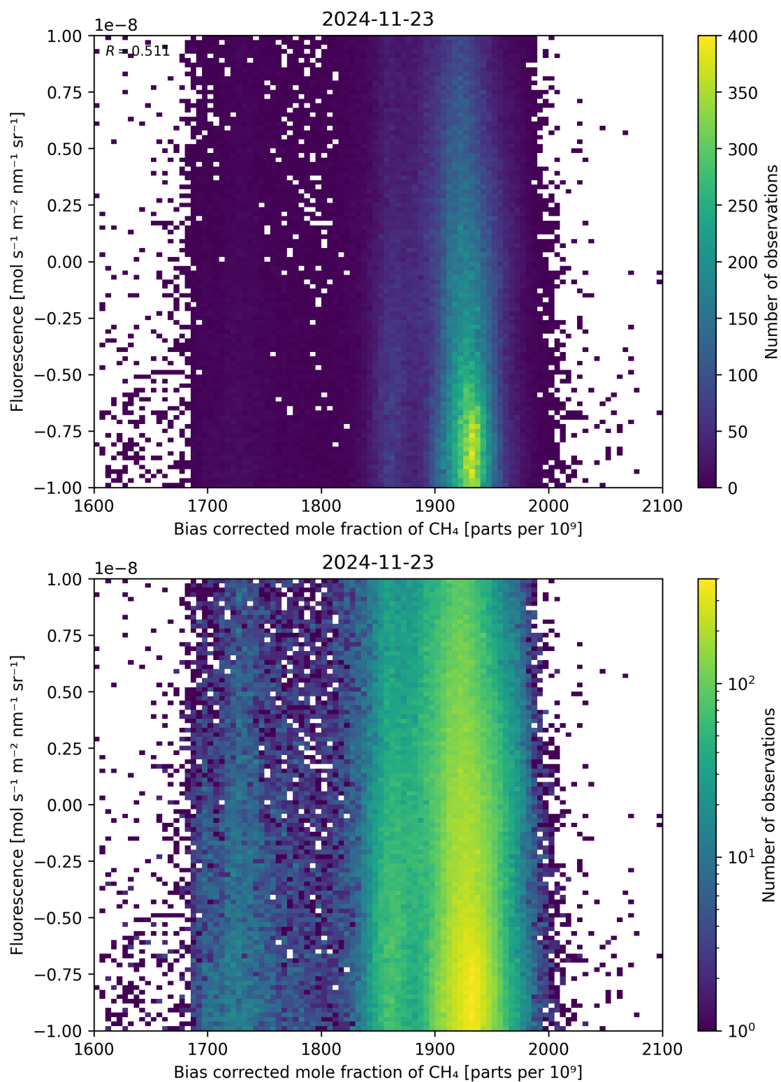
Figure 66: Scatter density plot of “Bias corrected mole fraction of \text{CH}_4 ” against “Fluorescence” for 2024-11-22 to 2024-11-24.
