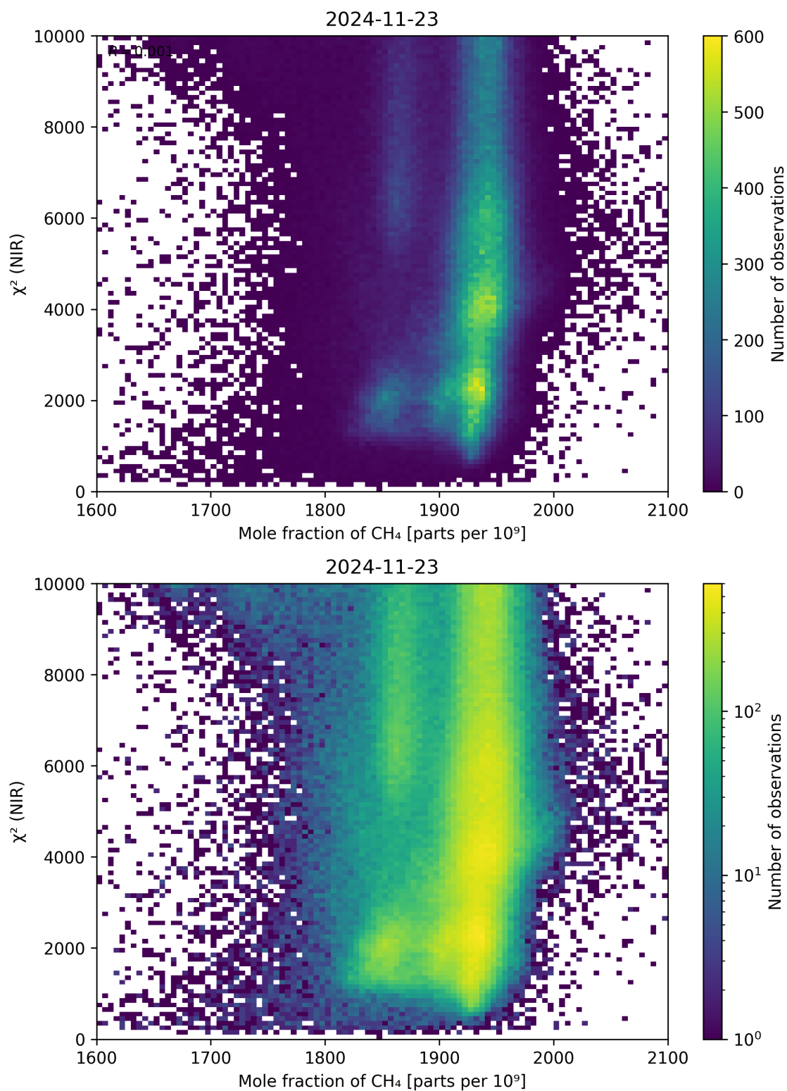
Figure 70: Scatter density plot of “Mole fraction of \text{CH}_4 ” against “ \chi^2 (NIR)” for 2024-11-22 to 2024-11-24.
