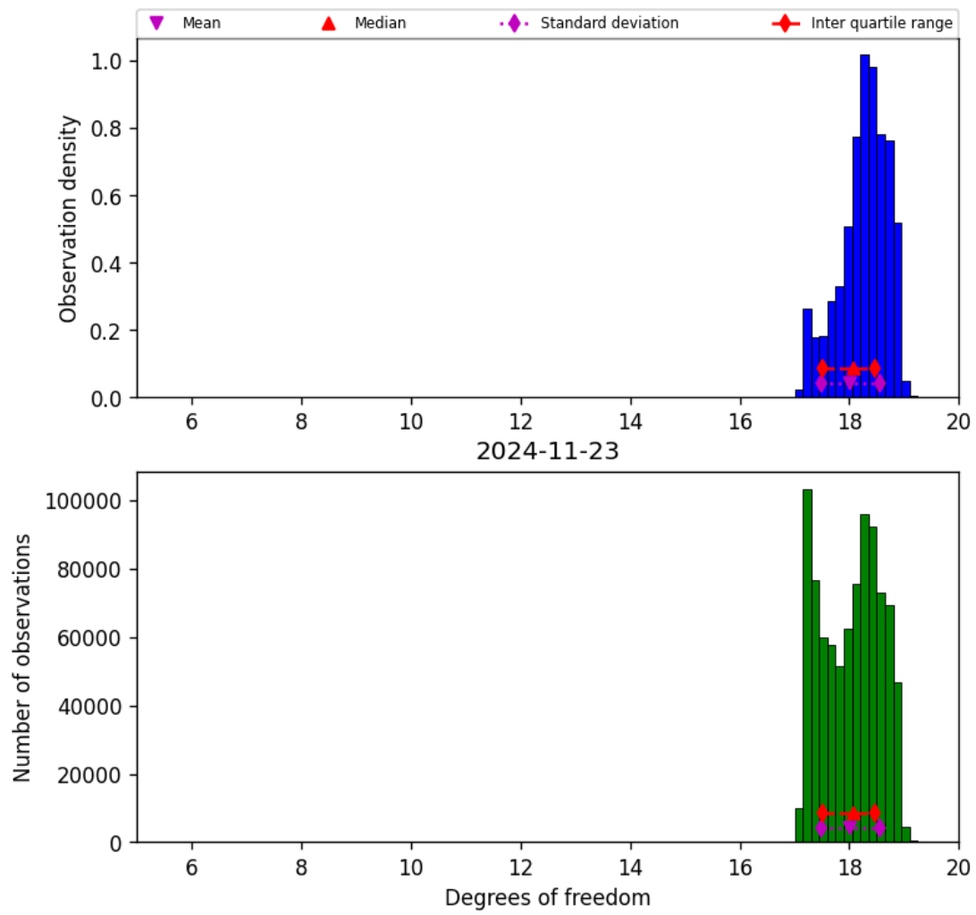
Figure 30: Histogram of “Degrees of freedom” for 2024-11-22 to 2024-11-24
