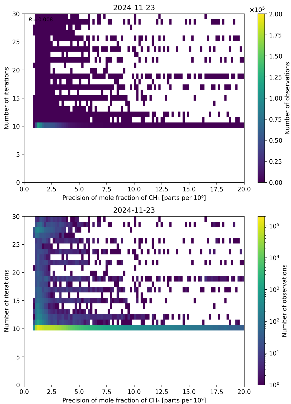
Figure 83: Scatter density plot of “Precision of mole fraction of \text{CH}_4 ” against “Number of iterations” for 2024-11-22 to 2024-11-24.
