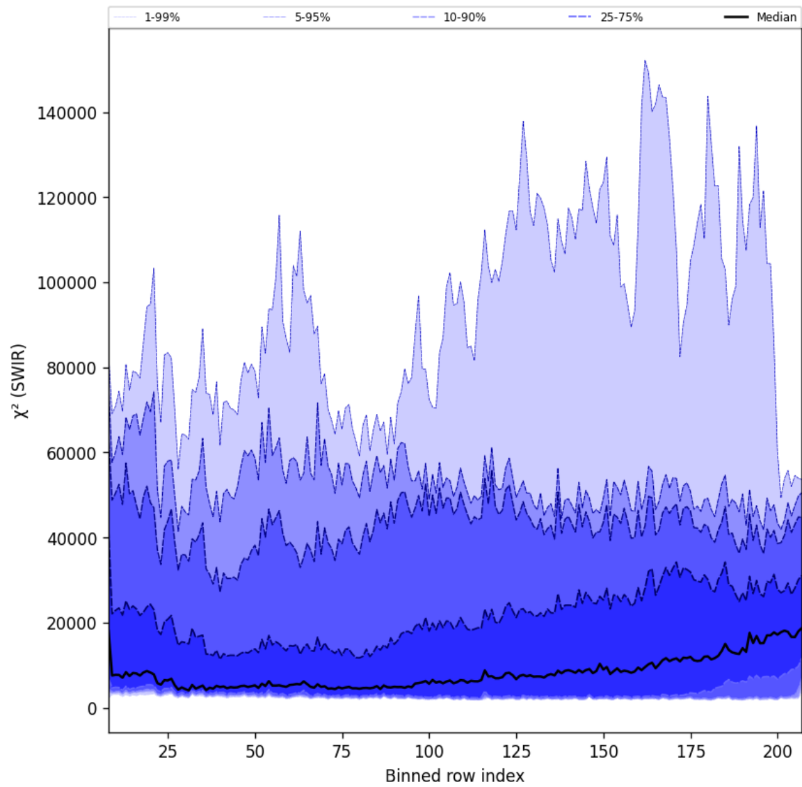
Figure 39: Along track statistics of “ \chi^2 (SWIR)” for 2024-11-22 to 2024-11-24
