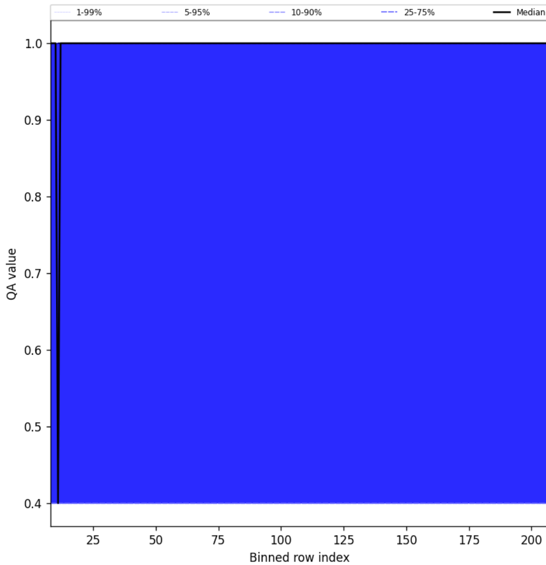
Figure 33: Along track statistics of “QA value” for 2024-11-22 to 2024-11-24
