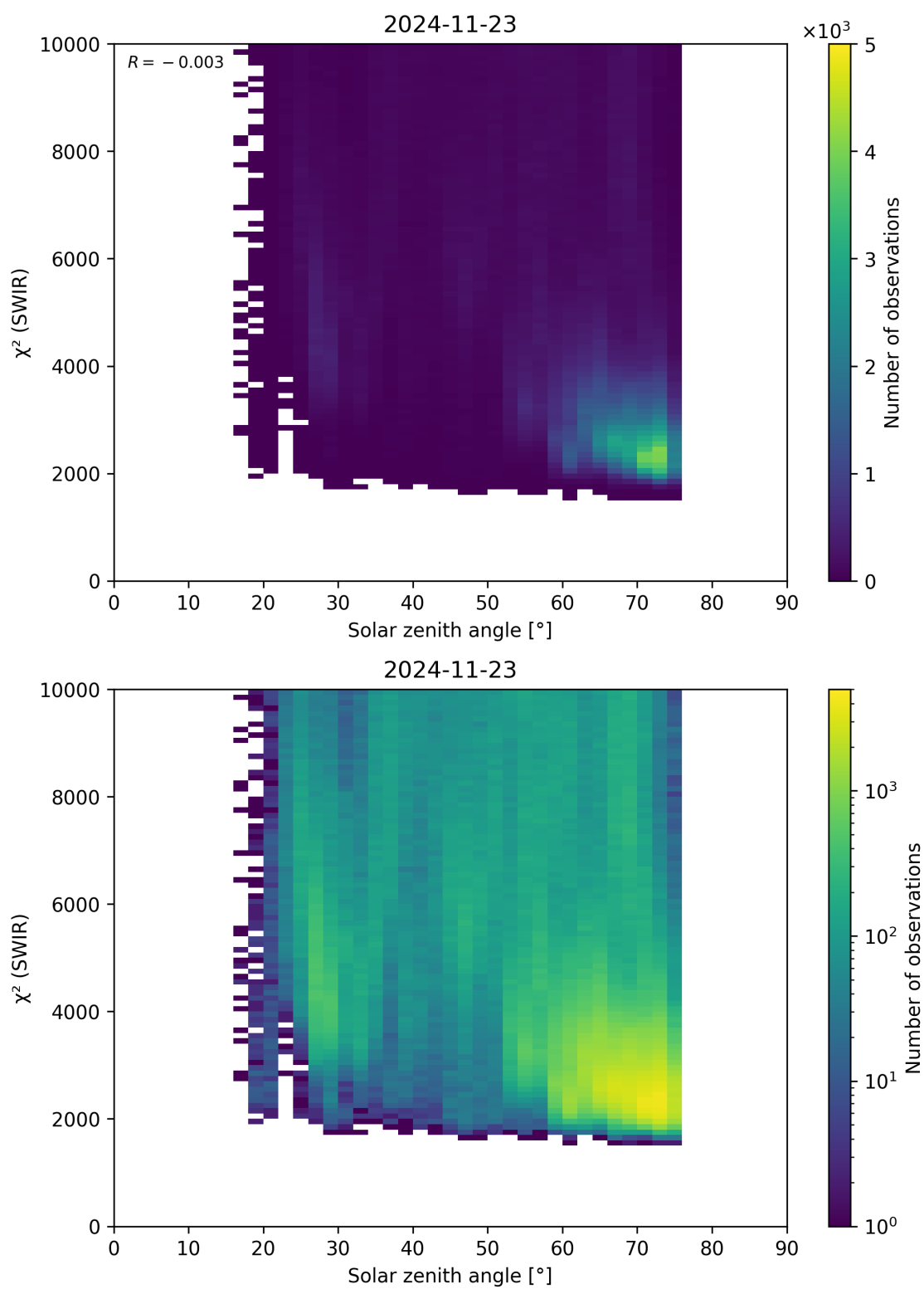
Figure 95: Scatter density plot of “Solar zenith angle” against “ \chi^2 (SWIR)” for 2024-11-22 to 2024-11-24.
