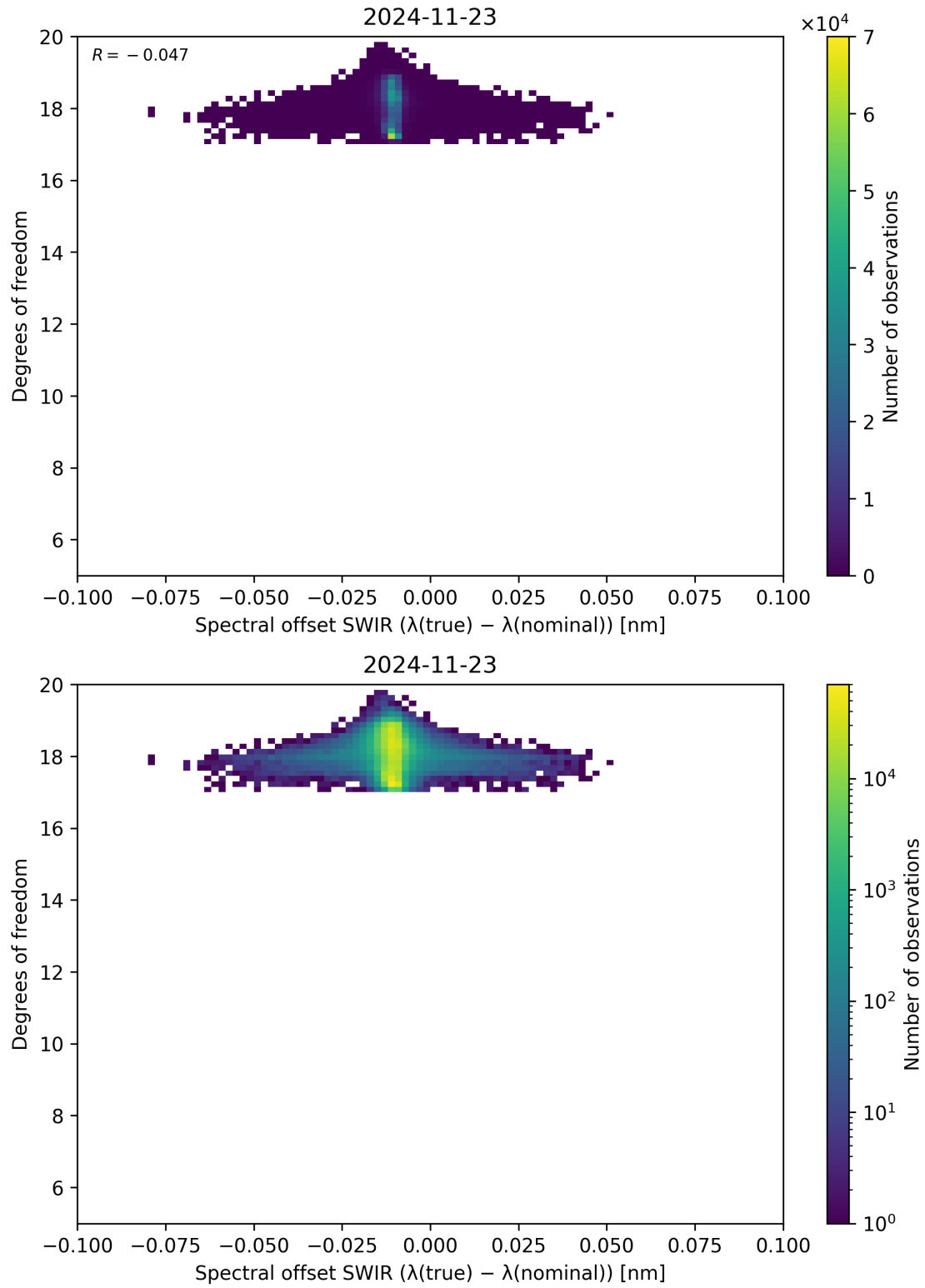
Figure 119: Scatter density plot of “Spectral offset SWIR ( \lambda_{\text{true}} - \lambda_{\text{nominal}} )” against “Degrees of freedom” for 2024-11-22 to 2024-11-24.
