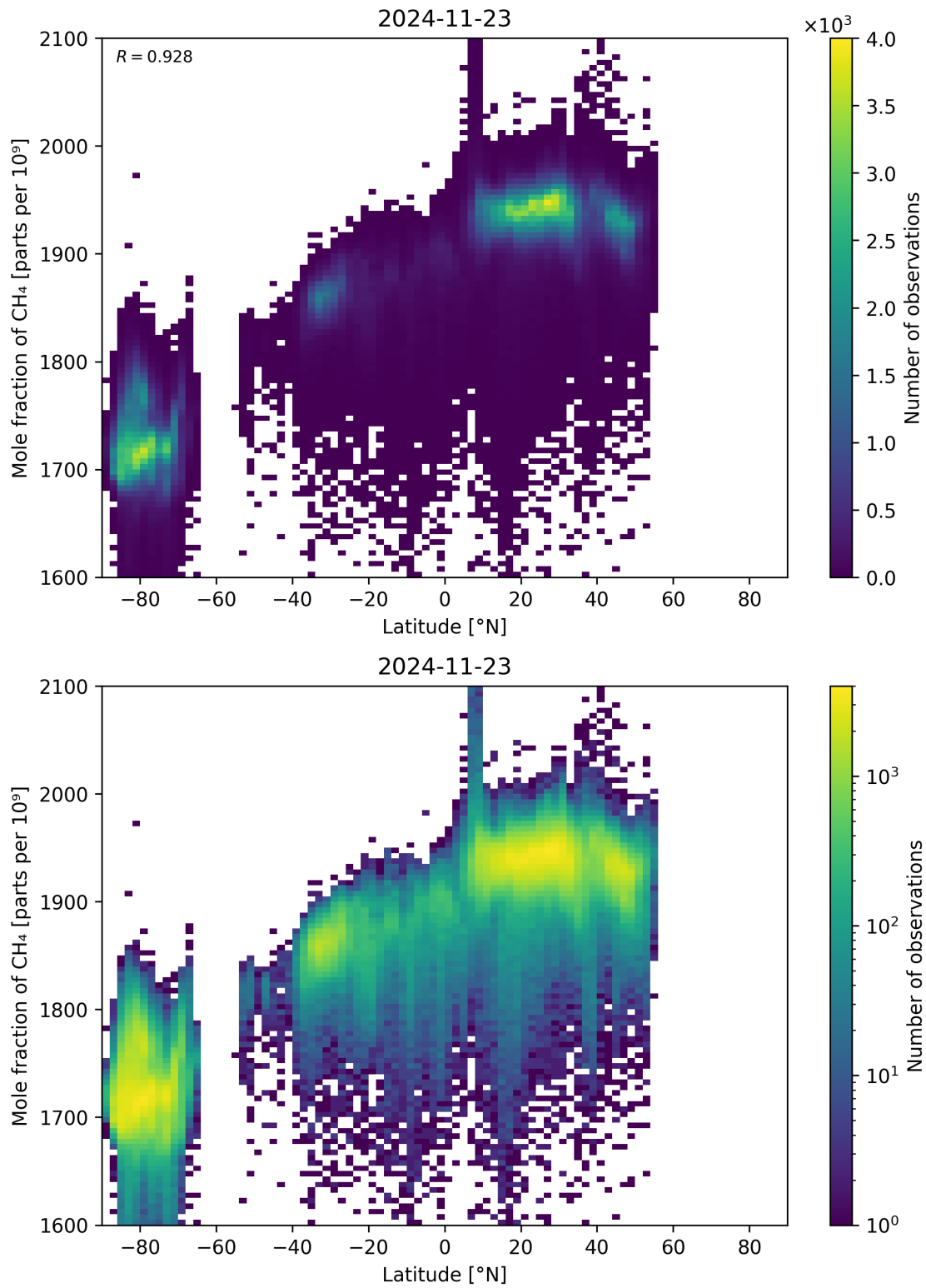
Figure 57: Scatter density plot of “Latitude” against “Mole fraction of \text{CH}_4 ” for 2024-11-22 to 2024-11-24.
