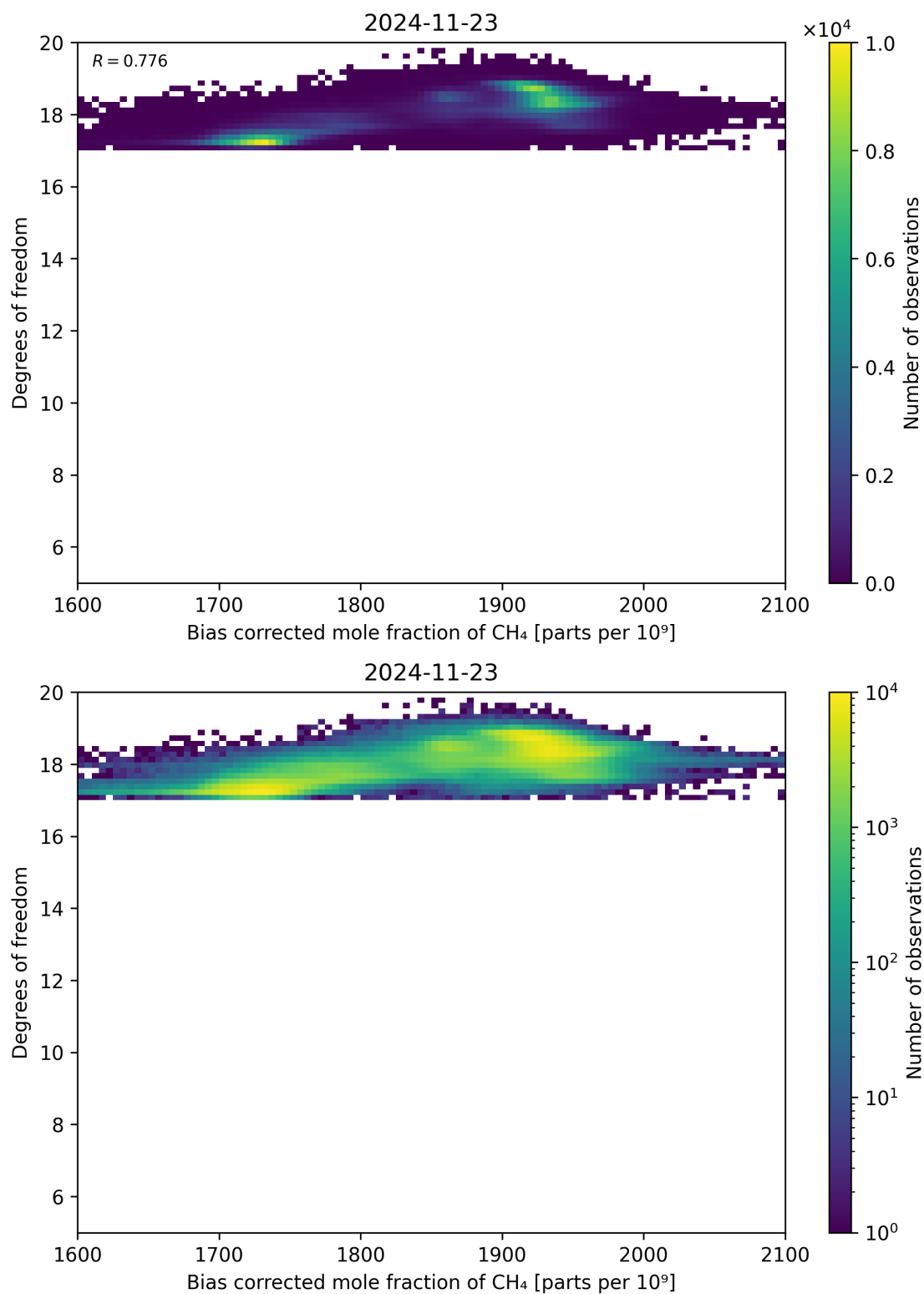
Figure 65: Scatter density plot of “Bias corrected mole fraction of CH 4 ” against “Degrees of freedom” for 2024-11-22 to 2024-11-24.
