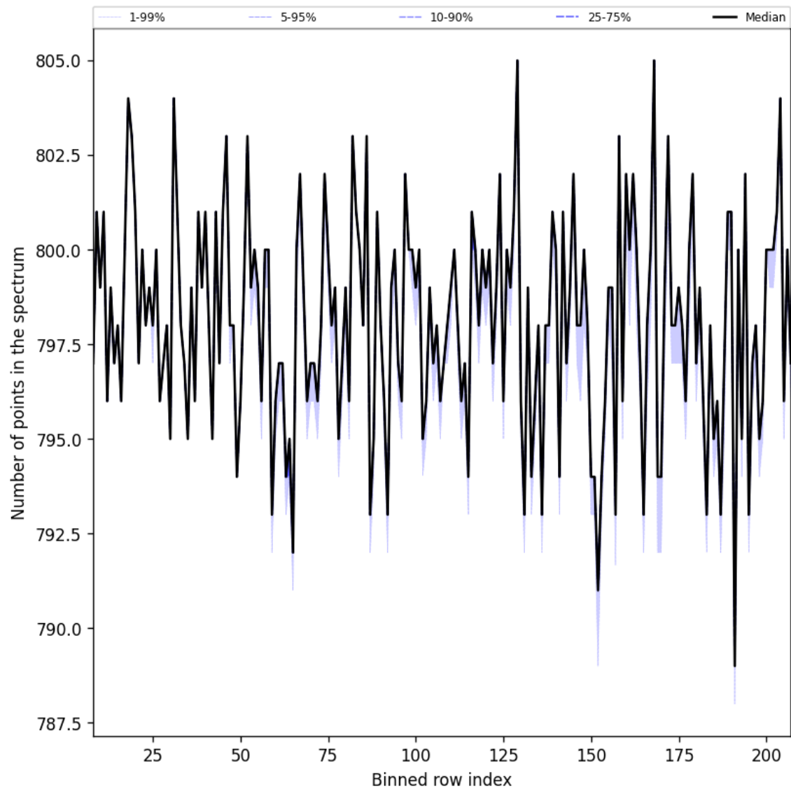
Figure 37: Along track statistics of “Number of points in the spectrum” for 2024-11-22 to 2024-11-24
