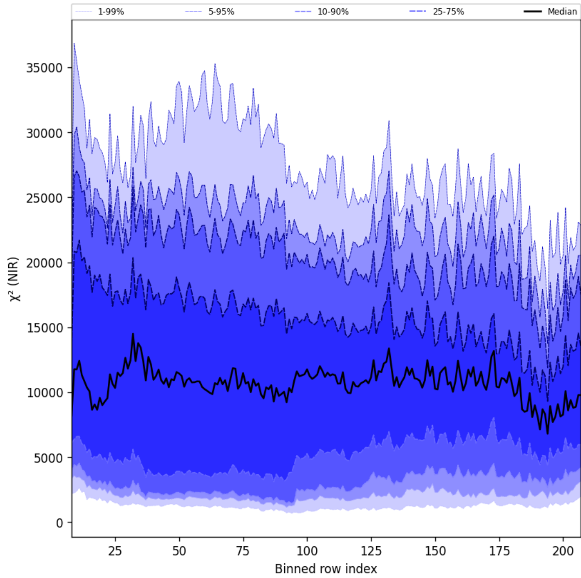
Figure 40: Along track statistics of “ \chi^2 (NIR)” for 2024-11-22 to 2024-11-24
