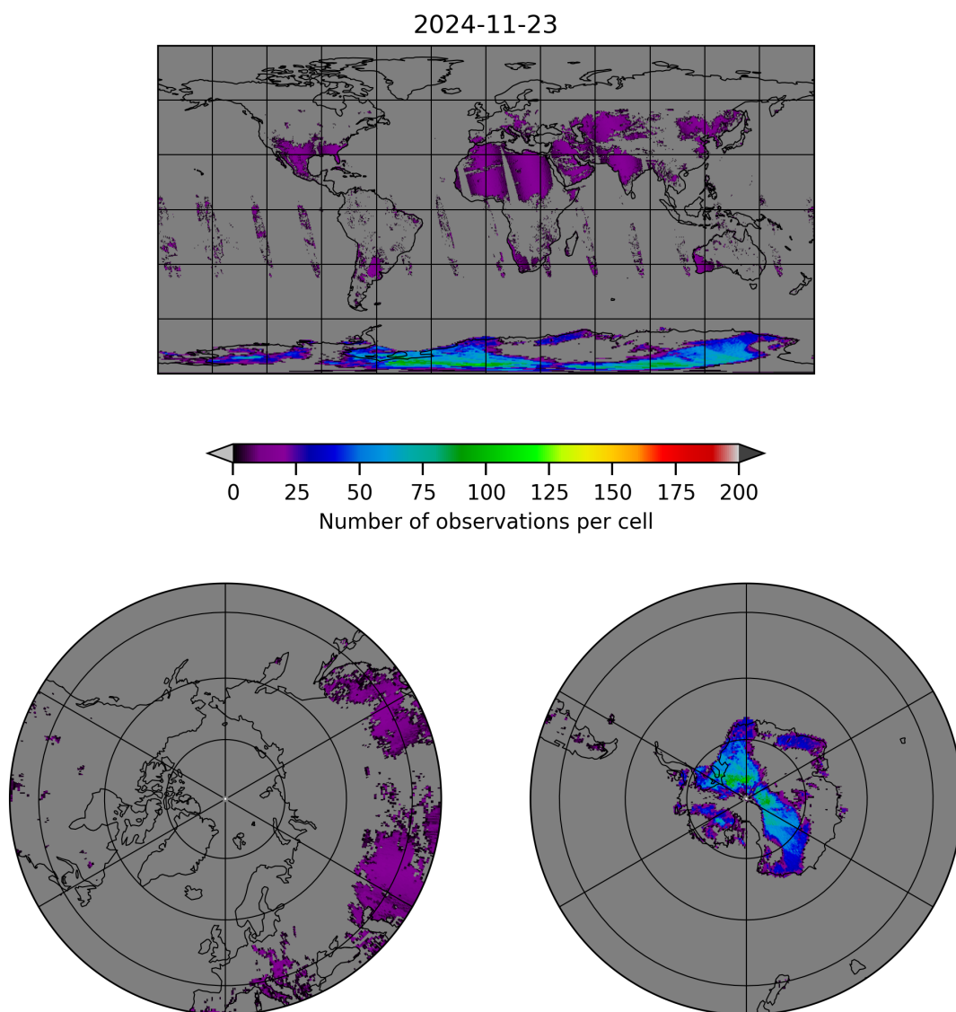
Figure 10: Map of the number of observations for 2024-11-22 to 2024-11-24
