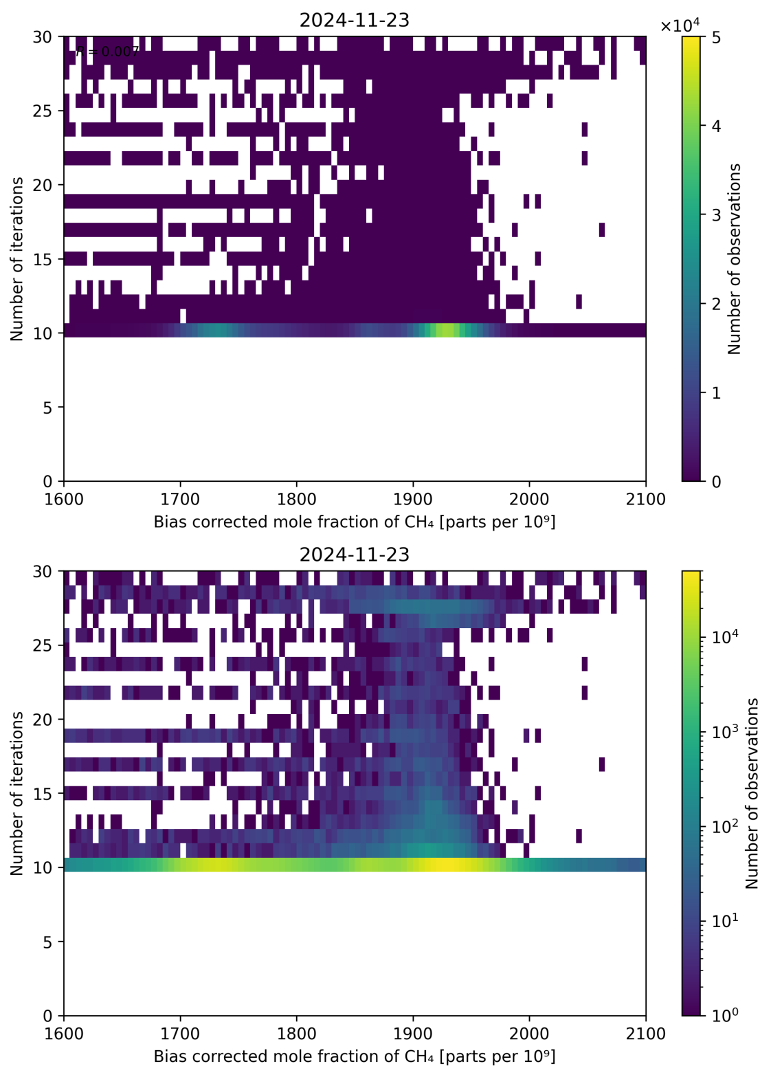
Figure 67: Scatter density plot of “Bias corrected mole fraction of \text{CH}_4 ” against “Number of iterations” for 2024-11-22 to 2024-11-24.
