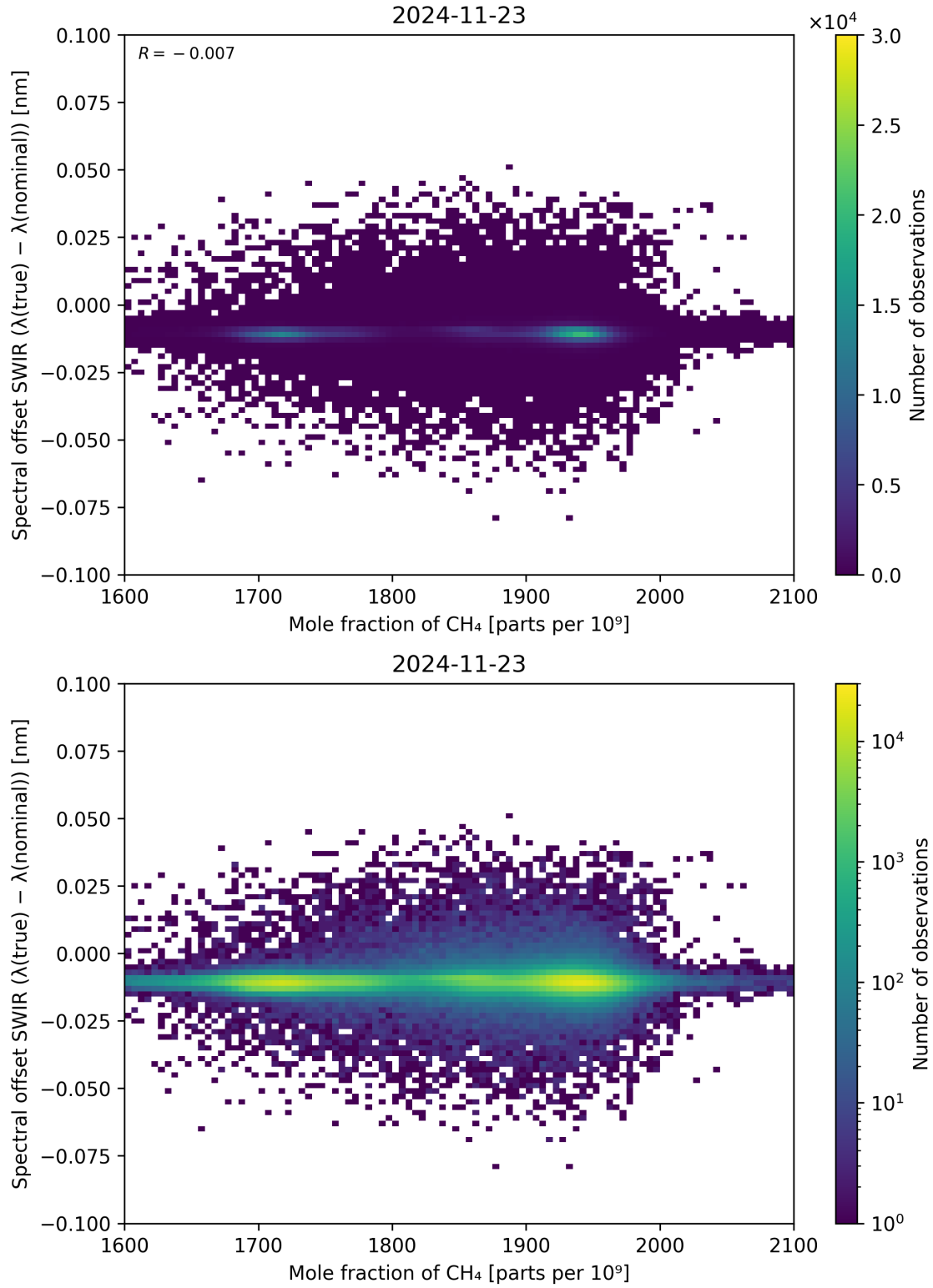
Figure 86: Scatter density plot of “Mole fraction of CH 4 ” against “Spectral offset SWIR ( \lambda_{\text{true}} - \lambda_{\text{nominal}} )” for 2024-11-22 to 2024-11-24.
