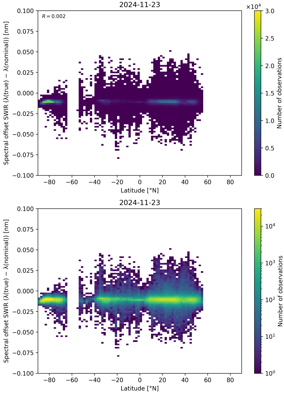
Figure 62: Scatter density plot of “Latitude” against “Spectral offset SWIR ( \lambda_{\text{true}} - \lambda_{\text{nominal}} )” for 2024-11-22 to 2024-11-24.
