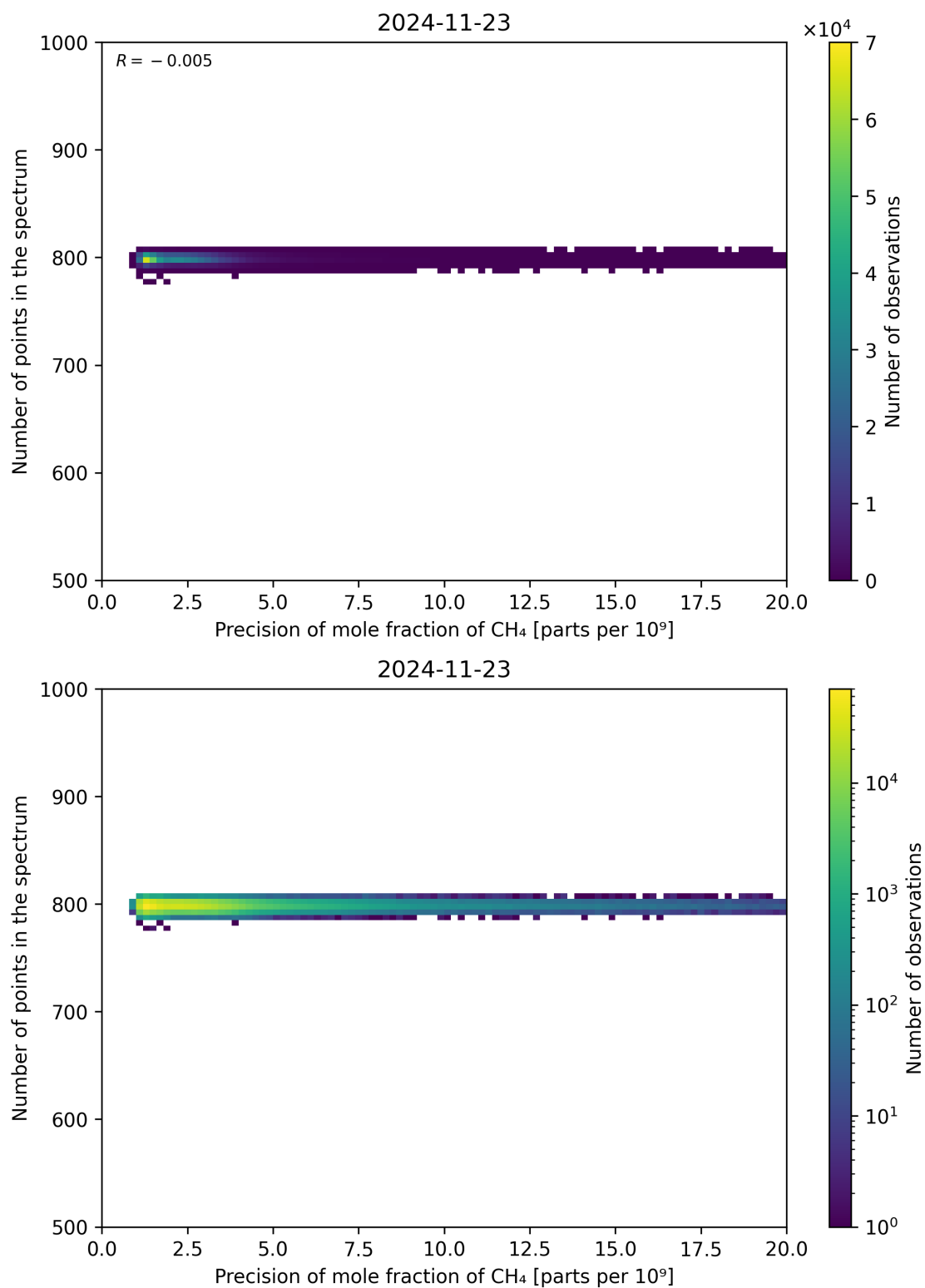
Figure 84: Scatter density plot of “Precision of mole fraction of CH 4 ” against “Number of points in the spectrum” for 2024-11-22 to 2024-11-24.
