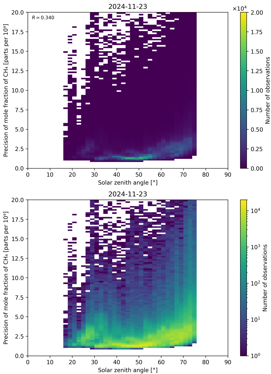
Figure 101: Scatter density plot of “Solar zenith angle” against “Precision of mole fraction of \text{CH}_4 ” for 2024-11-22 to 2024-11-24.
