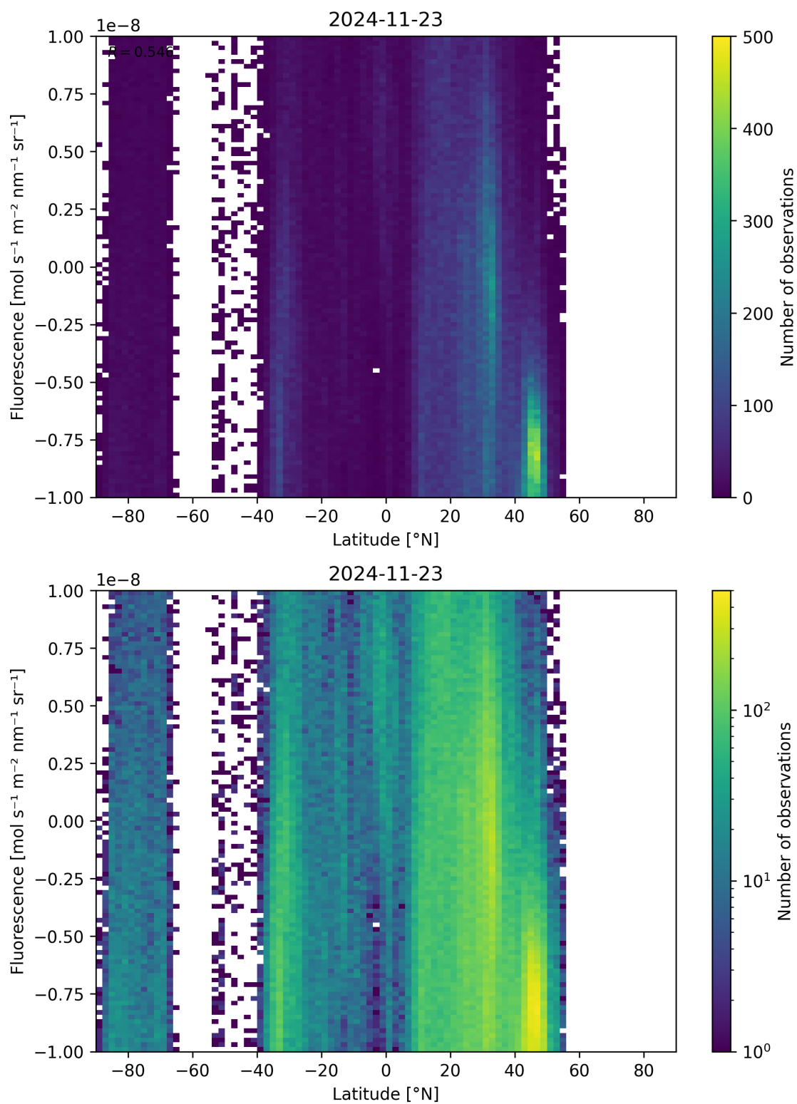
Figure 56: Scatter density plot of “Latitude” against “Fluorescence” for 2024-11-22 to 2024-11-24.
