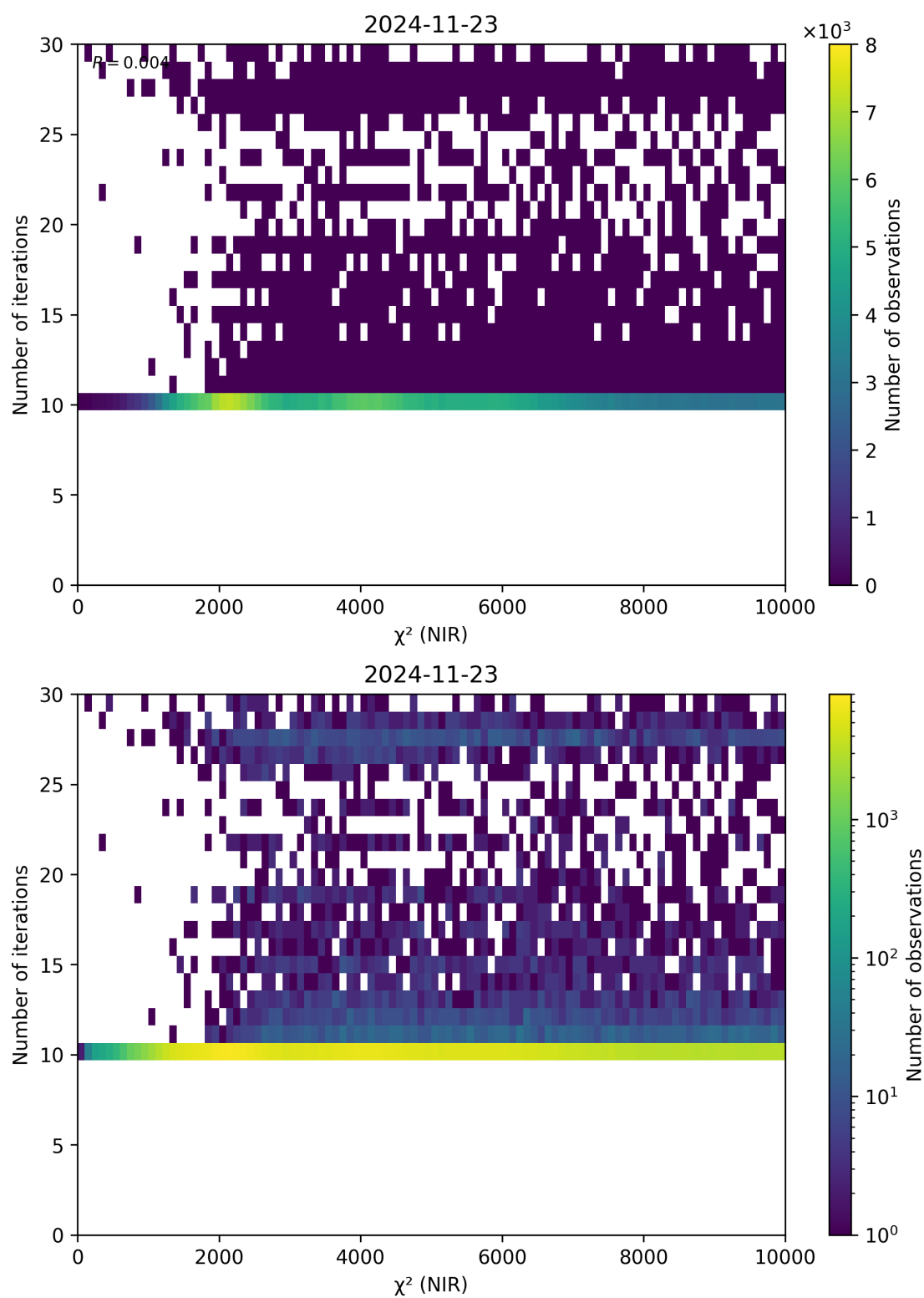
Figure 46: Scatter density plot of “ \chi^2 (NIR)” against “Number of iterations” for 2024-11-22 to 2024-11-24.
