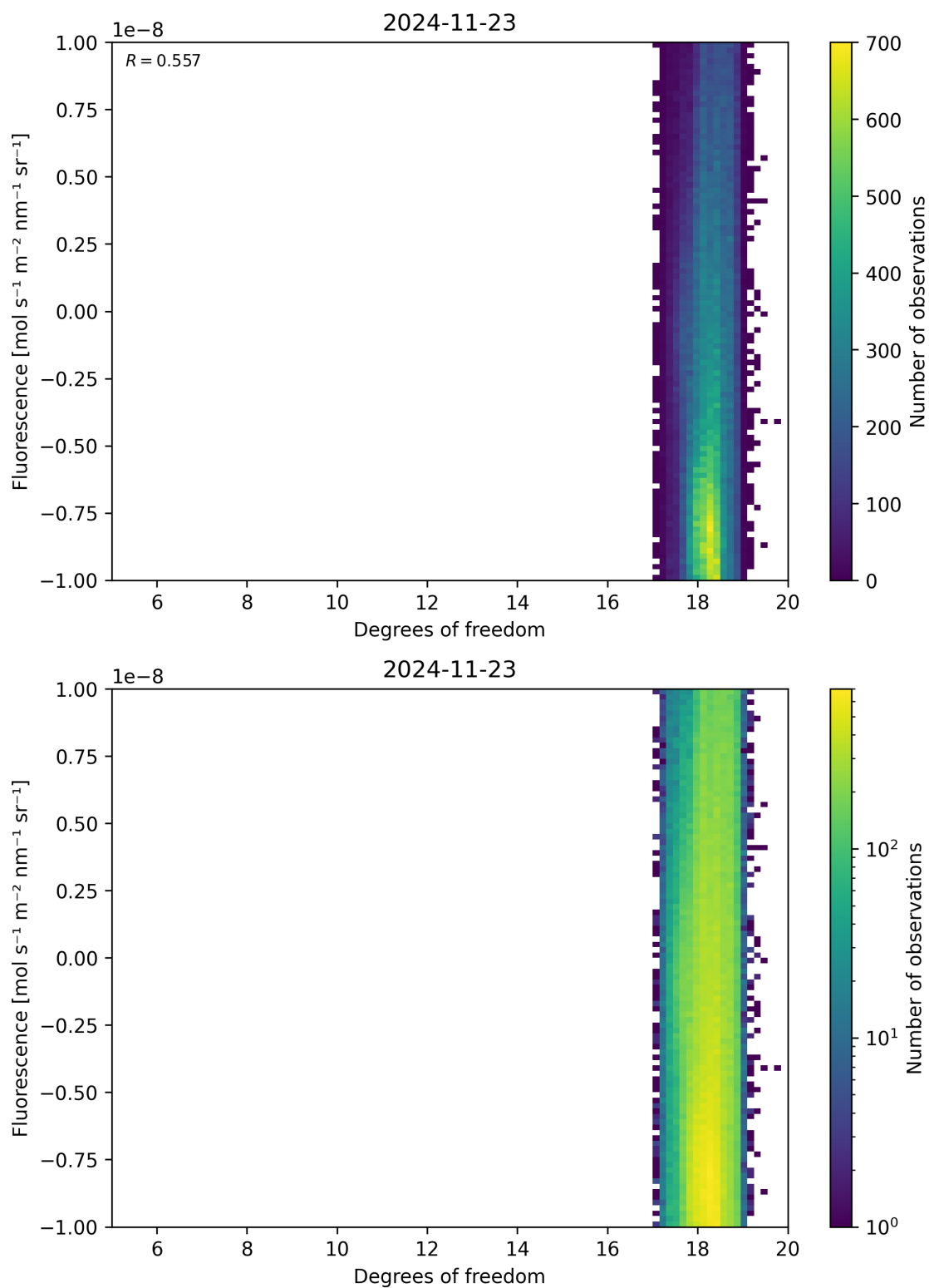
Figure 51: Scatter density plot of “Degrees of freedom” against “Fluorescence” for 2024-11-22 to 2024-11-24.
