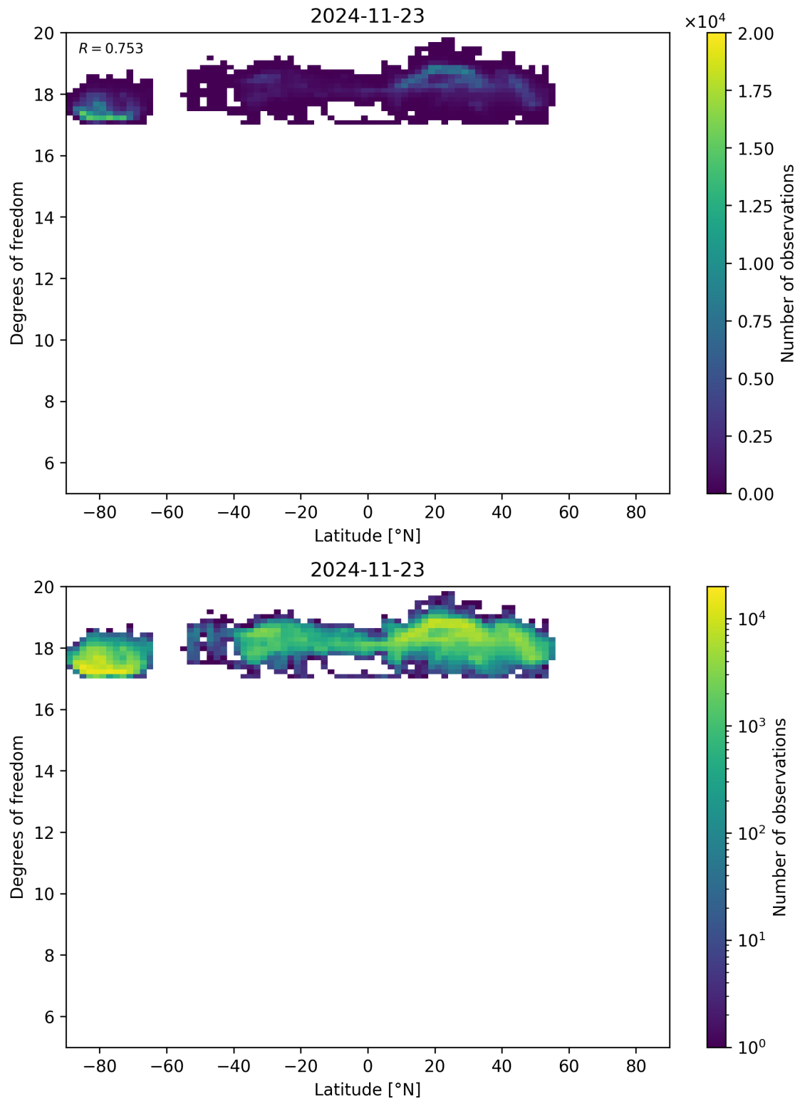
Figure 55: Scatter density plot of “Latitude” against “Degrees of freedom” for 2024-11-22 to 2024-11-24.
