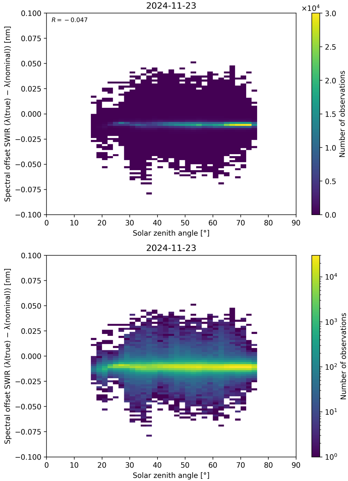
Figure 104: Scatter density plot of “Solar zenith angle” against “Spectral offset SWIR ( \lambda_{\text{true}} - \lambda_{\text{nominal}} )” for 2024-11-22 to 2024-11-24.
