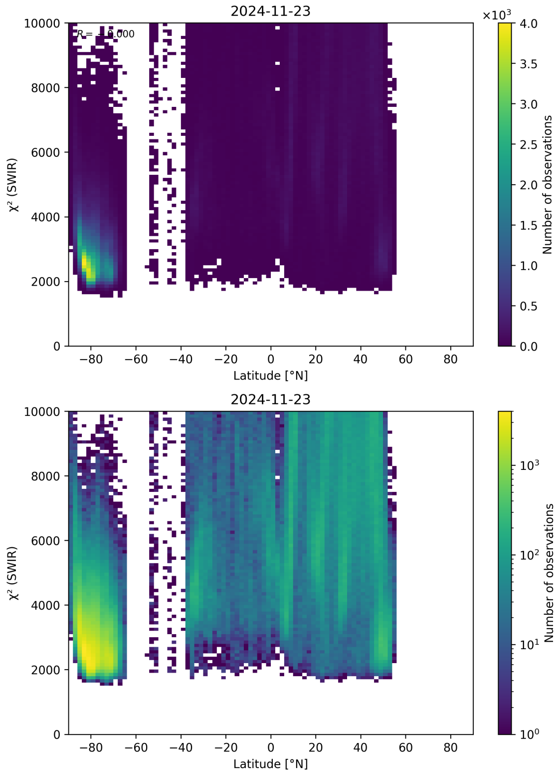
Figure 54: Scatter density plot of “Latitude” against “ \chi^2 (SWIR)” for 2024-11-22 to 2024-11-24.
