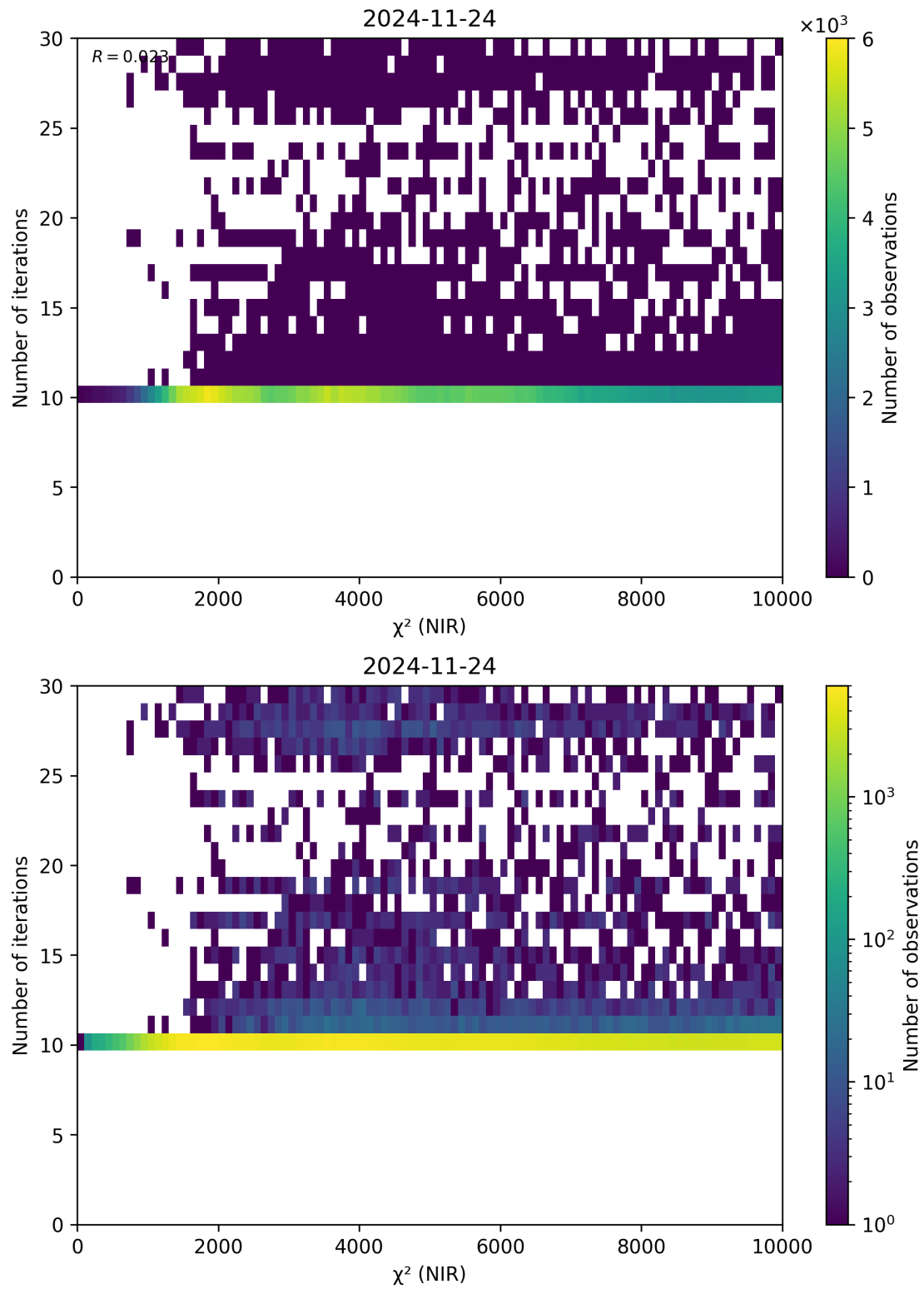
Figure 46: Scatter density plot of “ \chi^2 (NIR)” against “Number of iterations” for 2024-11-23 to 2024-11-25.
