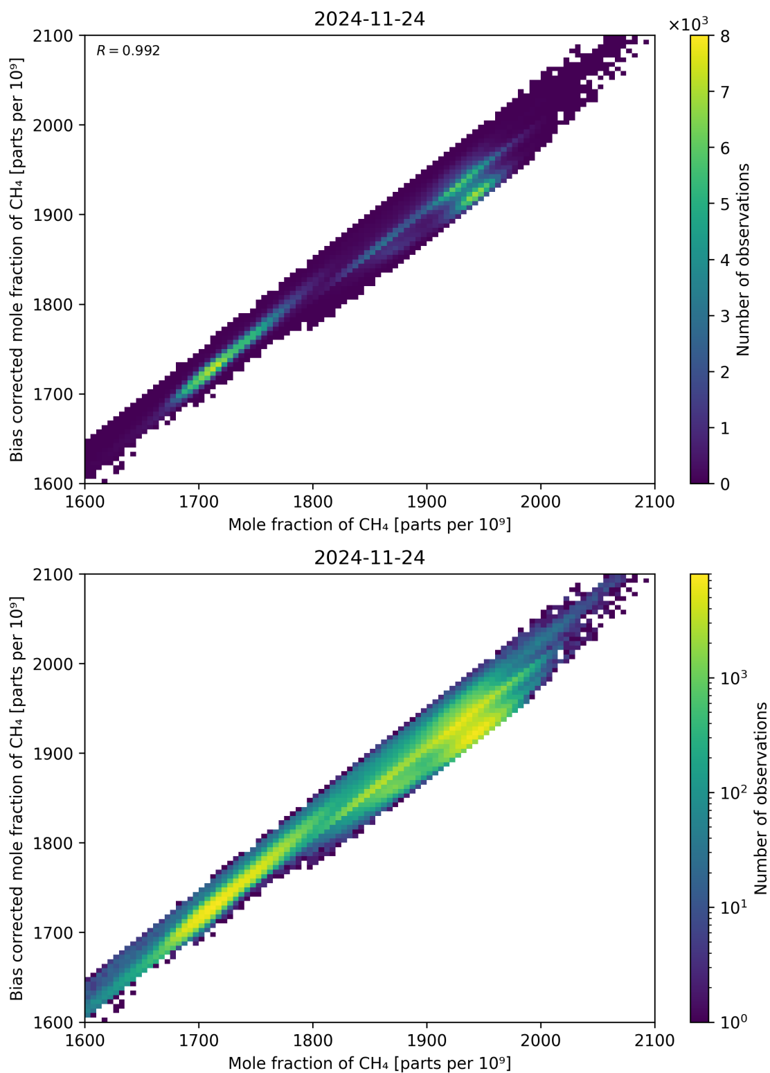
Figure 74: Scatter density plot of “Mole fraction of CH 4 ” against “Bias corrected mole fraction of CH 4 ” for 2024-11-23 to 2024-11-25.
