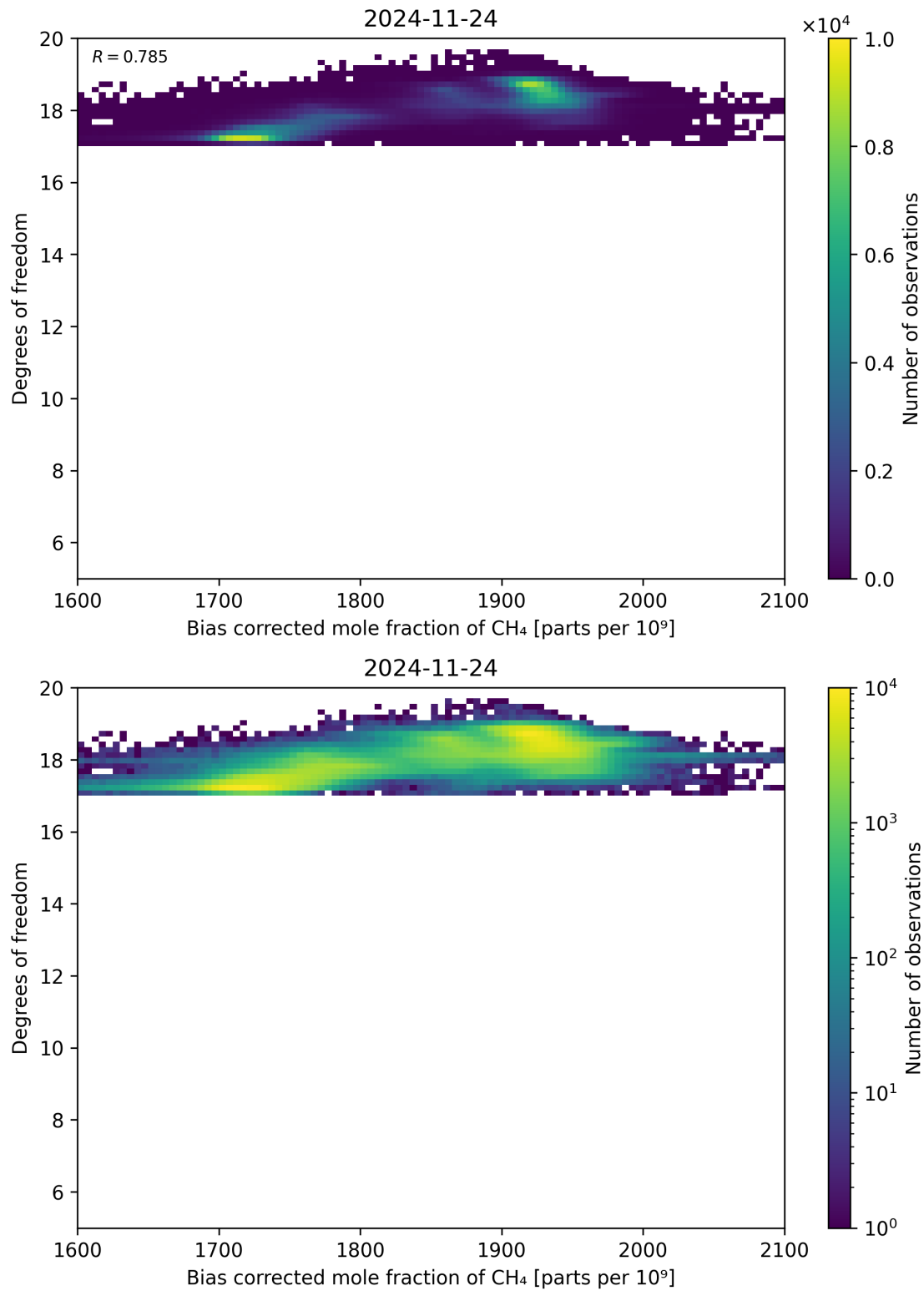
Figure 65: Scatter density plot of “Bias corrected mole fraction of \text{CH}_4 ” against “Degrees of freedom” for 2024-11-23 to 2024-11-25.
