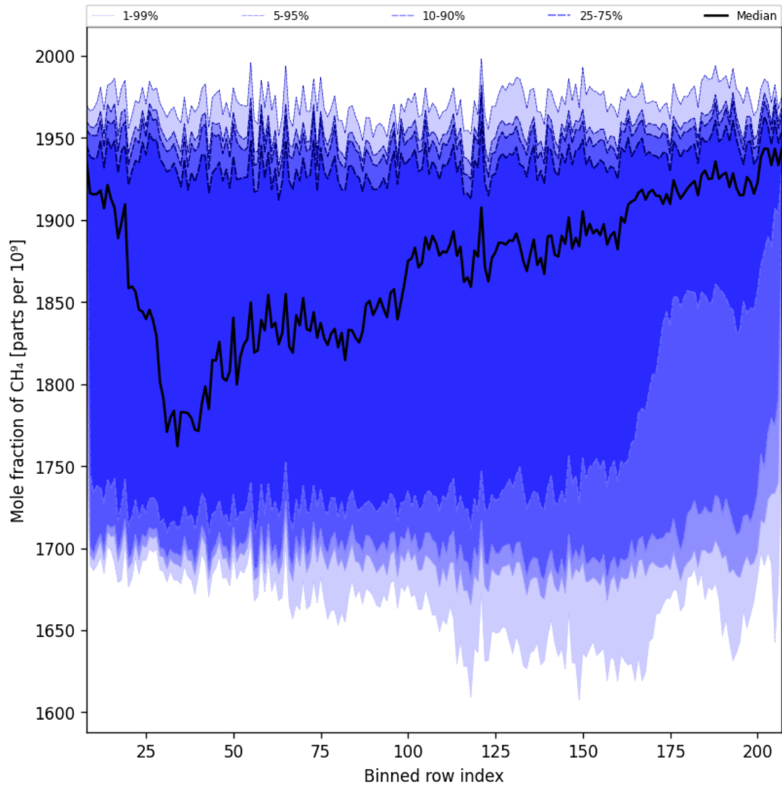
Figure 34: Along track statistics of “Mole fraction of CH 4 ” for 2024-11-23 to 2024-11-25
