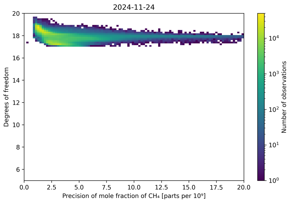
Figure 80: Scatter density plot of “Precision of mole fraction of CH 4 ” against “Degrees of freedom” for 2024-11-23 to 2024-11-25.
