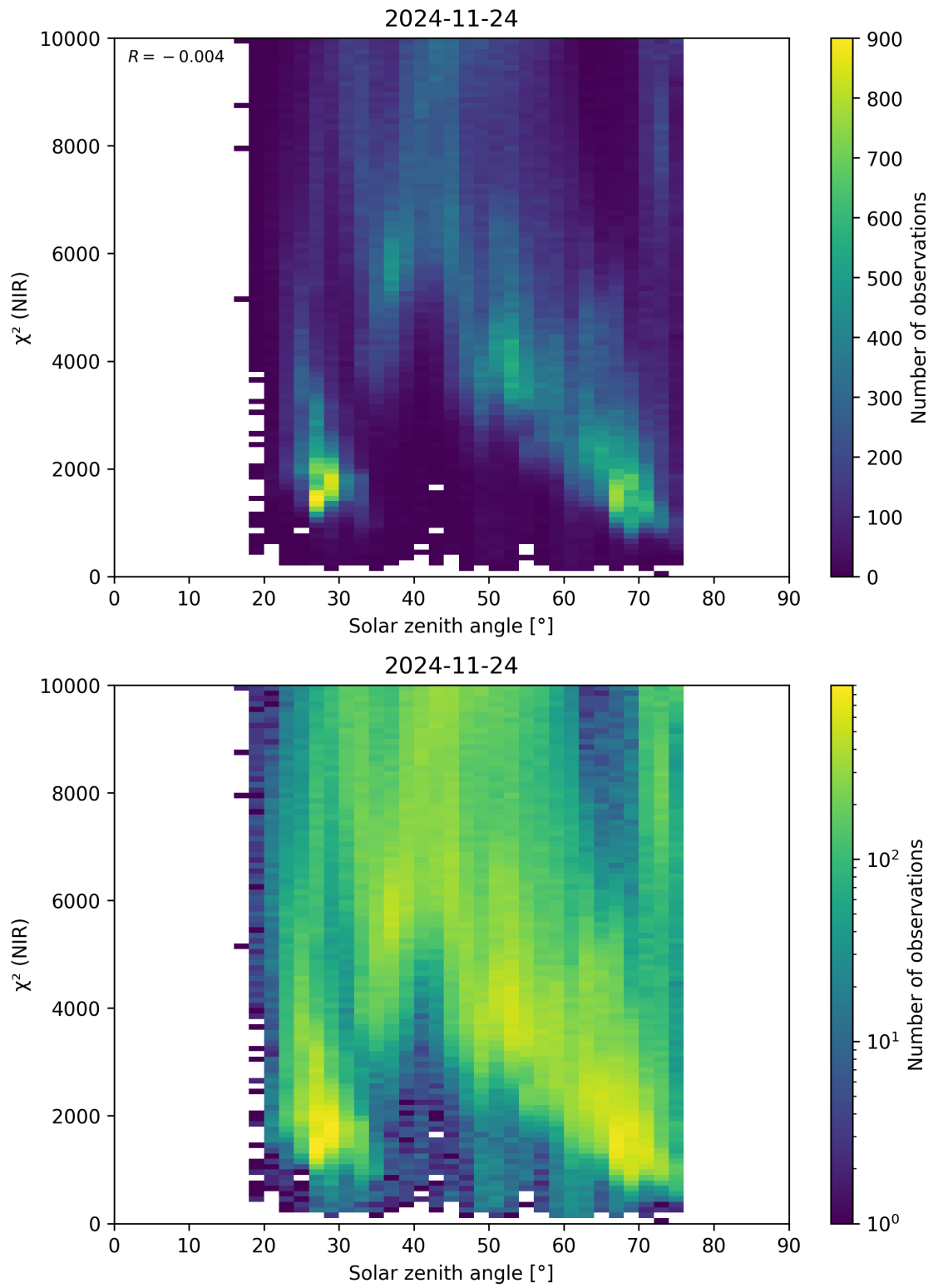
Figure 94: Scatter density plot of “Solar zenith angle” against “ \chi^2 (NIR)” for 2024-11-23 to 2024-11-25.
