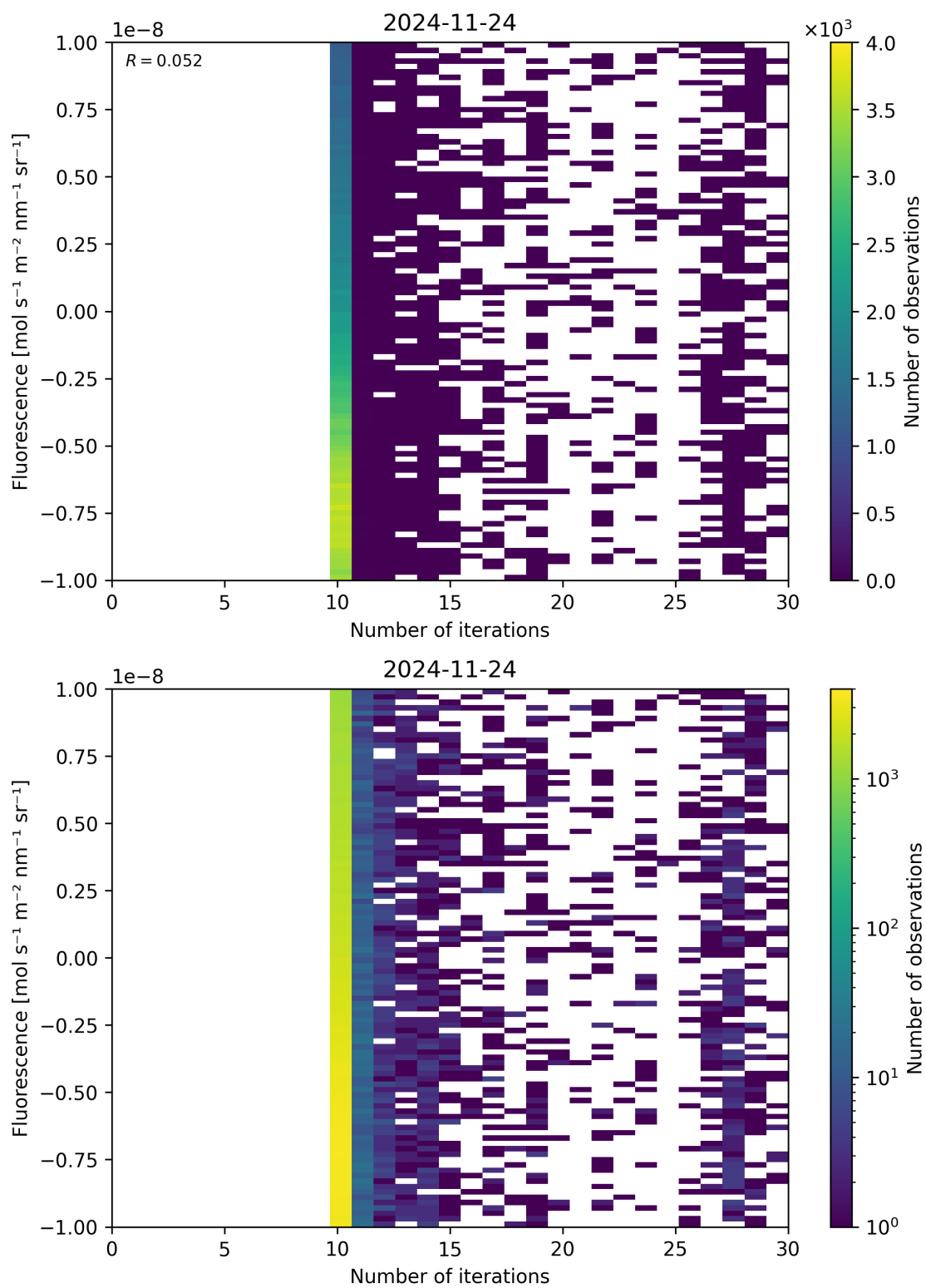
Figure 87: Scatter density plot of “Number of iterations” against “Fluorescence” for 2024-11-23 to 2024-11-25.
