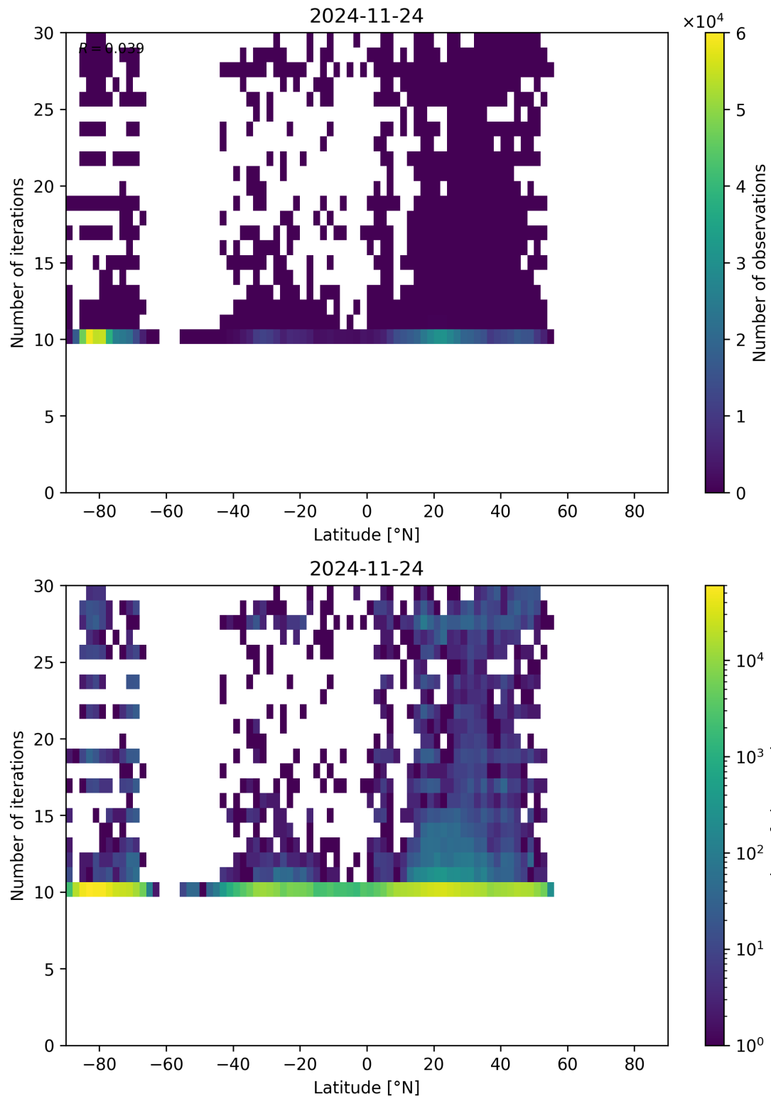
Figure 60: Scatter density plot of “Latitude” against “Number of iterations” for 2024-11-23 to 2024-11-25.
