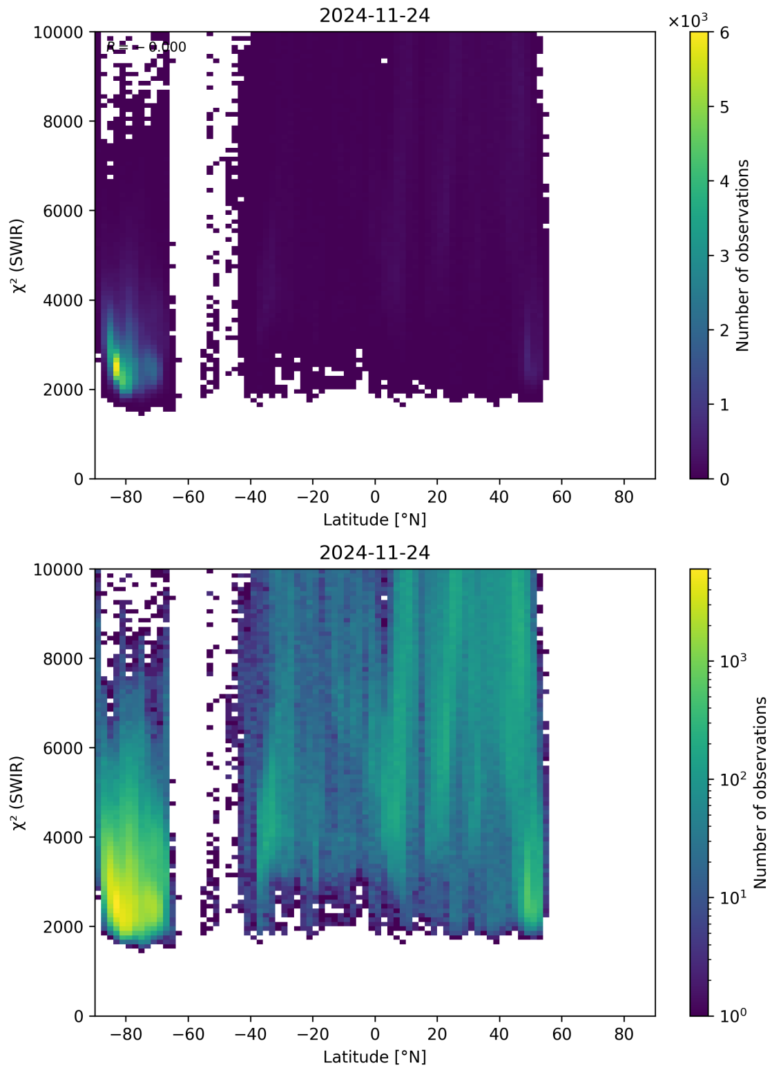
Figure 54: Scatter density plot of “Latitude” against “ \chi^2 (SWIR)” for 2024-11-23 to 2024-11-25.
