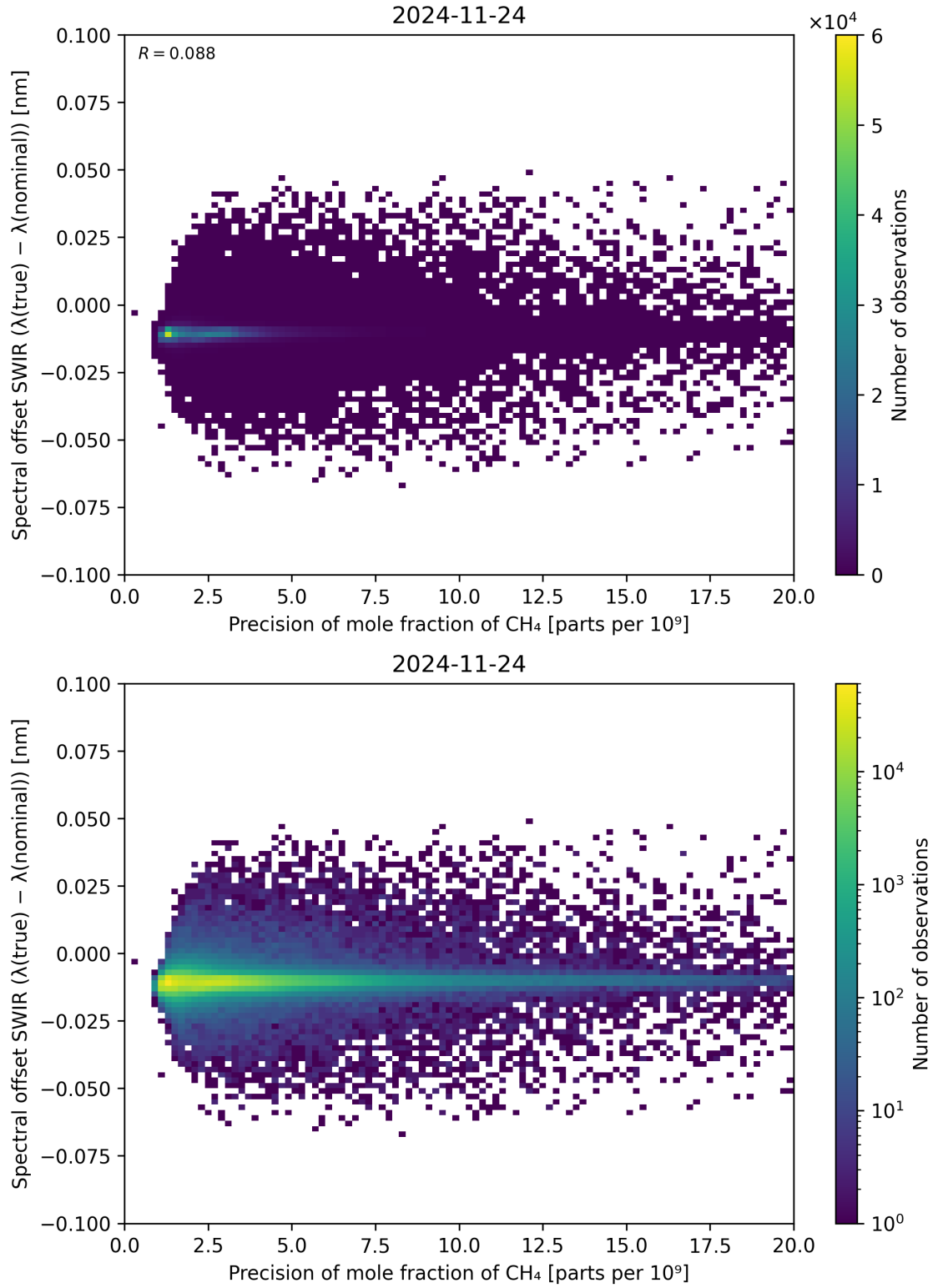
Figure 85: Scatter density plot of “Precision of mole fraction of CH 4 ” against “Spectral offset SWIR ( \lambda_{\text{true}} - \lambda_{\text{nominal}} )” for 2024-11-23 to 2024-11-25.
