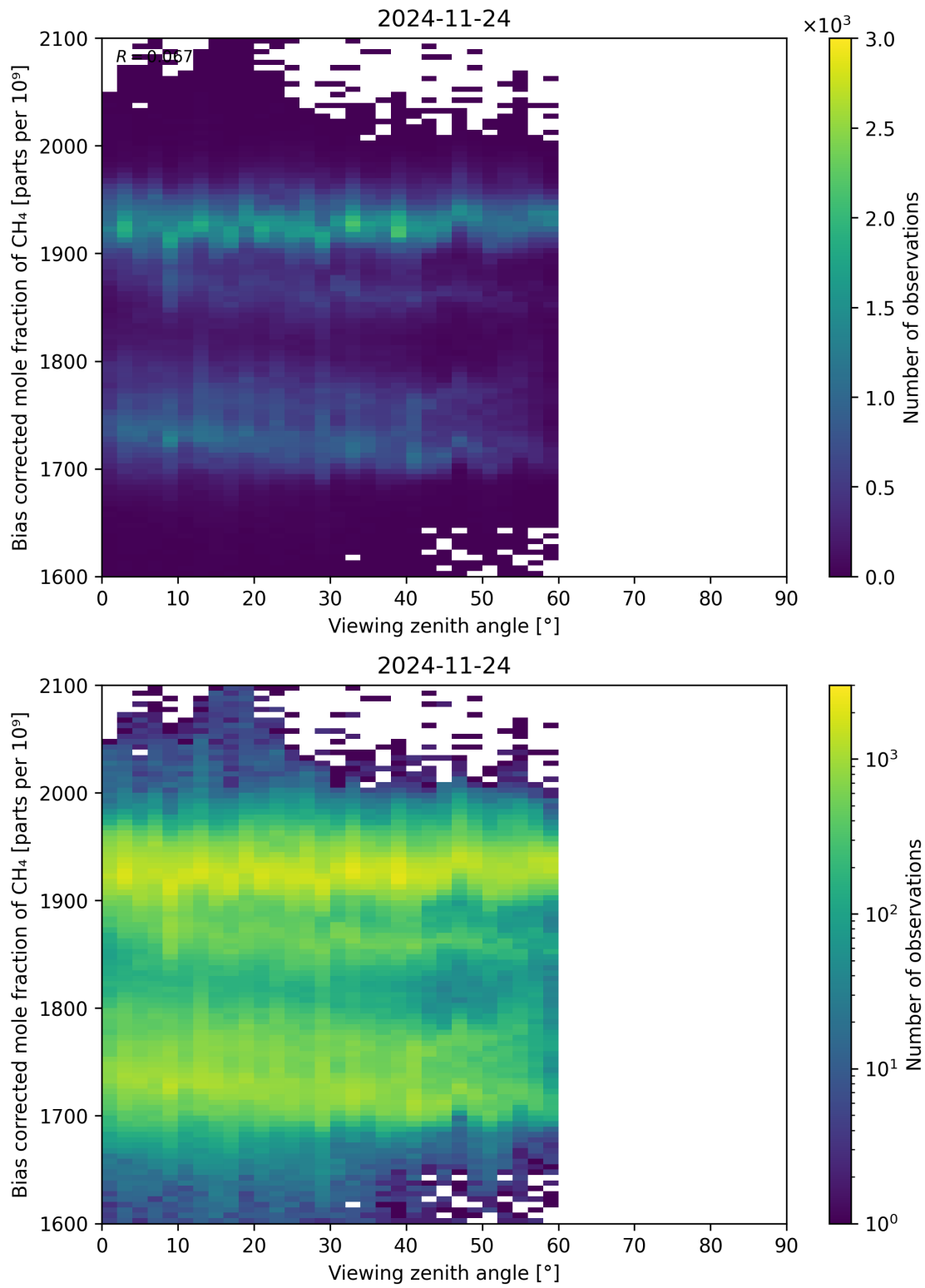
Figure 111: Scatter density plot of “Viewing zenith angle” against “Bias corrected mole fraction of CH 4 ” for 2024-11-23 to 2024-11-25.
