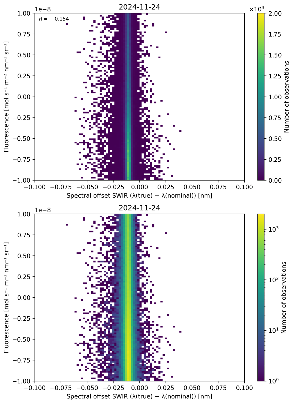
Figure 120: Scatter density plot of “Spectral offset SWIR ( \lambda_{\text{true}} - \lambda_{\text{nominal}} )” against “Fluorescence” for 2024-11-23 to 2024-11-25.
