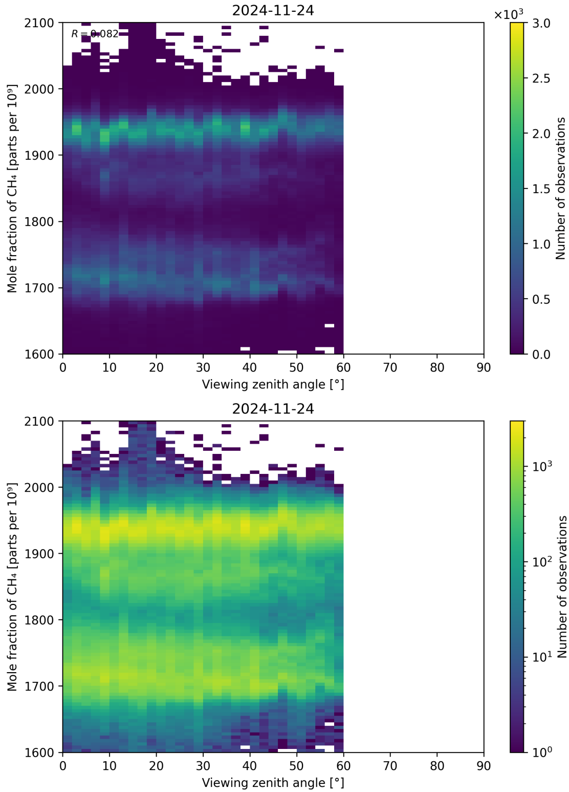
Figure 110: Scatter density plot of “Viewing zenith angle” against “Mole fraction of CH 4 ” for 2024-11-23 to 2024-11-25.
