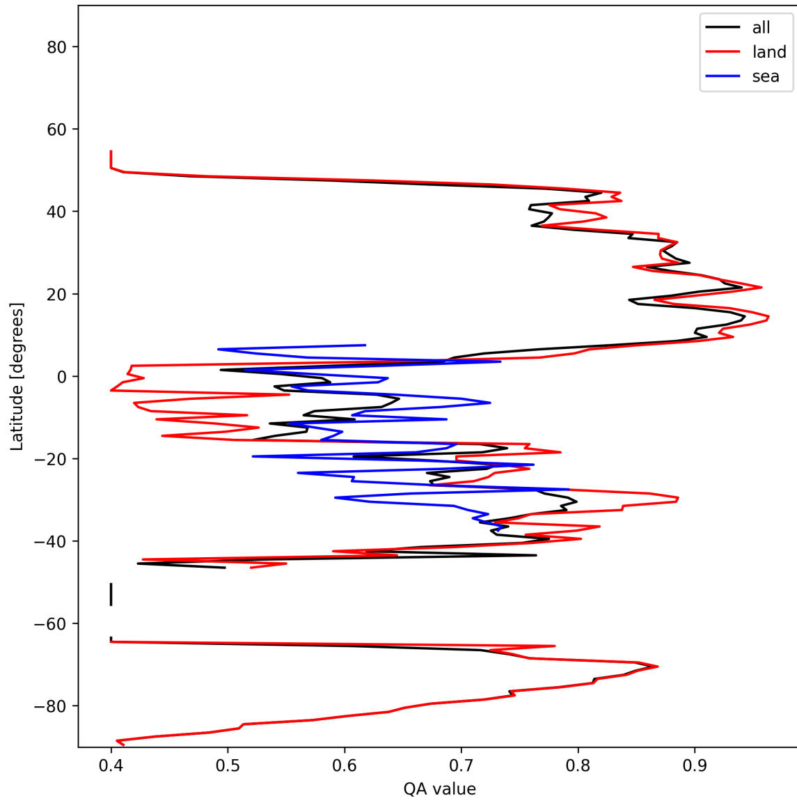
Figure 11: Zonal average of “QA value” for 2024-11-23 to 2024-11-25.
