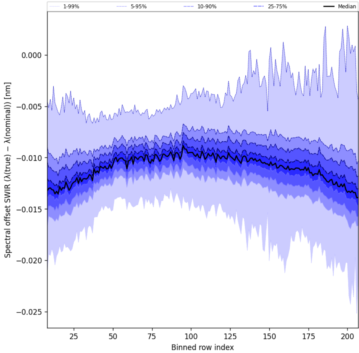
Figure 38: Along track statistics of “Spectral offset SWIR ( \lambda_{\text{true}} - \lambda_{\text{nominal}} )” for 2024-11-23 to 2024-11-25
