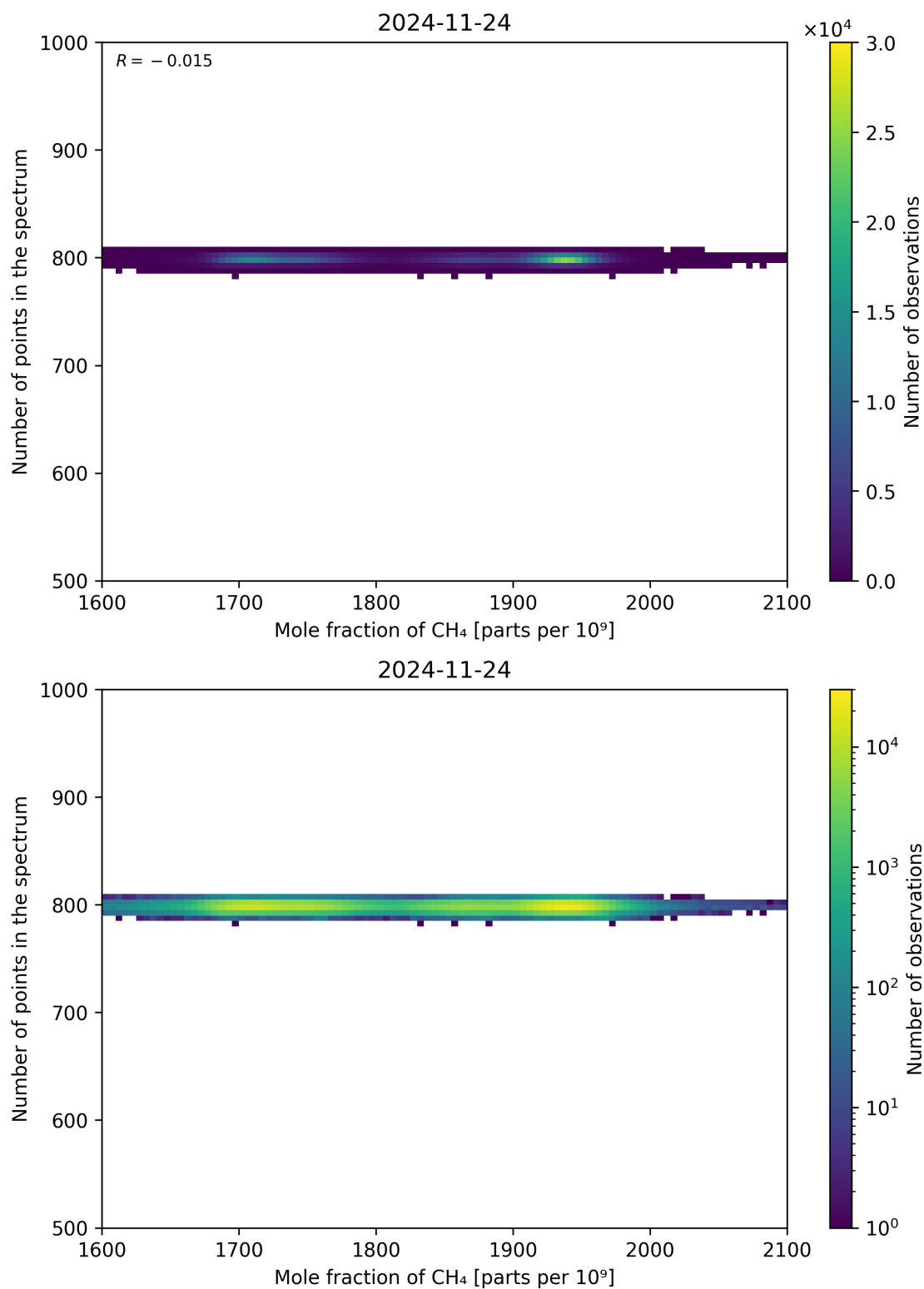
Figure 77: Scatter density plot of “Mole fraction of CH 4 ” against “Number of points in the spectrum” for 2024-11-23 to 2024-11-25.
