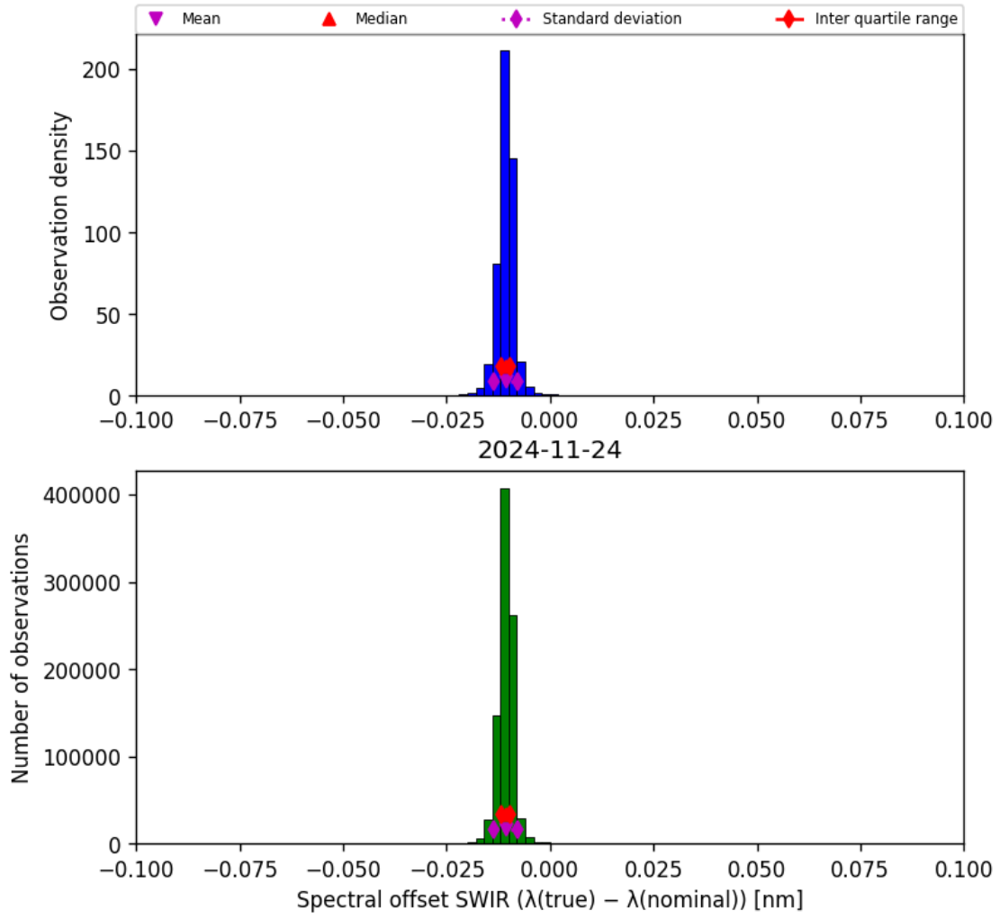
Figure 27: Histogram of “Spectral offset SWIR ( \lambda_{\text{true}} - \lambda_{\text{nominal}} )” for 2024-11-23 to 2024-11-25
