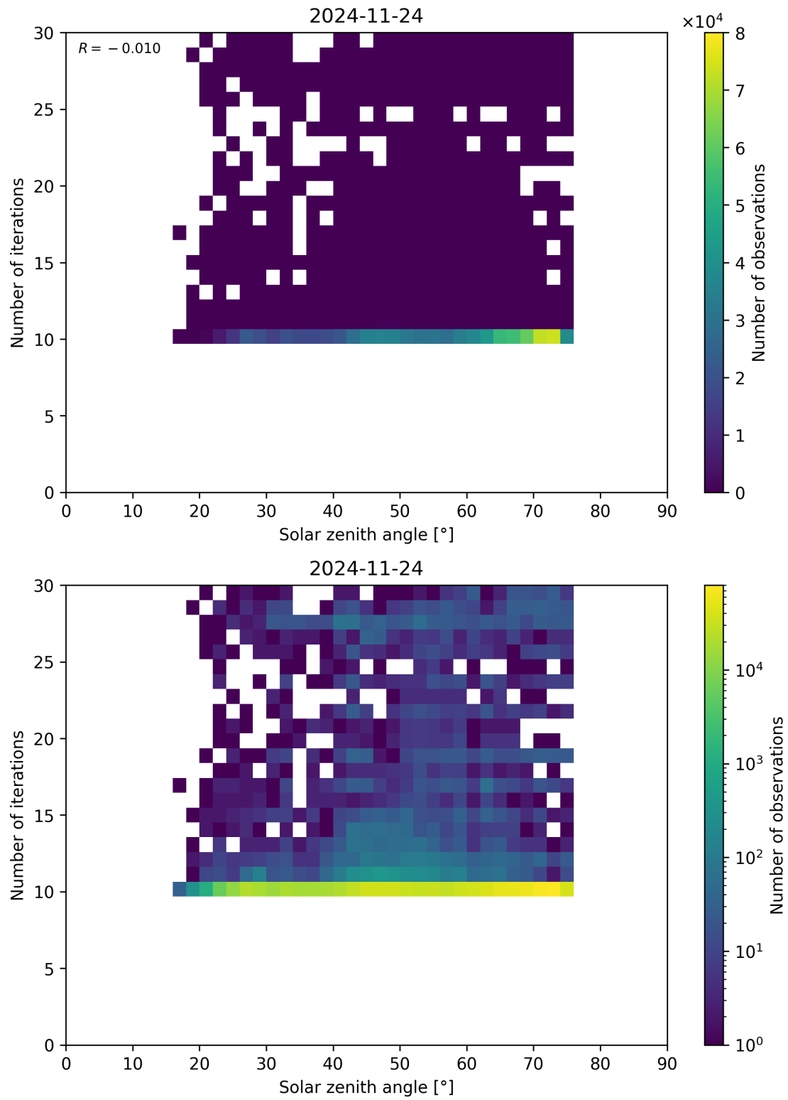
Figure 102: Scatter density plot of “Solar zenith angle” against “Number of iterations” for 2024-11-23 to 2024-11-25.
