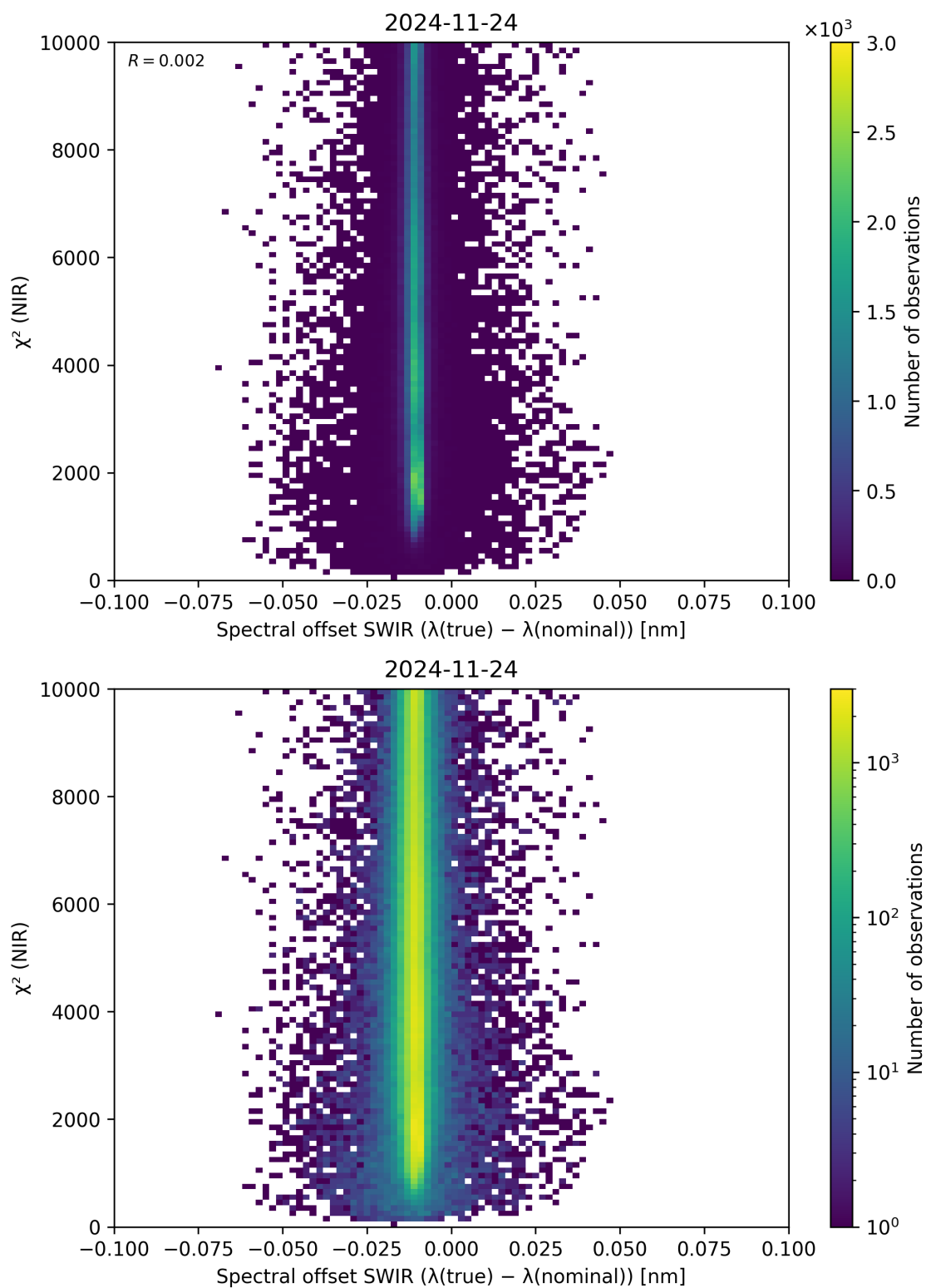
Figure 117: Scatter density plot of “Spectral offset SWIR ( \lambda_{\text{true}} - \lambda_{\text{nominal}} )” against “ \chi^2 (NIR)” for 2024-11-23 to 2024-11-25.
