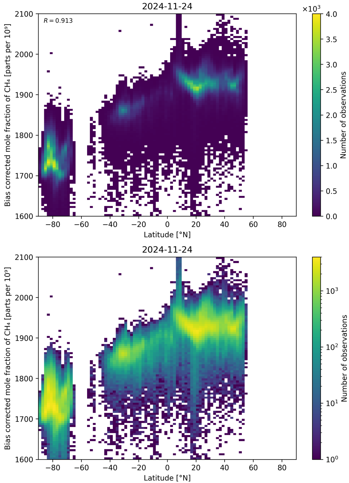
Figure 58: Scatter density plot of “Latitude” against “Bias corrected mole fraction of CH 4 ” for 2024-11-23 to 2024-11-25.
