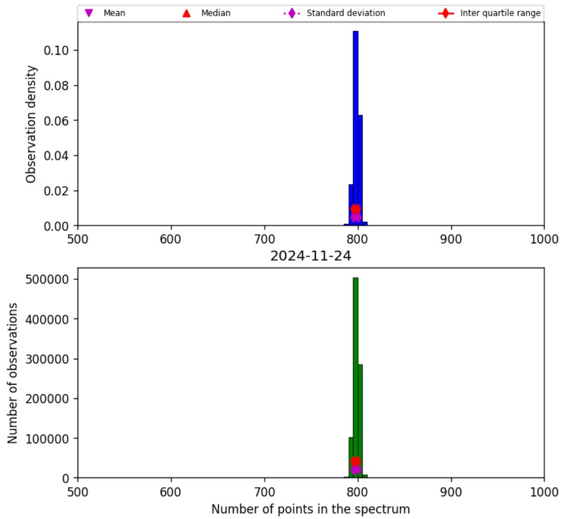
Figure 26: Histogram of “Number of points in the spectrum” for 2024-11-23 to 2024-11-25
