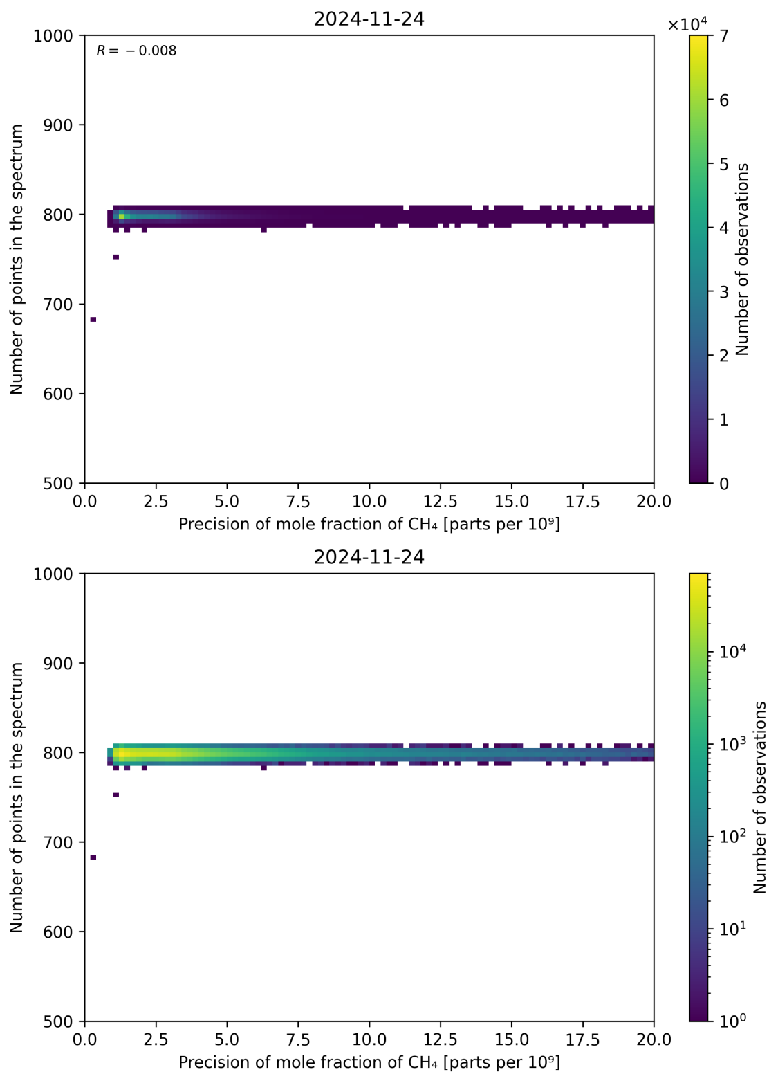
Figure 84: Scatter density plot of “Precision of mole fraction of CH 4 ” against “Number of points in the spectrum” for 2024-11-23 to 2024-11-25.
