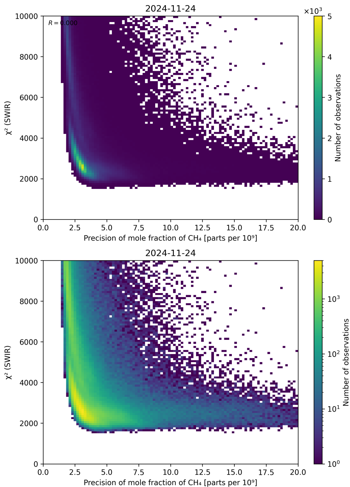
Figure 79: Scatter density plot of “Precision of mole fraction of \text{CH}_4 ” against “ \chi^2 (SWIR)” for 2024-11-23 to 2024-11-25.
