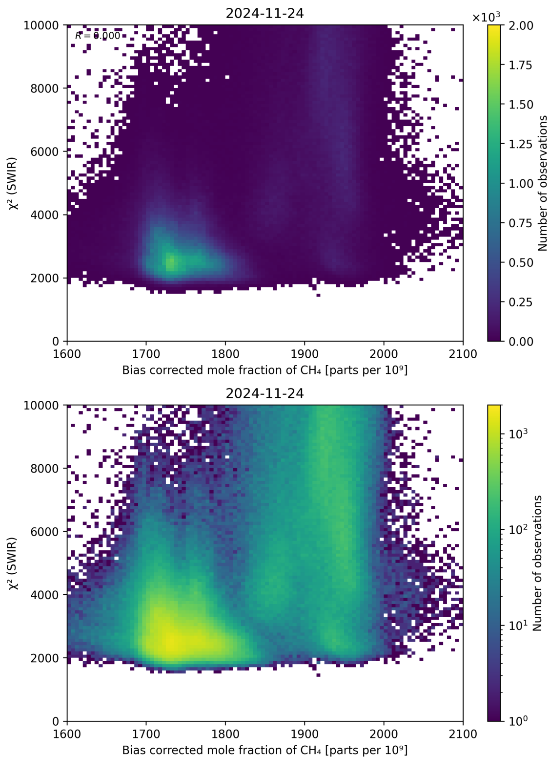
Figure 64: Scatter density plot of “Bias corrected mole fraction of \text{CH}_4 ” against “ \chi^2 (SWIR)” for 2024-11-23 to 2024-11-25.
