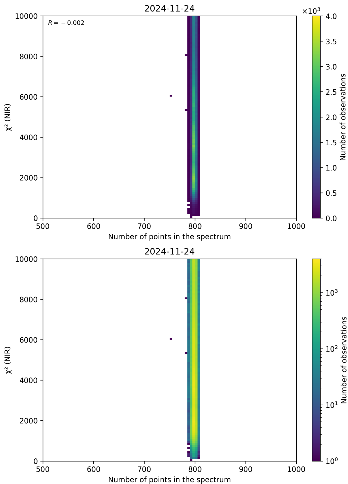
Figure 88: Scatter density plot of “Number of points in the spectrum” against “ \chi^2 (NIR)” for 2024-11-23 to 2024-11-25.
