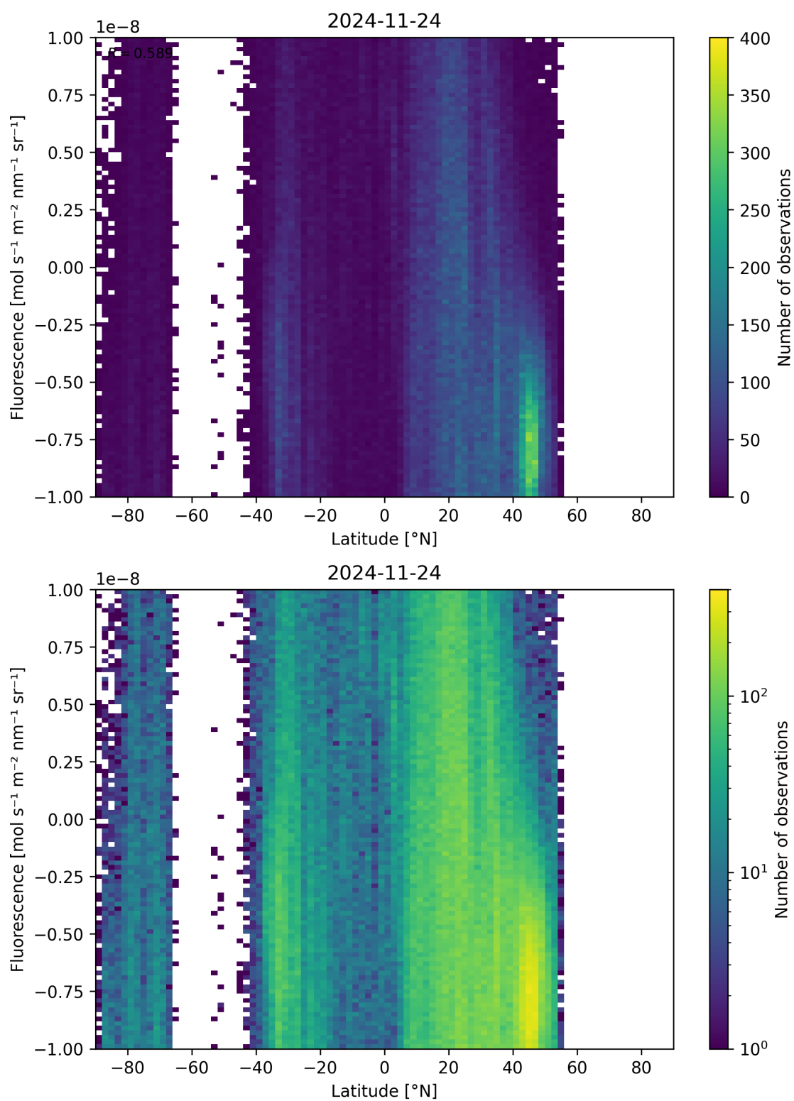
Figure 56: Scatter density plot of “Latitude” against “Fluorescence” for 2024-11-23 to 2024-11-25.
