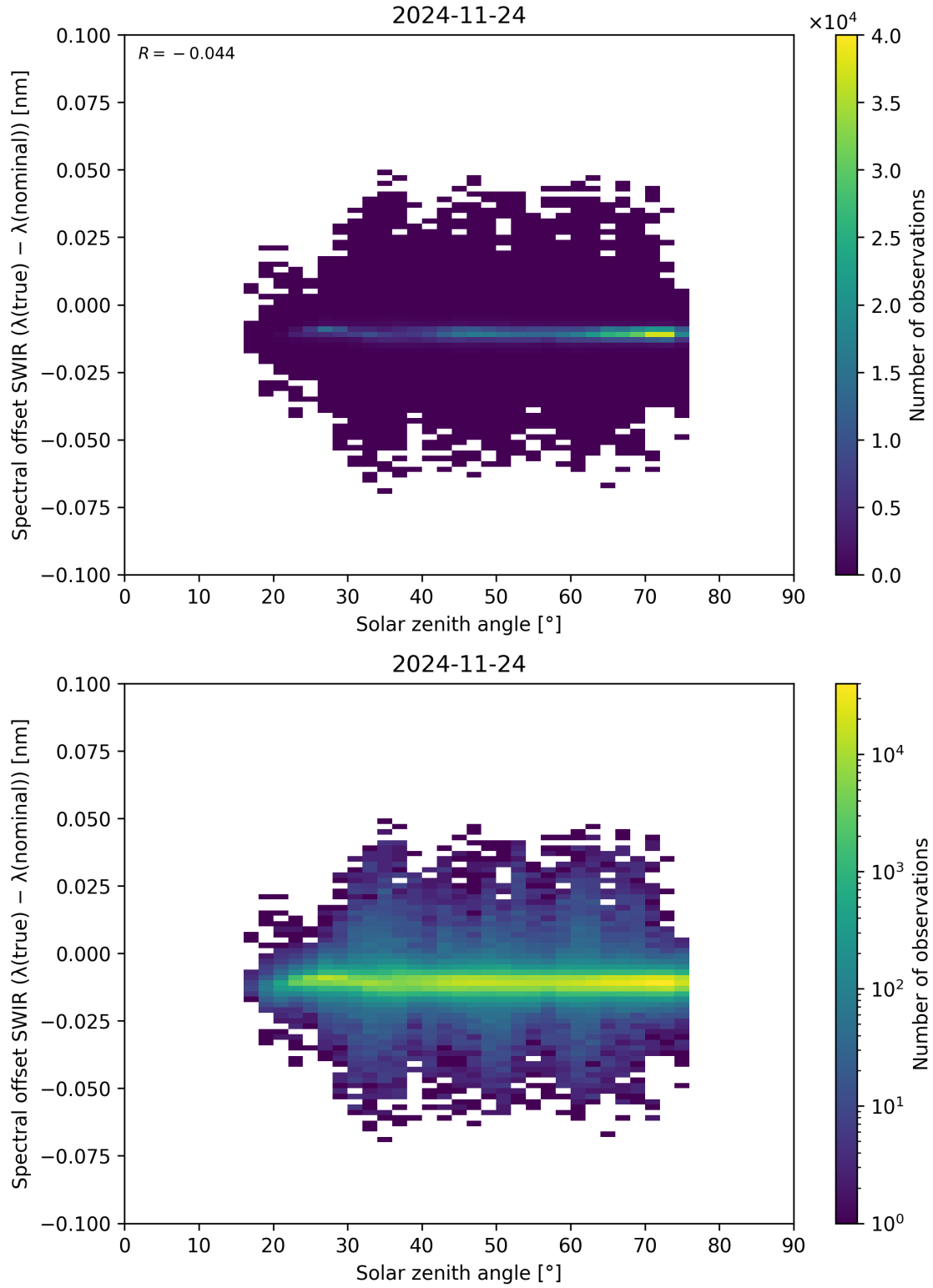
Figure 104: Scatter density plot of “Solar zenith angle” against “Spectral offset SWIR ( \lambda_{\text{true}} - \lambda_{\text{nominal}} )” for 2024-11-23 to 2024-11-25.
