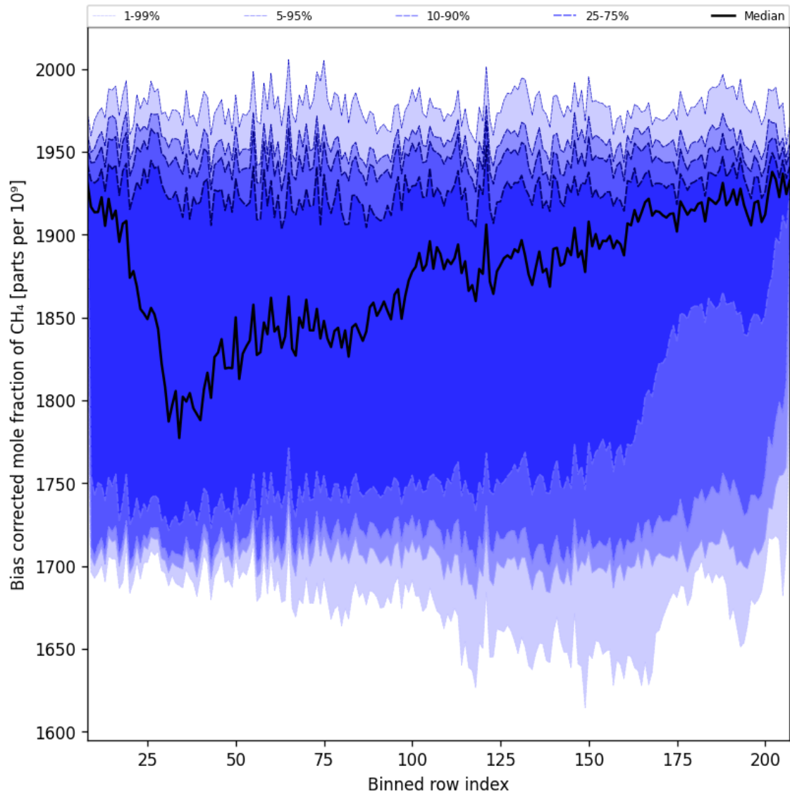
Figure 36: Along track statistics of “Bias corrected mole fraction of CH 4 ” for 2024-11-23 to 2024-11-25
