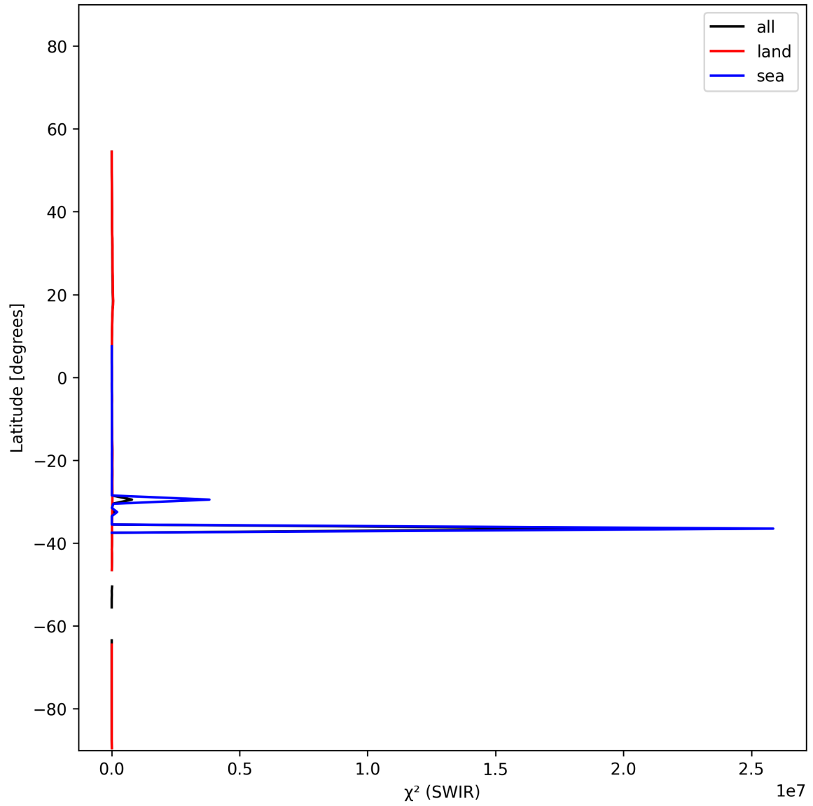
Figure 17: Zonal average of “ \chi^2 (SWIR)” for 2024-11-23 to 2024-11-25.
