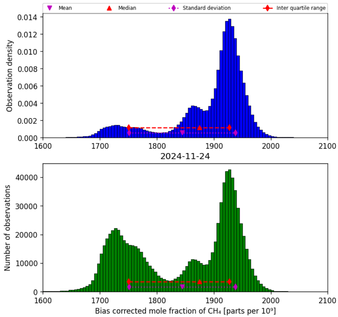
Figure 25: Histogram of “Bias corrected mole fraction of CH 4 ” for 2024-11-23 to 2024-11-25
