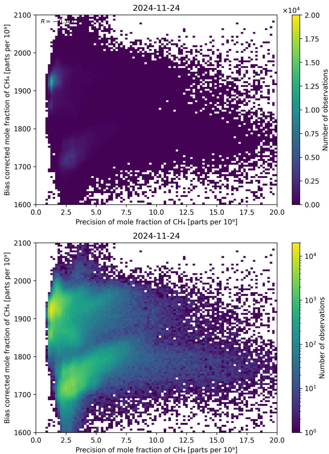
Figure 82: Scatter density plot of “Precision of mole fraction of CH 4 ” against “Bias corrected mole fraction of CH 4 ” for 2024-11-23 to 2024-11-25.
