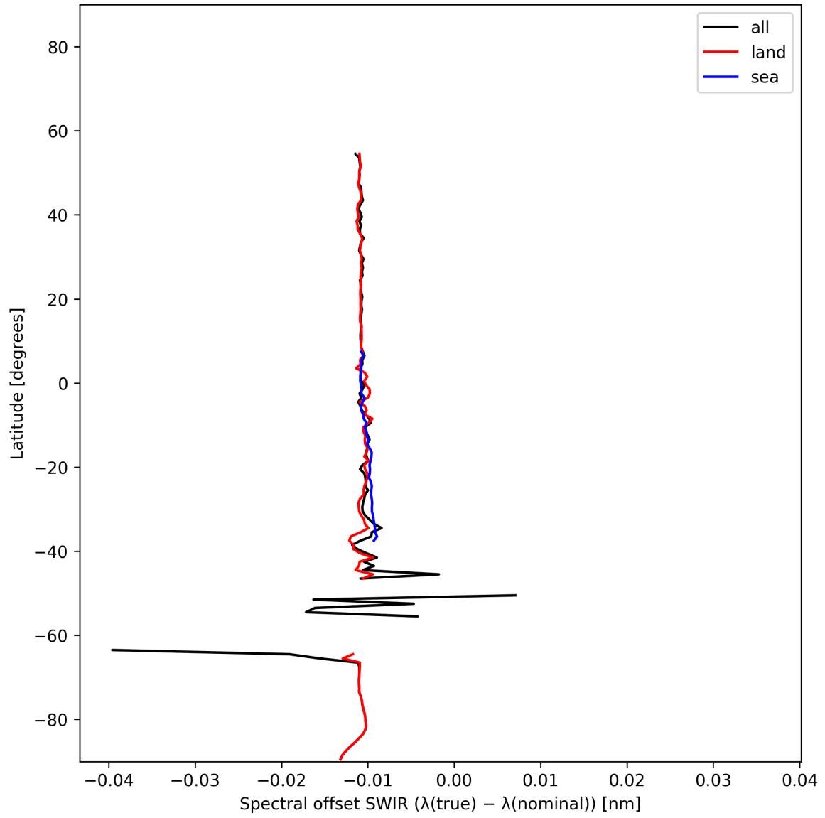
Figure 16: Zonal average of “Spectral offset SWIR ( \lambda_{\text{true}} - \lambda_{\text{nominal}} )” for 2024-11-23 to 2024-11-25.
