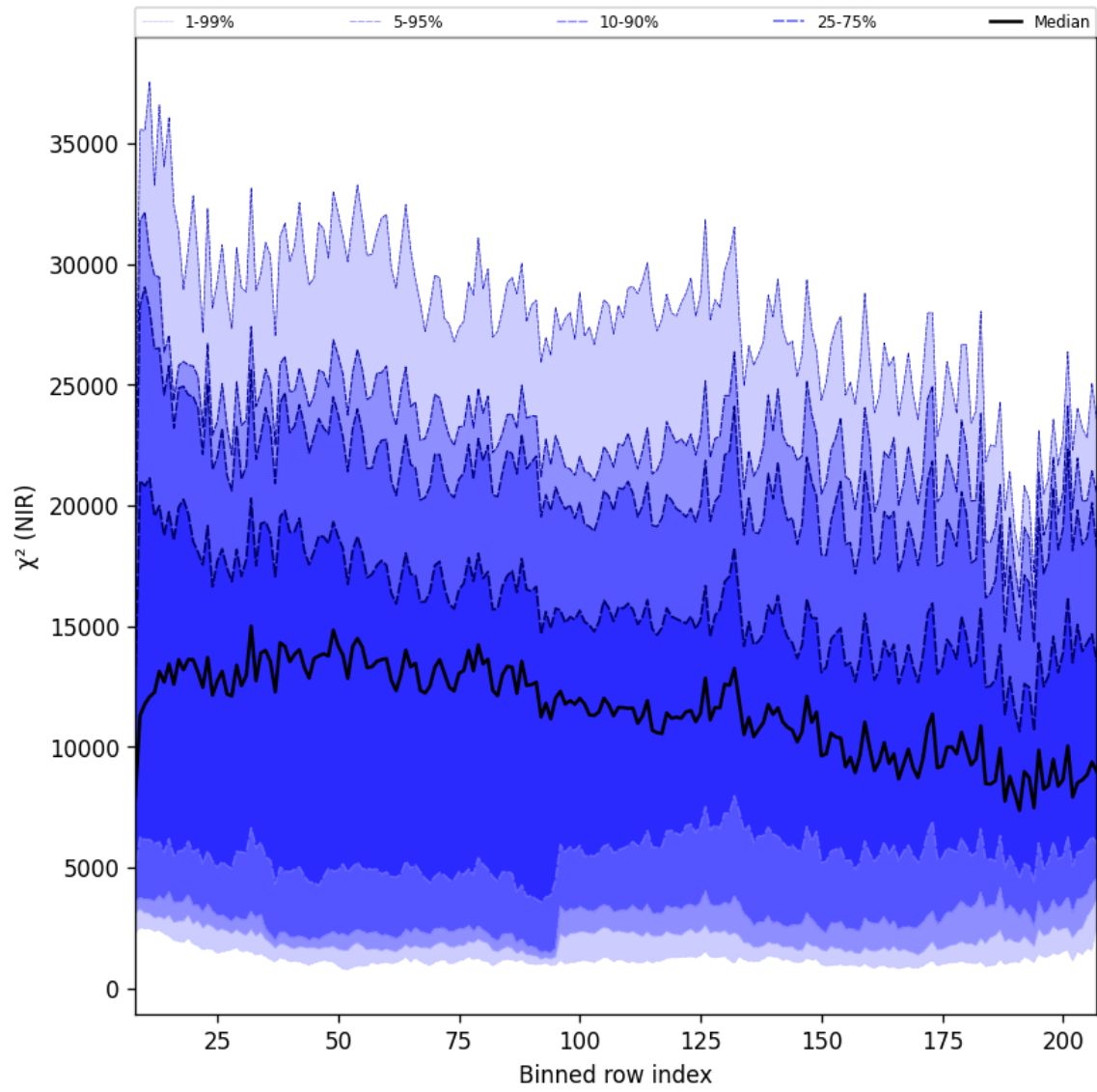
Figure 40: Along track statistics of " \chi^2 (NIR)" for 2024-11-23 to 2024-11-25
