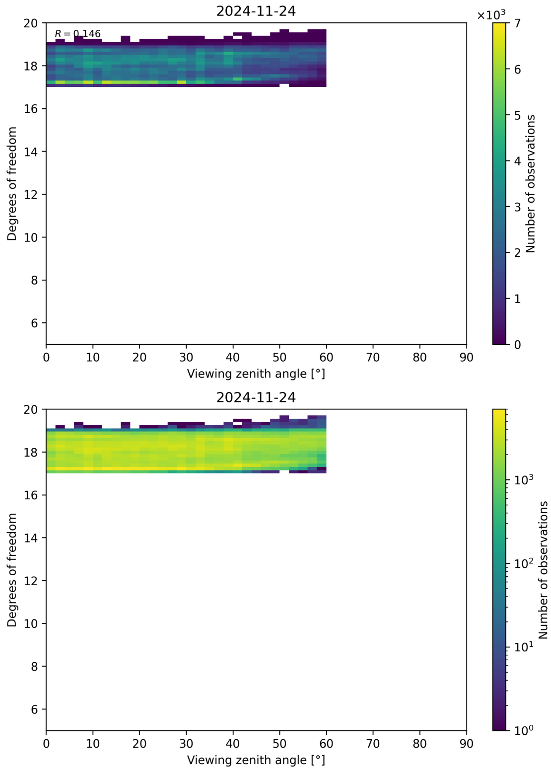
Figure 107: Scatter density plot of “Viewing zenith angle” against “Degrees of freedom” for 2024-11-23 to 2024-11-25.
