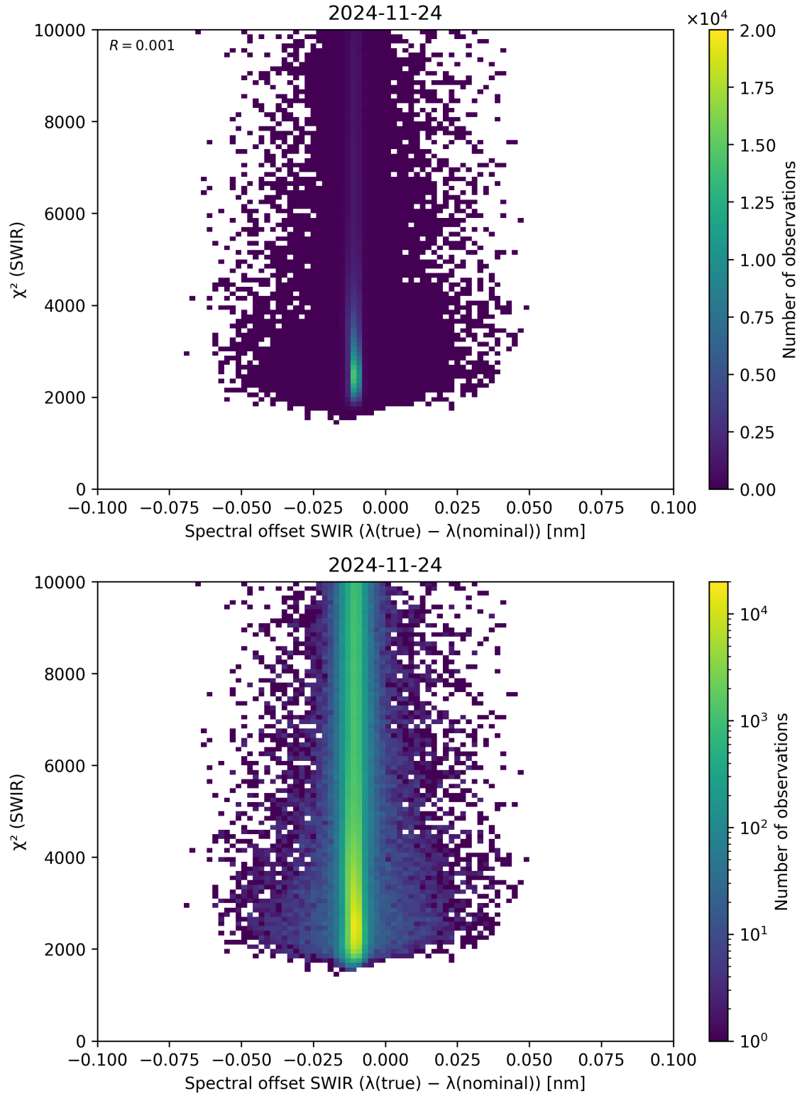
Figure 118: Scatter density plot of “Spectral offset SWIR ( \lambda_{\text{true}} - \lambda_{\text{nominal}} )” against “ \chi^2 (SWIR)” for 2024-11-23 to 2024-11-25.
