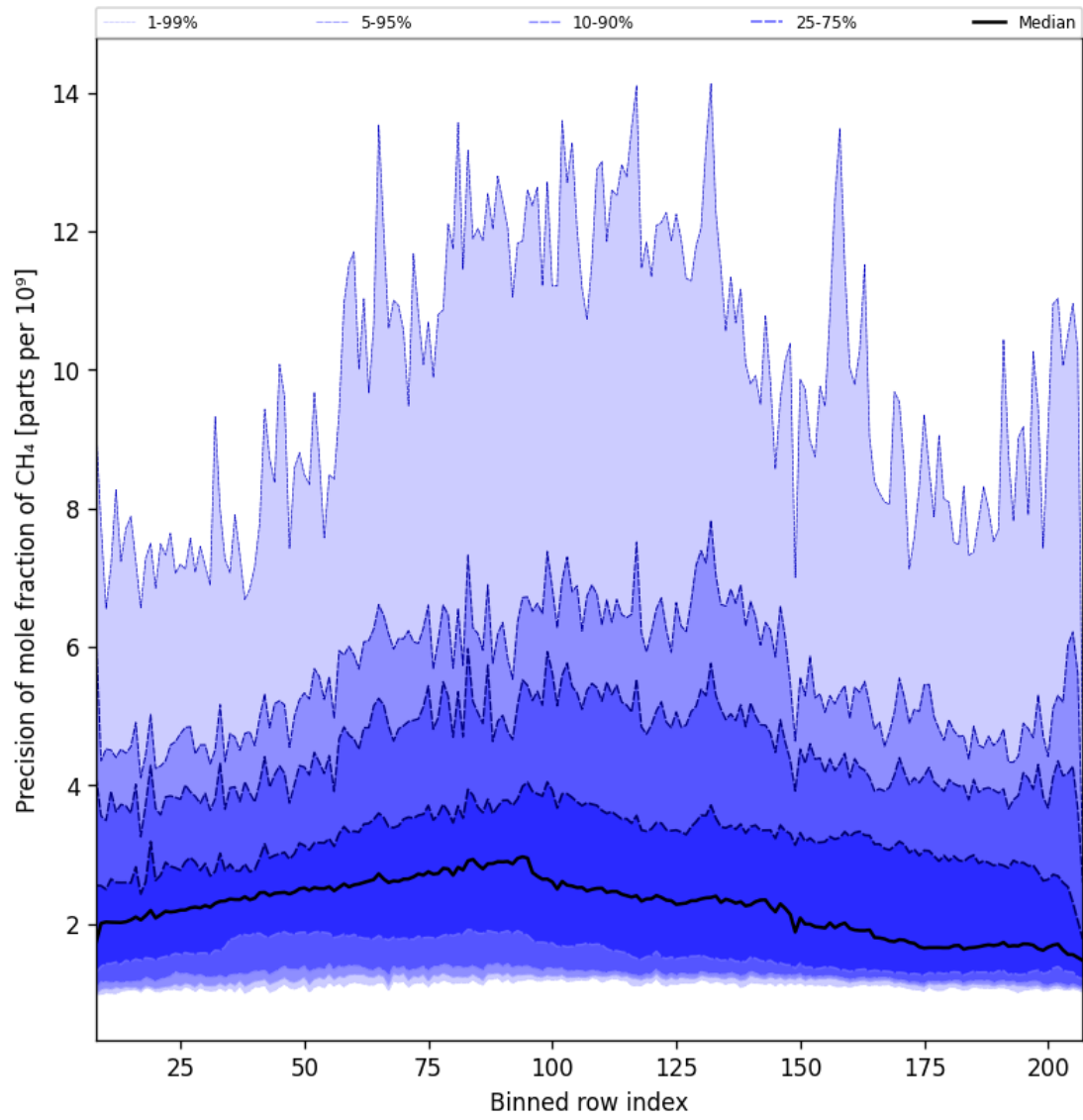
Figure 35: Along track statistics of “Precision of mole fraction of CH 4 ” for 2024-11-23 to 2024-11-25
