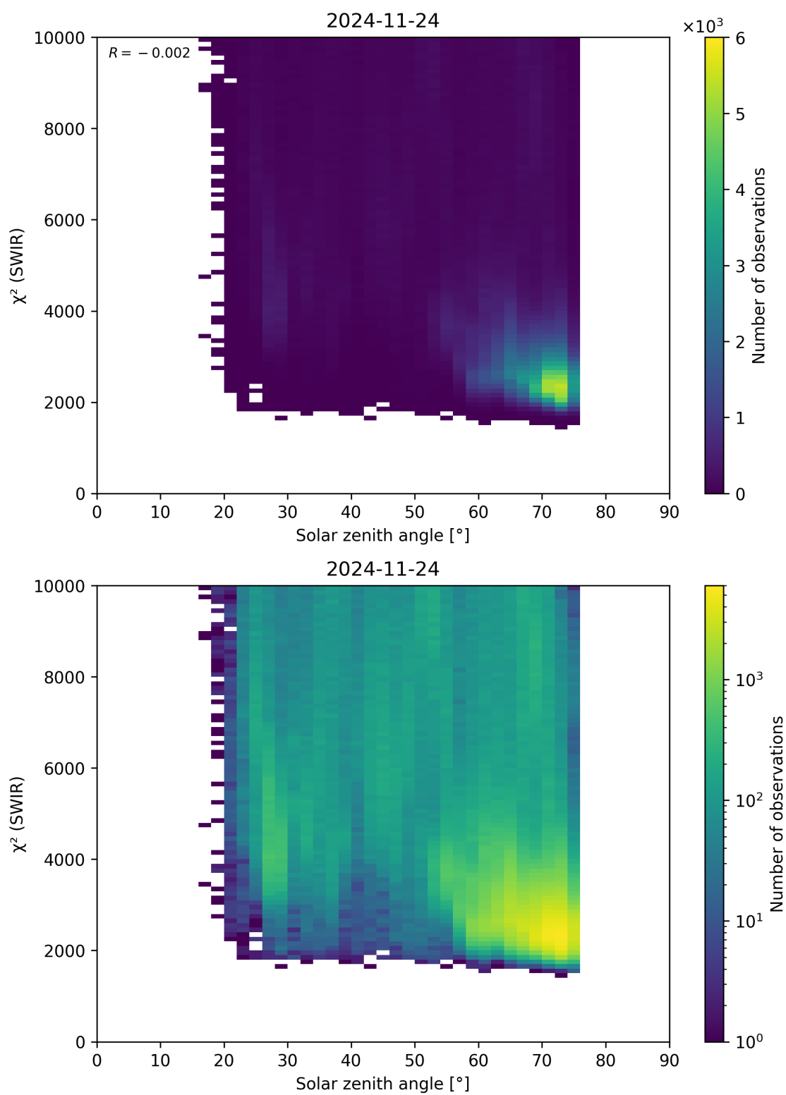
Figure 95: Scatter density plot of “Solar zenith angle” against “ \chi^2 (SWIR)” for 2024-11-23 to 2024-11-25.
