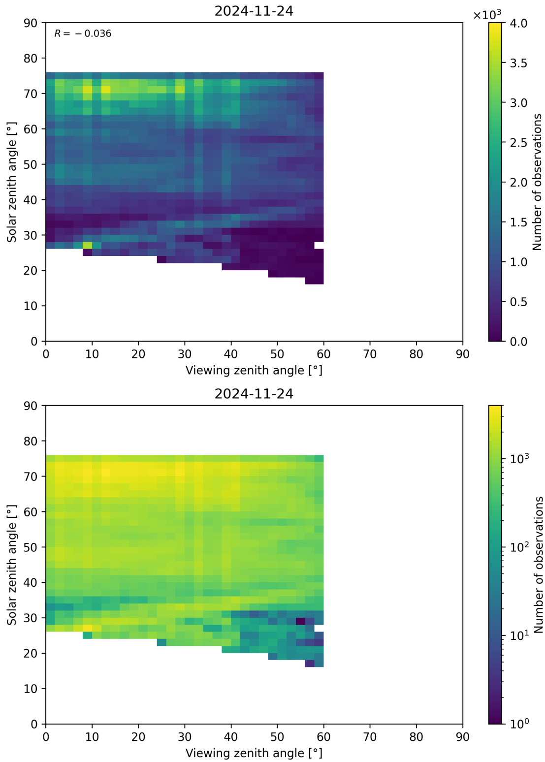
Figure 115: Scatter density plot of “Viewing zenith angle” against “Solar zenith angle” for 2024-11-23 to 2024-11-25.
