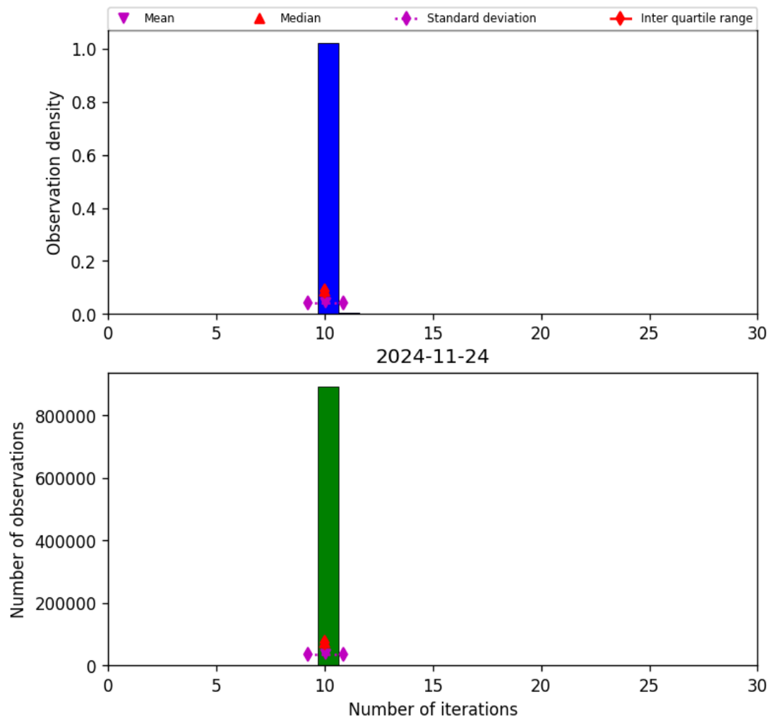
Figure 31: Histogram of “Number of iterations” for 2024-11-23 to 2024-11-25
