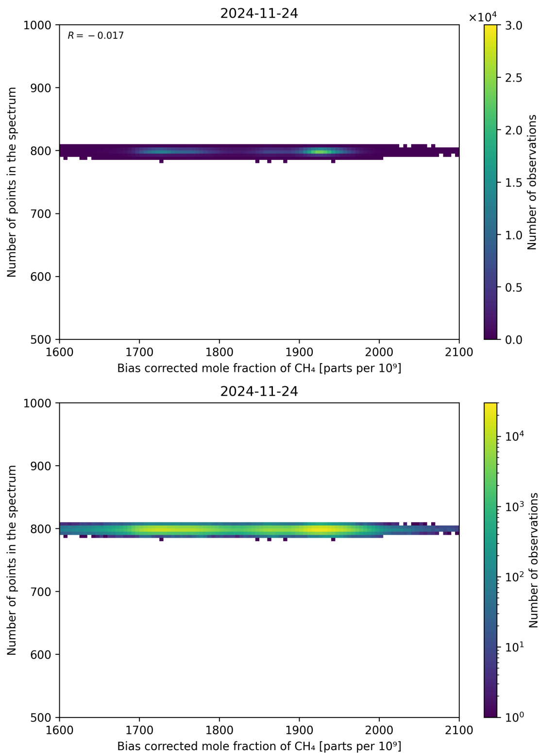
Figure 68: Scatter density plot of “Bias corrected mole fraction of CH 4 ” against “Number of points in the spectrum” for 2024-11-23 to 2024-11-25.
