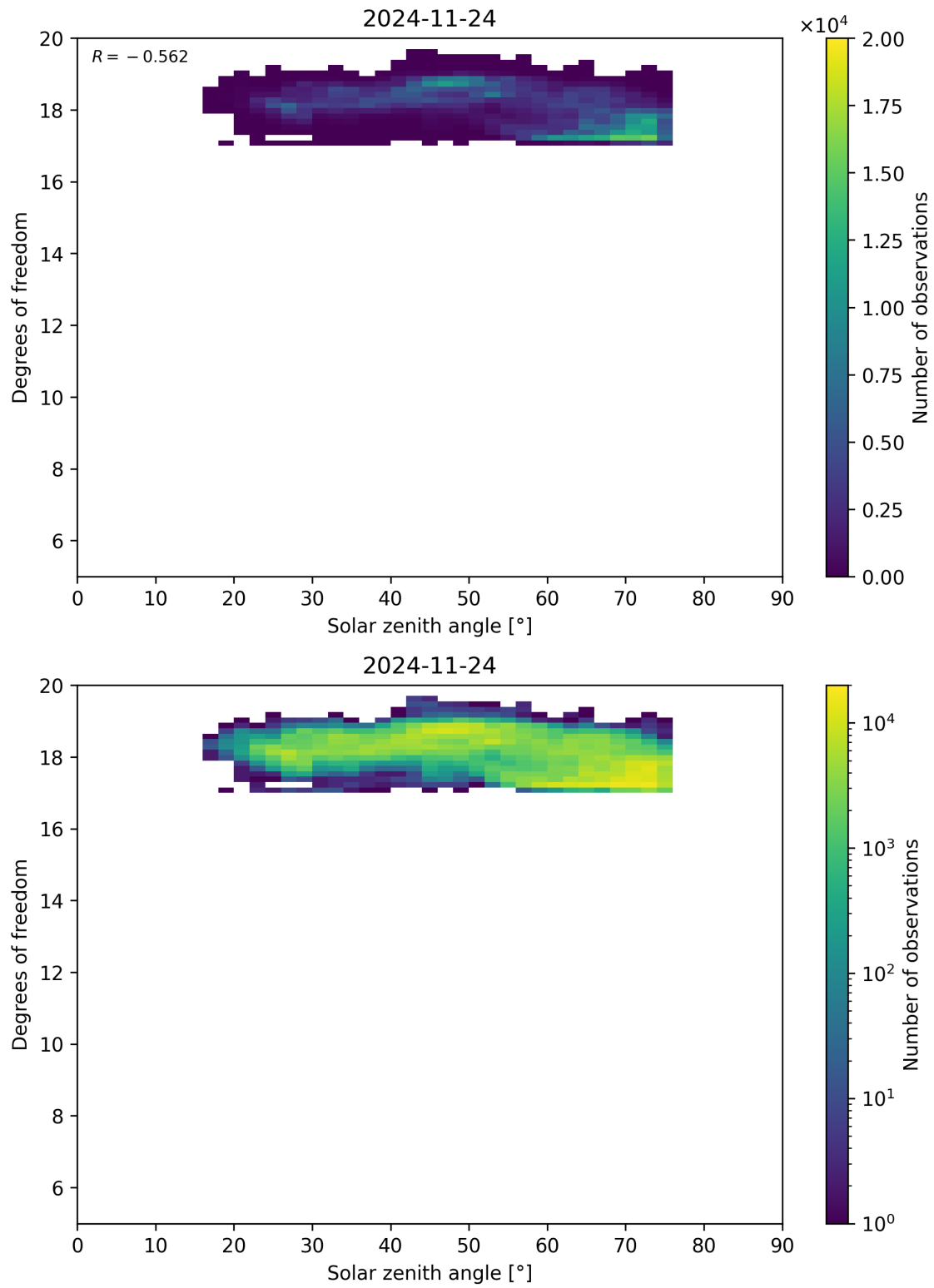
Figure 96: Scatter density plot of “Solar zenith angle” against “Degrees of freedom” for 2024-11-23 to 2024-11-25.
