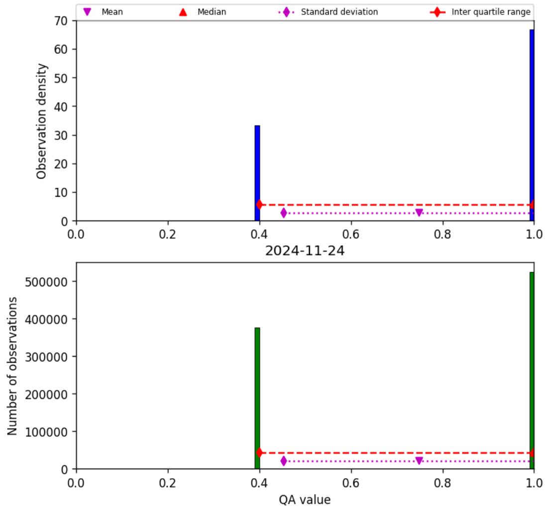
Figure 22: Histogram of “QA value” for 2024-11-23 to 2024-11-25
