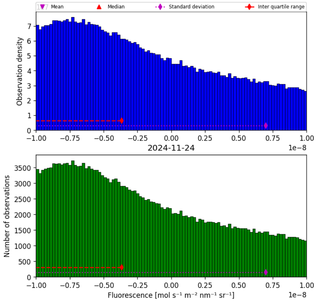
Figure 32: Histogram of “Fluorescence” for 2024-11-23 to 2024-11-25
