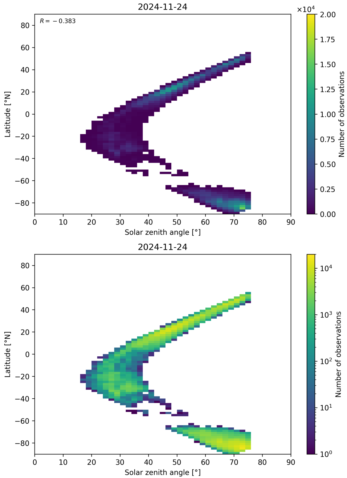
Figure 98: Scatter density plot of “Solar zenith angle” against “Latitude” for 2024-11-23 to 2024-11-25.
