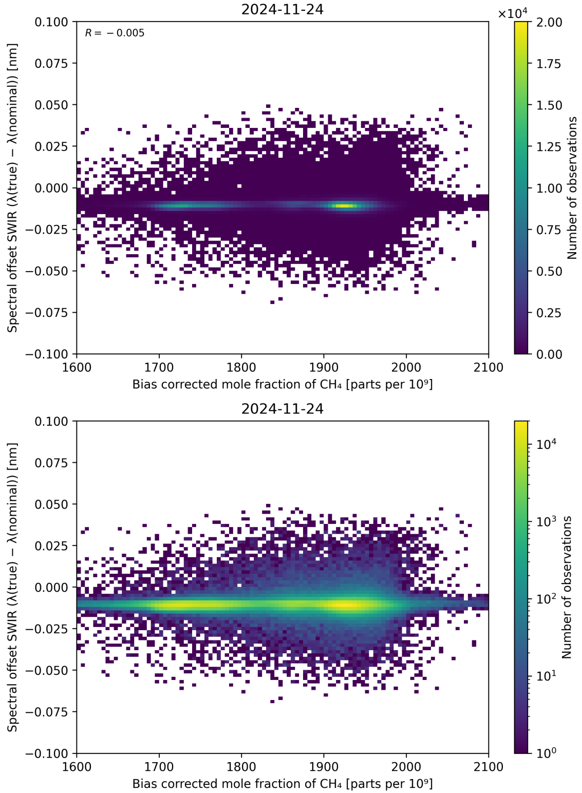
Figure 69: Scatter density plot of “Bias corrected mole fraction of \text{CH}_4 ” against “Spectral offset SWIR ( \lambda_{\text{true}} - \lambda_{\text{nominal}} )” for 2024-11-23 to 2024-11-25.
