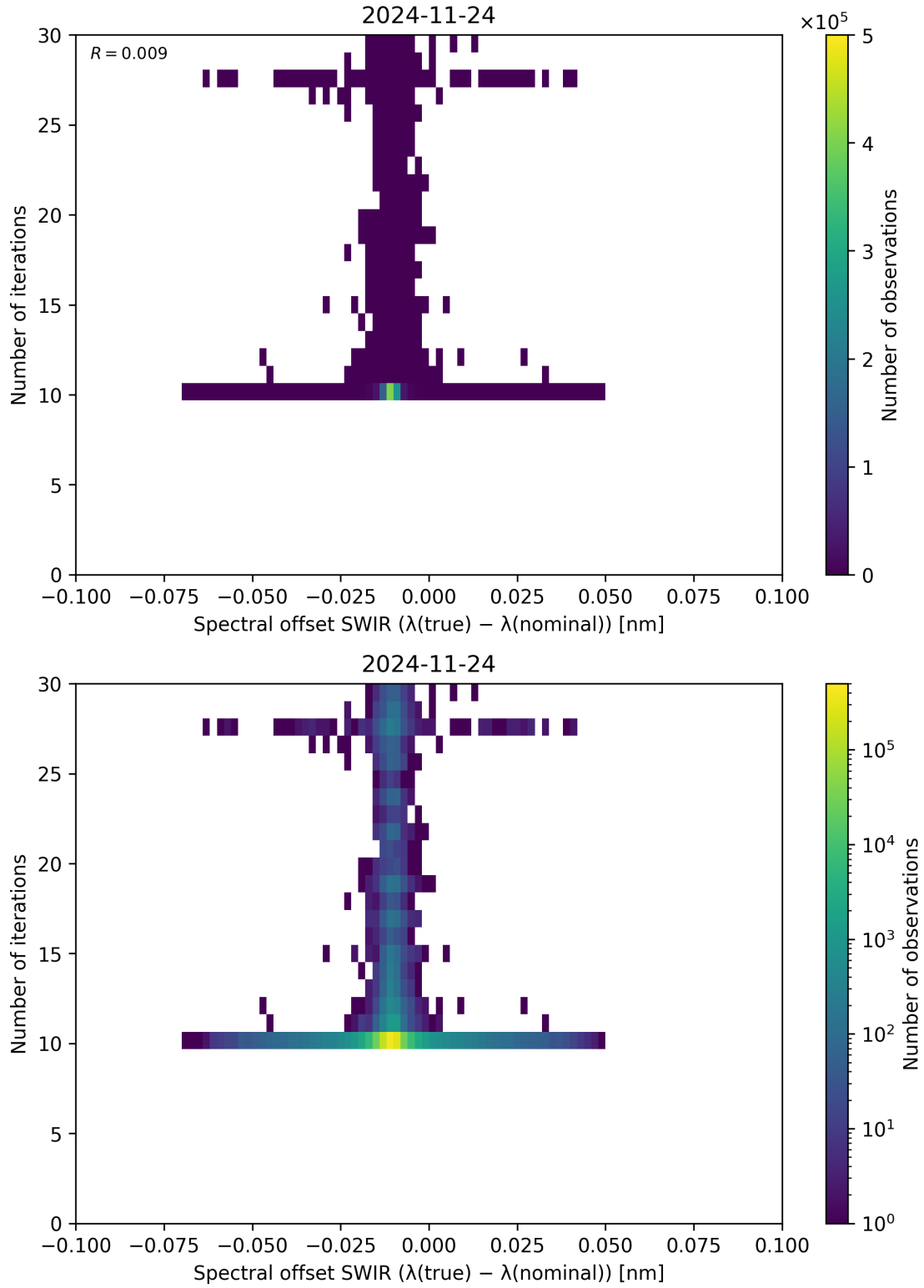
Figure 121: Scatter density plot of “Spectral offset SWIR ( \lambda_{\text{true}} - \lambda_{\text{nominal}} )” against “Number of iterations” for 2024-11-23 to 2024-11-25.
