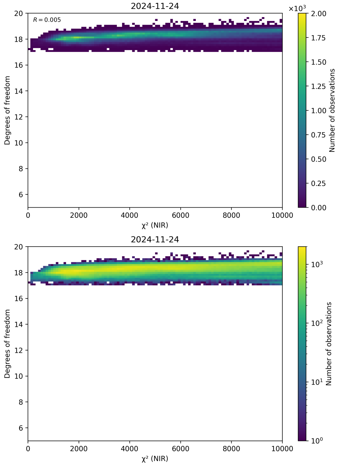
Figure 44: Scatter density plot of “ \chi^2 (NIR)” against “Degrees of freedom” for 2024-11-23 to 2024-11-25.
