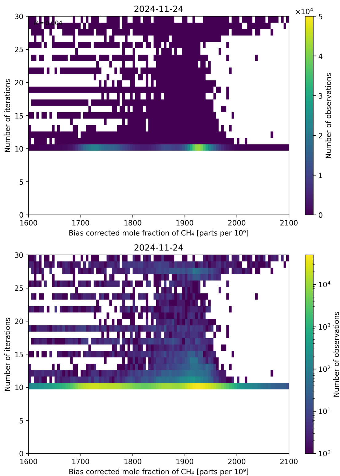
Figure 67: Scatter density plot of “Bias corrected mole fraction of \text{CH}_4 ” against “Number of iterations” for 2024-11-23 to 2024-11-25.
