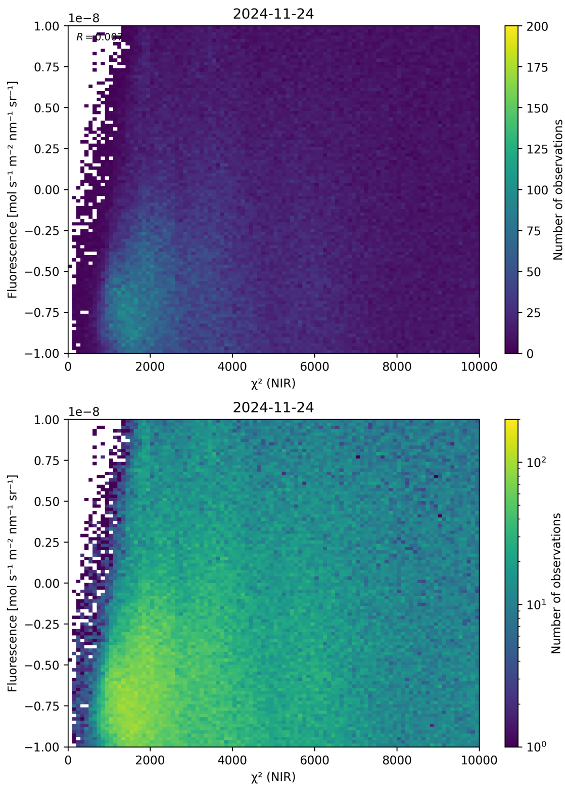
Figure 45: Scatter density plot of “ \chi^2 (NIR)” against “Fluorescence” for 2024-11-23 to 2024-11-25.
