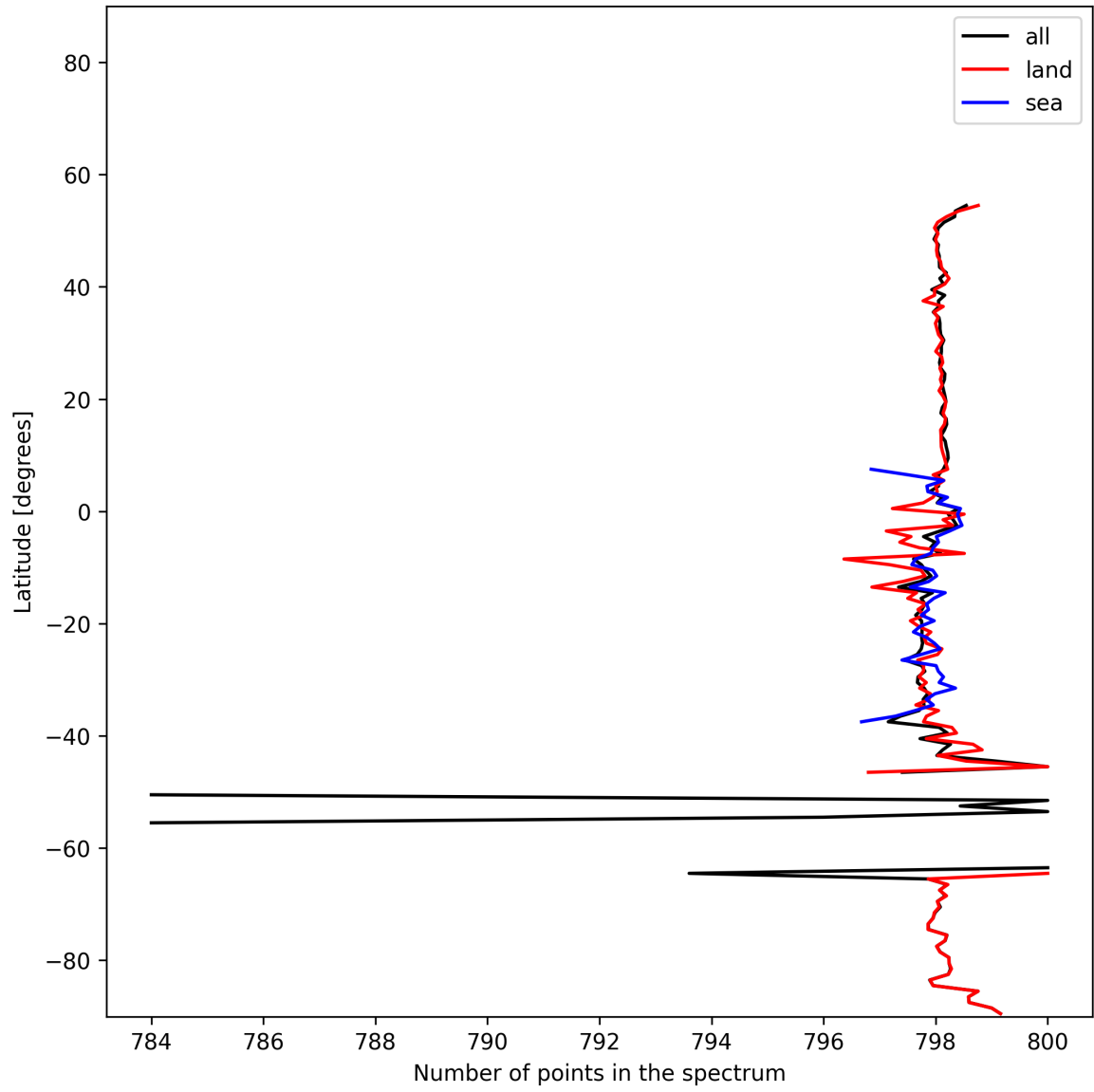
Figure 15: Zonal average of “Number of points in the spectrum” for 2024-11-23 to 2024-11-25.
