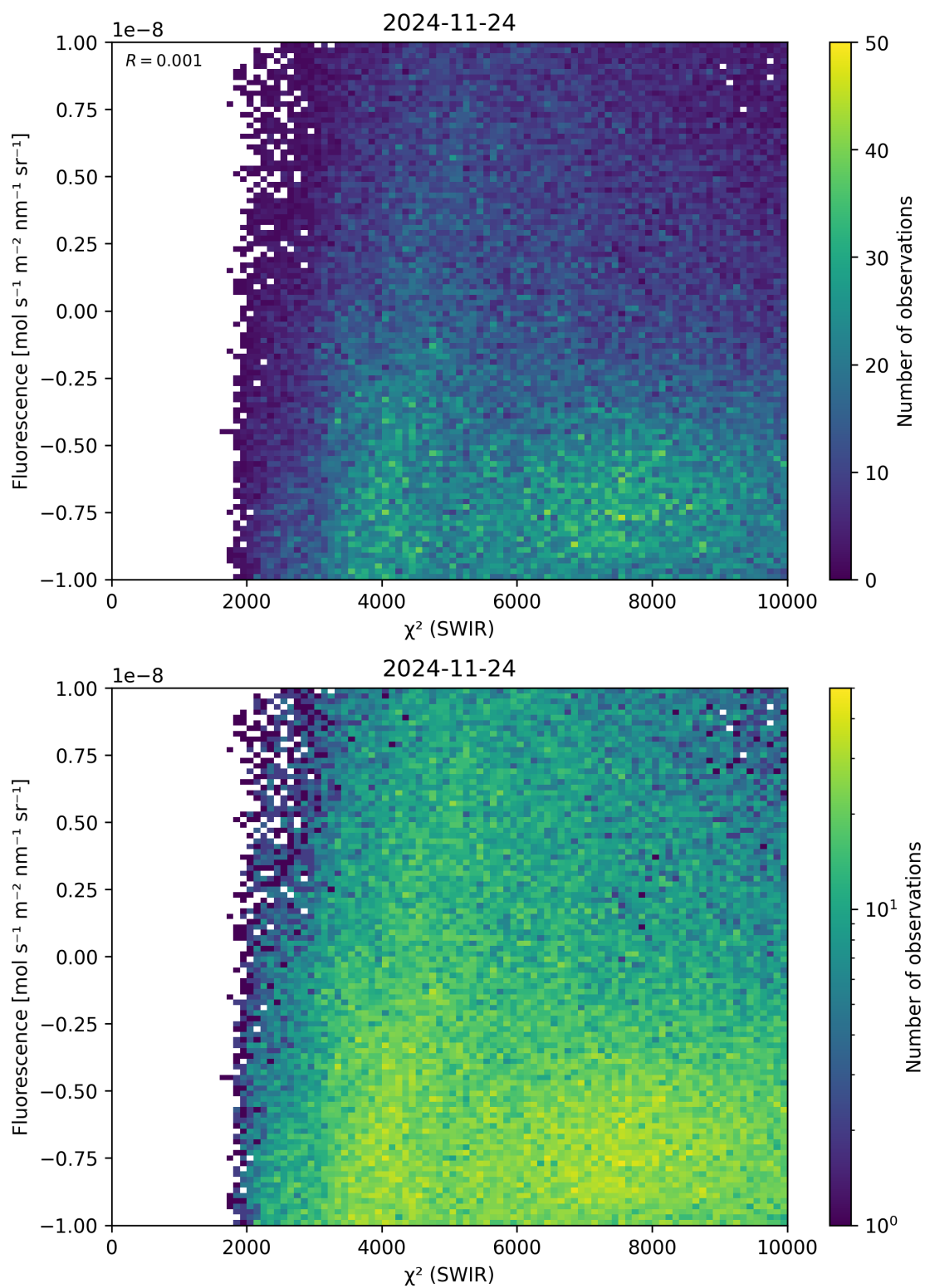
Figure 49: Scatter density plot of “ \chi^2 (SWIR)” against “Fluorescence” for 2024-11-23 to 2024-11-25.
