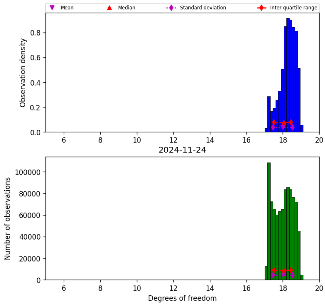
Figure 30: Histogram of “Degrees of freedom” for 2024-11-23 to 2024-11-25
