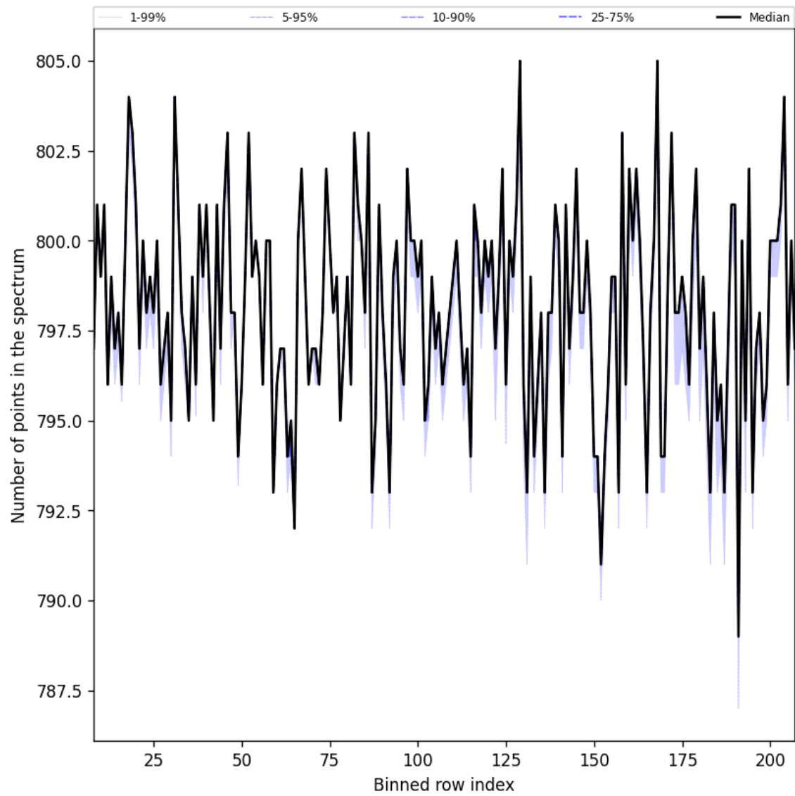
Figure 37: Along track statistics of “Number of points in the spectrum” for 2024-11-23 to 2024-11-25
