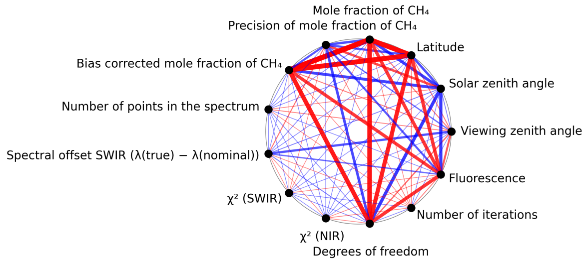
Figure 1: Map of correlation graph for 2024-11-23 to 2024-11-25.
