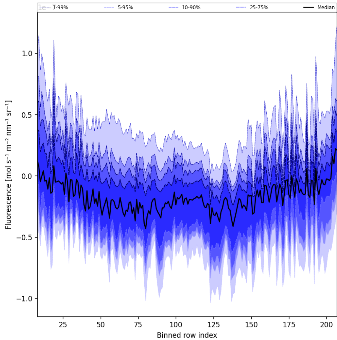
Figure 43: Along track statistics of “Fluorescence” for 2024-11-23 to 2024-11-25
