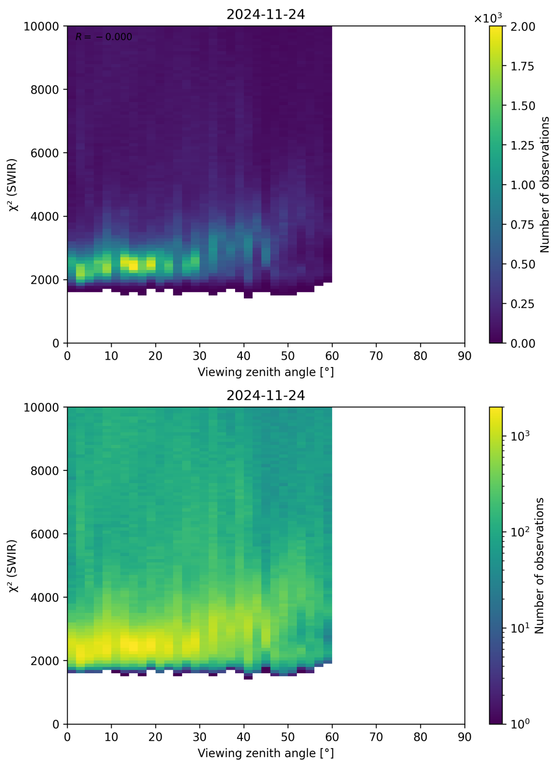
Figure 106: Scatter density plot of “Viewing zenith angle” against “ \chi^2 (SWIR)” for 2024-11-23 to 2024-11-25.
