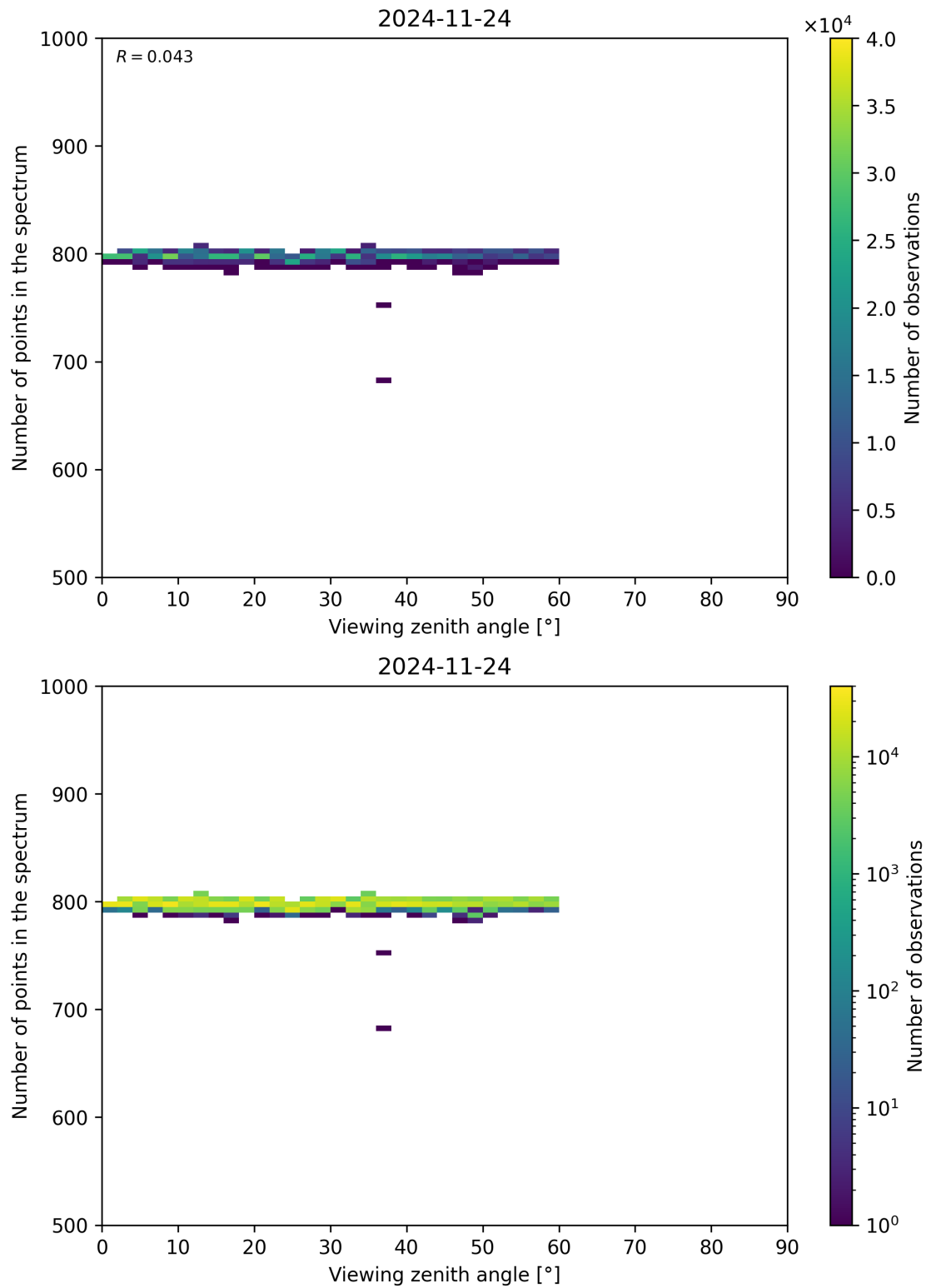
Figure 114: Scatter density plot of “Viewing zenith angle” against “Number of points in the spectrum” for 2024-11-23 to 2024-11-25.
