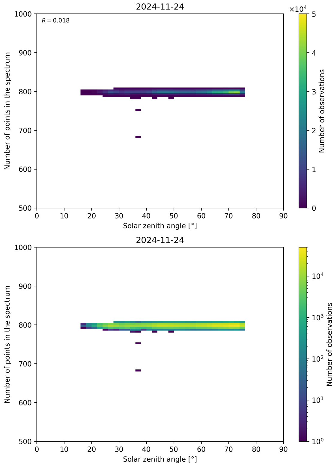
Figure 103: Scatter density plot of “Solar zenith angle” against “Number of points in the spectrum” for 2024-11-23 to 2024-11-25.
