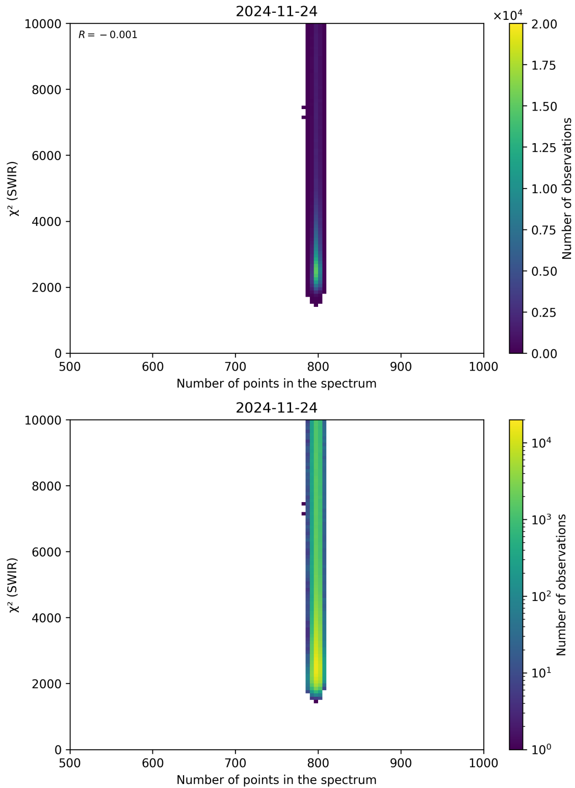
Figure 89: Scatter density plot of “Number of points in the spectrum” against “ \chi^2 (SWIR)” for 2024-11-23 to 2024-11-25.
