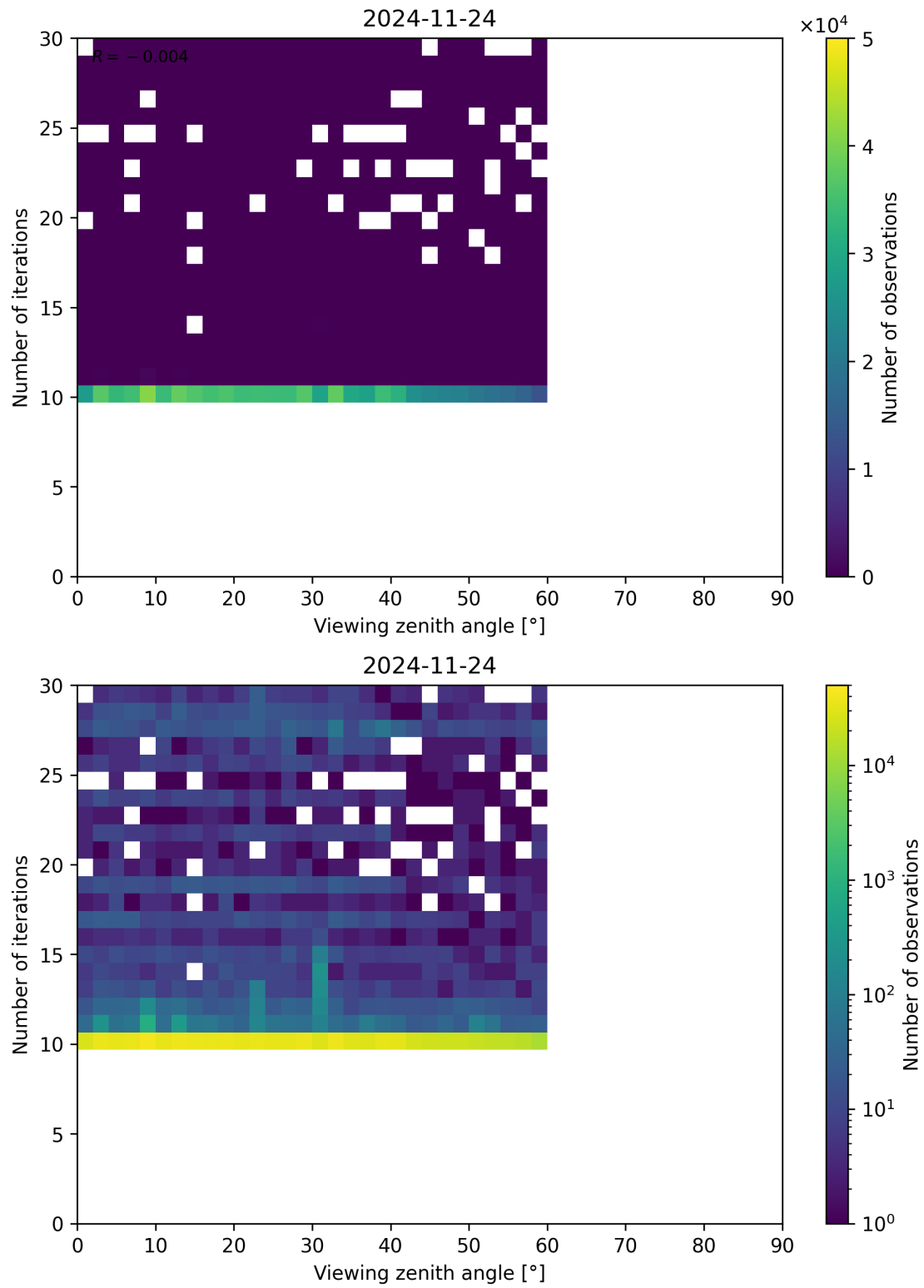
Figure 113: Scatter density plot of “Viewing zenith angle” against “Number of iterations” for 2024-11-23 to 2024-11-25.
