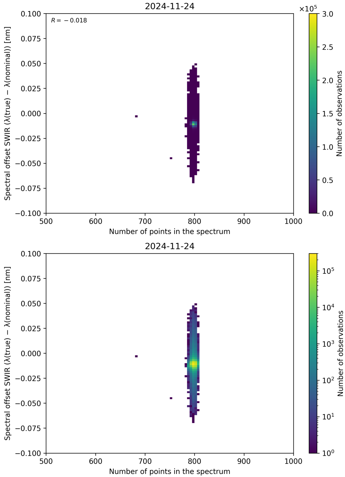
Figure 93: Scatter density plot of “Number of points in the spectrum” against “Spectral offset SWIR ( \lambda_{\text{true}} - \lambda_{\text{nominal}} )” for 2024-11-23 to 2024-11-25.
