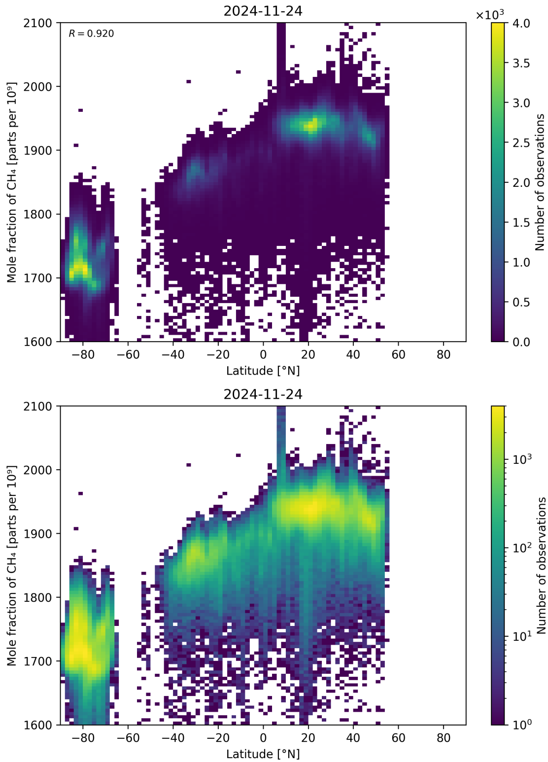
Figure 57: Scatter density plot of “Latitude” against “Mole fraction of CH 4 ” for 2024-11-23 to 2024-11-25.
