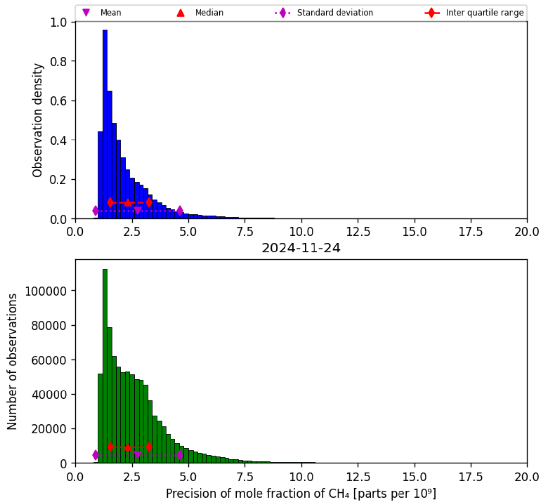
Figure 24: Histogram of “Precision of mole fraction of CH 4 ” for 2024-11-23 to 2024-11-25
