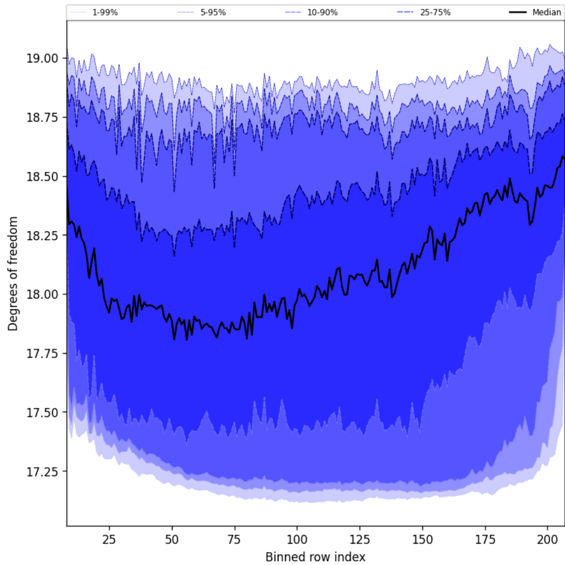
Figure 41: Along track statistics of “Degrees of freedom” for 2024-11-23 to 2024-11-25
