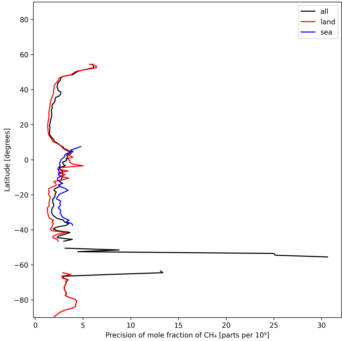
Figure 13: Zonal average of “Precision of mole fraction of CH 4 ” for 2024-11-23 to 2024-11-25.
