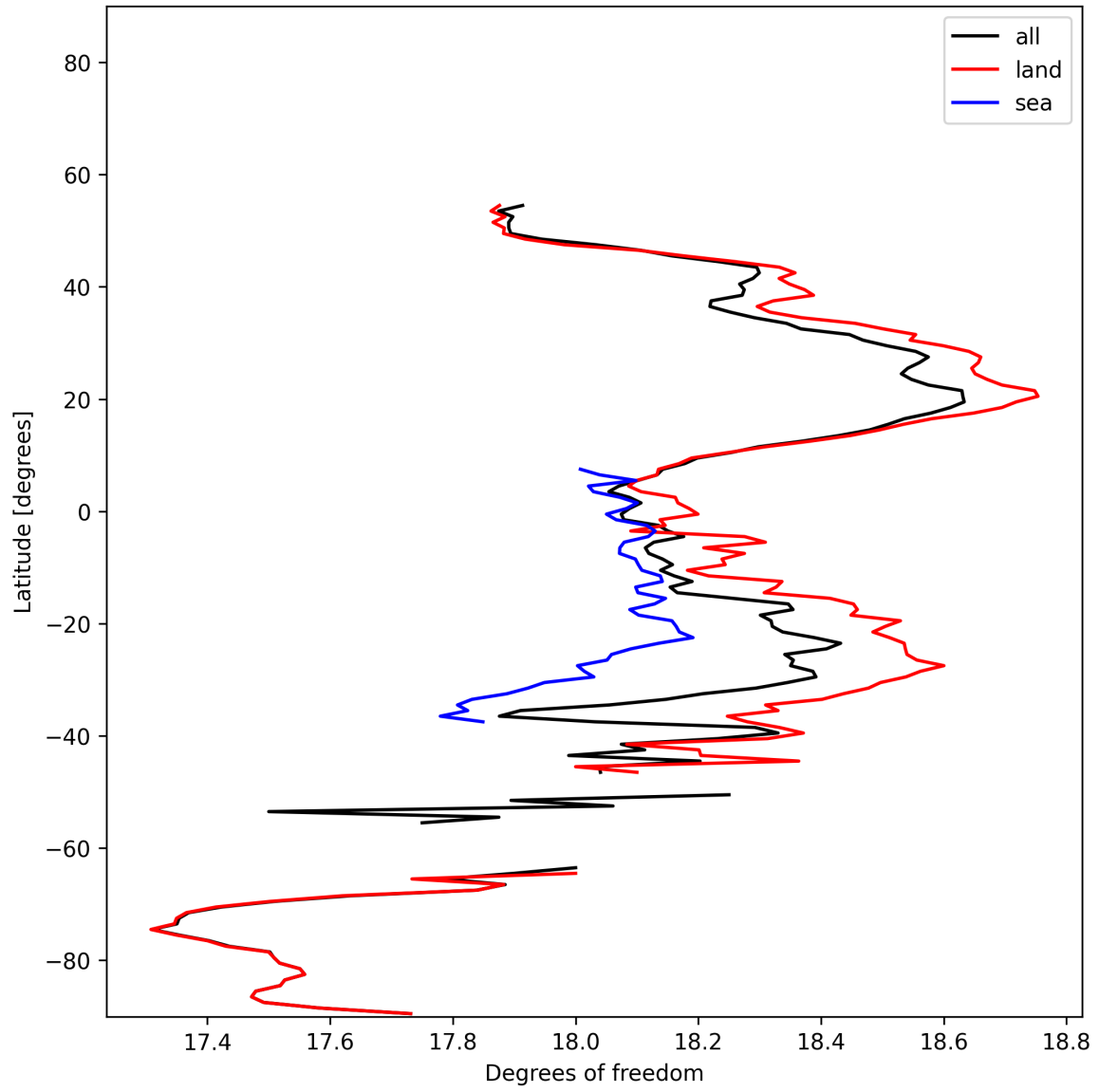
Figure 19: Zonal average of “Degrees of freedom” for 2024-11-23 to 2024-11-25.
