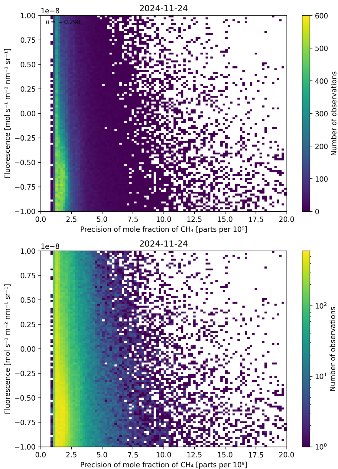
Figure 81: Scatter density plot of “Precision of mole fraction of \text{CH}_4 ” against “Fluorescence” for 2024-11-23 to 2024-11-25.
