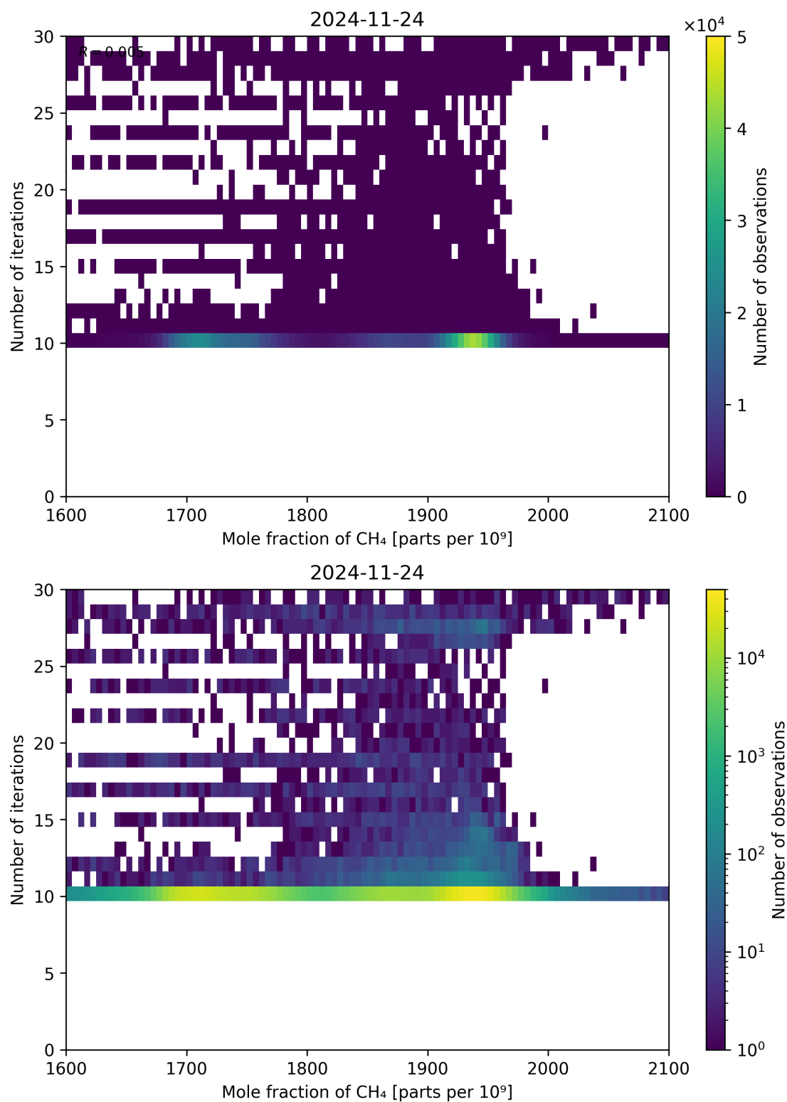
Figure 76: Scatter density plot of “Mole fraction of CH 4 ” against “Number of iterations” for 2024-11-23 to 2024-11-25.
