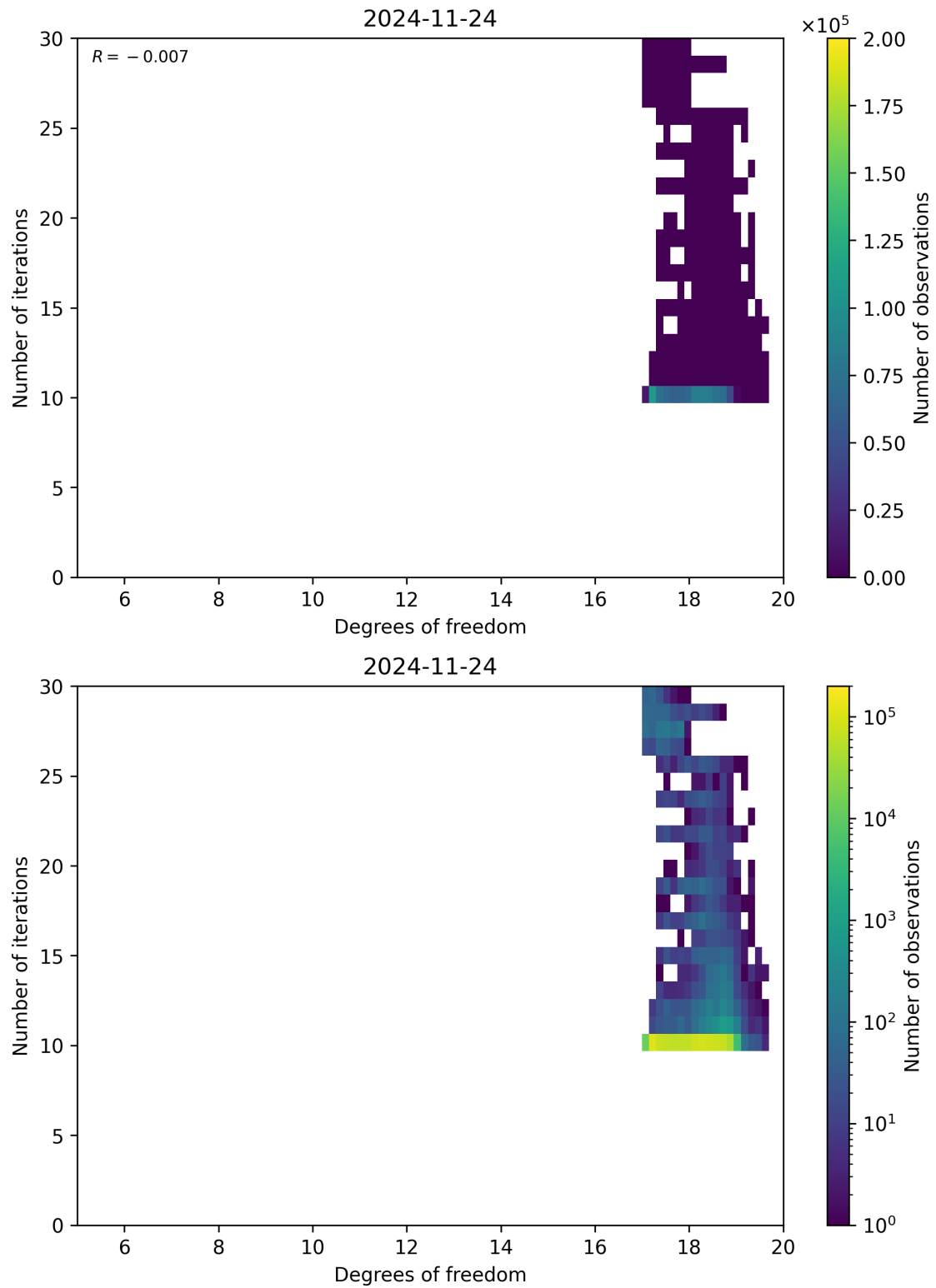
Figure 52: Scatter density plot of “Degrees of freedom” against “Number of iterations” for 2024-11-23 to 2024-11-25.
