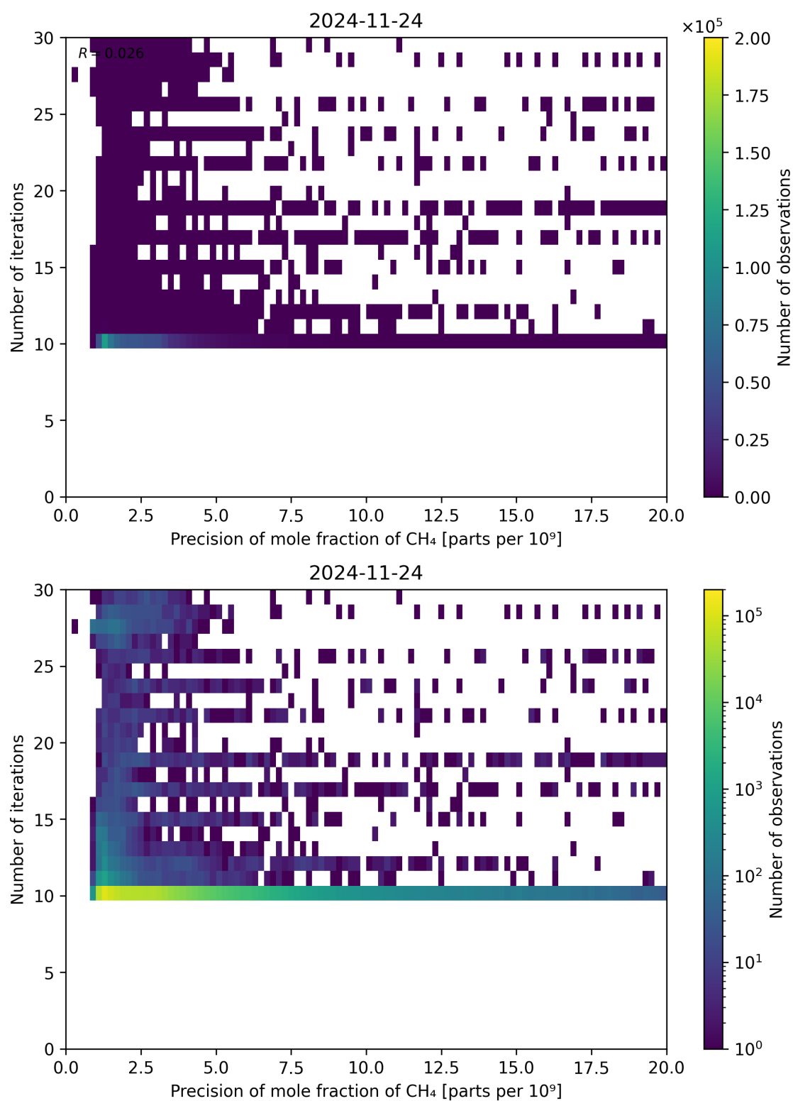
Figure 83: Scatter density plot of “Precision of mole fraction of CH 4 ” against “Number of iterations” for 2024-11-23 to 2024-11-25.
