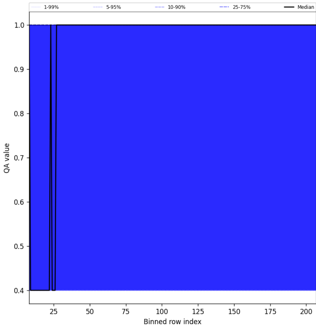
Figure 33: Along track statistics of “QA value” for 2024-11-23 to 2024-11-25
