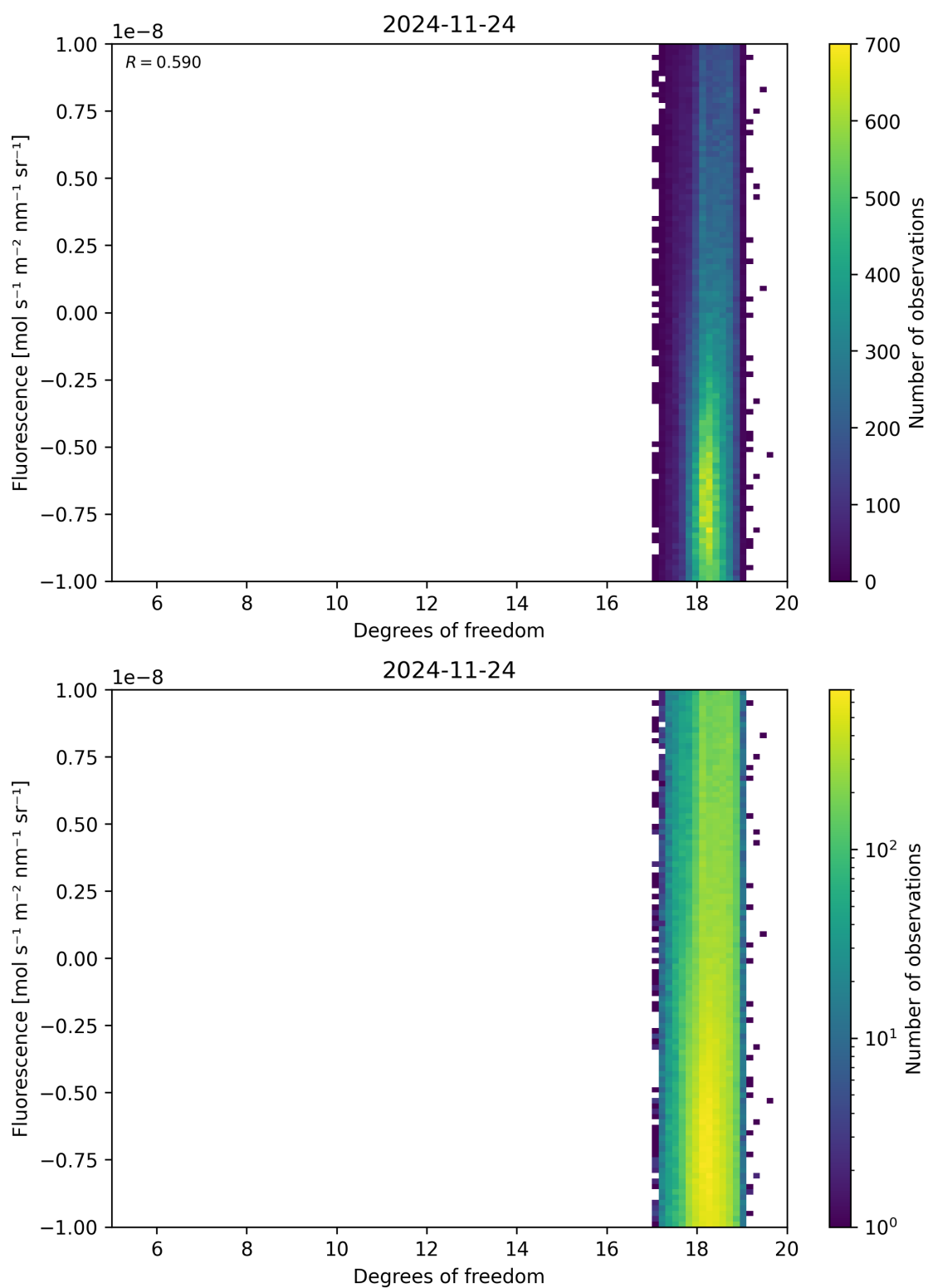
Figure 51: Scatter density plot of “Degrees of freedom” against “Fluorescence” for 2024-11-23 to 2024-11-25.
