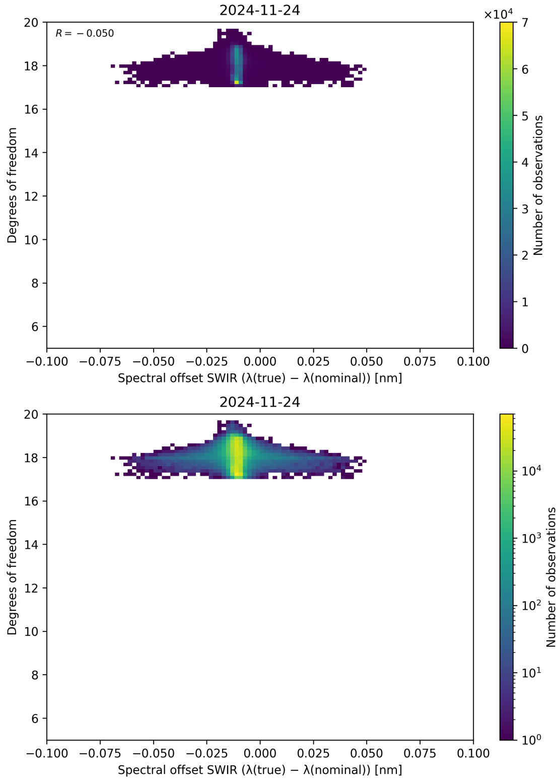
Figure 119: Scatter density plot of “Spectral offset SWIR ( \lambda_{\text{true}} - \lambda_{\text{nominal}} )” against “Degrees of freedom” for 2024-11-23 to 2024-11-25.
