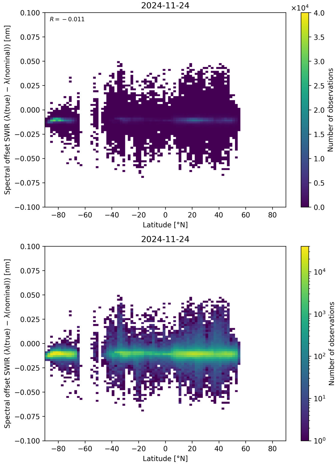
Figure 62: Scatter density plot of “Latitude” against “Spectral offset SWIR ( \lambda_{\text{true}} - \lambda_{\text{nominal}} )” for 2024-11-23 to 2024-11-25.
