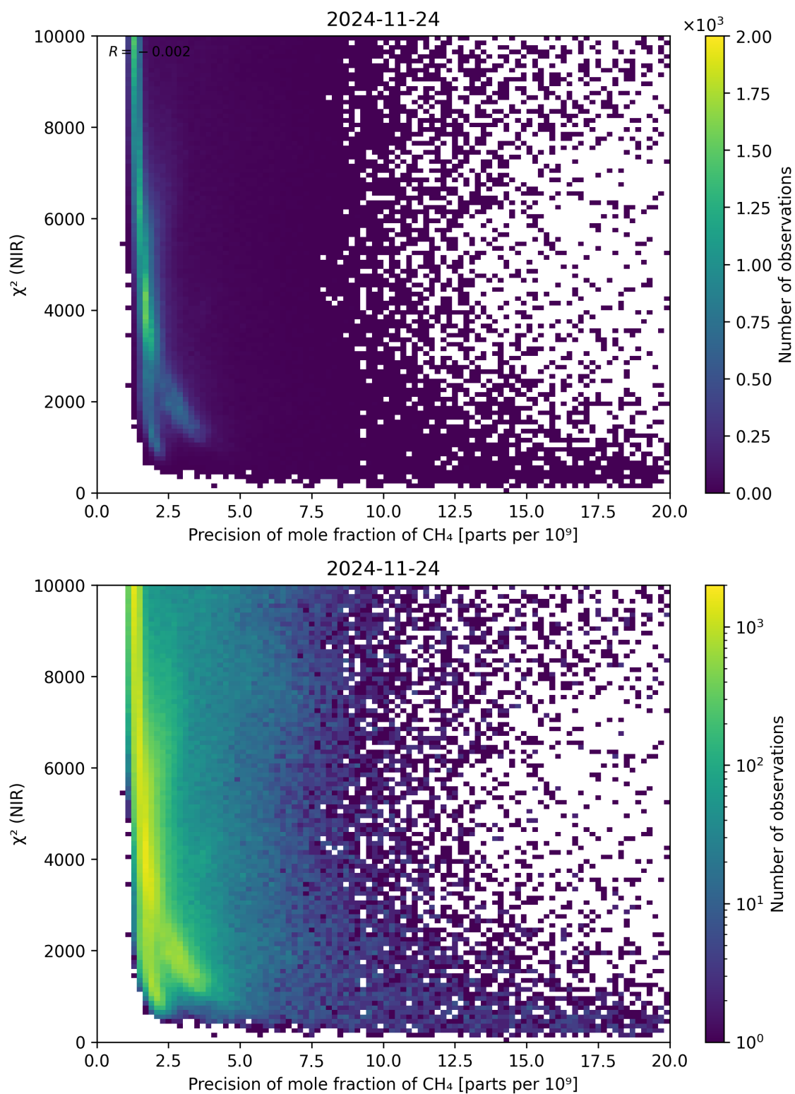
Figure 78: Scatter density plot of “Precision of mole fraction of CH 4 ” against “ \chi^2 (NIR)” for 2024-11-23 to 2024-11-25.
