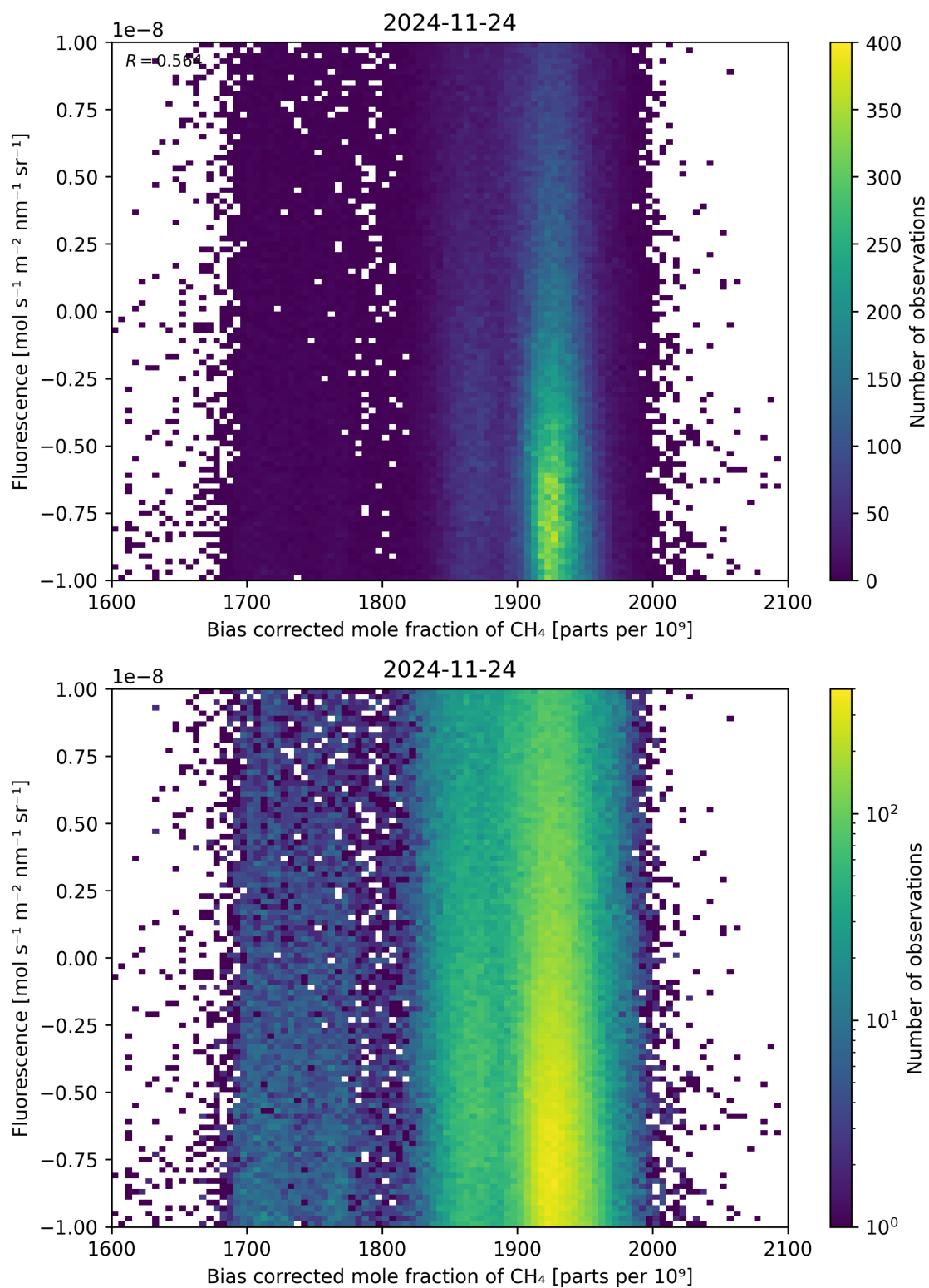
Figure 66: Scatter density plot of “Bias corrected mole fraction of \text{CH}_4 ” against “Fluorescence” for 2024-11-23 to 2024-11-25.
