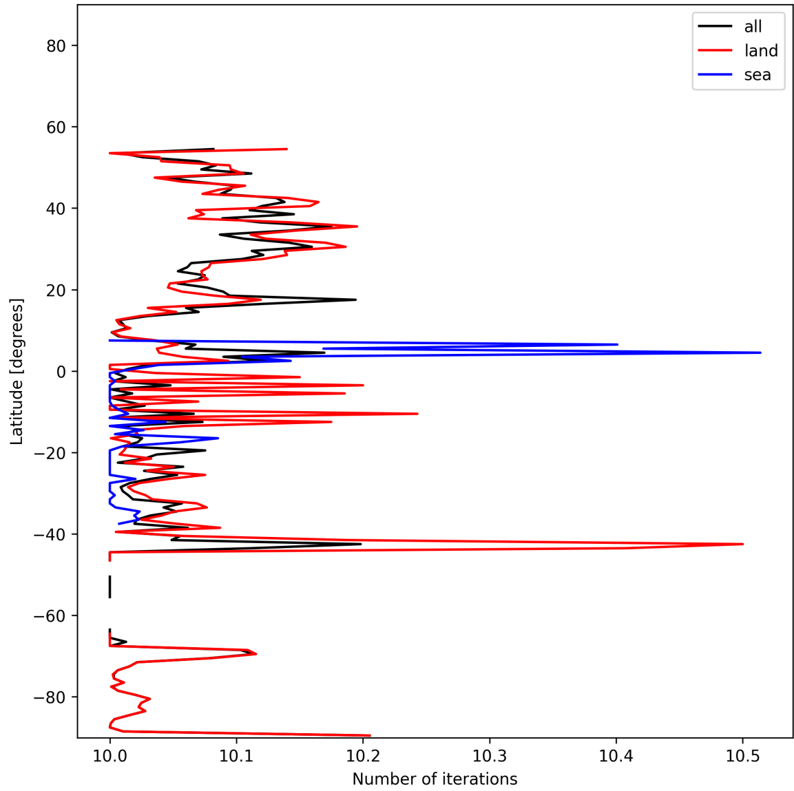
Figure 20: Zonal average of “Number of iterations” for 2024-11-23 to 2024-11-25.
