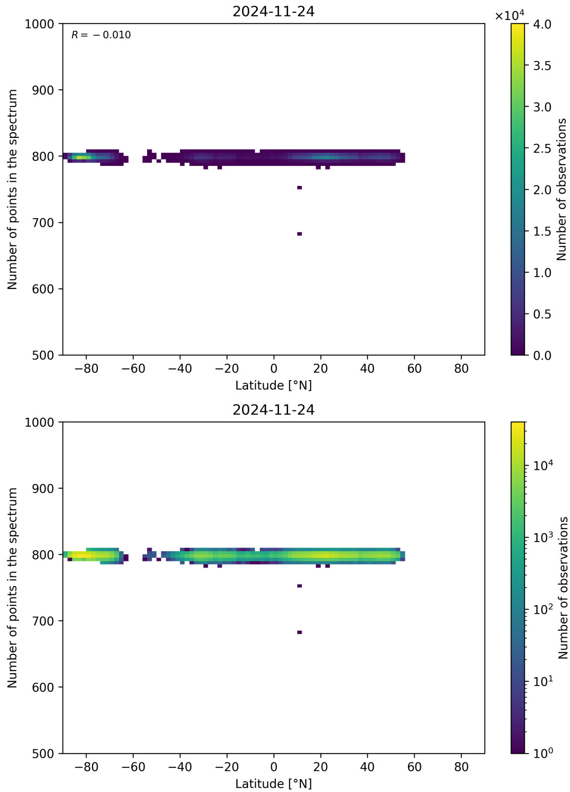
Figure 61: Scatter density plot of “Latitude” against “Number of points in the spectrum” for 2024-11-23 to 2024-11-25.
