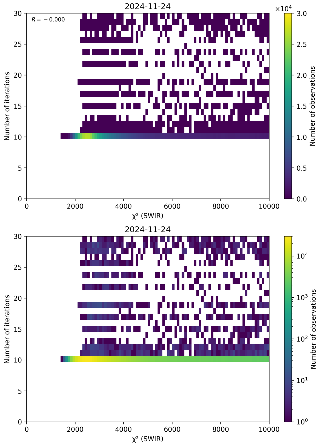
Figure 50: Scatter density plot of “ \chi^2 (SWIR)” against “Number of iterations” for 2024-11-23 to 2024-11-25.
