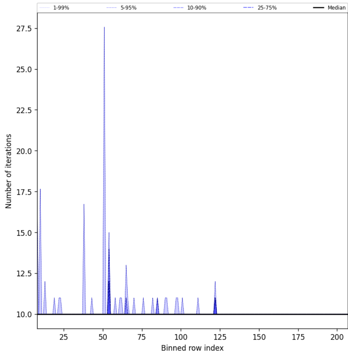
Figure 42: Along track statistics of “Number of iterations” for 2024-11-23 to 2024-11-25
