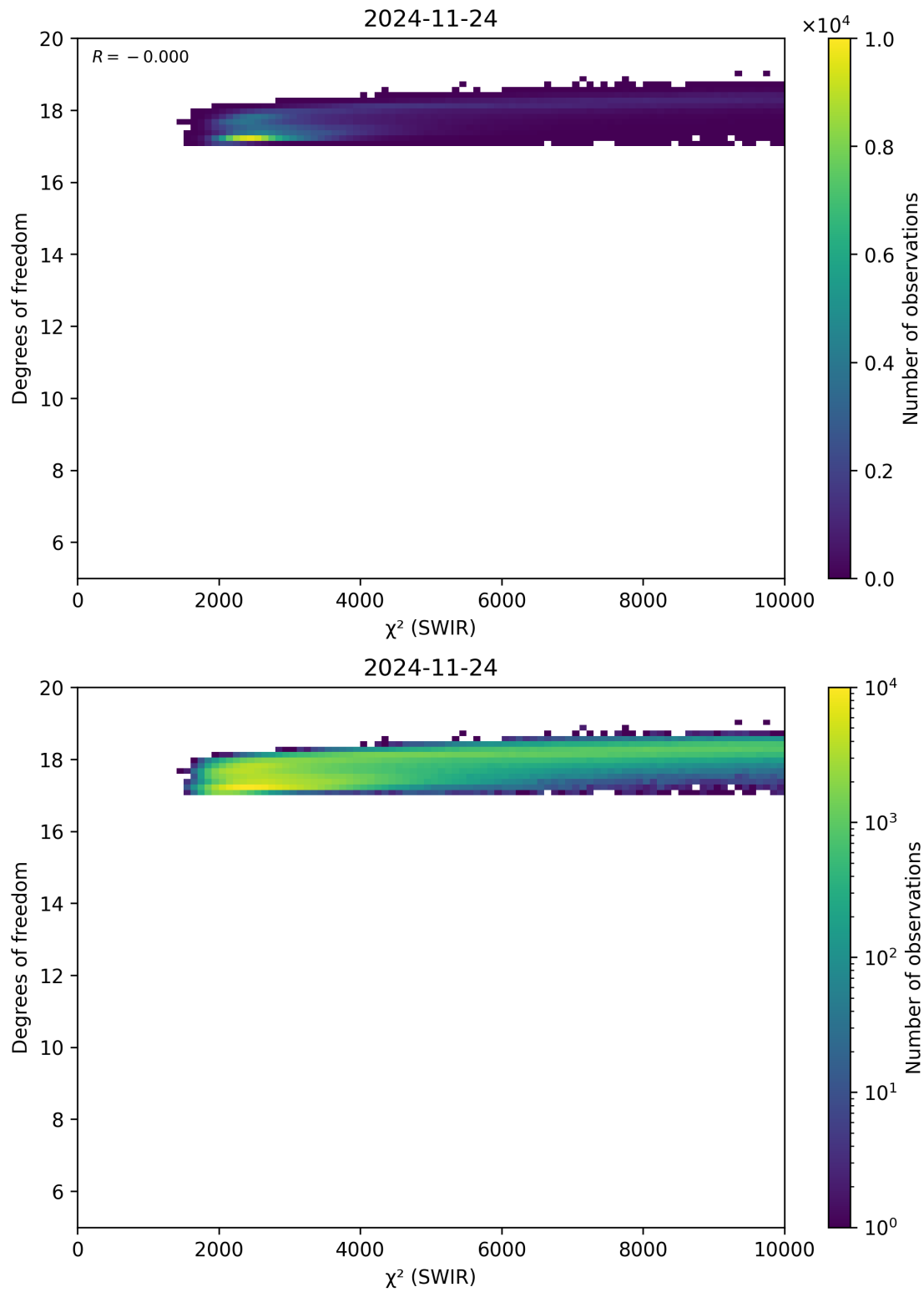
Figure 48: Scatter density plot of “ \chi^2 (SWIR)” against “Degrees of freedom” for 2024-11-23 to 2024-11-25.
