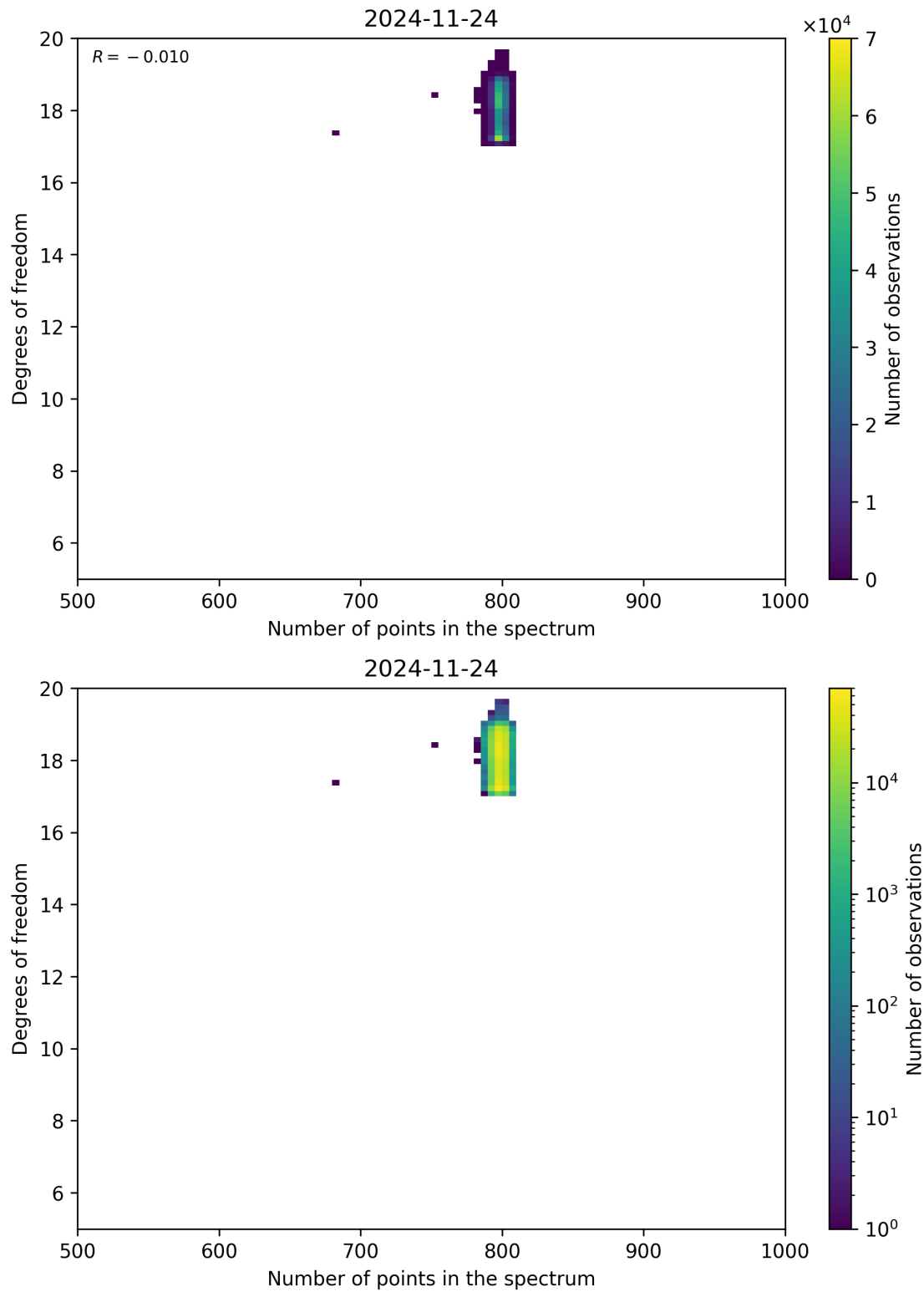
Figure 90: Scatter density plot of “Number of points in the spectrum” against “Degrees of freedom” for 2024-11-23 to 2024-11-25.
