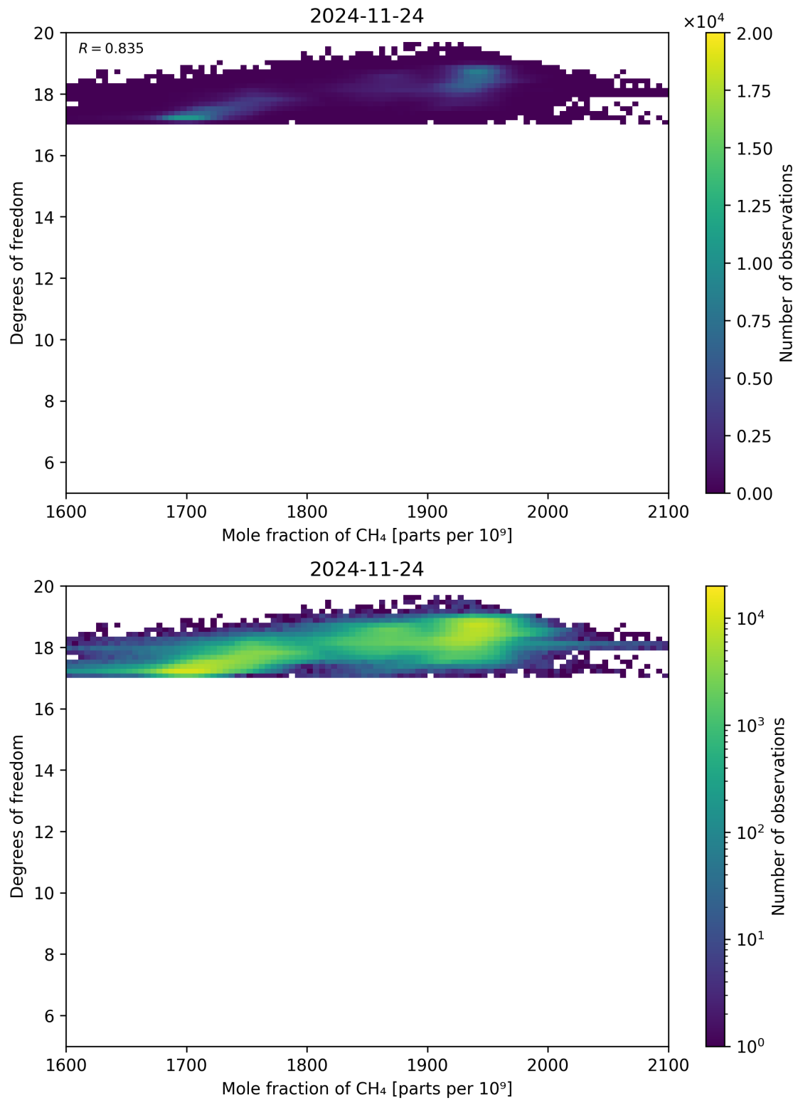
Figure 72: Scatter density plot of “Mole fraction of CH 4 ” against “Degrees of freedom” for 2024-11-23 to 2024-11-25.
