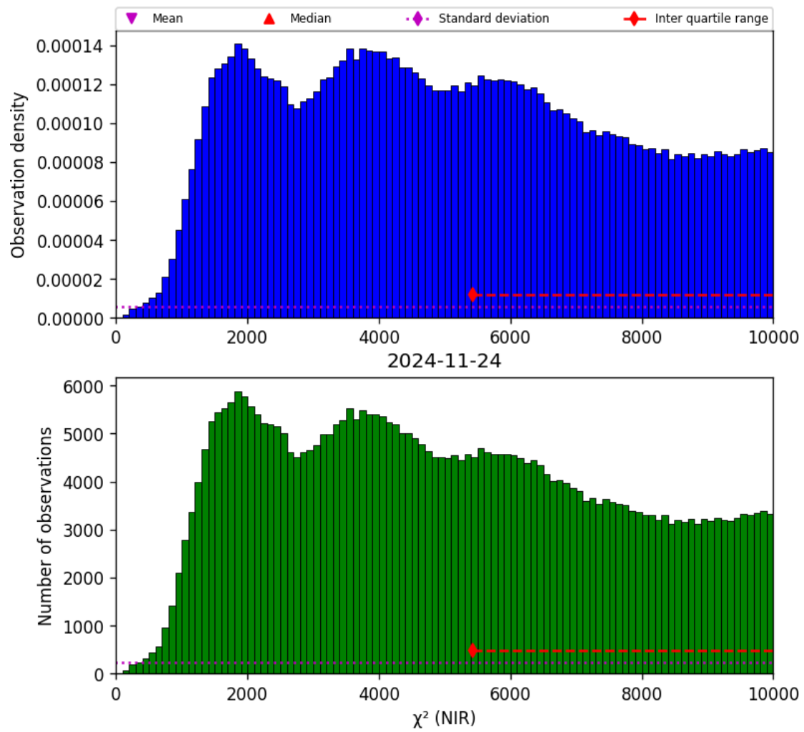
Figure 29: Histogram of “ \chi^2 (NIR)” for 2024-11-23 to 2024-11-25
