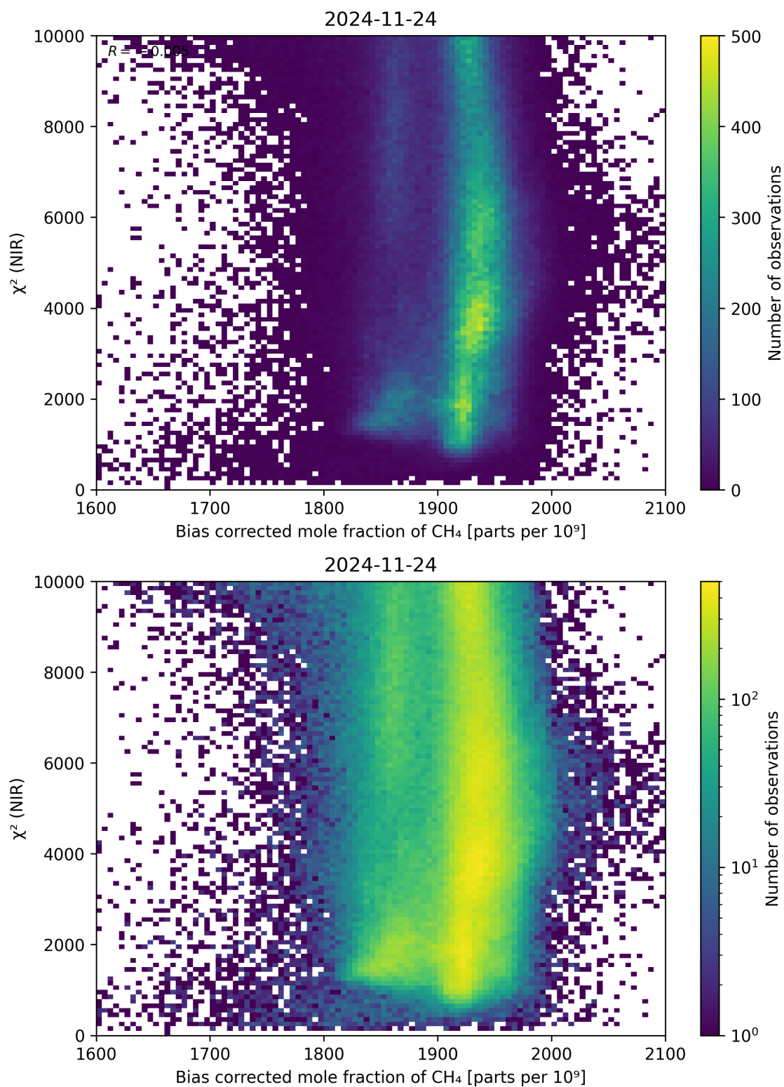
Figure 63: Scatter density plot of “Bias corrected mole fraction of CH 4 ” against “ \chi^2 (NIR)” for 2024-11-23 to 2024-11-25.
