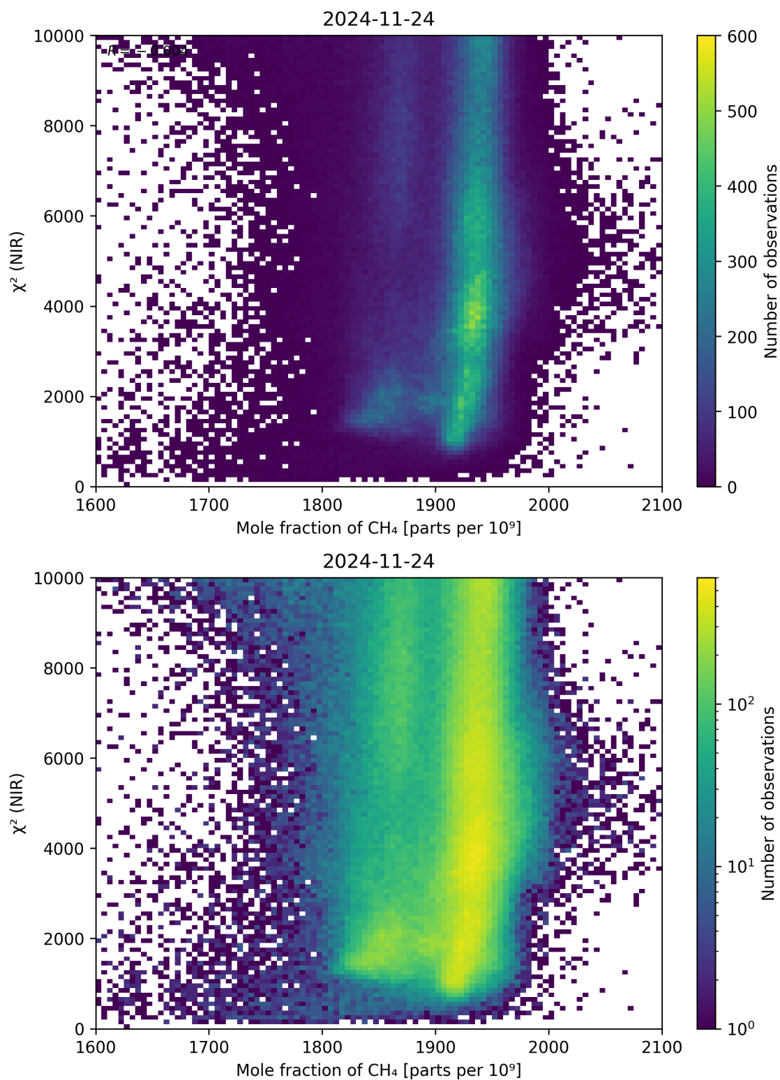
Figure 70: Scatter density plot of “Mole fraction of CH 4 ” against “ \chi^2 (NIR)” for 2024-11-23 to 2024-11-25.
