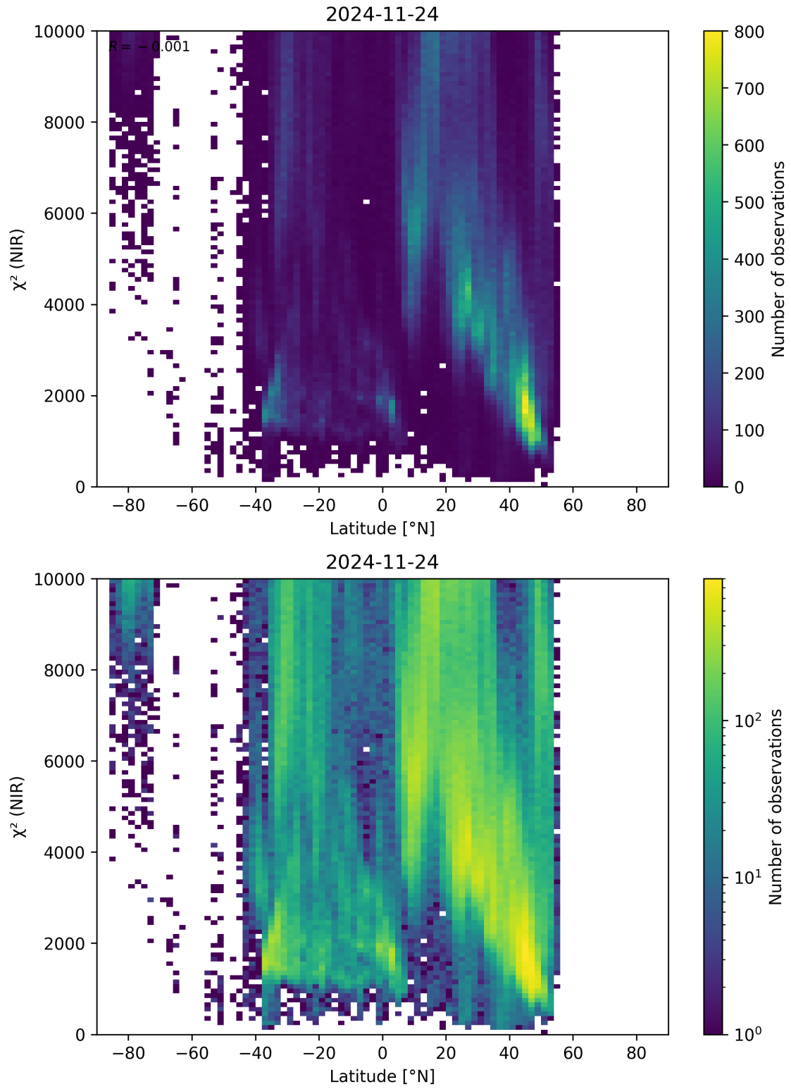
Figure 53: Scatter density plot of “Latitude” against “ \chi^2 (NIR)” for 2024-11-23 to 2024-11-25.
