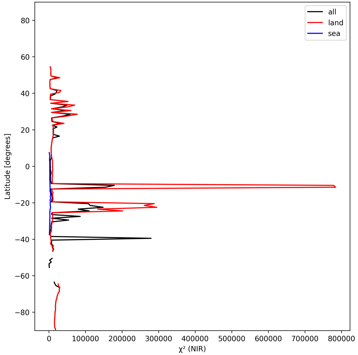
Figure 18: Zonal average of “ \chi^2 (NIR)” for 2024-11-23 to 2024-11-25.
