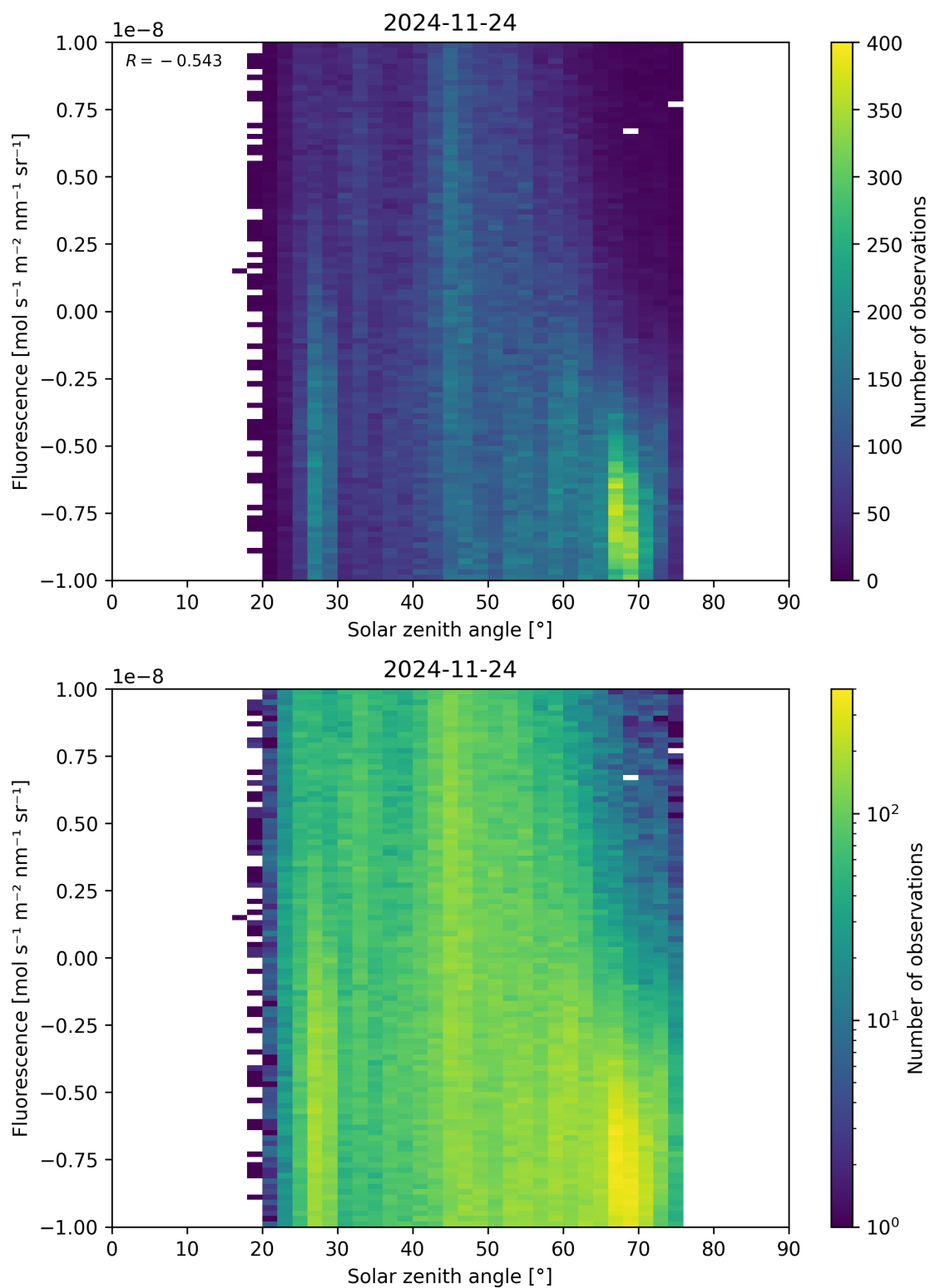
Figure 97: Scatter density plot of “Solar zenith angle” against “Fluorescence” for 2024-11-23 to 2024-11-25.
