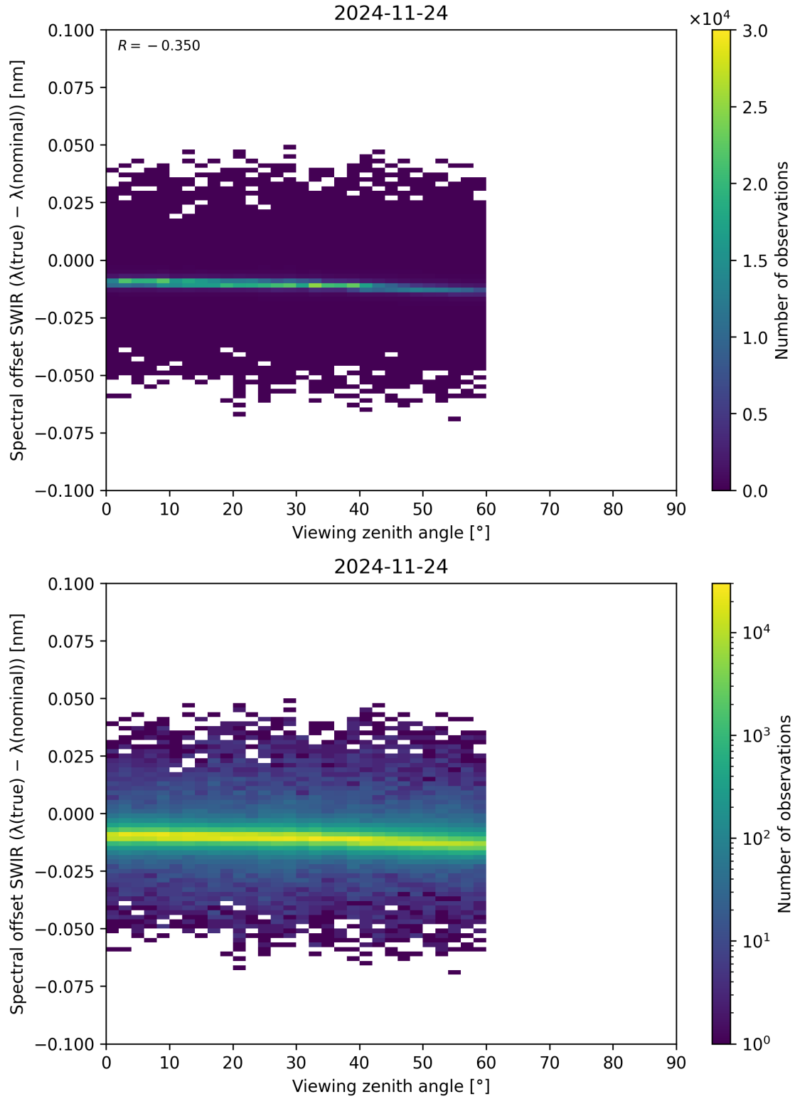
Figure 116: Scatter density plot of “Viewing zenith angle” against “Spectral offset SWIR ( \lambda_{\text{true}} - \lambda_{\text{nominal}} )” for 2024-11-23 to 2024-11-25.
