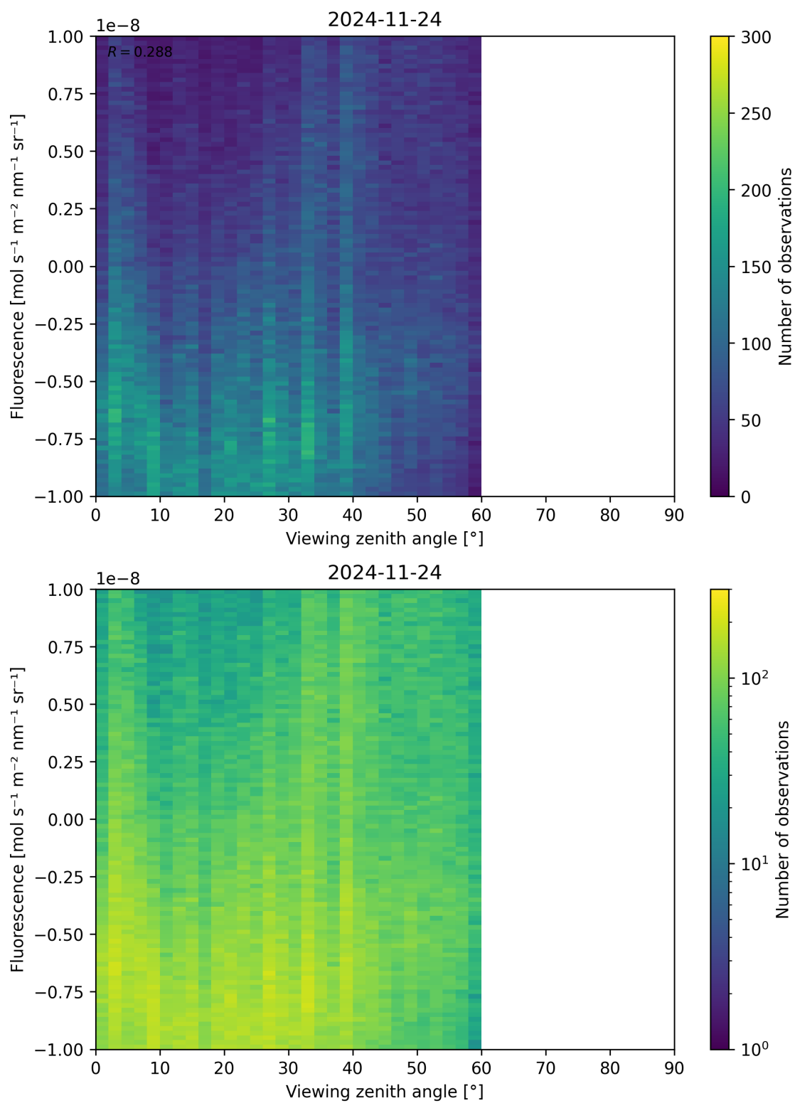
Figure 108: Scatter density plot of “Viewing zenith angle” against “Fluorescence” for 2024-11-23 to 2024-11-25.
