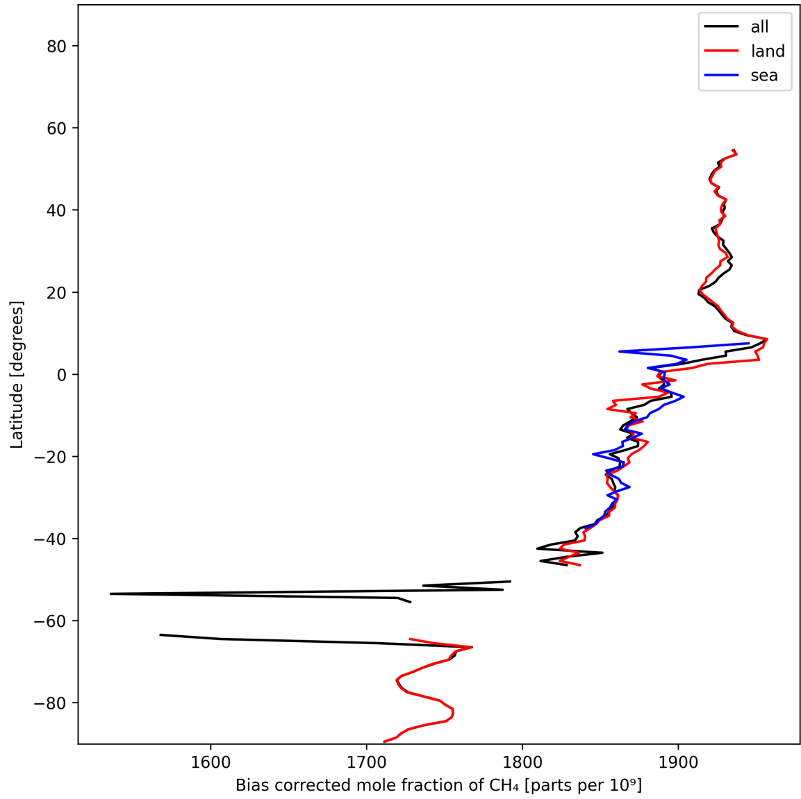
Figure 14: Zonal average of “Bias corrected mole fraction of CH 4 ” for 2024-11-23 to 2024-11-25.
