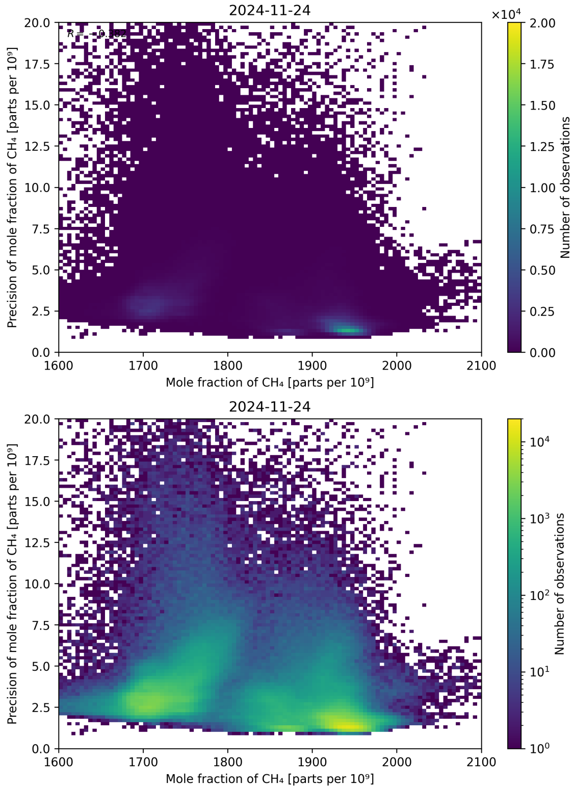
Figure 75: Scatter density plot of “Mole fraction of CH 4 ” against “Precision of mole fraction of CH 4 ” for 2024-11-23 to 2024-11-25.
