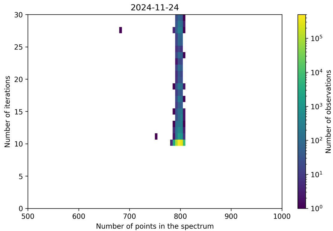
Figure 92: Scatter density plot of “Number of points in the spectrum” against “Number of iterations” for 2024-11-23 to 2024-11-25.
