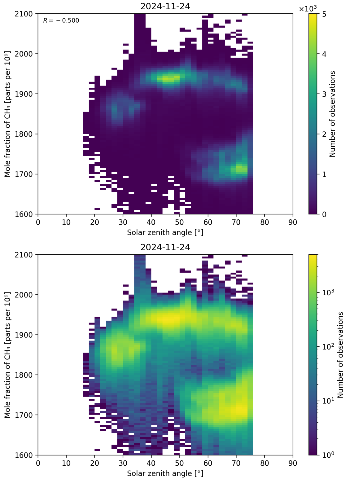
Figure 99: Scatter density plot of “Solar zenith angle” against “Mole fraction of CH 4 ” for 2024-11-23 to 2024-11-25.
