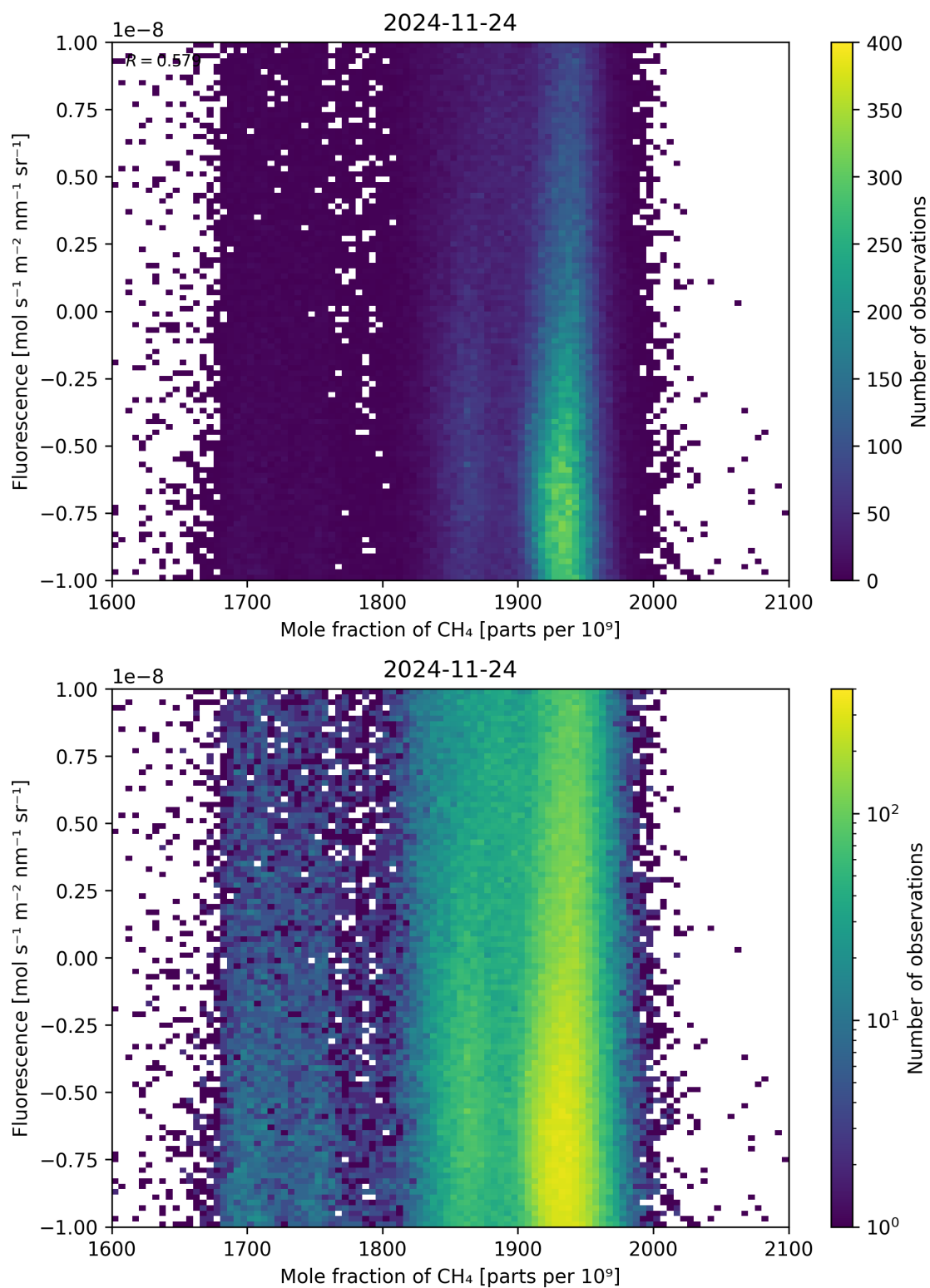
Figure 73: Scatter density plot of “Mole fraction of CH 4 ” against “Fluorescence” for 2024-11-23 to 2024-11-25.
