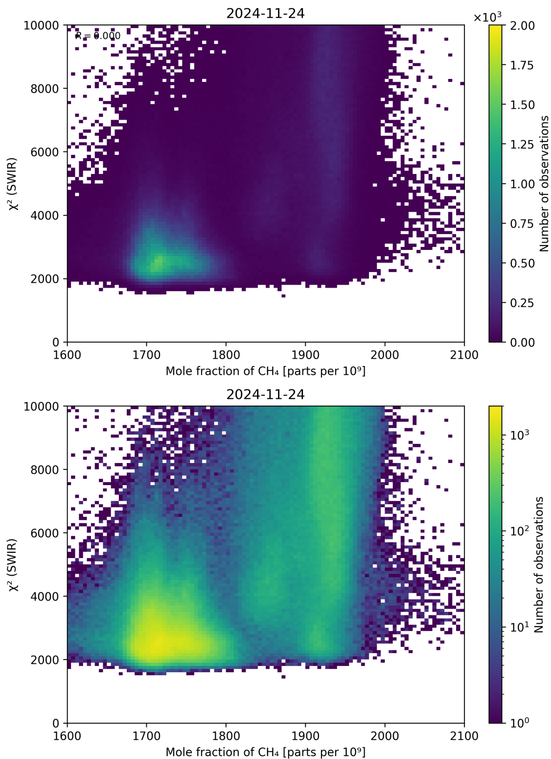
Figure 71: Scatter density plot of “Mole fraction of \text{CH}_4 ” against “ \chi^2 (SWIR)” for 2024-11-23 to 2024-11-25.
