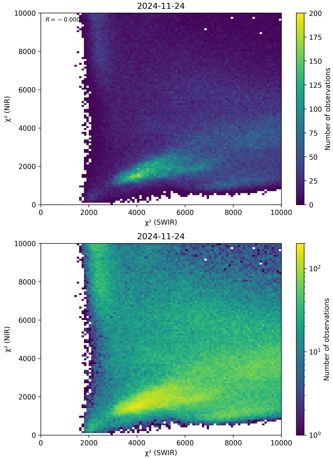
Figure 47: Scatter density plot of “ \chi^2 (SWIR)” against “ \chi^2 (NIR)” for 2024-11-23 to 2024-11-25.
