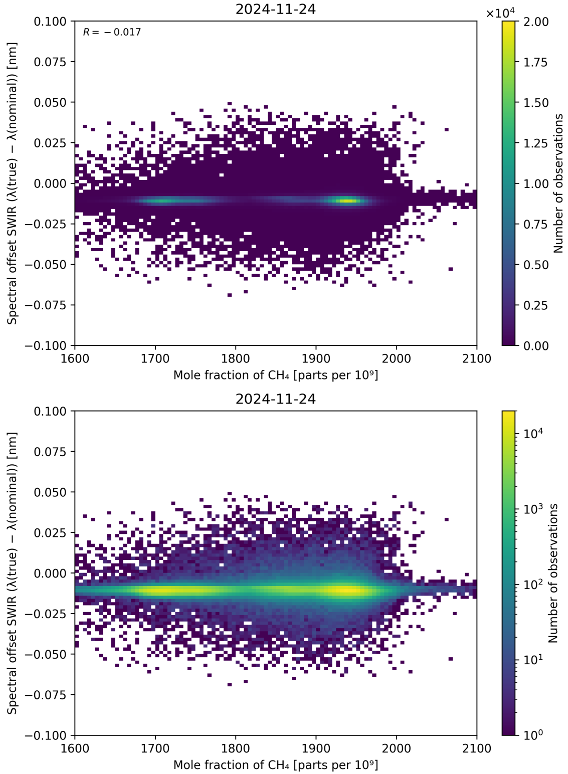
Figure 86: Scatter density plot of “Mole fraction of \text{CH}_4 ” against “Spectral offset SWIR ( \lambda_{\text{true}} - \lambda_{\text{nominal}} )” for 2024-11-23 to 2024-11-25.
