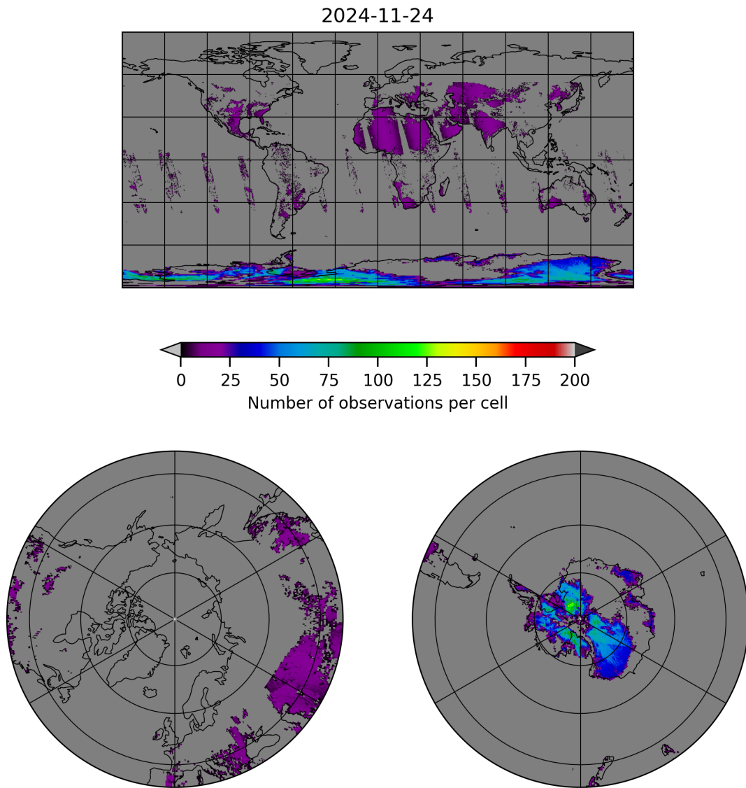
Figure 10: Map of the number of observations for 2024-11-23 to 2024-11-25
