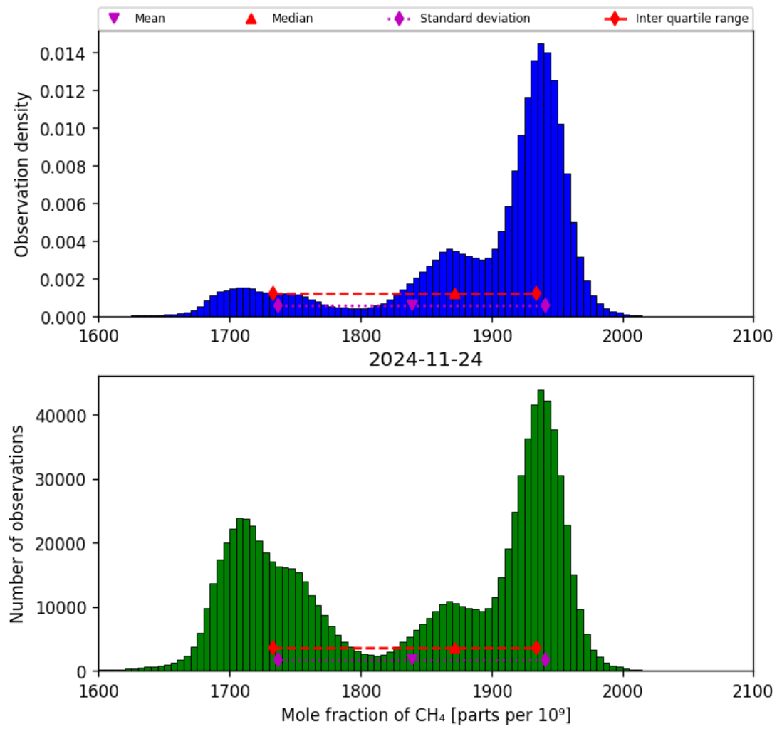
Figure 23: Histogram of “Mole fraction of CH 4 ” for 2024-11-23 to 2024-11-25
