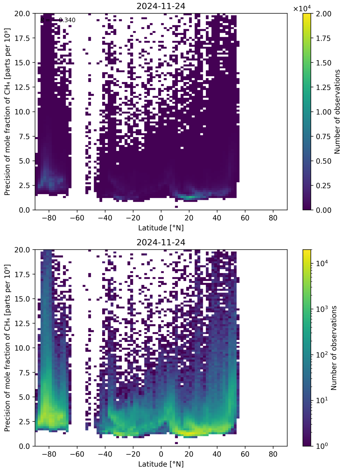
Figure 59: Scatter density plot of “Latitude” against “Precision of mole fraction of CH 4 ” for 2024-11-23 to 2024-11-25.
