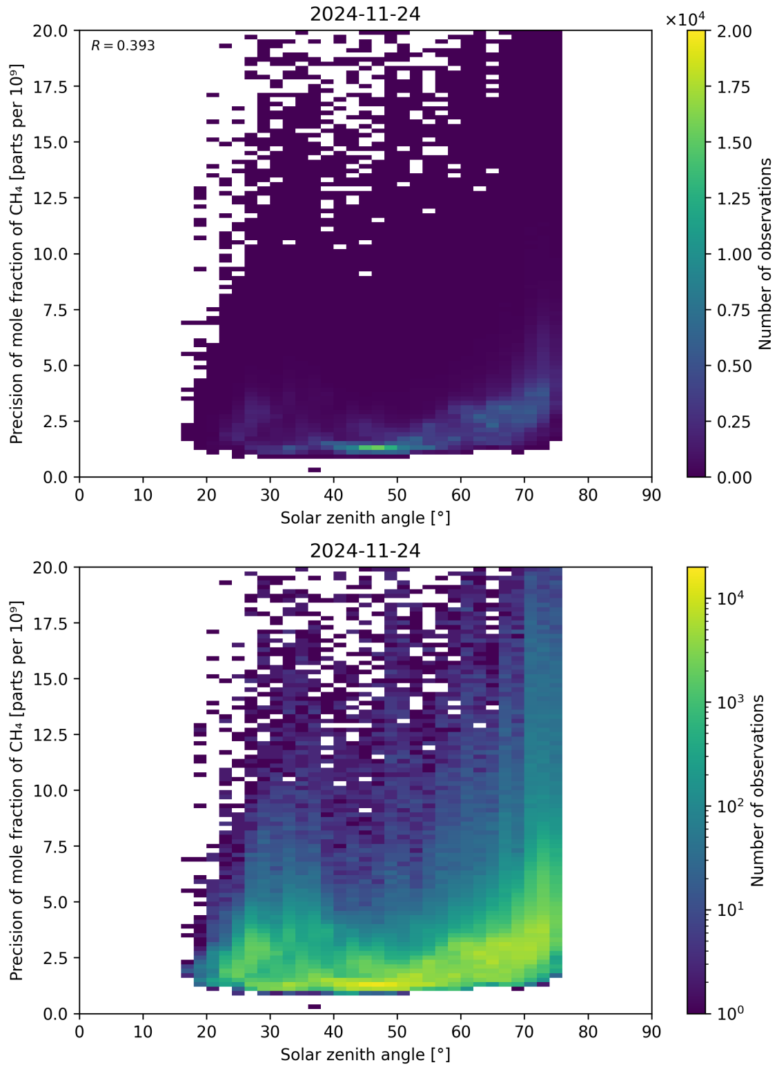
Figure 101: Scatter density plot of “Solar zenith angle” against “Precision of mole fraction of \text{CH}_4 ” for 2024-11-23 to 2024-11-25.
