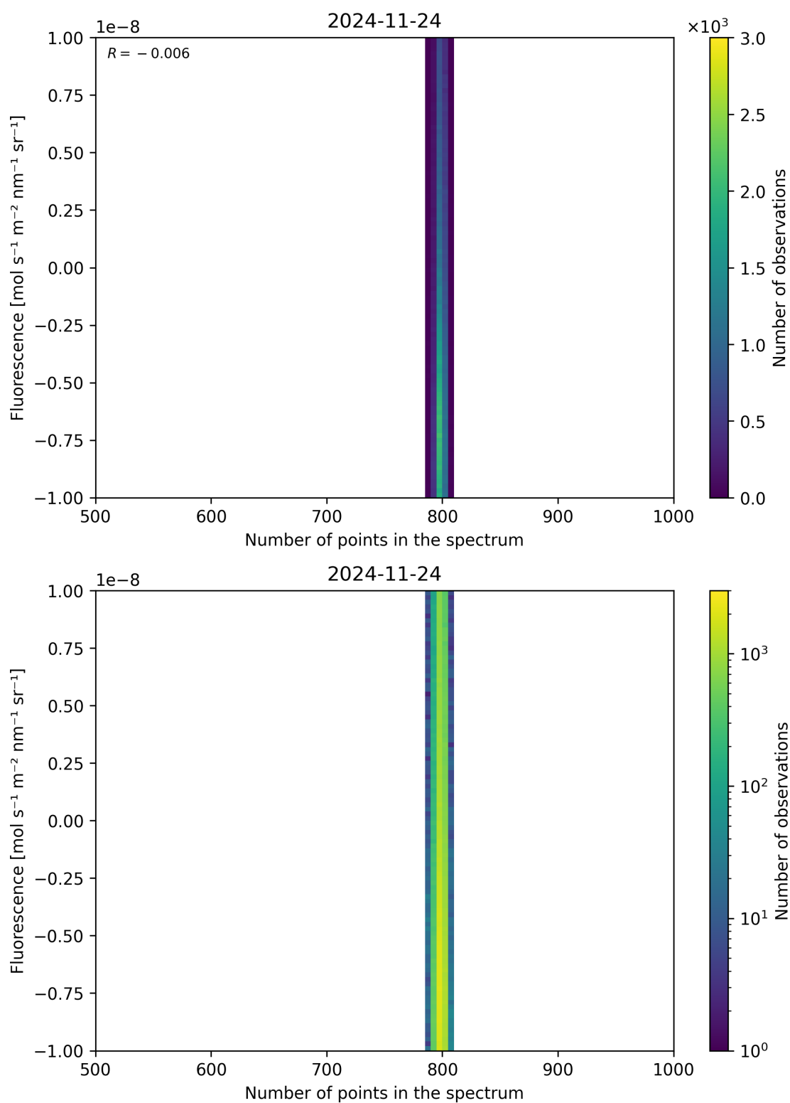
Figure 91: Scatter density plot of “Number of points in the spectrum” against “Fluorescence” for 2024-11-23 to 2024-11-25.
