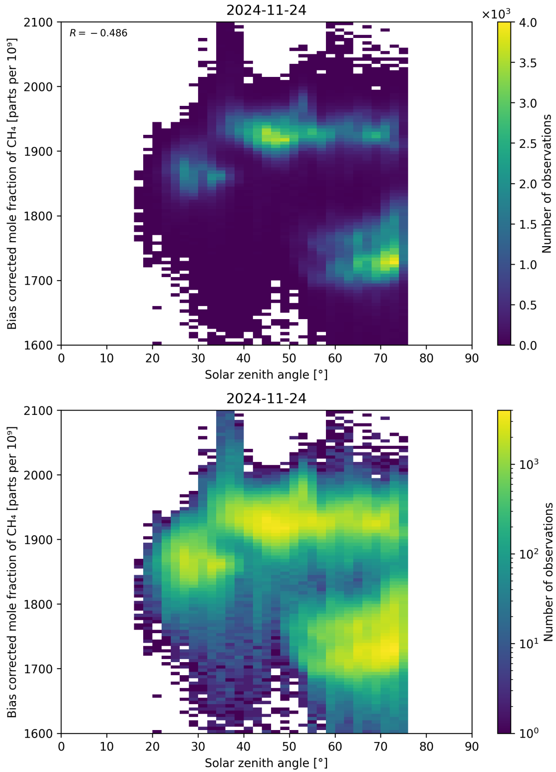
Figure 100: Scatter density plot of “Solar zenith angle” against “Bias corrected mole fraction of CH 4 ” for 2024-11-23 to 2024-11-25.
