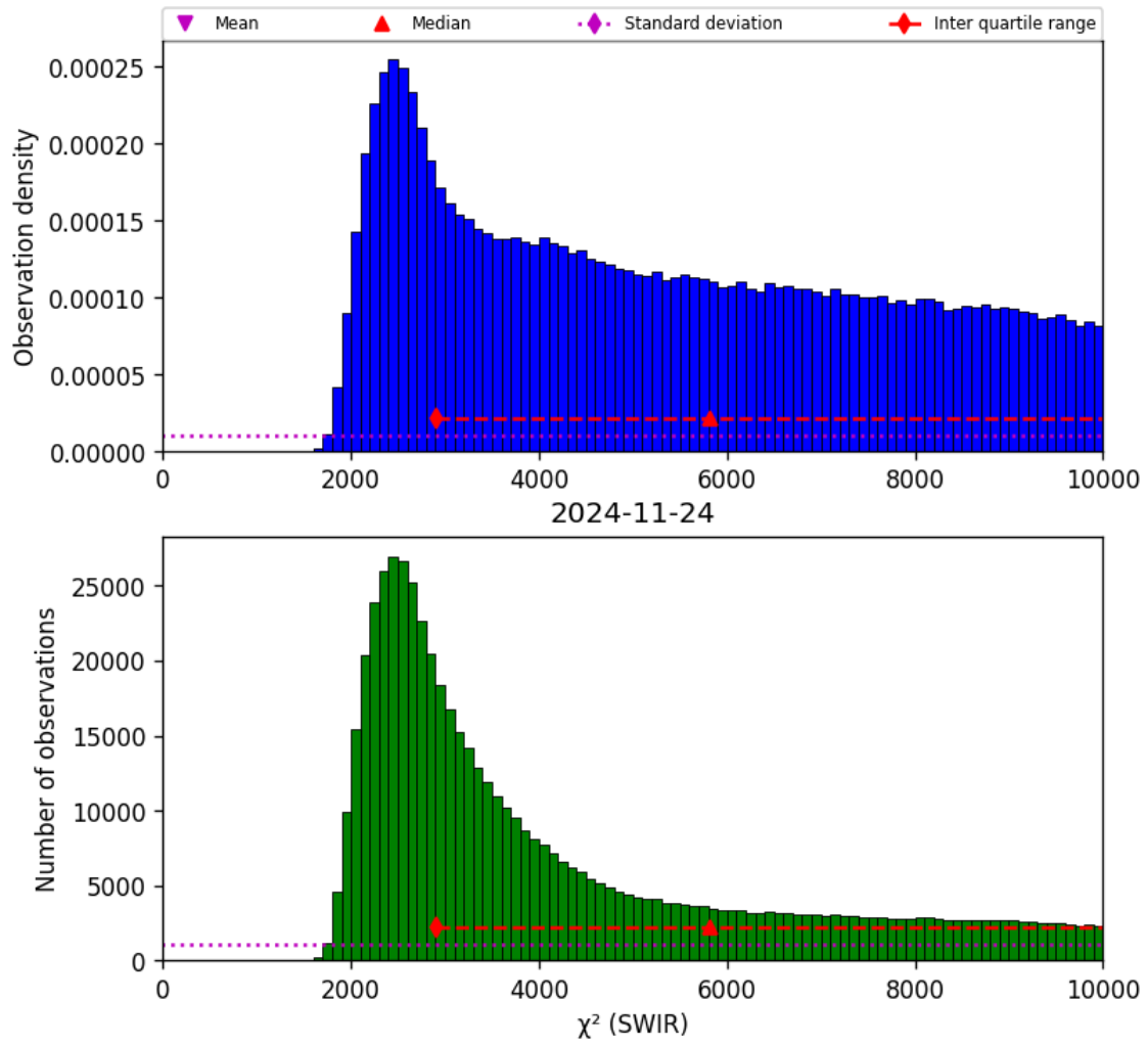
Figure 28: Histogram of “ \chi^2 (SWIR)” for 2024-11-23 to 2024-11-25
