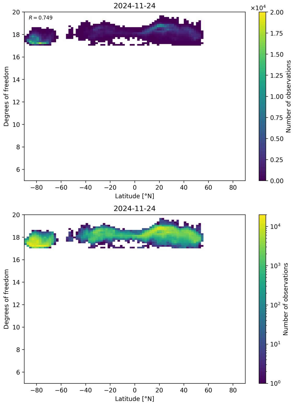
Figure 55: Scatter density plot of “Latitude” against “Degrees of freedom” for 2024-11-23 to 2024-11-25.
