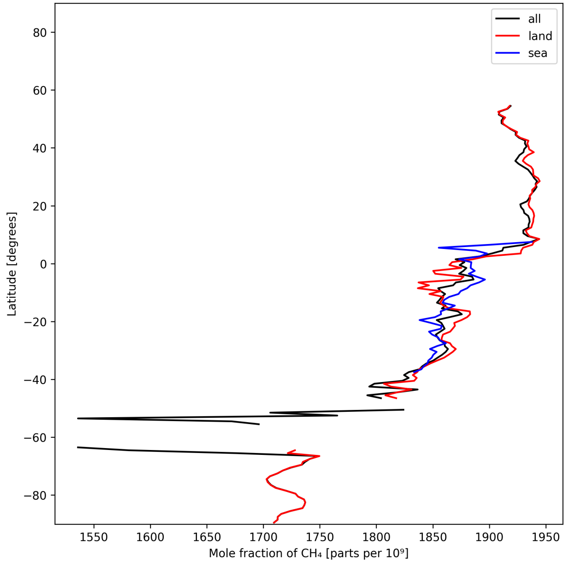
Figure 12: Zonal average of “Mole fraction of \text{CH}_4 ” for 2024-11-23 to 2024-11-25.
