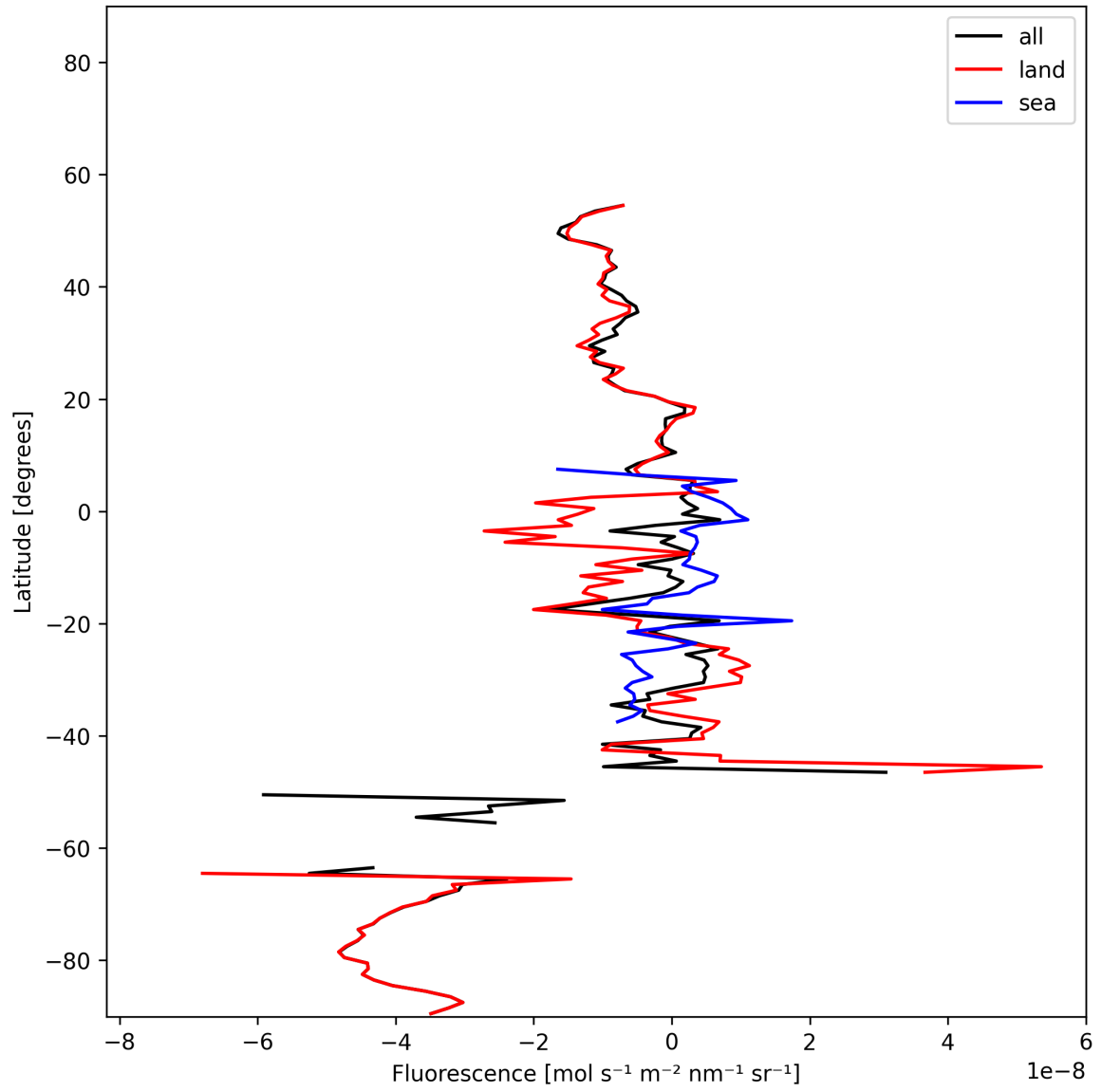
Figure 21: Zonal average of “Fluorescence” for 2024-11-23 to 2024-11-25.
