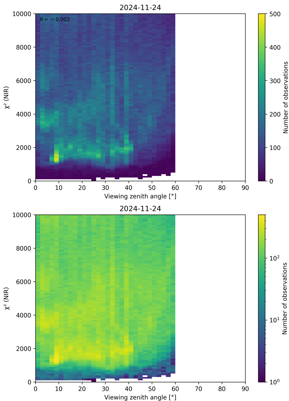
Figure 105: Scatter density plot of “Viewing zenith angle” against “ \chi^2 (NIR)” for 2024-11-23 to 2024-11-25.
