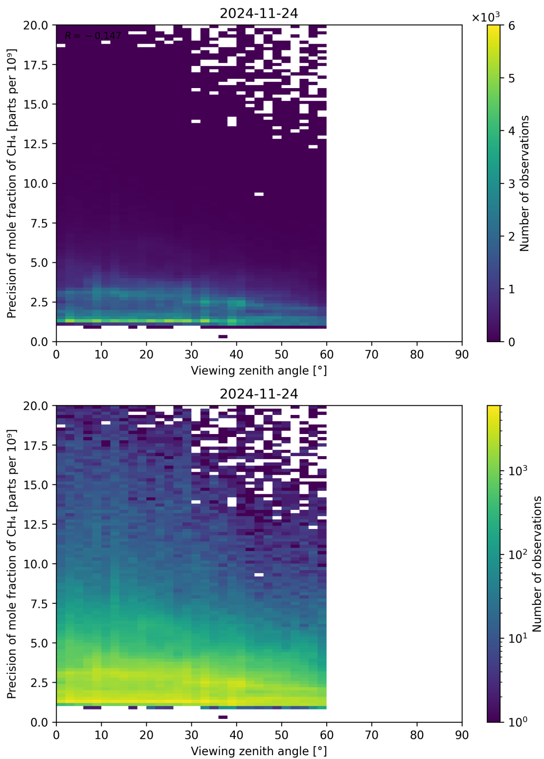
Figure 112: Scatter density plot of “Viewing zenith angle” against “Precision of mole fraction of \text{CH}_4 ” for 2024-11-23 to 2024-11-25.
