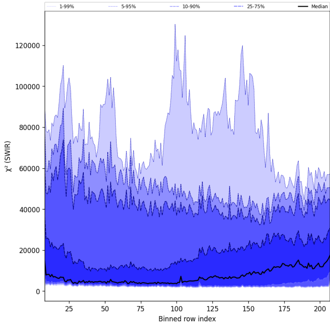
Figure 39: Along track statistics of “ \chi^2 (SWIR)” for 2024-11-23 to 2024-11-25
