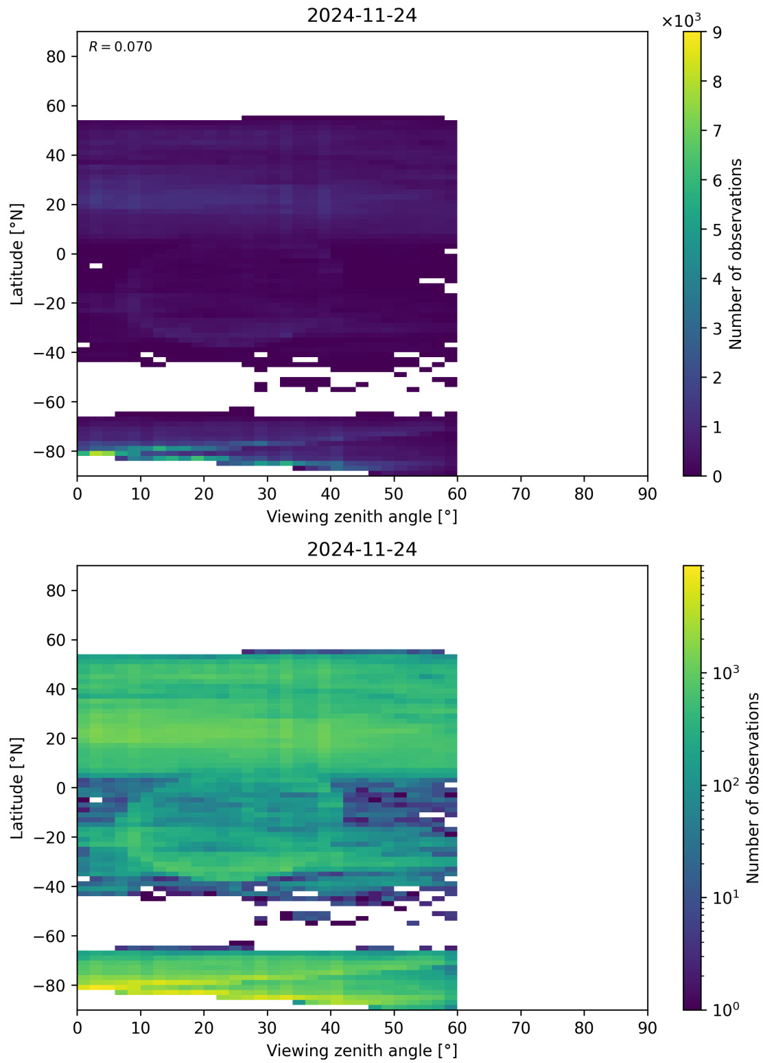
Figure 109: Scatter density plot of “Viewing zenith angle” against “Latitude” for 2024-11-23 to 2024-11-25.
