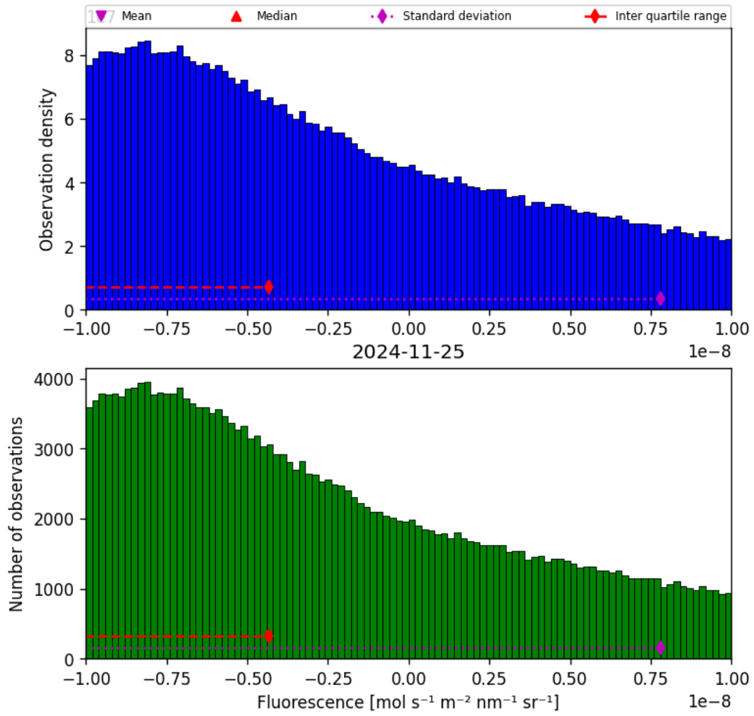
Figure 32: Histogram of “Fluorescence” for 2024-11-25 to 2024-11-26
