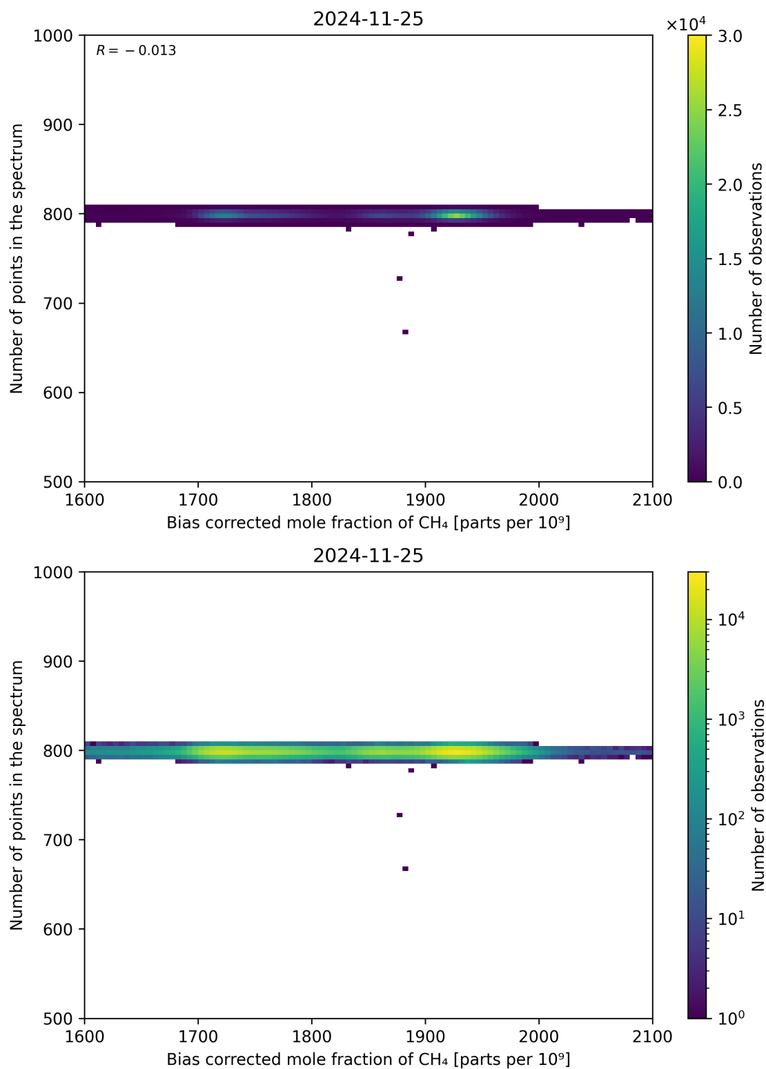
Figure 68: Scatter density plot of “Bias corrected mole fraction of \text{CH}_4 ” against “Number of points in the spectrum” for 2024-11-25 to 2024-11-26.
