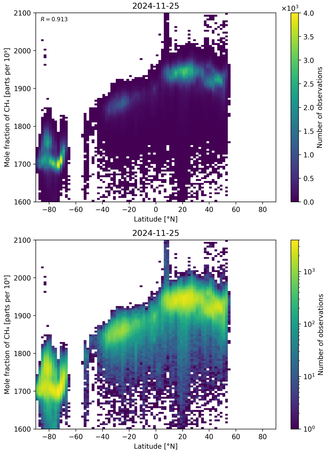
Figure 57: Scatter density plot of “Latitude” against “Mole fraction of CH 4 ” for 2024-11-25 to 2024-11-26.
