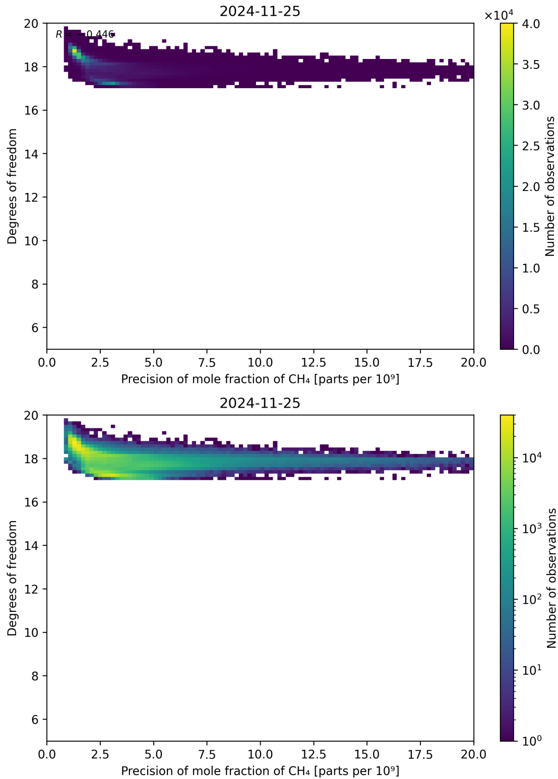
Figure 80: Scatter density plot of “Precision of mole fraction of CH 4 ” against “Degrees of freedom” for 2024-11-25 to 2024-11-26.
