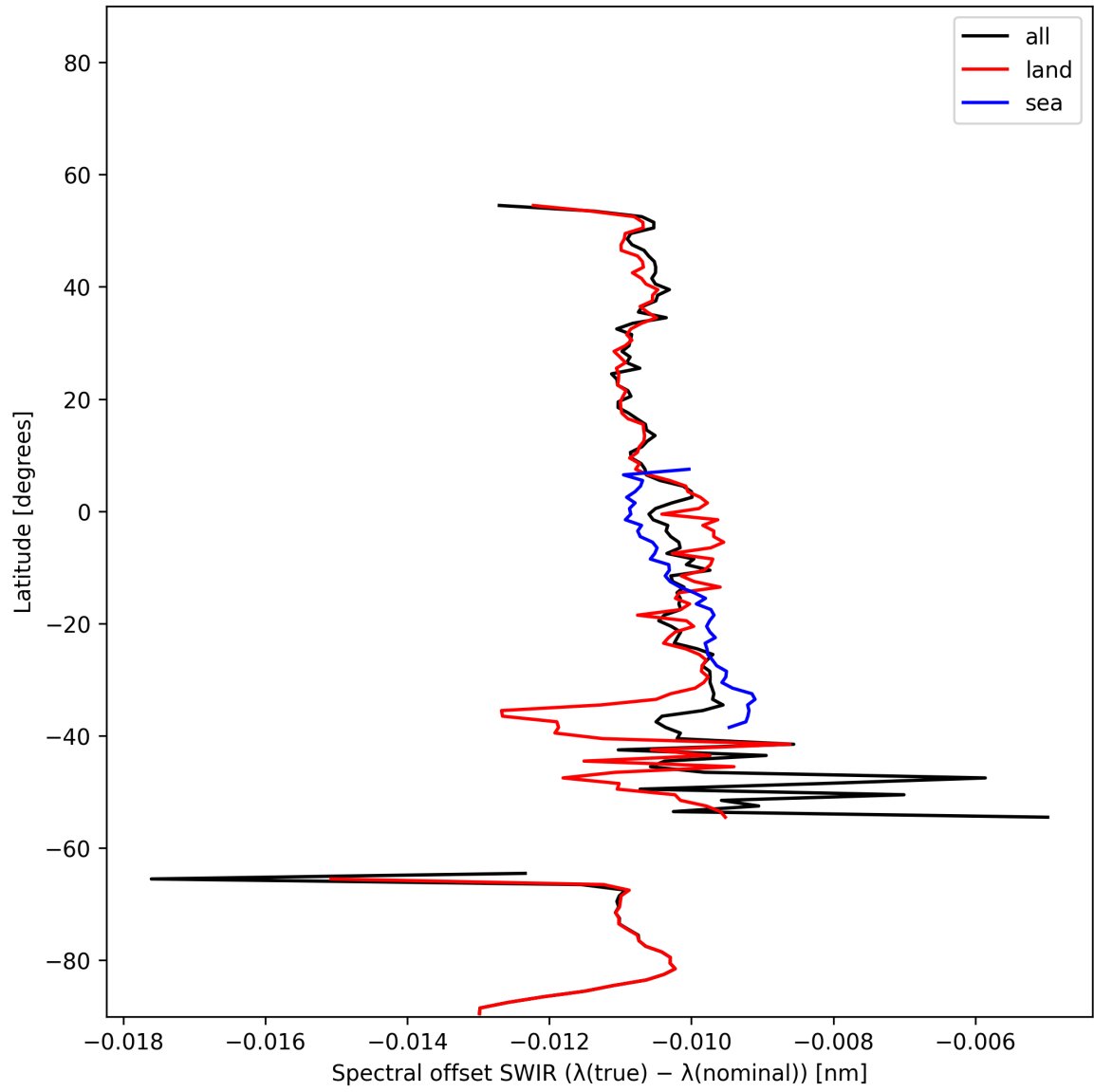
Figure 16: Zonal average of “Spectral offset SWIR ( \lambda_{\text{true}} - \lambda_{\text{nominal}} )” for 2024-11-25 to 2024-11-26.
