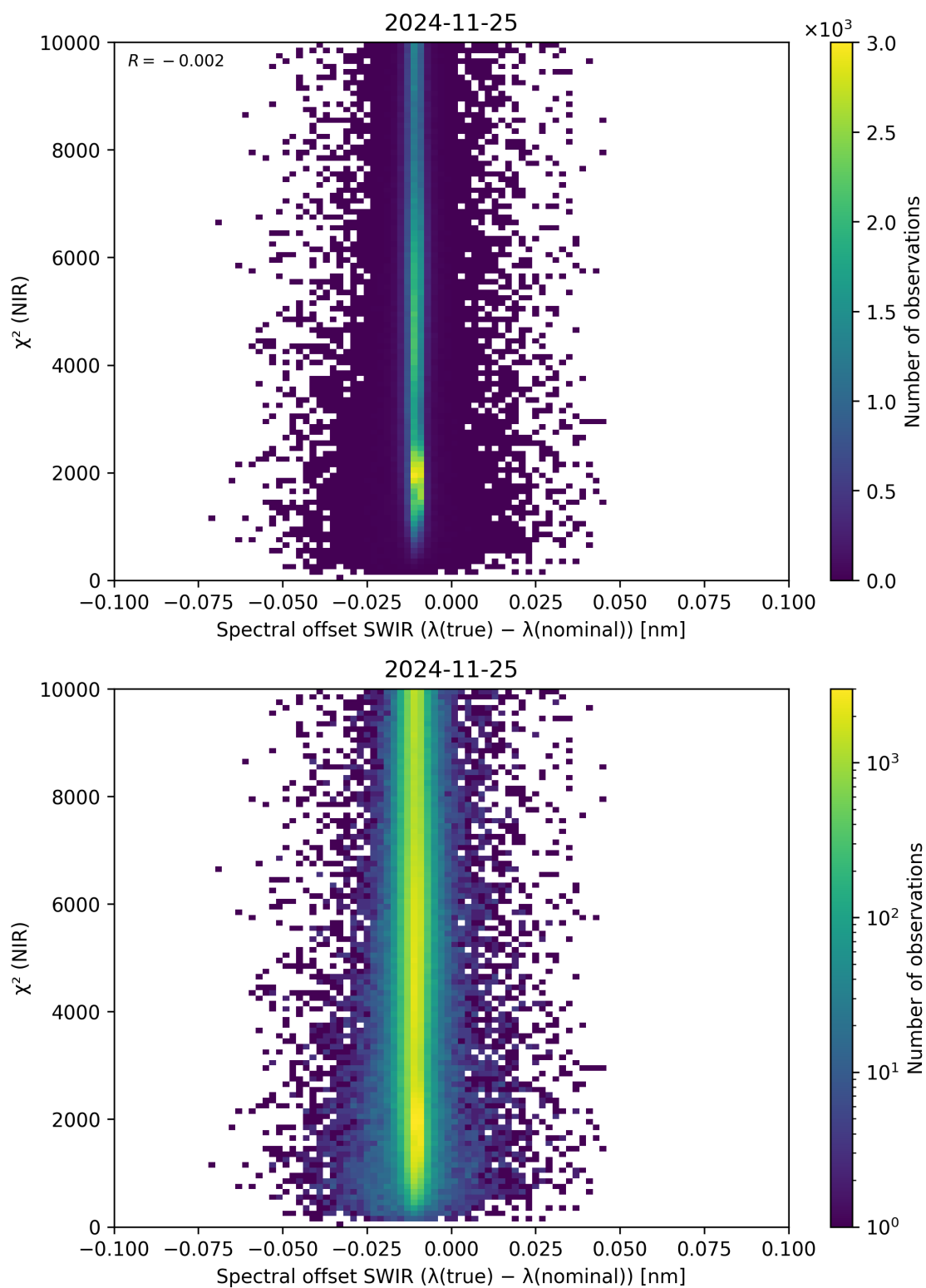
Figure 117: Scatter density plot of “Spectral offset SWIR ( \lambda_{\text{true}} - \lambda_{\text{nominal}} )” against “ \chi^2 (NIR)” for 2024-11-25 to 2024-11-26.
