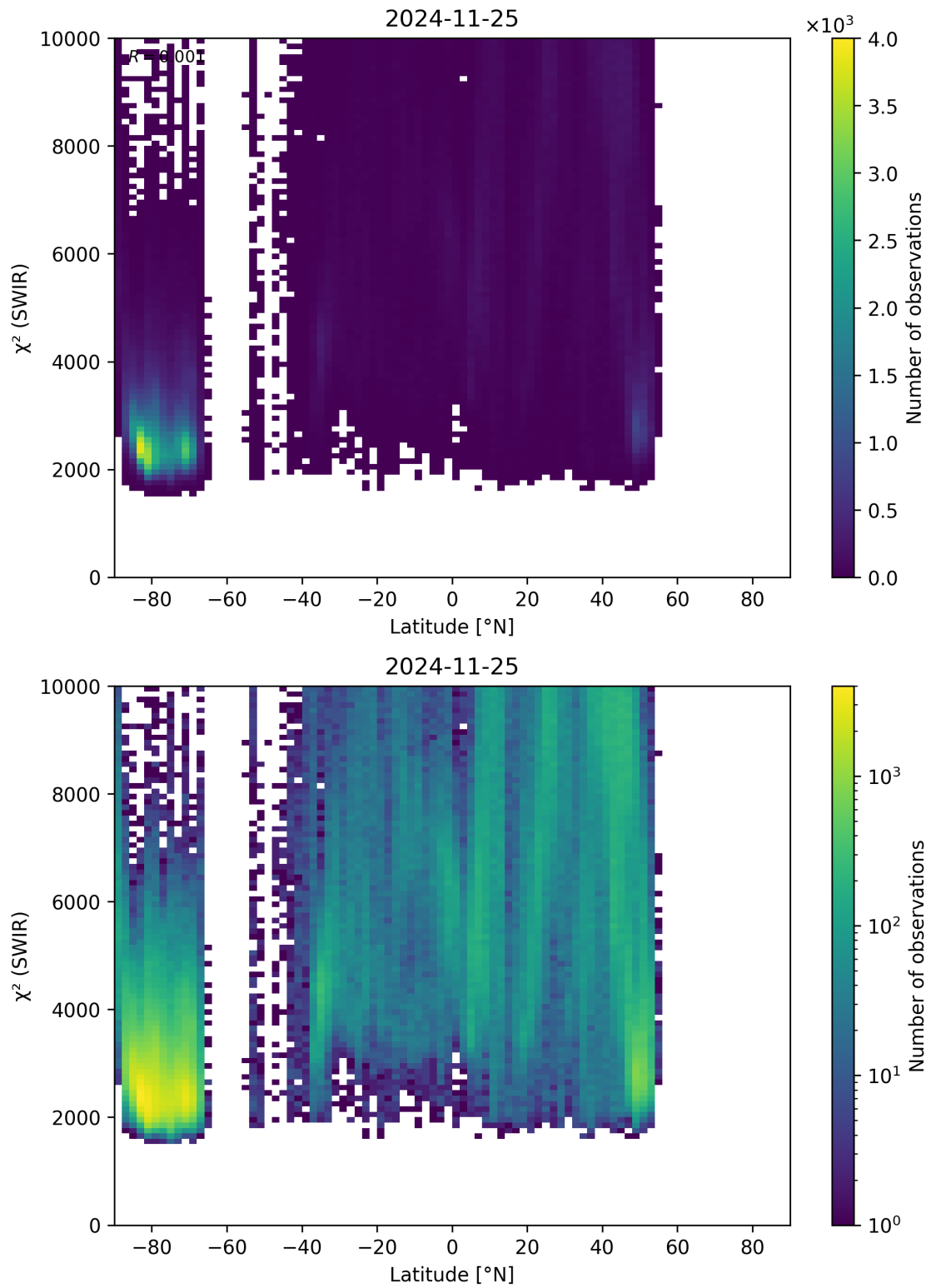
Figure 54: Scatter density plot of “Latitude” against “ \chi^2 (SWIR)” for 2024-11-25 to 2024-11-26.
