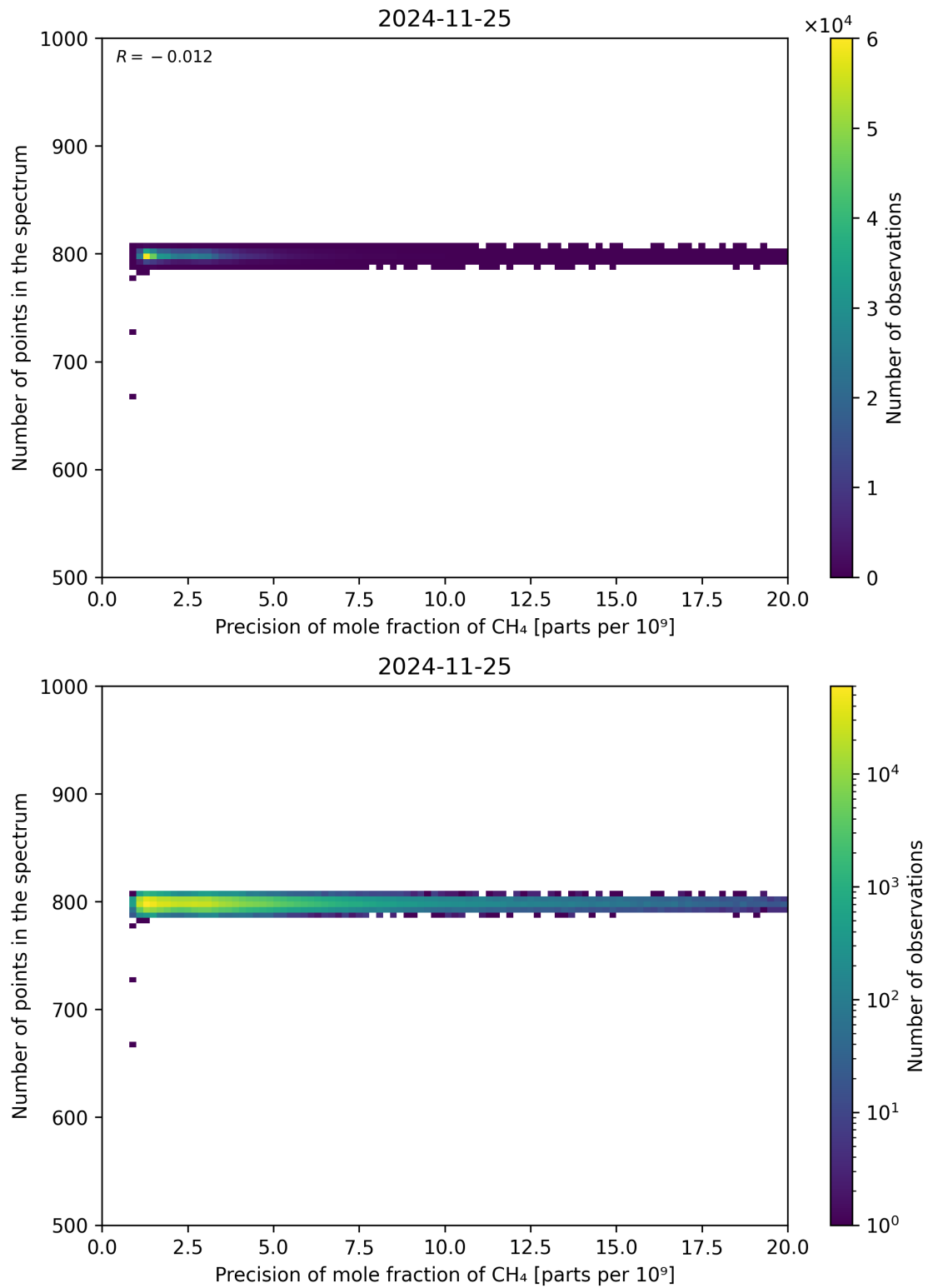
Figure 84: Scatter density plot of “Precision of mole fraction of CH 4 ” against “Number of points in the spectrum” for 2024-11-25 to 2024-11-26.
