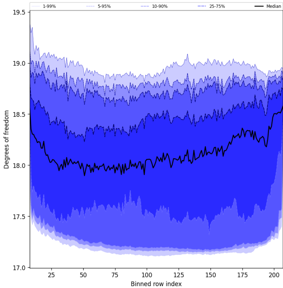
Figure 41: Along track statistics of “Degrees of freedom” for 2024-11-25 to 2024-11-26
