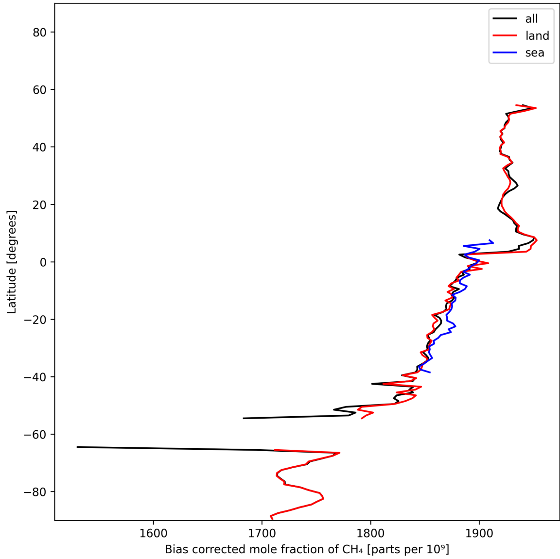
Figure 14: Zonal average of “Bias corrected mole fraction of CH 4 ” for 2024-11-25 to 2024-11-26.
