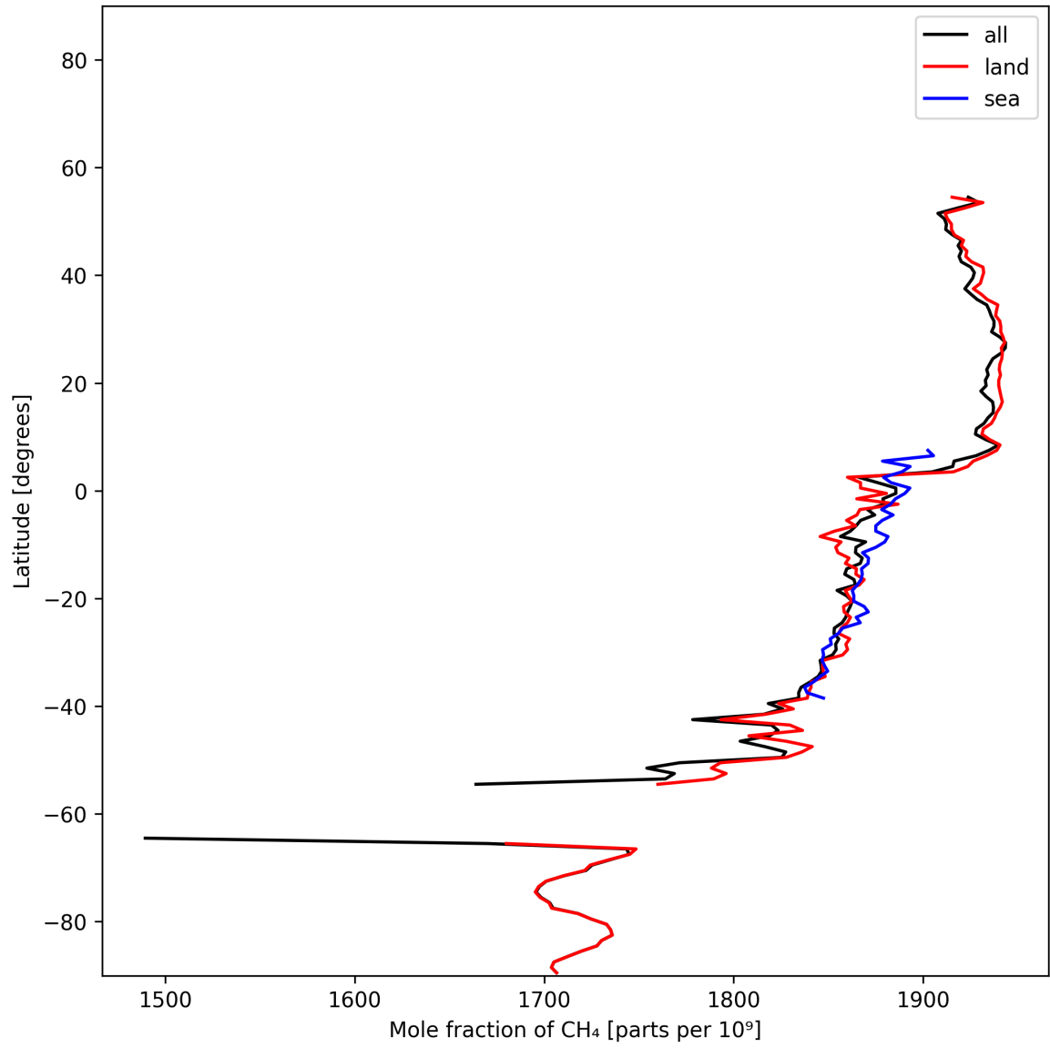
Figure 12: Zonal average of “Mole fraction of \text{CH}_4 ” for 2024-11-25 to 2024-11-26.
