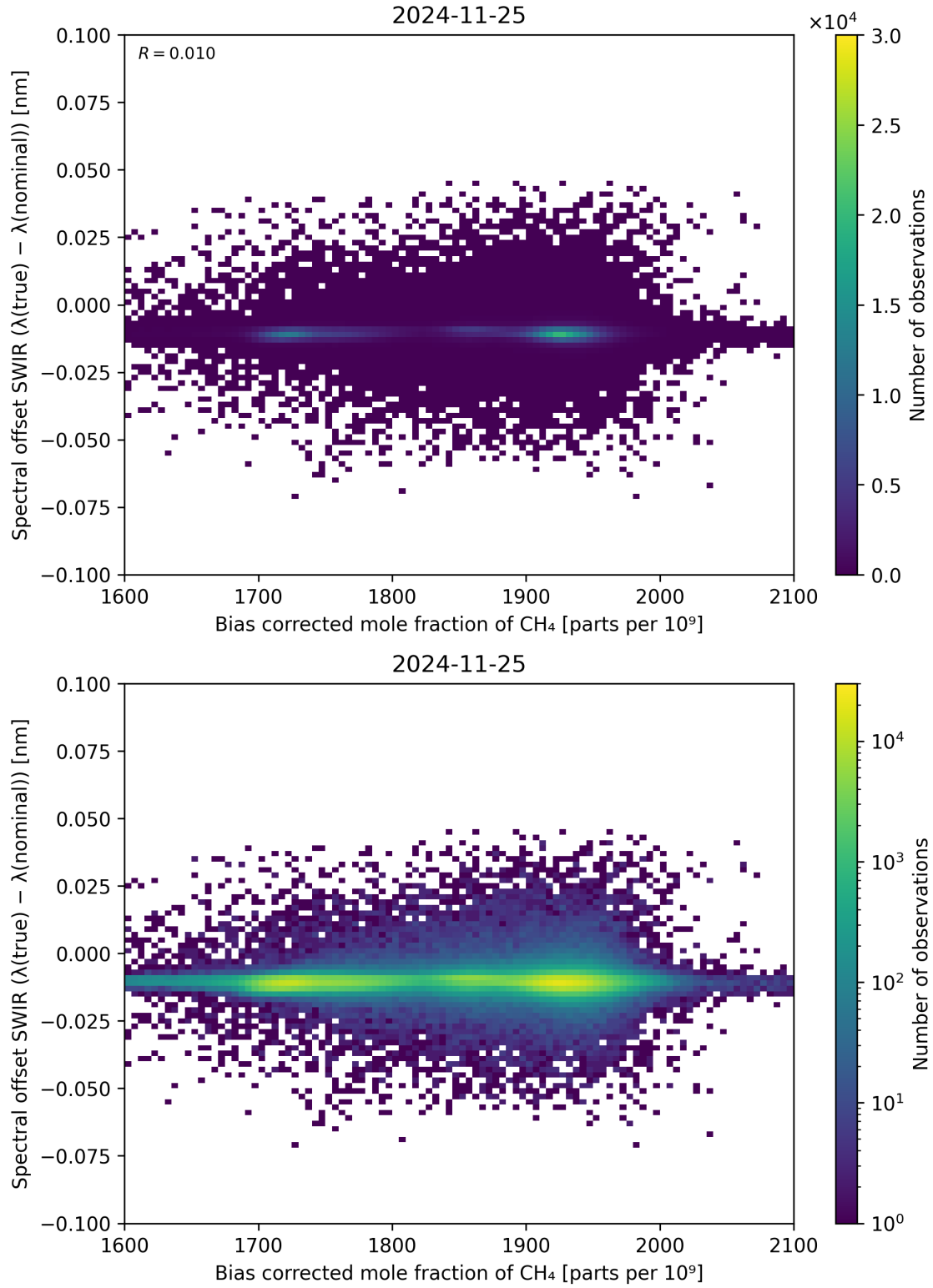
Figure 69: Scatter density plot of “Bias corrected mole fraction of \text{CH}_4 ” against “Spectral offset SWIR ( \lambda_{\text{true}} - \lambda_{\text{nominal}} )” for 2024-11-25 to 2024-11-26.
