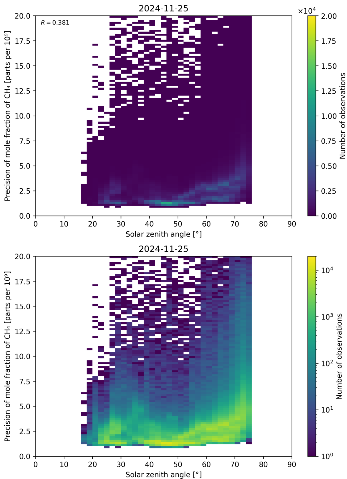
Figure 101: Scatter density plot of “Solar zenith angle” against “Precision of mole fraction of CH 4 ” for 2024-11-25 to 2024-11-26.
