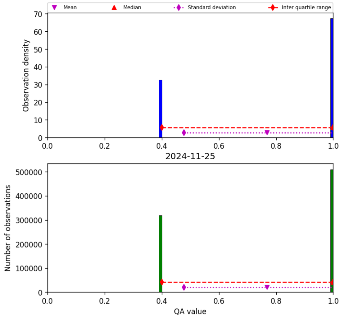
Figure 22: Histogram of “QA value” for 2024-11-25 to 2024-11-26
