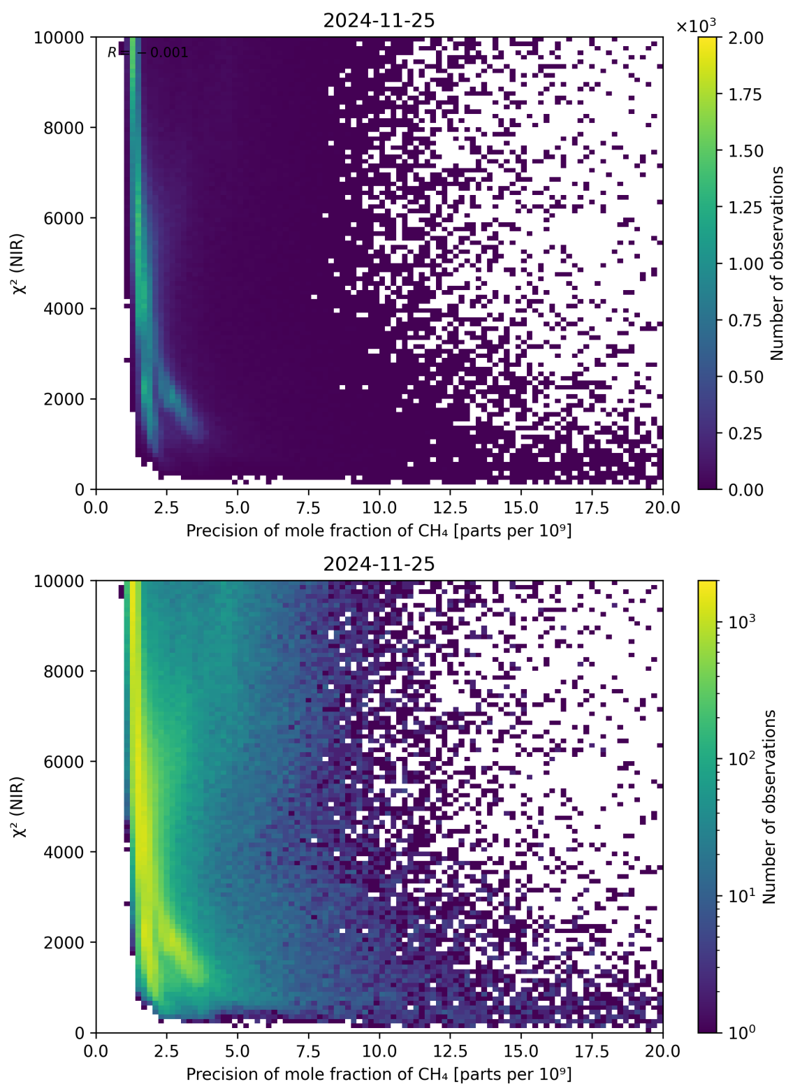
Figure 78: Scatter density plot of “Precision of mole fraction of CH 4 ” against “ \chi^2 (NIR)” for 2024-11-25 to 2024-11-26.
