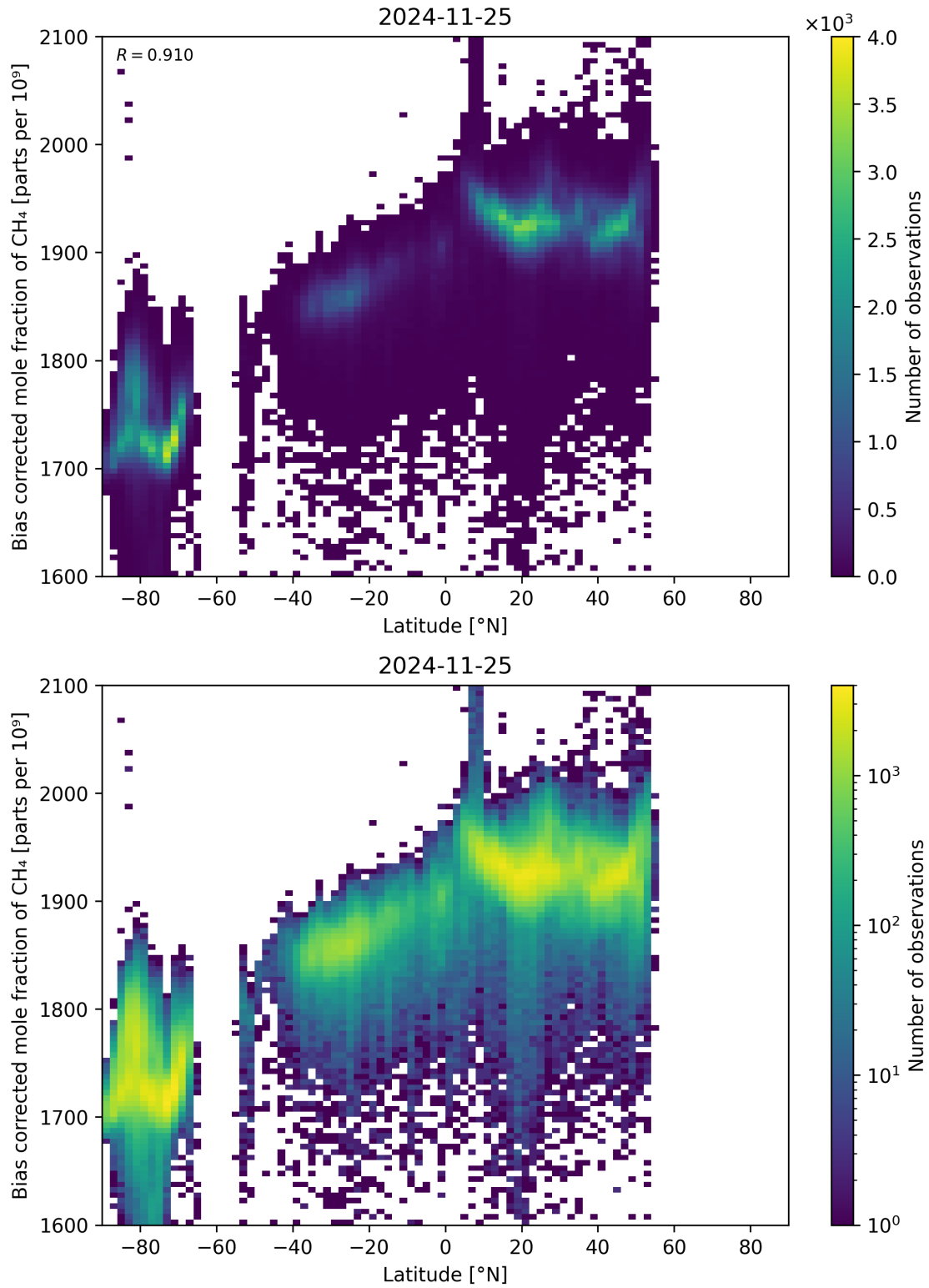
Figure 58: Scatter density plot of “Latitude” against “Bias corrected mole fraction of CH 4 ” for 2024-11-25 to 2024-11-26.
