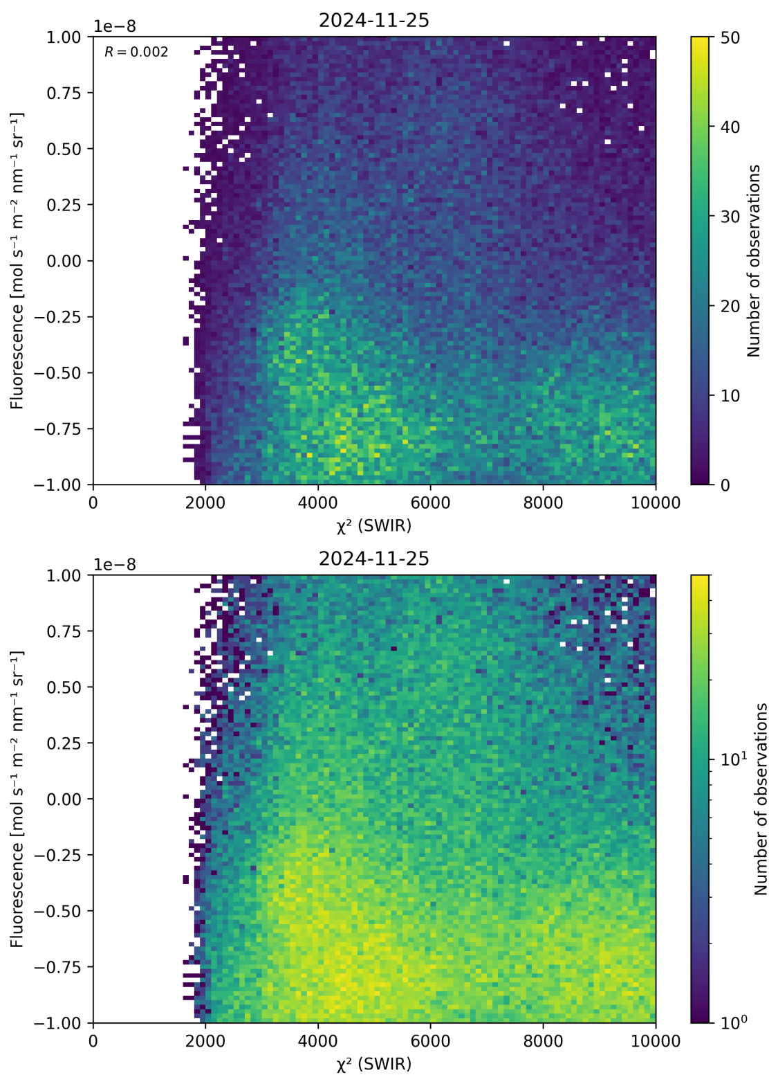
Figure 49: Scatter density plot of “ \chi^2 (SWIR)” against “Fluorescence” for 2024-11-25 to 2024-11-26.
