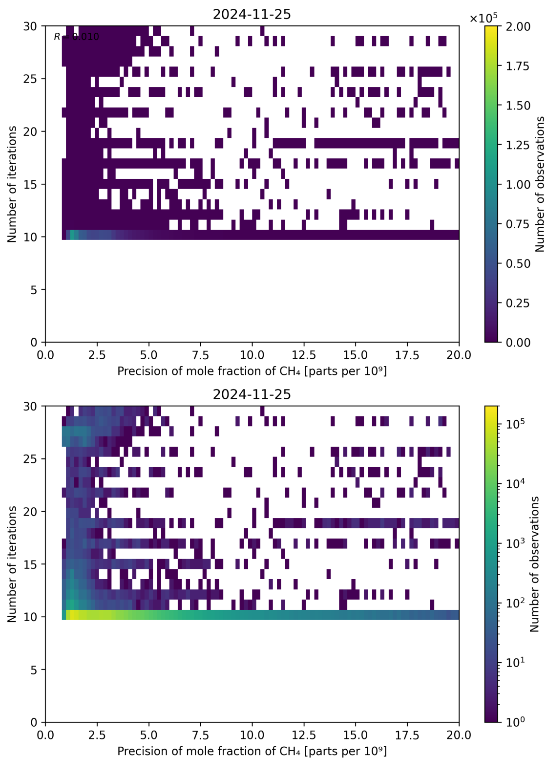
Figure 83: Scatter density plot of “Precision of mole fraction of CH 4 ” against “Number of iterations” for 2024-11-25 to 2024-11-26.
