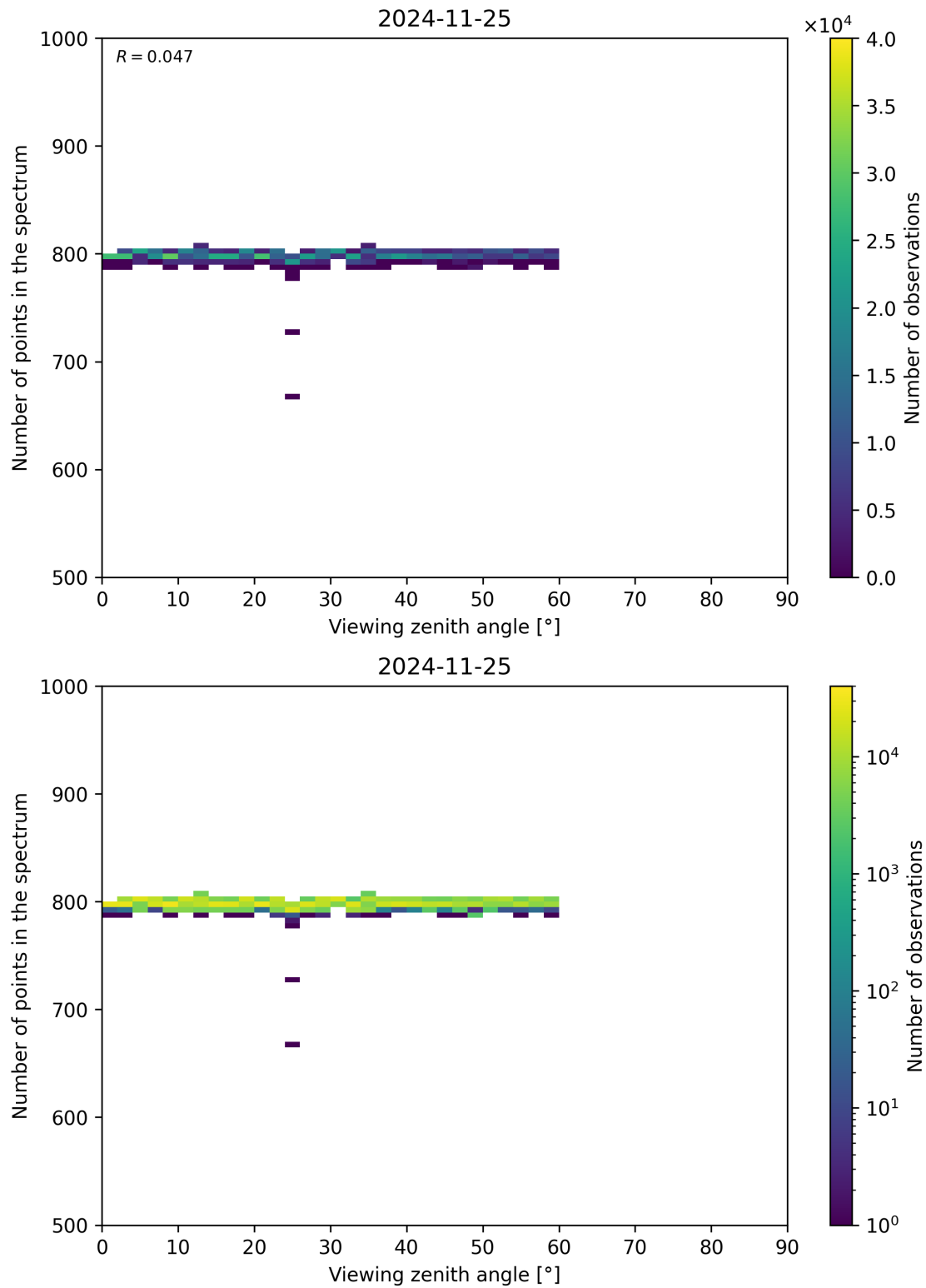
Figure 114: Scatter density plot of “Viewing zenith angle” against “Number of points in the spectrum” for 2024-11-25 to 2024-11-26.
