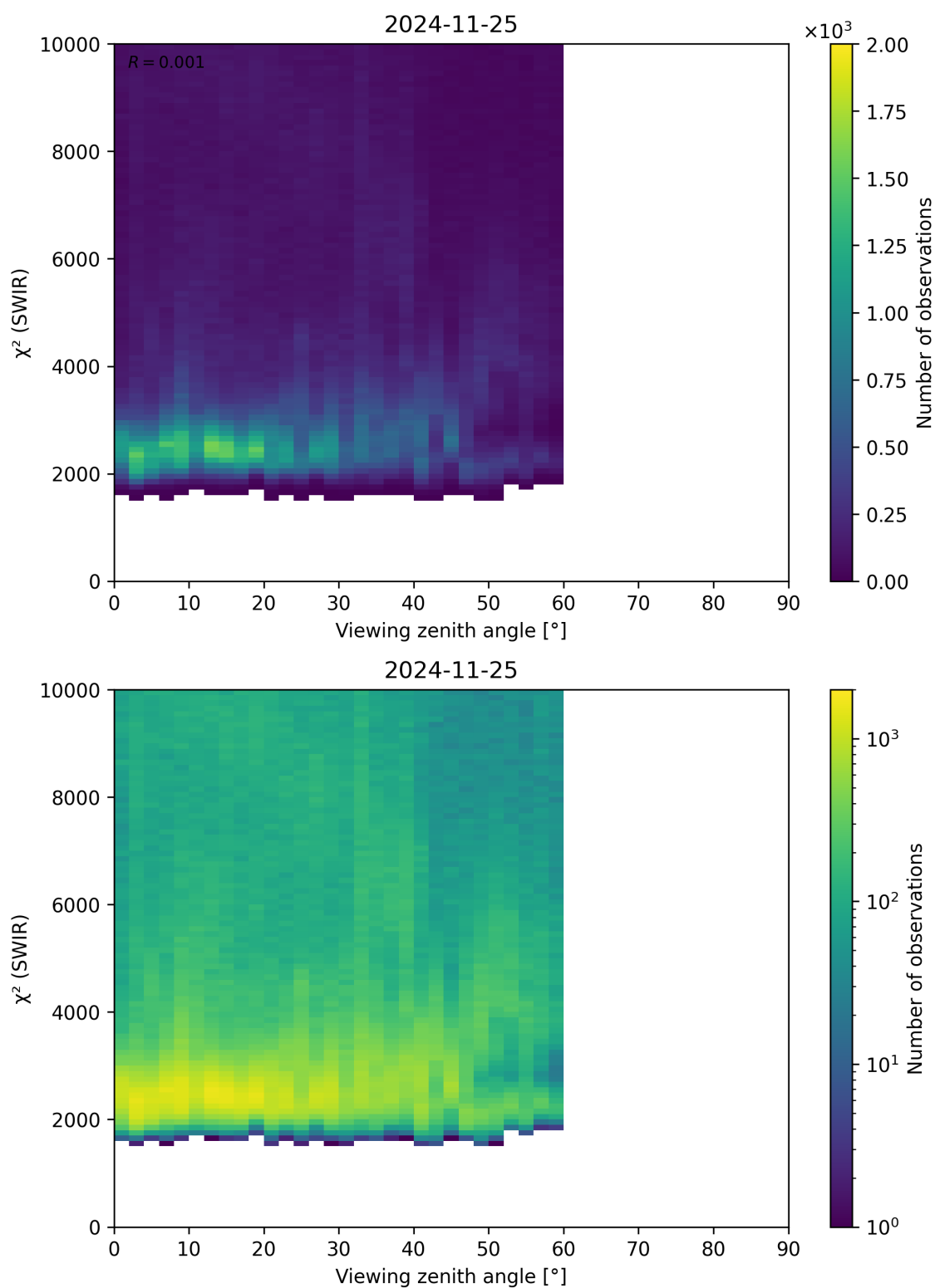
Figure 106: Scatter density plot of “Viewing zenith angle” against “ \chi^2 (SWIR)” for 2024-11-25 to 2024-11-26.
