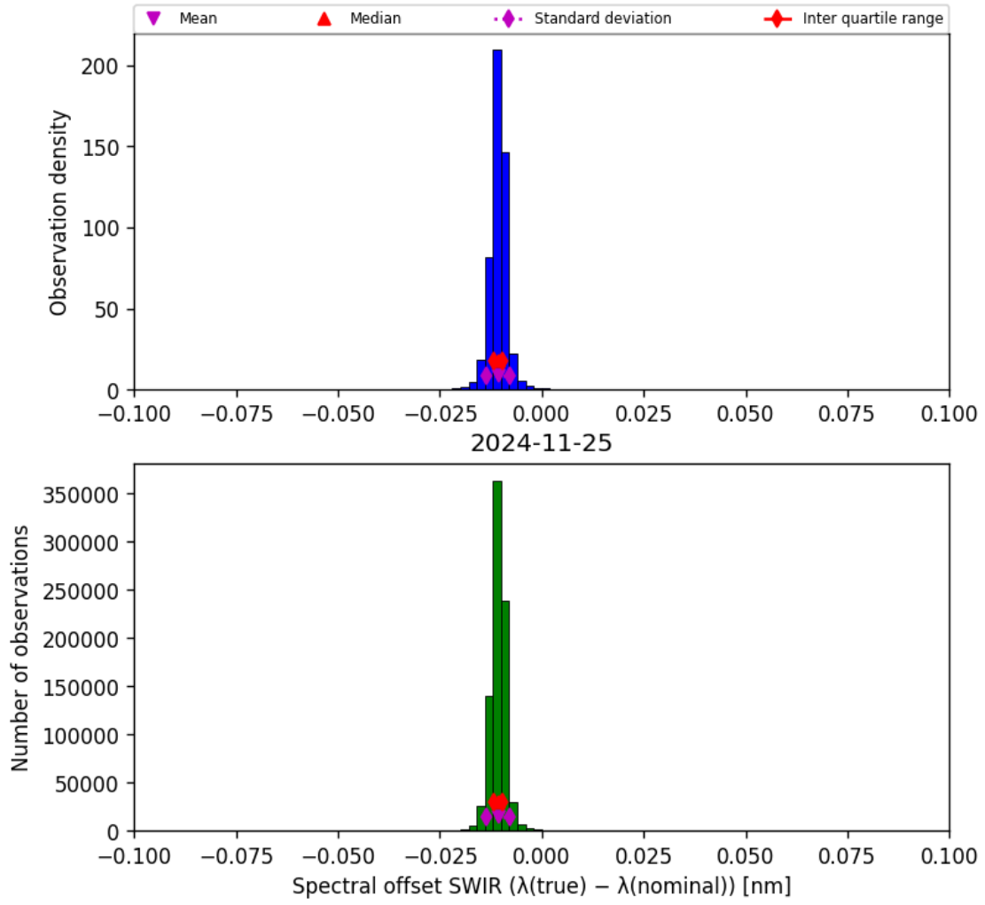
Figure 27: Histogram of “Spectral offset SWIR ( \lambda_{\text{true}} - \lambda_{\text{nominal}} )” for 2024-11-25 to 2024-11-26
