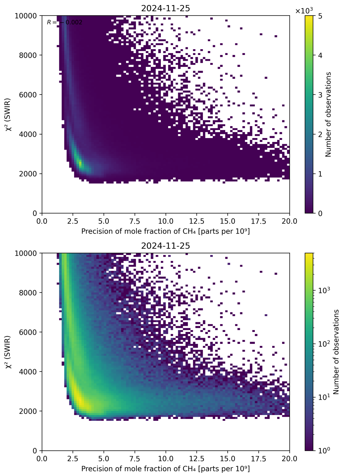
Figure 79: Scatter density plot of “Precision of mole fraction of \text{CH}_4 ” against “ \chi^2 (SWIR)” for 2024-11-25 to 2024-11-26.
