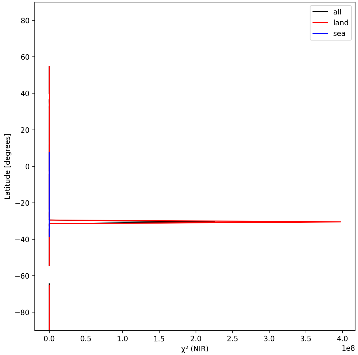
Figure 18: Zonal average of “ \chi^2 (NIR)” for 2024-11-25 to 2024-11-26.
