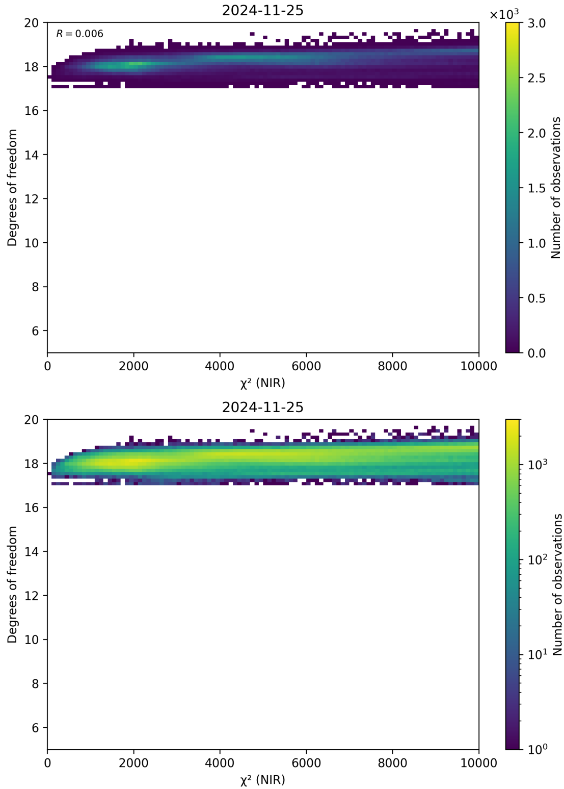
Figure 44: Scatter density plot of “ \chi^2 (NIR)” against “Degrees of freedom” for 2024-11-25 to 2024-11-26.
