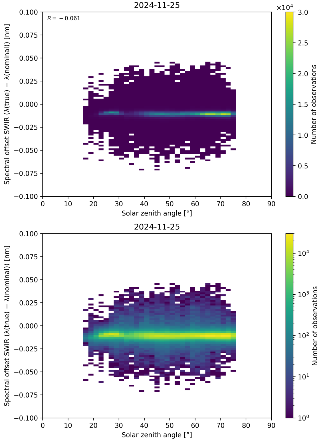
Figure 104: Scatter density plot of “Solar zenith angle” against “Spectral offset SWIR ( \lambda_{\text{true}} - \lambda_{\text{nominal}} )” for 2024-11-25 to 2024-11-26.
