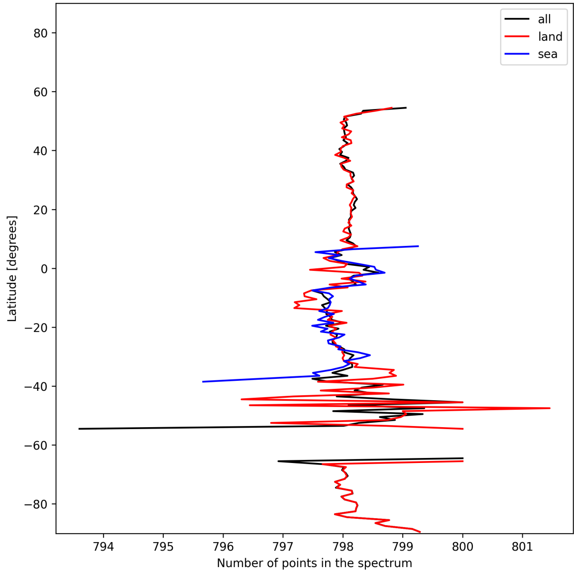
Figure 15: Zonal average of “Number of points in the spectrum” for 2024-11-25 to 2024-11-26.
