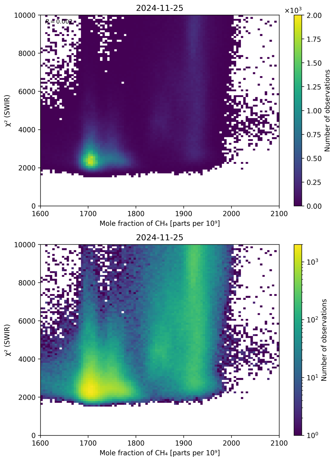
Figure 71: Scatter density plot of “Mole fraction of \text{CH}_4 ” against “ \chi^2 (SWIR)” for 2024-11-25 to 2024-11-26.
