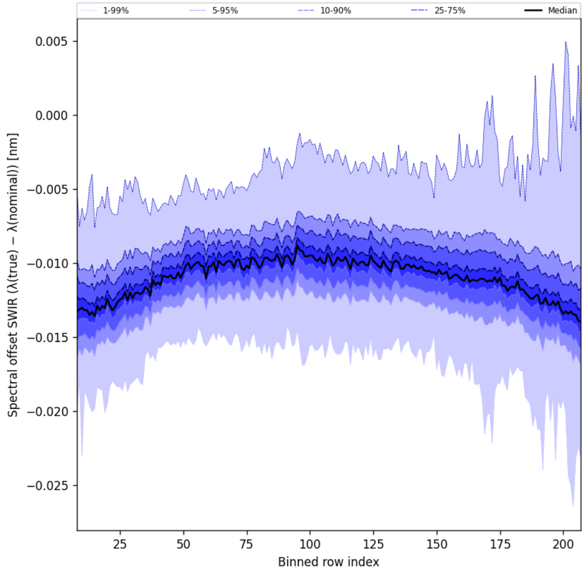
Figure 38: Along track statistics of “Spectral offset SWIR ( \lambda_{\text{true}} - \lambda_{\text{nominal}} )” for 2024-11-25 to 2024-11-26
