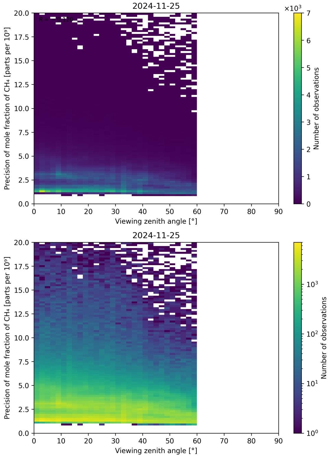
Figure 112: Scatter density plot of “Viewing zenith angle” against “Precision of mole fraction of \text{CH}_4 ” for 2024-11-25 to 2024-11-26.
