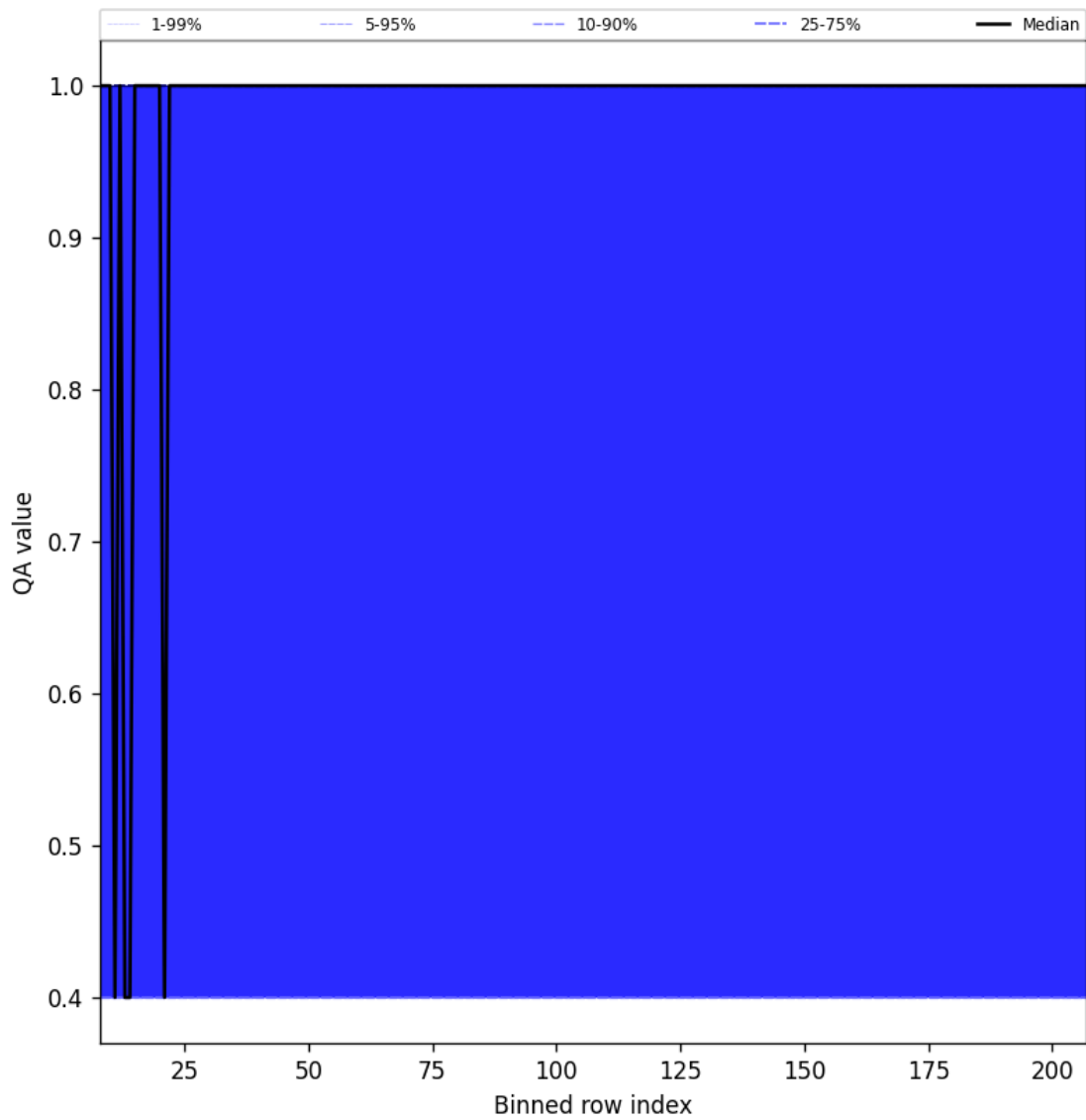
Figure 33: Along track statistics of “QA value” for 2024-11-25 to 2024-11-26
