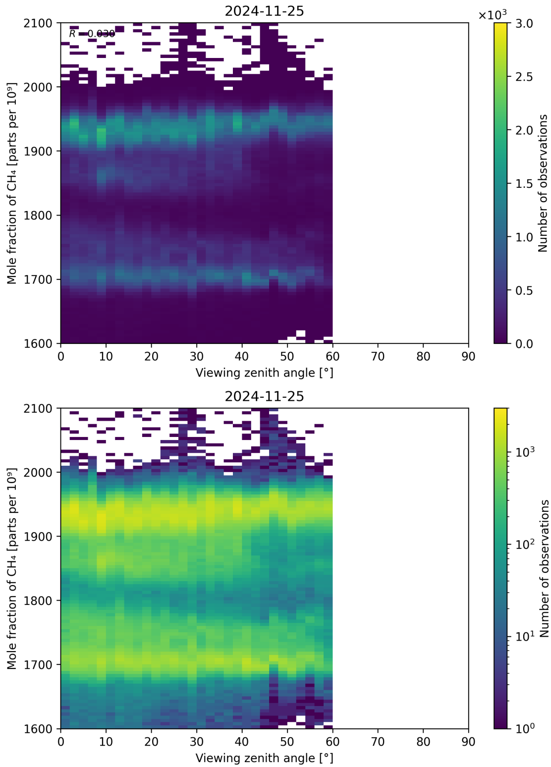
Figure 110: Scatter density plot of “Viewing zenith angle” against “Mole fraction of CH 4 ” for 2024-11-25 to 2024-11-26.
