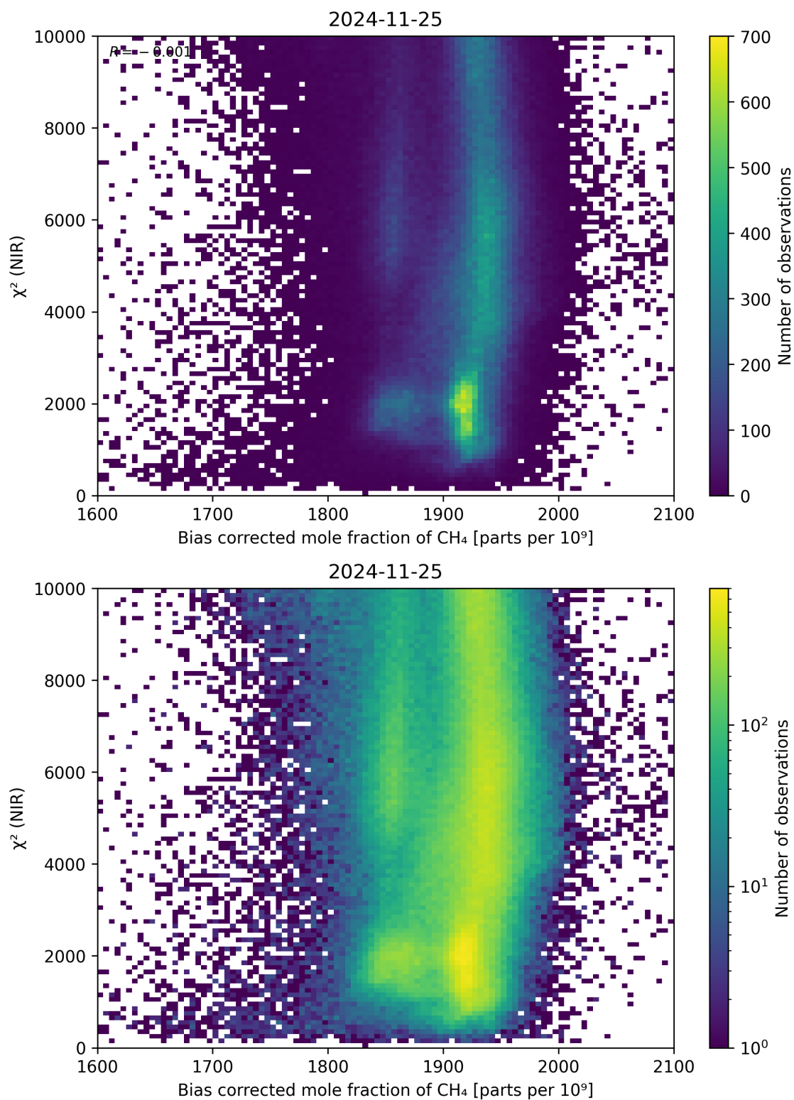
Figure 63: Scatter density plot of “Bias corrected mole fraction of \text{CH}_4 ” against “ \chi^2 (NIR)” for 2024-11-25 to 2024-11-26.
