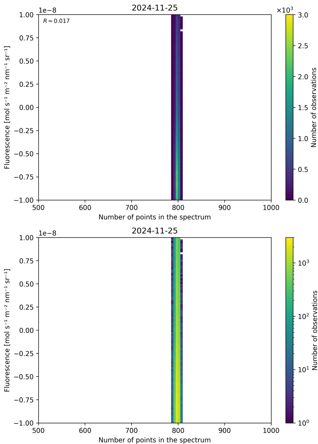
Figure 91: Scatter density plot of “Number of points in the spectrum” against “Fluorescence” for 2024-11-25 to 2024-11-26.
