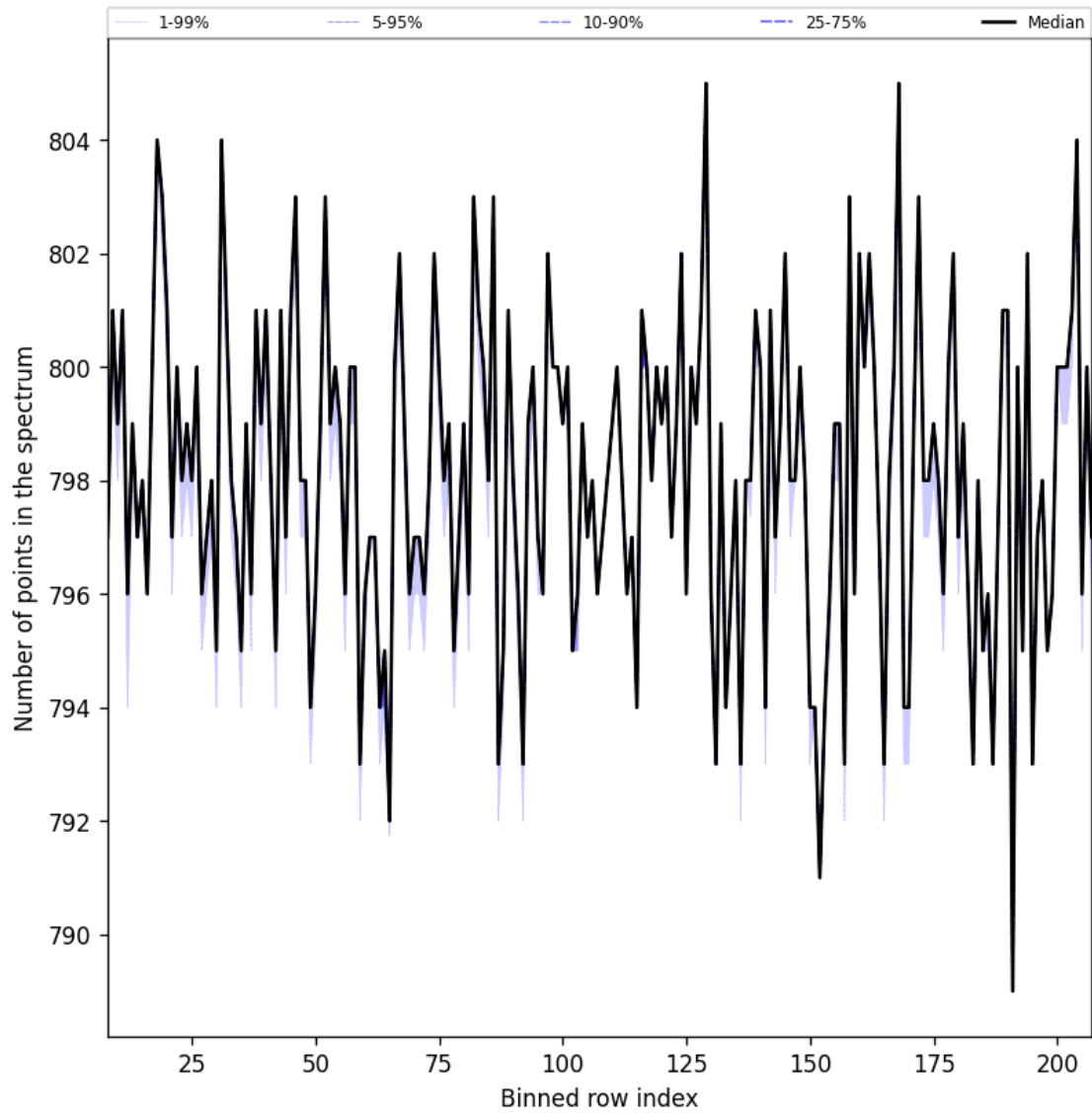
Figure 37: Along track statistics of “Number of points in the spectrum” for 2024-11-25 to 2024-11-26
