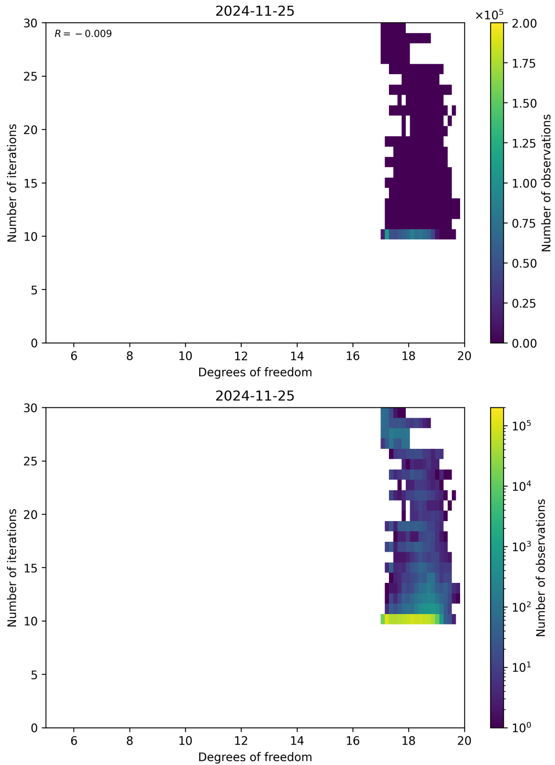
Figure 52: Scatter density plot of “Degrees of freedom” against “Number of iterations” for 2024-11-25 to 2024-11-26.
