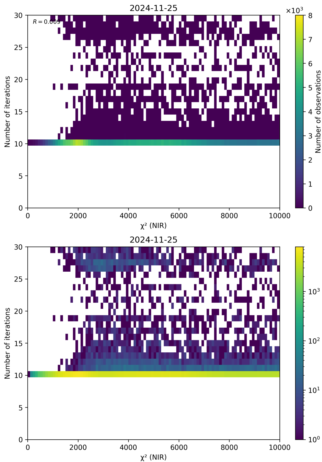
Figure 46: Scatter density plot of “ \chi^2 (NIR)” against “Number of iterations” for 2024-11-25 to 2024-11-26.
