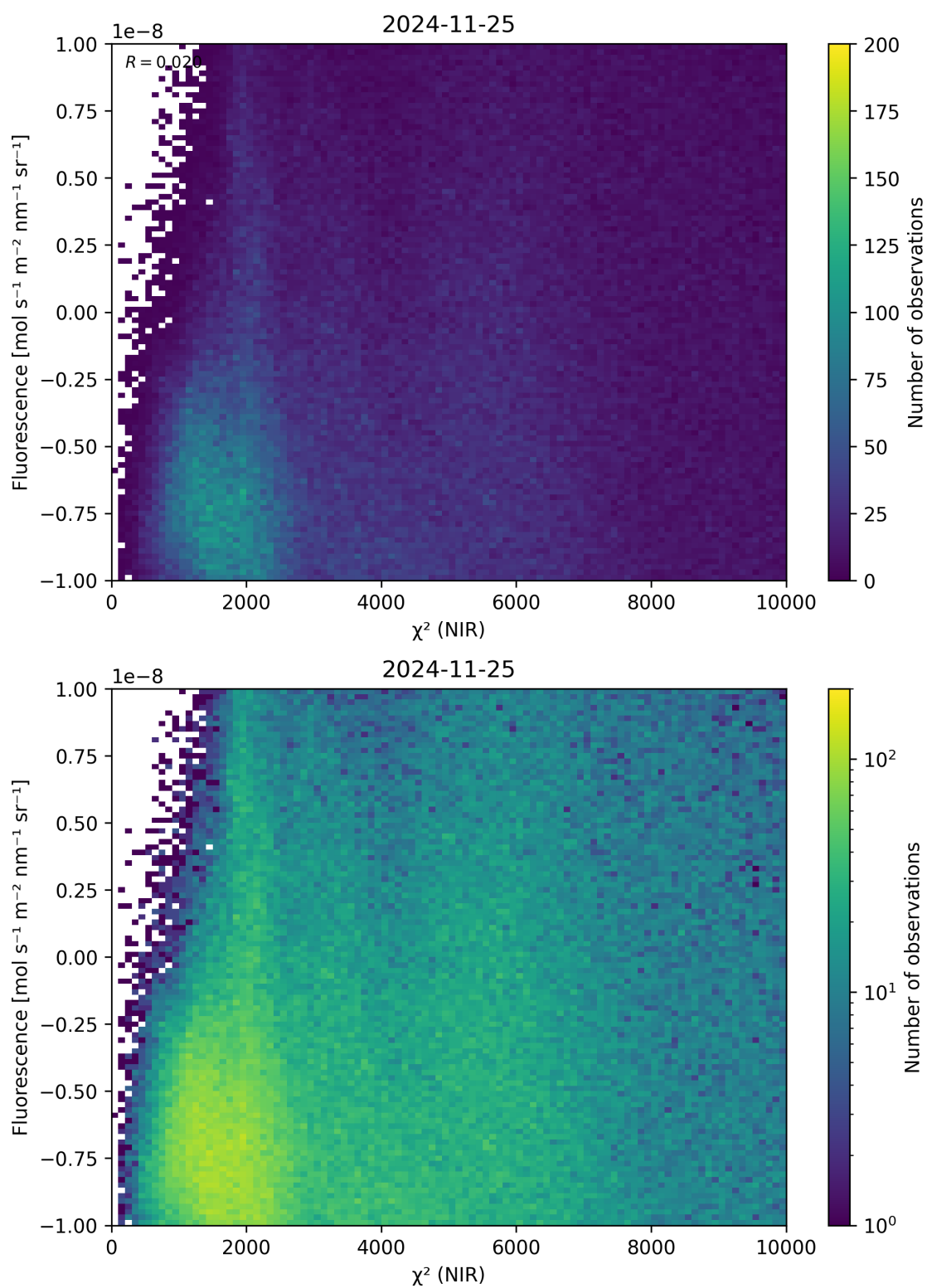
Figure 45: Scatter density plot of “ \chi^2 (NIR)” against “Fluorescence” for 2024-11-25 to 2024-11-26.
