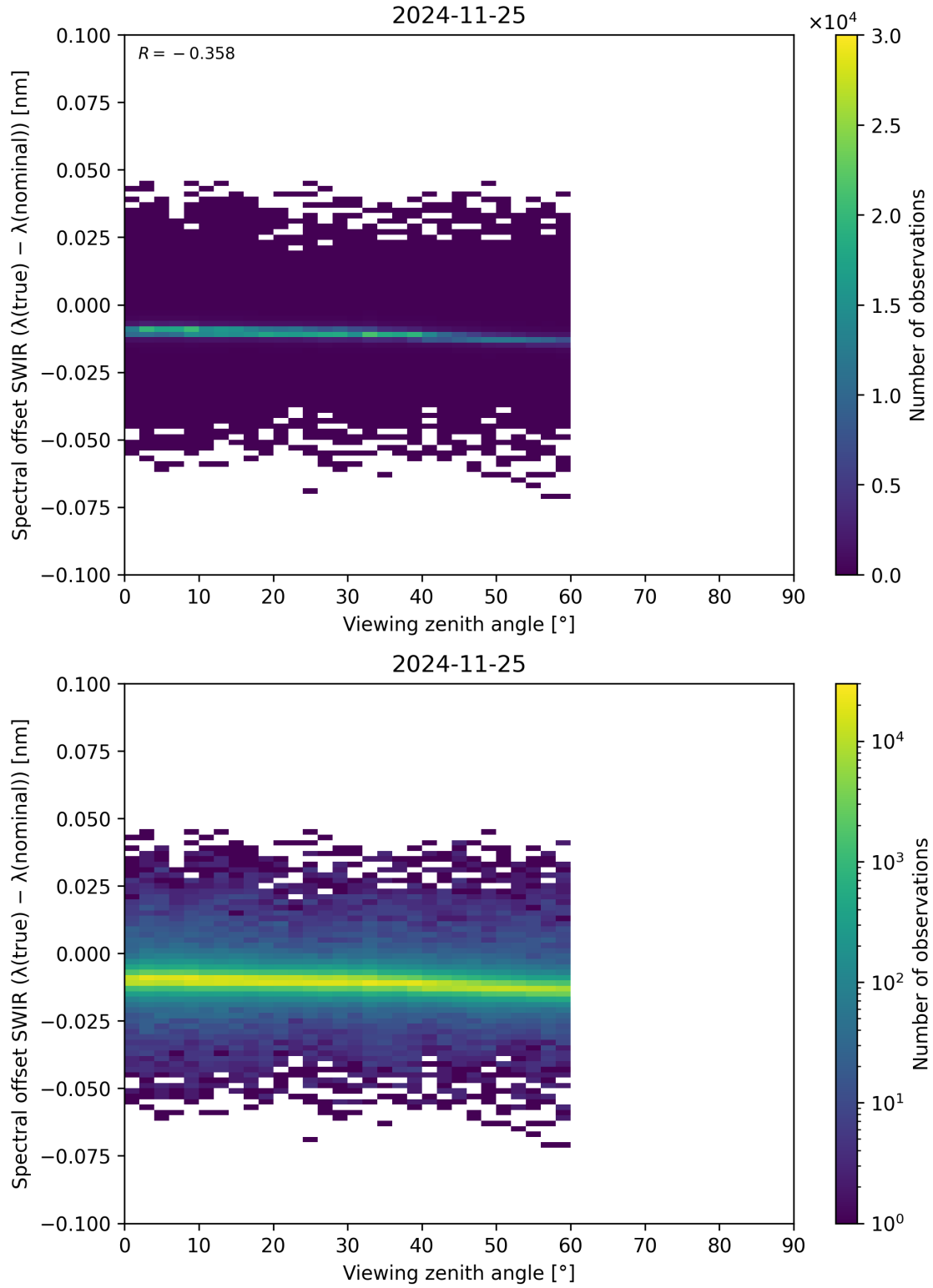
Figure 116: Scatter density plot of “Viewing zenith angle” against “Spectral offset SWIR ( \lambda_{\text{true}} - \lambda_{\text{nominal}} )” for 2024-11-25 to 2024-11-26.
