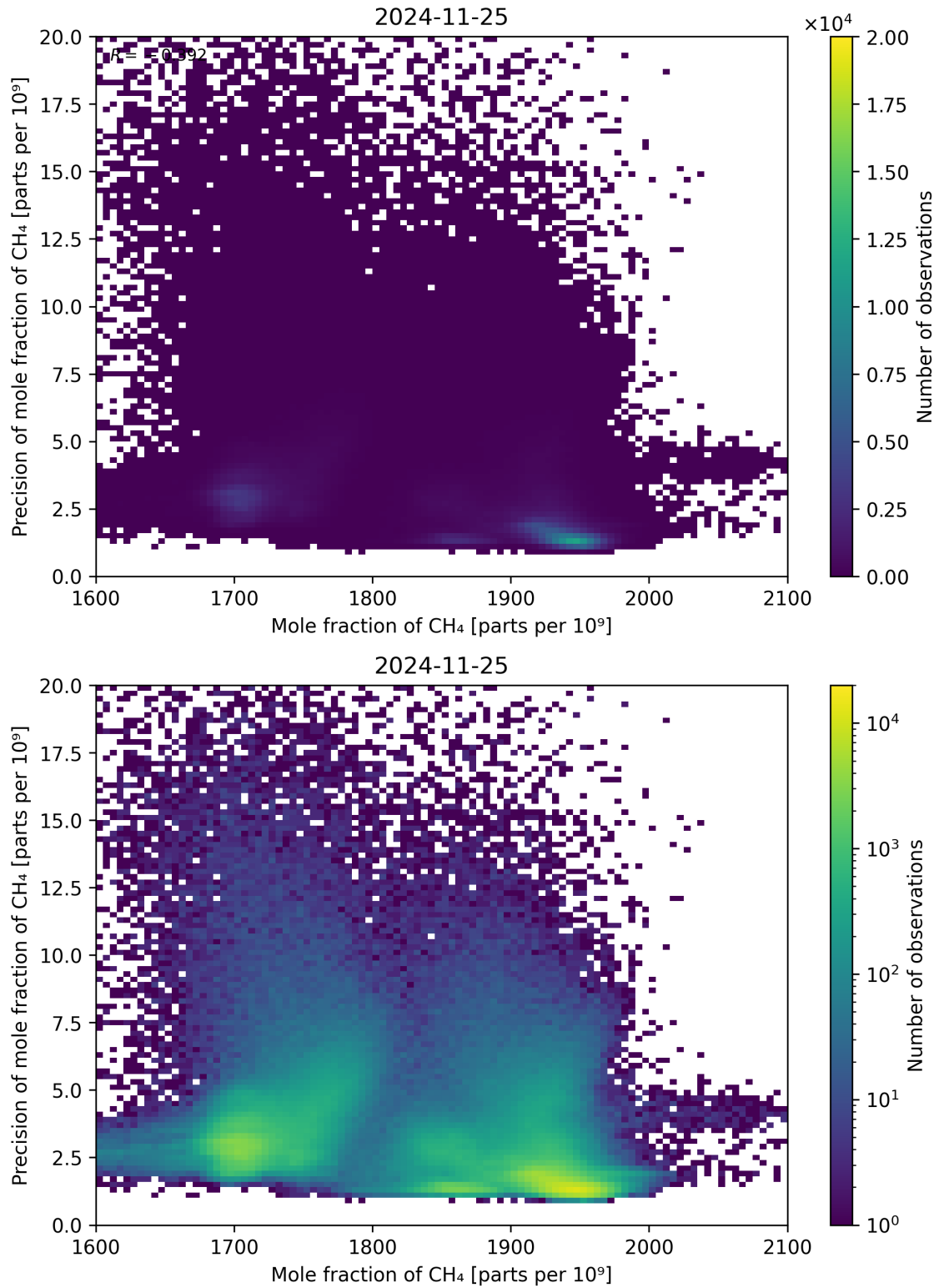
Figure 75: Scatter density plot of “Mole fraction of CH 4 ” against “Precision of mole fraction of CH 4 ” for 2024-11-25 to 2024-11-26.
