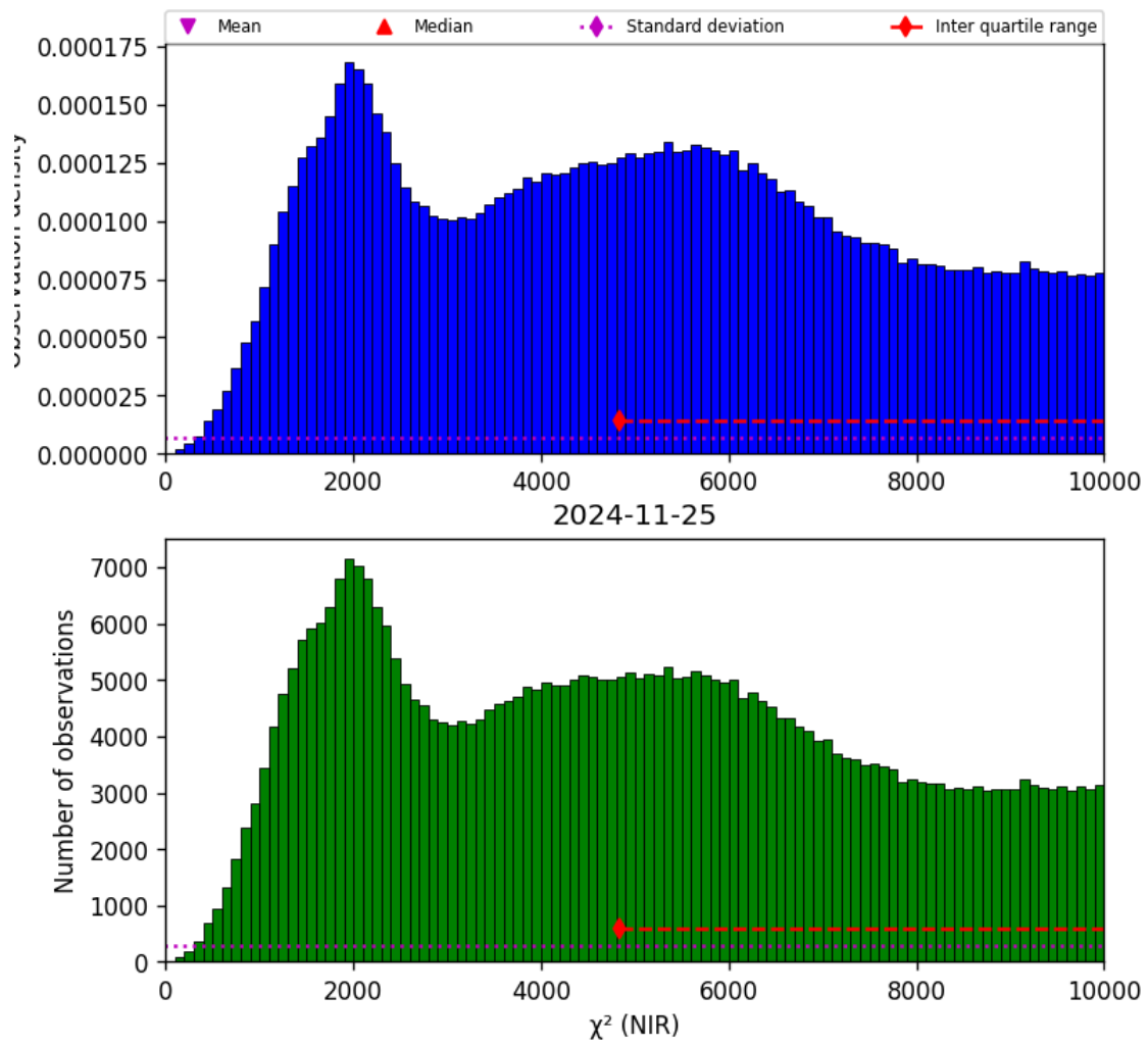
Figure 29: Histogram of “ \chi^2 (NIR)” for 2024-11-25 to 2024-11-26
