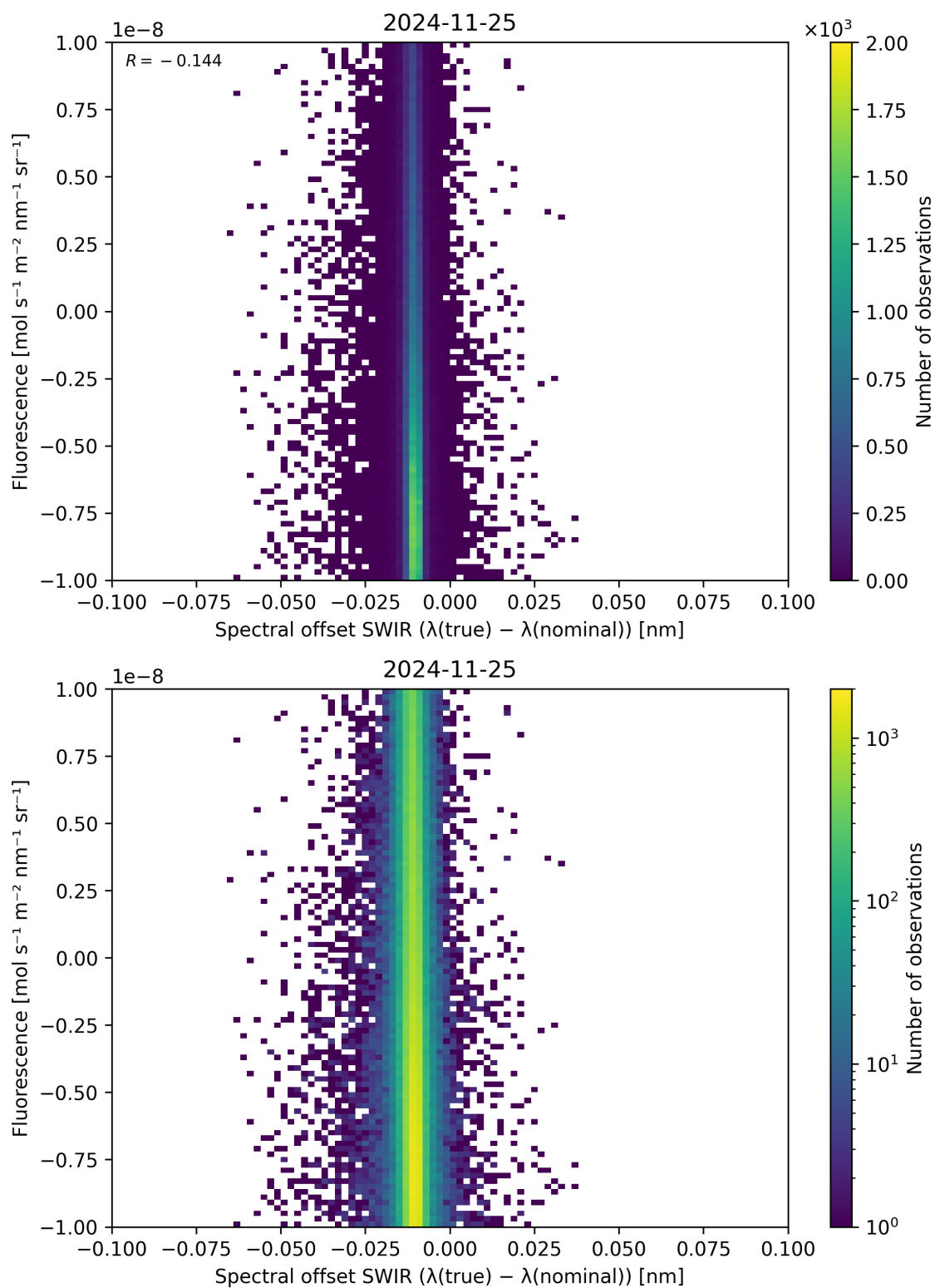
Figure 120: Scatter density plot of “Spectral offset SWIR ( \lambda_{\text{true}} - \lambda_{\text{nominal}} )” against “Fluorescence” for 2024-11-25 to 2024-11-26.
