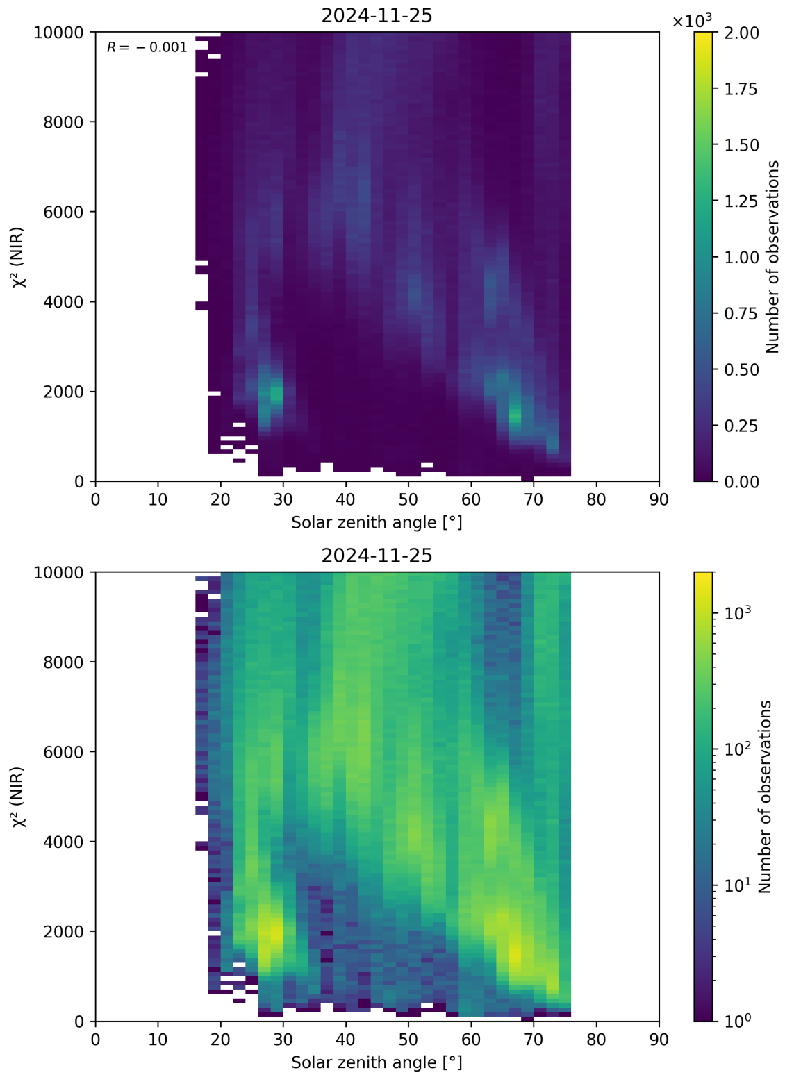
Figure 94: Scatter density plot of “Solar zenith angle” against “ \chi^2 (NIR)” for 2024-11-25 to 2024-11-26.
