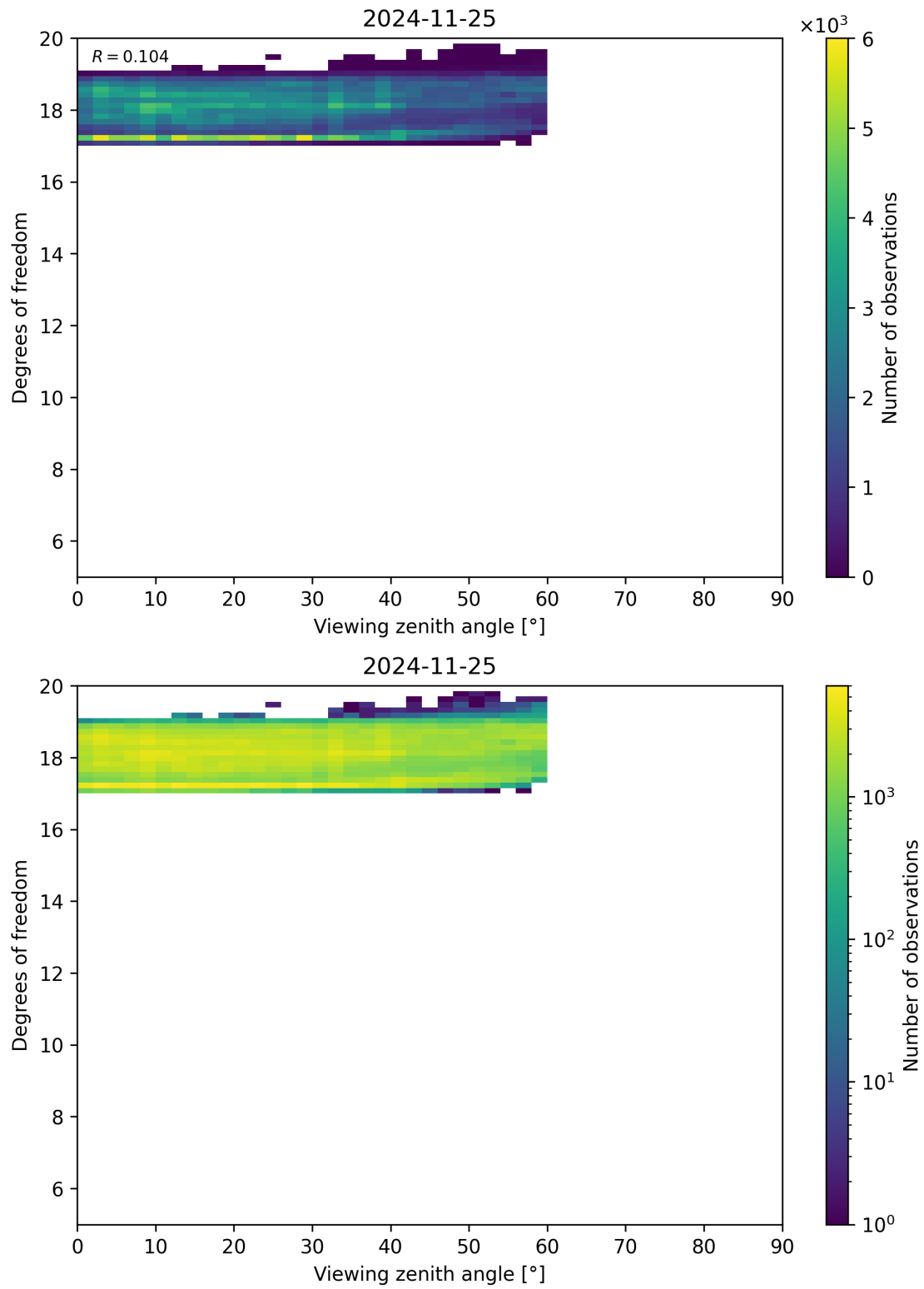
Figure 107: Scatter density plot of “Viewing zenith angle” against “Degrees of freedom” for 2024-11-25 to 2024-11-26.
