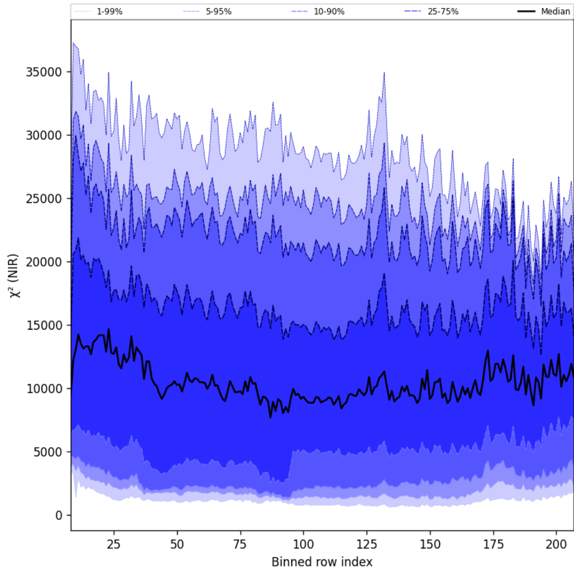
Figure 40: Along track statistics of “ \chi^2 (NIR)” for 2024-11-25 to 2024-11-26
