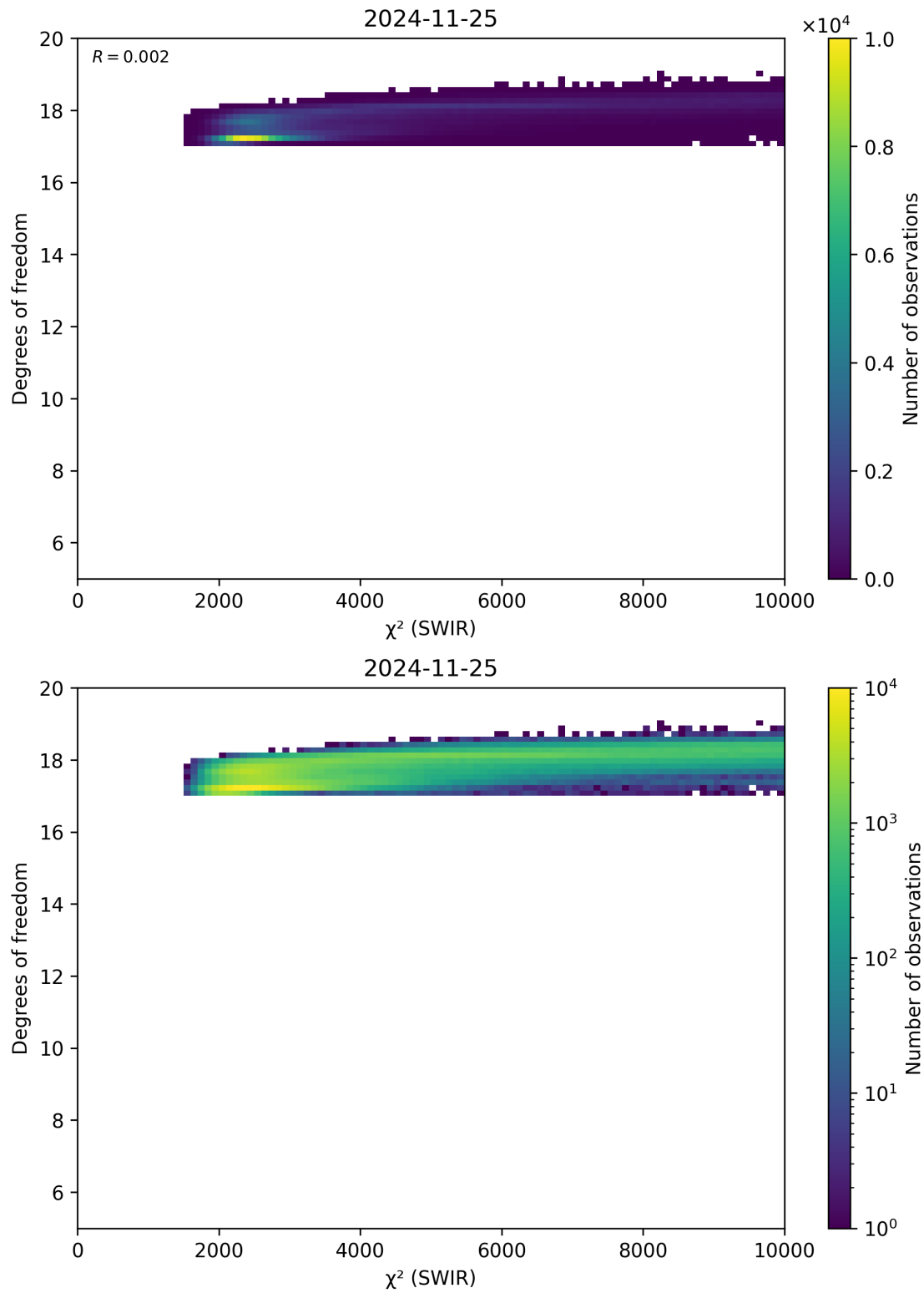
Figure 48: Scatter density plot of “ \chi^2 (SWIR)” against “Degrees of freedom” for 2024-11-25 to 2024-11-26.
