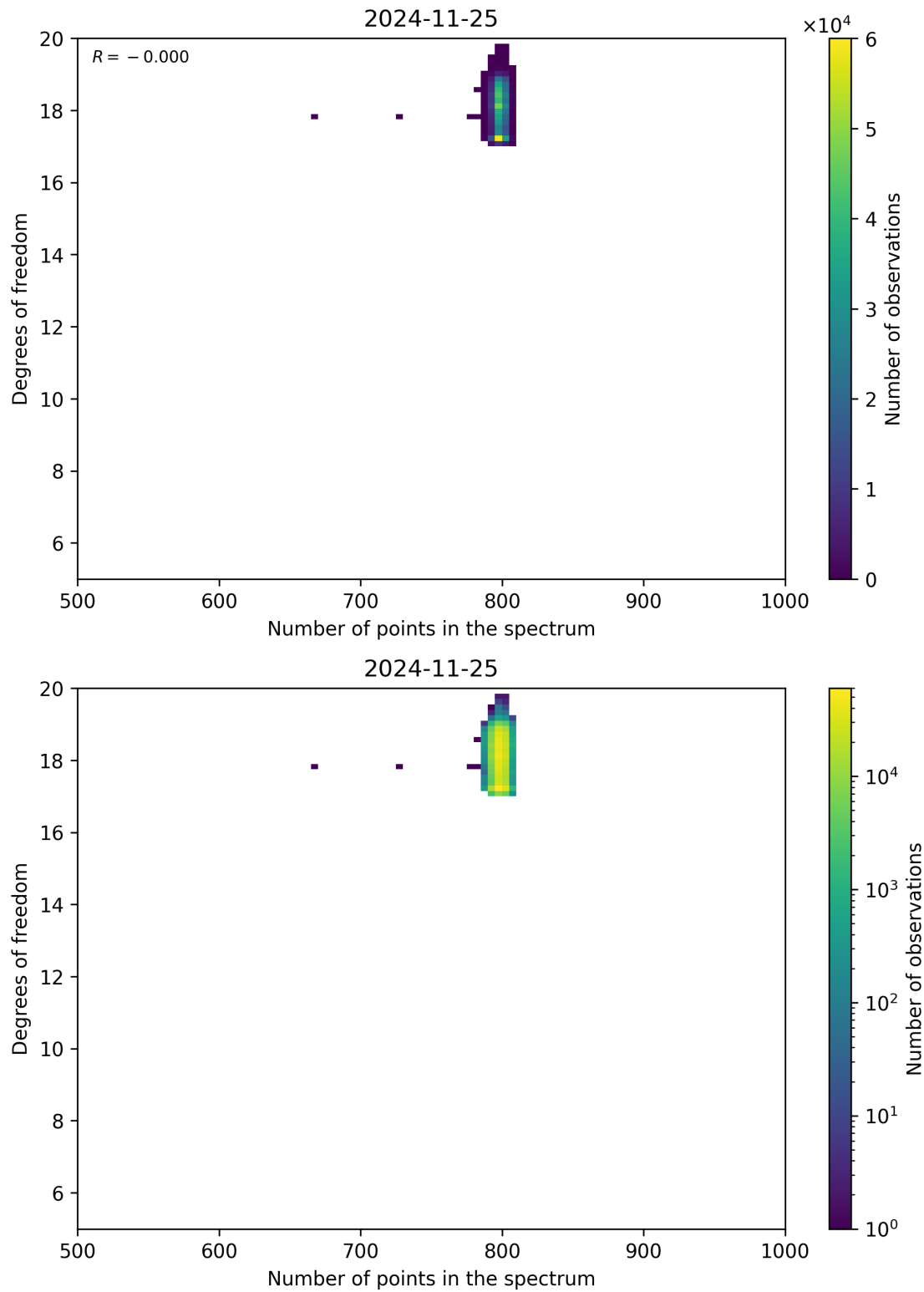
Figure 90: Scatter density plot of “Number of points in the spectrum” against “Degrees of freedom” for 2024-11-25 to 2024-11-26.
