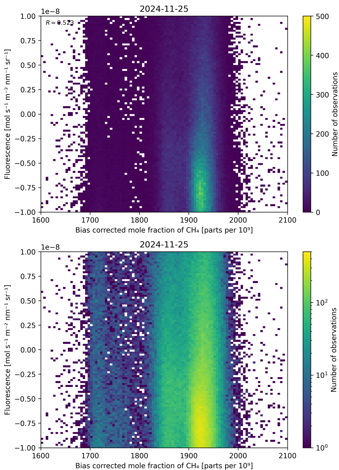
Figure 66: Scatter density plot of “Bias corrected mole fraction of \text{CH}_4 ” against “Fluorescence” for 2024-11-25 to 2024-11-26.
