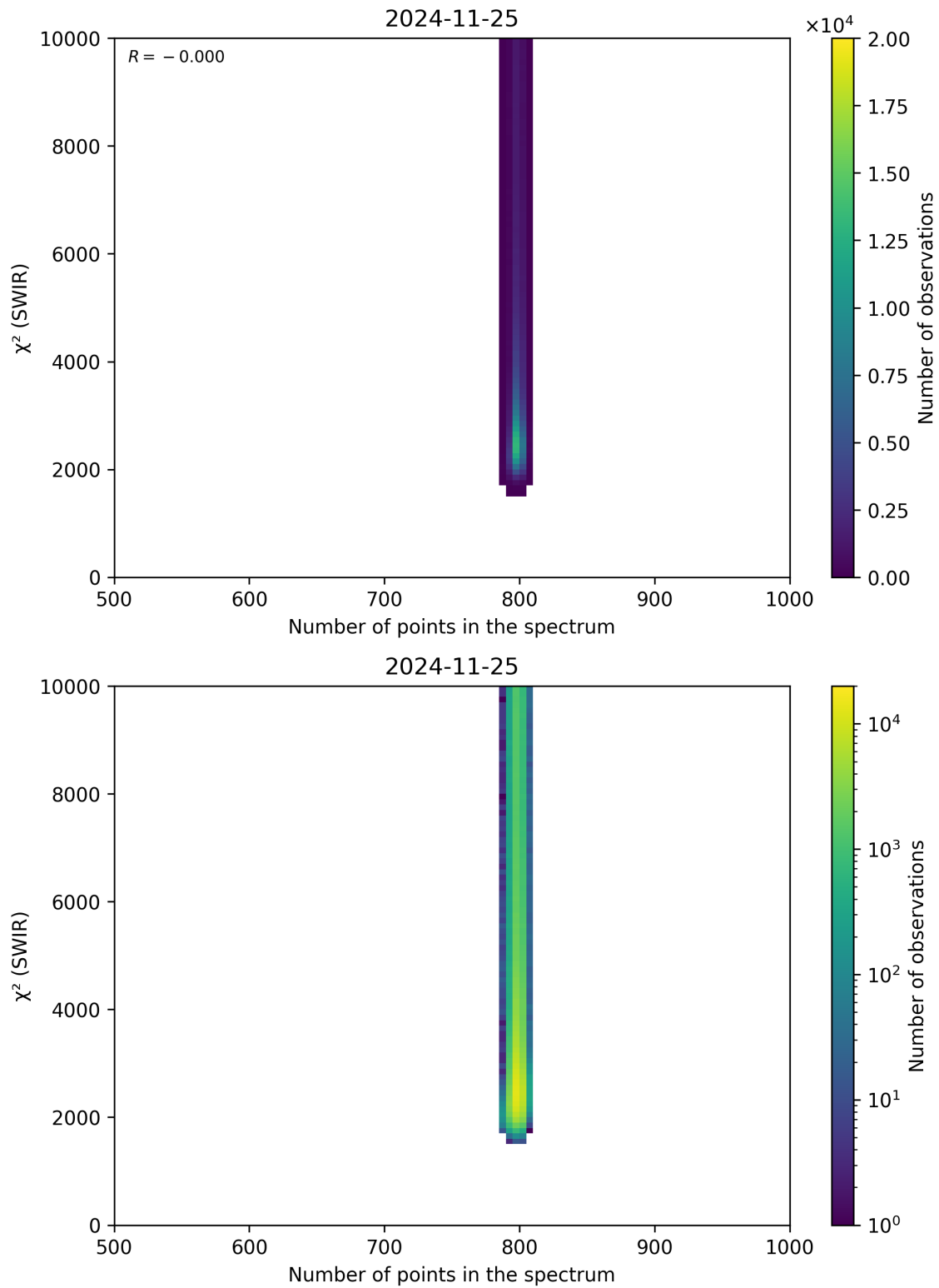
Figure 89: Scatter density plot of “Number of points in the spectrum” against “ \chi^2 (SWIR)” for 2024-11-25 to 2024-11-26.
