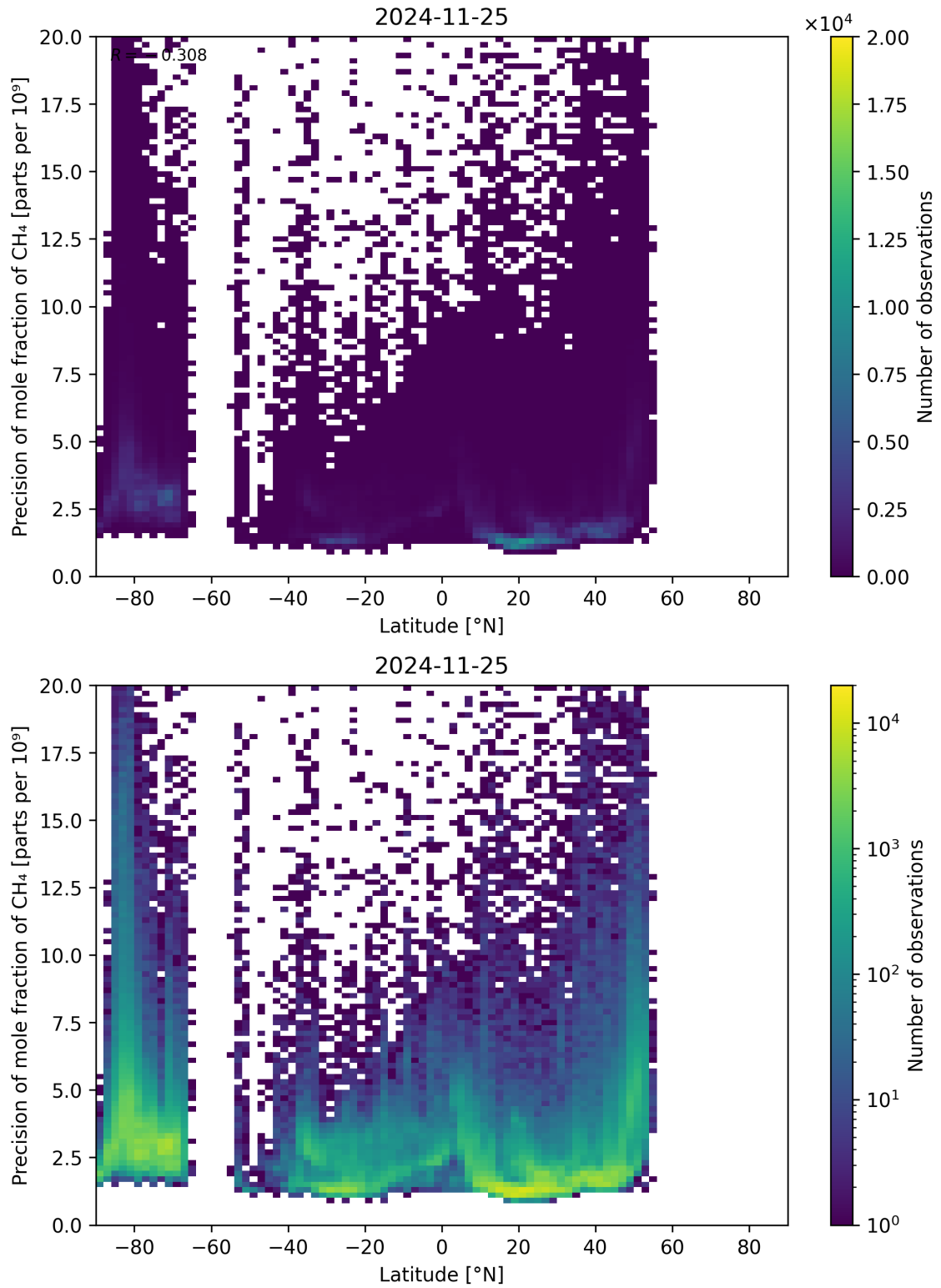
Figure 59: Scatter density plot of “Latitude” against “Precision of mole fraction of CH 4 ” for 2024-11-25 to 2024-11-26.
