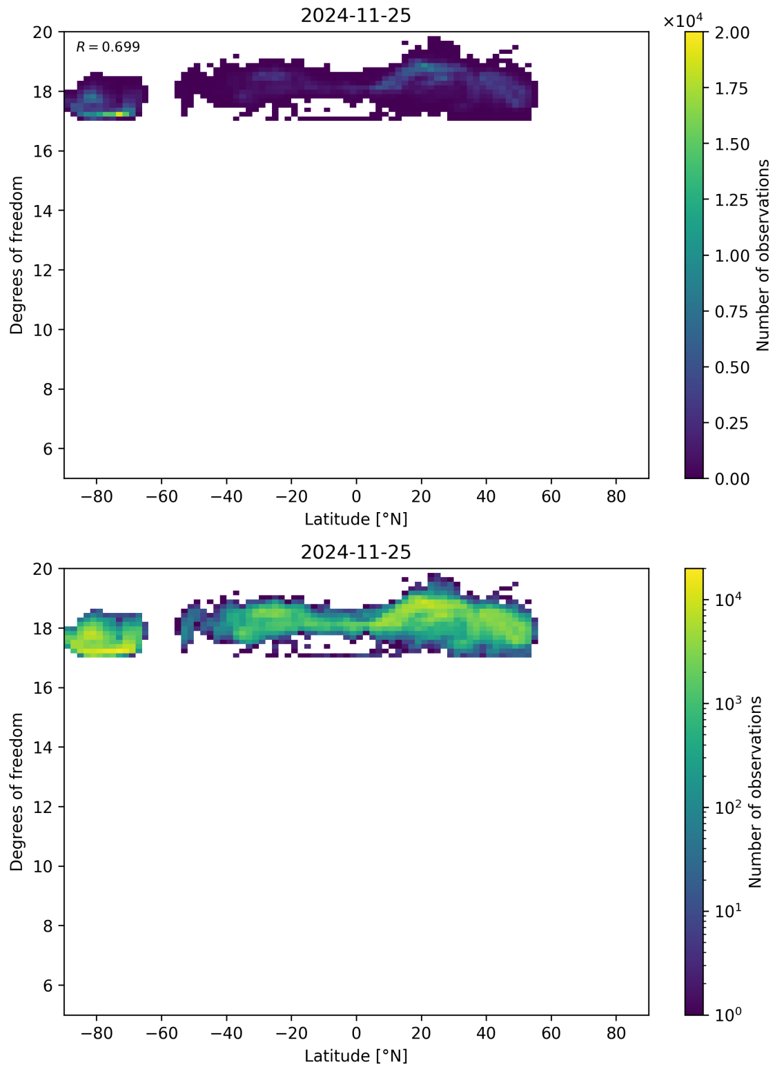
Figure 55: Scatter density plot of “Latitude” against “Degrees of freedom” for 2024-11-25 to 2024-11-26.
