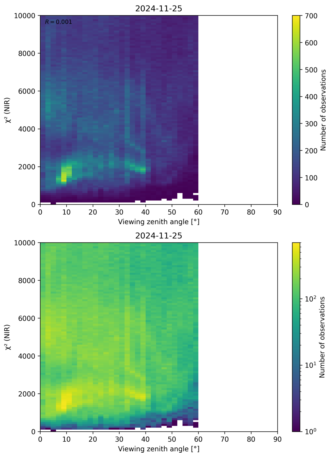
Figure 105: Scatter density plot of “Viewing zenith angle” against “ \chi^2 (NIR)” for 2024-11-25 to 2024-11-26.
