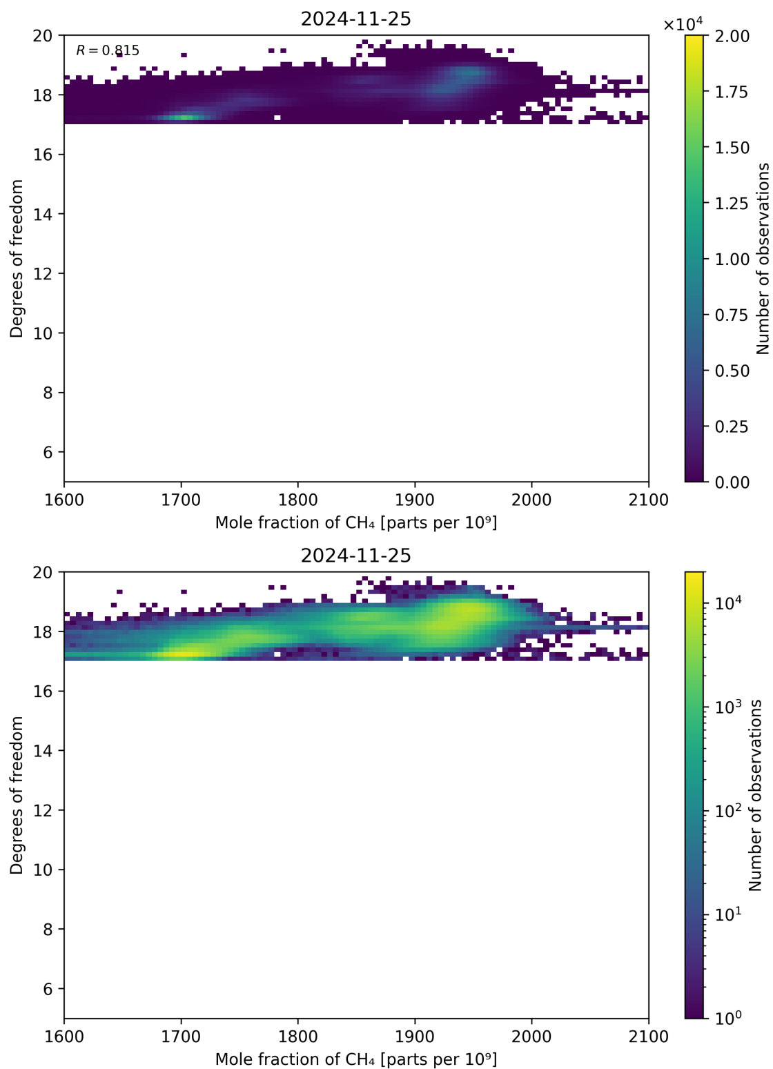
Figure 72: Scatter density plot of “Mole fraction of CH 4 ” against “Degrees of freedom” for 2024-11-25 to 2024-11-26.
