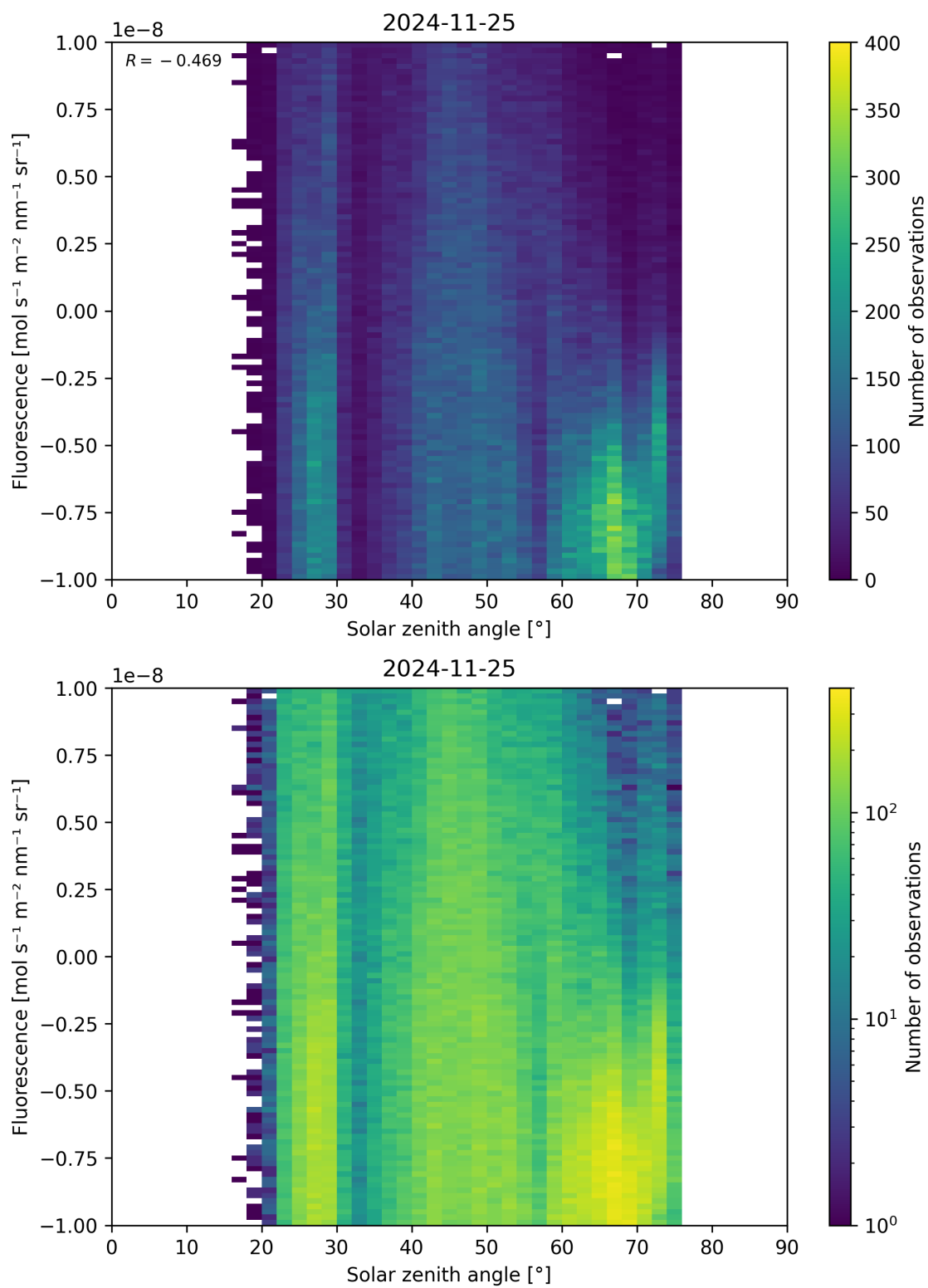
Figure 97: Scatter density plot of “Solar zenith angle” against “Fluorescence” for 2024-11-25 to 2024-11-26.
