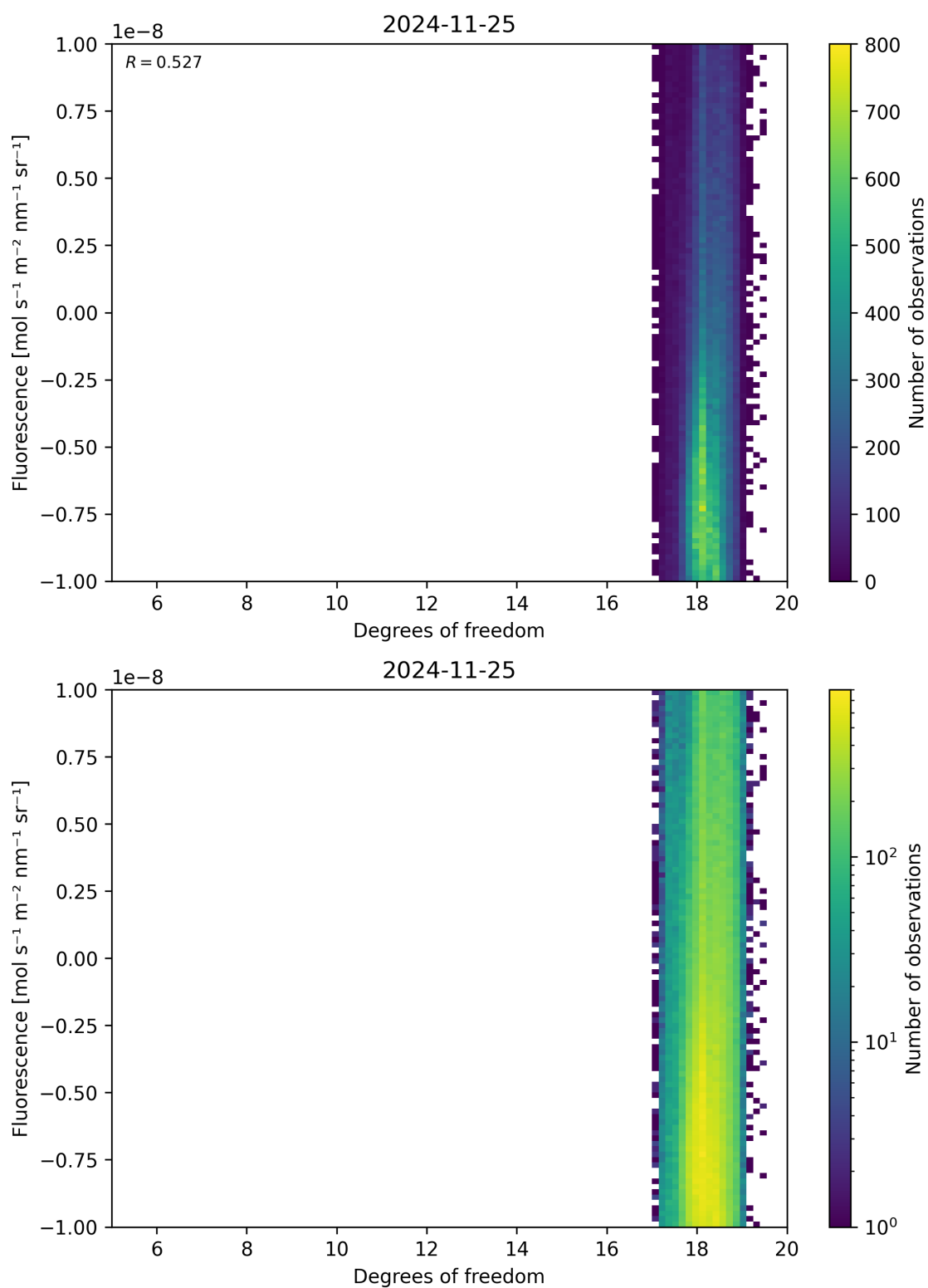
Figure 51: Scatter density plot of “Degrees of freedom” against “Fluorescence” for 2024-11-25 to 2024-11-26.
