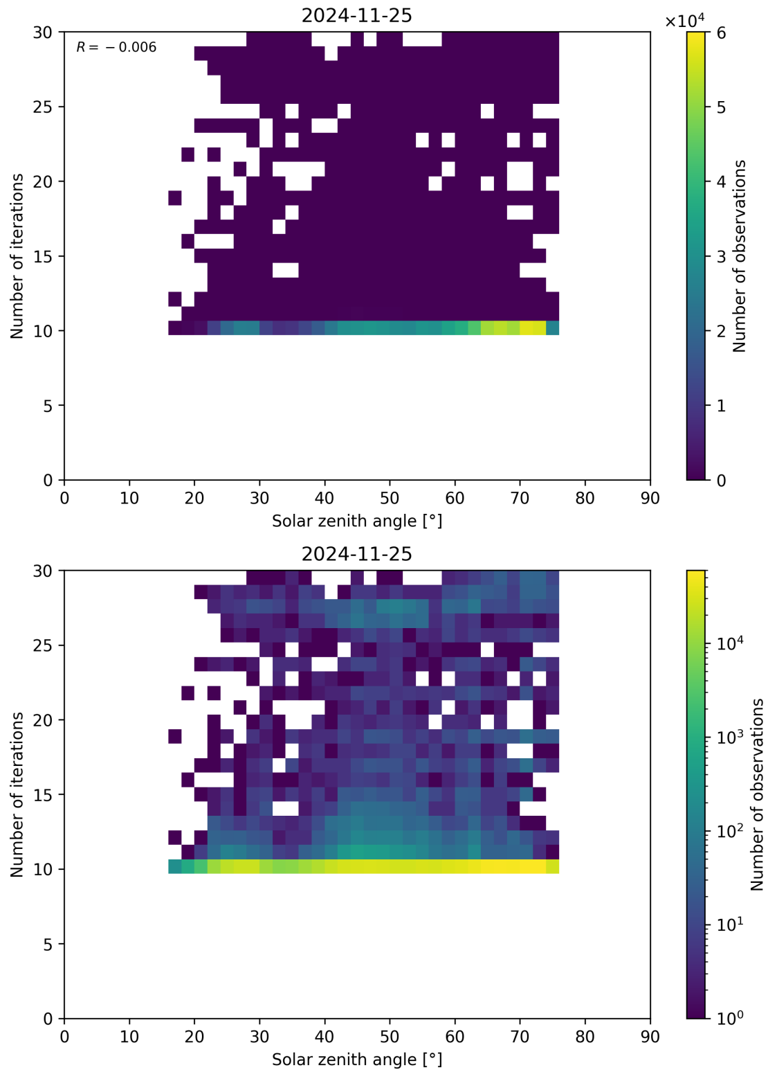
Figure 102: Scatter density plot of “Solar zenith angle” against “Number of iterations” for 2024-11-25 to 2024-11-26.
