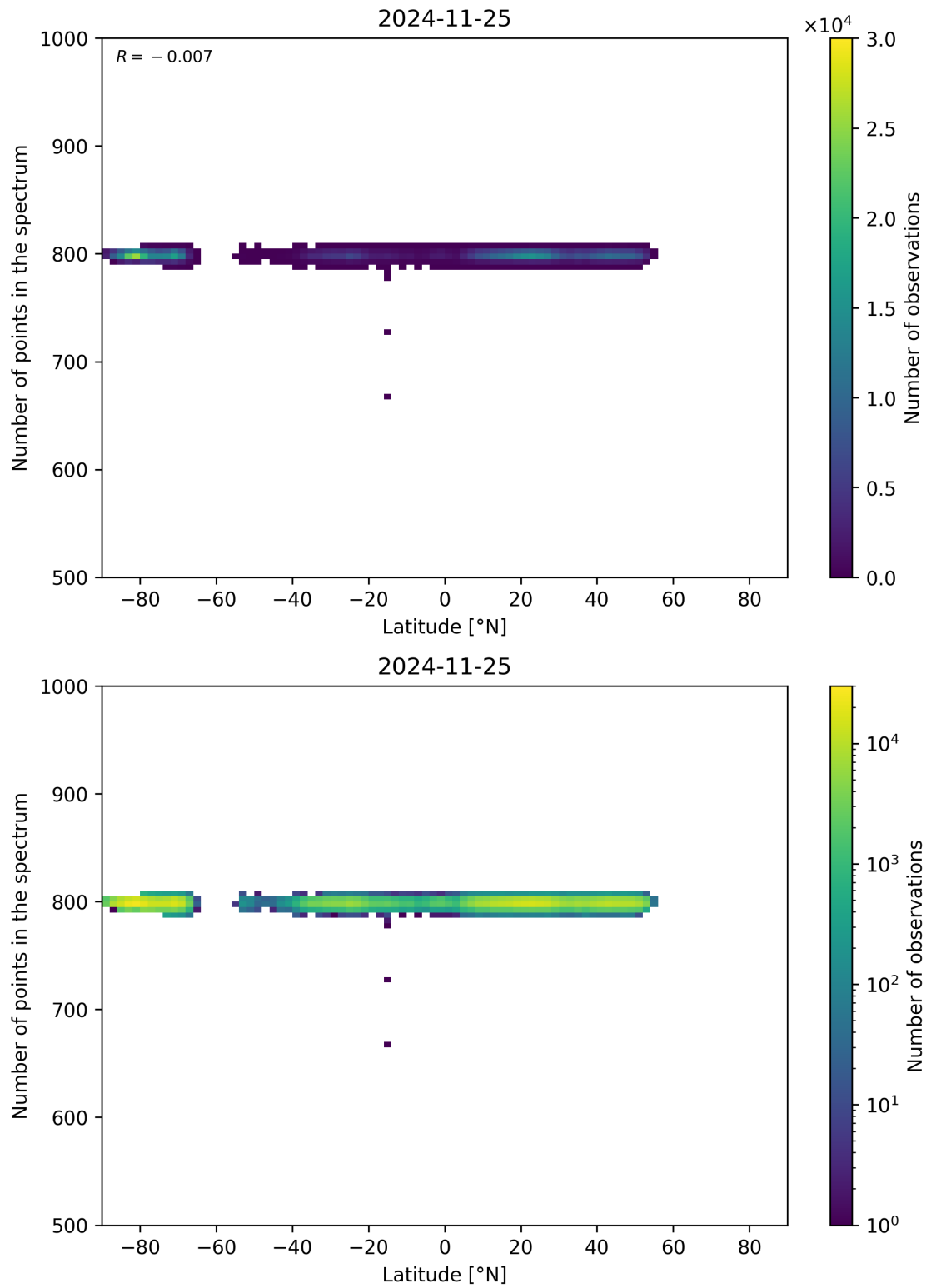
Figure 61: Scatter density plot of “Latitude” against “Number of points in the spectrum” for 2024-11-25 to 2024-11-26.
