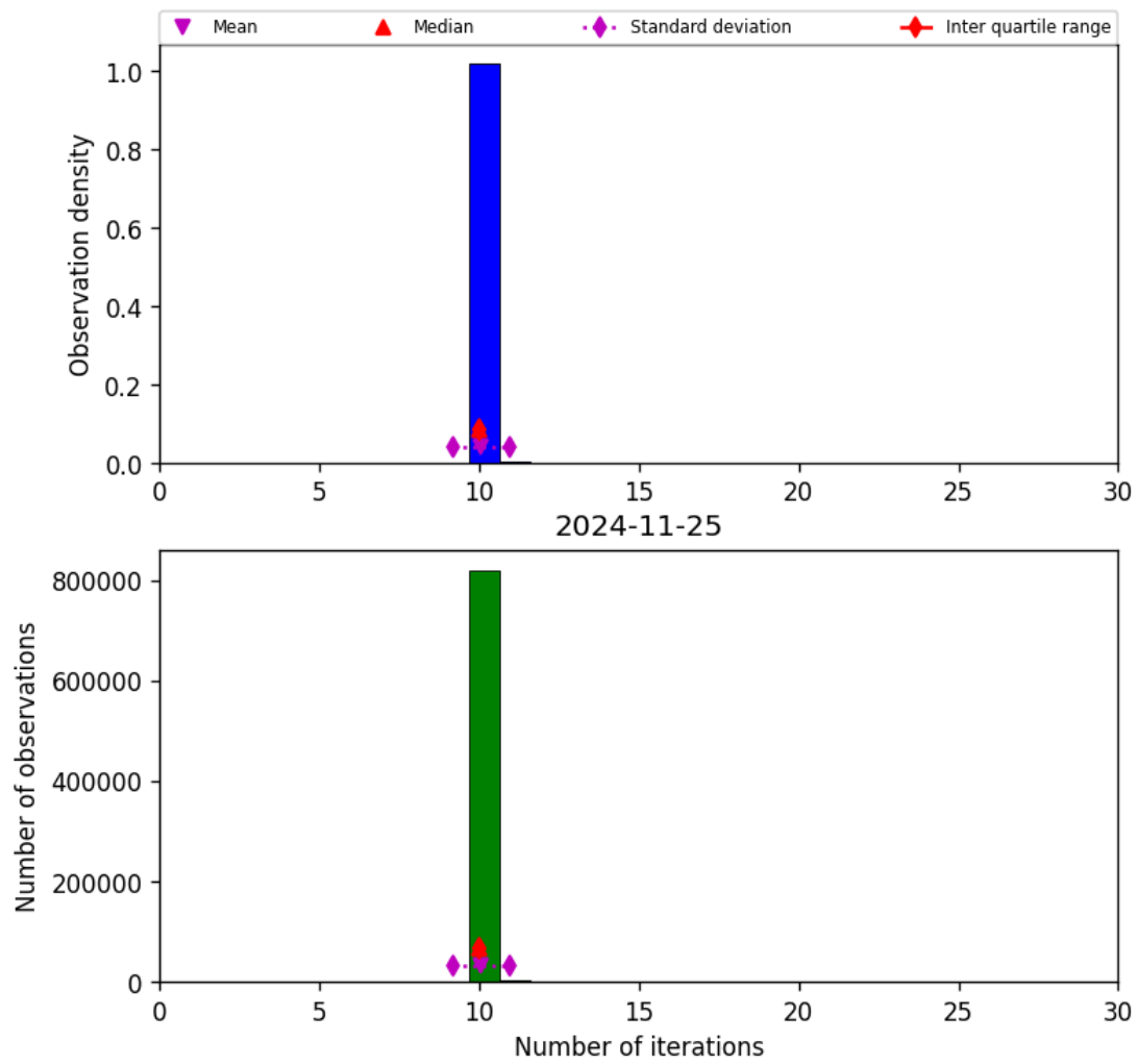
Figure 31: Histogram of “Number of iterations” for 2024-11-25 to 2024-11-26
