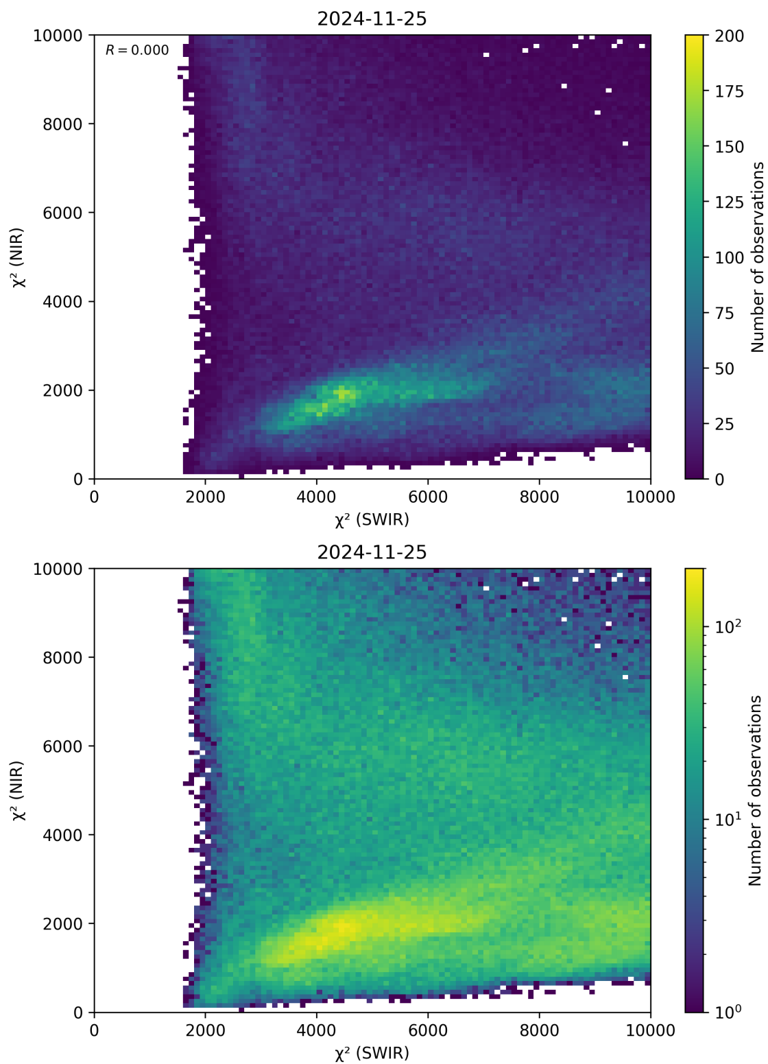
Figure 47: Scatter density plot of “ \chi^2 (SWIR)” against “ \chi^2 (NIR)” for 2024-11-25 to 2024-11-26.
