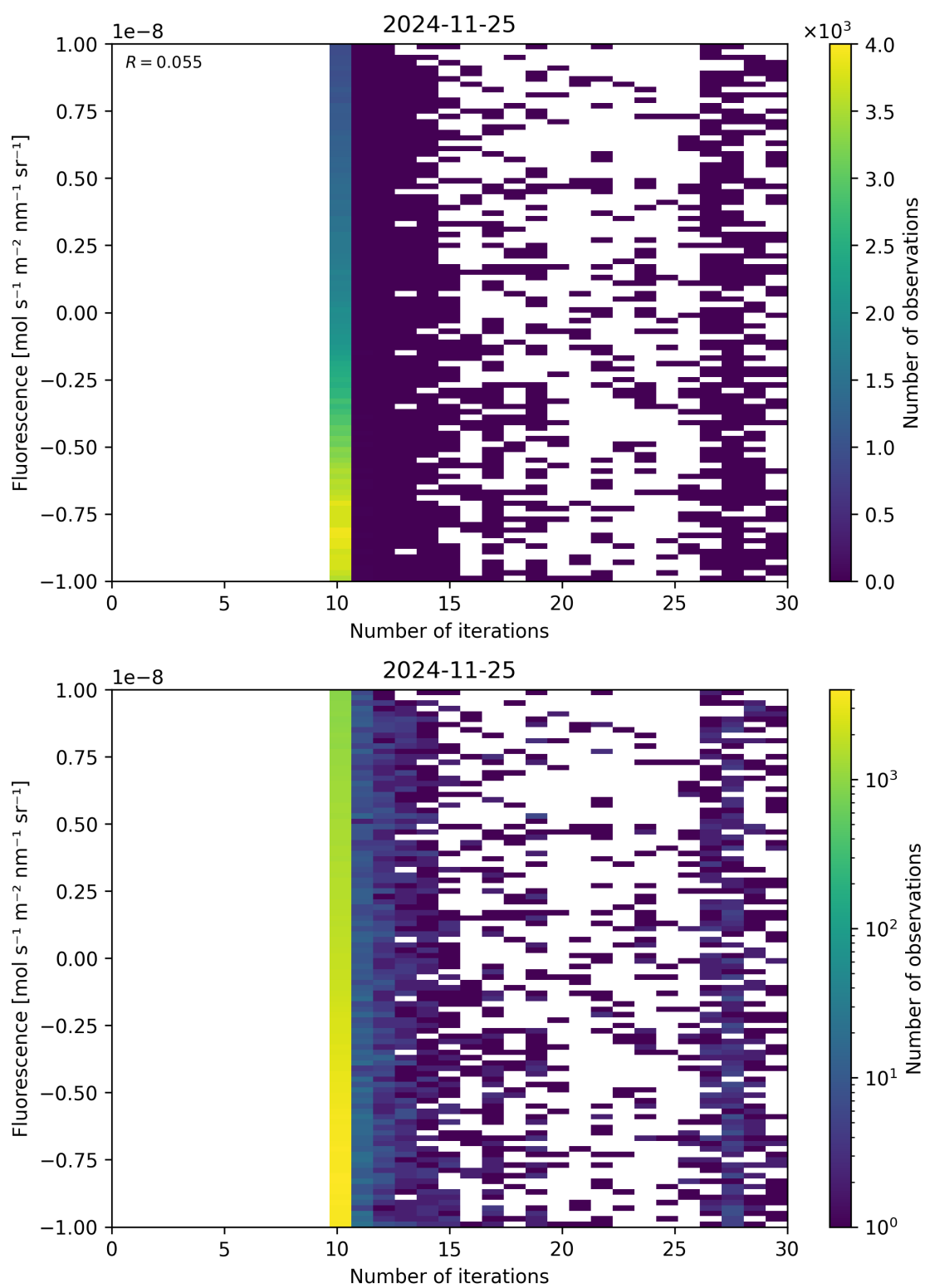
Figure 87: Scatter density plot of “Number of iterations” against “Fluorescence” for 2024-11-25 to 2024-11-26.
