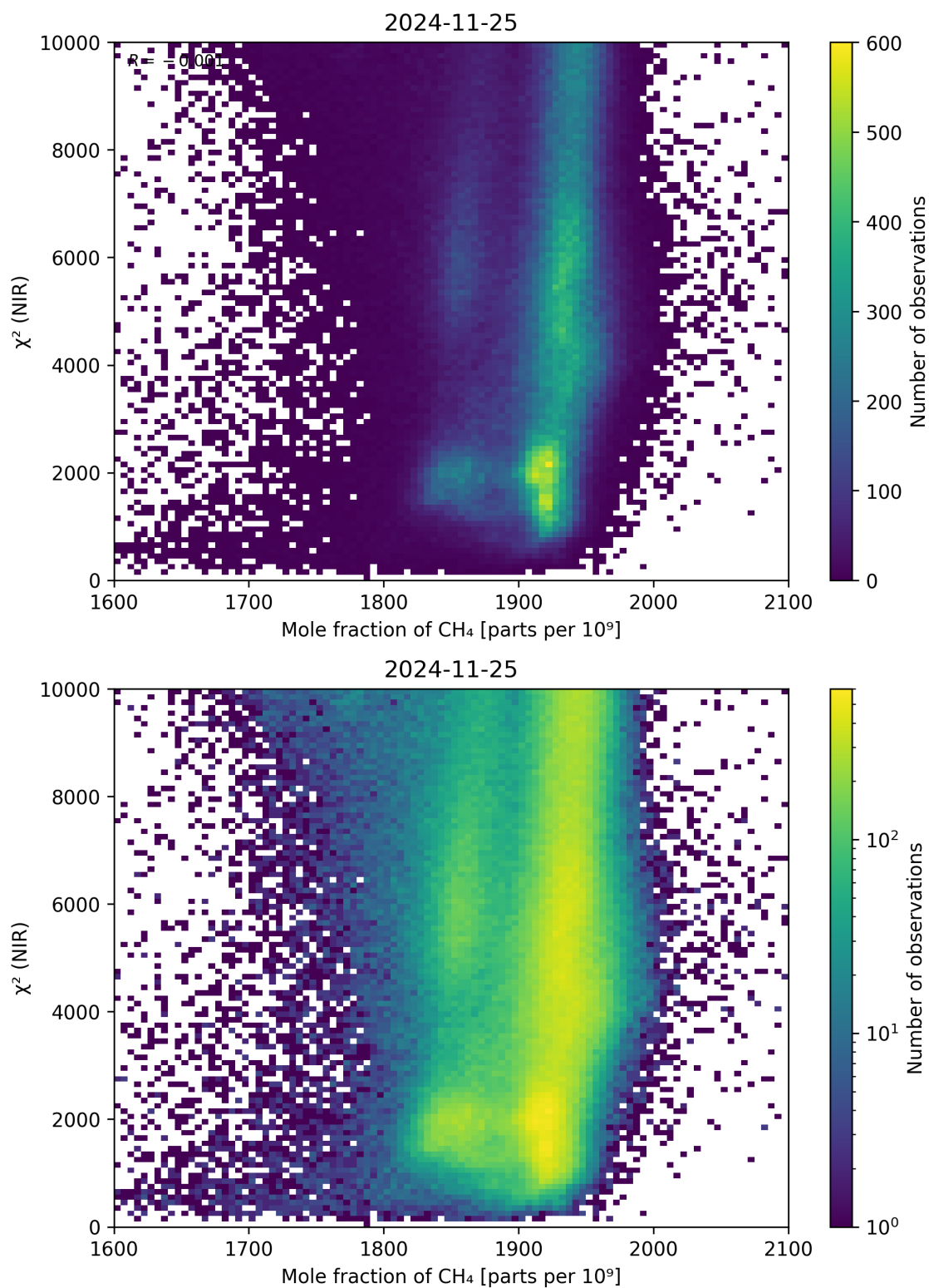
Figure 70: Scatter density plot of “Mole fraction of \text{CH}_4 ” against “ \chi^2 (NIR)” for 2024-11-25 to 2024-11-26.
