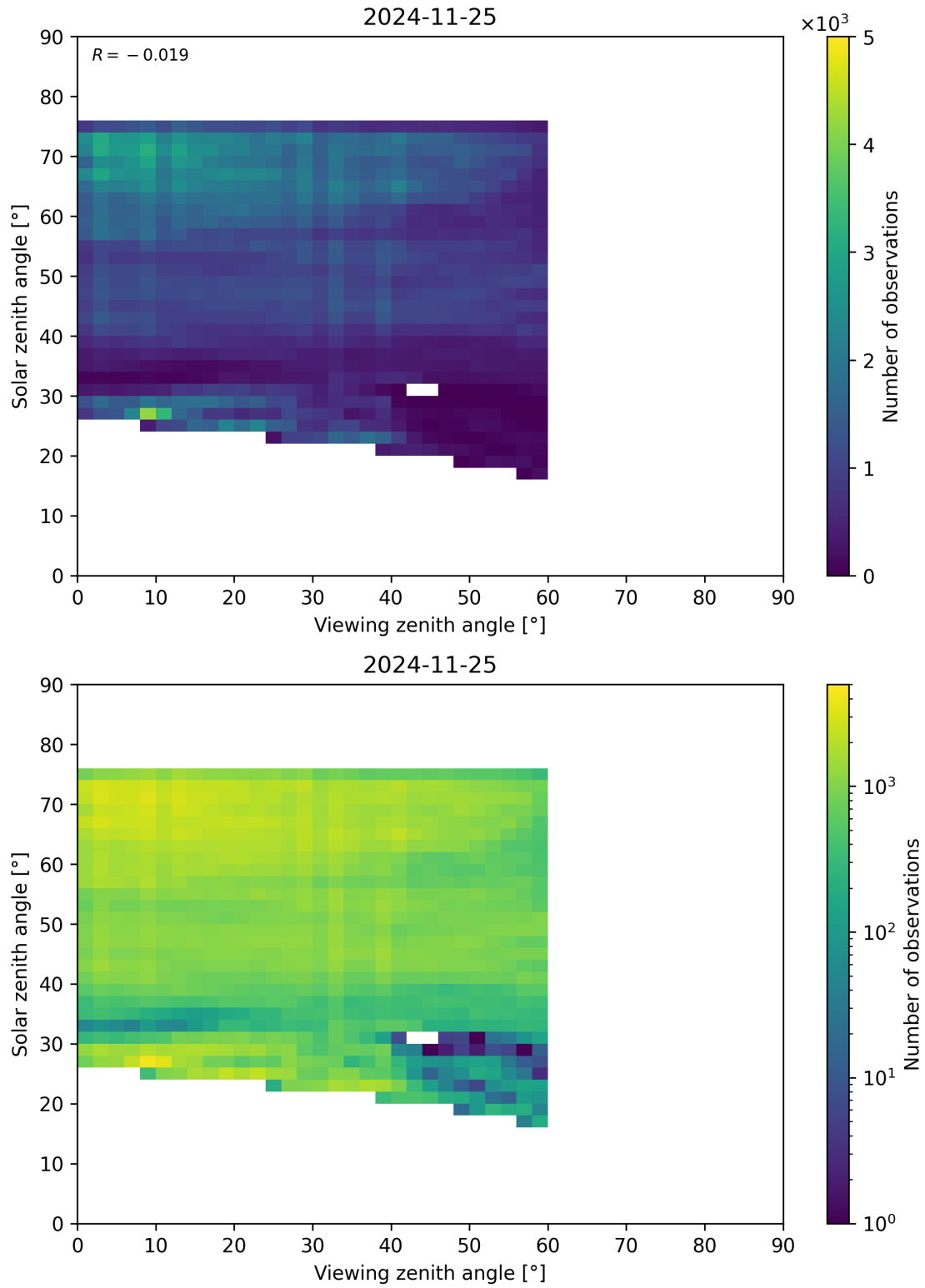
Figure 115: Scatter density plot of “Viewing zenith angle” against “Solar zenith angle” for 2024-11-25 to 2024-11-26.
