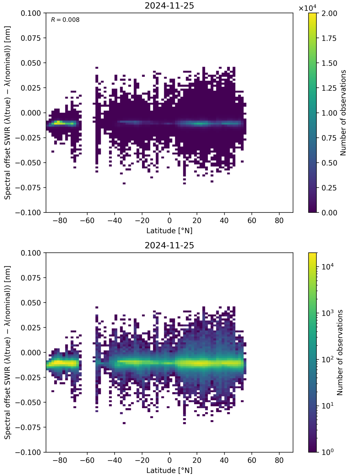
Figure 62: Scatter density plot of “Latitude” against “Spectral offset SWIR ( \lambda_{\text{true}} - \lambda_{\text{nominal}} )” for 2024-11-25 to 2024-11-26.
