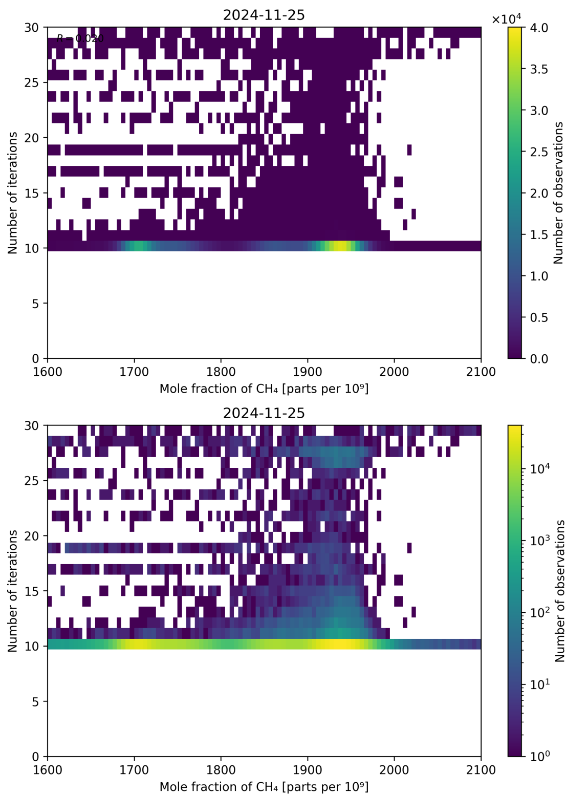
Figure 76: Scatter density plot of “Mole fraction of CH 4 ” against “Number of iterations” for 2024-11-25 to 2024-11-26.
