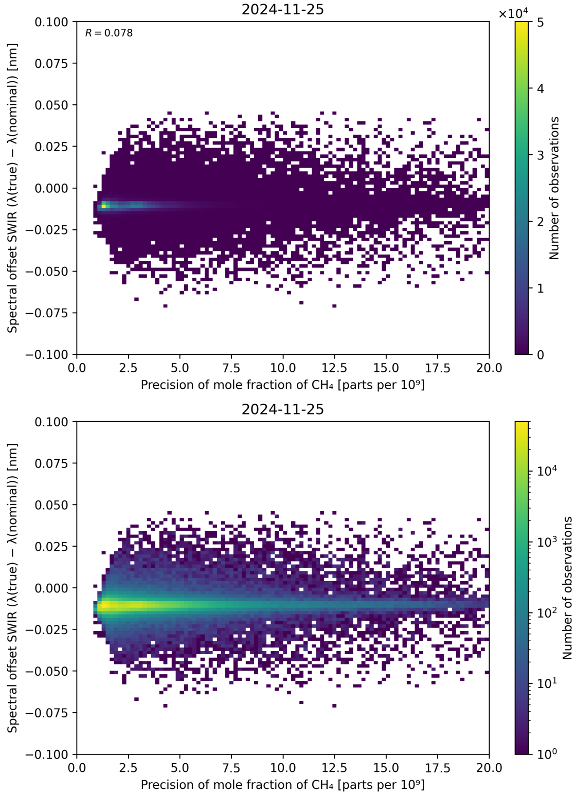
Figure 85: Scatter density plot of “Precision of mole fraction of \text{CH}_4 ” against “Spectral offset SWIR ( \lambda_{\text{true}} - \lambda_{\text{nominal}} )” for 2024-11-25 to 2024-11-26.
