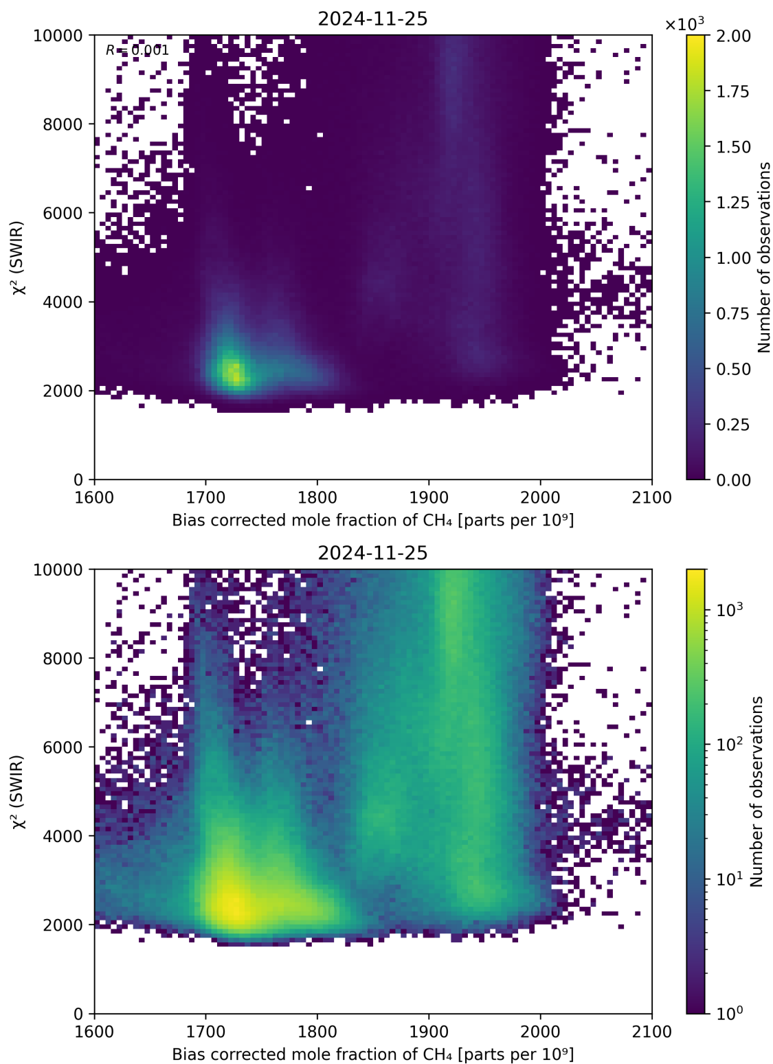
Figure 64: Scatter density plot of “Bias corrected mole fraction of CH 4 ” against “ \chi^2 (SWIR)” for 2024-11-25 to 2024-11-26.
