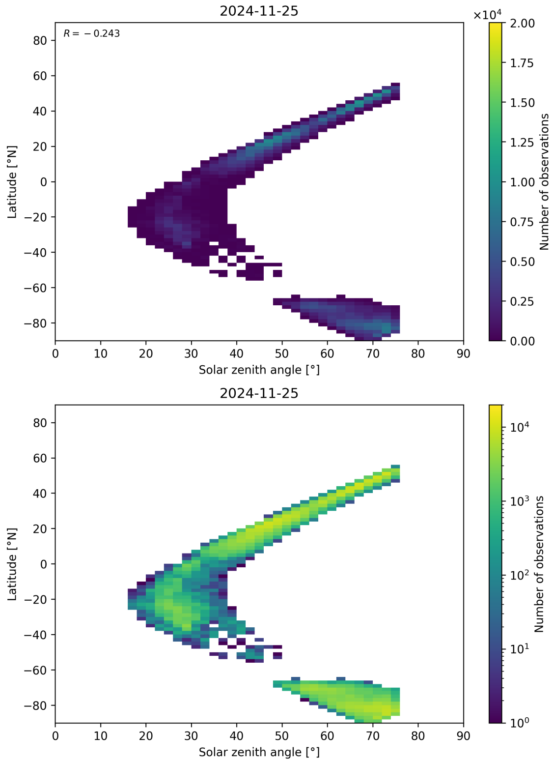
Figure 98: Scatter density plot of “Solar zenith angle” against “Latitude” for 2024-11-25 to 2024-11-26.
