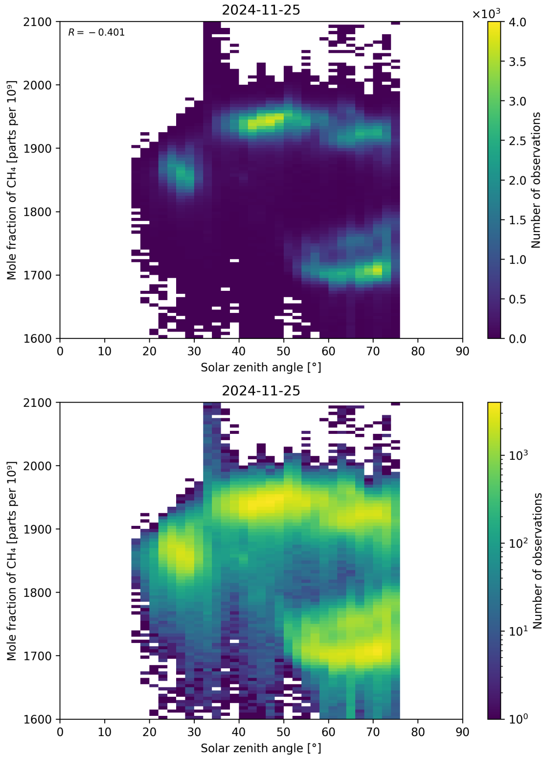
Figure 99: Scatter density plot of “Solar zenith angle” against “Mole fraction of CH 4 ” for 2024-11-25 to 2024-11-26.
