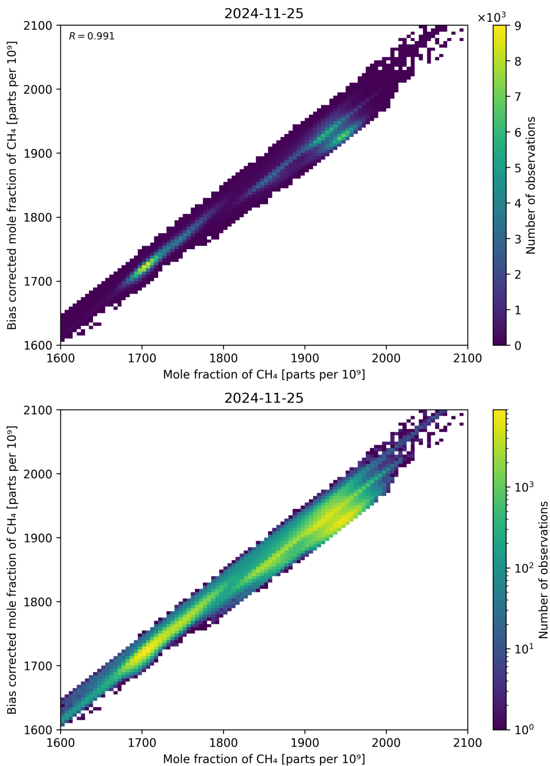
Figure 74: Scatter density plot of “Mole fraction of CH 4 ” against “Bias corrected mole fraction of CH 4 ” for 2024-11-25 to 2024-11-26.
