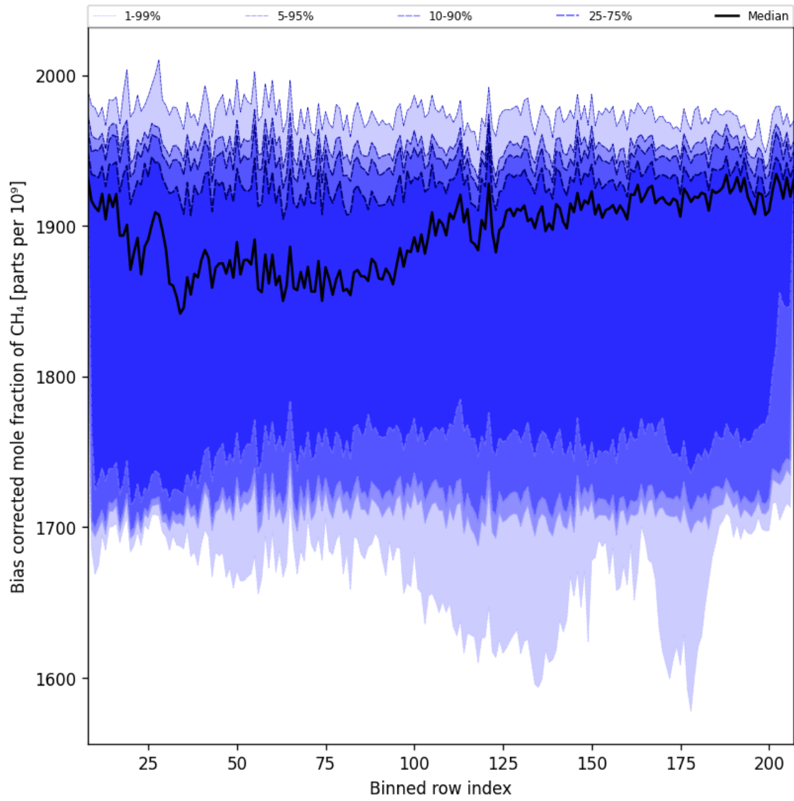
Figure 36: Along track statistics of “Bias corrected mole fraction of CH 4 ” for 2024-11-25 to 2024-11-26
