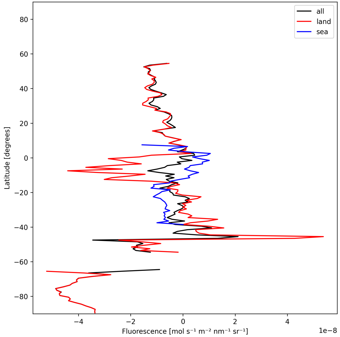
Figure 21: Zonal average of “Fluorescence” for 2024-11-25 to 2024-11-26.
