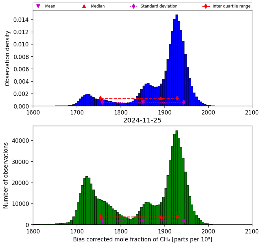
Figure 25: Histogram of “Bias corrected mole fraction of CH 4 ” for 2024-11-25 to 2024-11-26
