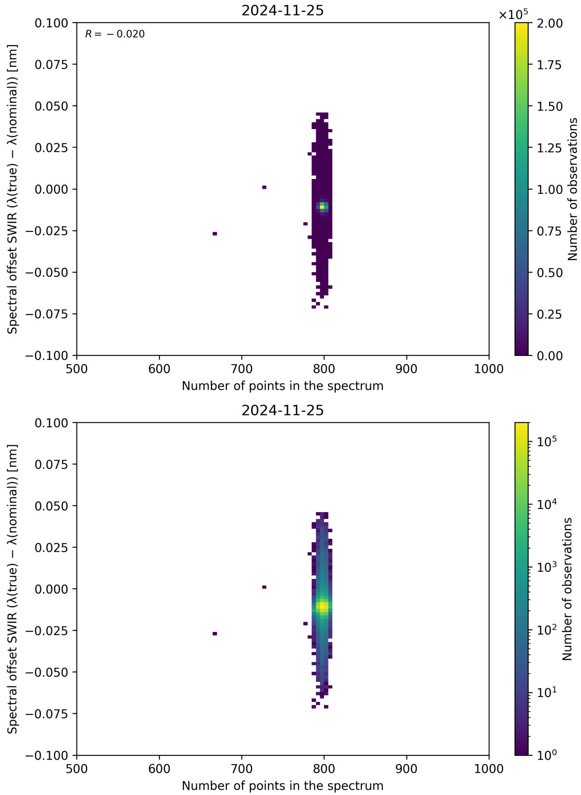
Figure 93: Scatter density plot of “Number of points in the spectrum” against “Spectral offset SWIR ( \lambda_{\text{true}} - \lambda_{\text{nominal}} )” for 2024-11-25 to 2024-11-26.
