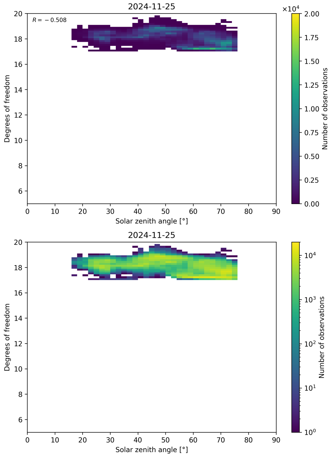
Figure 96: Scatter density plot of “Solar zenith angle” against “Degrees of freedom” for 2024-11-25 to 2024-11-26.
