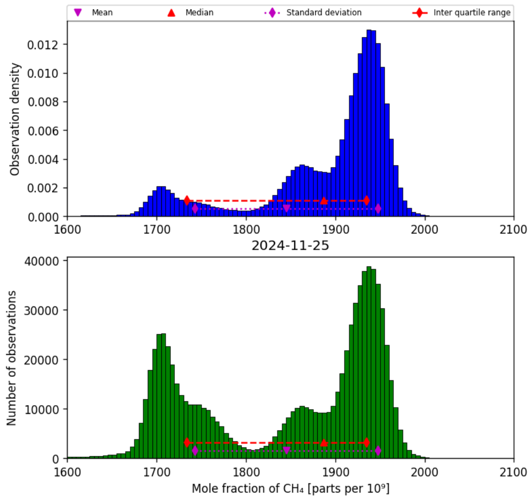
Figure 23: Histogram of “Mole fraction of CH 4 ” for 2024-11-25 to 2024-11-26
