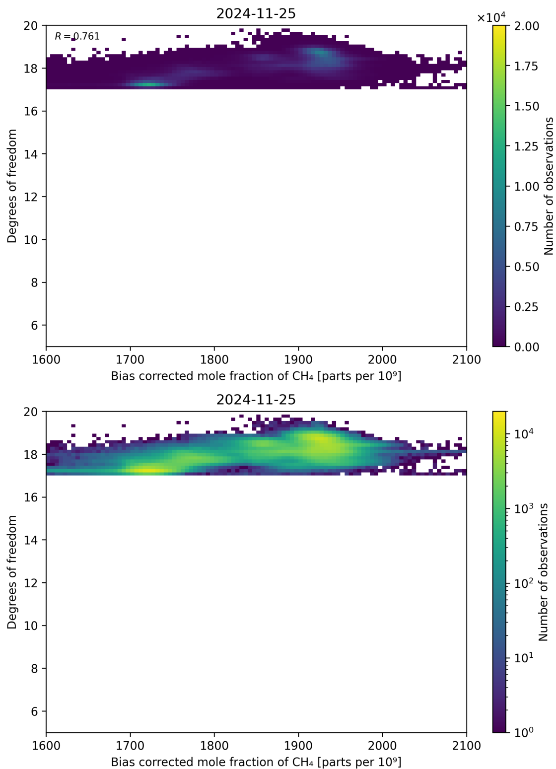
Figure 65: Scatter density plot of “Bias corrected mole fraction of CH 4 ” against “Degrees of freedom” for 2024-11-25 to 2024-11-26.
