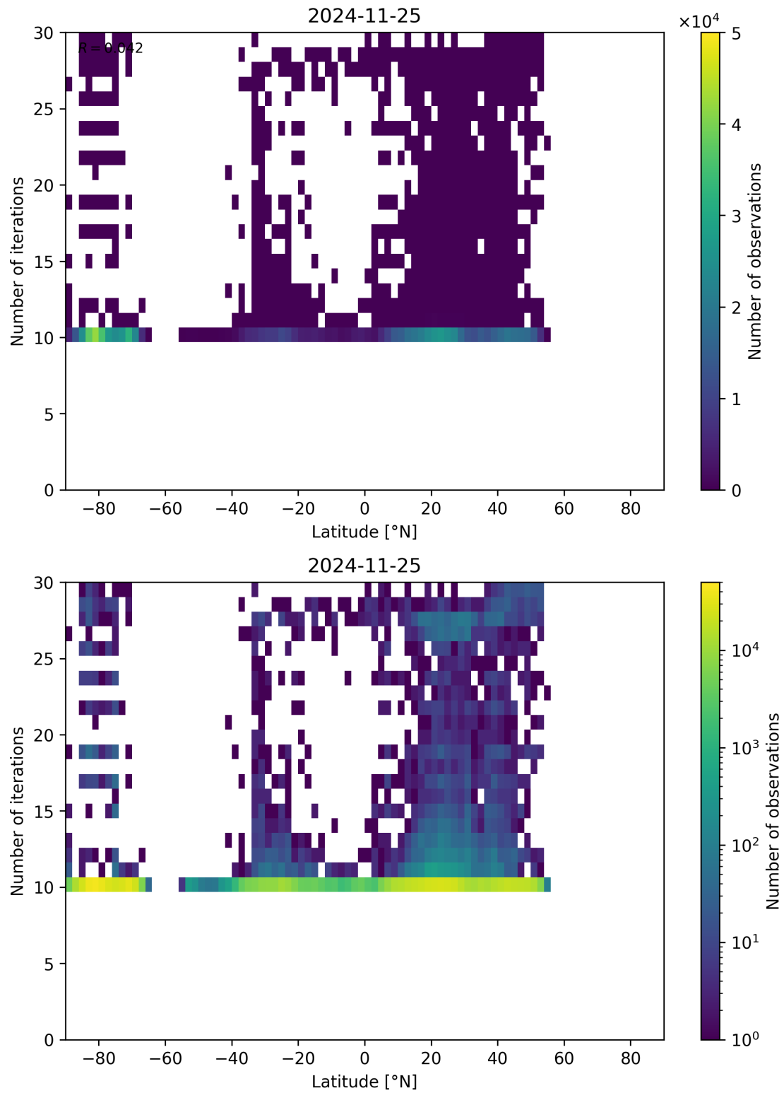
Figure 60: Scatter density plot of “Latitude” against “Number of iterations” for 2024-11-25 to 2024-11-26.
