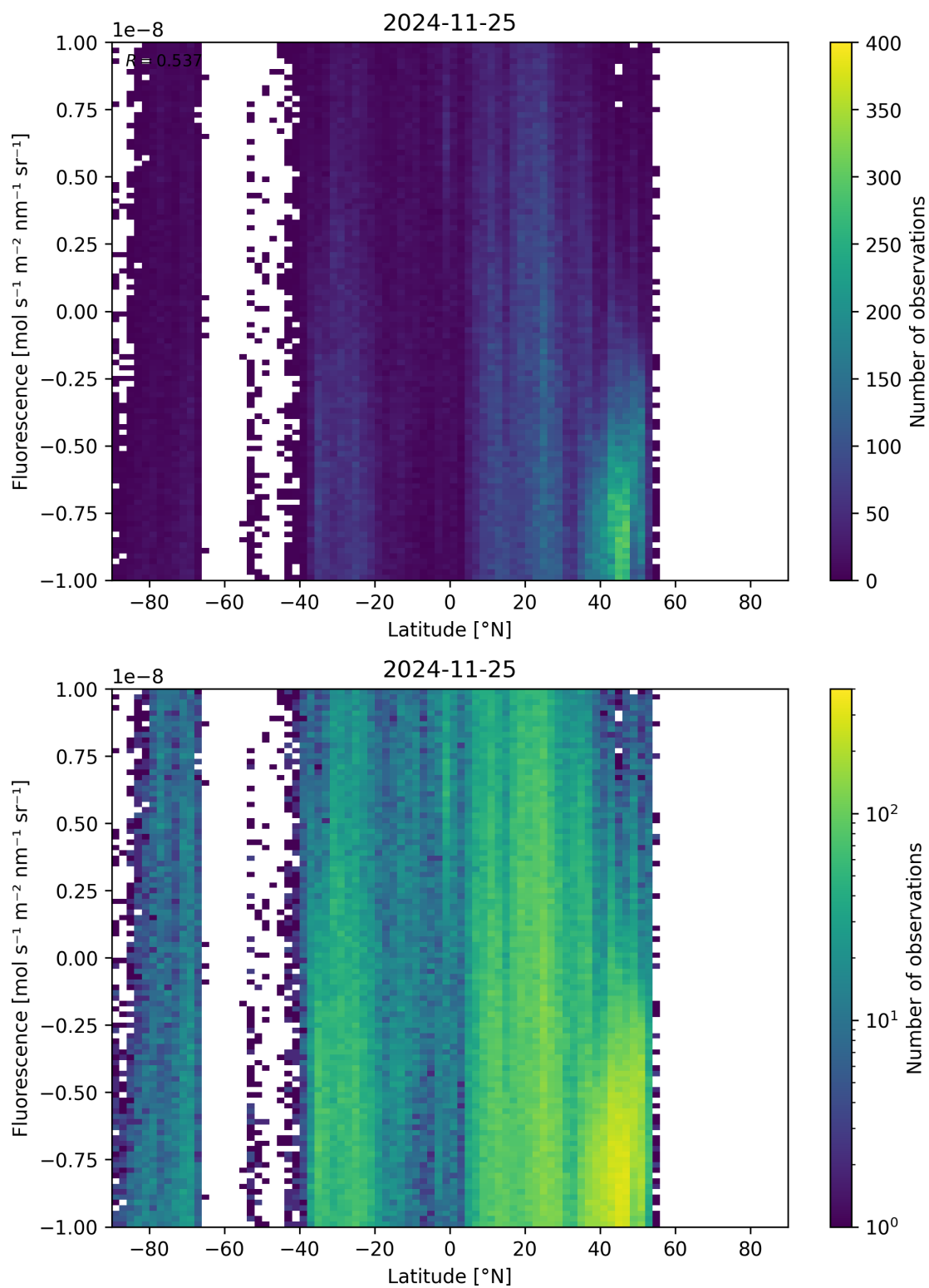
Figure 56: Scatter density plot of “Latitude” against “Fluorescence” for 2024-11-25 to 2024-11-26.
