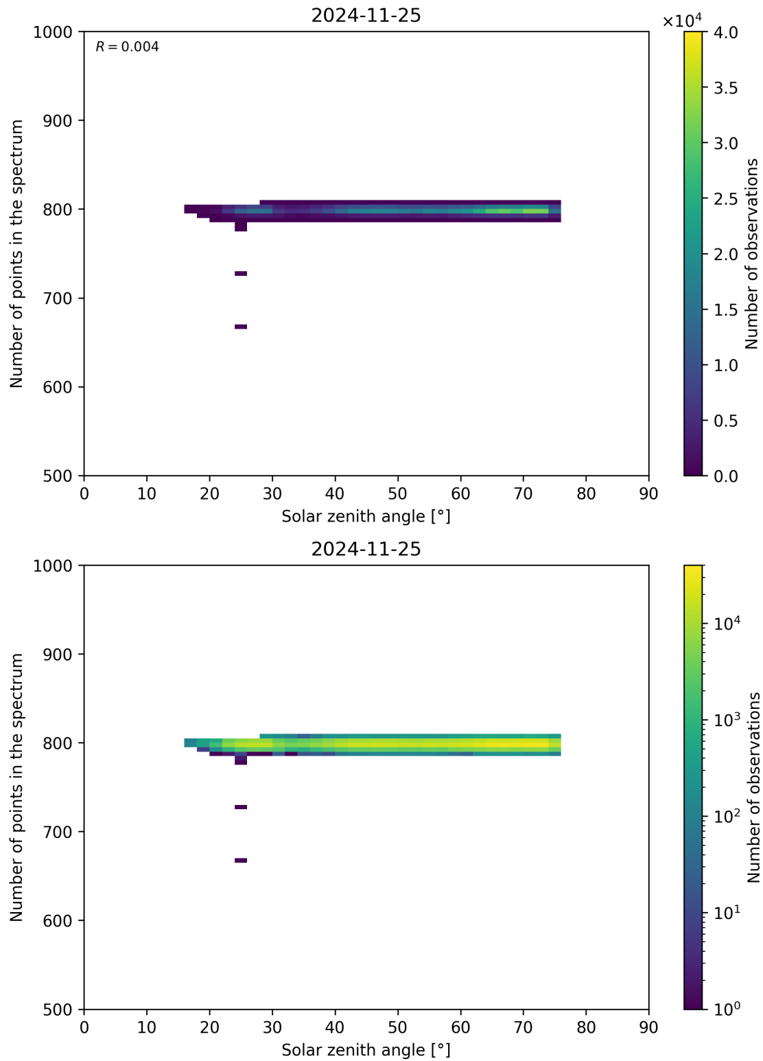
Figure 103: Scatter density plot of “Solar zenith angle” against “Number of points in the spectrum” for 2024-11-25 to 2024-11-26.
