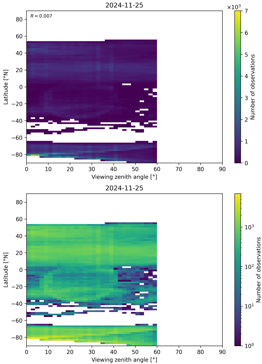
Figure 109: Scatter density plot of “Viewing zenith angle” against “Latitude” for 2024-11-25 to 2024-11-26.
