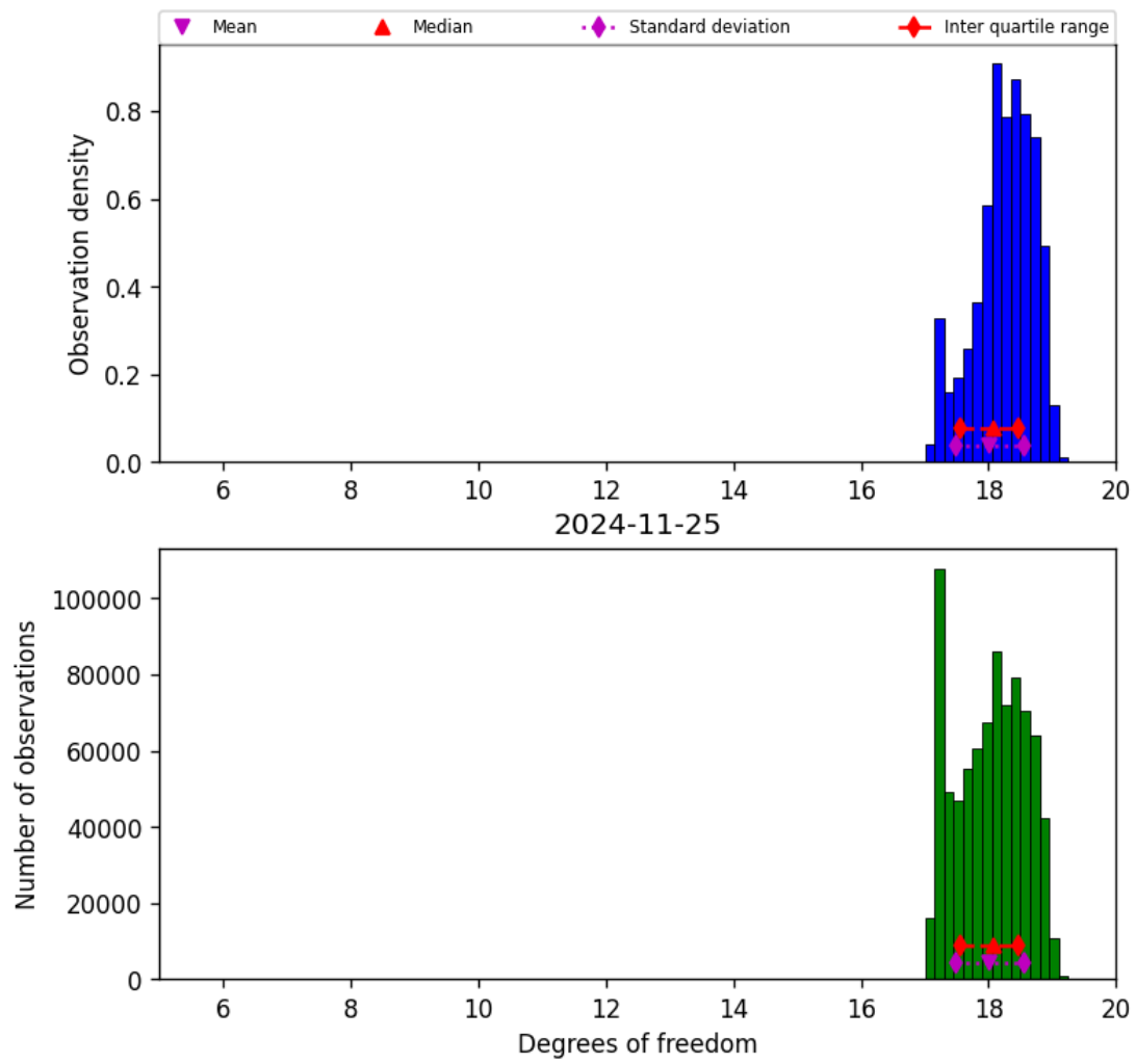
Figure 30: Histogram of “Degrees of freedom” for 2024-11-25 to 2024-11-26
