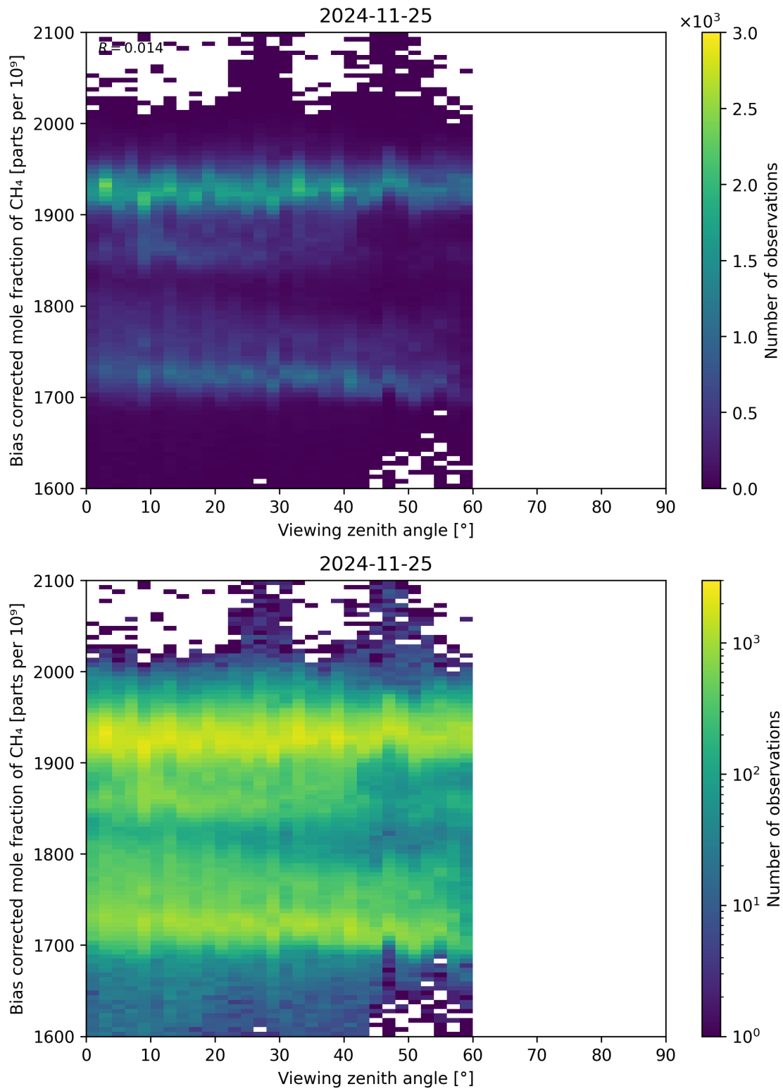
Figure 111: Scatter density plot of “Viewing zenith angle” against “Bias corrected mole fraction of CH 4 ” for 2024-11-25 to 2024-11-26.
