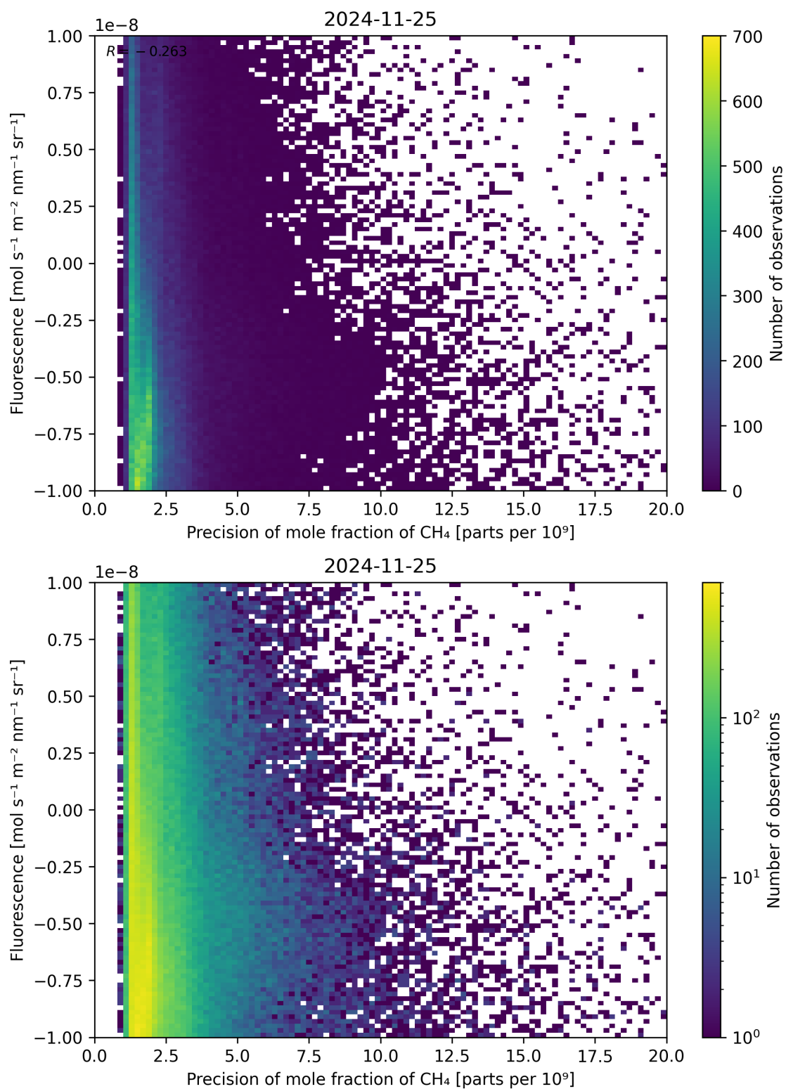
Figure 81: Scatter density plot of “Precision of mole fraction of \text{CH}_4 ” against “Fluorescence” for 2024-11-25 to 2024-11-26.
