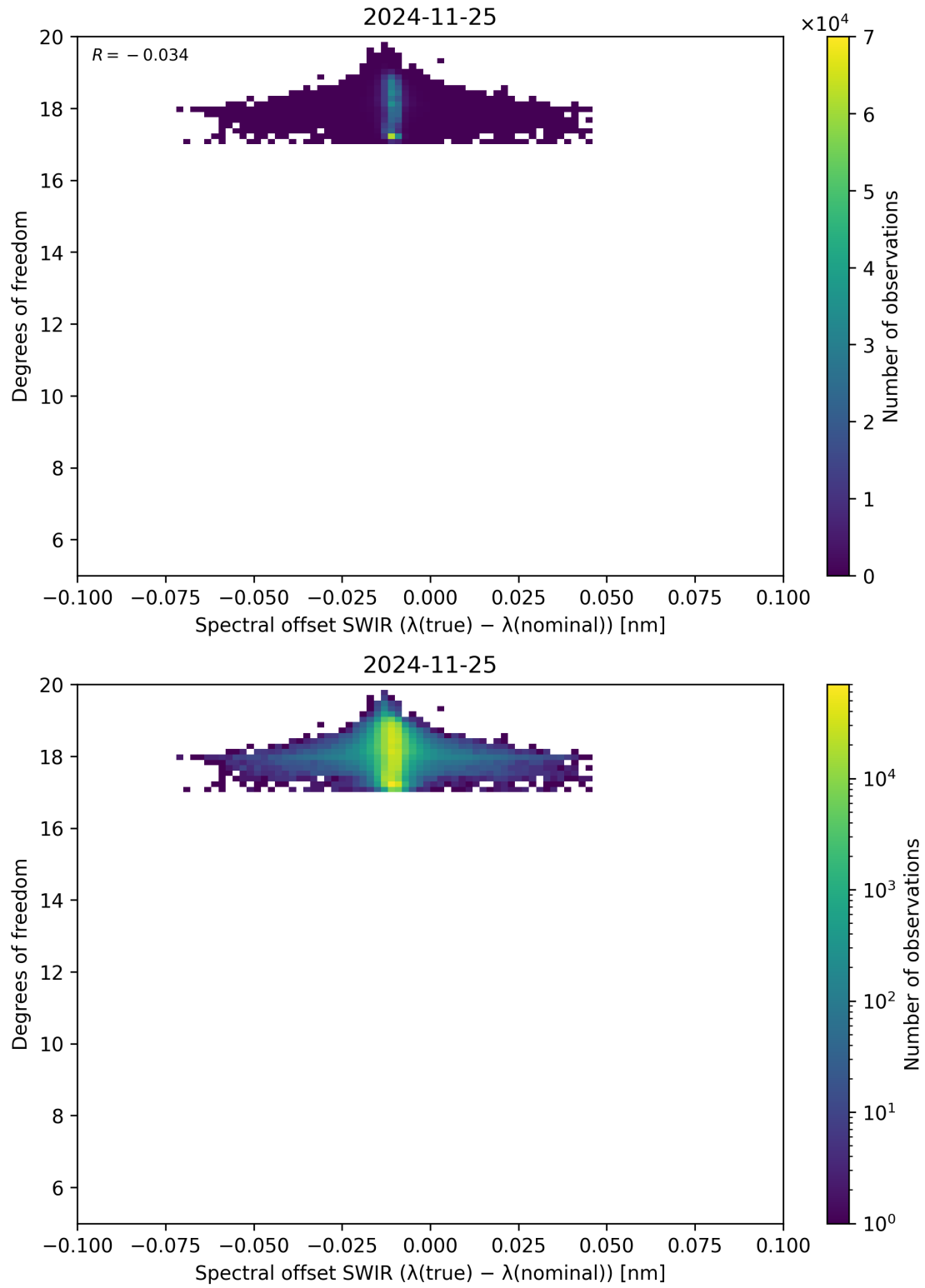
Figure 119: Scatter density plot of “Spectral offset SWIR ( \lambda_{\text{true}} - \lambda_{\text{nominal}} )” against “Degrees of freedom” for 2024-11-25 to 2024-11-26.
