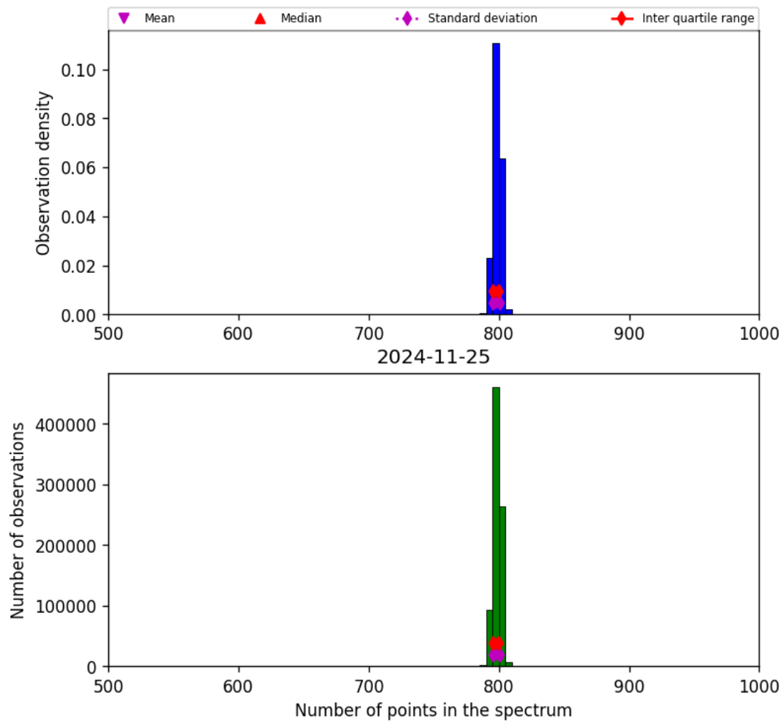
Figure 26: Histogram of “Number of points in the spectrum” for 2024-11-25 to 2024-11-26
