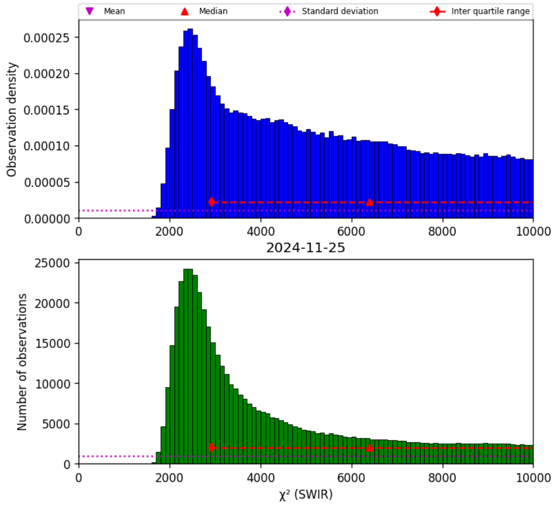
Figure 28: Histogram of “ \chi^2 (SWIR)” for 2024-11-25 to 2024-11-26
