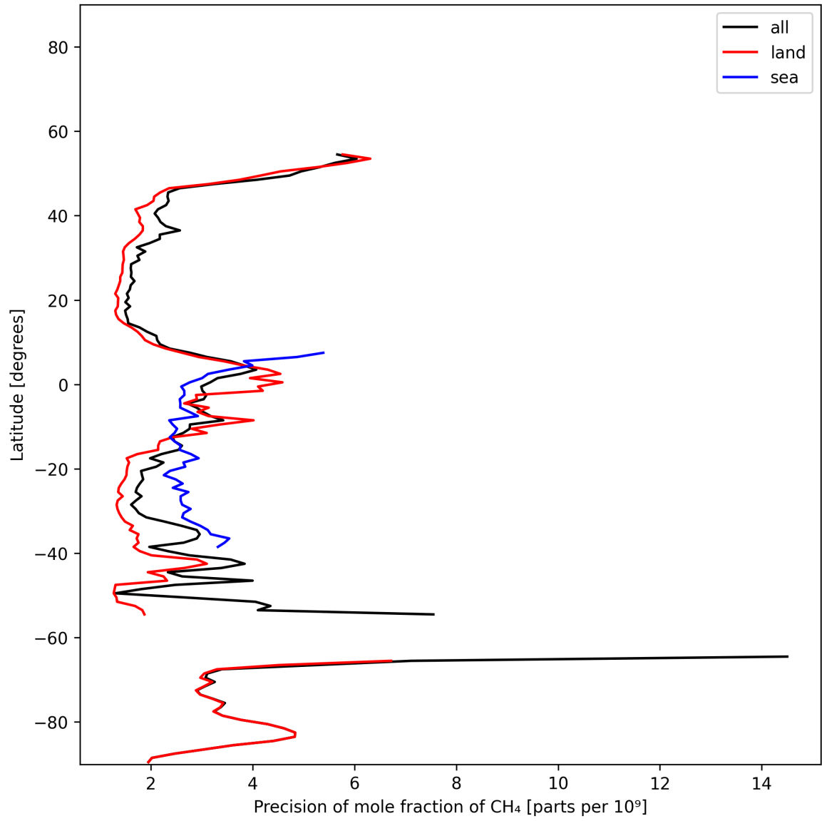
Figure 13: Zonal average of “Precision of mole fraction of CH 4 ” for 2024-11-25 to 2024-11-26.
