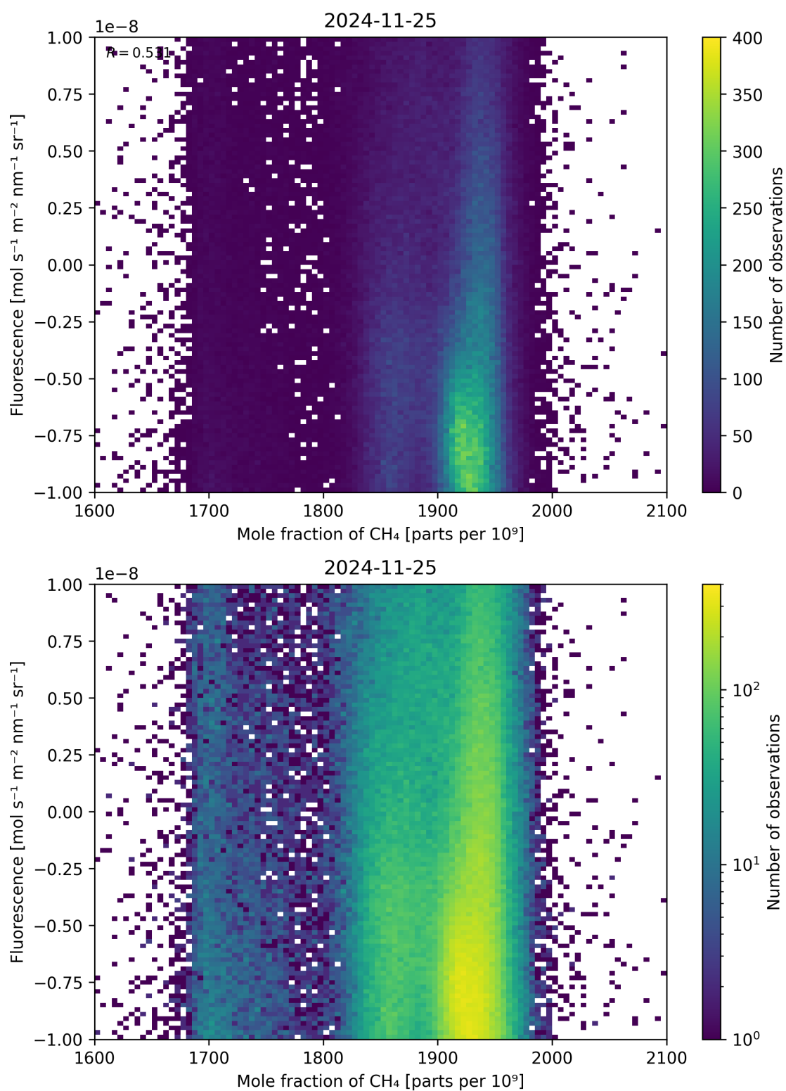
Figure 73: Scatter density plot of “Mole fraction of \text{CH}_4 ” against “Fluorescence” for 2024-11-25 to 2024-11-26.
