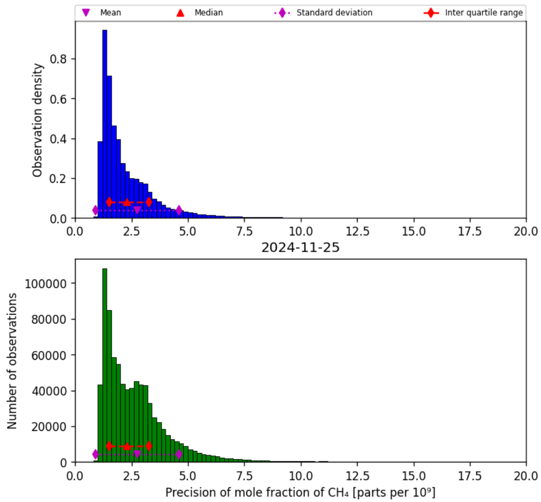
Figure 24: Histogram of “Precision of mole fraction of CH 4 ” for 2024-11-25 to 2024-11-26
