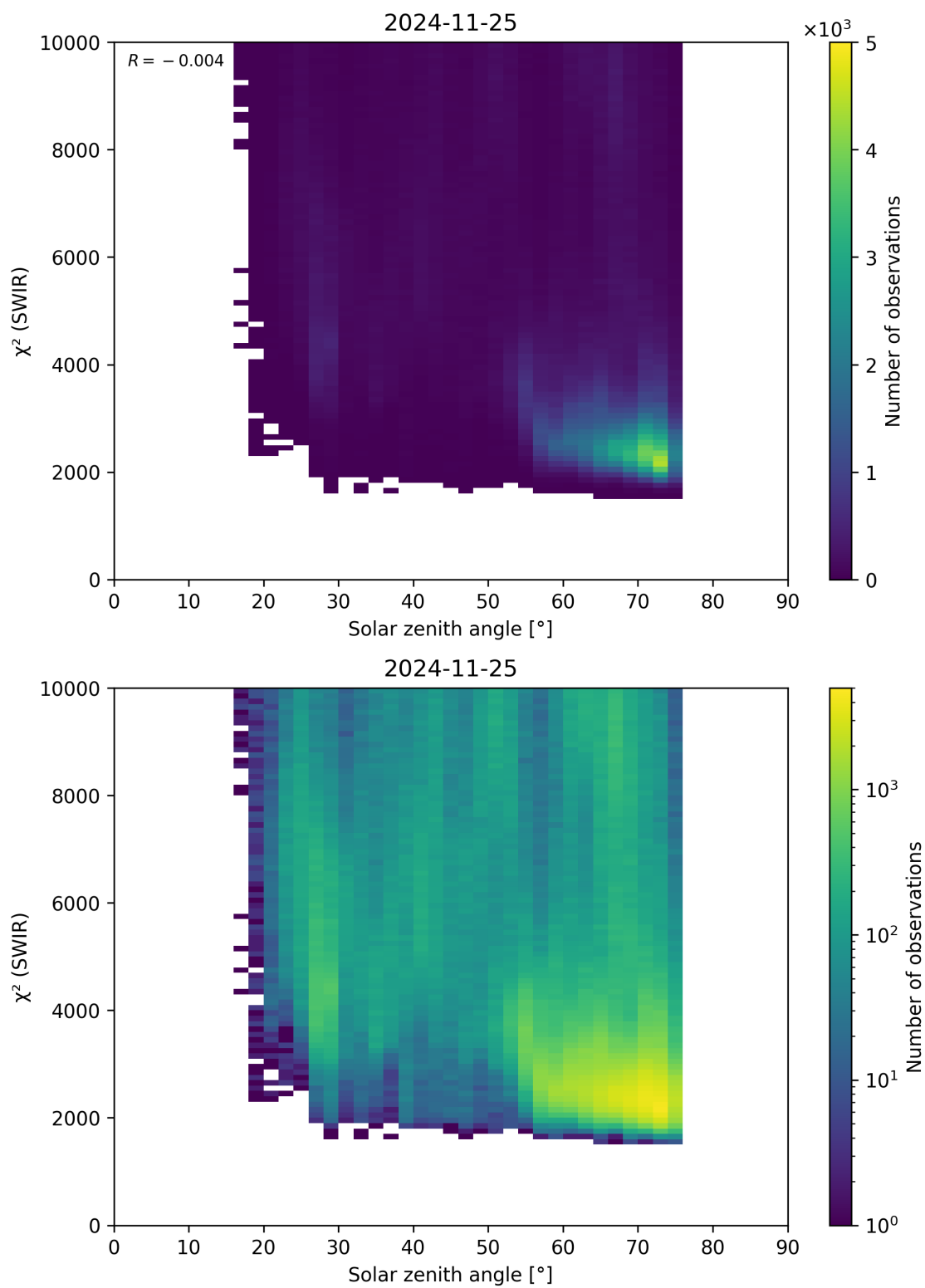
Figure 95: Scatter density plot of “Solar zenith angle” against “ \chi^2 (SWIR)” for 2024-11-25 to 2024-11-26.
