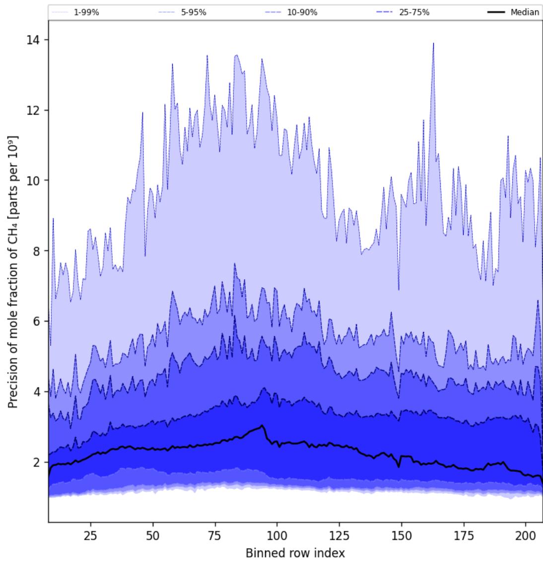
Figure 35: Along track statistics of “Precision of mole fraction of CH 4 ” for 2024-11-25 to 2024-11-26
