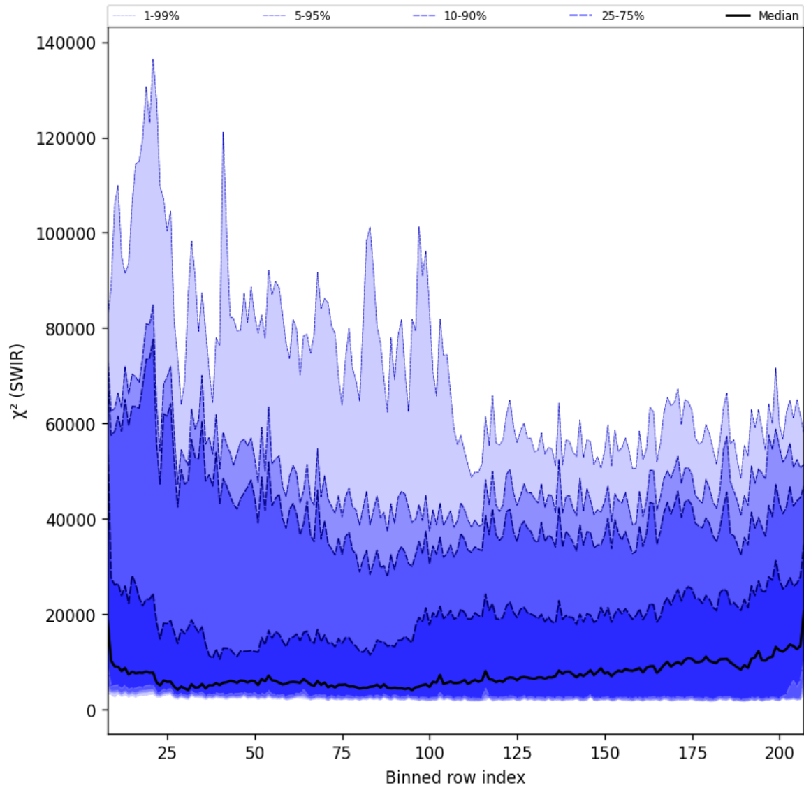
Figure 39: Along track statistics of “ \chi^2 (SWIR)” for 2024-11-25 to 2024-11-26
