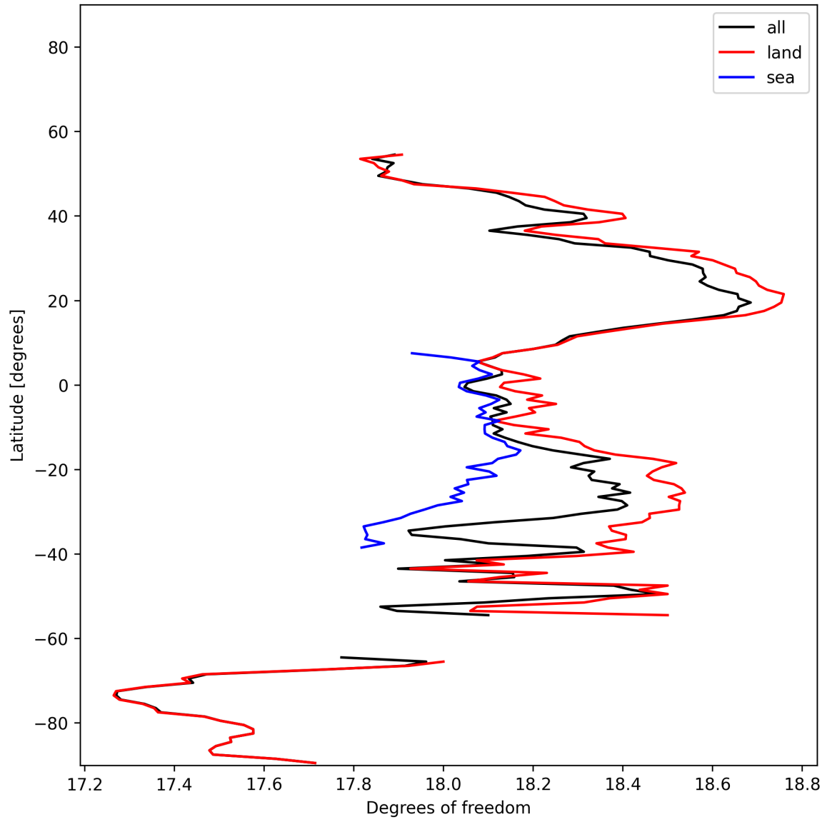
Figure 19: Zonal average of “Degrees of freedom” for 2024-11-25 to 2024-11-26.
