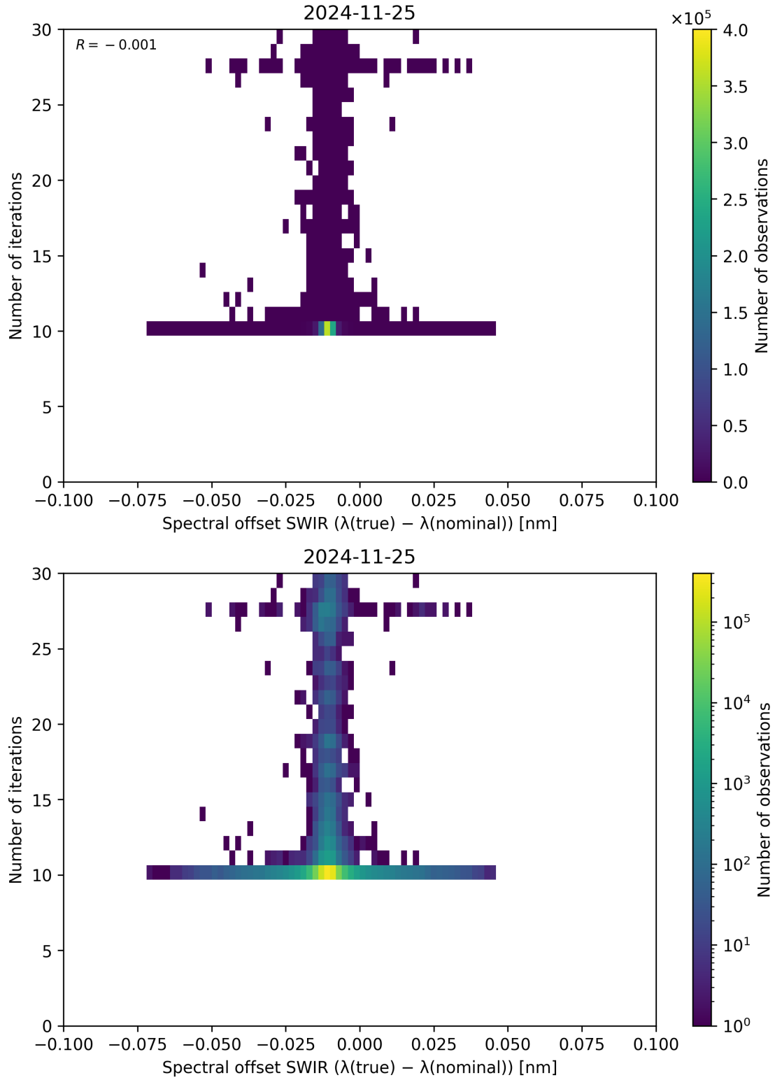
Figure 121: Scatter density plot of “Spectral offset SWIR ( \lambda_{\text{true}} - \lambda_{\text{nominal}} )” against “Number of iterations” for 2024-11-25 to 2024-11-26.
