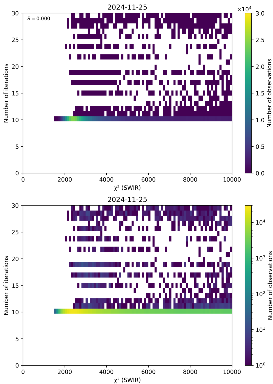
Figure 50: Scatter density plot of “ \chi^2 (SWIR)” against “Number of iterations” for 2024-11-25 to 2024-11-26.
