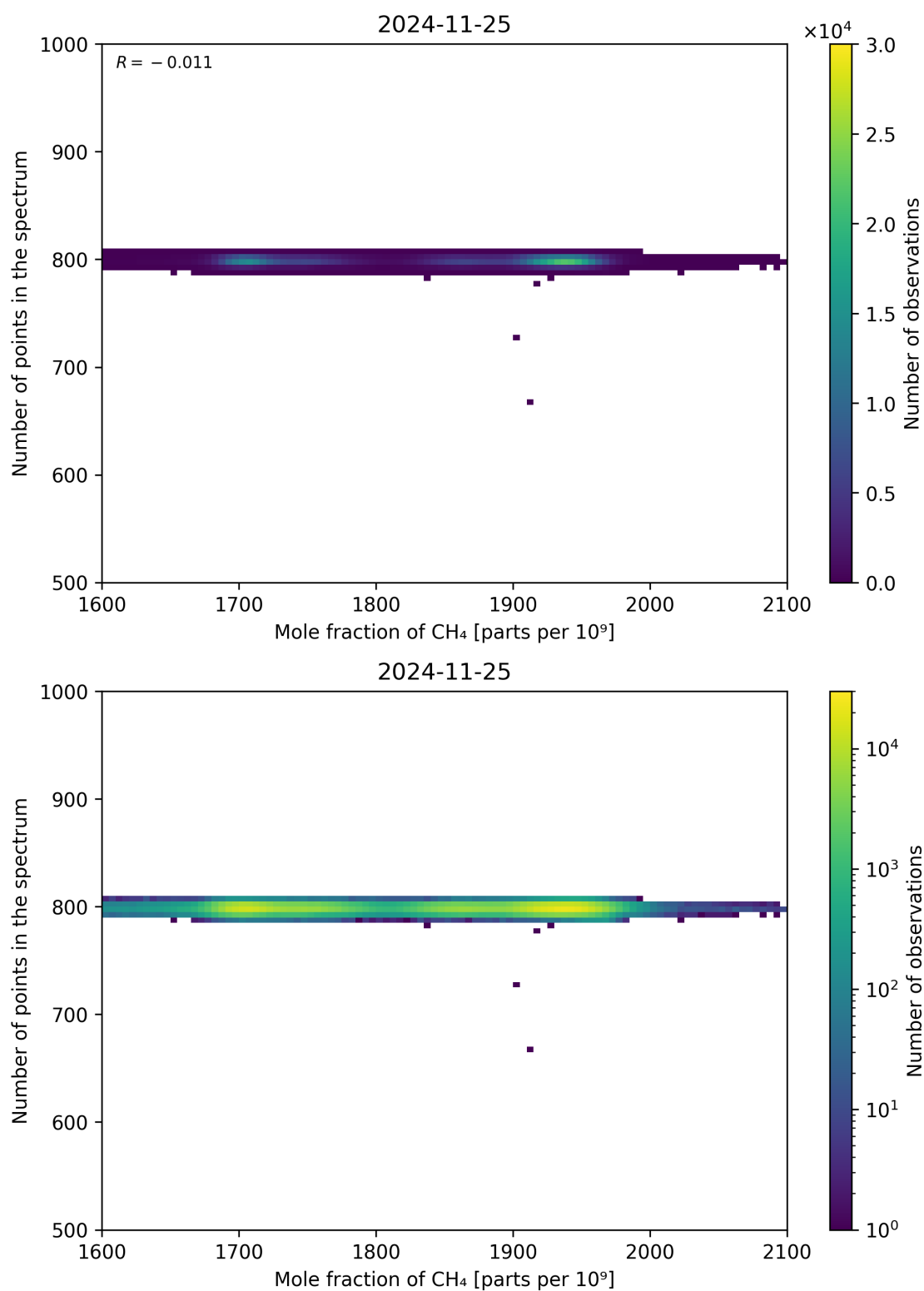
Figure 77: Scatter density plot of “Mole fraction of CH 4 ” against “Number of points in the spectrum” for 2024-11-25 to 2024-11-26.
