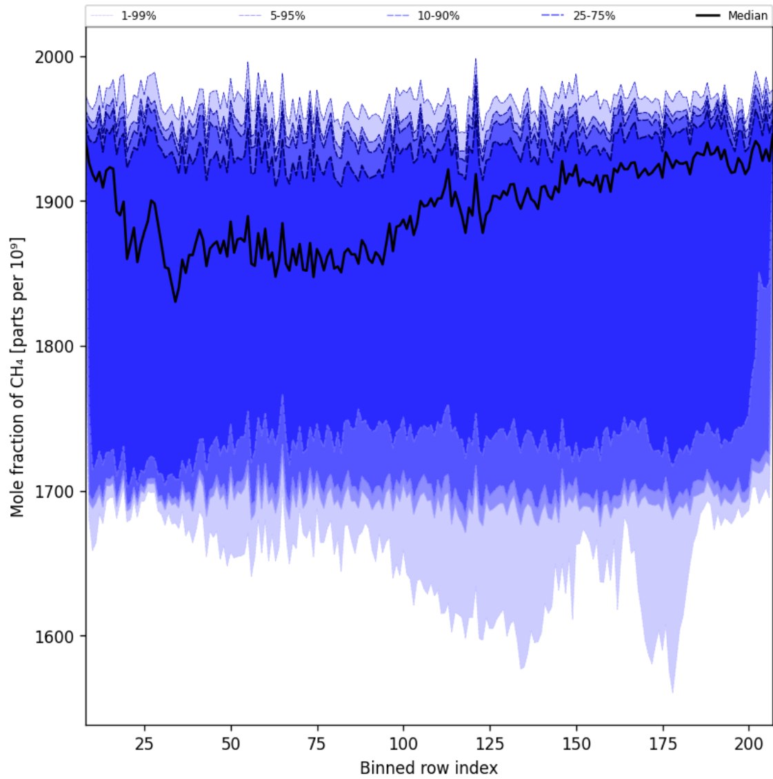
Figure 34: Along track statistics of “Mole fraction of CH 4 ” for 2024-11-25 to 2024-11-26
