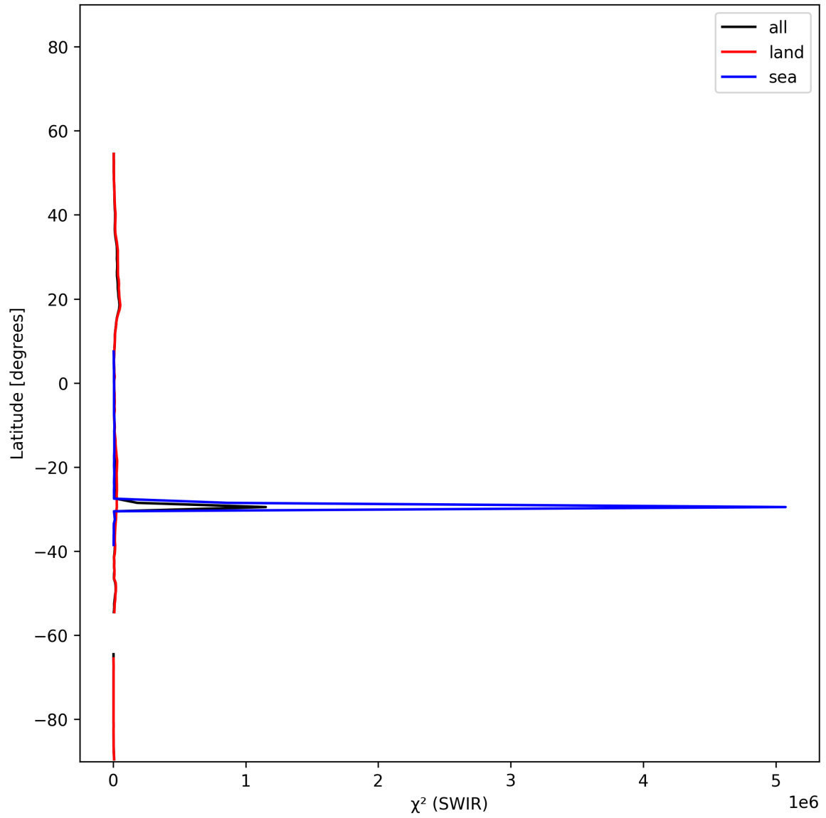
Figure 17: Zonal average of “ \chi^2 (SWIR)” for 2024-11-25 to 2024-11-26.
