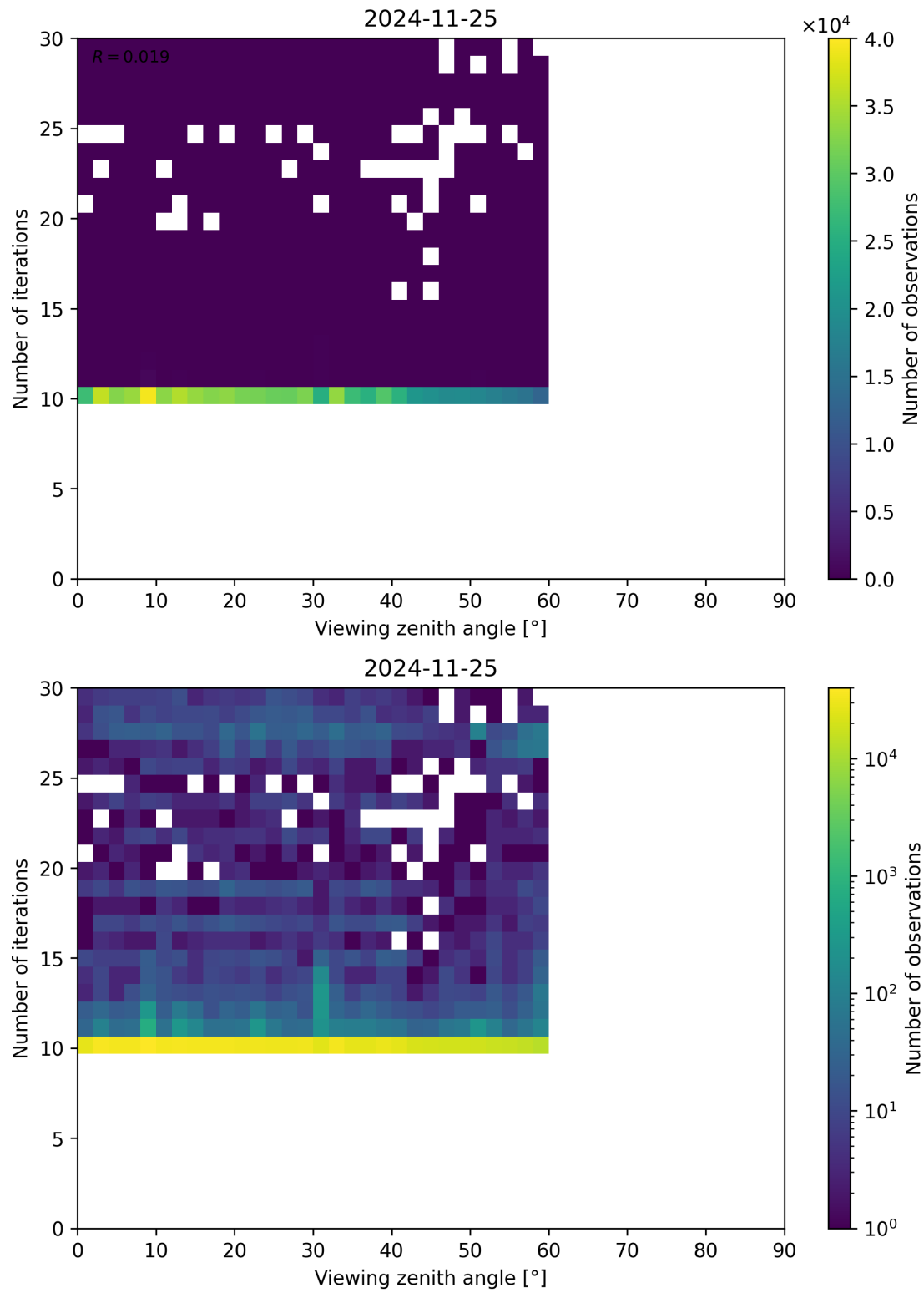
Figure 113: Scatter density plot of “Viewing zenith angle” against “Number of iterations” for 2024-11-25 to 2024-11-26.
