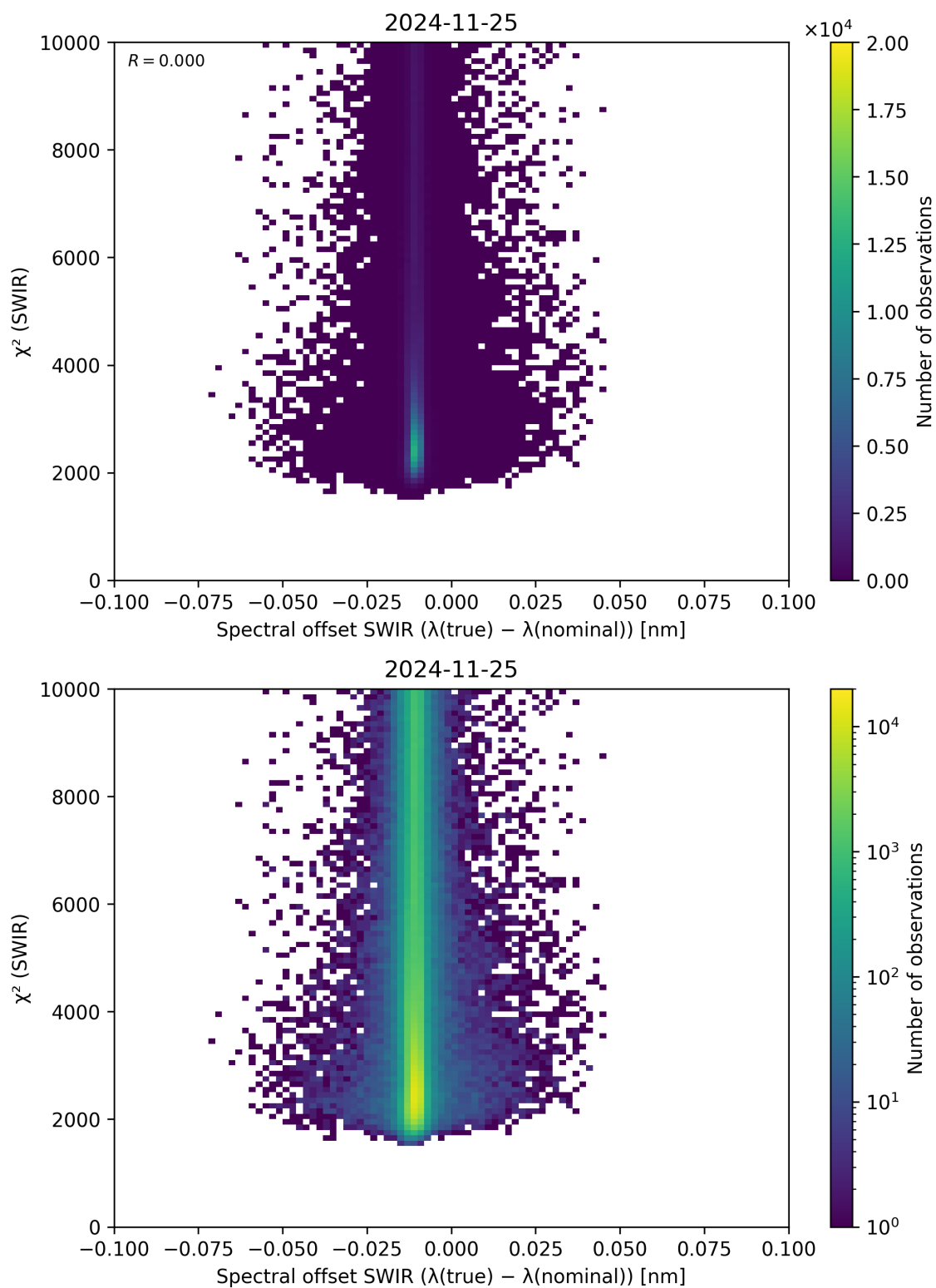
Figure 118: Scatter density plot of “Spectral offset SWIR ( \lambda_{\text{true}} - \lambda_{\text{nominal}} )” against “ \chi^2 (SWIR)” for 2024-11-25 to 2024-11-26.
