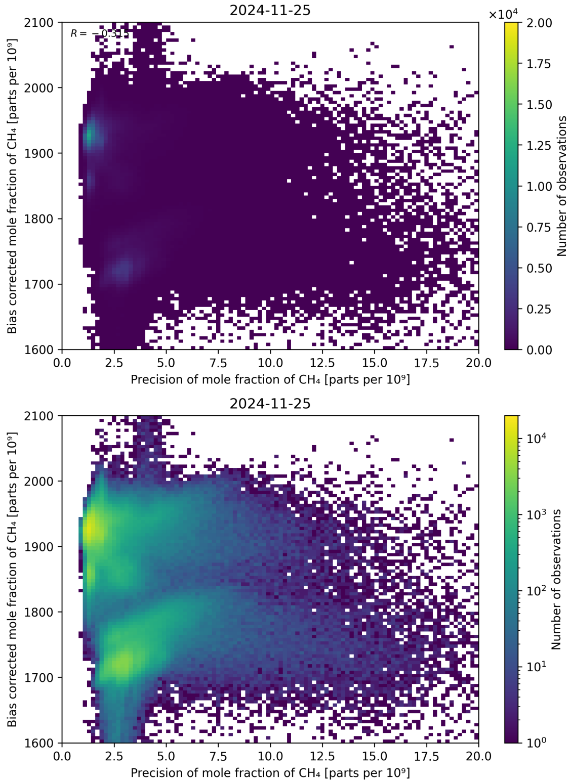
Figure 82: Scatter density plot of “Precision of mole fraction of CH 4 ” against “Bias corrected mole fraction of CH 4 ” for 2024-11-25 to 2024-11-26.
