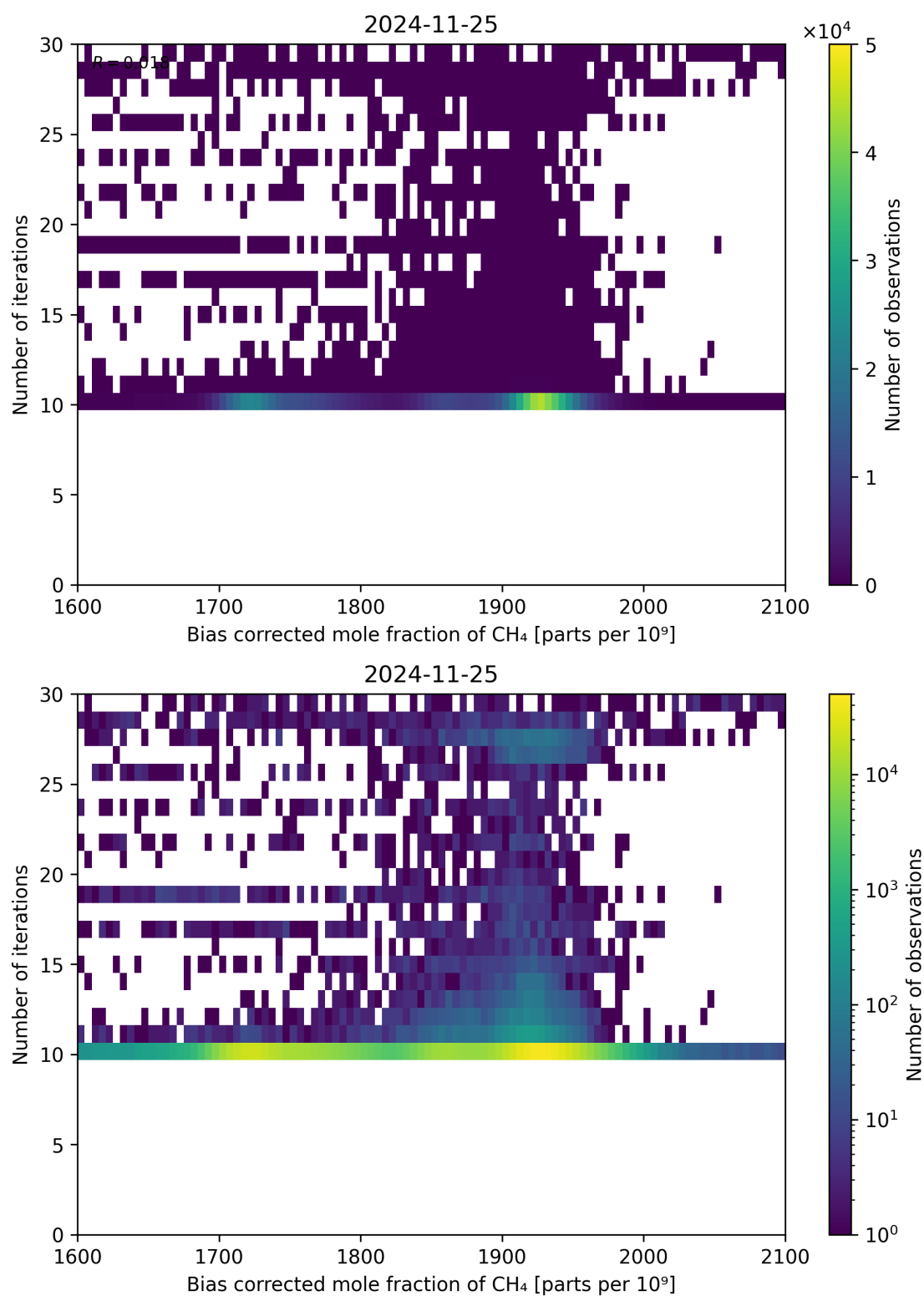
Figure 67: Scatter density plot of “Bias corrected mole fraction of CH 4 ” against “Number of iterations” for 2024-11-25 to 2024-11-26.
