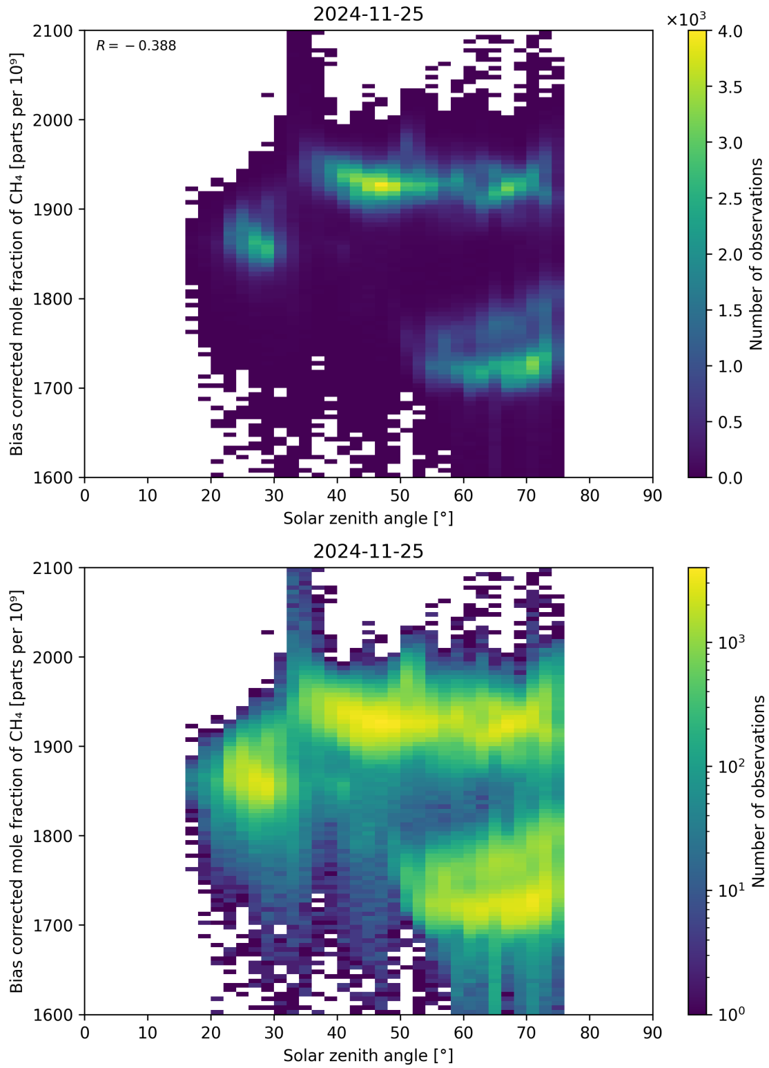
Figure 100: Scatter density plot of “Solar zenith angle” against “Bias corrected mole fraction of CH 4 ” for 2024-11-25 to 2024-11-26.
