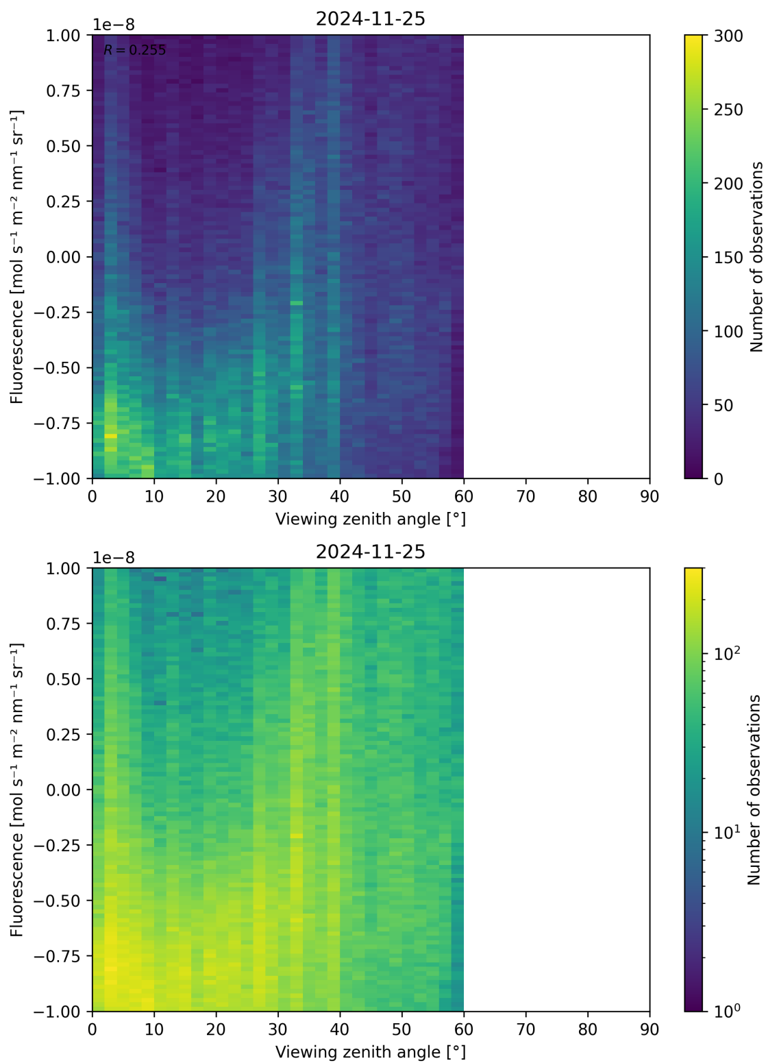
Figure 108: Scatter density plot of “Viewing zenith angle” against “Fluorescence” for 2024-11-25 to 2024-11-26.
