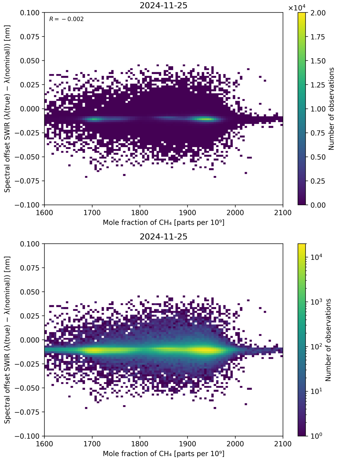
Figure 86: Scatter density plot of “Mole fraction of CH 4 ” against “Spectral offset SWIR ( \lambda_{\text{true}} - \lambda_{\text{nominal}} )” for 2024-11-25 to 2024-11-26.
