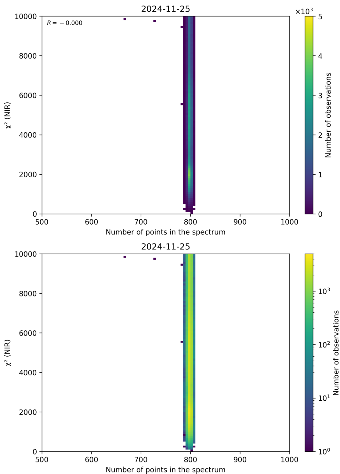
Figure 88: Scatter density plot of “Number of points in the spectrum” against “ \chi^2 (NIR)” for 2024-11-25 to 2024-11-26.
