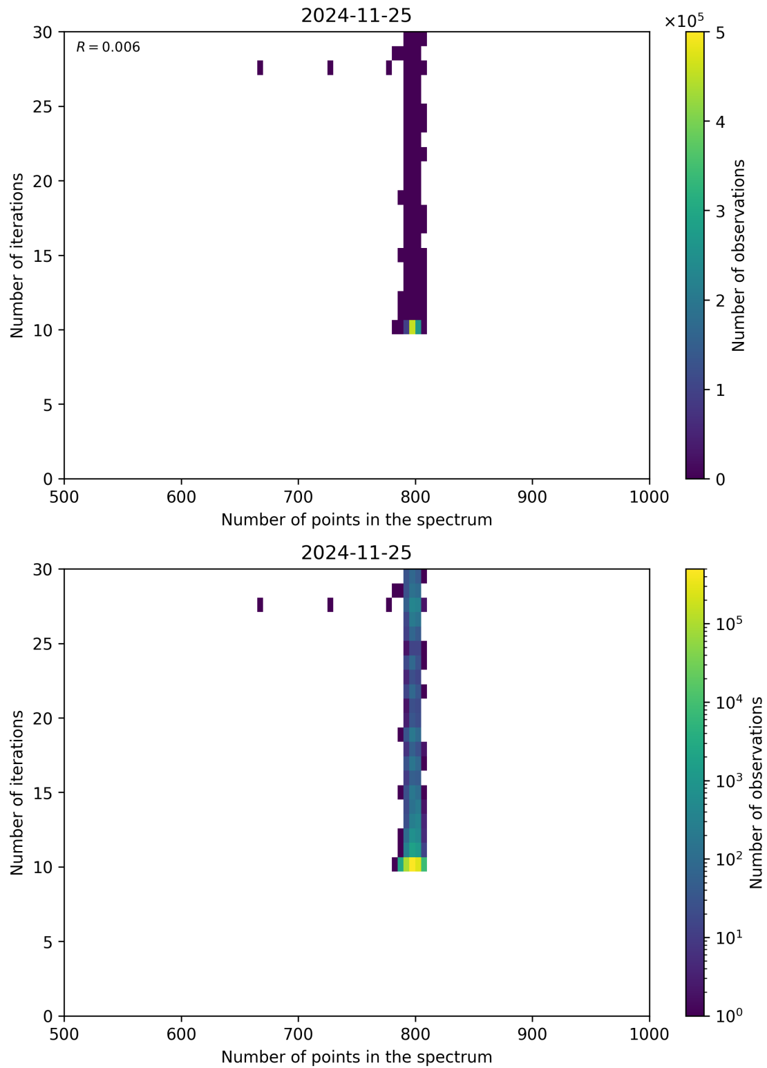
Figure 92: Scatter density plot of “Number of points in the spectrum” against “Number of iterations” for 2024-11-25 to 2024-11-26.
