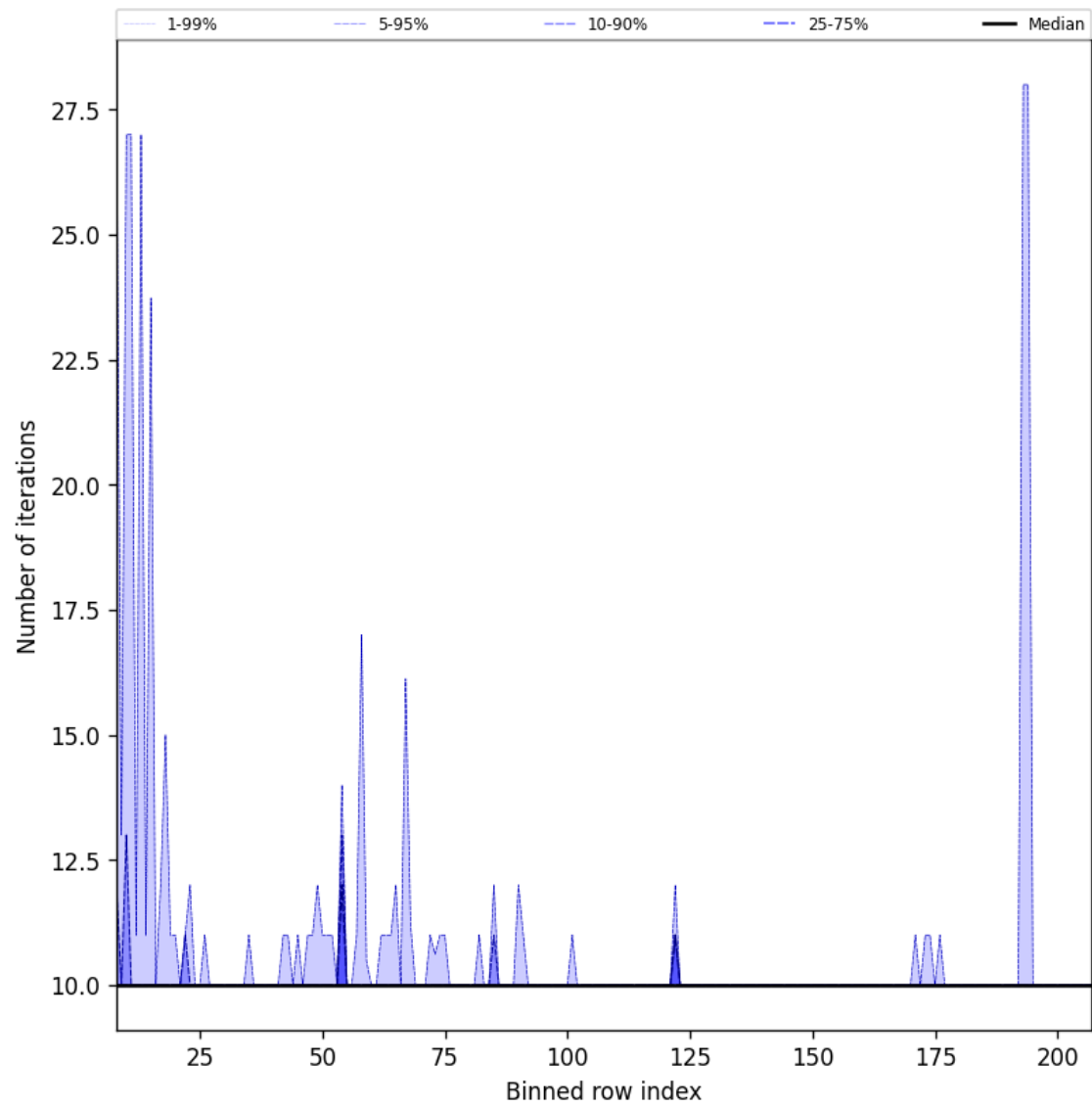
Figure 42: Along track statistics of “Number of iterations” for 2024-11-25 to 2024-11-26
