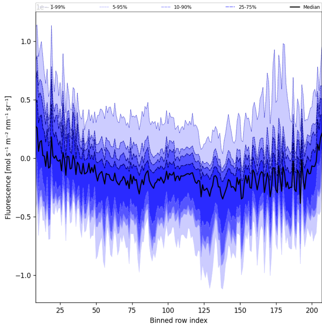
Figure 43: Along track statistics of “Fluorescence” for 2024-11-25 to 2024-11-26
