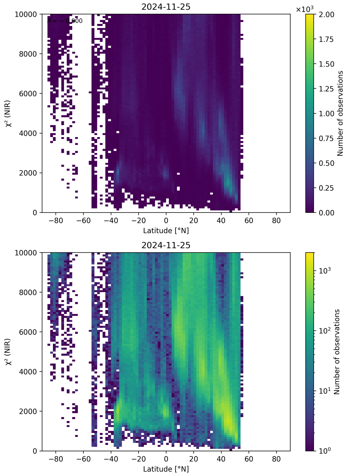
Figure 53: Scatter density plot of “Latitude” against “ \chi^2 (NIR)” for 2024-11-25 to 2024-11-26.
