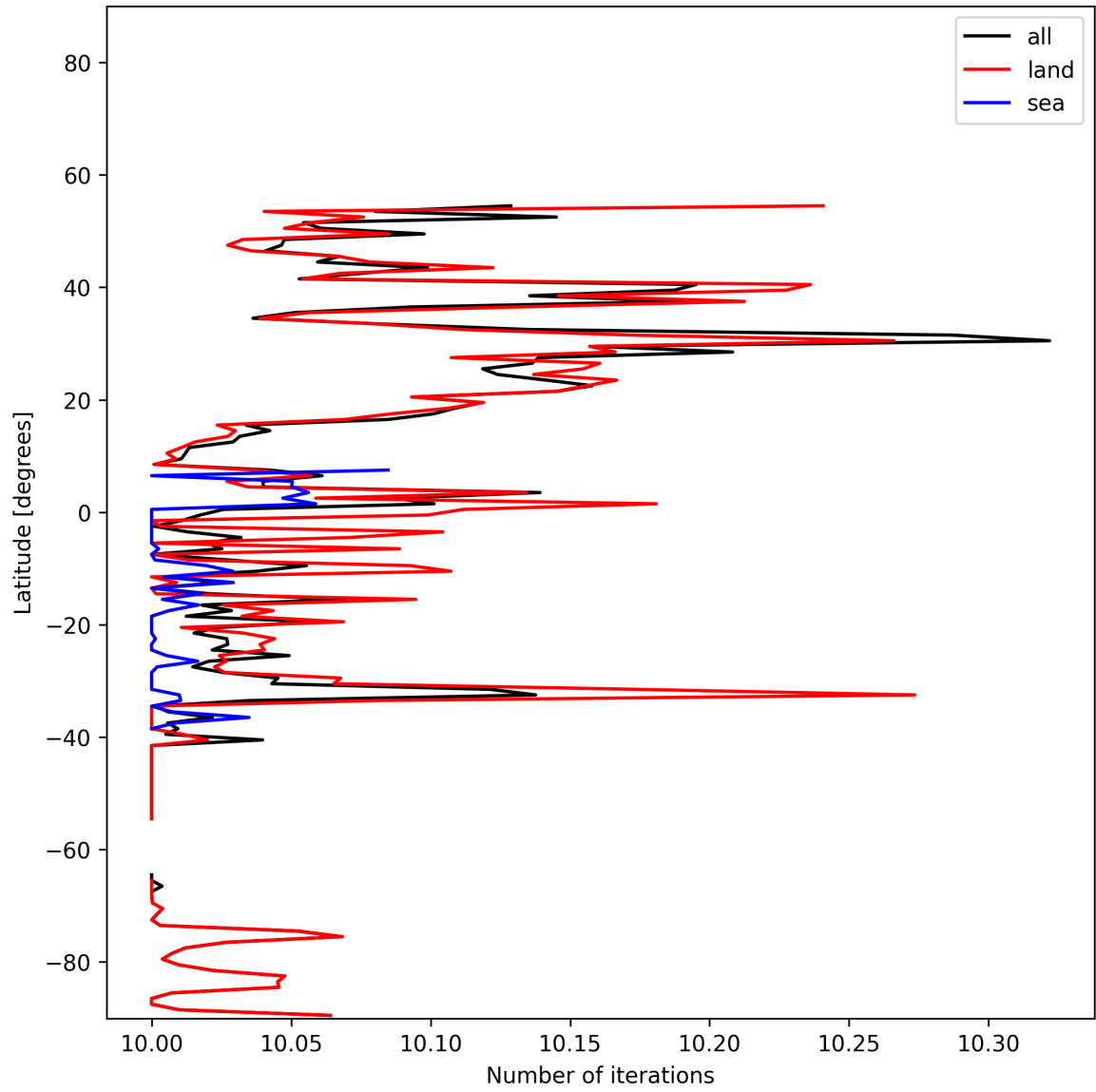
Figure 20: Zonal average of “Number of iterations” for 2024-11-25 to 2024-11-26.
