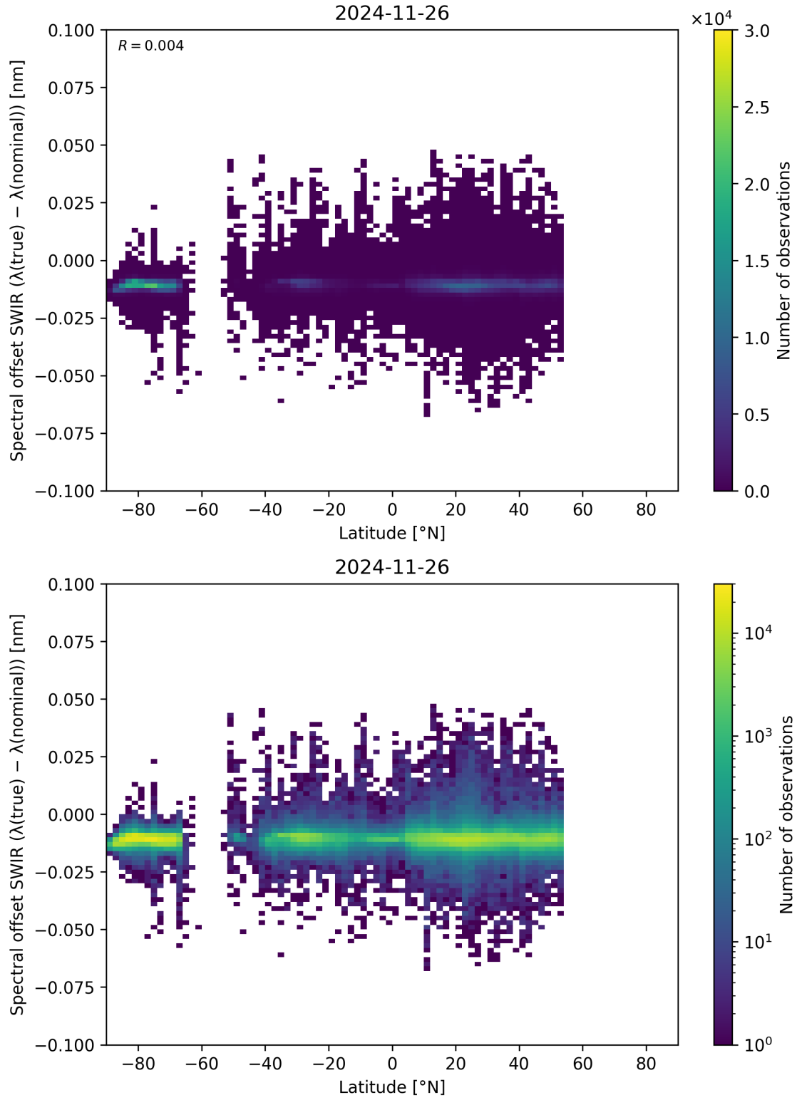
Figure 62: Scatter density plot of “Latitude” against “Spectral offset SWIR ( \lambda_{\text{true}} - \lambda_{\text{nominal}} )” for 2024-11-25 to 2024-11-27.
