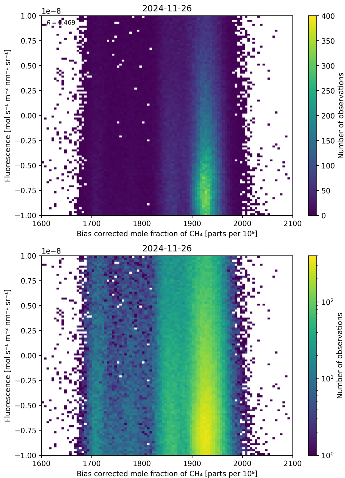
Figure 66: Scatter density plot of “Bias corrected mole fraction of \text{CH}_4 ” against “Fluorescence” for 2024-11-25 to 2024-11-27.
