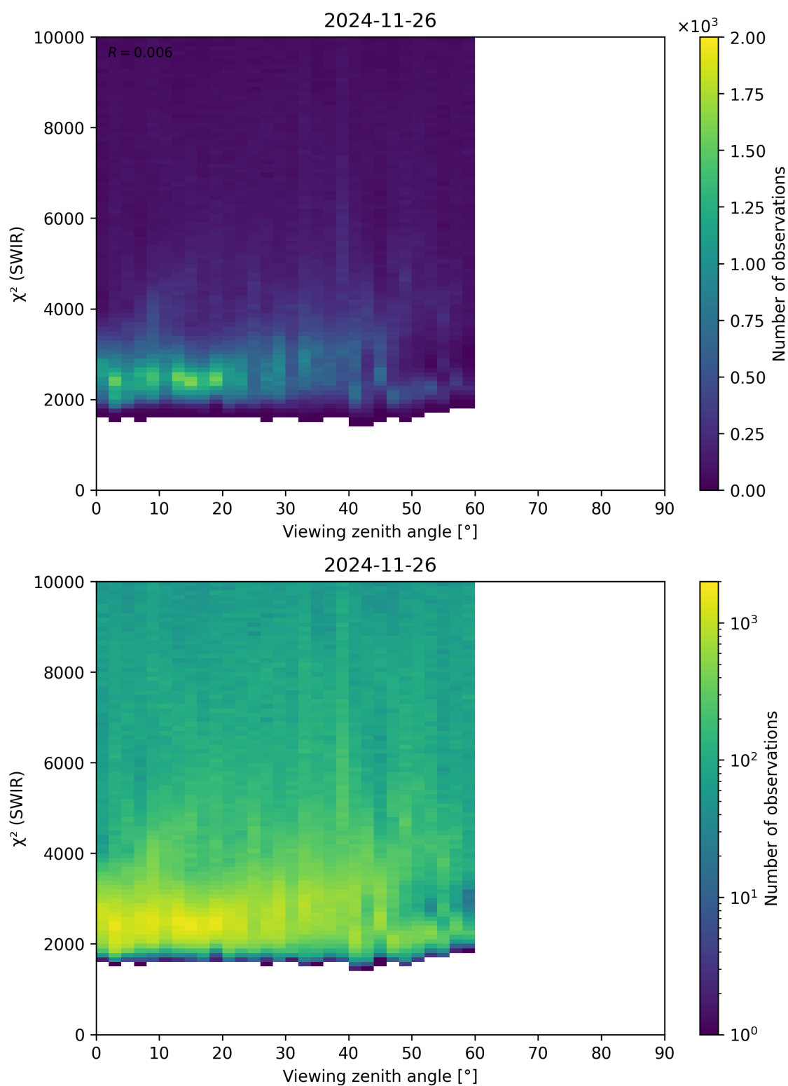
Figure 106: Scatter density plot of “Viewing zenith angle” against “ \chi^2 (SWIR)” for 2024-11-25 to 2024-11-27.
