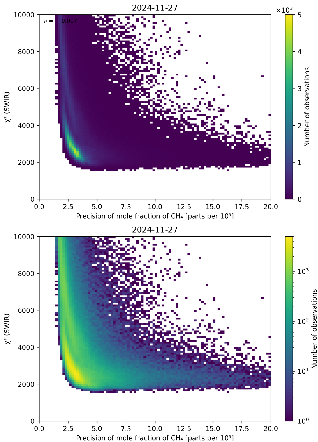
Figure 79: Scatter density plot of “Precision of mole fraction of \text{CH}_4 ” against “ \chi^2 (SWIR)” for 2024-11-26 to 2024-11-28.
