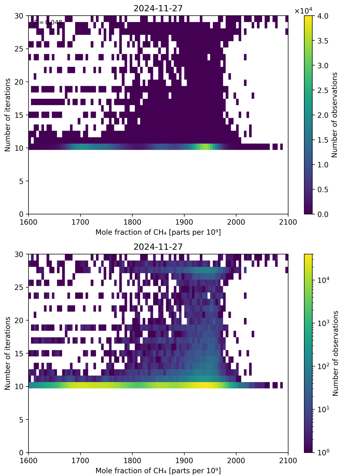
Figure 76: Scatter density plot of “Mole fraction of CH 4 ” against “Number of iterations” for 2024-11-26 to 2024-11-28.
