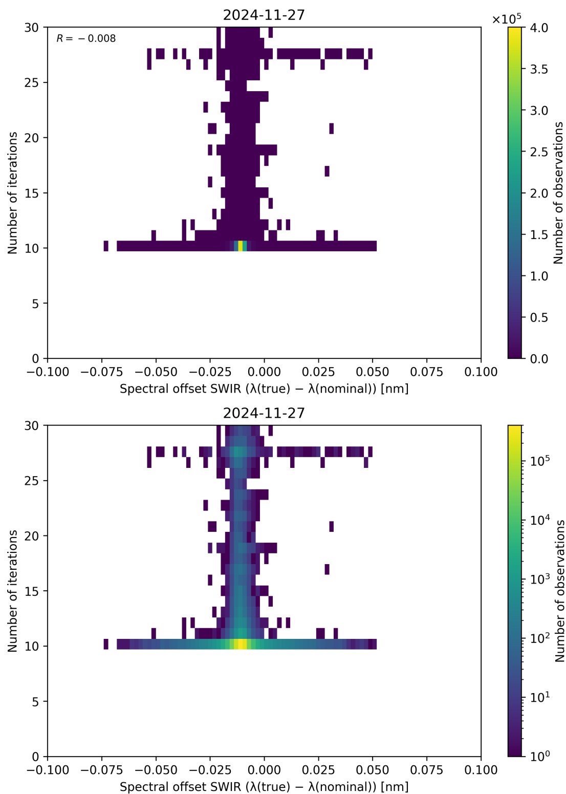
Figure 121: Scatter density plot of “Spectral offset SWIR ( \lambda_{\text{true}} - \lambda_{\text{nominal}} )” against “Number of iterations” for 2024-11-26 to 2024-11-28.
