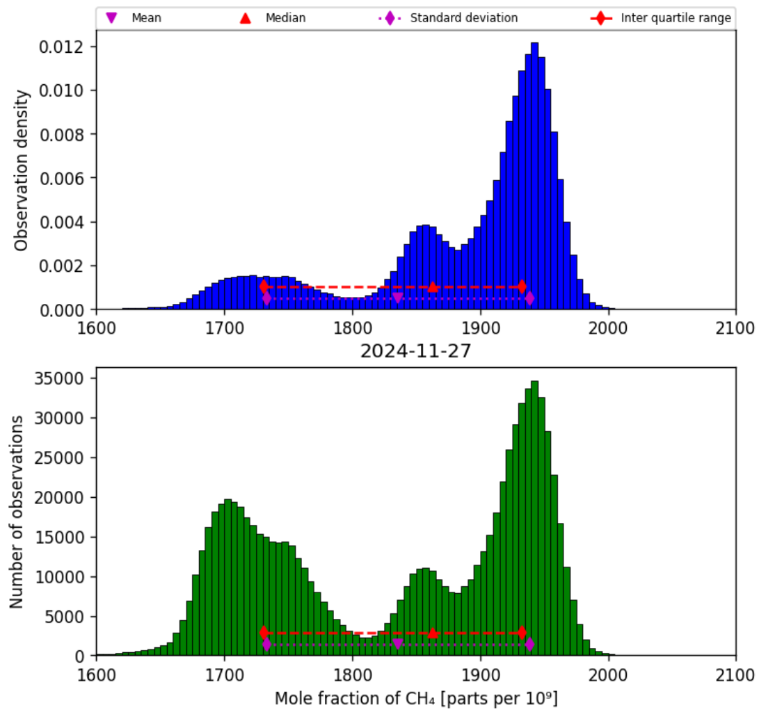
Figure 23: Histogram of “Mole fraction of CH 4 ” for 2024-11-26 to 2024-11-28
