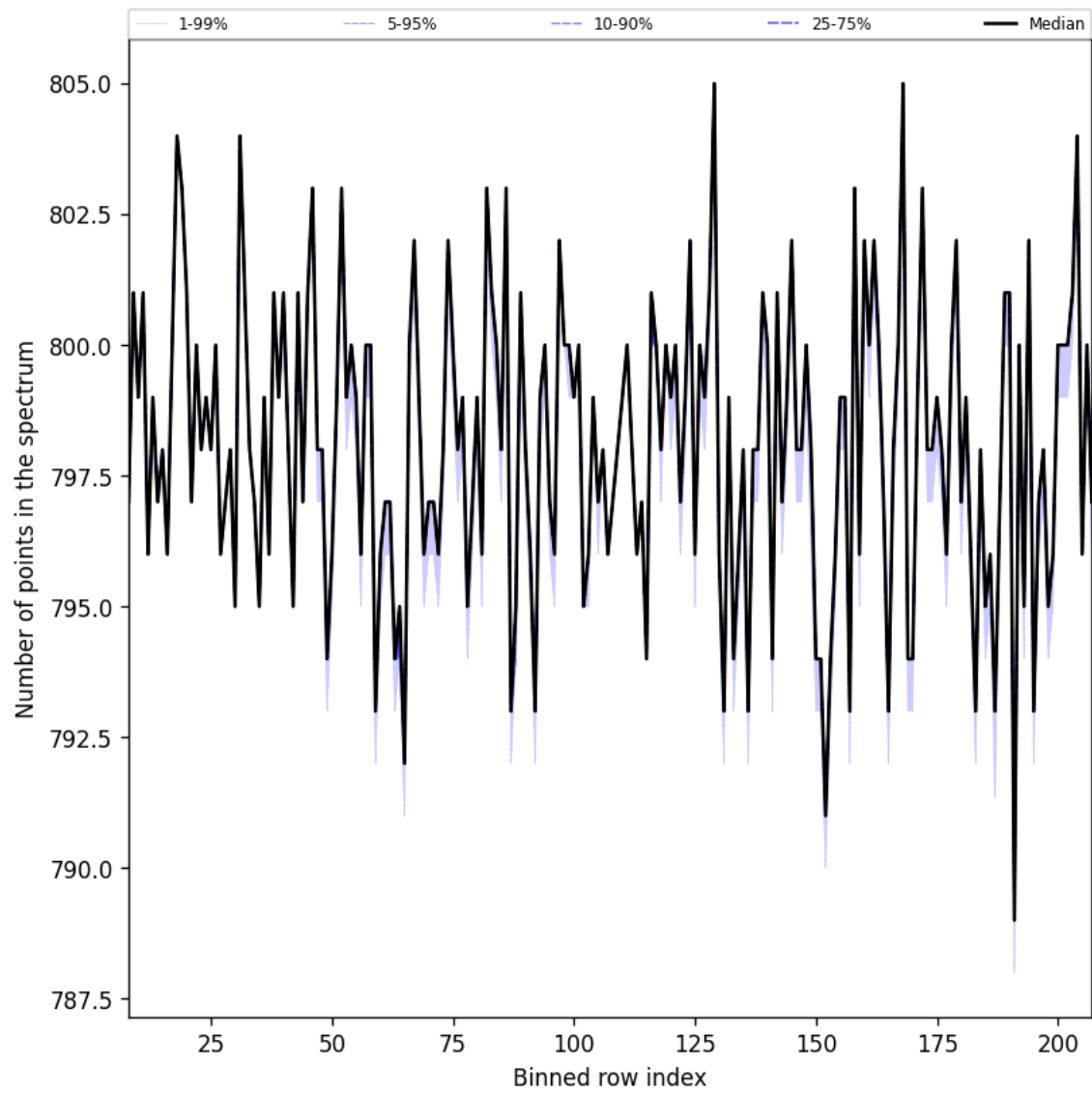
Figure 37: Along track statistics of “Number of points in the spectrum” for 2024-11-26 to 2024-11-28
