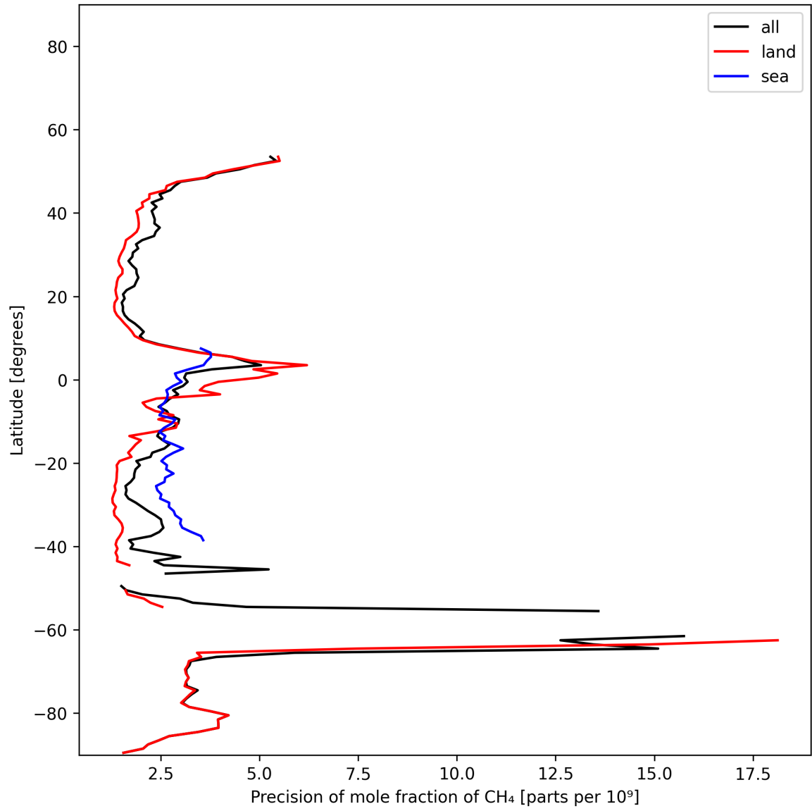
Figure 13: Zonal average of “Precision of mole fraction of CH 4 ” for 2024-11-26 to 2024-11-28.
