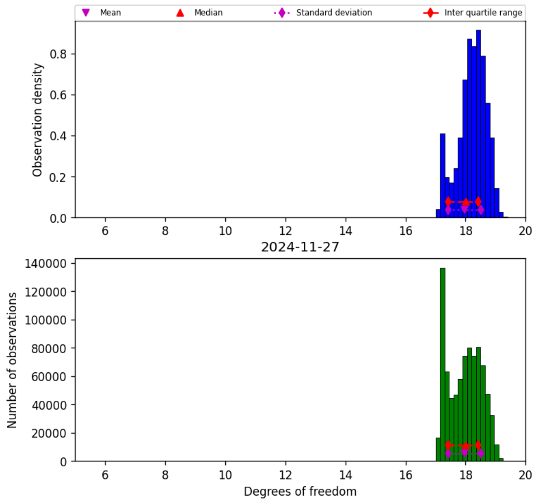
Figure 30: Histogram of “Degrees of freedom” for 2024-11-26 to 2024-11-28
