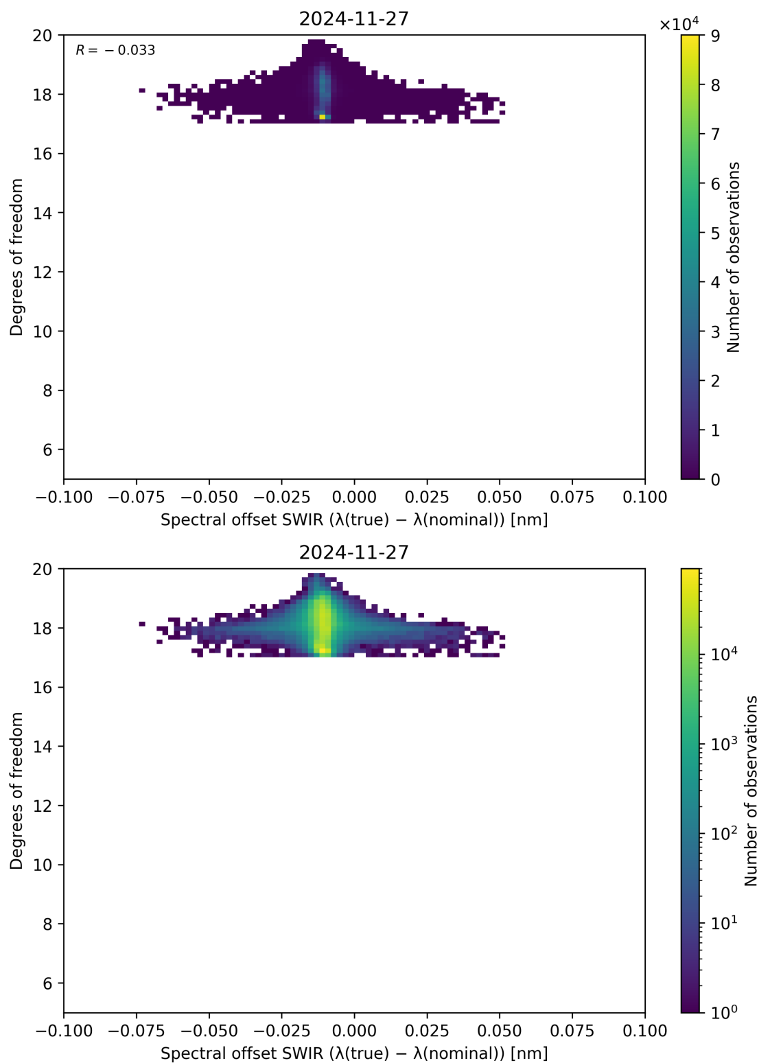
Figure 119: Scatter density plot of “Spectral offset SWIR ( \lambda_{\text{true}} - \lambda_{\text{nominal}} )” against “Degrees of freedom” for 2024-11-26 to 2024-11-28.
