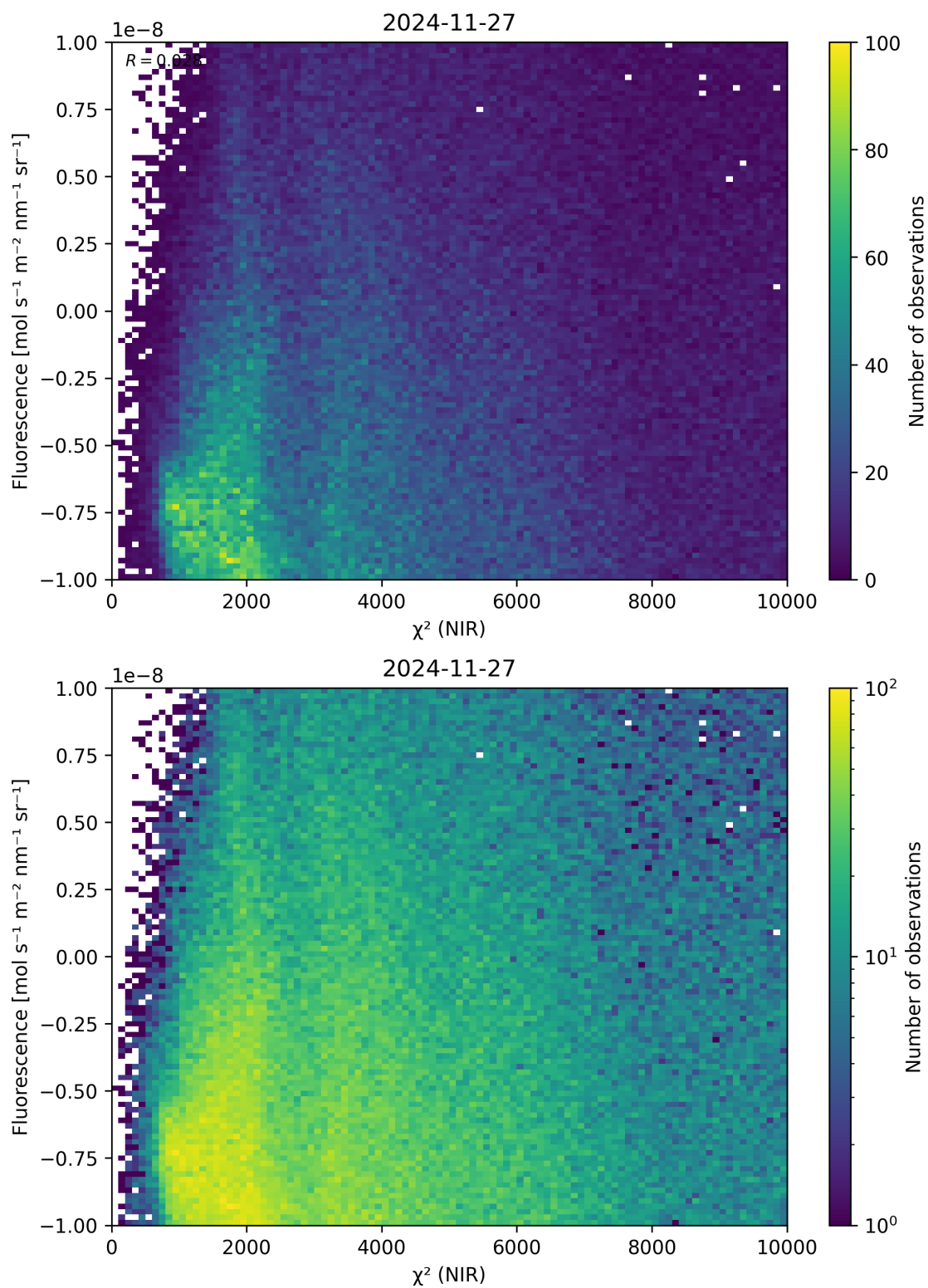
Figure 45: Scatter density plot of “ \chi^2 (NIR)” against “Fluorescence” for 2024-11-26 to 2024-11-28.
