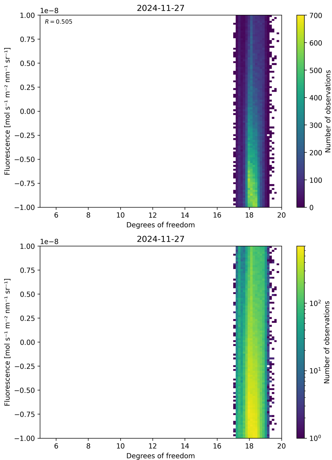
Figure 51: Scatter density plot of “Degrees of freedom” against “Fluorescence” for 2024-11-26 to 2024-11-28.
