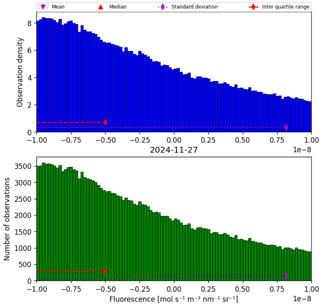
Figure 32: Histogram of “Fluorescence” for 2024-11-26 to 2024-11-28
