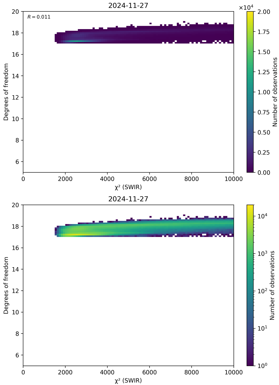
Figure 48: Scatter density plot of “ \chi^2 (SWIR)” against “Degrees of freedom” for 2024-11-26 to 2024-11-28.
