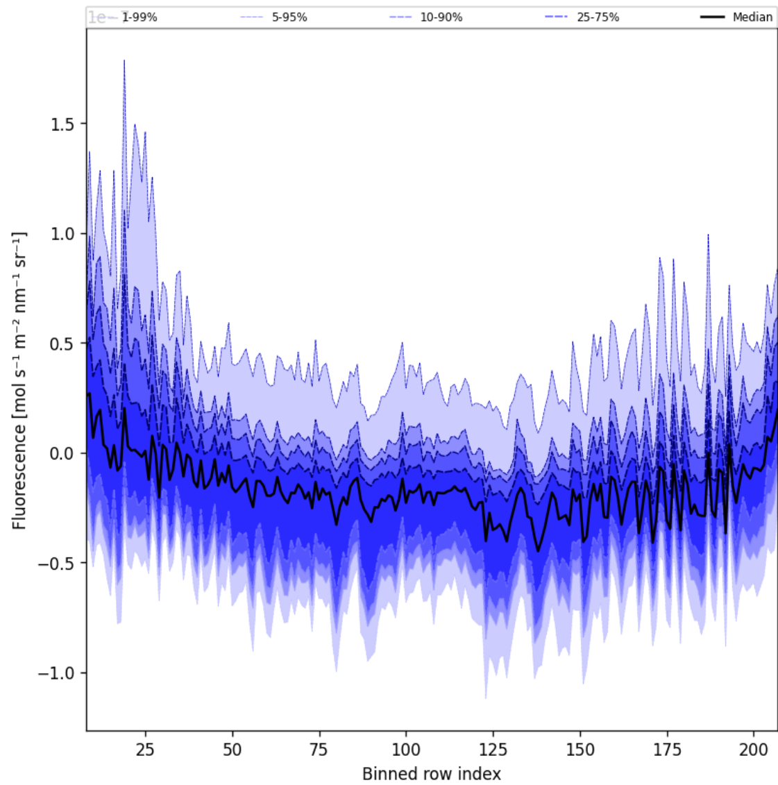
Figure 43: Along track statistics of “Fluorescence” for 2024-11-26 to 2024-11-28
