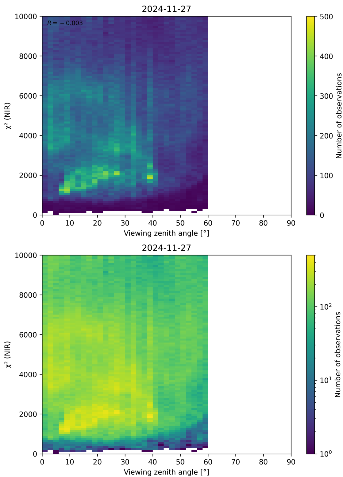
Figure 105: Scatter density plot of “Viewing zenith angle” against “ \chi^2 (NIR)” for 2024-11-26 to 2024-11-28.
