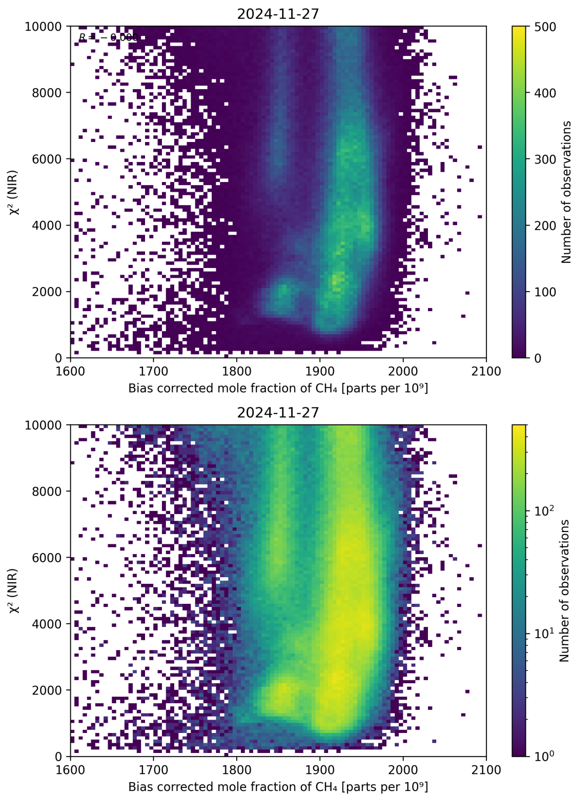
Figure 63: Scatter density plot of “Bias corrected mole fraction of \text{CH}_4 ” against “ \chi^2 (NIR)” for 2024-11-26 to 2024-11-28.
