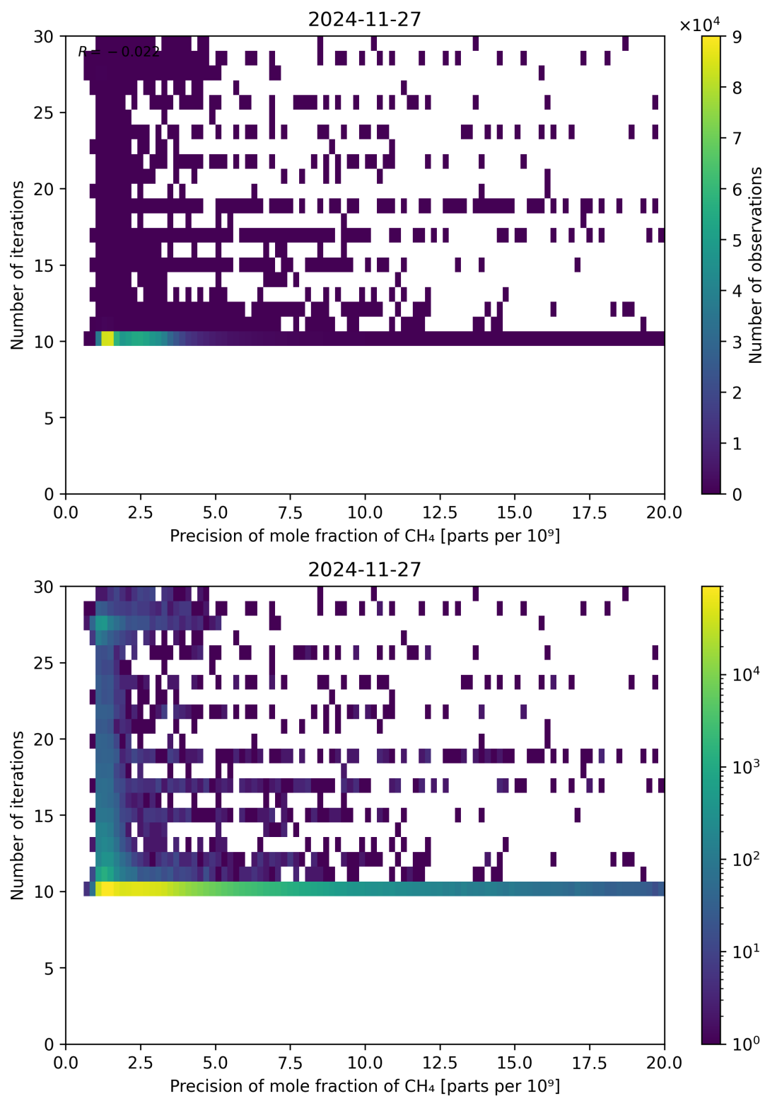
Figure 83: Scatter density plot of “Precision of mole fraction of CH 4 ” against “Number of iterations” for 2024-11-26 to 2024-11-28.
