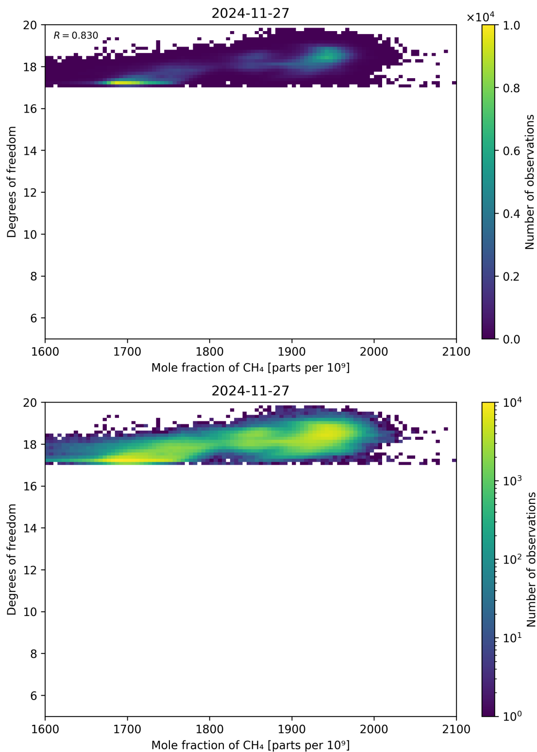
Figure 72: Scatter density plot of “Mole fraction of CH 4 ” against “Degrees of freedom” for 2024-11-26 to 2024-11-28.
