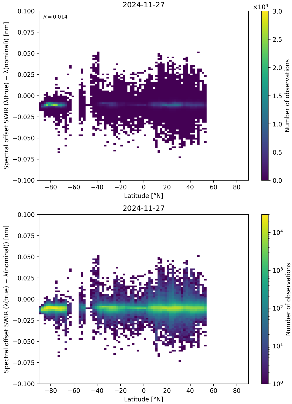
Figure 62: Scatter density plot of “Latitude” against “Spectral offset SWIR ( \lambda_{\text{true}} - \lambda_{\text{nominal}} )” for 2024-11-26 to 2024-11-28.
