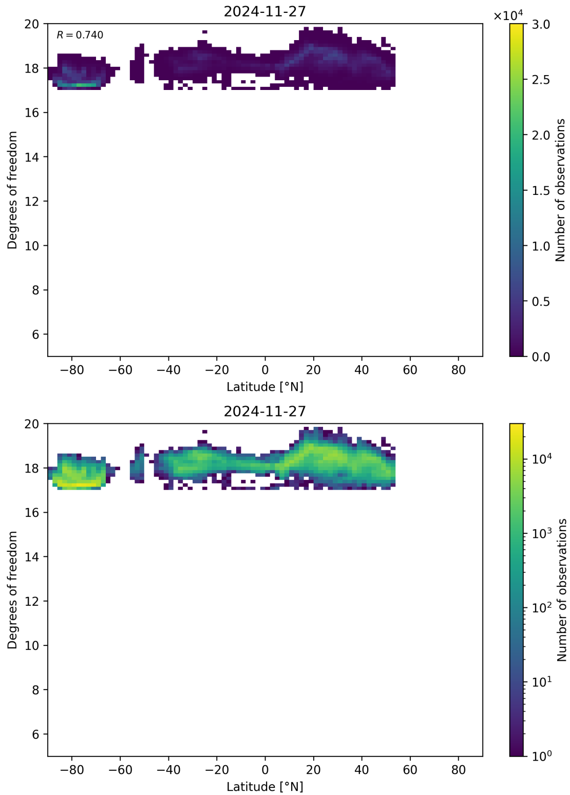
Figure 55: Scatter density plot of “Latitude” against “Degrees of freedom” for 2024-11-26 to 2024-11-28.
