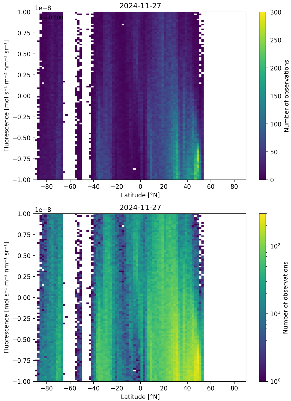
Figure 56: Scatter density plot of “Latitude” against “Fluorescence” for 2024-11-26 to 2024-11-28.
