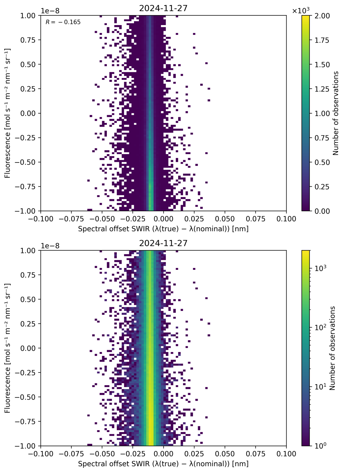
Figure 120: Scatter density plot of “Spectral offset SWIR ( \lambda_{\text{true}} - \lambda_{\text{nominal}} )” against “Fluorescence” for 2024-11-26 to 2024-11-28.
