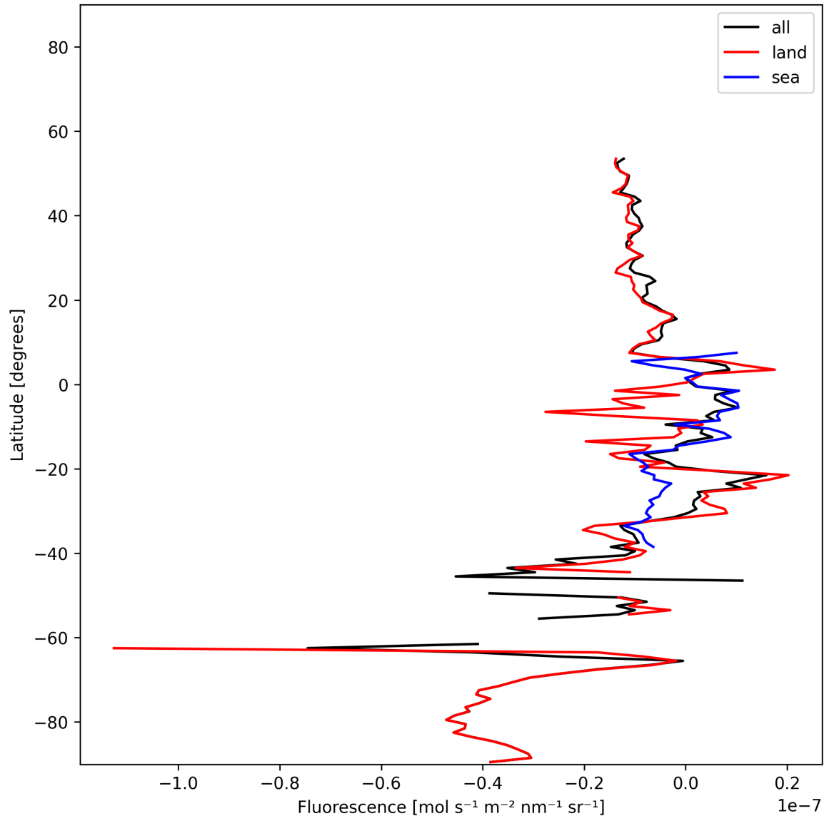
Figure 21: Zonal average of “Fluorescence” for 2024-11-26 to 2024-11-28.
