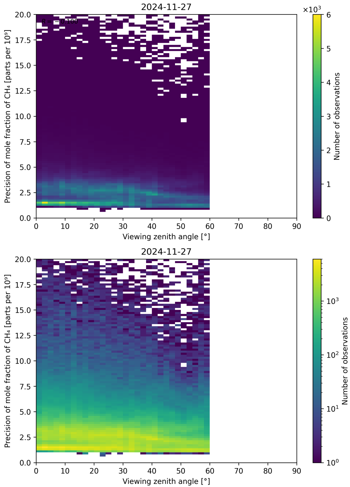
Figure 112: Scatter density plot of “Viewing zenith angle” against “Precision of mole fraction of CH 4 ” for 2024-11-26 to 2024-11-28.
