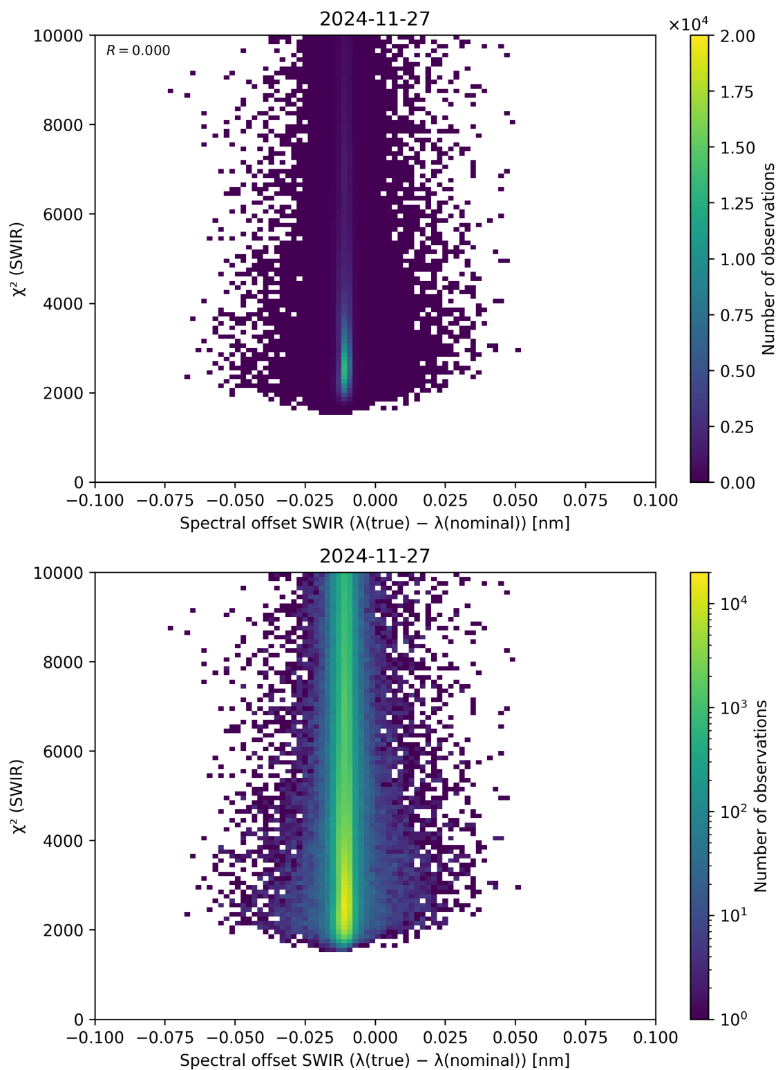
Figure 118: Scatter density plot of “Spectral offset SWIR ( \lambda_{\text{true}} - \lambda_{\text{nominal}} )” against “ \chi^2 (SWIR)” for 2024-11-26 to 2024-11-28.
