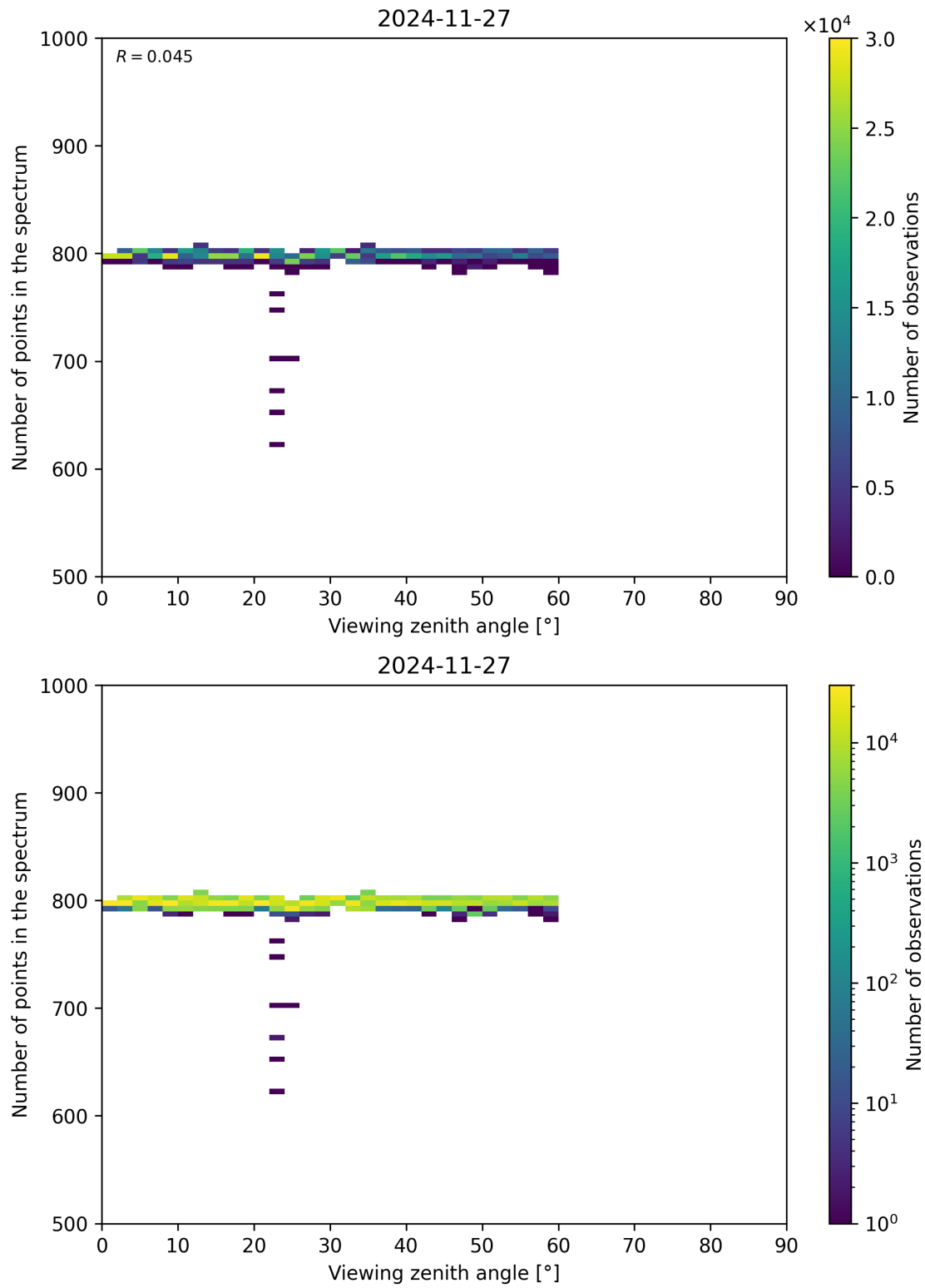
Figure 114: Scatter density plot of “Viewing zenith angle” against “Number of points in the spectrum” for 2024-11-26 to 2024-11-28.
