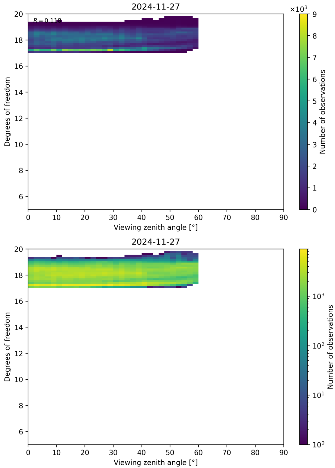
Figure 107: Scatter density plot of “Viewing zenith angle” against “Degrees of freedom” for 2024-11-26 to 2024-11-28.
