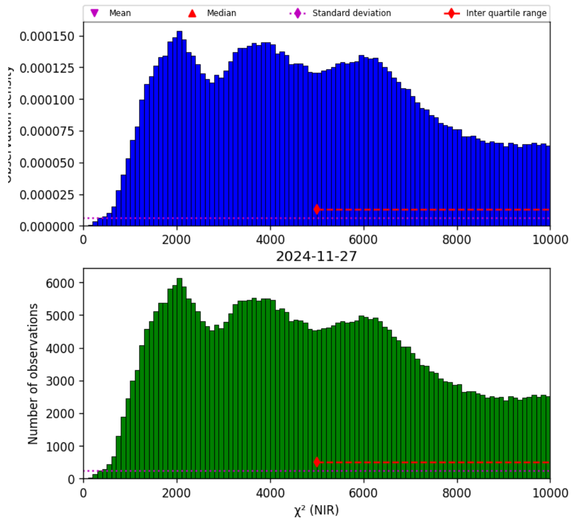
Figure 29: Histogram of “ \chi^2 (NIR)” for 2024-11-26 to 2024-11-28
