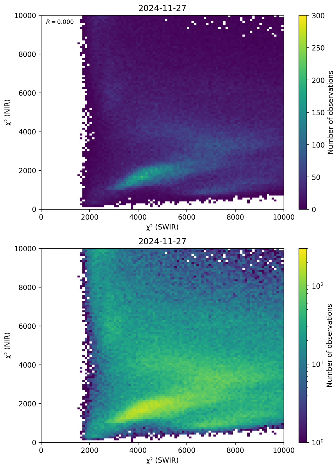
Figure 47: Scatter density plot of “ \chi^2 (SWIR)” against “ \chi^2 (NIR)” for 2024-11-26 to 2024-11-28.
