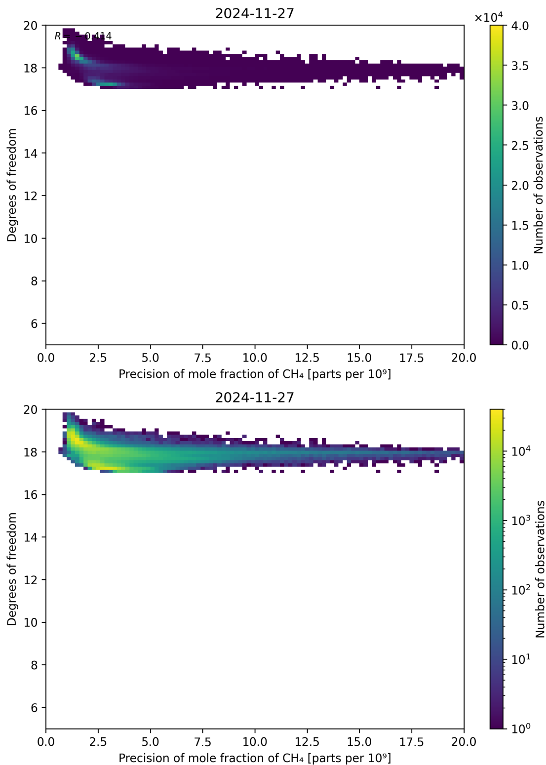
Figure 80: Scatter density plot of “Precision of mole fraction of CH 4 ” against “Degrees of freedom” for 2024-11-26 to 2024-11-28.
