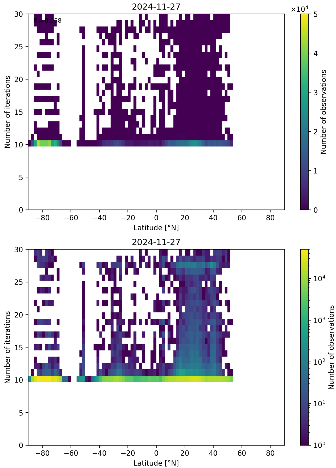
Figure 60: Scatter density plot of “Latitude” against “Number of iterations” for 2024-11-26 to 2024-11-28.
