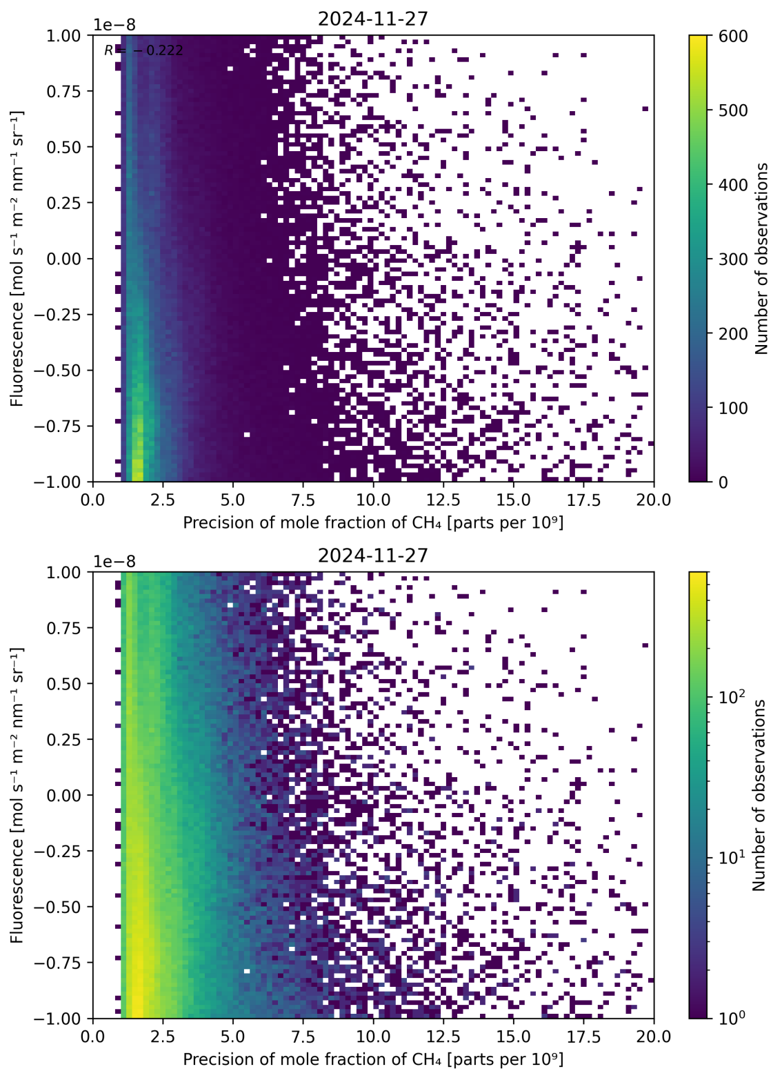
Figure 81: Scatter density plot of “Precision of mole fraction of \text{CH}_4 ” against “Fluorescence” for 2024-11-26 to 2024-11-28.
