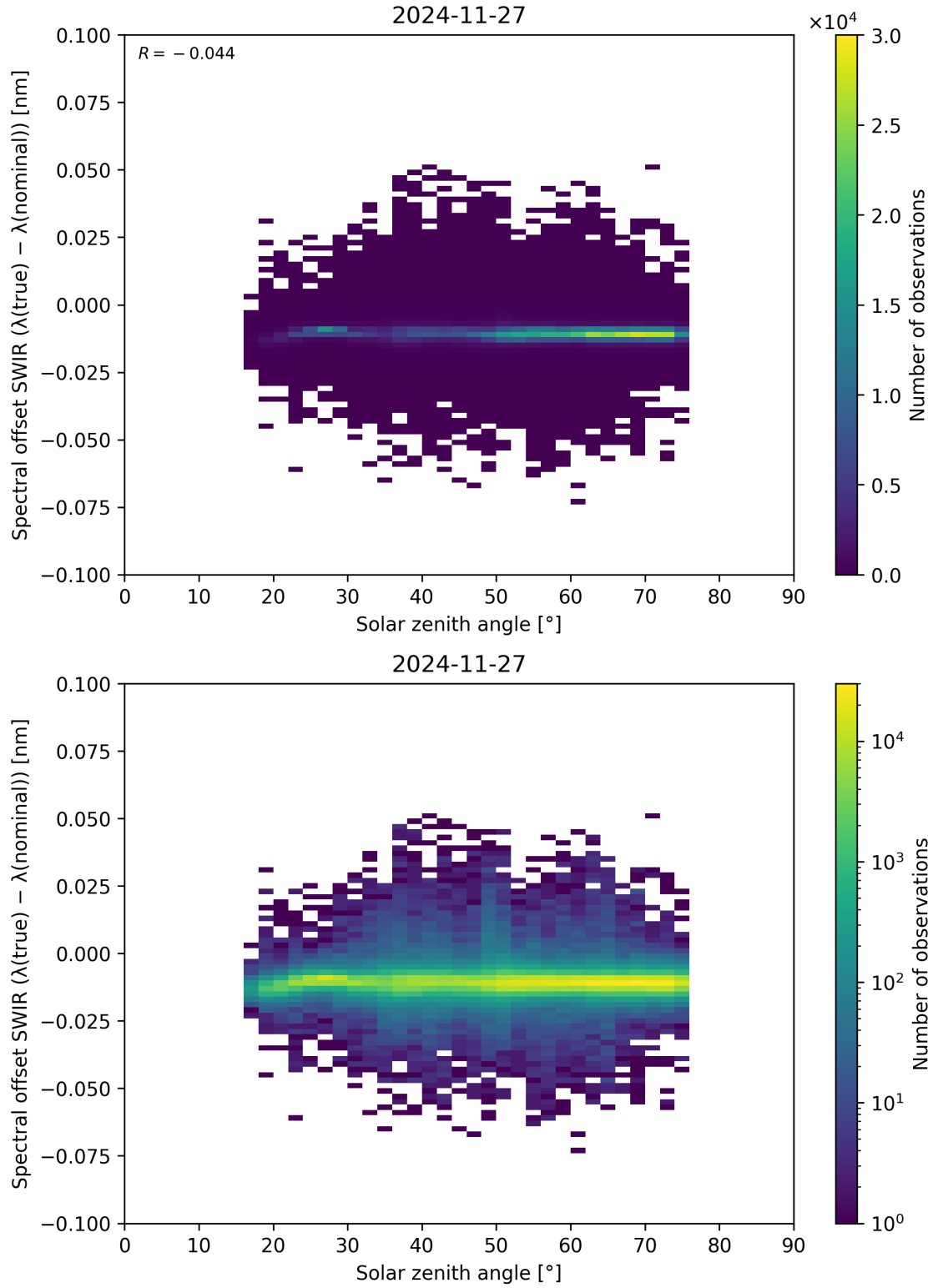
Figure 104: Scatter density plot of “Solar zenith angle” against “Spectral offset SWIR ( \lambda_{\text{true}} - \lambda_{\text{nominal}} )” for 2024-11-26 to 2024-11-28.
