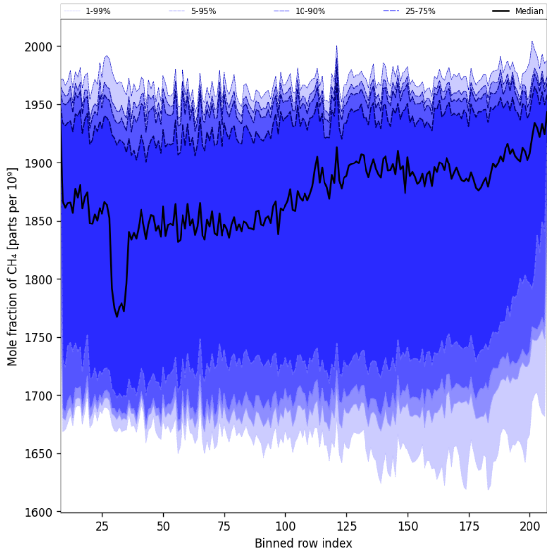
Figure 34: Along track statistics of “Mole fraction of CH 4 ” for 2024-11-26 to 2024-11-28
