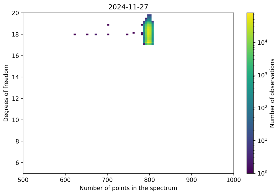
Figure 90: Scatter density plot of “Number of points in the spectrum” against “Degrees of freedom” for 2024-11-26 to 2024-11-28.
