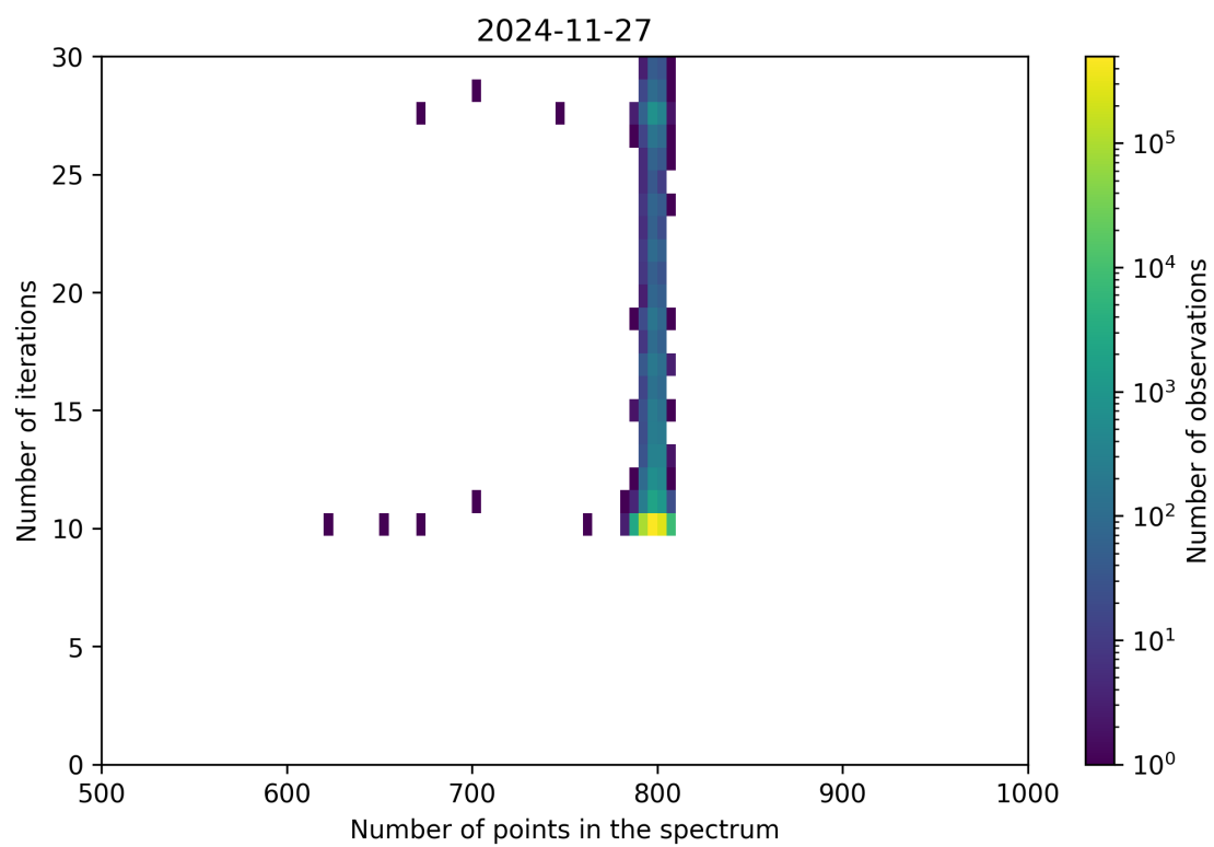
Figure 92: Scatter density plot of “Number of points in the spectrum” against “Number of iterations” for 2024-11-26 to 2024-11-28.
