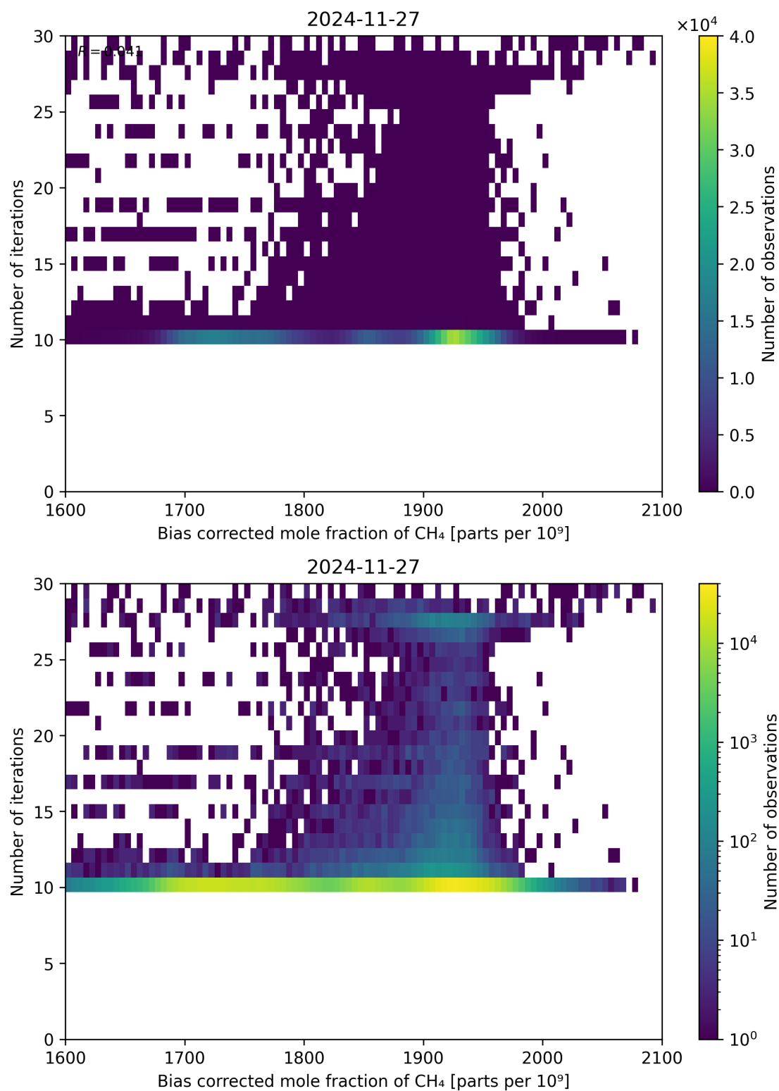
Figure 67: Scatter density plot of “Bias corrected mole fraction of \text{CH}_4 ” against “Number of iterations” for 2024-11-26 to 2024-11-28.
