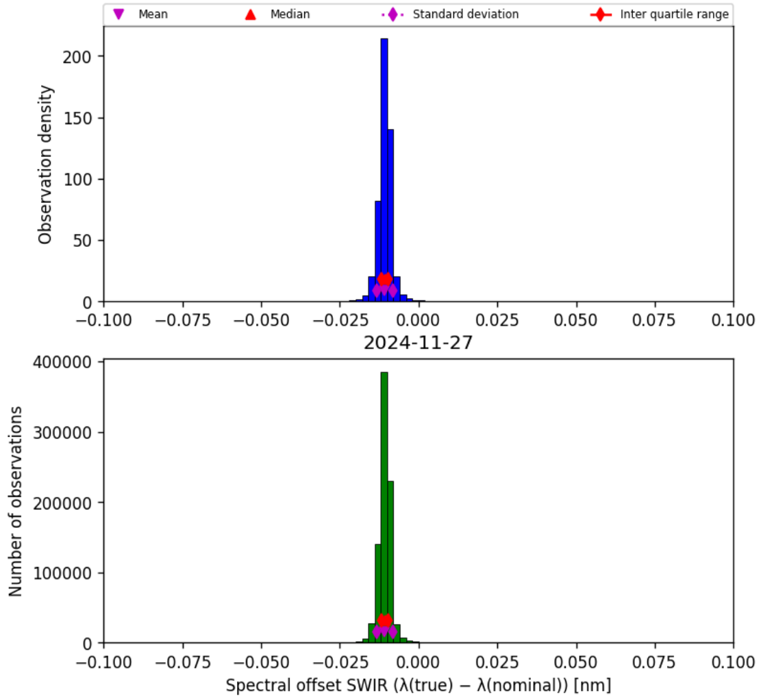
Figure 27: Histogram of “Spectral offset SWIR ( \lambda_{\text{true}} - \lambda_{\text{nominal}} )” for 2024-11-26 to 2024-11-28
