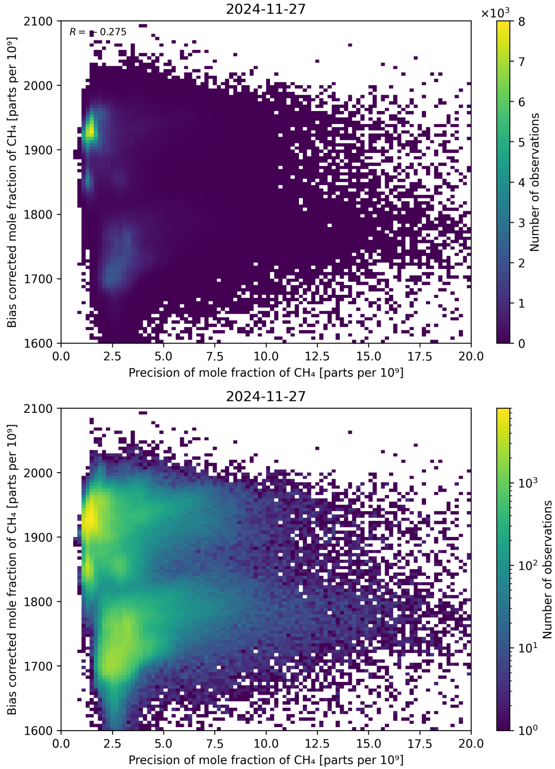
Figure 82: Scatter density plot of “Precision of mole fraction of CH 4 ” against “Bias corrected mole fraction of CH 4 ” for 2024-11-26 to 2024-11-28.
