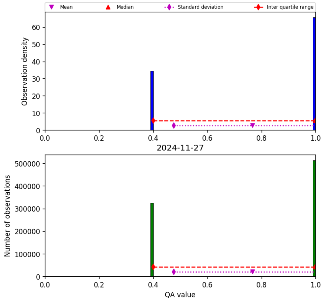
Figure 22: Histogram of “QA value” for 2024-11-26 to 2024-11-28
