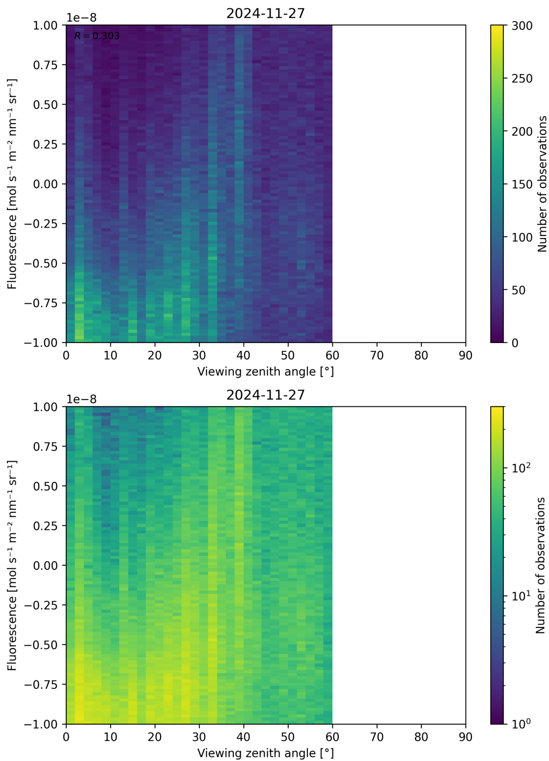
Figure 108: Scatter density plot of “Viewing zenith angle” against “Fluorescence” for 2024-11-26 to 2024-11-28.
