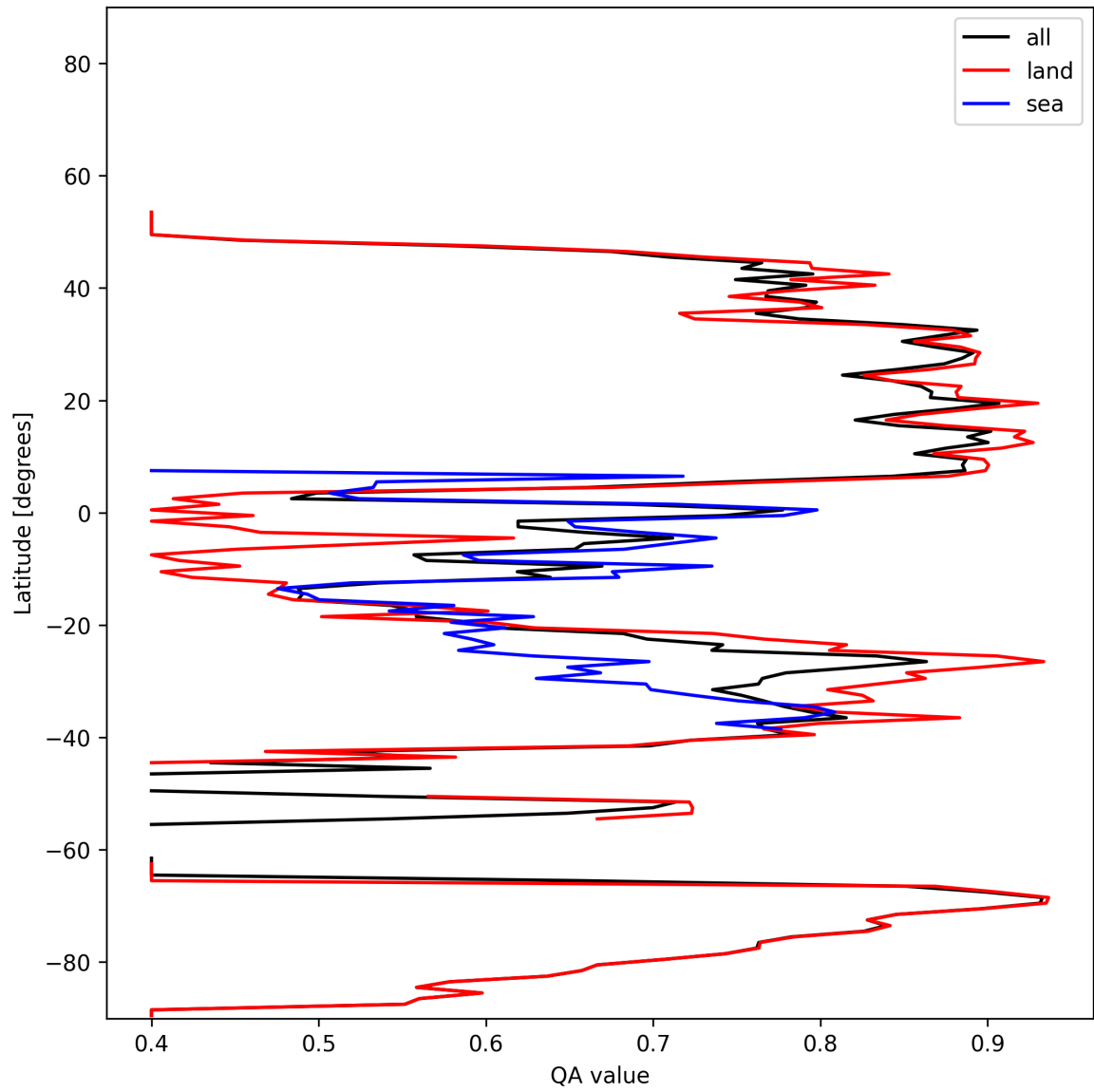
Figure 11: Zonal average of “QA value” for 2024-11-26 to 2024-11-28.
