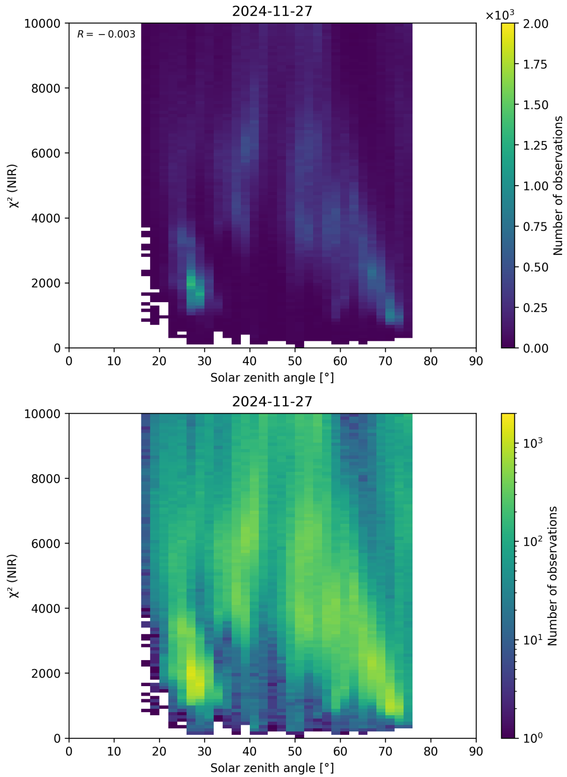
Figure 94: Scatter density plot of “Solar zenith angle” against “ \chi^2 (NIR)” for 2024-11-26 to 2024-11-28.
