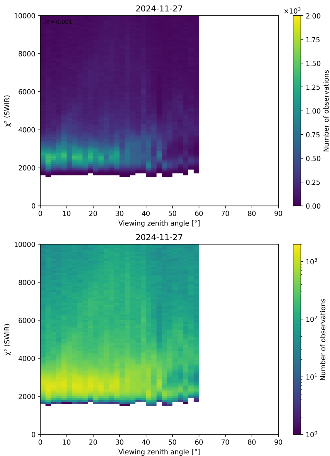
Figure 106: Scatter density plot of “Viewing zenith angle” against “ \chi^2 (SWIR)” for 2024-11-26 to 2024-11-28.
