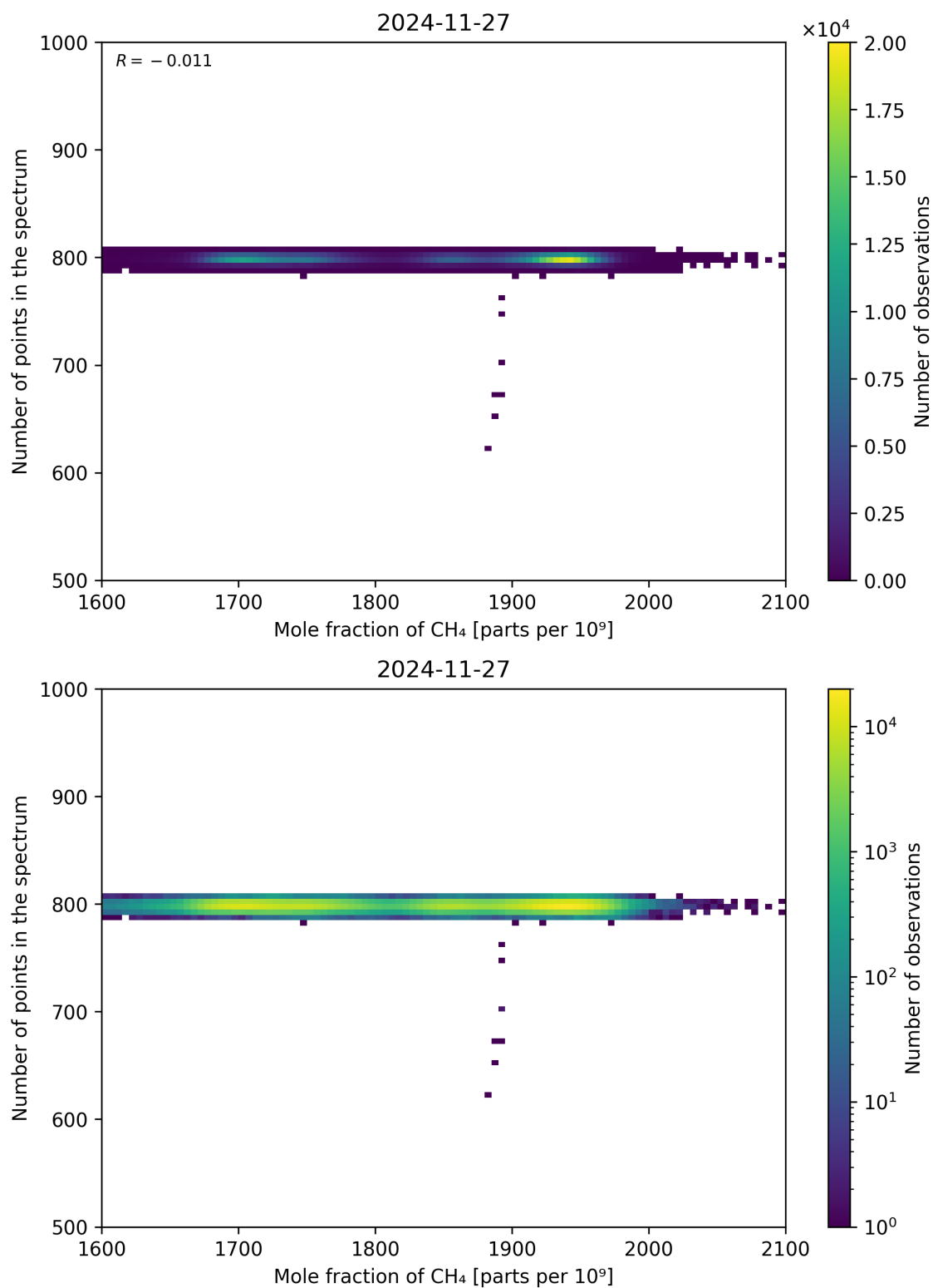
Figure 77: Scatter density plot of “Mole fraction of CH 4 ” against “Number of points in the spectrum” for 2024-11-26 to 2024-11-28.
