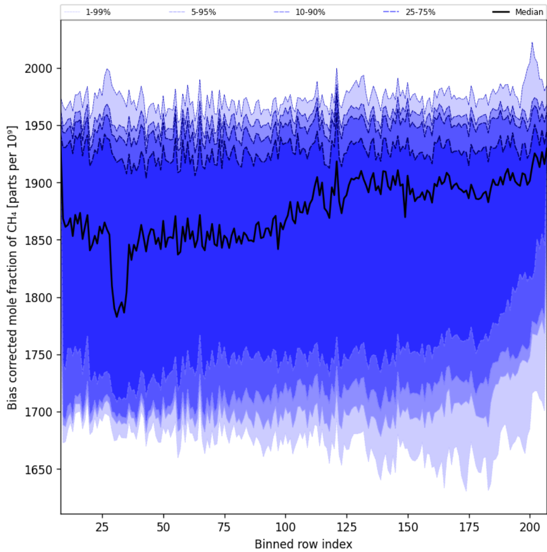
Figure 36: Along track statistics of “Bias corrected mole fraction of CH 4 ” for 2024-11-26 to 2024-11-28
