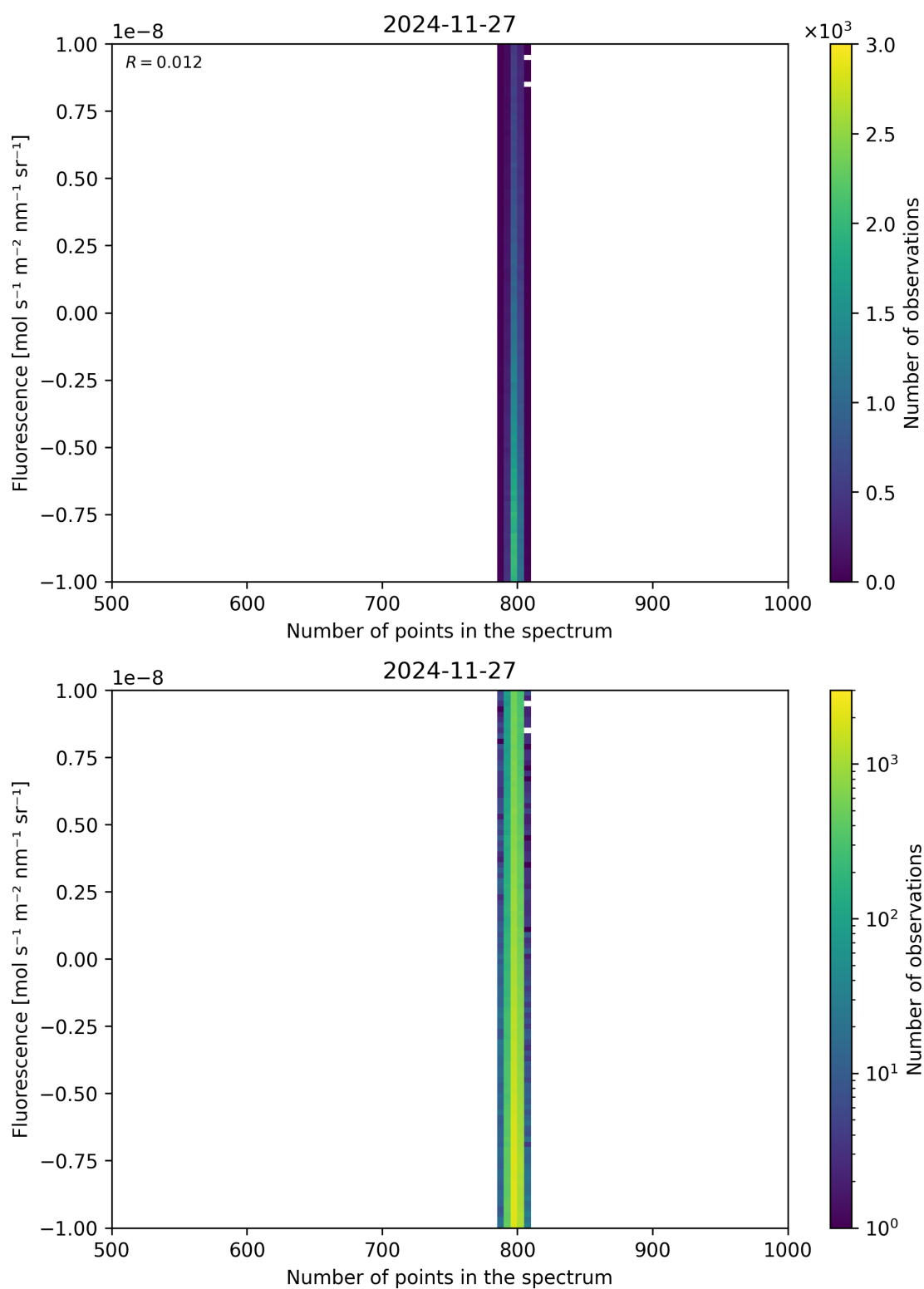
Figure 91: Scatter density plot of “Number of points in the spectrum” against “Fluorescence” for 2024-11-26 to 2024-11-28.
