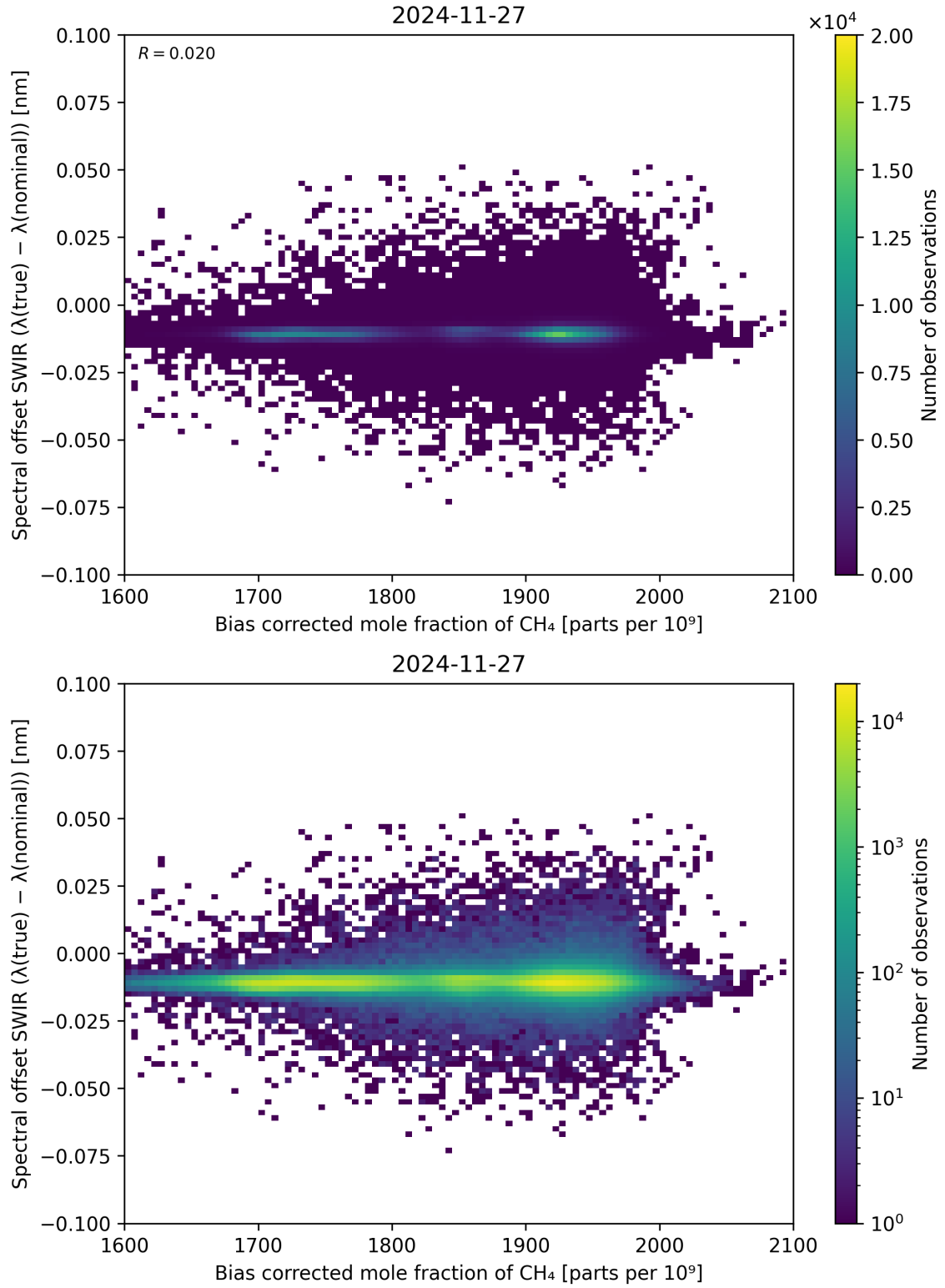
Figure 69: Scatter density plot of “Bias corrected mole fraction of \text{CH}_4 ” against “Spectral offset SWIR ( \lambda_{\text{true}} - \lambda_{\text{nominal}} )” for 2024-11-26 to 2024-11-28.
