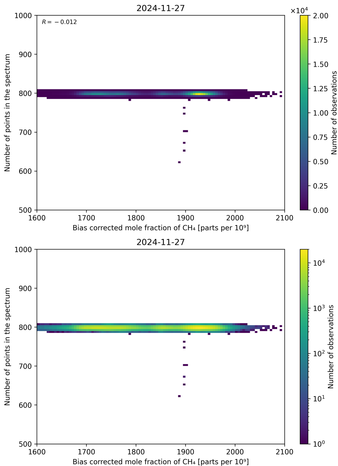
Figure 68: Scatter density plot of “Bias corrected mole fraction of CH 4 ” against “Number of points in the spectrum” for 2024-11-26 to 2024-11-28.
