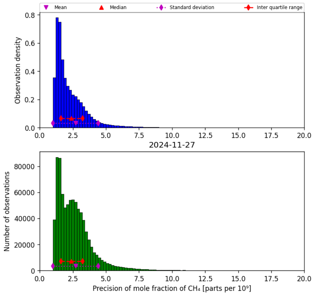
Figure 24: Histogram of “Precision of mole fraction of CH 4 ” for 2024-11-26 to 2024-11-28
