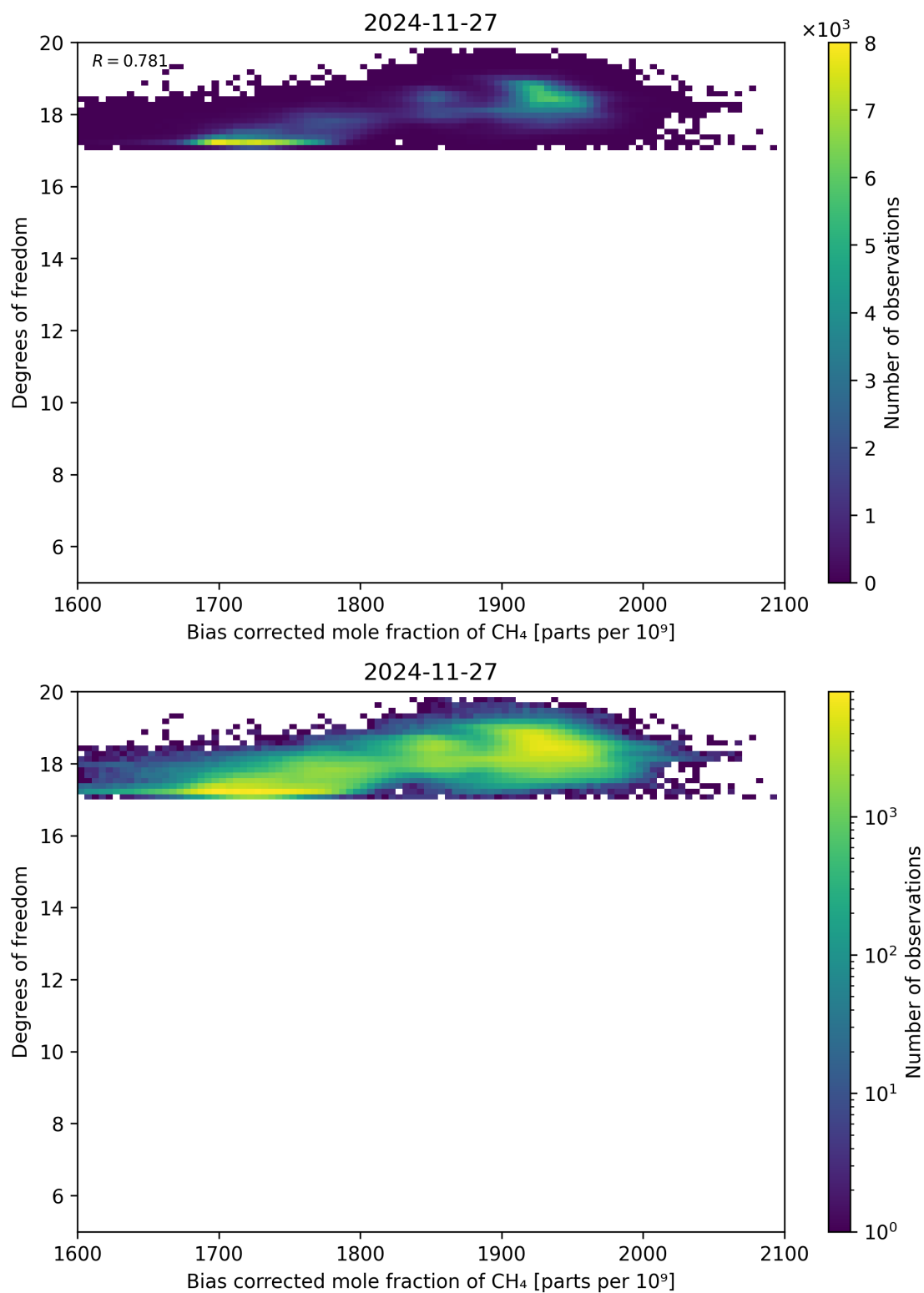
Figure 65: Scatter density plot of “Bias corrected mole fraction of CH 4 ” against “Degrees of freedom” for 2024-11-26 to 2024-11-28.
