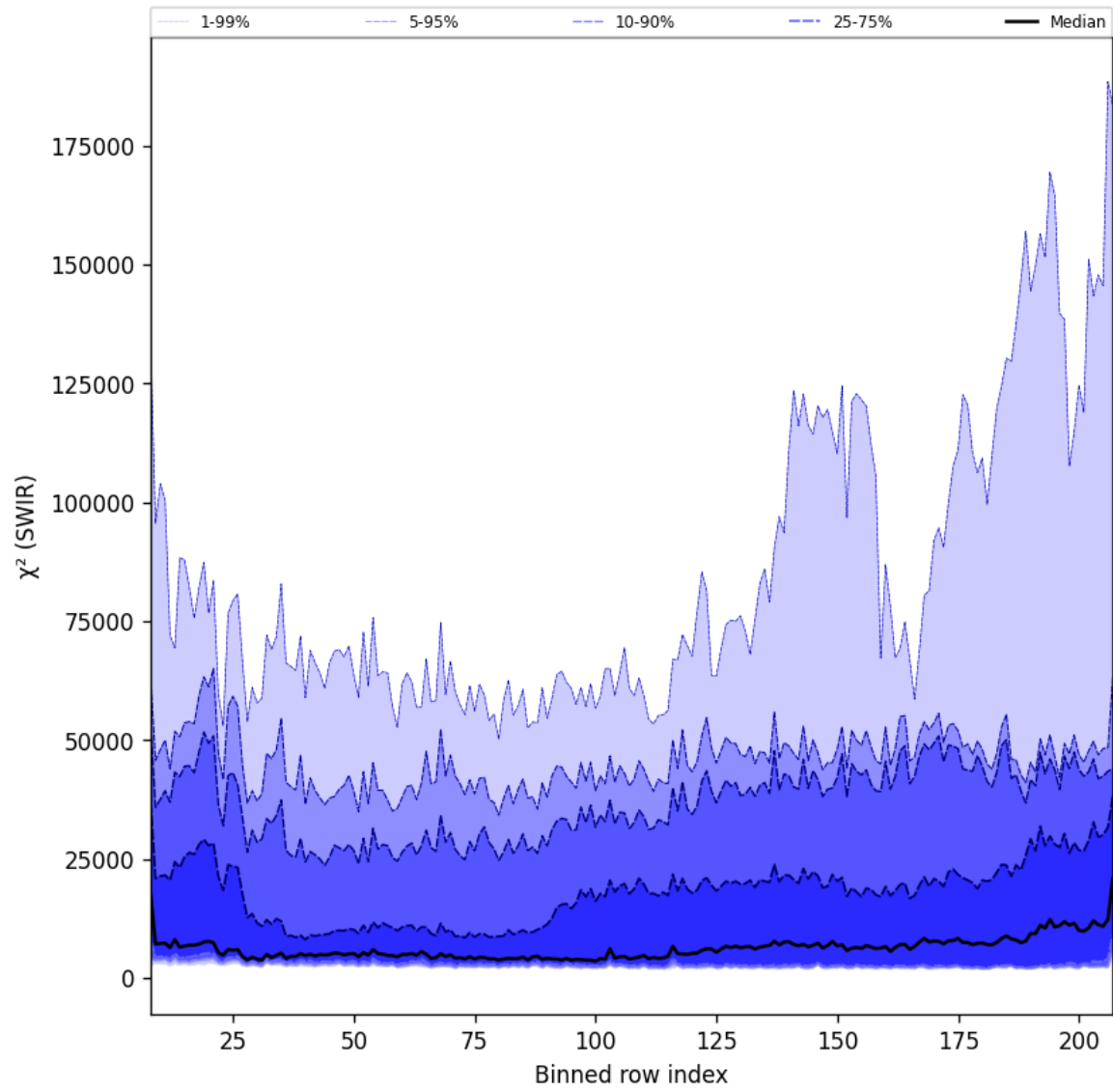
Figure 39: Along track statistics of “ \chi^2 (SWIR)” for 2024-11-26 to 2024-11-28
