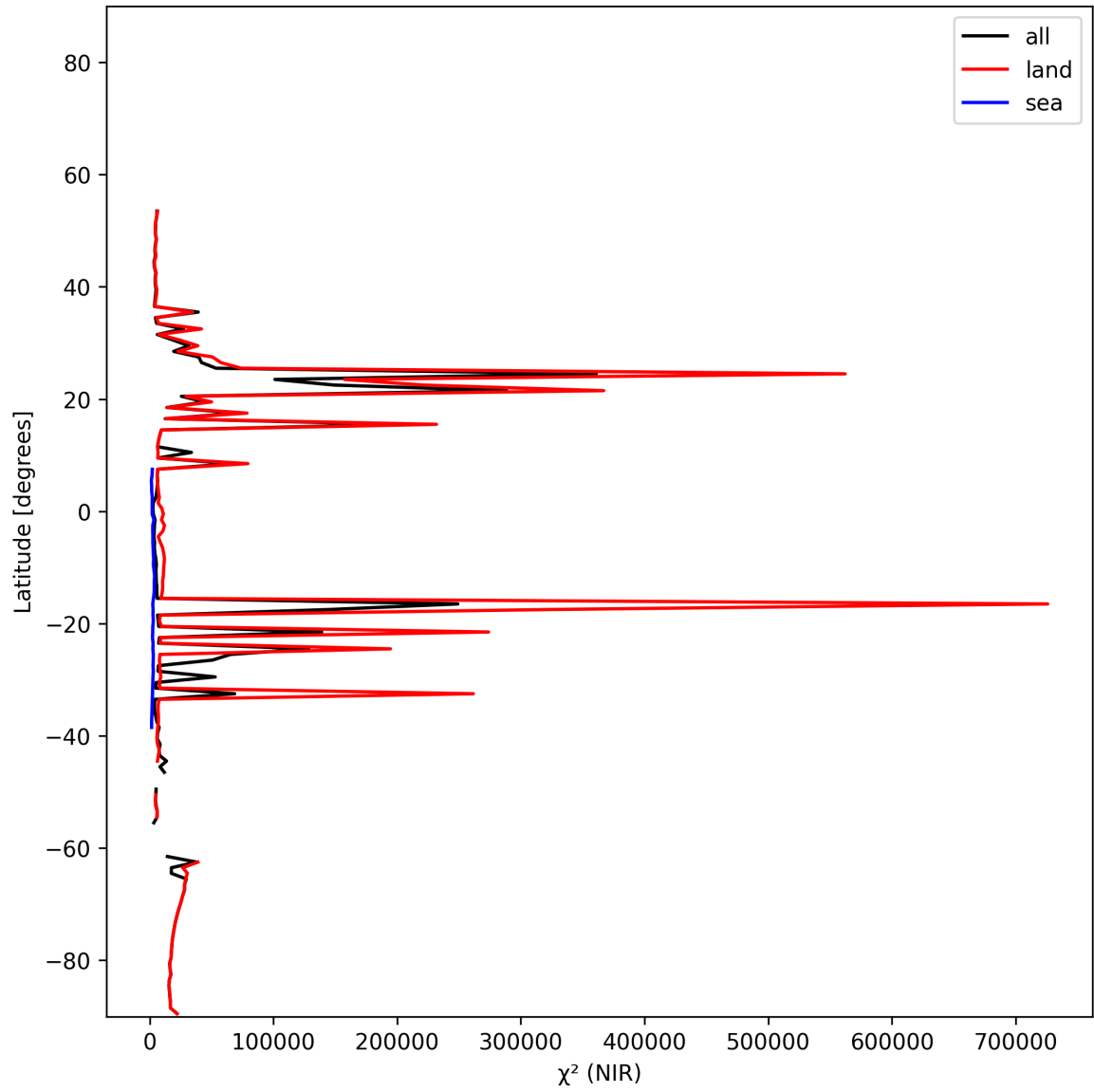
Figure 18: Zonal average of “ \chi^2 (NIR)” for 2024-11-26 to 2024-11-28.
