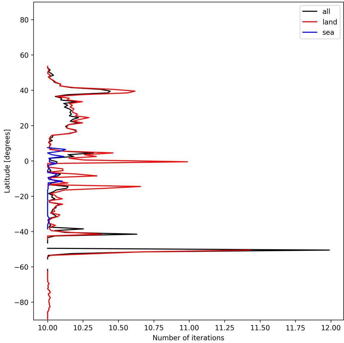
Figure 20: Zonal average of “Number of iterations” for 2024-11-26 to 2024-11-28.
