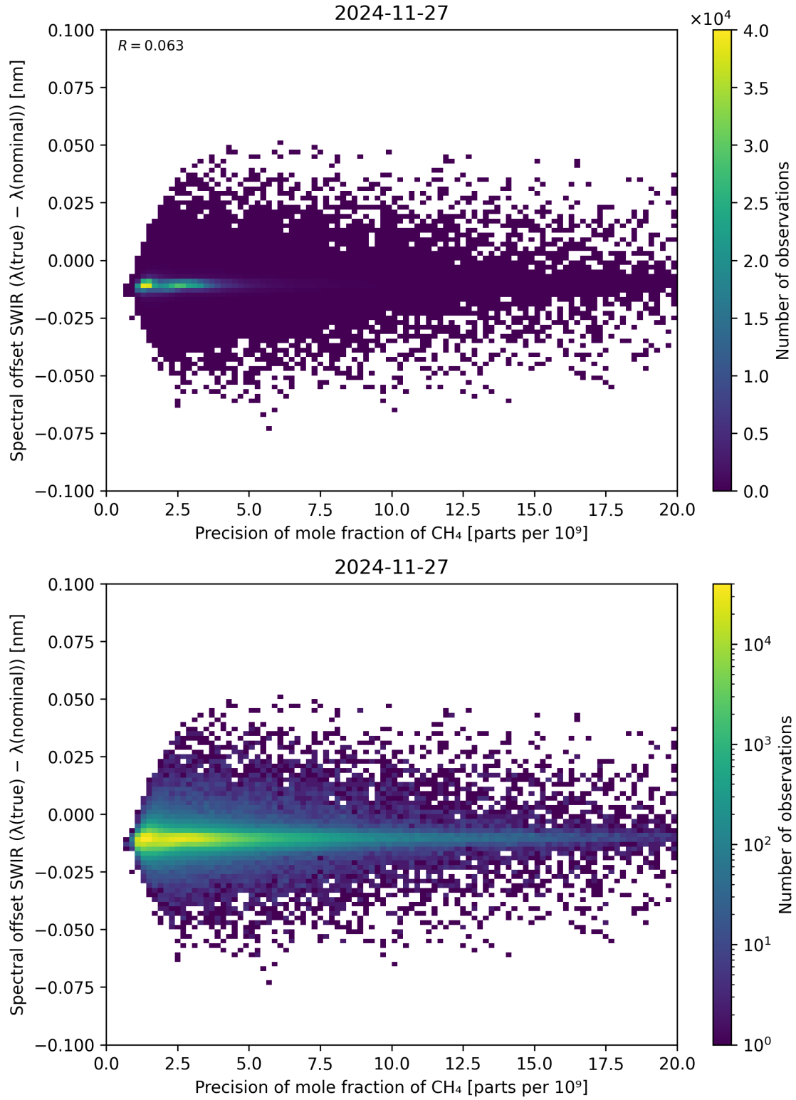
Figure 85: Scatter density plot of “Precision of mole fraction of CH 4 ” against “Spectral offset SWIR ( \lambda_{\text{true}} - \lambda_{\text{nominal}} )” for 2024-11-26 to 2024-11-28.
