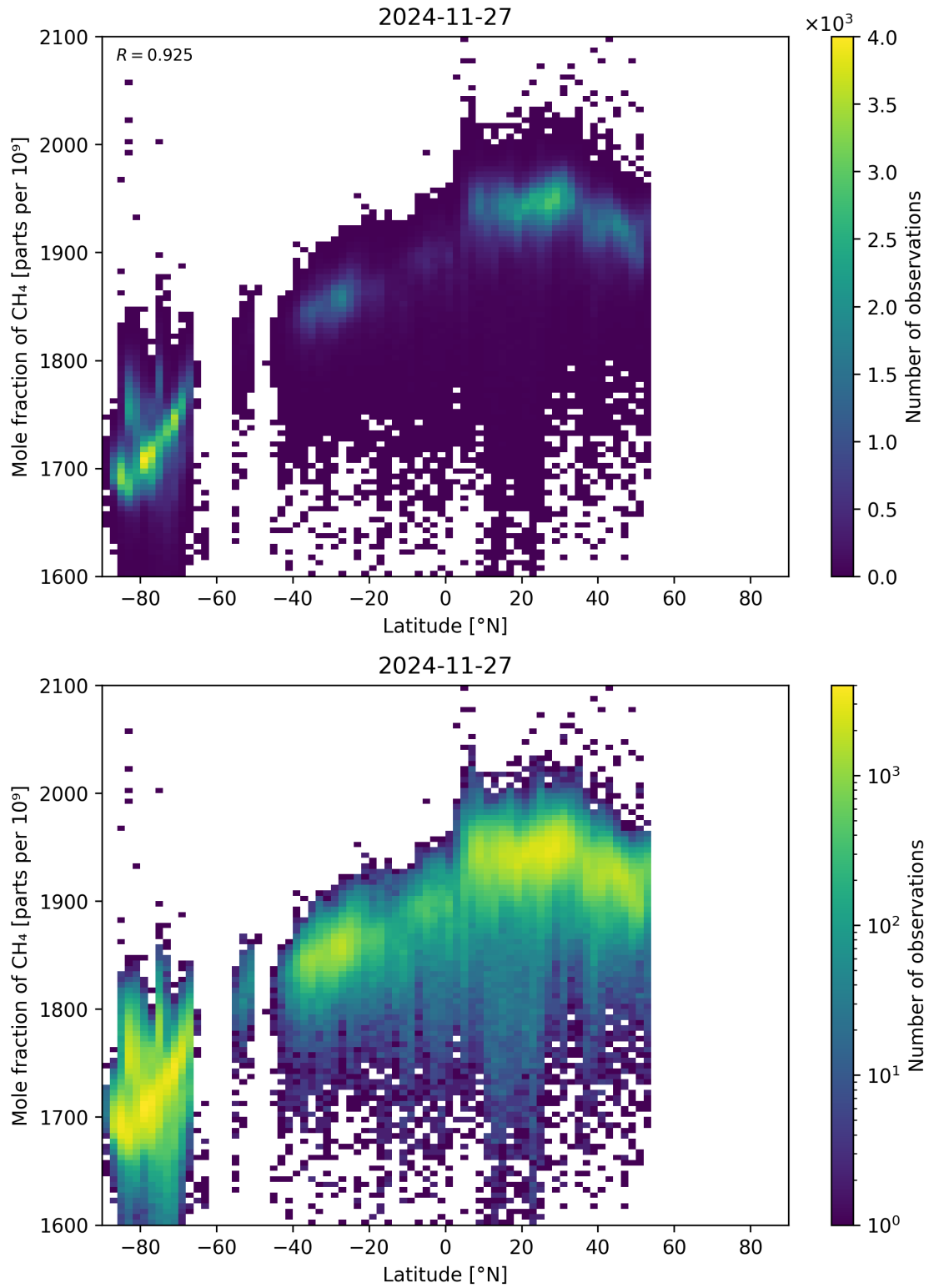
Figure 57: Scatter density plot of “Latitude” against “Mole fraction of CH 4 ” for 2024-11-26 to 2024-11-28.
