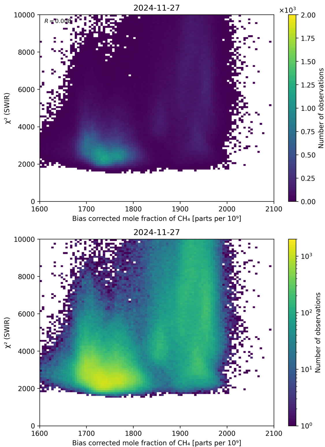
Figure 64: Scatter density plot of “Bias corrected mole fraction of \text{CH}_4 ” against “ \chi^2 (SWIR)” for 2024-11-26 to 2024-11-28.
