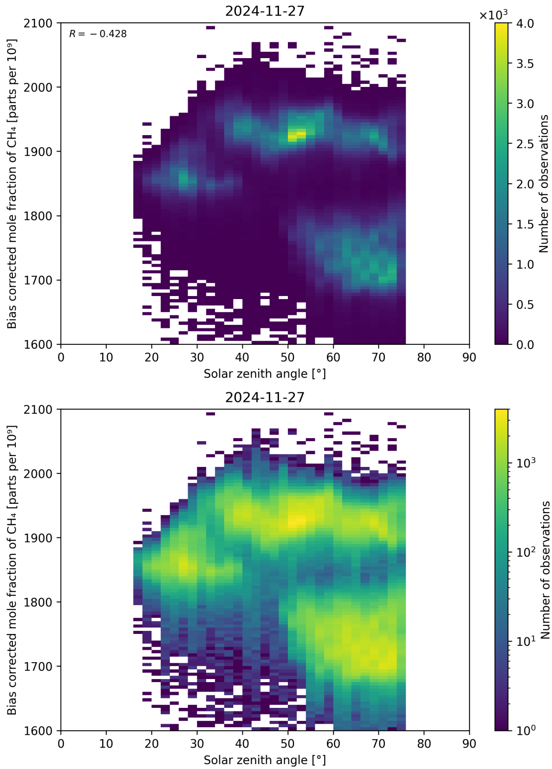
Figure 100: Scatter density plot of “Solar zenith angle” against “Bias corrected mole fraction of CH 4 ” for 2024-11-26 to 2024-11-28.
