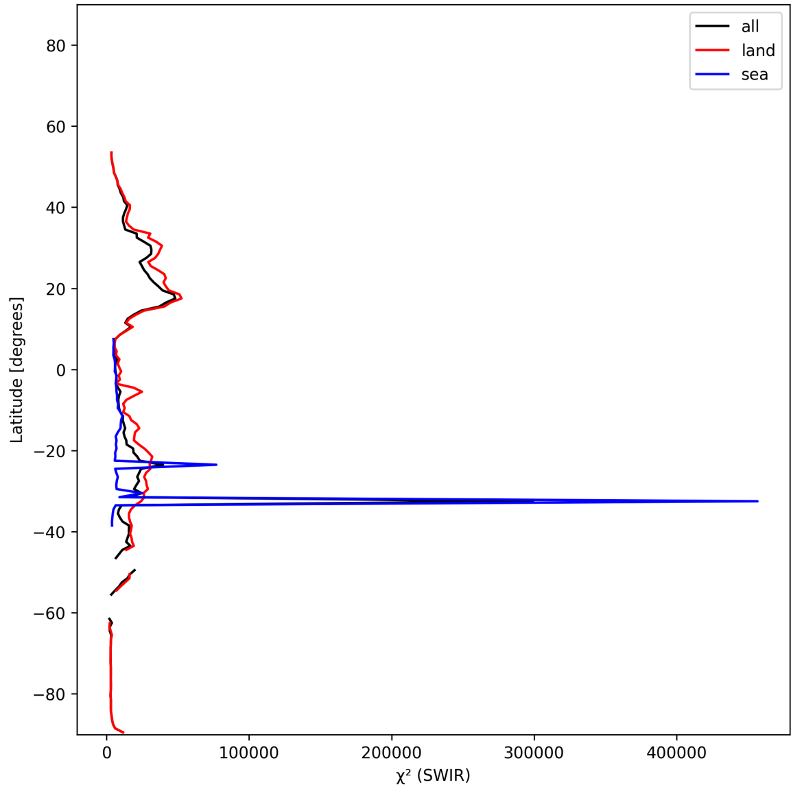
Figure 17: Zonal average of “ \chi^2 (SWIR)” for 2024-11-26 to 2024-11-28.
