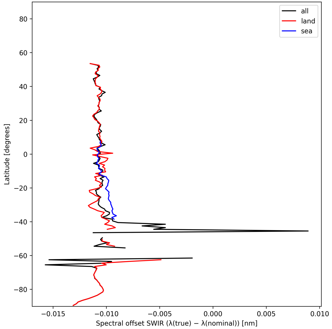
Figure 16: Zonal average of “Spectral offset SWIR ( \lambda_{\text{true}} - \lambda_{\text{nominal}} )” for 2024-11-26 to 2024-11-28.
