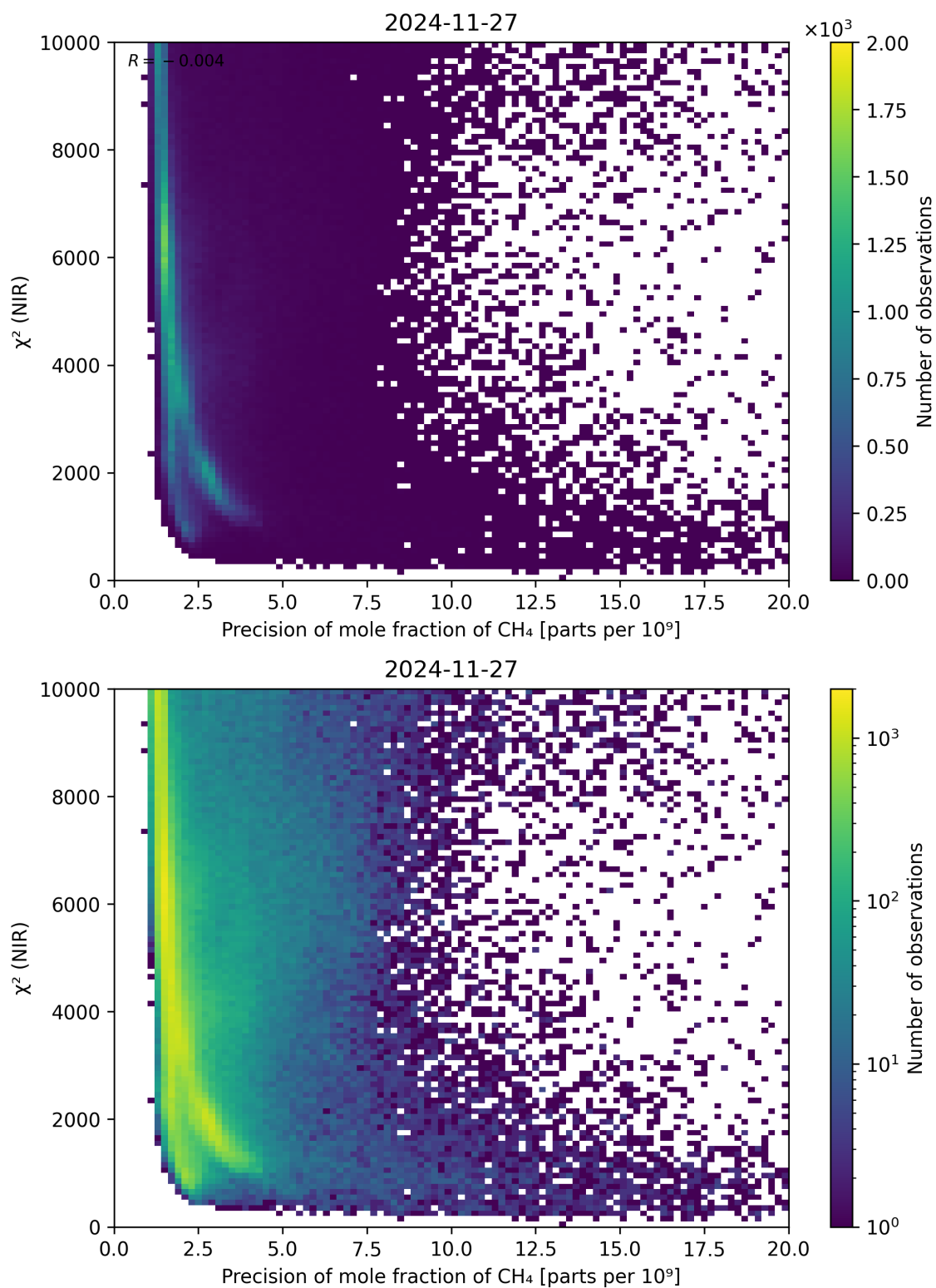
Figure 78: Scatter density plot of “Precision of mole fraction of \text{CH}_4 ” against “ \chi^2 (NIR)” for 2024-11-26 to 2024-11-28.
