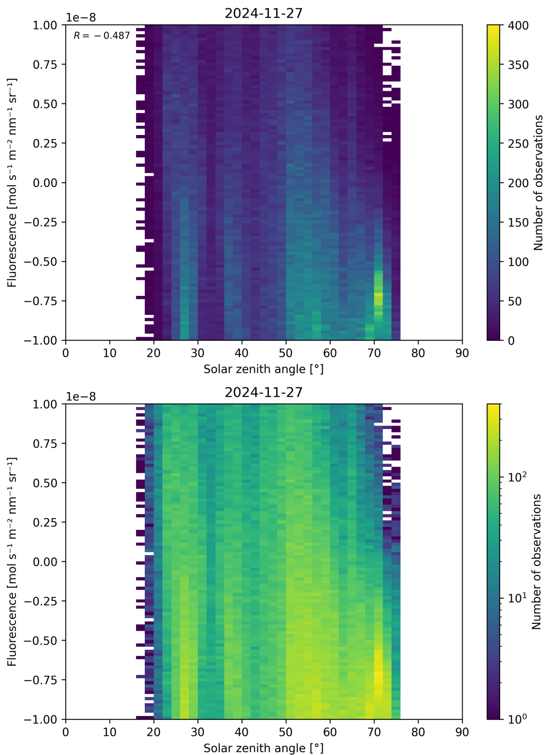
Figure 97: Scatter density plot of “Solar zenith angle” against “Fluorescence” for 2024-11-26 to 2024-11-28.
