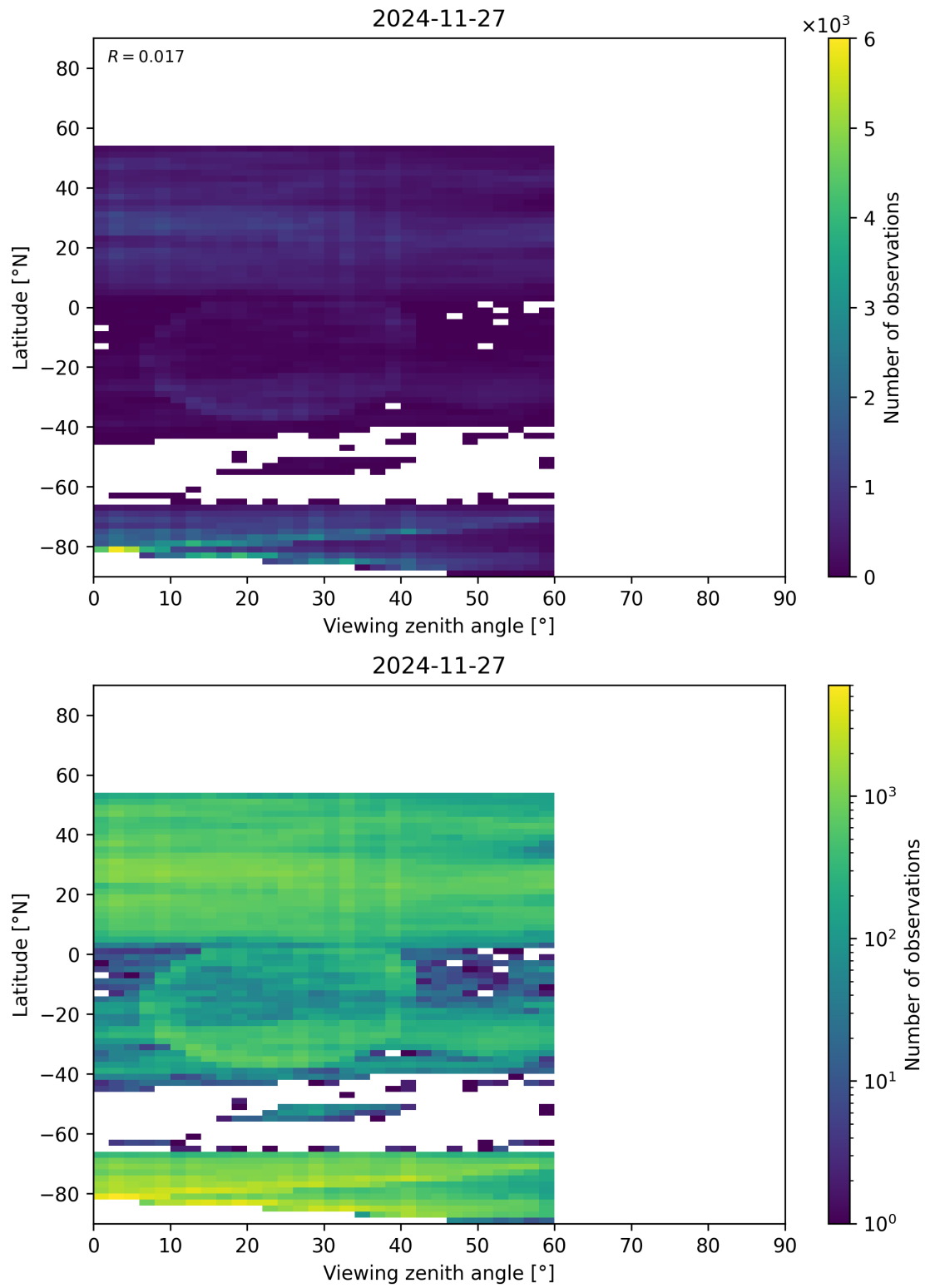
Figure 109: Scatter density plot of “Viewing zenith angle” against “Latitude” for 2024-11-26 to 2024-11-28.
