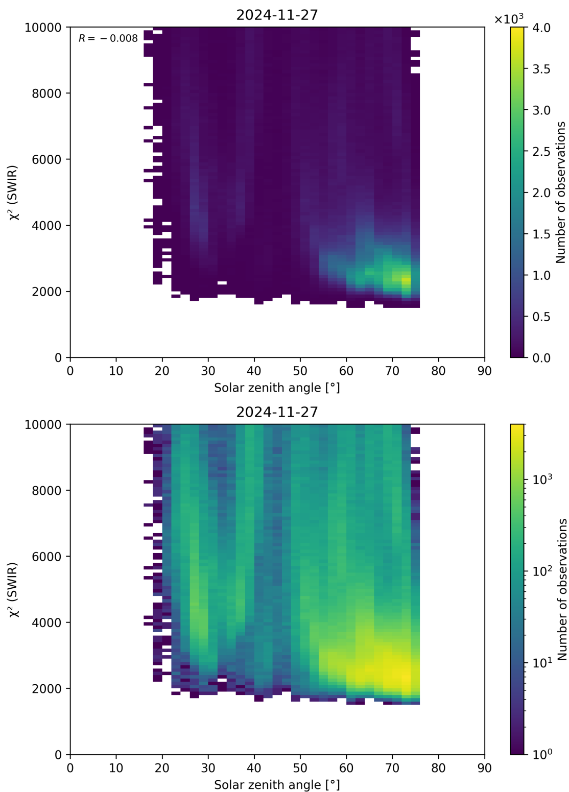
Figure 95: Scatter density plot of “Solar zenith angle” against “ \chi^2 (SWIR)” for 2024-11-26 to 2024-11-28.
