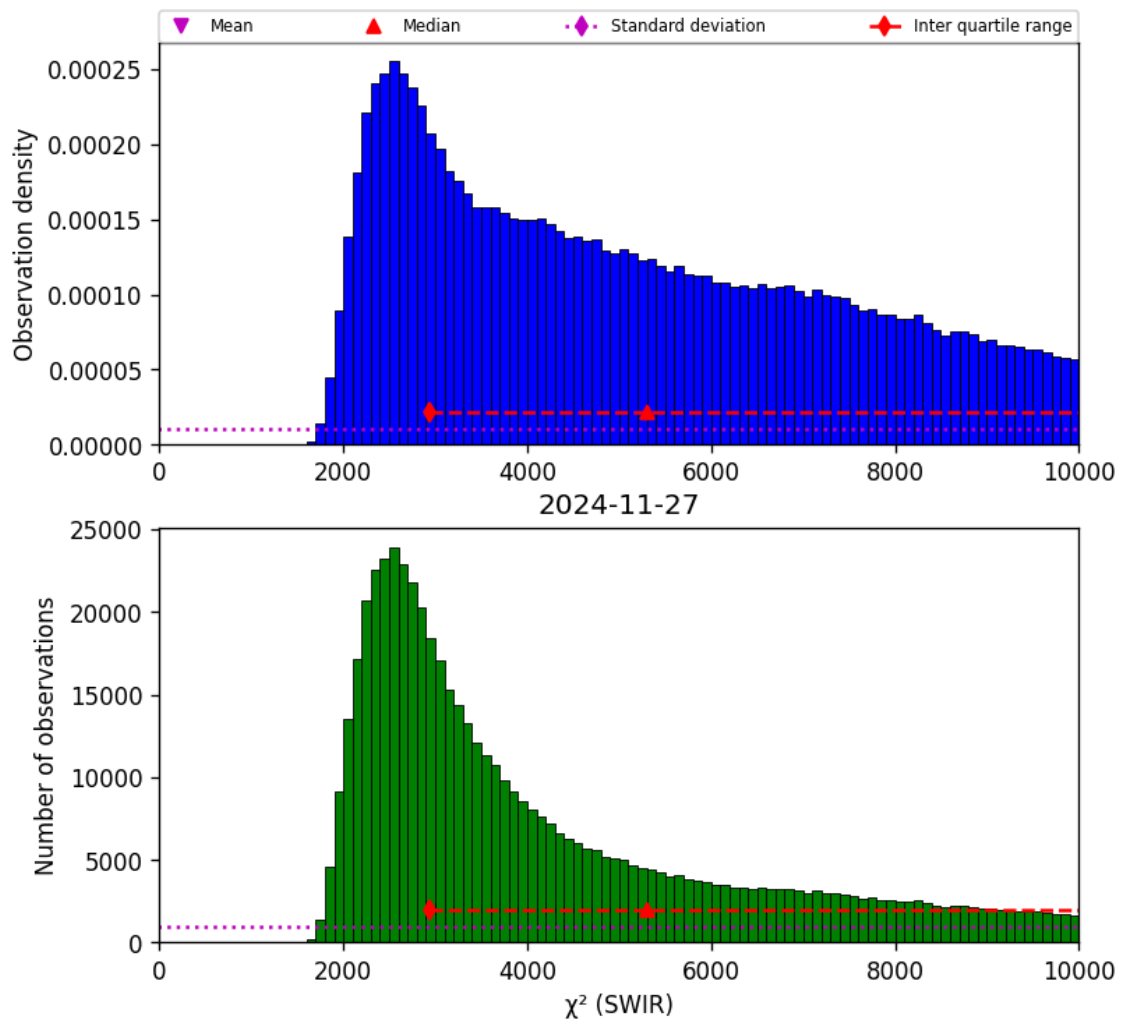
Figure 28: Histogram of “ \chi^2 (SWIR)” for 2024-11-26 to 2024-11-28
