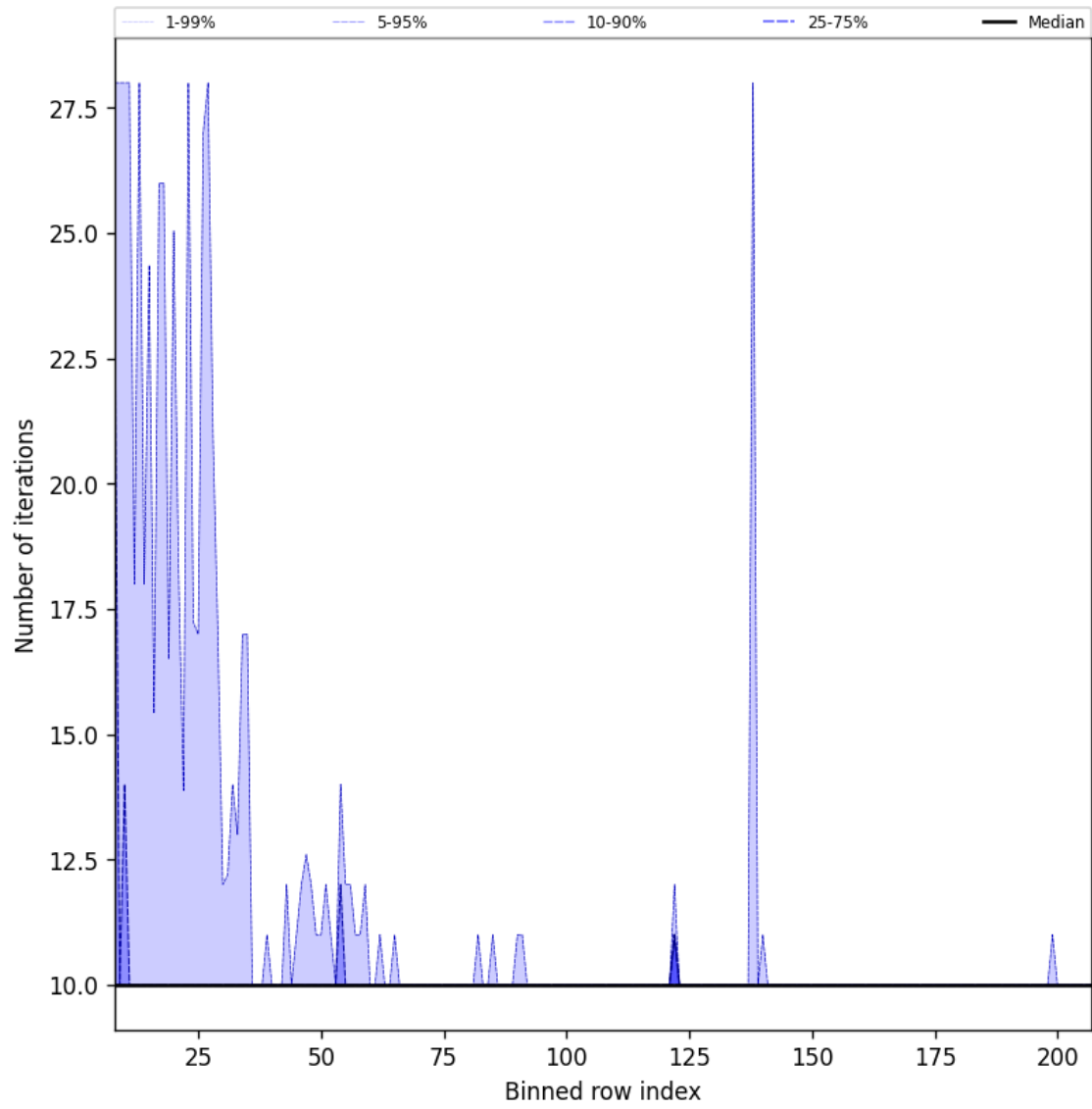
Figure 42: Along track statistics of “Number of iterations” for 2024-11-26 to 2024-11-28
