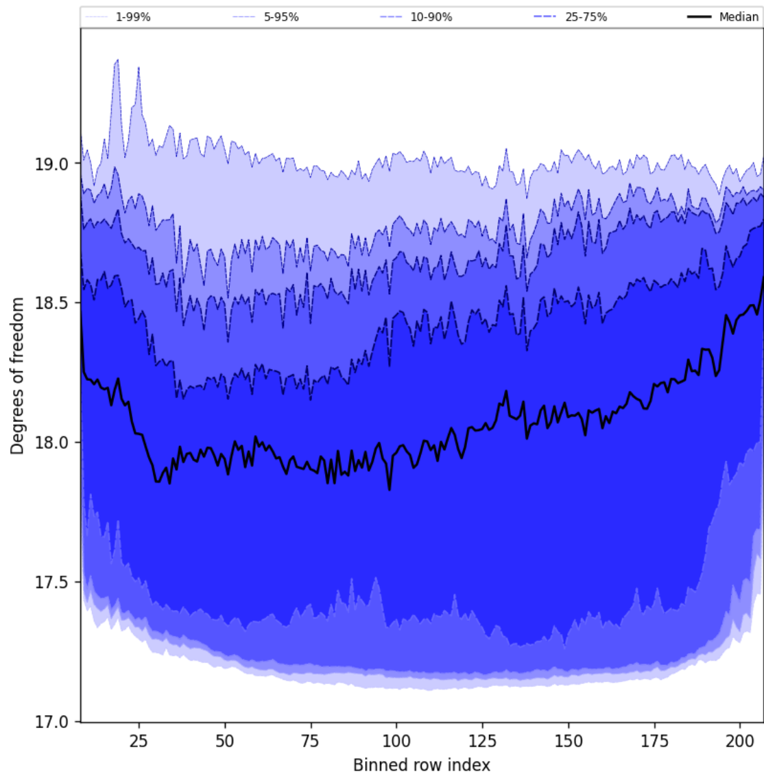
Figure 41: Along track statistics of “Degrees of freedom” for 2024-11-26 to 2024-11-28
