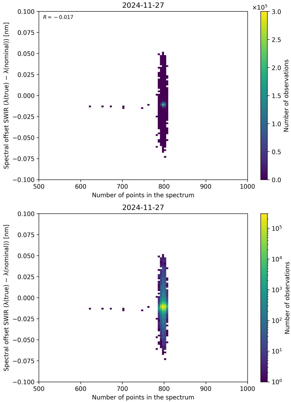
Figure 93: Scatter density plot of “Number of points in the spectrum” against “Spectral offset SWIR ( \lambda_{\text{true}} - \lambda_{\text{nominal}} )” for 2024-11-26 to 2024-11-28.
