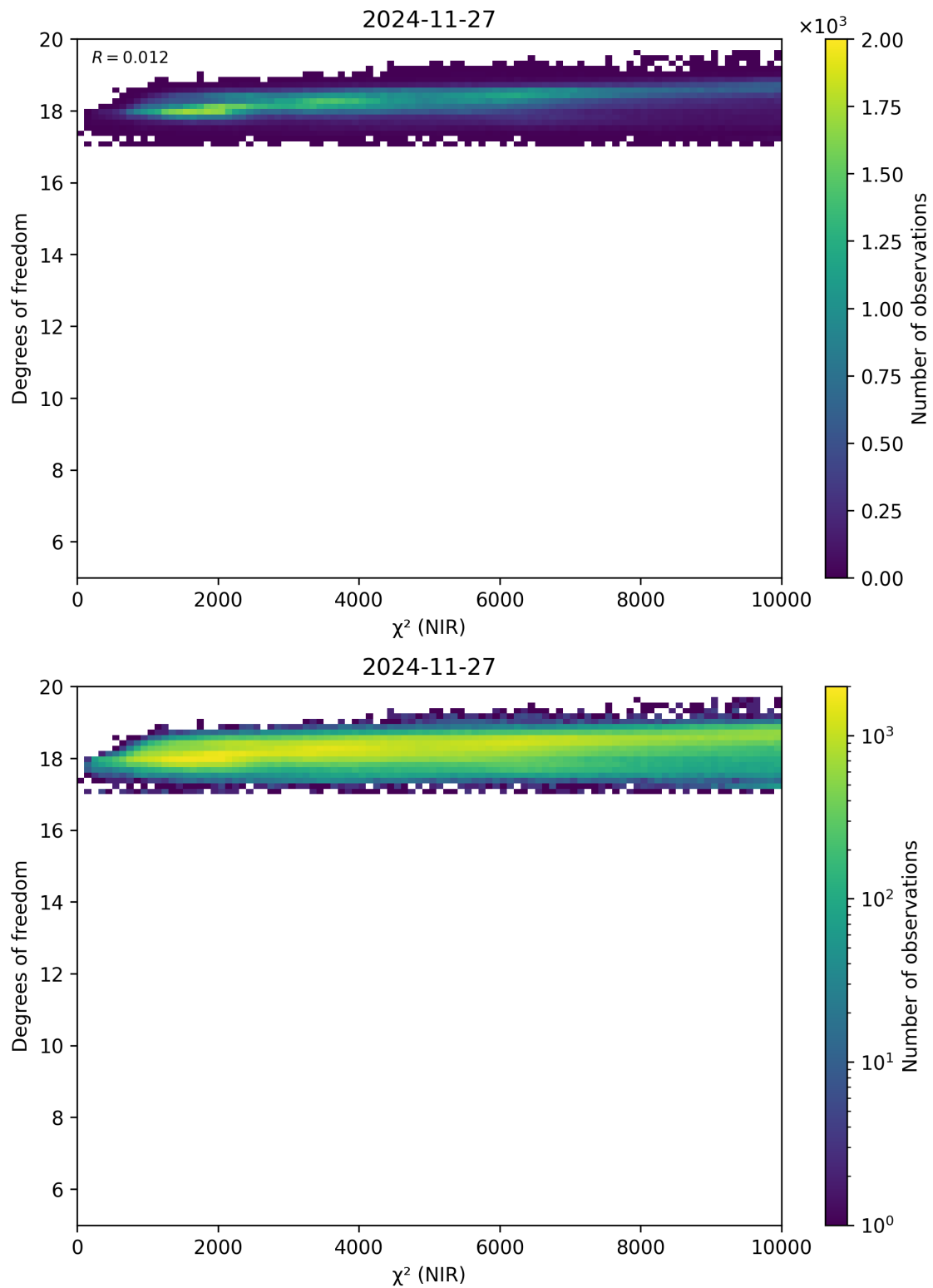
Figure 44: Scatter density plot of “ \chi^2 (NIR)” against “Degrees of freedom” for 2024-11-26 to 2024-11-28.
