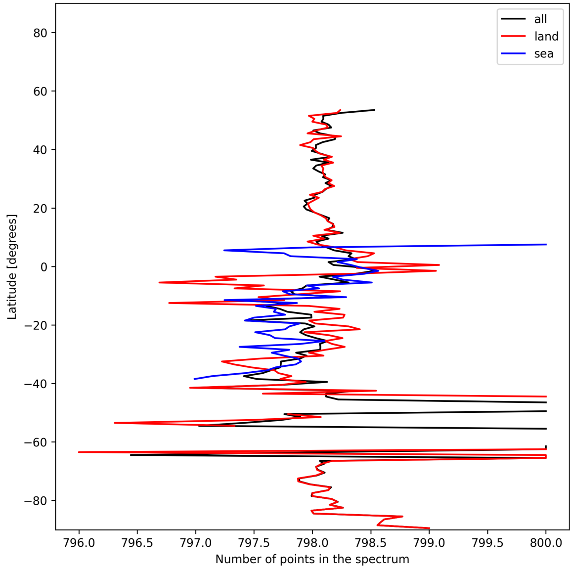
Figure 15: Zonal average of “Number of points in the spectrum” for 2024-11-26 to 2024-11-28.
