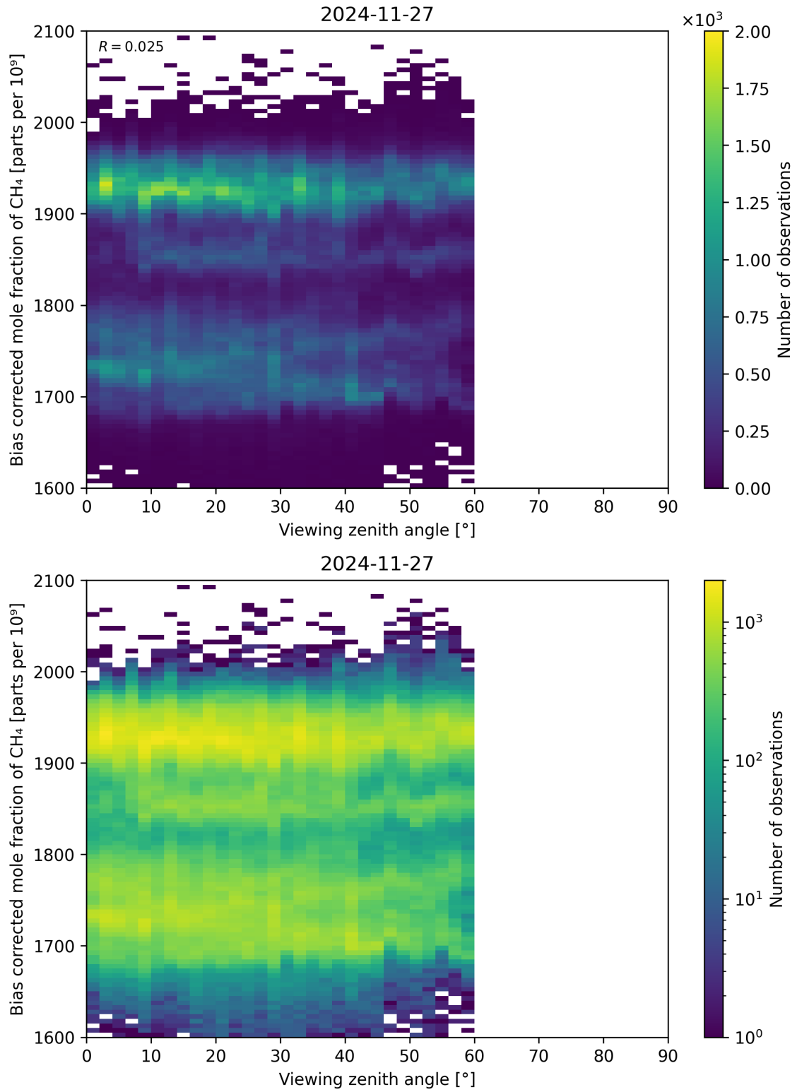
Figure 111: Scatter density plot of “Viewing zenith angle” against “Bias corrected mole fraction of CH 4 ” for 2024-11-26 to 2024-11-28.
