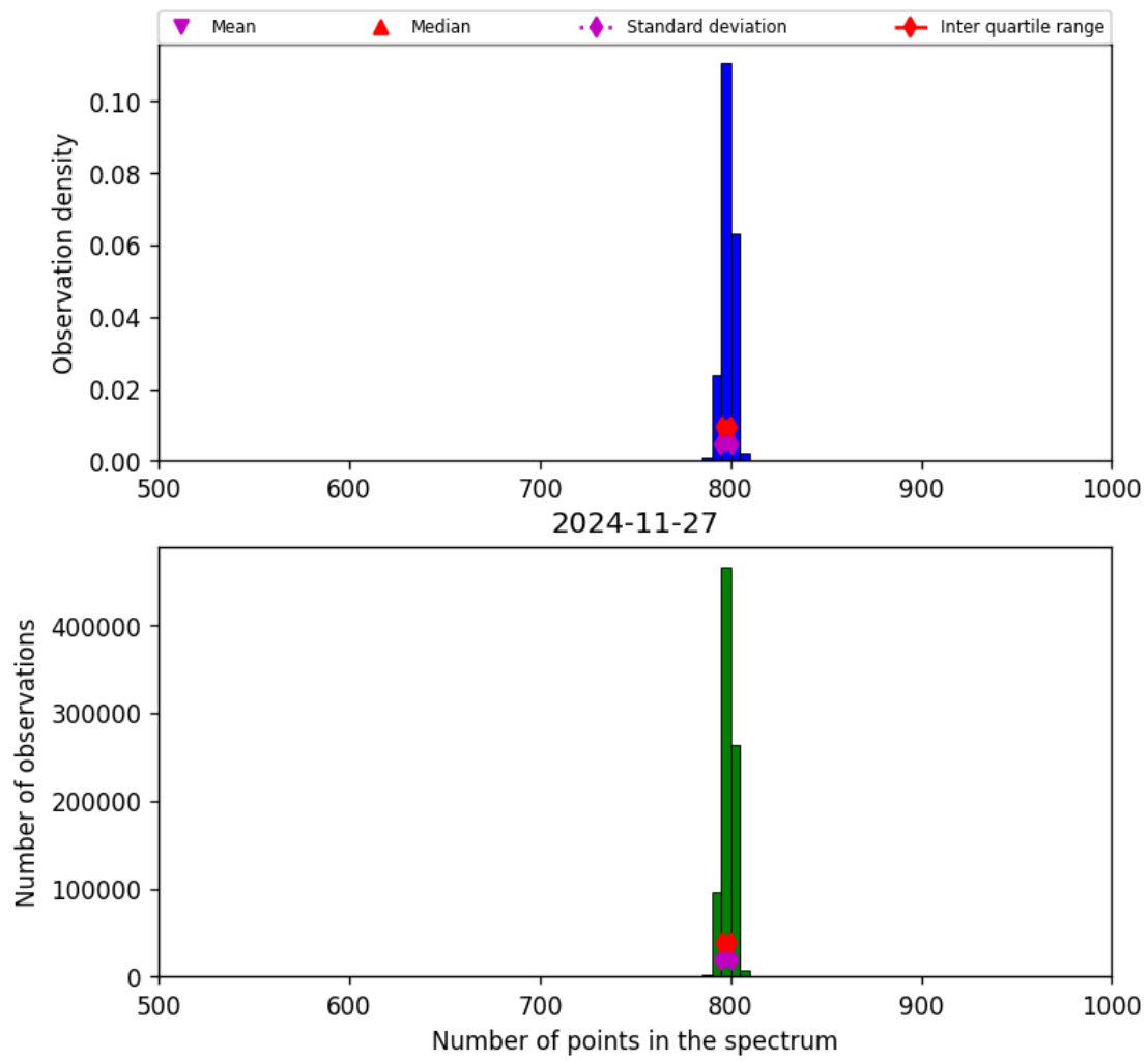
Figure 26: Histogram of “Number of points in the spectrum” for 2024-11-26 to 2024-11-28
