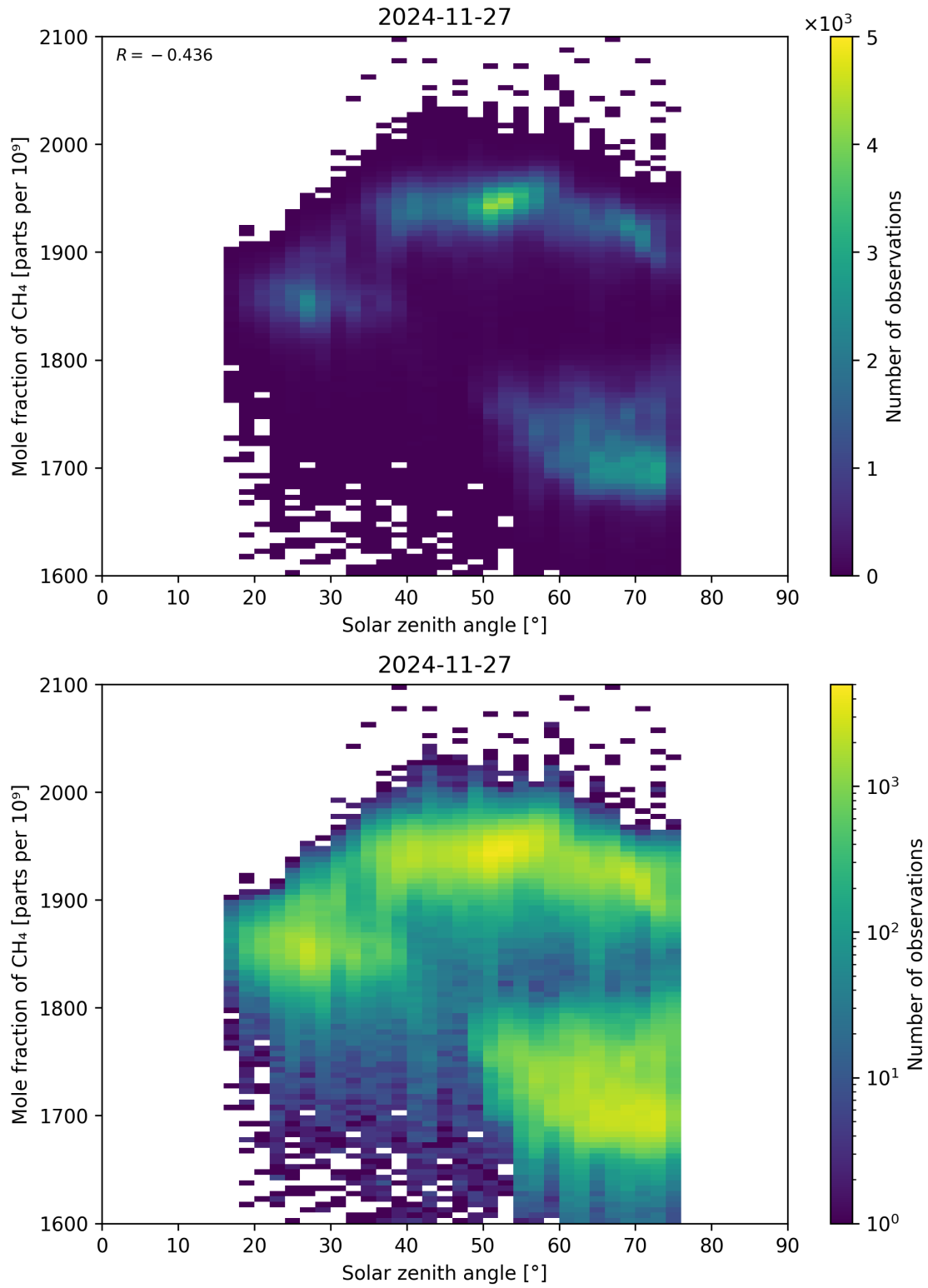
Figure 99: Scatter density plot of “Solar zenith angle” against “Mole fraction of CH 4 ” for 2024-11-26 to 2024-11-28.
