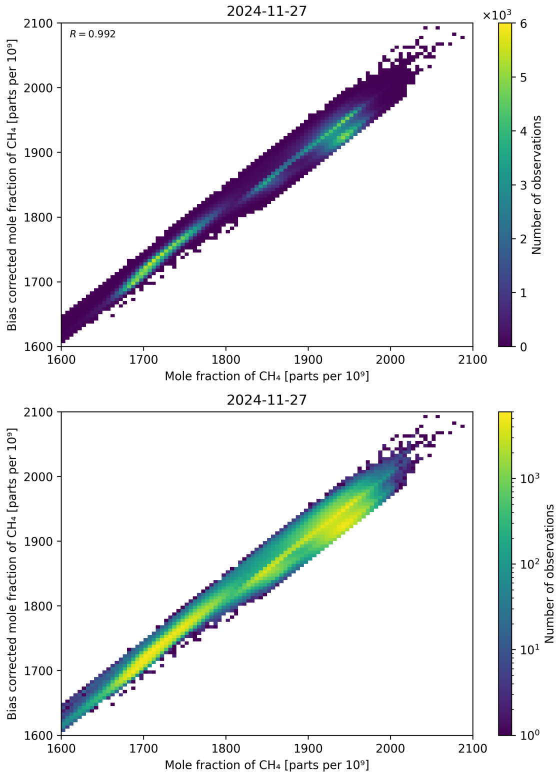
Figure 74: Scatter density plot of “Mole fraction of CH 4 ” against “Bias corrected mole fraction of CH 4 ” for 2024-11-26 to 2024-11-28.
