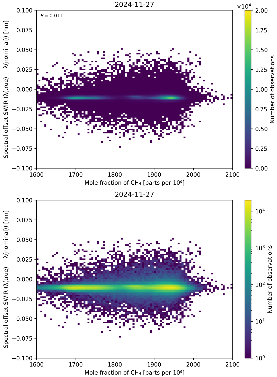
Figure 86: Scatter density plot of “Mole fraction of CH 4 ” against “Spectral offset SWIR ( \lambda_{\text{true}} - \lambda_{\text{nominal}} )” for 2024-11-26 to 2024-11-28.
