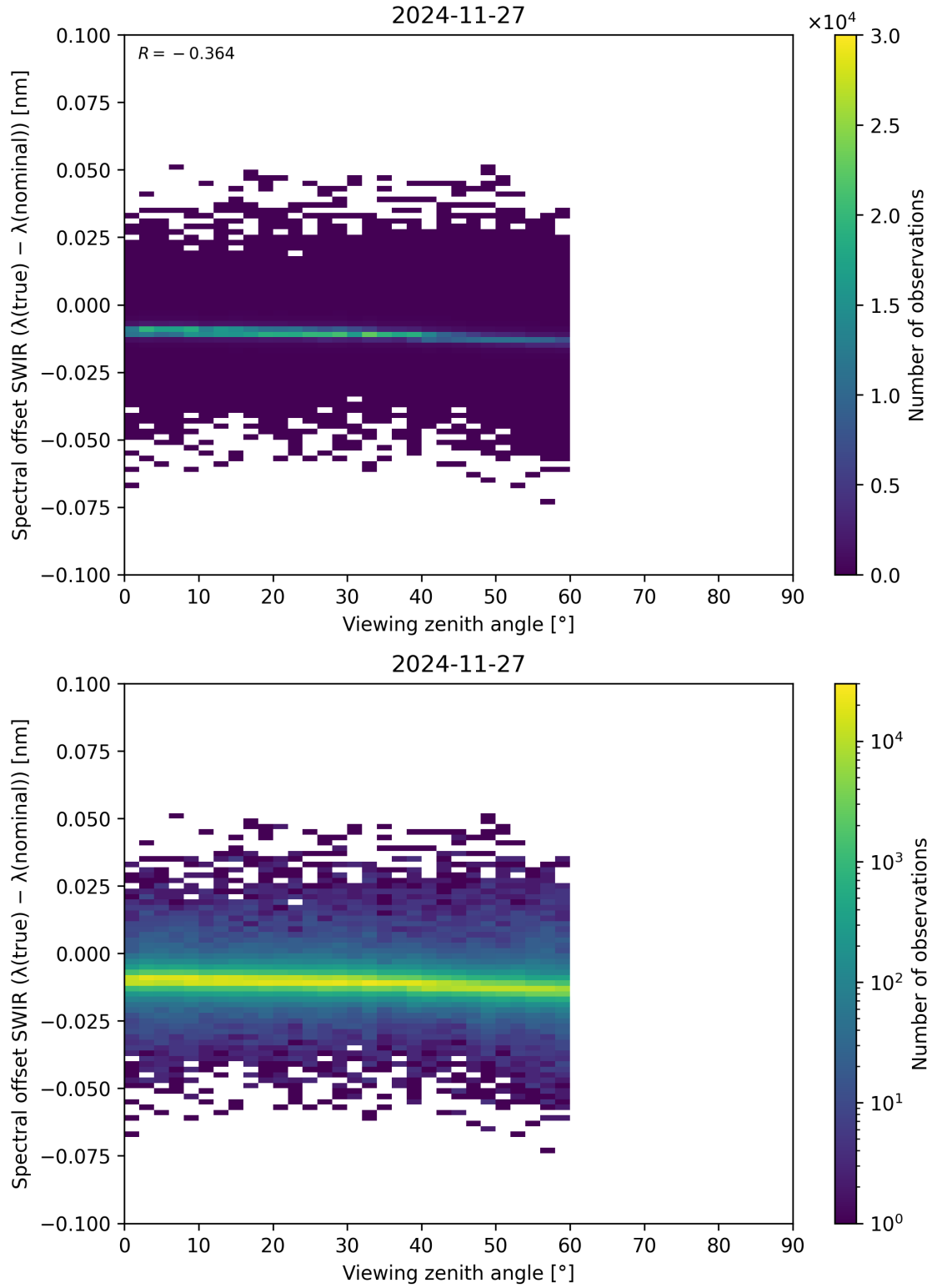
Figure 116: Scatter density plot of “Viewing zenith angle” against “Spectral offset SWIR ( \lambda_{\text{true}} - \lambda_{\text{nominal}} )” for 2024-11-26 to 2024-11-28.
