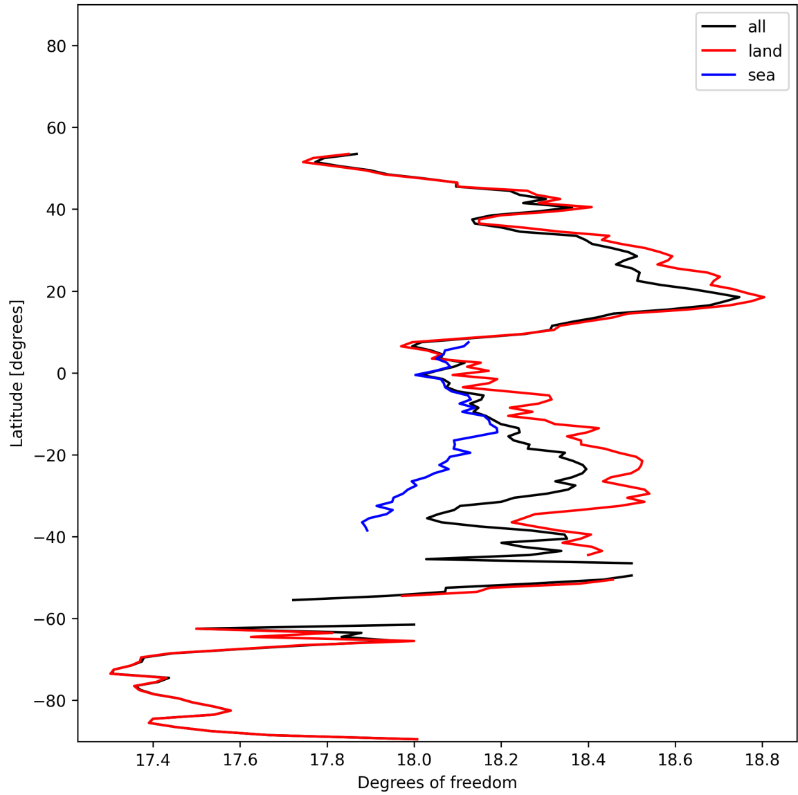
Figure 19: Zonal average of “Degrees of freedom” for 2024-11-26 to 2024-11-28.
