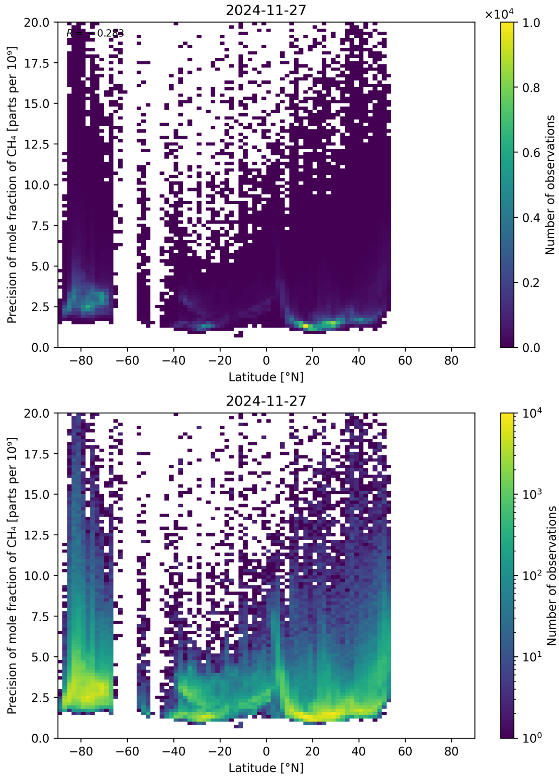
Figure 59: Scatter density plot of “Latitude” against “Precision of mole fraction of CH 4 ” for 2024-11-26 to 2024-11-28.
