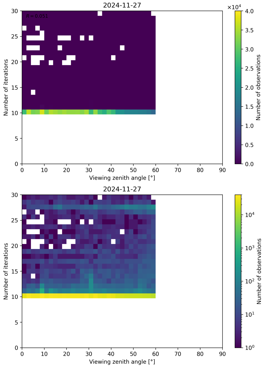
Figure 113: Scatter density plot of “Viewing zenith angle” against “Number of iterations” for 2024-11-26 to 2024-11-28.
