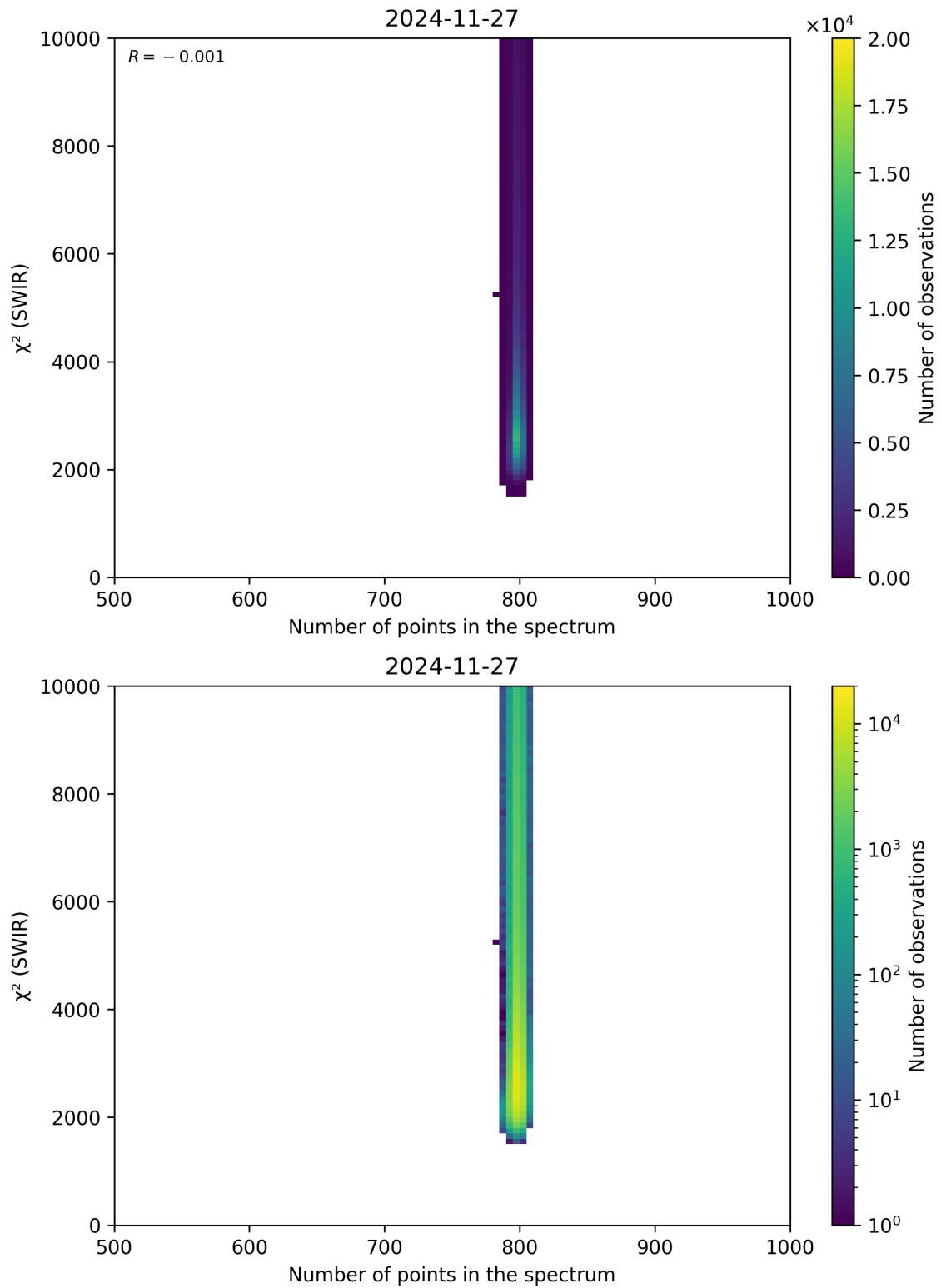
Figure 89: Scatter density plot of “Number of points in the spectrum” against “ \chi^2 (SWIR)” for 2024-11-26 to 2024-11-28.
