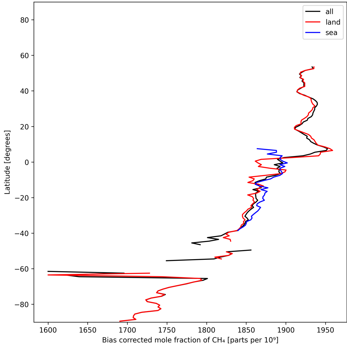
Figure 14: Zonal average of “Bias corrected mole fraction of CH 4 ” for 2024-11-26 to 2024-11-28.
