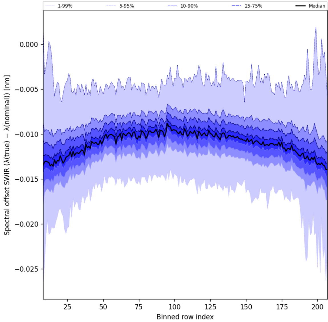
Figure 38: Along track statistics of “Spectral offset SWIR ( \lambda_{\text{true}} - \lambda_{\text{nominal}} )” for 2024-11-26 to 2024-11-28
