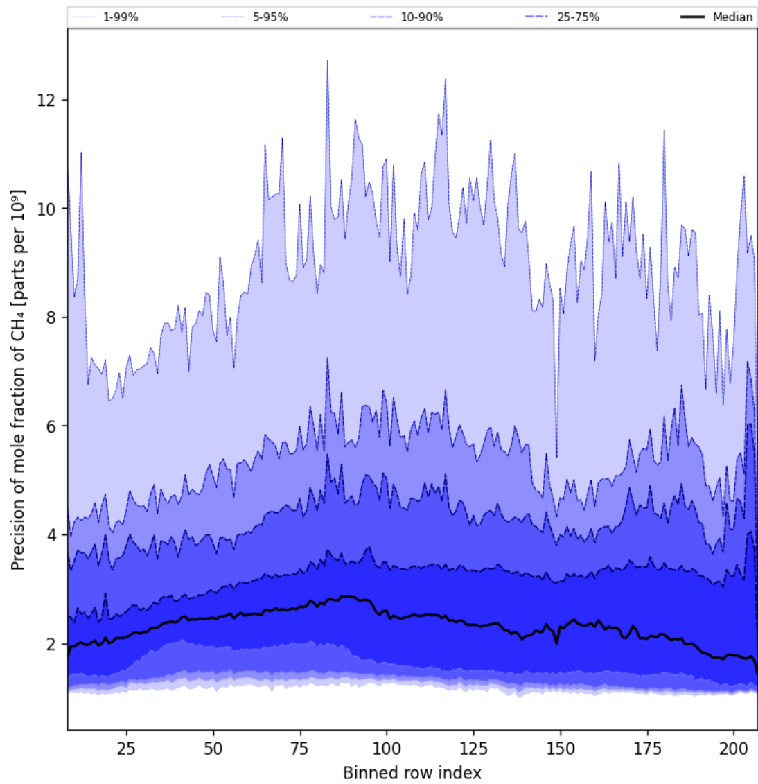
Figure 35: Along track statistics of “Precision of mole fraction of CH 4 ” for 2024-11-26 to 2024-11-28
