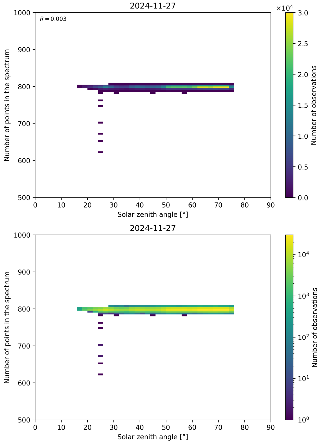
Figure 103: Scatter density plot of “Solar zenith angle” against “Number of points in the spectrum” for 2024-11-26 to 2024-11-28.
