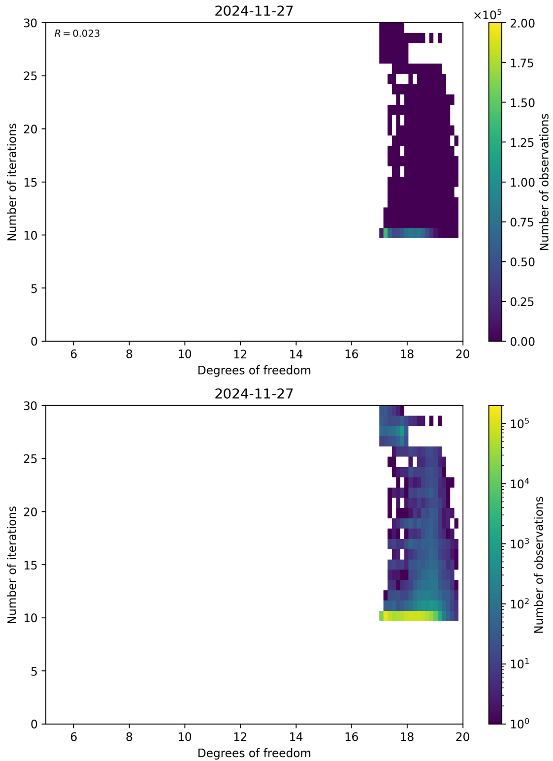
Figure 52: Scatter density plot of “Degrees of freedom” against “Number of iterations” for 2024-11-26 to 2024-11-28.
