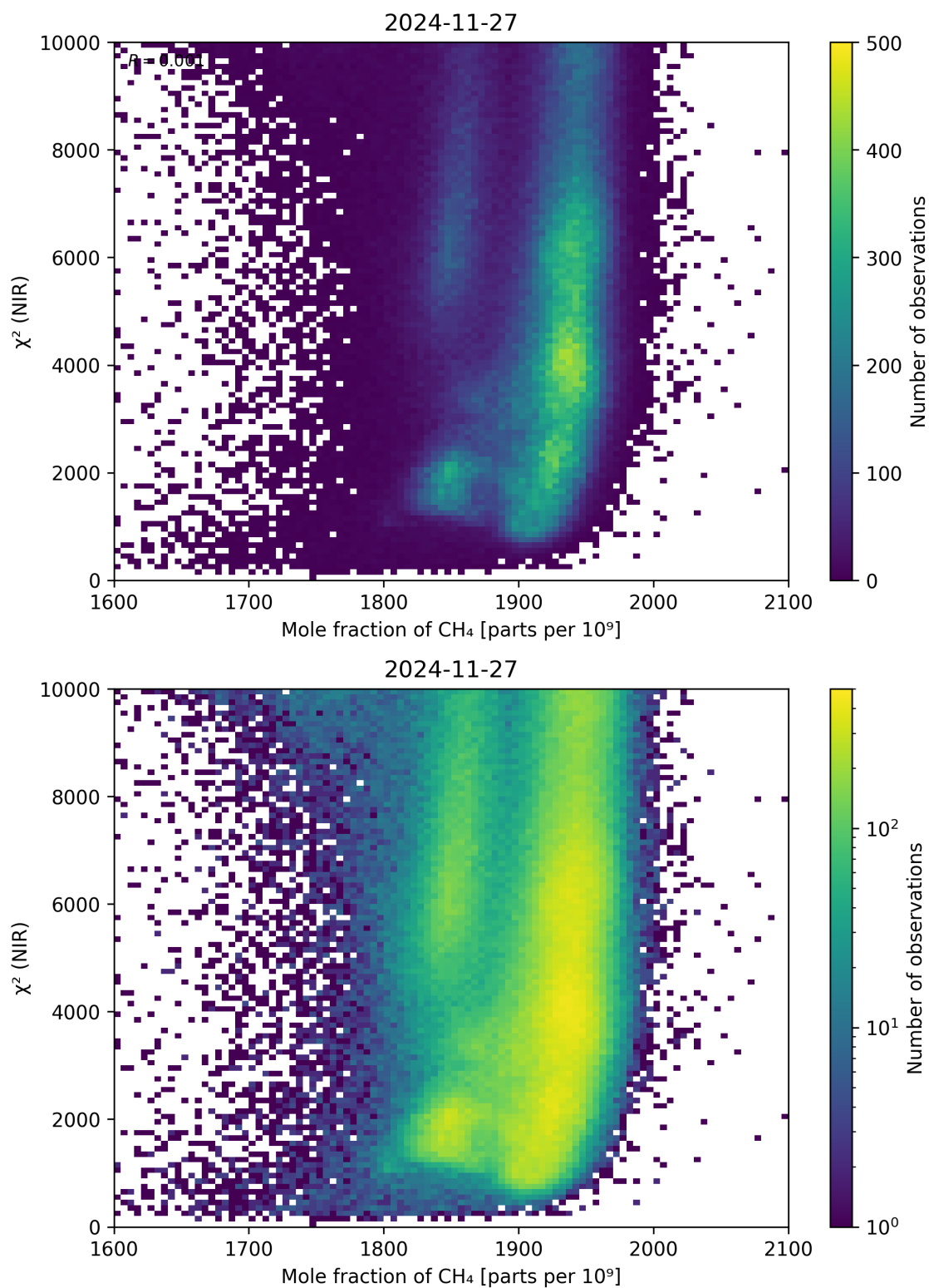
Figure 70: Scatter density plot of “Mole fraction of \text{CH}_4 ” against “ \chi^2 (NIR)” for 2024-11-26 to 2024-11-28.
