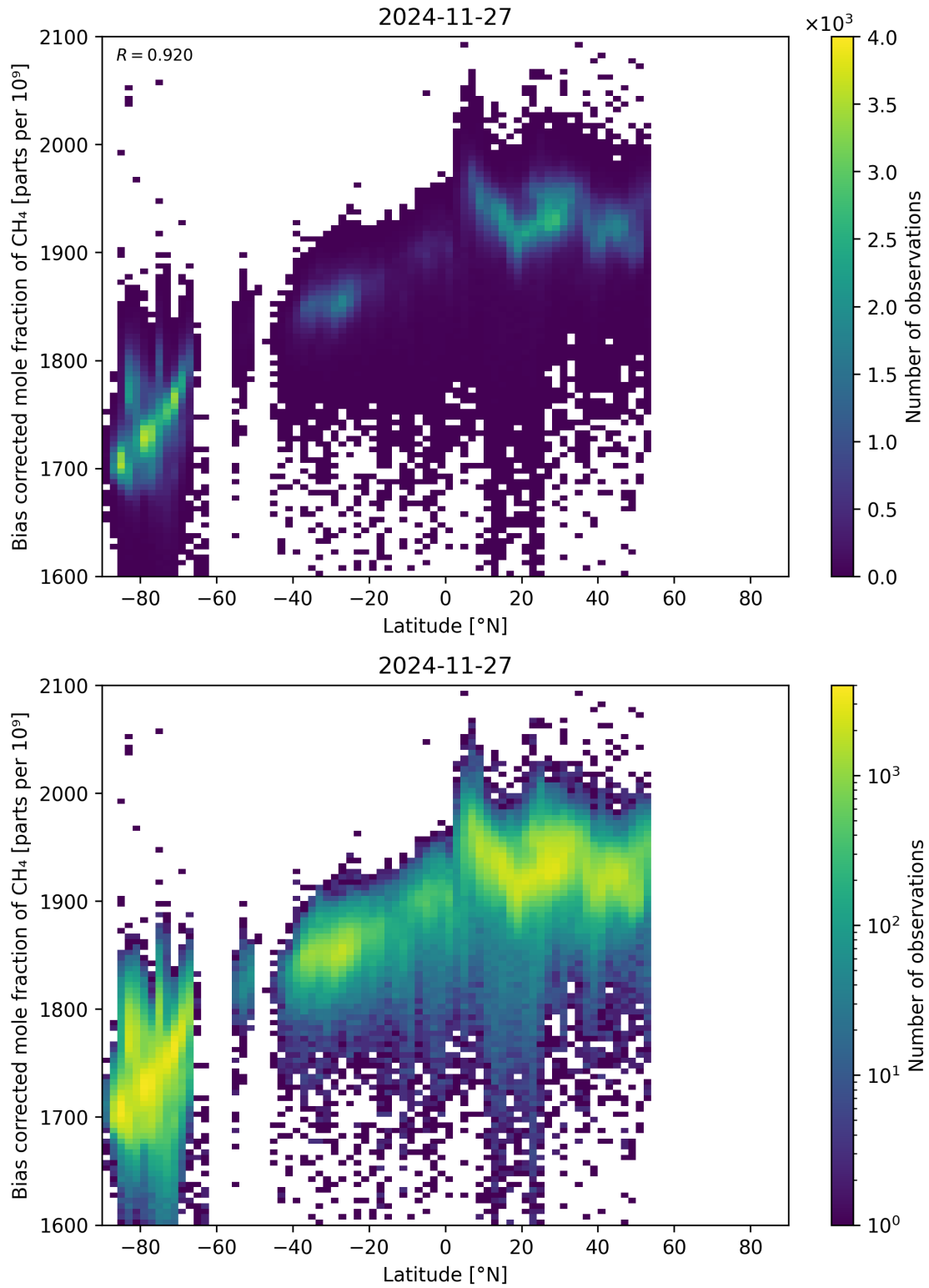
Figure 58: Scatter density plot of “Latitude” against “Bias corrected mole fraction of CH 4 ” for 2024-11-26 to 2024-11-28.
