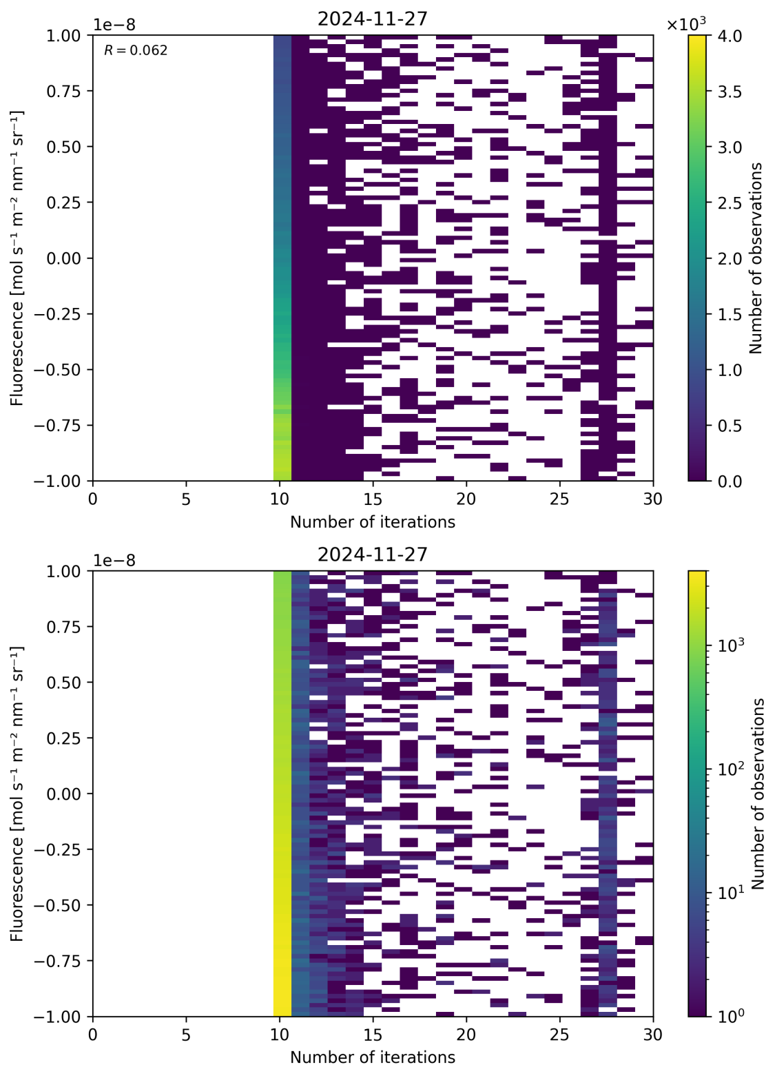
Figure 87: Scatter density plot of “Number of iterations” against “Fluorescence” for 2024-11-26 to 2024-11-28.
