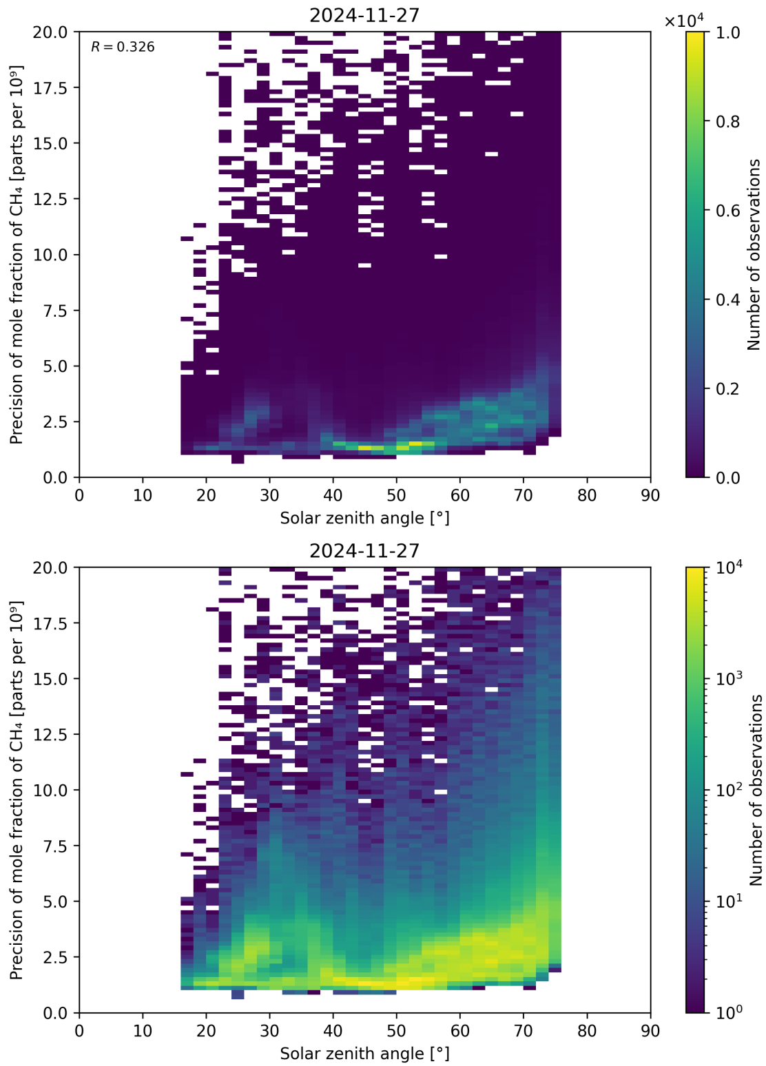
Figure 101: Scatter density plot of “Solar zenith angle” against “Precision of mole fraction of \text{CH}_4 ” for 2024-11-26 to 2024-11-28.
