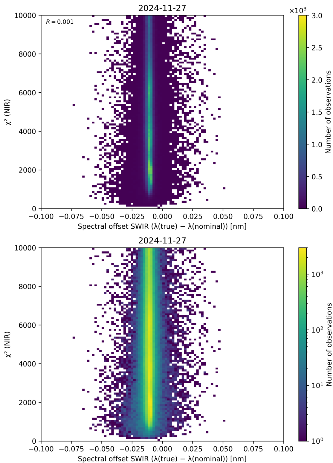
Figure 117: Scatter density plot of “Spectral offset SWIR ( \lambda_{\text{true}} - \lambda_{\text{nominal}} )” against “ \chi^2 (NIR)” for 2024-11-26 to 2024-11-28.
