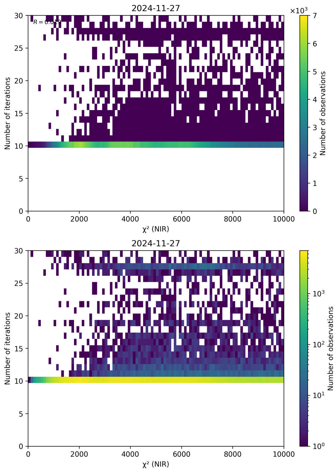
Figure 46: Scatter density plot of “ \chi^2 (NIR)” against “Number of iterations” for 2024-11-26 to 2024-11-28.
