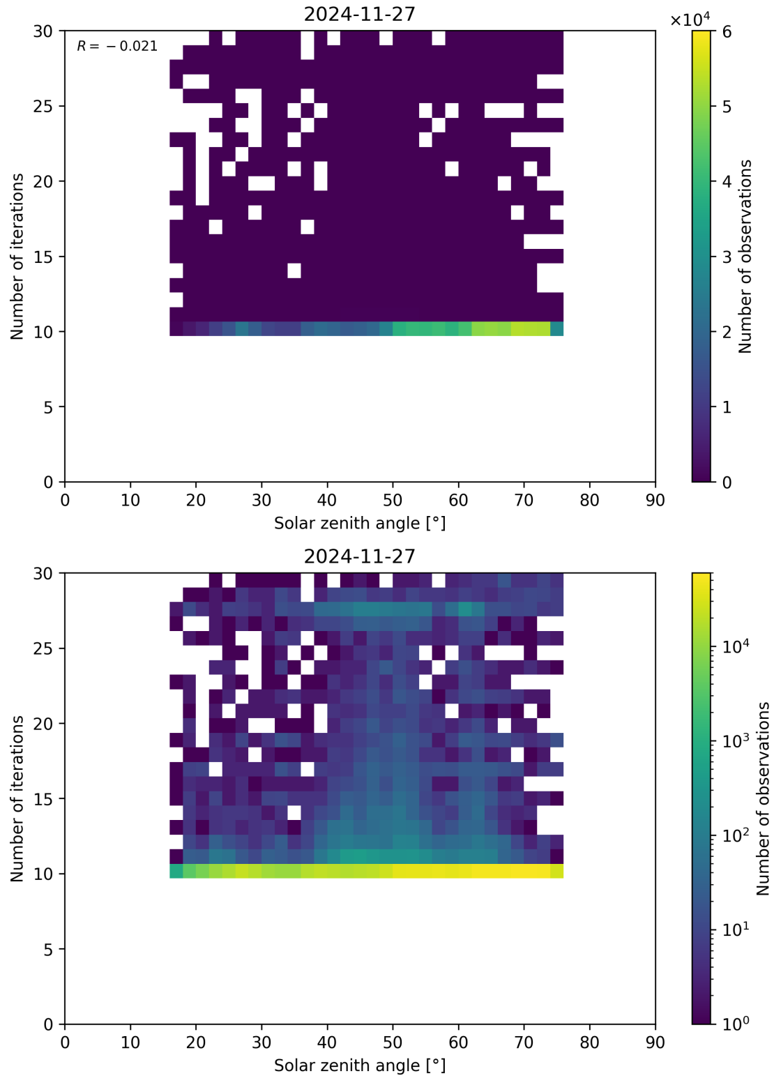
Figure 102: Scatter density plot of “Solar zenith angle” against “Number of iterations” for 2024-11-26 to 2024-11-28.
