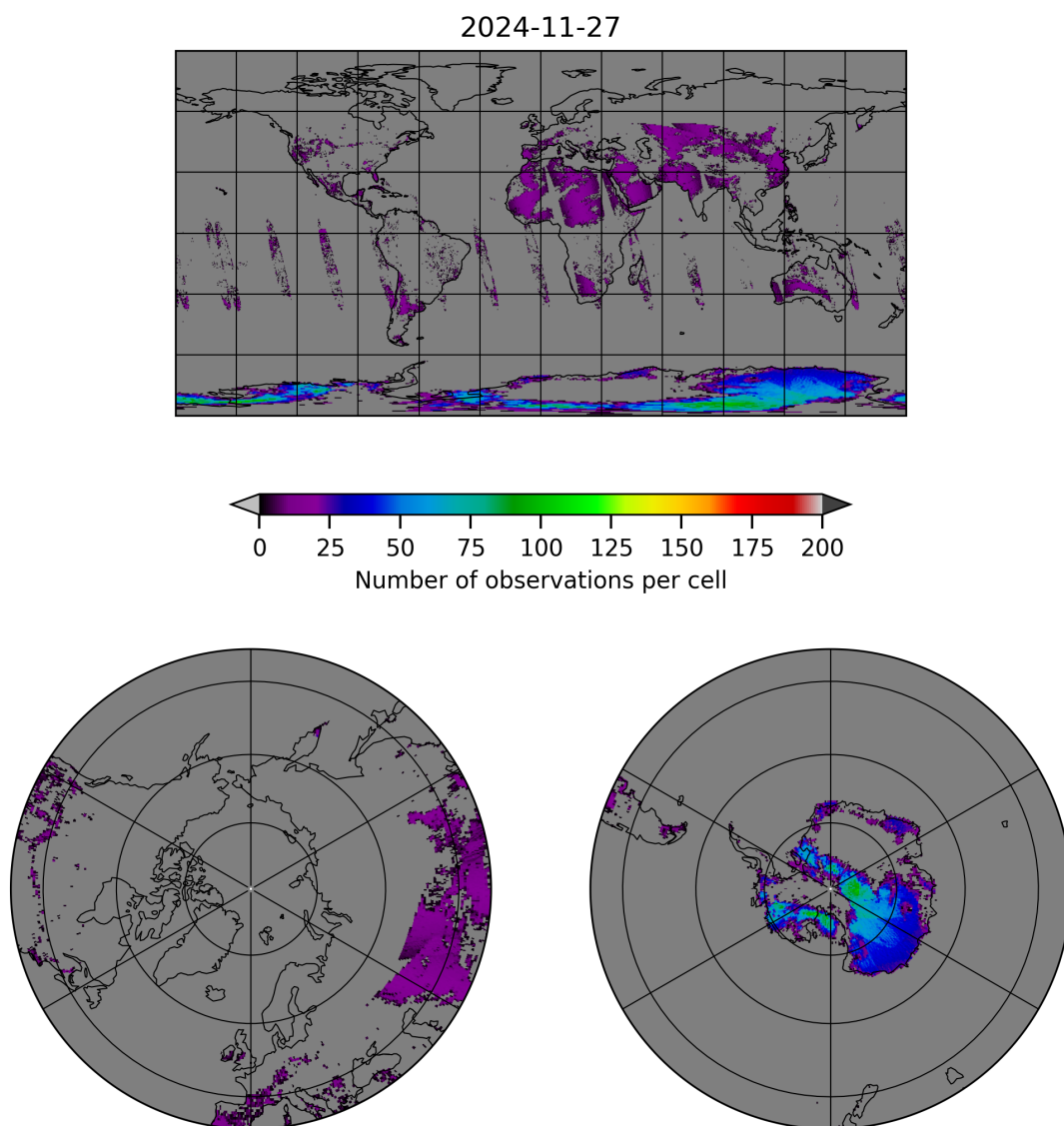
Figure 10: Map of the number of observations for 2024-11-26 to 2024-11-28
