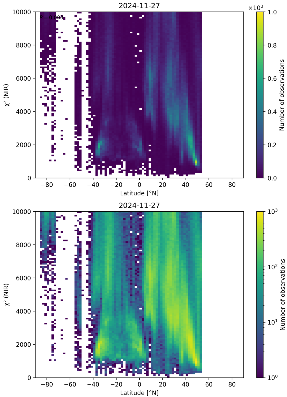
Figure 53: Scatter density plot of “Latitude” against “ \chi^2 (NIR)” for 2024-11-26 to 2024-11-28.
