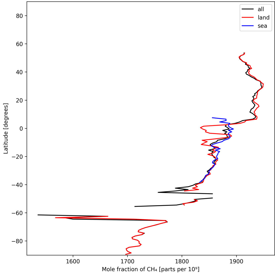
Figure 12: Zonal average of “Mole fraction of \text{CH}_4 ” for 2024-11-26 to 2024-11-28.
