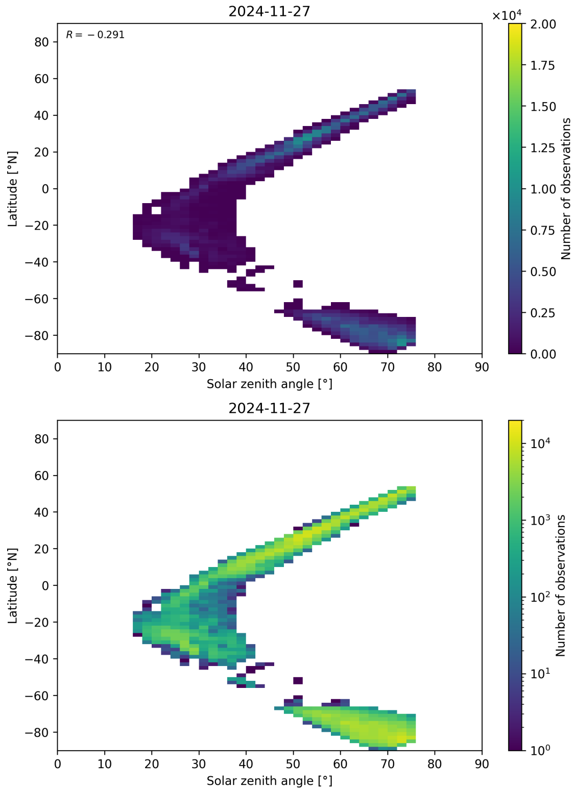
Figure 98: Scatter density plot of “Solar zenith angle” against “Latitude” for 2024-11-26 to 2024-11-28.
