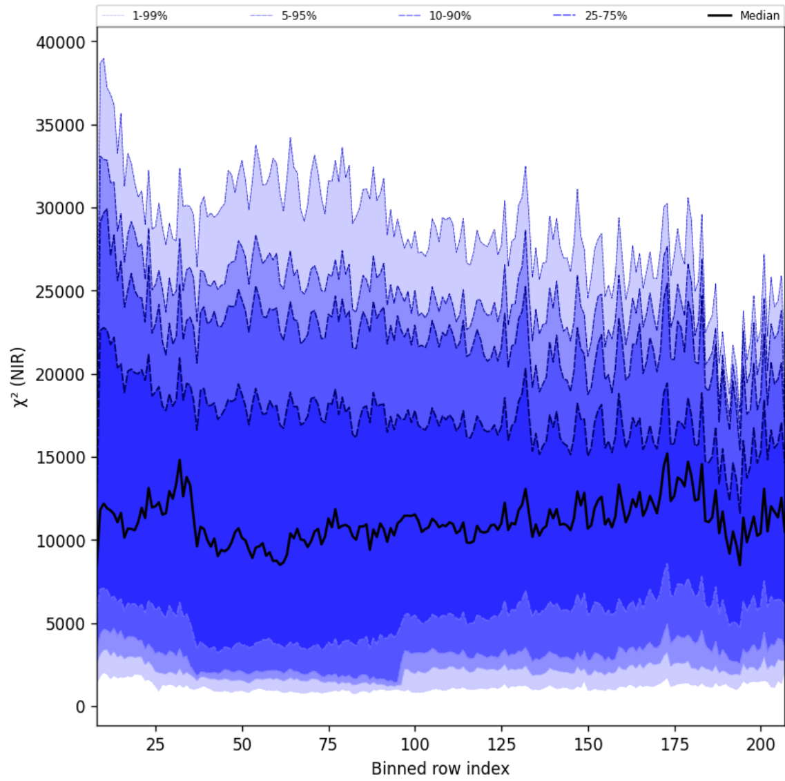
Figure 40: Along track statistics of “ \chi^2 (NIR)” for 2024-11-26 to 2024-11-28
