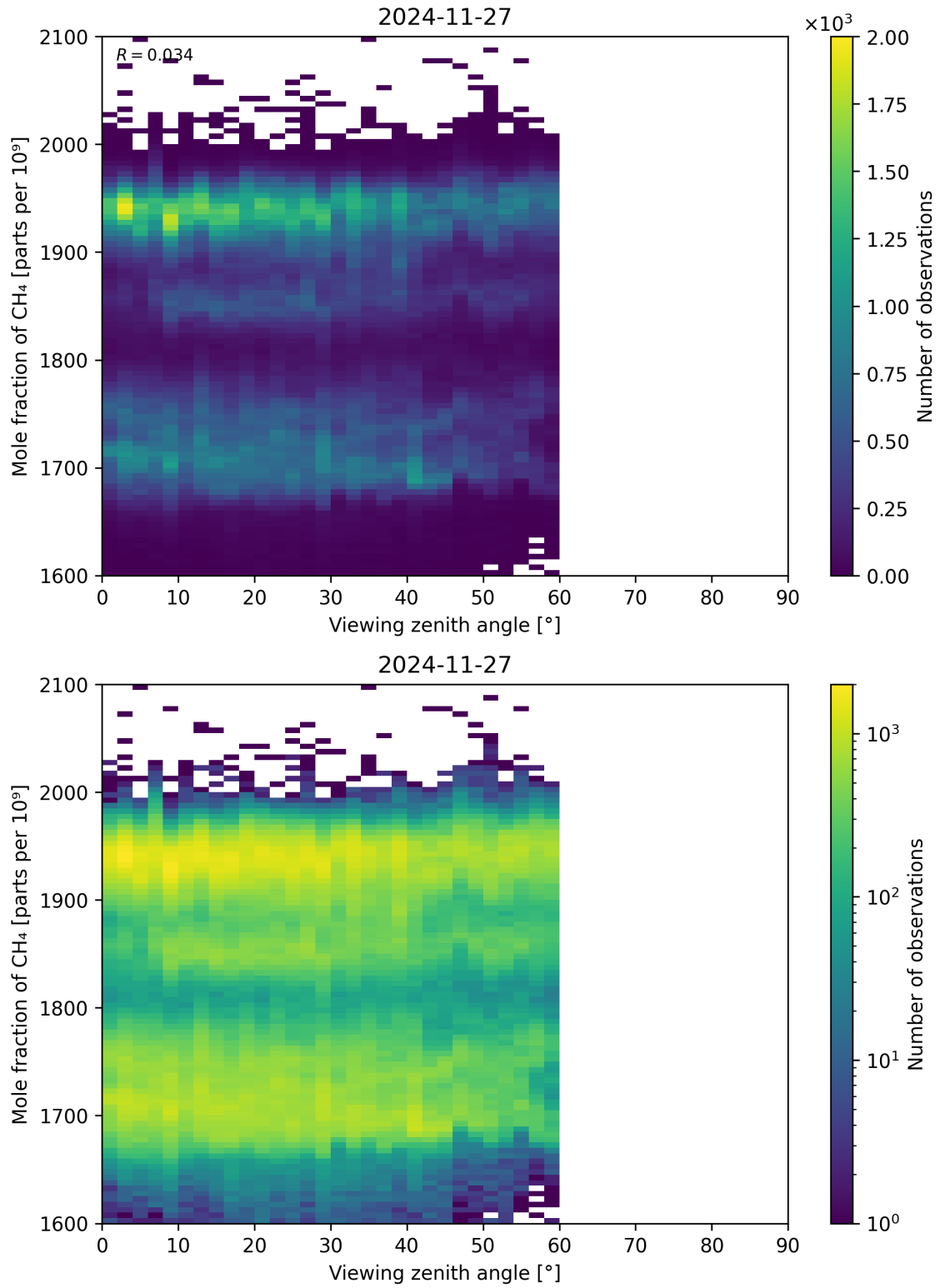
Figure 110: Scatter density plot of “Viewing zenith angle” against “Mole fraction of \text{CH}_4 ” for 2024-11-26 to 2024-11-28.
