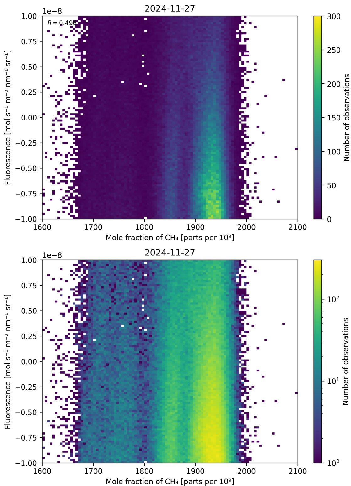
Figure 73: Scatter density plot of “Mole fraction of CH 4 ” against “Fluorescence” for 2024-11-26 to 2024-11-28.
