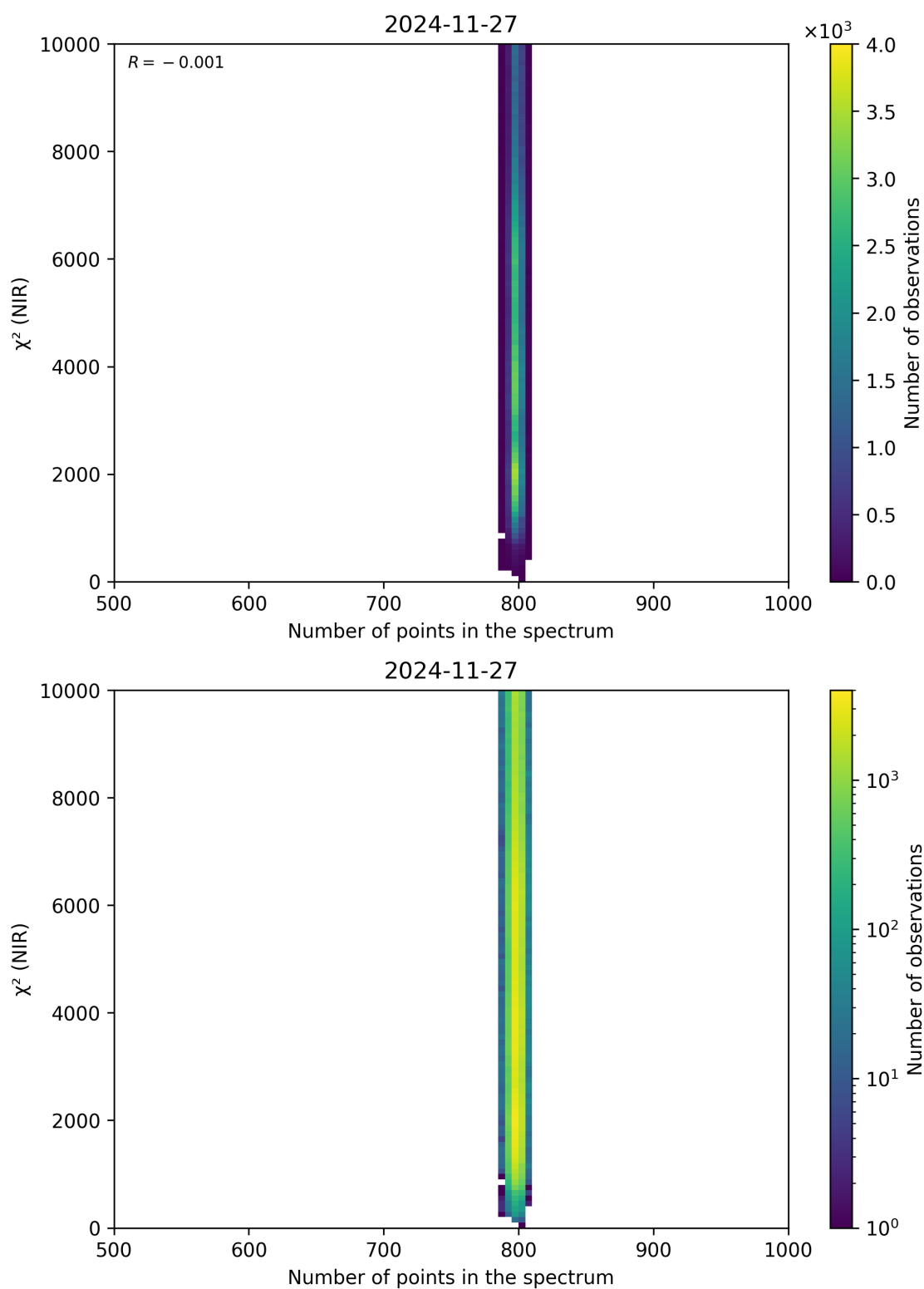
Figure 88: Scatter density plot of “Number of points in the spectrum” against “ \chi^2 (NIR)” for 2024-11-26 to 2024-11-28.
