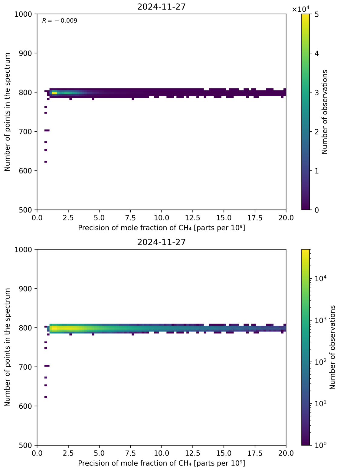
Figure 84: Scatter density plot of “Precision of mole fraction of CH 4 ” against “Number of points in the spectrum” for 2024-11-26 to 2024-11-28.
