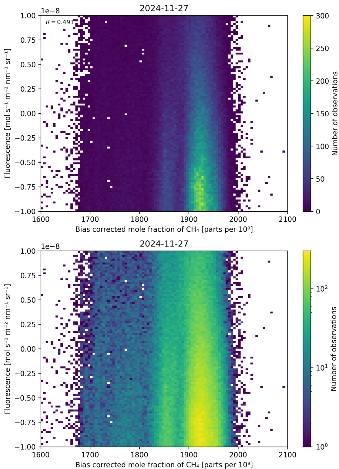
Figure 66: Scatter density plot of “Bias corrected mole fraction of \text{CH}_4 ” against “Fluorescence” for 2024-11-26 to 2024-11-28.
