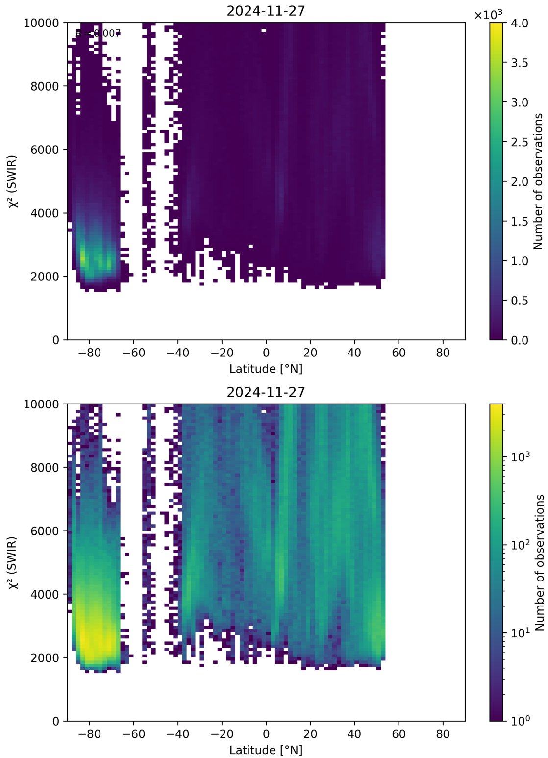
Figure 54: Scatter density plot of “Latitude” against “ \chi^2 (SWIR)” for 2024-11-26 to 2024-11-28.
