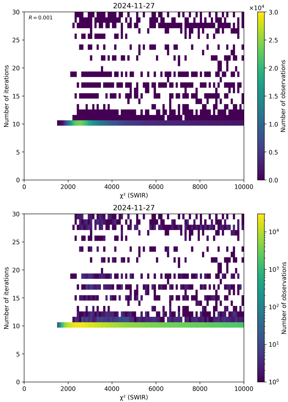
Figure 50: Scatter density plot of “ \chi^2 (SWIR)” against “Number of iterations” for 2024-11-26 to 2024-11-28.
