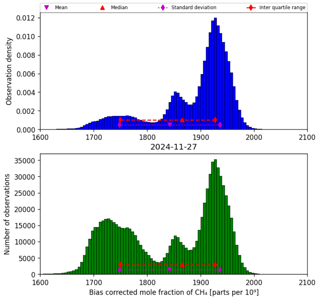
Figure 25: Histogram of “Bias corrected mole fraction of CH 4 ” for 2024-11-26 to 2024-11-28
