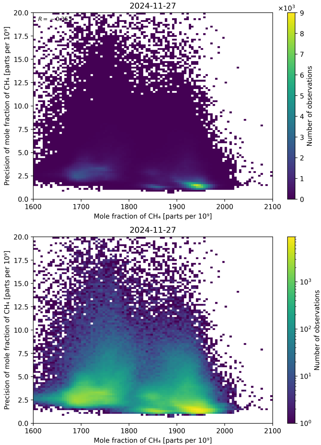
Figure 75: Scatter density plot of “Mole fraction of CH 4 ” against “Precision of mole fraction of CH 4 ” for 2024-11-26 to 2024-11-28.
