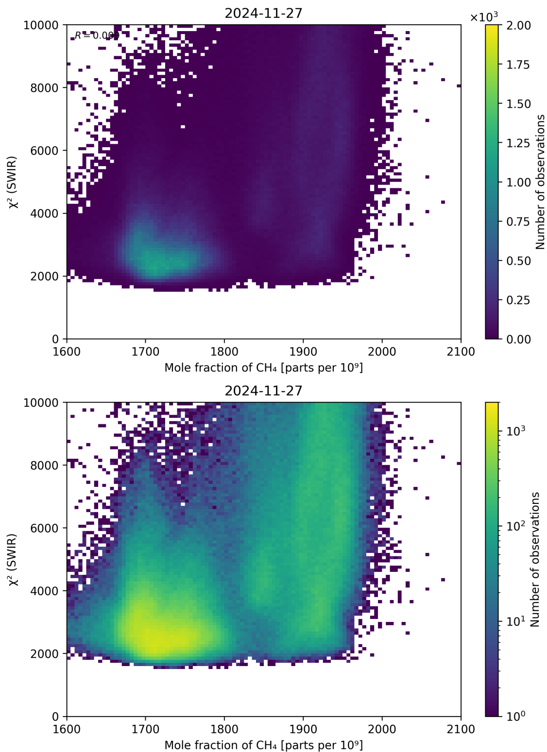
Figure 71: Scatter density plot of “Mole fraction of \text{CH}_4 ” against “ \chi^2 (SWIR)” for 2024-11-26 to 2024-11-28.
