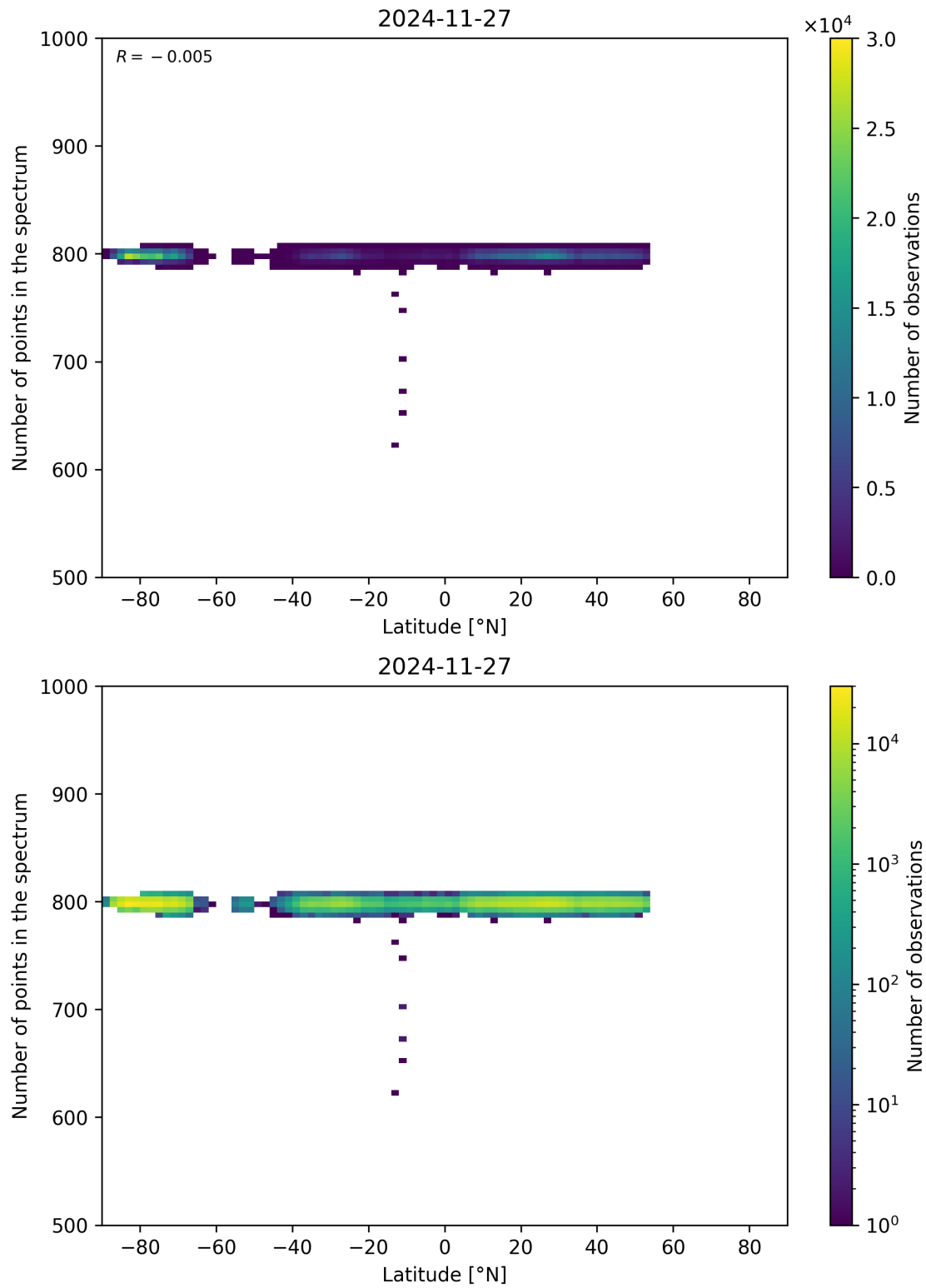
Figure 61: Scatter density plot of “Latitude” against “Number of points in the spectrum” for 2024-11-26 to 2024-11-28.
