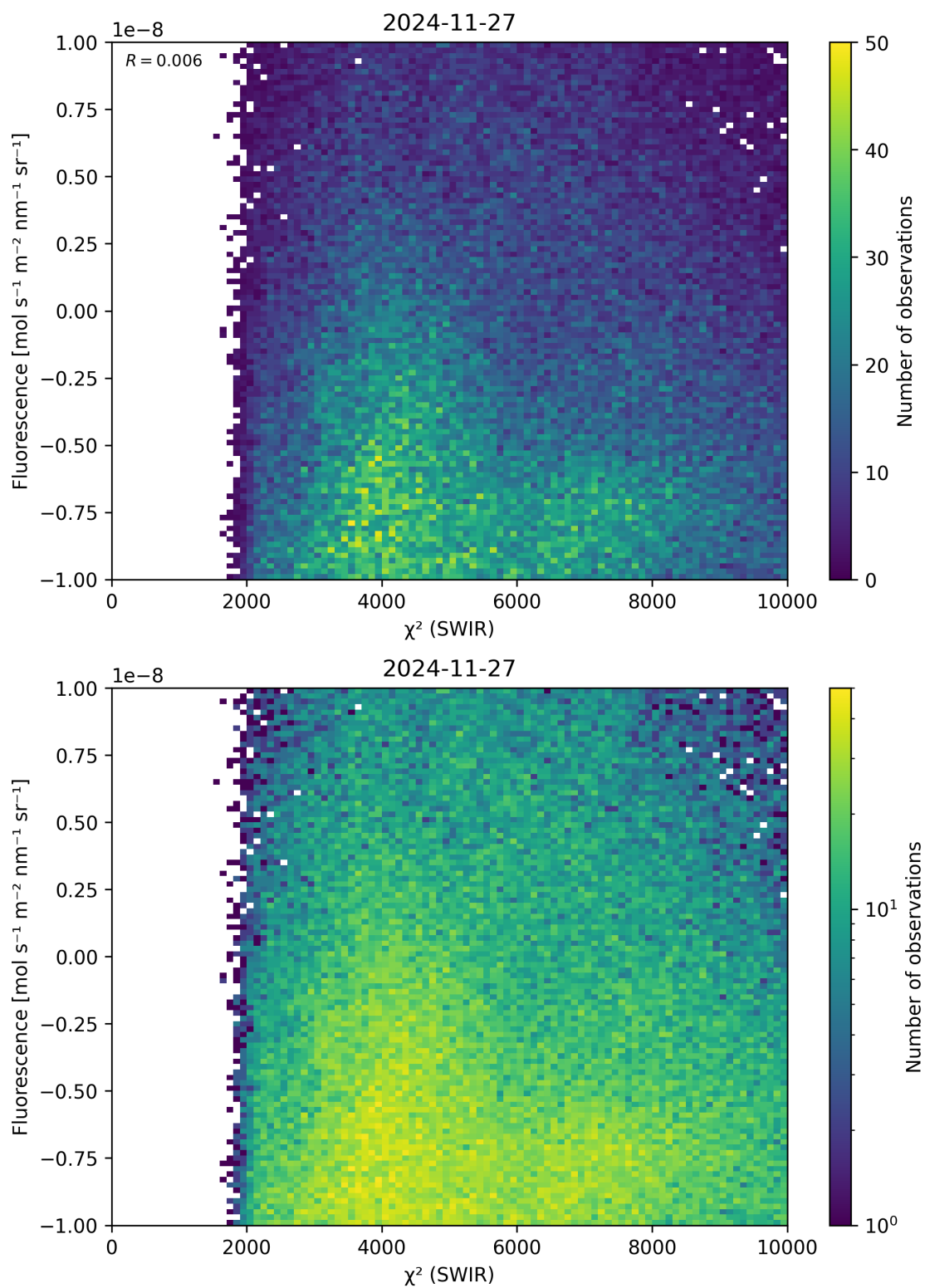
Figure 49: Scatter density plot of “ \chi^2 (SWIR)” against “Fluorescence” for 2024-11-26 to 2024-11-28.
