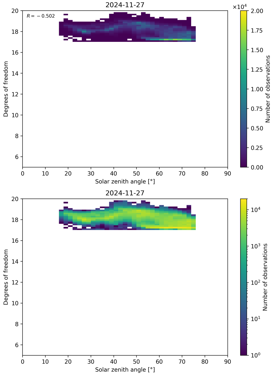
Figure 96: Scatter density plot of “Solar zenith angle” against “Degrees of freedom” for 2024-11-26 to 2024-11-28.
