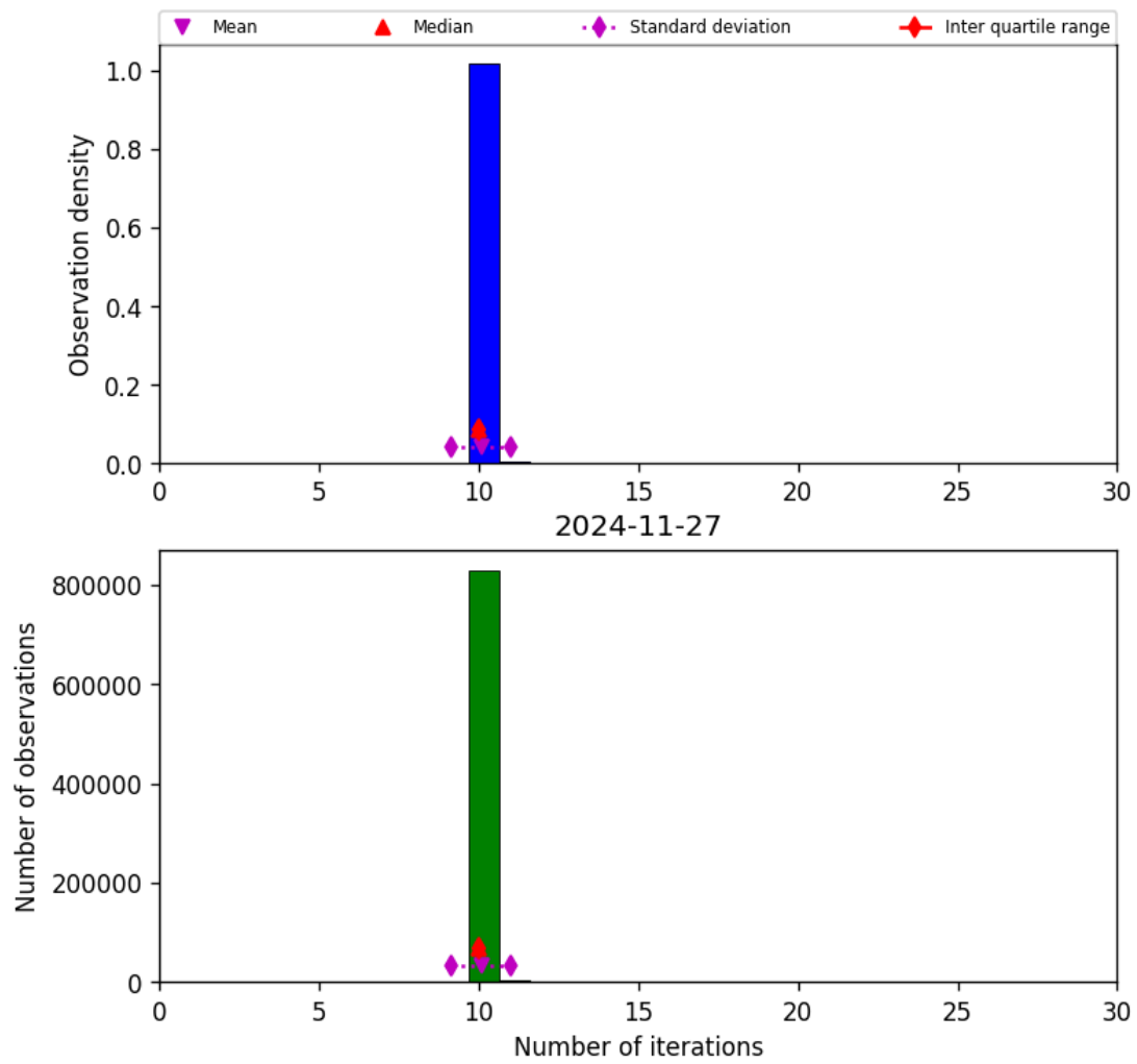
Figure 31: Histogram of “Number of iterations” for 2024-11-26 to 2024-11-28
